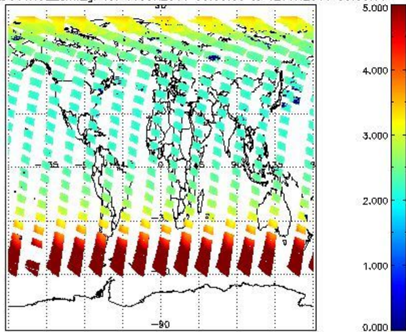
SCIOL2P_NADUV1N02_amf_gr for 11JUN2011 00:00:00 to 12JUN2011 00:00:00
