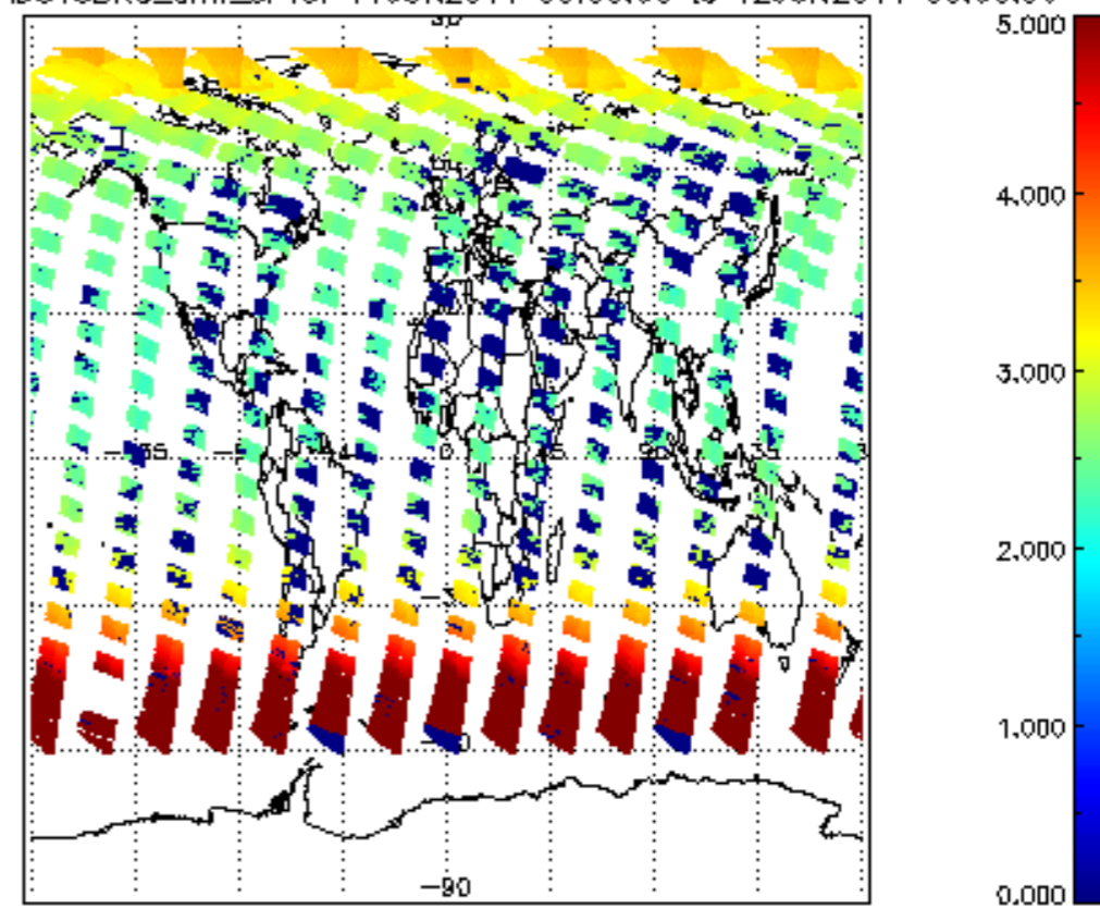
SCIOL2P_NADUV3BRO_amf_sl for 11JUN2011 00:00:00 to 12JUN2011 00:00:00
