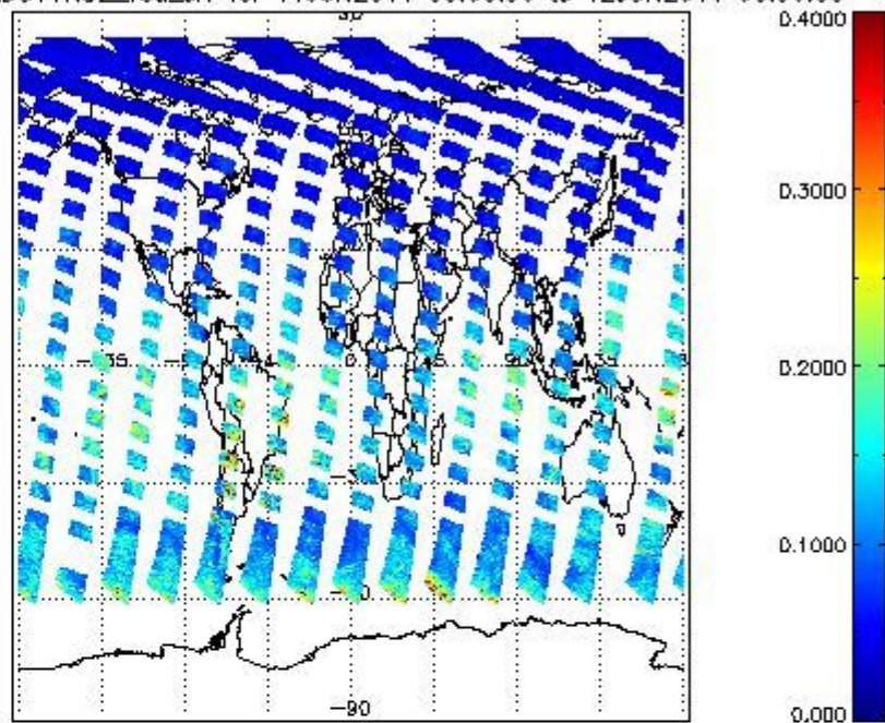
SCIOL2P_NADUV1N02_vcd_err for 11JUN2011 00:00:00 to 12JUN2011 00:00:00
