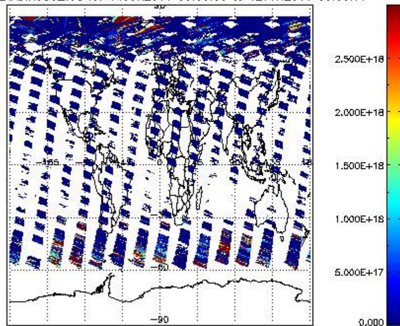
SCIDL2P_NADIR3CO_vcd for 11JUN2011 00:00:00 to 12JUN2011 00:00:00
