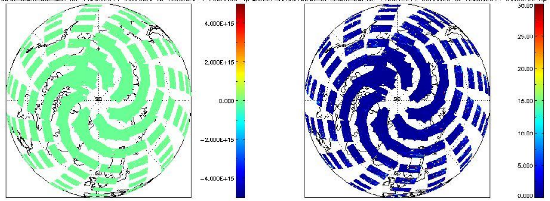
CIOL2P_NADUV6OCLslant_col_den for 11JUN2011 00:00:00 to 12JUN2011 00:00:00 np; CIOL2P_NADUV6OCLarr_slant_col for 11JUN2011 00:00:00 to 12JUN2011 00:00:00 np
