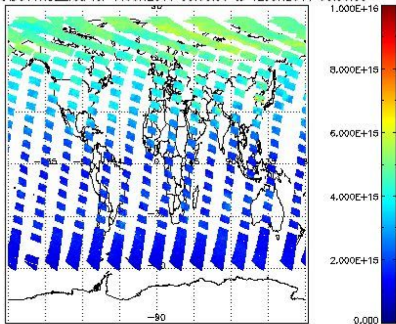
SCIOL2P_NADUV1N02_vcd for 11JUN2011 00:00:00 to 12JUN2011 00:00:00
