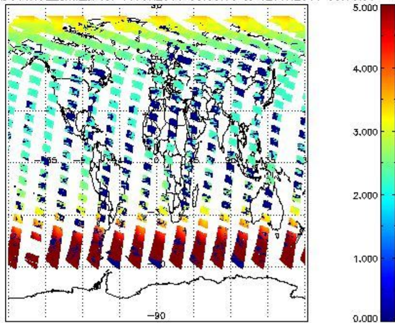
SCIOL2P_NADUV1N02_amf_cl for 11JUN2011 00:00:00 to 12JUN2011 00:00:00
