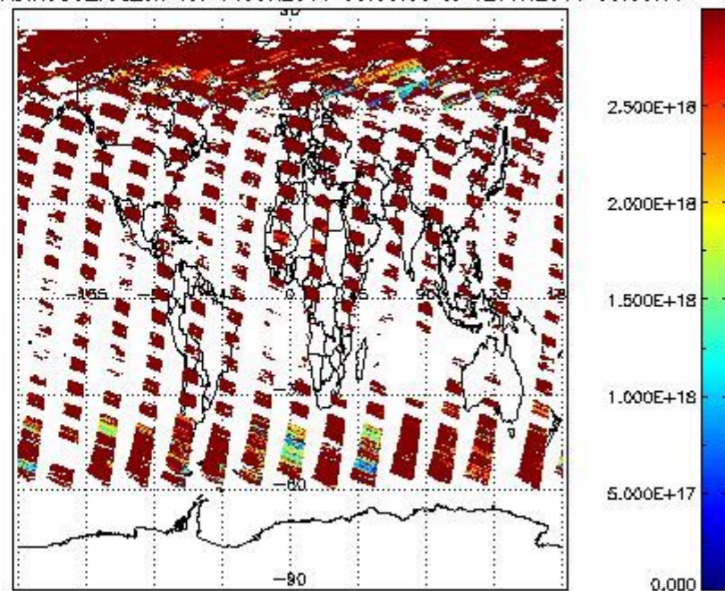
SCIDL2P_NADIR3CO_vcd_err for 11JUN2011 00:00:00 to 12JUN2011 00:00:00
