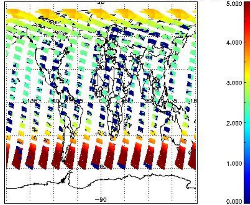
SCIOL2P_NADUV3BRO_amf_cl for 10JUN2011 00:00:00 to 11JUN2011 00:00:00
