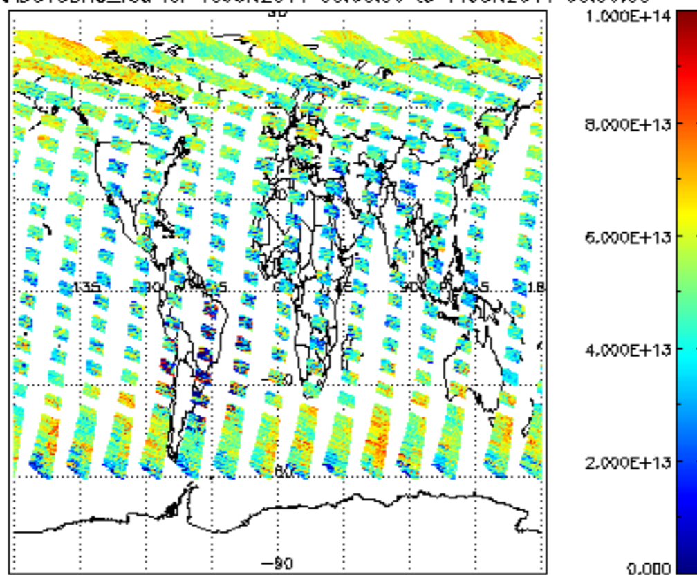
SCIOL2P_NADUV3BRO_vcd for 10JUN2011 00:00:00 to 11JUN2011 00:00:00
