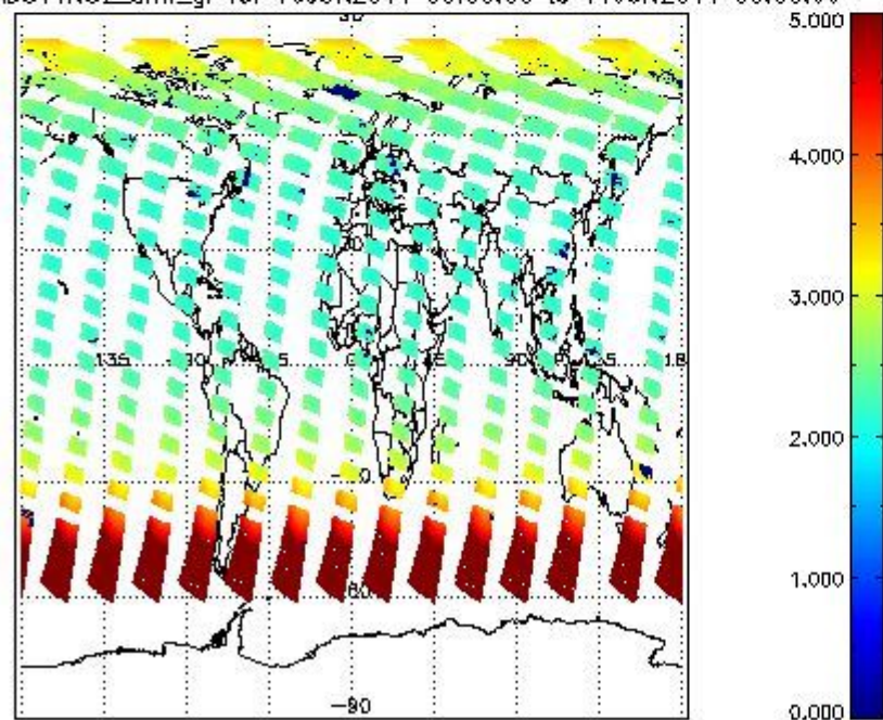
SCIOL2P_NADUV1NO2_amf_gr for 10JUN2011 00:00:00 to 11JUN2011 00:00:00
