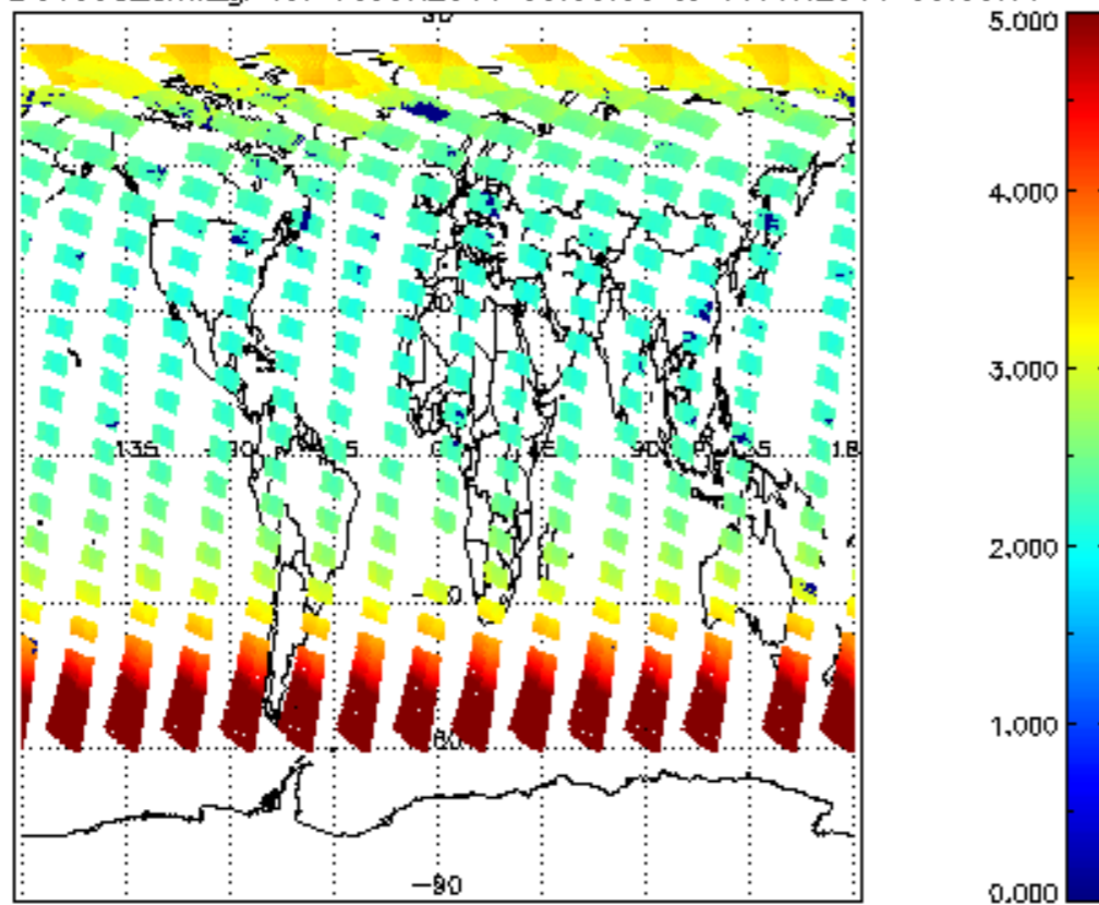
SCIOL2P_NADUV003_amf_gr for 10JUN2011 00:00:00 to 11JUN2011 00:00:00
