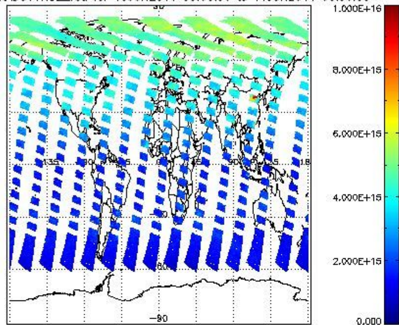
SCIOL2P_NADUV1NO2_vcd for 10JUN2011 00:00:00 to 11JUN2011 00:00:00
