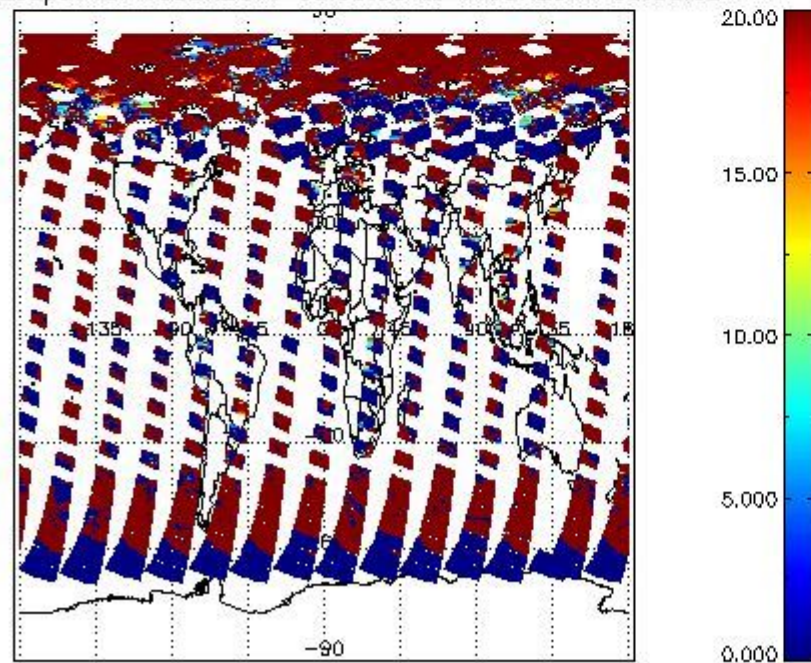
cL_opt_depth for 10JUN2011 00:00:00 to 11JUN2011 00:00:00
