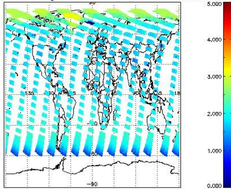
SCIOL2P_NADUV7S02_amf_gr for 10JUN2011 00:00:00 to 11JUN2011 00:00:00
