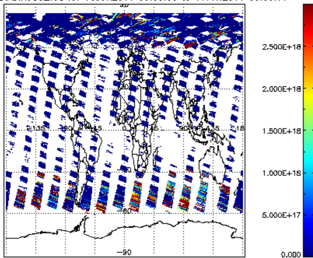
SCIOL2P_NADIR3CO_vcd for 10JUN2011 00:00:00 to 11JUN2011 00:00:00
