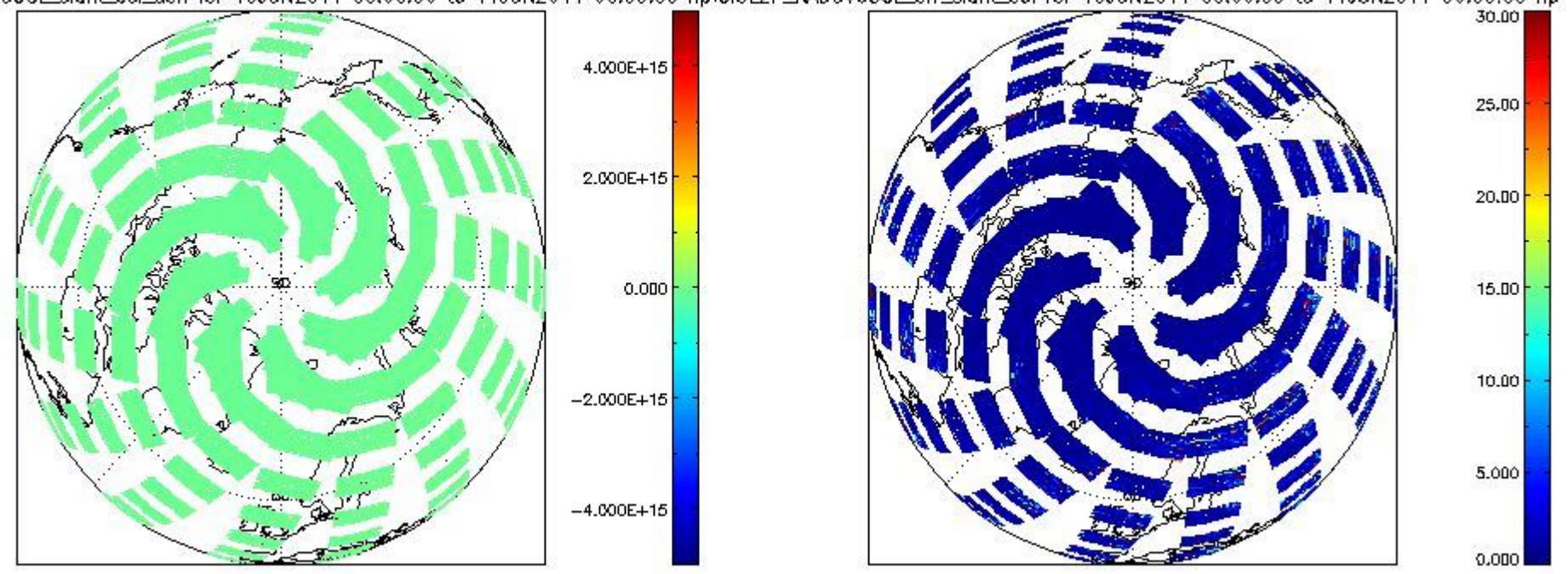
CIOL2P_NADUV60CL_slant_col_den for 10JUN2011 00:00:00 to 11JUN2011 00:00:00 np; CIOL2P_NADUV60CL_err_slant_col for 10JUN2011 00:00:00 to 11JUN2011 00:00:00 np
