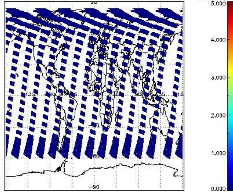
SCIOL2P_NADUV5S02_amf_cl for 10JUN2011 00:00:00 to 11JUN2011 00:00:00
