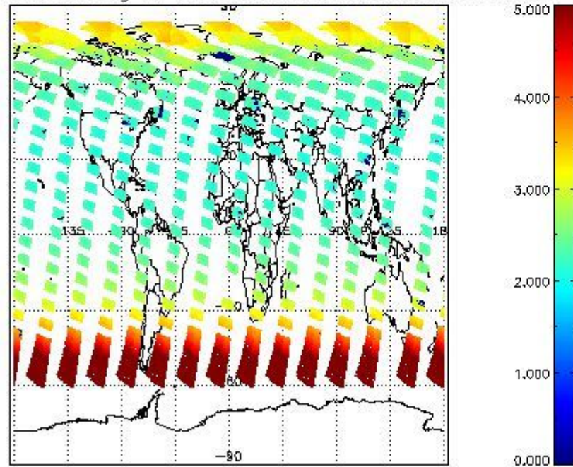
SCIOL2P_NADUV003_amf_gr for 10JUN2011 00:00:00 to 11JUN2011 00:00:00
