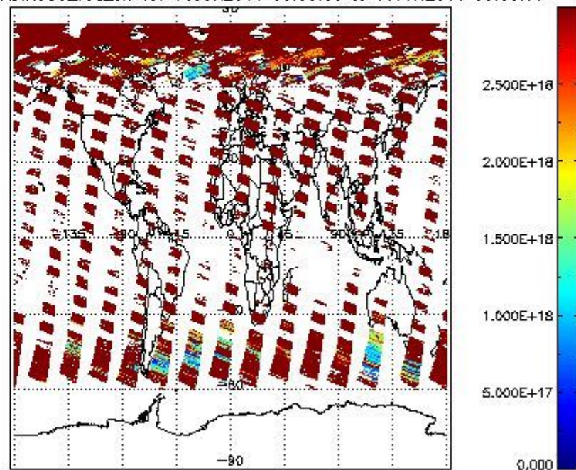
SCIDL2P_NADIR3CO_vcd_err for 10JUN2011 00:00:00 to 11JUN2011 00:00:00
