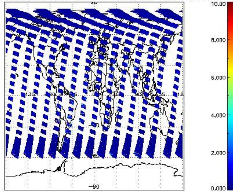
SCIOL2P_NADUV3BRO_vcd_err for 10JUN2011 00:00:00 to 11JUN2011 00:00:00
