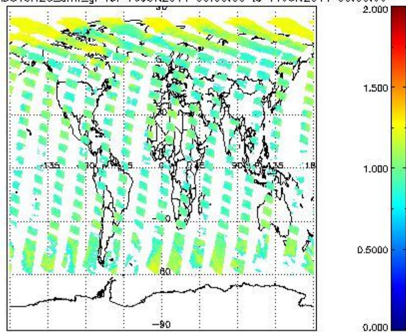
SCIOL2P_NADUV8H2O_arnf_gr for 10JUN2011 00:00:00 to 11JUN2011 00:00:00
