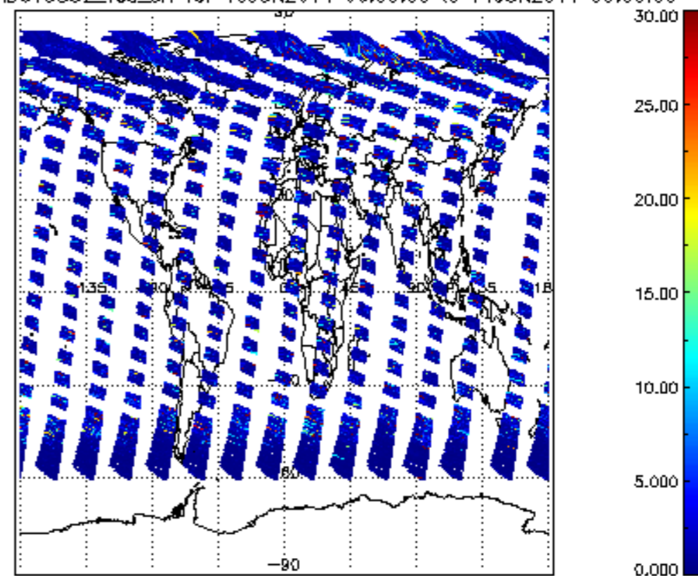
SCIOL2P_NADUV5S02_vcd_err for 10JUN2011 00:00:00 to 11JUN2011 00:00:00
