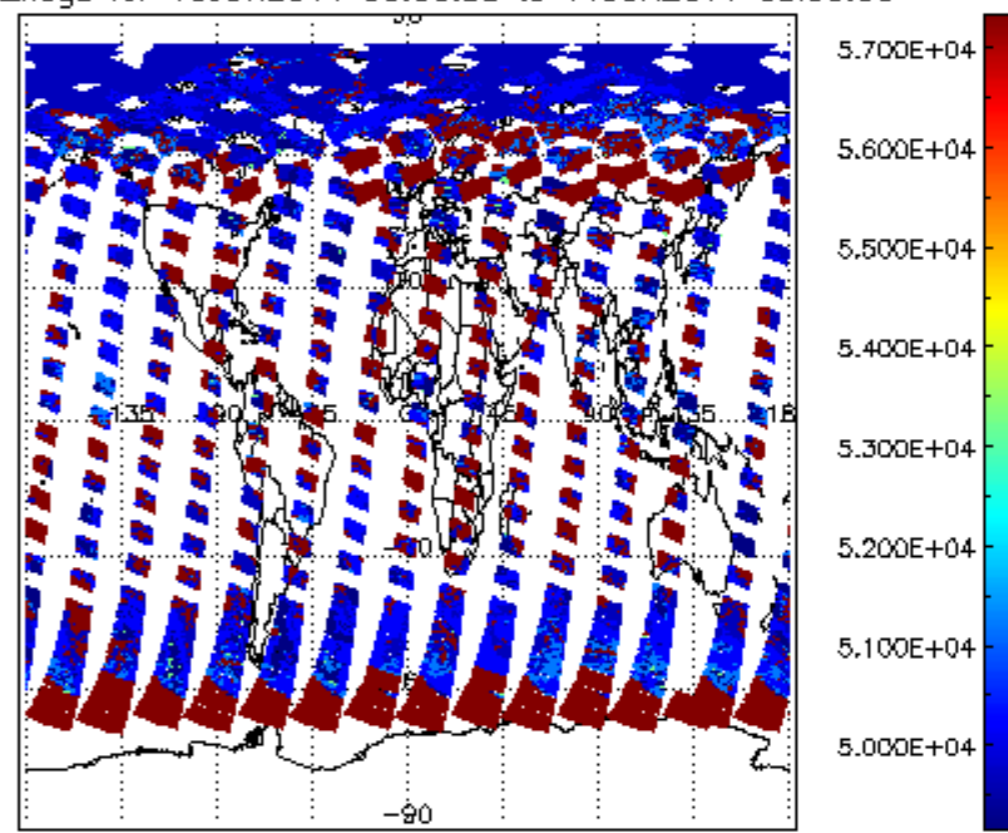
cloud_flags for 10JUN2011 00:00:00 to 11JUN2011 00:00:00
