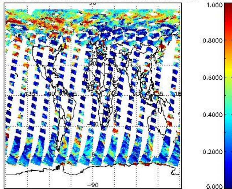
cL_frac for 10JUN2011 00:00:00 to 11JUN2011 00:00:00
