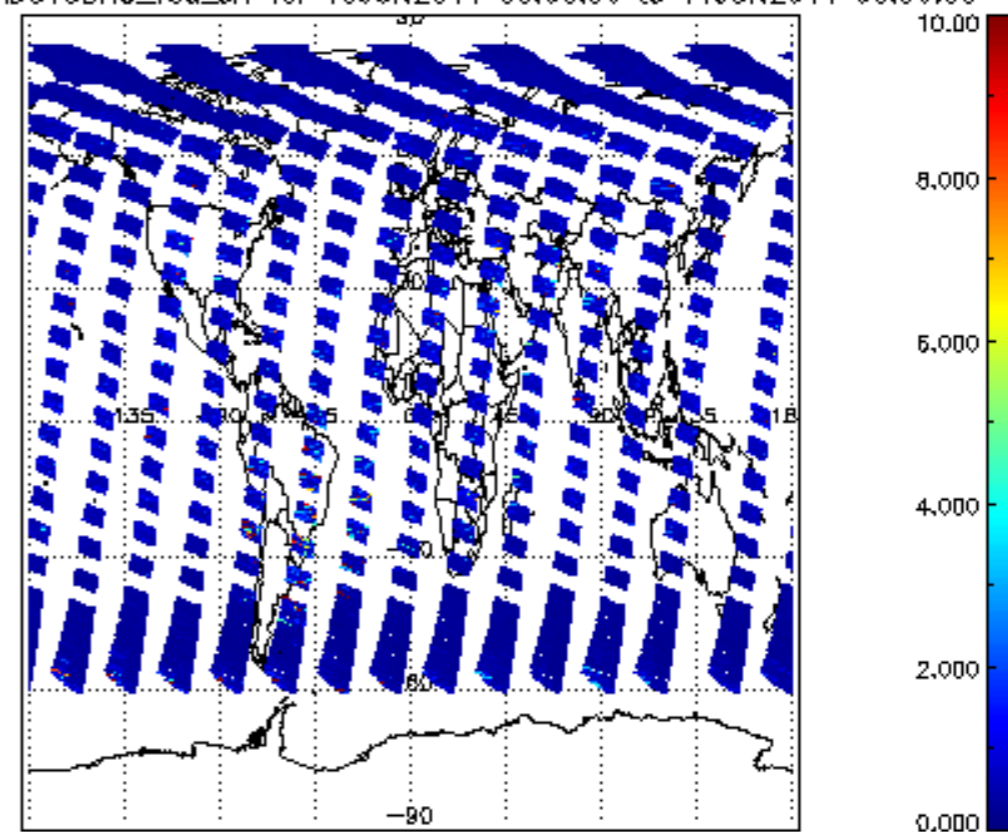
SCIOL2P_NADUV3BRO_vcd_err for 10JUN2011 00:00:00 to 11JUN2011 00:00:00
