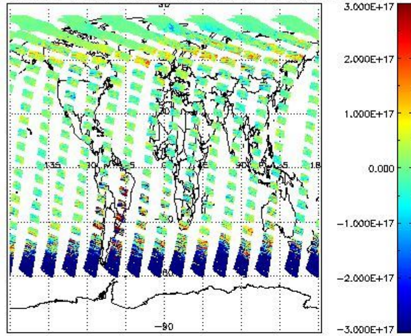
SCIOL2P_NADUV5S02_vcd for 10JUN2011 00:00:00 to 11JUN2011 00:00:00
