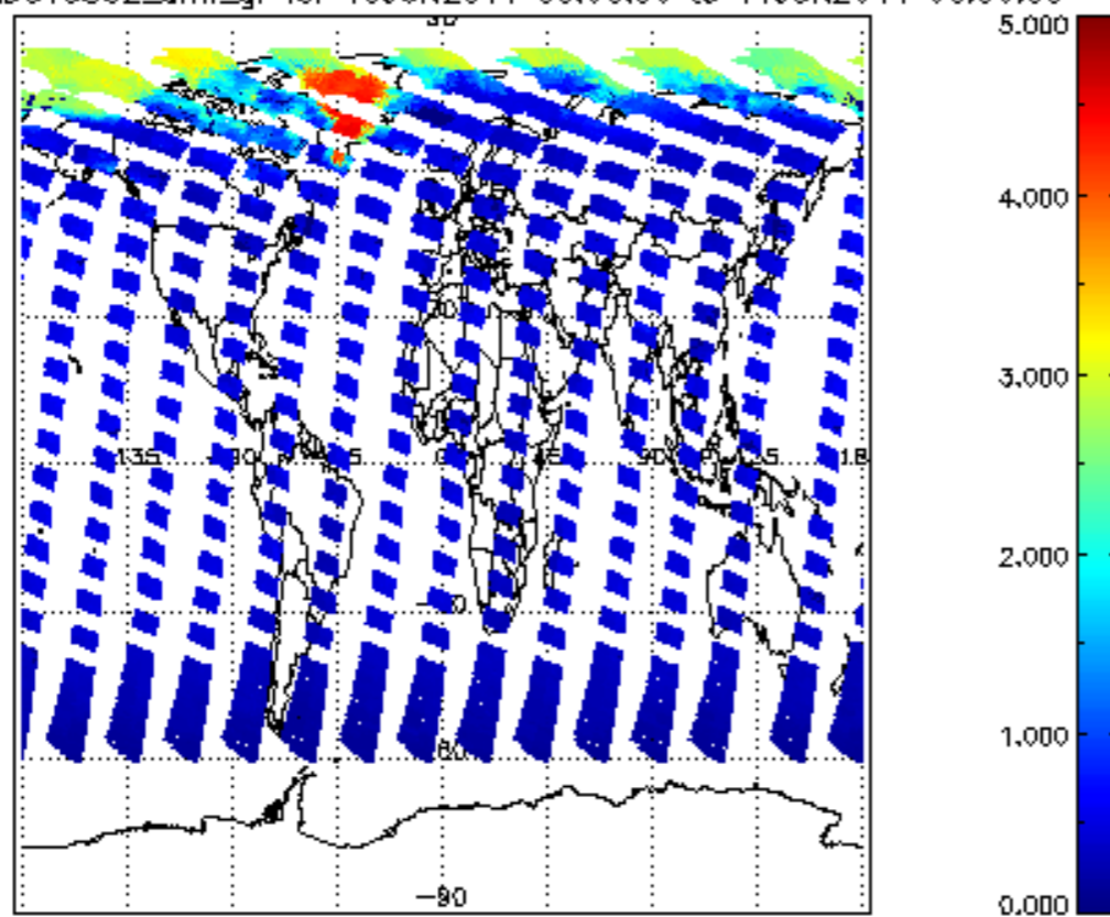
SCIOL2P_NADUV5S02_amf_gr for 10JUN2011 00:00:00 to 11JUN2011 00:00:00
