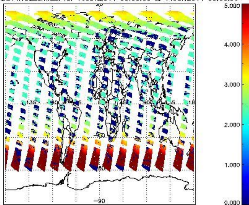
SCIOL2P_NADUV1NO2_amf_cl for 10JUN2011 00:00:00 to 11JUN2011 00:00:00
