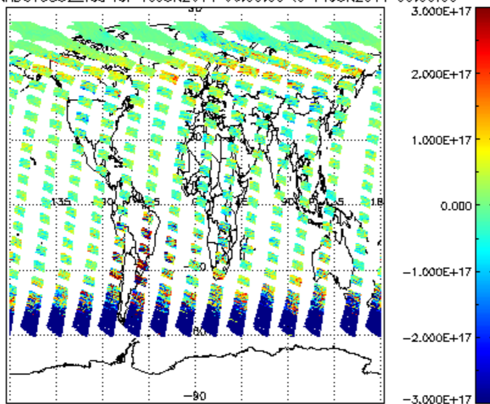
SCIOL2P_NADUV5S02_vcd for 10JUN2011 00:00:00 to 11JUN2011 00:00:00
