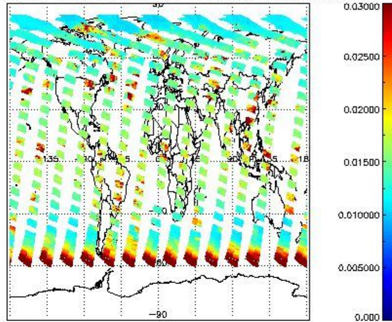
SCIOL2P_NADUV003_vcd_err for 10JUN2011 00:00:00 to 11JUN2011 00:00:00
