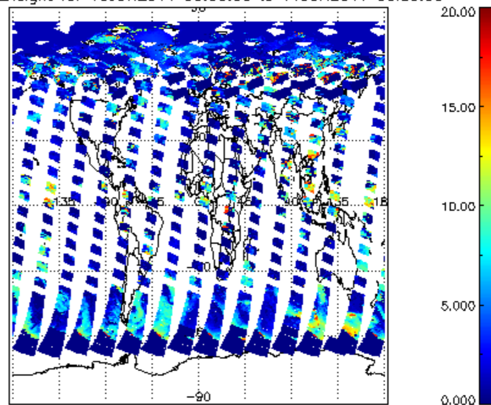
cl_top_height for 10JUN2011 00:00:00 to 11JUN2011 00:00:00
