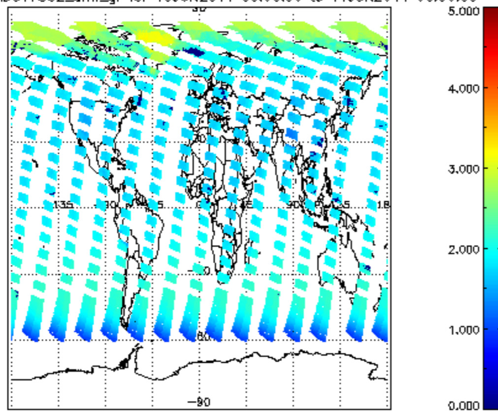
SCIOL2P_NADUV7S02_amf_gr for 10JUN2011 00:00:00 to 11JUN2011 00:00:00
