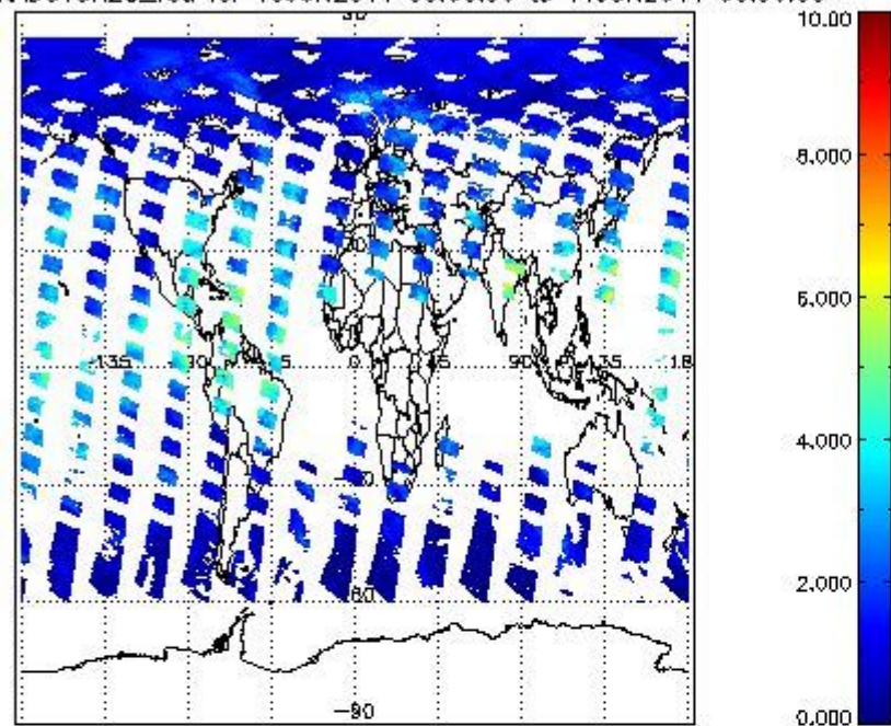
SCIOL2P_NADUV8H2O_vcd for 10JUN2011 00:00:00 to 11JUN2011 00:00:00
