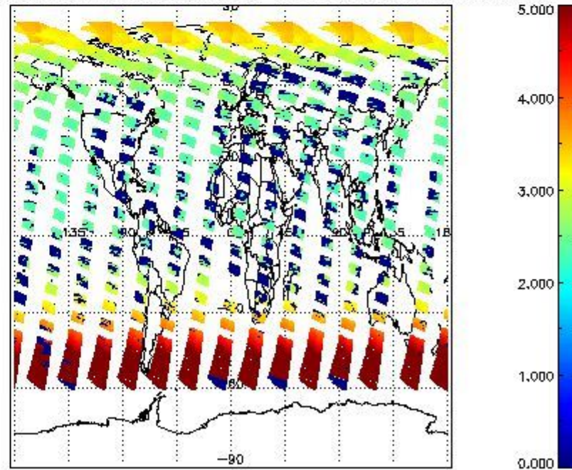
SCIOL2P_NADUV003_amf_cl for 10JUN2011 00:00:00 to 11JUN2011 00:00:00
