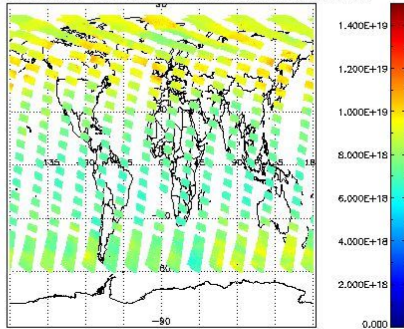
SCIOL2P_NADUV003_vcd for 10JUN2011 00:00:00 to 11JUN2011 00:00:00
