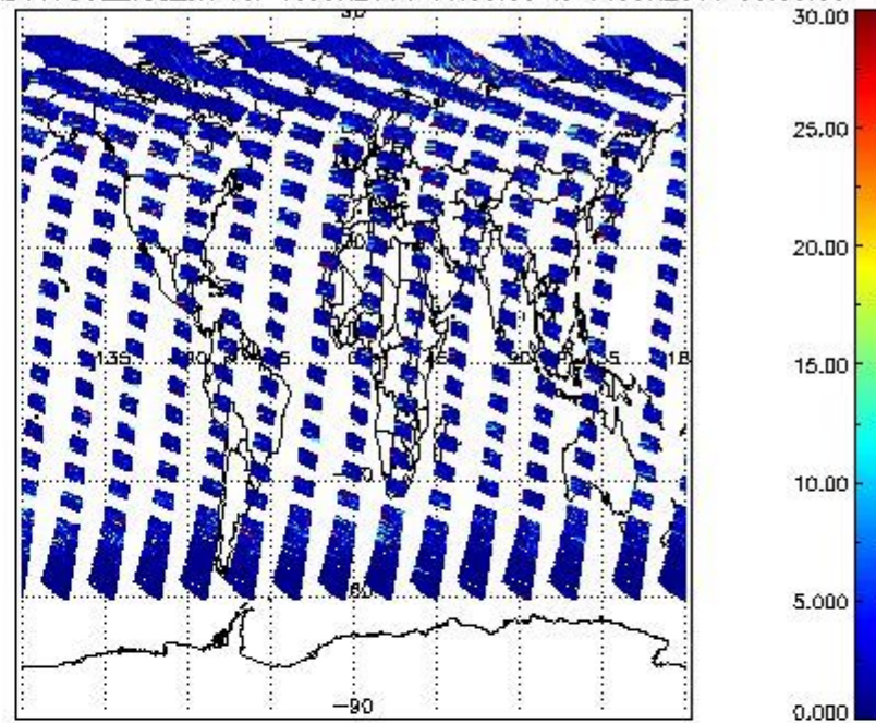
SCIOL2P_NADUV7S02_vcd_err for 10JUN2011 00:00:00 to 11JUN2011 00:00:00
