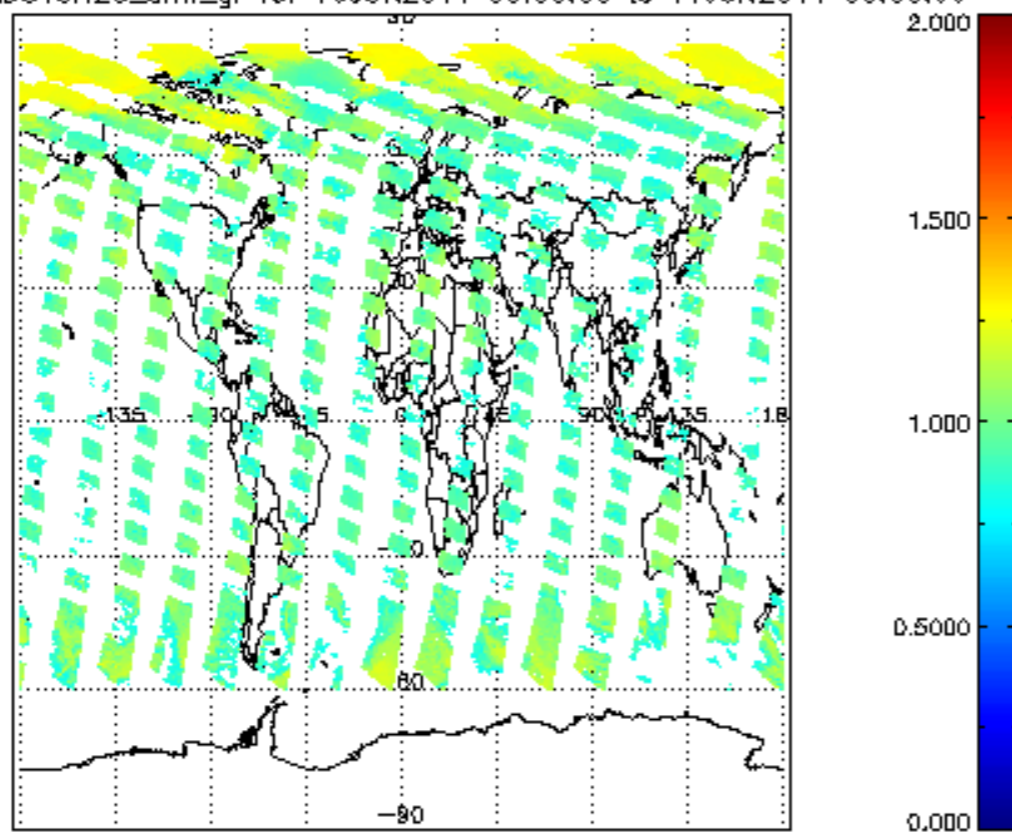
SCIOL2P_NADUV8H2O_amf_gr for 10JUN2011 00:00:00 to 11JUN2011 00:00:00
