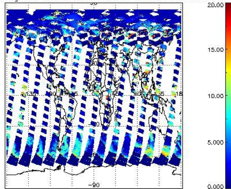
cL_top_height for 10JUN2011 00:00:00 to 11JUN2011 00:00:00
