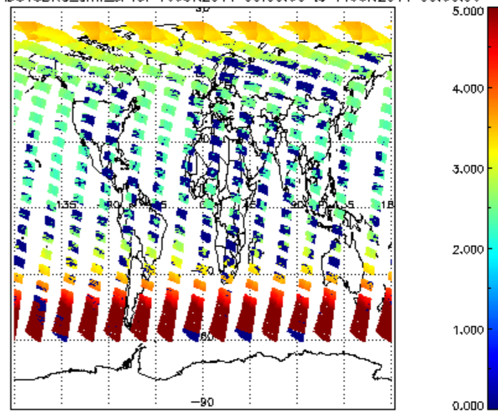
SCIOL2P_NADUV3BRO_amf_cl for 10JUN2011 00:00:00 to 11JUN2011 00:00:00
