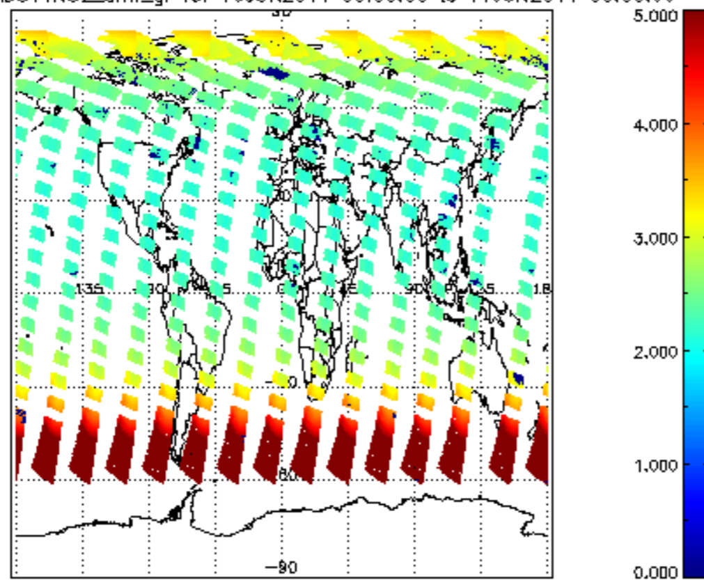
SCIOL2P_NADUV1NO2_amf_gr for 10JUN2011 00:00:00 to 11JUN2011 00:00:00
