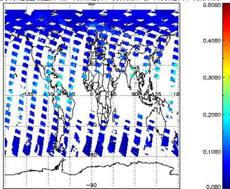
SCIOL2P_NADUV8H2O_vcd_err for 10JUN2011 00:00:00 to 11JUN2011 00:00:00
