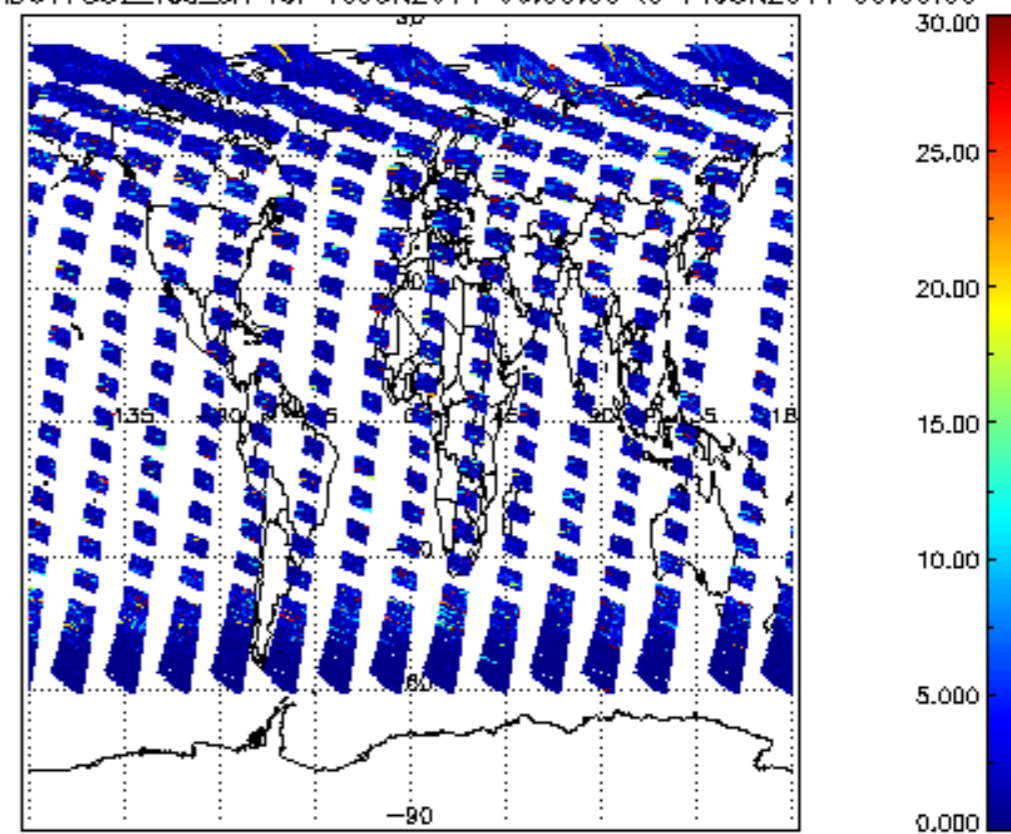
SCIOL2P_NADUV7S02_vcd_err for 10JUN2011 00:00:00 to 11JUN2011 00:00:00
