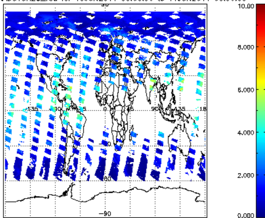
SCIOL2P_NADUV8H2O_vcd for 10JUN2011 00:00:00 to 11JUN2011 00:00:00
