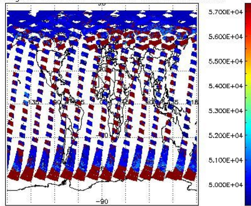
cloud_flags for 10JUN2011 00:00:00 to 11JUN2011 00:00:00
