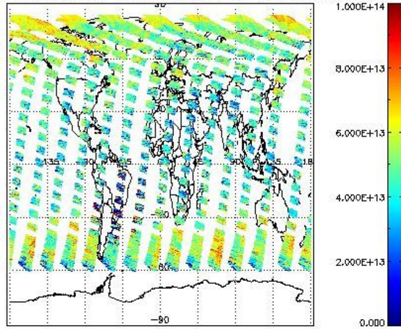
SCIOL2P_NADUV3BRO_vcd for 10JUN2011 00:00:00 to 11JUN2011 00:00:00
