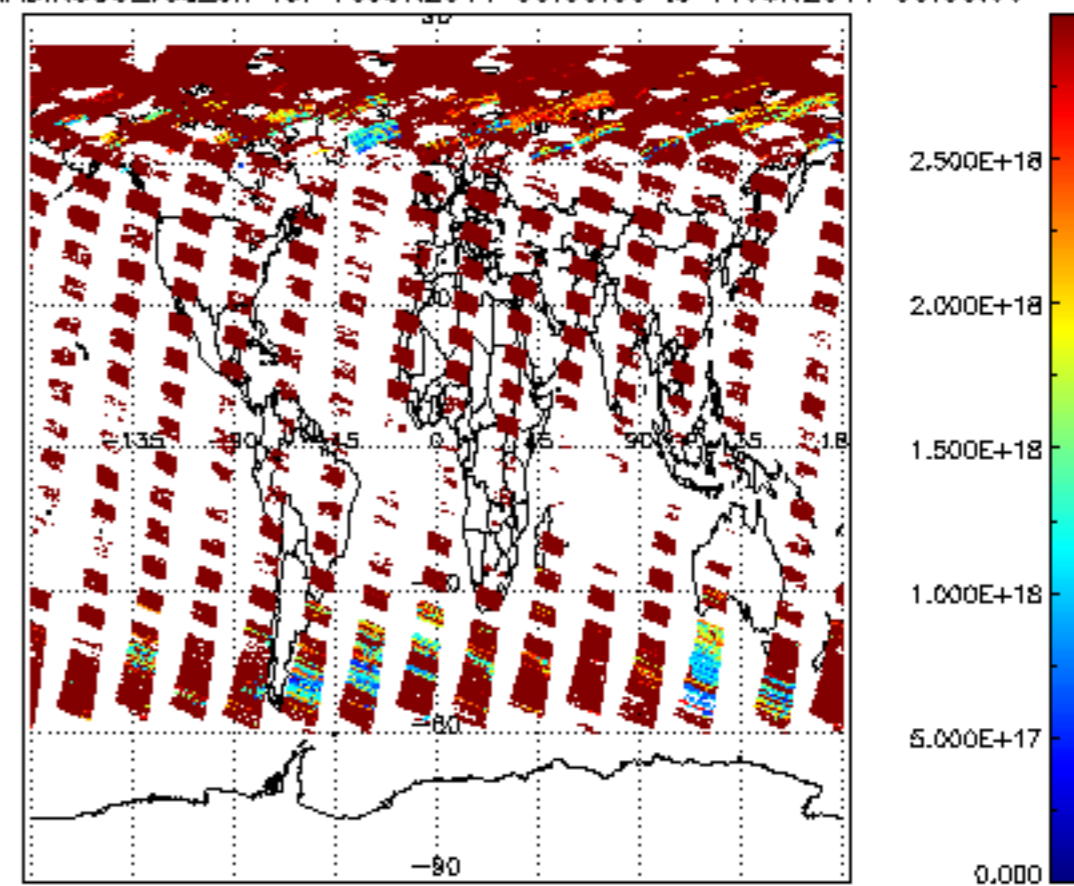
SCIOL2P_NADIR3CO_vcd_err for 10JUN2011 00:00:00 to 11JUN2011 00:00:00
