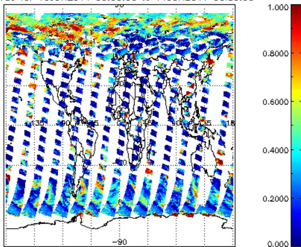
cl_frac for 10JUN2011 00:00:00 to 11JUN2011 00:00:00
