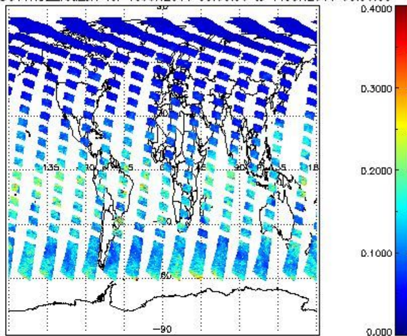
SCIOL2P_NADUV1NO2_vcd_err for 10JUN2011 00:00:00 to 11JUN2011 00:00:00
