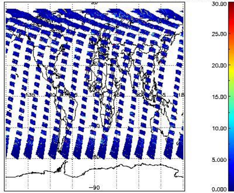
SCIOL2P_NADUV5S02_vcd_err for 10JUN2011 00:00:00 to 11JUN2011 00:00:00
