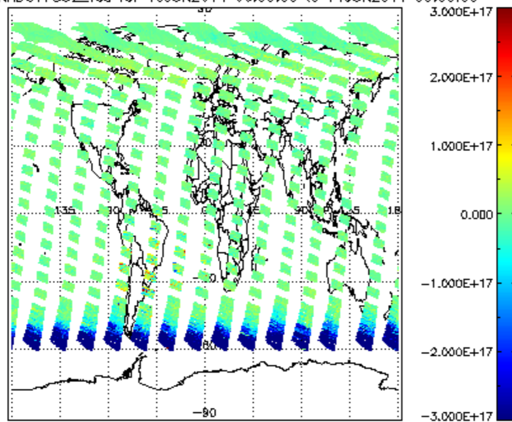
SCIOL2P_NADUV7S02_vcd for 10JUN2011 00:00:00 to 11JUN2011 00:00:00
