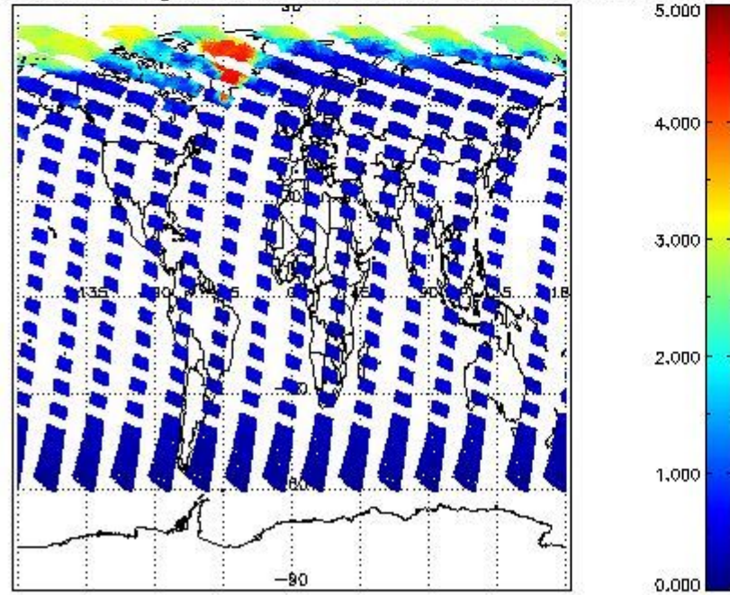
SCIOL2P_NADUV5S02_amf_gr for 10JUN2011 00:00:00 to 11JUN2011 00:00:00
