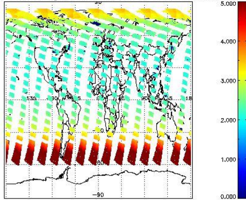
SCIOL2P_NADUV3BRO_amf_gr for 10JUN2011 00:00:00 to 11JUN2011 00:00:00
