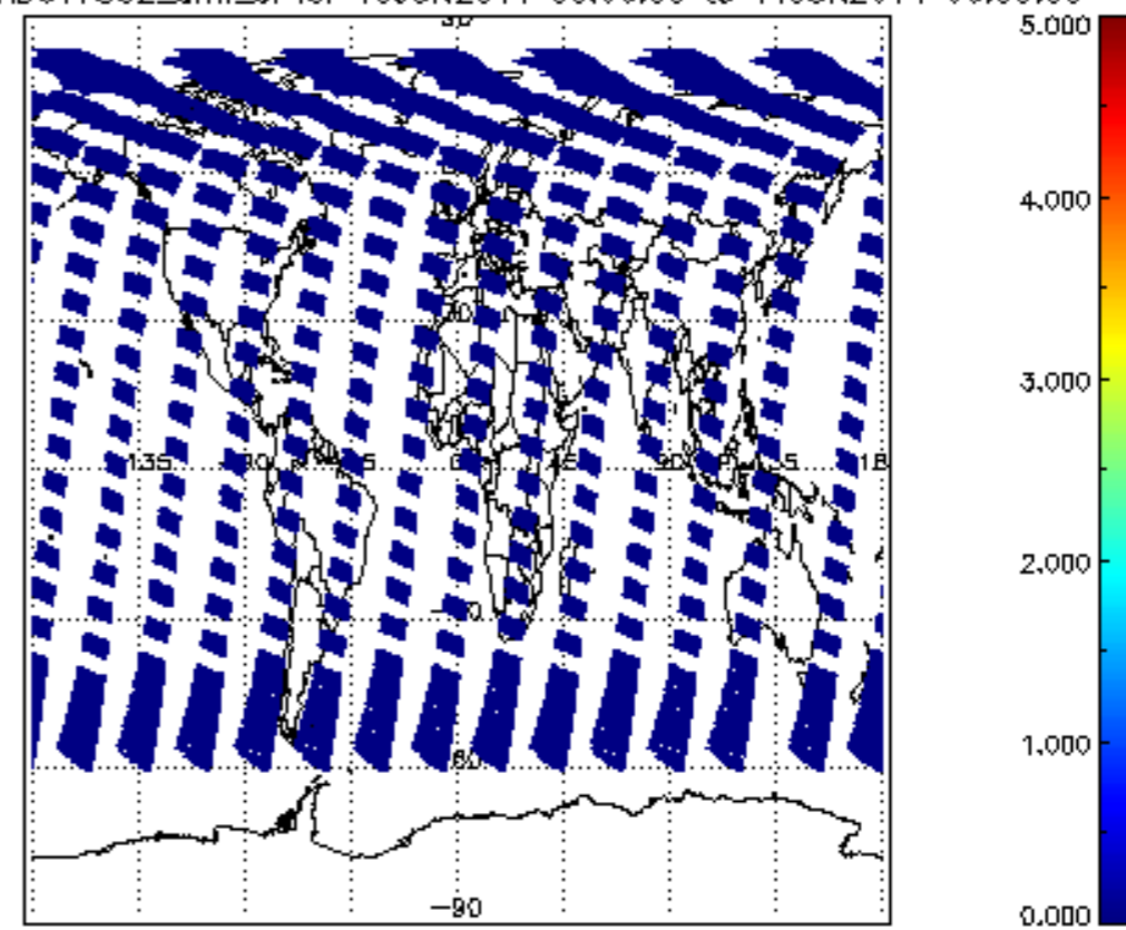
SCIOL2P_NADUV7S02_amf_cl for 10JUN2011 00:00:00 to 11JUN2011 00:00:00
