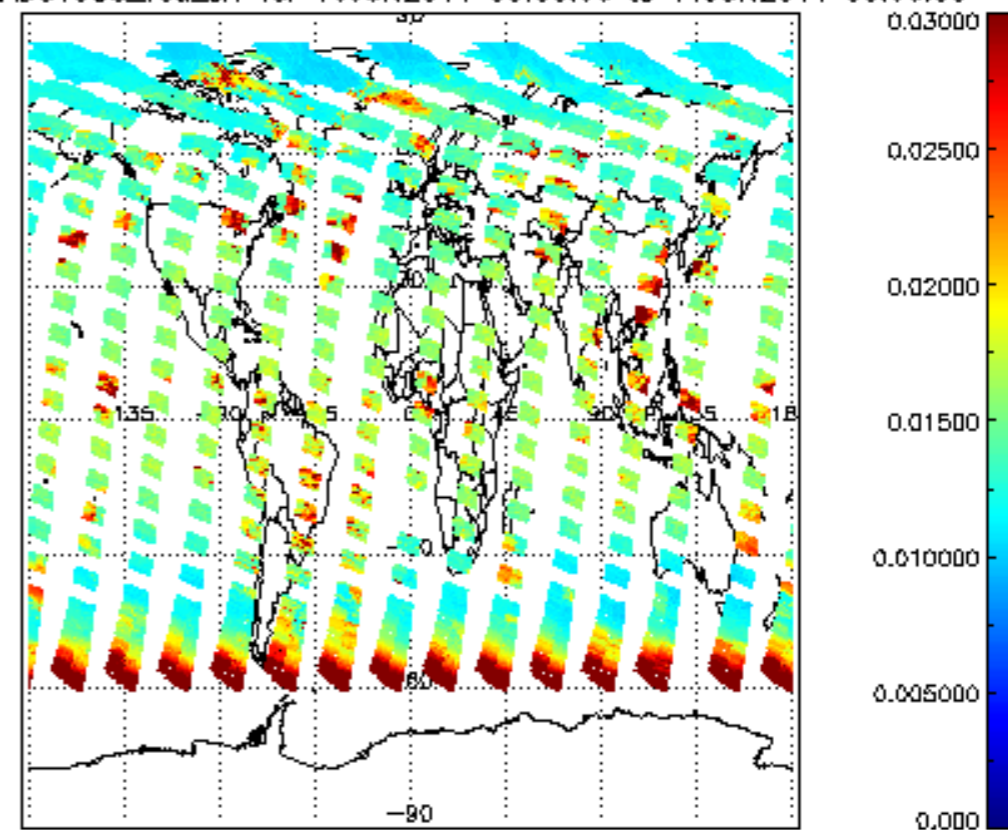
SCIOL2P_NADUV003_vcd_err for 10JUN2011 00:00:00 to 11JUN2011 00:00:00
