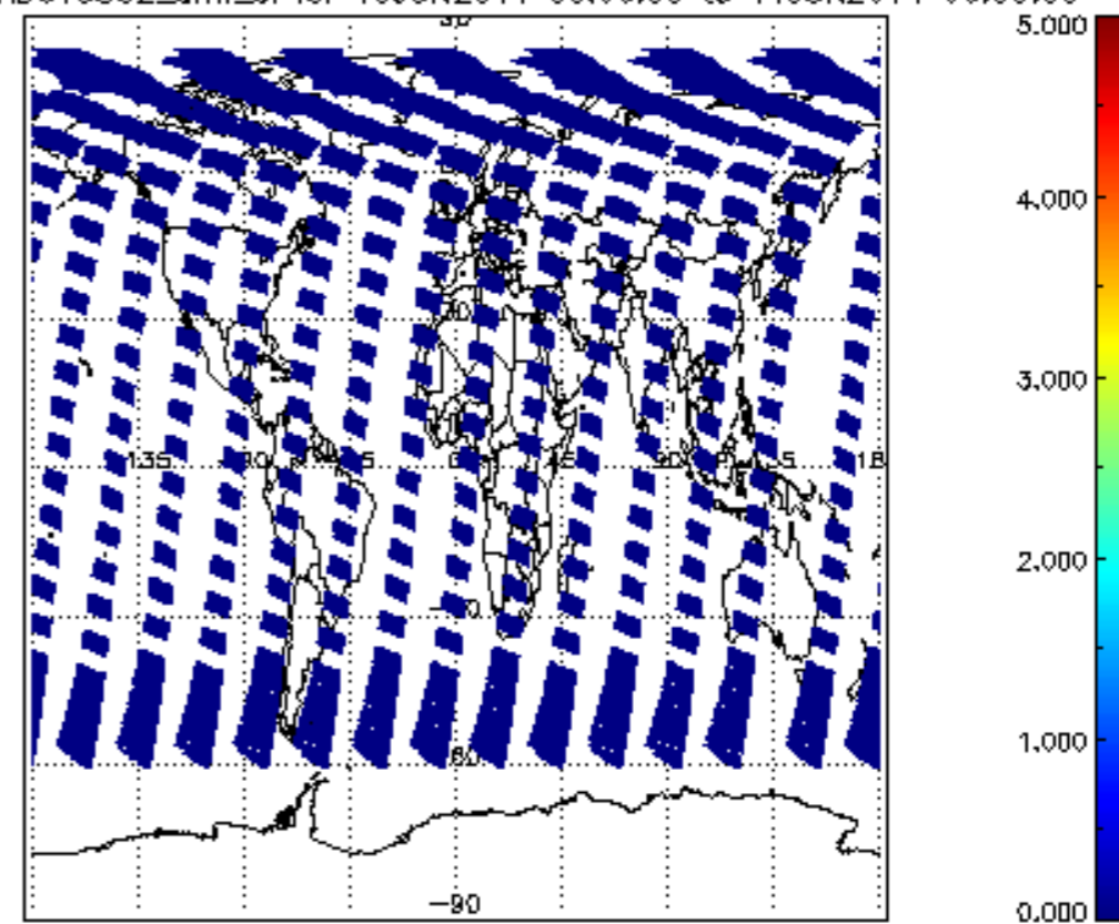
SCIOL2P_NADUV5S02_amf_cl for 10JUN2011 00:00:00 to 11JUN2011 00:00:00
