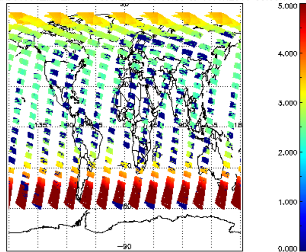
SCIOL2P_NADUV003_amf_cl for 10JUN2011 00:00:00 to 11JUN2011 00:00:00
