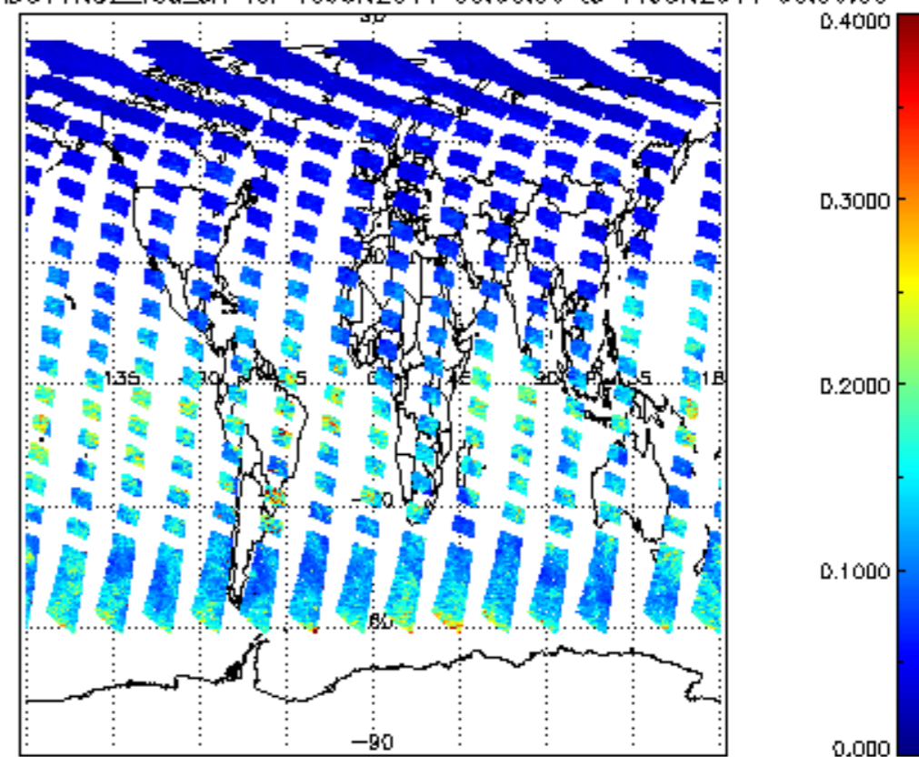
SCIOL2P_NADUV1NO2_vcd_err for 10JUN2011 00:00:00 to 11JUN2011 00:00:00
