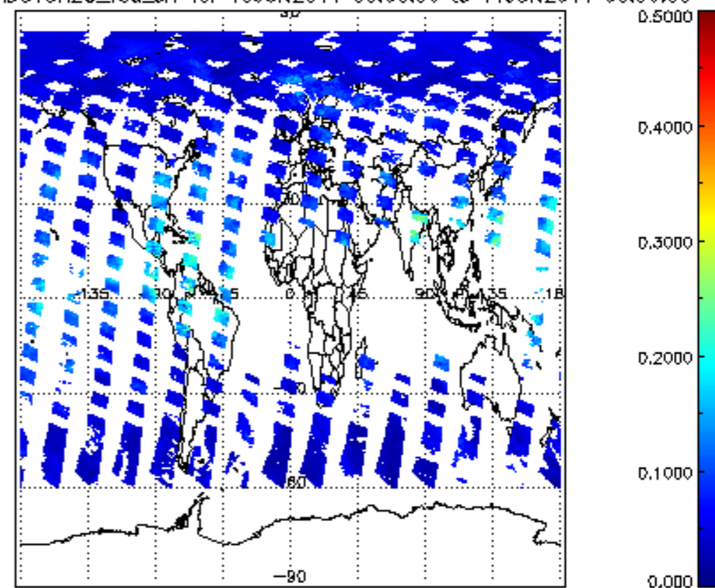
SCIOL2P_NADUV8H2O_vcd_err for 10JUN2011 00:00:00 to 11JUN2011 00:00:00
