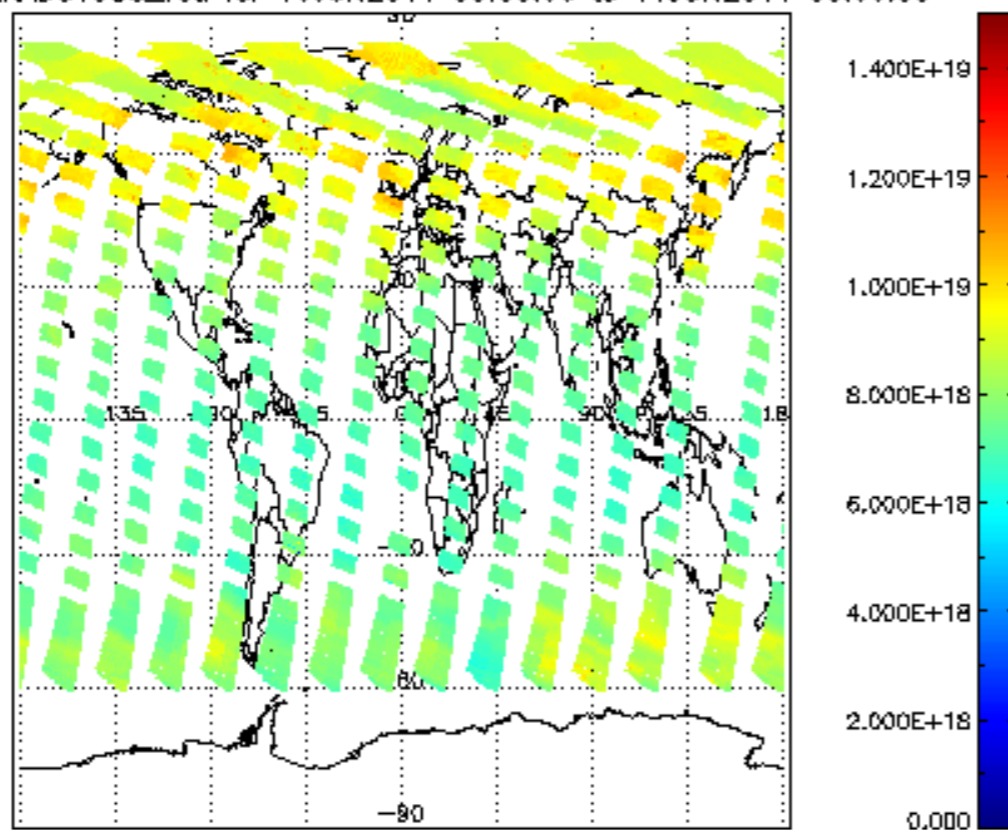
SCIOL2P_NADUV003_vcd for 10JUN2011 00:00:00 to 11JUN2011 00:00:00
