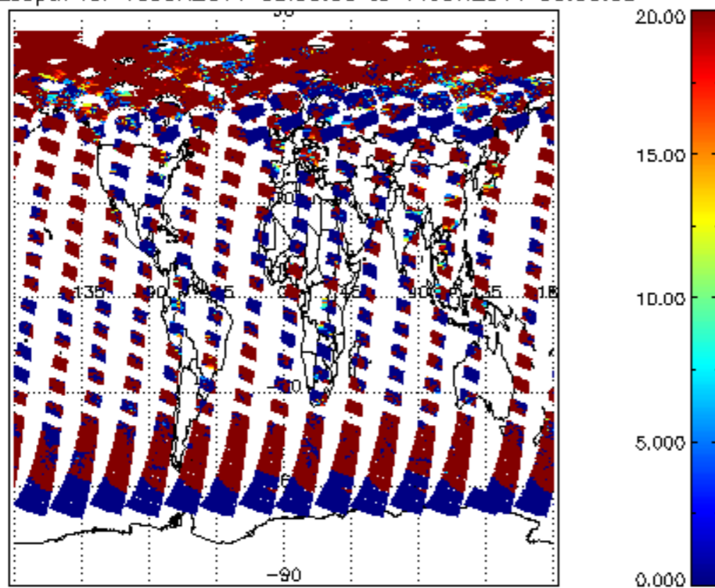
cl_opt_depth for 10JUN2011 00:00:00 to 11JUN2011 00:00:00
