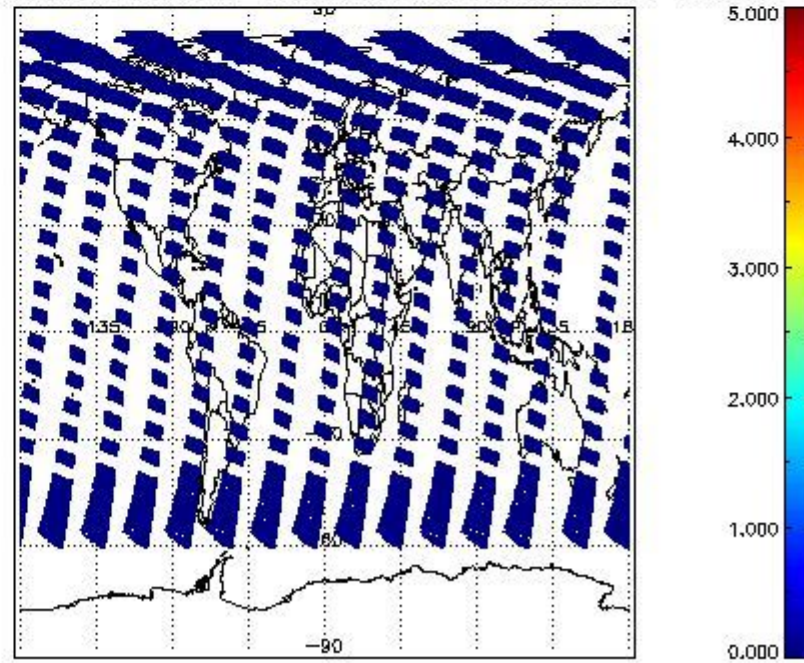
SCIOL2P_NADUV7S02_amf_cl for 10JUN2011 00:00:00 to 11JUN2011 00:00:00
