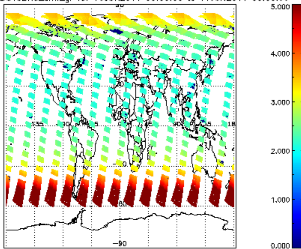
SCIOL2P_NADUV3BRO_amf_gr for 10JUN2011 00:00:00 to 11JUN2011 00:00:00
