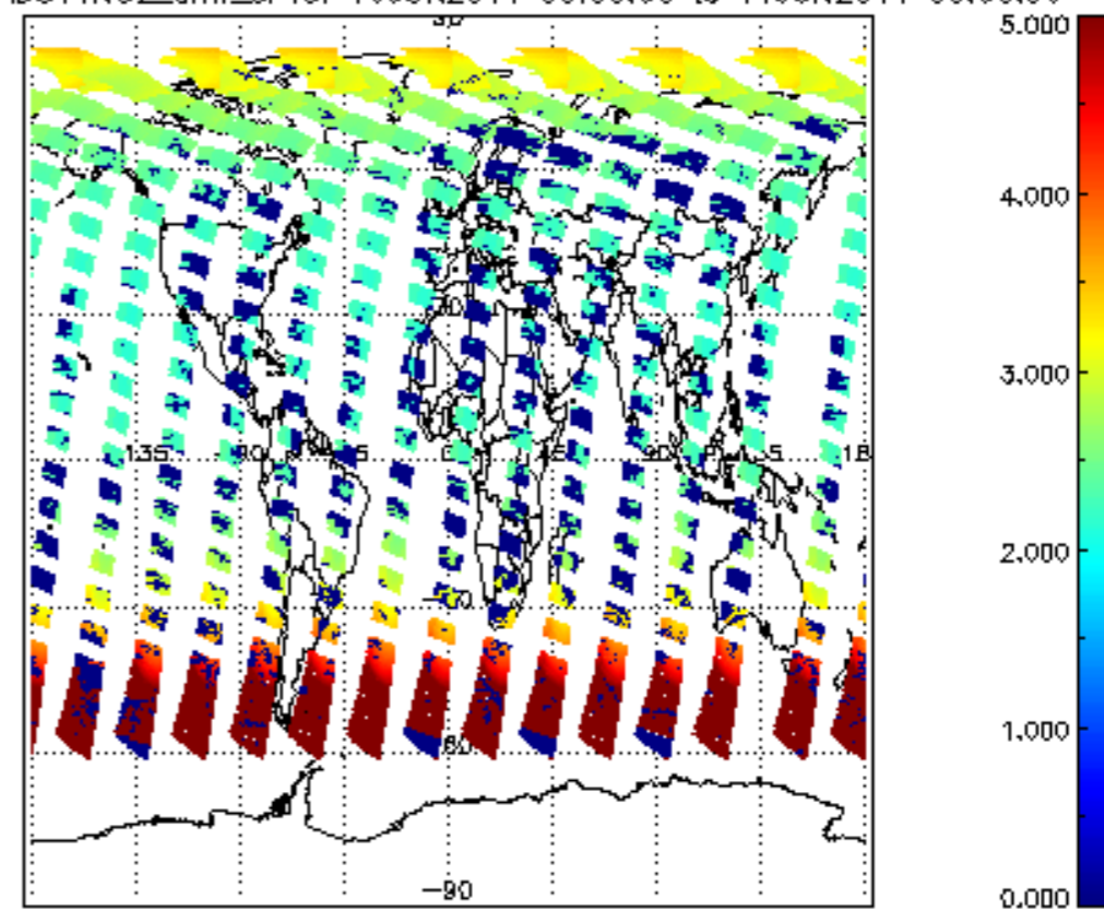
SCIOL2P_NADUV1NO2_amf_sl for 10JUN2011 00:00:00 to 11JUN2011 00:00:00
