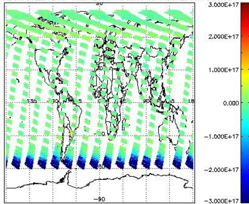
SCIOL2P_NADUV7S02_vcd for 10JUN2011 00:00:00 to 11JUN2011 00:00:00
