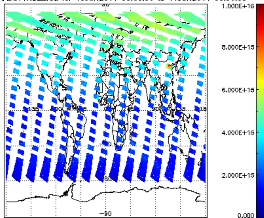
SCIOL2P_NADUV1NO2_vcd for 10JUN2011 00:00:00 to 11JUN2011 00:00:00
