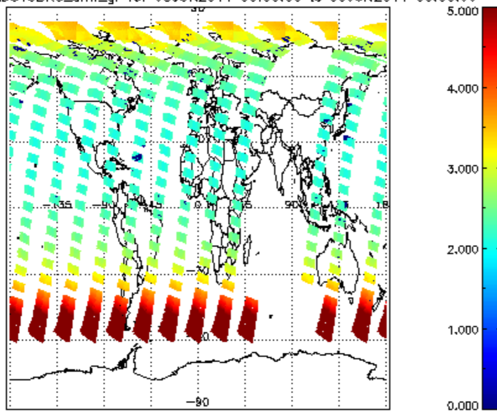
SCIOL2P_NADUV3BRO_amf_gr for 08JUN2011 00:00:00 to 09JUN2011 00:00:00
