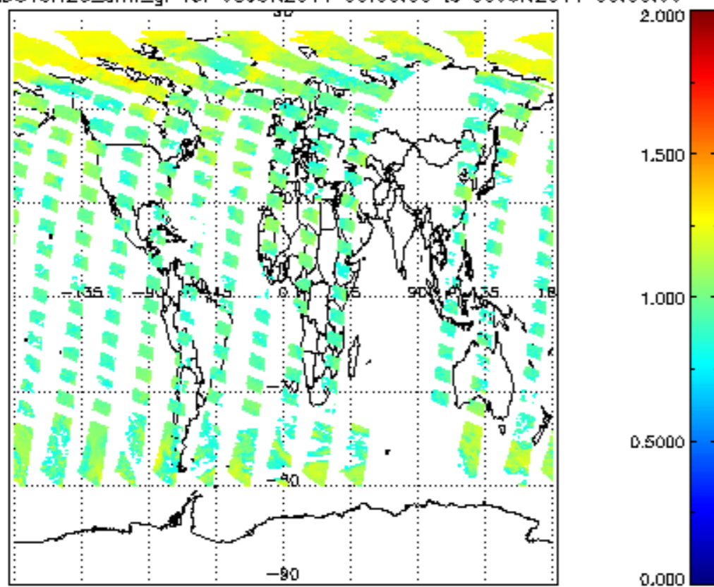
SCIOL2P_NADUV8H2O_amf_gr for 08JUN2011 00:00:00 to 09JUN2011 00:00:00
