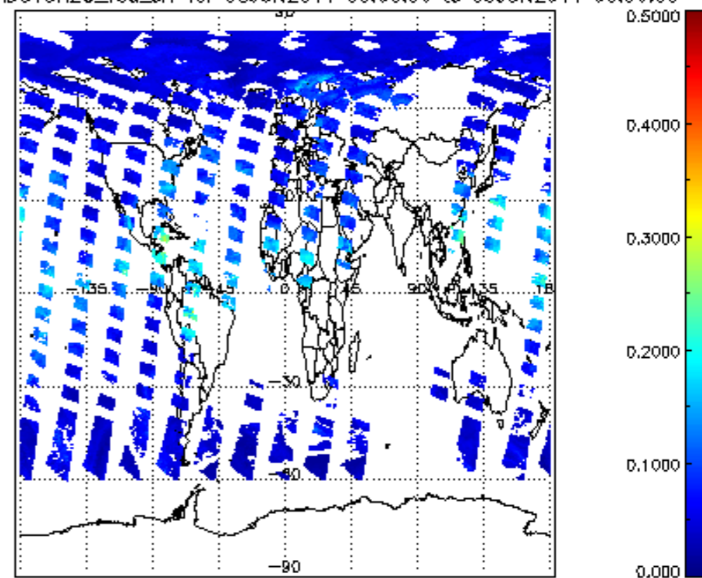
SCIOL2P_NADUV8H2O_vcd_err for 08JUN2011 00:00:00 to 09JUN2011 00:00:00
