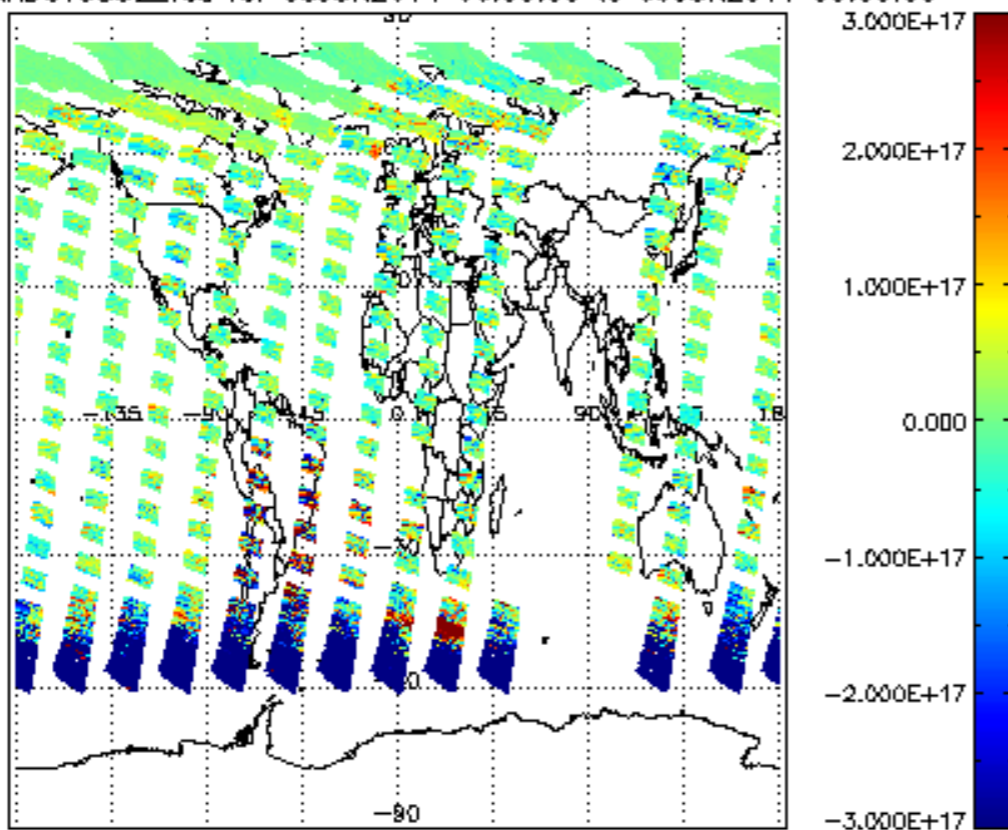
SCIOL2P_NADUV5S02_vcd for 08JUN2011 00:00:00 to 09JUN2011 00:00:00
