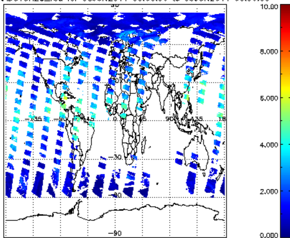
SCIOL2P_NADUV8H2O_vcd for 08JUN2011 00:00:00 to 09JUN2011 00:00:00
