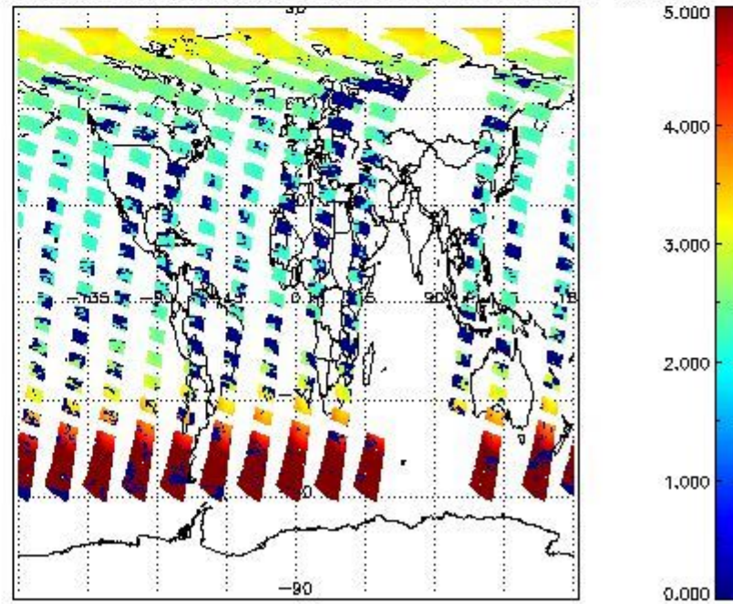
SCIOL2P_NADUV1N02_amf_cl for 08JUN2011 00:00:00 to 09JUN2011 00:00:00
