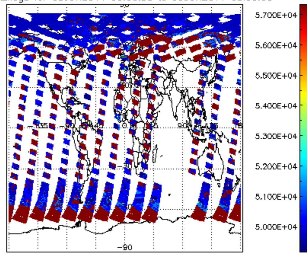
cloud_flags for 08JUN2011 00:00:00 to 09JUN2011 00:00:00
