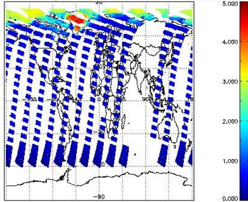
SCIOL2P_NADUV5S02_amf_gr for 08JUN2011 00:00:00 to 09JUN2011 00:00:00
