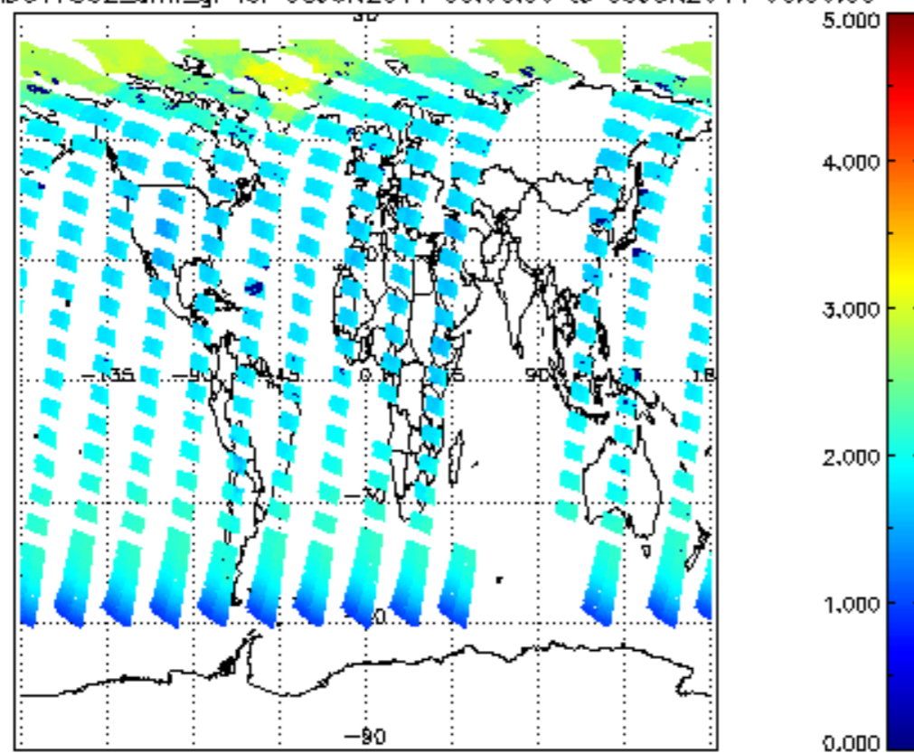
SCIOL2P_NADUV7S02_amf_gr for 08JUN2011 00:00:00 to 09JUN2011 00:00:00
