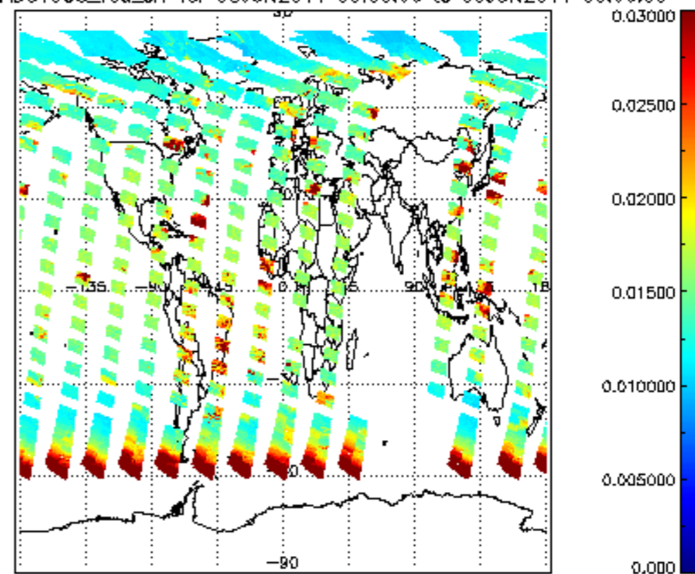
SCIOL2P_NADUV003_vcd_err for 08JUN2011 00:00:00 to 09JUN2011 00:00:00
