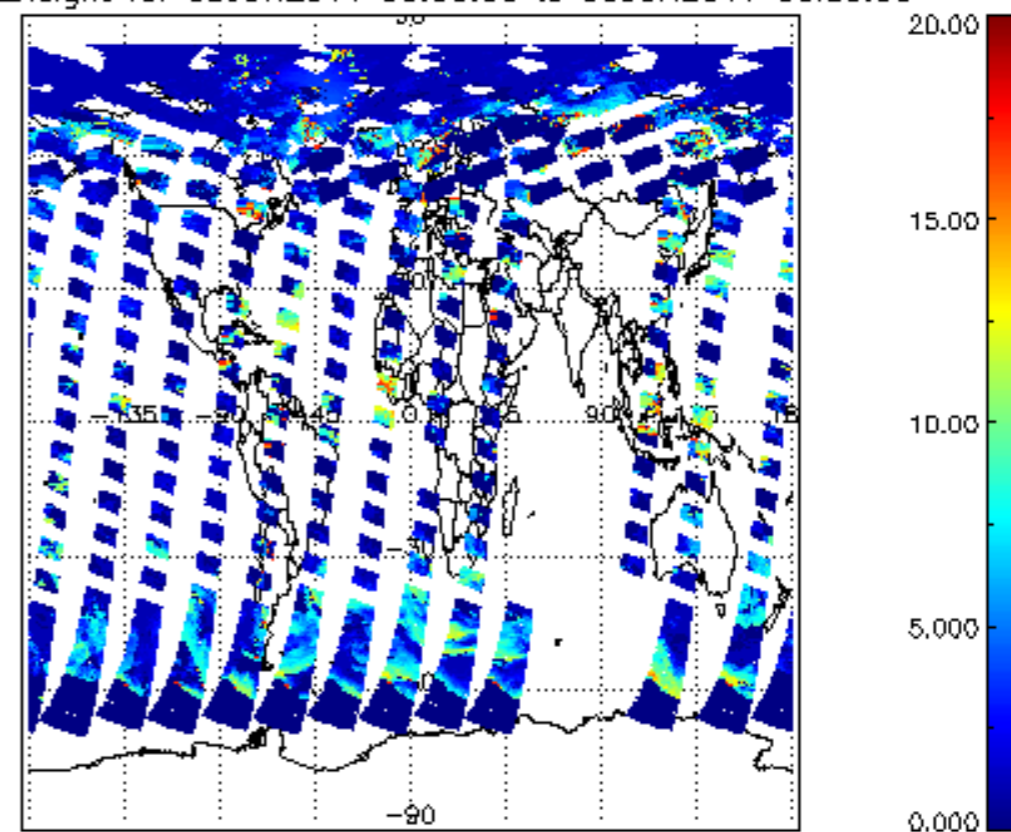
cl_top_height for 08JUN2011 00:00:00 to 09JUN2011 00:00:00
