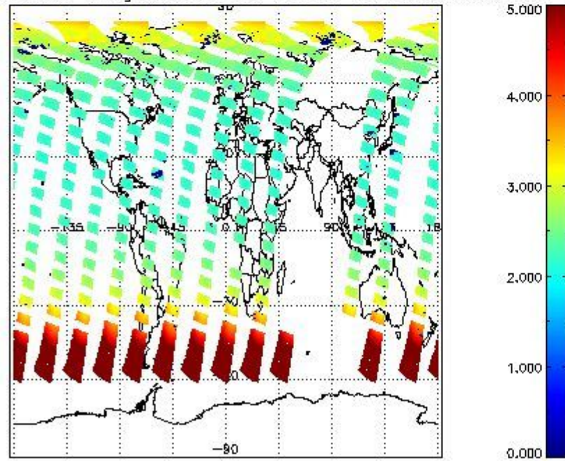
SCIOL2P_NADUV1N02_amf_gr for 08JUN2011 00:00:00 to 09JUN2011 00:00:00
