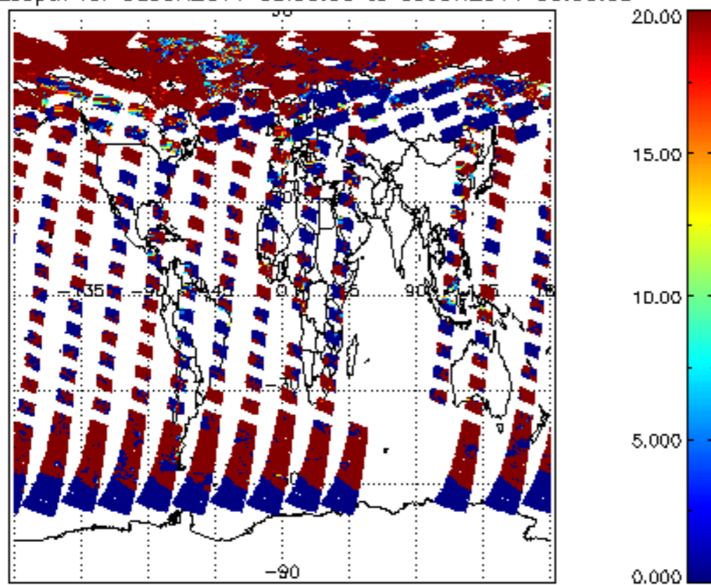
cl_opt_depth for 08JUN2011 00:00:00 to 09JUN2011 00:00:00
