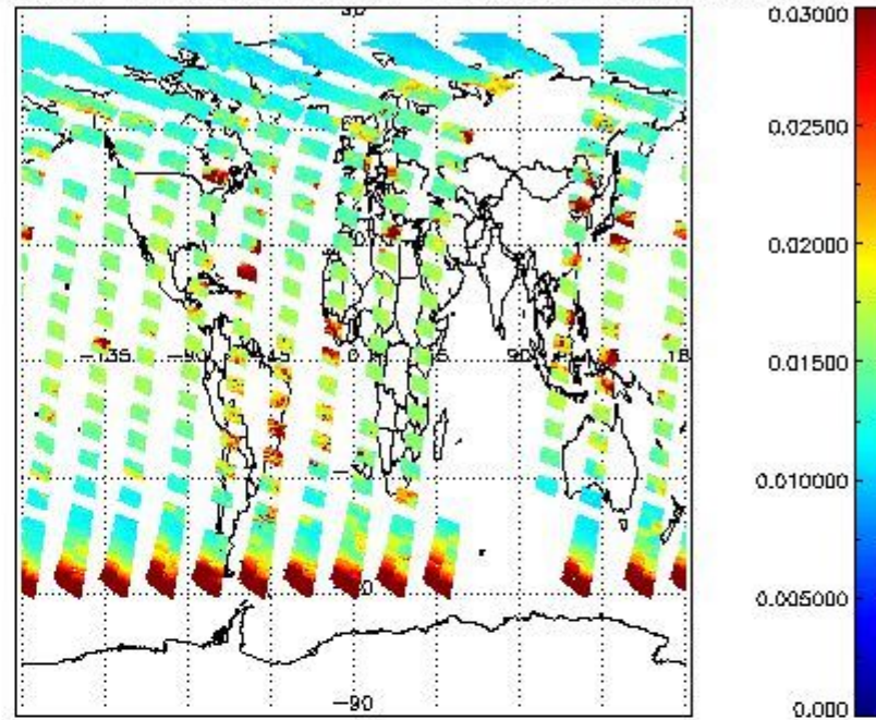
SCIOL2P_NADUV003_vcd_err for 08JUN2011 00:00:00 to 09JUN2011 00:00:00
