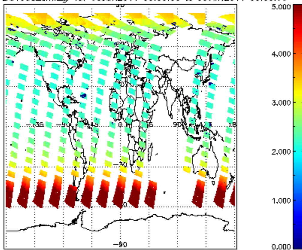
SCIOL2P_NADUV003_amf_gr for 08JUN2011 00:00:00 to 09JUN2011 00:00:00
