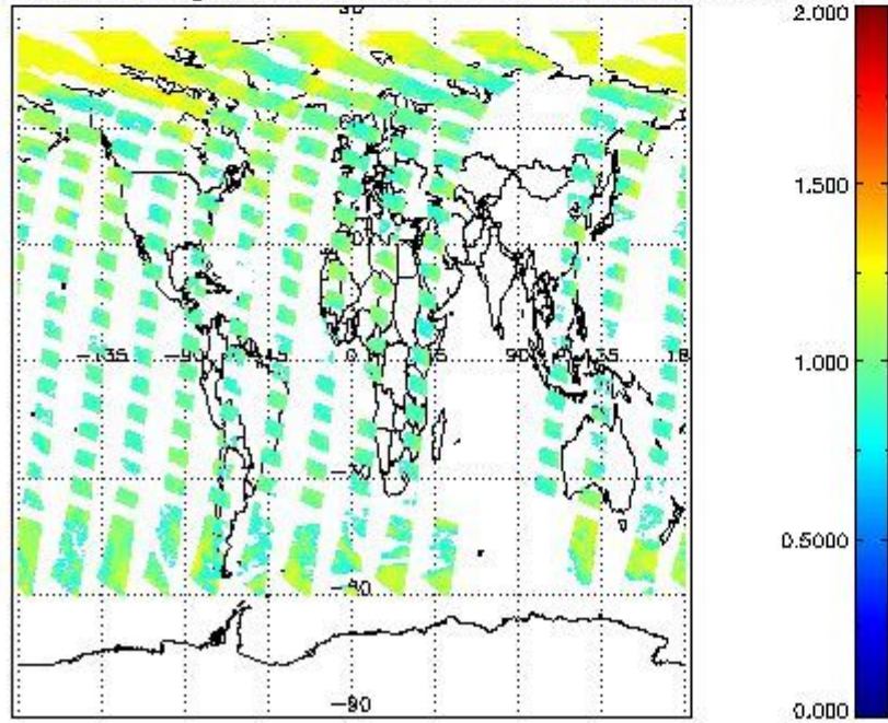
SCIOL2P_NADUV8H2O_arnf_gr for 08JUN2011 00:00:00 to 09JUN2011 00:00:00
