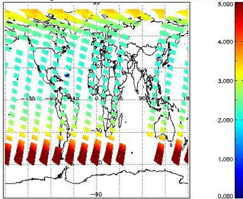
SCIOL2P_NADUV003_amf_gr for 08JUN2011 00:00:00 to 09JUN2011 00:00:00
