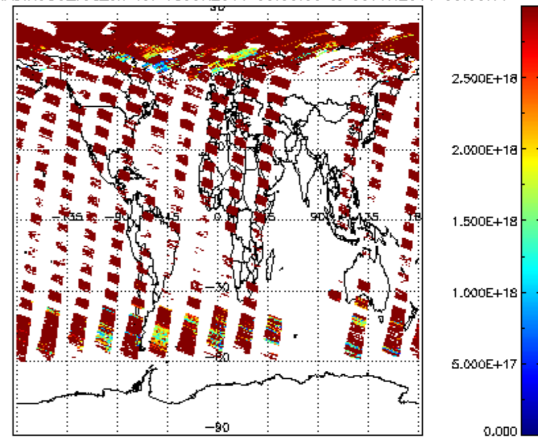
SCIOL2P_NADIR3CO_vcd_err for 08JUN2011 00:00:00 to 09JUN2011 00:00:00
