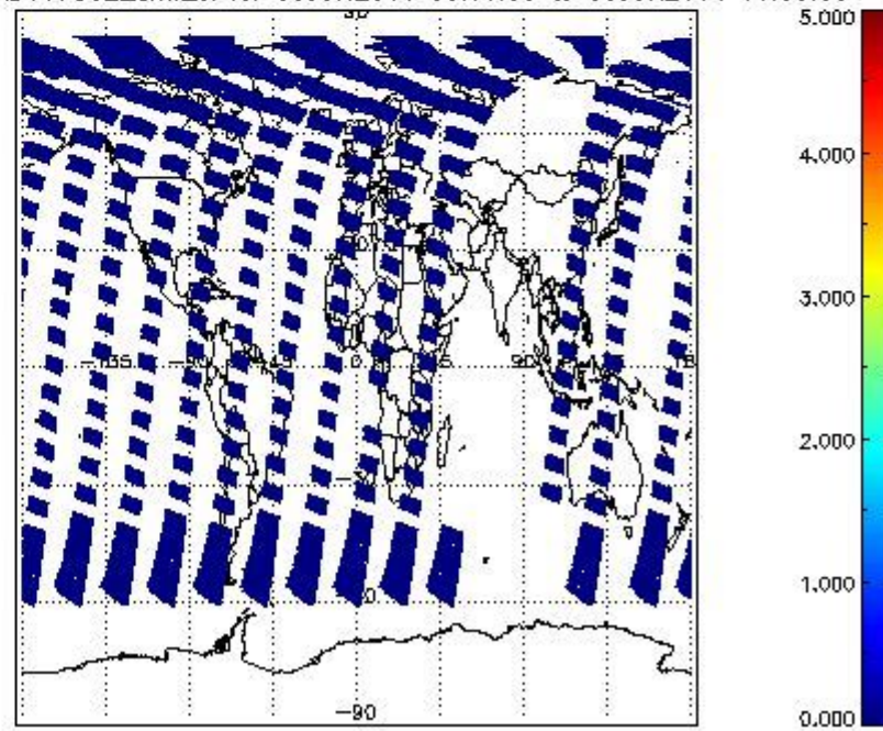
SCIOL2P_NADUV7S02_amf_cl for 08JUN2011 00:00:00 to 09JUN2011 00:00:00
