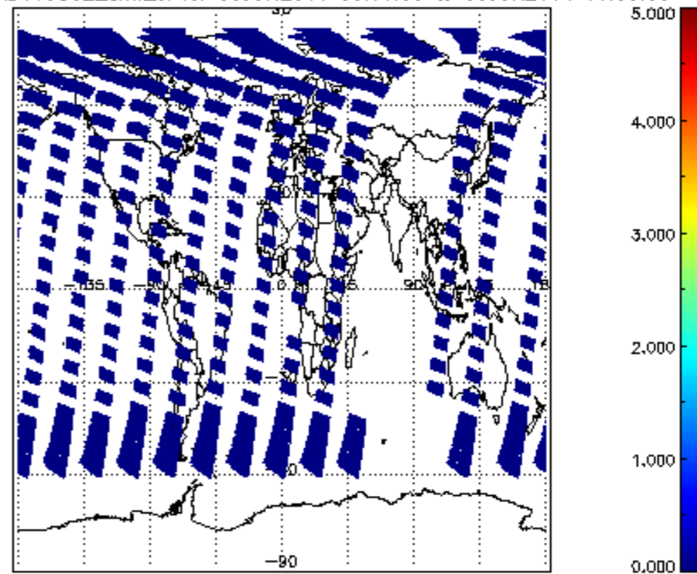
SCIOL2P_NADUV5S02_amf_cl for 08JUN2011 00:00:00 to 09JUN2011 00:00:00
