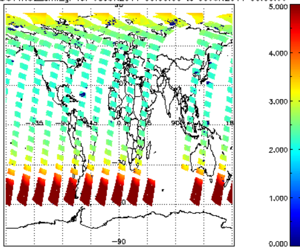
SCIOL2P_NADUV1NO2_amf_gr for 08JUN2011 00:00:00 to 09JUN2011 00:00:00
