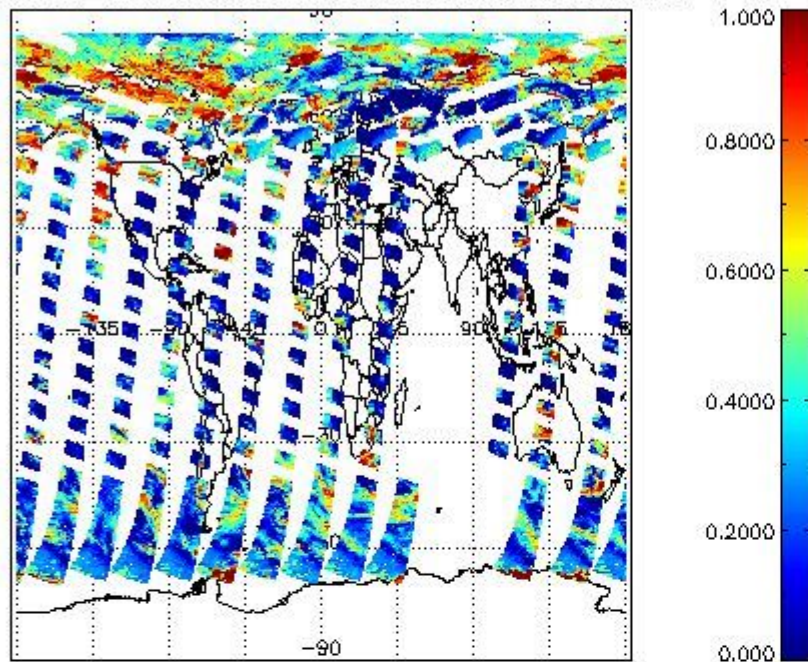
cL_frac for 08JUN2011 00:00:00 to 09JUN2011 00:00:00
