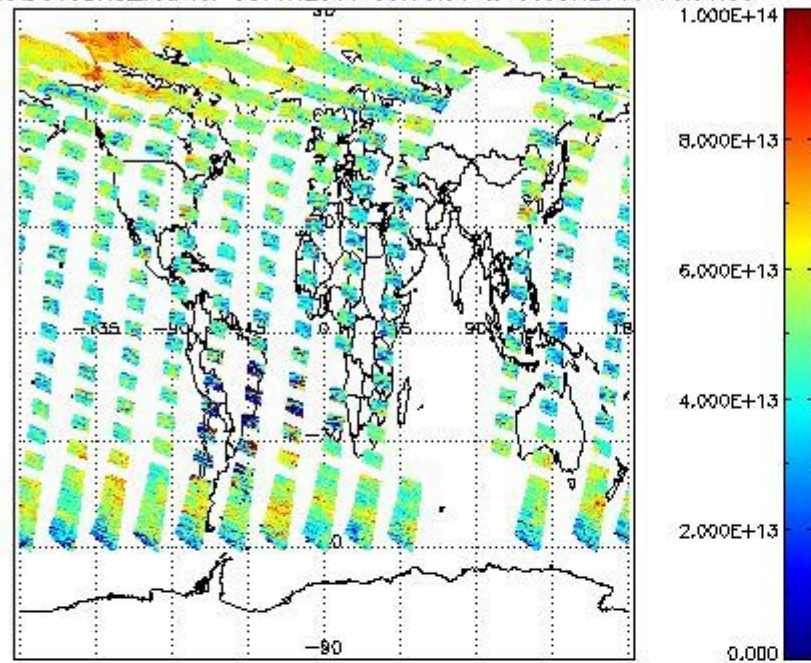
SCIOL2P_NADUV3BRO_vcd for 08JUN2011 00:00:00 to 09JUN2011 00:00:00
