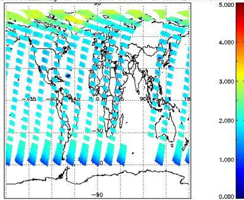
SCIOL2P_NADUV7S02_amf_gr for 08JUN2011 00:00:00 to 09JUN2011 00:00:00
