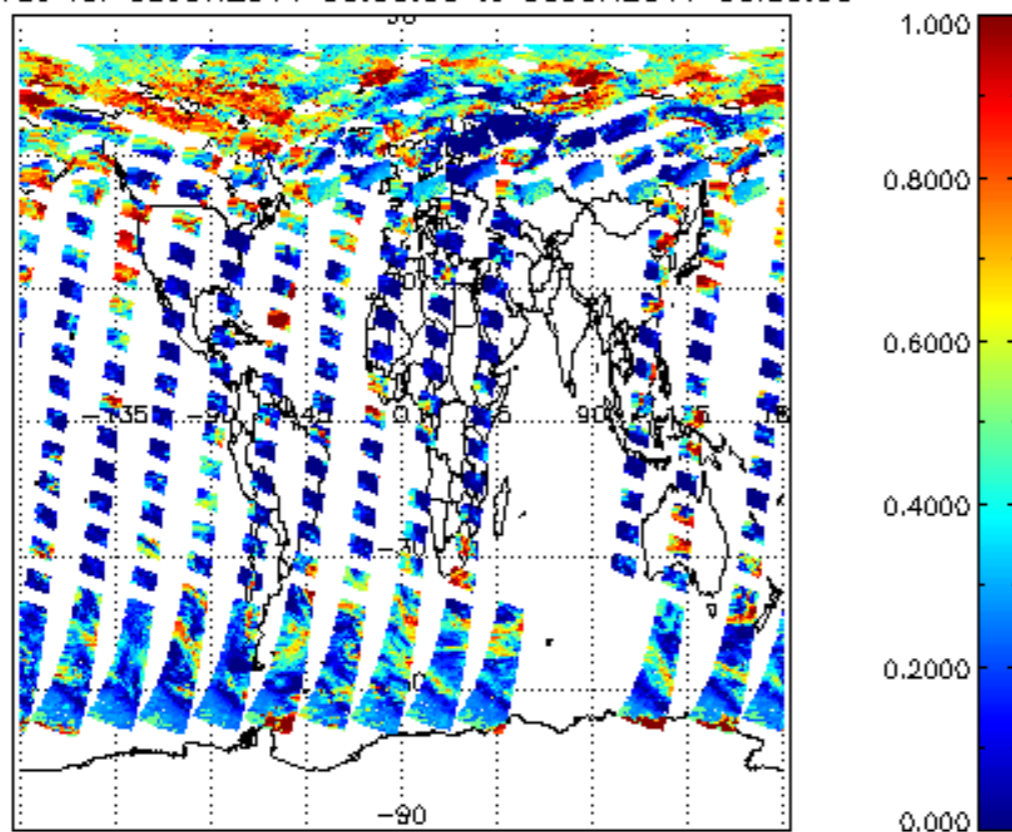
cl_frac for 08JUN2011 00:00:00 to 09JUN2011 00:00:00
