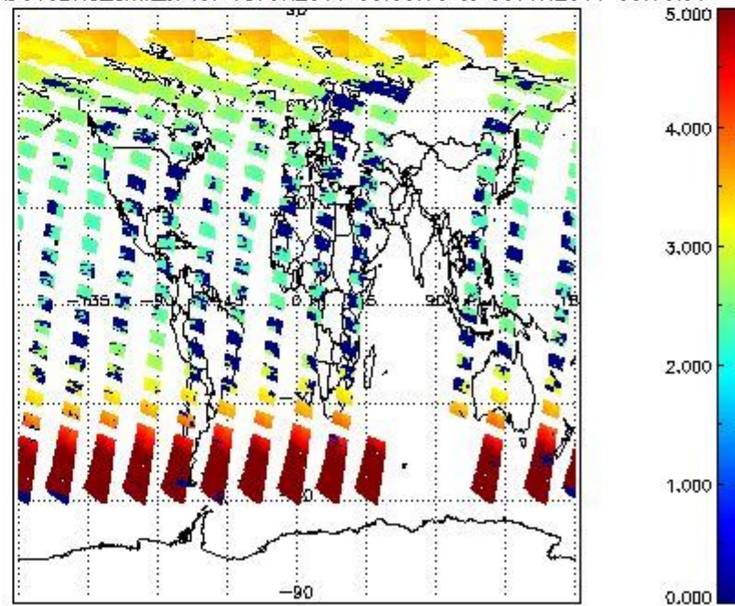
SCIOL2P_NADUV3BRO_amf_cl for 08JUN2011 00:00:00 to 09JUN2011 00:00:00
