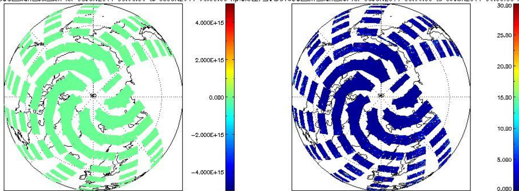
CIOL2P_NADUV6OCLslant_col_den for 08JUN2011 00:00:00 to 09JUN2011 00:00:00 np; CIOL2P_NADUV6OCLarr_slant_col for 08JUN2011 00:00:00 to 09JUN2011 00:00:00 np
