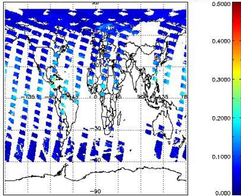
SCIOL2P_NADUV8H2O_vcd_err for 08JUN2011 00:00:00 to 09JUN2011 00:00:00
