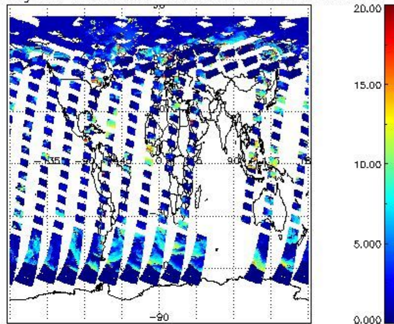
cL_top_height for 08JUN2011 00:00:00 to 09JUN2011 00:00:00
