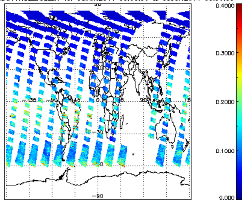
SCIOL2P_NADUV1NO2_vcd_err for 08JUN2011 00:00:00 to 09JUN2011 00:00:00
