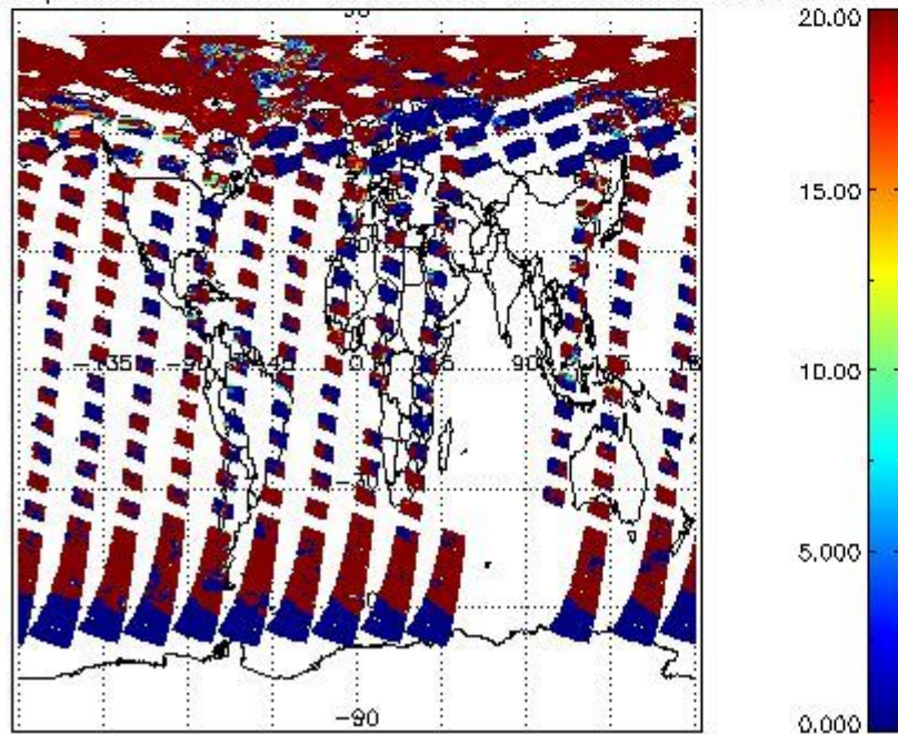
cL_opt_depth for 08JUN2011 00:00:00 to 09JUN2011 00:00:00
