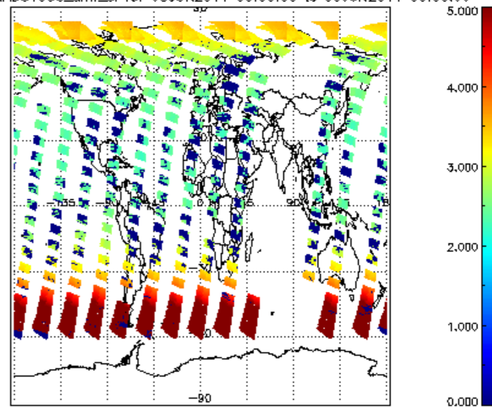
SCIOL2P_NADUV003_amf_cl for 08JUN2011 00:00:00 to 09JUN2011 00:00:00
