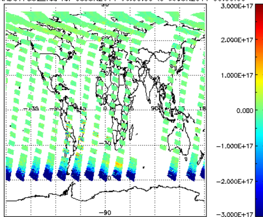
SCIOL2P_NADUV7S02_vcd for 08JUN2011 00:00:00 to 09JUN2011 00:00:00
