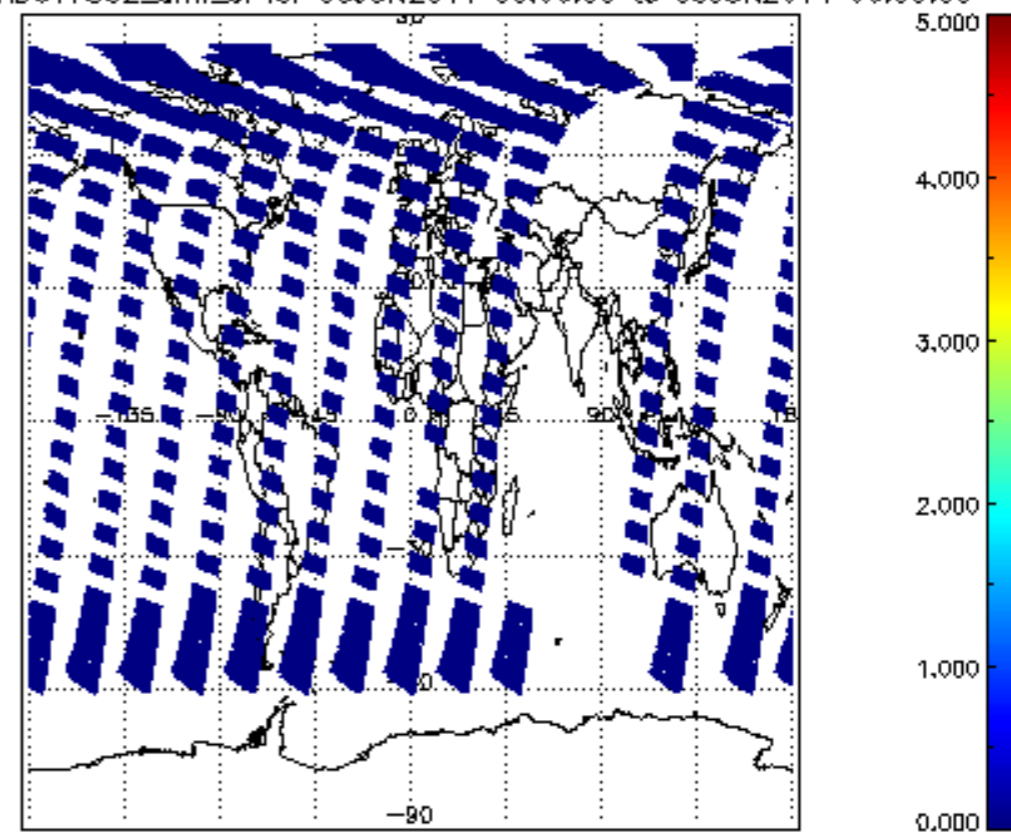
SCIOL2P_NADUV7S02_amf_cl for 08JUN2011 00:00:00 to 09JUN2011 00:00:00
