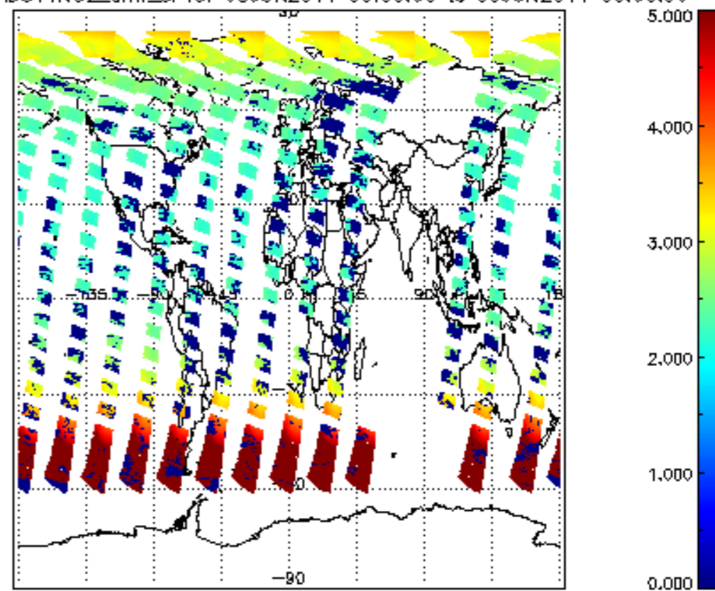
SCIOL2P_NADUV1NO2_amf_sl for 08JUN2011 00:00:00 to 09JUN2011 00:00:00
