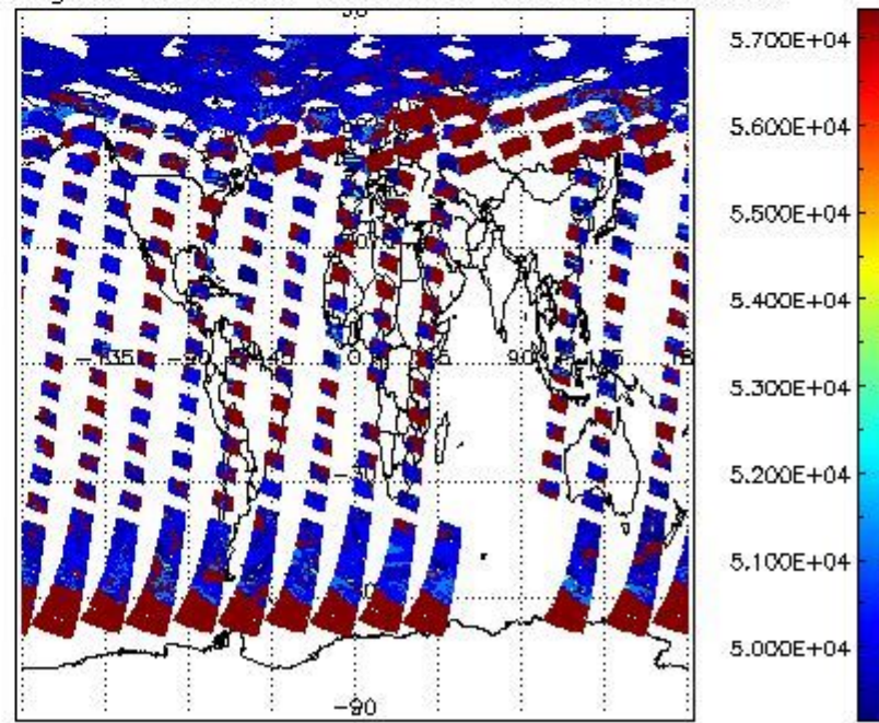
cloud_flags for 08JUN2011 00:00:00 to 09JUN2011 00:00:00
