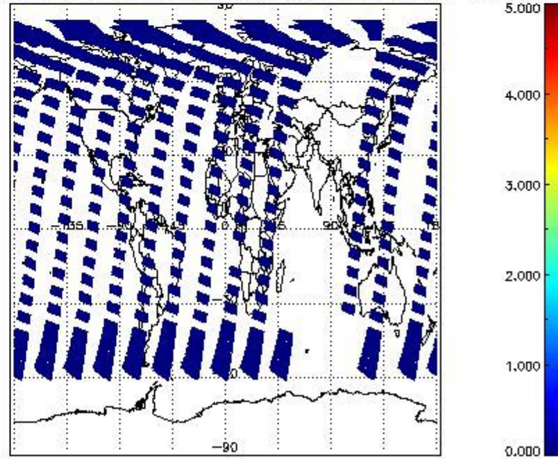
SCIOL2P_NADUV5S02_amf_cl for 08JUN2011 00:00:00 to 09JUN2011 00:00:00
