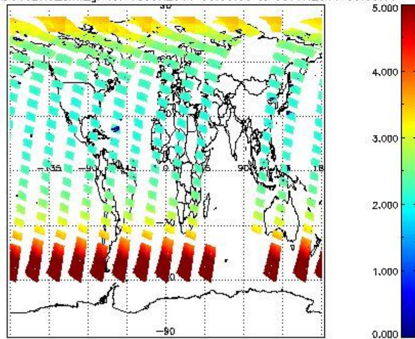
SCIOL2P_NADUV3BRO_amf_gr for 08JUN2011 00:00:00 to 09JUN2011 00:00:00
