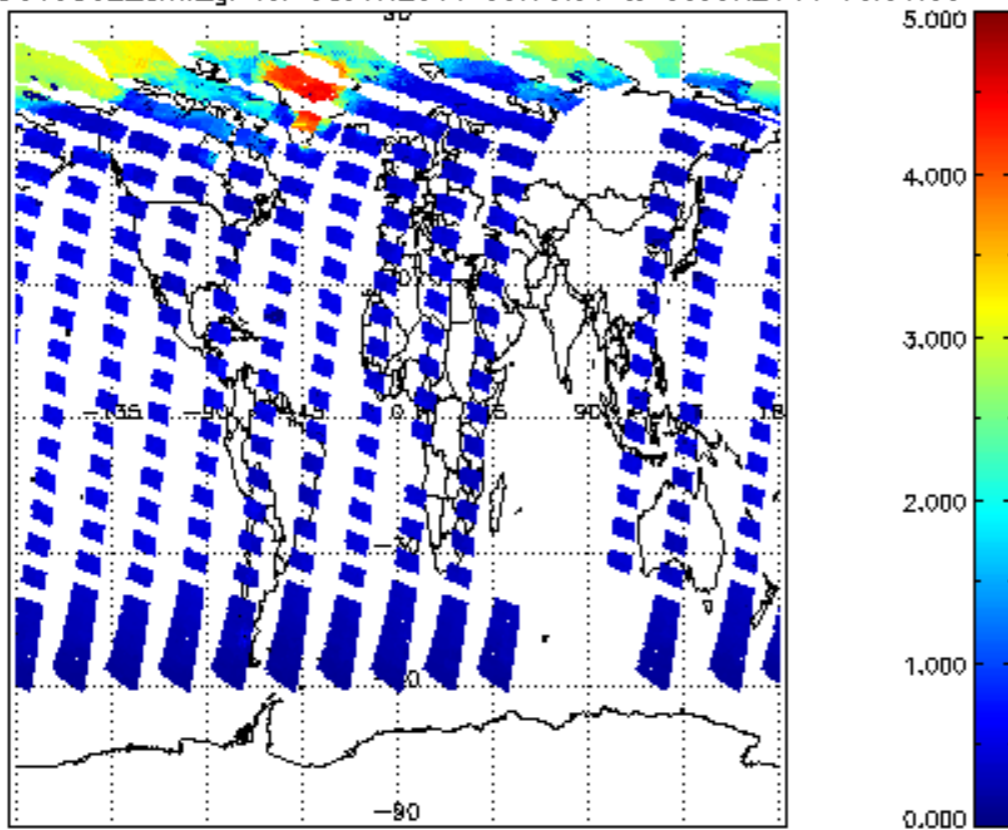
SCIOL2P_NADUV5S02_amf_gr for 08JUN2011 00:00:00 to 09JUN2011 00:00:00
