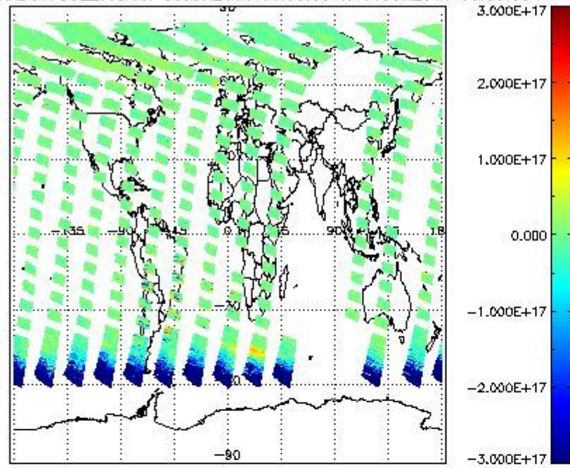
SCIOL2P_NADUV7S02_vcd for 08JUN2011 00:00:00 to 09JUN2011 00:00:00
