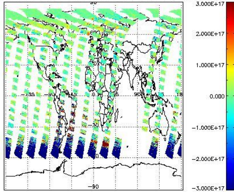
SCIOL2P_NADUV5S02_vcd for 08JUN2011 00:00:00 to 09JUN2011 00:00:00
