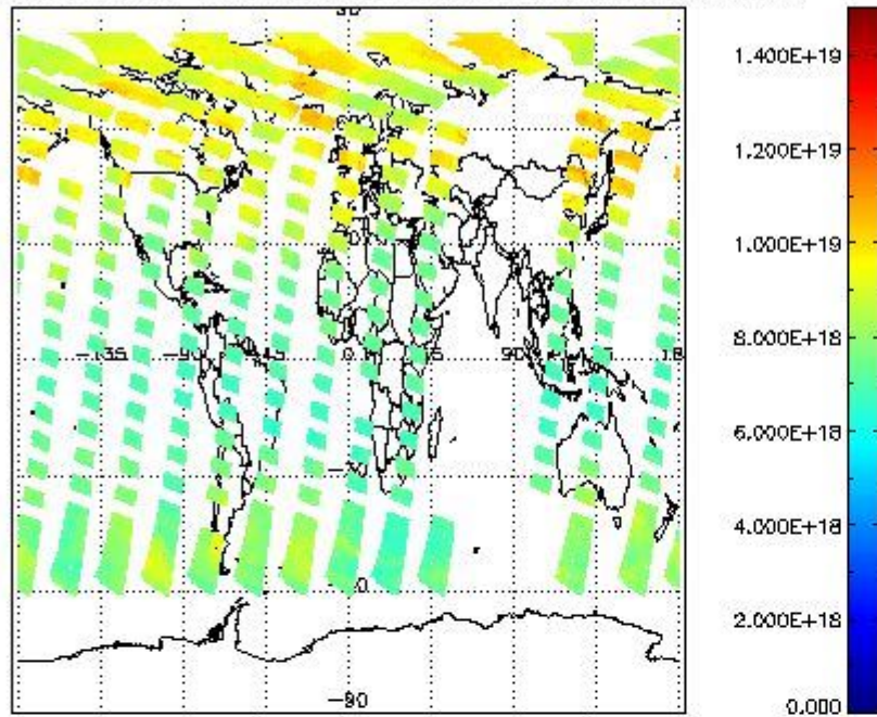
SCIOL2P_NADUV003_vcd for 08JUN2011 00:00:00 to 09JUN2011 00:00:00
