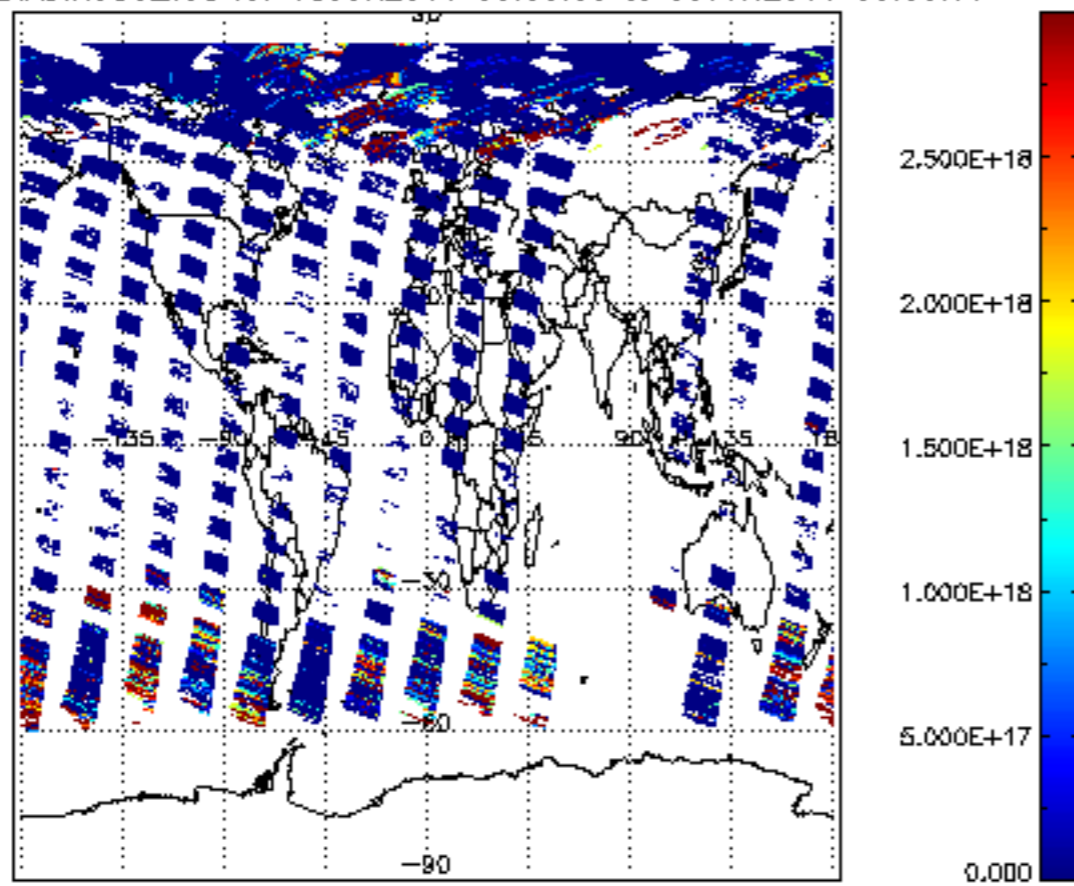
SCIOL2P_NADIR3CO_vcd for 08JUN2011 00:00:00 to 09JUN2011 00:00:00
