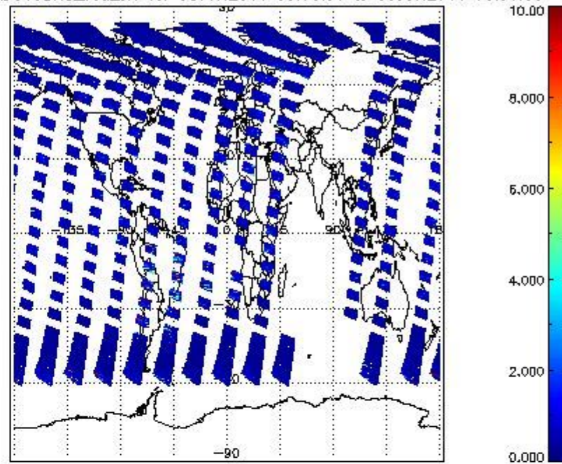
SCIOL2P_NADUV3BRO_vcd_err for 08JUN2011 00:00:00 to 09JUN2011 00:00:00
