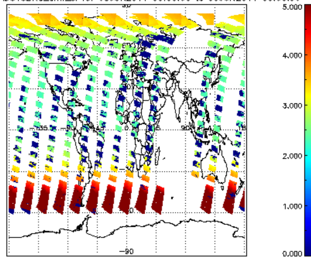
SCIOL2P_NADUV3BRO_amf_cl for 08JUN2011 00:00:00 to 09JUN2011 00:00:00
