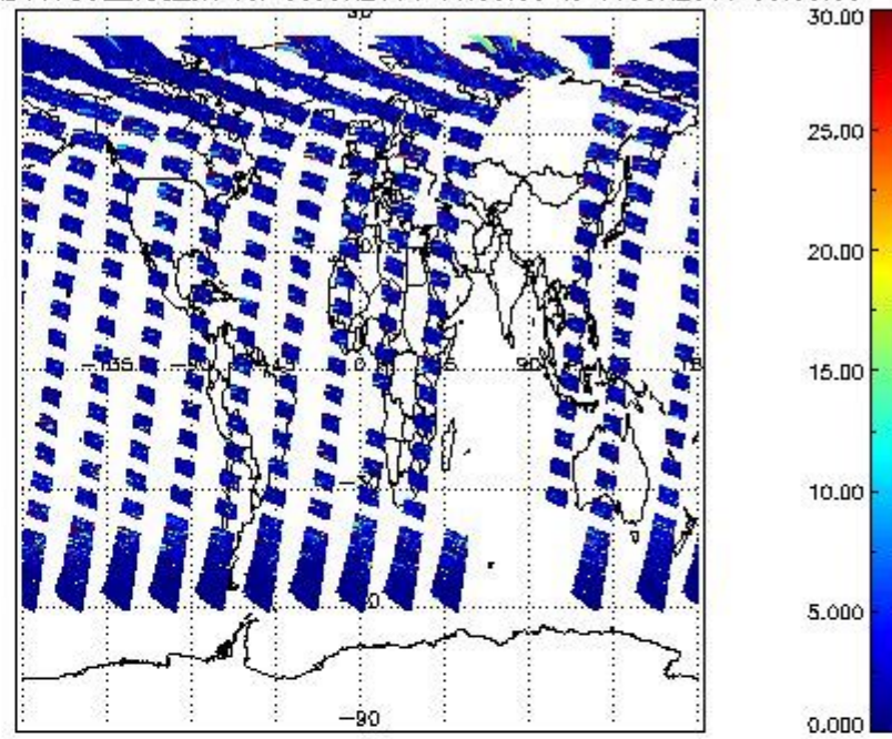
SCIOL2P_NADUV7S02_vcd_err for 08JUN2011 00:00:00 to 09JUN2011 00:00:00
