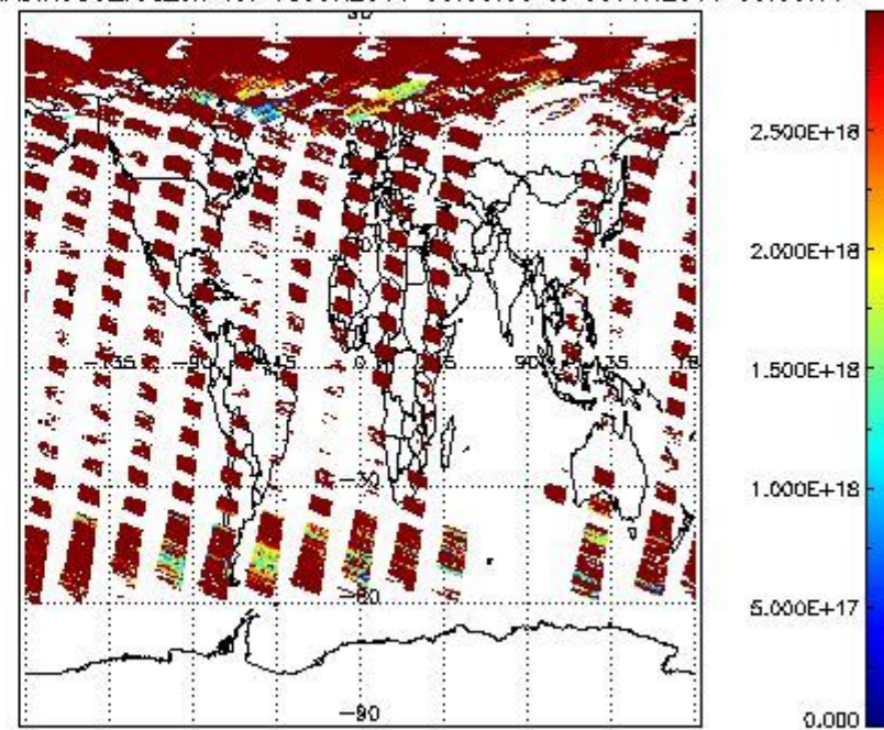
SCIOL2P_NADIR3CO_vcd_err for 08JUN2011 00:00:00 to 09JUN2011 00:00:00
