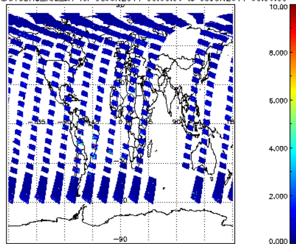
SCIOL2P_NADUV3BRO_vcd_err for 08JUN2011 00:00:00 to 09JUN2011 00:00:00
