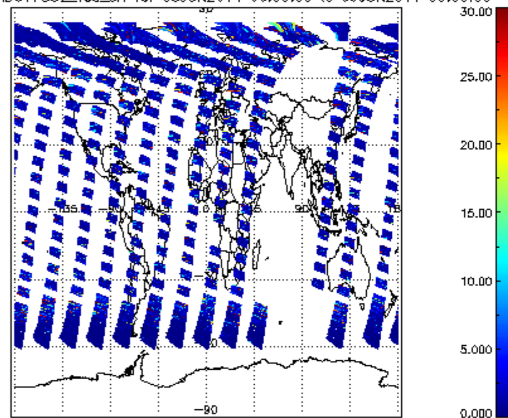
SCIOL2P_NADUV7S02_vcd_err for 08JUN2011 00:00:00 to 09JUN2011 00:00:00
