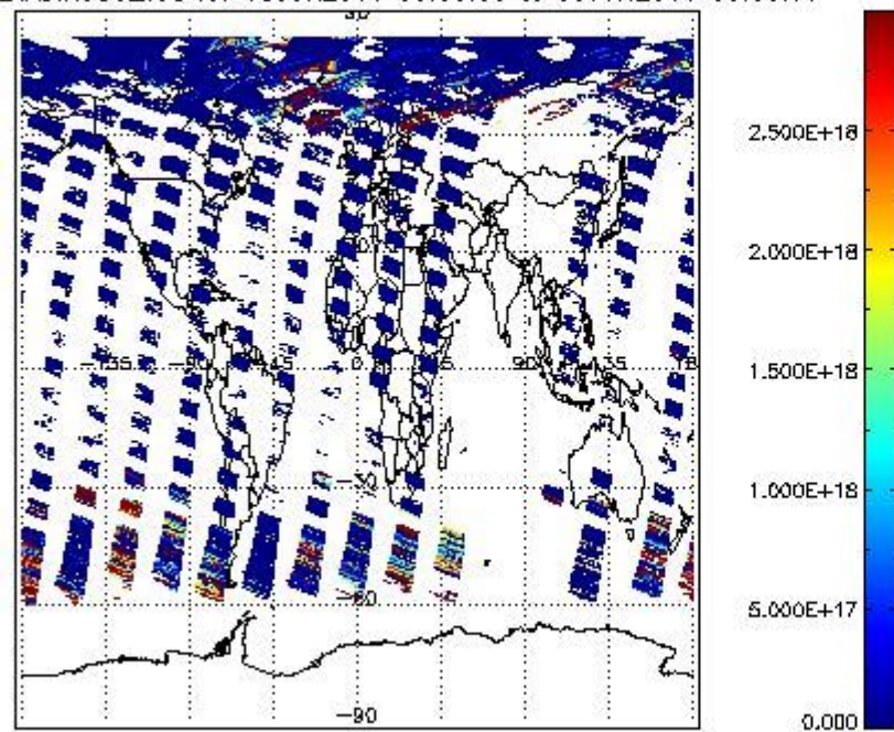
SCIOL2P_NADIR3CO_vcd for 08JUN2011 00:00:00 to 09JUN2011 00:00:00
