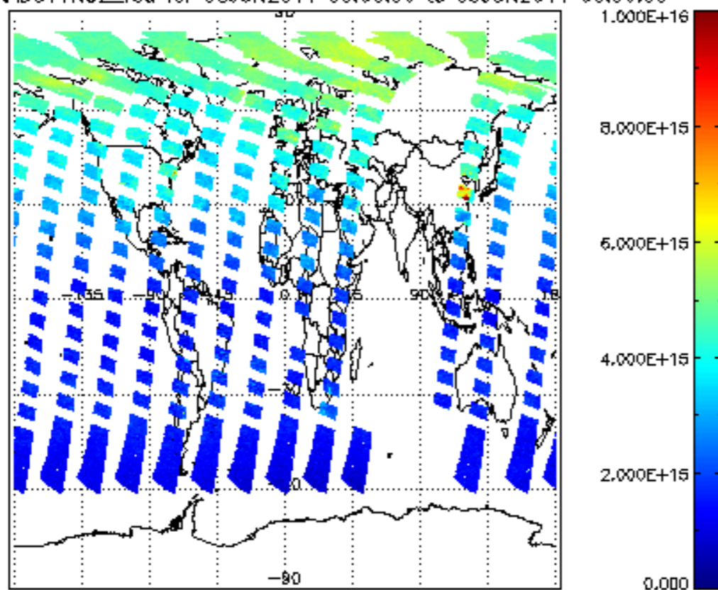
SCIOL2P_NADUV1NO2_vcd for 08JUN2011 00:00:00 to 09JUN2011 00:00:00
