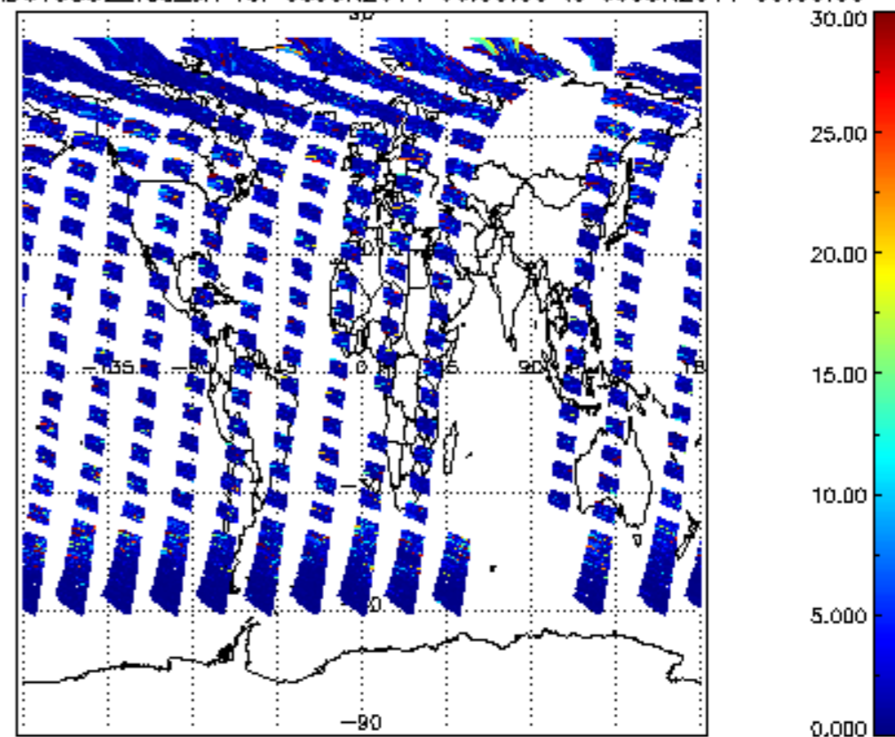
SCIOL2P_NADUV5S02_vcd_err for 08JUN2011 00:00:00 to 09JUN2011 00:00:00
