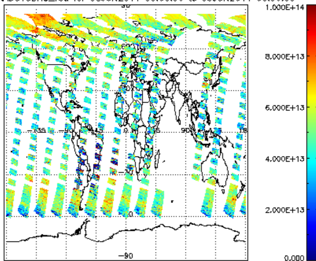
SCIOL2P_NADUV3BRO_vcd for 08JUN2011 00:00:00 to 09JUN2011 00:00:00
