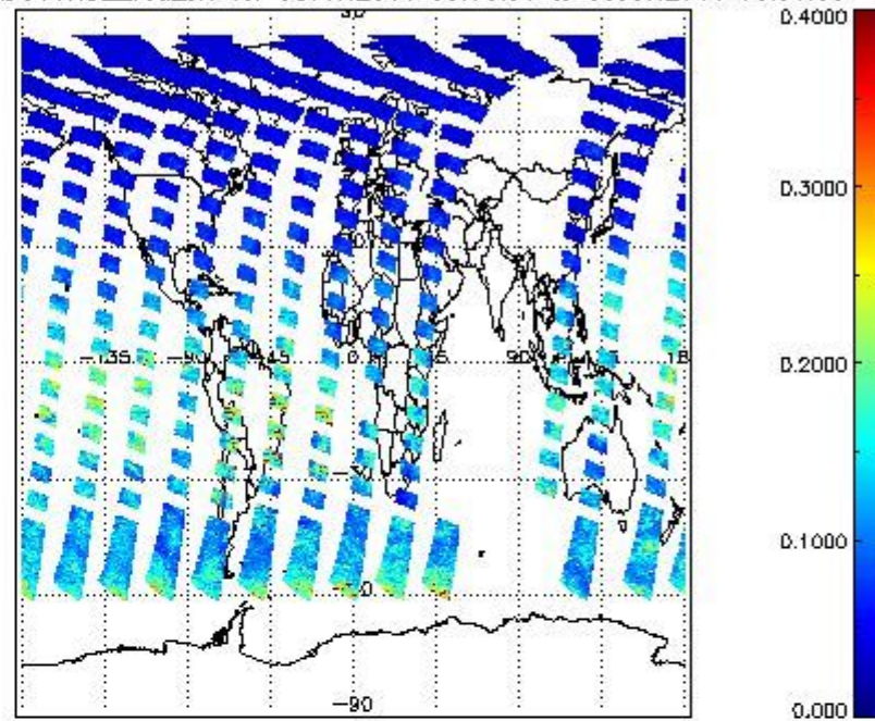
SCIOL2P_NADUV1N02_vcd_err for 08JUN2011 00:00:00 to 09JUN2011 00:00:00
