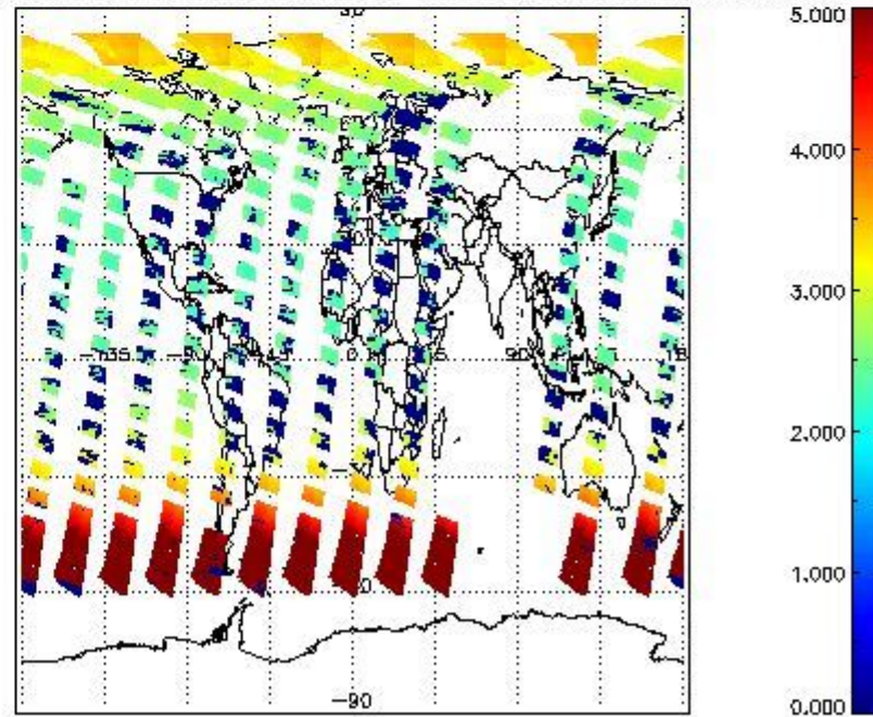
SCIOL2P_NADUV003_amf_cl for 08JUN2011 00:00:00 to 09JUN2011 00:00:00
