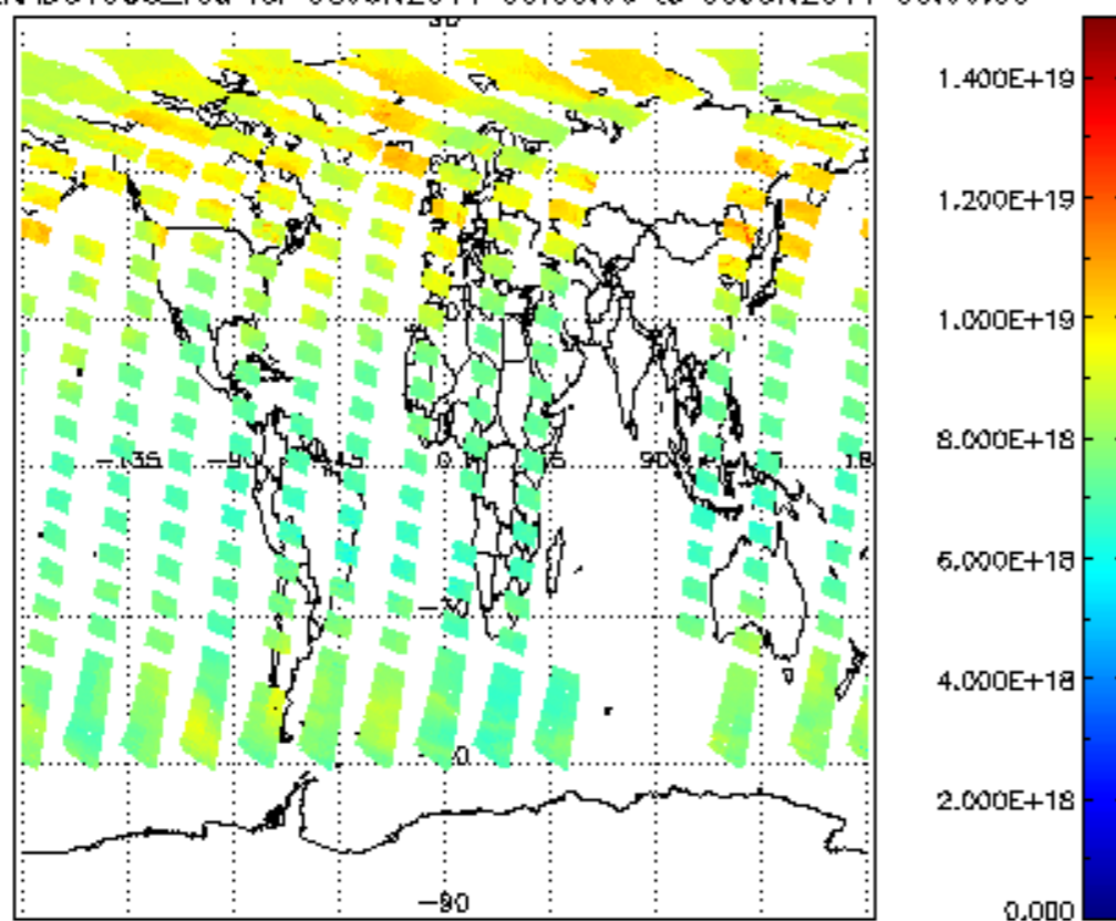
SCIOL2P_NADUV003_vcd for 08JUN2011 00:00:00 to 09JUN2011 00:00:00
