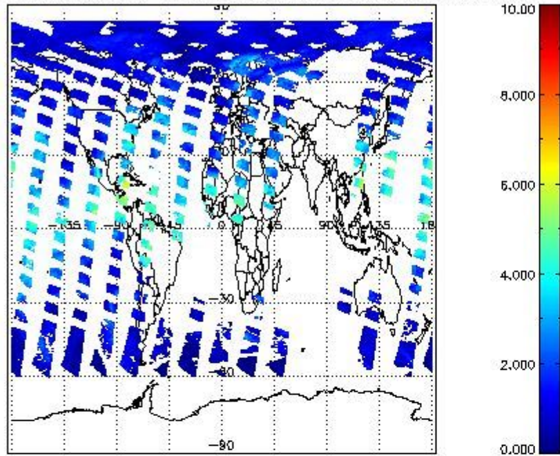
SCIOL2P_NADUV8H2O_vcd for 08JUN2011 00:00:00 to 09JUN2011 00:00:00
