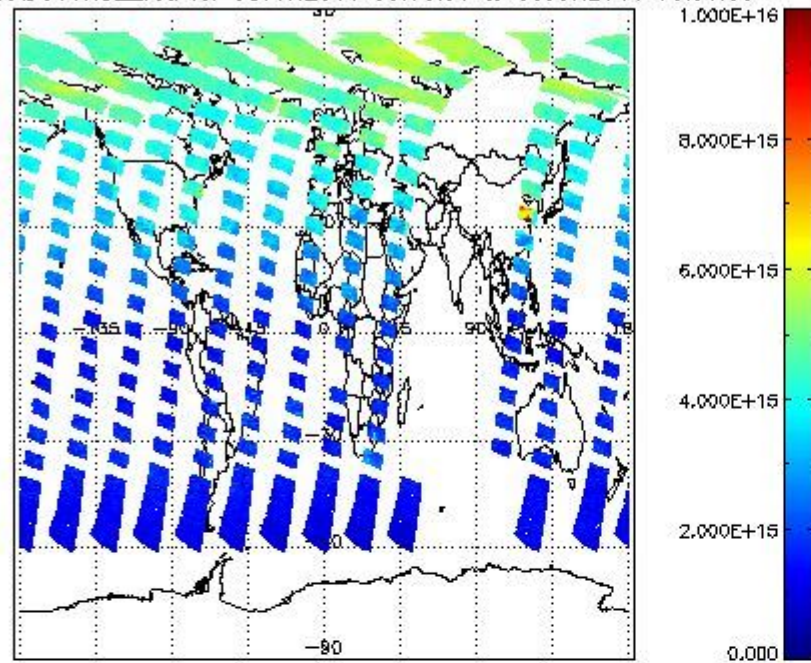
SCIOL2P_NADUV1N02_vcd for 08JUN2011 00:00:00 to 09JUN2011 00:00:00
