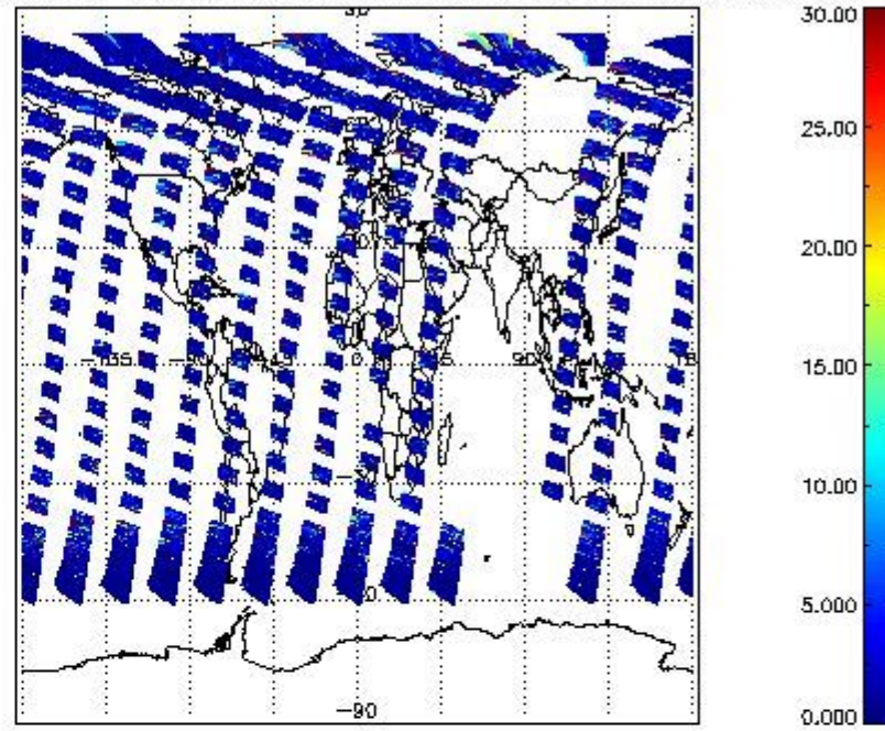
SCIOL2P_NADUV5S02_vcd_err for 08JUN2011 00:00:00 to 09JUN2011 00:00:00
