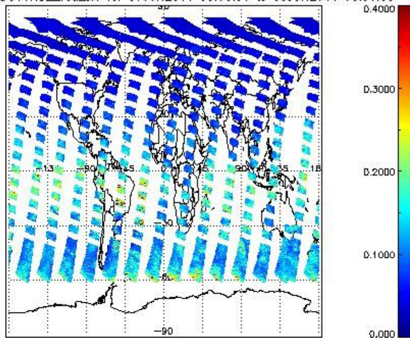
SCIOL2P_NADUV1NO2_vcd_err for 07JUN2011 00:00:00 to 06JUN2011 00:00:00
