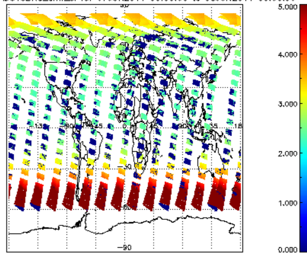
SCIOL2P_NADUV3BRO_amf_sl for 07JUN2011 00:00:00 to 08JUN2011 00:00:00
