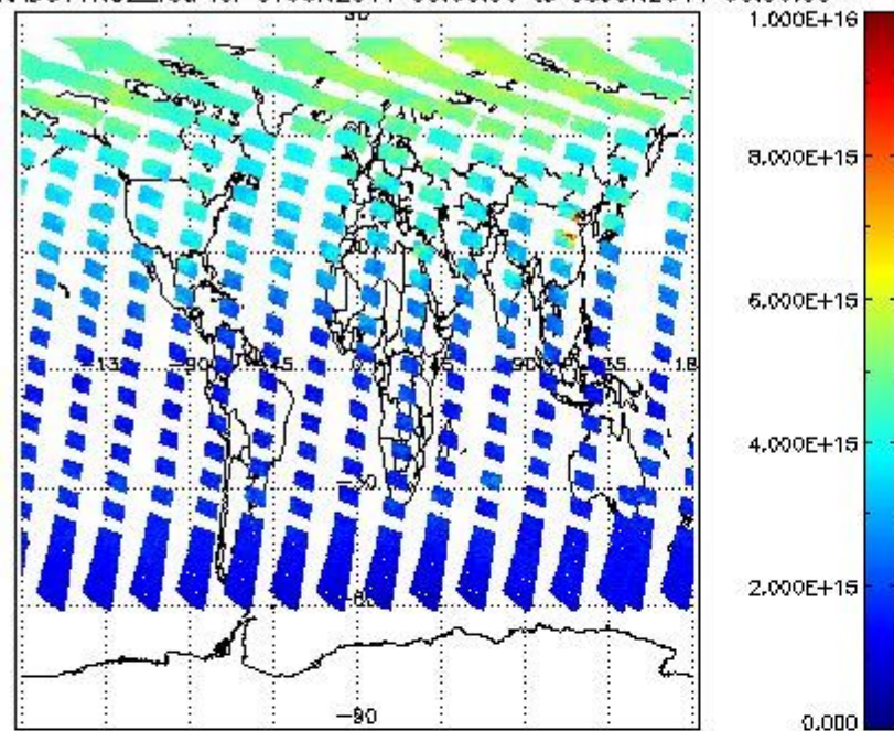
SCIOL2P_NADUV1NO2_vcd for 07JUN2011 00:00:00 to 06JUN2011 00:00:00
