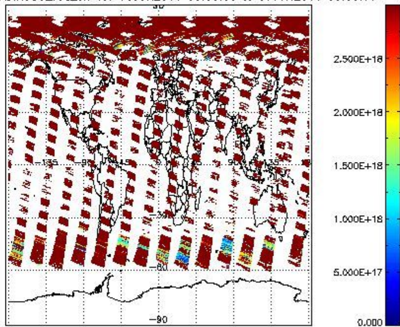
SCIDL2P_NADIR3CO_vcd_err for 06JUN2011 00:00:00 to 07JUN2011 00:00:00
