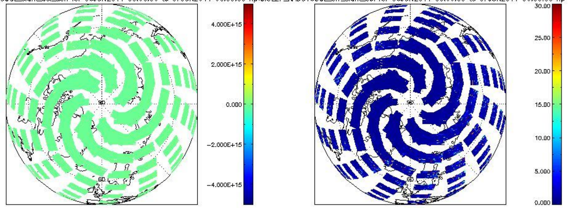
CIOL2P_NADUV60CLslant_col_den for 06JUN2011 00:00:00 to 07JUN2011 00:00:00 np; CIOL2P_NADUV60CLerr_slant_col for 06JUN2011 00:00:00 to 07JUN2011 00:00:00 np
