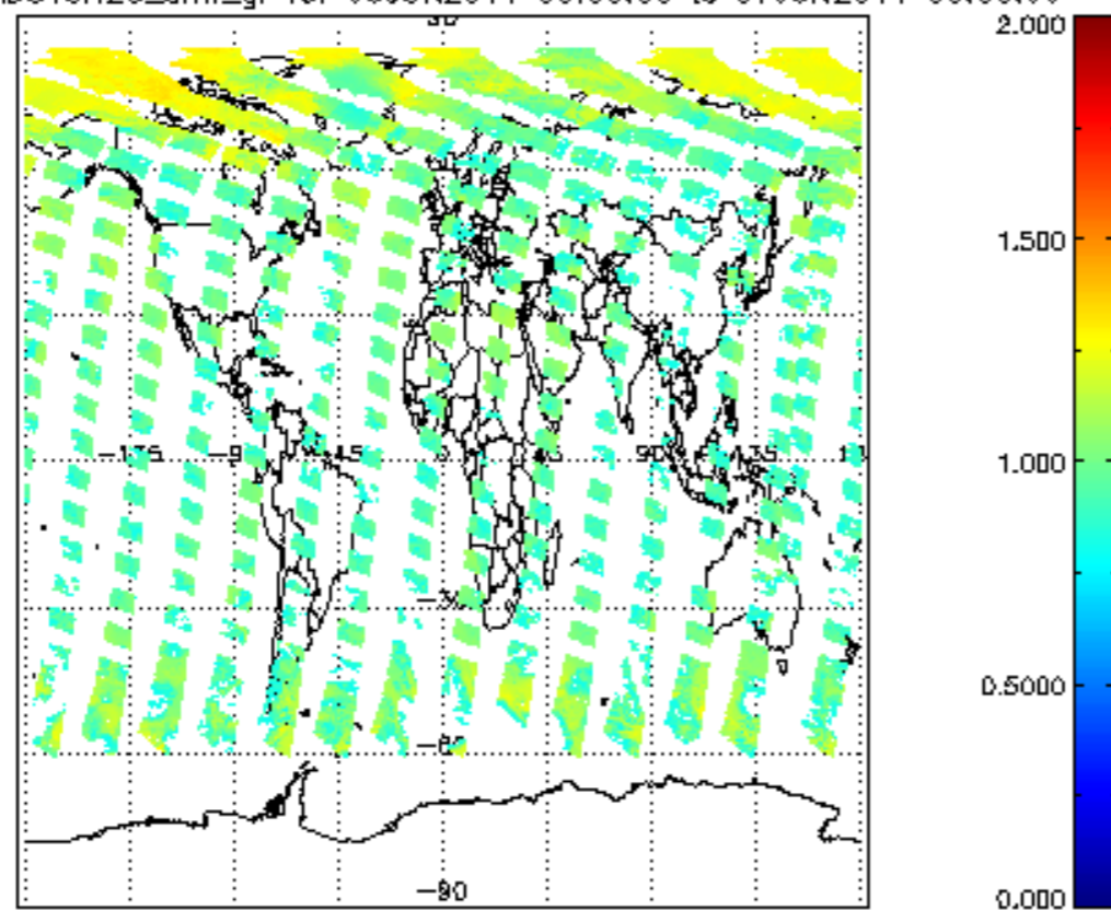
SCIOL2P_NADUV8H2O_amf_gr for 06JUN2011 00:00:00 to 07JUN2011 00:00:00
