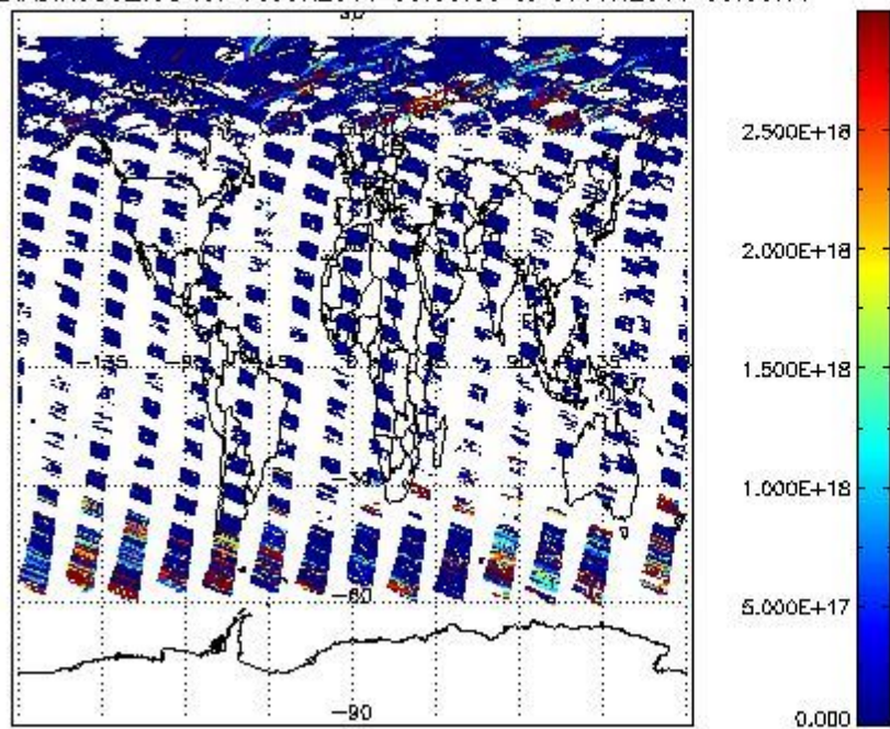
SCIDL2P_NADIR3CO_vcd for 06JUN2011 00:00:00 to 07JUN2011 00:00:00
