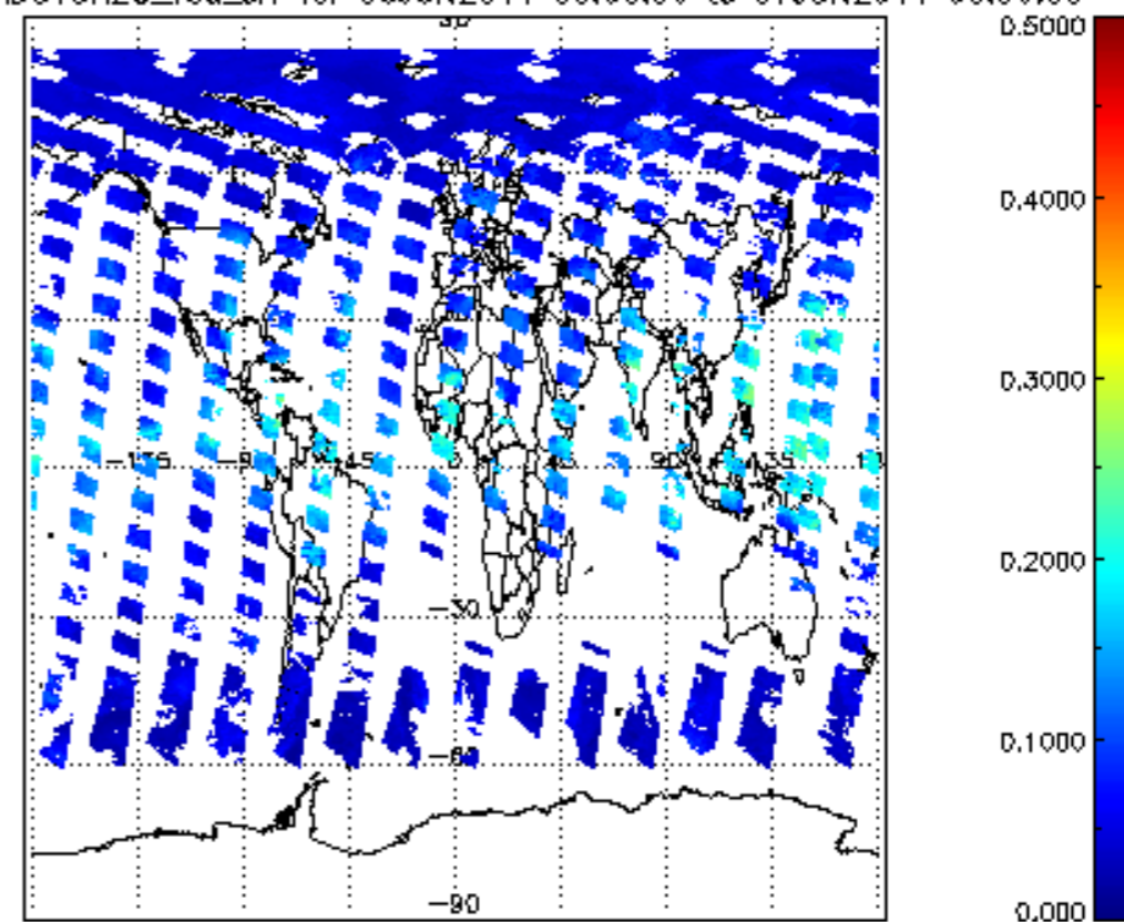
SCIOL2P_NADUV8H2O_vcd_err for 06JUN2011 00:00:00 to 07JUN2011 00:00:00
