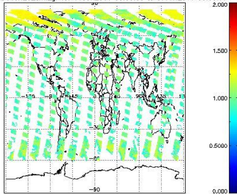
SCIOL2P_NADUV8H2O_arnf_gr for 06JUN2011 00:00:00 to 07JUN2011 00:00:00
