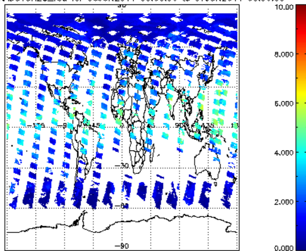
SCIOL2P_NADUV8H2O_vcd for 06JUN2011 00:00:00 to 07JUN2011 00:00:00
