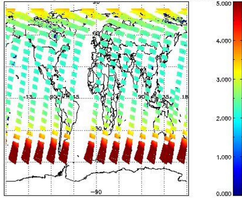
SCIOL2P_NADUV1NO2_amf_gr for 04JUN2011 00:00:00 to 05JUN2011 00:00:00
