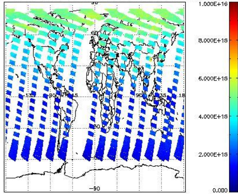
SCIOL2P_NADUV1NO2_vcd for 04JUN2011 00:00:00 to 05JUN2011 00:00:00
