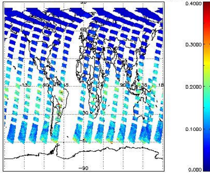
SCIOL2P_NADUV1NO2_vcd_err for 04JUN2011 00:00:00 to 05JUN2011 00:00:00
