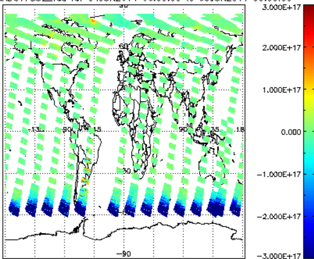
SCIOL2P_NADUV7S02_vcd for 04JUN2011 00:00:00 to 05JUN2011 00:00:00
