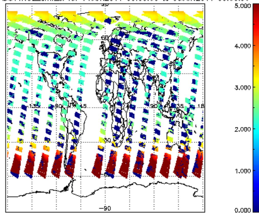
SCIOL2P_NADUV1NO2_amf_sl for 04JUN2011 00:00:00 to 05JUN2011 00:00:00
