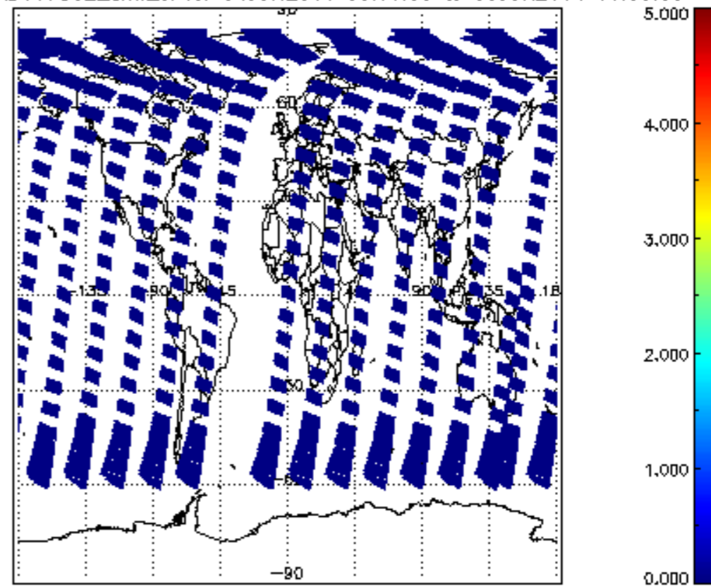
SCIOL2P_NADUV7S02_amf_cl for 04JUN2011 00:00:00 to 05JUN2011 00:00:00
