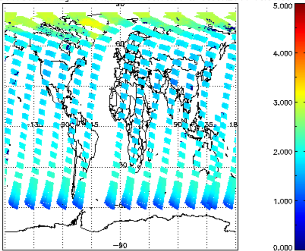
SCIOL2P_NADUV7S02_amf_gr for 04JUN2011 00:00:00 to 05JUN2011 00:00:00
