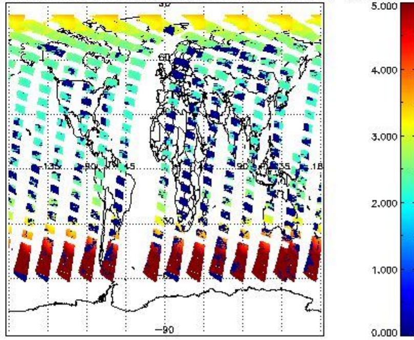
SCIOL2P_NADUV1NO2_amf_cl for 04JUN2011 00:00:00 to 05JUN2011 00:00:00
