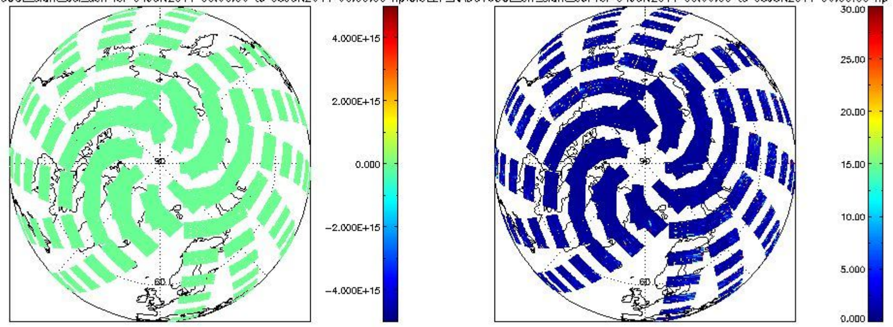
CIOL2P_NADUV60CLslant_col_den for 04JUN2011 00:00:00 to 05JUN2011 00:00:00 np; CIOL2P_NADUV60CLerr_slant_col for 04JUN2011 00:00:00 to 05JUN2011 00:00:00 np
