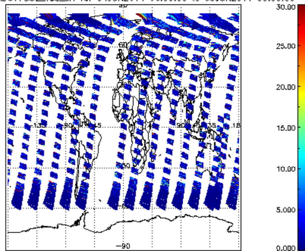
SCIOL2P_NADUV7S02_vcd_err for 04JUN2011 00:00:00 to 05JUN2011 00:00:00
