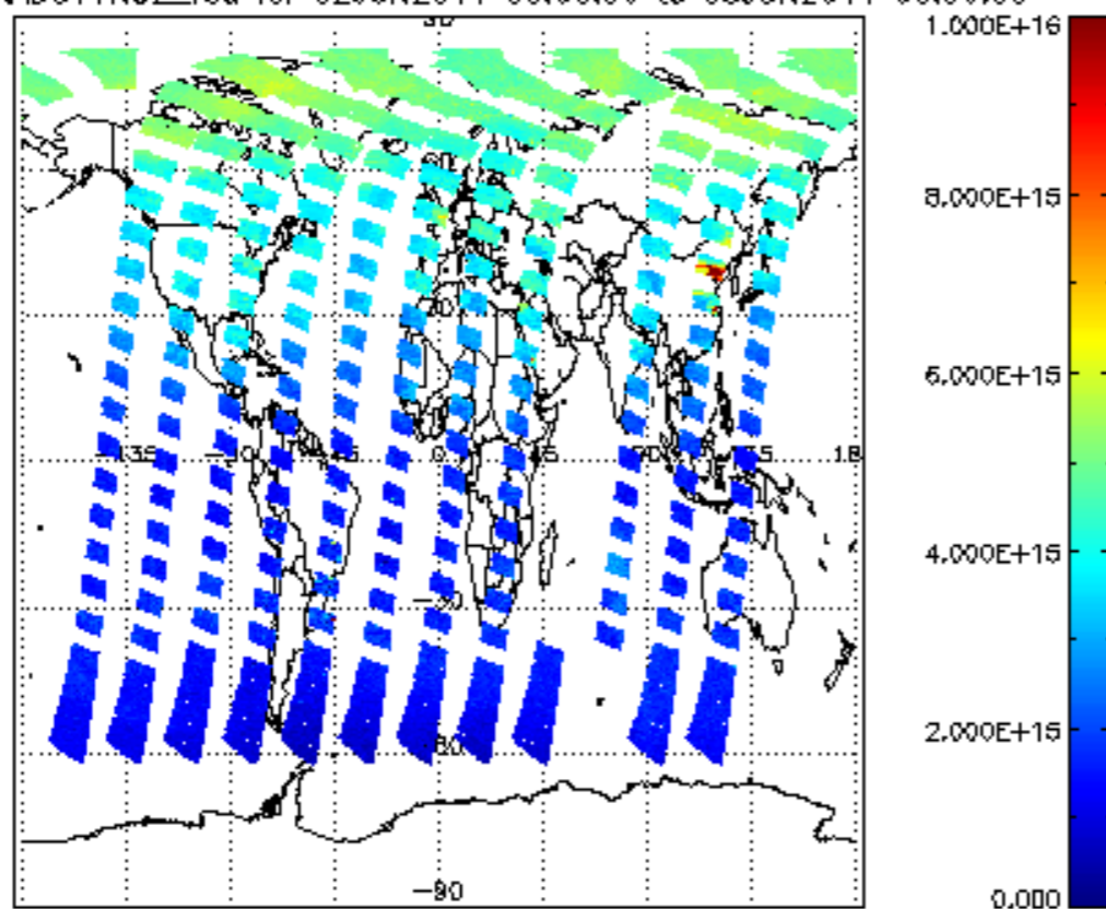
SCIOL2P_NADUV1NO2_vcd for 02JUN2011 00:00:00 to 03JUN2011 00:00:00
