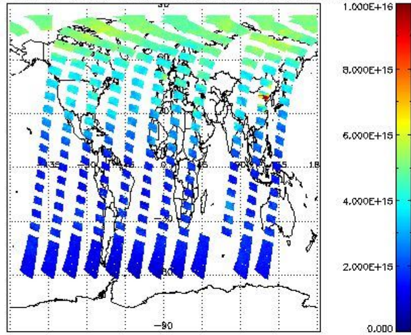
SCIOL2P_NADUV1NO2_vcd for 02JUN2011 00:00:00 to 03JUN2011 00:00:00
