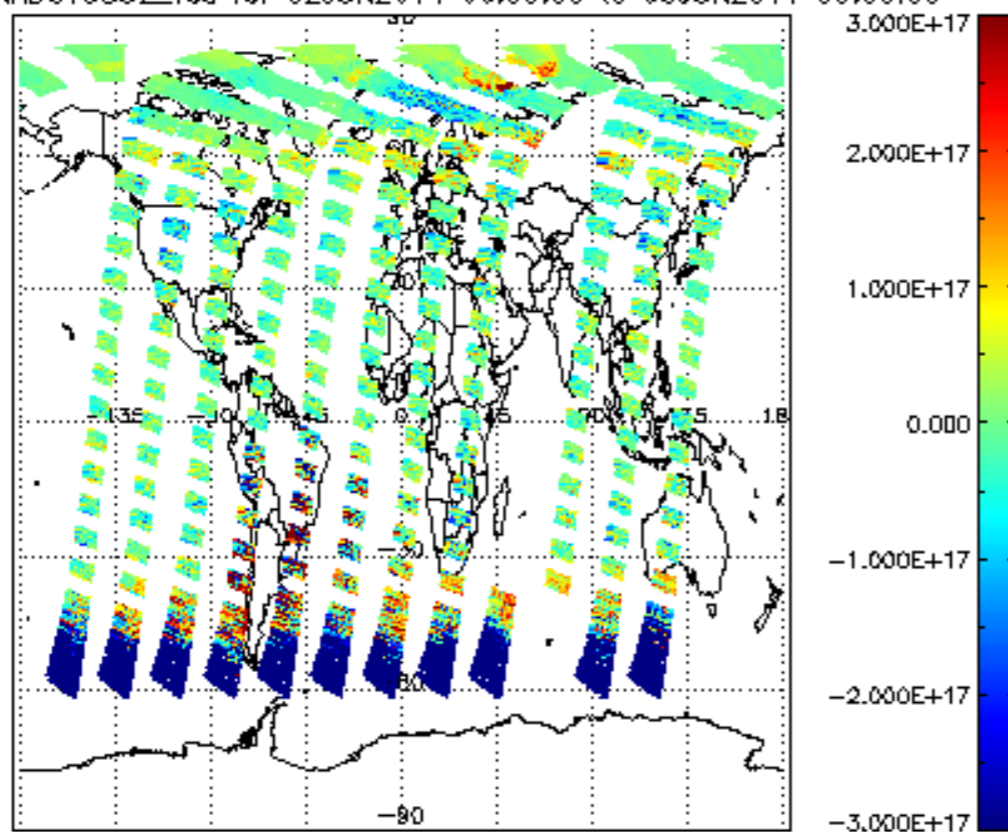
SCIOL2P_NADUV5S02_vcd for 02JUN2011 00:00:00 to 03JUN2011 00:00:00
