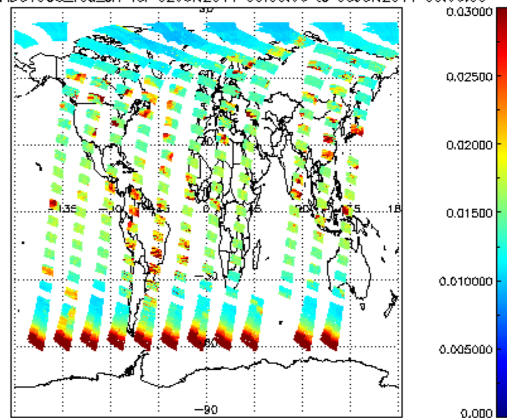
SCIOL2P_NADUV003_vcd_err for 02JUN2011 00:00:00 to 03JUN2011 00:00:00
