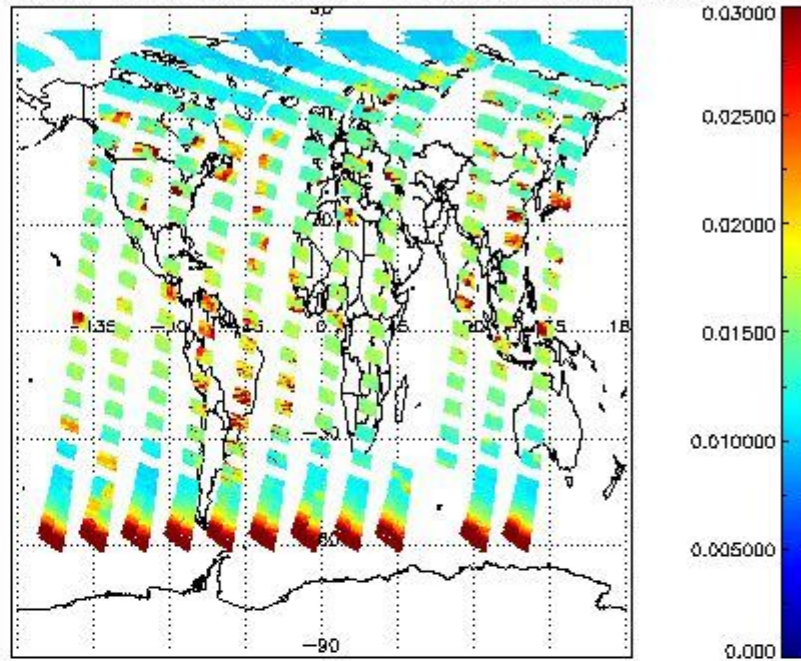
SCIOL2P_NADUV003_vcd_err for 02JUN2011 00:00:00 to 03JUN2011 00:00:00
