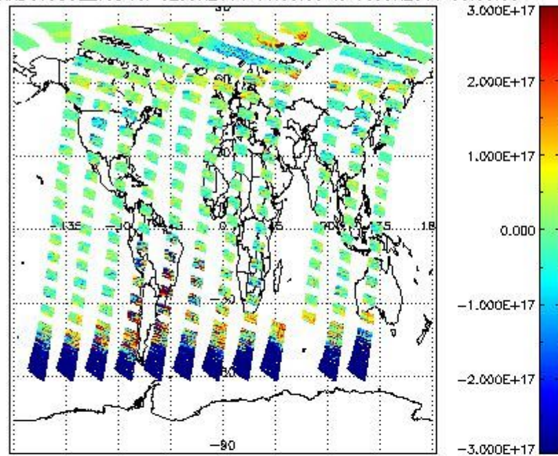
SCIOL2P_NADUV5S02_vcd for 02JUN2011 00:00:00 to 03JUN2011 00:00:00
