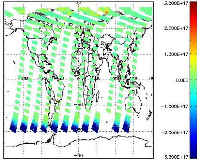
SCIOL2P_NADUV7S02_vcd for 02JUN2011 00:00:00 to 03JUN2011 00:00:00
