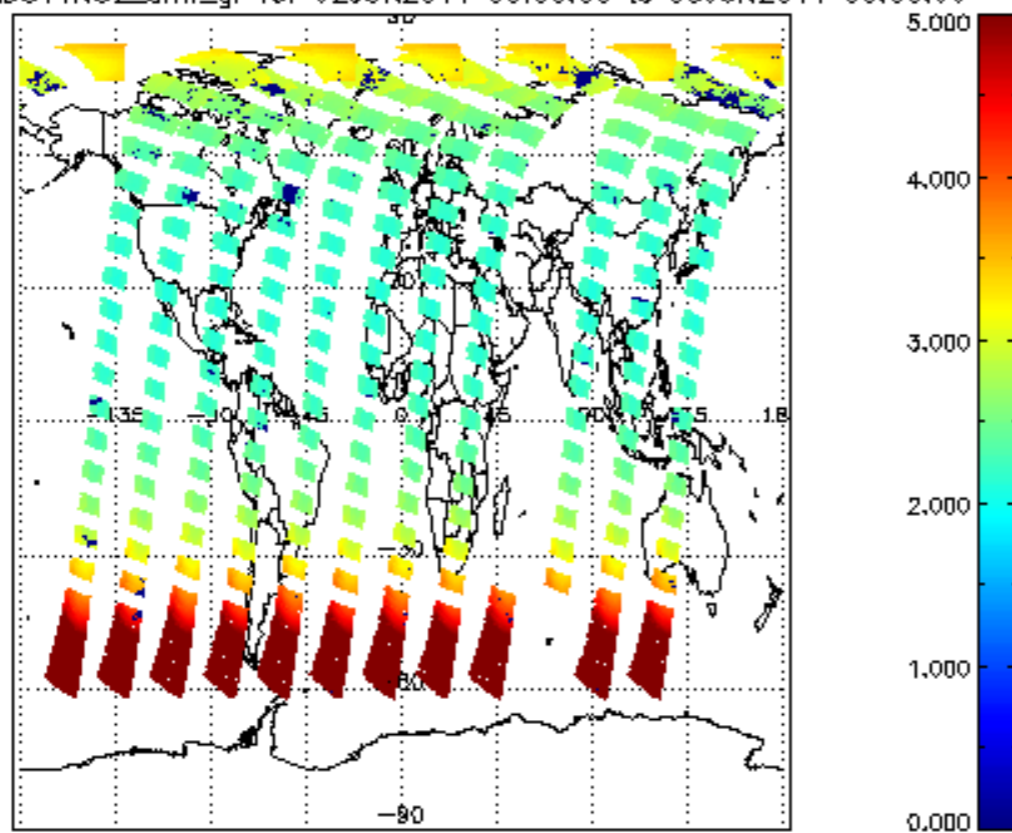
SCIOL2P_NADUV1NO2_amf_gr for 02JUN2011 00:00:00 to 03JUN2011 00:00:00
