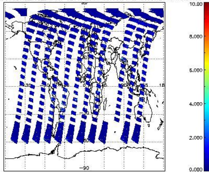
SCIOL2P_NADUV3BRO_vcd_err for 02JUN2011 00:00:00 to 03JUN2011 00:00:00
