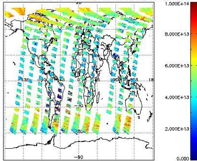
SCIOL2P_NADUV3BRO_vcd for 02JUN2011 00:00:00 to 03JUN2011 00:00:00
