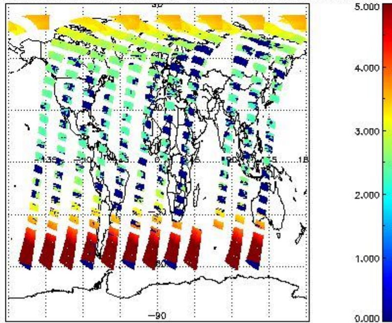
SCIOL2P_NADUV003_amf_cl for 02JUN2011 00:00:00 to 03JUN2011 00:00:00
