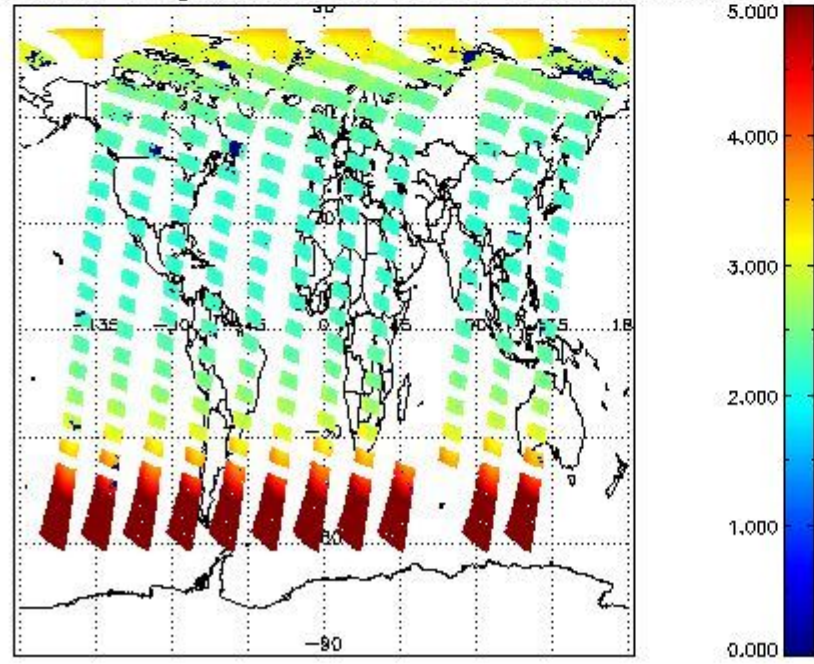
SCIOL2P_NADUV1NO2_amf_gr for 02JUN2011 00:00:00 to 03JUN2011 00:00:00
