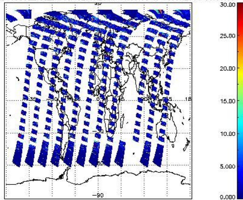
SCIOL2P_NADUV5S02_vcd_err for 02JUN2011 00:00:00 to 03JUN2011 00:00:00
