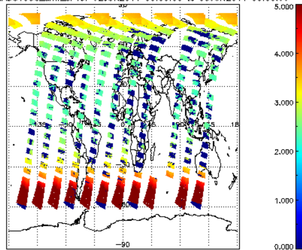
SCIOL2P_NADUV003_amf_cl for 02JUN2011 00:00:00 to 03JUN2011 00:00:00
