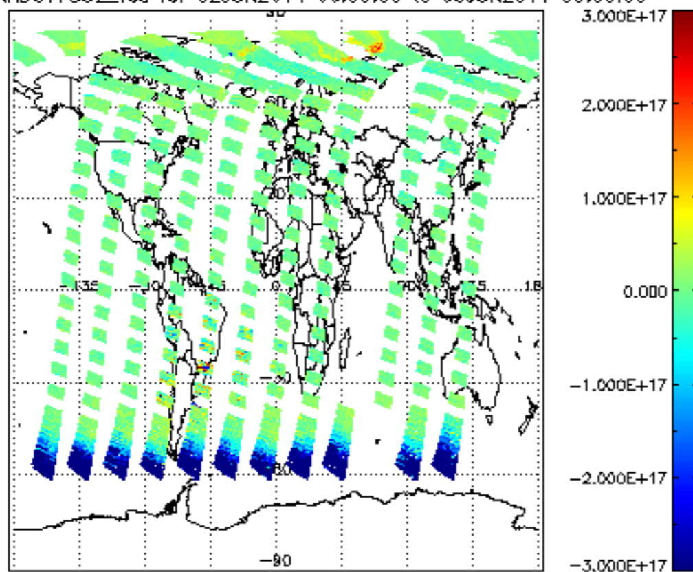
SCIOL2P_NADUV7S02_vcd for 02JUN2011 00:00:00 to 03JUN2011 00:00:00
