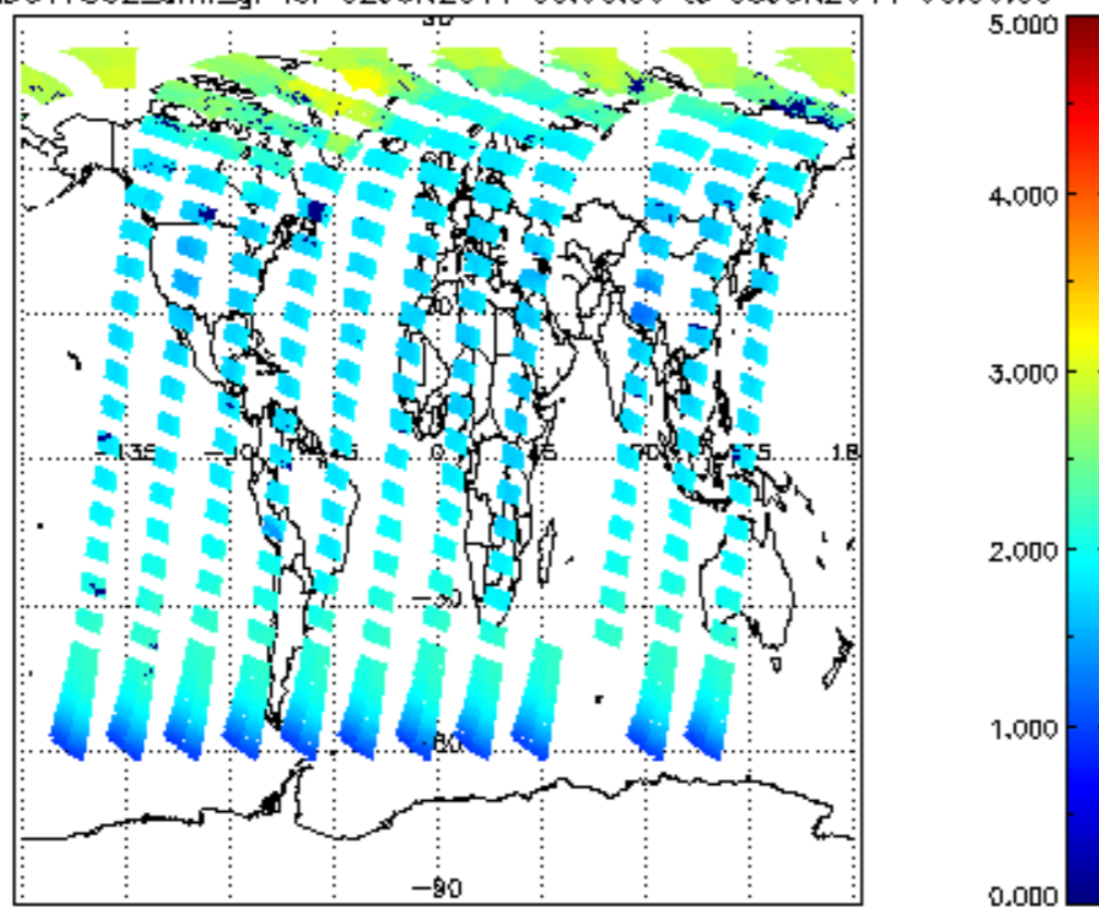
SCIOL2P_NADUV7S02_amf_gr for 02JUN2011 00:00:00 to 03JUN2011 00:00:00
