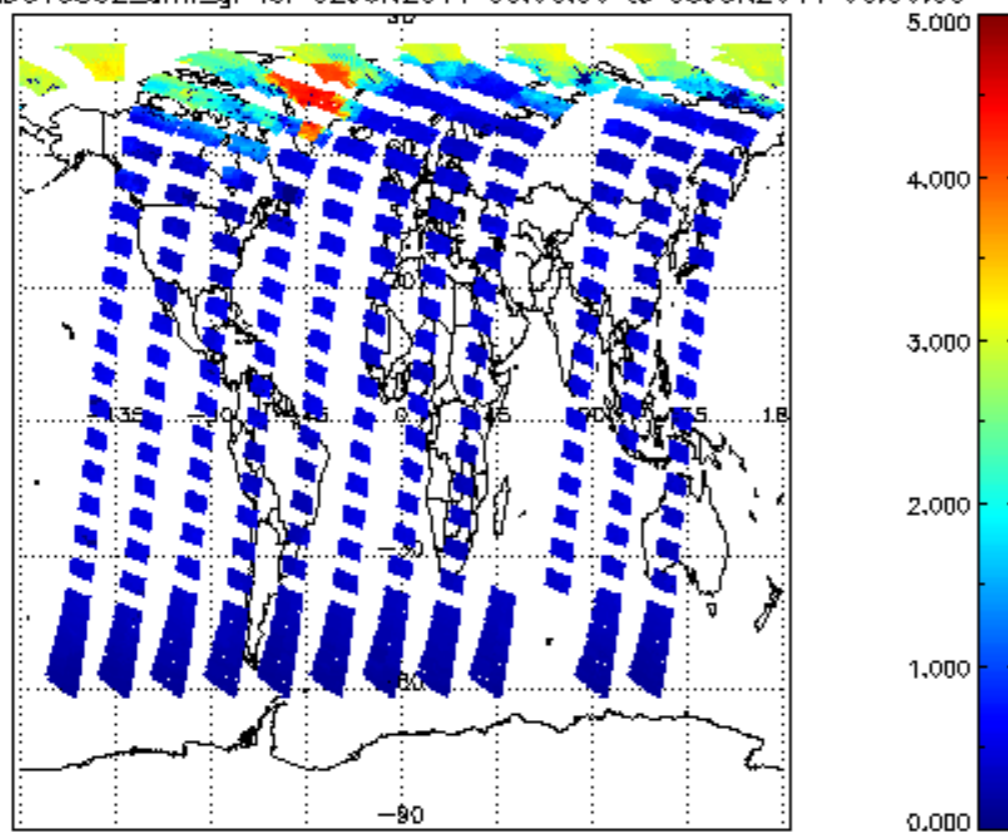
SCIOL2P_NADUV5S02_amf_gr for 02JUN2011 00:00:00 to 03JUN2011 00:00:00
