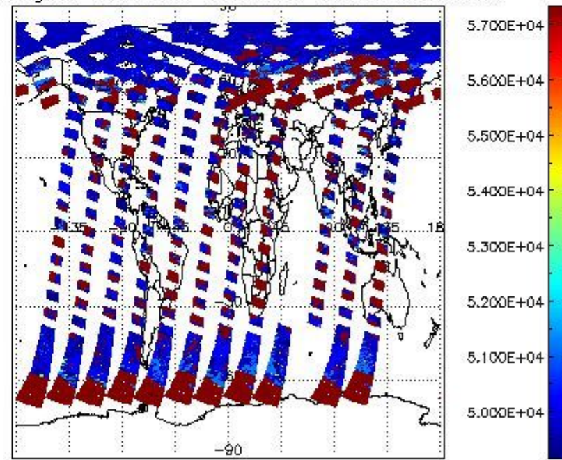
cloud_flags for 02JUN2011 00:00:00 to 03JUN2011 00:00:00
