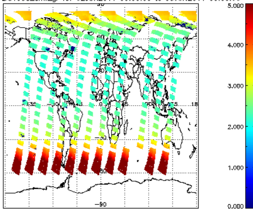
SCIOL2P_NADUV003_amf_gr for 02JUN2011 00:00:00 to 03JUN2011 00:00:00
