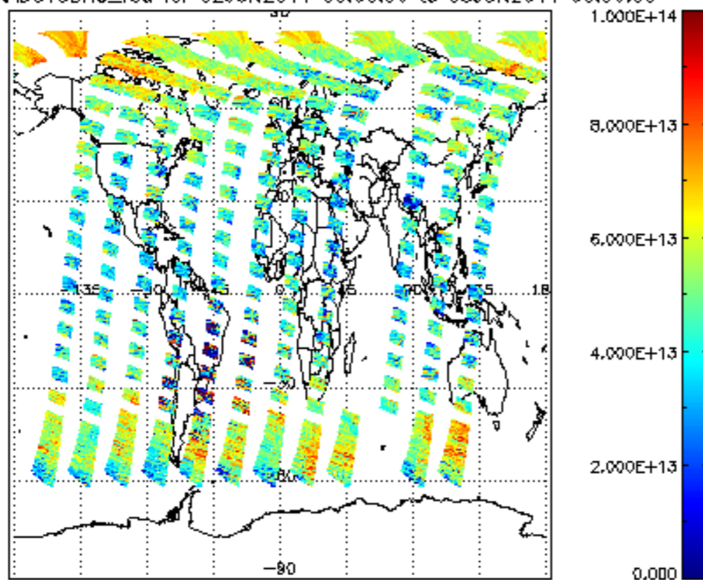
SCIOL2P_NADUV3BRO_vcd for 02JUN2011 00:00:00 to 03JUN2011 00:00:00
