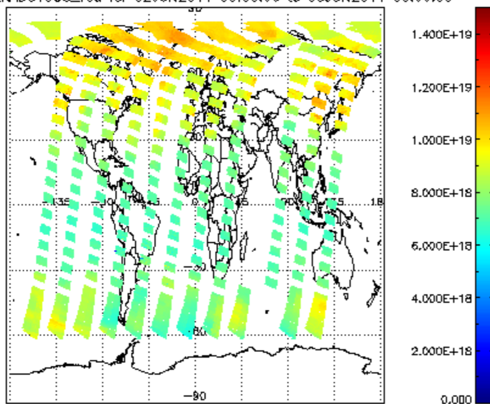
SCIOL2P_NADUV003_vcd for 02JUN2011 00:00:00 to 03JUN2011 00:00:00
