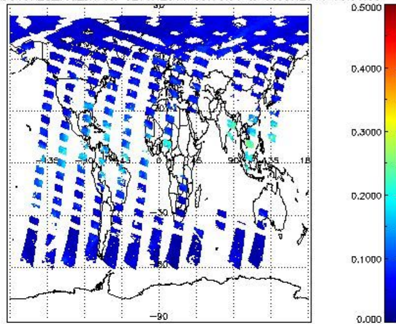
SCIOL2P_NADUV8H2O_vcd_err for 02JUN2011 00:00:00 to 03JUN2011 00:00:00
