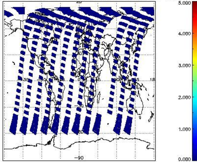
SCIOL2P_NADUV7S02_amf_cl for 02JUN2011 00:00:00 to 03JUN2011 00:00:00
