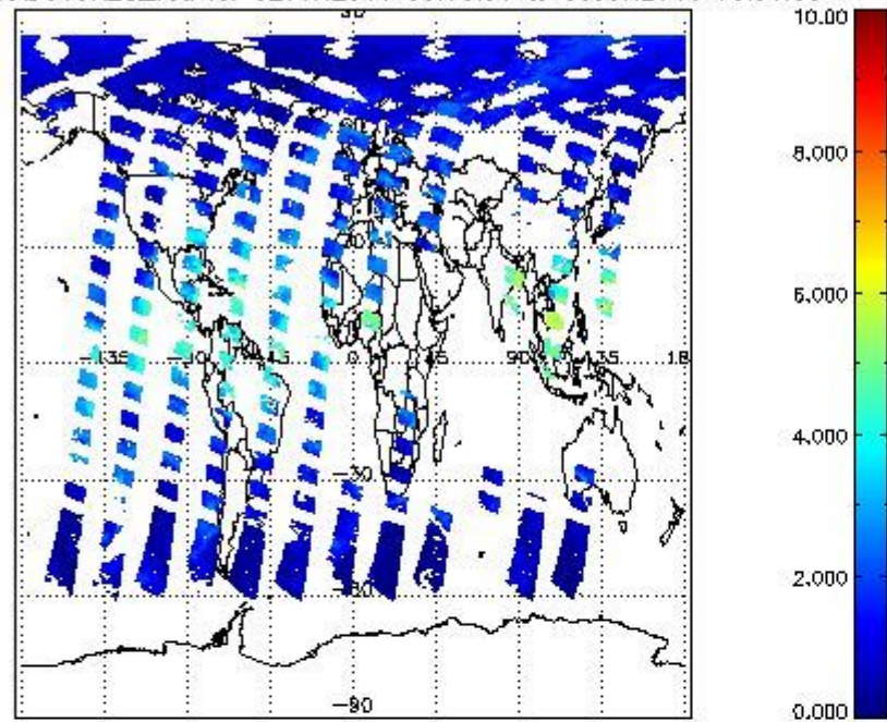
SCIOL2P_NADUV8H2O_vcd for 02JUN2011 00:00:00 to 03JUN2011 00:00:00
