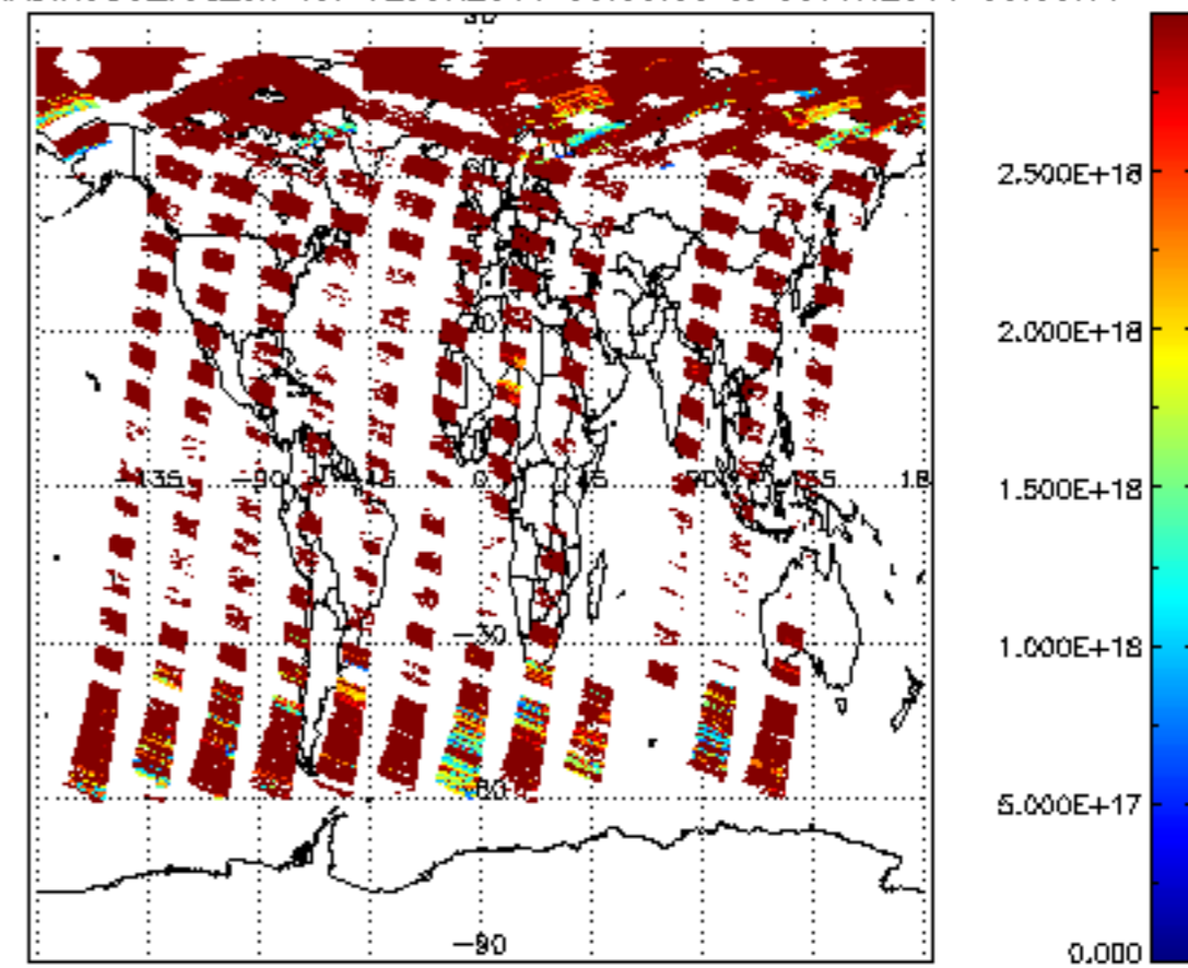
SCIOL2P_NADIR3CO_vcd_err for 02JUN2011 00:00:00 to 03JUN2011 00:00:00
