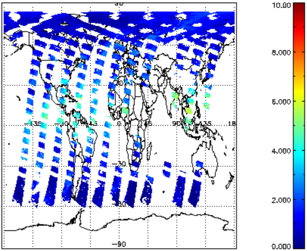
SCIOL2P_NADUV8H2O_vcd for 02JUN2011 00:00:00 to 03JUN2011 00:00:00
