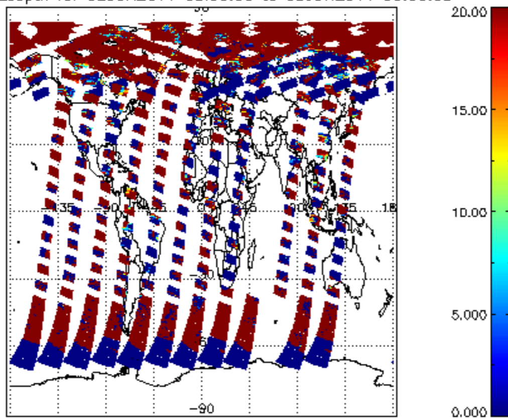
cl_opt_depth for 02JUN2011 00:00:00 to 03JUN2011 00:00:00
