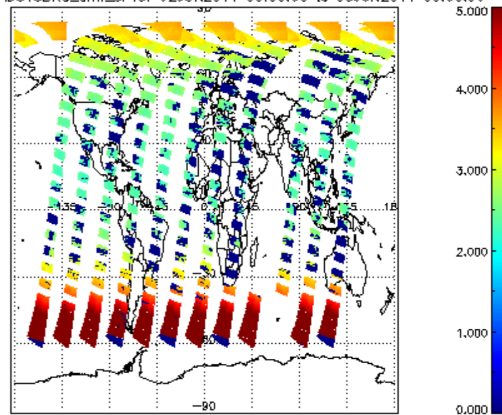
SCIOL2P_NADUV3BRO_amf_cl for 02JUN2011 00:00:00 to 03JUN2011 00:00:00
