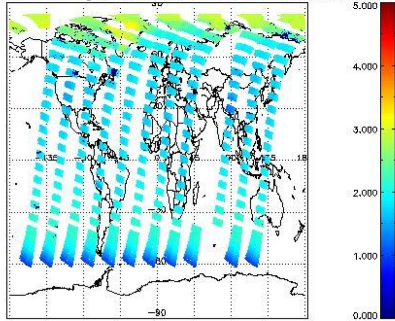
SCIOL2P_NADUV7S02_amf_gr for 02JUN2011 00:00:00 to 03JUN2011 00:00:00
