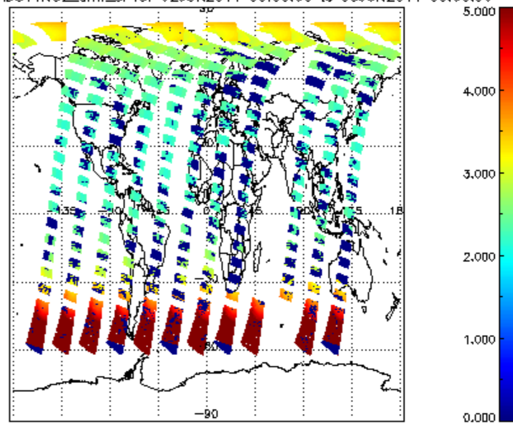
SCIOL2P_NADUV1NO2_amf_sl for 02JUN2011 00:00:00 to 03JUN2011 00:00:00
