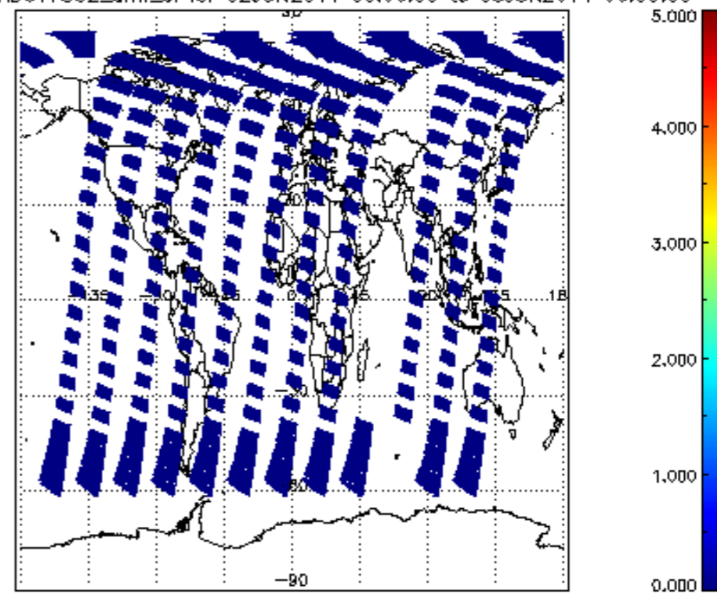
SCIOL2P_NADUV7S02_amf_cl for 02JUN2011 00:00:00 to 03JUN2011 00:00:00
