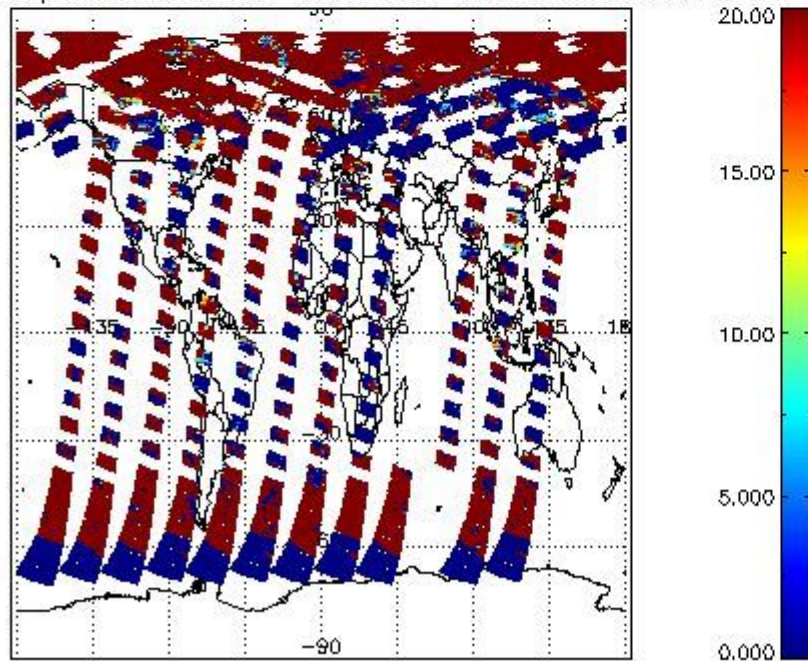
cL_opt_depth for 02JUN2011 00:00:00 to 03JUN2011 00:00:00
