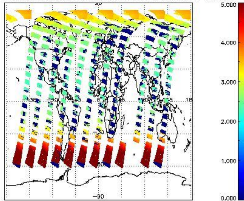
SCIOL2P_NADUV3BRO_amf_cl for 02JUN2011 00:00:00 to 03JUN2011 00:00:00
