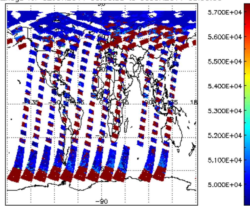
cloud_flags for 02JUN2011 00:00:00 to 03JUN2011 00:00:00
