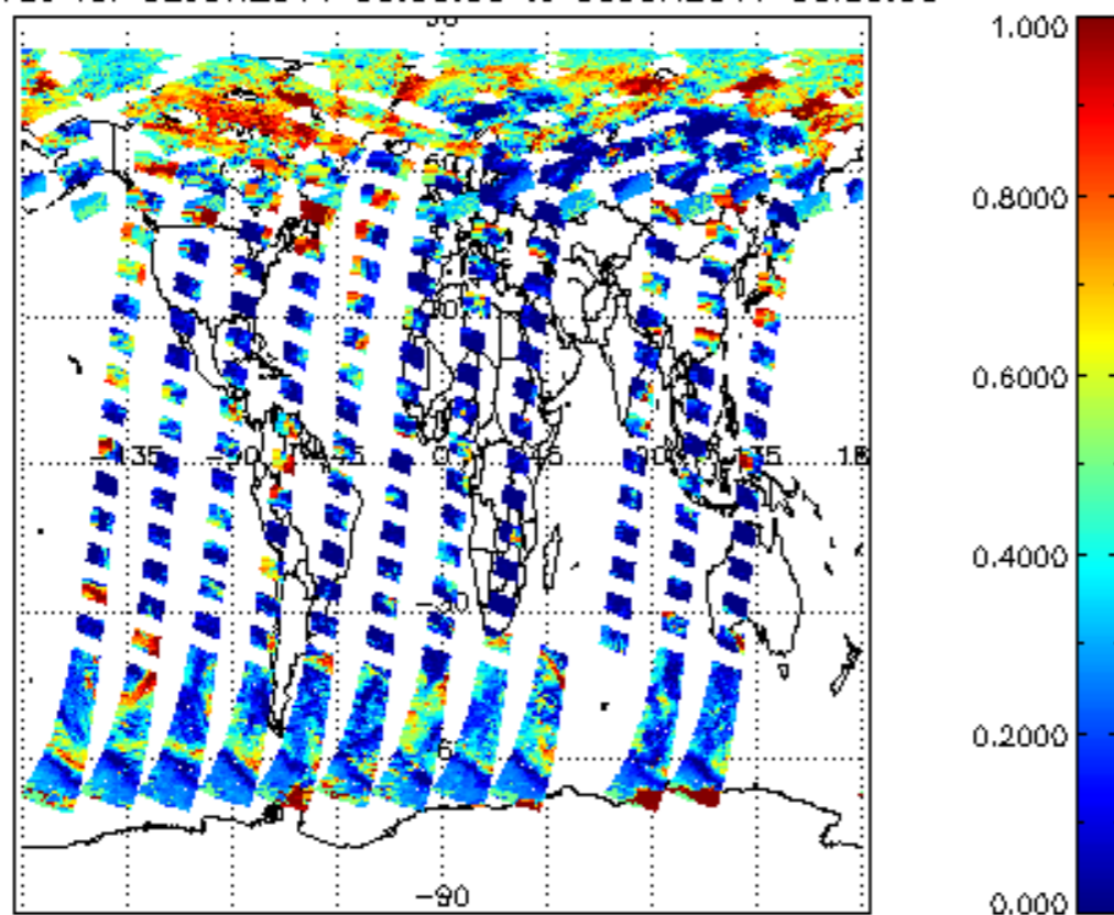
cl_frac for 02JUN2011 00:00:00 to 03JUN2011 00:00:00
