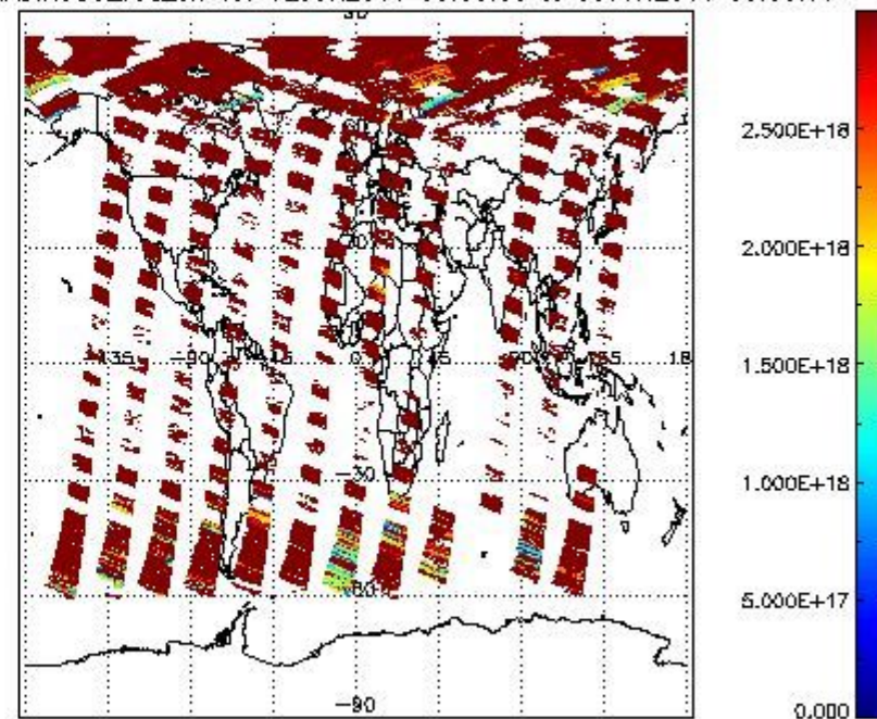
SCIDL2P_NADIR3CO_vcd_err for 02JUN2011 00:00:00 to 03JUN2011 00:00:00
