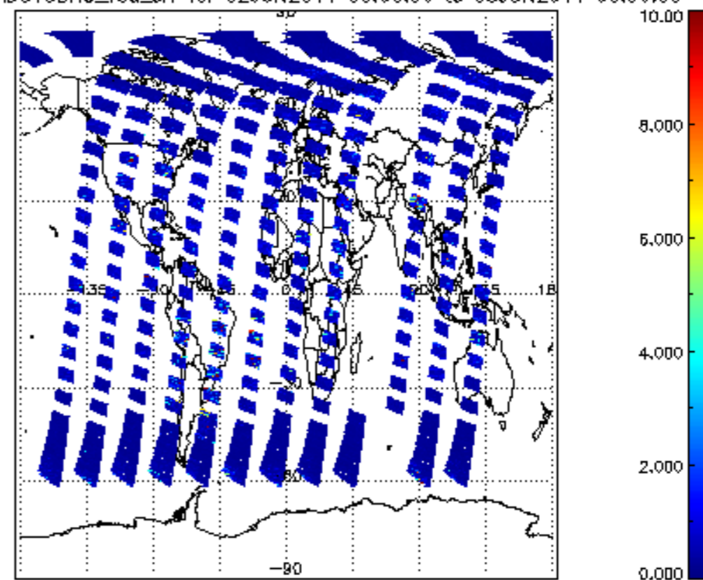
SCIOL2P_NADUV3BRO_vcd_err for 02JUN2011 00:00:00 to 03JUN2011 00:00:00
