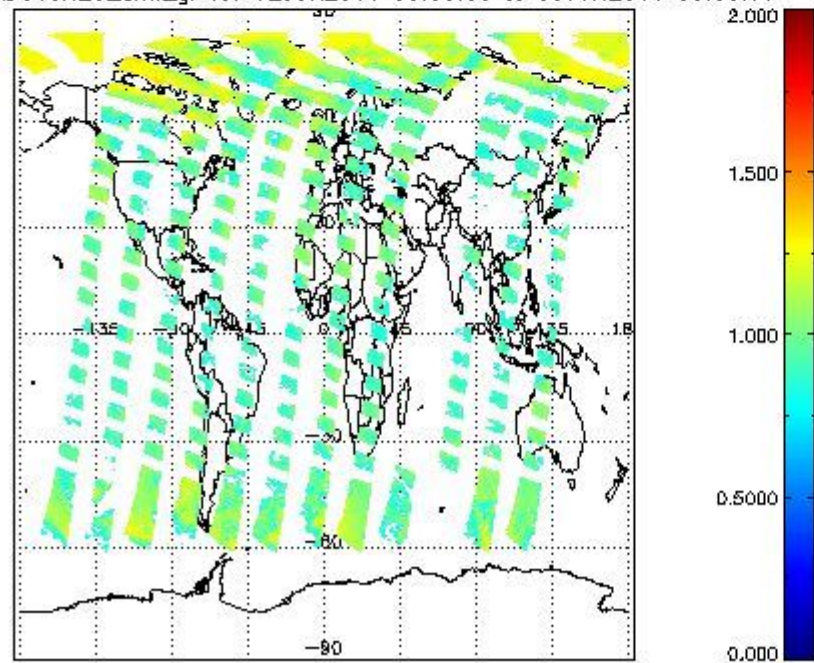
SCIOL2P_NADUV8H2O_arnf_gr for 02JUN2011 00:00:00 to 03JUN2011 00:00:00
