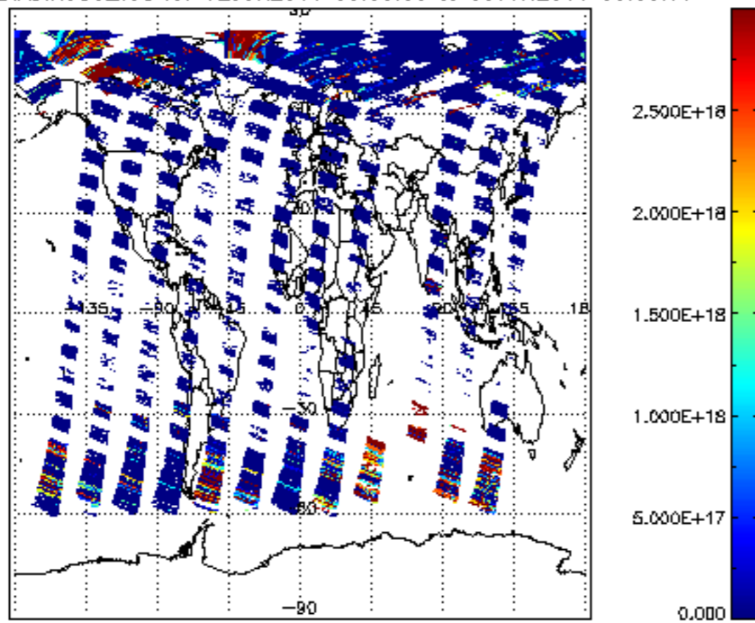
SCIOL2P_NADIR3CO_vcd for 02JUN2011 00:00:00 to 03JUN2011 00:00:00
