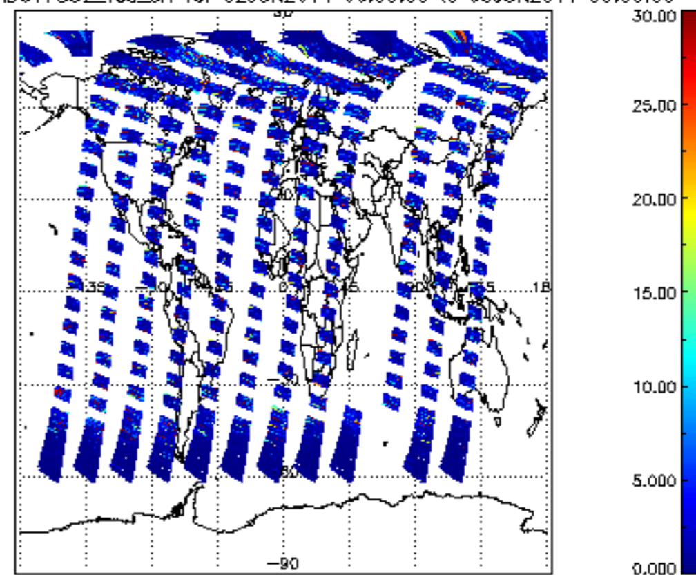
SCIOL2P_NADUV7S02_vcd_err for 02JUN2011 00:00:00 to 03JUN2011 00:00:00
