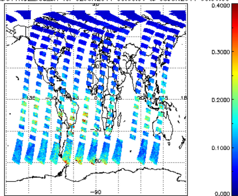
SCIOL2P_NADUV1NO2_vcd_err for 02JUN2011 00:00:00 to 03JUN2011 00:00:00
