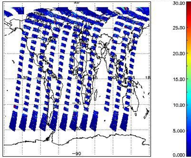
SCIOL2P_NADUV7S02_vcd_err for 02JUN2011 00:00:00 to 03JUN2011 00:00:00
