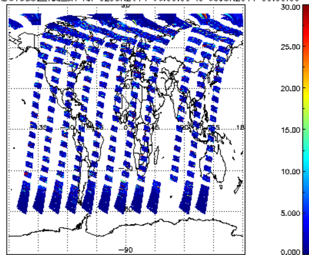
SCIOL2P_NADUV5S02_vcd_err for 02JUN2011 00:00:00 to 03JUN2011 00:00:00
