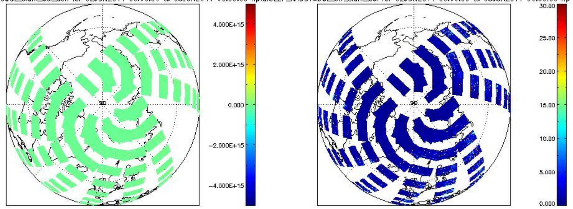
CIOL2P_NADUV60CLslant_col_den for 02JUN2011 00:00:00 to 03JUN2011 00:00:00 np; CIOL2P_NADUV60CLerr_slant_col for 02JUN2011 00:00:00 to 03JUN2011 00:00:00 np
