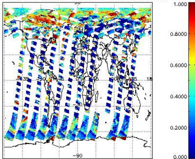
cL_frac for 02JUN2011 00:00:00 to 03JUN2011 00:00:00
