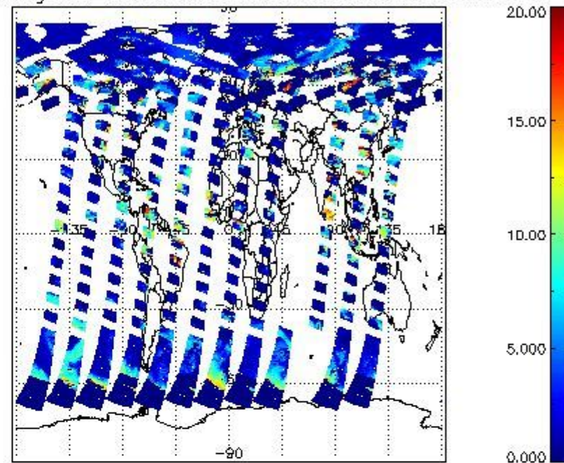
cL_top_height for 02JUN2011 00:00:00 to 03JUN2011 00:00:00
