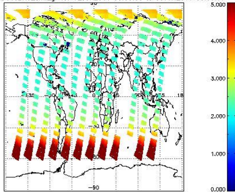
SCIOL2P_NADUV3BRO_amf_gr for 02JUN2011 00:00:00 to 03JUN2011 00:00:00
