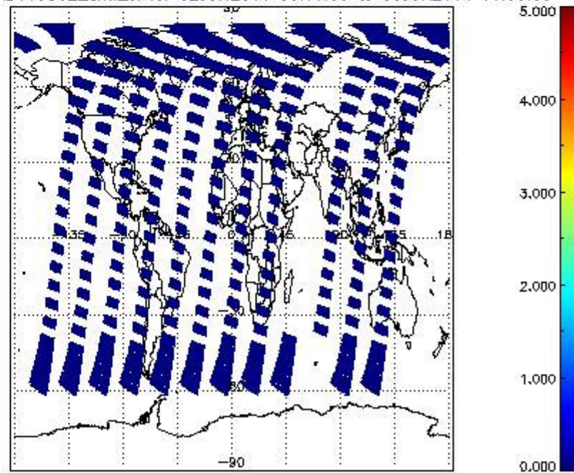
SCIOL2P_NADUV5S02_amf_cl for 02JUN2011 00:00:00 to 03JUN2011 00:00:00
