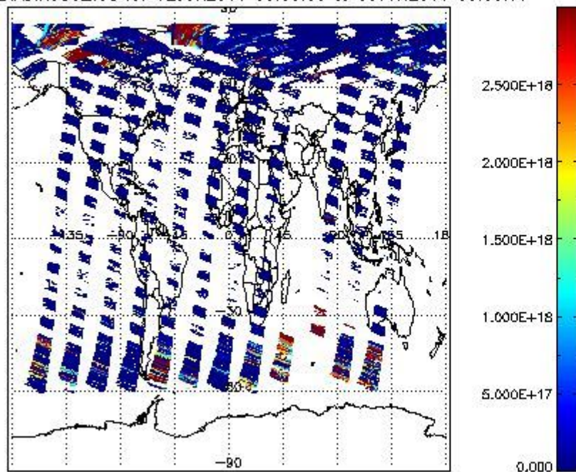
SCIDL2P_NADIR3CO_vcd for 02JUN2011 00:00:00 to 03JUN2011 00:00:00
