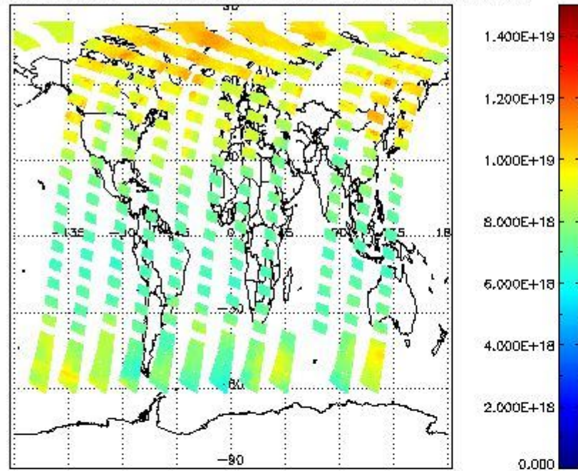
SCIOL2P_NADUV003_vcd for 02JUN2011 00:00:00 to 03JUN2011 00:00:00
