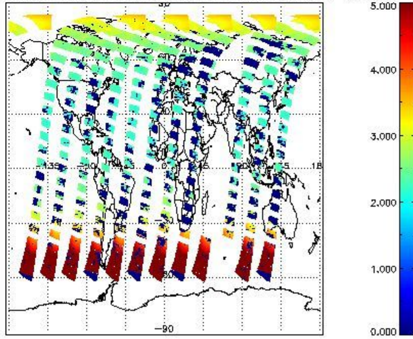
SCIOL2P_NADUV1NO2_amf_cl for 02JUN2011 00:00:00 to 03JUN2011 00:00:00
