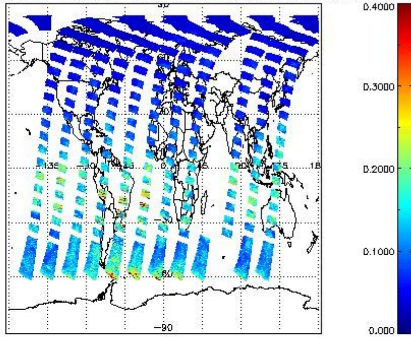
SCIOL2P_NADUV1NO2_vcd_err for 02JUN2011 00:00:00 to 03JUN2011 00:00:00
