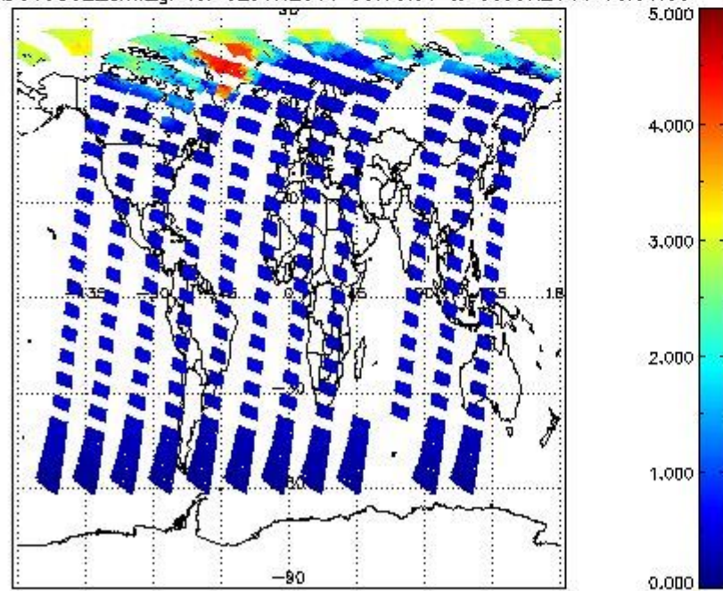
SCIOL2P_NADUV5S02_amf_gr for 02JUN2011 00:00:00 to 03JUN2011 00:00:00
