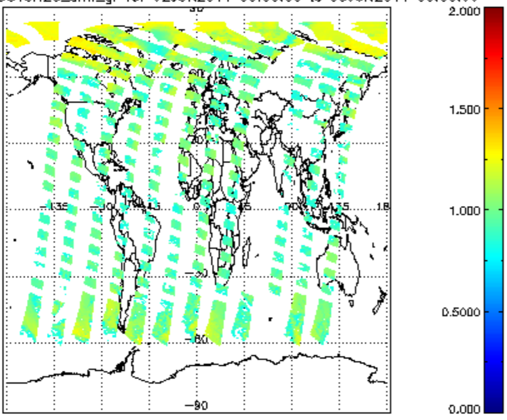
SCIOL2P_NADUV8H2O_amf_gr for 02JUN2011 00:00:00 to 03JUN2011 00:00:00
