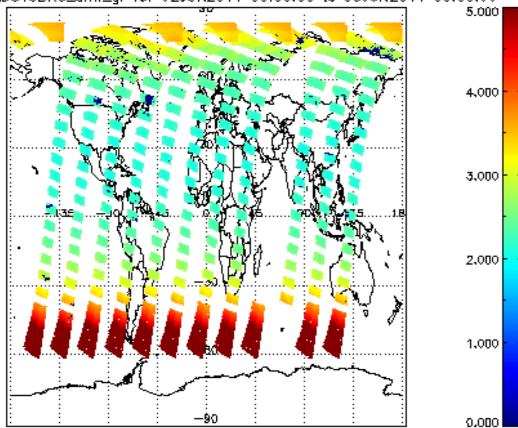
SCIOL2P_NADUV3BRO_amf_gr for 02JUN2011 00:00:00 to 03JUN2011 00:00:00
