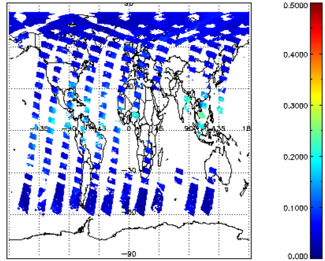
SCIOL2P_NADUV8H2O_vcd_err for 02JUN2011 00:00:00 to 03JUN2011 00:00:00
