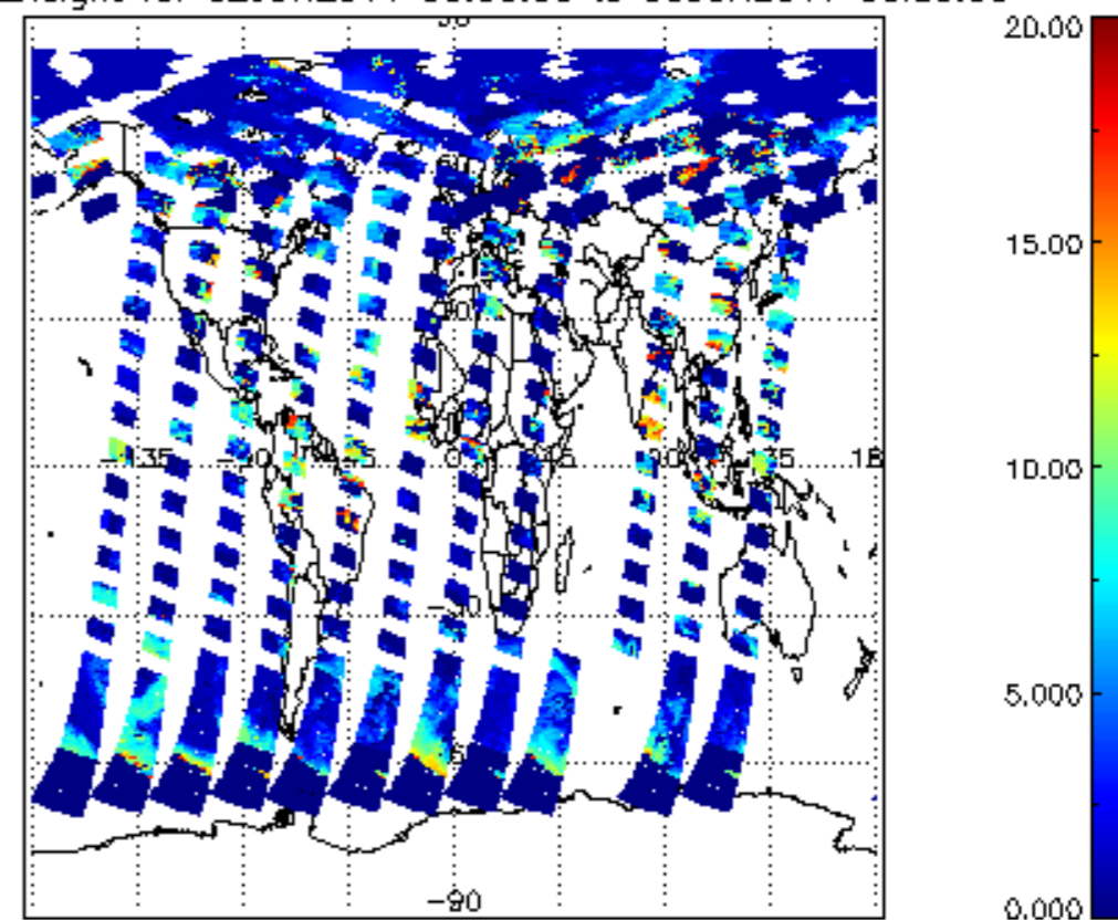
cl_top_height for 02JUN2011 00:00:00 to 03JUN2011 00:00:00
