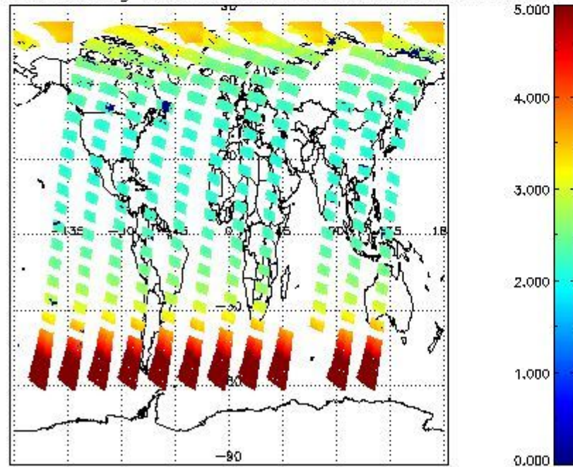
SCIOL2P_NADUV003_amf_gr for 02JUN2011 00:00:00 to 03JUN2011 00:00:00
