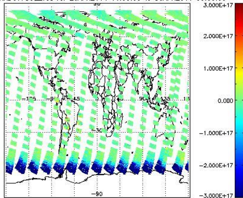
SCIOL2P_NADUV7S02_vcd for 29APR2011 00:00:00 to 30APR2011 00:00:00
