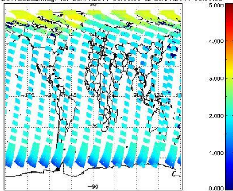
SCIOL2P_NADUV7S02_amf_gr for 29APR2011 00:00:00 to 30APR2011 00:00:00
