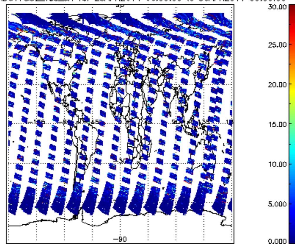
SCIOL2P_NADUV7S02_vcd_err for 29APR2011 00:00:00 to 30APR2011 00:00:00
