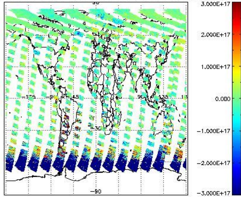
SCIOL2P_NADUV5S02_vcd for 29APR2011 00:00:00 to 30APR2011 00:00:00
