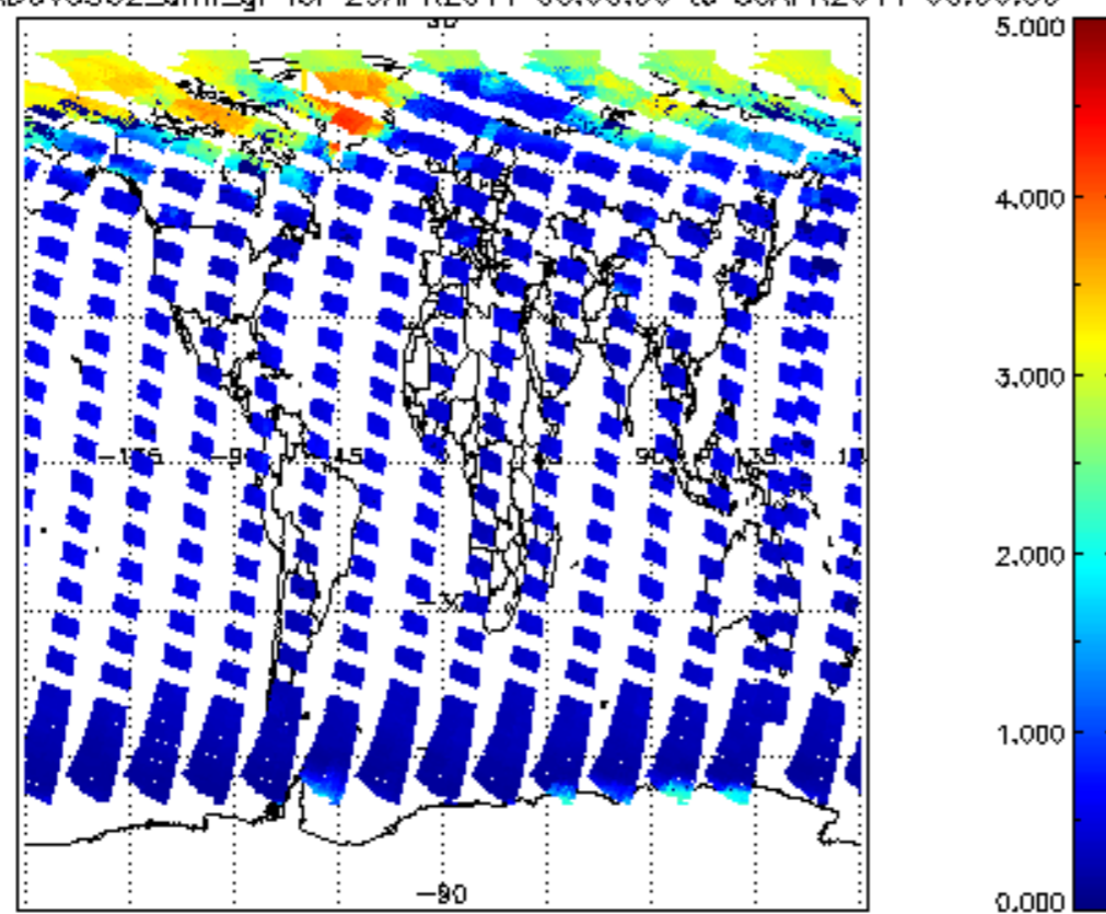
SCIOL2P_NADUV5S02_amf_gr for 29APR2011 00:00:00 to 30APR2011 00:00:00
