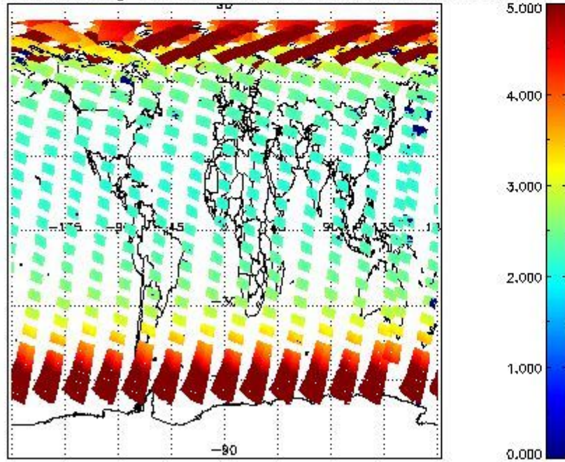
SCIOL2P_NADUV003_amf_gr for 29APR2011 00:00:00 to 30APR2011 00:00:00
