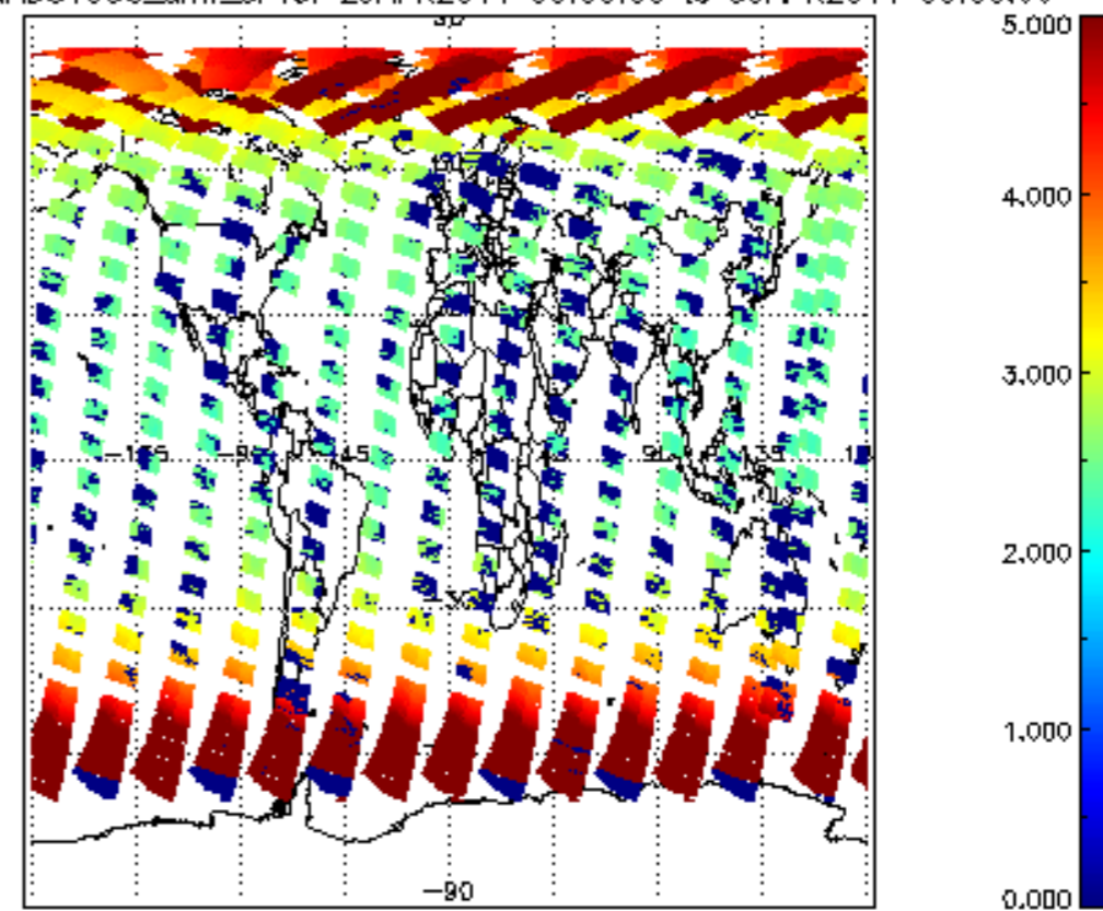
SCIOL2P_NADUV003_amf_cl for 29APR2011 00:00:00 to 30APR2011 00:00:00
