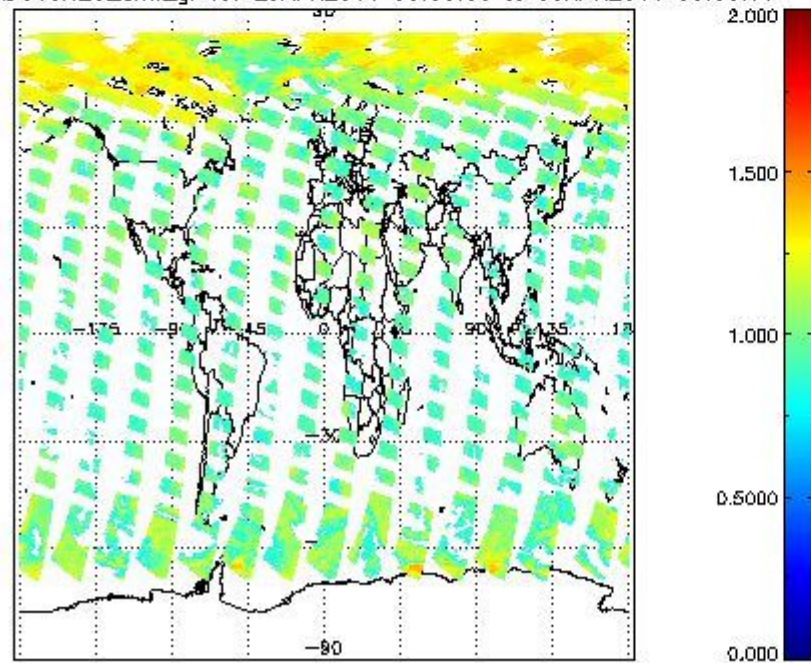
SCIOL2P_NADUV8H2O_arnf_gr for 29APR2011 00:00:00 to 30APR2011 00:00:00
