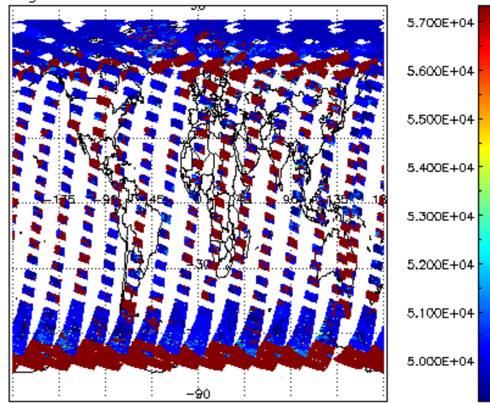
cloud_flags for 29APR2011 00:00:00 to 30APR2011 00:00:00
