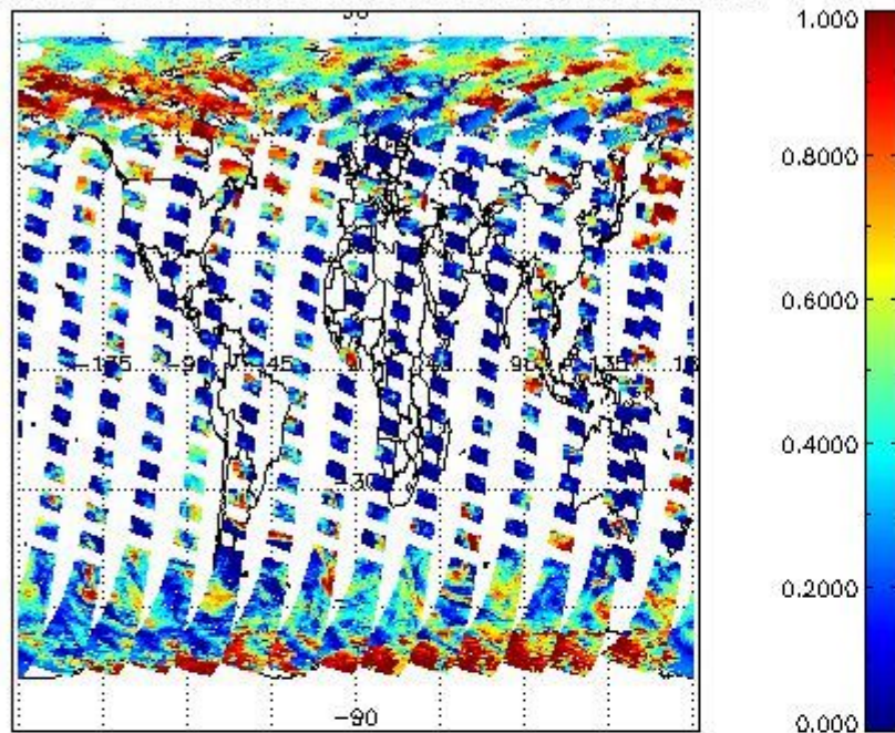
cL_frac for 29APR2011 00:00:00 to 30APR2011 00:00:00
