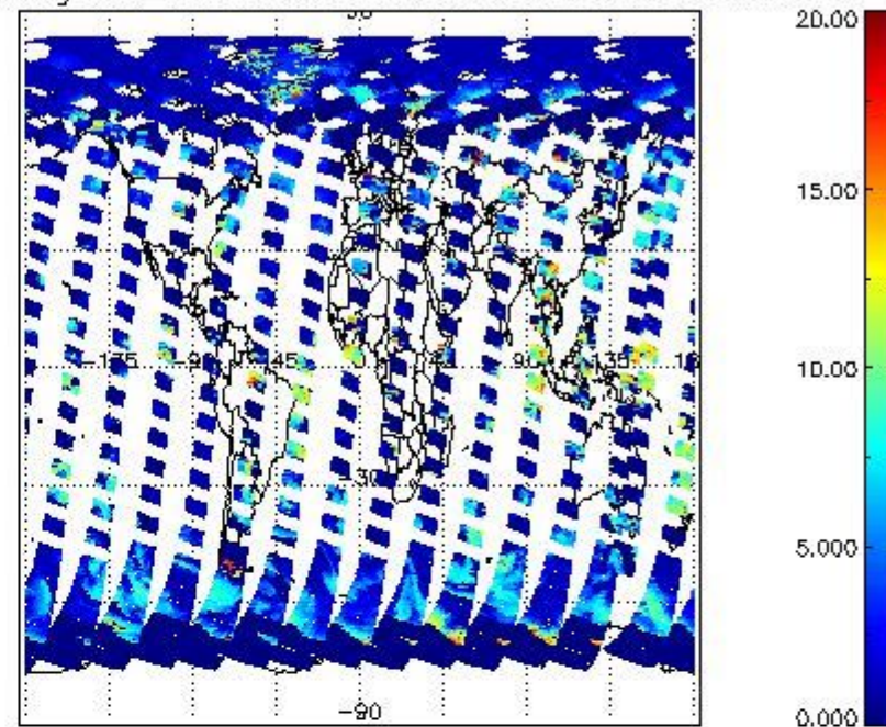
cL_top_height for 29APR2011 00:00:00 to 30APR2011 00:00:00
