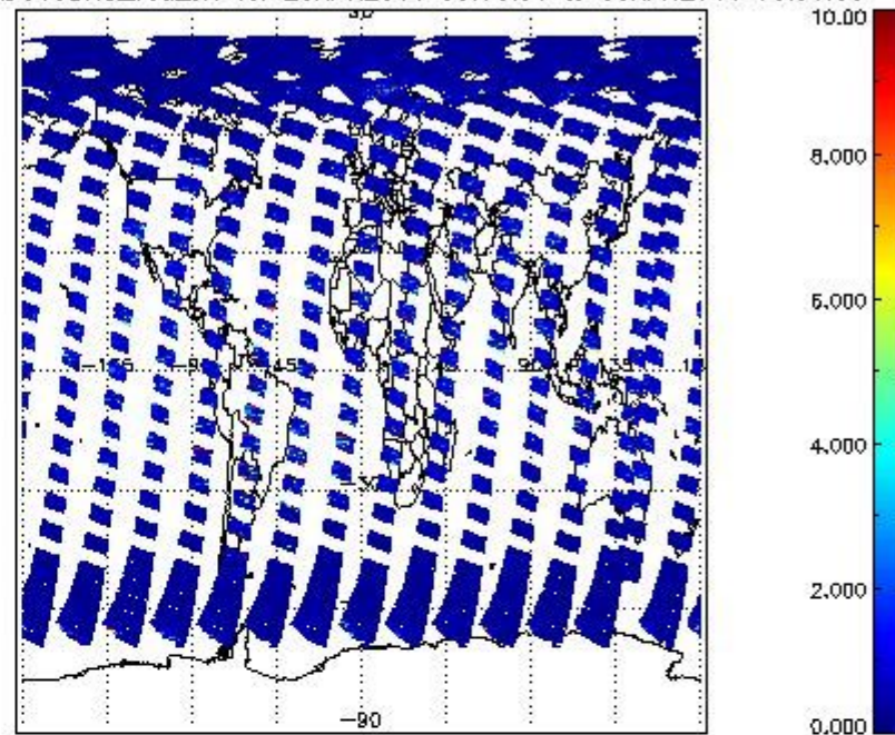
SCIOL2P_NADUV3BRO_vcd_err for 29APR2011 00:00:00 to 30APR2011 00:00:00
