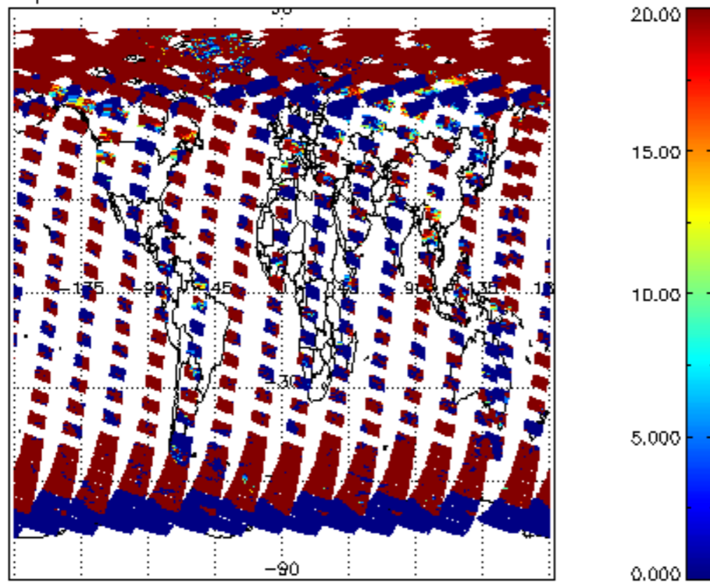
cl_opt_depth for 29APR2011 00:00:00 to 30APR2011 00:00:00
