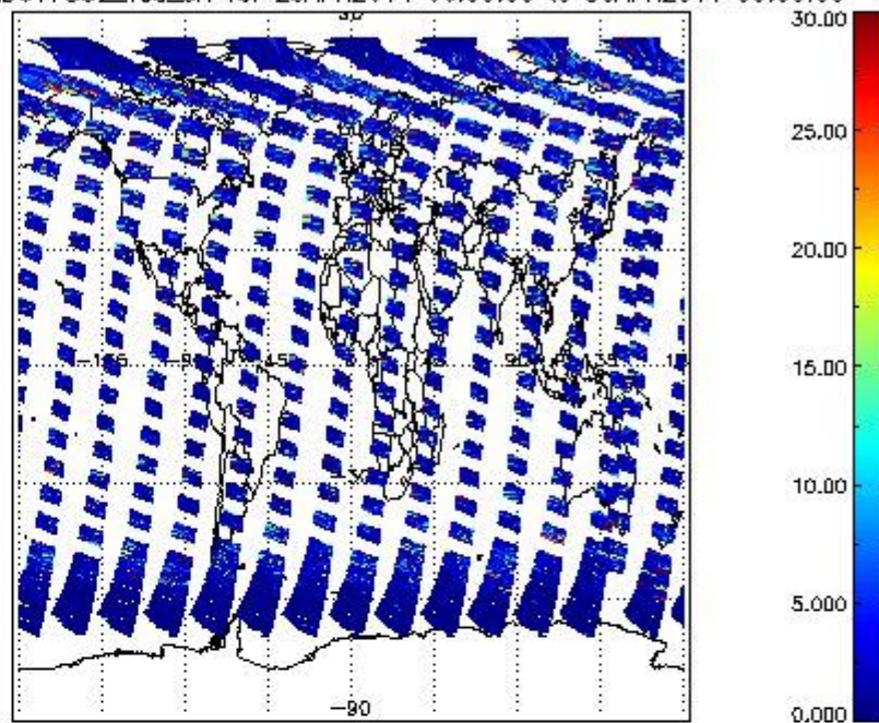
SCIOL2P_NADUV7S02_vcd_err for 29APR2011 00:00:00 to 30APR2011 00:00:00
