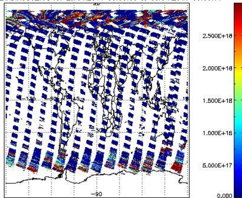
SCIDL2P_NADIR3CO_vcd for 29APR2011 00:00:00 to 30APR2011 00:00:00
