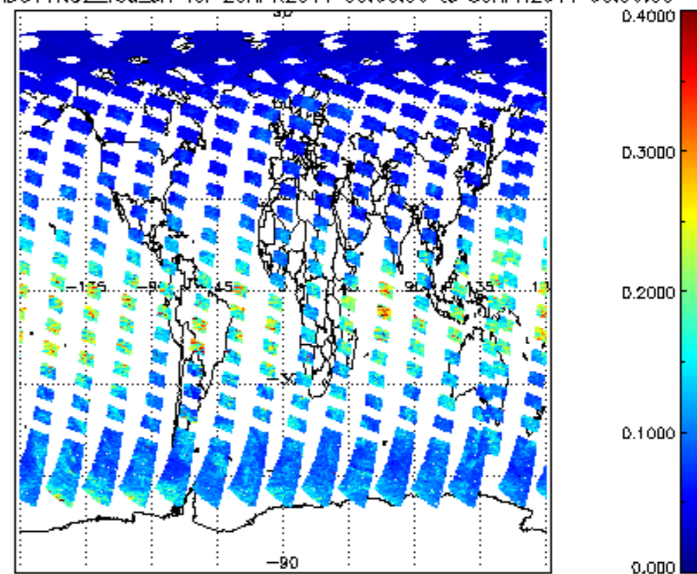
SCIOL2P_NADUV1NO2_vcd_err for 29APR2011 00:00:00 to 30APR2011 00:00:00
