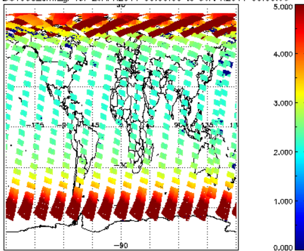
SCIOL2P_NADUV003_amf_gr for 29APR2011 00:00:00 to 30APR2011 00:00:00
