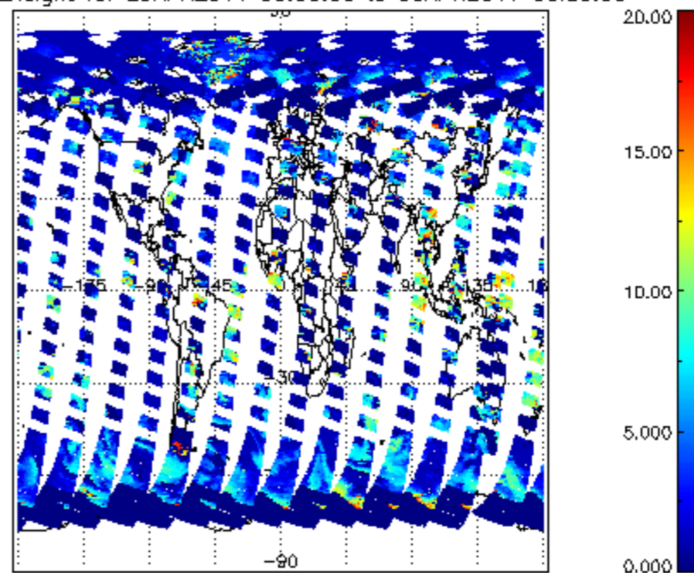
cl_top_height for 29APR2011 00:00:00 to 30APR2011 00:00:00
