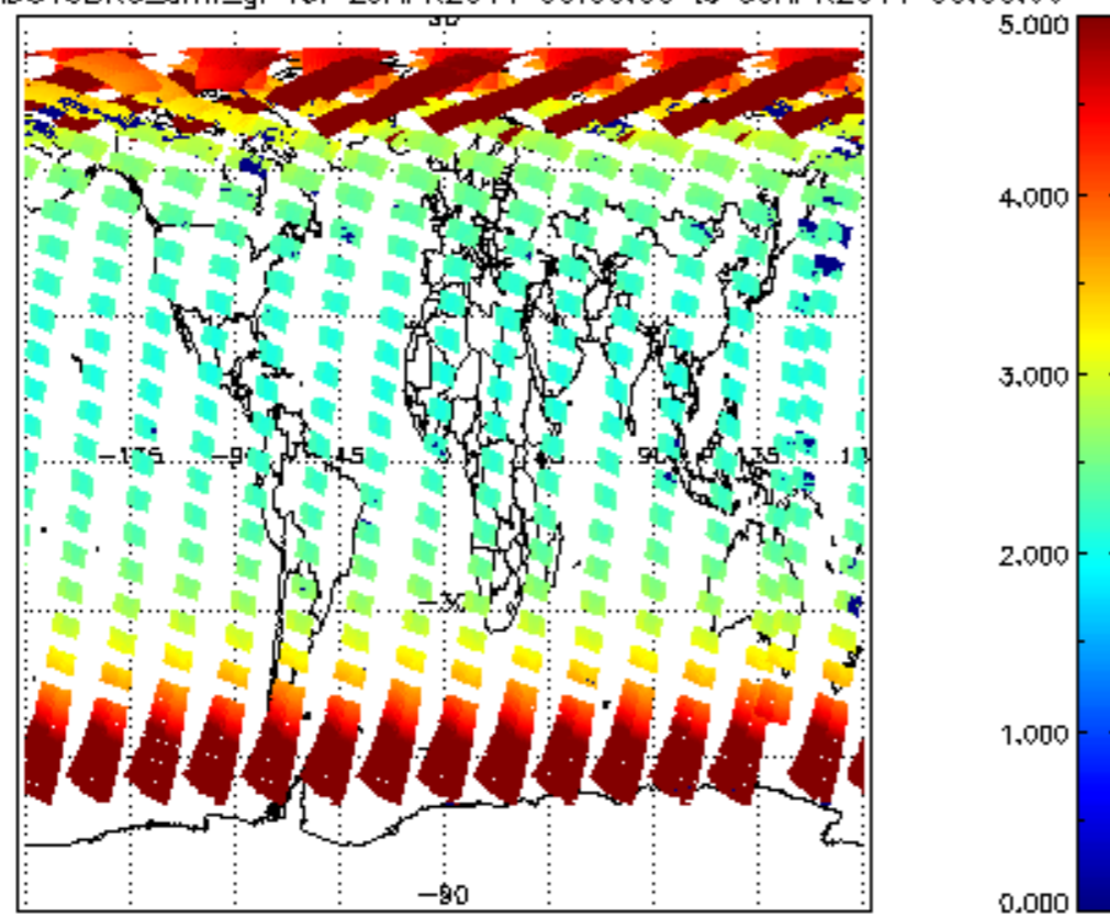
SCIOL2P_NADUV3BRO_amf_gr for 29APR2011 00:00:00 to 30APR2011 00:00:00
