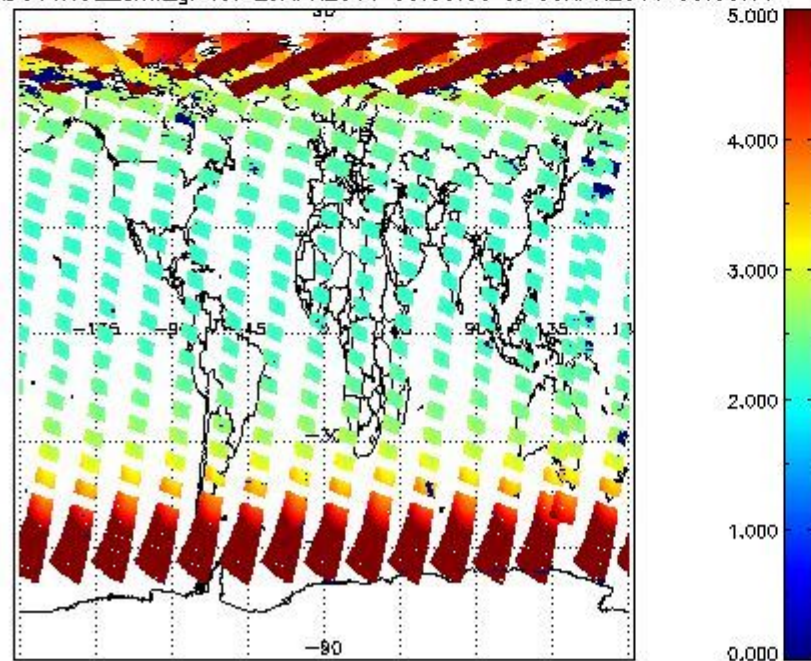
SCIOL2P_NADUV1NO2_amf_gr for 29APR2011 00:00:00 to 30APR2011 00:00:00
