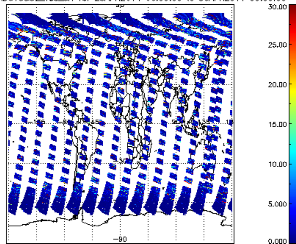
SCIOL2P_NADUV5S02_vcd_err for 29APR2011 00:00:00 to 30APR2011 00:00:00
