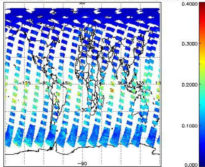
SCIOL2P_NADUV1NO2_vcd_err for 29APR2011 00:00:00 to 30APR2011 00:00:00
