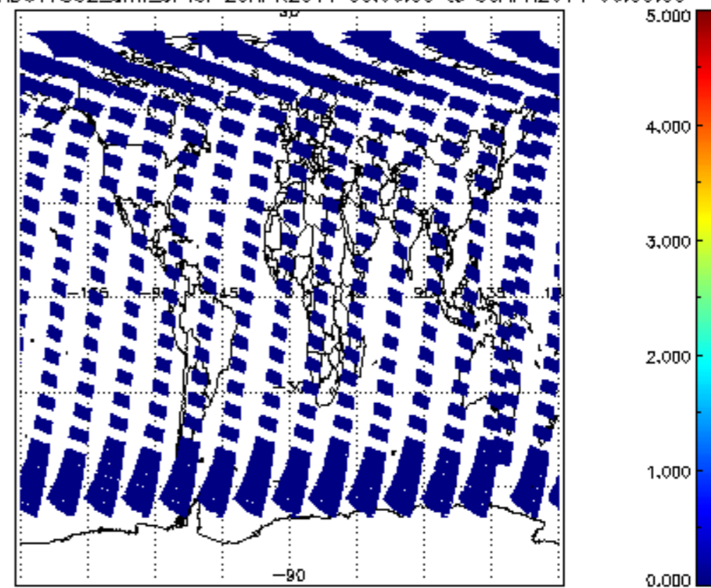
SCIOL2P_NADUV7S02_amf_cl for 29APR2011 00:00:00 to 30APR2011 00:00:00
