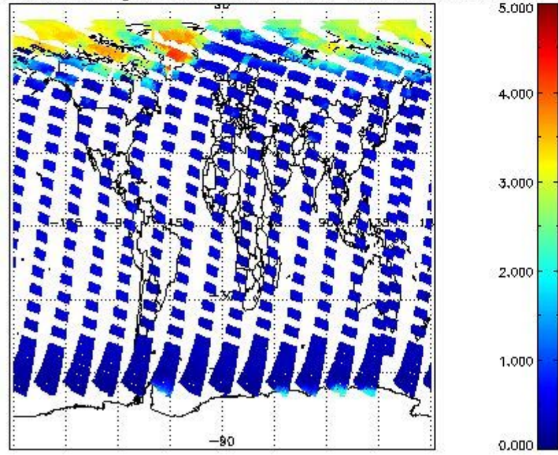
SCIOL2P_NADUV5S02_amf_gr for 29APR2011 00:00:00 to 30APR2011 00:00:00
