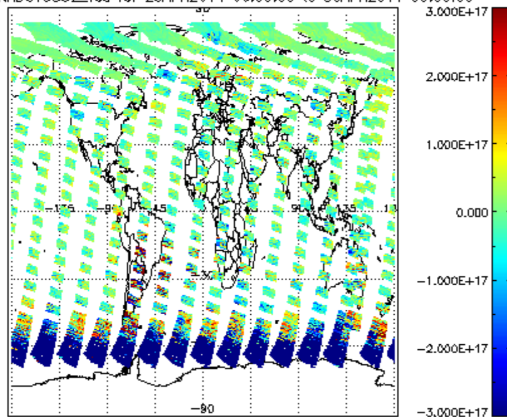
SCIOL2P_NADUV5S02_vcd for 29APR2011 00:00:00 to 30APR2011 00:00:00
