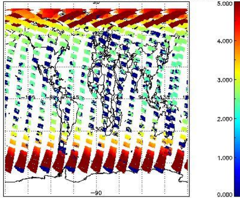
SCIOL2P_NADUV003_amf_cl for 29APR2011 00:00:00 to 30APR2011 00:00:00
