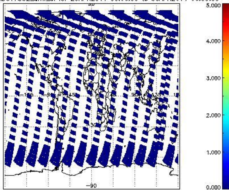
SCIOL2P_NADUV7S02_amf_cl for 29APR2011 00:00:00 to 30APR2011 00:00:00
