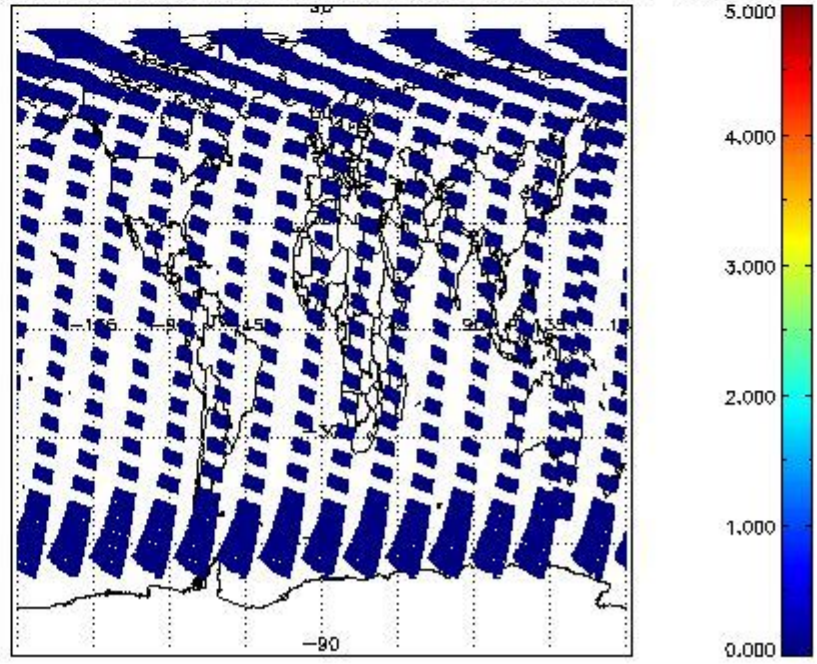
SCIOL2P_NADUV5S02_amf_cl for 29APR2011 00:00:00 to 30APR2011 00:00:00
