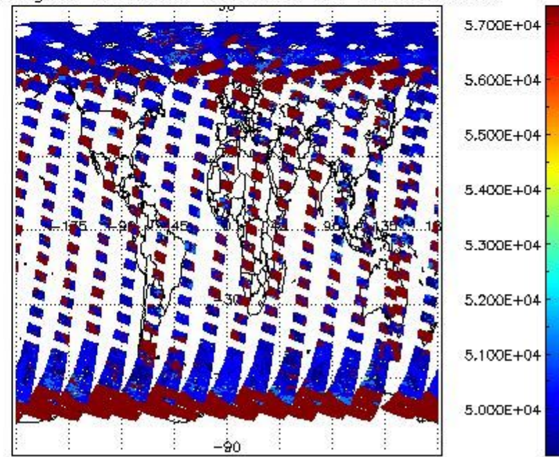
cloud_flags for 29APR2011 00:00:00 to 30APR2011 00:00:00
