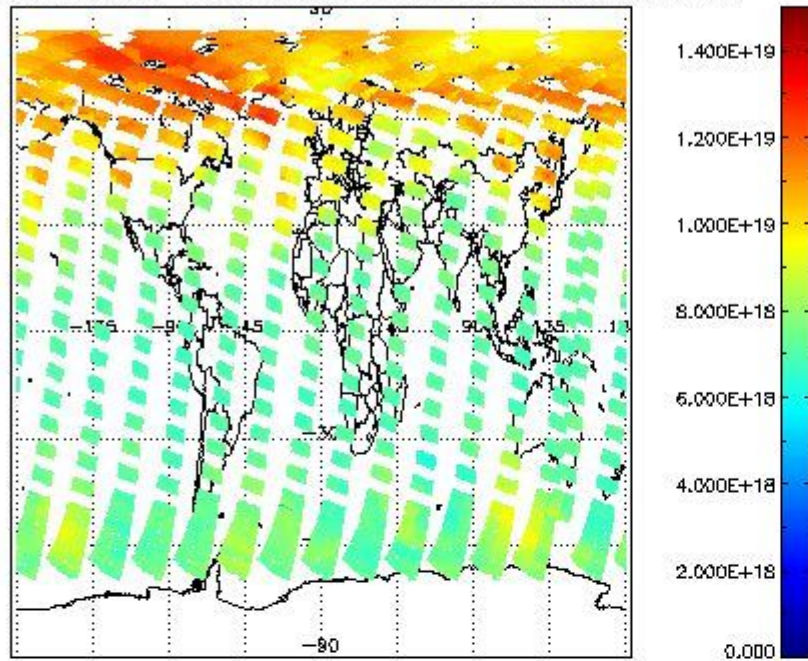
SCIOL2P_NADUV003_vcd for 29APR2011 00:00:00 to 30APR2011 00:00:00
