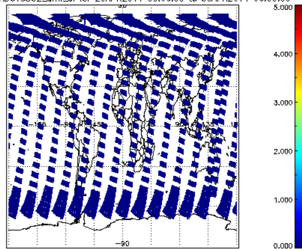
SCIOL2P_NADUV5S02_amf_cl for 29APR2011 00:00:00 to 30APR2011 00:00:00
