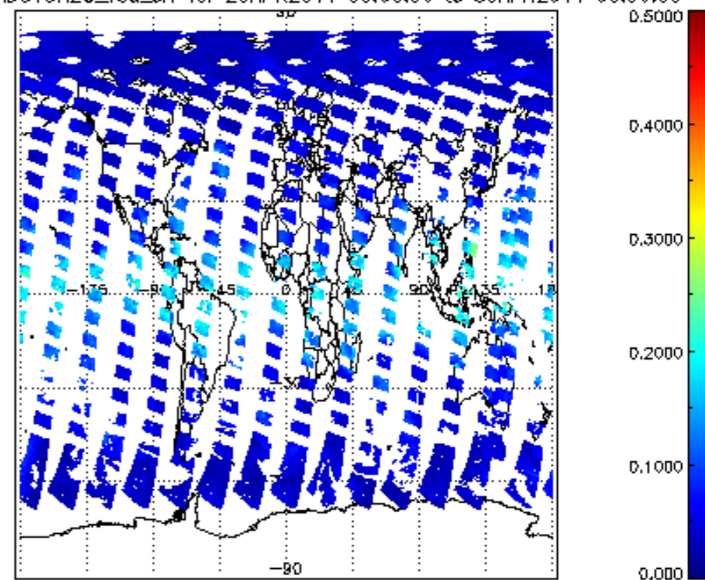
SCIOL2P_NADUV8H2O_vcd_err for 29APR2011 00:00:00 to 30APR2011 00:00:00
