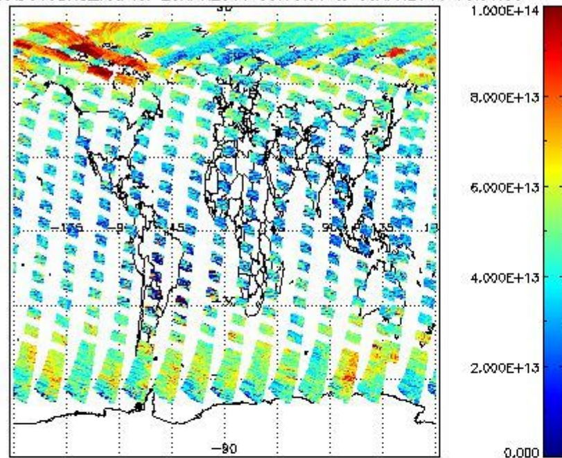
SCIOL2P_NADUV3BRO_vcd for 29APR2011 00:00:00 to 30APR2011 00:00:00
