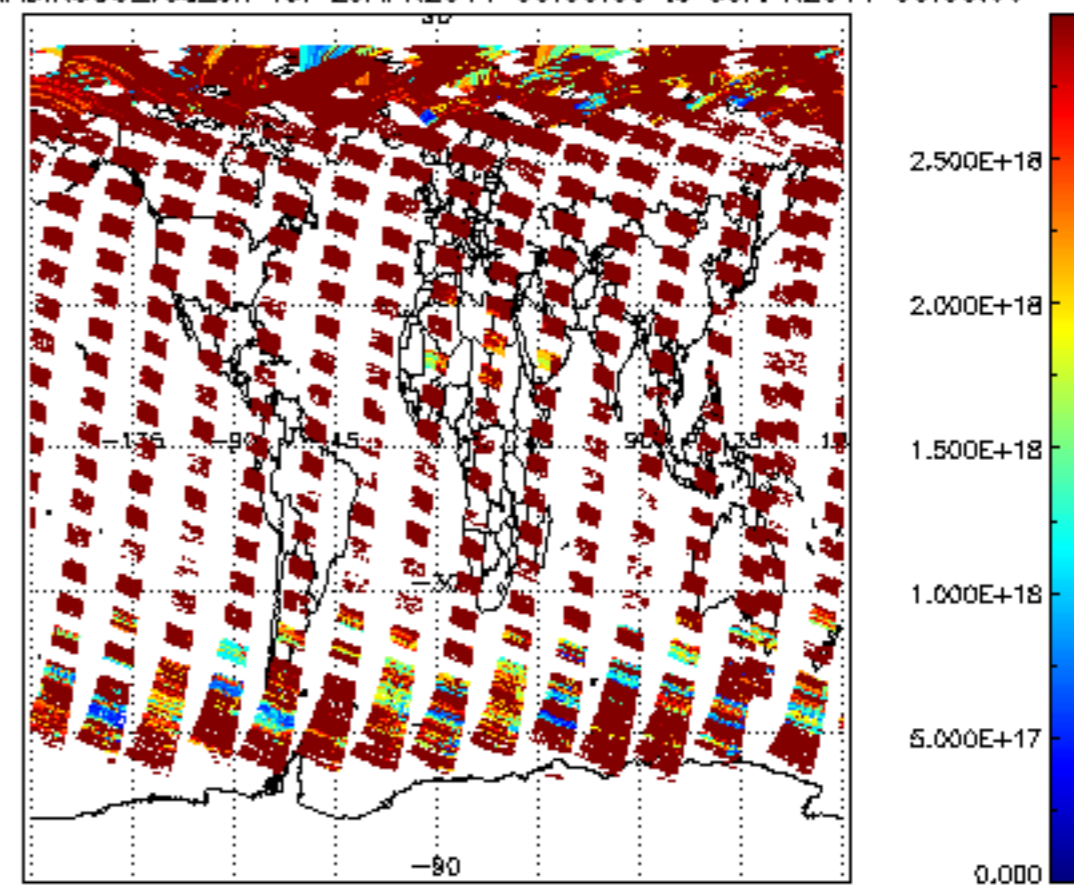
SCIOL2P_NADIR3CO_vcd_err for 29APR2011 00:00:00 to 30APR2011 00:00:00
