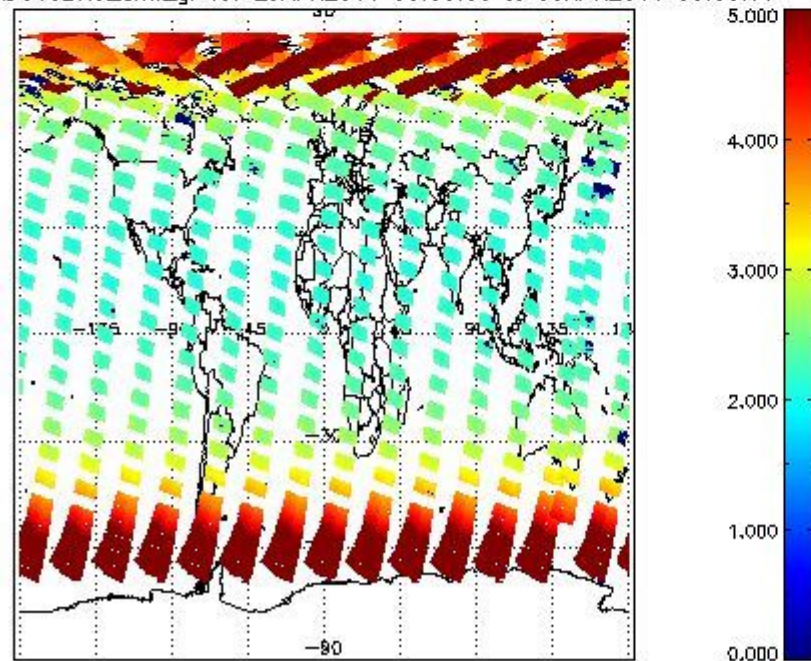
SCIOL2P_NADUV3BRO_amf_gr for 29APR2011 00:00:00 to 30APR2011 00:00:00
