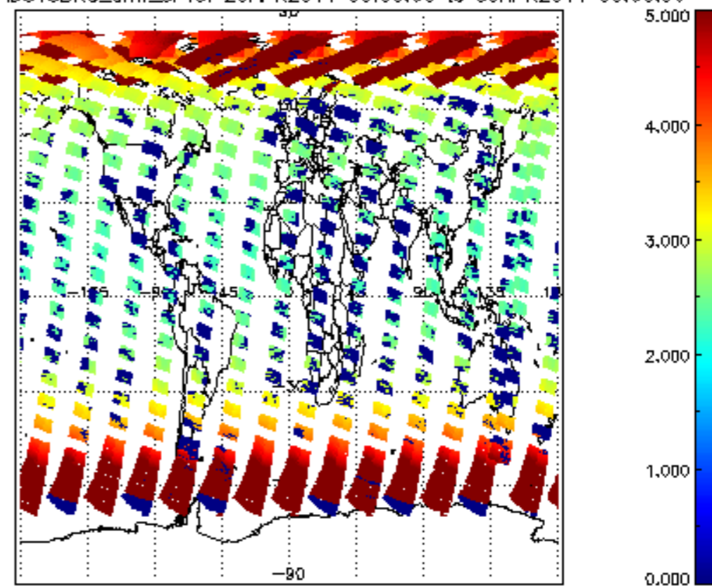
SCIOL2P_NADUV3BRO_amf_cl for 29APR2011 00:00:00 to 30APR2011 00:00:00
