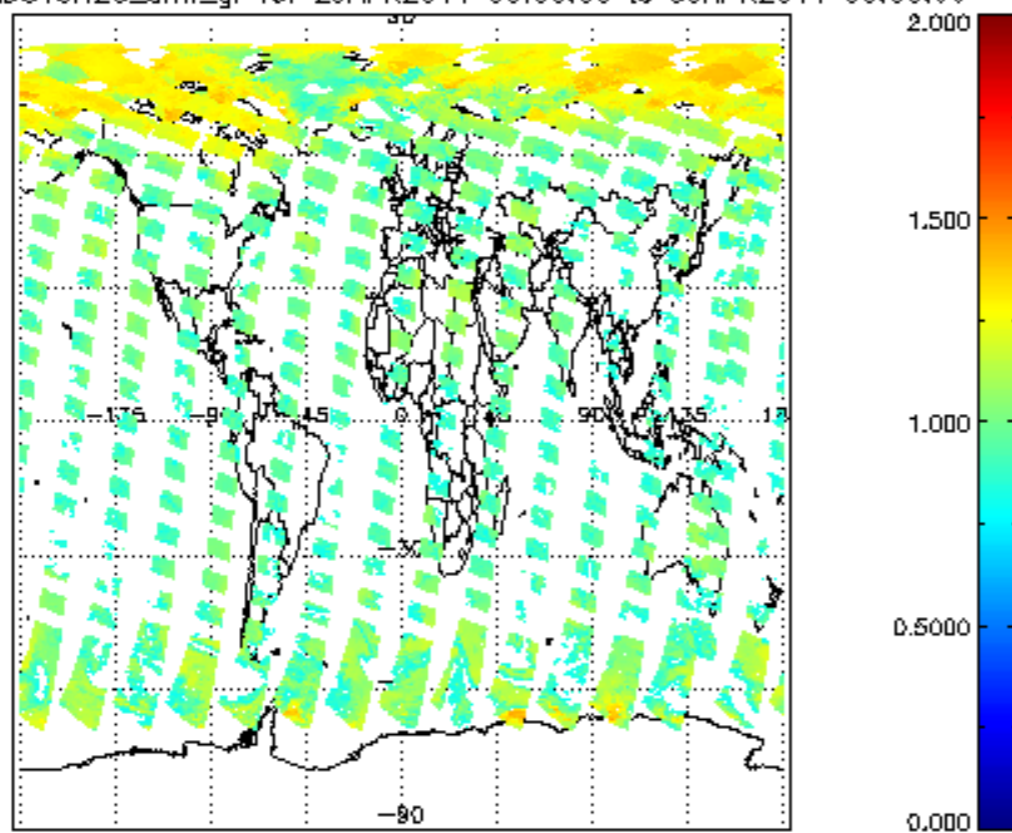
SCIOL2P_NADUV8H2O_amf_gr for 29APR2011 00:00:00 to 30APR2011 00:00:00
