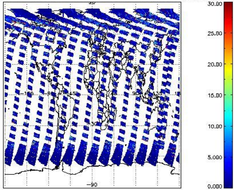
SCIOL2P_NADUV5S02_vcd_err for 29APR2011 00:00:00 to 30APR2011 00:00:00
