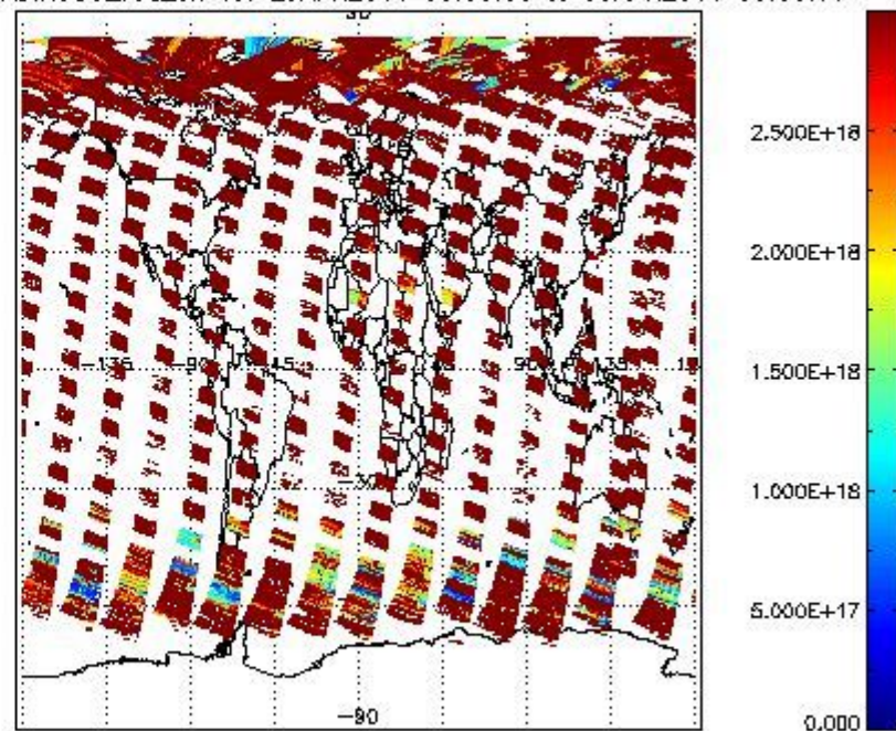
SCIDL2P_NADIR3CO_vcd_err for 29APR2011 00:00:00 to 30APR2011 00:00:00
