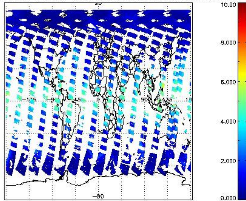
SCIOL2P_NADUV8H2O_vcd for 29APR2011 00:00:00 to 30APR2011 00:00:00
