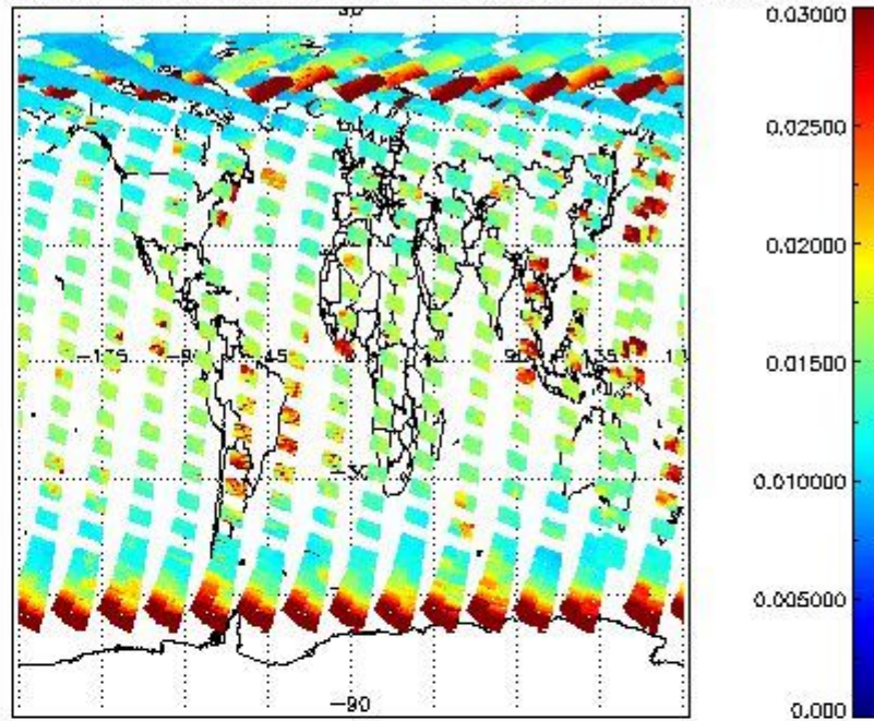
SCIOL2P_NADUV003_vcd_err for 29APR2011 00:00:00 to 30APR2011 00:00:00
