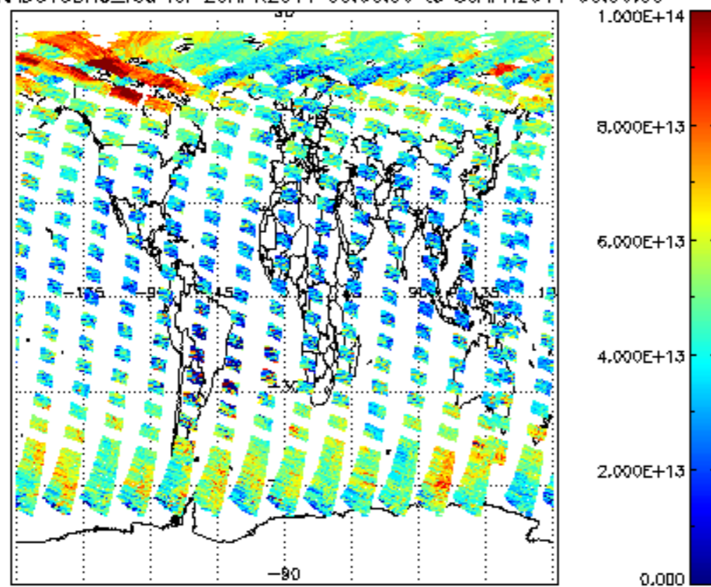
SCIOL2P_NADUV3BRO_vcd for 29APR2011 00:00:00 to 30APR2011 00:00:00
