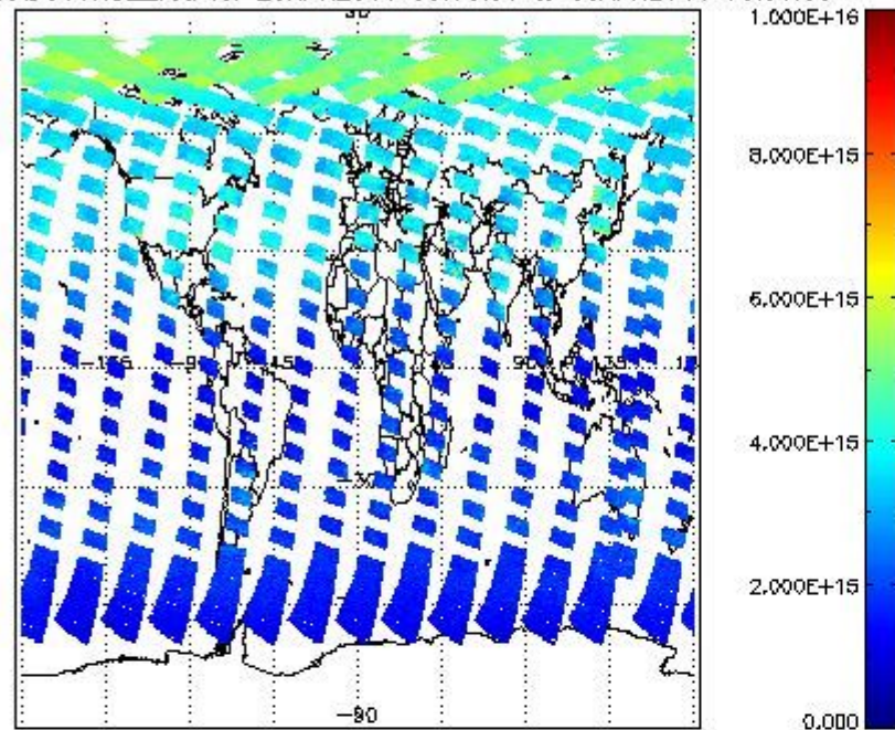
SCIOL2P_NADUV1NO2_vcd for 29APR2011 00:00:00 to 30APR2011 00:00:00
