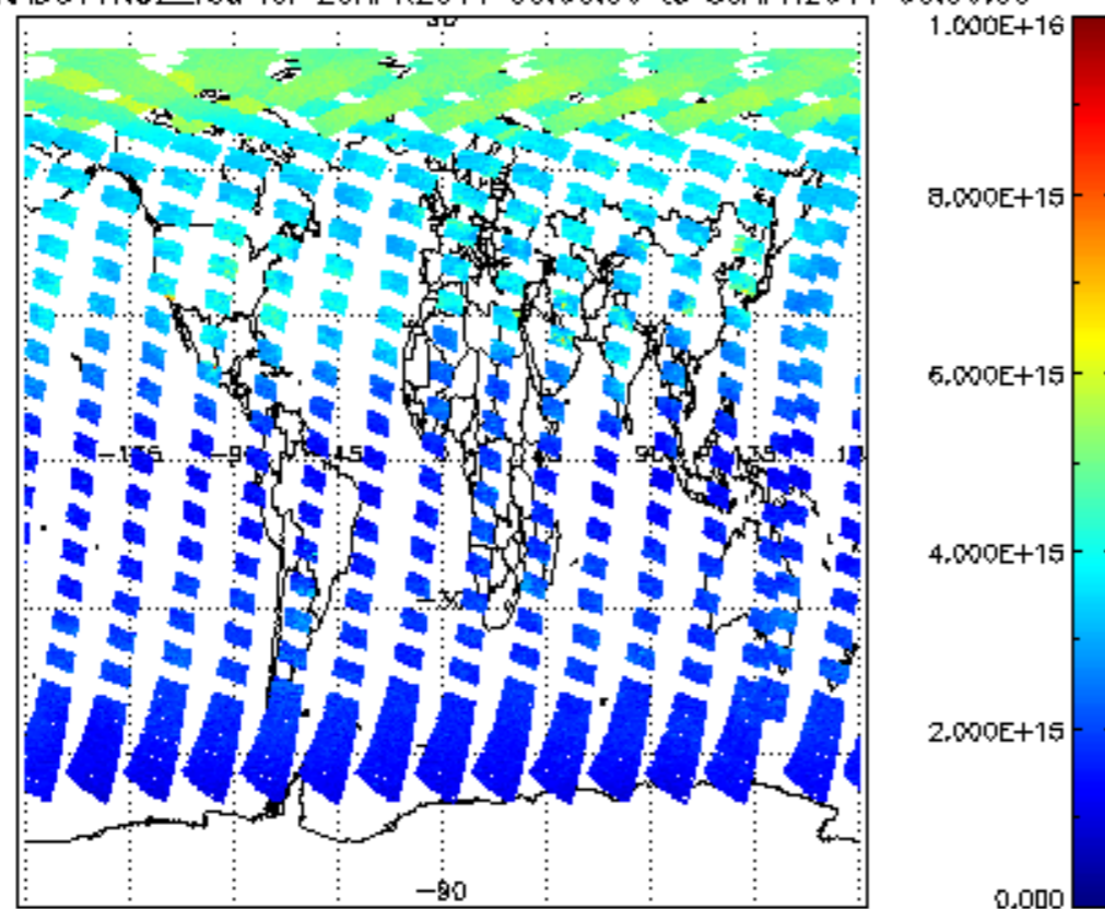
SCIOL2P_NADUV1NO2_vcd for 29APR2011 00:00:00 to 30APR2011 00:00:00
