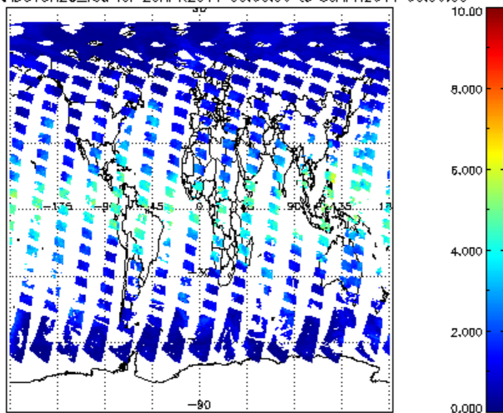
SCIOL2P_NADUV8H2O_vcd for 29APR2011 00:00:00 to 30APR2011 00:00:00
