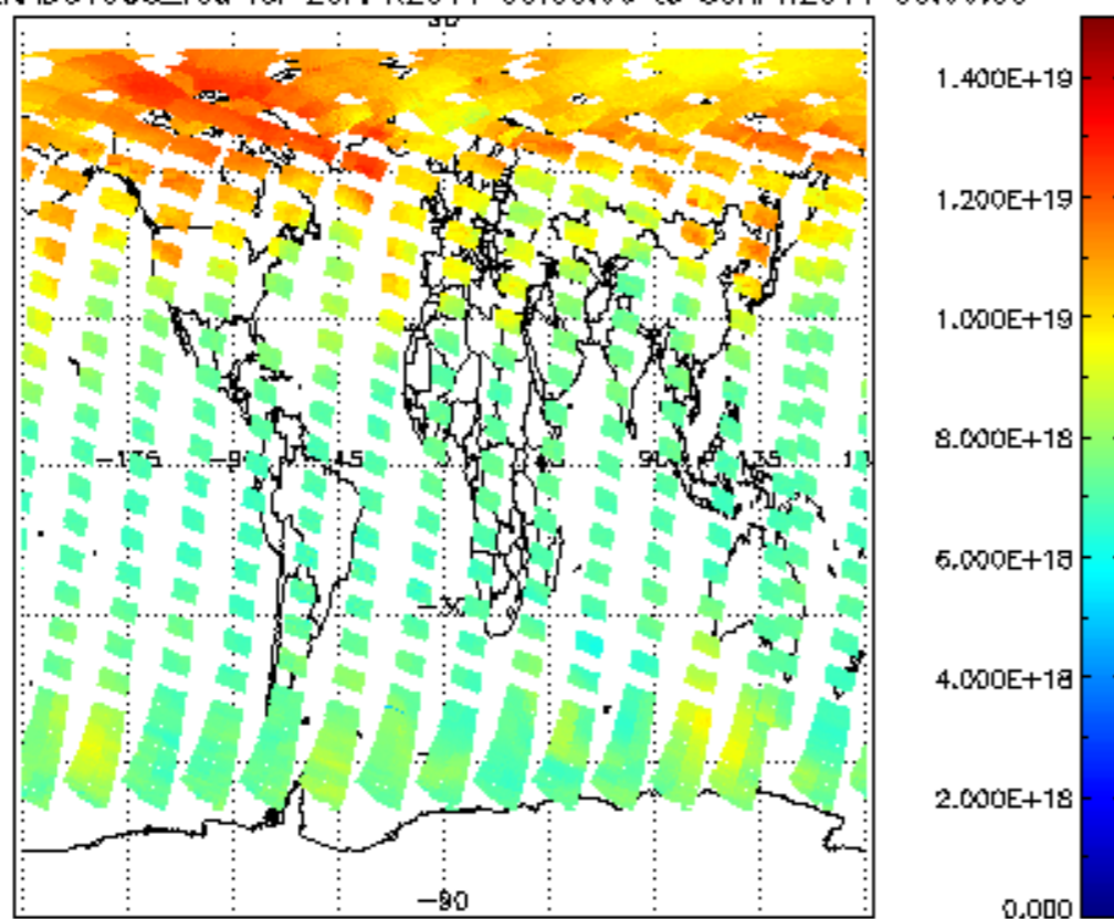
SCIOL2P_NADUV003_vcd for 29APR2011 00:00:00 to 30APR2011 00:00:00
