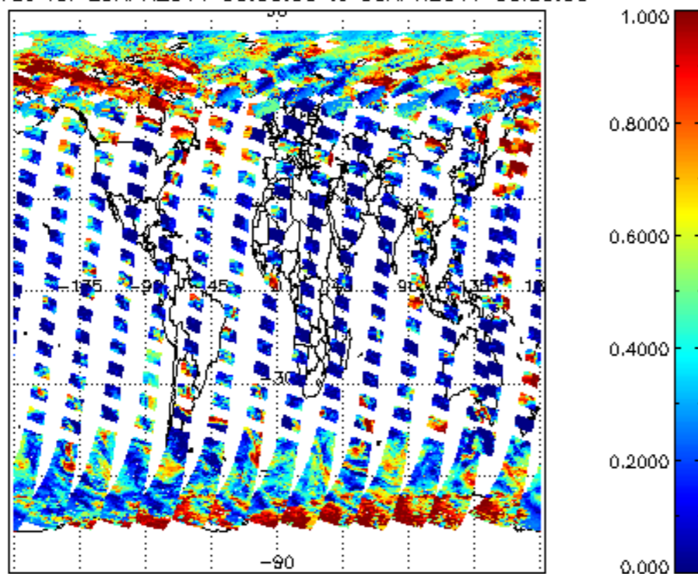
cl_frac for 29APR2011 00:00:00 to 30APR2011 00:00:00
