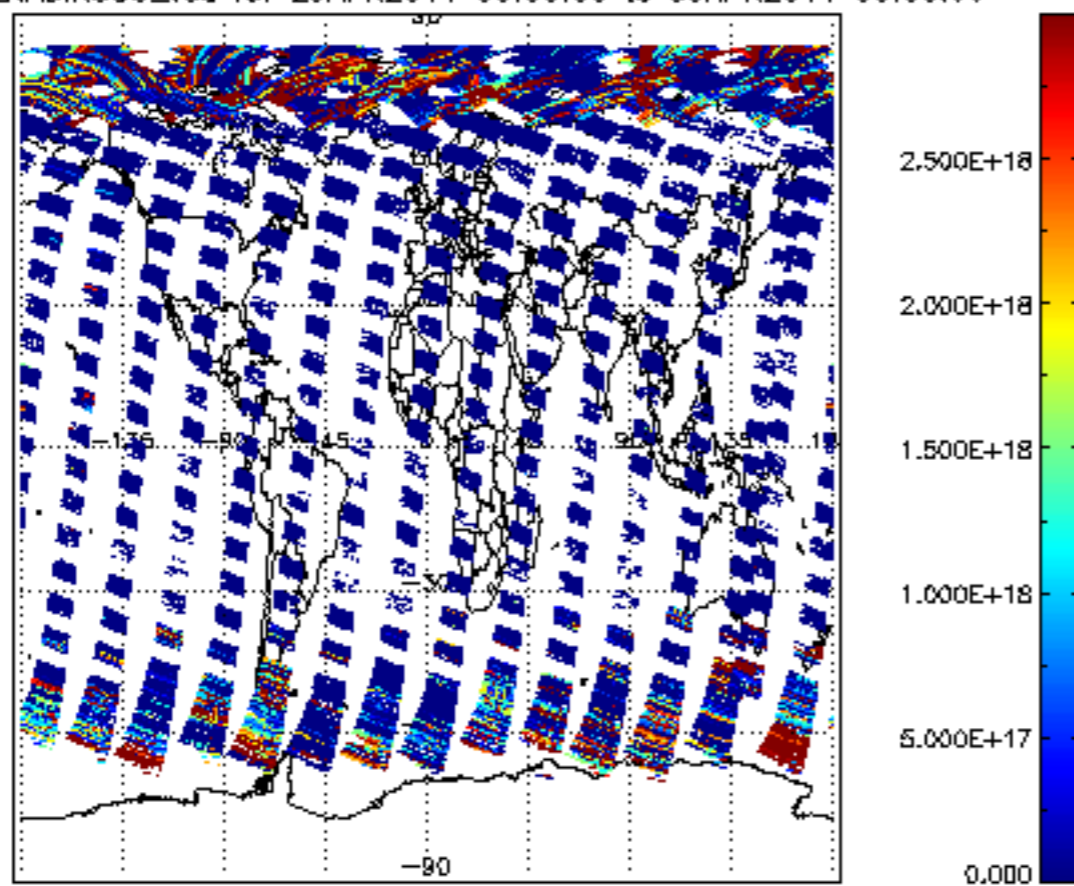
SCIOL2P_NADIR3CO_vcd for 29APR2011 00:00:00 to 30APR2011 00:00:00
