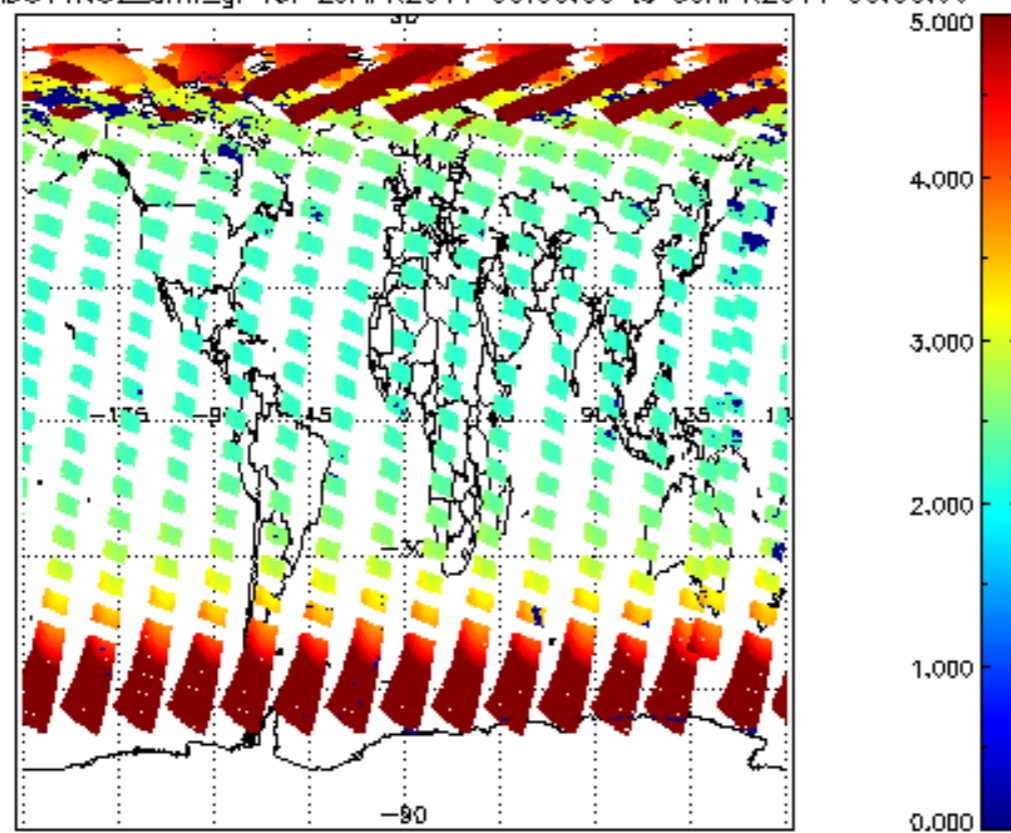
SCIOL2P_NADUV1NO2_amf_gr for 29APR2011 00:00:00 to 30APR2011 00:00:00
