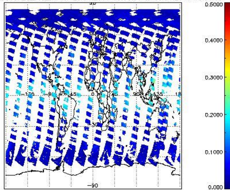
SCIOL2P_NADUV8H2O_vcd_err for 29APR2011 00:00:00 to 30APR2011 00:00:00
