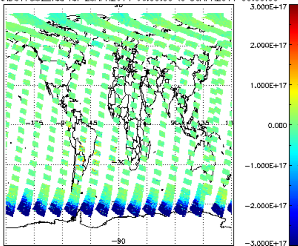
SCIOL2P_NADUV7S02_vcd for 29APR2011 00:00:00 to 30APR2011 00:00:00
