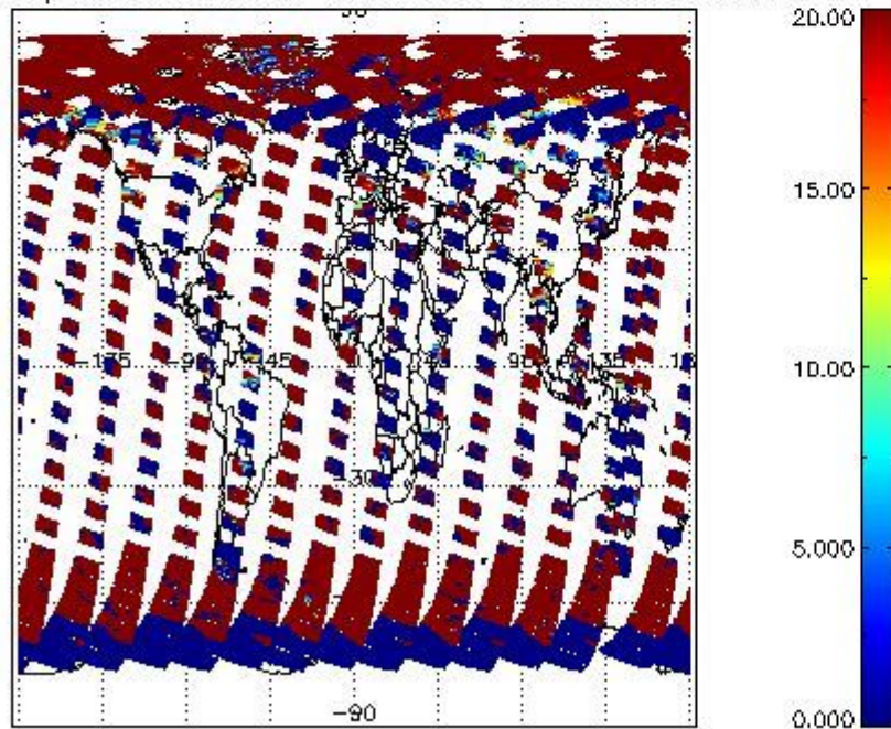
cL_opt_depth for 29APR2011 00:00:00 to 30APR2011 00:00:00
