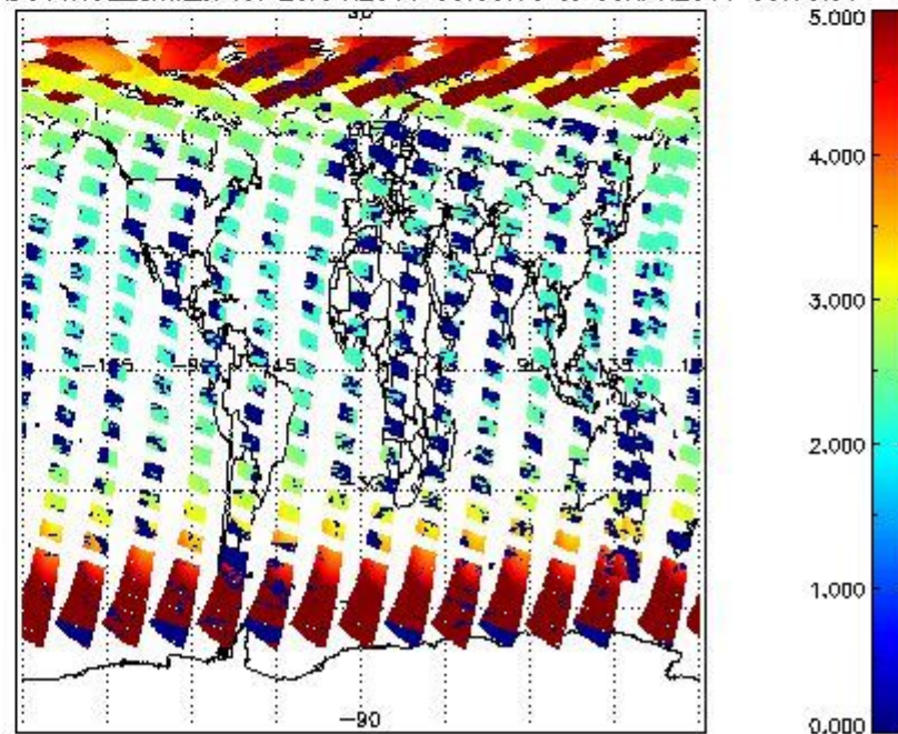
SCIOL2P_NADUV1NO2_amf_cl for 29APR2011 00:00:00 to 30APR2011 00:00:00
