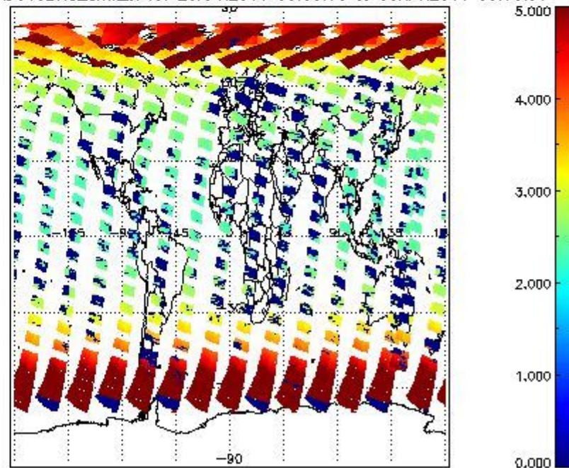
SCIOL2P_NADUV3BRO_amf_cl for 29APR2011 00:00:00 to 30APR2011 00:00:00
