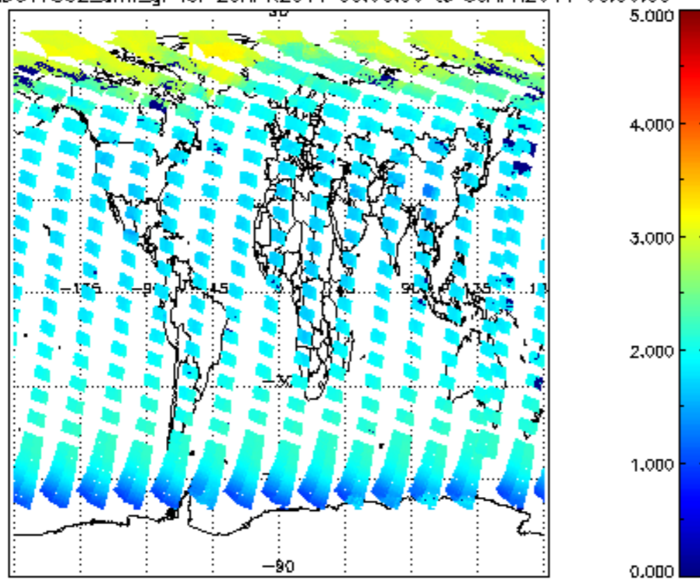
SCIOL2P_NADUV7S02_amf_gr for 29APR2011 00:00:00 to 30APR2011 00:00:00
