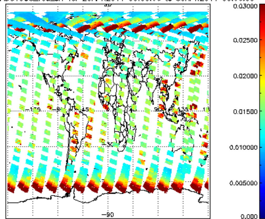
SCIOL2P_NADUV003_vcd_err for 29APR2011 00:00:00 to 30APR2011 00:00:00
