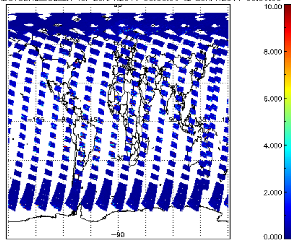
SCIOL2P_NADUV3BRO_vcd_err for 29APR2011 00:00:00 to 30APR2011 00:00:00
