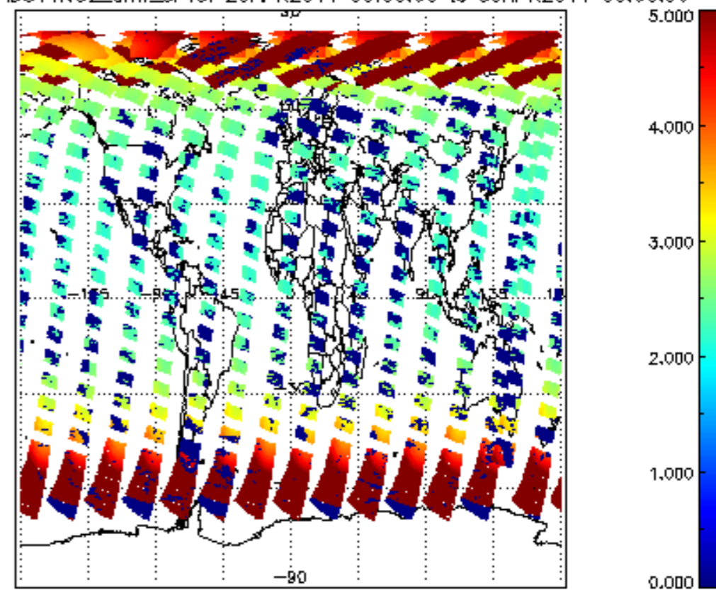
SCIOL2P_NADUV1NO2_amf_sl for 29APR2011 00:00:00 to 30APR2011 00:00:00
