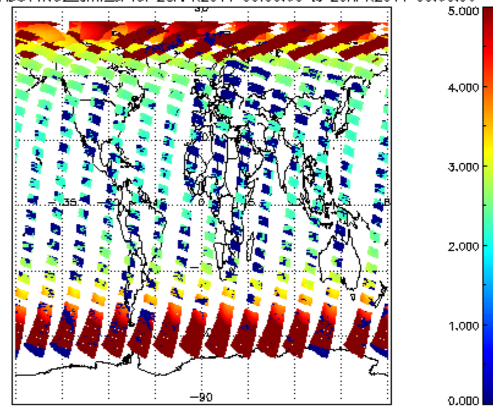
SCIOL2P_NADUV1NO2_amf_sl for 28APR2011 00:00:00 to 29APR2011 00:00:00
