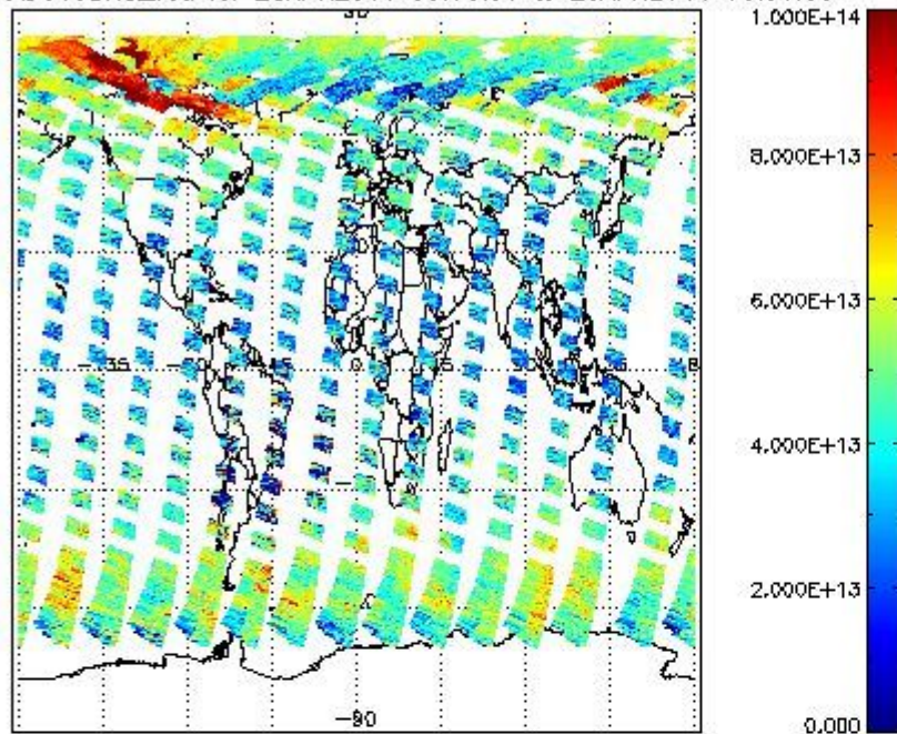
SCIOL2P_NADUV3BRO_vcd for 28APR2011 00:00:00 to 29APR2011 00:00:00
