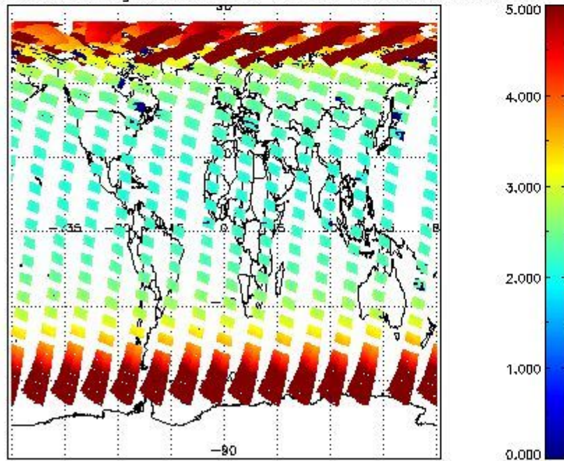
SCIOL2P_NADUV3BRO_amf_gr for 28APR2011 00:00:00 to 29APR2011 00:00:00
