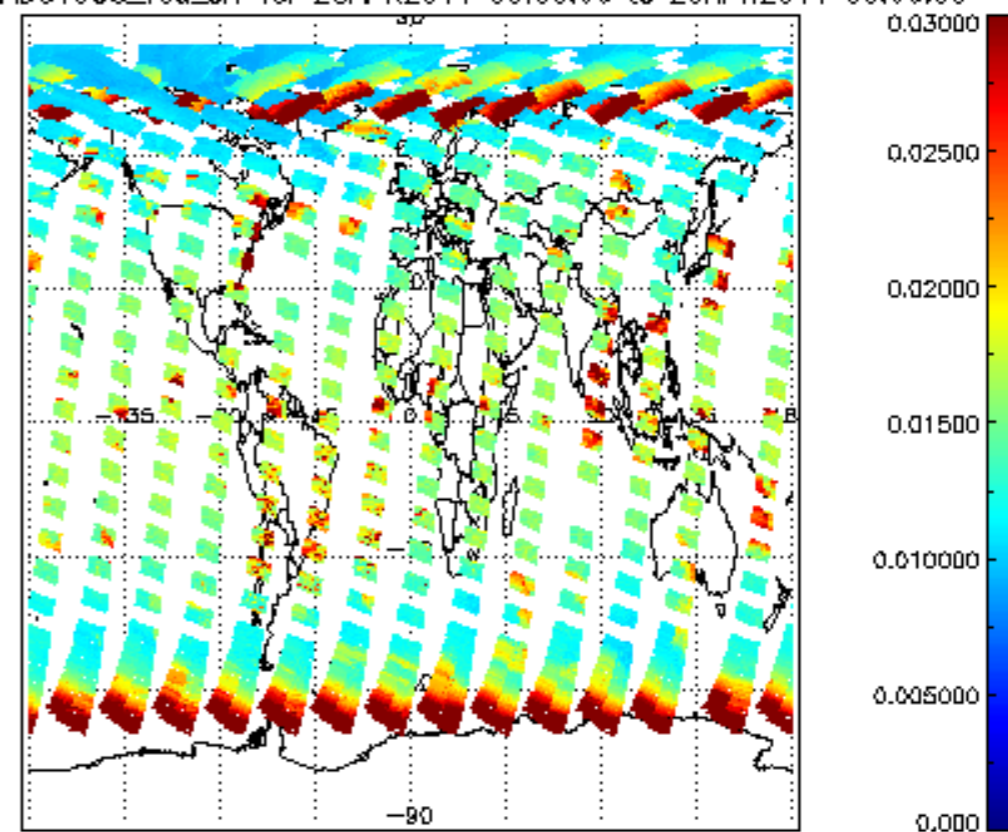
SCIOL2P_NADUV003_vcd_err for 28APR2011 00:00:00 to 29APR2011 00:00:00
