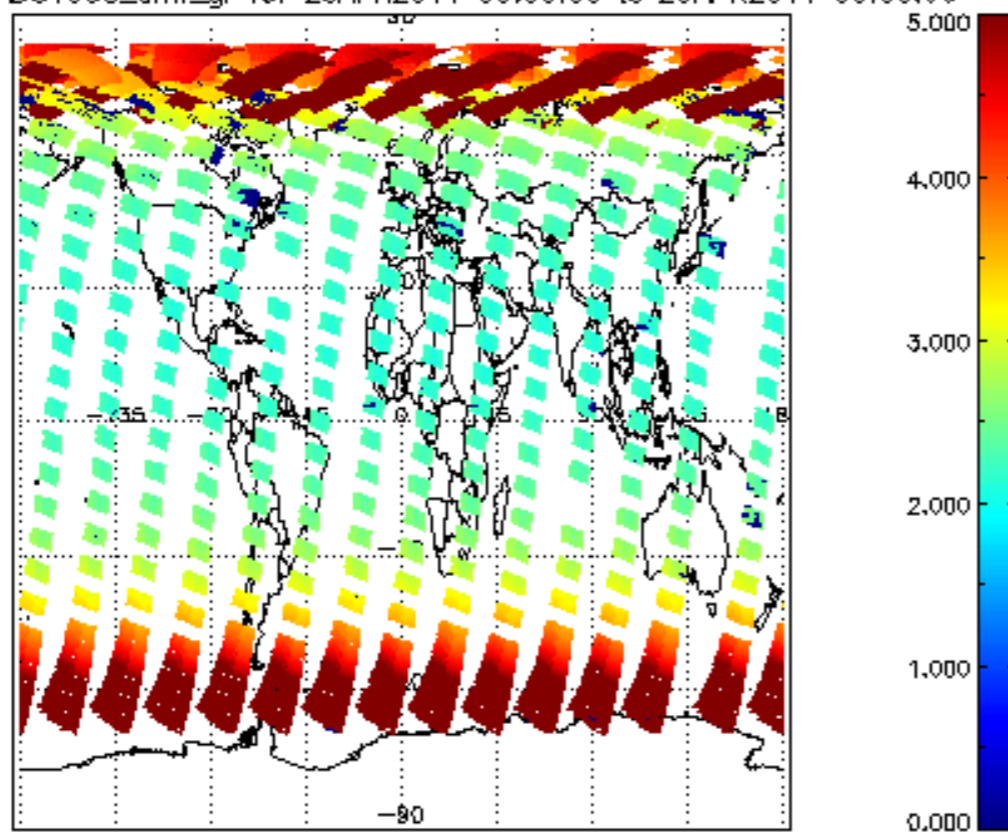
SCIOL2P_NADUV003_amf_gr for 28APR2011 00:00:00 to 29APR2011 00:00:00
