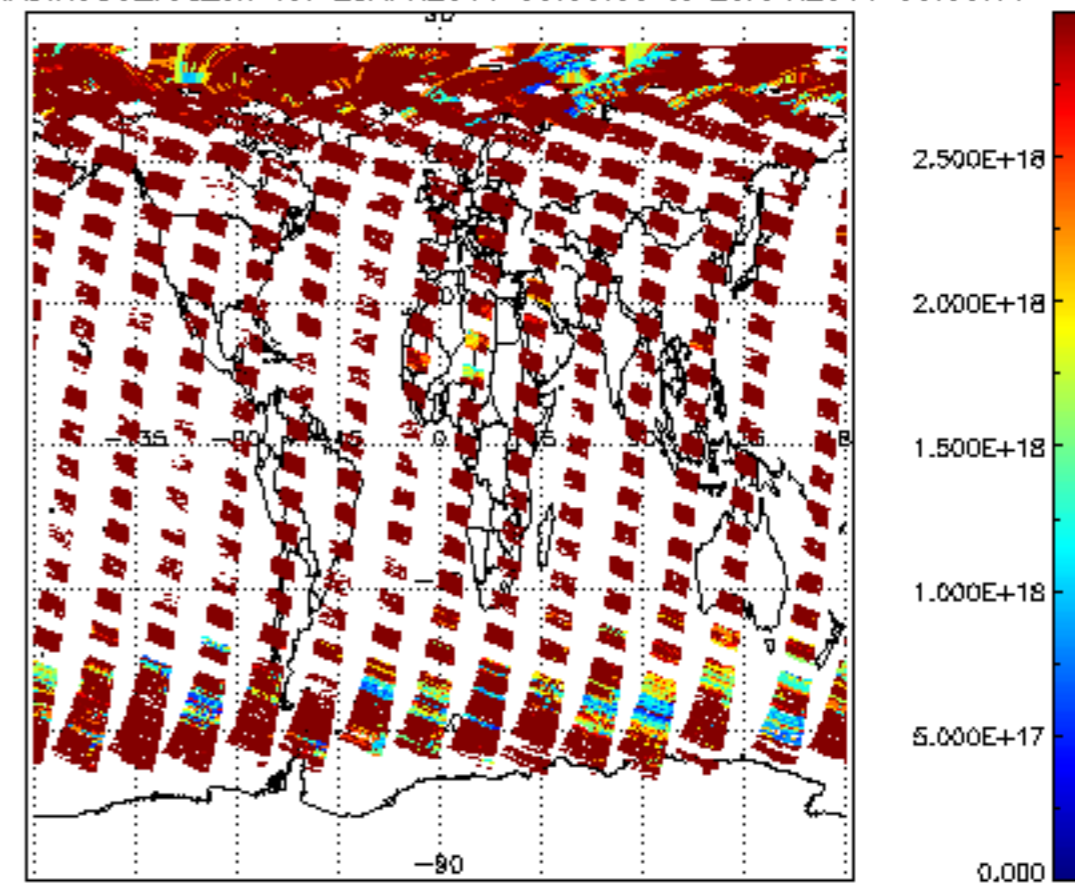
SCIOL2P_NADIR3CO_vcd_err for 28APR2011 00:00:00 to 29APR2011 00:00:00
