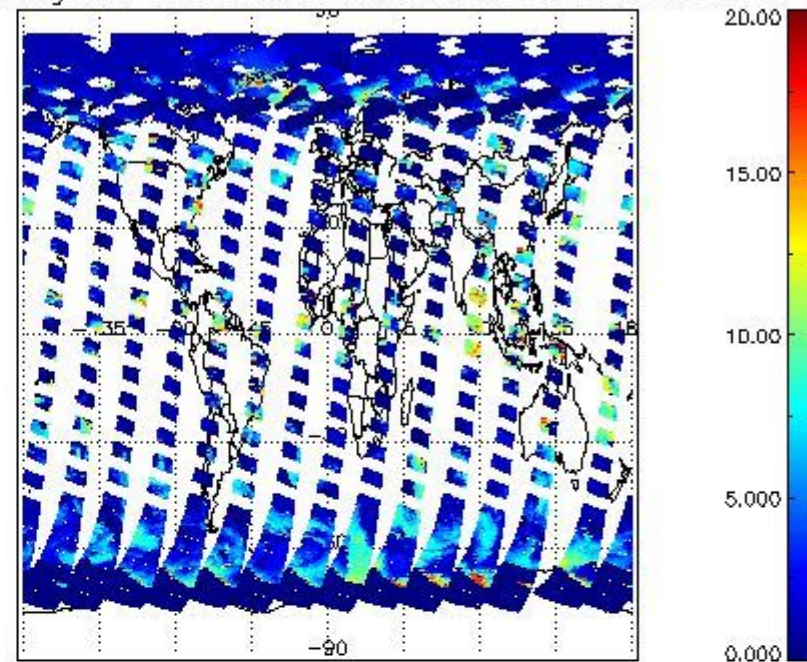
cL_top_height for 28APR2011 00:00:00 to 29APR2011 00:00:00
