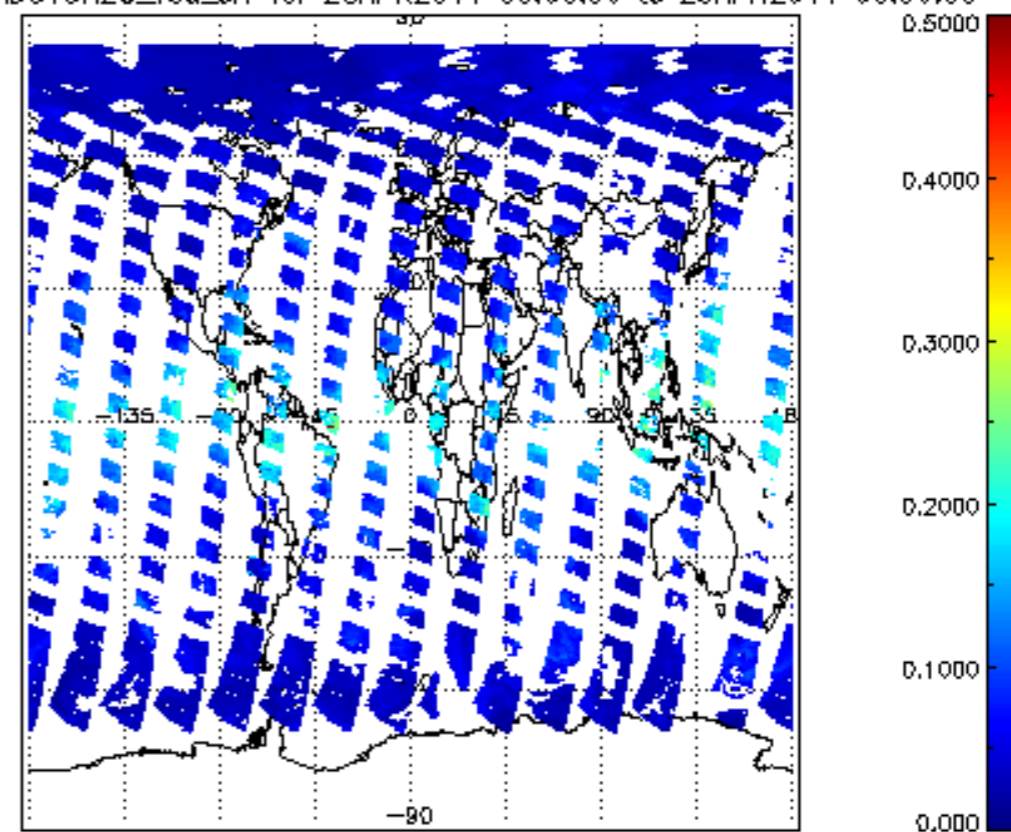
SCIOL2P_NADUV8H2O_vcd_err for 28APR2011 00:00:00 to 29APR2011 00:00:00
