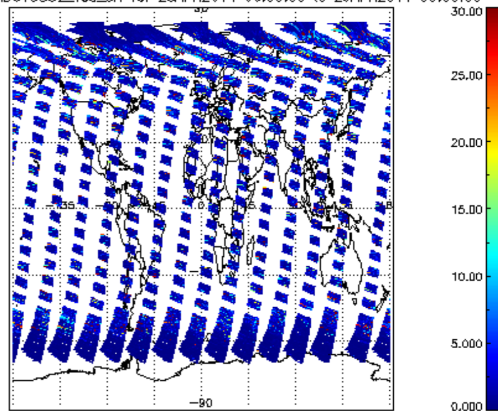
SCIOL2P_NADUV5S02_vcd_err for 28APR2011 00:00:00 to 29APR2011 00:00:00
