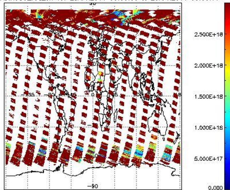
SCIO2P_NADIR3CO_vcd_err for 28APR2011 00:00:00 to 29APR2011 00:00:00
