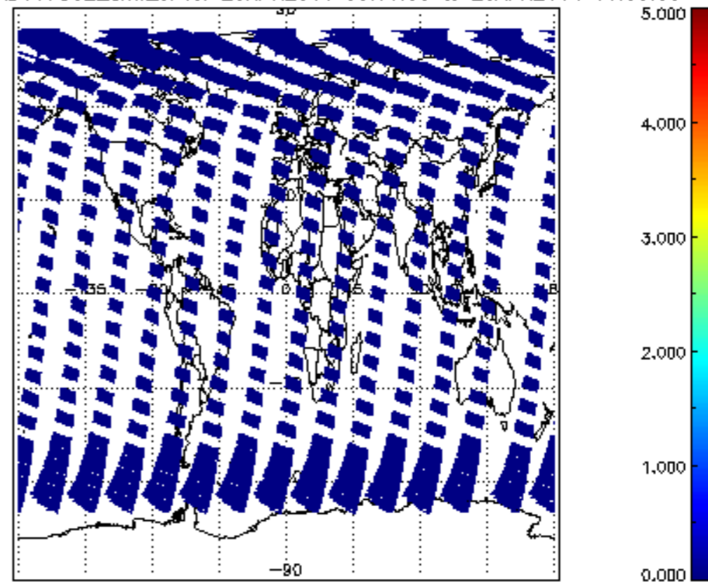
SCIOL2P_NADUV7S02_amf_cl for 28APR2011 00:00:00 to 29APR2011 00:00:00
