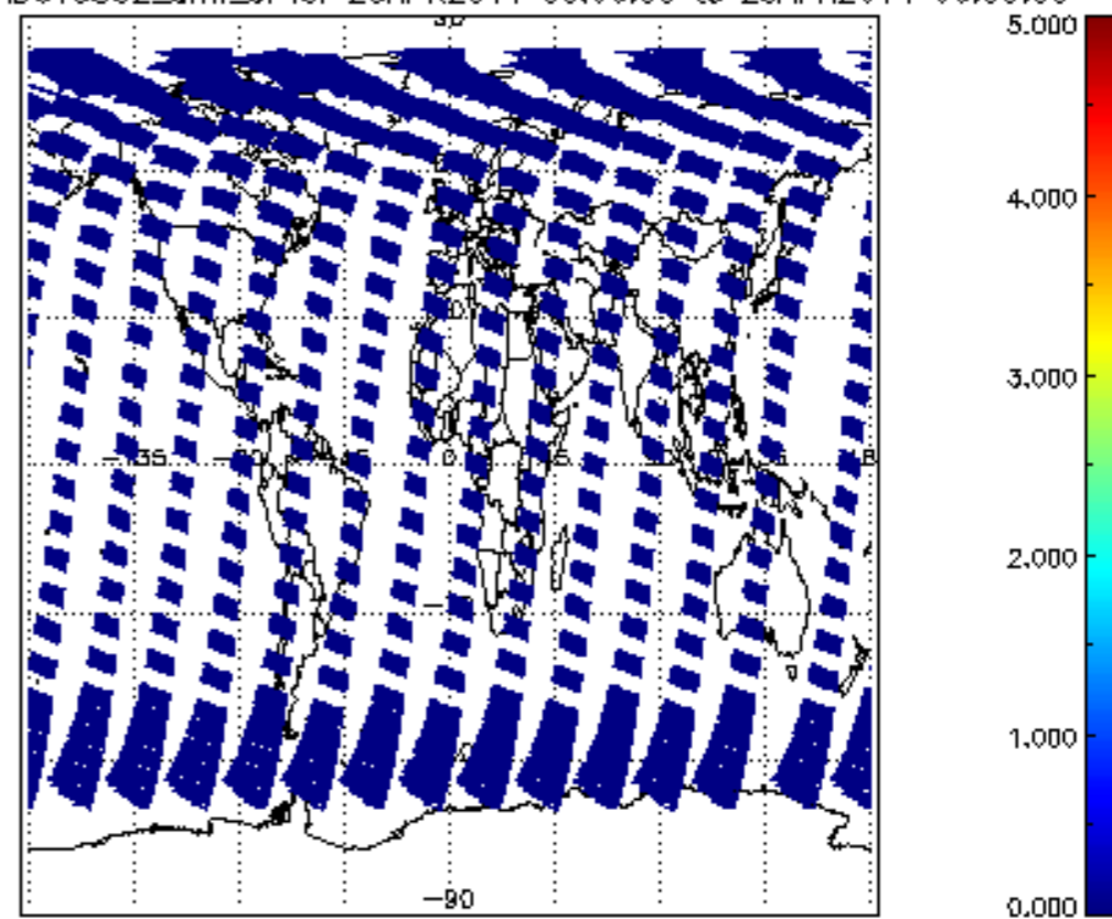
SCIOL2P_NADUV5S02_amf_cl for 28APR2011 00:00:00 to 29APR2011 00:00:00
