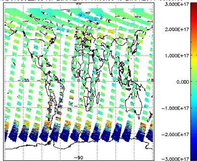
SCIOL2P_NADUV5S02_vcd for 28APR2011 00:00:00 to 29APR2011 00:00:00
