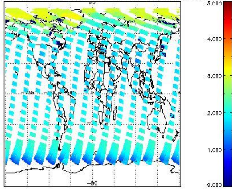
SCIOL2P_NADUV7S02_amf_gr for 28APR2011 00:00:00 to 29APR2011 00:00:00
