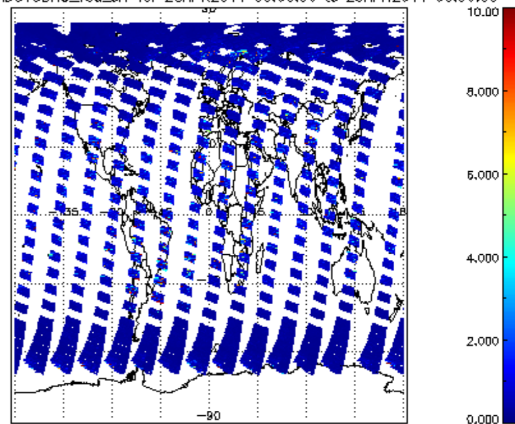
SCIOL2P_NADUV3BRO_vcd_err for 28APR2011 00:00:00 to 29APR2011 00:00:00
