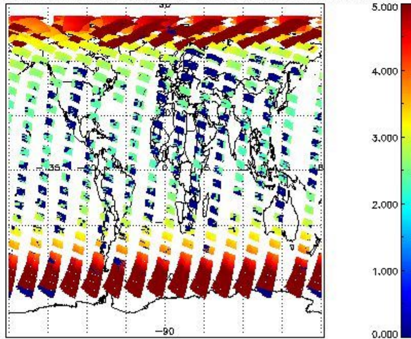
SCIOL2P_NADUV003_amf_cl for 28APR2011 00:00:00 to 29APR2011 00:00:00
