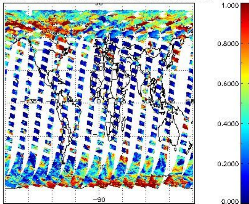
cL_frac for 28APR2011 00:00:00 to 29APR2011 00:00:00
