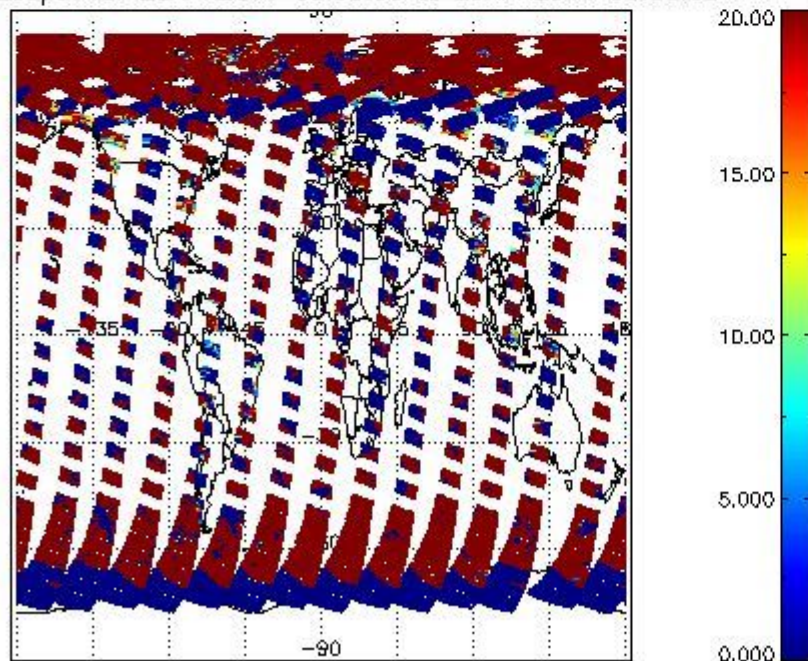
cL_opt_depth for 28APR2011 00:00:00 to 29APR2011 00:00:00
