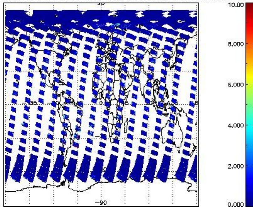
SCIOL2P_NADUV3BRO_vcd_err for 28APR2011 00:00:00 to 29APR2011 00:00:00
