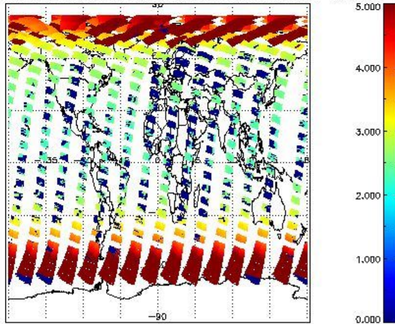
SCIOL2P_NADUV3BRO_amf_cl for 28APR2011 00:00:00 to 29APR2011 00:00:00
