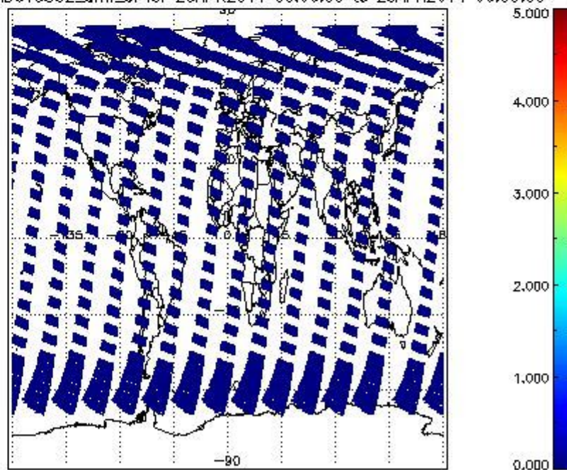
SCIOL2P_NADUV5S02_amf_cl for 28APR2011 00:00:00 to 29APR2011 00:00:00
