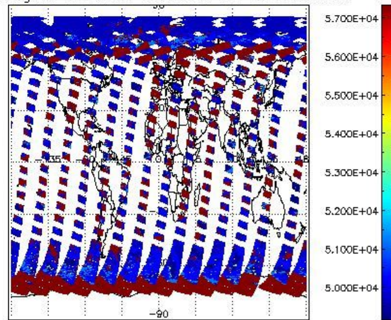
cloud_flags for 28APR2011 00:00:00 to 29APR2011 00:00:00
