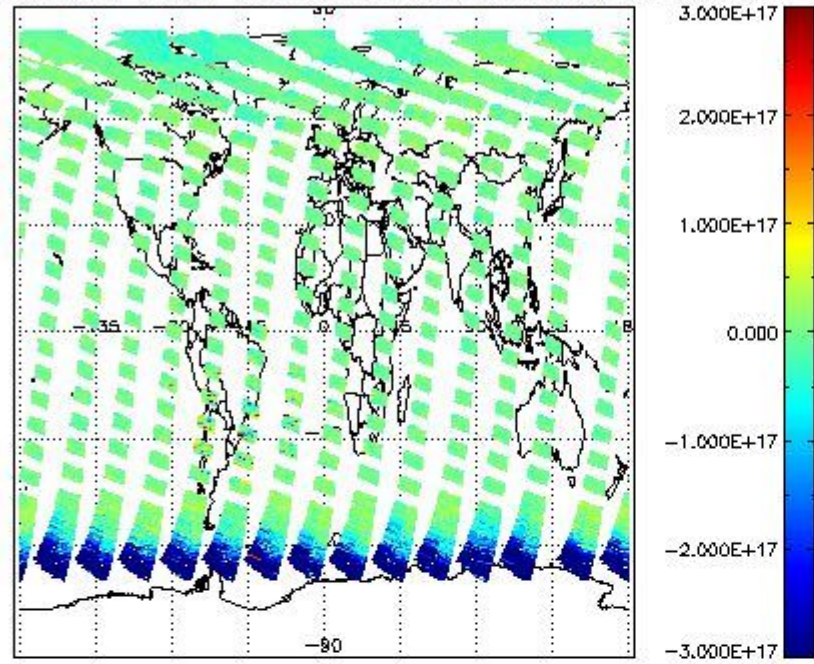
SCIOL2P_NADUV7S02_vcd for 28APR2011 00:00:00 to 29APR2011 00:00:00
