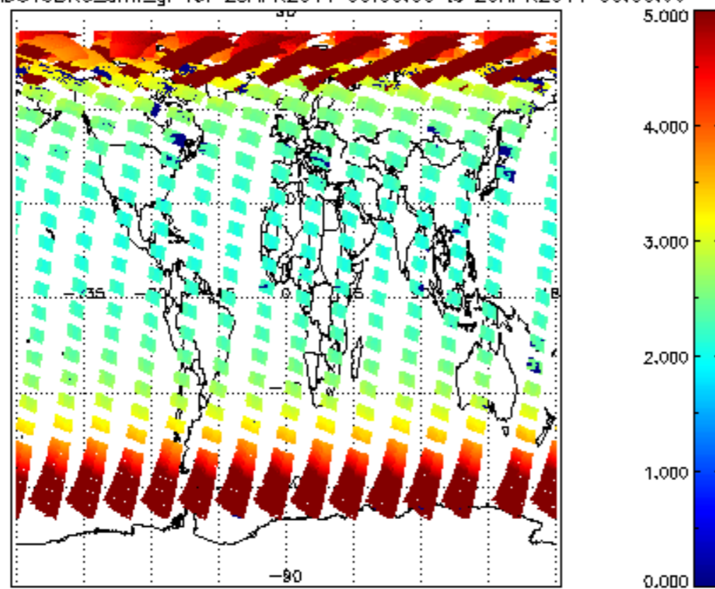
SCIOL2P_NADUV3BRO_amf_gr for 28APR2011 00:00:00 to 29APR2011 00:00:00
