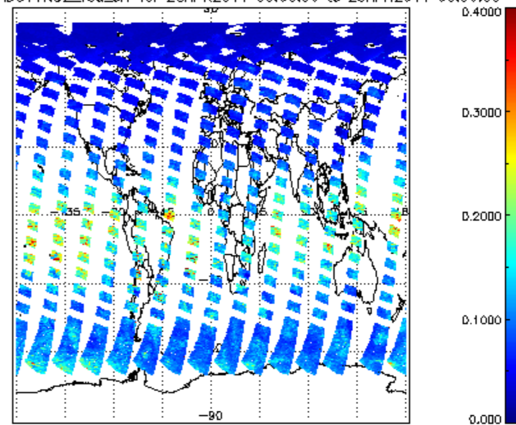
SCIOL2P_NADUV1NO2_vcd_err for 28APR2011 00:00:00 to 29APR2011 00:00:00
