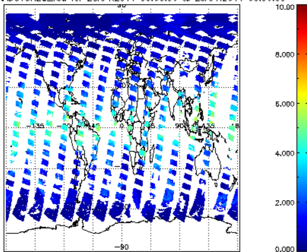
SCIOL2P_NADUV8H2O_vcd for 28APR2011 00:00:00 to 29APR2011 00:00:00
