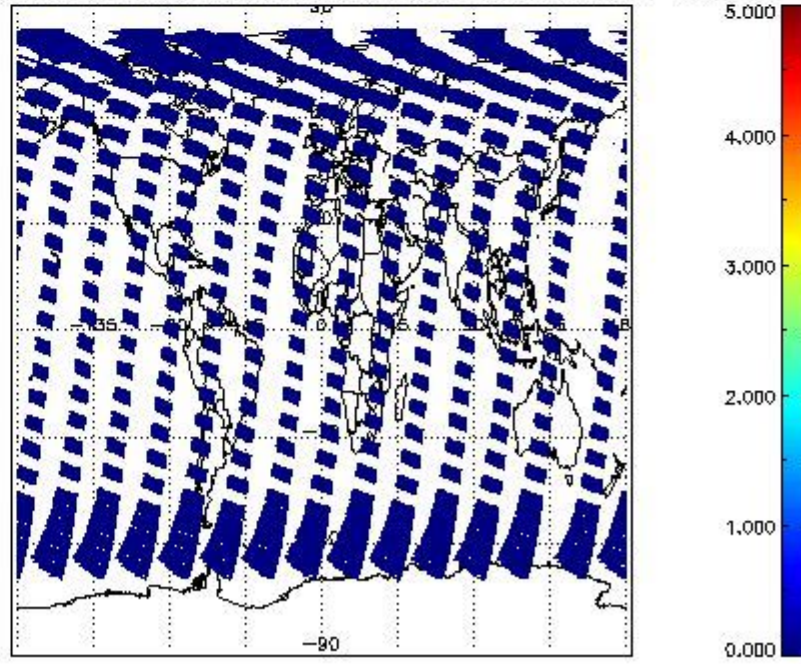
SCIOL2P_NADUV7S02_amf_cl for 28APR2011 00:00:00 to 29APR2011 00:00:00
