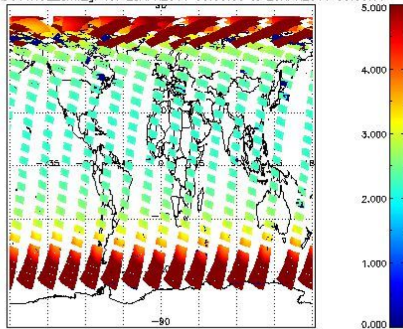
SCIOL2P_NADUV1NO2_amf_gr for 28APR2011 00:00:00 to 29APR2011 00:00:00
