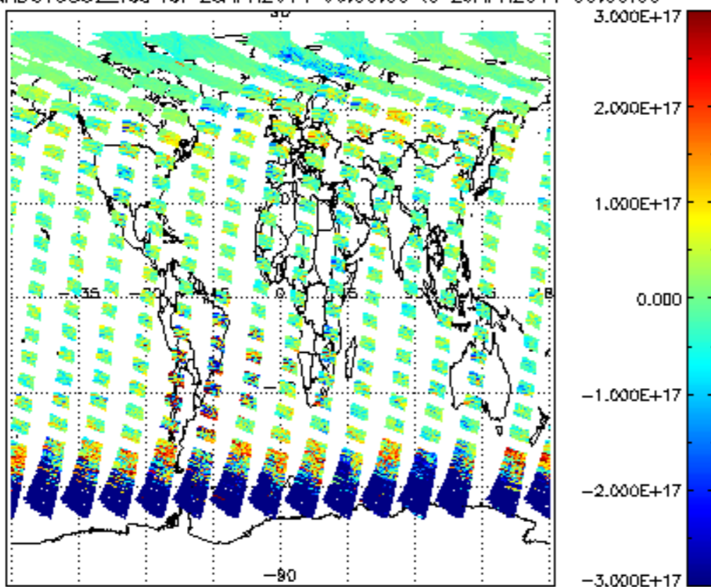
SCIOL2P_NADUV5S02_vcd for 28APR2011 00:00:00 to 29APR2011 00:00:00
