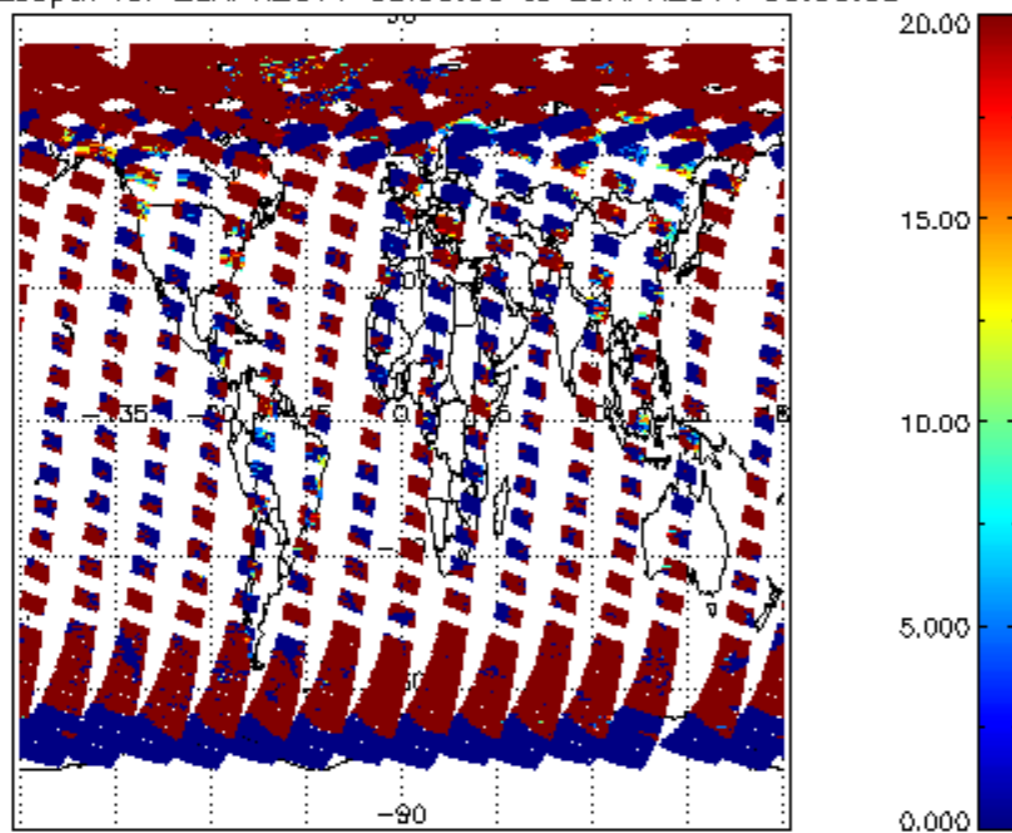
cl_opt_depth for 28APR2011 00:00:00 to 29APR2011 00:00:00
