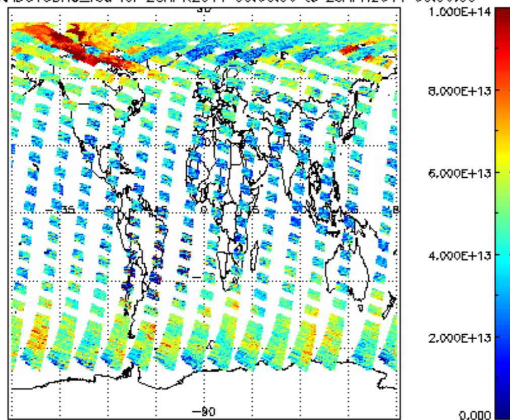
SCIOL2P_NADUV3BRO_vcd for 28APR2011 00:00:00 to 29APR2011 00:00:00
