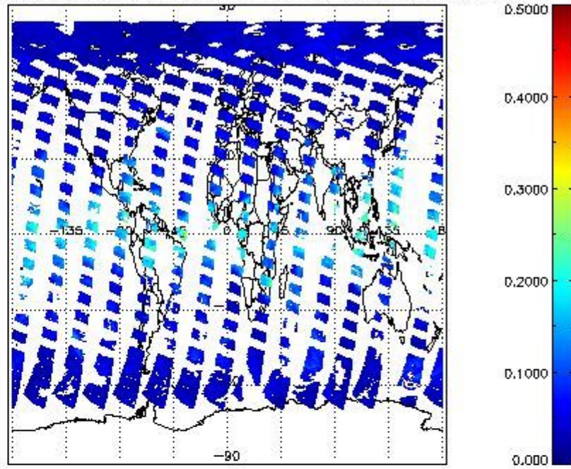
SCIOL2P_NADUV6H2O_vcd_err for 28APR2011 00:00:00 to 29APR2011 00:00:00
