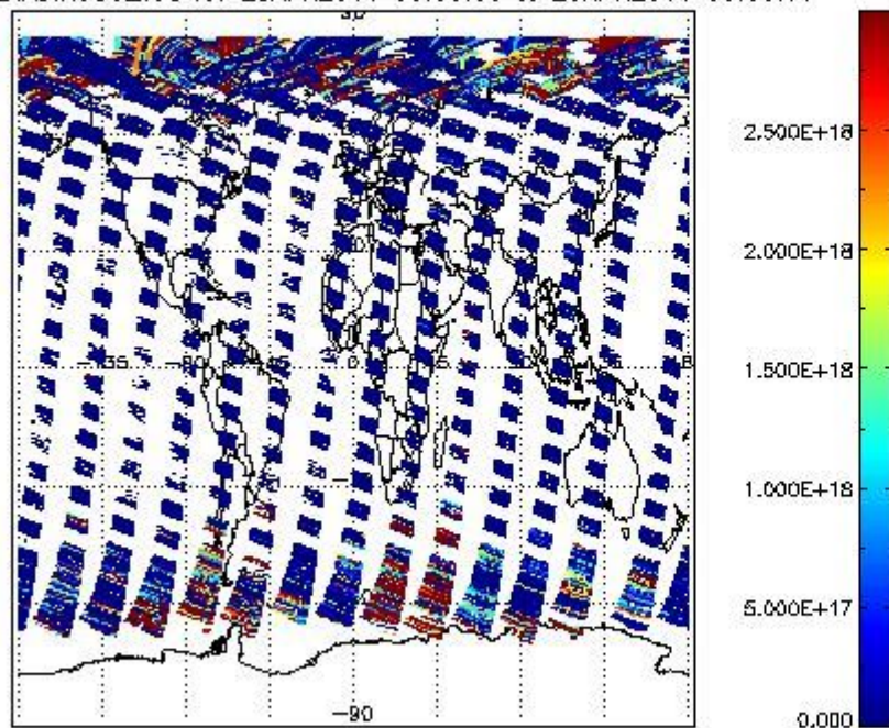
SCIO2P_NADIR3CO_vcd for 28APR2011 00:00:00 to 29APR2011 00:00:00
