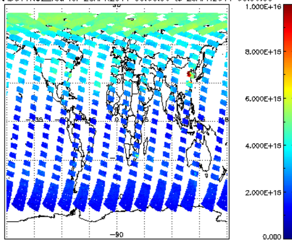
SCIOL2P_NADUV1NO2_vcd for 28APR2011 00:00:00 to 29APR2011 00:00:00
