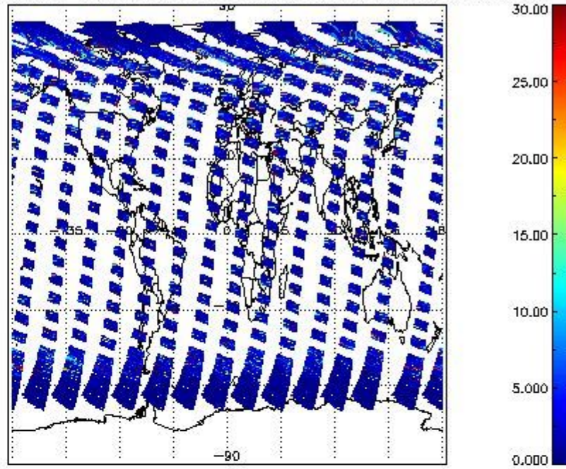
SCIOL2P_NADUV7S02_vcd_err for 28APR2011 00:00:00 to 29APR2011 00:00:00
