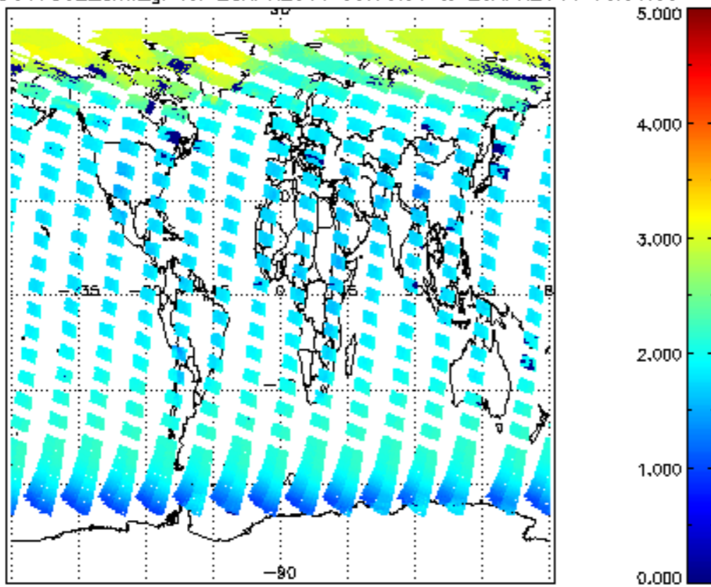
SCIOL2P_NADUV7S02_amf_gr for 28APR2011 00:00:00 to 29APR2011 00:00:00
