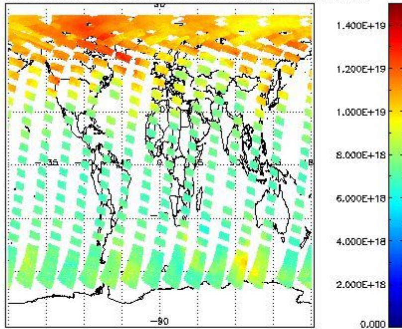
SCIOL2P_NADUV003_vcd for 28APR2011 00:00:00 to 29APR2011 00:00:00
