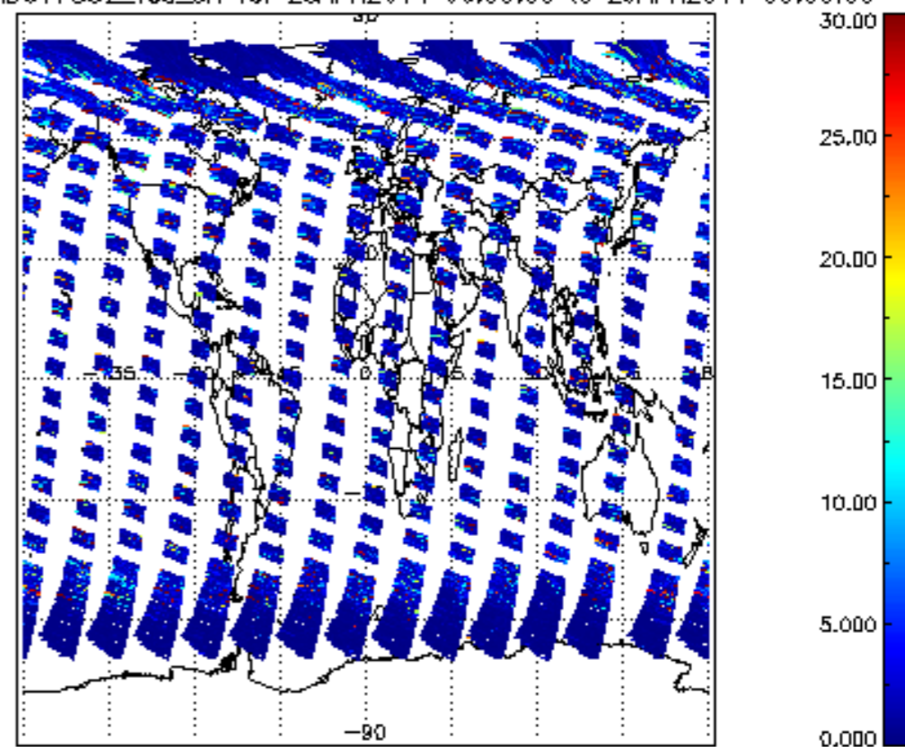
SCIOL2P_NADUV7S02_vcd_err for 28APR2011 00:00:00 to 29APR2011 00:00:00
