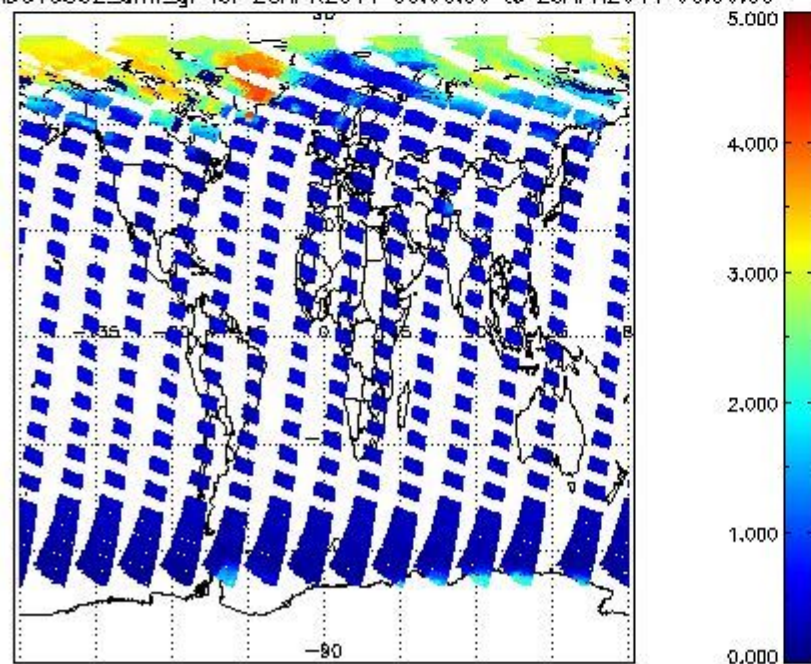
SCIOL2P_NADUV5S02_amf_gr for 28APR2011 00:00:00 to 29APR2011 00:00:00
