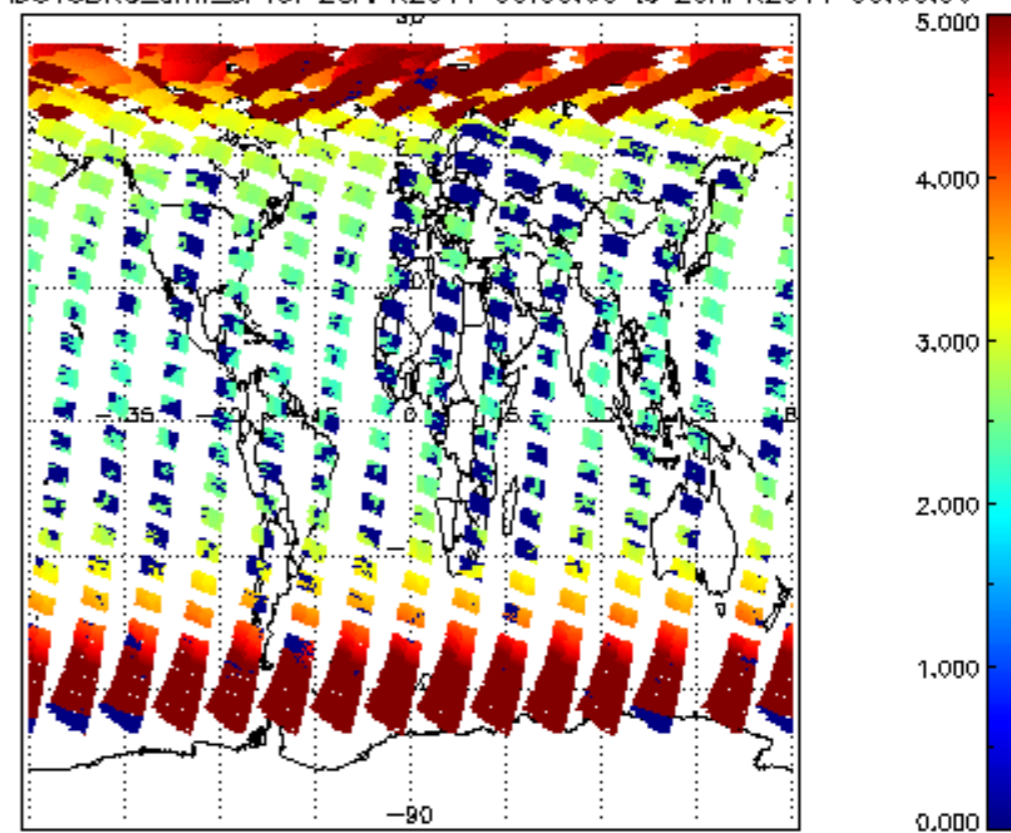
SCIOL2P_NADUV3BRO_amf_cl for 28APR2011 00:00:00 to 29APR2011 00:00:00
