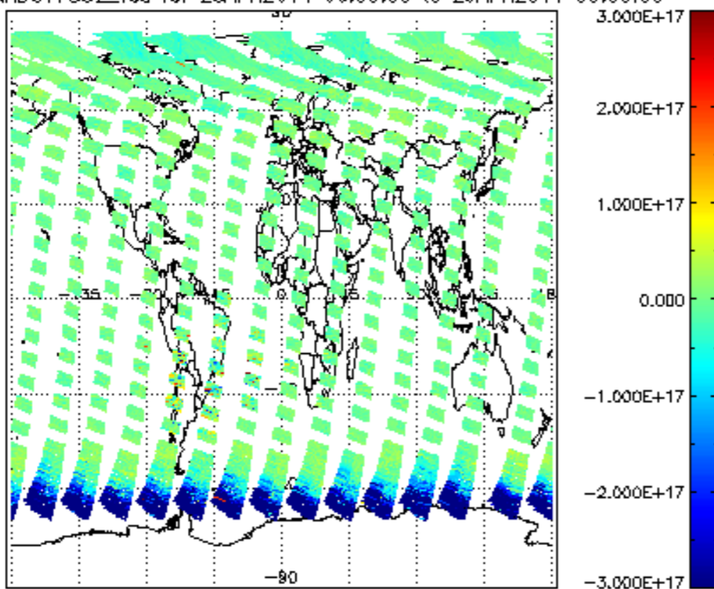
SCIOL2P_NADUV7S02_vcd for 28APR2011 00:00:00 to 29APR2011 00:00:00
