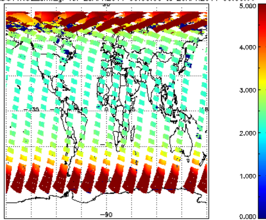
SCIOL2P_NADUV1NO2_amf_gr for 28APR2011 00:00:00 to 29APR2011 00:00:00
