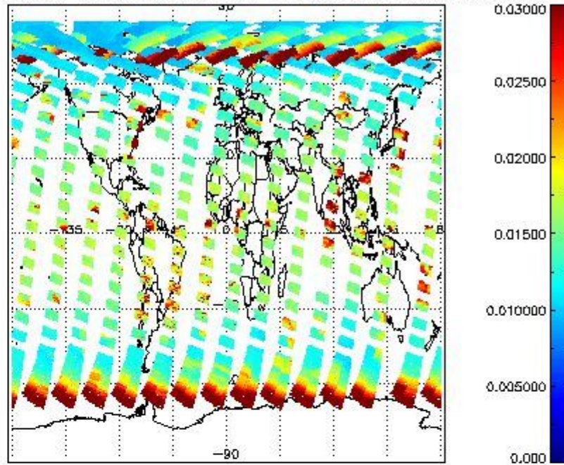
SCIOL2P_NADUV003_vcd_err for 28APR2011 00:00:00 to 29APR2011 00:00:00
