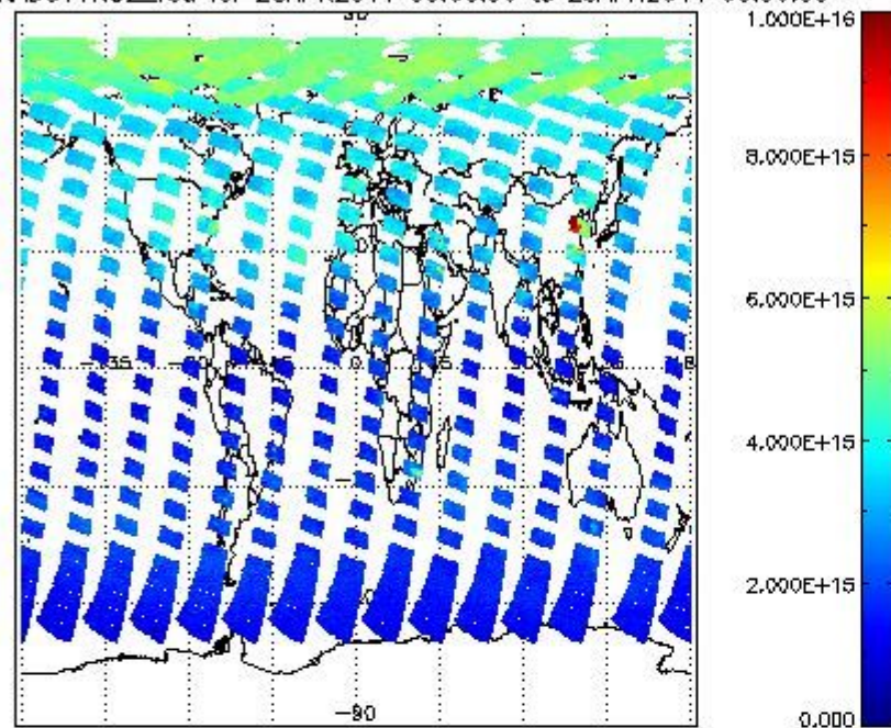
SCIOL2P_NADUV1NO2_vcd for 28APR2011 00:00:00 to 29APR2011 00:00:00
