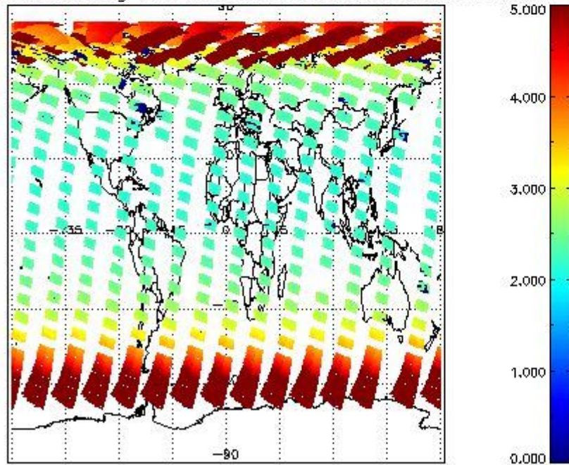
SCIOL2P_NADUV003_amf_gr for 28APR2011 00:00:00 to 29APR2011 00:00:00
