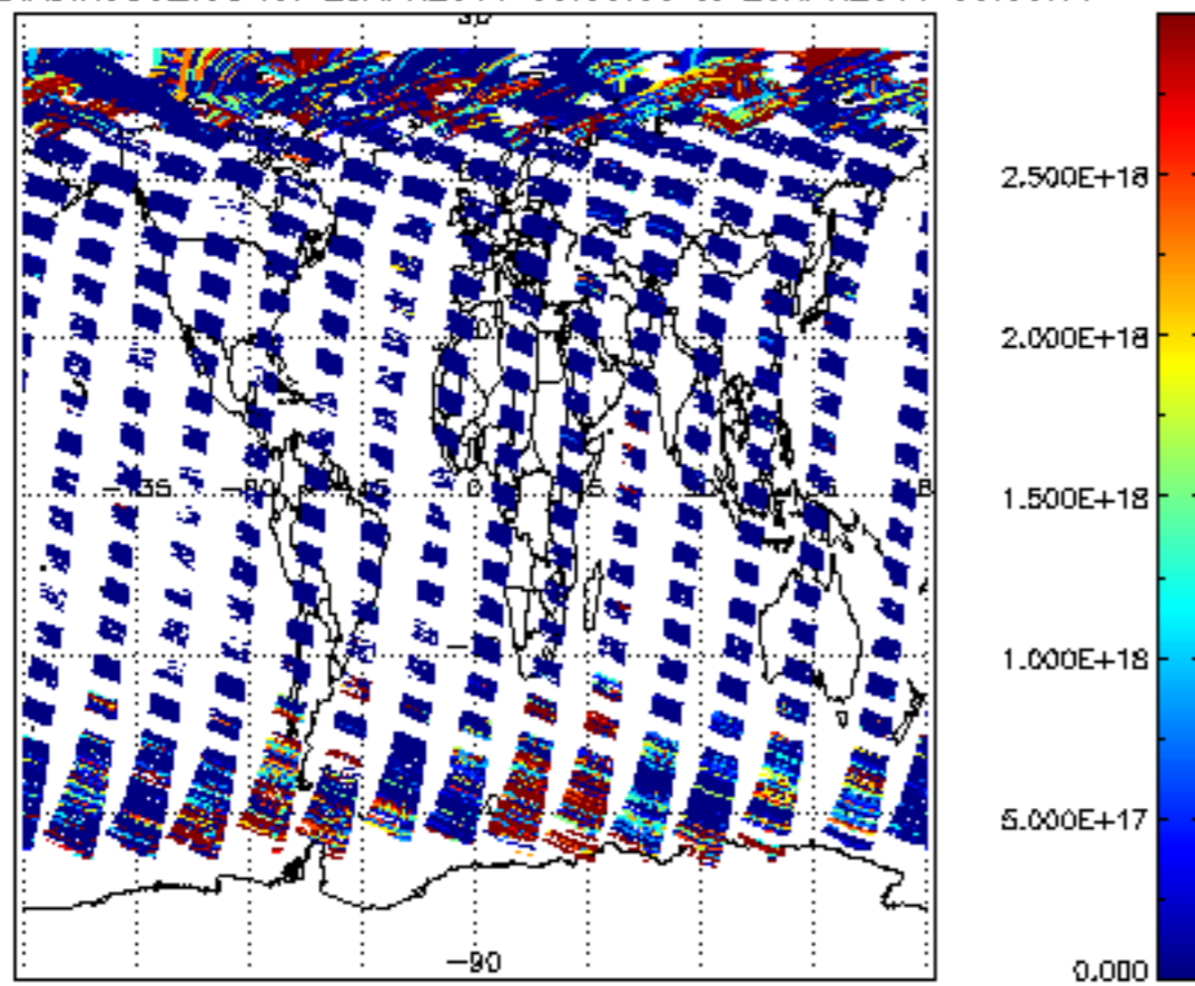
SCIOL2P_NADIR3CO_vcd for 28APR2011 00:00:00 to 29APR2011 00:00:00
