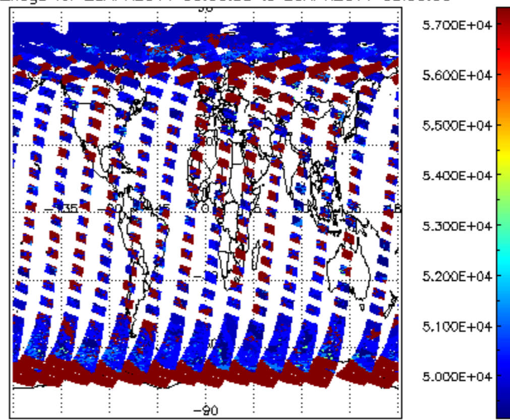
cloud_flags for 28APR2011 00:00:00 to 29APR2011 00:00:00
