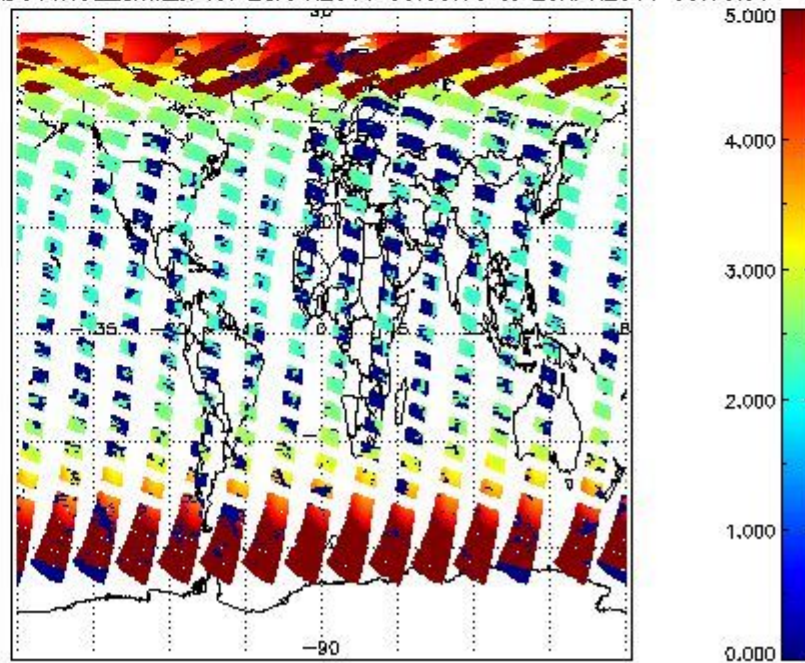
SCIOL2P_NADUV1NO2_amf_cl for 28APR2011 00:00:00 to 29APR2011 00:00:00
