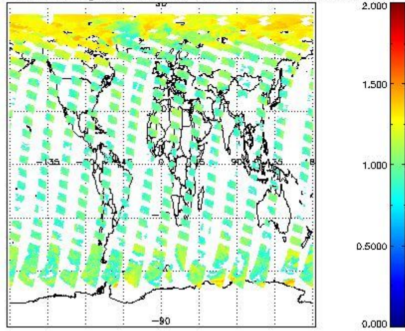
SCIOL2P_NADUV6H2O_arnf_gr for 28APR2011 00:00:00 to 29APR2011 00:00:00
