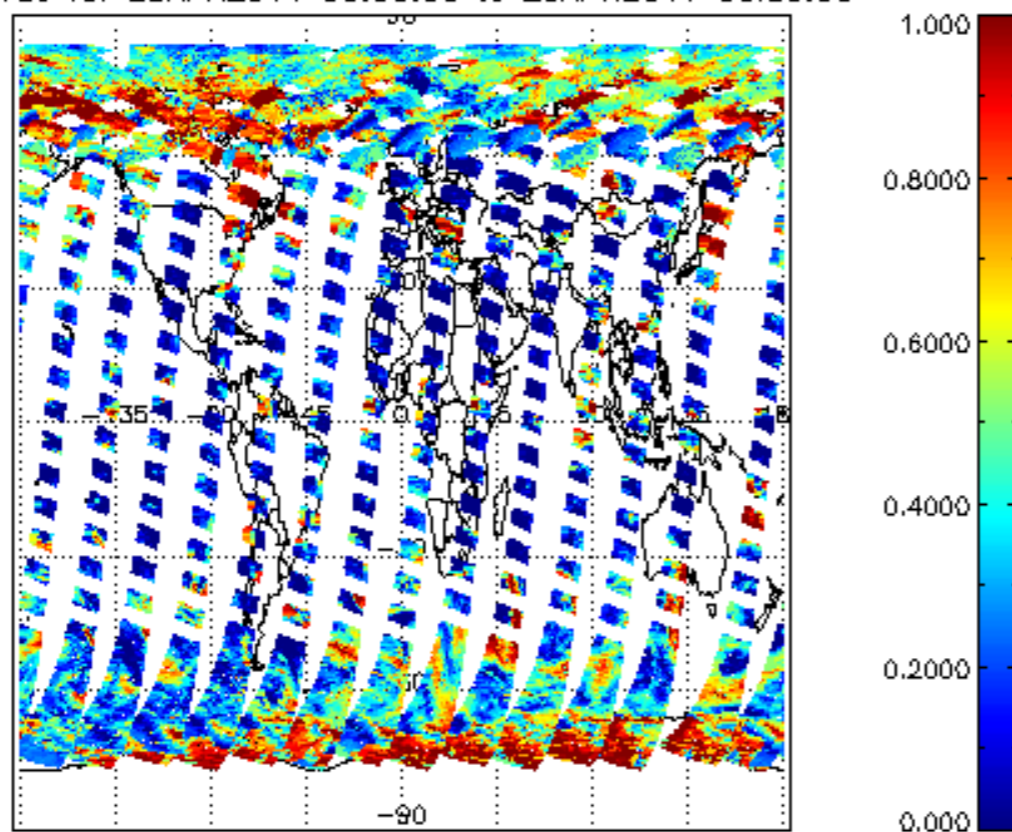
cl_frac for 28APR2011 00:00:00 to 29APR2011 00:00:00
