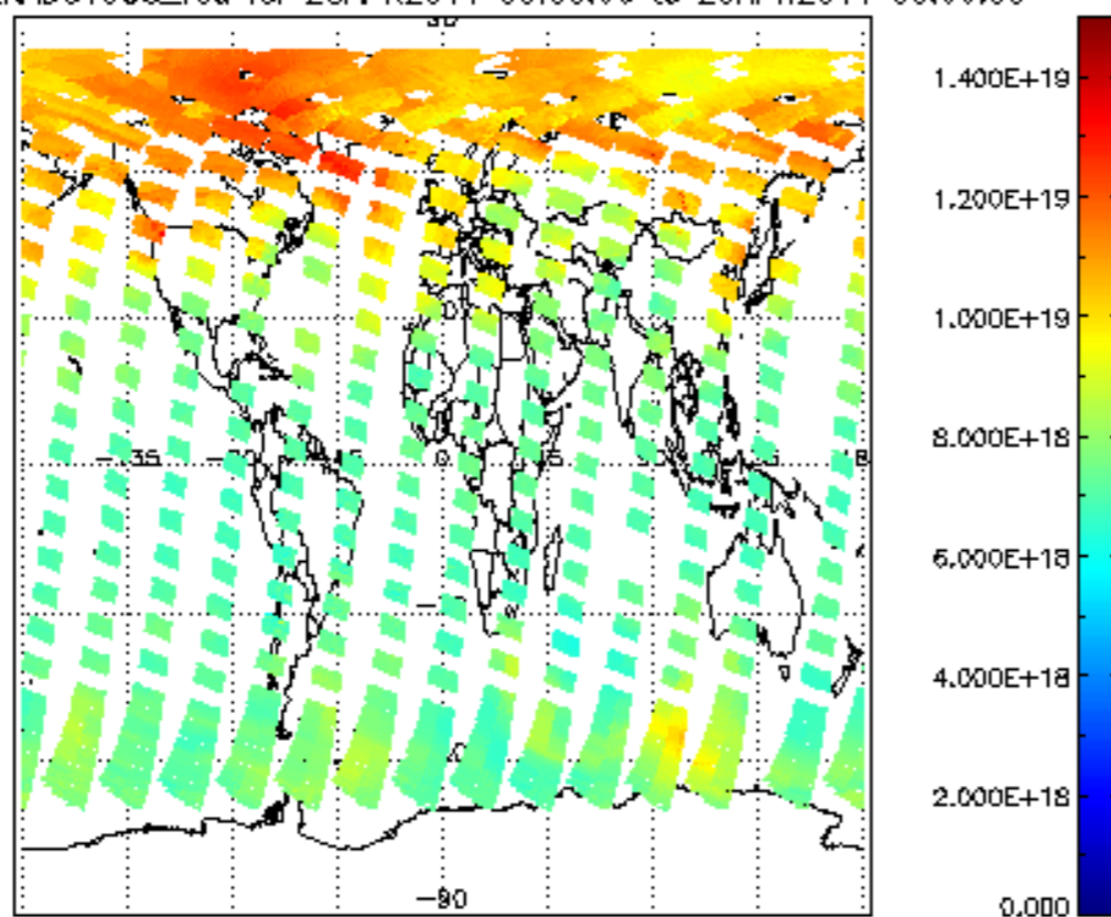
SCIOL2P_NADUV003_vcd for 28APR2011 00:00:00 to 29APR2011 00:00:00
