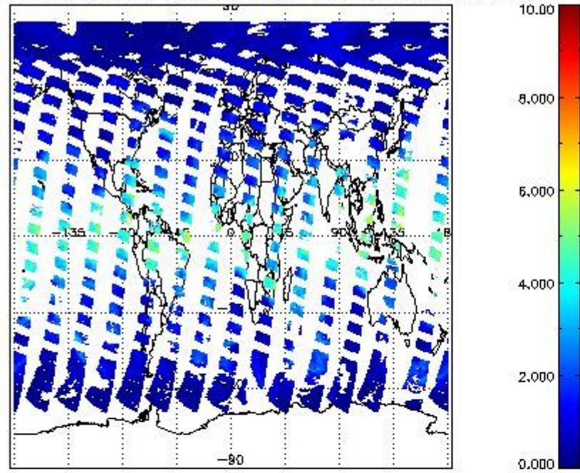
SCIOL2P_NADUV6H2O_vcd for 28APR2011 00:00:00 to 29APR2011 00:00:00
