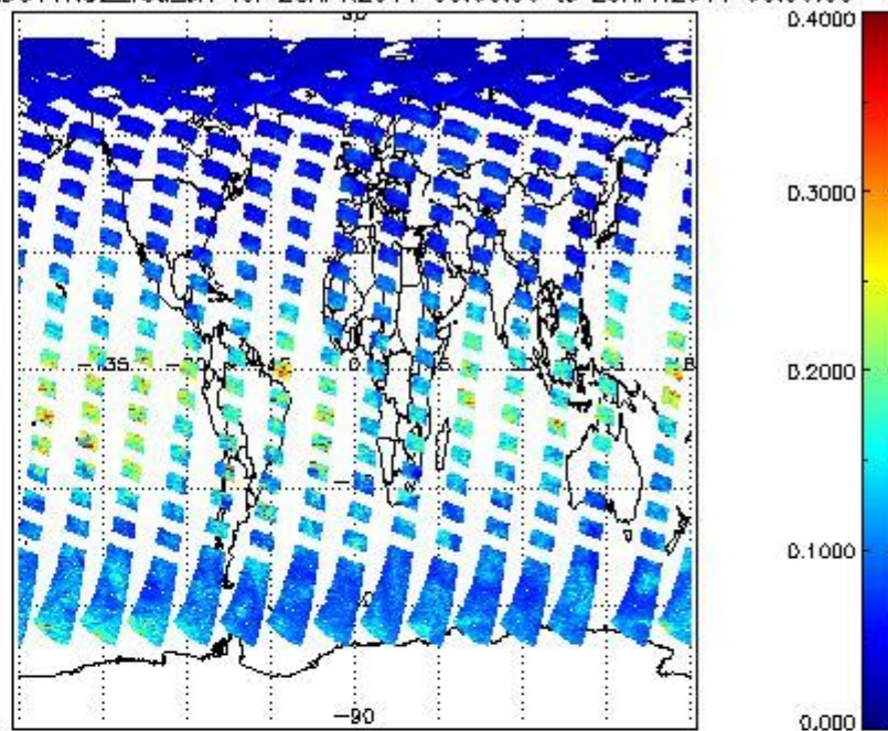
SCIOL2P_NADUV1NO2_vcd_err for 28APR2011 00:00:00 to 29APR2011 00:00:00
