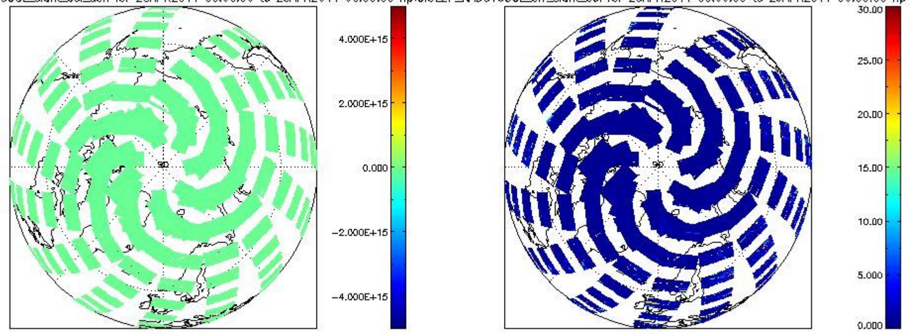
CIOL2P_NADUV6OCLslant_col_den for 28APR2011 00:00:00 to 29APR2011 00:00:00 np; CIOL2P_NADUV6OCLarr_slant_col for 28APR2011 00:00:00 to 29APR2011 00:00:00 np
