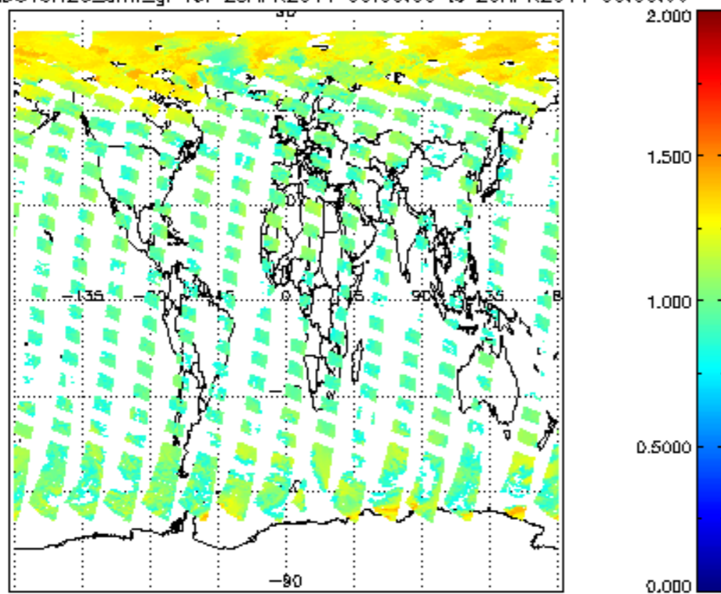
SCIOL2P_NADUV8H2O_amf_gr for 28APR2011 00:00:00 to 29APR2011 00:00:00
