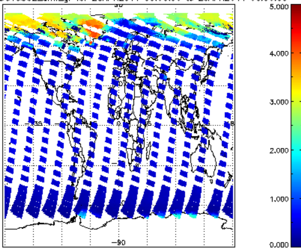
SCIOL2P_NADUV5S02_amf_gr for 28APR2011 00:00:00 to 29APR2011 00:00:00
