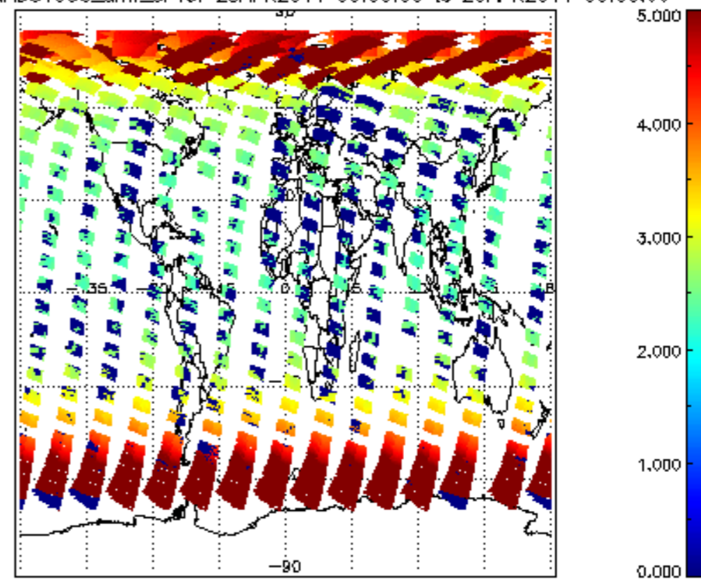
SCIOL2P_NADUV003_amf_cl for 28APR2011 00:00:00 to 29APR2011 00:00:00
