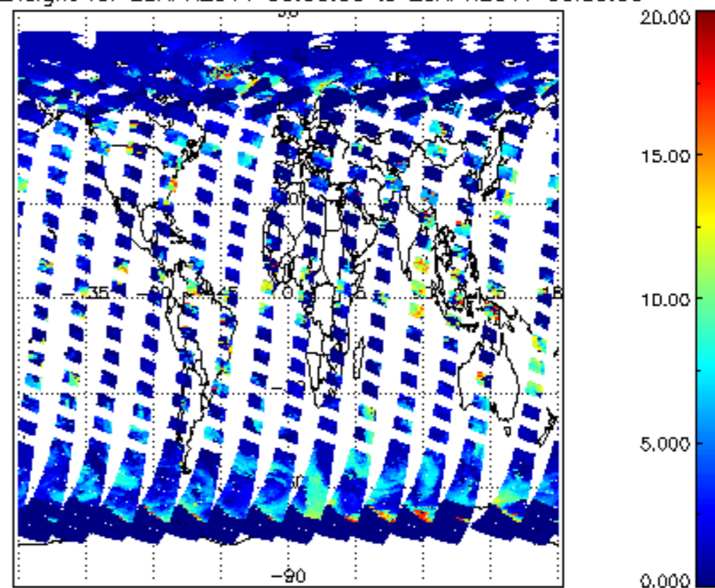
cl_top_height for 28APR2011 00:00:00 to 29APR2011 00:00:00
