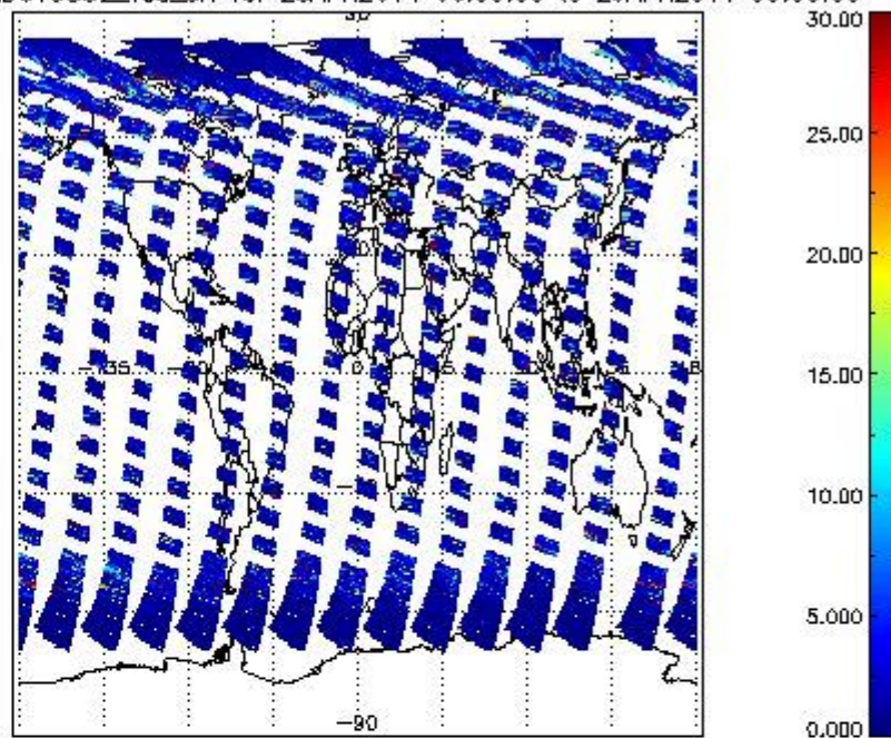
SCIOL2P_NADUV5S02_vcd_err for 28APR2011 00:00:00 to 29APR2011 00:00:00
