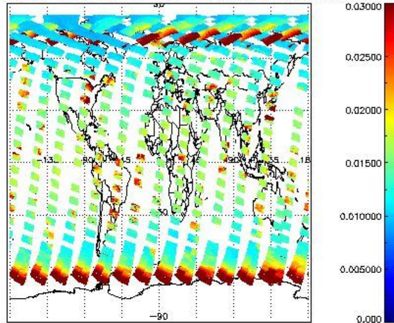
SCIOL2P_NADUV003_vcd_err for 27APR2011 00:00:00 to 28APR2011 00:00:00
