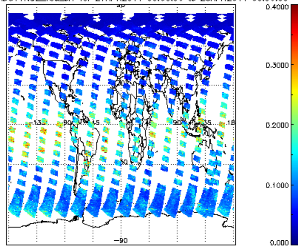
SCIOL2P_NADUV1NO2_vcd_err for 27APR2011 00:00:00 to 28APR2011 00:00:00
