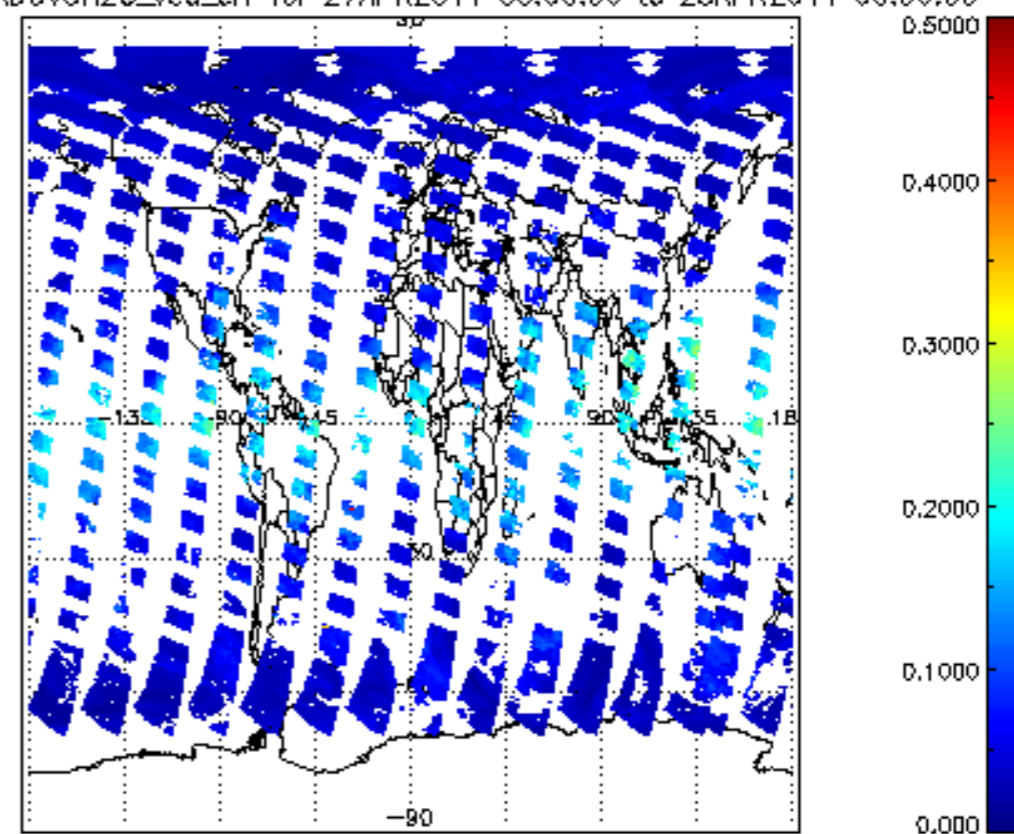
SCIOL2P_NADUV8H2O_vcd_err for 27APR2011 00:00:00 to 28APR2011 00:00:00
