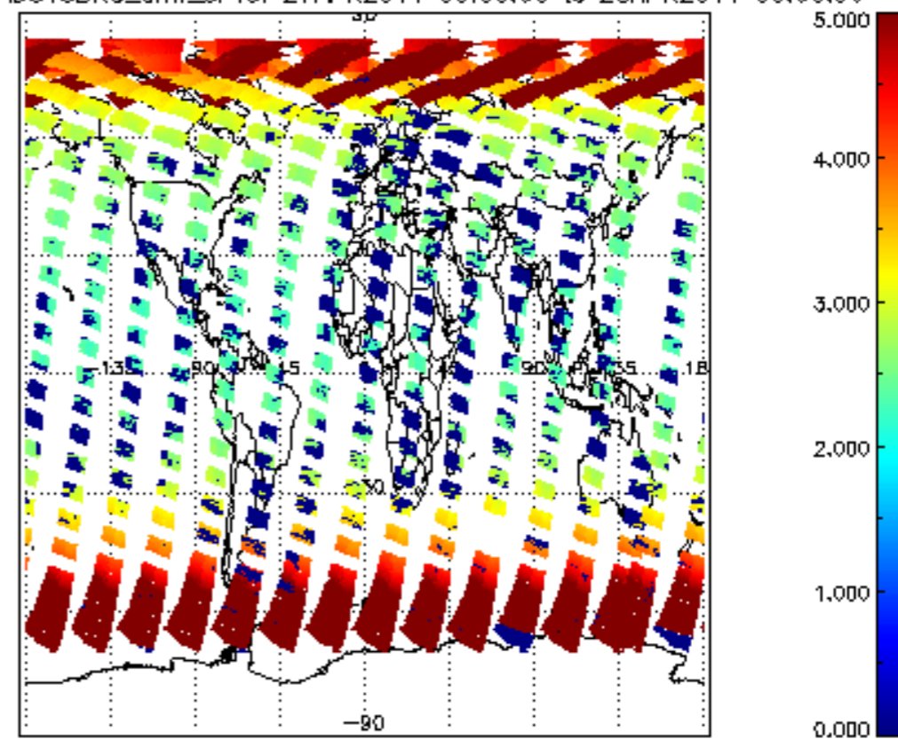
SCIOL2P_NADUV3BRO_amf_sl for 27APR2011 00:00:00 to 28APR2011 00:00:00
