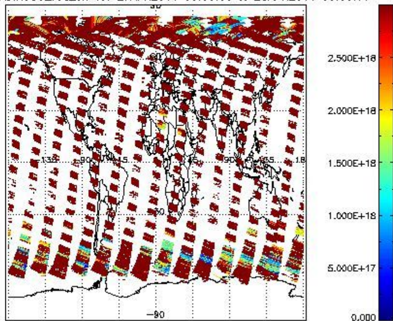
SCIDL2P_NADIR3CO_vcd_err for 27APR2011 00:00:00 to 28APR2011 00:00:00
