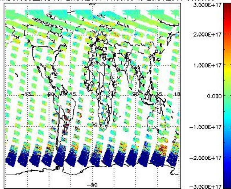
SCIOL2P_NADUV5S02_vcd for 27APR2011 00:00:00 to 28APR2011 00:00:00
