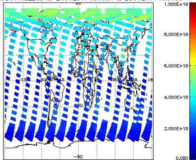
SCIOL2P_NADUV1N02_vcd for 27APR2011 00:00:00 to 28APR2011 00:00:00
