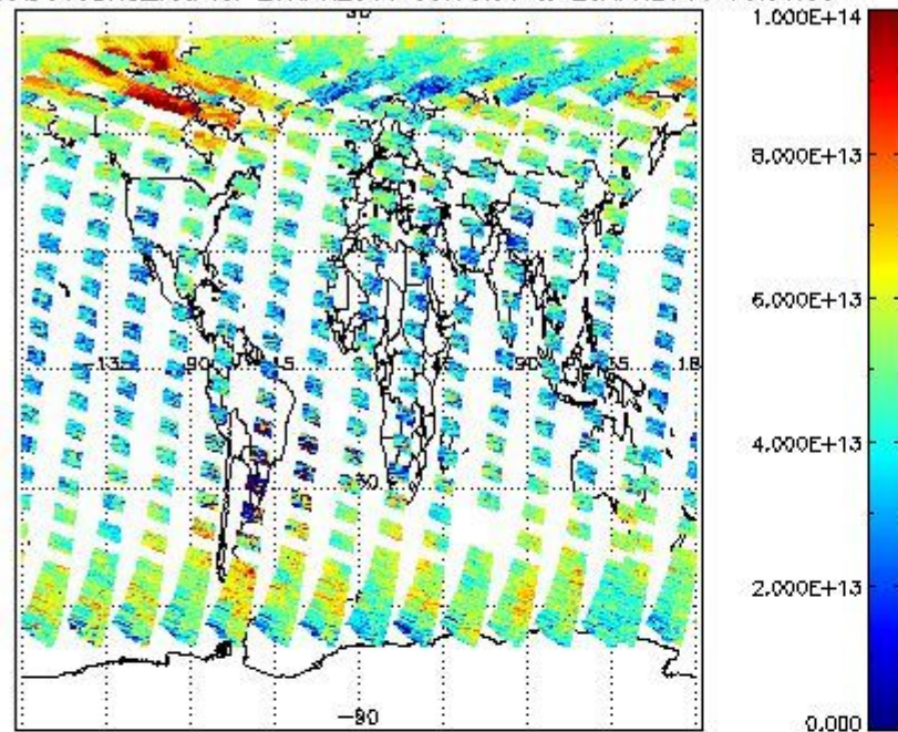
SCIOL2P_NADUV3BRO_vcd for 27APR2011 00:00:00 to 28APR2011 00:00:00
