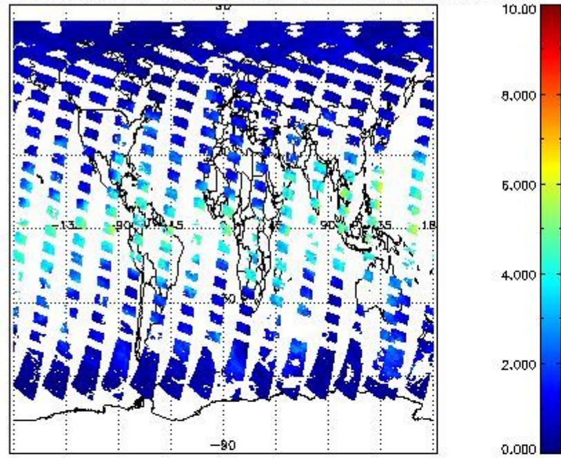
SCIOL2P_NADUV6H2O_vcd for 27APR2011 00:00:00 to 28APR2011 00:00:00
