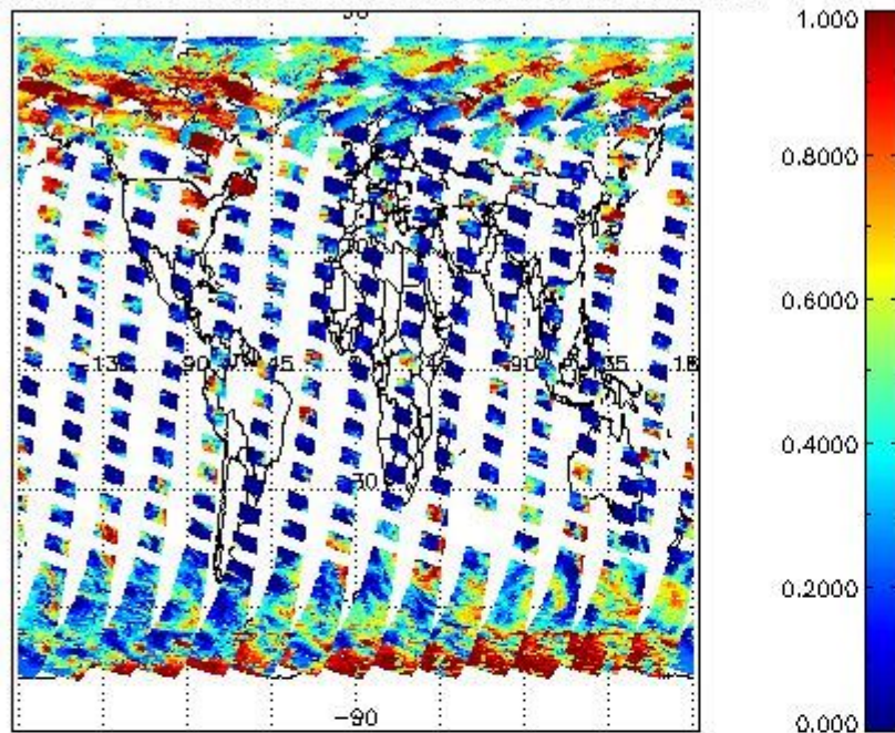
cL_frac for 27APR2011 00:00:00 to 28APR2011 00:00:00
