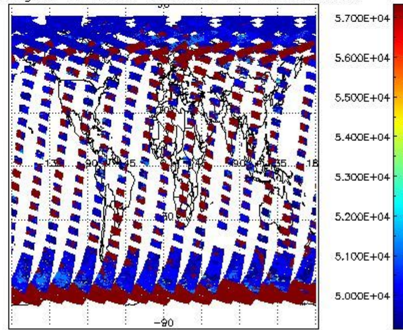
cloud_flags for 27APR2011 00:00:00 to 28APR2011 00:00:00
