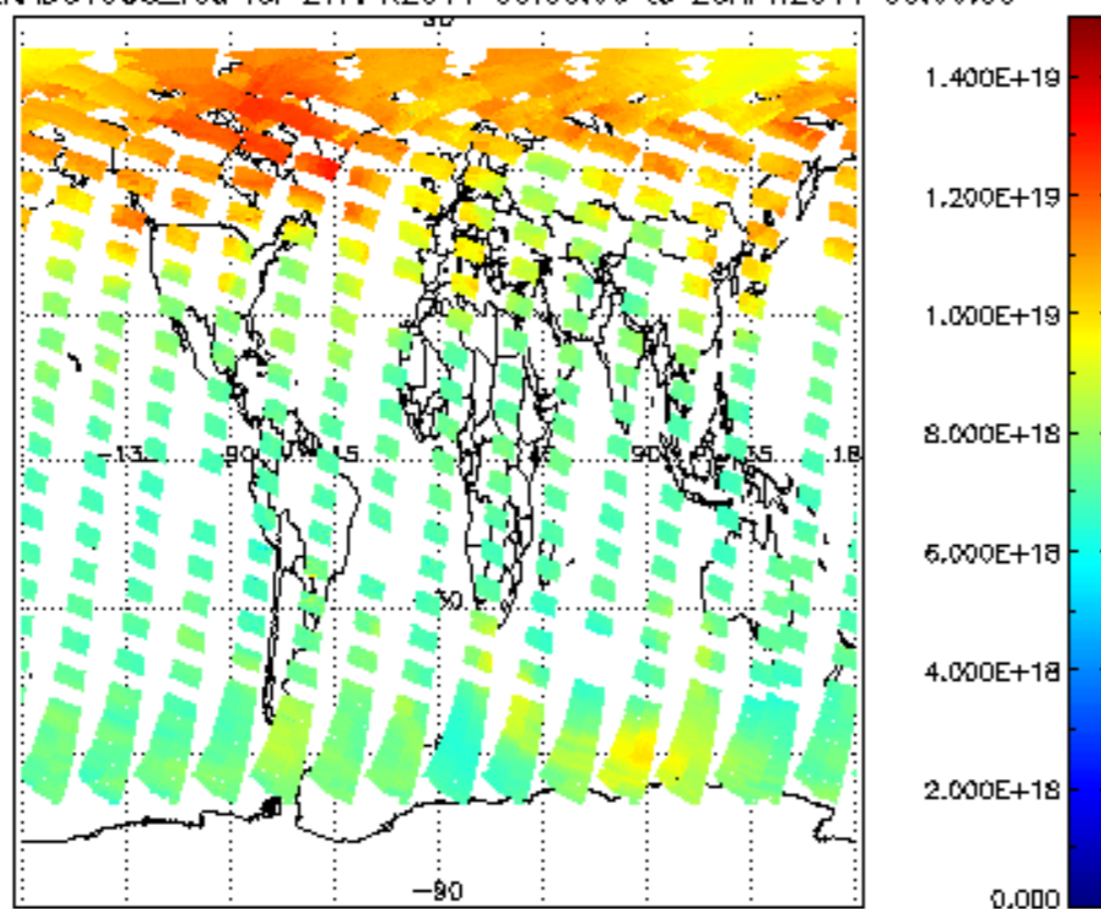
SCIOL2P_NADUV003_vcd for 27APR2011 00:00:00 to 28APR2011 00:00:00
