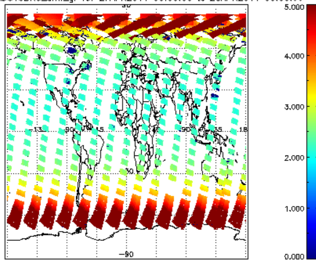
SCIOL2P_NADUV3BRO_amf_gr for 27APR2011 00:00:00 to 28APR2011 00:00:00
