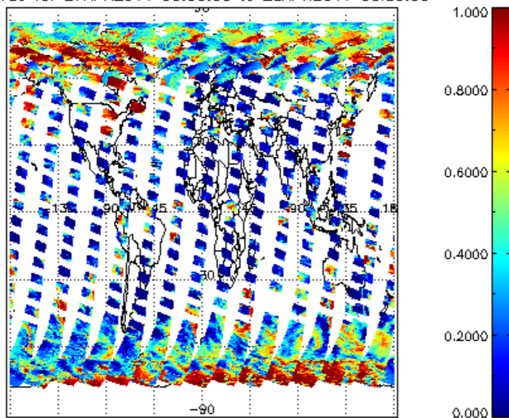
cL_frac for 27APR2011 00:00:00 to 28APR2011 00:00:00
