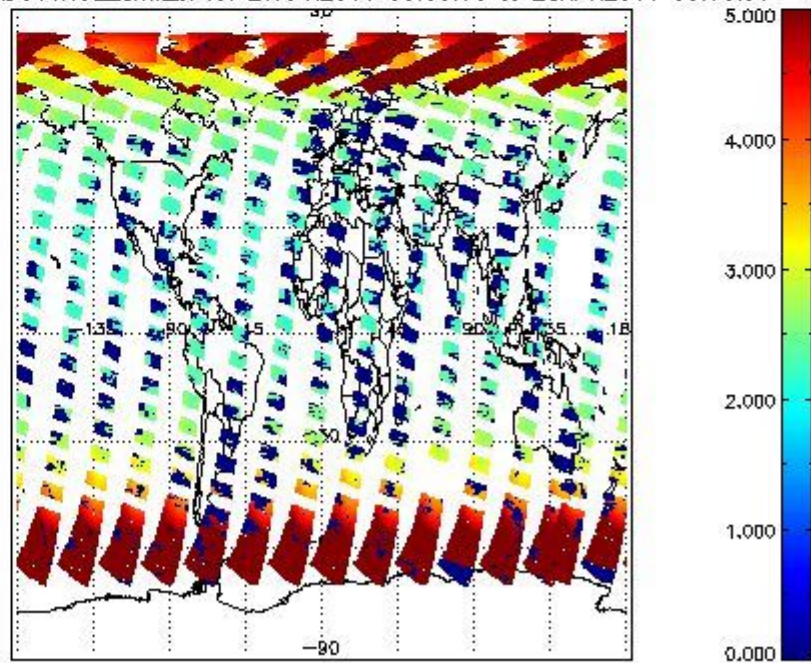
SCIOL2P_NADUV1N02_amf_cl for 27APR2011 00:00:00 to 28APR2011 00:00:00
