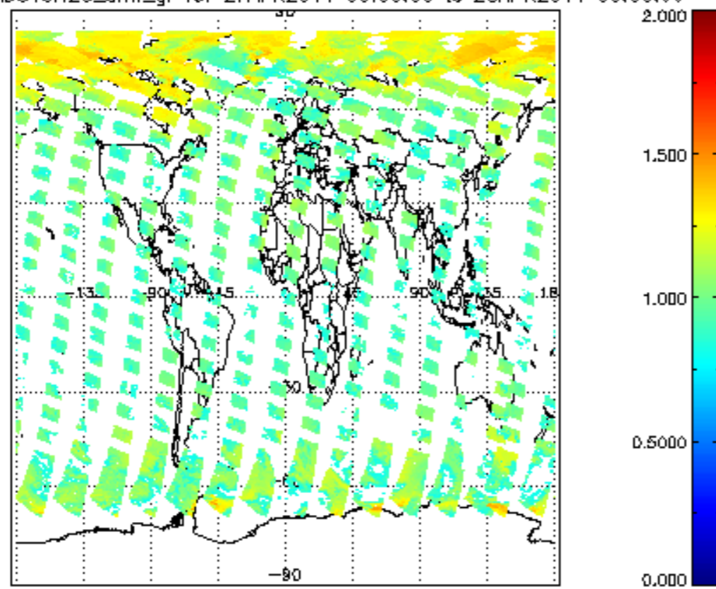
SCIOL2P_NADUV8H2O_amf_gr for 27APR2011 00:00:00 to 28APR2011 00:00:00
