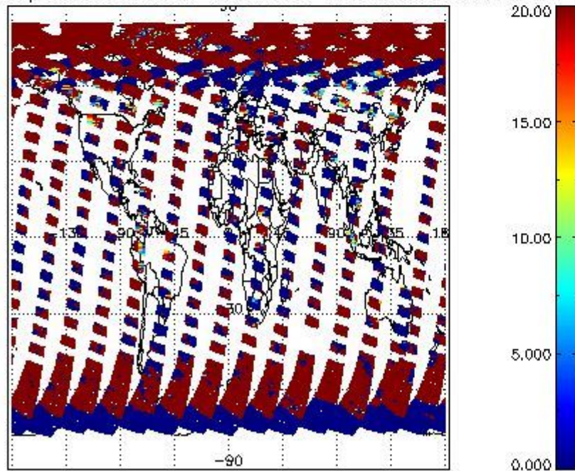
cL_opt_depth for 27APR2011 00:00:00 to 28APR2011 00:00:00
