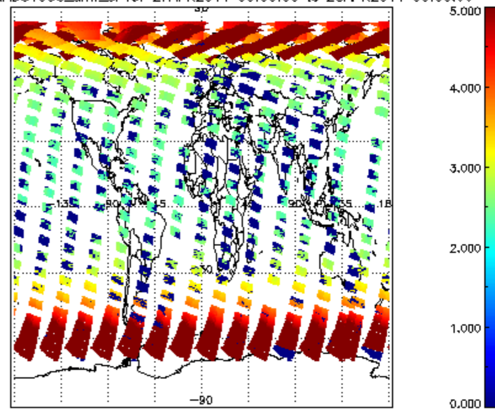
SCIOL2P_NADUV003_amf_cl for 27APR2011 00:00:00 to 28APR2011 00:00:00
