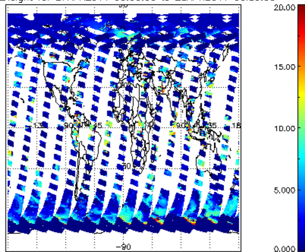
cL_top_height for 27APR2011 00:00:00 to 28APR2011 00:00:00
