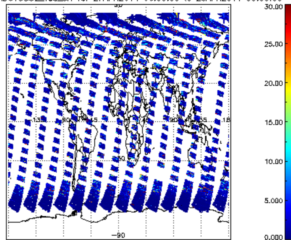
SCIOL2P_NADUV5S02_vcd_err for 27APR2011 00:00:00 to 28APR2011 00:00:00
