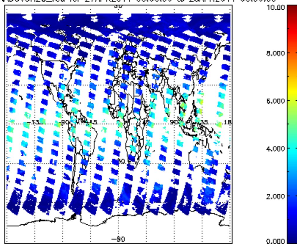
SCIOL2P_NADUV8H2O_vcd for 27APR2011 00:00:00 to 28APR2011 00:00:00
