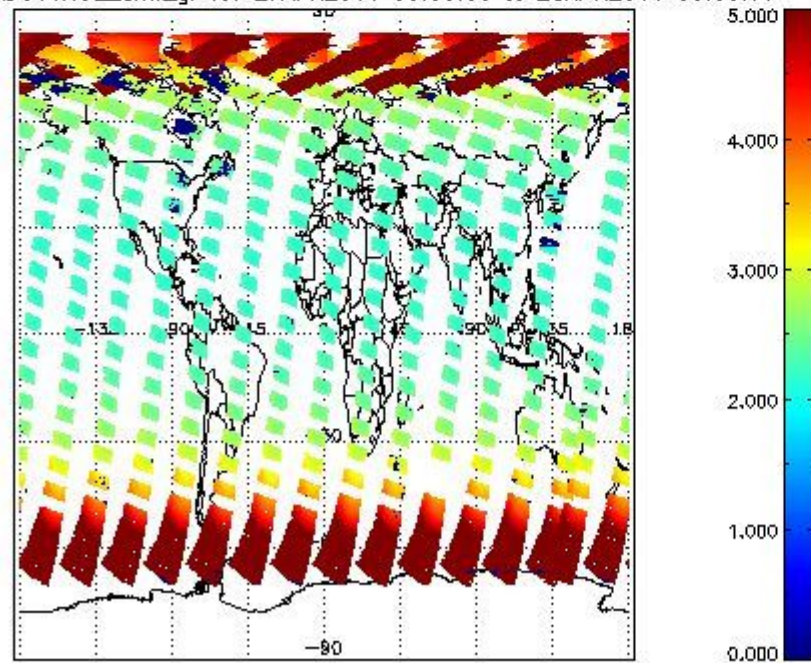
SCIOL2P_NADUV1N02_amf_gr for 27APR2011 00:00:00 to 28APR2011 00:00:00
