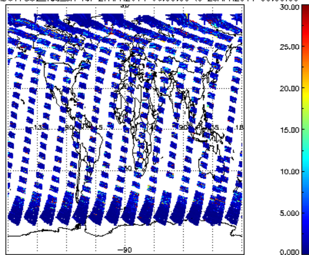
SCIOL2P_NADUV7S02_vcd_err for 27APR2011 00:00:00 to 28APR2011 00:00:00
