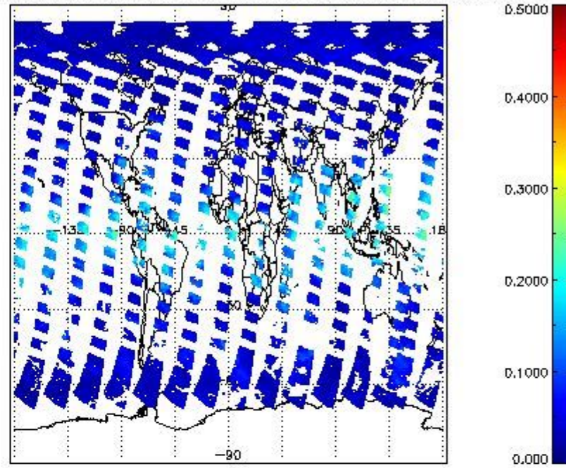
SCIOL2P_NADUV6H2O_vcd_err for 27APR2011 00:00:00 to 28APR2011 00:00:00
