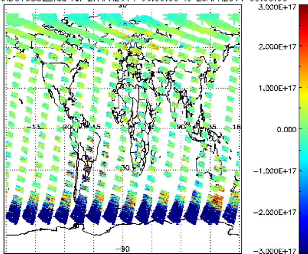
SCIOL2P_NADUV5S02_vcd for 27APR2011 00:00:00 to 28APR2011 00:00:00
