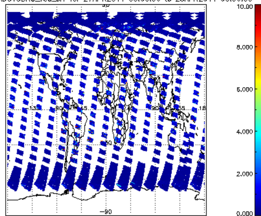
SCIOL2P_NADUV3BRO_vcd_err for 27APR2011 00:00:00 to 28APR2011 00:00:00
