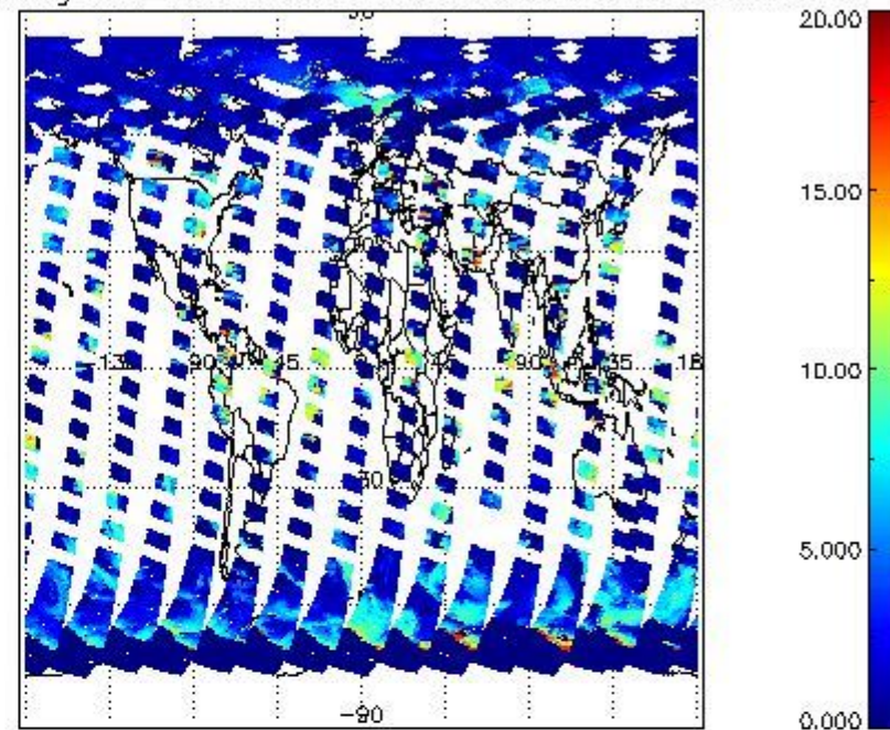
cL_top_height for 27APR2011 00:00:00 to 28APR2011 00:00:00
