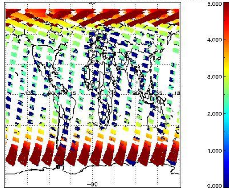
SCIOL2P_NADUV003_amf_cl for 27APR2011 00:00:00 to 28APR2011 00:00:00
