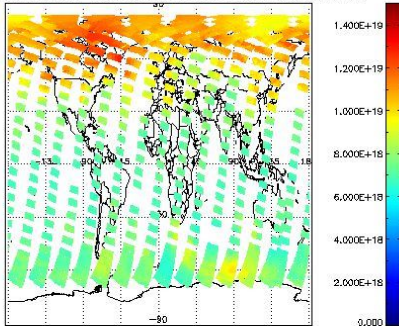
SCIOL2P_NADUV003_vcd for 27APR2011 00:00:00 to 28APR2011 00:00:00
