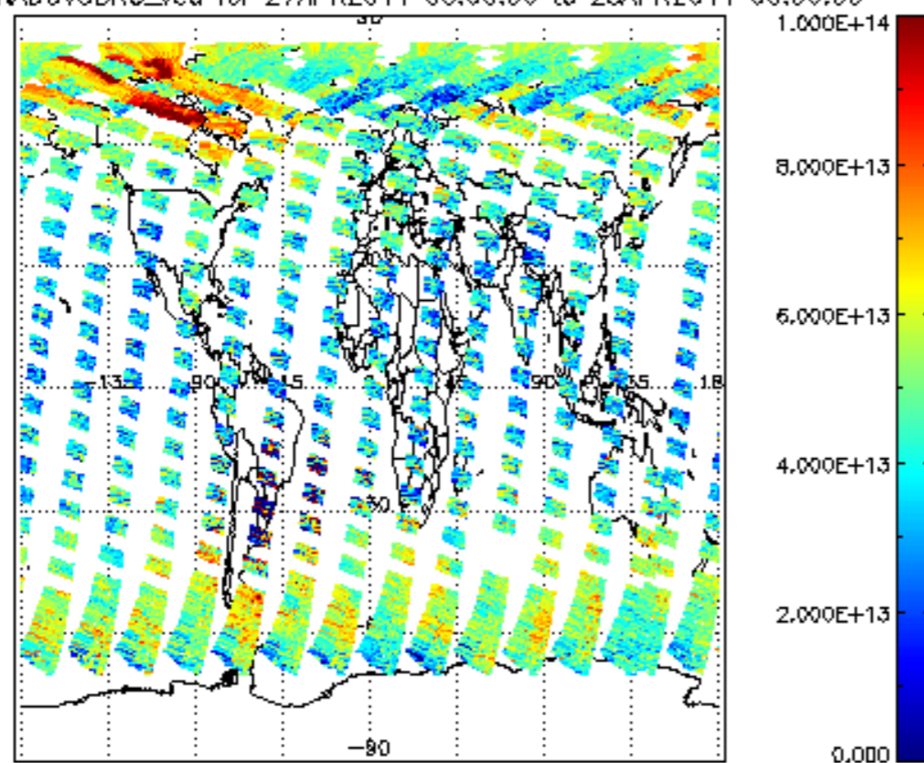
SCIOL2P_NADUV3BRO_vcd for 27APR2011 00:00:00 to 28APR2011 00:00:00
