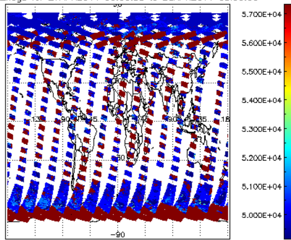
cloud_flags for 27APR2011 00:00:00 to 28APR2011 00:00:00
