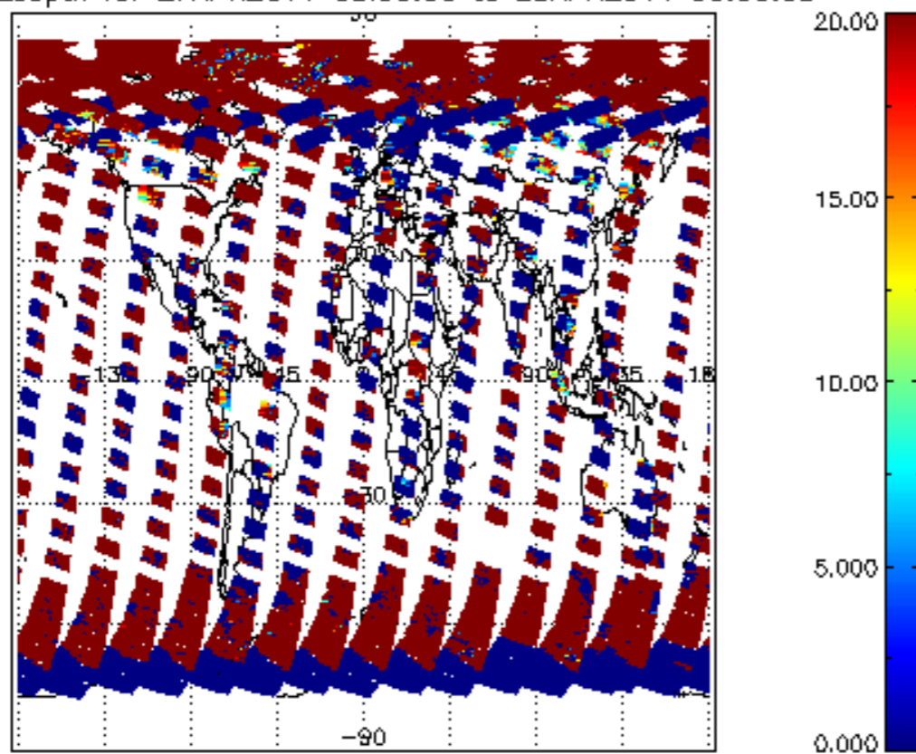
cL_opt_depth for 27APR2011 00:00:00 to 28APR2011 00:00:00
