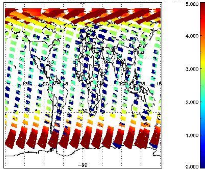
SCIOL2P_NADUV3BRO_amf_cl for 27APR2011 00:00:00 to 28APR2011 00:00:00
