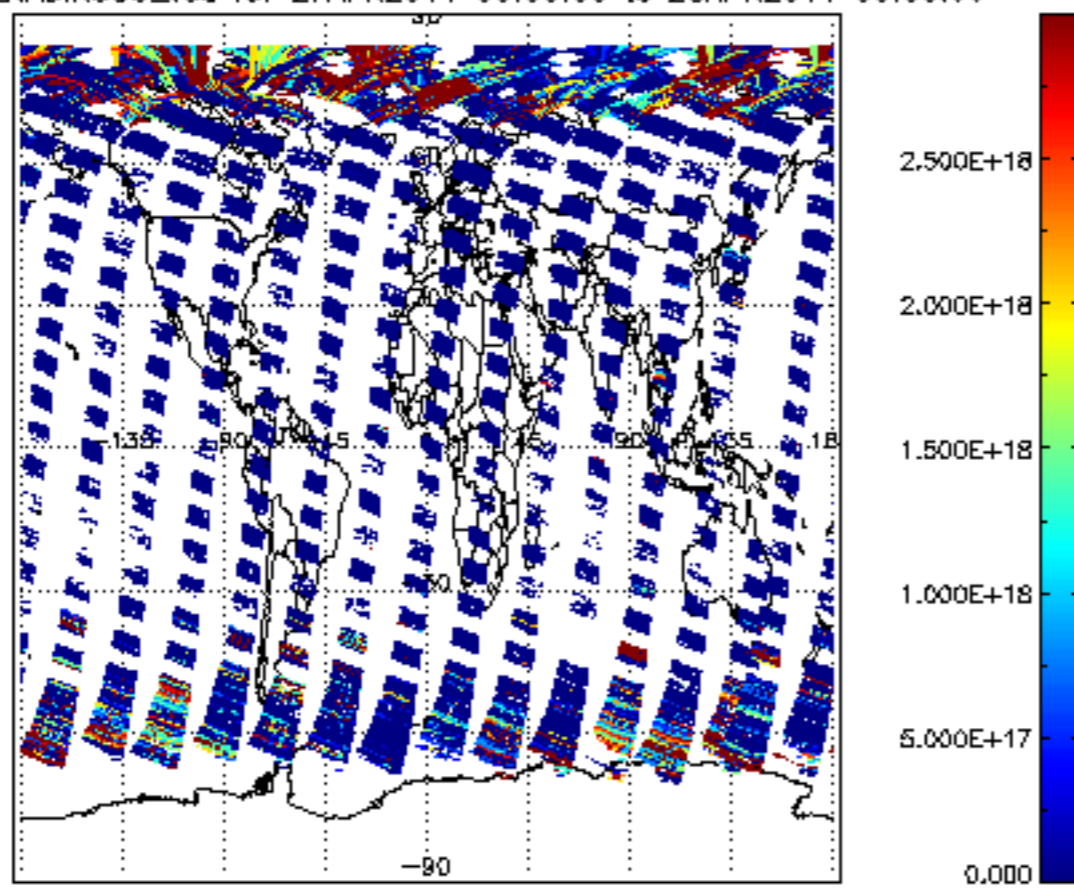
SCIOL2P_NADIR3CO_vcd for 27APR2011 00:00:00 to 28APR2011 00:00:00
