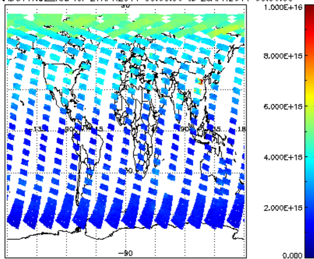
SCIOL2P_NADUV1NO2_vcd for 27APR2011 00:00:00 to 28APR2011 00:00:00
