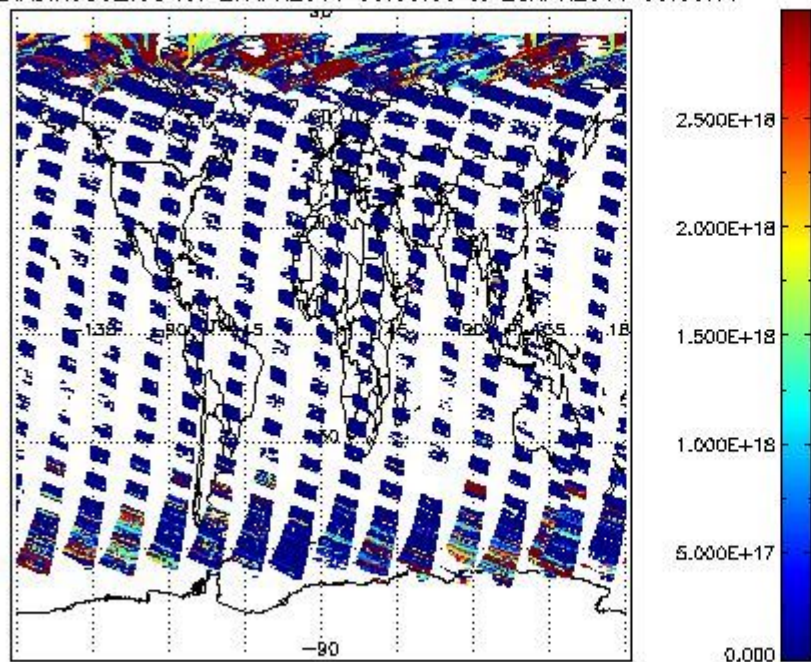
SCIDL2P_NADIR3CO_vcd for 27APR2011 00:00:00 to 28APR2011 00:00:00
