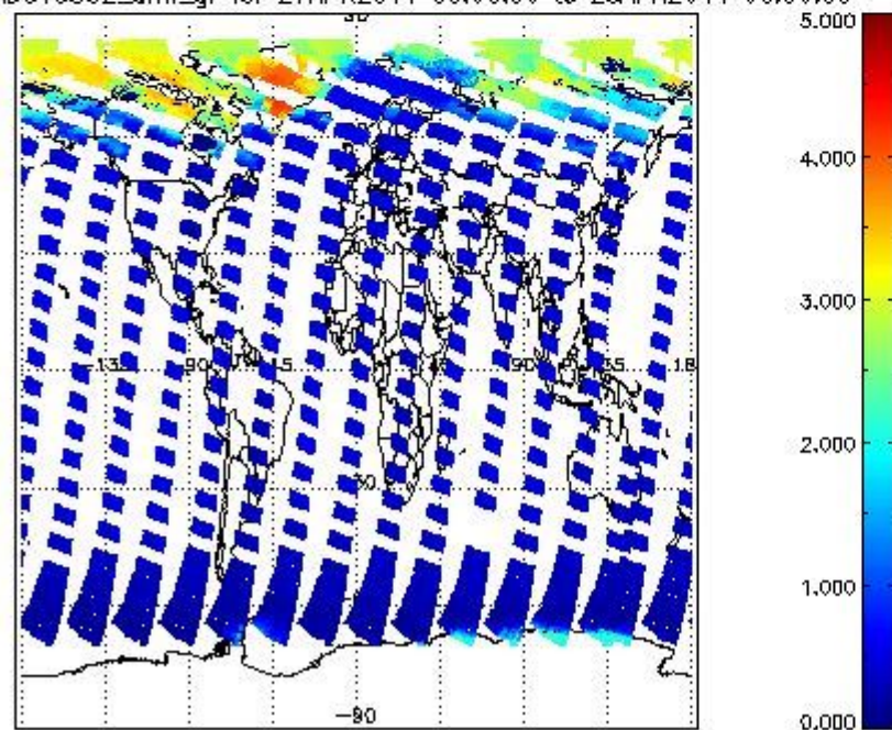
SCIOL2P_NADUV5S02_amf_gr for 27APR2011 00:00:00 to 28APR2011 00:00:00
