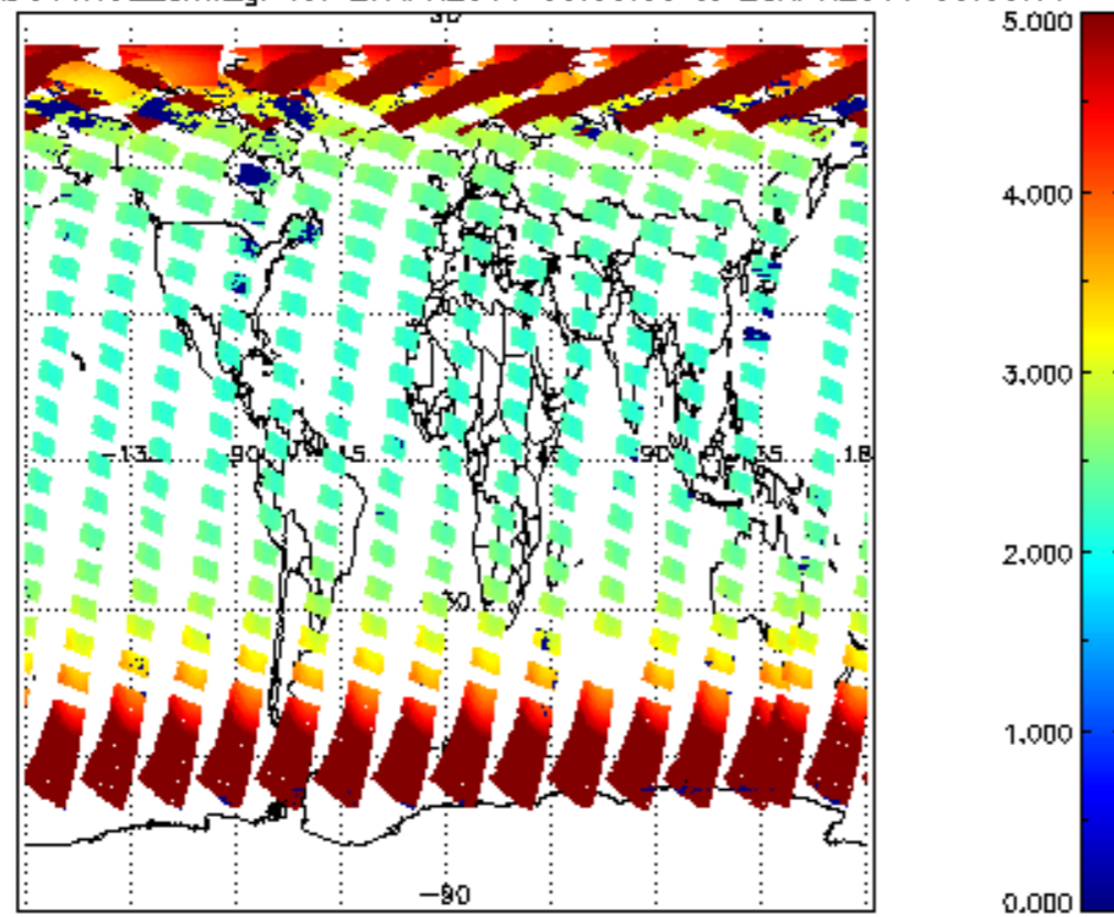
SCIOL2P_NADUV1NO2_amf_gr for 27APR2011 00:00:00 to 28APR2011 00:00:00
