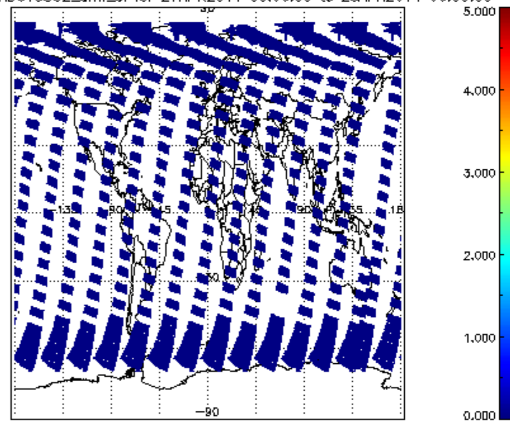
SCIOL2P_NADUV5S02_amf_cl for 27APR2011 00:00:00 to 28APR2011 00:00:00
