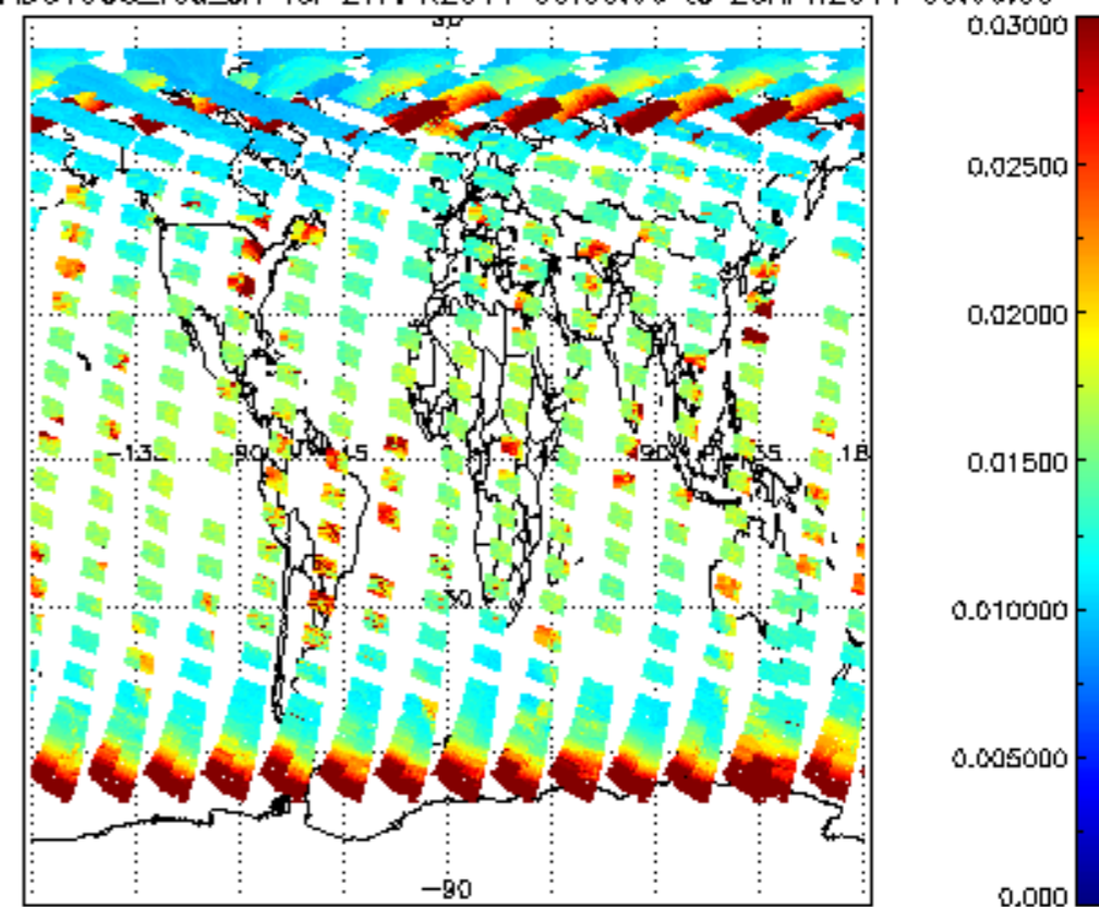
SCIOL2P_NADUV003_vcd_err for 27APR2011 00:00:00 to 28APR2011 00:00:00
