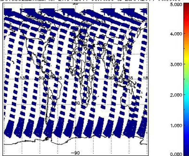
SCIOL2P_NADUV5S02_amf_cl for 27APR2011 00:00:00 to 28APR2011 00:00:00
