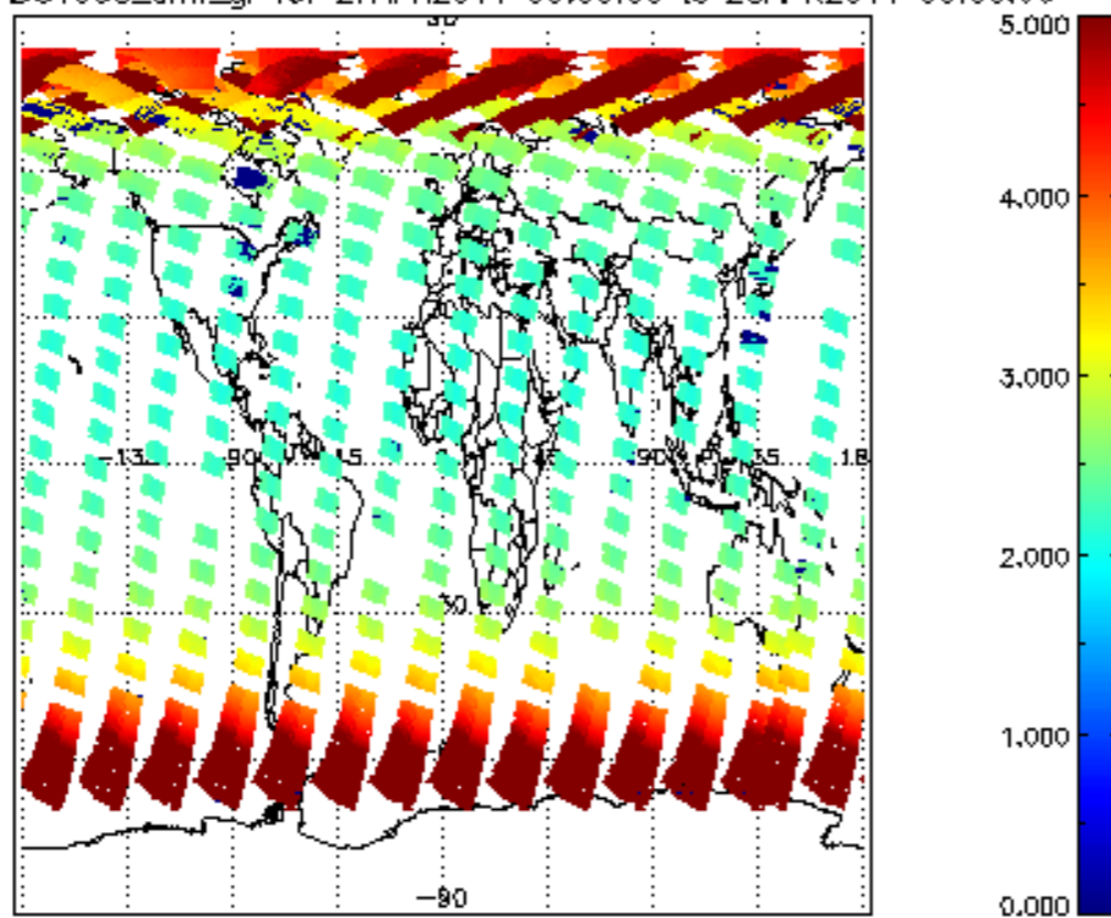
SCIOL2P_NADUV003_amf_gr for 27APR2011 00:00:00 to 28APR2011 00:00:00
