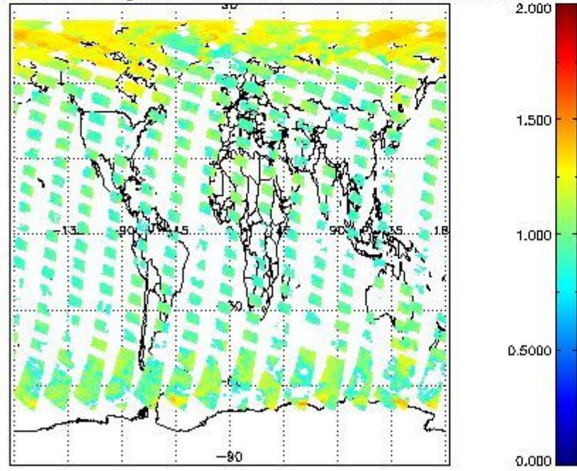
SCIOL2P_NADUV6H2O_amf_gr for 27APR2011 00:00:00 to 28APR2011 00:00:00
