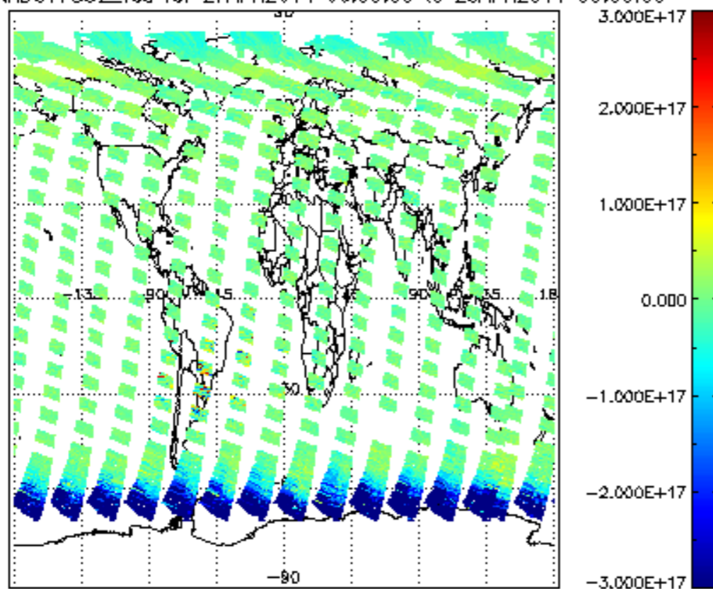
SCIOL2P_NADUV7S02_vcd for 27APR2011 00:00:00 to 28APR2011 00:00:00
