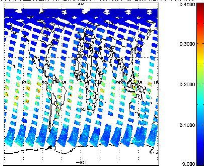
SCIOL2P_NADUV1N02_vcd_err for 27APR2011 00:00:00 to 28APR2011 00:00:00
