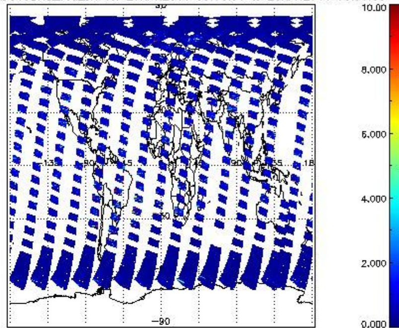
SCIOL2P_NADUV3BRO_vcd_err for 27APR2011 00:00:00 to 28APR2011 00:00:00
