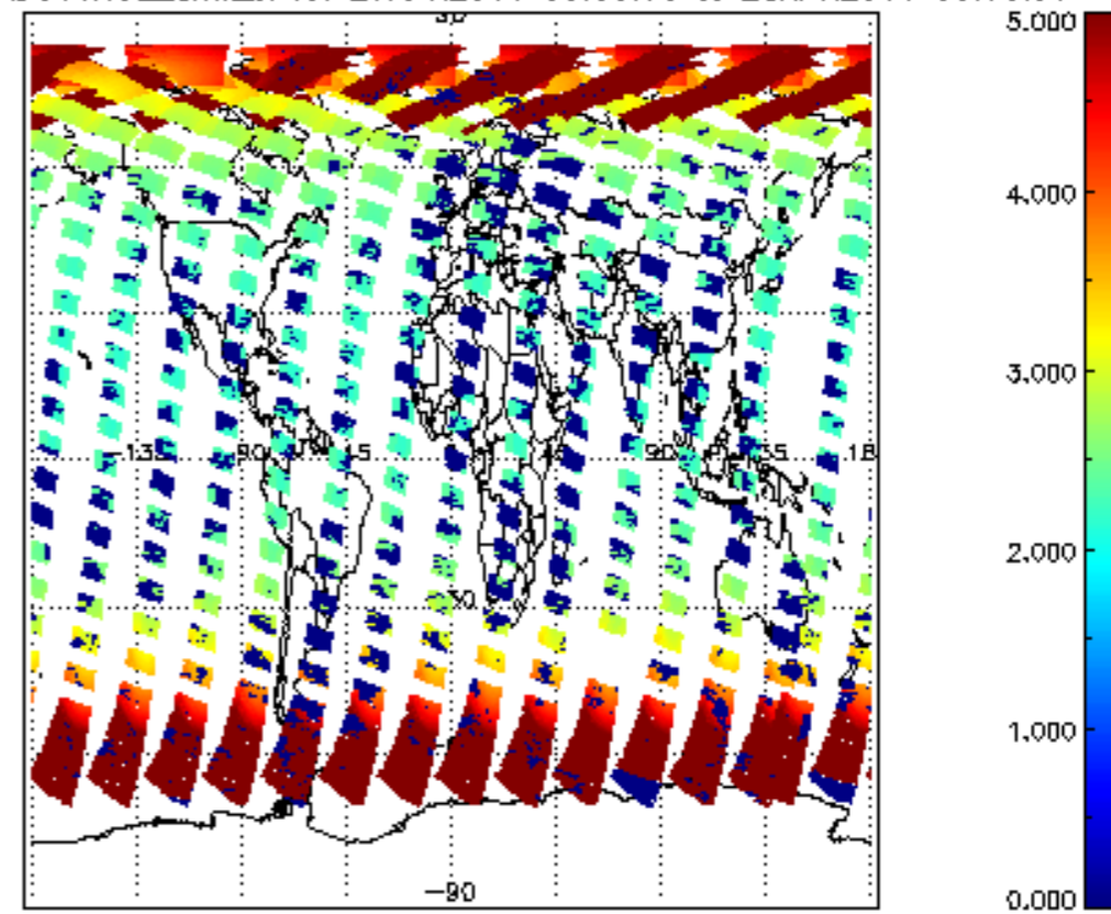
SCIOL2P_NADUV1NO2_amf_sl for 27APR2011 00:00:00 to 28APR2011 00:00:00
