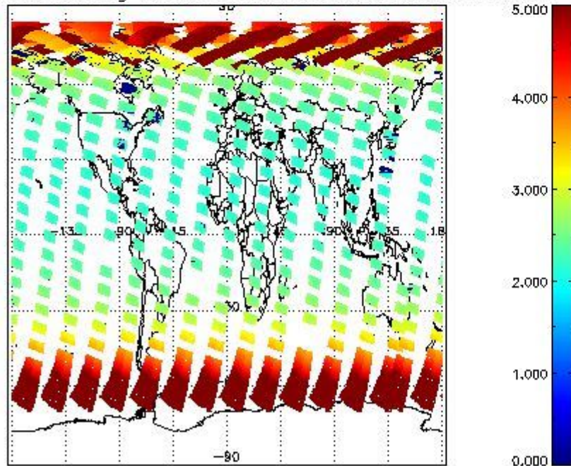
SCIOL2P_NADUV003_amf_gr for 27APR2011 00:00:00 to 28APR2011 00:00:00
