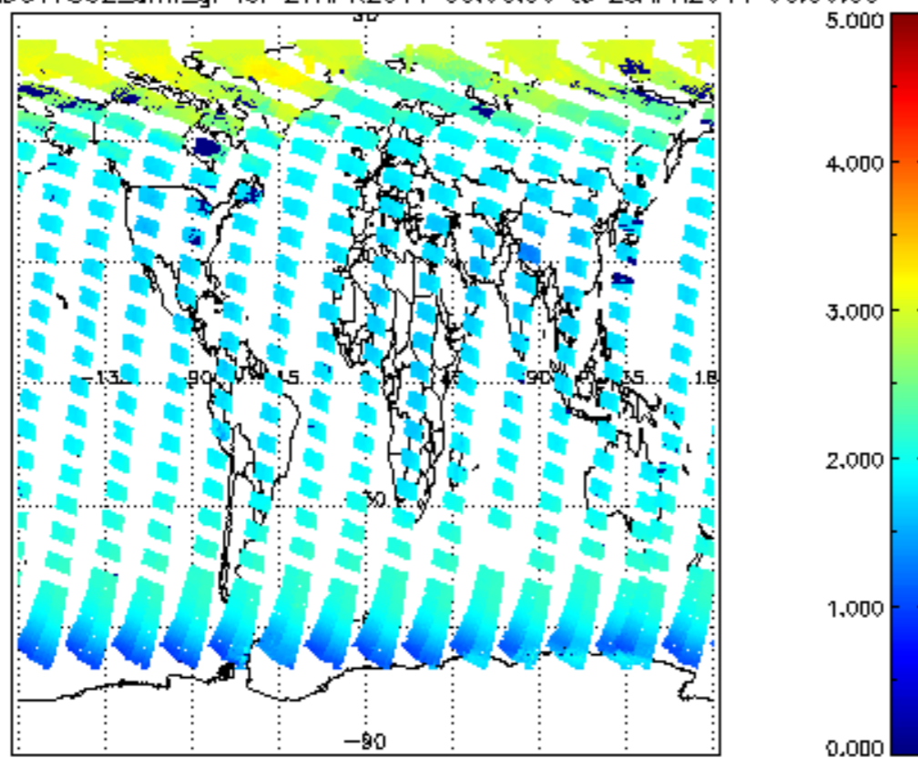
SCIOL2P_NADUV7S02_amf_gr for 27APR2011 00:00:00 to 28APR2011 00:00:00
