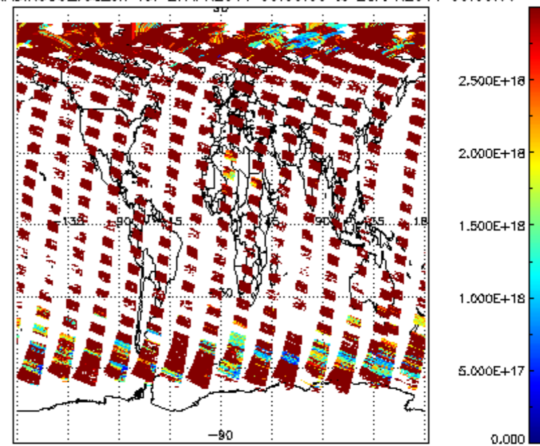
SCIOL2P_NADIR3CO_vcd_err for 27APR2011 00:00:00 to 28APR2011 00:00:00
