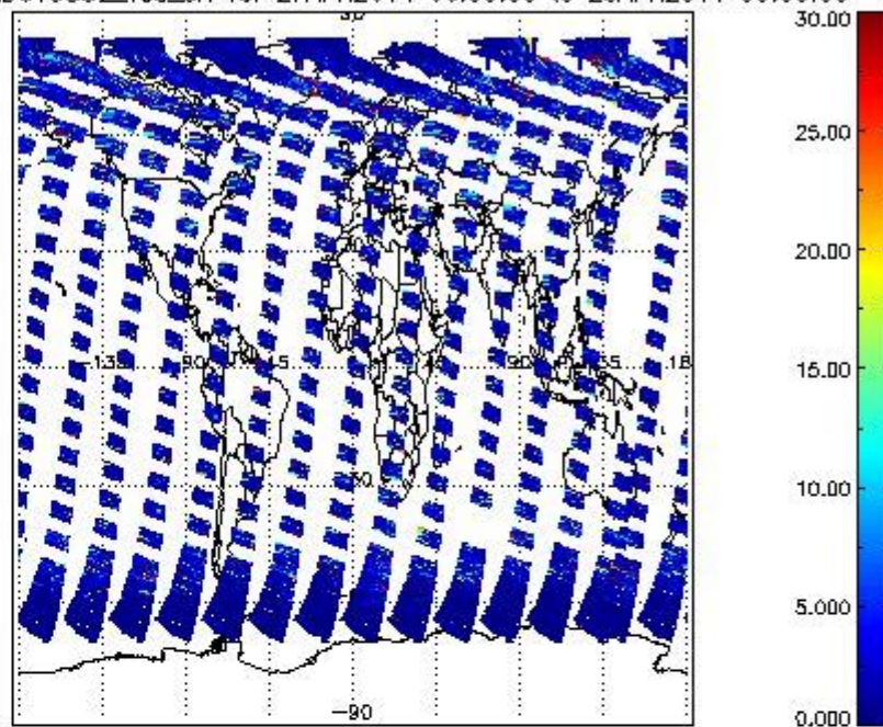
SCIOL2P_NADUV5S02_vcd_err for 27APR2011 00:00:00 to 28APR2011 00:00:00
