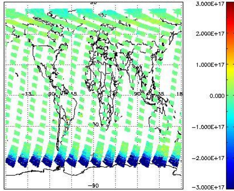
SCIOL2P_NADUV7S02_vcd for 27APR2011 00:00:00 to 28APR2011 00:00:00
