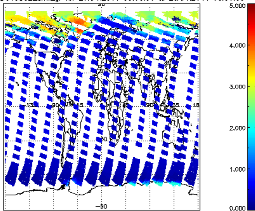
SCIOL2P_NADUV5S02_amf_gr for 27APR2011 00:00:00 to 28APR2011 00:00:00
