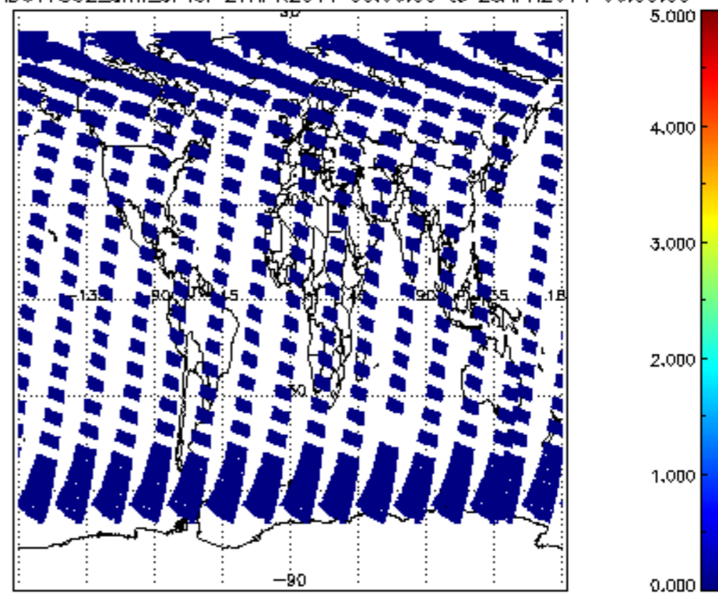
SCIOL2P_NADUV7S02_amf_cl for 27APR2011 00:00:00 to 28APR2011 00:00:00
