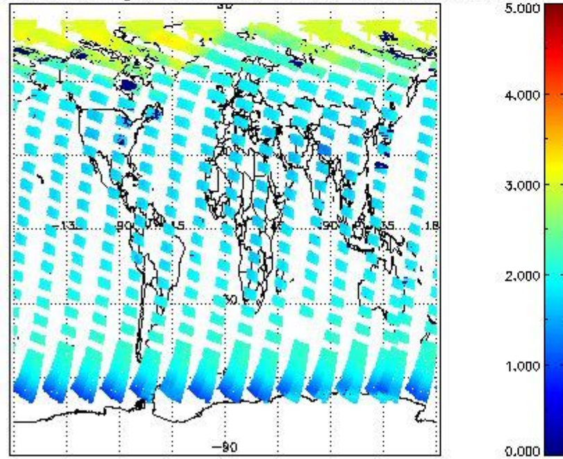
SCIOL2P_NADUV7S02_amf_gr for 27APR2011 00:00:00 to 28APR2011 00:00:00
