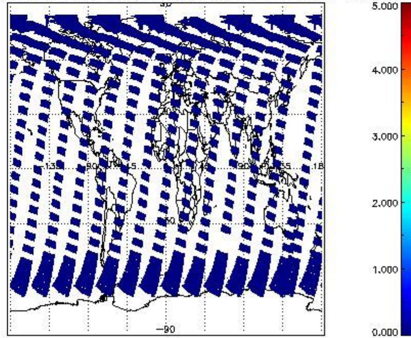
SCIOL2P_NADUV7S02_amf_cl for 27APR2011 00:00:00 to 28APR2011 00:00:00
