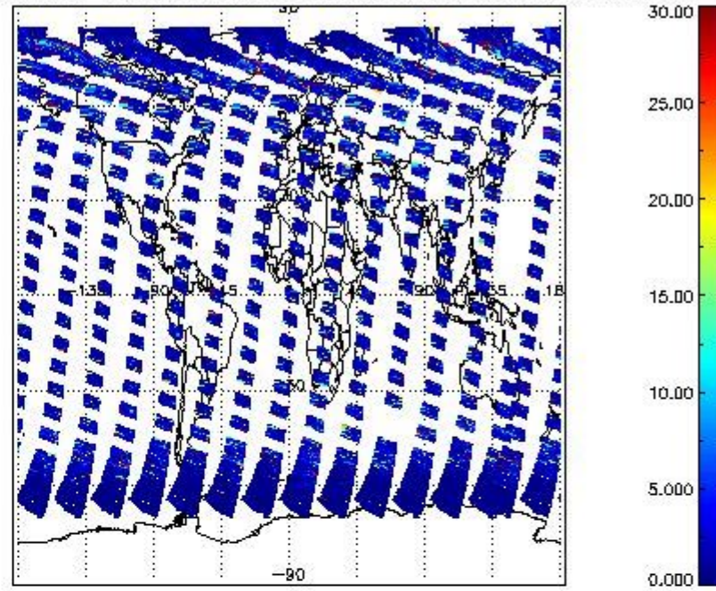
SCIOL2P_NADUV7S02_vcd_err for 27APR2011 00:00:00 to 28APR2011 00:00:00
