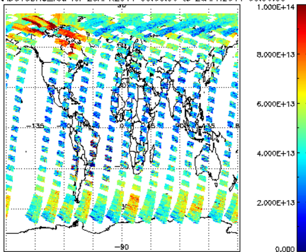
SCIOL2P_NADUV3BRO_vcd for 25APR2011 00:00:00 to 26APR2011 00:00:00
