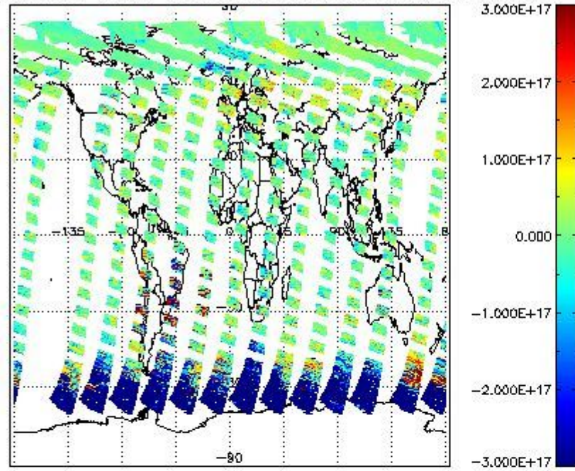
SCIOL2P_NADUV5S02_vcd for 25APR2011 00:00:00 to 26APR2011 00:00:00
