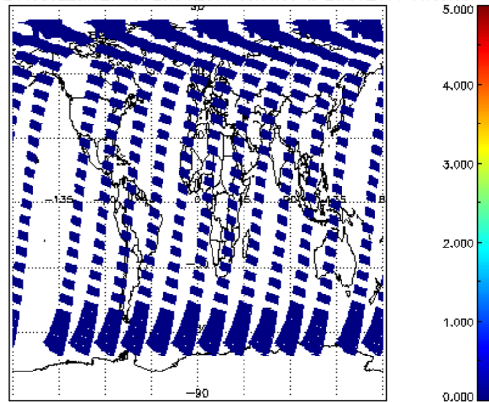
SCIOL2P_NADUV5S02_amf_cl for 25APR2011 00:00:00 to 26APR2011 00:00:00
