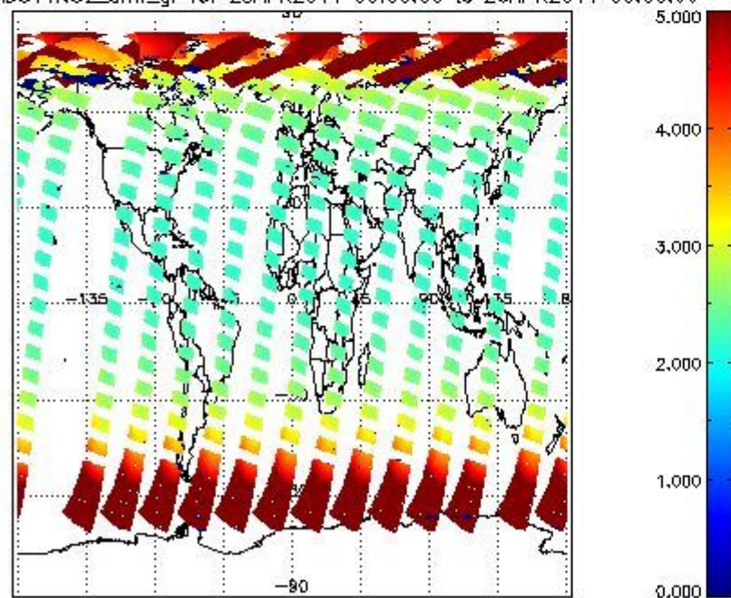
SCIOL2P_NADUV1NO2_amf_gr for 25APR2011 00:00:00 to 26APR2011 00:00:00
