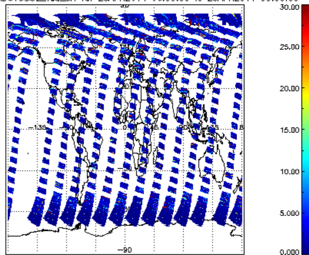
SCIOL2P_NADUV5S02_vcd_err for 25APR2011 00:00:00 to 26APR2011 00:00:00
