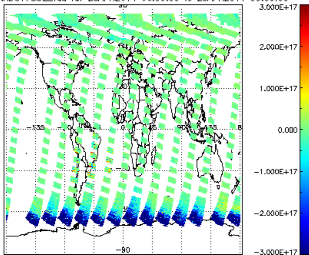
SCIOL2P_NADUV7S02_vcd for 25APR2011 00:00:00 to 26APR2011 00:00:00
