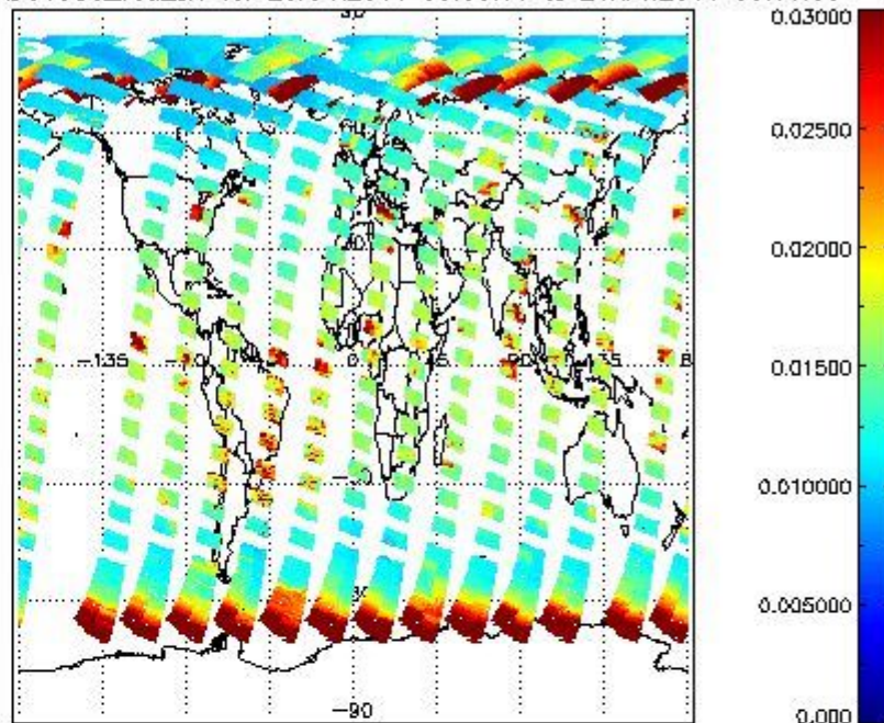
SCIOL2P_NADUV003_vcd_err for 25APR2011 00:00:00 to 26APR2011 00:00:00
