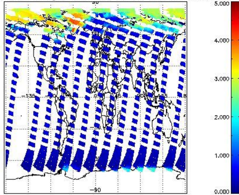
SCIOL2P_NADUV5S02_amf_gr for 25APR2011 00:00:00 to 26APR2011 00:00:00
