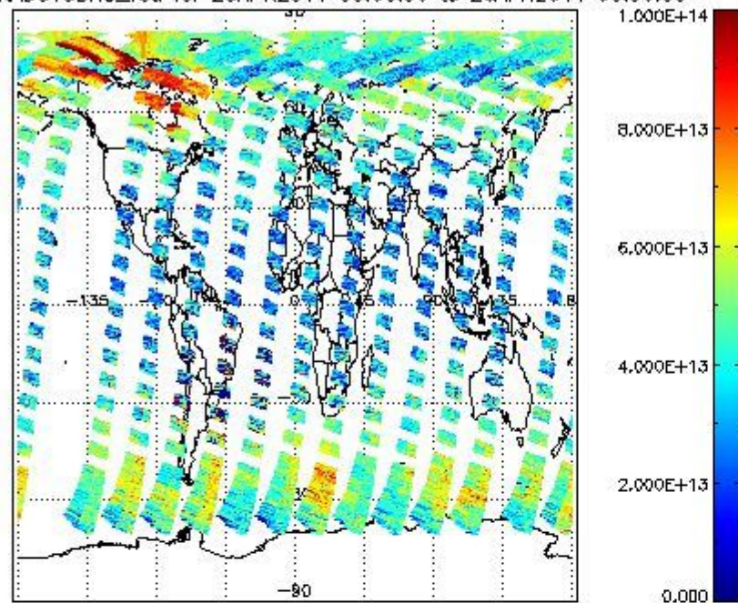
SCIOL2P_NADUV3BRO_vcd for 25APR2011 00:00:00 to 26APR2011 00:00:00
