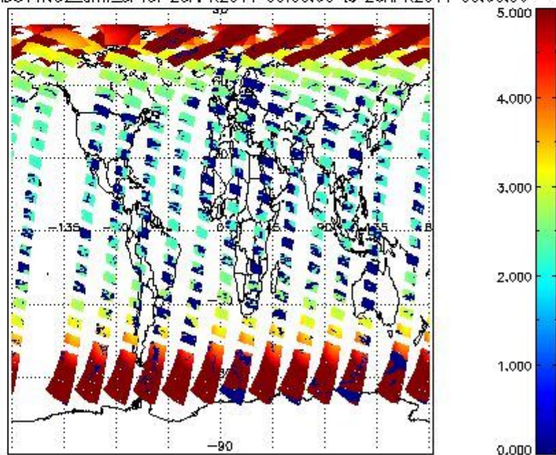
SCIOL2P_NADUV1NO2_amf_cl for 25APR2011 00:00:00 to 26APR2011 00:00:00
