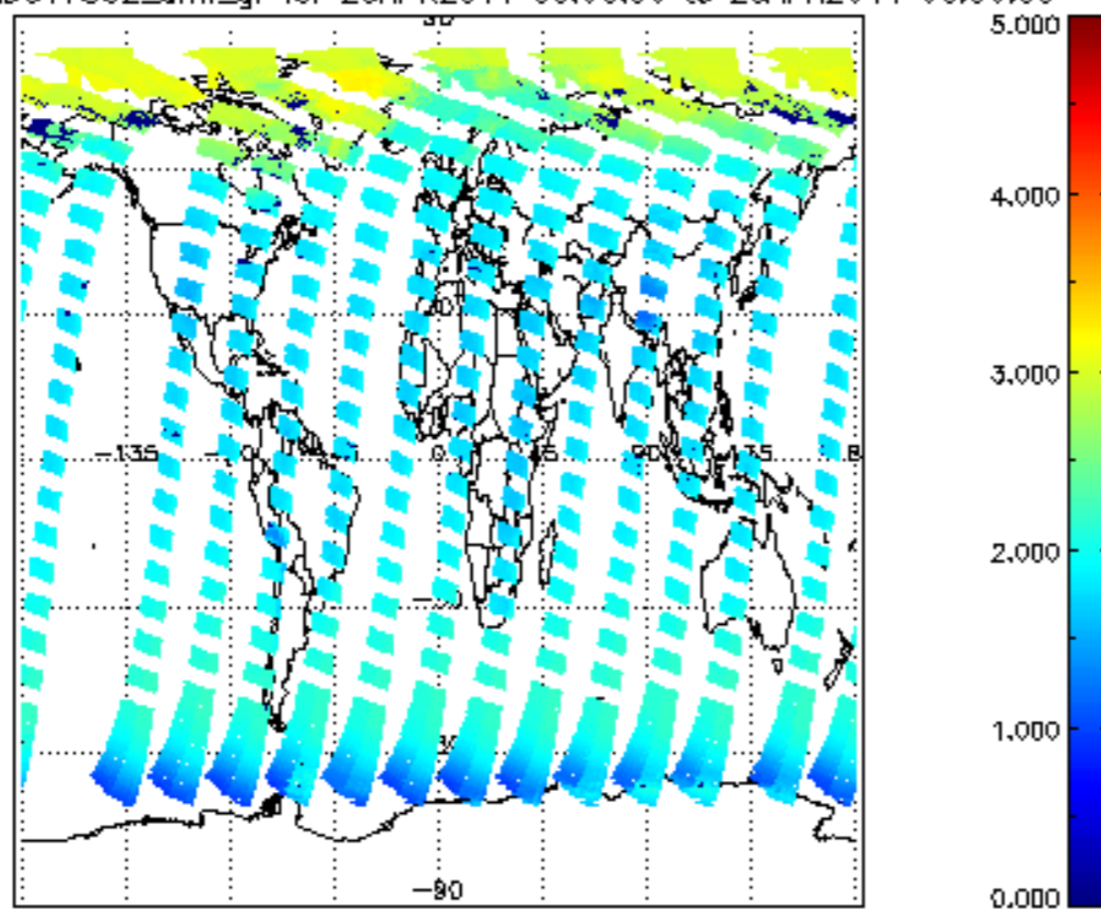
SCIOL2P_NADUV7S02_amf_gr for 25APR2011 00:00:00 to 26APR2011 00:00:00
