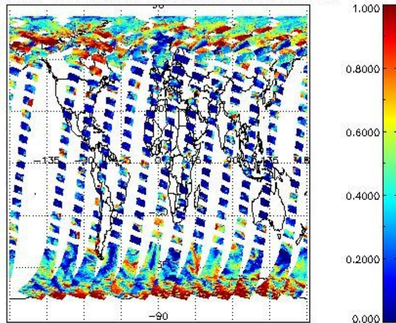
cL_frac for 25APR2011 00:00:00 to 26APR2011 00:00:00
