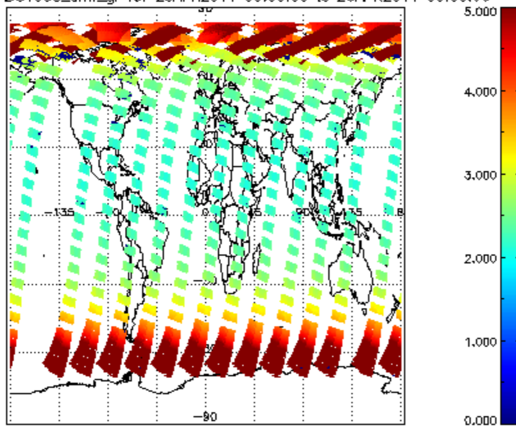
SCIOL2P_NADUV003_amf_gr for 25APR2011 00:00:00 to 26APR2011 00:00:00
