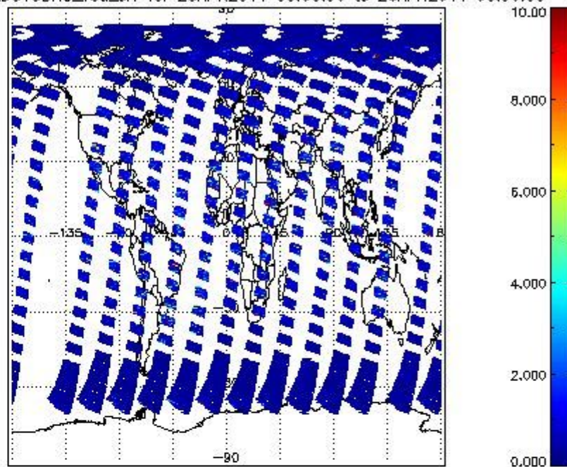
SCIOL2P_NADUV3BRO_vcd_err for 25APR2011 00:00:00 to 26APR2011 00:00:00
