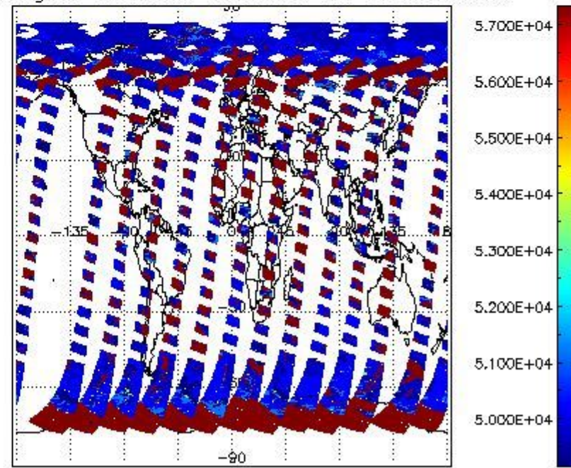
cloud_flags for 25APR2011 00:00:00 to 26APR2011 00:00:00
