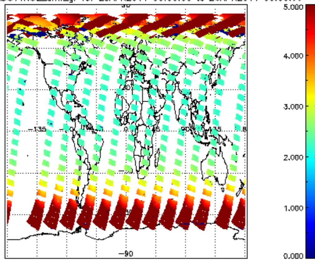
SCIOL2P_NADUV1NO2_amf_gr for 25APR2011 00:00:00 to 26APR2011 00:00:00
