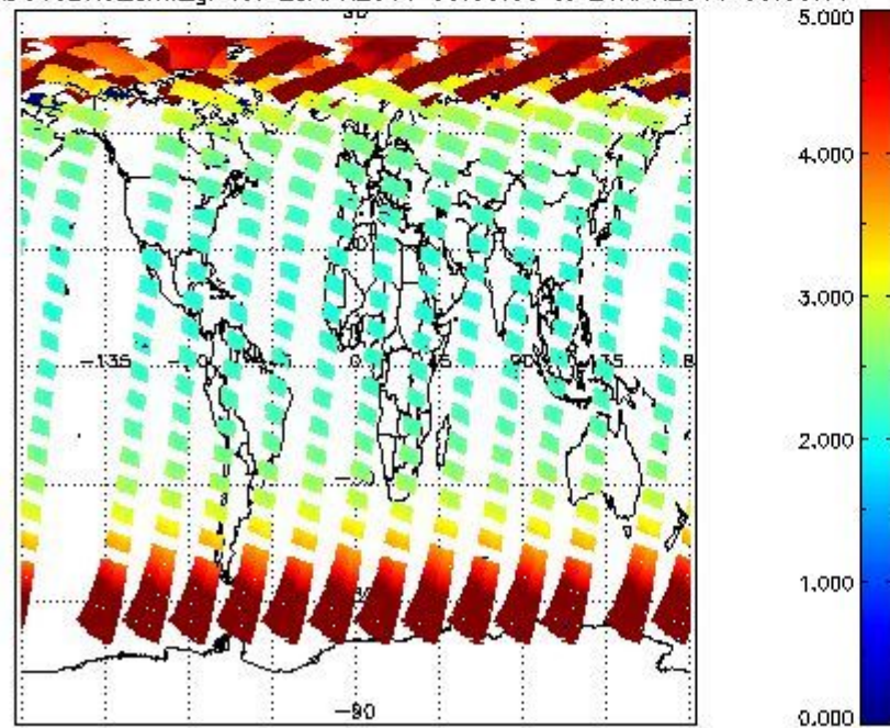
SCIOL2P_NADUV3BRO_amf_gr for 25APR2011 00:00:00 to 26APR2011 00:00:00
