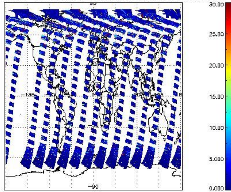
SCIOL2P_NADUV7S02_vcd_err for 25APR2011 00:00:00 to 26APR2011 00:00:00
