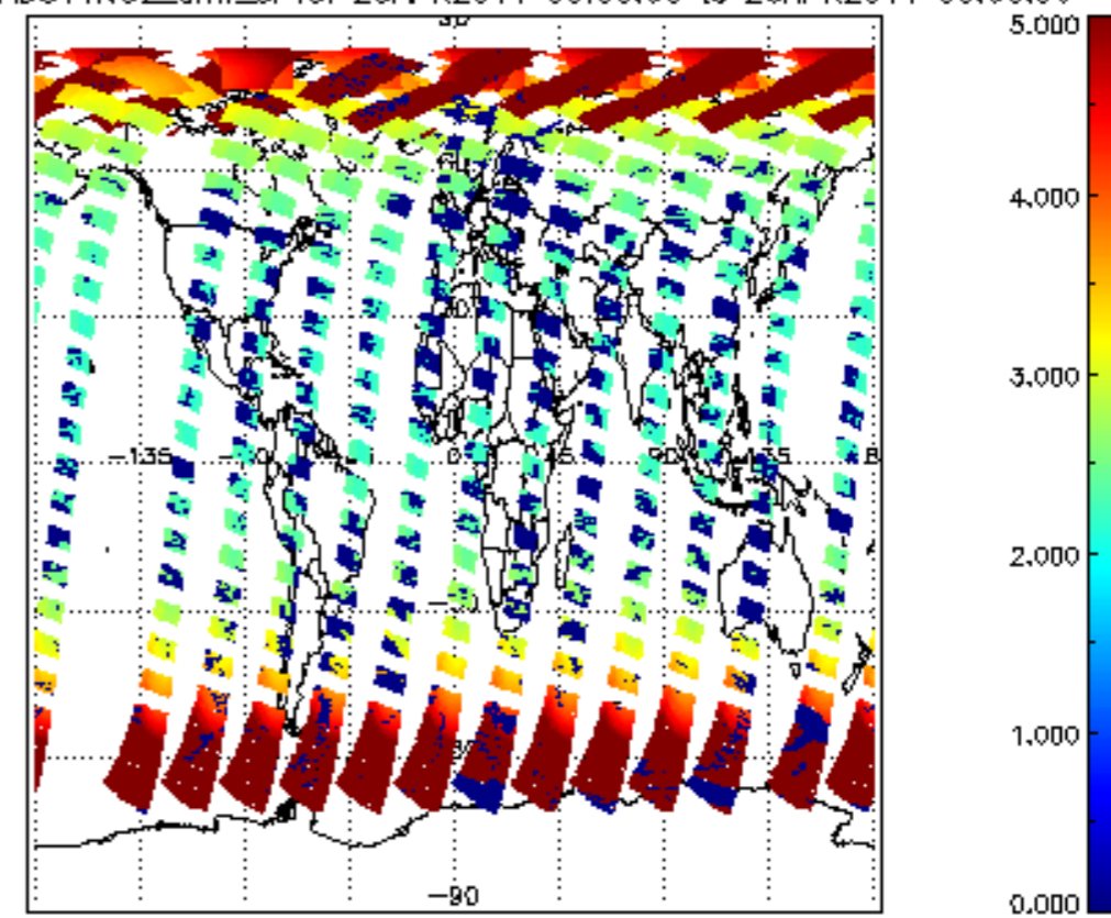
SCIOL2P_NADUV1NO2_amf_sl for 25APR2011 00:00:00 to 26APR2011 00:00:00
