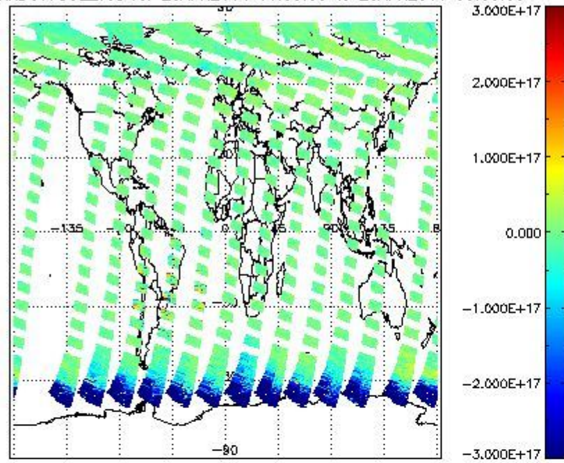
SCIOL2P_NADUV7S02_vcd for 25APR2011 00:00:00 to 26APR2011 00:00:00
