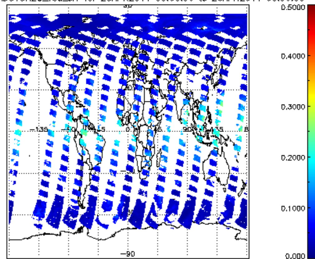
SCIOL2P_NADUV8H2O_vcd_err for 25APR2011 00:00:00 to 26APR2011 00:00:00
