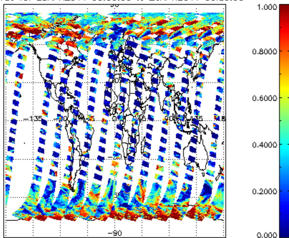
cL_frac for 25APR2011 00:00:00 to 26APR2011 00:00:00
