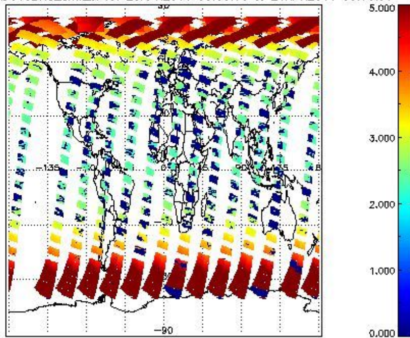
SCIOL2P_NADUV3BRO_amf_cl for 25APR2011 00:00:00 to 26APR2011 00:00:00
