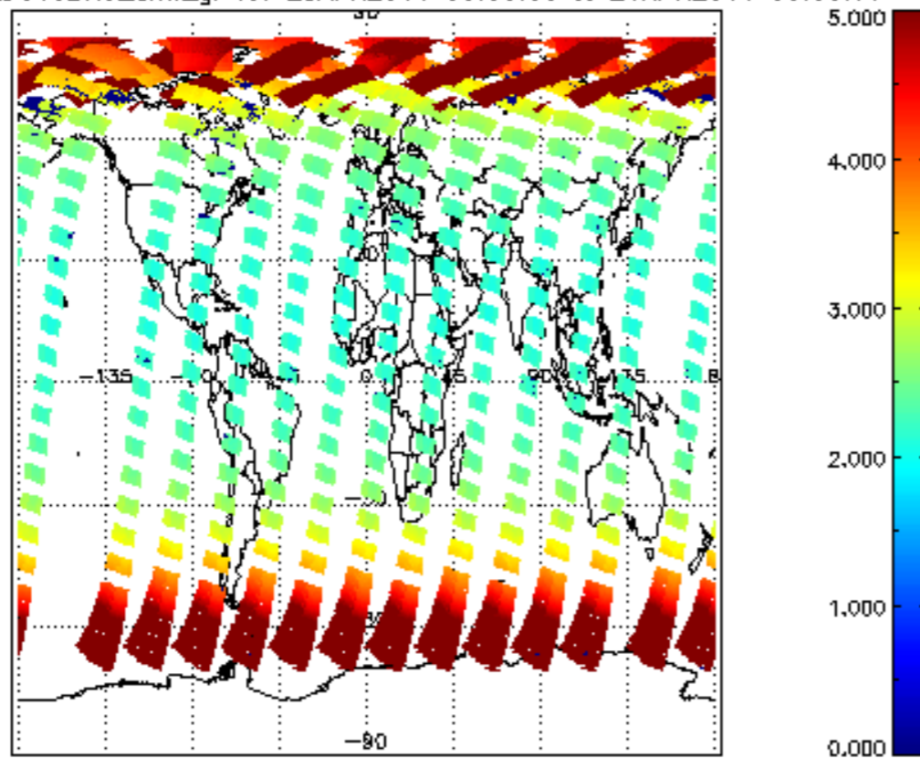
SCIOL2P_NADUV3BRO_amf_gr for 25APR2011 00:00:00 to 26APR2011 00:00:00
