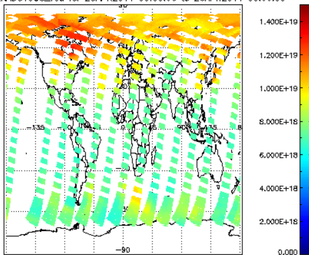
SCIOL2P_NADUV003_vcd for 25APR2011 00:00:00 to 26APR2011 00:00:00
