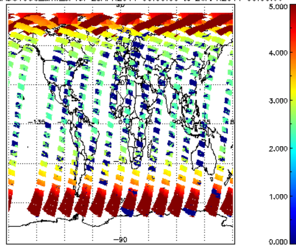
SCIOL2P_NADUV003_amf_cl for 25APR2011 00:00:00 to 26APR2011 00:00:00
