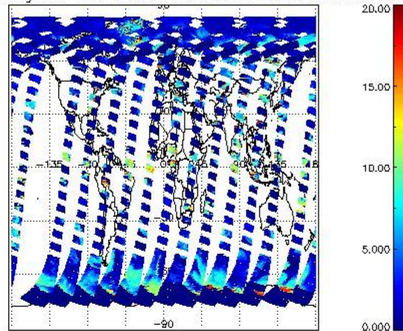
cL_top_height for 25APR2011 00:00:00 to 26APR2011 00:00:00
