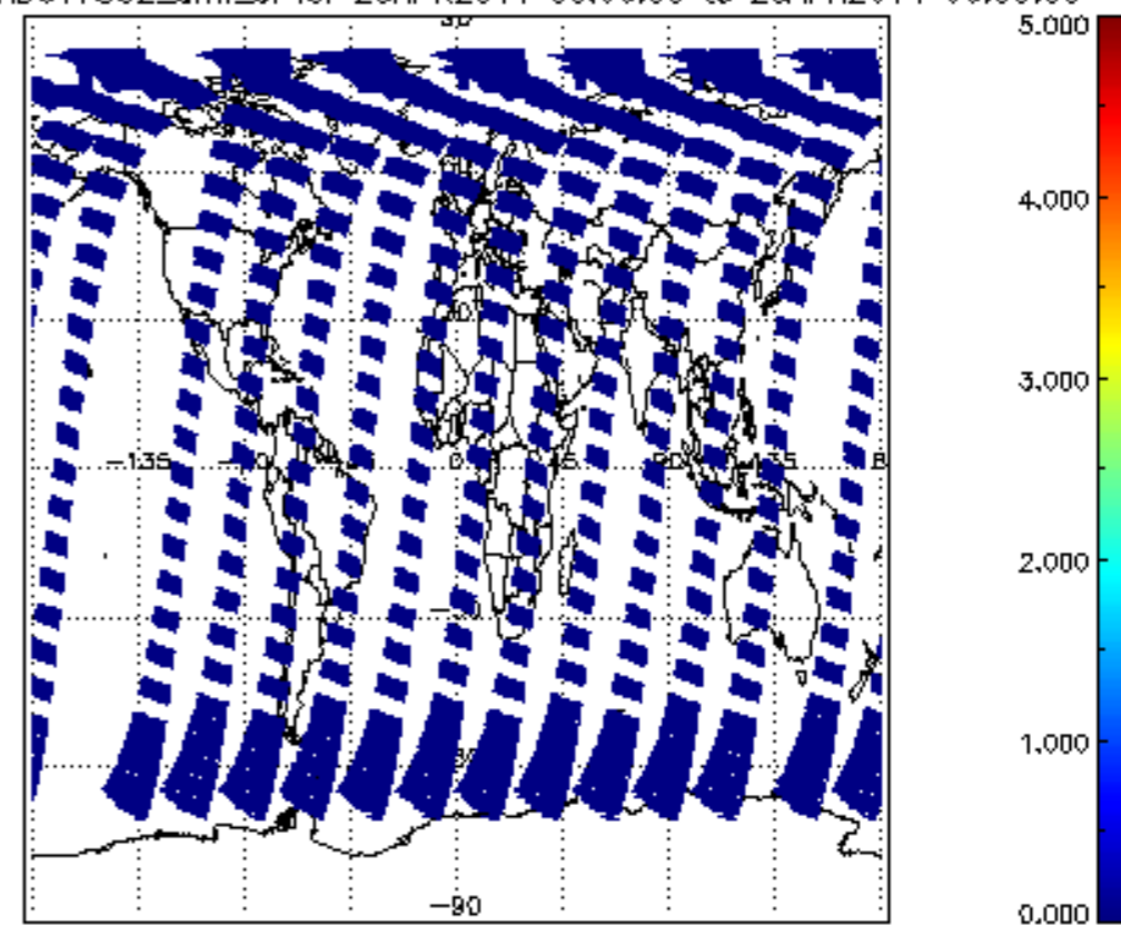
SCIOL2P_NADUV7S02_amf_cl for 25APR2011 00:00:00 to 26APR2011 00:00:00
