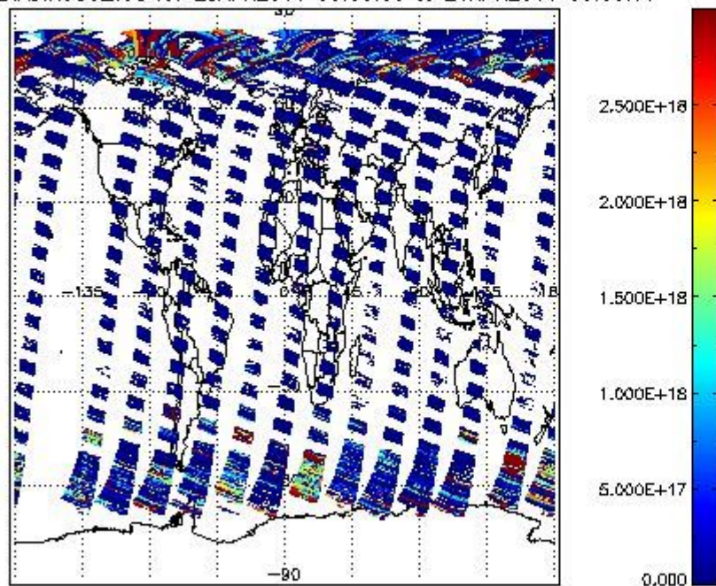
SCIDL2P_NADIR3CO_vcd for 25APR2011 00:00:00 to 26APR2011 00:00:00
