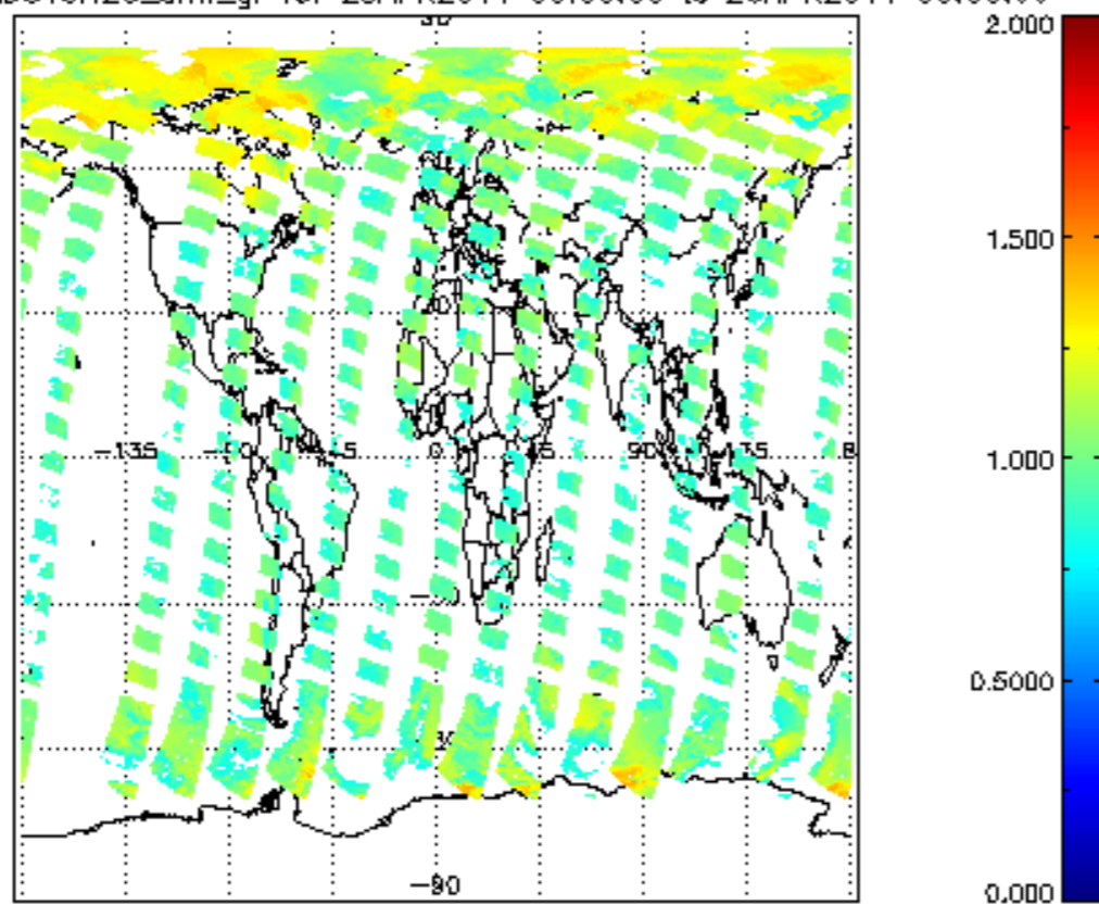
SCIOL2P_NADUV8H2O_amf_gr for 25APR2011 00:00:00 to 26APR2011 00:00:00
