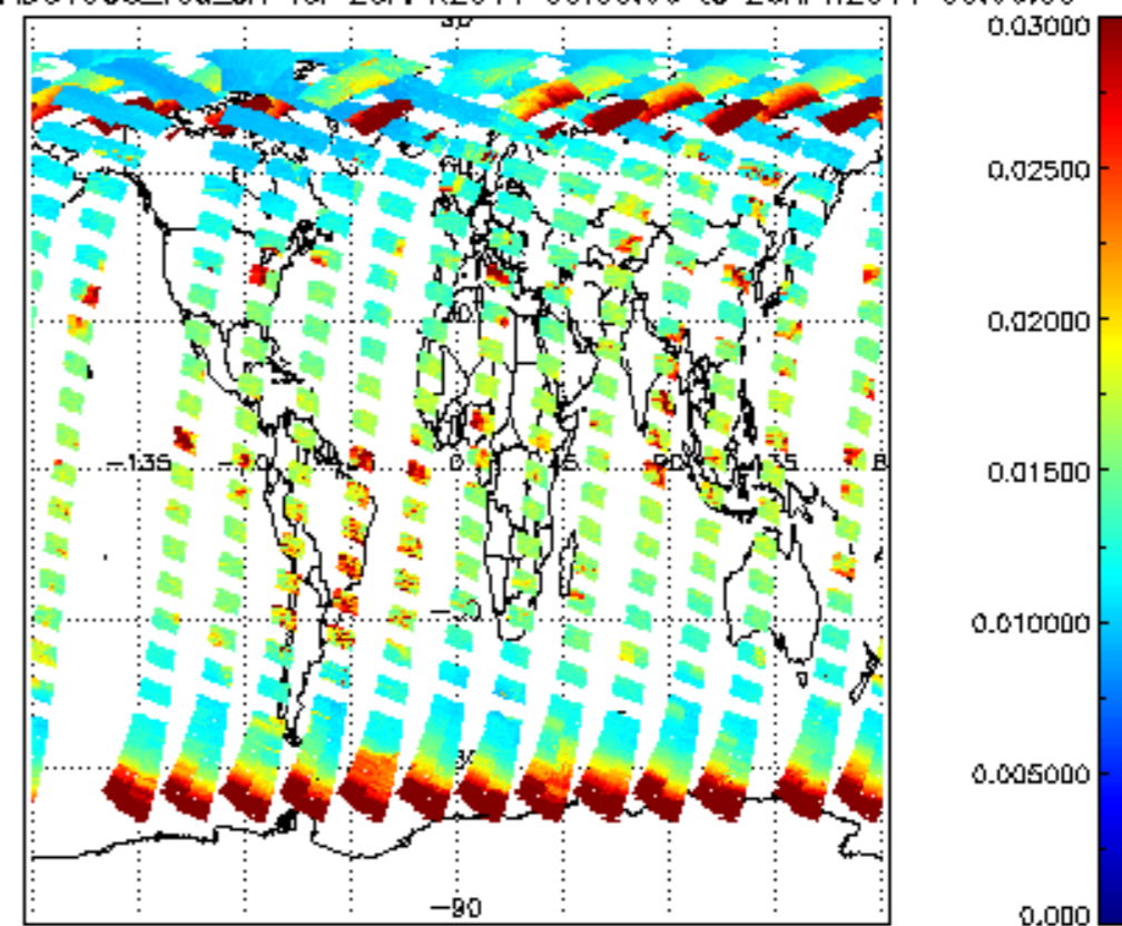
SCIOL2P_NADUV003_vcd_err for 25APR2011 00:00:00 to 26APR2011 00:00:00
