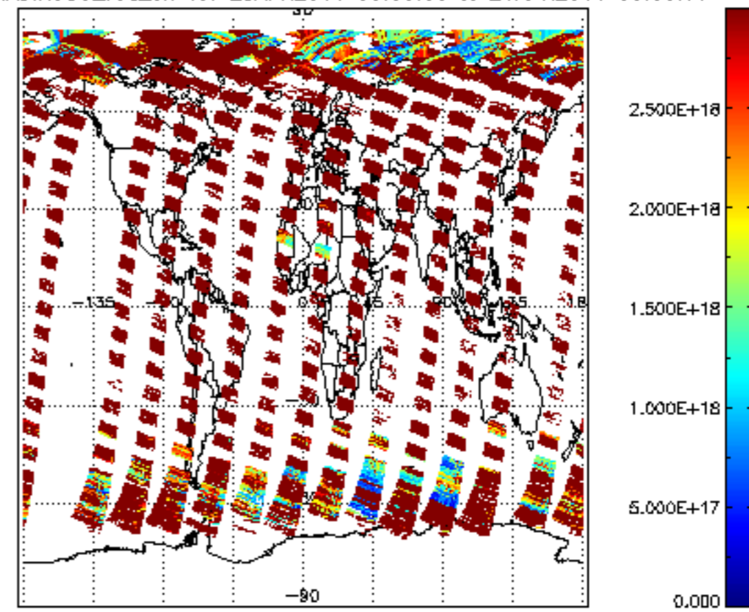
SCIOL2P_NADIR3CO_vcd_err for 25APR2011 00:00:00 to 26APR2011 00:00:00
