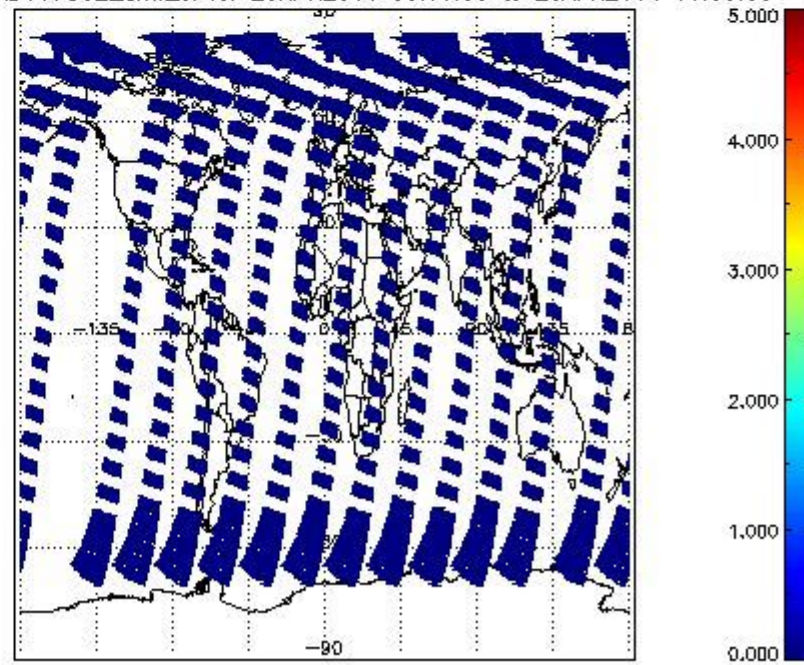
SCIOL2P_NADUV7S02_amf_cl for 25APR2011 00:00:00 to 26APR2011 00:00:00
