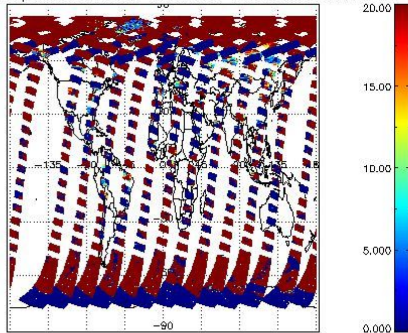
cL_opt_depth for 25APR2011 00:00:00 to 26APR2011 00:00:00
