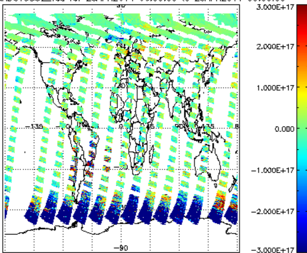
SCIOL2P_NADUV5S02_vcd for 25APR2011 00:00:00 to 26APR2011 00:00:00
