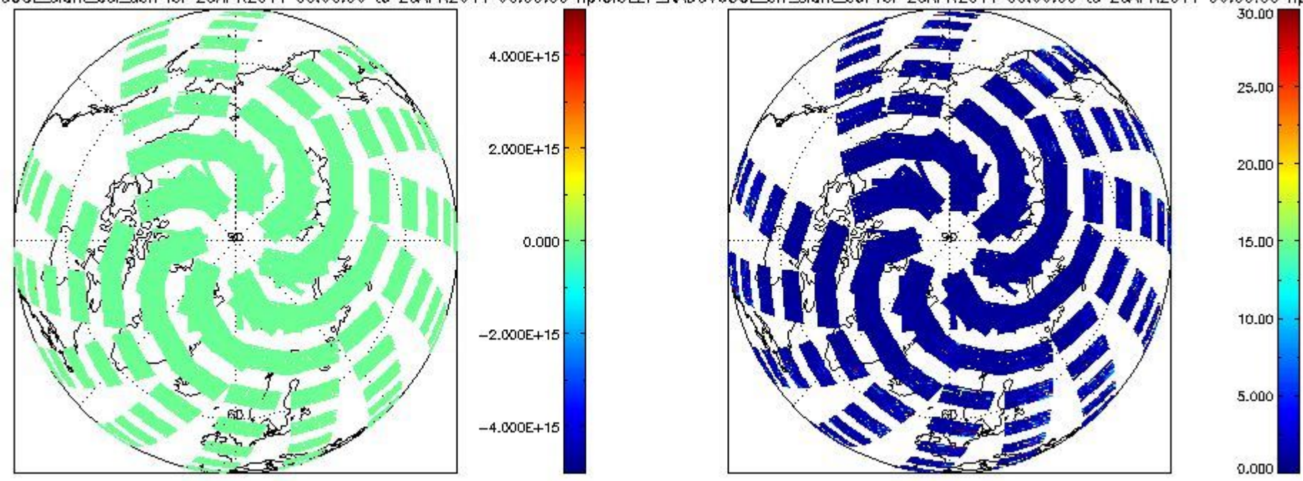
CIOL2P_NADUV60CLslant_col_den for 25APR2011 00:00:00 to 26APR2011 00:00:00 np; CIOL2P_NADUV60CLarr_slant_col for 25APR2011 00:00:00 to 26APR2011 00:00:00 np
