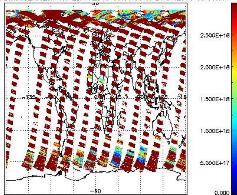
SCIDL2P_NADIR3CO_vcd_err for 25APR2011 00:00:00 to 26APR2011 00:00:00
