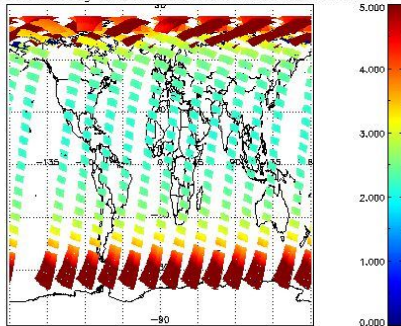
SCIOL2P_NADUV003_amf_gr for 25APR2011 00:00:00 to 26APR2011 00:00:00
