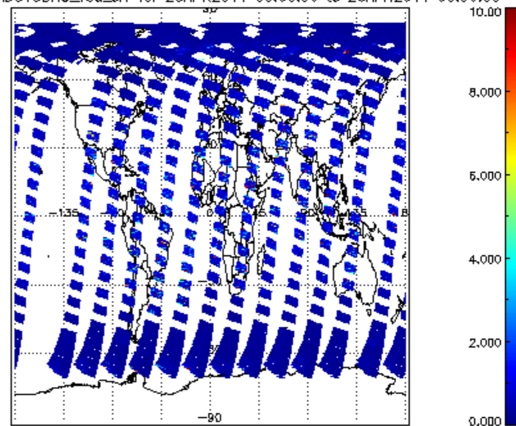
SCIOL2P_NADUV3BRO_vcd_err for 25APR2011 00:00:00 to 26APR2011 00:00:00
