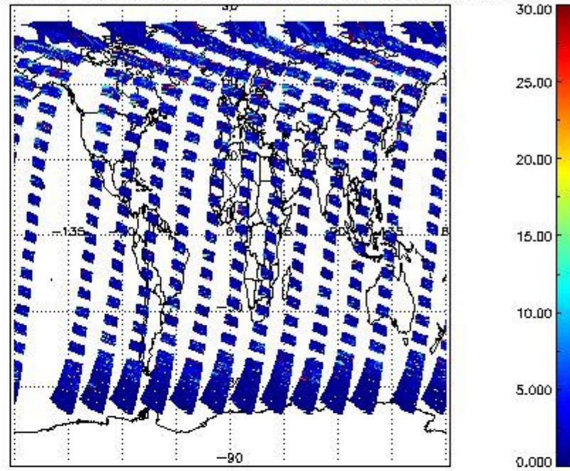
SCIOL2P_NADUV5S02_vcd_err for 25APR2011 00:00:00 to 26APR2011 00:00:00
