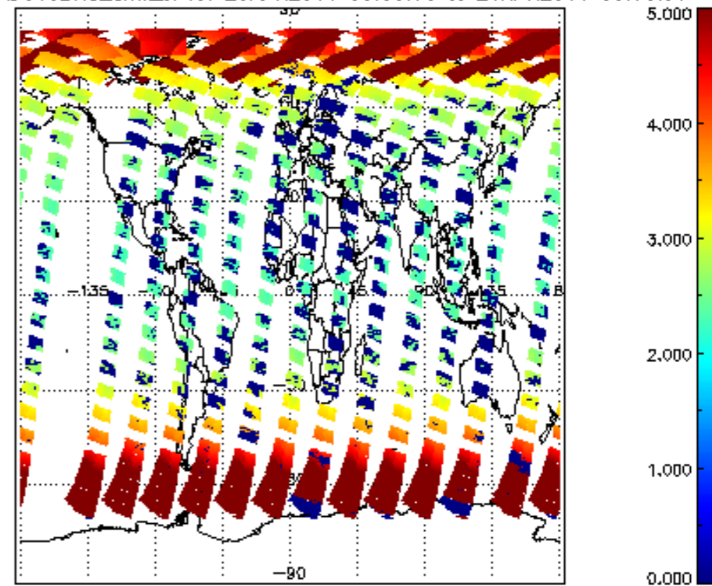
SCIOL2P_NADUV3BRO_amf_sl for 25APR2011 00:00:00 to 26APR2011 00:00:00
