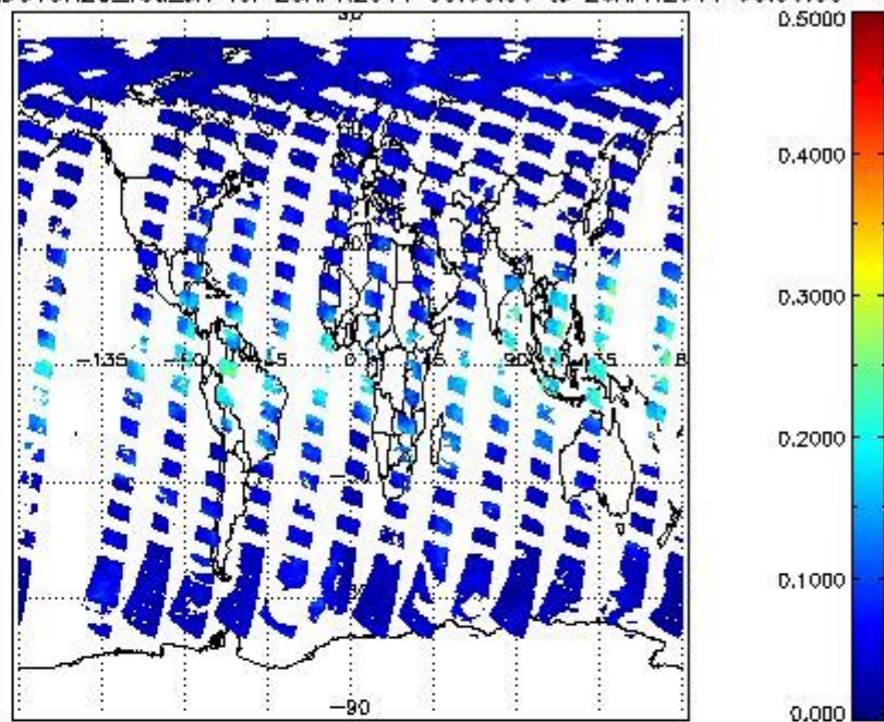
SCIOL2P_NADUV8H2O_vcd_err for 25APR2011 00:00:00 to 26APR2011 00:00:00
