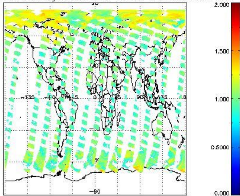
SCIOL2P_NADUV8H2O_arnf_gr for 25APR2011 00:00:00 to 26APR2011 00:00:00
