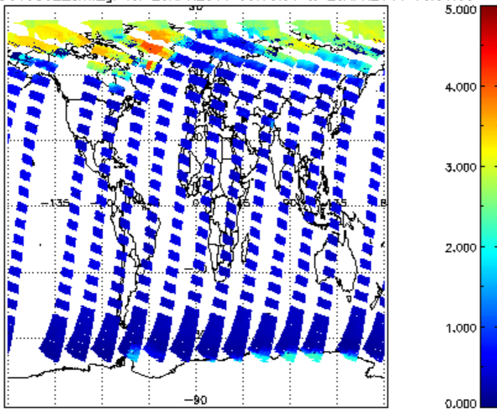
SCIOL2P_NADUV5S02_amf_gr for 25APR2011 00:00:00 to 26APR2011 00:00:00
