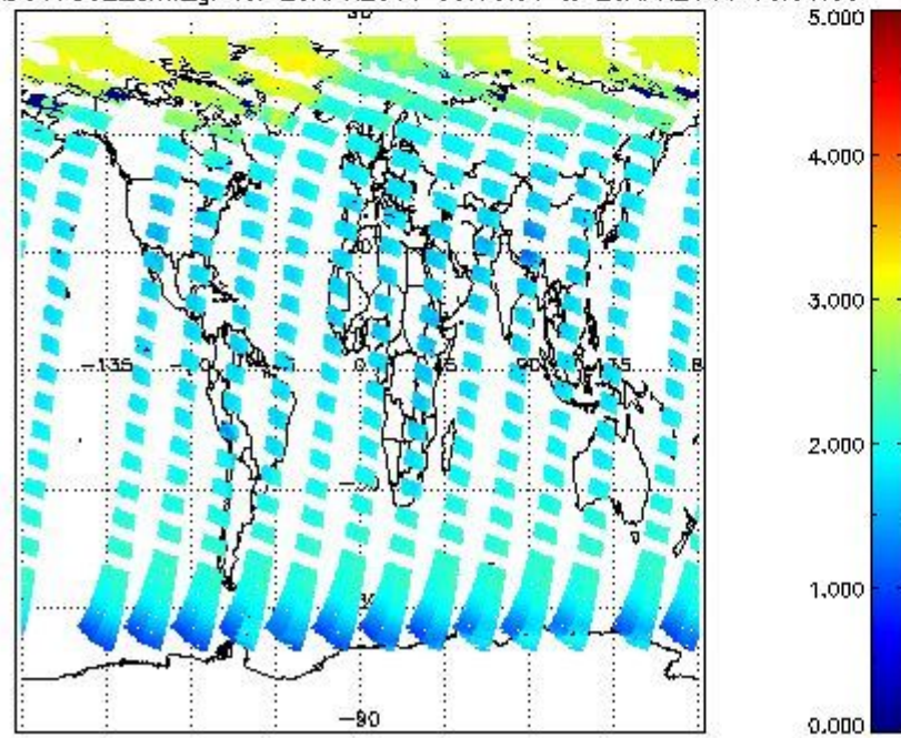
SCIOL2P_NADUV7S02_amf_gr for 25APR2011 00:00:00 to 26APR2011 00:00:00
