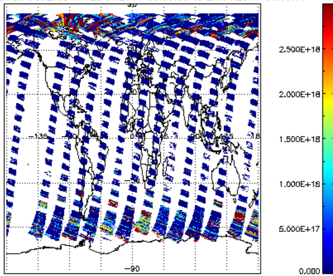
SCIOL2P_NADIR3CO_vcd for 25APR2011 00:00:00 to 26APR2011 00:00:00
