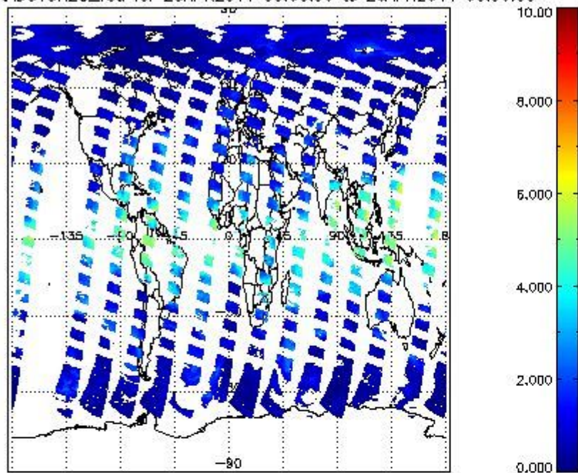
SCIOL2P_NADUV8H2O_vcd for 25APR2011 00:00:00 to 26APR2011 00:00:00
