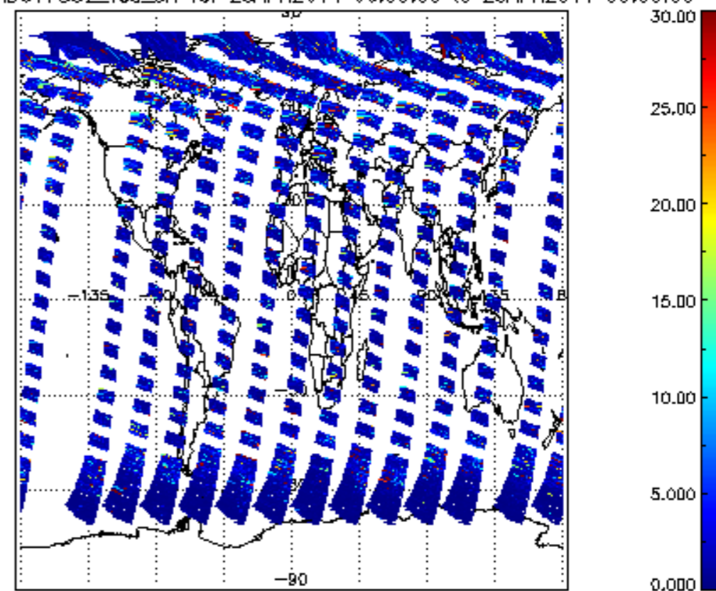
SCIOL2P_NADUV7S02_vcd_err for 25APR2011 00:00:00 to 26APR2011 00:00:00
