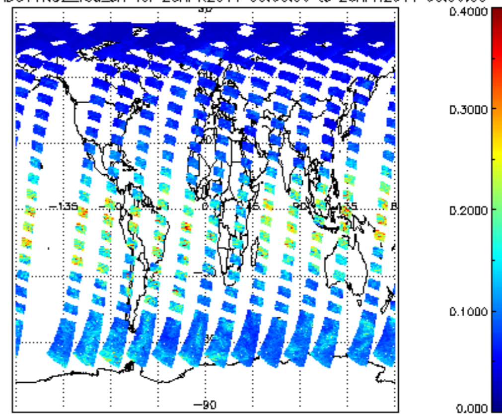
SCIOL2P_NADUV1NO2_vcd_err for 25APR2011 00:00:00 to 26APR2011 00:00:00
