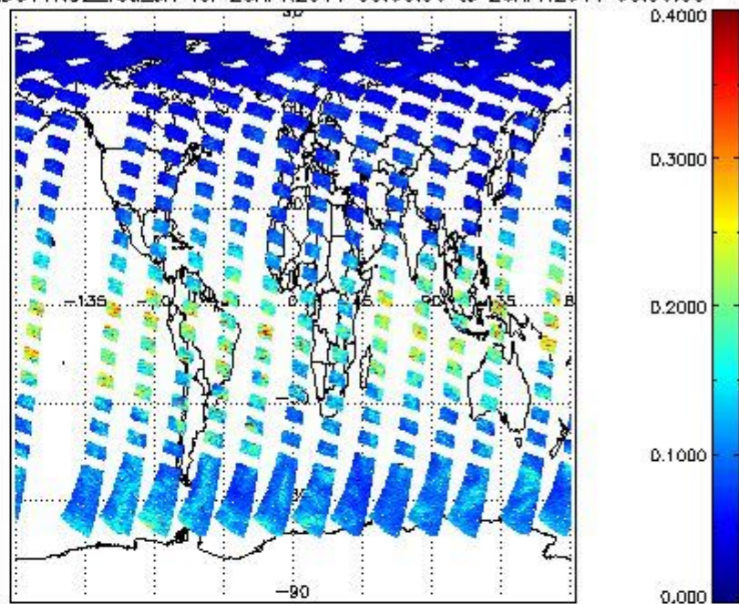
SCIOL2P_NADUV1NO2_vcd_err for 25APR2011 00:00:00 to 26APR2011 00:00:00
