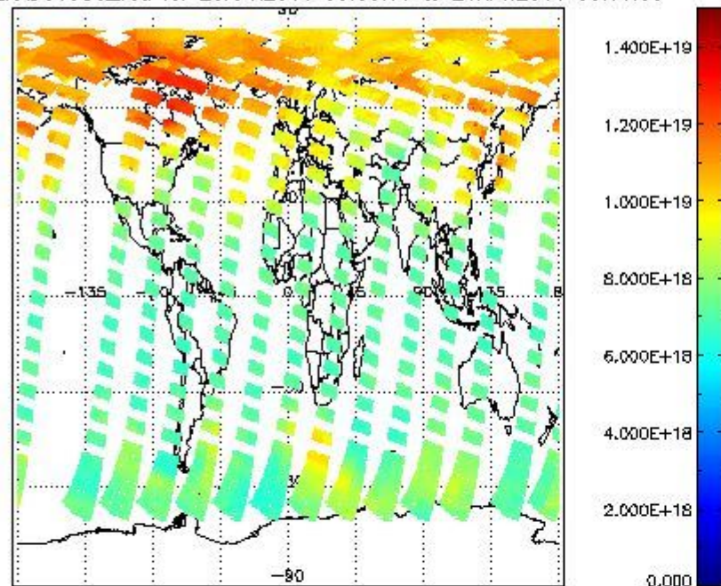
SCIOL2P_NADUV003_vcd for 25APR2011 00:00:00 to 26APR2011 00:00:00
