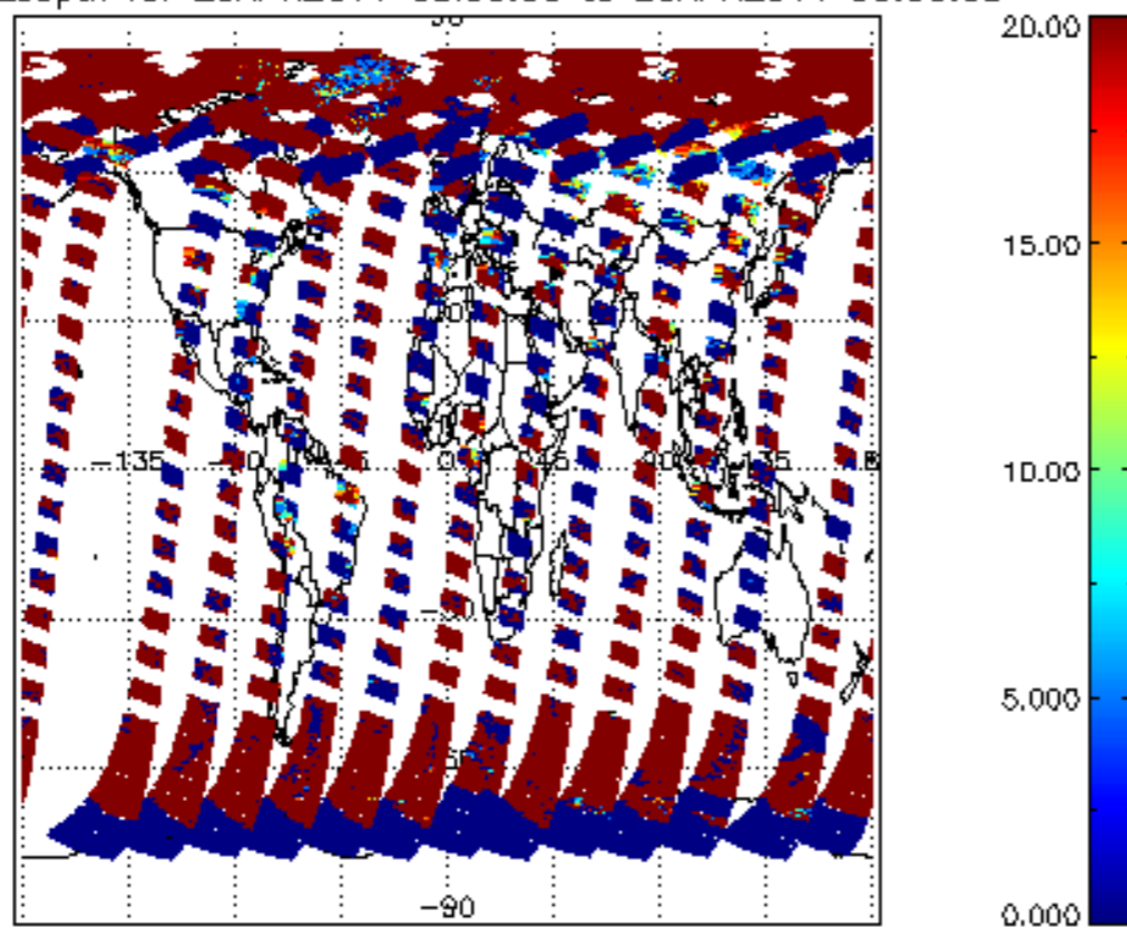
cL_opt_depth for 25APR2011 00:00:00 to 26APR2011 00:00:00
