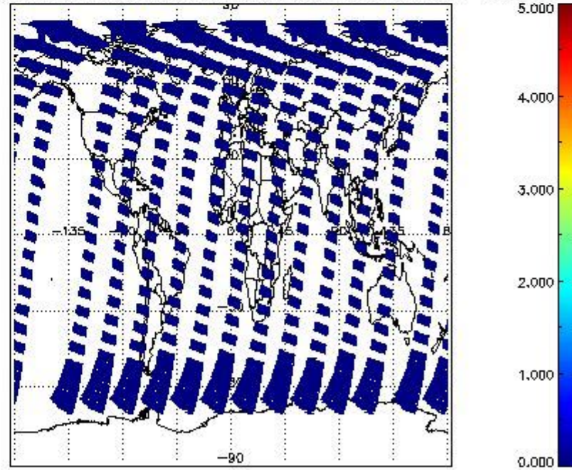
SCIOL2P_NADUV5S02_amf_cl for 25APR2011 00:00:00 to 26APR2011 00:00:00
