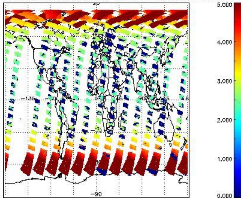
SCIOL2P_NADUV003_amf_cl for 25APR2011 00:00:00 to 26APR2011 00:00:00
