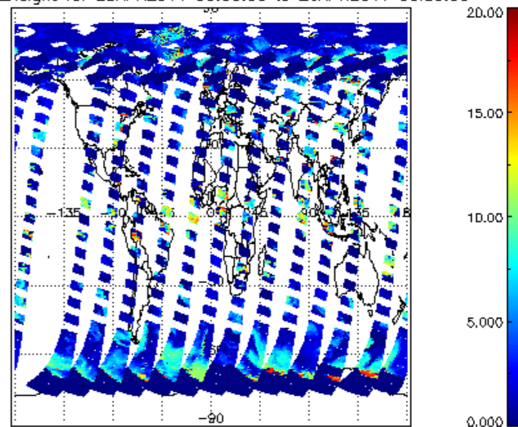
cL_top_height for 25APR2011 00:00:00 to 26APR2011 00:00:00
