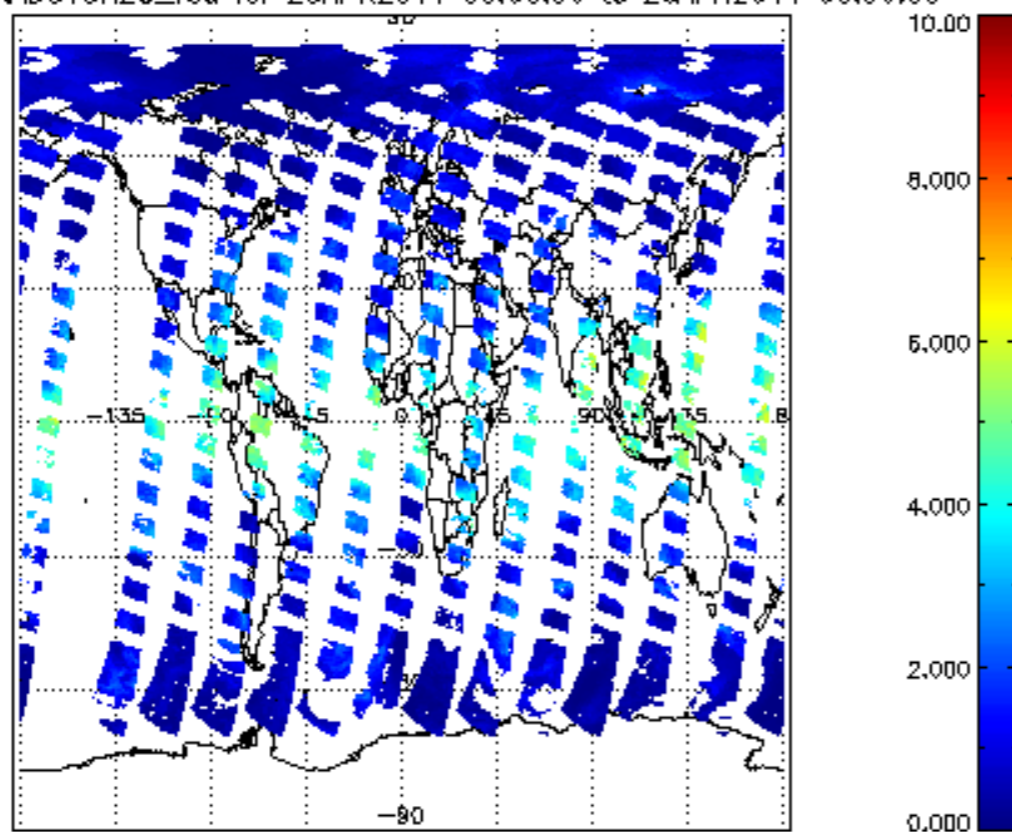
SCIOL2P_NADUV8H2O_vcd for 25APR2011 00:00:00 to 26APR2011 00:00:00
