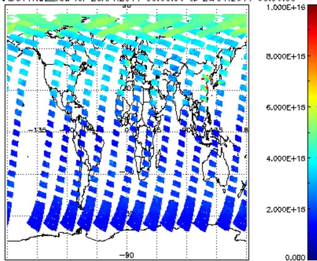
SCIOL2P_NADUV1NO2_vcd for 25APR2011 00:00:00 to 26APR2011 00:00:00
