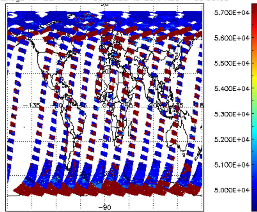
cloud_flags for 25APR2011 00:00:00 to 26APR2011 00:00:00
