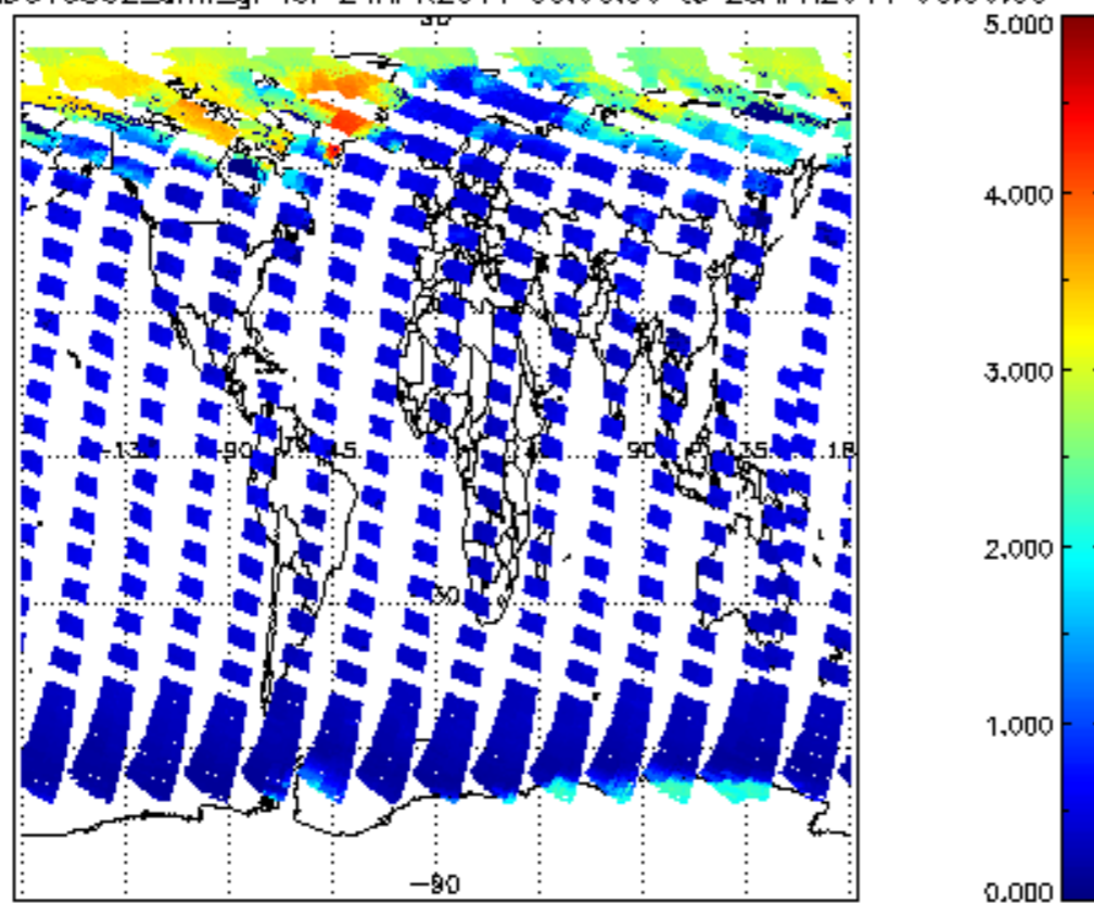
SCIOL2P_NADUV5S02_amf_gr for 24APR2011 00:00:00 to 25APR2011 00:00:00
