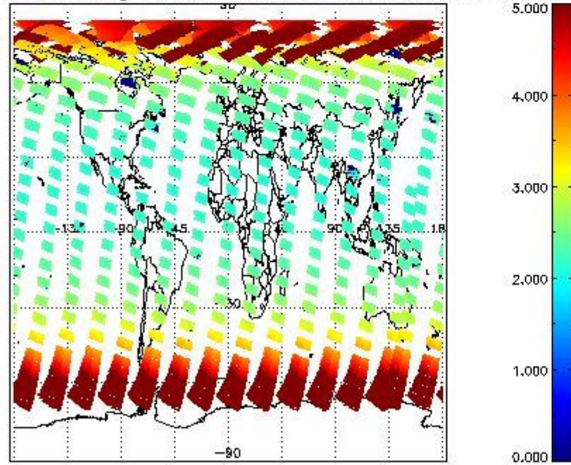
SCIOL2P_NADUV003_amf_gr for 24APR2011 00:00:00 to 25APR2011 00:00:00
