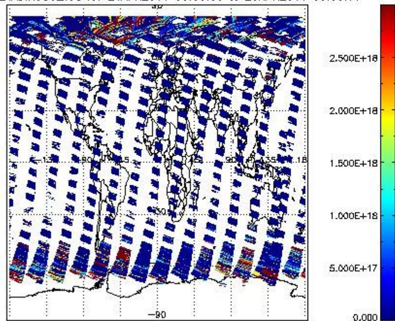
SCIOL2P_NADIR3CO_vcd for 24APR2011 00:00:00 to 25APR2011 00:00:00
