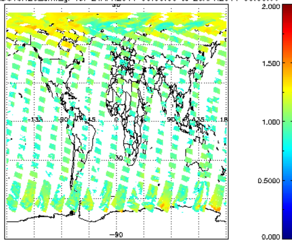
SCIOL2P_NADUV8H20_amf_gr for 24APR2011 00:00:00 to 25APR2011 00:00:00
