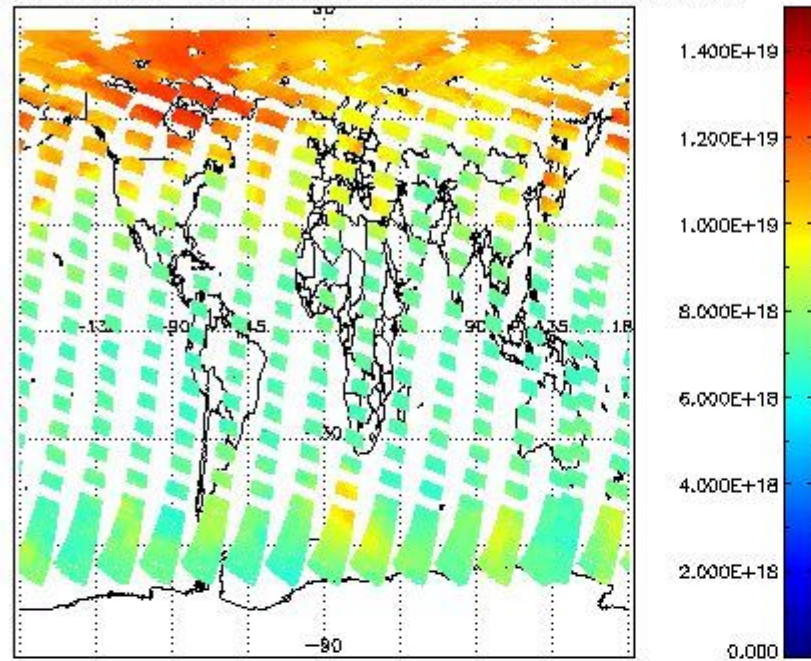
SCIOL2P_NADUV003_vcd for 24APR2011 00:00:00 to 25APR2011 00:00:00
