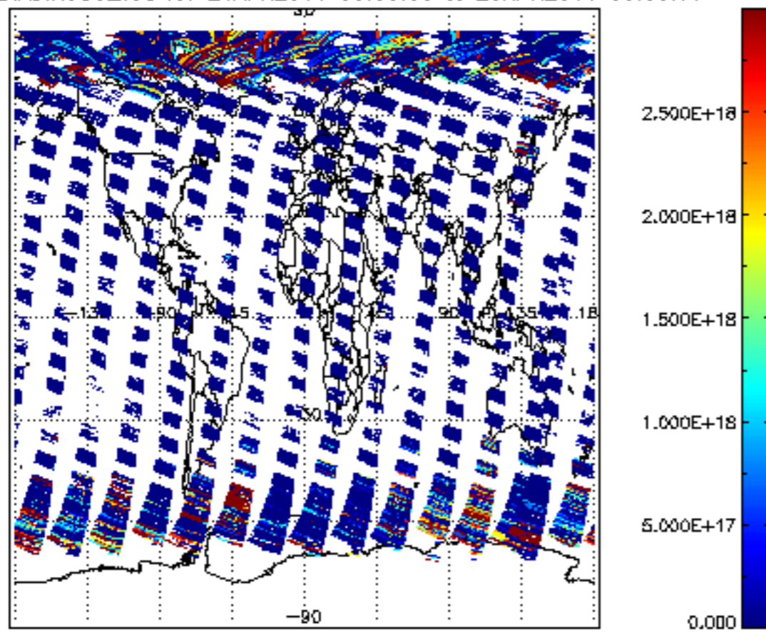
SCIOL2P_NADIR3CO_vcd for 24APR2011 00:00:00 to 25APR2011 00:00:00
