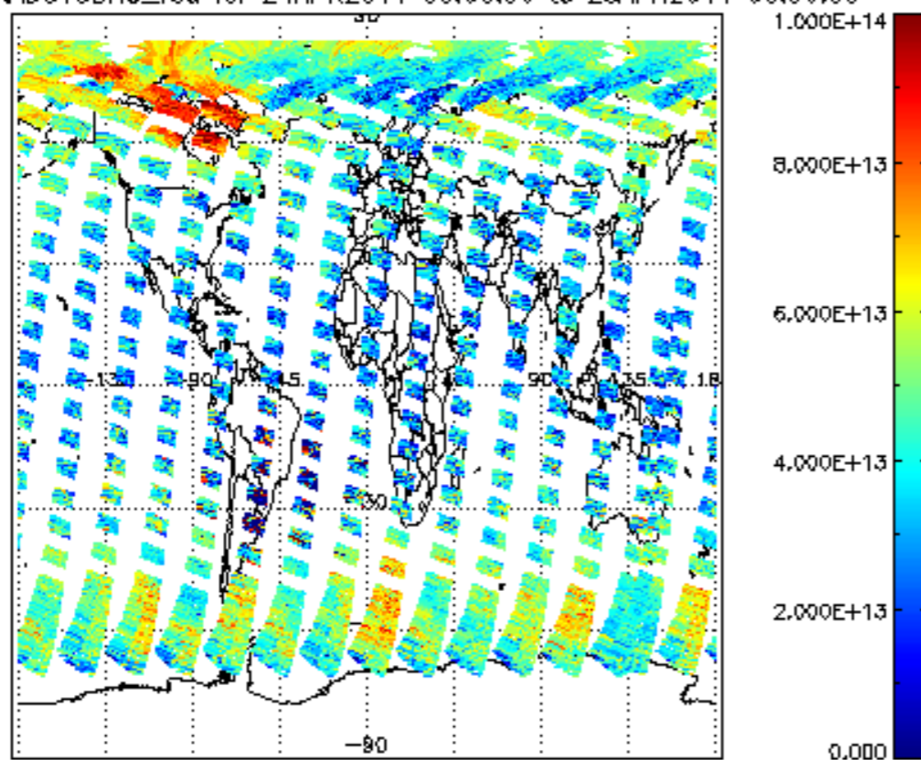
SCIOL2P_NADUV3BRO_vcd for 24APR2011 00:00:00 to 25APR2011 00:00:00
