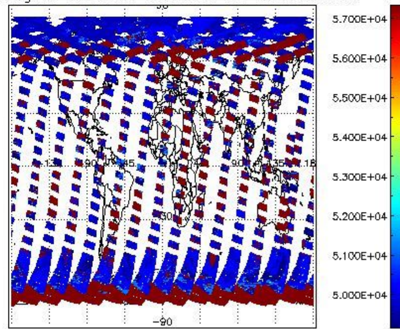
cloud_flags for 24APR2011 00:00:00 to 25APR2011 00:00:00
