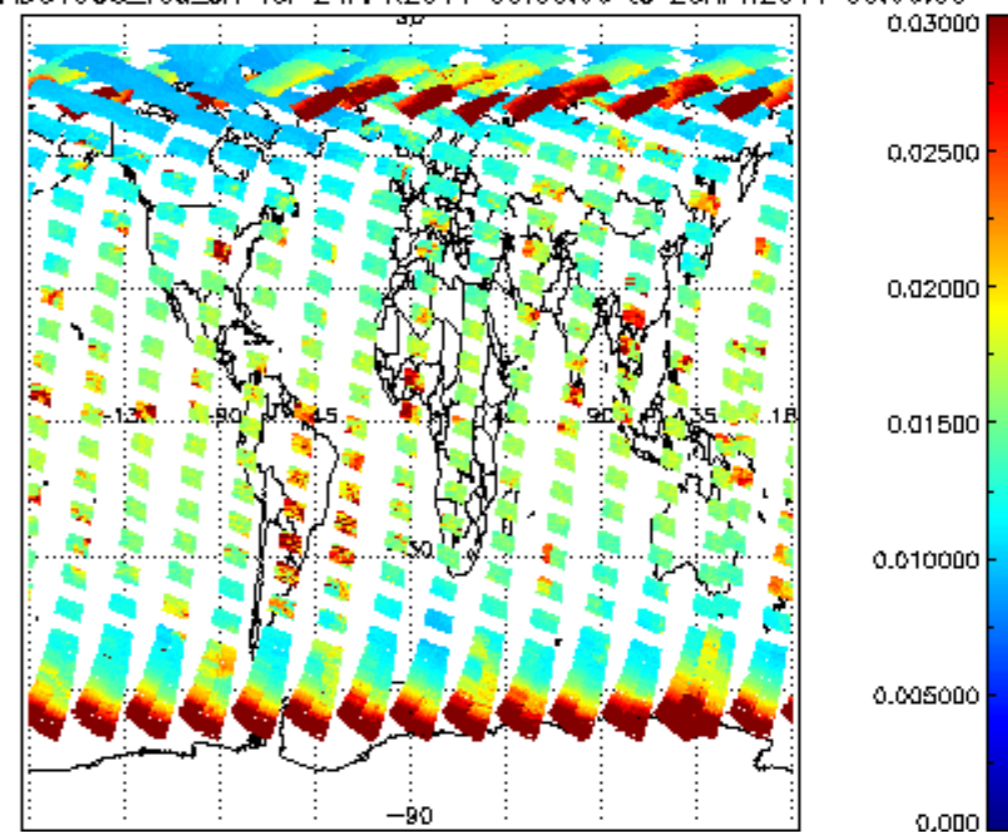
SCIOL2P_NADUV003_vcd_err for 24APR2011 00:00:00 to 25APR2011 00:00:00
