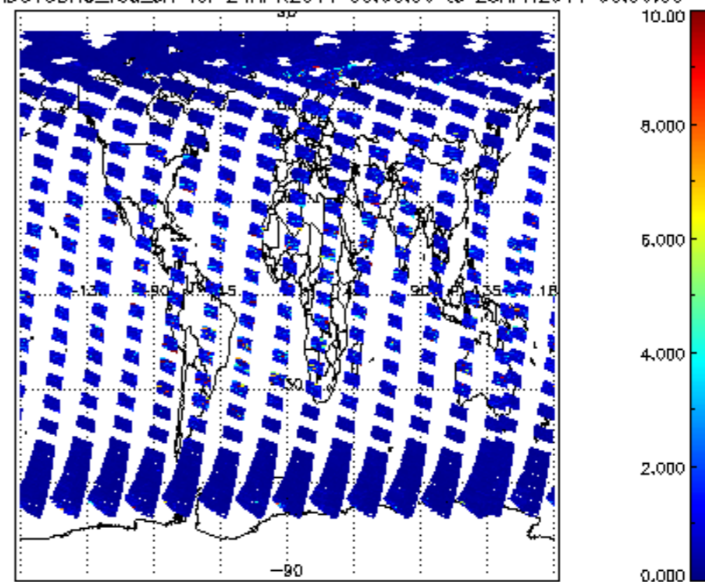
SCIOL2P_NADUV3BRO_vcd_err for 24APR2011 00:00:00 to 25APR2011 00:00:00
