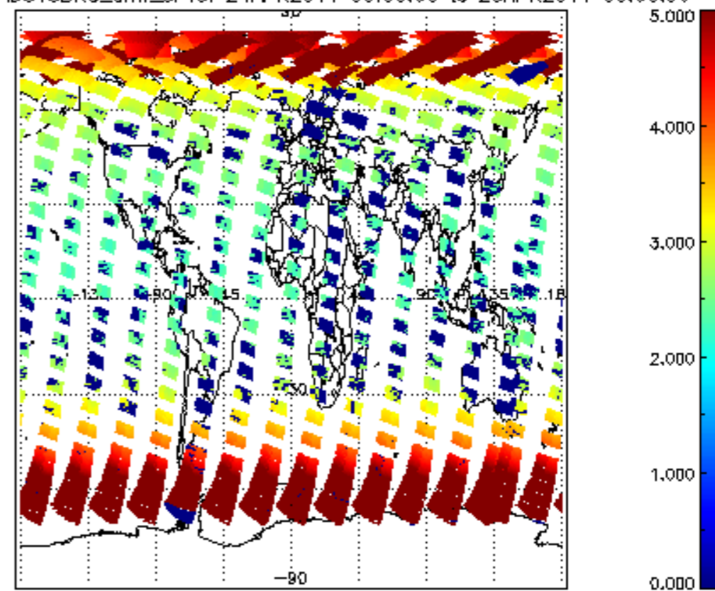
SCIOL2P_NADUV3BRO_amf_sl for 24APR2011 00:00:00 to 25APR2011 00:00:00
