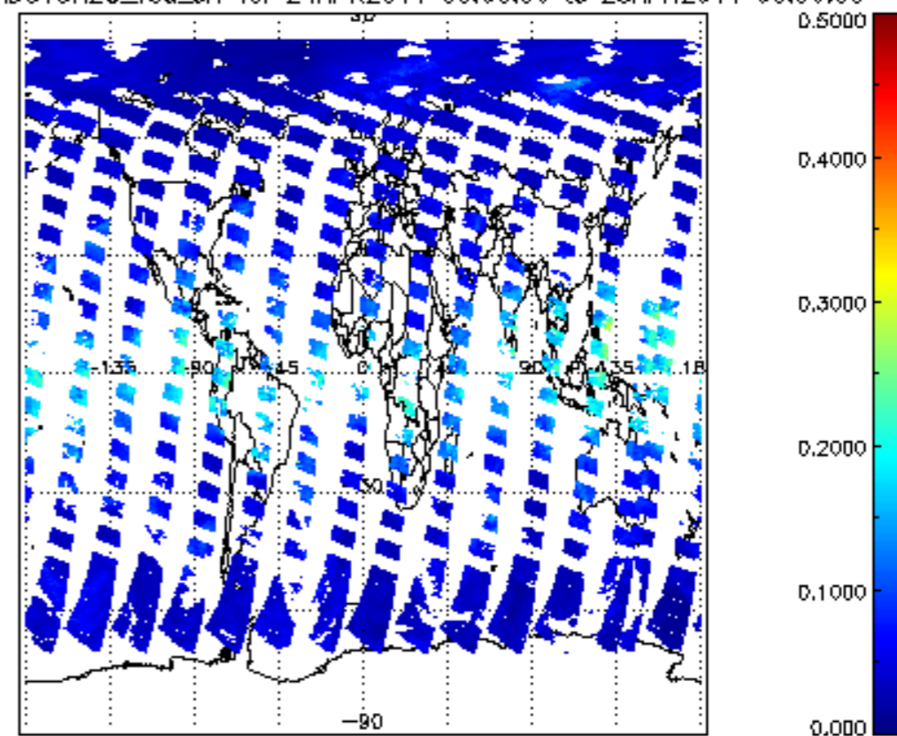
SCIOL2P_NADUV8H20_vcd_err for 24APR2011 00:00:00 to 25APR2011 00:00:00
