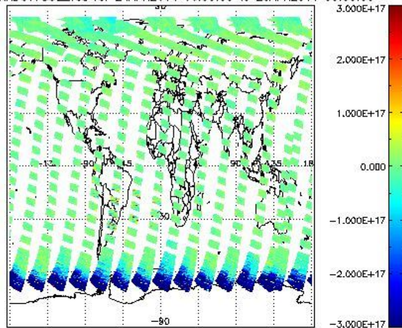
SCIOL2P_NADUV7S02_vcd for 24APR2011 00:00:00 to 25APR2011 00:00:00
