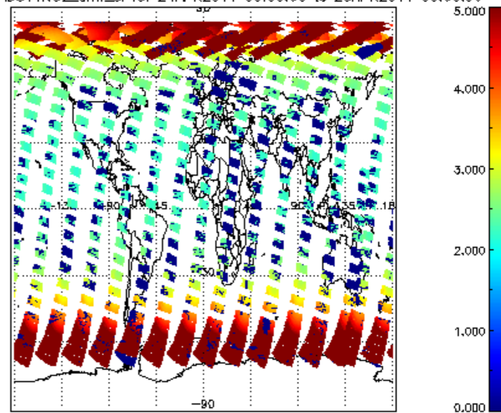
SCIOL2P_NADUV1NO2_amf_sl for 24APR2011 00:00:00 to 25APR2011 00:00:00
