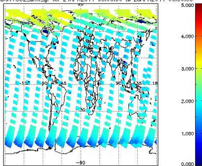
SCIOL2P_NADUV7S02_amf_gr for 24APR2011 00:00:00 to 25APR2011 00:00:00
