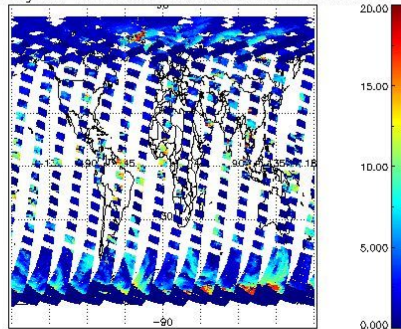
cL_top_height for 24APR2011 00:00:00 to 25APR2011 00:00:00
