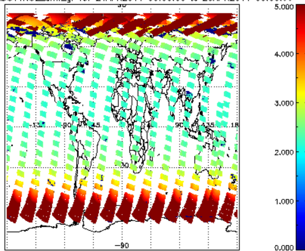
SCIOL2P_NADUV1NO2_amf_gr for 24APR2011 00:00:00 to 25APR2011 00:00:00
