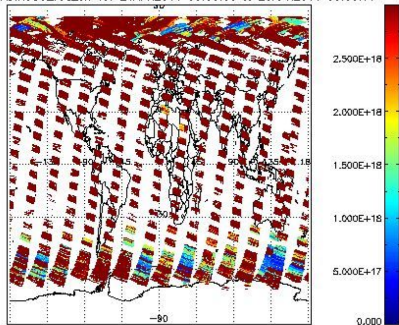
SCIOL2P_NADIR3CO_vcd_err for 24APR2011 00:00:00 to 25APR2011 00:00:00
