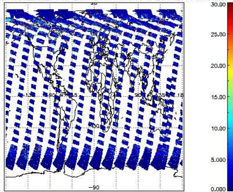
SCIOL2P_NADUV5S02_vcd_err for 24APR2011 00:00:00 to 25APR2011 00:00:00
