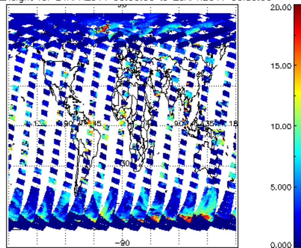
cL_top_height for 24APR2011 00:00:00 to 25APR2011 00:00:00
