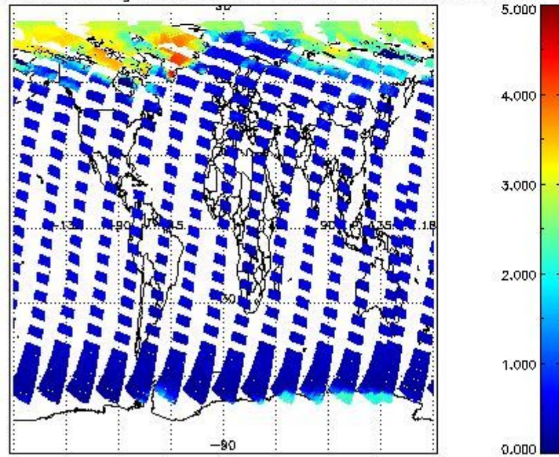
SCIOL2P_NADUV5S02_amf_gr for 24APR2011 00:00:00 to 25APR2011 00:00:00
