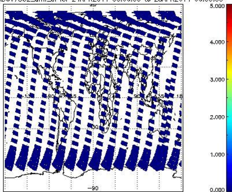
SCIOL2P_NADUV7S02_amf_cl for 24APR2011 00:00:00 to 25APR2011 00:00:00
