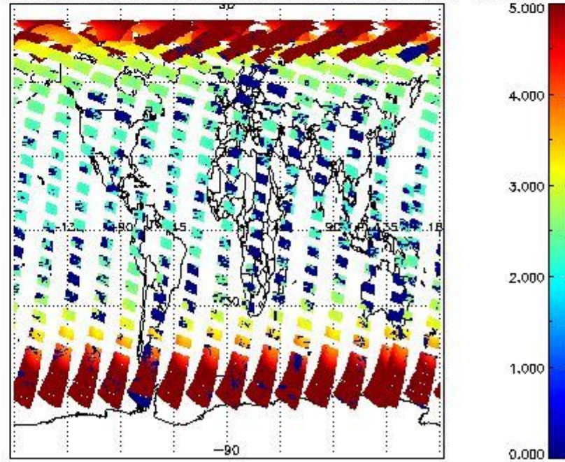
SCIOL2P_NADUV1NO2_amf_cl for 24APR2011 00:00:00 to 25APR2011 00:00:00
