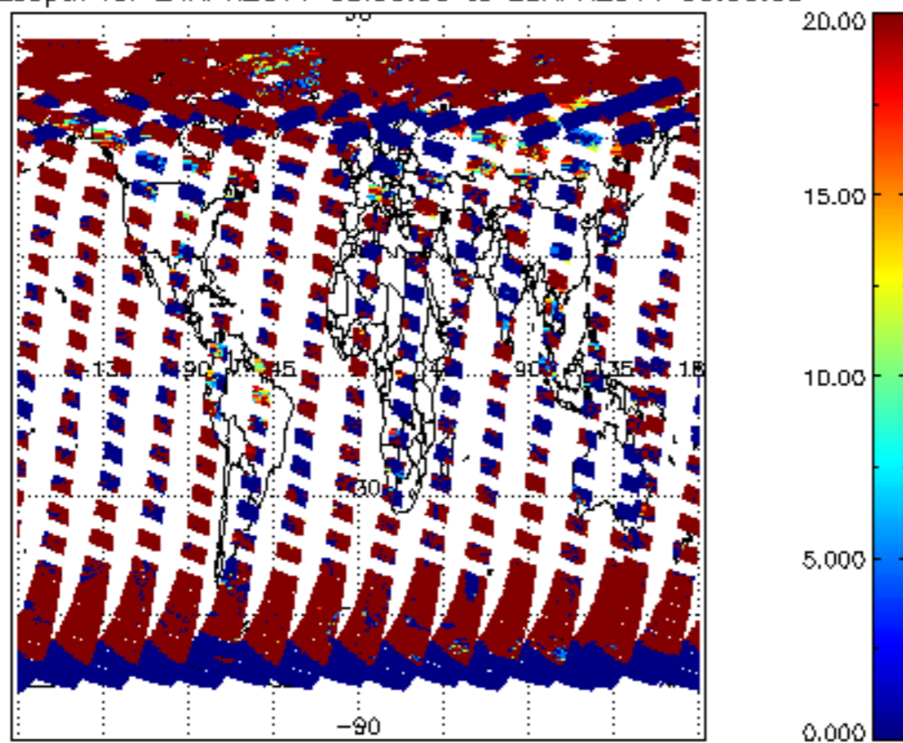
cL_opt_depth for 24APR2011 00:00:00 to 25APR2011 00:00:00
