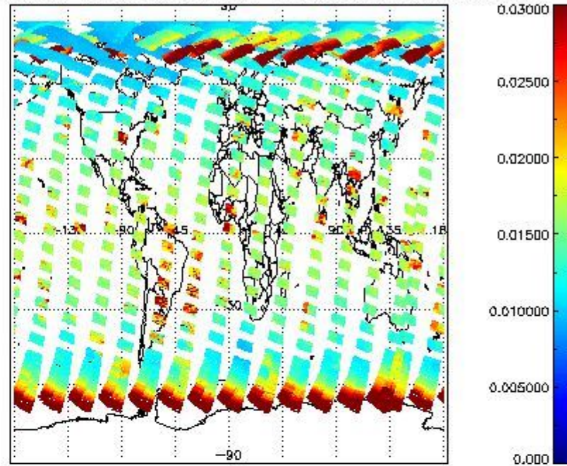
SCIOL2P_NADUV003_vcd_err for 24APR2011 00:00:00 to 25APR2011 00:00:00
