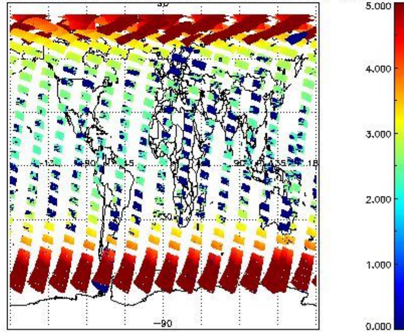
SCIOL2P_NADUV3BRO_amf_cl for 24APR2011 00:00:00 to 25APR2011 00:00:00
