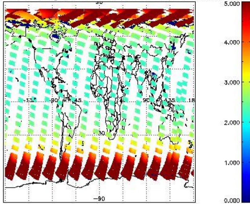
SCIOL2P_NADUV1NO2_amf_gr for 24APR2011 00:00:00 to 25APR2011 00:00:00
