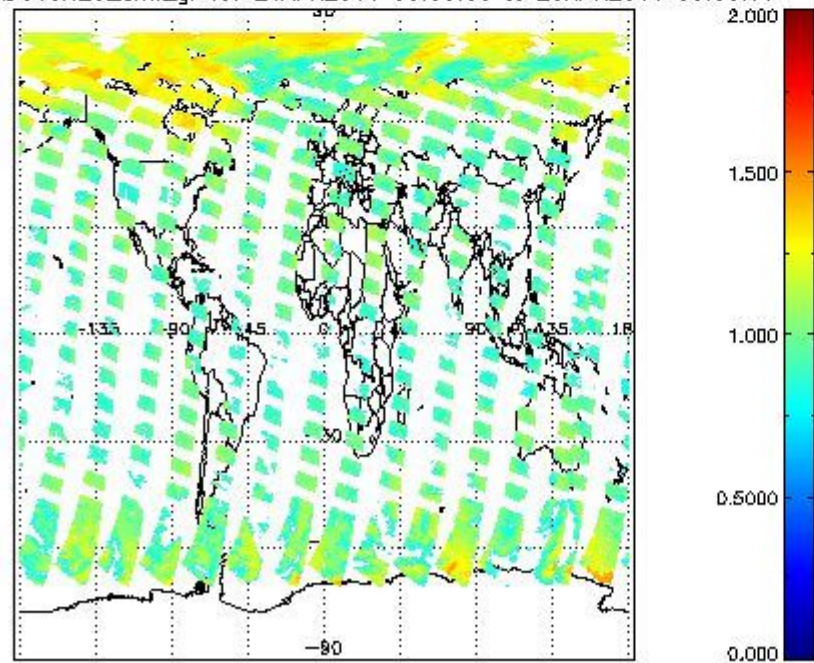
SCIOL2P_NADUV8H2O_arnf_gr for 24APR2011 00:00:00 to 25APR2011 00:00:00
