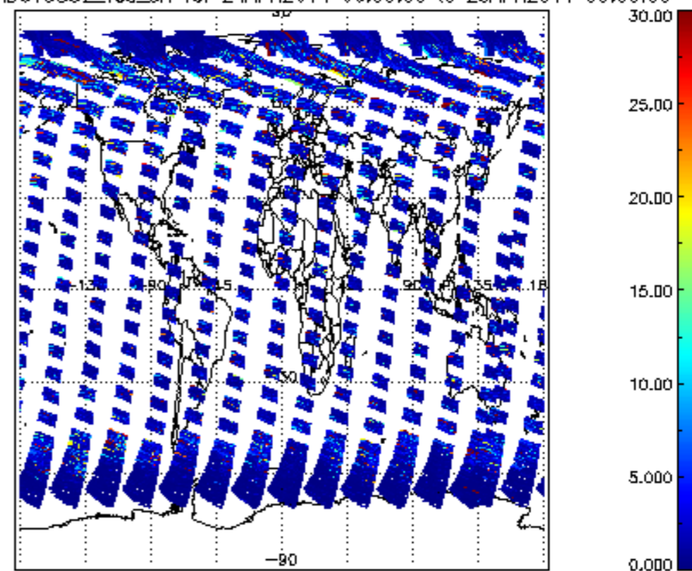
SCIOL2P_NADUV5S02_vcd_err for 24APR2011 00:00:00 to 25APR2011 00:00:00
