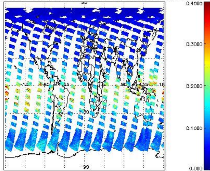
SCIOL2P_NADUV1NO2_vcd_err for 24APR2011 00:00:00 to 25APR2011 00:00:00
