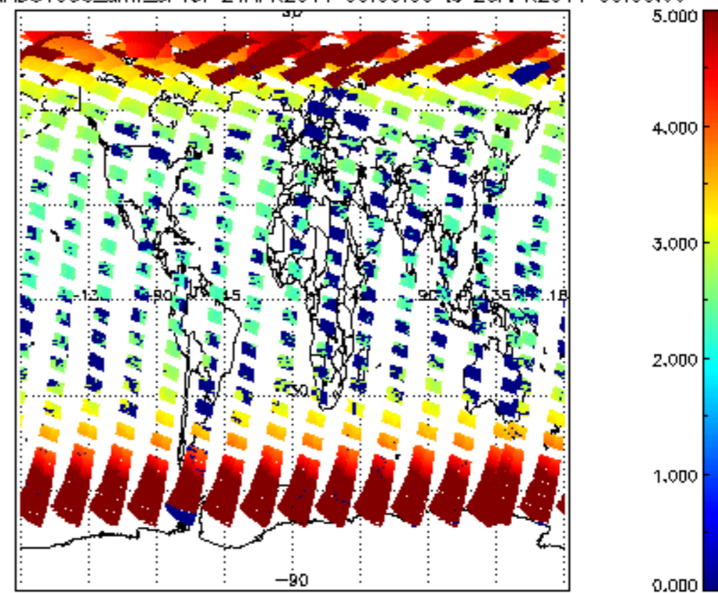
SCIOL2P_NADUV003_amf_cl for 24APR2011 00:00:00 to 25APR2011 00:00:00
