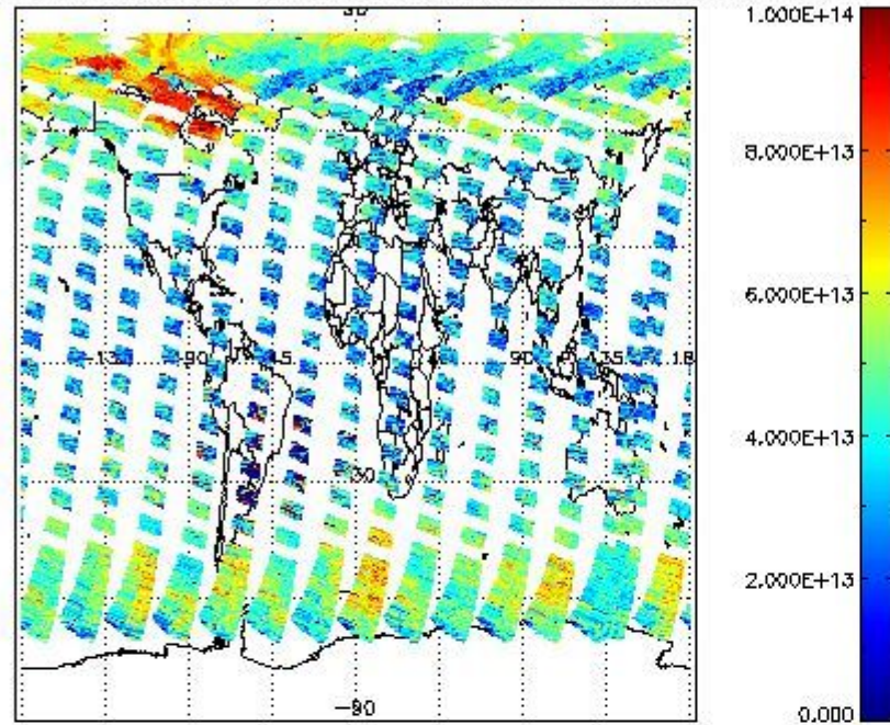
SCIOL2P_NADUV3BRO_vcd for 24APR2011 00:00:00 to 25APR2011 00:00:00
