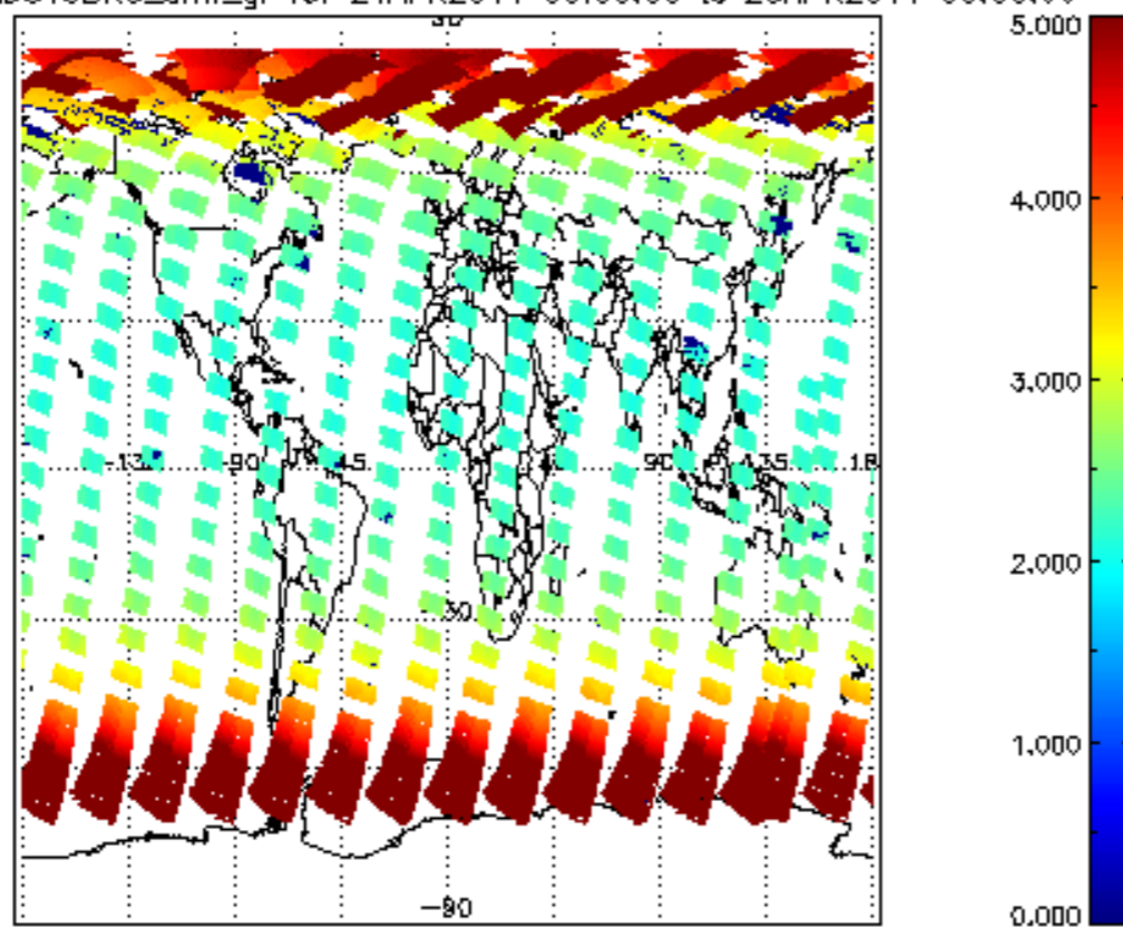
SCIOL2P_NADUV3BRO_amf_gr for 24APR2011 00:00:00 to 25APR2011 00:00:00
