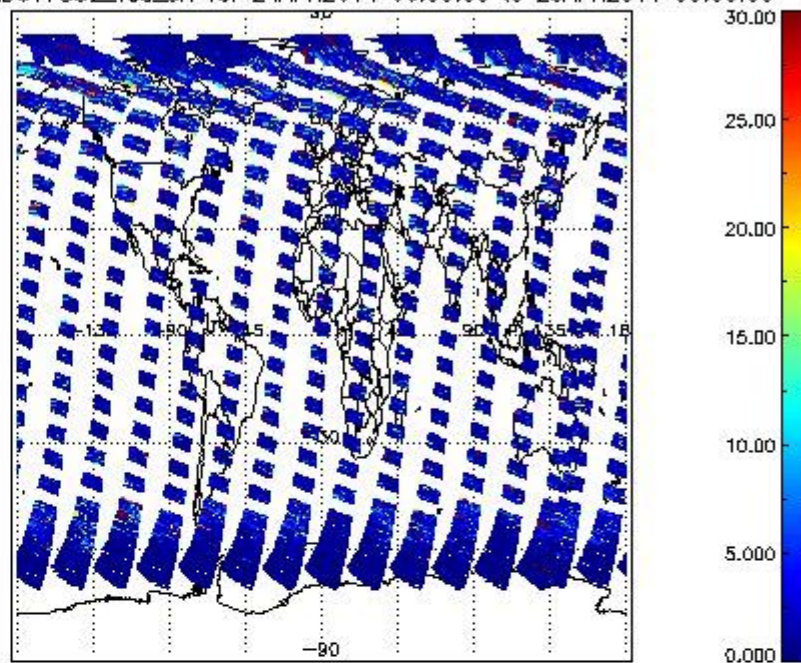
SCIOL2P_NADUV7S02_vcd_err for 24APR2011 00:00:00 to 25APR2011 00:00:00
