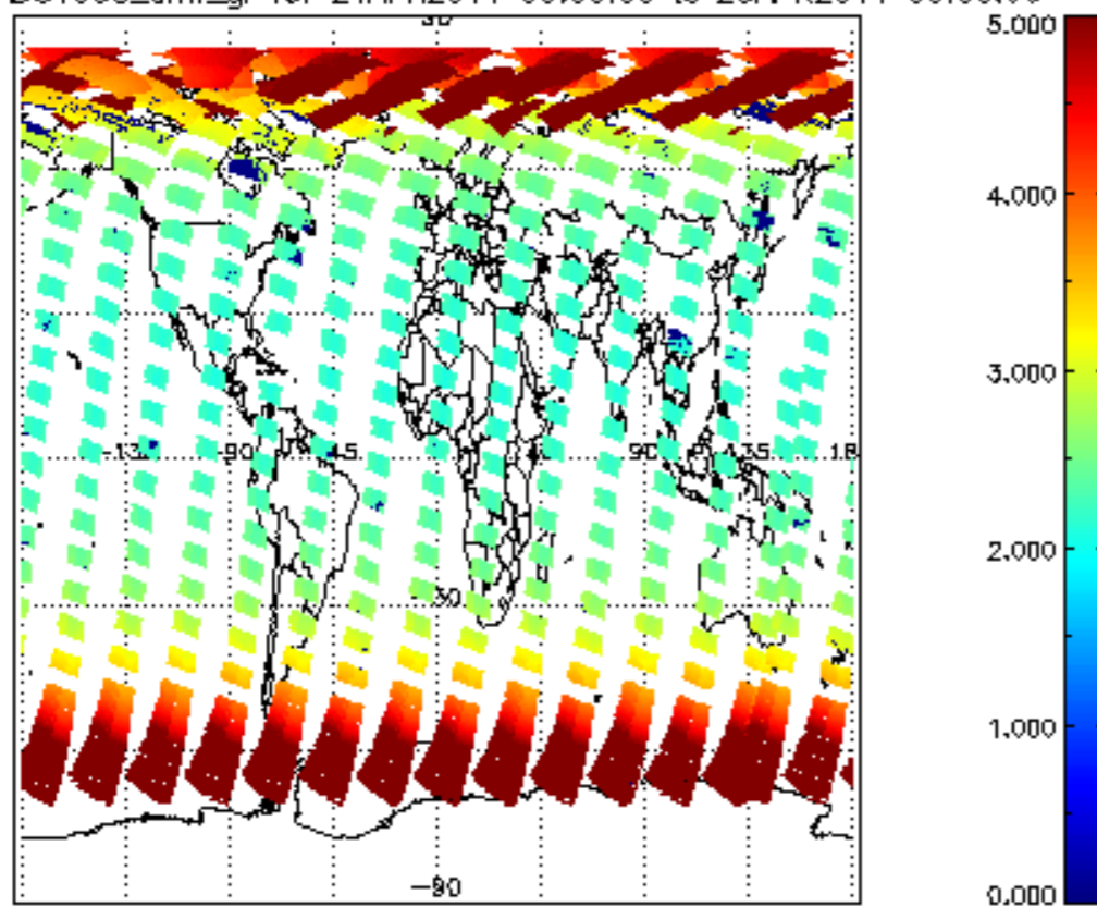
SCIOL2P_NADUV003_amf_gr for 24APR2011 00:00:00 to 25APR2011 00:00:00
