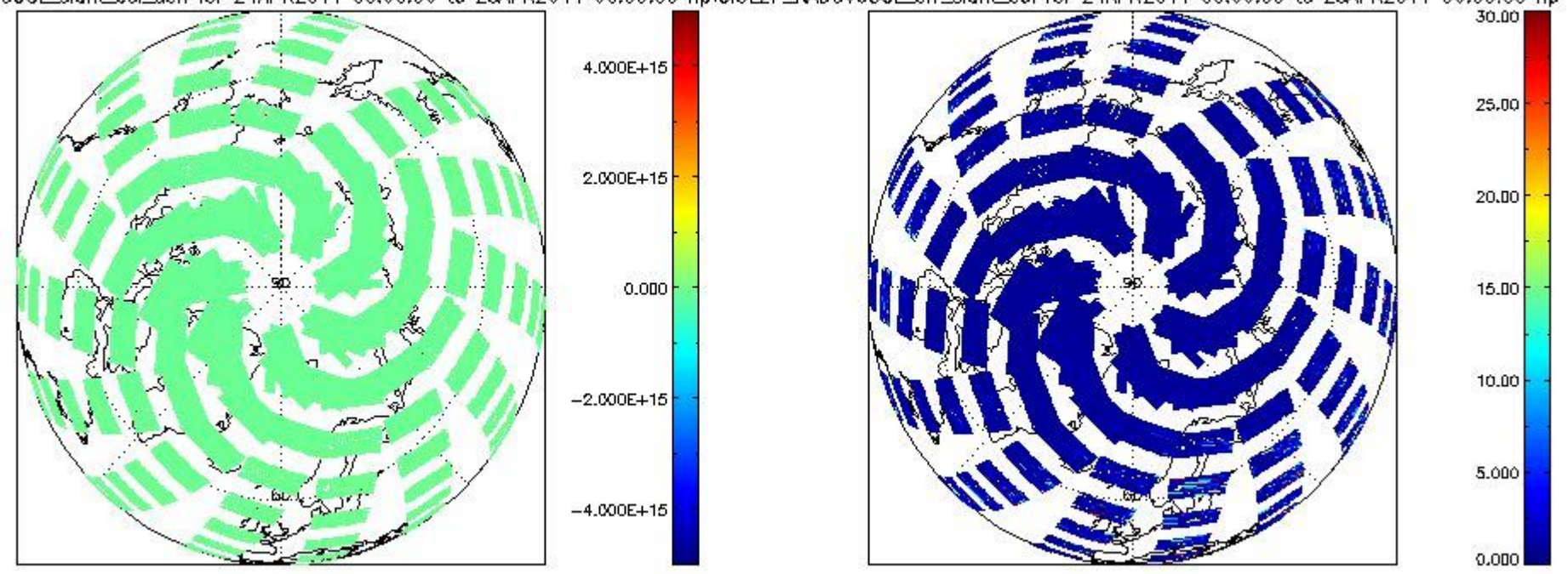
CIOL2P_NADUV60CLslant_col_den for 24APR2011 00:00:00 to 25APR2011 00:00:00 np; CIOL2P_NADUV60CLerr_slant_col for 24APR2011 00:00:00 to 25APR2011 00:00:00 np
