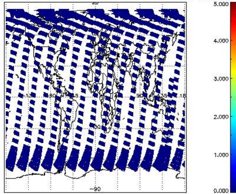
SCIOL2P_NADUV5S02_amf_cl for 24APR2011 00:00:00 to 25APR2011 00:00:00
