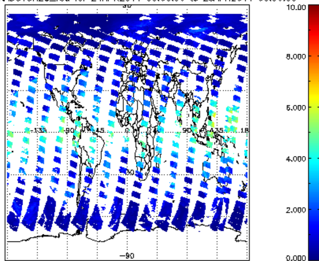
SCIOL2P_NADUV8H20_vcd for 24APR2011 00:00:00 to 25APR2011 00:00:00
