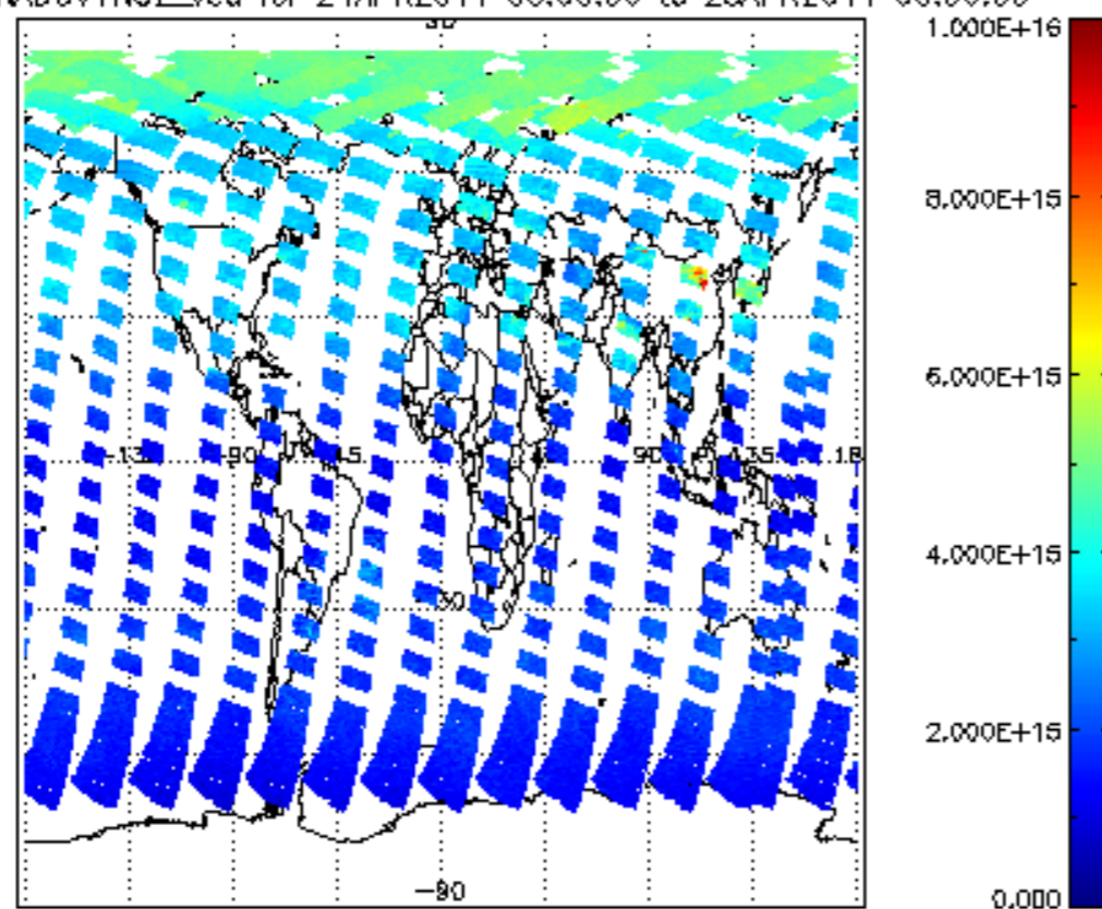
SCIOL2P_NADUV1NO2_vcd for 24APR2011 00:00:00 to 25APR2011 00:00:00
