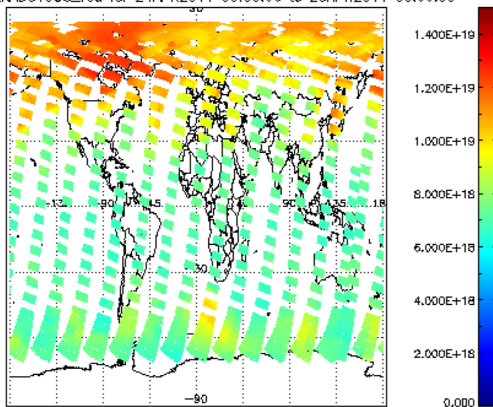
SCIOL2P_NADUV003_vcd for 24APR2011 00:00:00 to 25APR2011 00:00:00
