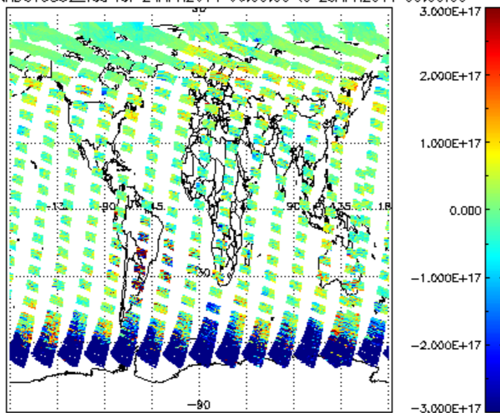
SCIOL2P_NADUV5S02_vcd for 24APR2011 00:00:00 to 25APR2011 00:00:00
