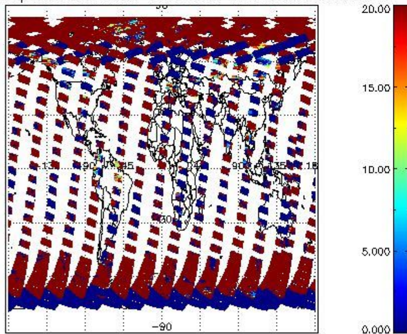
cL_opt_depth for 24APR2011 00:00:00 to 25APR2011 00:00:00
