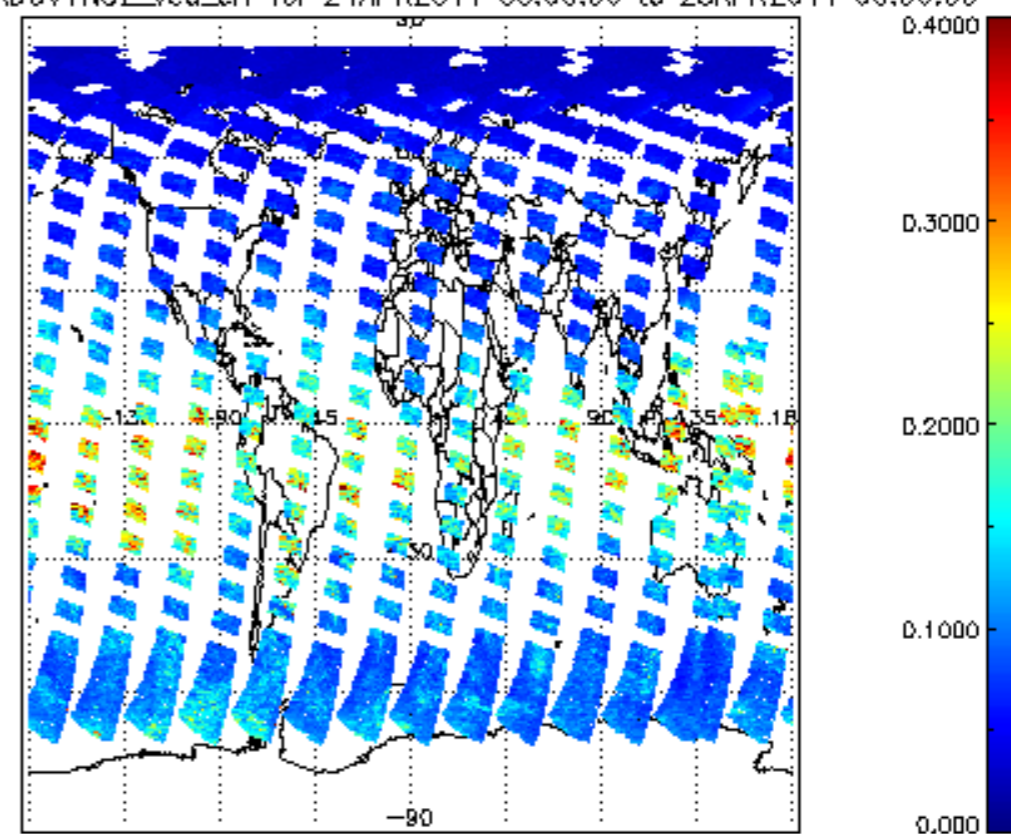
SCIOL2P_NADUV1NO2_vcd_err for 24APR2011 00:00:00 to 25APR2011 00:00:00
