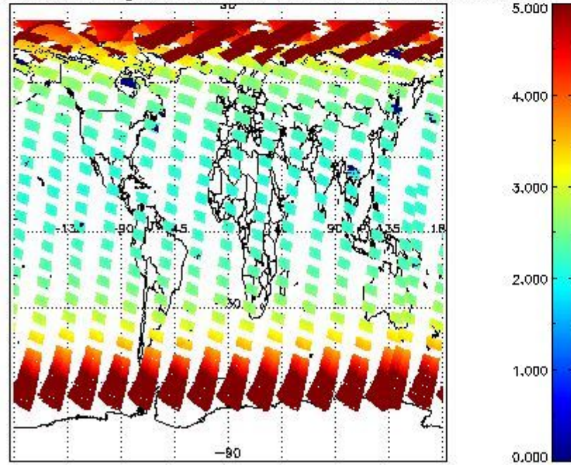
SCIOL2P_NADUV3BRO_amf_gr for 24APR2011 00:00:00 to 25APR2011 00:00:00
