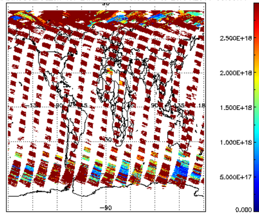
SCIOL2P_NADIR3CO_vcd_err for 24APR2011 00:00:00 to 25APR2011 00:00:00
