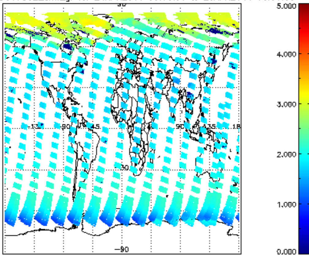
SCIOL2P_NADUV7S02_amf_gr for 24APR2011 00:00:00 to 25APR2011 00:00:00
