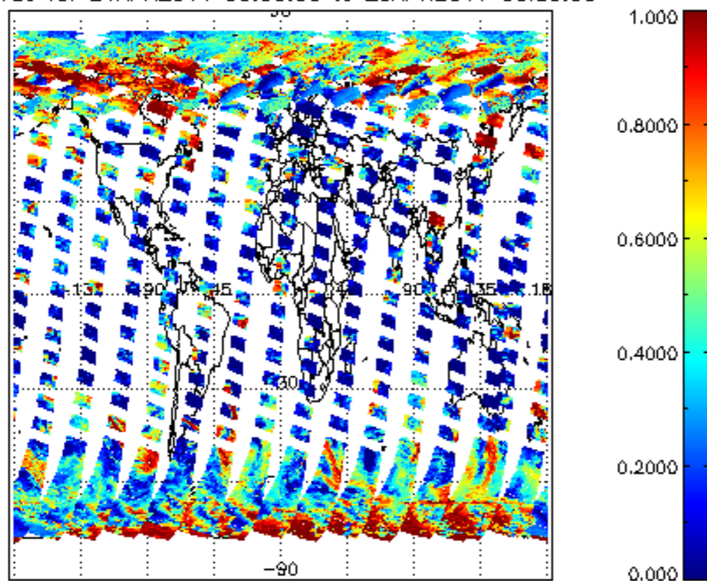
cL_frac for 24APR2011 00:00:00 to 25APR2011 00:00:00
