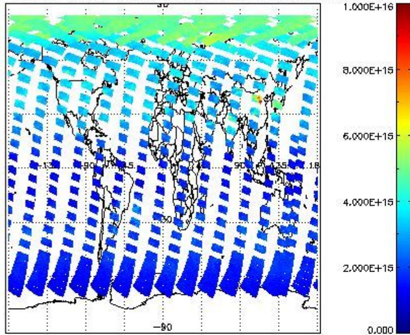
SCIOL2P_NADUV1NO2_vcd for 24APR2011 00:00:00 to 25APR2011 00:00:00
