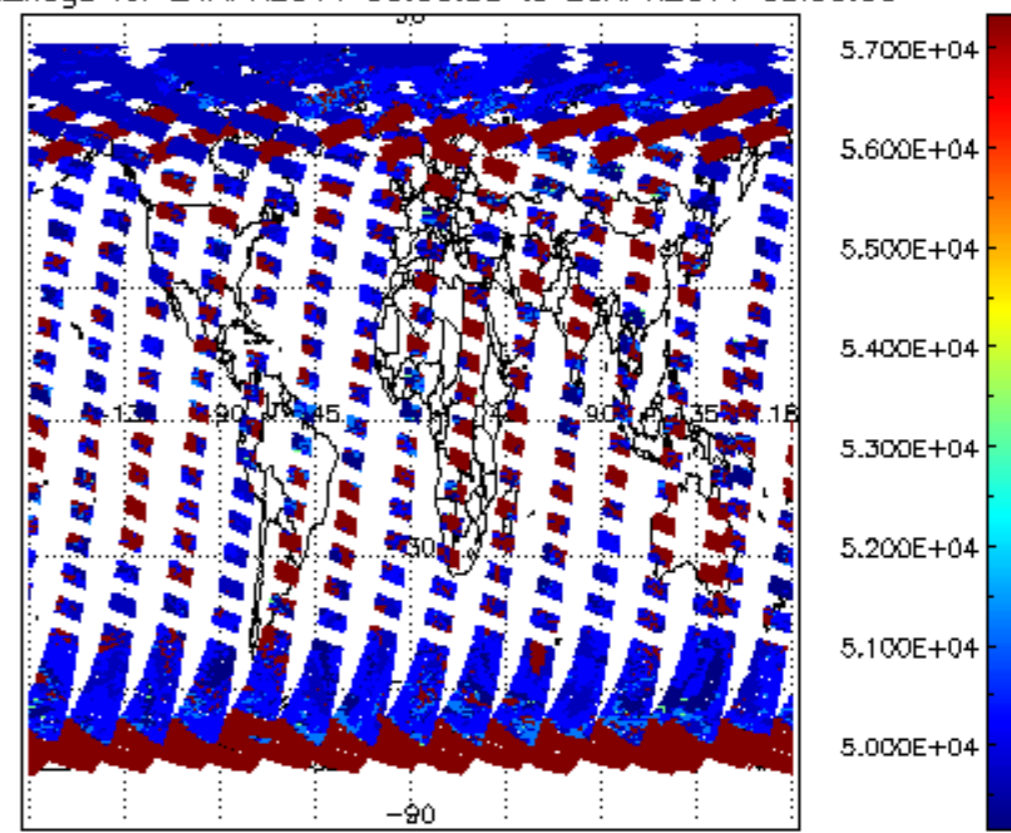
cloud_flags for 24APR2011 00:00:00 to 25APR2011 00:00:00
