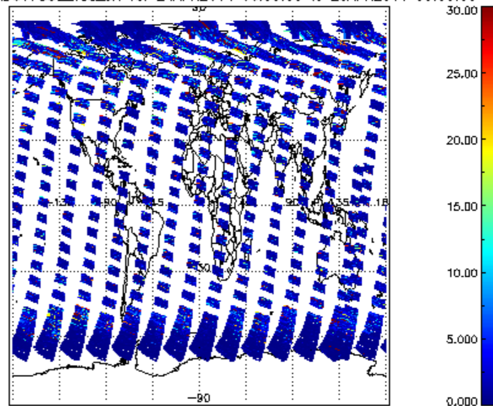
SCIOL2P_NADUV7S02_vcd_err for 24APR2011 00:00:00 to 25APR2011 00:00:00
