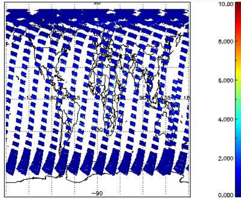
SCIOL2P_NADUV3BRO_vcd_err for 24APR2011 00:00:00 to 25APR2011 00:00:00
