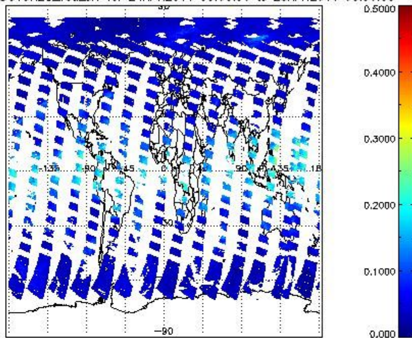
SCIOL2P_NADUV8H2O_vcd_err for 24APR2011 00:00:00 to 25APR2011 00:00:00
