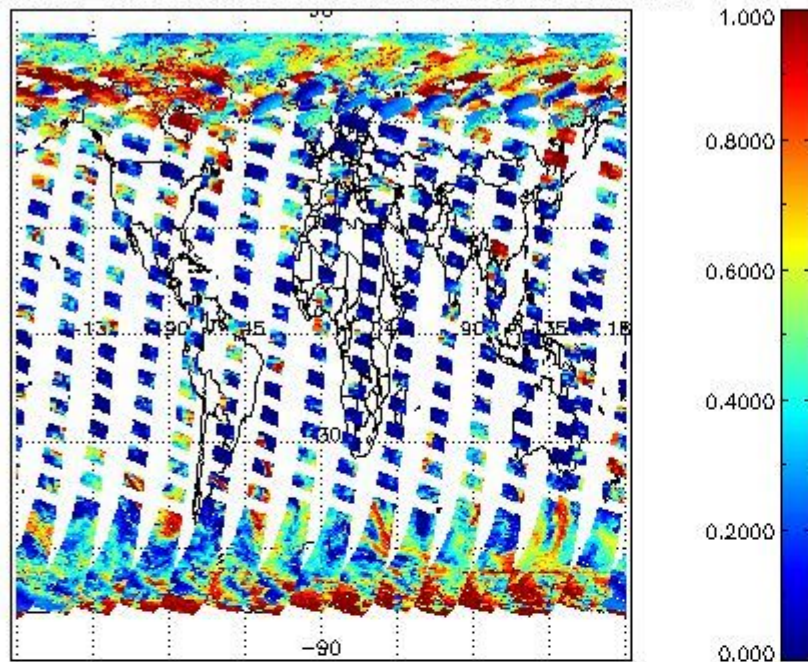
cL_frac for 24APR2011 00:00:00 to 25APR2011 00:00:00
