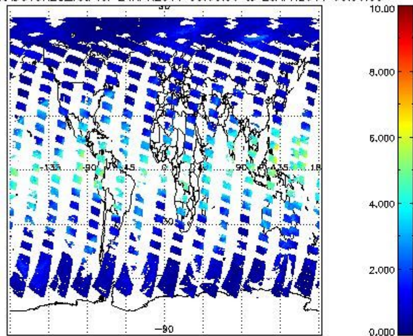
SCIOL2P_NADUV8H2O_vcd for 24APR2011 00:00:00 to 25APR2011 00:00:00
