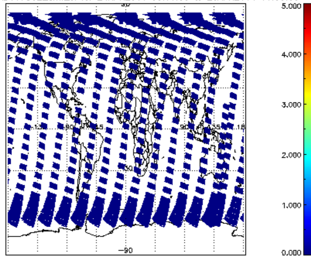
SCIOL2P_NADUV7S02_amf_cl for 24APR2011 00:00:00 to 25APR2011 00:00:00
