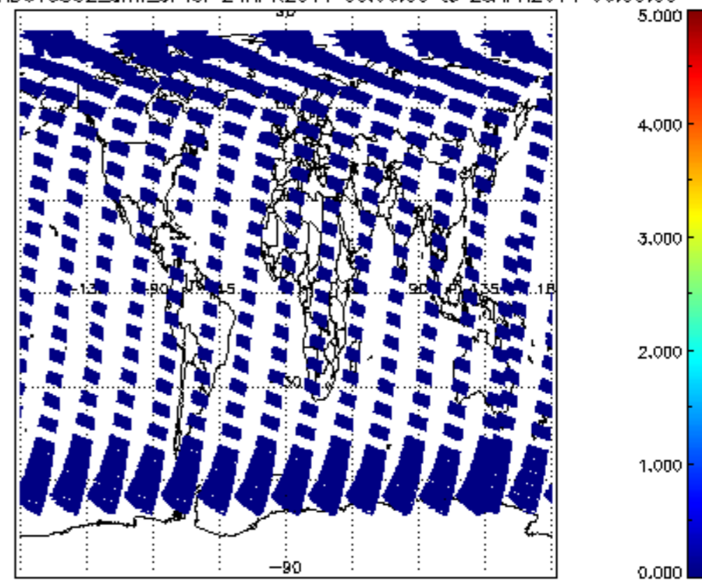
SCIOL2P_NADUV5S02_amf_cl for 24APR2011 00:00:00 to 25APR2011 00:00:00
