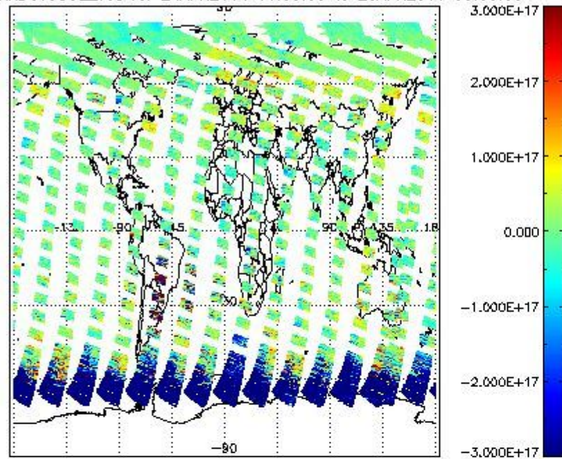
SCIOL2P_NADUV5S02_vcd for 24APR2011 00:00:00 to 25APR2011 00:00:00
