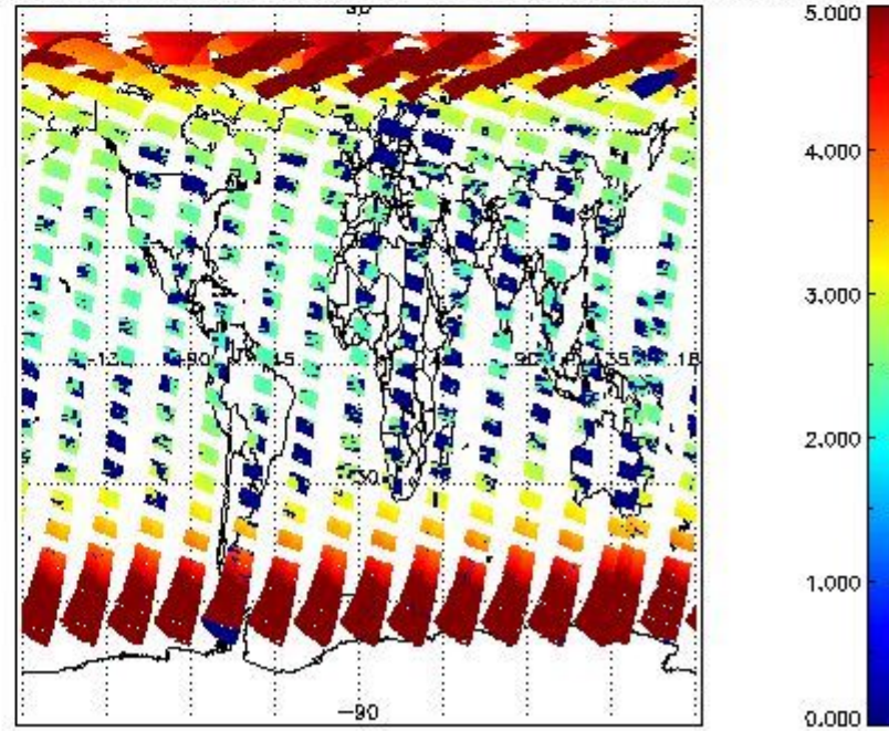
SCIOL2P_NADUV003_amf_cl for 24APR2011 00:00:00 to 25APR2011 00:00:00
