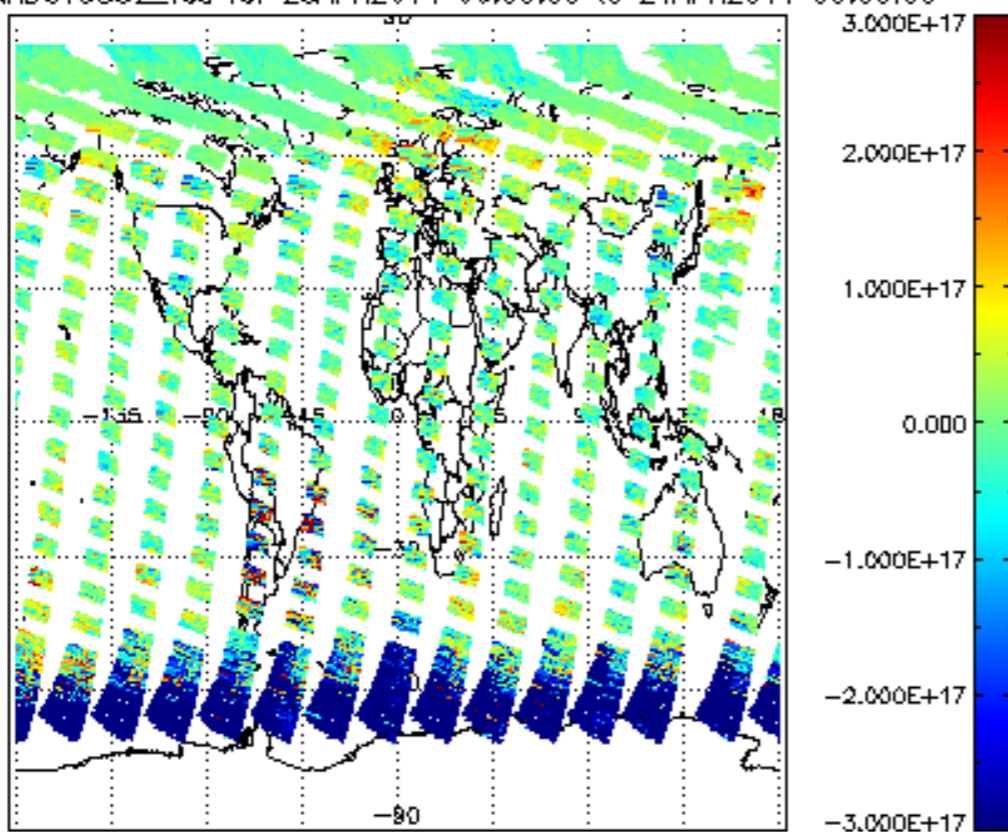
SCIOL2P_NADUV5S02_vcd for 23APR2011 00:00:00 to 24APR2011 00:00:00
