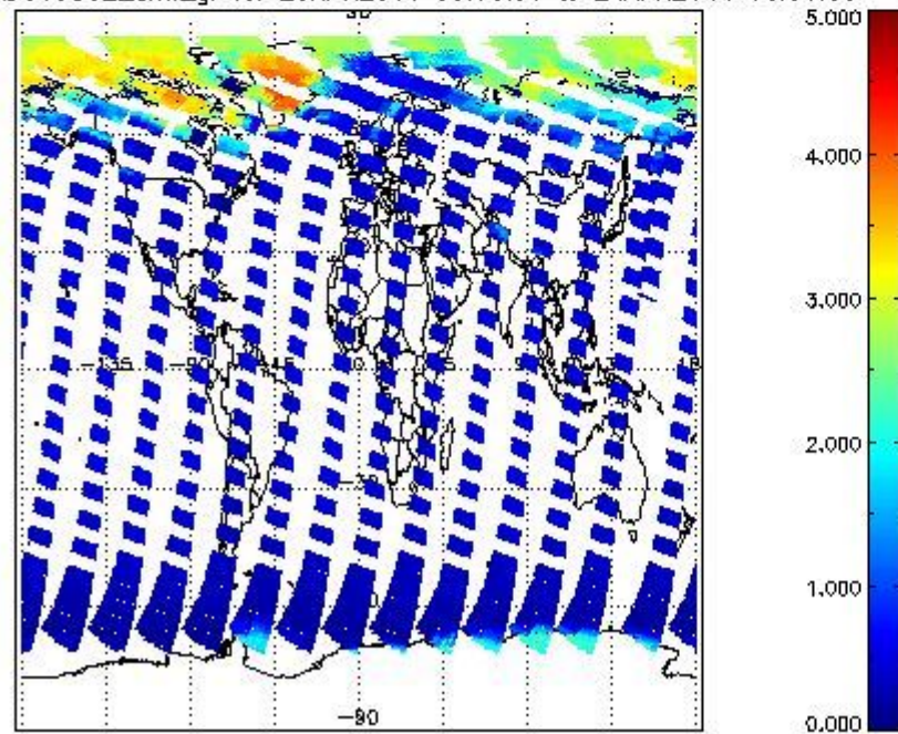
SCIOL2P_NADUV5S02_amf_gr for 23APR2011 00:00:00 to 24APR2011 00:00:00
