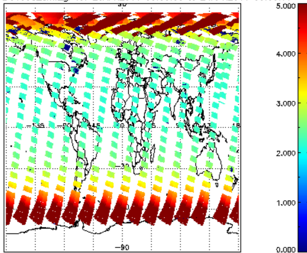
SCIOL2P_NADUV003_amf_gr for 23APR2011 00:00:00 to 24APR2011 00:00:00
