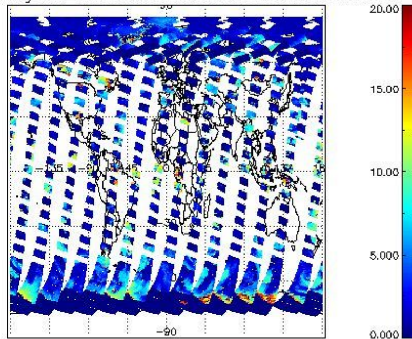
cL_top_height for 23APR2011 00:00:00 to 24APR2011 00:00:00
