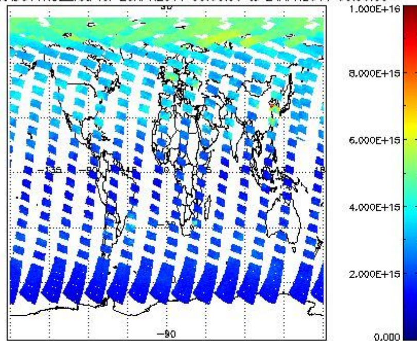
SCIOL2P_NADUV1NO2_vcd for 23APR2011 00:00:00 to 24APR2011 00:00:00
