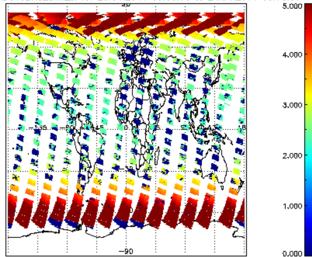
SCIOL2P_NADUV3BRO_amf_sl for 23APR2011 00:00:00 to 24APR2011 00:00:00
