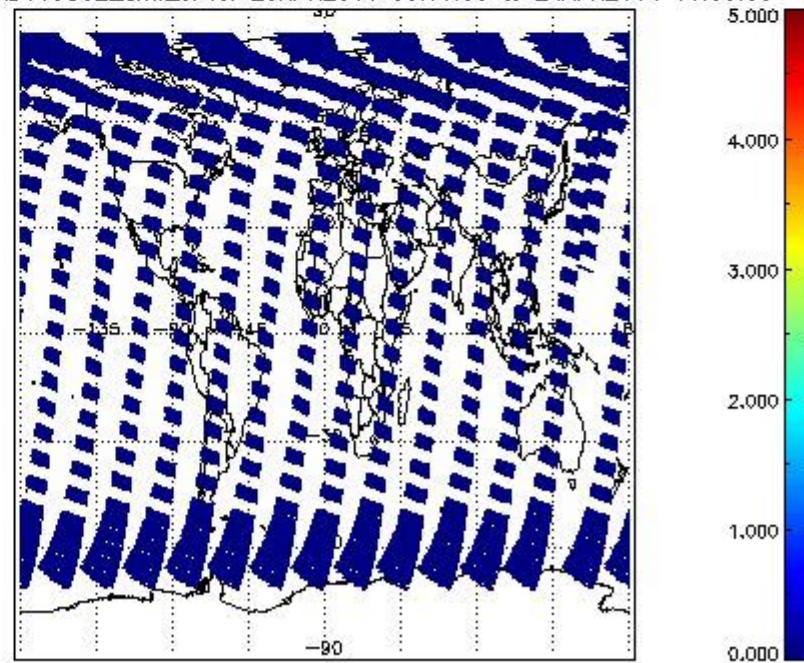
SCIOL2P_NADUV5S02_amf_cl for 23APR2011 00:00:00 to 24APR2011 00:00:00
