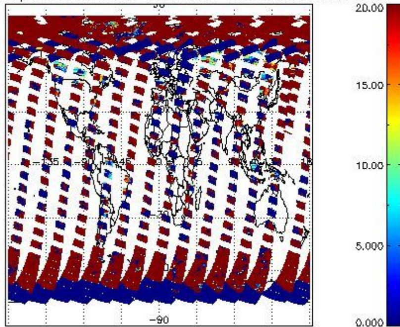
cL_opt_depth for 23APR2011 00:00:00 to 24APR2011 00:00:00
