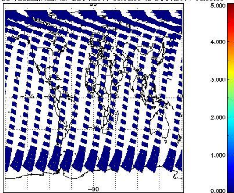
SCIOL2P_NADUV7S02_amf_cl for 23APR2011 00:00:00 to 24APR2011 00:00:00
