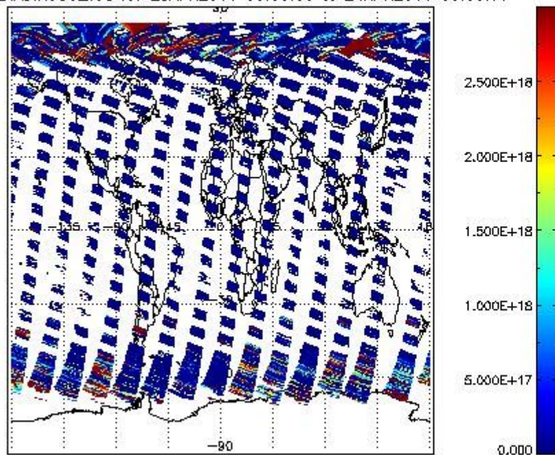
SCIO2P_NADIR3CO_vcd for 23APR2011 00:00:00 to 24APR2011 00:00:00
