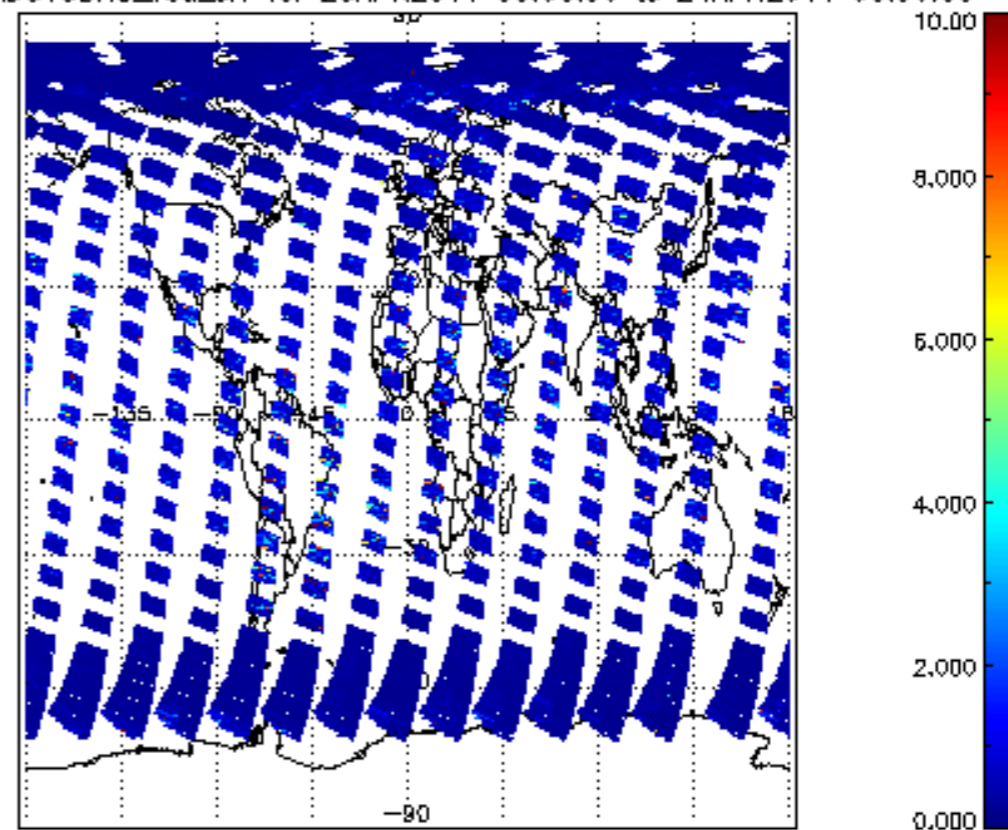
SCIOL2P_NADUV3BRO_vcd_err for 23APR2011 00:00:00 to 24APR2011 00:00:00
