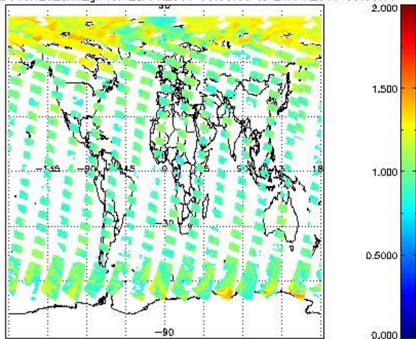
SCIOL2P_NADUV6H2O_arnf_gr for 23APR2011 00:00:00 to 24APR2011 00:00:00
