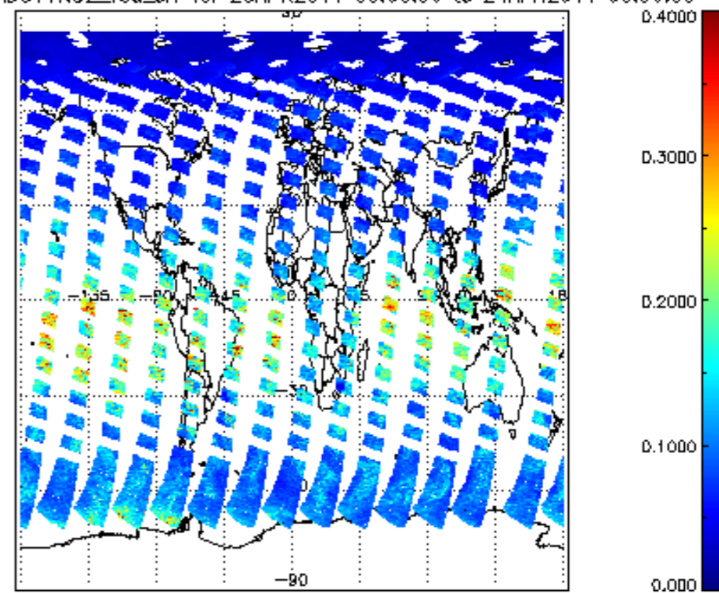
SCIOL2P_NADUV1NO2_vcd_err for 23APR2011 00:00:00 to 24APR2011 00:00:00
