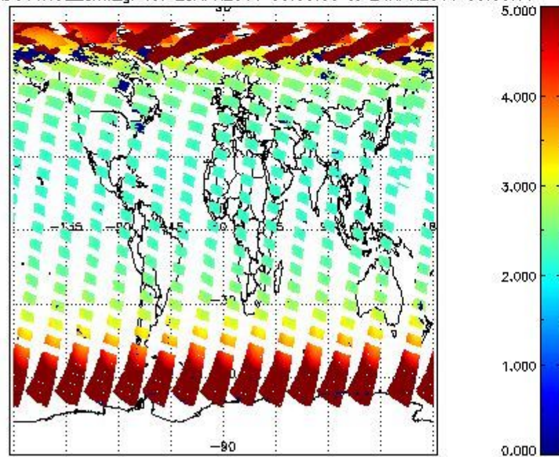
SCIOL2P_NADUV1NO2_amf_gr for 23APR2011 00:00:00 to 24APR2011 00:00:00
