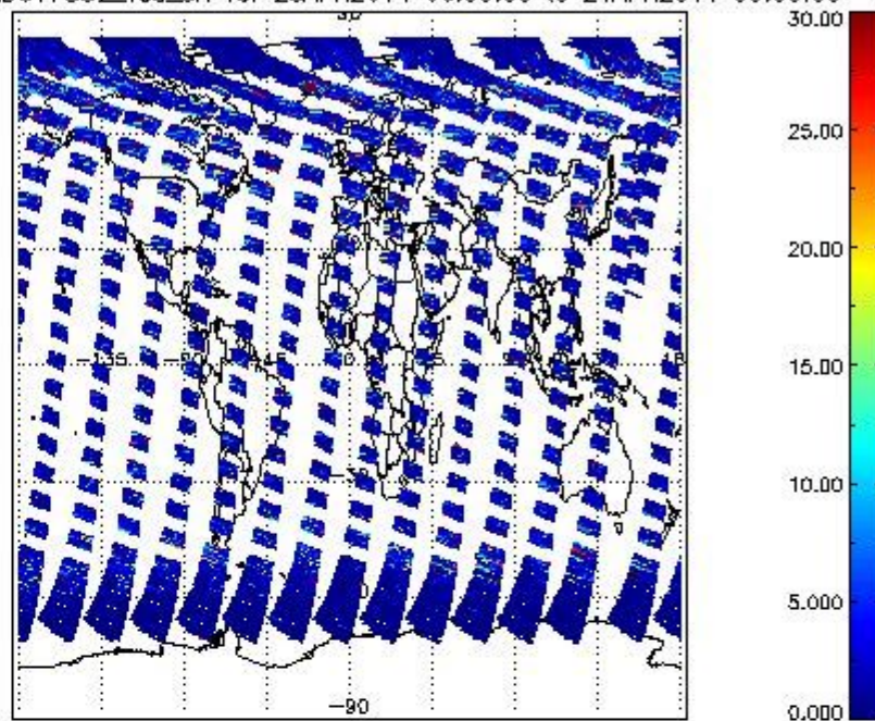
SCIOL2P_NADUV7S02_vcd_err for 23APR2011 00:00:00 to 24APR2011 00:00:00
