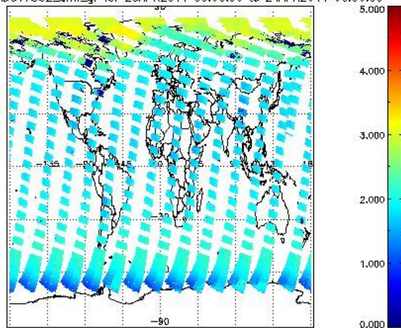
SCIOL2P_NADUV7S02_amf_gr for 23APR2011 00:00:00 to 24APR2011 00:00:00
