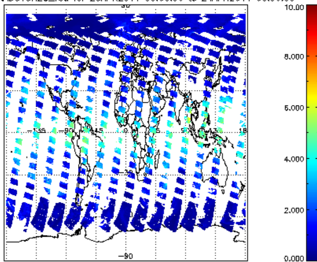
SCIOL2P_NADUV8H2O_vcd for 23APR2011 00:00:00 to 24APR2011 00:00:00
