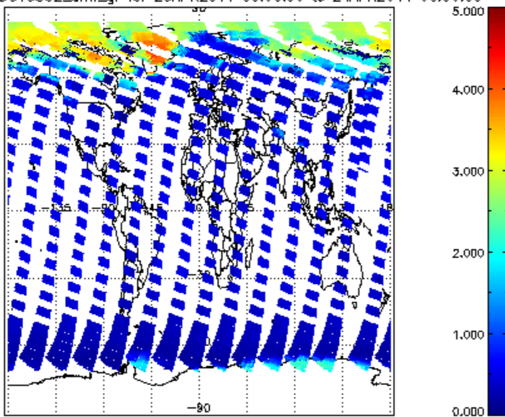
SCIOL2P_NADUV5S02_amf_gr for 23APR2011 00:00:00 to 24APR2011 00:00:00
