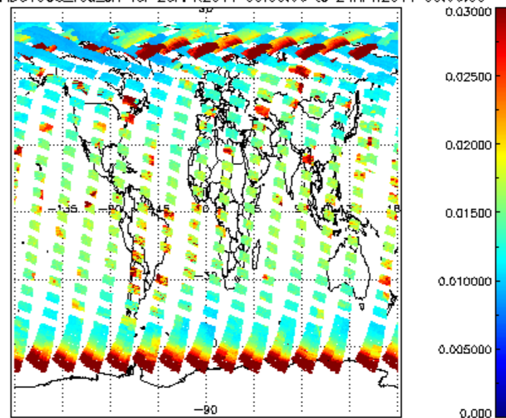
SCIOL2P_NADUV003_vcd_err for 23APR2011 00:00:00 to 24APR2011 00:00:00
