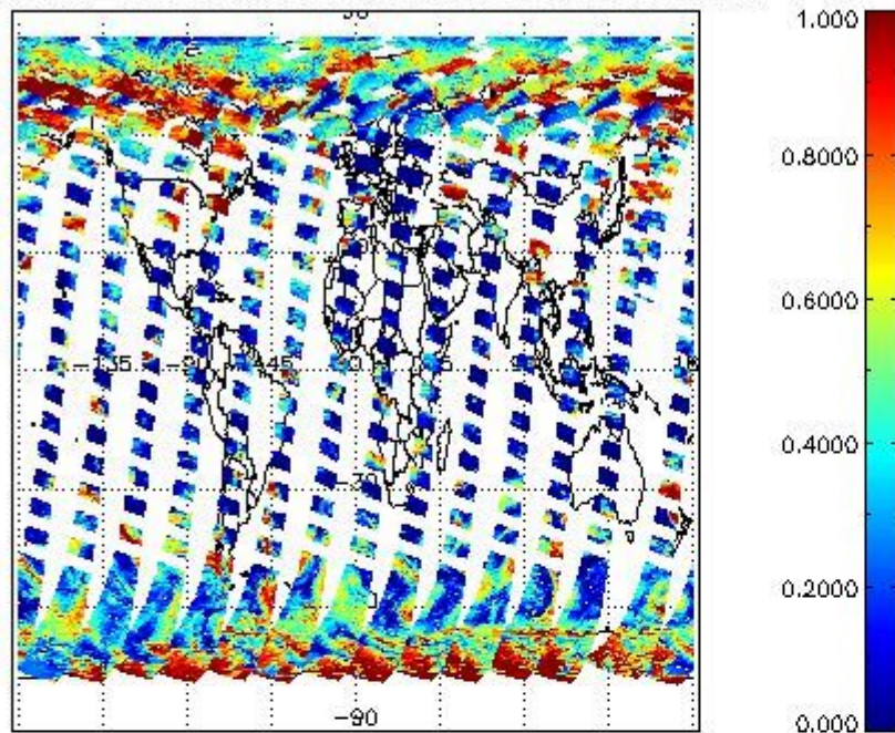
cL_frac for 23APR2011 00:00:00 to 24APR2011 00:00:00
