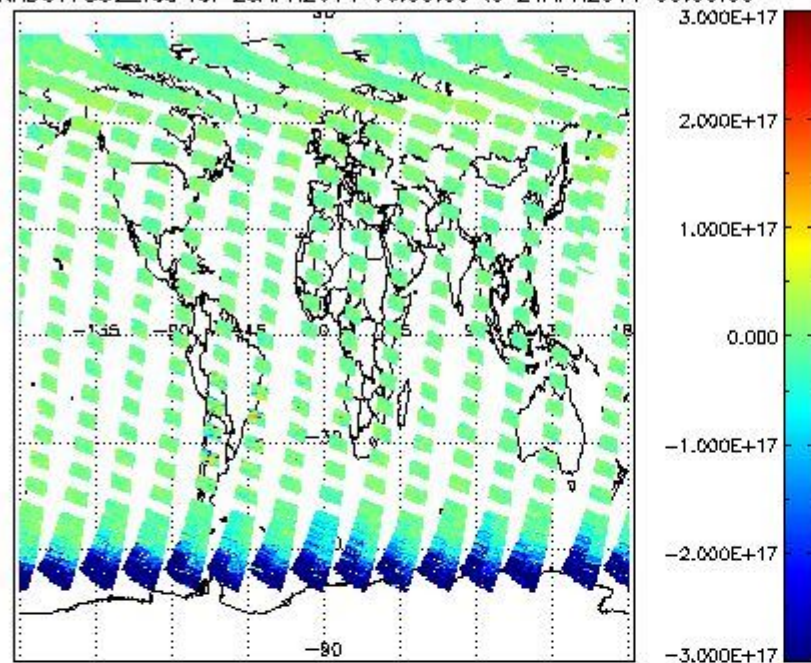
SCIOL2P_NADUV7S02_vcd for 23APR2011 00:00:00 to 24APR2011 00:00:00
