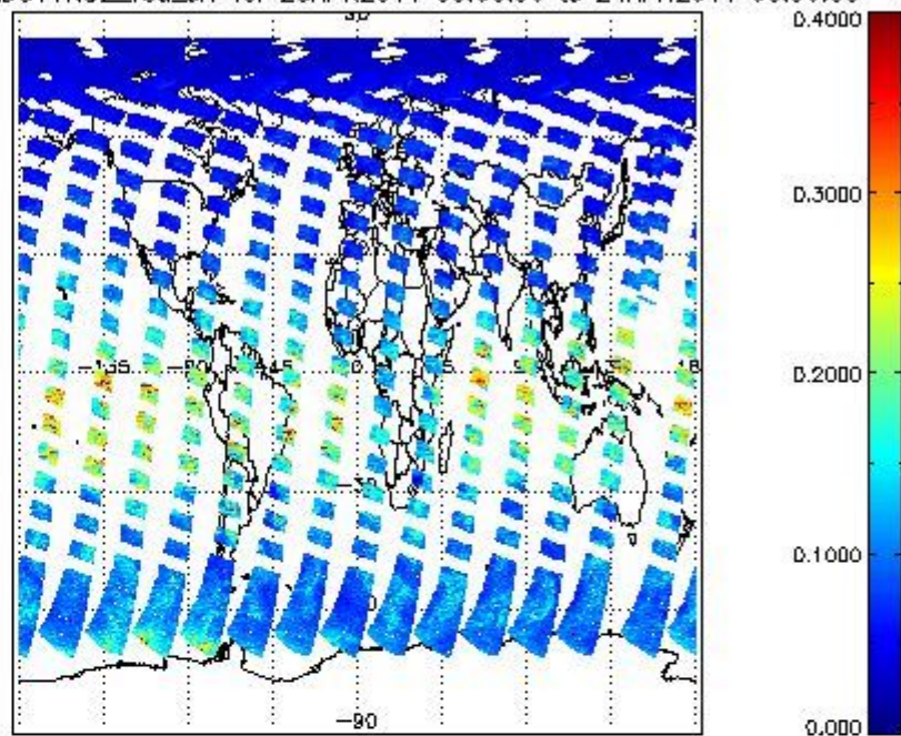
SCIOL2P_NADUV1NO2_vcd_err for 23APR2011 00:00:00 to 24APR2011 00:00:00
