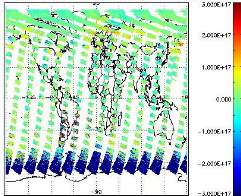
SCIOL2P_NADUV5S02_vcd for 23APR2011 00:00:00 to 24APR2011 00:00:00
