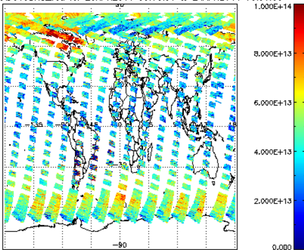
SCIOL2P_NADUV3BRO_vcd for 23APR2011 00:00:00 to 24APR2011 00:00:00
