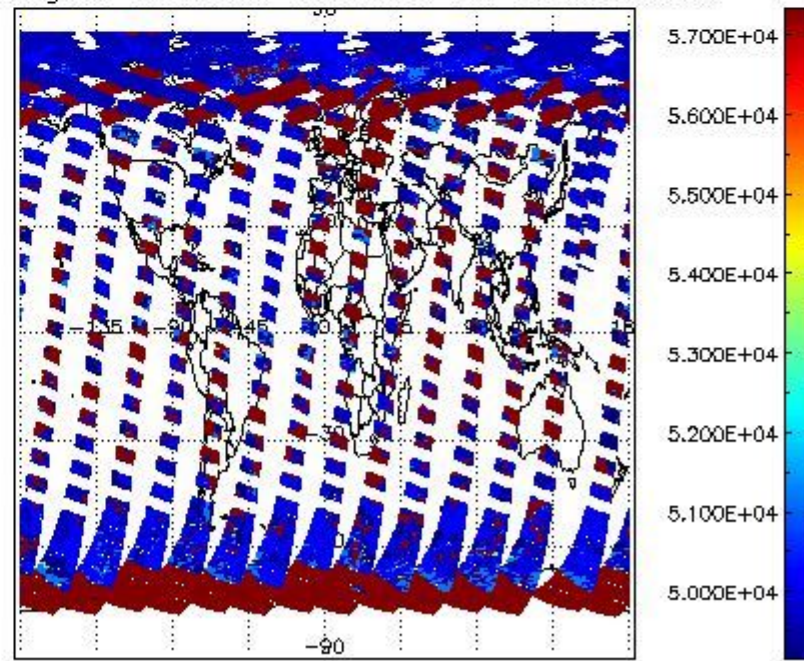
cloud_flags for 23APR2011 00:00:00 to 24APR2011 00:00:00
