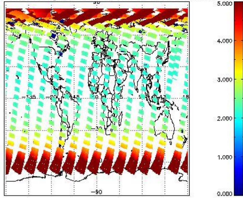
SCIOL2P_NADUV3BRO_amf_gr for 23APR2011 00:00:00 to 24APR2011 00:00:00
