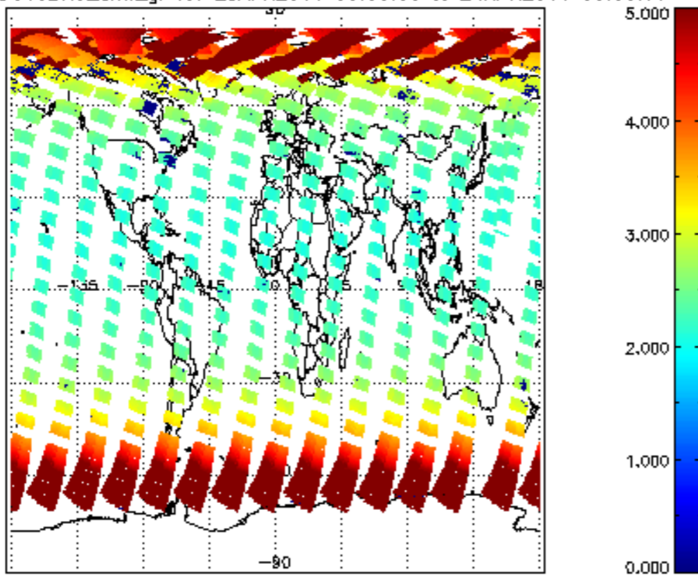
SCIOL2P_NADUV3BRO_amf_gr for 23APR2011 00:00:00 to 24APR2011 00:00:00
