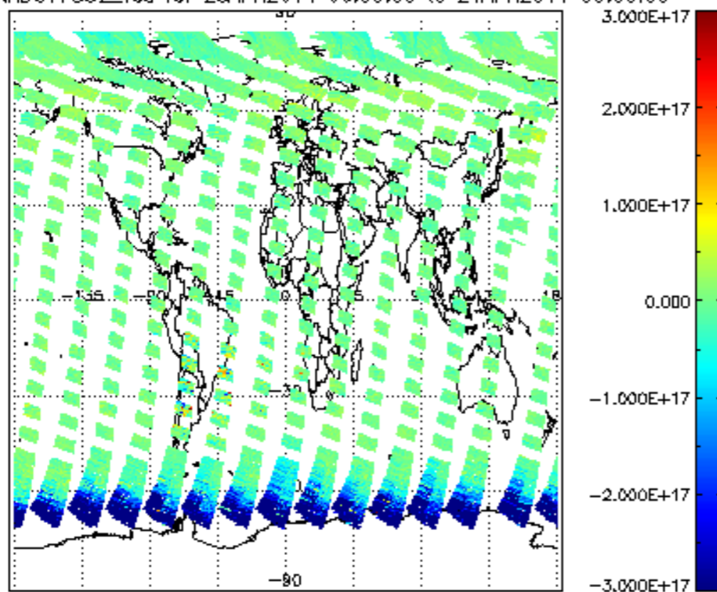
SCIOL2P_NADUV7S02_vcd for 23APR2011 00:00:00 to 24APR2011 00:00:00
