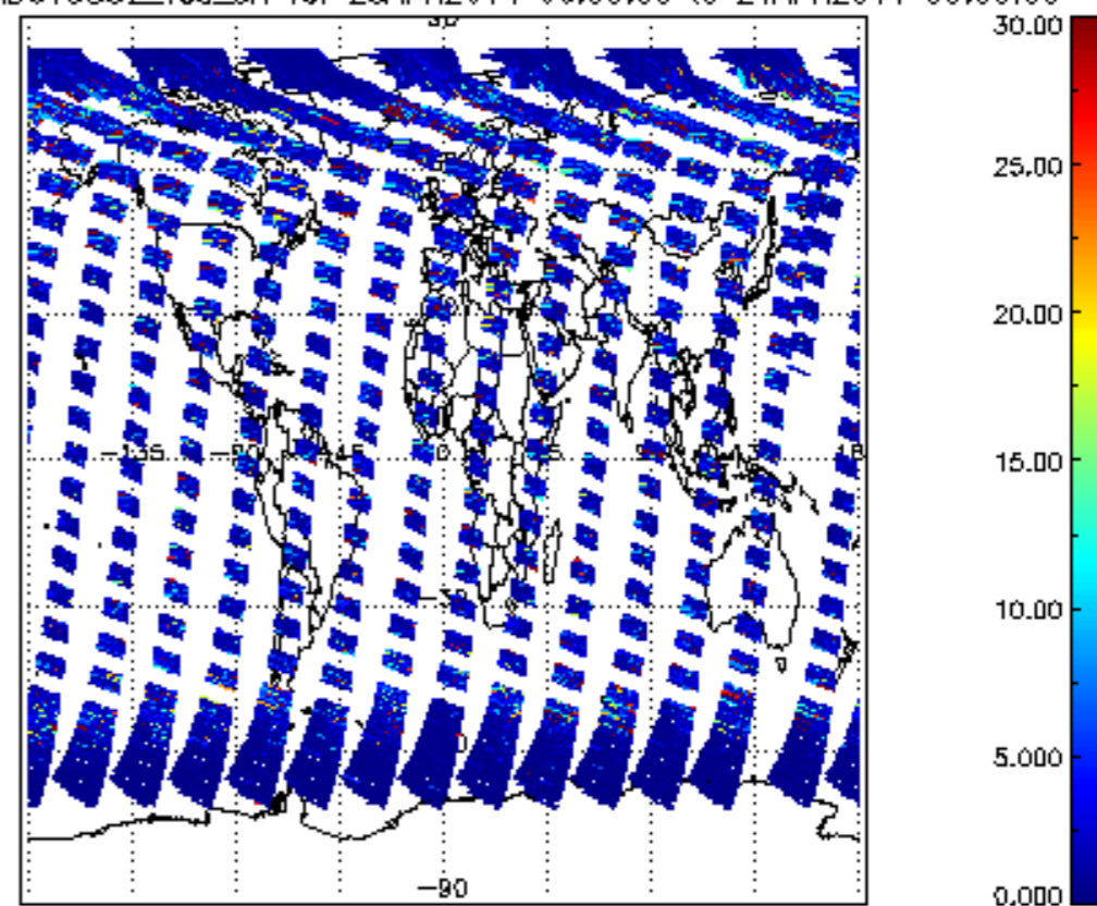
SCIOL2P_NADUV5S02_vcd_err for 23APR2011 00:00:00 to 24APR2011 00:00:00
