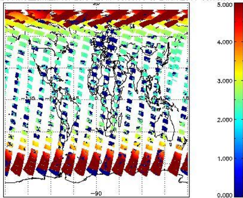
SCIOL2P_NADUV1NO2_amf_cl for 23APR2011 00:00:00 to 24APR2011 00:00:00
