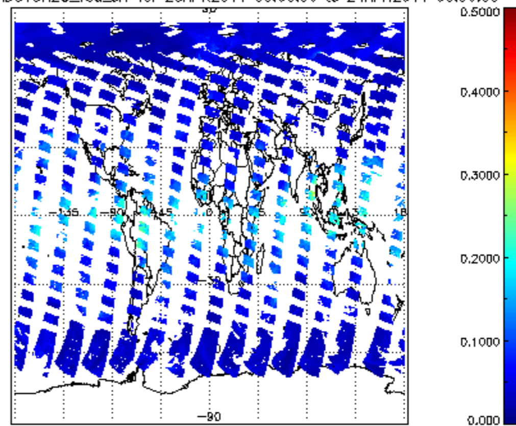
SCIOL2P_NADUV8H2O_vcd_err for 23APR2011 00:00:00 to 24APR2011 00:00:00
