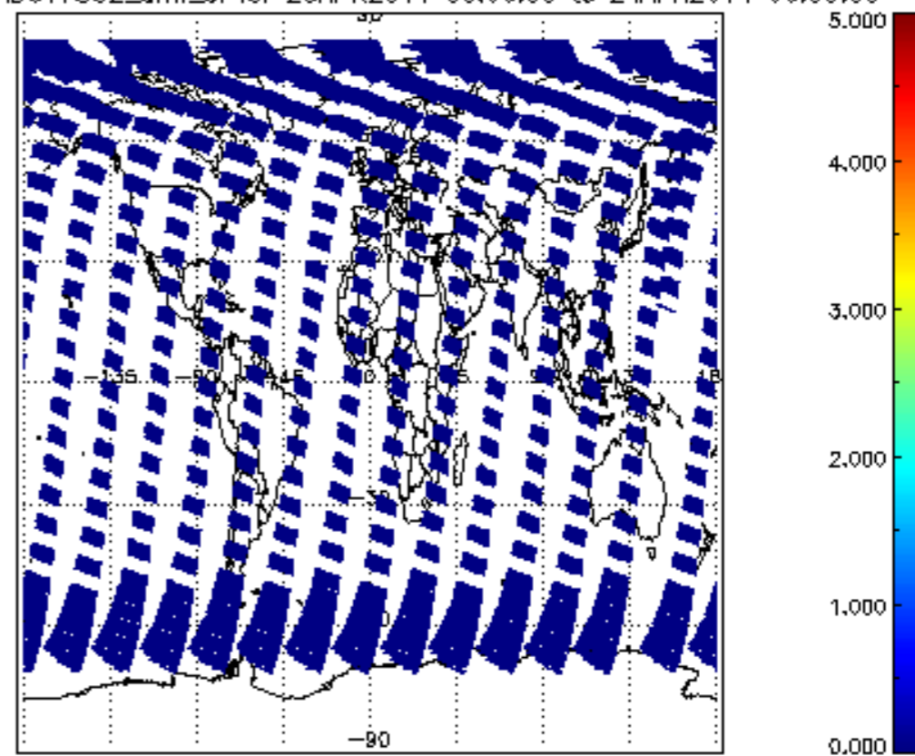
SCIOL2P_NADUV7S02_amf_cl for 23APR2011 00:00:00 to 24APR2011 00:00:00
