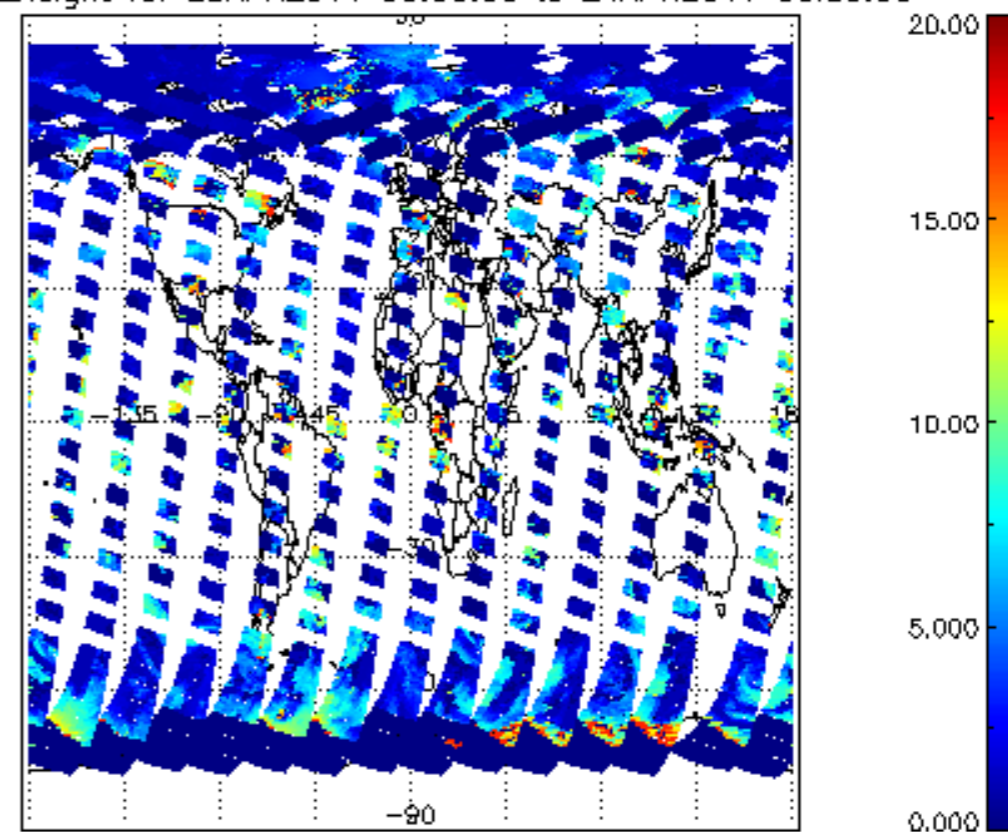
cL_top_height for 23APR2011 00:00:00 to 24APR2011 00:00:00
