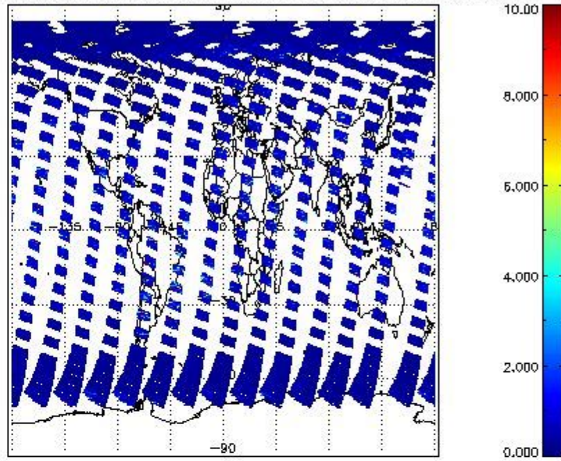
SCIOL2P_NADUV3BRO_vcd_err for 23APR2011 00:00:00 to 24APR2011 00:00:00
