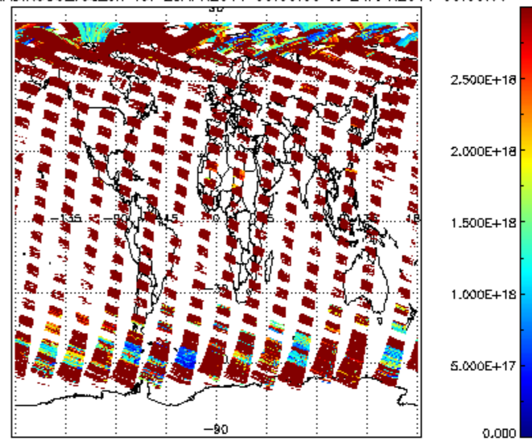
SCIOL2P_NADIR3CO_vcd_err for 23APR2011 00:00:00 to 24APR2011 00:00:00
