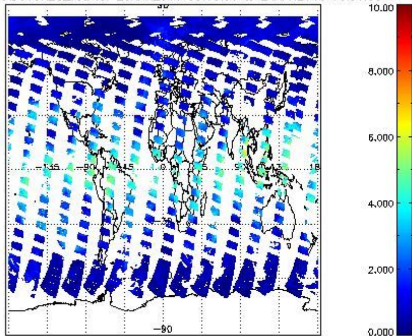
SCIOL2P_NADUV6H2O_vcd for 23APR2011 00:00:00 to 24APR2011 00:00:00
