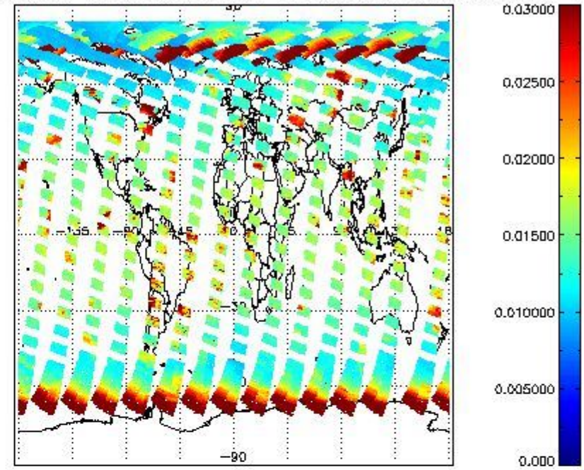
SCIOL2P_NADUV003_vcd_err for 23APR2011 00:00:00 to 24APR2011 00:00:00
