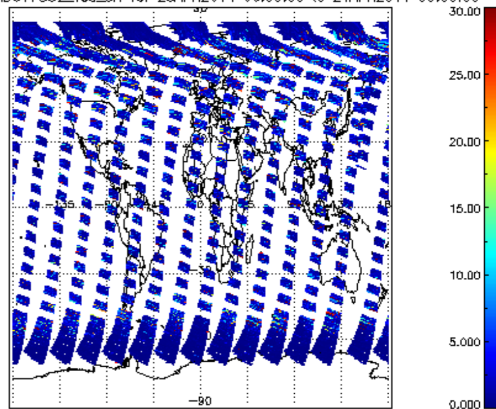
SCIOL2P_NADUV7S02_vcd_err for 23APR2011 00:00:00 to 24APR2011 00:00:00
