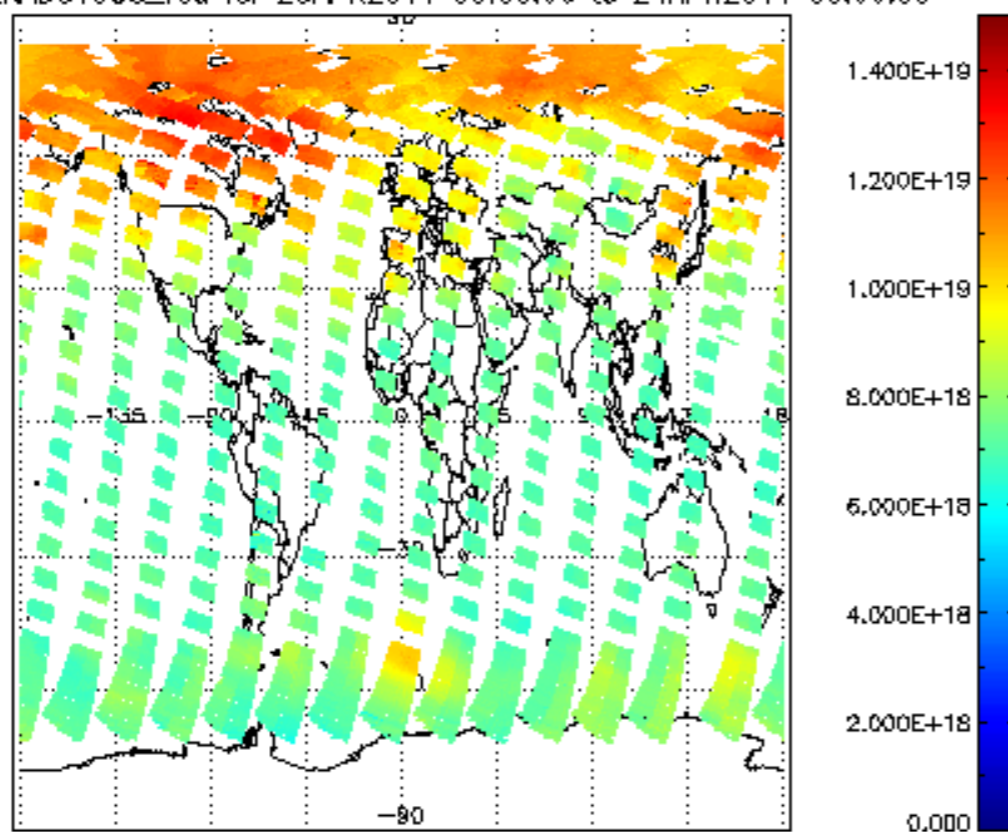
SCIOL2P_NADUV003_vcd for 23APR2011 00:00:00 to 24APR2011 00:00:00
