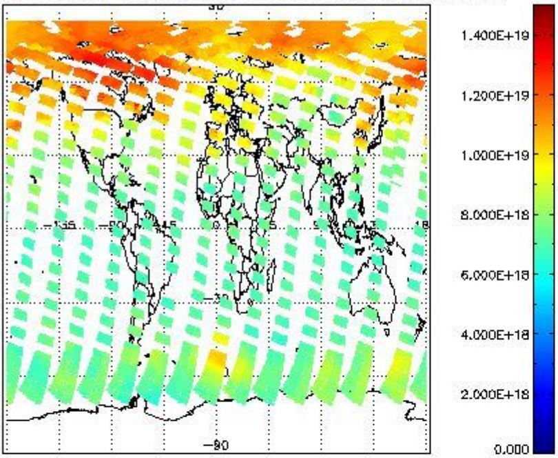
SCIOL2P_NADUV003_vcd for 23APR2011 00:00:00 to 24APR2011 00:00:00
