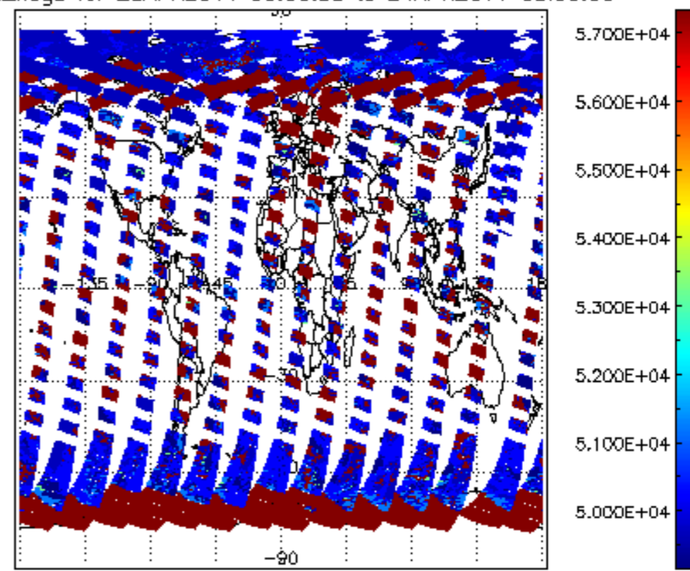
cloud_flags for 23APR2011 00:00:00 to 24APR2011 00:00:00
