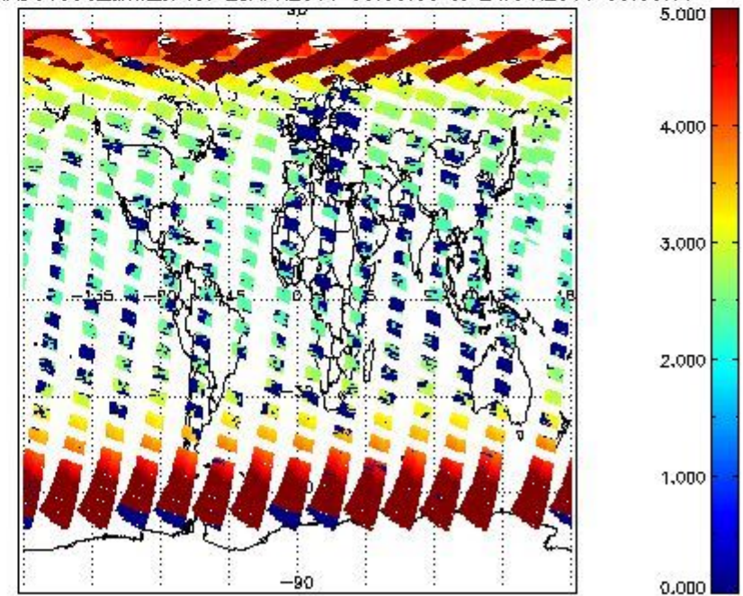
SCIOL2P_NADUV003_amf_cl for 23APR2011 00:00:00 to 24APR2011 00:00:00
