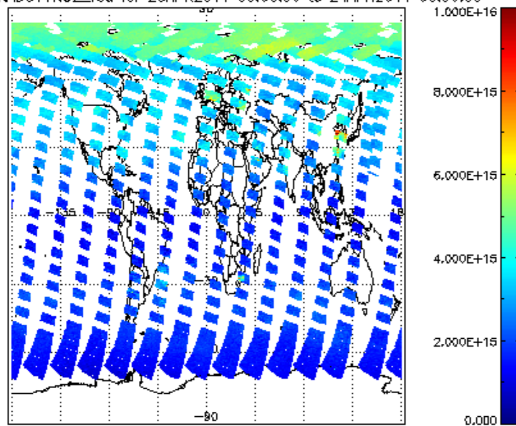
SCIOL2P_NADUV1NO2_vcd for 23APR2011 00:00:00 to 24APR2011 00:00:00
