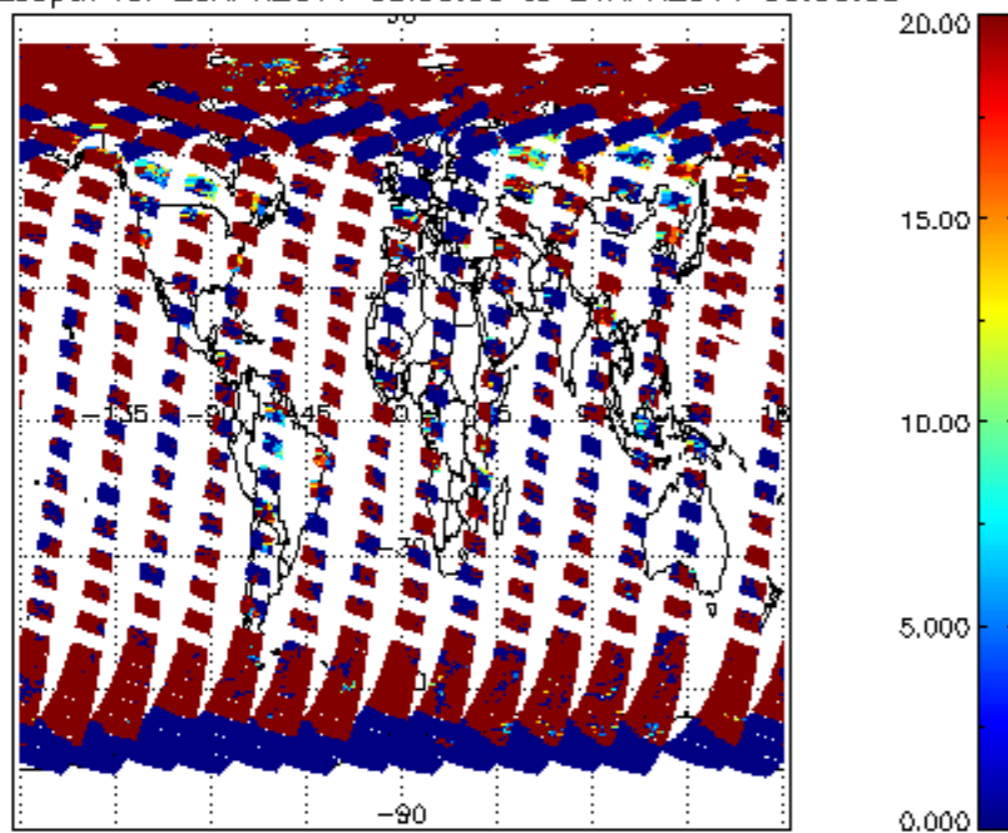
cL_opt_depth for 23APR2011 00:00:00 to 24APR2011 00:00:00
