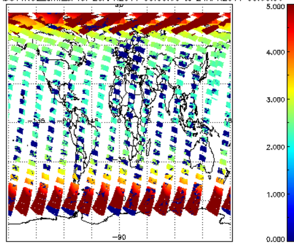
SCIOL2P_NADUV1NO2_amf_sl for 23APR2011 00:00:00 to 24APR2011 00:00:00
