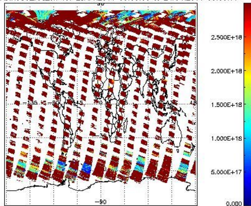
SCIO2P_NADIR3CO_vcd_err for 23APR2011 00:00:00 to 24APR2011 00:00:00
