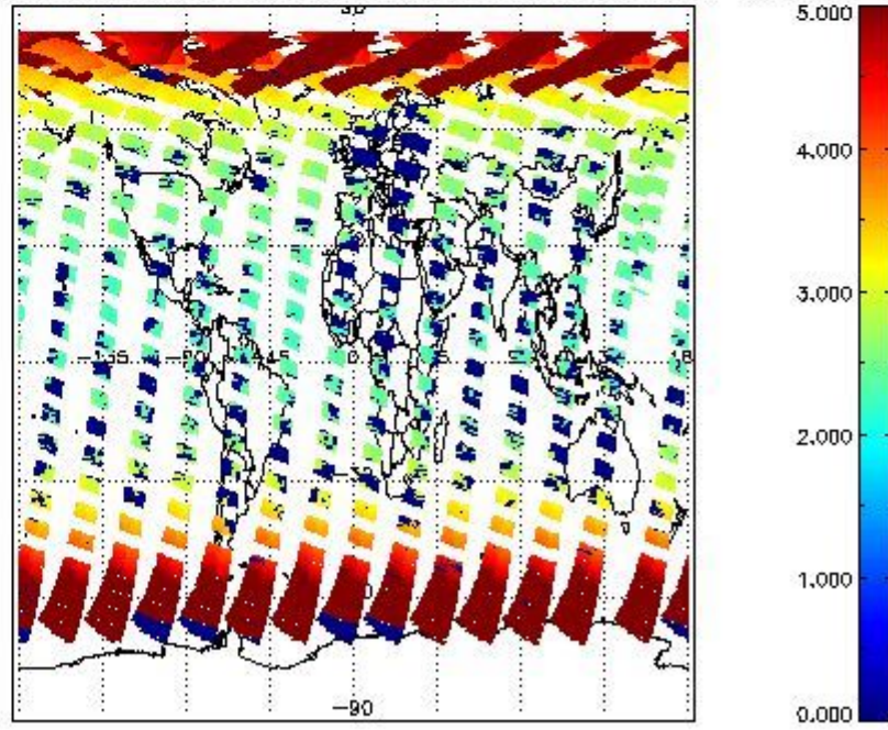
SCIOL2P_NADUV3BRO_amf_cl for 23APR2011 00:00:00 to 24APR2011 00:00:00
