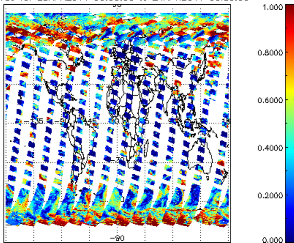
cL_frac for 23APR2011 00:00:00 to 24APR2011 00:00:00
