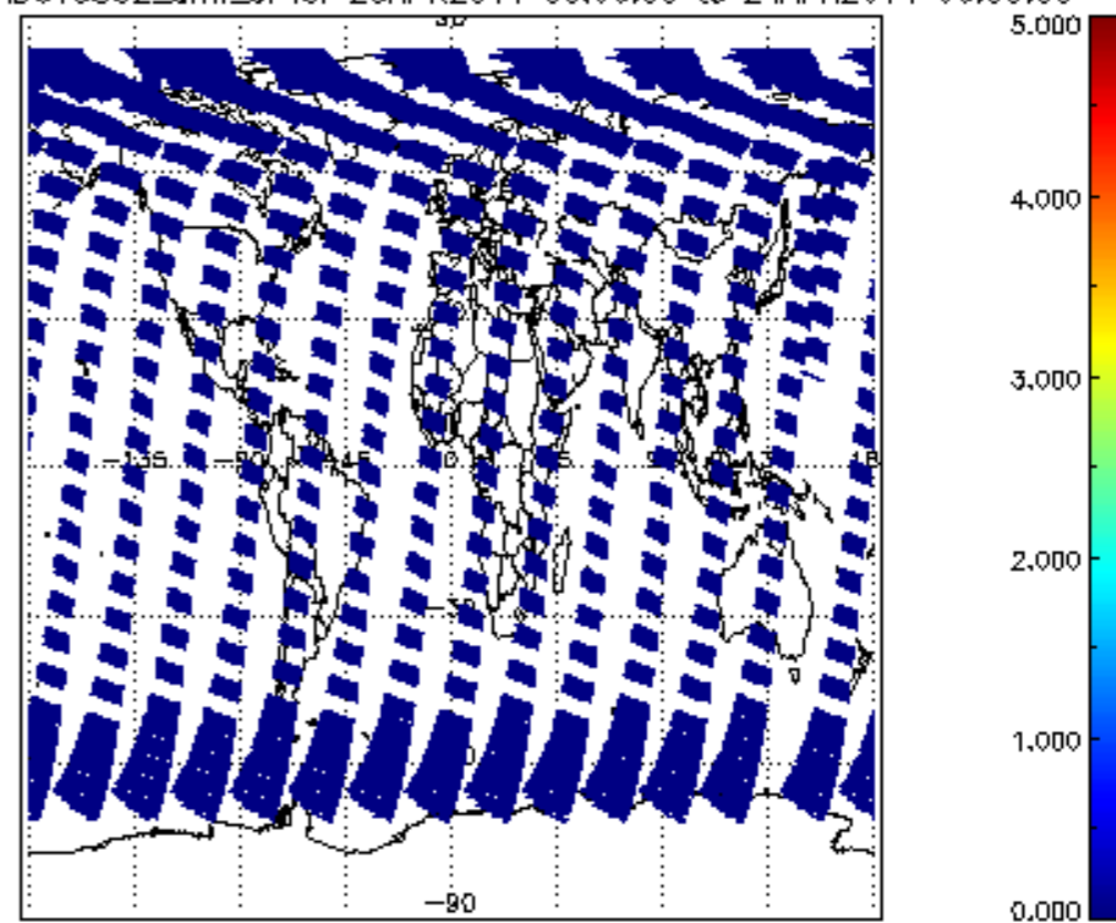
SCIOL2P_NADUV5S02_amf_cl for 23APR2011 00:00:00 to 24APR2011 00:00:00
