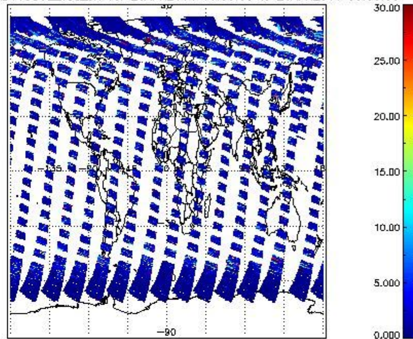
SCIOL2P_NADUV5S02_vcd_err for 23APR2011 00:00:00 to 24APR2011 00:00:00
