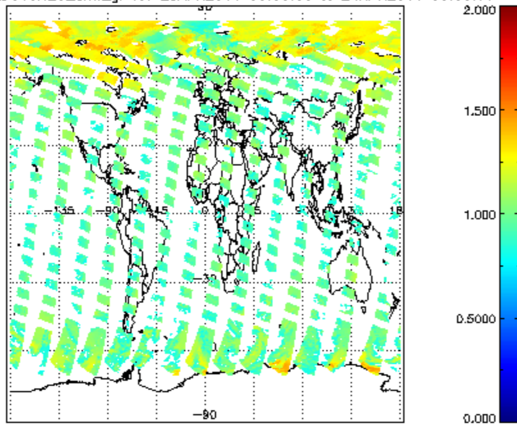
SCIOL2P_NADUV8H2O_amf_gr for 23APR2011 00:00:00 to 24APR2011 00:00:00
