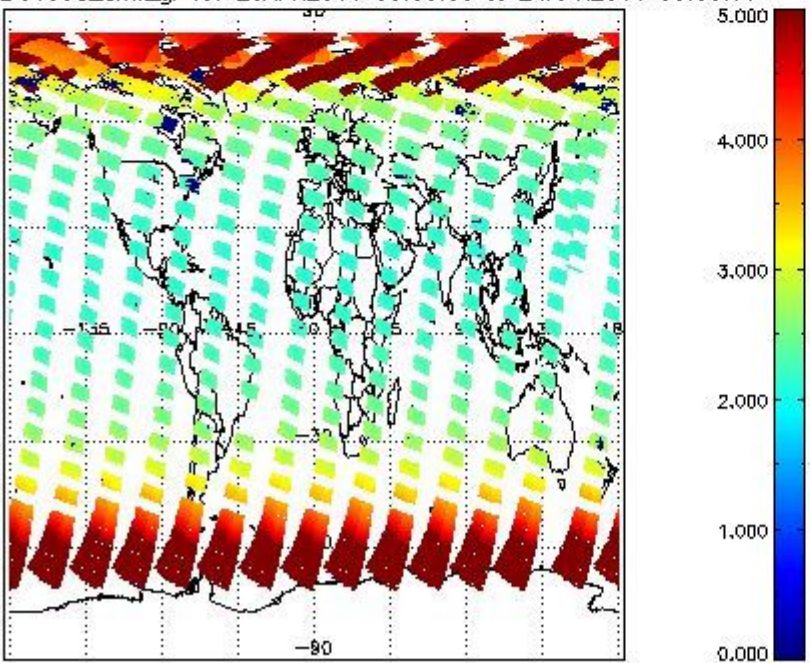
SCIOL2P_NADUV003_amf_gr for 23APR2011 00:00:00 to 24APR2011 00:00:00
