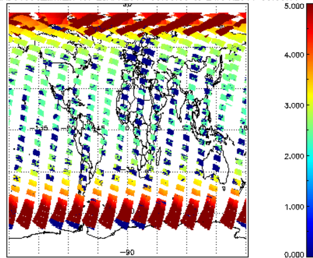
SCIOL2P_NADUV003_amf_cl for 23APR2011 00:00:00 to 24APR2011 00:00:00
