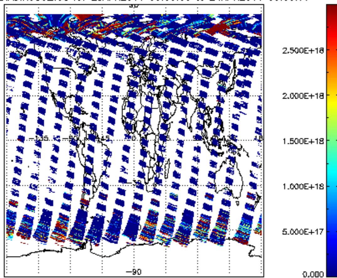
SCIOL2P_NADIR3CO_vcd for 23APR2011 00:00:00 to 24APR2011 00:00:00
