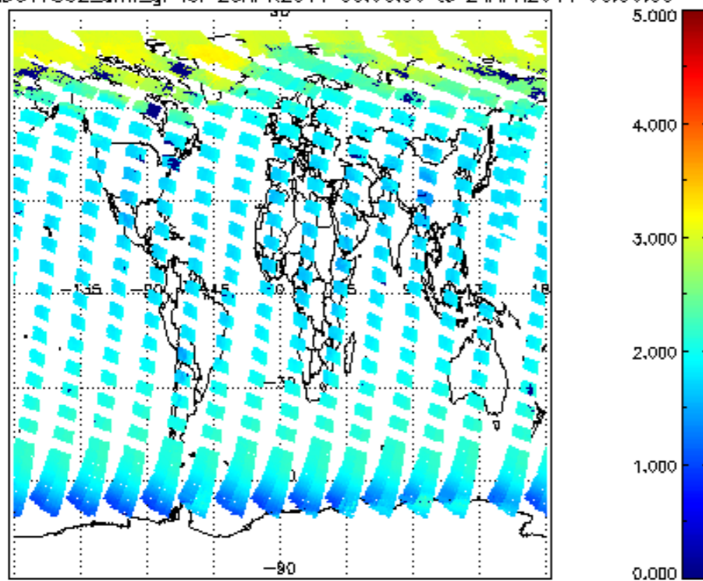
SCIOL2P_NADUV7S02_amf_gr for 23APR2011 00:00:00 to 24APR2011 00:00:00
