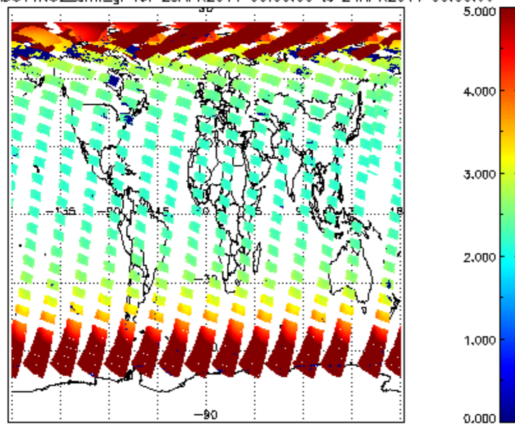
SCIOL2P_NADUV1NO2_amf_gr for 23APR2011 00:00:00 to 24APR2011 00:00:00
