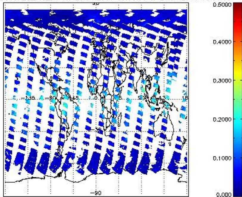
SCIOL2P_NADUV6H2O_vcd_err for 23APR2011 00:00:00 to 24APR2011 00:00:00
