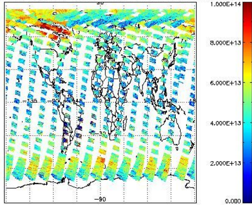
SCIOL2P_NADUV3BRO_vcd for 23APR2011 00:00:00 to 24APR2011 00:00:00
