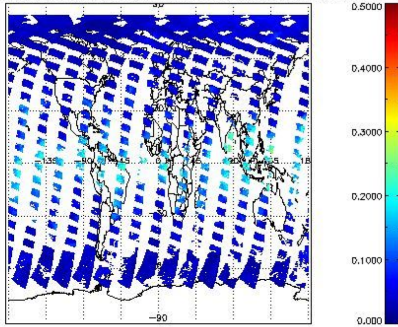
SCIOL2P_NADUV8H2O_vcd_err for 22APR2011 00:00:00 to 23APR2011 00:00:00
