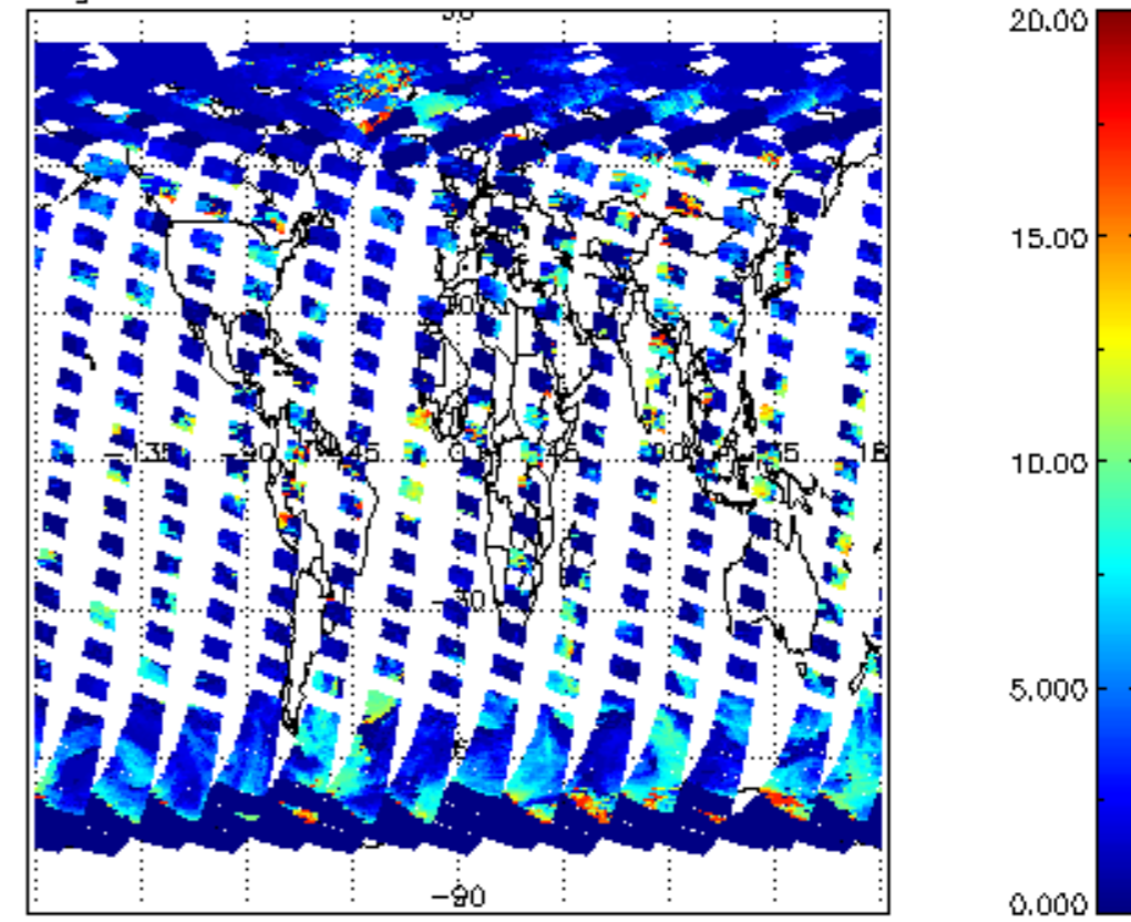
cl_top_height for 22APR2011 00:00:00 to 23APR2011 00:00:00
