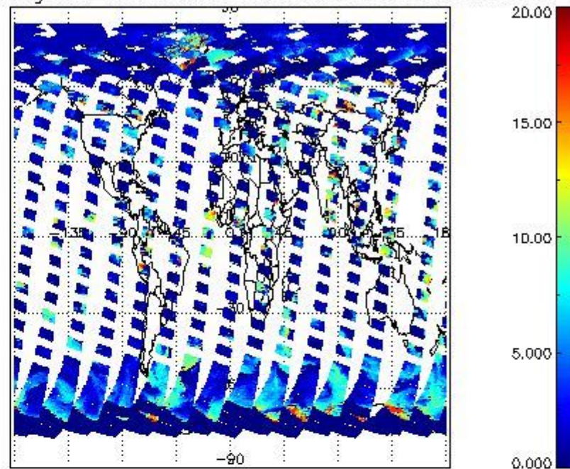
cL_top_height for 22APR2011 00:00:00 to 23APR2011 00:00:00
