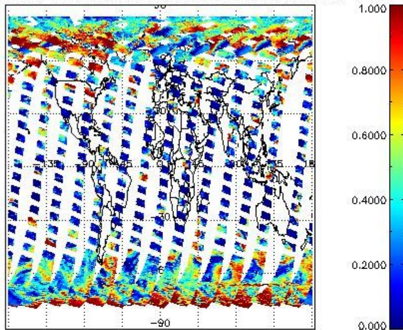
cL_frac for 22APR2011 00:00:00 to 23APR2011 00:00:00
