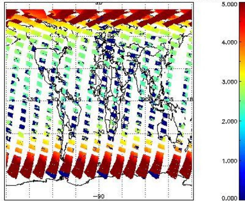
SCIOL2P_NADUV003_amf_cl for 22APR2011 00:00:00 to 23APR2011 00:00:00
