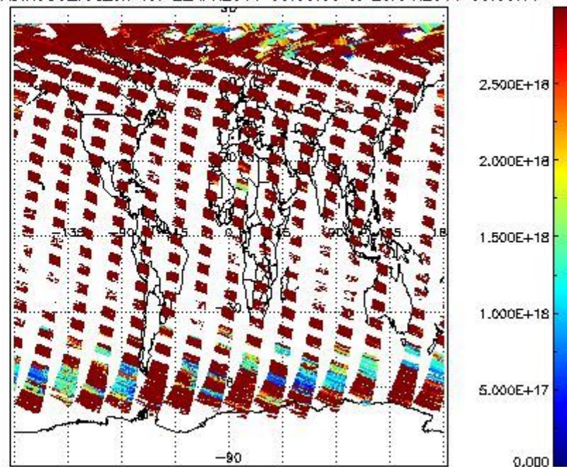
SCIDL2P_NADIR3CO_vcd_err for 22APR2011 00:00:00 to 23APR2011 00:00:00
