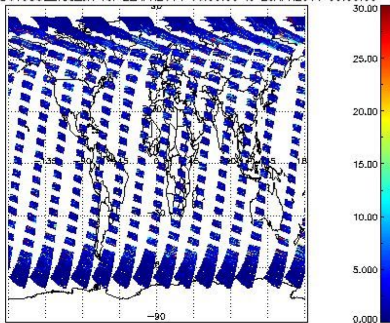
SCIOL2P_NADUV5S02_vcd_err for 22APR2011 00:00:00 to 23APR2011 00:00:00
