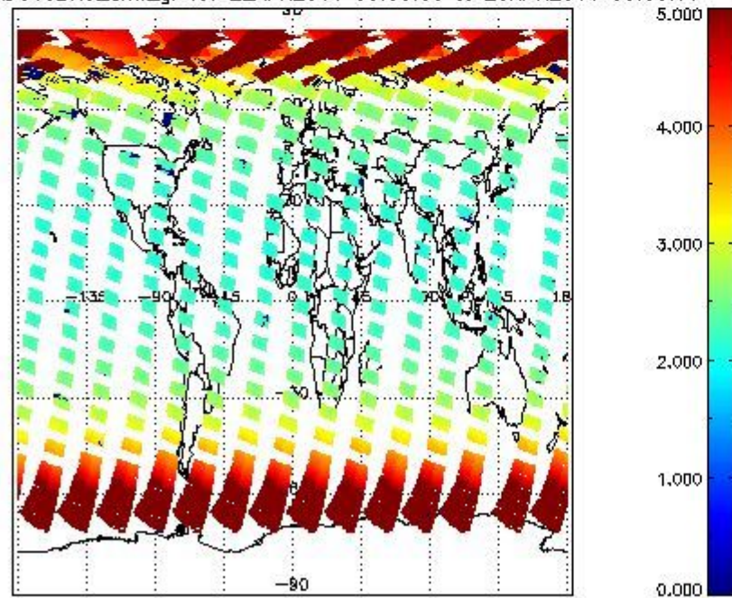
SCIOL2P_NADUV3BRO_amf_gr for 22APR2011 00:00:00 to 23APR2011 00:00:00
