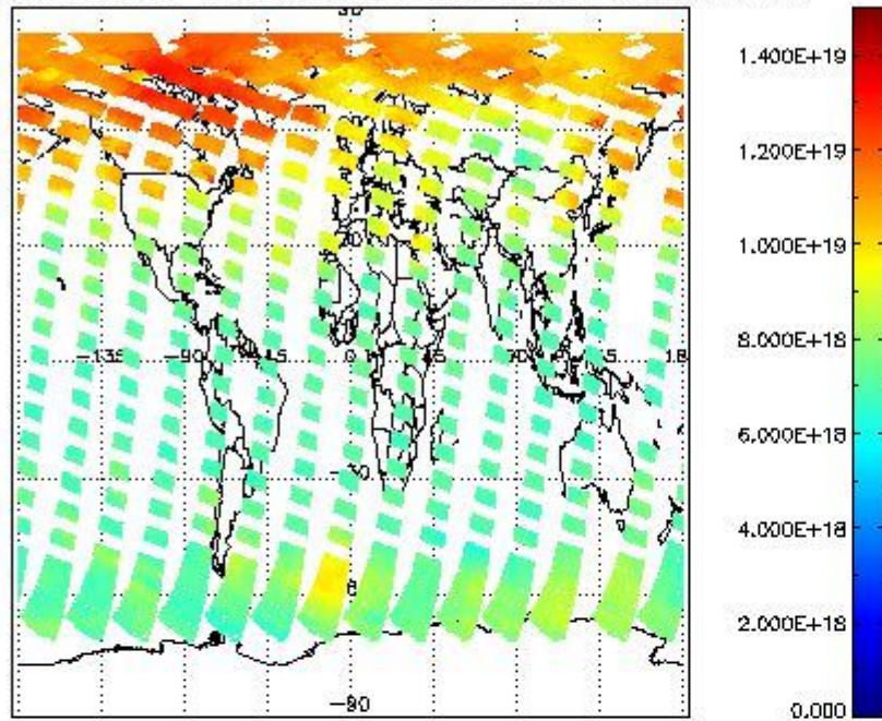
SCIOL2P_NADUV003_vcd for 22APR2011 00:00:00 to 23APR2011 00:00:00
