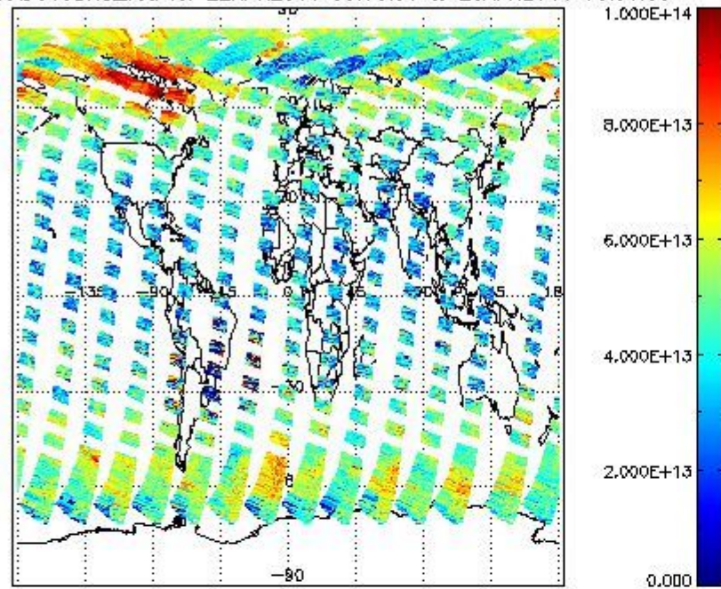
SCIOL2P_NADUV3BRO_vcd for 22APR2011 00:00:00 to 23APR2011 00:00:00
