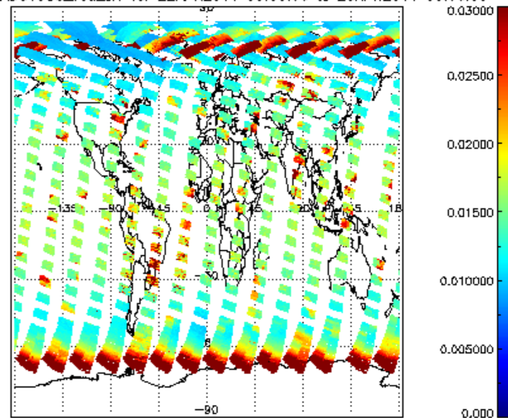
SCIOL2P_NADUV003_vcd_err for 22APR2011 00:00:00 to 23APR2011 00:00:00
