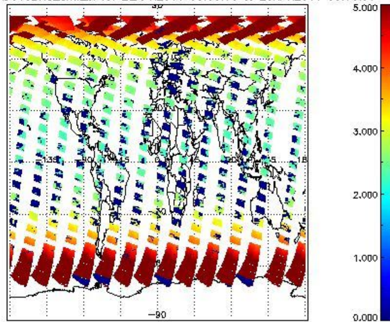
SCIOL2P_NADUV3BRO_amf_cl for 22APR2011 00:00:00 to 23APR2011 00:00:00
