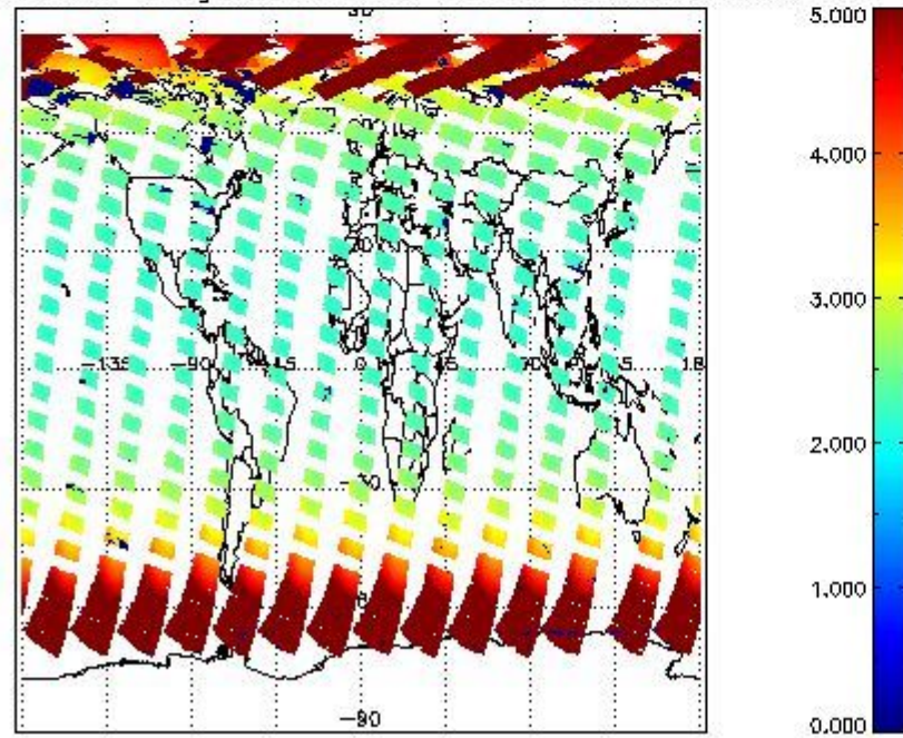
SCIOL2P_NADUV1NO2_amf_gr for 22APR2011 00:00:00 to 23APR2011 00:00:00
