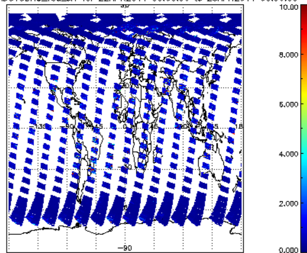
SCIOL2P_NADUV3BRO_vcd_err for 22APR2011 00:00:00 to 23APR2011 00:00:00
