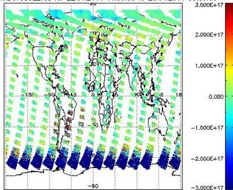
SCIOL2P_NADUV5S02_vcd for 22APR2011 00:00:00 to 23APR2011 00:00:00
