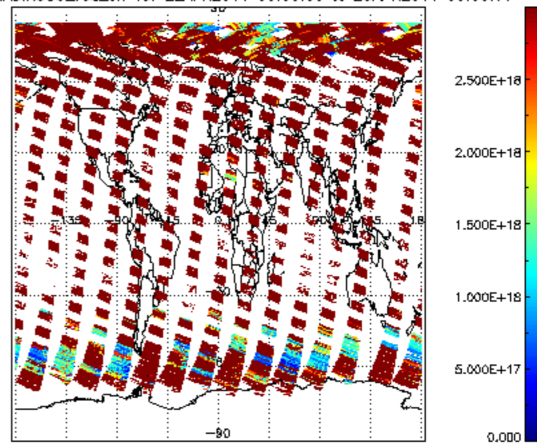
SCIOL2P_NADIR3CO_vcd_err for 22APR2011 00:00:00 to 23APR2011 00:00:00
