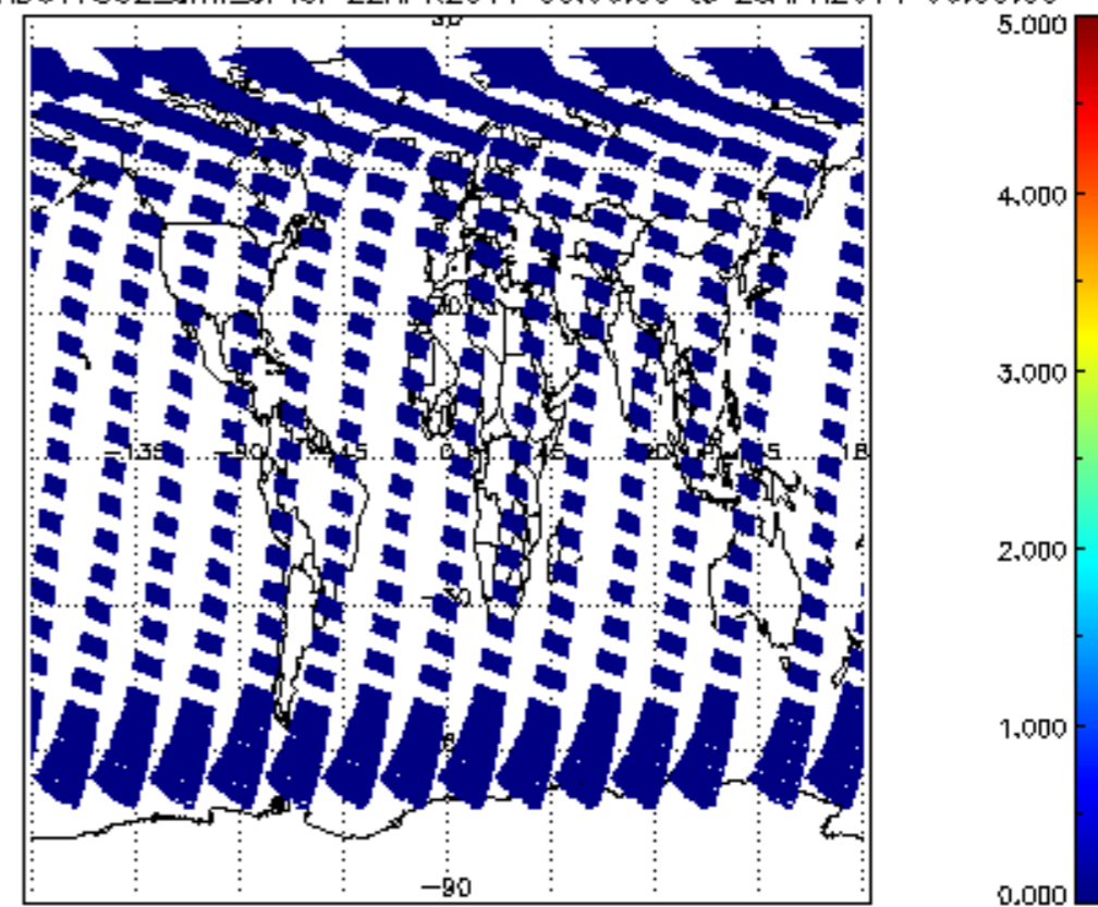
SCIOL2P_NADUV7S02_amf_cl for 22APR2011 00:00:00 to 23APR2011 00:00:00
