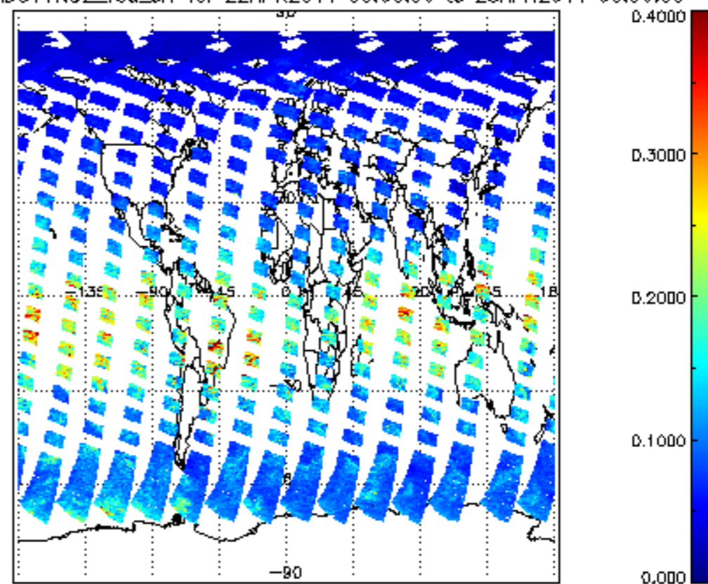
SCIOL2P_NADUV1NO2_vcd_err for 22APR2011 00:00:00 to 23APR2011 00:00:00
