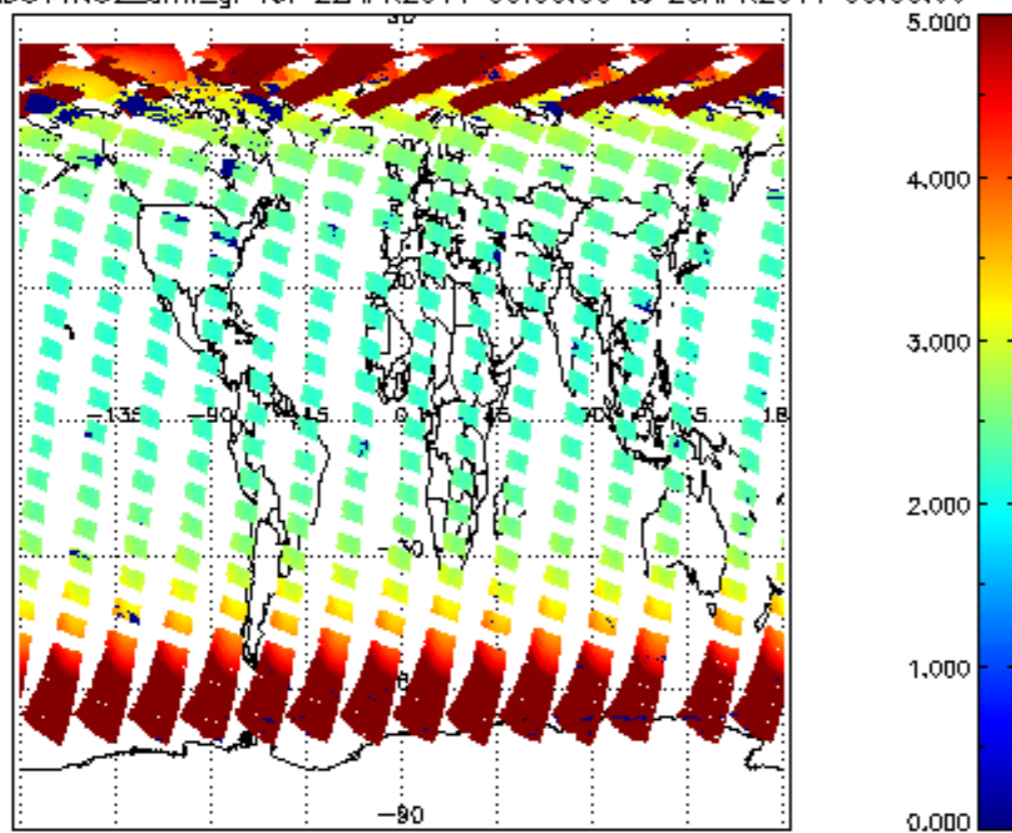
SCIOL2P_NADUV1NO2_amf_gr for 22APR2011 00:00:00 to 23APR2011 00:00:00
