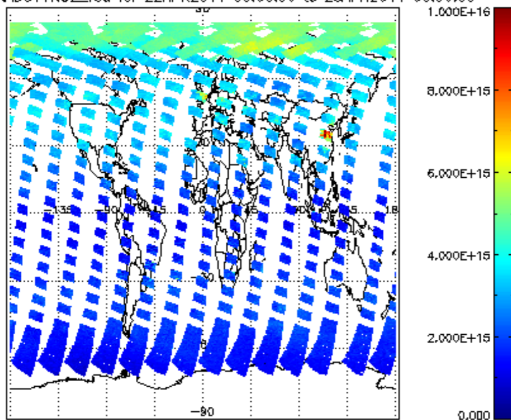
SCIOL2P_NADUV1NO2_vcd for 22APR2011 00:00:00 to 23APR2011 00:00:00
