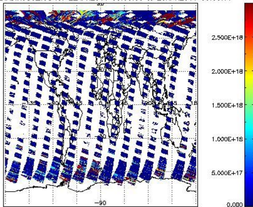
SCIDL2P_NADIR3CO_vcd for 22APR2011 00:00:00 to 23APR2011 00:00:00
