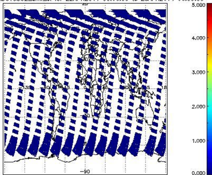
SCIOL2P_NADUV5S02_amf_cl for 22APR2011 00:00:00 to 23APR2011 00:00:00
