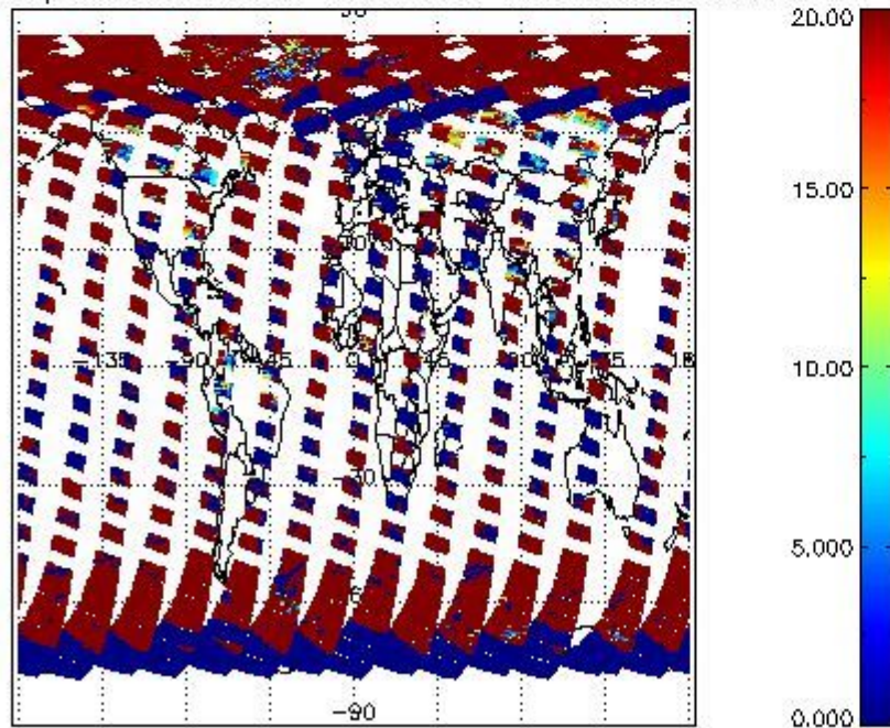
cL_opt_depth for 22APR2011 00:00:00 to 23APR2011 00:00:00
