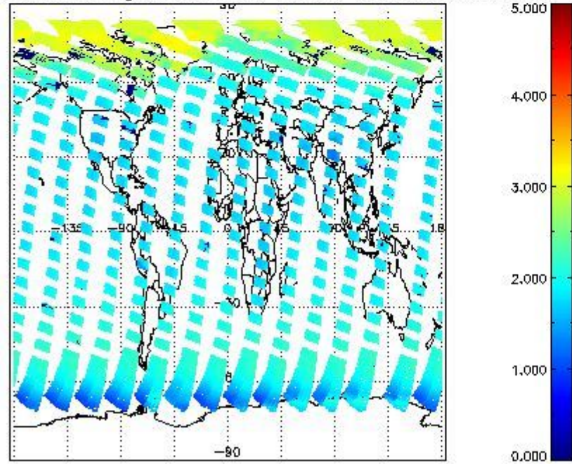
SCIOL2P_NADUV7S02_amf_gr for 22APR2011 00:00:00 to 23APR2011 00:00:00
