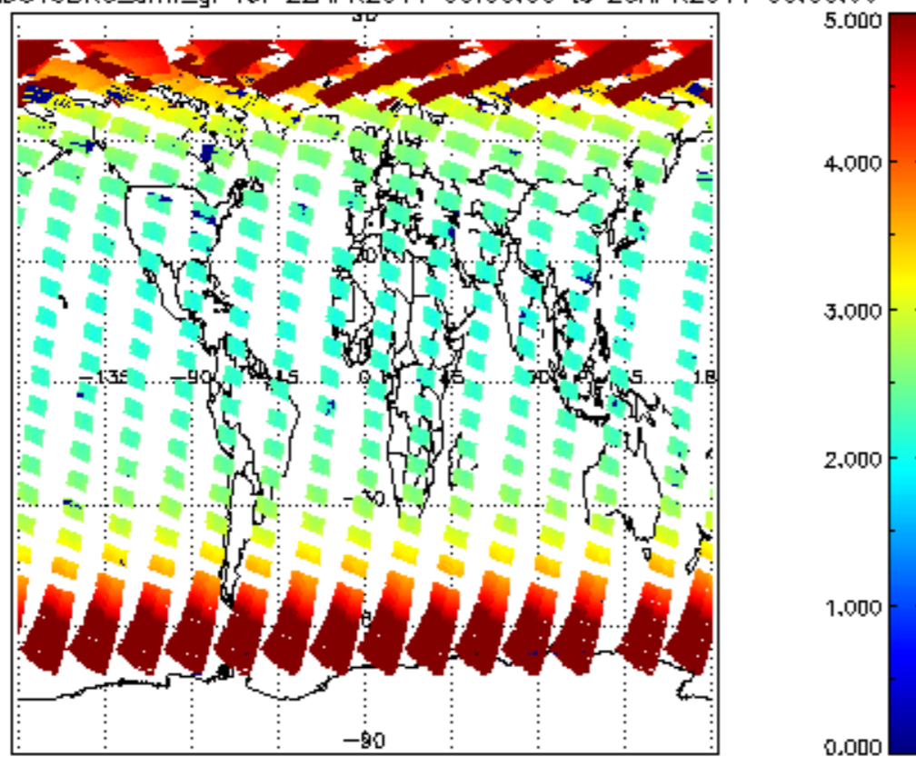
SCIOL2P_NADUV3BRO_amf_gr for 22APR2011 00:00:00 to 23APR2011 00:00:00
