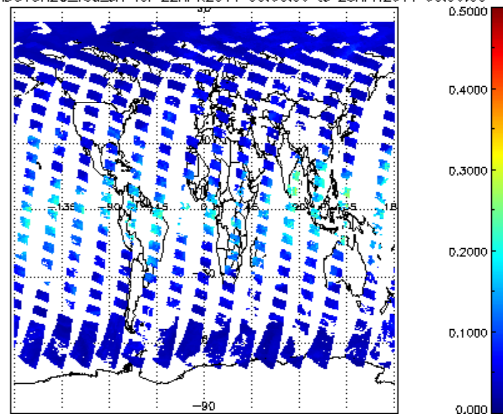
SCIOL2P_NADUV8H2O_vcd_err for 22APR2011 00:00:00 to 23APR2011 00:00:00
