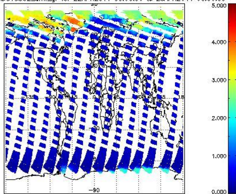
SCIOL2P_NADUV5S02_amf_gr for 22APR2011 00:00:00 to 23APR2011 00:00:00
