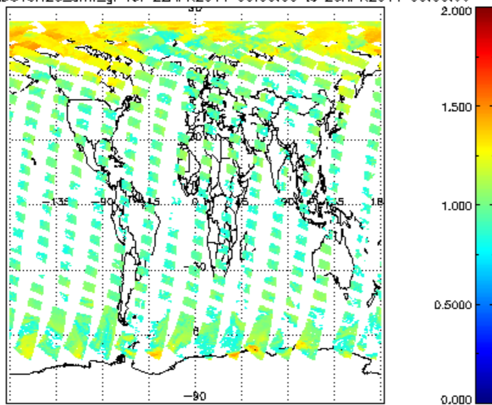
SCIOL2P_NADUV8H2O_amf_gr for 22APR2011 00:00:00 to 23APR2011 00:00:00
