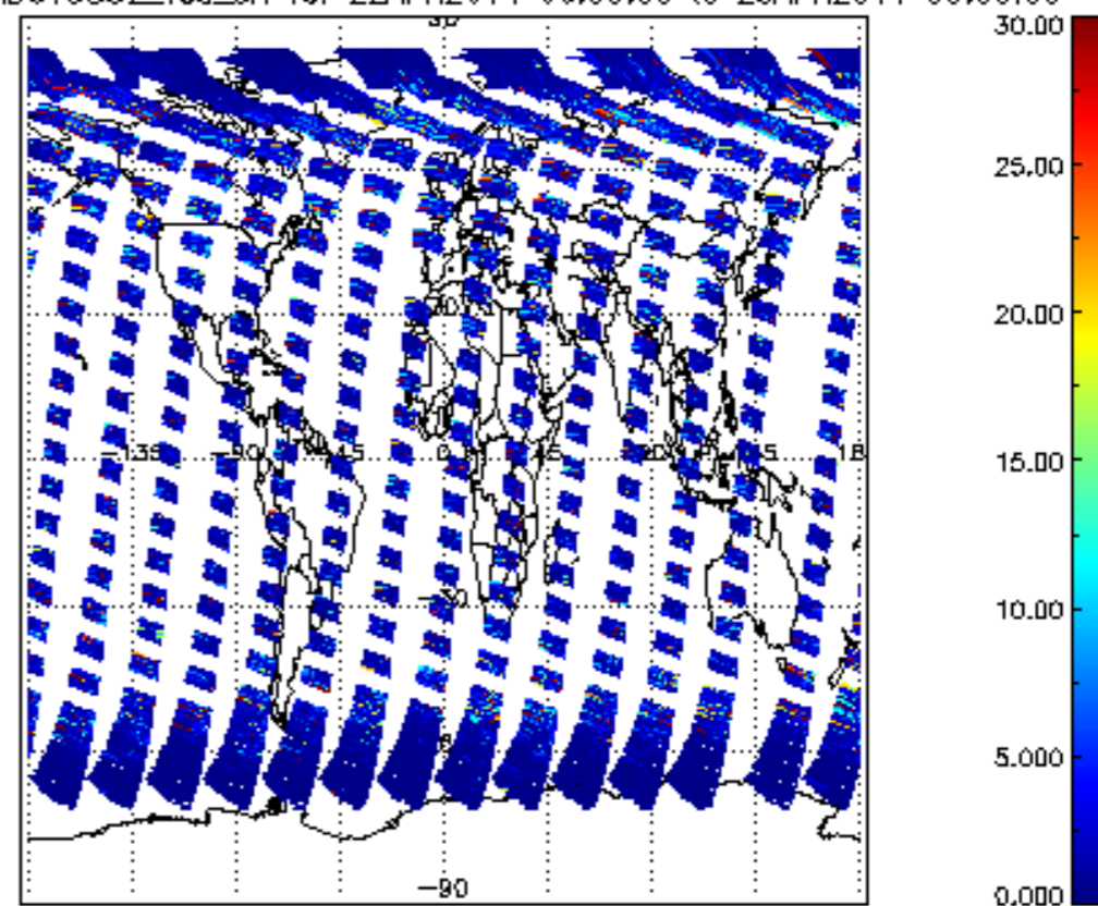
SCIOL2P_NADUV5S02_vcd_err for 22APR2011 00:00:00 to 23APR2011 00:00:00
