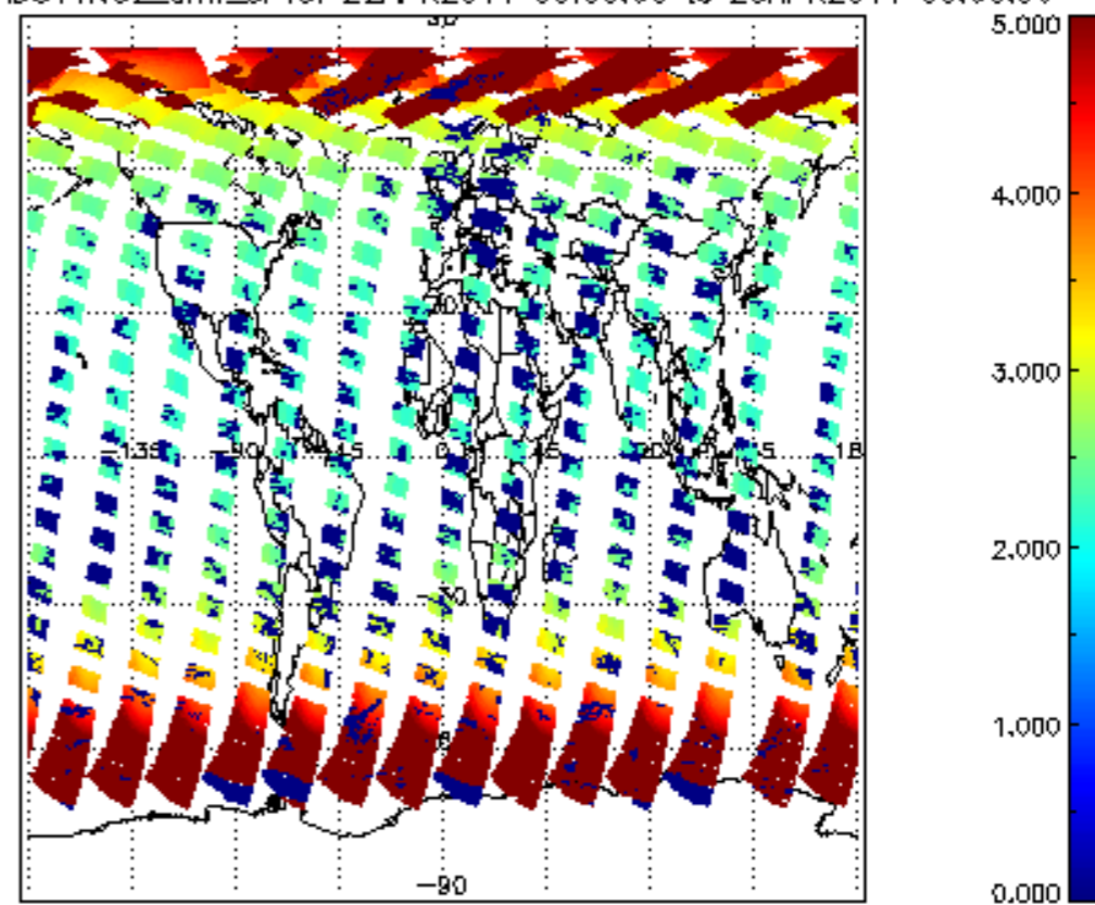
SCIOL2P_NADUV1NO2_amf_sl for 22APR2011 00:00:00 to 23APR2011 00:00:00
