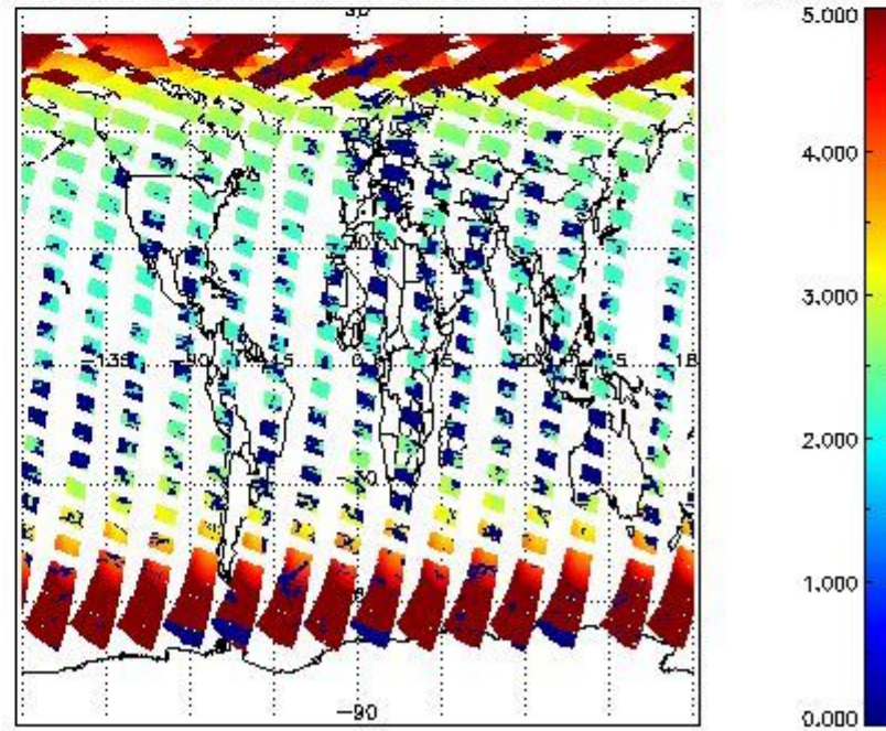
SCIOL2P_NADUV1NO2_amf_cl for 22APR2011 00:00:00 to 23APR2011 00:00:00
