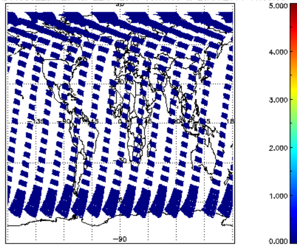
SCIOL2P_NADUV5S02_amf_cl for 22APR2011 00:00:00 to 23APR2011 00:00:00
