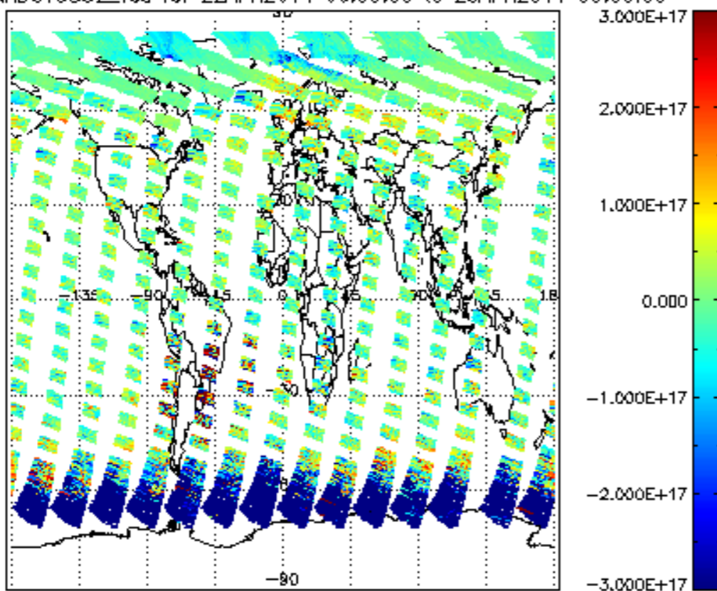
SCIOL2P_NADUV5S02_vcd for 22APR2011 00:00:00 to 23APR2011 00:00:00
