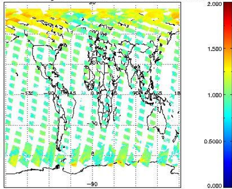
SCIOL2P_NADUV8H2O_amf_gr for 22APR2011 00:00:00 to 23APR2011 00:00:00
