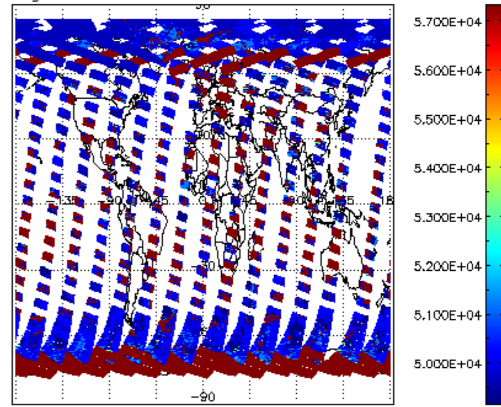
cloud_flags for 22APR2011 00:00:00 to 23APR2011 00:00:00
