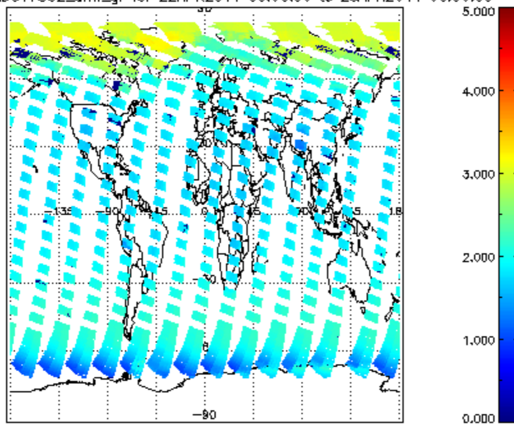
SCIOL2P_NADUV7S02_amf_gr for 22APR2011 00:00:00 to 23APR2011 00:00:00
