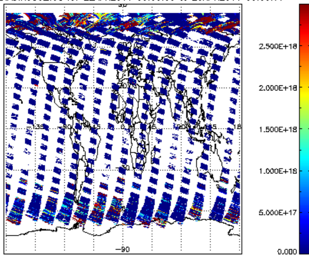
SCIOL2P_NADIR3CO_vcd for 22APR2011 00:00:00 to 23APR2011 00:00:00
