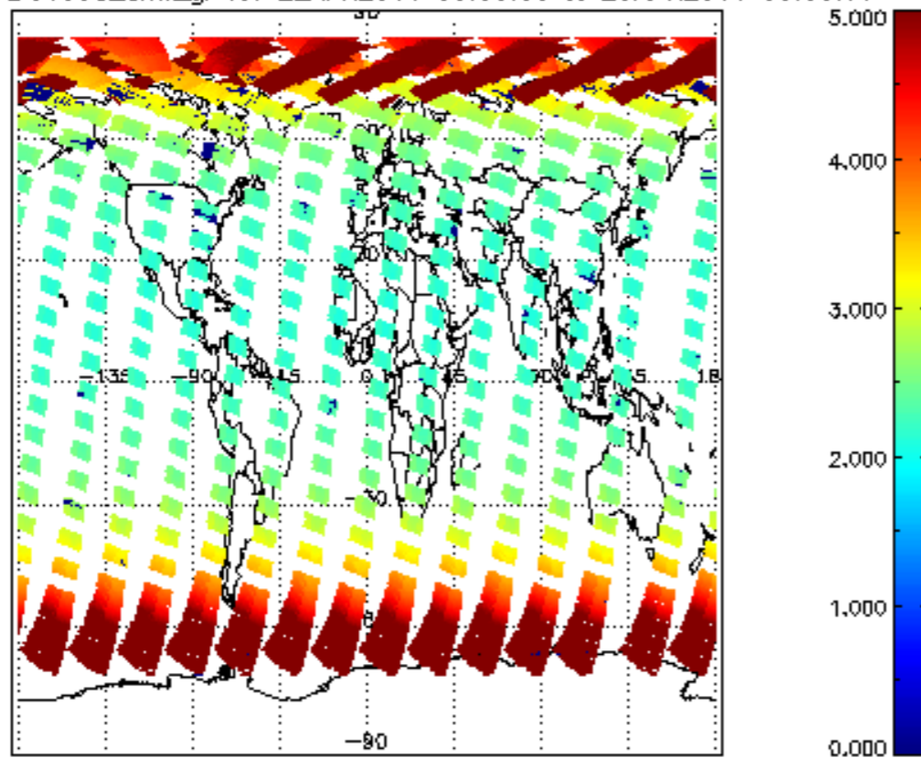
SCIOL2P_NADUV003_amf_gr for 22APR2011 00:00:00 to 23APR2011 00:00:00
