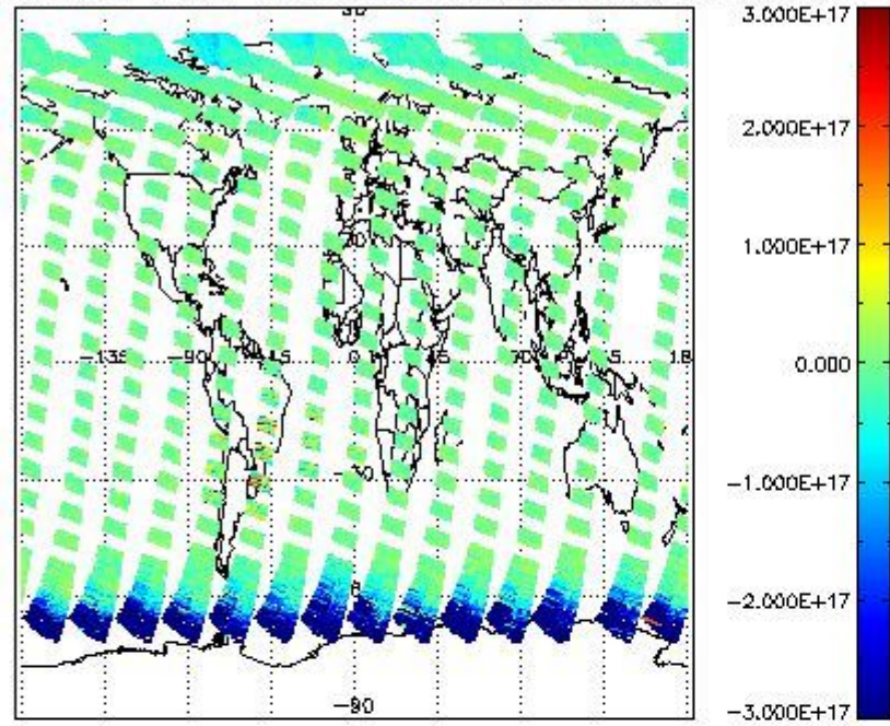
SCIOL2P_NADUV7S02_vcd for 22APR2011 00:00:00 to 23APR2011 00:00:00
