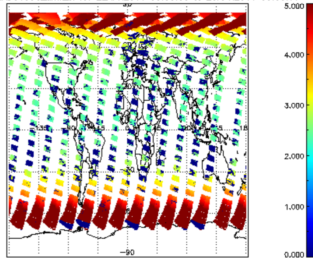
SCIOL2P_NADUV003_amf_cl for 22APR2011 00:00:00 to 23APR2011 00:00:00
