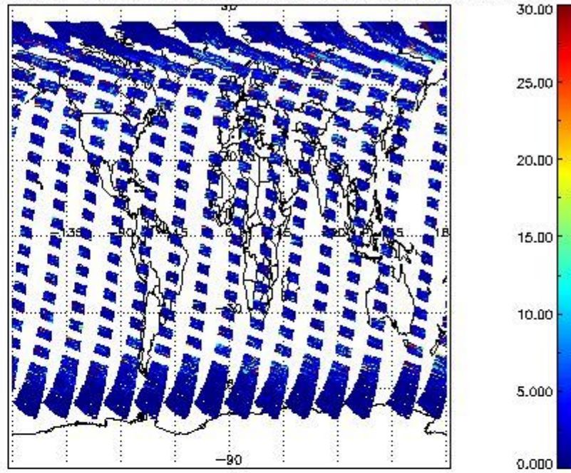
SCIOL2P_NADUV7S02_vcd_err for 22APR2011 00:00:00 to 23APR2011 00:00:00
