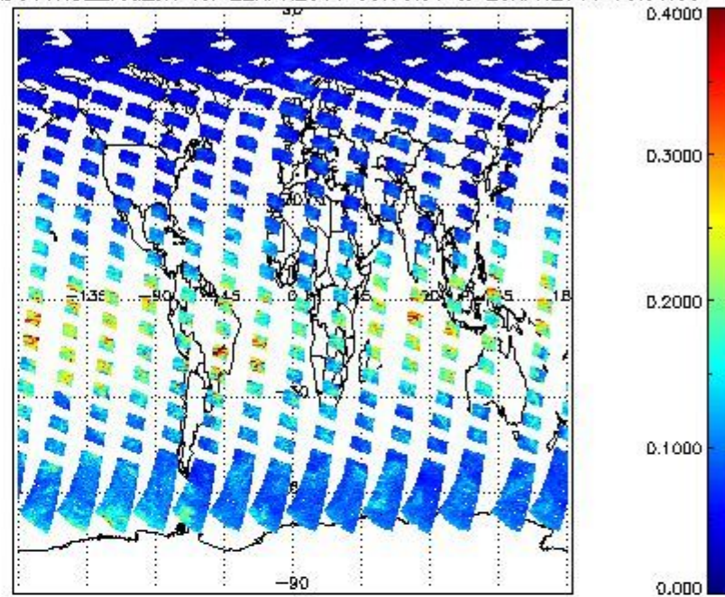
SCIOL2P_NADUV1NO2_vcd_err for 22APR2011 00:00:00 to 23APR2011 00:00:00
