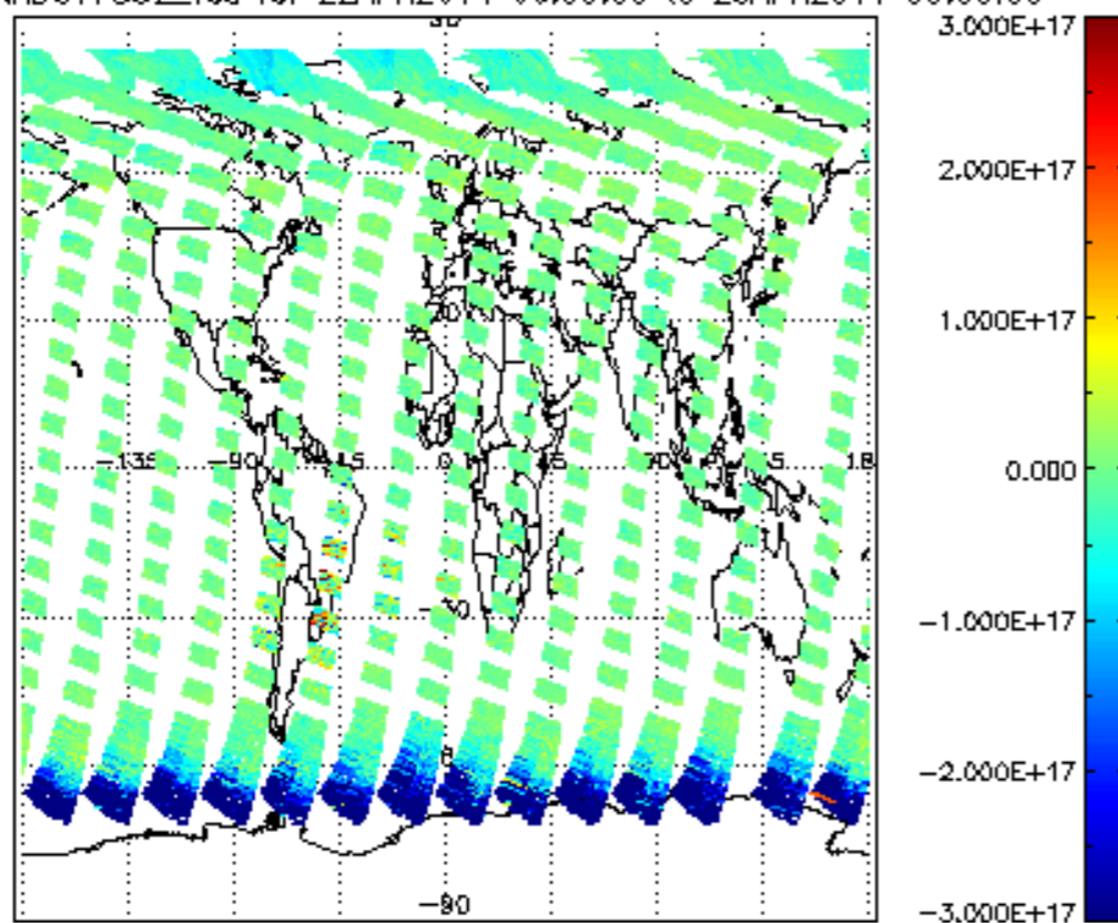
SCIOL2P_NADUV7S02_vcd for 22APR2011 00:00:00 to 23APR2011 00:00:00
