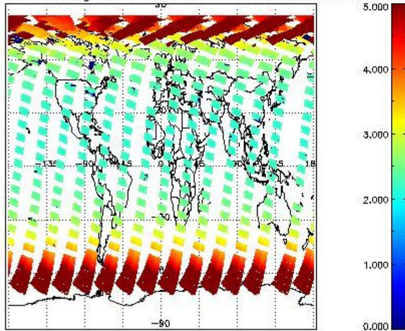
SCIOL2P_NADUV003_amf_gr for 22APR2011 00:00:00 to 23APR2011 00:00:00
