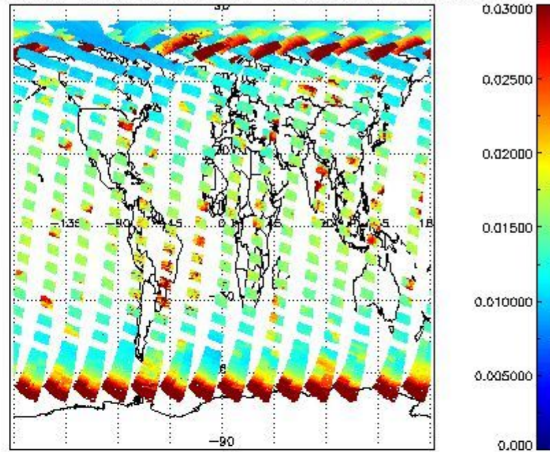
SCIOL2P_NADUV003_vcd_err for 22APR2011 00:00:00 to 23APR2011 00:00:00
