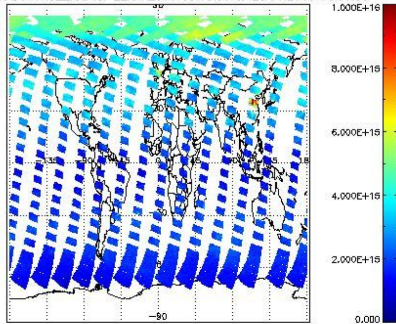
SCIOL2P_NADUV1NO2_vcd for 22APR2011 00:00:00 to 23APR2011 00:00:00
