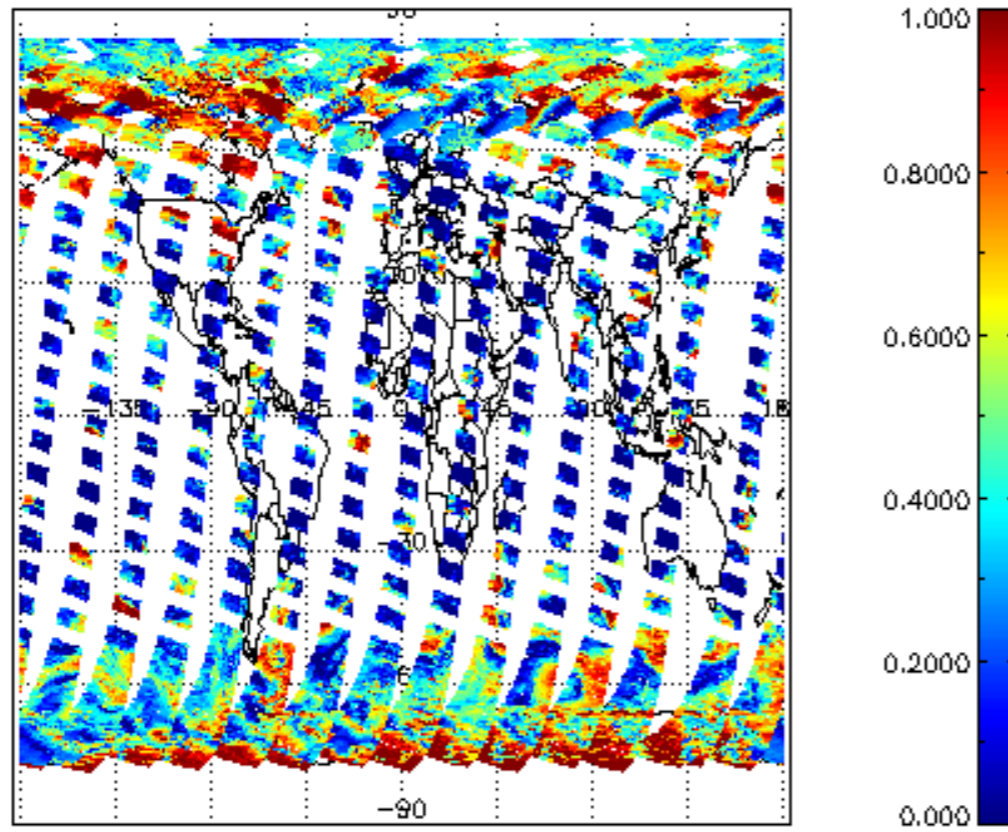
cl_frac for 22APR2011 00:00:00 to 23APR2011 00:00:00
