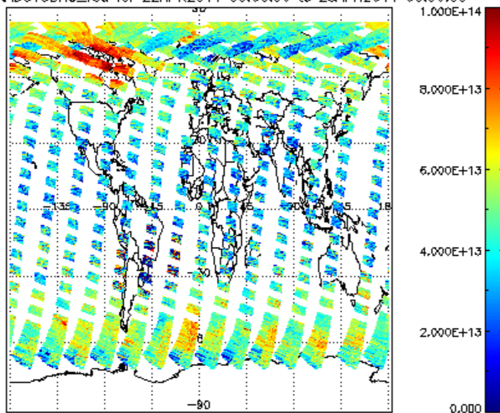
SCIOL2P_NADUV3BRO_vcd for 22APR2011 00:00:00 to 23APR2011 00:00:00
