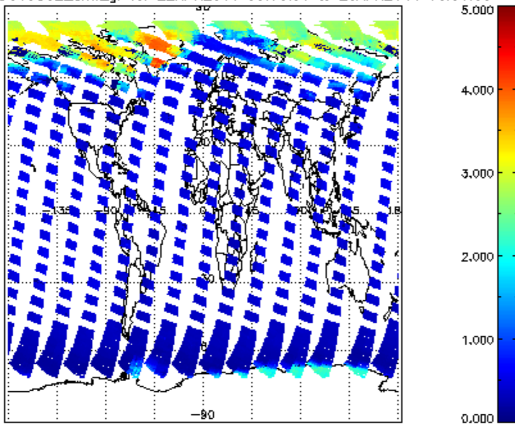
SCIOL2P_NADUV5S02_amf_gr for 22APR2011 00:00:00 to 23APR2011 00:00:00
