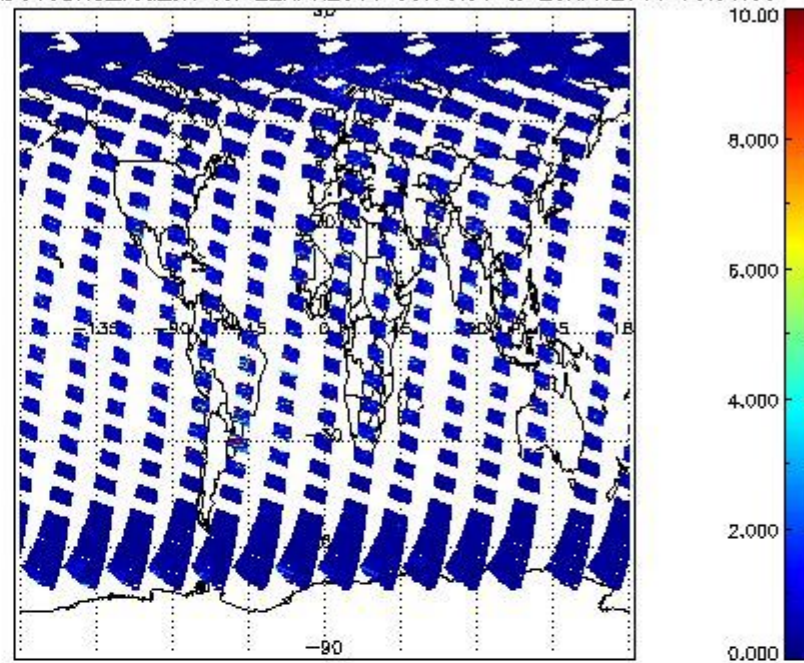
SCIOL2P_NADUV3BRO_vcd_err for 22APR2011 00:00:00 to 23APR2011 00:00:00
