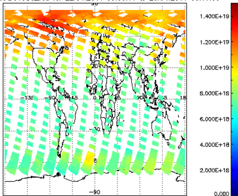
SCIOL2P_NADUV003_vcd for 22APR2011 00:00:00 to 23APR2011 00:00:00
