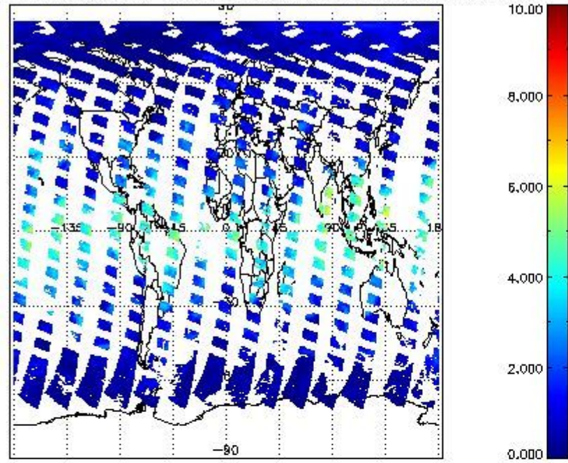
SCIOL2P_NADUV8H2O_vcd for 22APR2011 00:00:00 to 23APR2011 00:00:00
