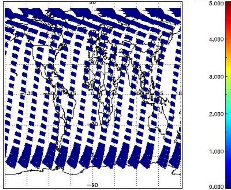
SCIOL2P_NADUV7S02_amf_cl for 22APR2011 00:00:00 to 23APR2011 00:00:00
