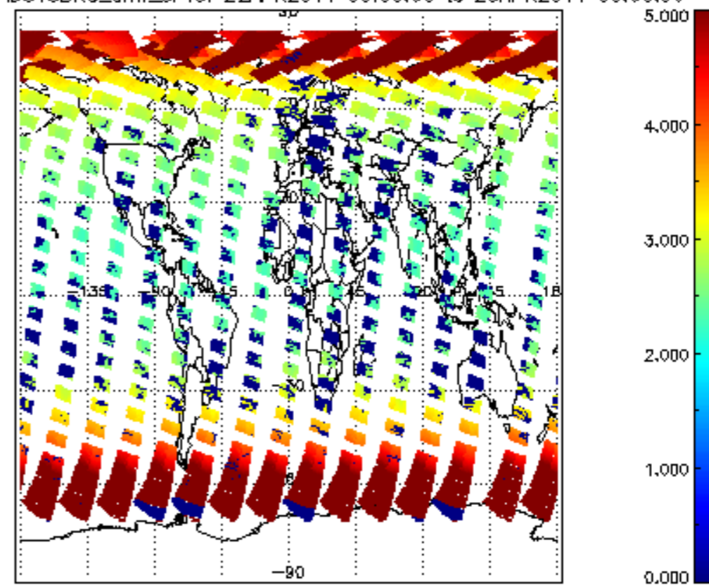
SCIOL2P_NADUV3BRO_amf_sl for 22APR2011 00:00:00 to 23APR2011 00:00:00
