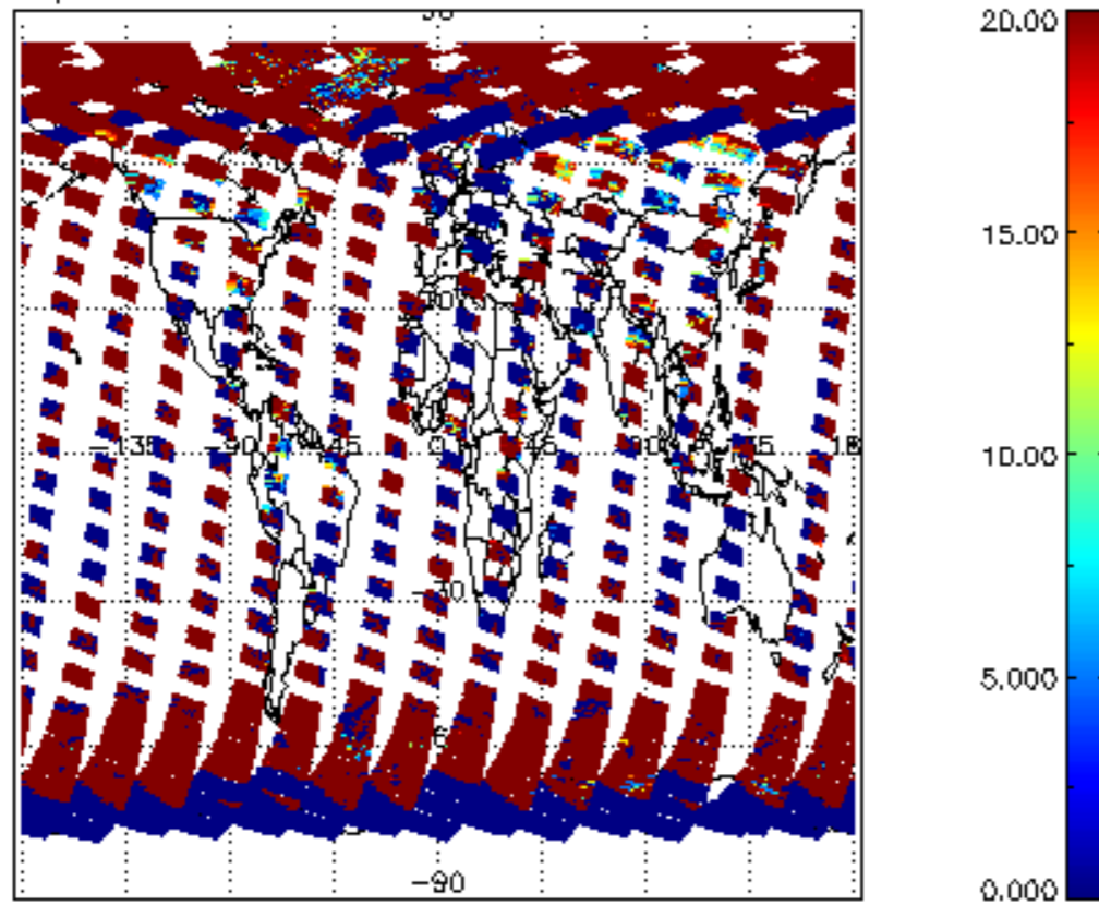
cl_opt_depth for 22APR2011 00:00:00 to 23APR2011 00:00:00
