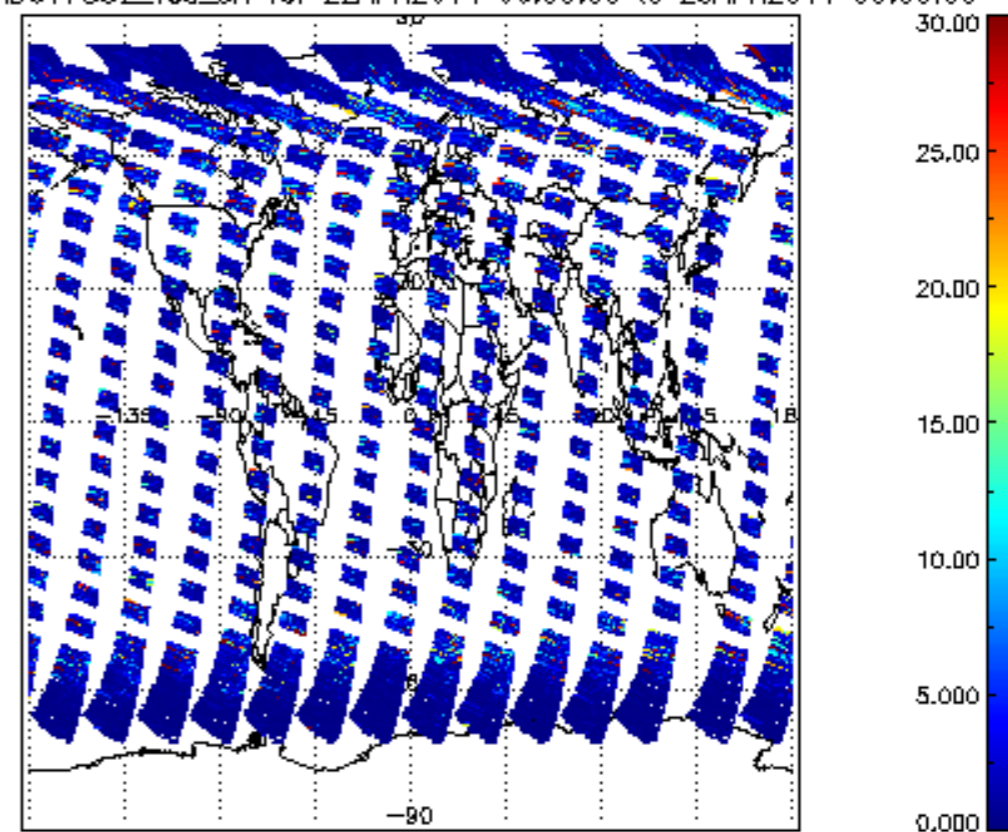
SCIOL2P_NADUV7S02_vcd_err for 22APR2011 00:00:00 to 23APR2011 00:00:00
