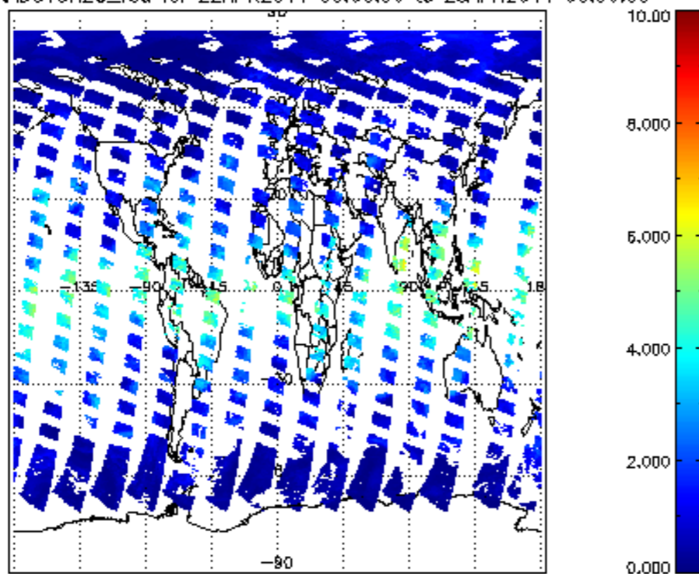
SCIOL2P_NADUV8H2O_vcd for 22APR2011 00:00:00 to 23APR2011 00:00:00
