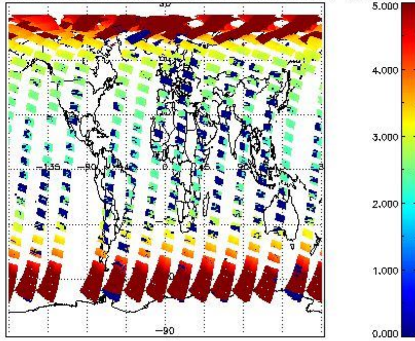
SCIOL2P_NADUV3BRO_amf_cl for 20APR2011 00:00:00 to 21APR2011 00:00:00
