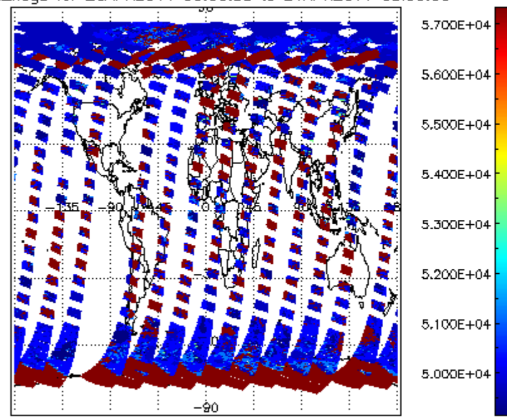
cloud_flags for 20APR2011 00:00:00 to 21APR2011 00:00:00
