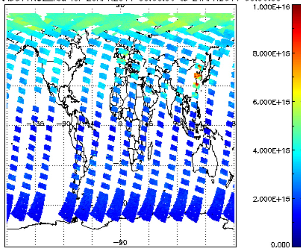
SCIOL2P_NADUV1NO2_vcd for 20APR2011 00:00:00 to 21APR2011 00:00:00
