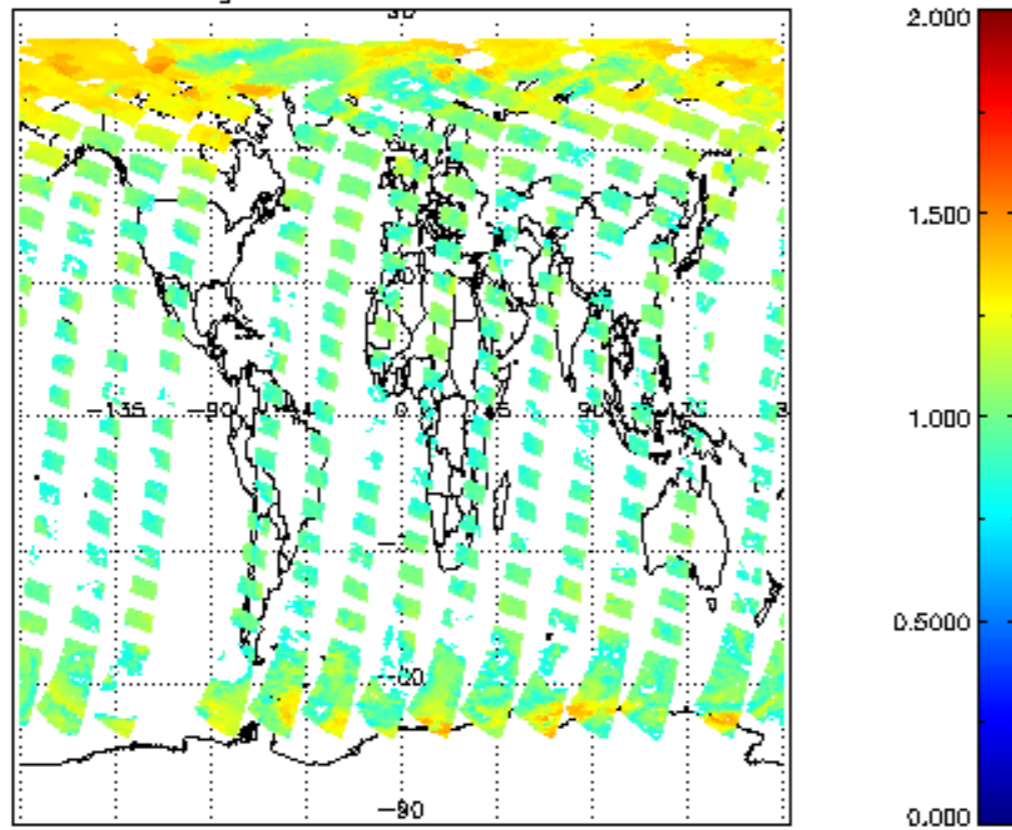
SCIOL2P_NADUV8H2O_amf_gr for 20APR2011 00:00:00 to 21APR2011 00:00:00
