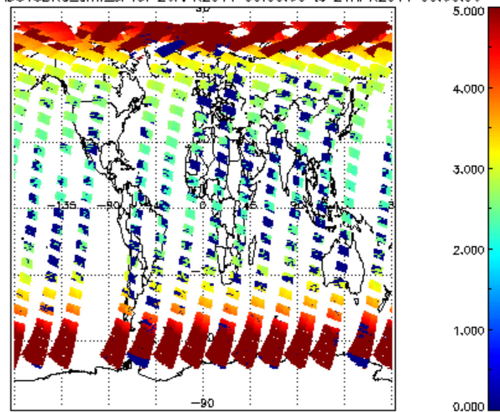
SCIOL2P_NADUV3BRO_amf_cl for 20APR2011 00:00:00 to 21APR2011 00:00:00
