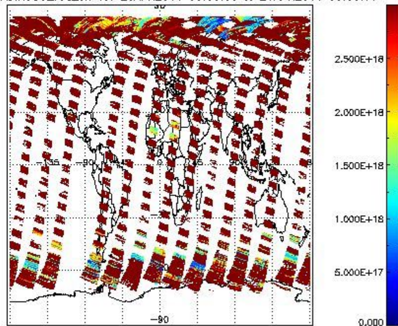
SCIDL2P_NADIR3CO_vcd_err for 20APR2011 00:00:00 to 21APR2011 00:00:00
