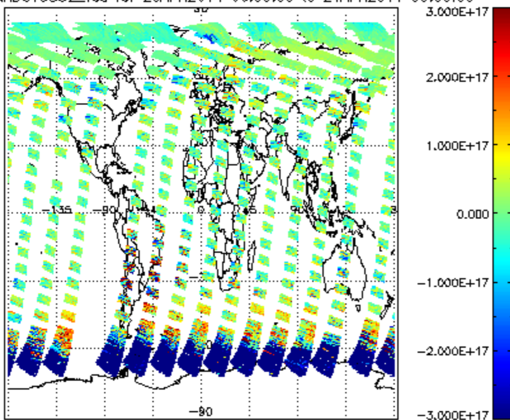
SCIOL2P_NADUV5S02_vcd for 20APR2011 00:00:00 to 21APR2011 00:00:00
