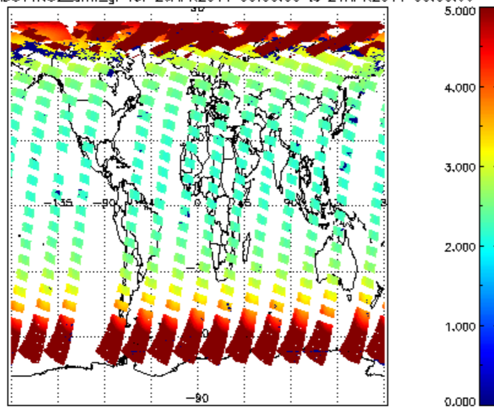
SCIOL2P_NADUV1NO2_amf_gr for 20APR2011 00:00:00 to 21APR2011 00:00:00
