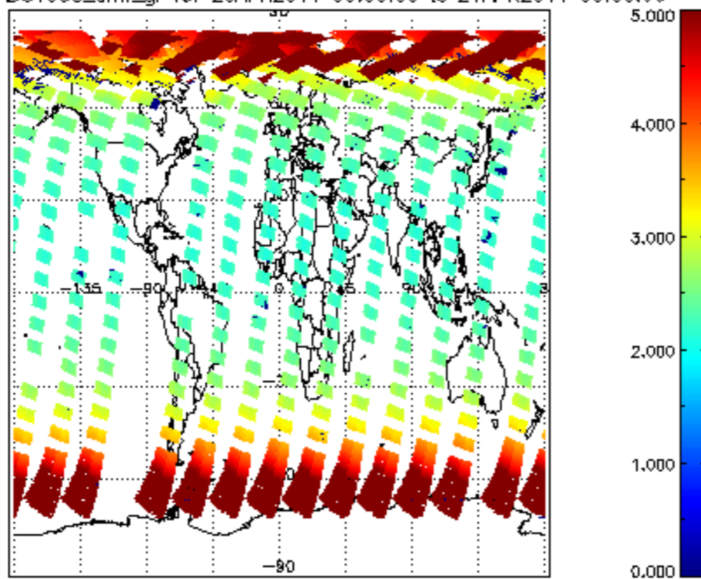
SCIOL2P_NADUV003_amf_gr for 20APR2011 00:00:00 to 21APR2011 00:00:00
