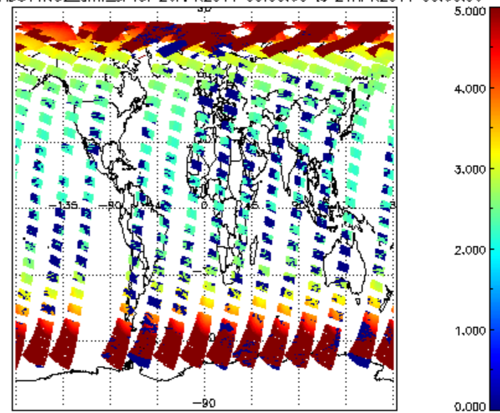
SCIOL2P_NADUV1NO2_amf_sl for 20APR2011 00:00:00 to 21APR2011 00:00:00
