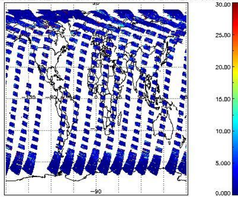
SCIOL2P_NADUV7S02_vcd_err for 20APR2011 00:00:00 to 21APR2011 00:00:00
