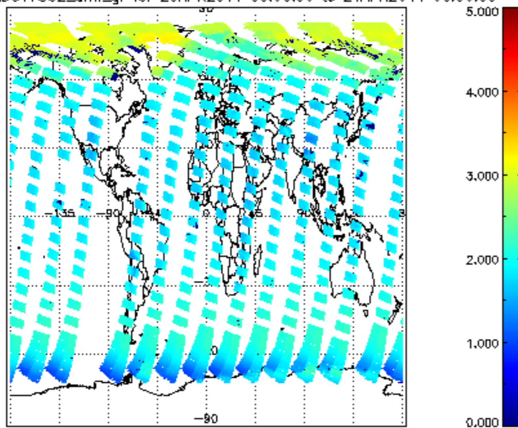
SCIOL2P_NADUV7S02_amf_gr for 20APR2011 00:00:00 to 21APR2011 00:00:00
