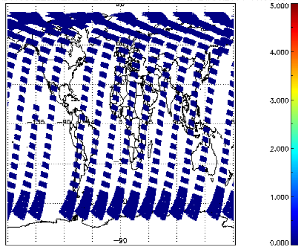
SCIOL2P_NADUV5S02_amf_cl for 20APR2011 00:00:00 to 21APR2011 00:00:00
