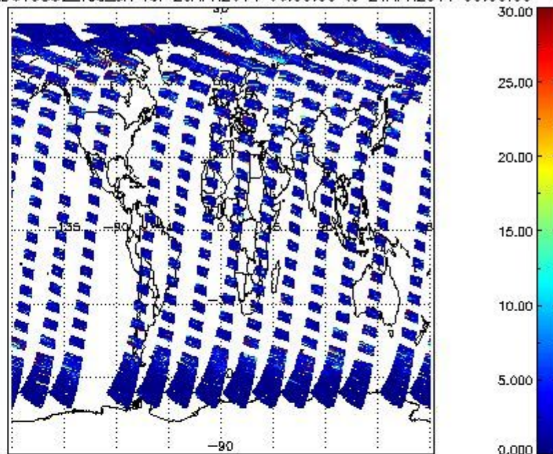
SCIOL2P_NADUV5S02_vcd_err for 20APR2011 00:00:00 to 21APR2011 00:00:00
