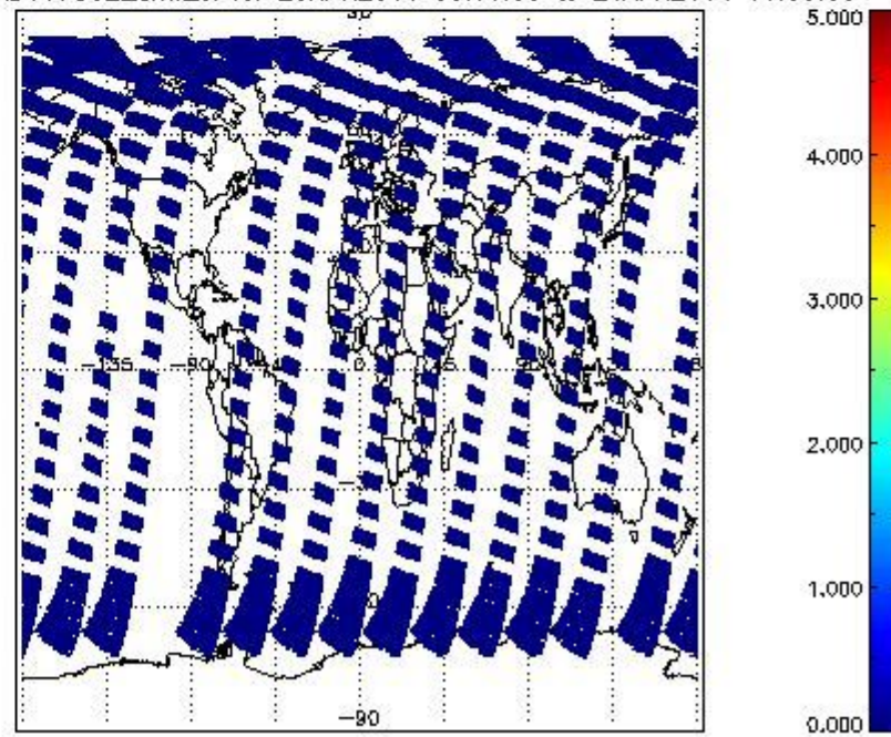
SCIOL2P_NADUV7S02_amf_cl for 20APR2011 00:00:00 to 21APR2011 00:00:00
