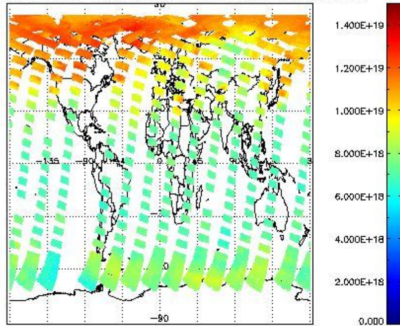
SCIOL2P_NADUV003_vcd for 20APR2011 00:00:00 to 21APR2011 00:00:00
