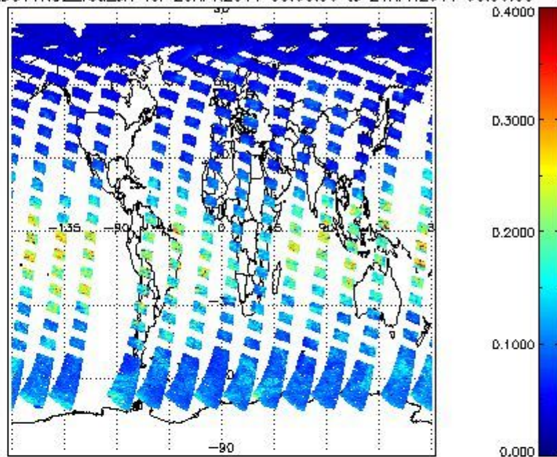
SCIOL2P_NADUV1NO2_vcd_err for 20APR2011 00:00:00 to 21APR2011 00:00:00
