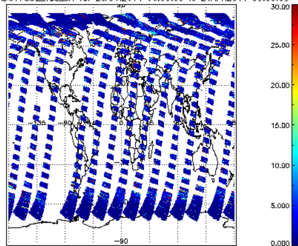
SCIOL2P_NADUV7S02_vcd_err for 20APR2011 00:00:00 to 21APR2011 00:00:00
