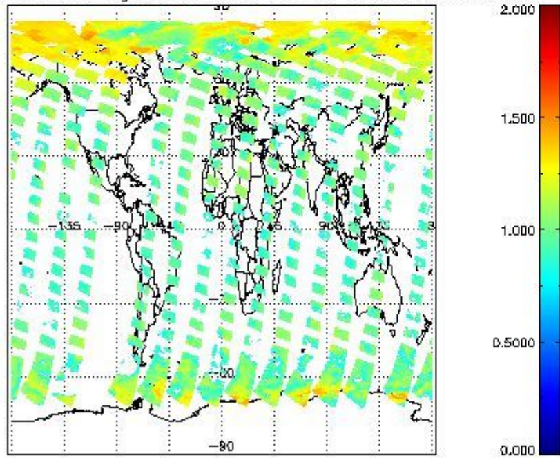
SCIOL2P_NADUV8H2O_arnf_gr for 20APR2011 00:00:00 to 21APR2011 00:00:00
