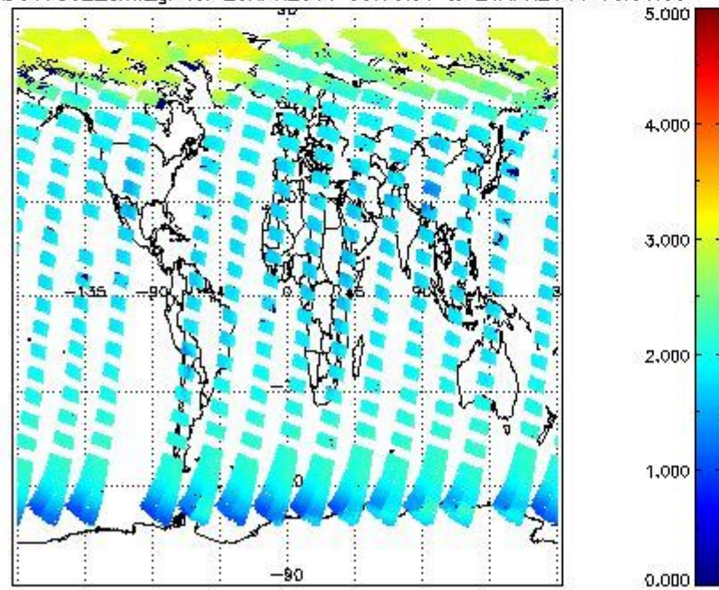
SCIOL2P_NADUV7S02_amf_gr for 20APR2011 00:00:00 to 21APR2011 00:00:00
