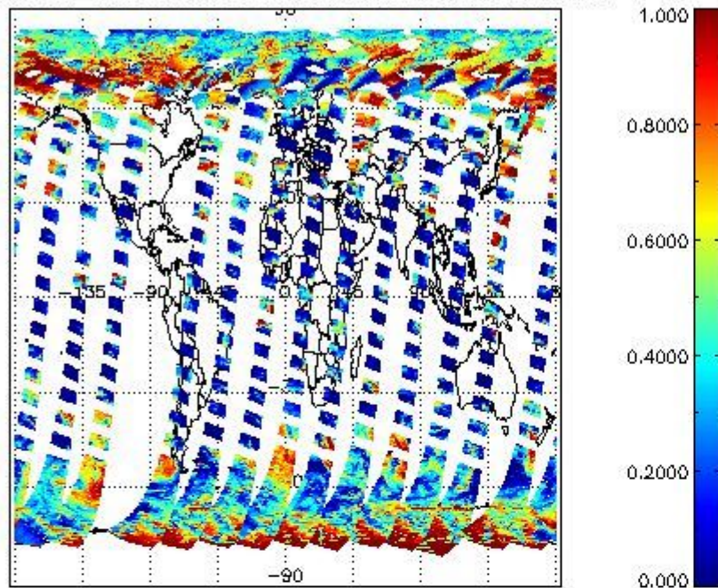
cL_frac for 20APR2011 00:00:00 to 21APR2011 00:00:00
