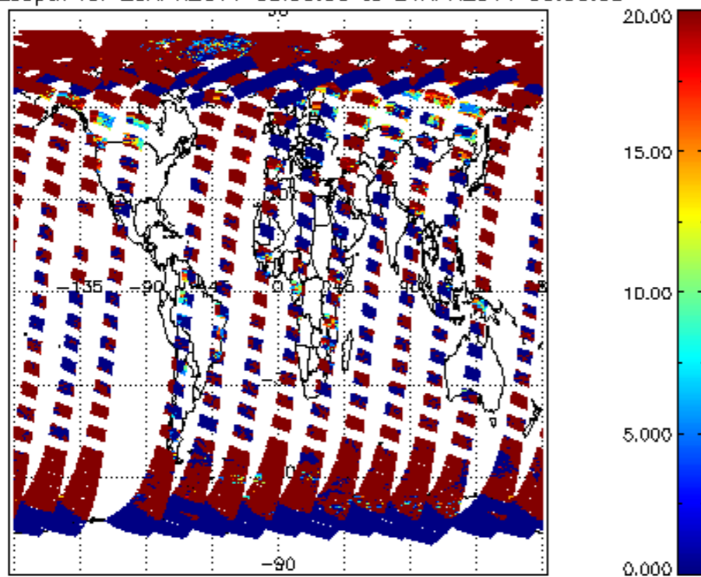
cl_opt_depth for 20APR2011 00:00:00 to 21APR2011 00:00:00
