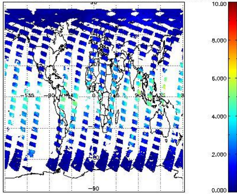
SCIOL2P_NADUV8H2O_vcd for 20APR2011 00:00:00 to 21APR2011 00:00:00
