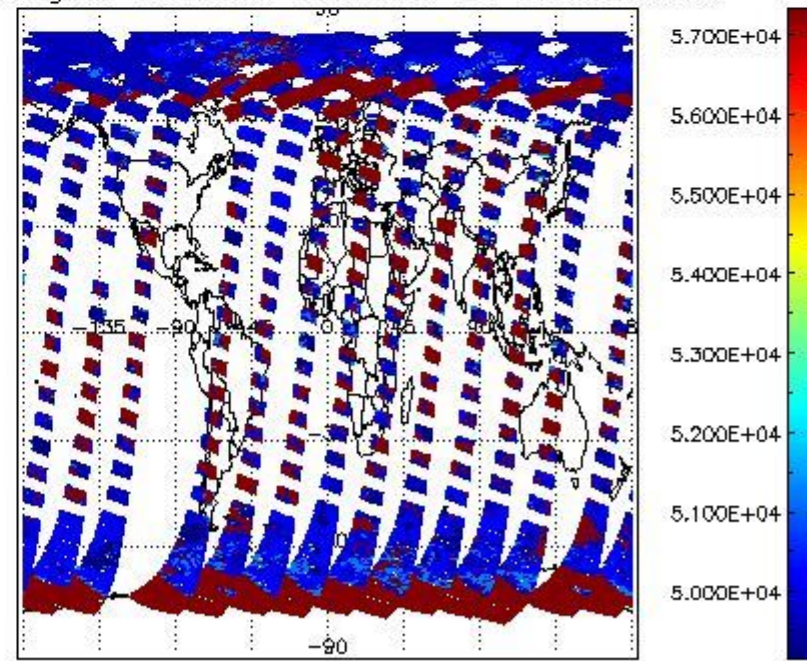
cloud_flags for 20APR2011 00:00:00 to 21APR2011 00:00:00
