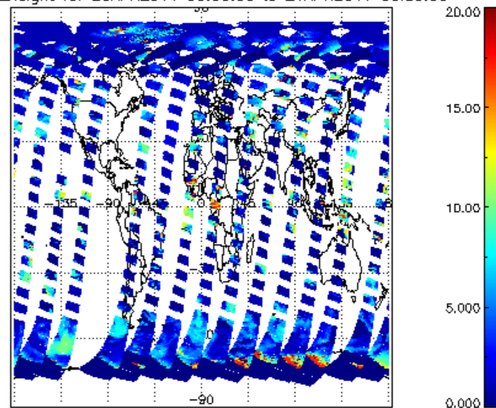
cl_top_height for 20APR2011 00:00:00 to 21APR2011 00:00:00
