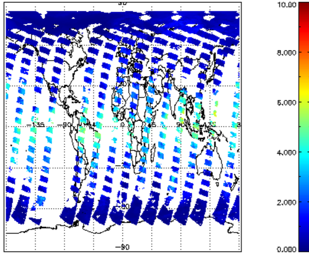
SCIOL2P_NADUV8H2O_vcd for 20APR2011 00:00:00 to 21APR2011 00:00:00
