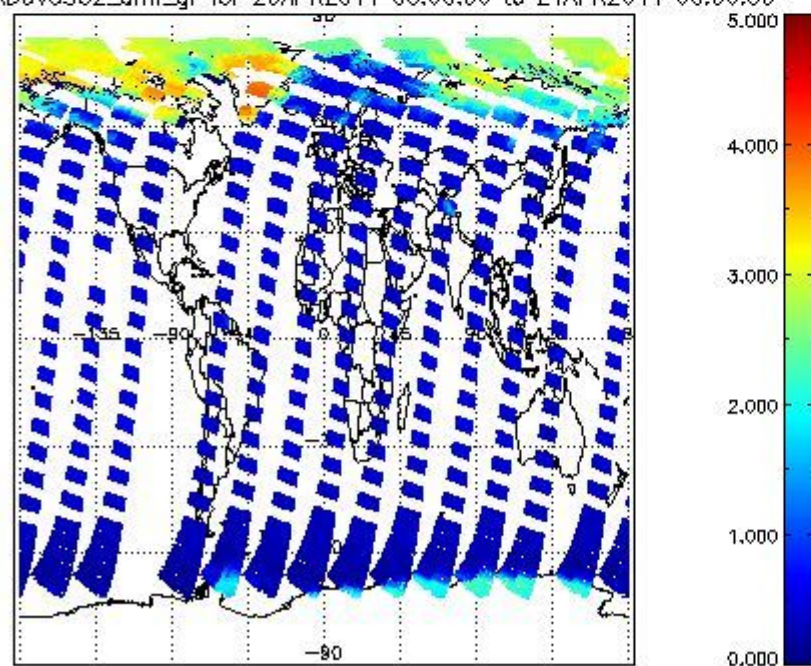
SCIOL2P_NADUV5S02_amf_gr for 20APR2011 00:00:00 to 21APR2011 00:00:00
