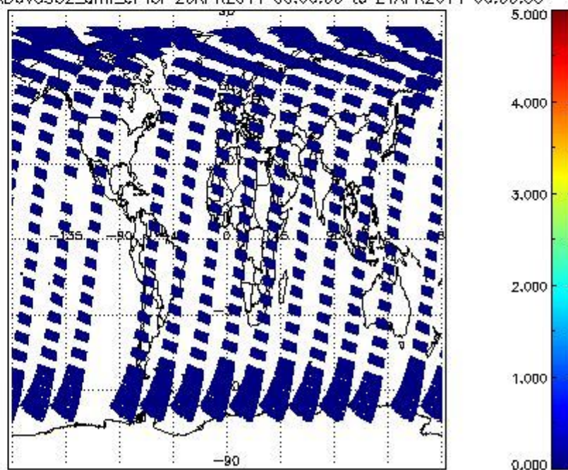
SCIOL2P_NADUV5S02_amf_cl for 20APR2011 00:00:00 to 21APR2011 00:00:00
