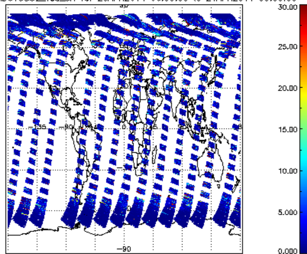
SCIOL2P_NADUV5S02_vcd_err for 20APR2011 00:00:00 to 21APR2011 00:00:00
