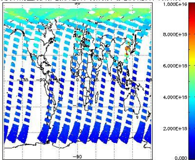
SCIOL2P_NADUV1NO2_vcd for 20APR2011 00:00:00 to 21APR2011 00:00:00
