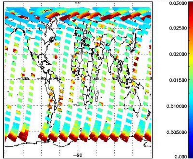
SCIOL2P_NADUV003_vcd_err for 20APR2011 00:00:00 to 21APR2011 00:00:00
