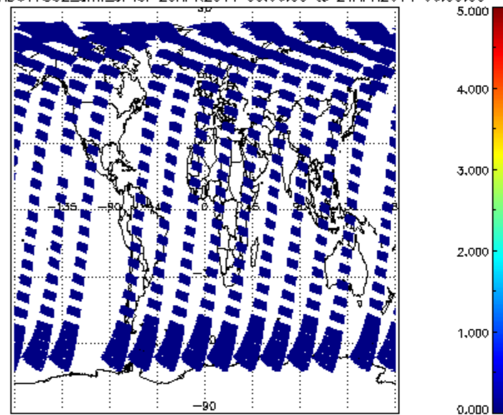
SCIOL2P_NADUV7S02_amf_cl for 20APR2011 00:00:00 to 21APR2011 00:00:00
