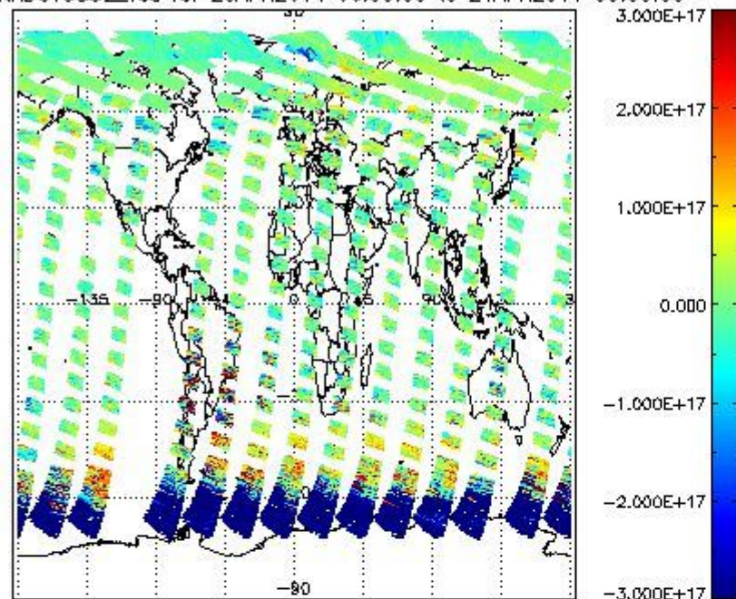
SCIOL2P_NADUV5S02_vcd for 20APR2011 00:00:00 to 21APR2011 00:00:00
