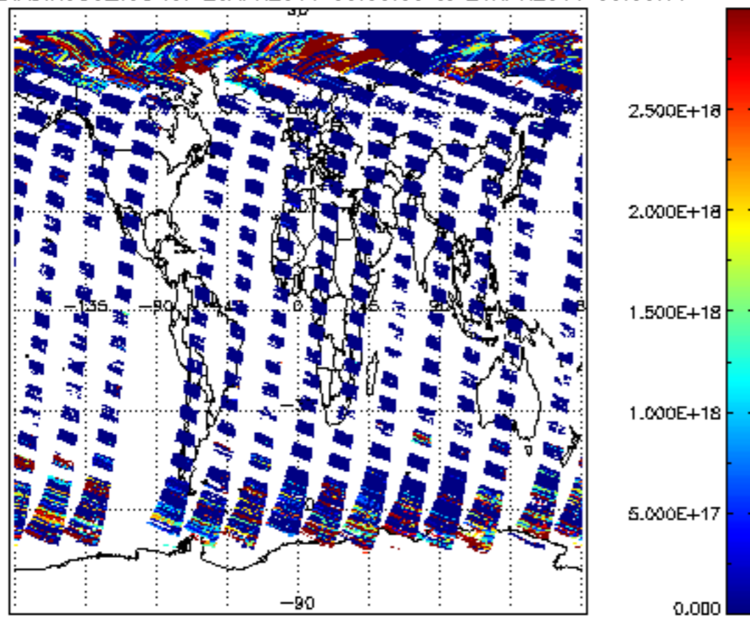
SCIOL2P_NADIR3CO_vcd for 20APR2011 00:00:00 to 21APR2011 00:00:00
