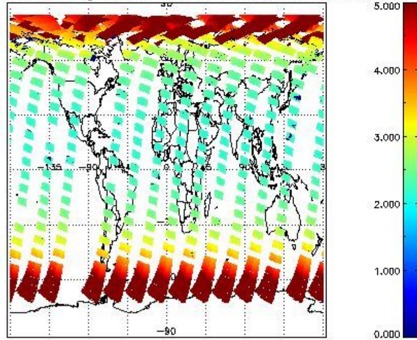
SCIOL2P_NADUV003_amf_gr for 20APR2011 00:00:00 to 21APR2011 00:00:00
