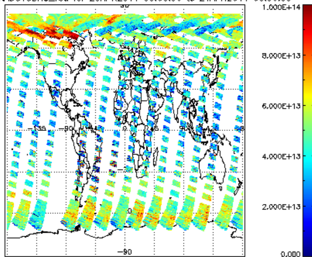
SCIOL2P_NADUV3BRO_vcd for 20APR2011 00:00:00 to 21APR2011 00:00:00
