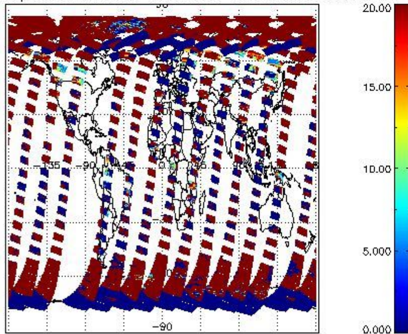
cL_opt_depth for 20APR2011 00:00:00 to 21APR2011 00:00:00
