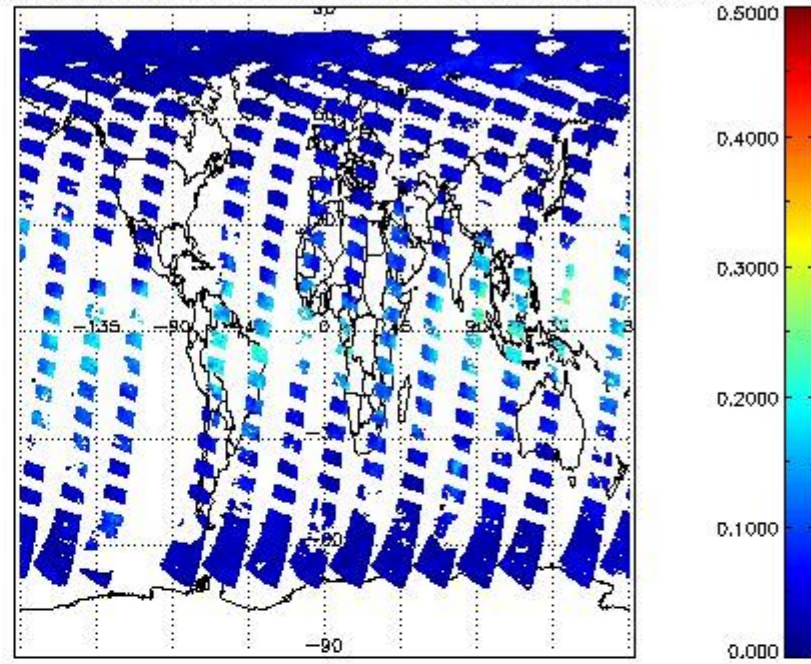
SCIOL2P_NADUV8H2O_vcd_err for 20APR2011 00:00:00 to 21APR2011 00:00:00
