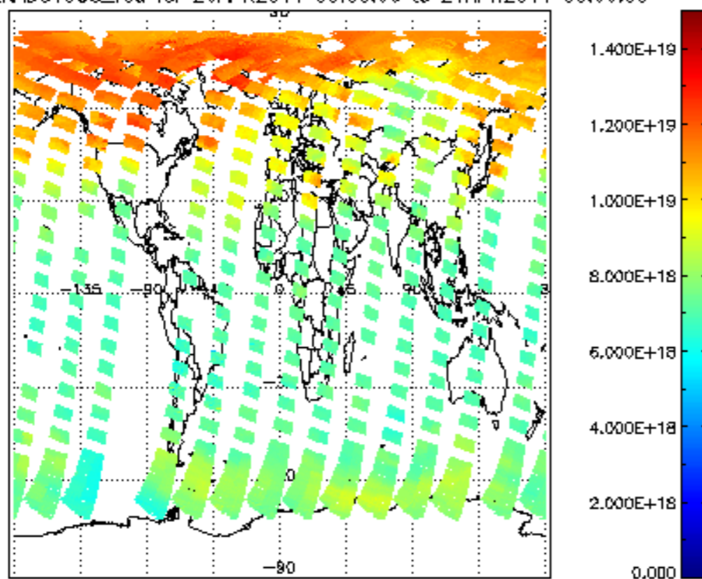
SCIOL2P_NADUV003_vcd for 20APR2011 00:00:00 to 21APR2011 00:00:00
