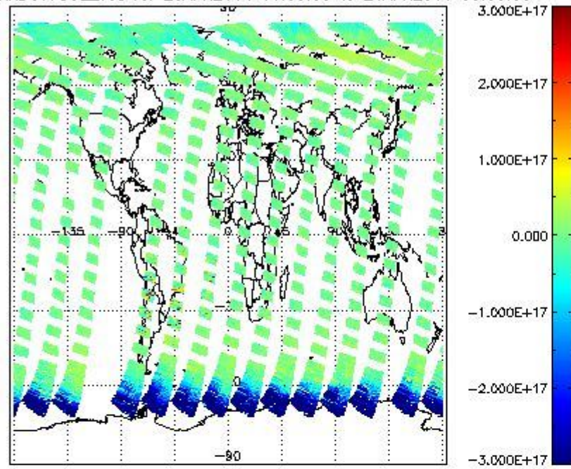
SCIOL2P_NADUV7S02_vcd for 20APR2011 00:00:00 to 21APR2011 00:00:00
