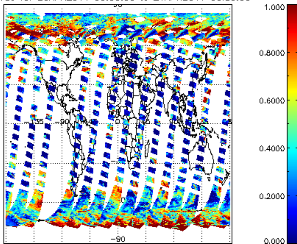
cl_frac for 20APR2011 00:00:00 to 21APR2011 00:00:00
