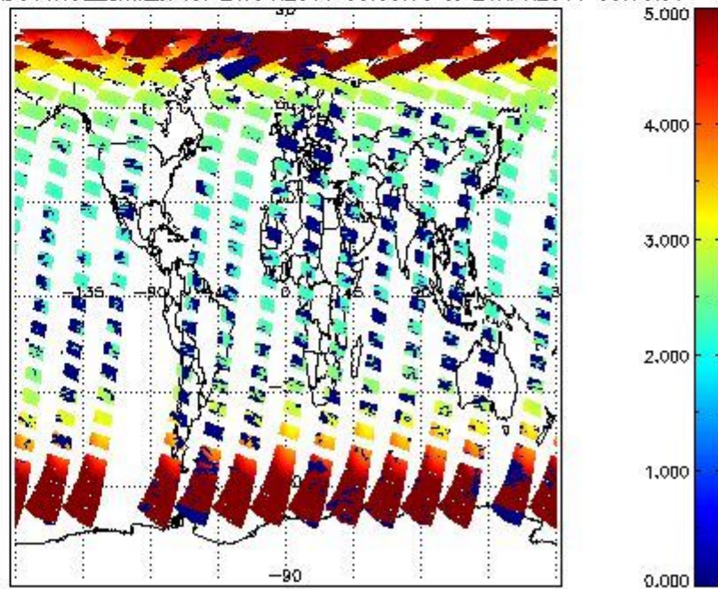
SCIOL2P_NADUV1NO2_amf_cl for 20APR2011 00:00:00 to 21APR2011 00:00:00
