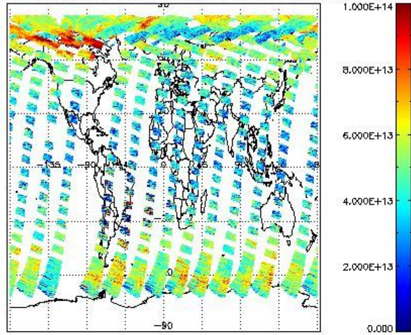
SCIOL2P_NADUV3BRO_vcd for 20APR2011 00:00:00 to 21APR2011 00:00:00
