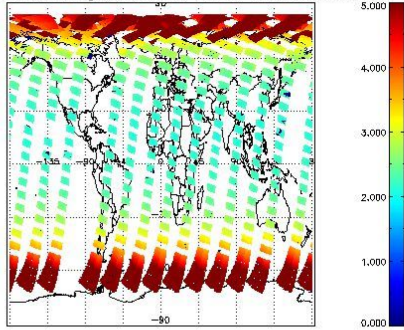
SCIOL2P_NADUV3BRO_amf_gr for 20APR2011 00:00:00 to 21APR2011 00:00:00
