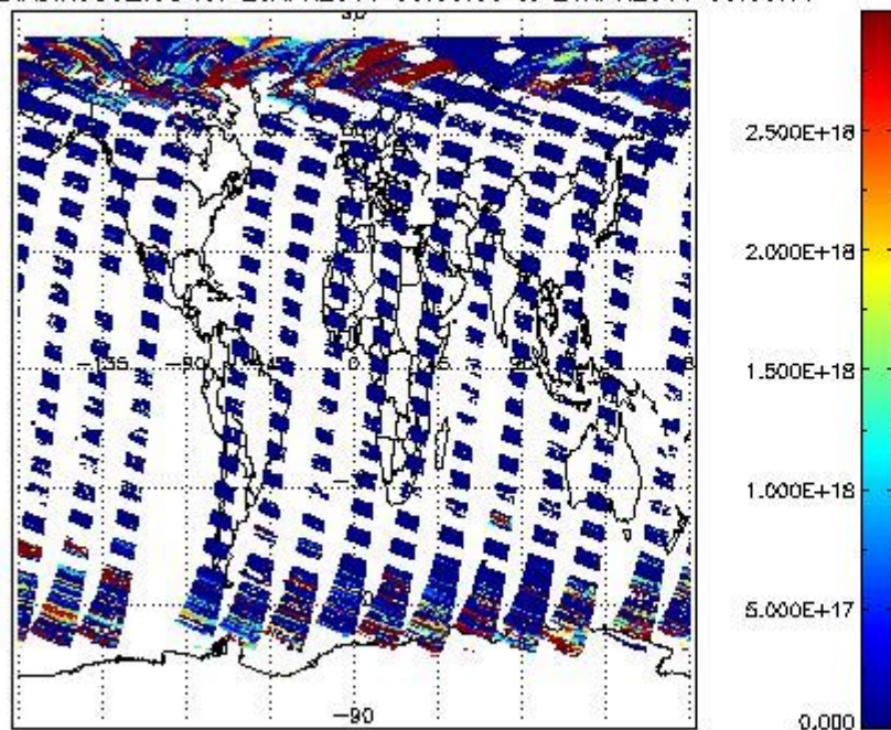
SCIDL2P_NADIR3CO_vcd for 20APR2011 00:00:00 to 21APR2011 00:00:00
