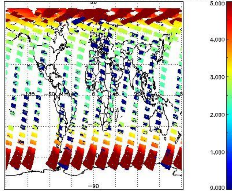
SCIOL2P_NADUV003_amf_cl for 20APR2011 00:00:00 to 21APR2011 00:00:00
