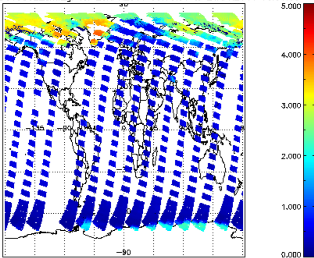
SCIOL2P_NADUV5S02_amf_gr for 20APR2011 00:00:00 to 21APR2011 00:00:00
