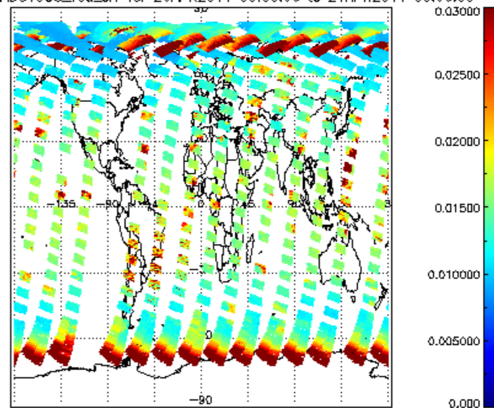
SCIOL2P_NADUV003_vcd_err for 20APR2011 00:00:00 to 21APR2011 00:00:00
