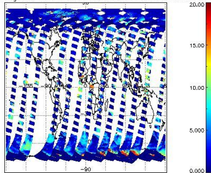
cL_top_height for 20APR2011 00:00:00 to 21APR2011 00:00:00
