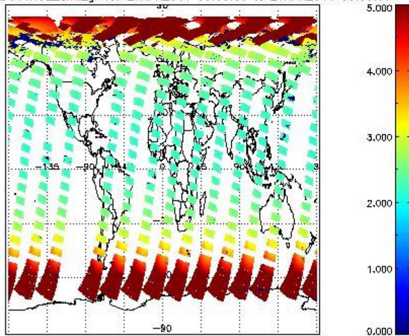
SCIOL2P_NADUV1NO2_amf_gr for 20APR2011 00:00:00 to 21APR2011 00:00:00
