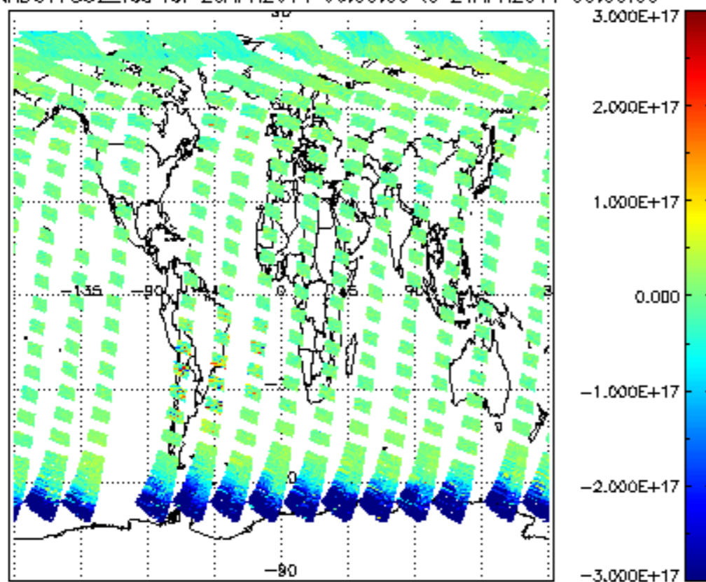
SCIOL2P_NADUV7S02_vcd for 20APR2011 00:00:00 to 21APR2011 00:00:00
