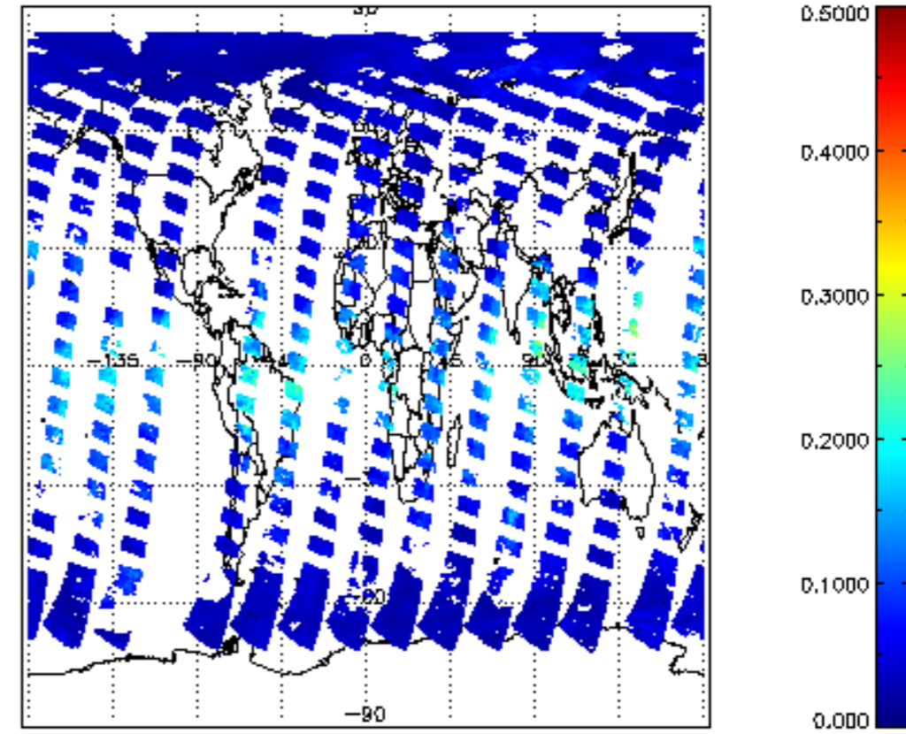
SCIOL2P_NADUV8H2O_vcd_err for 20APR2011 00:00:00 to 21APR2011 00:00:00
