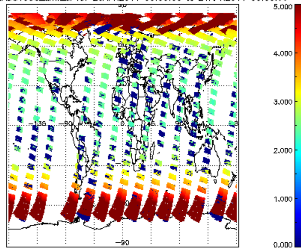
SCIOL2P_NADUV003_amf_cl for 20APR2011 00:00:00 to 21APR2011 00:00:00
