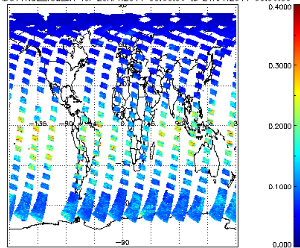
SCIOL2P_NADUV1NO2_vcd_err for 20APR2011 00:00:00 to 21APR2011 00:00:00
