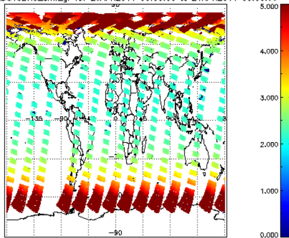
SCIOL2P_NADUV3BRO_amf_gr for 20APR2011 00:00:00 to 21APR2011 00:00:00
