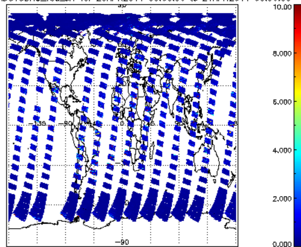
SCIOL2P_NADUV3BRO_vcd_err for 20APR2011 00:00:00 to 21APR2011 00:00:00
