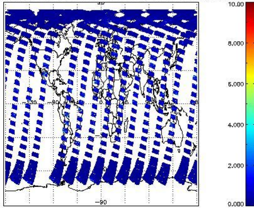
SCIOL2P_NADUV3BRO_vcd_err for 20APR2011 00:00:00 to 21APR2011 00:00:00
