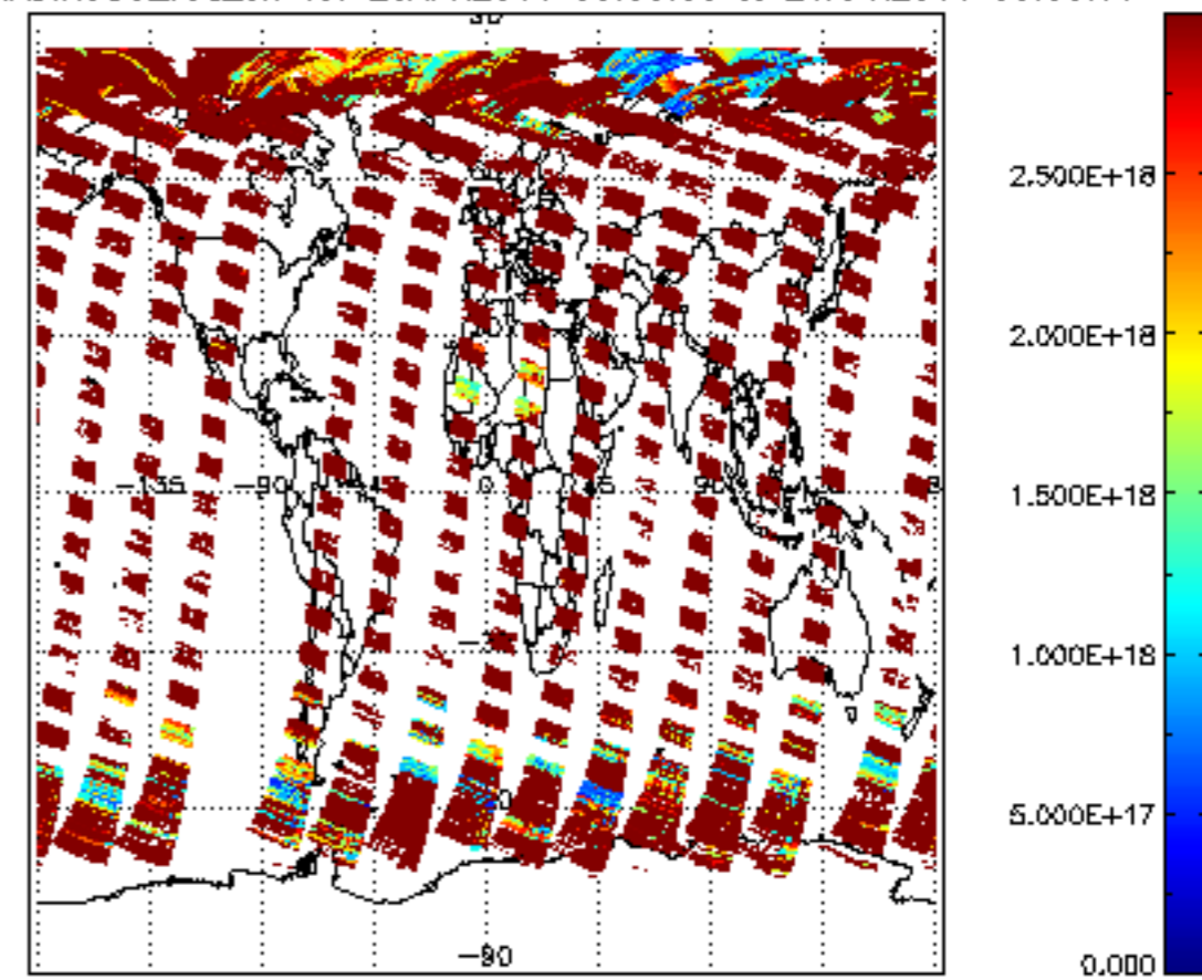
SCIOL2P_NADIR3CO_vcd_err for 20APR2011 00:00:00 to 21APR2011 00:00:00
