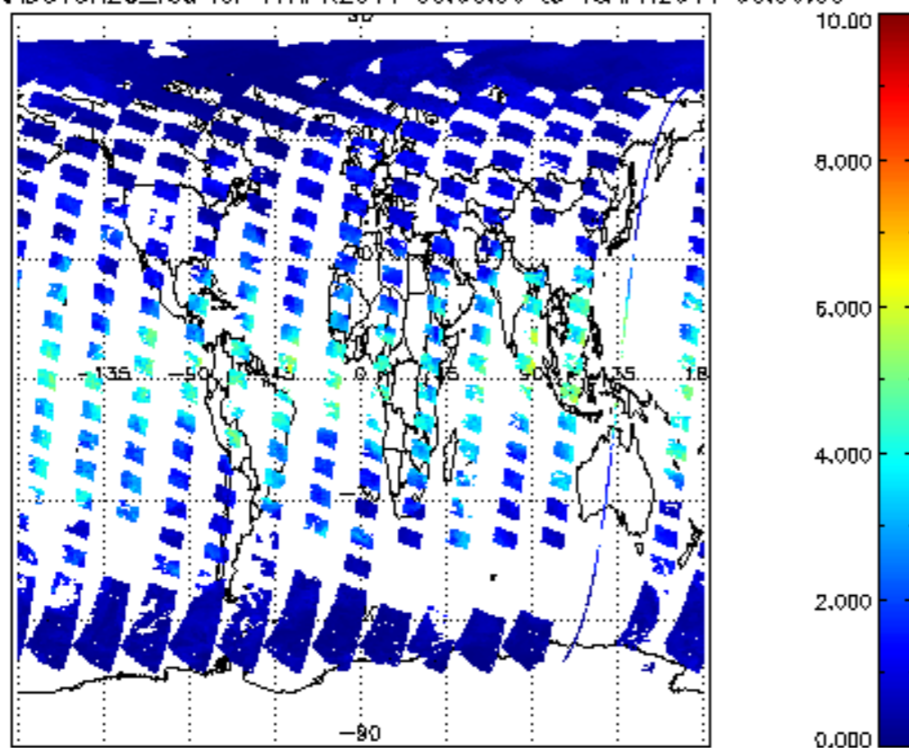
SCIOL2P_NADUV8H2O_vcd for 17APR2011 00:00:00 to 18APR2011 00:00:00
