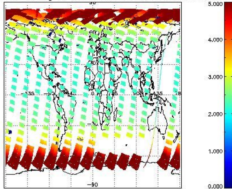
SCIOL2P_NADUV003_amf_gr for 17APR2011 00:00:00 to 18APR2011 00:00:00
