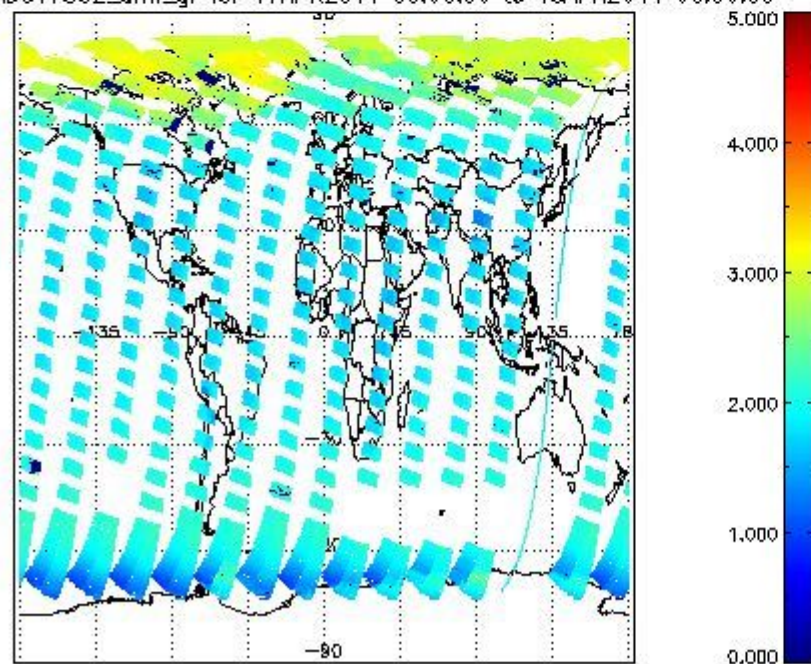
SCIOL2P_NADUV7S02_amf_gr for 17APR2011 00:00:00 to 18APR2011 00:00:00
