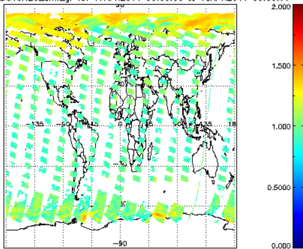
SCIOL2P_NADUV8H2O_amf_gr for 17APR2011 00:00:00 to 18APR2011 00:00:00
