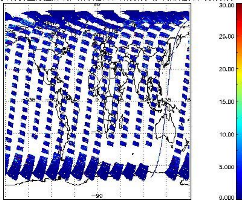
SCIOL2P_NADUV5S02_vcd_err for 17APR2011 00:00:00 to 18APR2011 00:00:00
