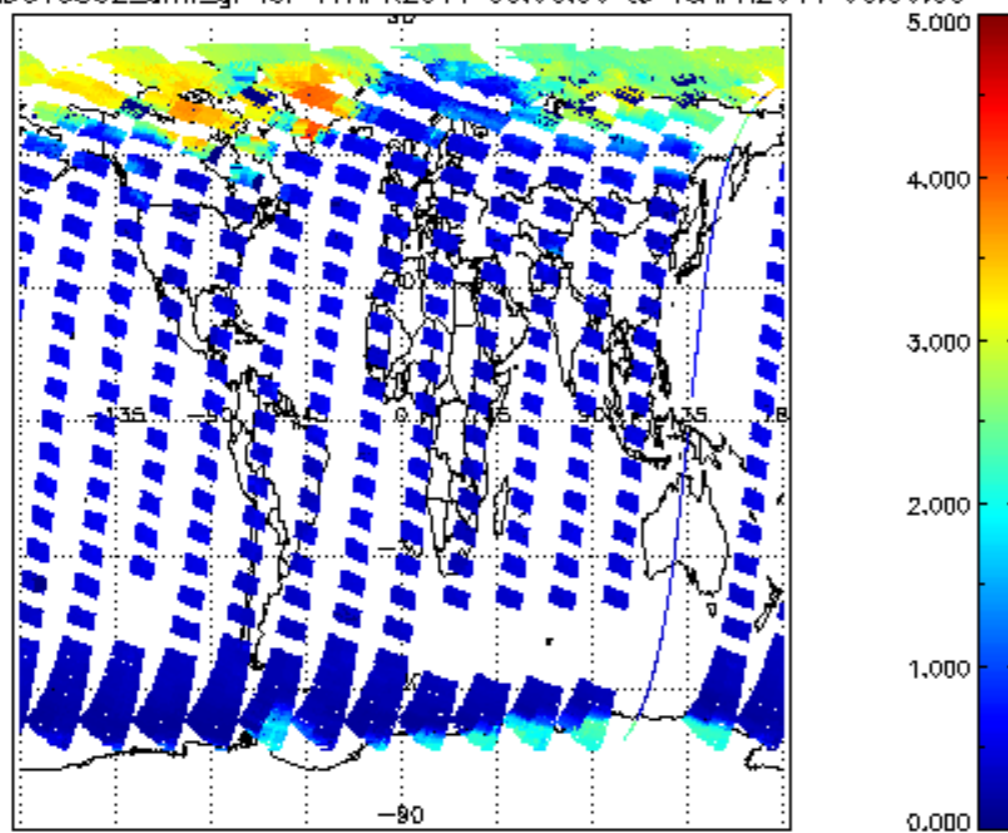
SCIOL2P_NADUV5S02_amf_gr for 17APR2011 00:00:00 to 18APR2011 00:00:00
