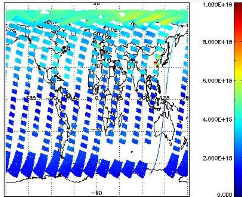
SCIOL2P_NADUV1NO2_vcd for 17APR2011 00:00:00 to 18APR2011 00:00:00
