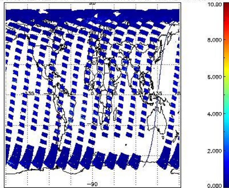
SCIOL2P_NADUV3BRO_vcd_err for 17APR2011 00:00:00 to 18APR2011 00:00:00
