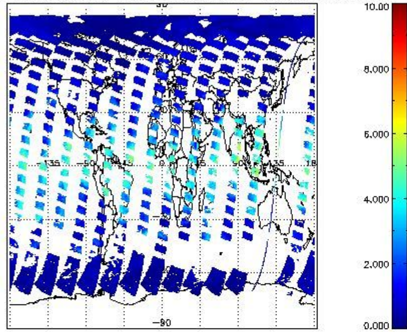
SCIOL2P_NADUV8H2O_vcd for 17APR2011 00:00:00 to 18APR2011 00:00:00
