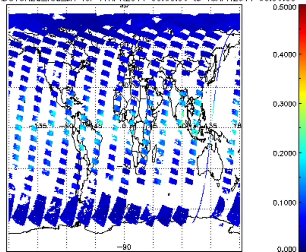
SCIOL2P_NADUV8H2O_vcd_err for 17APR2011 00:00:00 to 18APR2011 00:00:00
