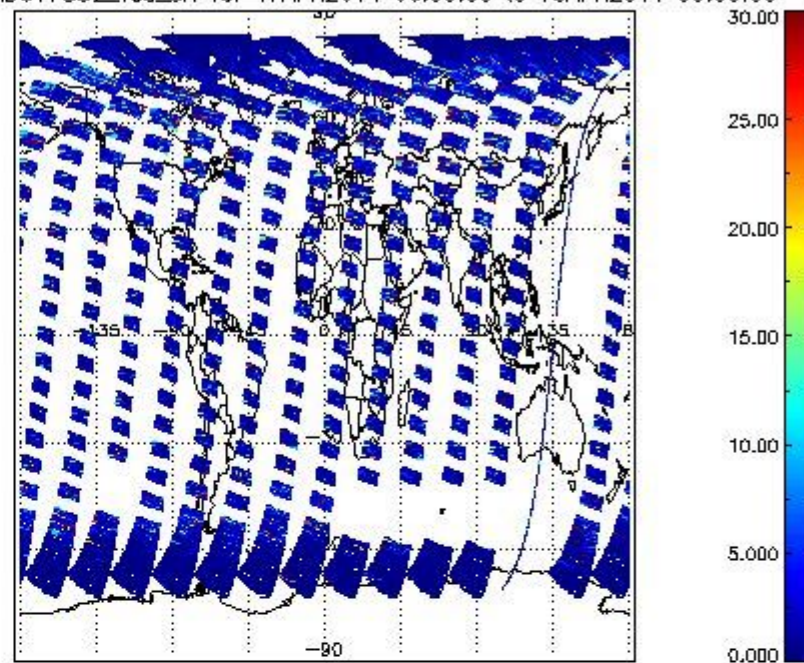
SCIOL2P_NADUV7S02_vcd_err for 17APR2011 00:00:00 to 18APR2011 00:00:00
