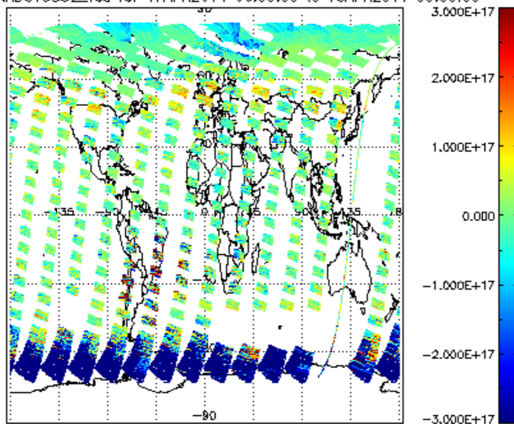
SCIOL2P_NADUV5S02_vcd for 17APR2011 00:00:00 to 18APR2011 00:00:00
