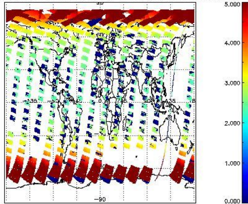
SCIOL2P_NADUV003_amf_cl for 17APR2011 00:00:00 to 18APR2011 00:00:00
