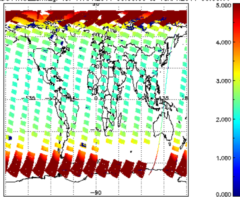
SCIOL2P_NADUV1NO2_amf_gr for 17APR2011 00:00:00 to 18APR2011 00:00:00
