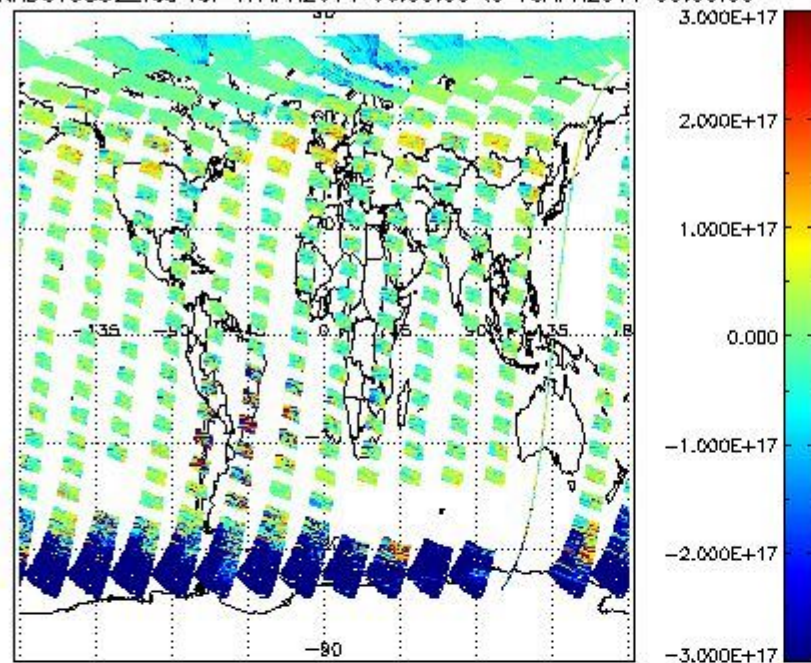
SCIOL2P_NADUV5S02_vcd for 17APR2011 00:00:00 to 18APR2011 00:00:00
