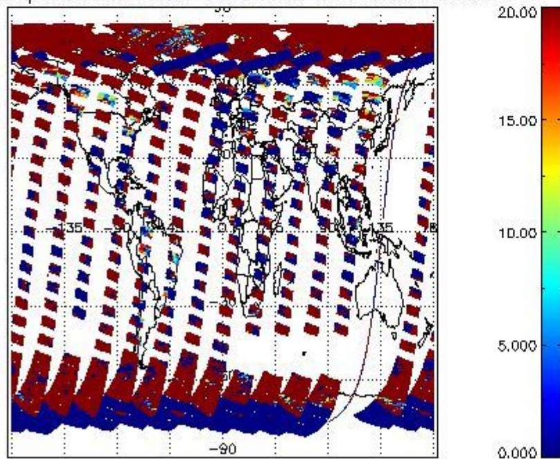
cL_opt_depth for 17APR2011 00:00:00 to 18APR2011 00:00:00
