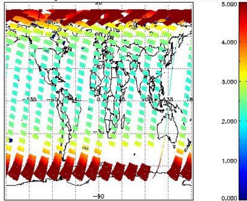
SCIOL2P_NADUV3BRO_amf_gr for 17APR2011 00:00:00 to 18APR2011 00:00:00
