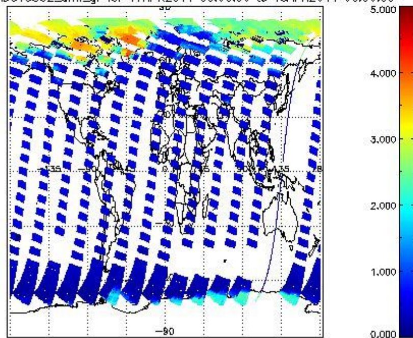
SCIOL2P_NADUV5S02_amf_gr for 17APR2011 00:00:00 to 18APR2011 00:00:00
