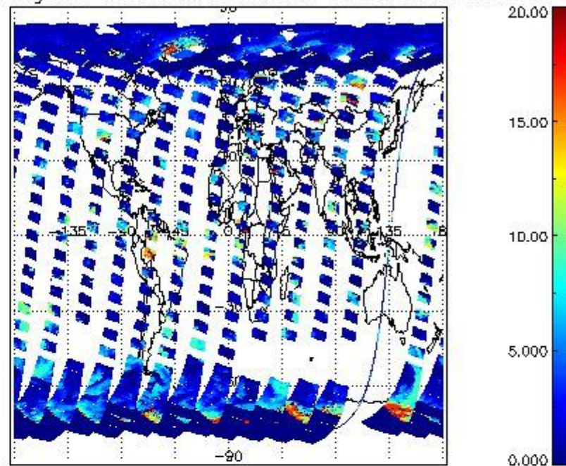
cL_top_height for 17APR2011 00:00:00 to 18APR2011 00:00:00
