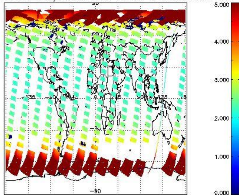
SCIOL2P_NADUV1NO2_amf_gr for 17APR2011 00:00:00 to 18APR2011 00:00:00
