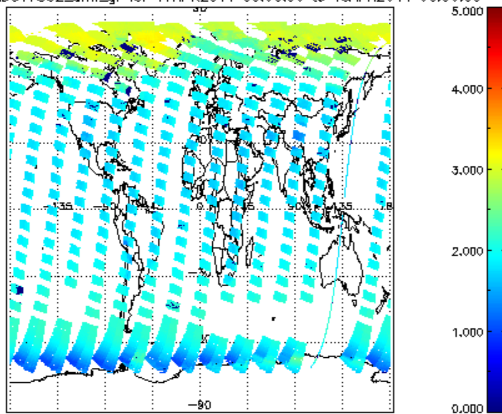
SCIOL2P_NADUV7S02_amf_gr for 17APR2011 00:00:00 to 18APR2011 00:00:00
