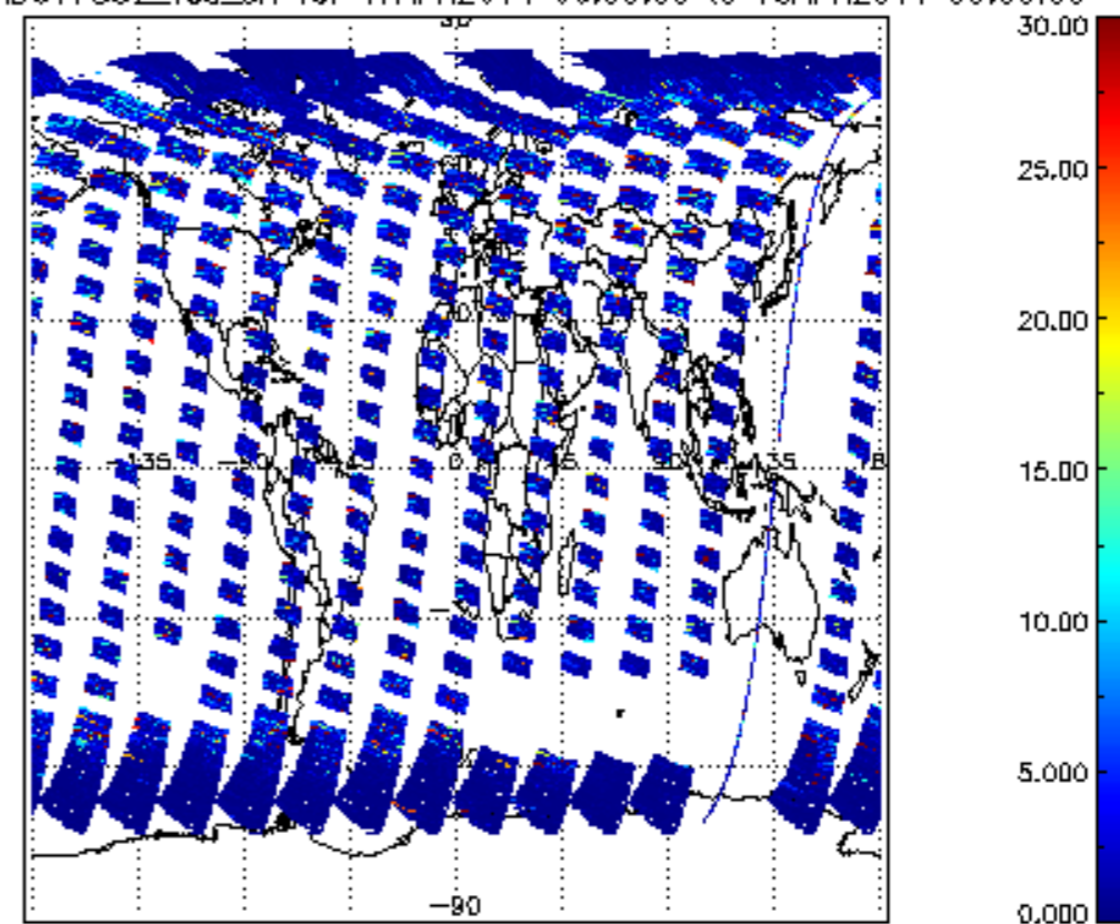
SCIOL2P_NADUV7S02_vcd_err for 17APR2011 00:00:00 to 18APR2011 00:00:00
