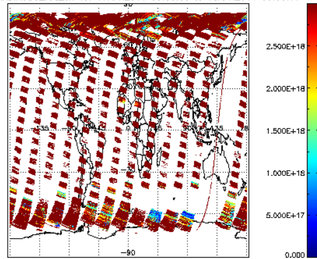
SCIOL2P_NADIR3CO_vcd_err for 17APR2011 00:00:00 to 18APR2011 00:00:00
