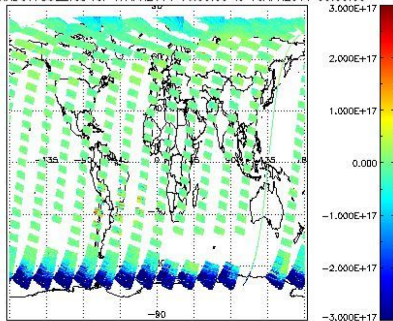
SCIOL2P_NADUV7S02_vcd for 17APR2011 00:00:00 to 18APR2011 00:00:00
