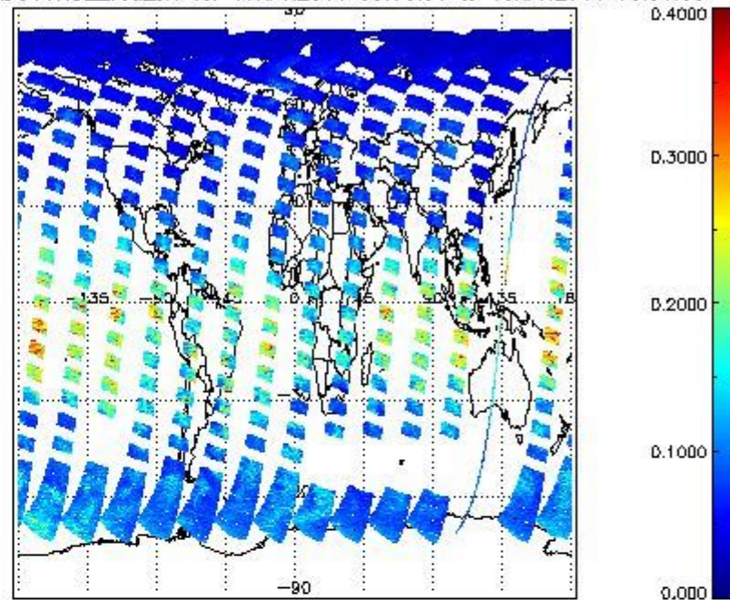
SCIOL2P_NADUV1NO2_vcd_err for 17APR2011 00:00:00 to 18APR2011 00:00:00
