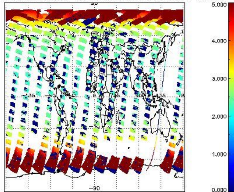
SCIOL2P_NADUV1NO2_amf_cl for 17APR2011 00:00:00 to 18APR2011 00:00:00
