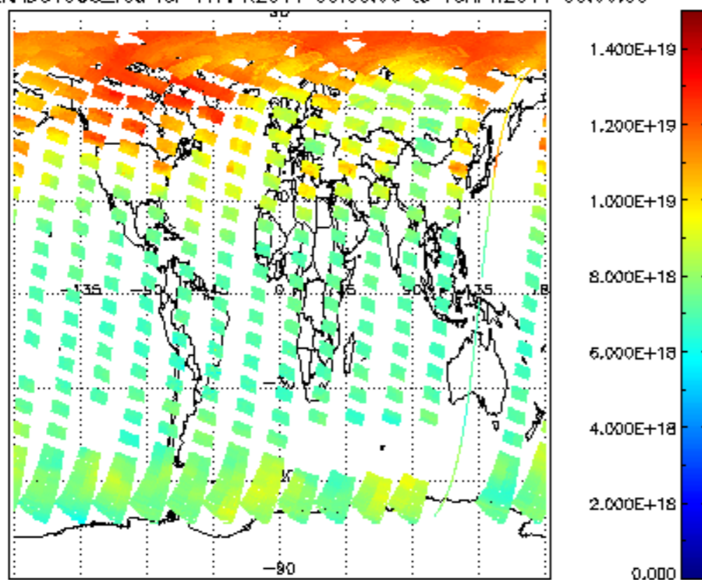
SCIOL2P_NADUV003_vcd for 17APR2011 00:00:00 to 18APR2011 00:00:00
