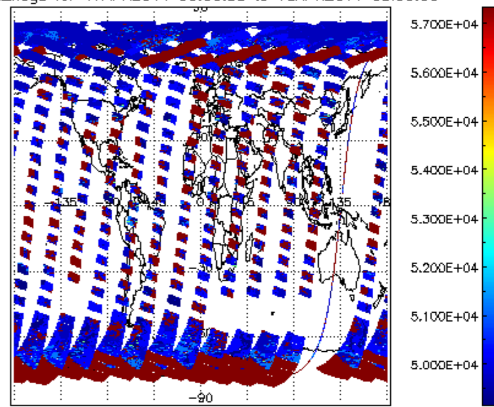
cloud_flags for 17APR2011 00:00:00 to 18APR2011 00:00:00
