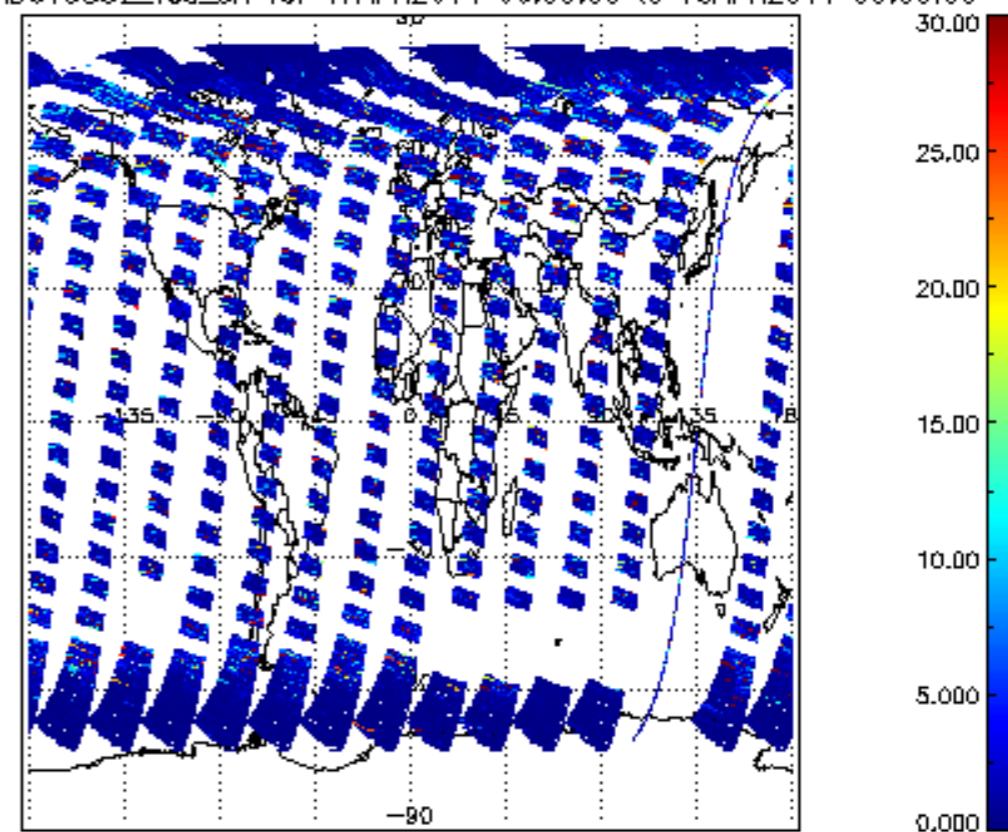
SCIOL2P_NADUV5S02_vcd_err for 17APR2011 00:00:00 to 18APR2011 00:00:00
