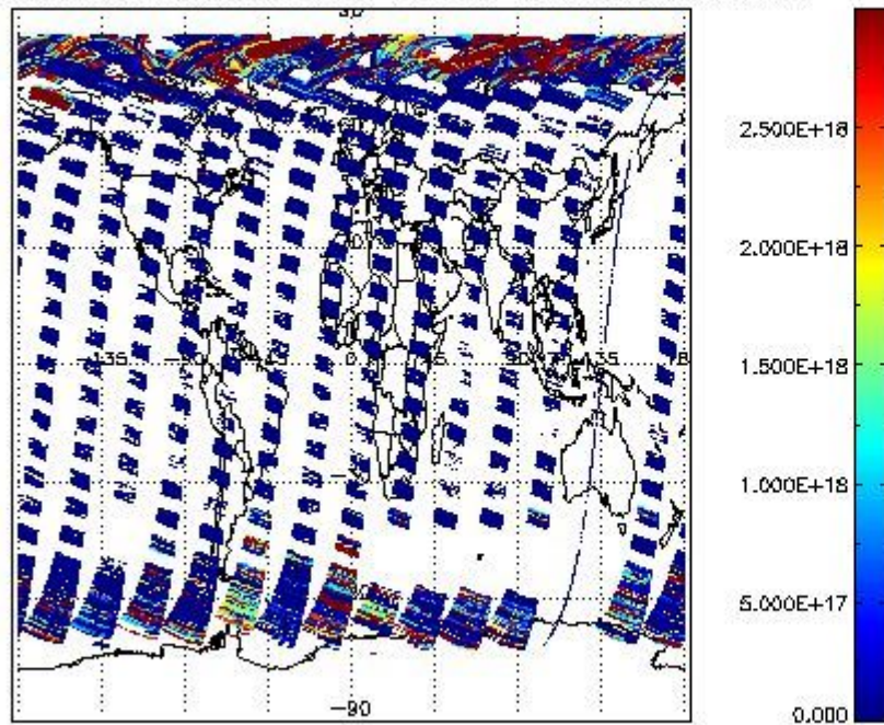
SCIDL2P_NADIR3CO_vcd for 17APR2011 00:00:00 to 18APR2011 00:00:00
