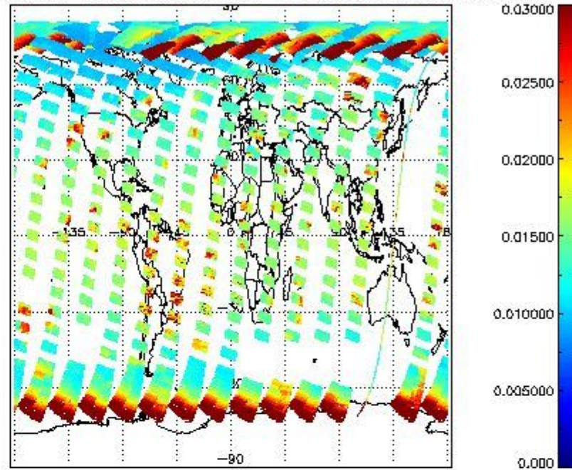
SCIOL2P_NADUV003_vcd_err for 17APR2011 00:00:00 to 18APR2011 00:00:00
