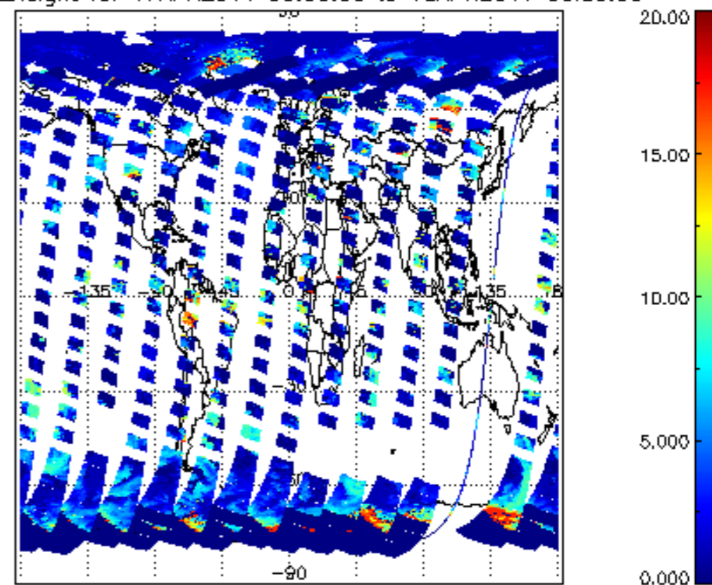
cL_top_height for 17APR2011 00:00:00 to 18APR2011 00:00:00
