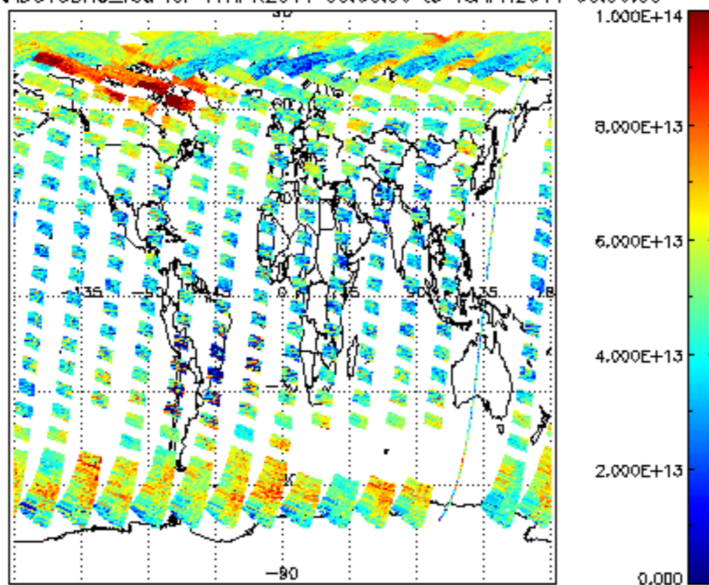
SCIOL2P_NADUV3BRO_vcd for 17APR2011 00:00:00 to 18APR2011 00:00:00
