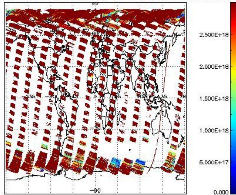
SCIDL2P_NADIR3CO_vcd_err for 17APR2011 00:00:00 to 18APR2011 00:00:00
