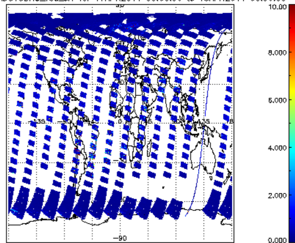
SCIOL2P_NADUV3BRO_vcd_err for 17APR2011 00:00:00 to 18APR2011 00:00:00
