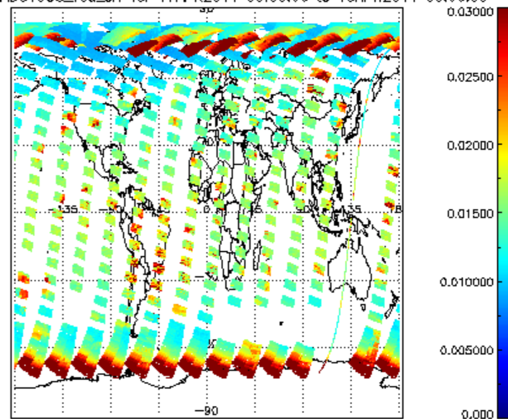
SCIOL2P_NADUV003_vcd_err for 17APR2011 00:00:00 to 18APR2011 00:00:00
