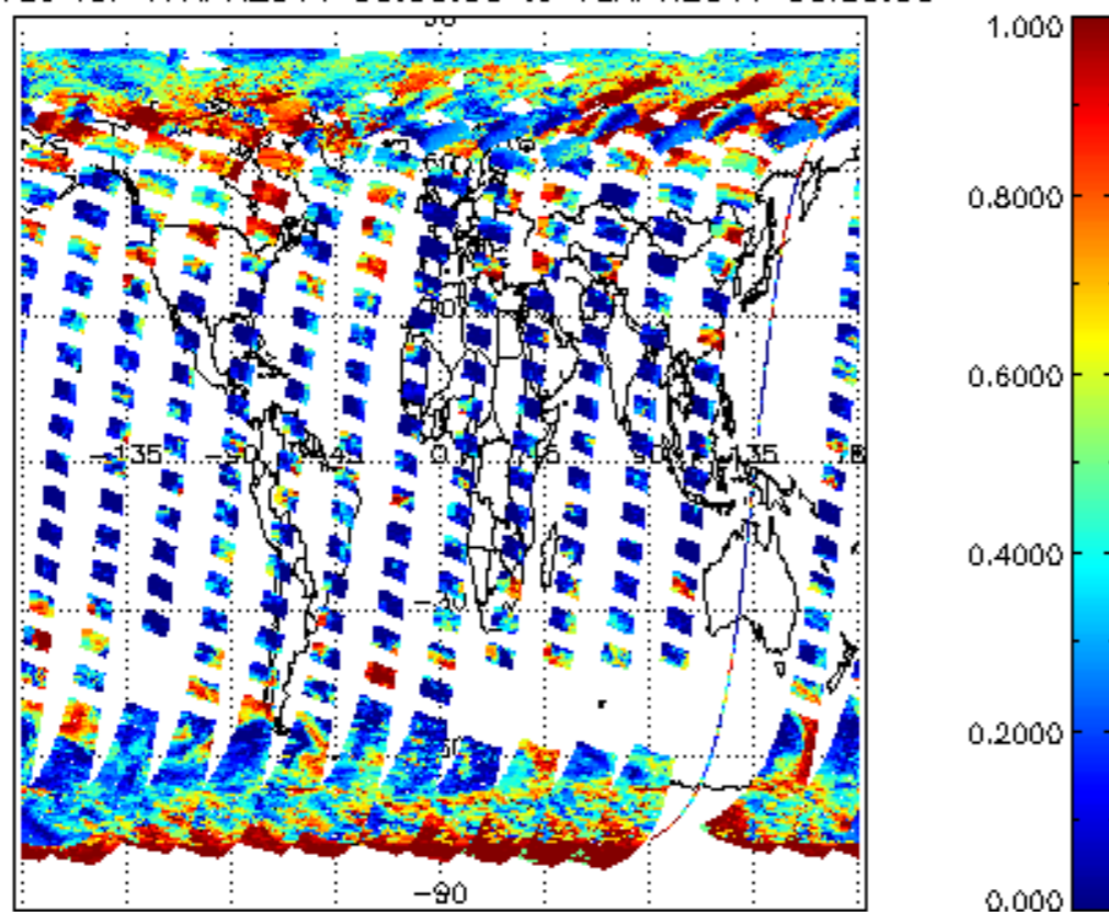
cL_frac for 17APR2011 00:00:00 to 18APR2011 00:00:00
