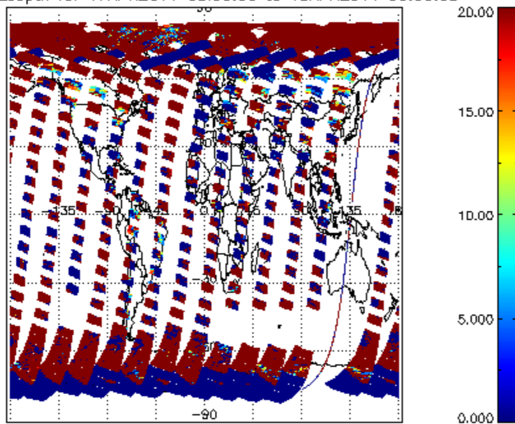
cL_opt_depth for 17APR2011 00:00:00 to 18APR2011 00:00:00
