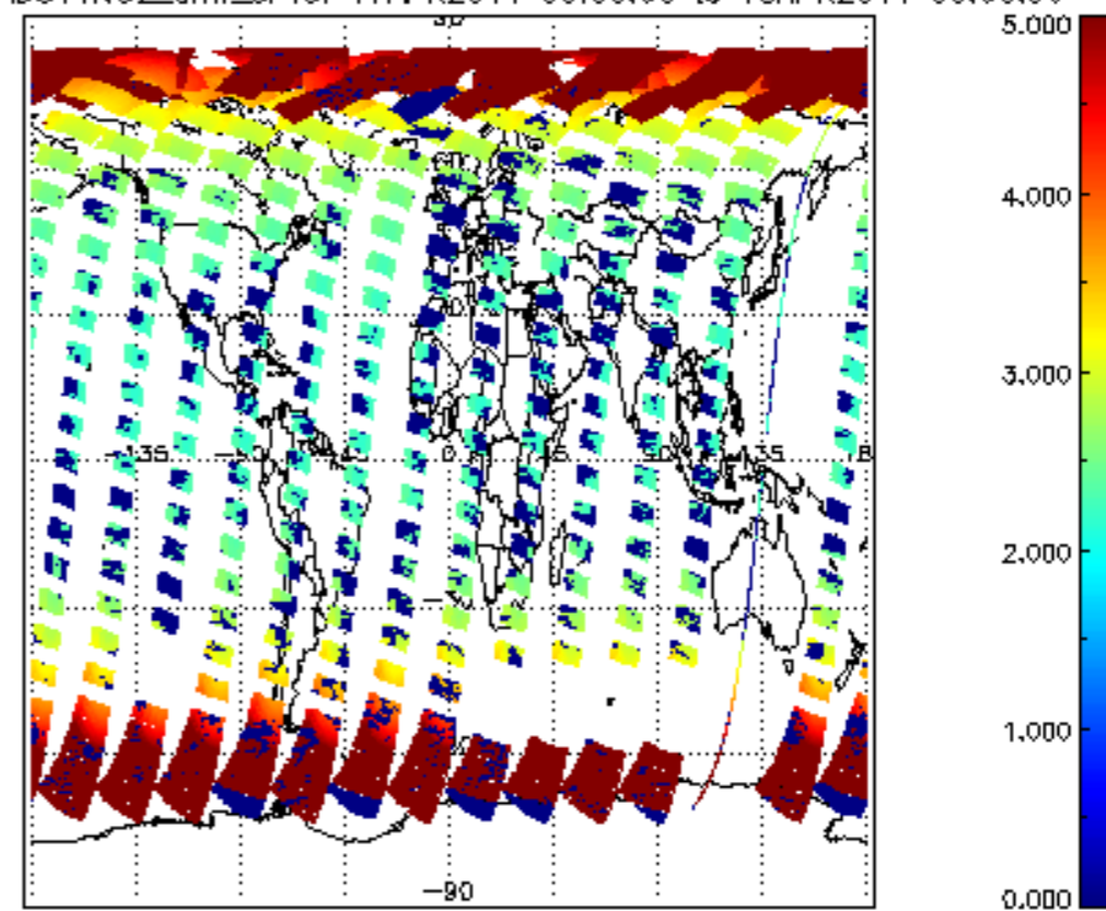
SCIOL2P_NADUV1NO2_amf_sl for 17APR2011 00:00:00 to 18APR2011 00:00:00
