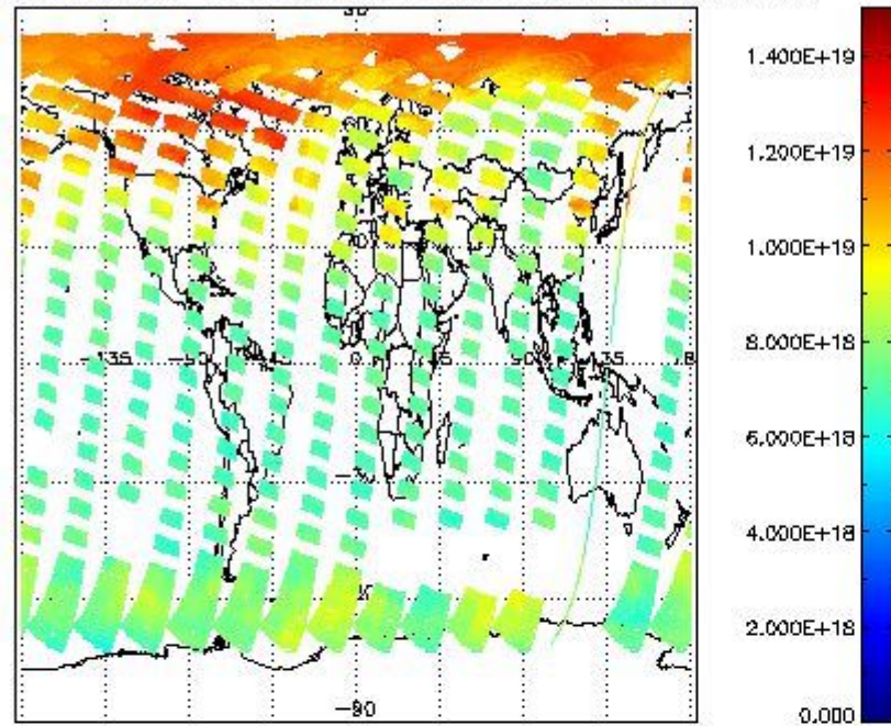
SCIOL2P_NADUV003_vcd for 17APR2011 00:00:00 to 18APR2011 00:00:00
