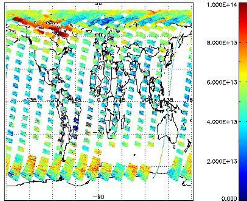
SCIOL2P_NADUV3BRO_vcd for 17APR2011 00:00:00 to 18APR2011 00:00:00
