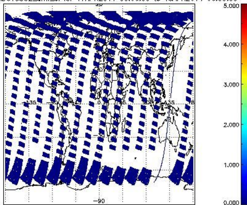
SCIOL2P_NADUV5S02_amf_cl for 17APR2011 00:00:00 to 18APR2011 00:00:00
