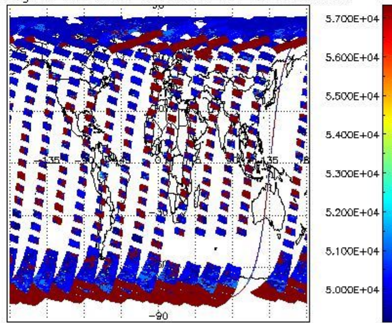
cloud_flags for 17APR2011 00:00:00 to 18APR2011 00:00:00
