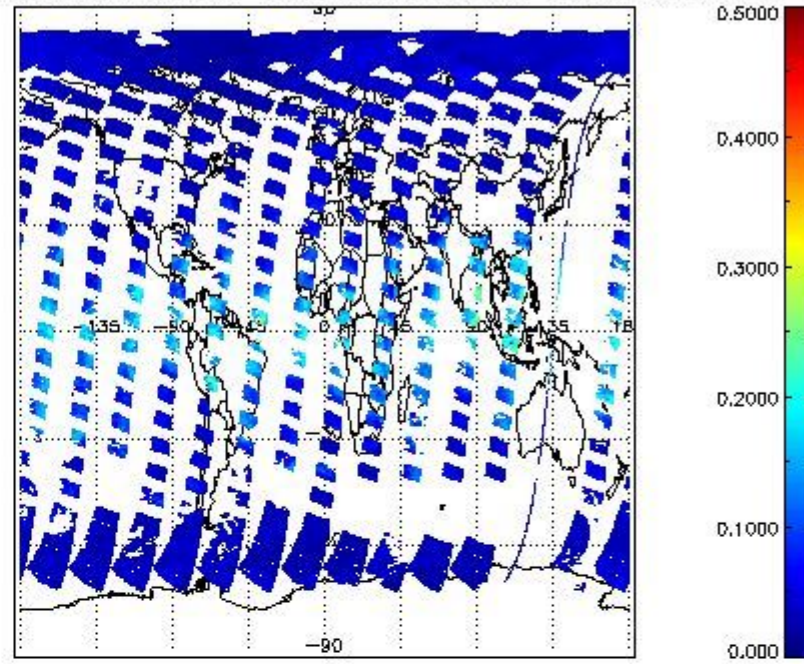
SCIOL2P_NADUV8H2O_vcd_err for 17APR2011 00:00:00 to 18APR2011 00:00:00
