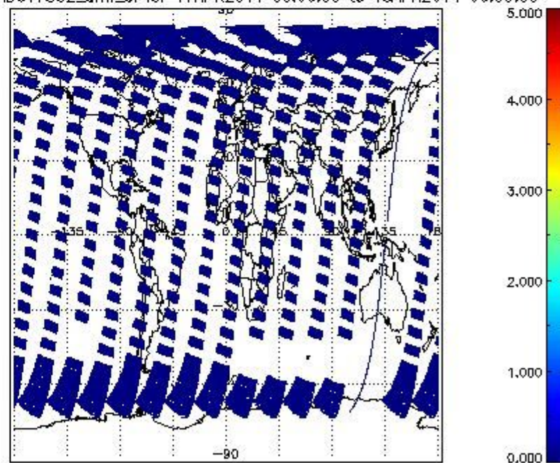
SCIOL2P_NADUV7S02_amf_cl for 17APR2011 00:00:00 to 18APR2011 00:00:00
