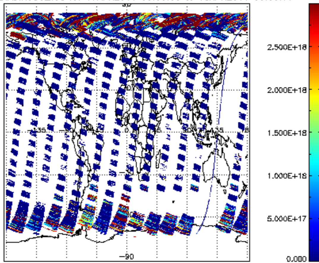
SCIOL2P_NADIR3CO_vcd for 17APR2011 00:00:00 to 18APR2011 00:00:00
