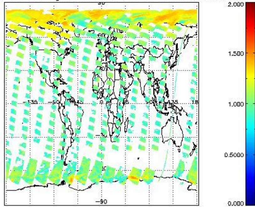
SCIOL2P_NADUV8H2O_arnf_gr for 17APR2011 00:00:00 to 18APR2011 00:00:00
