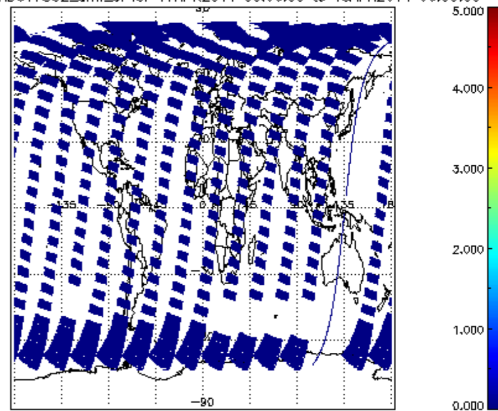
SCIOL2P_NADUV7S02_amf_cl for 17APR2011 00:00:00 to 18APR2011 00:00:00
