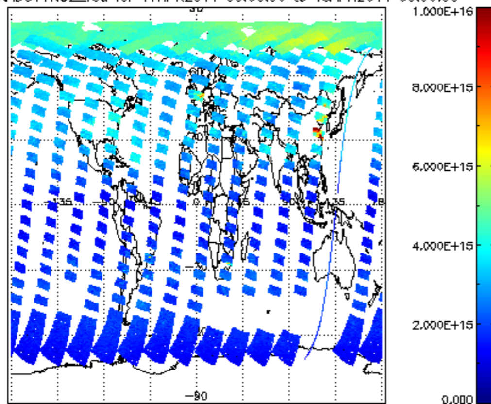
SCIOL2P_NADUV1NO2_vcd for 17APR2011 00:00:00 to 18APR2011 00:00:00
