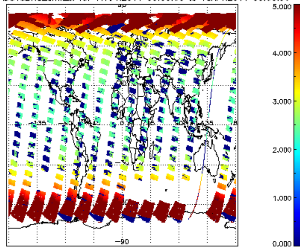
SCIOL2P_NADUV3BRO_amf_cl for 17APR2011 00:00:00 to 18APR2011 00:00:00
