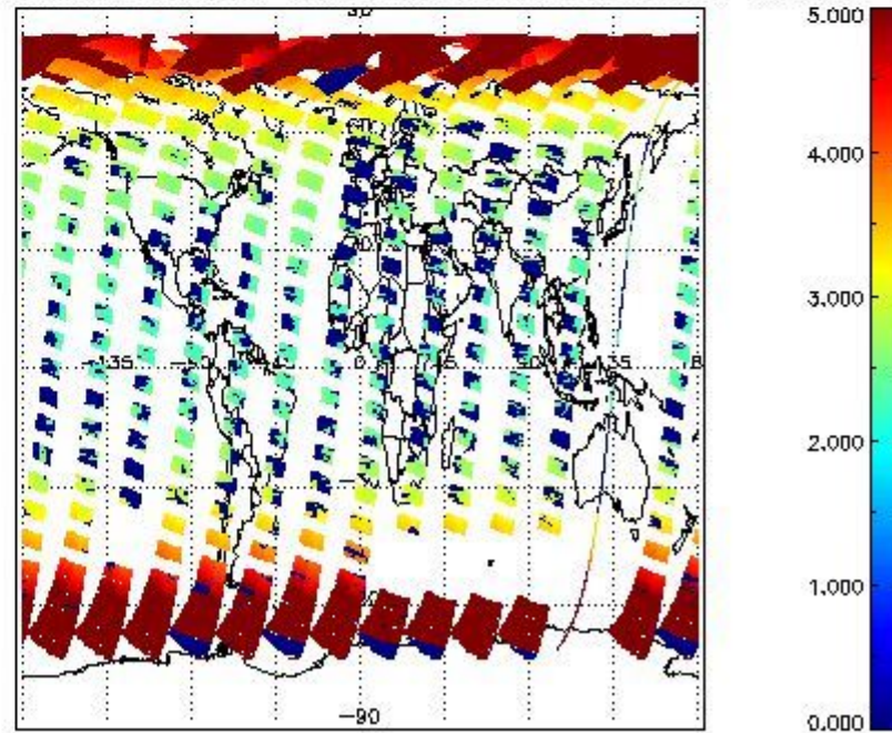
SCIOL2P_NADUV3BRO_amf_cl for 17APR2011 00:00:00 to 18APR2011 00:00:00
