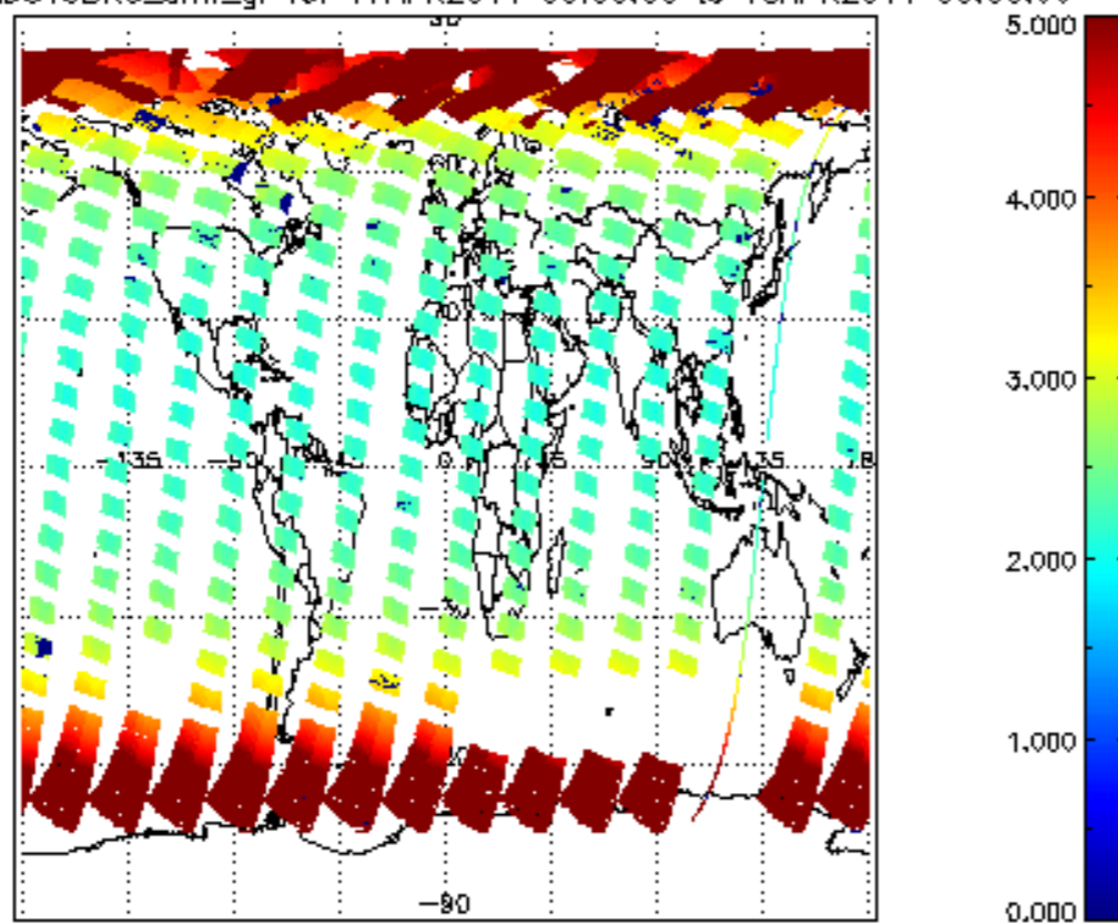
SCIOL2P_NADUV3BRO_amf_gr for 17APR2011 00:00:00 to 18APR2011 00:00:00
