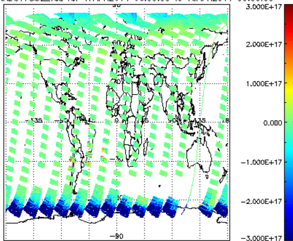
SCIOL2P_NADUV7S02_vcd for 17APR2011 00:00:00 to 18APR2011 00:00:00
