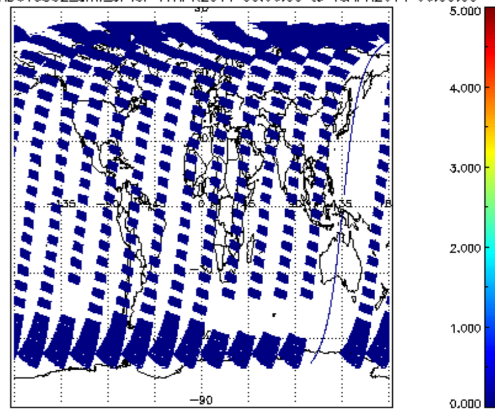
SCIOL2P_NADUV5S02_amf_cl for 17APR2011 00:00:00 to 18APR2011 00:00:00
