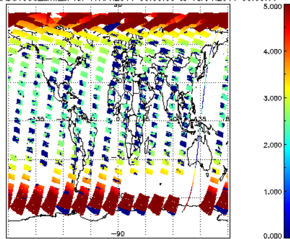
SCIOL2P_NADUV003_amf_cl for 17APR2011 00:00:00 to 18APR2011 00:00:00
