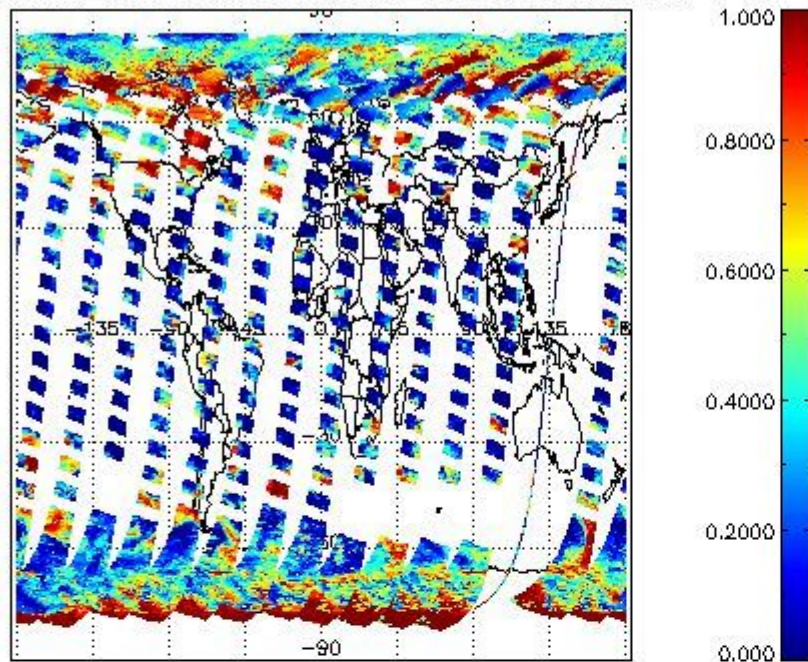
cL_frac for 17APR2011 00:00:00 to 18APR2011 00:00:00
