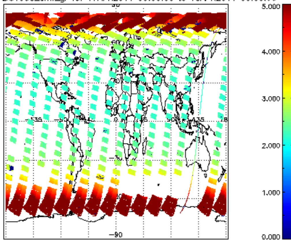
SCIOL2P_NADUV003_amf_gr for 17APR2011 00:00:00 to 18APR2011 00:00:00
