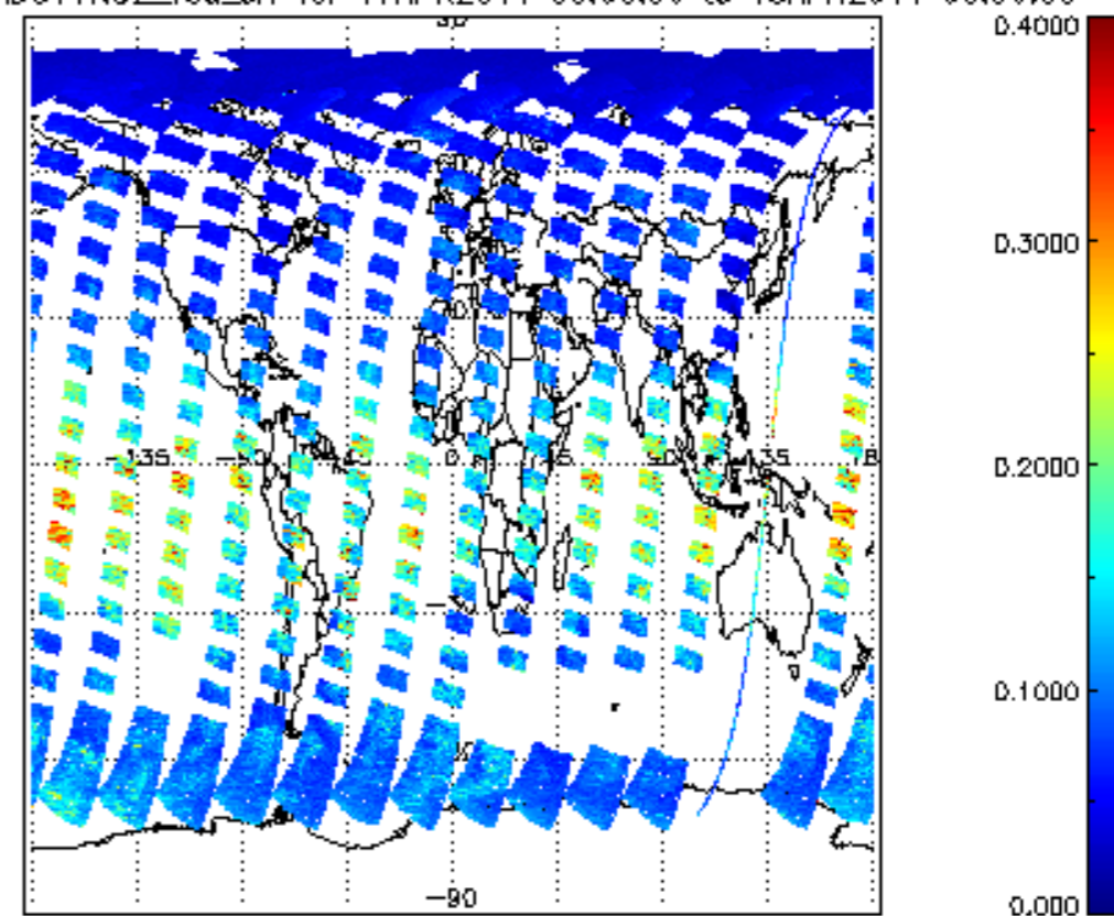
SCIOL2P_NADUV1NO2_vcd_err for 17APR2011 00:00:00 to 18APR2011 00:00:00
