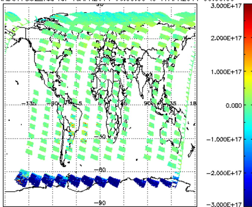
SCIOL2P_NADUV7S02_vcd for 16APR2011 00:00:00 to 17APR2011 00:00:00
