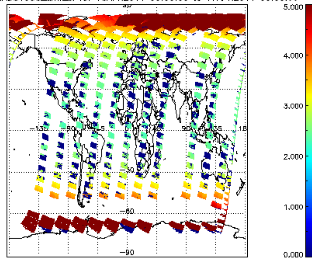
SCIOL2P_NADUV003_amf_cl for 16APR2011 00:00:00 to 17APR2011 00:00:00
