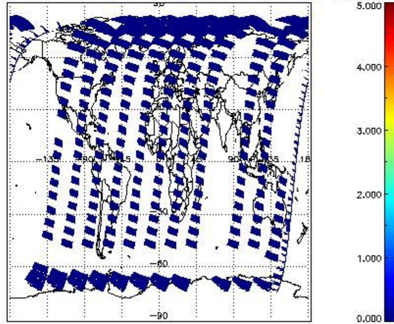
SCIOL2P_NADUV7S02_amf_cl for 16APR2011 00:00:00 to 17APR2011 00:00:00
