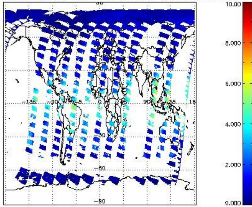
SCIOL2P_NADUV8H2O_vcd for 16APR2011 00:00:00 to 17APR2011 00:00:00
