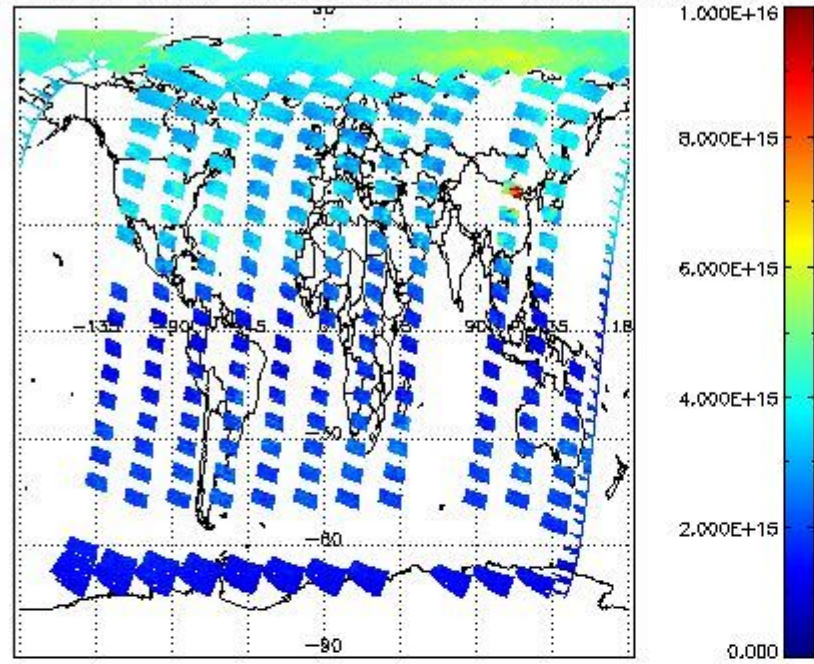
SCIOL2P_NADUV1NO2_vcd for 16APR2011 00:00:00 to 17APR2011 00:00:00
