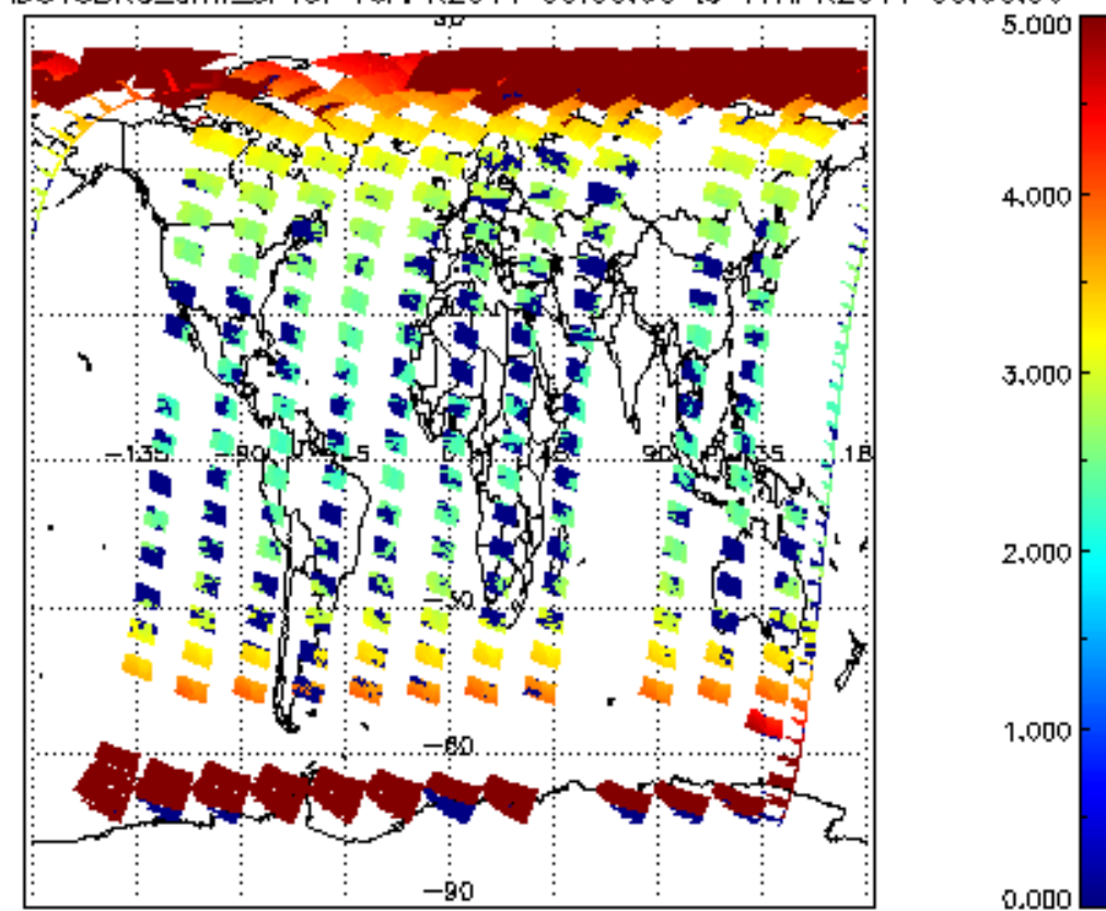
SCIOL2P_NADUV3BRO_amf_cl for 16APR2011 00:00:00 to 17APR2011 00:00:00
