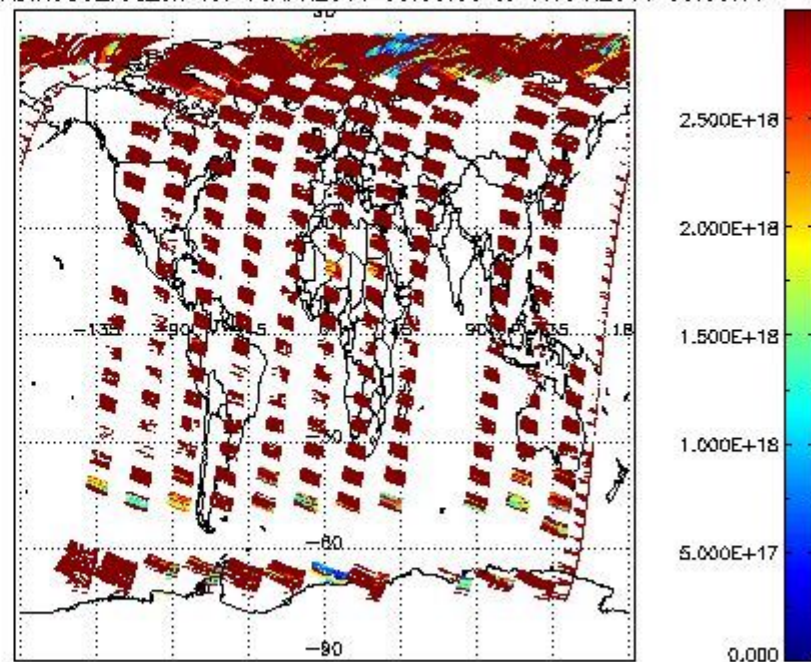
SCIDL2P_NADIR3CO_vcd_err for 16APR2011 00:00:00 to 17APR2011 00:00:00
