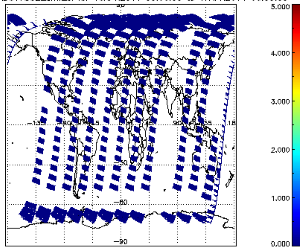
SCIOL2P_NADUV7S02_amf_cl for 16APR2011 00:00:00 to 17APR2011 00:00:00
