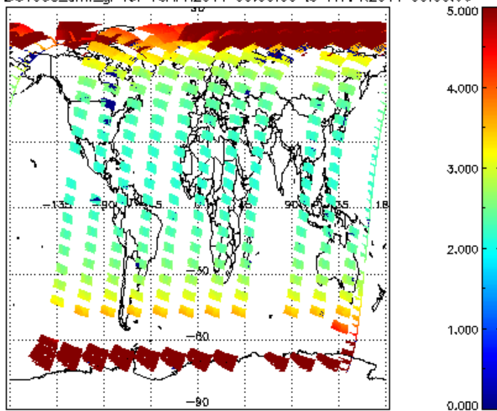
SCIOL2P_NADUV003_amf_gr for 16APR2011 00:00:00 to 17APR2011 00:00:00
