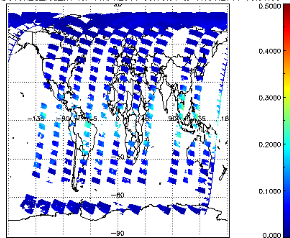
SCIOL2P_NADUV8H2O_vcd_err for 16APR2011 00:00:00 to 17APR2011 00:00:00
