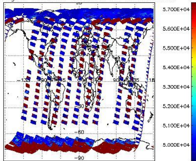
cloud_flags for 16APR2011 00:00:00 to 17APR2011 00:00:00
