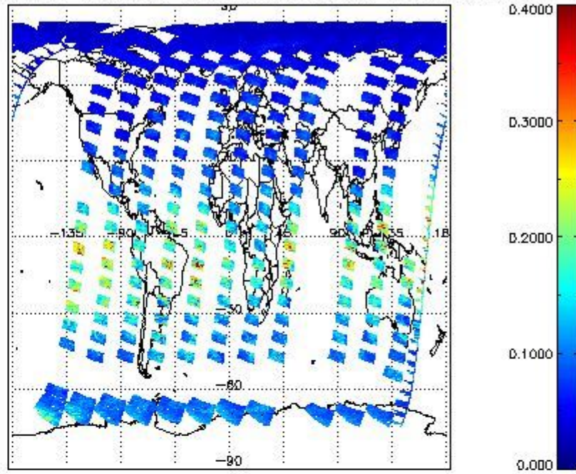
SCIOL2P_NADUV1NO2_vcd_err for 16APR2011 00:00:00 to 17APR2011 00:00:00
