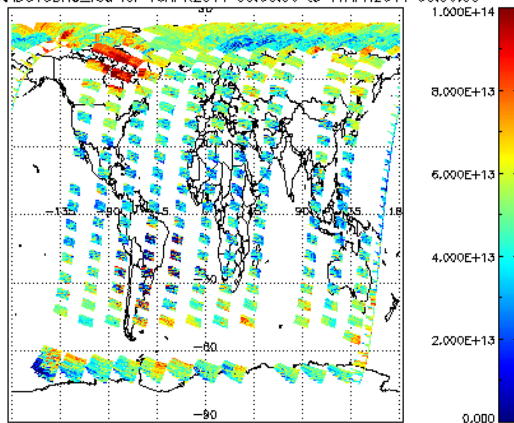
SCIOL2P_NADUV3BRO_vcd for 16APR2011 00:00:00 to 17APR2011 00:00:00
