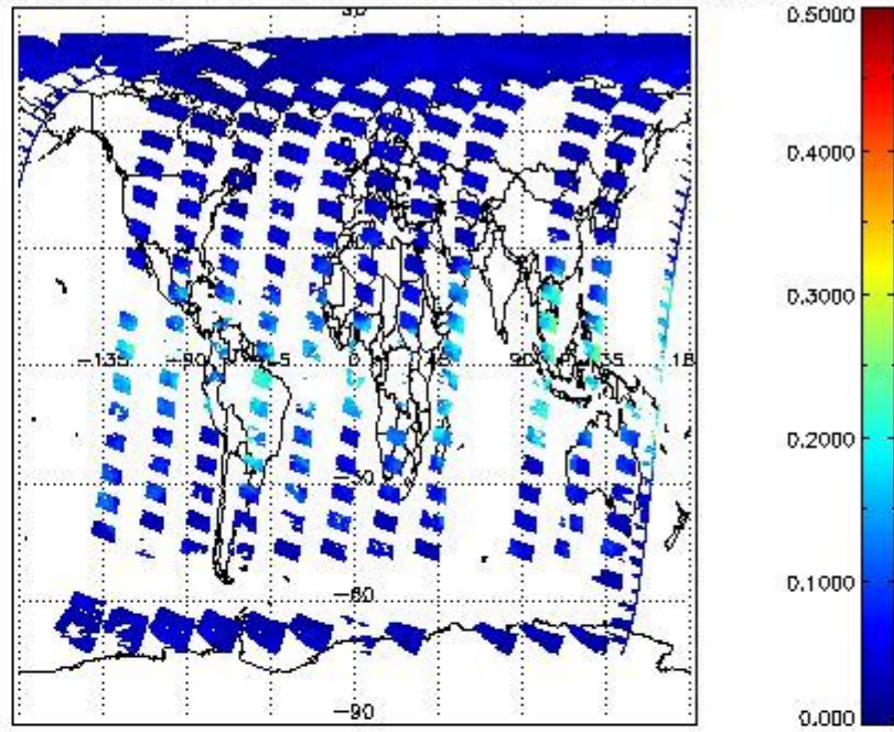
SCIOL2P_NADUV8H2O_vcd_err for 16APR2011 00:00:00 to 17APR2011 00:00:00
