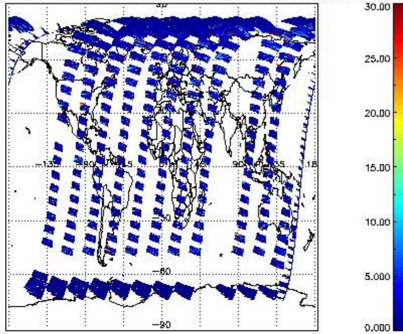
SCIOL2P_NADUV5S02_vcd_err for 16APR2011 00:00:00 to 17APR2011 00:00:00
