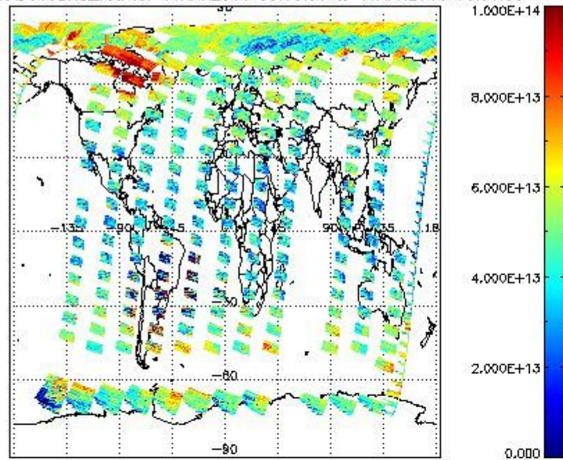
SCIOL2P_NADUV3BRO_vcd for 16APR2011 00:00:00 to 17APR2011 00:00:00
