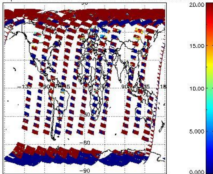
cL_opt_depth for 16APR2011 00:00:00 to 17APR2011 00:00:00
