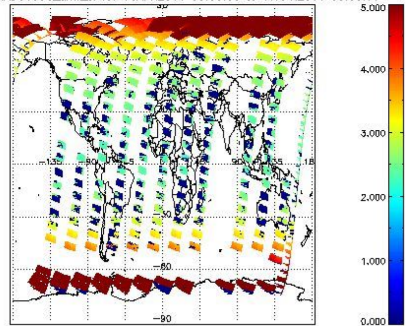
SCIOL2P_NADUV003_amf_cl for 16APR2011 00:00:00 to 17APR2011 00:00:00
