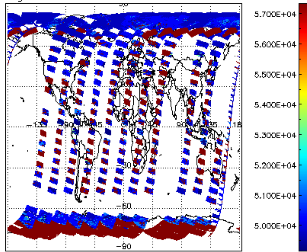
cloud_flags for 16APR2011 00:00:00 to 17APR2011 00:00:00
