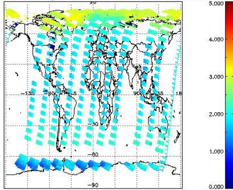
SCIOL2P_NADUV7S02_amf_gr for 16APR2011 00:00:00 to 17APR2011 00:00:00
