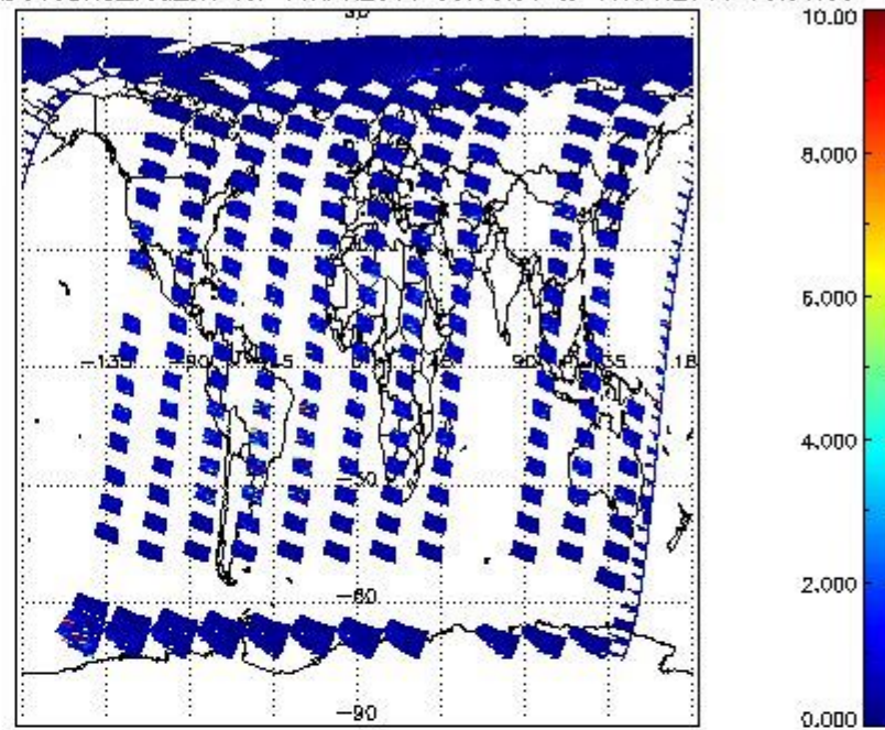
SCIOL2P_NADUV3BRO_vcd_err for 16APR2011 00:00:00 to 17APR2011 00:00:00
