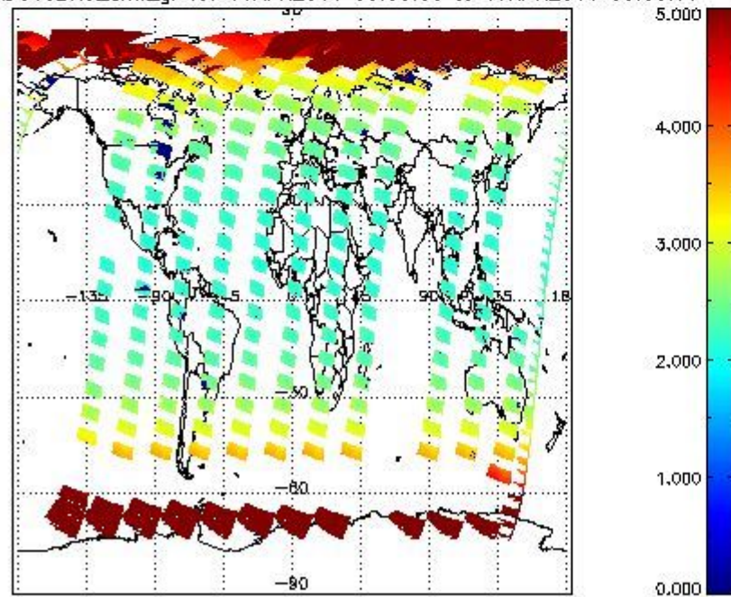
SCIOL2P_NADUV3BRO_amf_gr for 16APR2011 00:00:00 to 17APR2011 00:00:00
