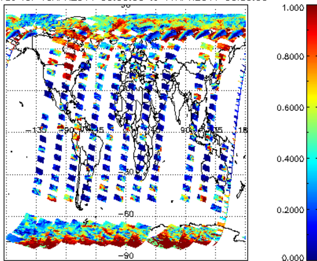
cl_frac for 16APR2011 00:00:00 to 17APR2011 00:00:00
