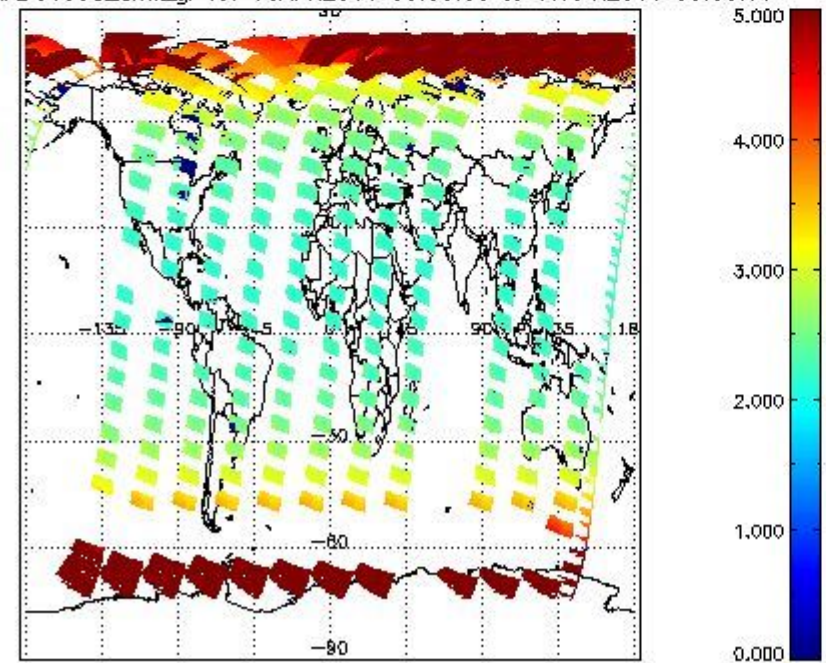
SCIOL2P_NADUV003_amf_gr for 16APR2011 00:00:00 to 17APR2011 00:00:00
