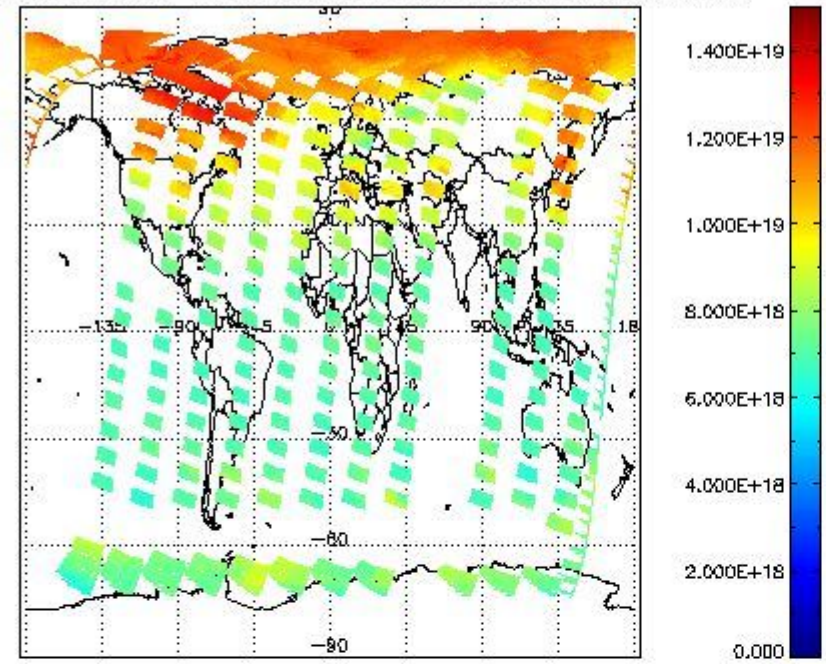
SCIOL2P_NADUV003_vcd for 16APR2011 00:00:00 to 17APR2011 00:00:00
