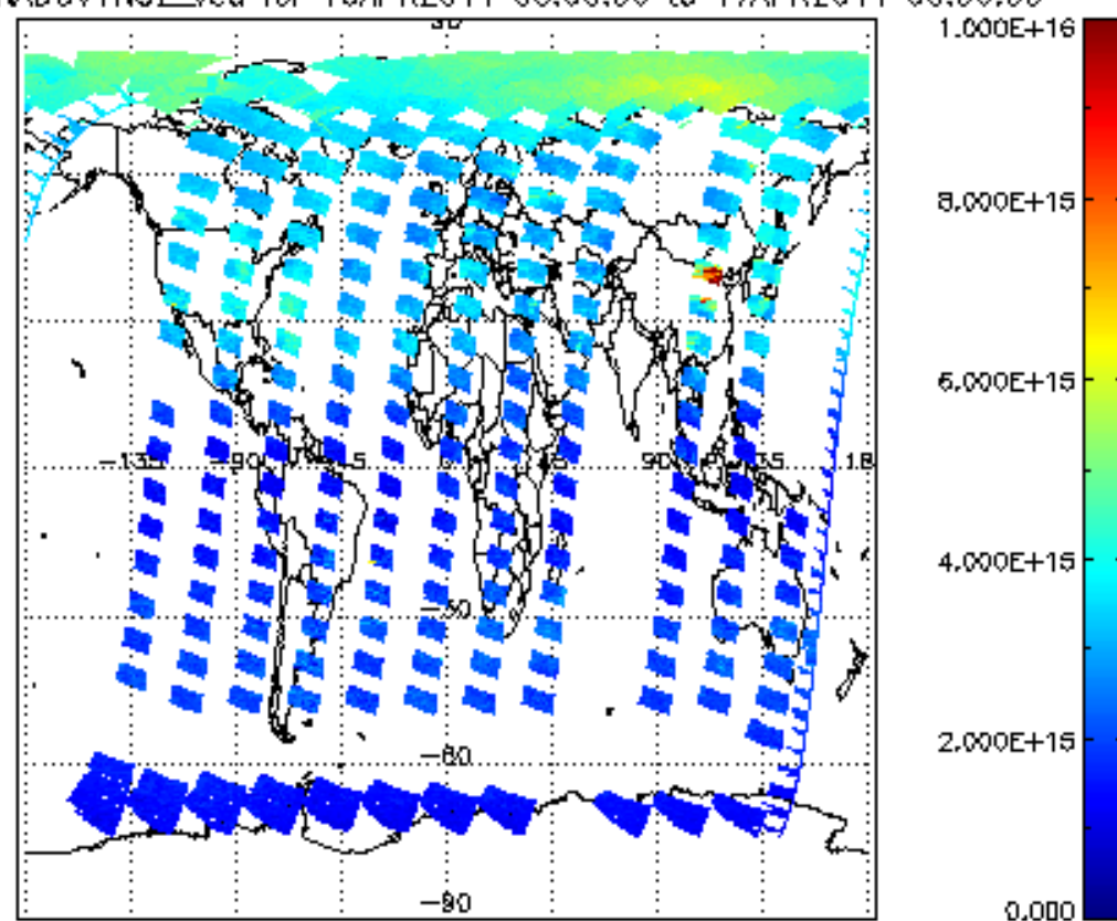
SCIOL2P_NADUV1NO2_vcd for 16APR2011 00:00:00 to 17APR2011 00:00:00
