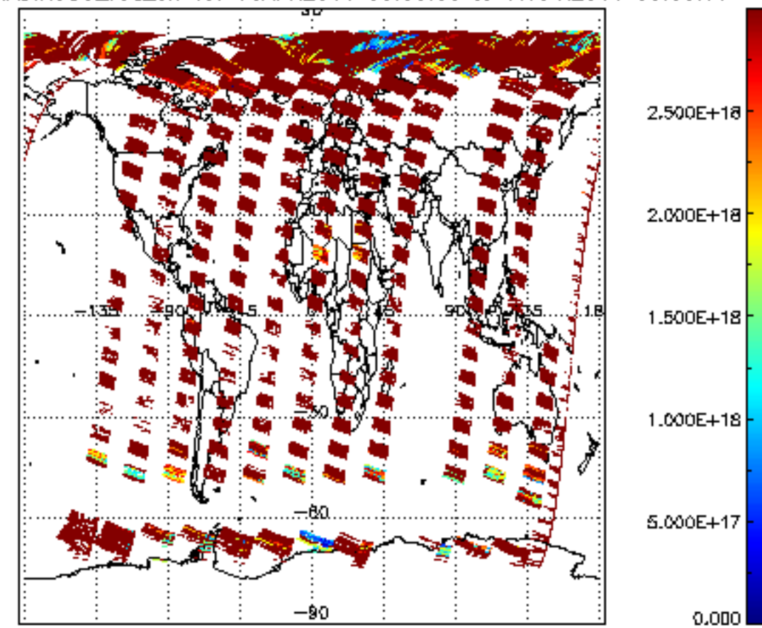
SCIOL2P_NADIR3CO_vcd_err for 16APR2011 00:00:00 to 17APR2011 00:00:00
