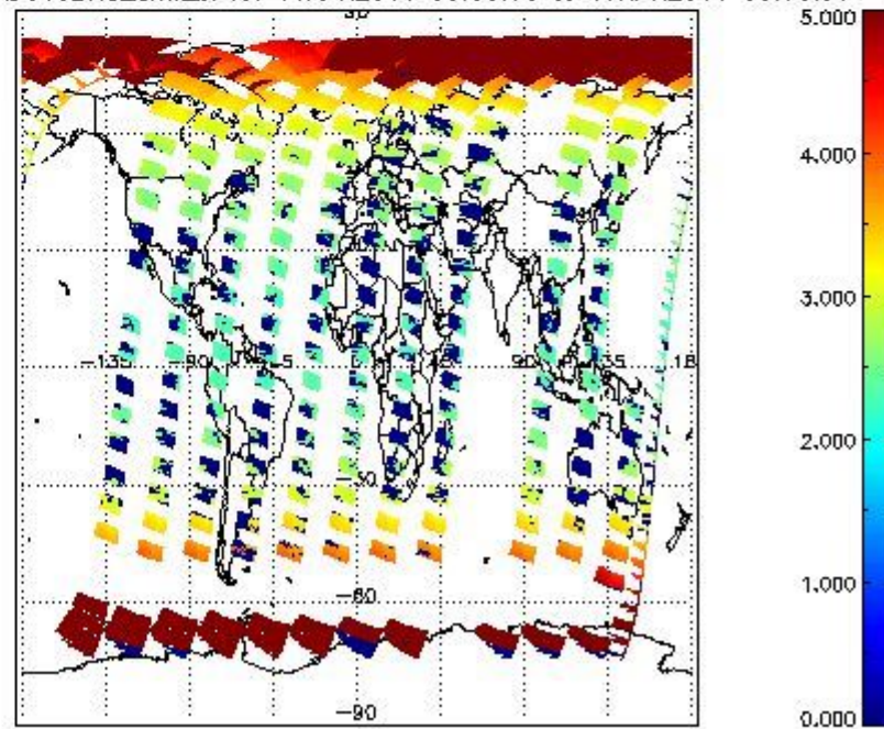
SCIOL2P_NADUV3BRO_amf_cl for 16APR2011 00:00:00 to 17APR2011 00:00:00
