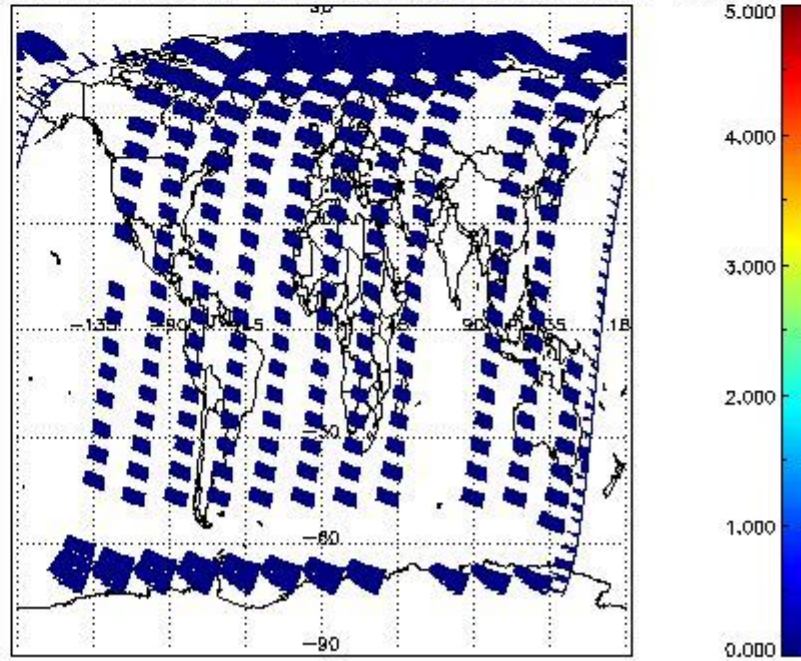
SCIOL2P_NADUV5S02_amf_cl for 16APR2011 00:00:00 to 17APR2011 00:00:00
