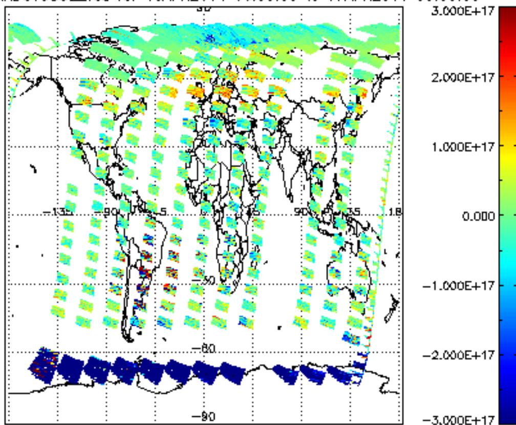
SCIOL2P_NADUV5S02_vcd for 16APR2011 00:00:00 to 17APR2011 00:00:00
