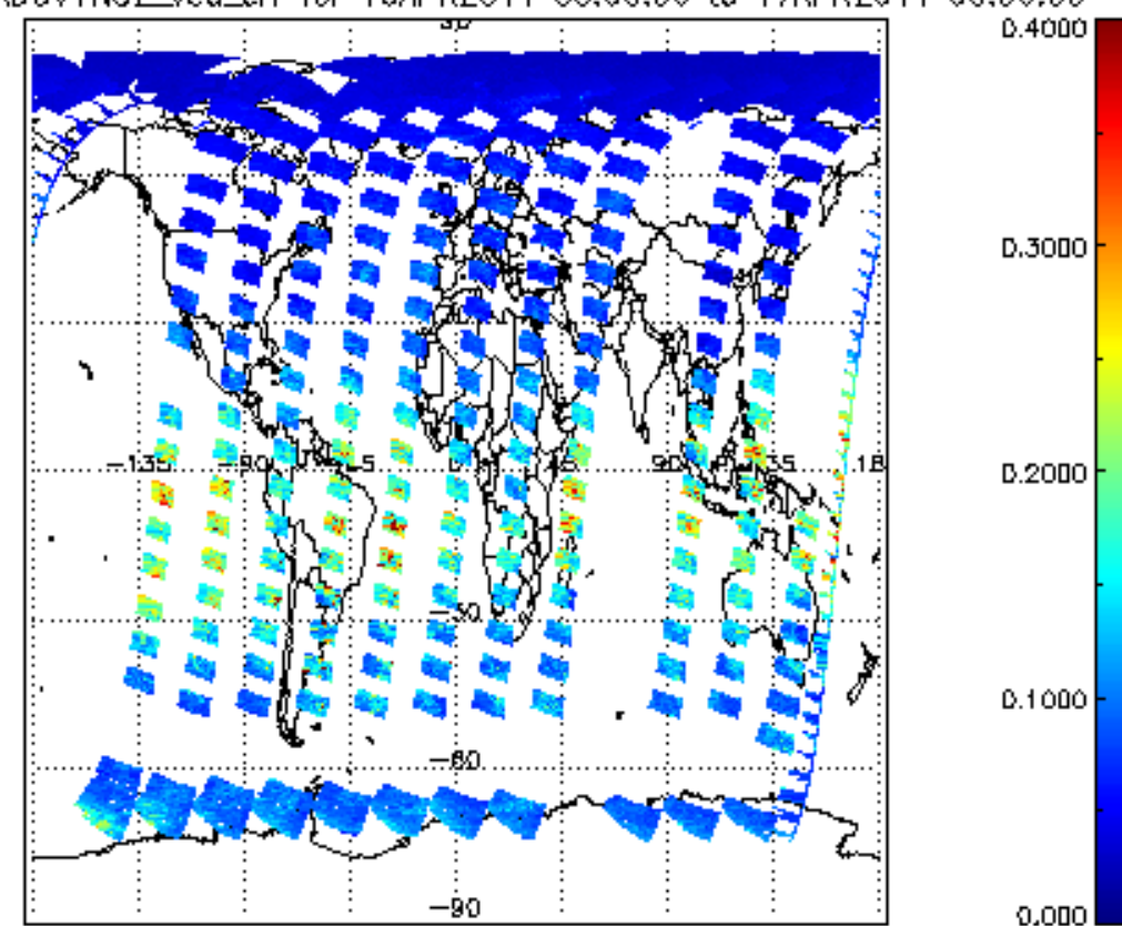
SCIOL2P_NADUV1NO2_vcd_err for 16APR2011 00:00:00 to 17APR2011 00:00:00
