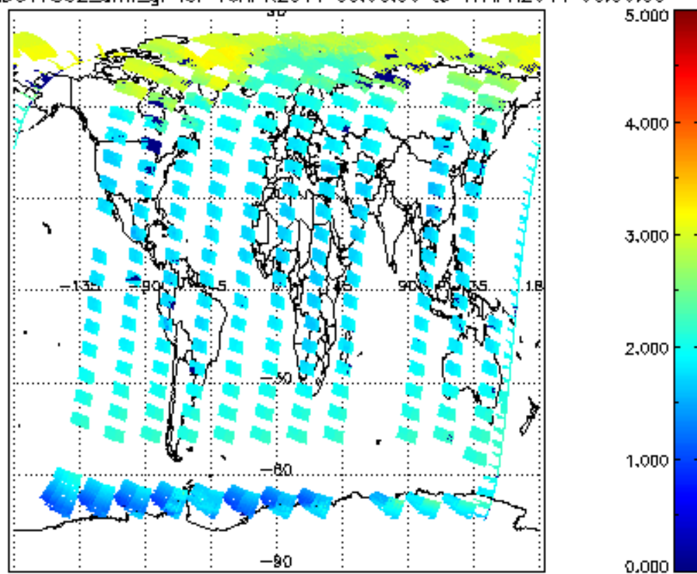
SCIOL2P_NADUV7S02_amf_gr for 16APR2011 00:00:00 to 17APR2011 00:00:00
