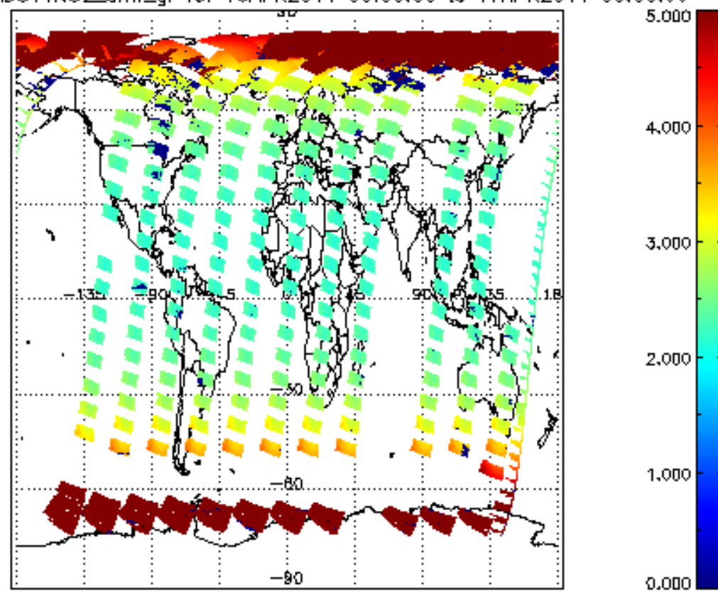
SCIOL2P_NADUV1NO2_amf_gr for 16APR2011 00:00:00 to 17APR2011 00:00:00
