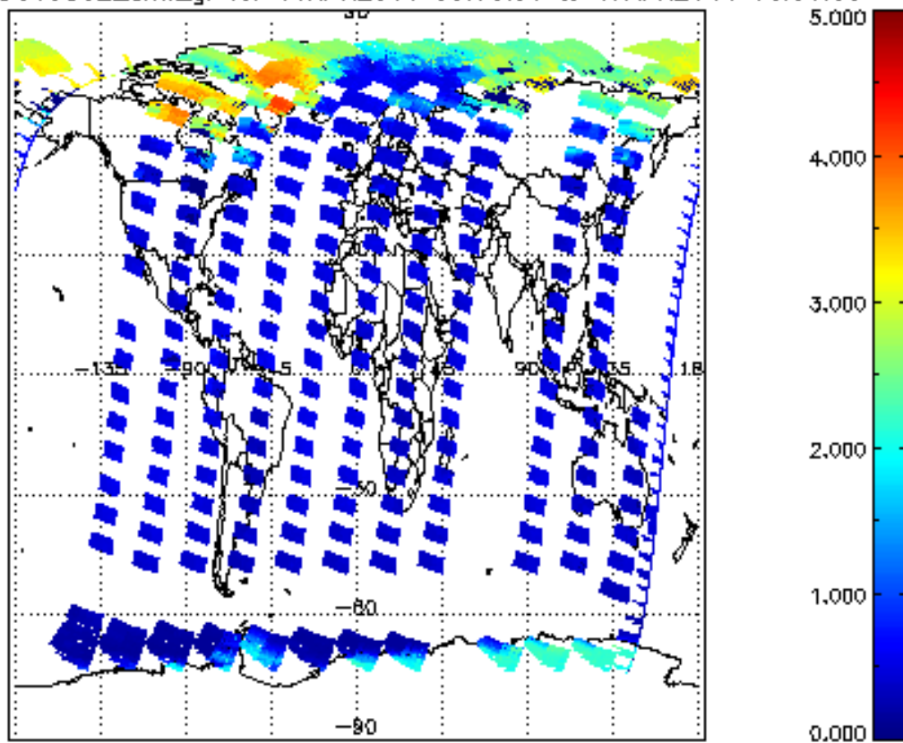
SCIOL2P_NADUV5S02_amf_gr for 16APR2011 00:00:00 to 17APR2011 00:00:00
