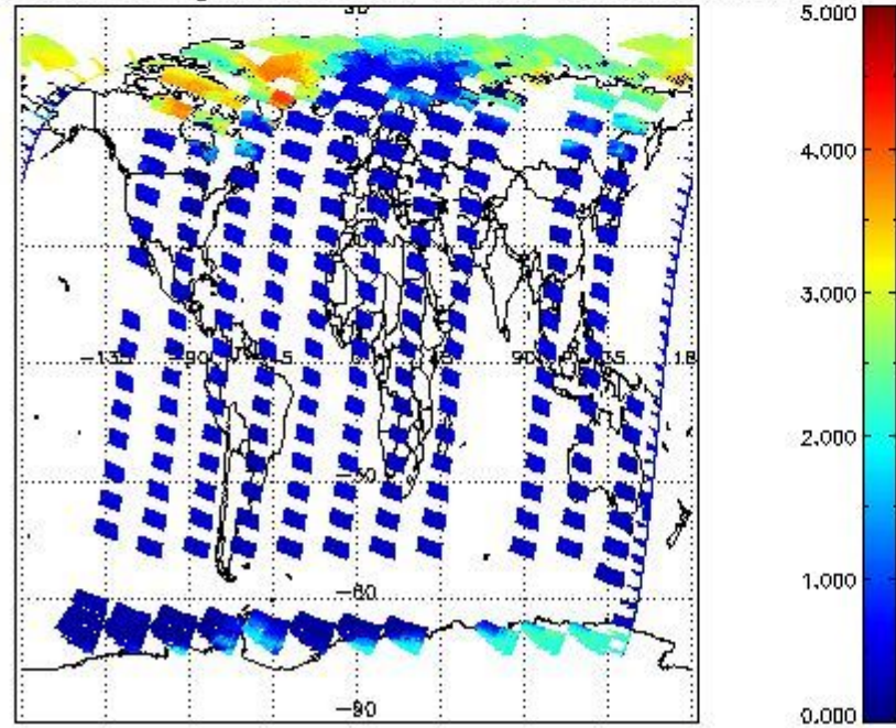
SCIOL2P_NADUV5S02_amf_gr for 16APR2011 00:00:00 to 17APR2011 00:00:00
