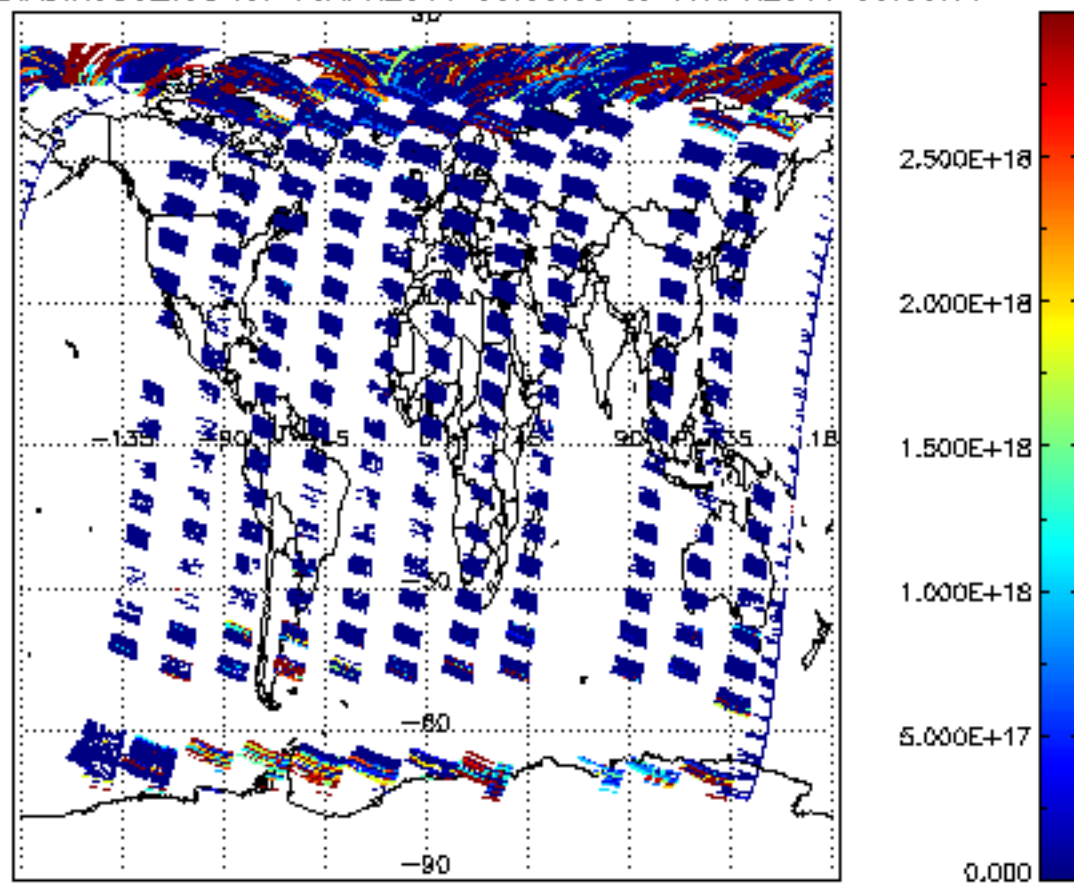
SCIOL2P_NADIR3CO_vcd for 16APR2011 00:00:00 to 17APR2011 00:00:00
