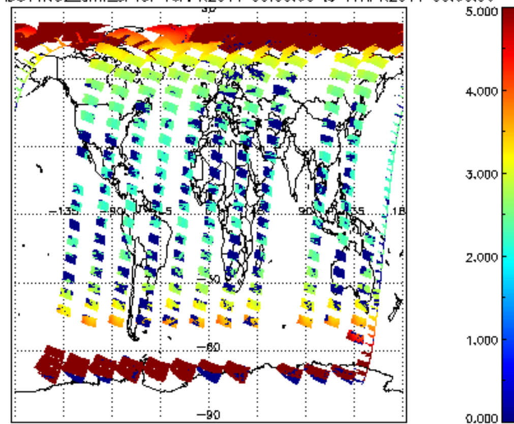
SCIOL2P_NADUV1NO2_amf_sl for 16APR2011 00:00:00 to 17APR2011 00:00:00
