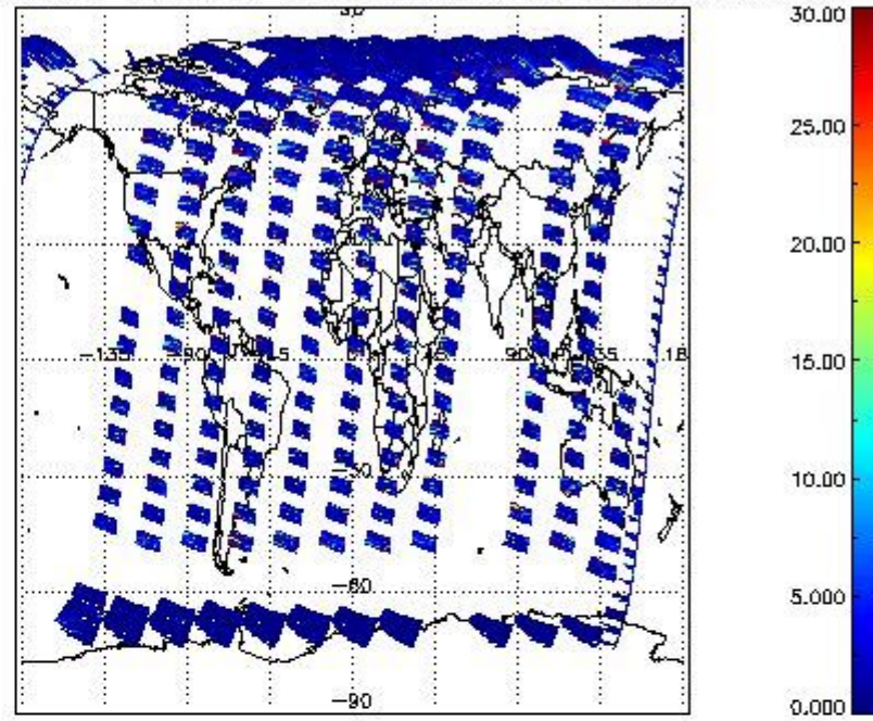
SCIOL2P_NADUV7S02_vcd_err for 16APR2011 00:00:00 to 17APR2011 00:00:00
