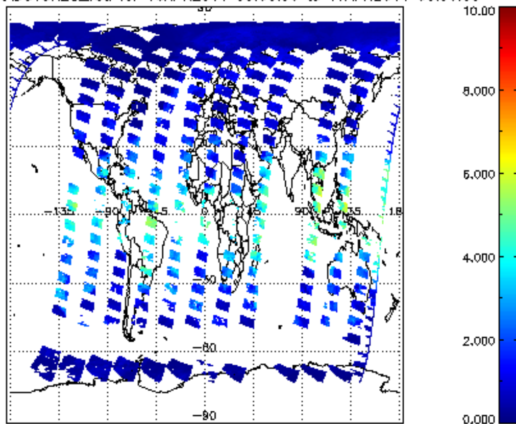
SCIOL2P_NADUV8H2O_vcd for 16APR2011 00:00:00 to 17APR2011 00:00:00
