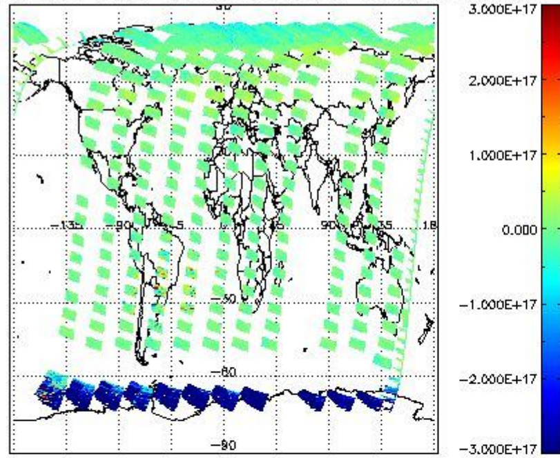
SCIOL2P_NADUV7S02_vcd for 16APR2011 00:00:00 to 17APR2011 00:00:00
