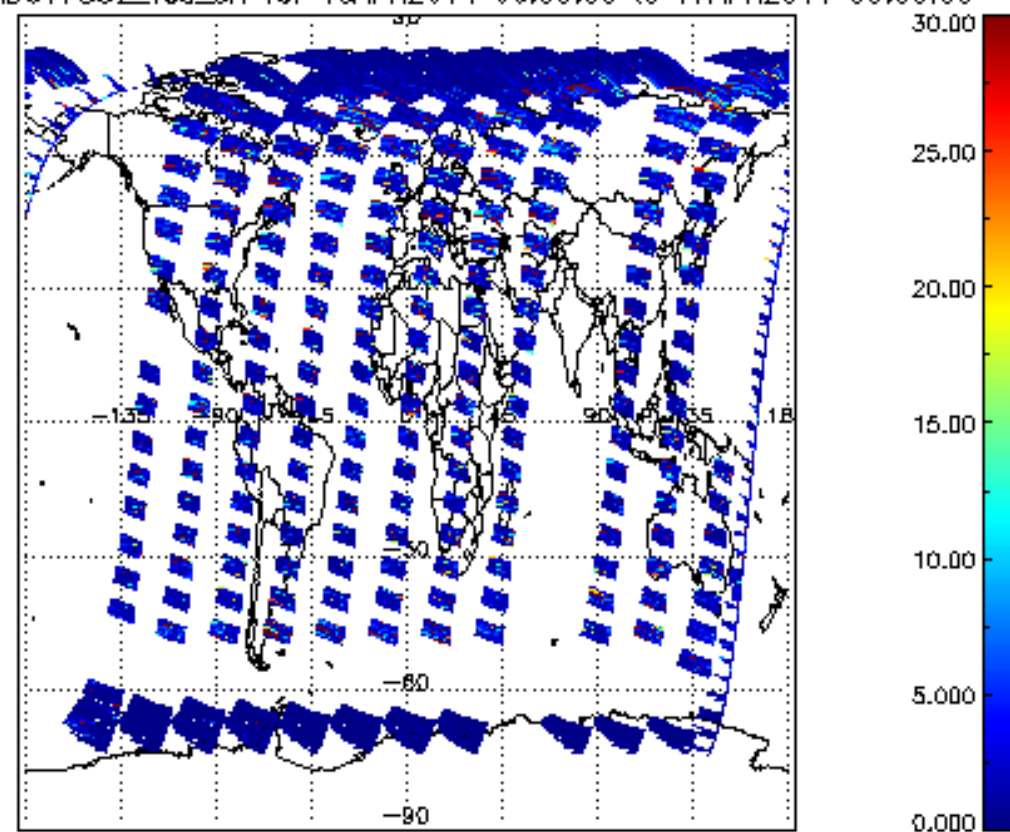
SCIOL2P_NADUV7S02_vcd_err for 16APR2011 00:00:00 to 17APR2011 00:00:00
