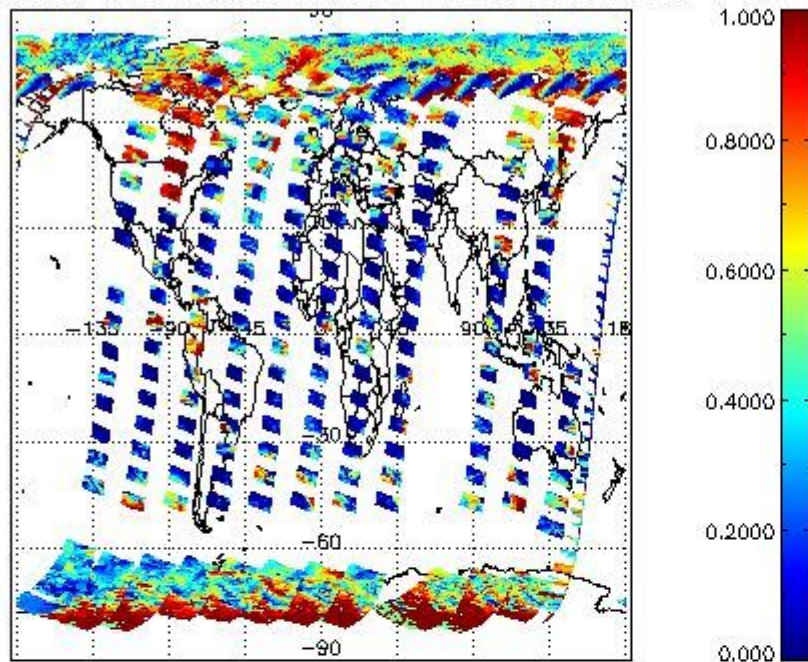
cL_frac for 16APR2011 00:00:00 to 17APR2011 00:00:00
