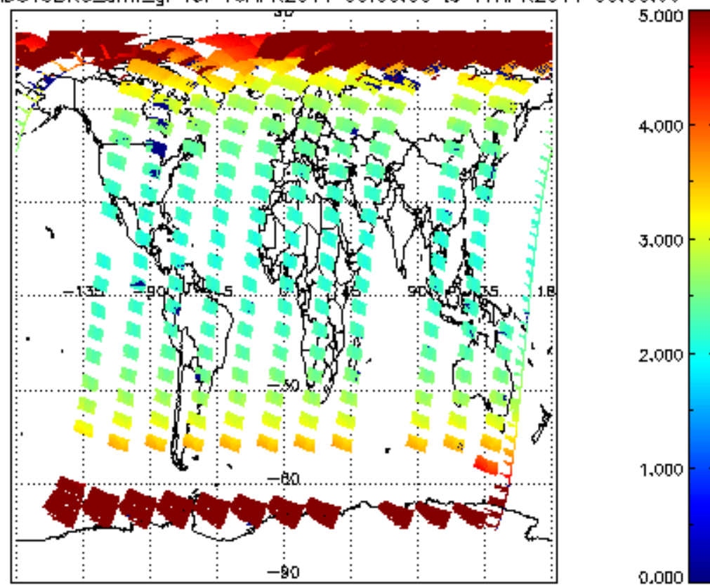
SCIOL2P_NADUV3BRO_amf_gr for 16APR2011 00:00:00 to 17APR2011 00:00:00
