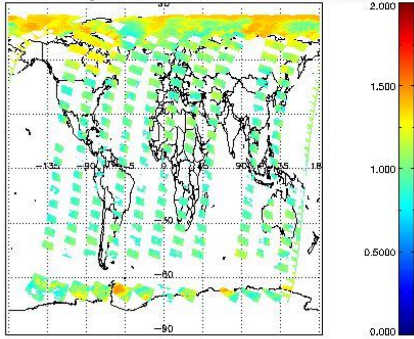
SCIOL2P_NADUV8H2O_arnf_gr for 16APR2011 00:00:00 to 17APR2011 00:00:00
