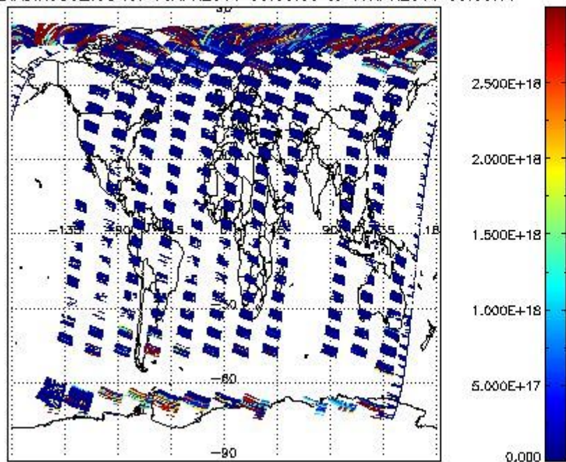
SCIDL2P_NADIR3CO_vcd for 16APR2011 00:00:00 to 17APR2011 00:00:00
