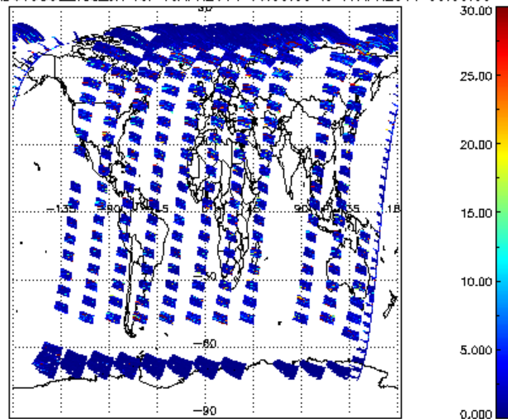
SCIOL2P_NADUV5S02_vcd_err for 16APR2011 00:00:00 to 17APR2011 00:00:00
