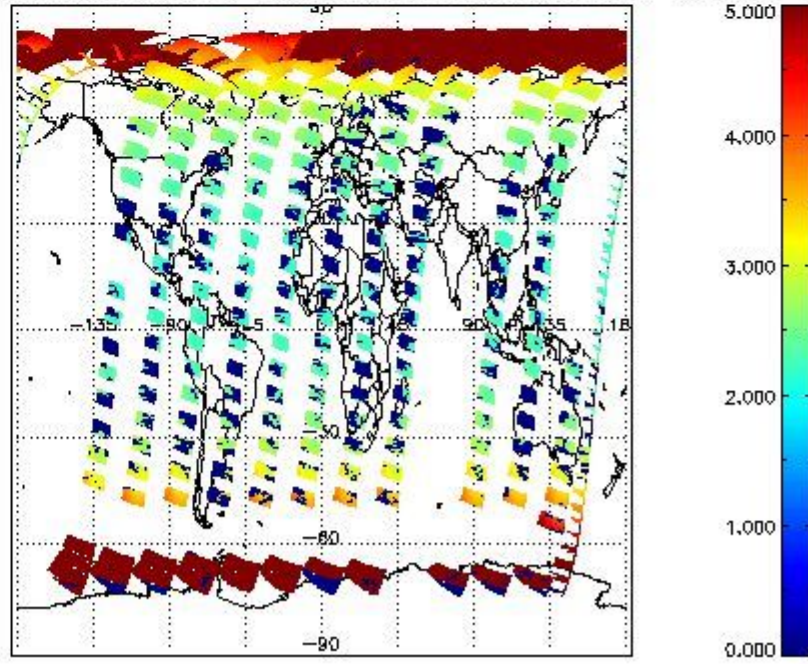
SCIOL2P_NADUV1NO2_amf_cl for 16APR2011 00:00:00 to 17APR2011 00:00:00
