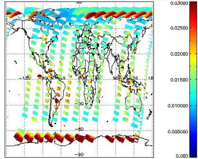
SCIOL2P_NADUV003_vcd_err for 16APR2011 00:00:00 to 17APR2011 00:00:00
