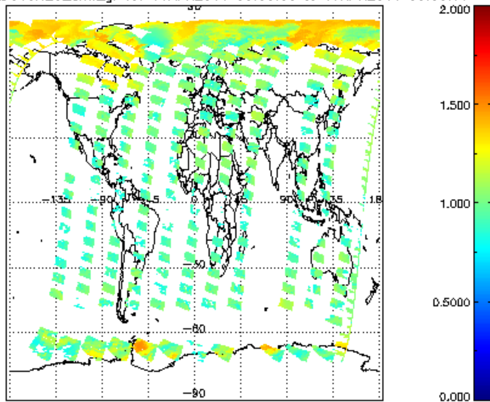
SCIOL2P_NADUV8H2O_amf_gr for 16APR2011 00:00:00 to 17APR2011 00:00:00
