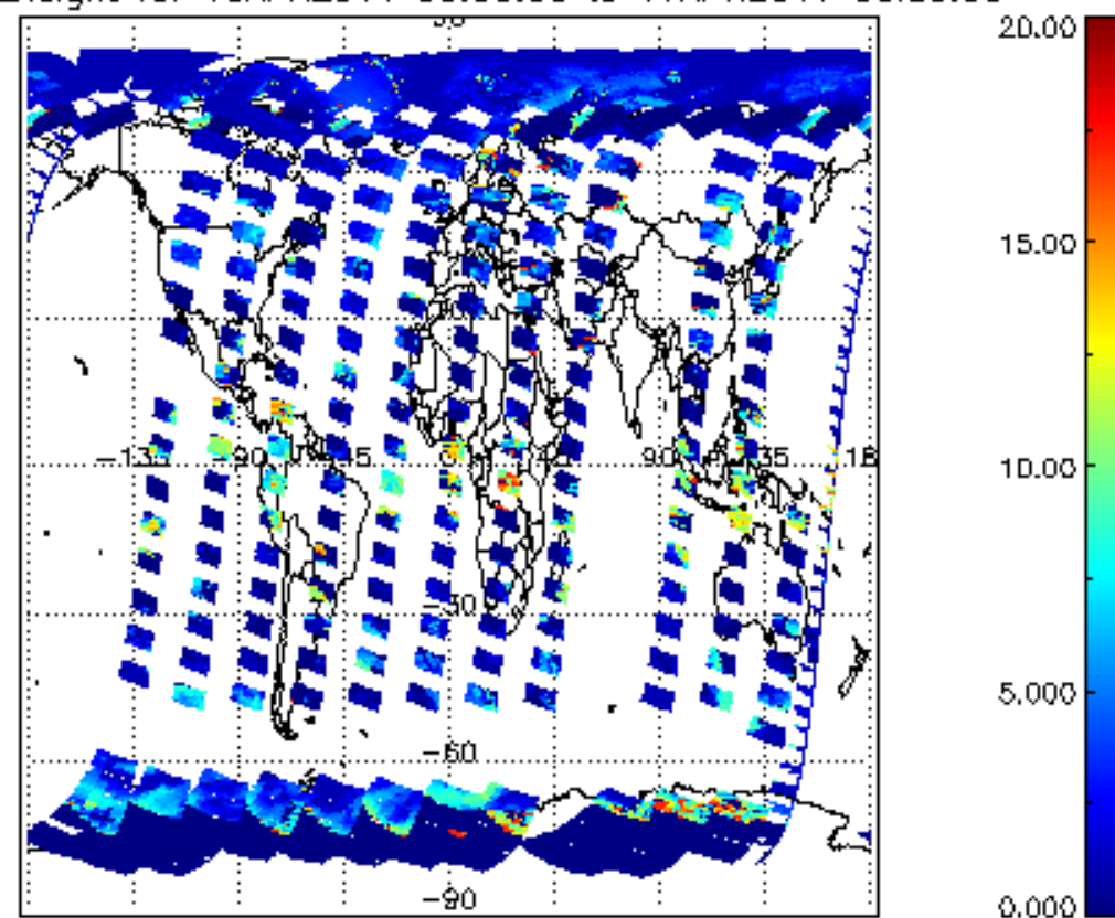
cl_top_height for 16APR2011 00:00:00 to 17APR2011 00:00:00
