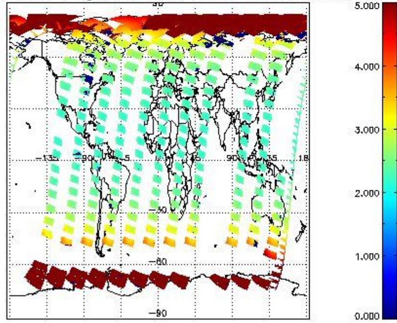
SCIOL2P_NADUV1NO2_amf_gr for 16APR2011 00:00:00 to 17APR2011 00:00:00
