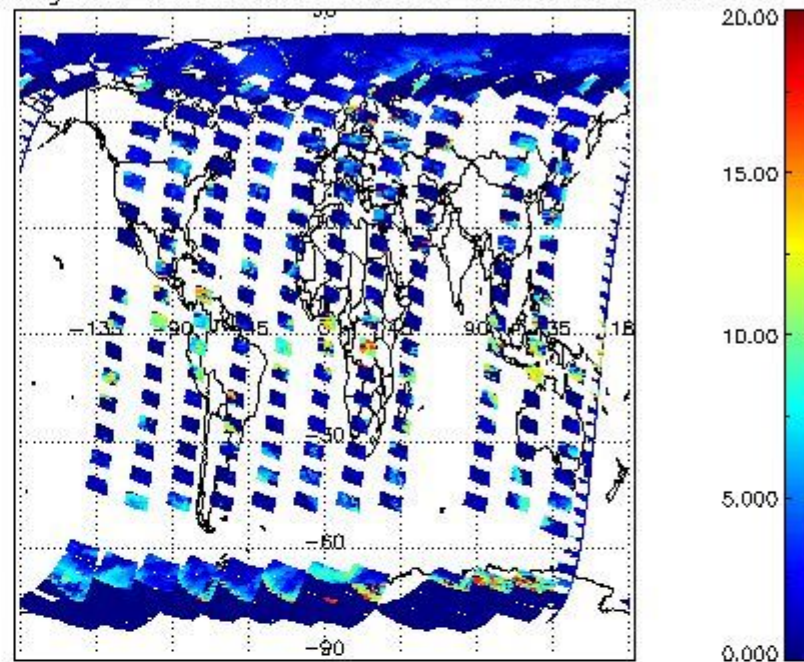
cL_top_height for 16APR2011 00:00:00 to 17APR2011 00:00:00
