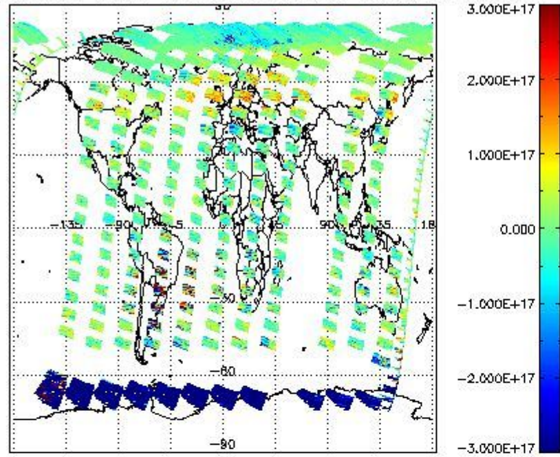
SCIOL2P_NADUV5S02_vcd for 16APR2011 00:00:00 to 17APR2011 00:00:00
