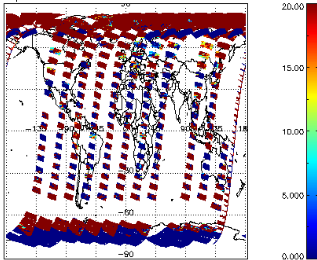
cl_opt_depth for 16APR2011 00:00:00 to 17APR2011 00:00:00
