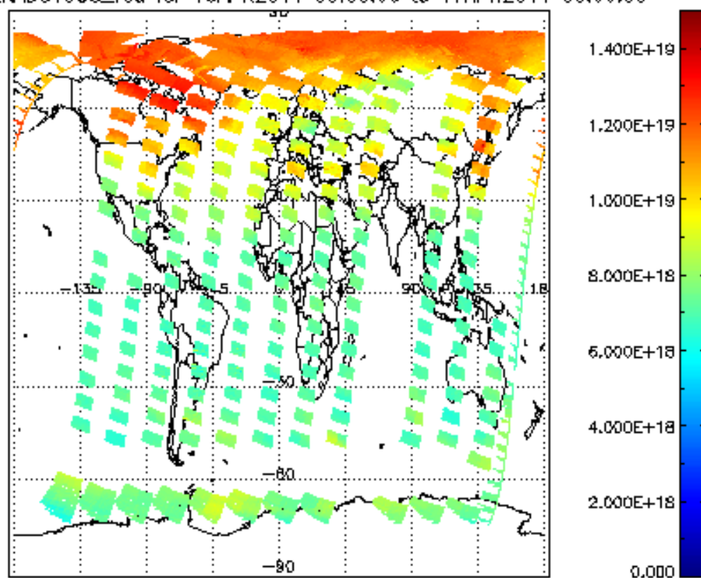
SCIOL2P_NADUV003_vcd for 16APR2011 00:00:00 to 17APR2011 00:00:00
