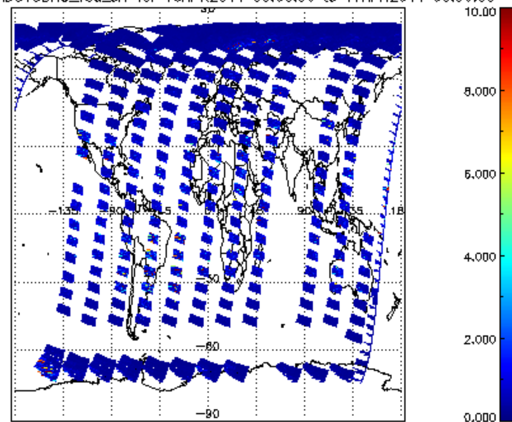
SCIOL2P_NADUV3BRO_vcd_err for 16APR2011 00:00:00 to 17APR2011 00:00:00
