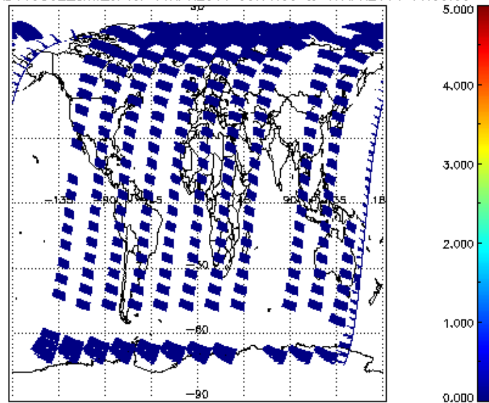
SCIOL2P_NADUV5S02_amf_cl for 16APR2011 00:00:00 to 17APR2011 00:00:00
