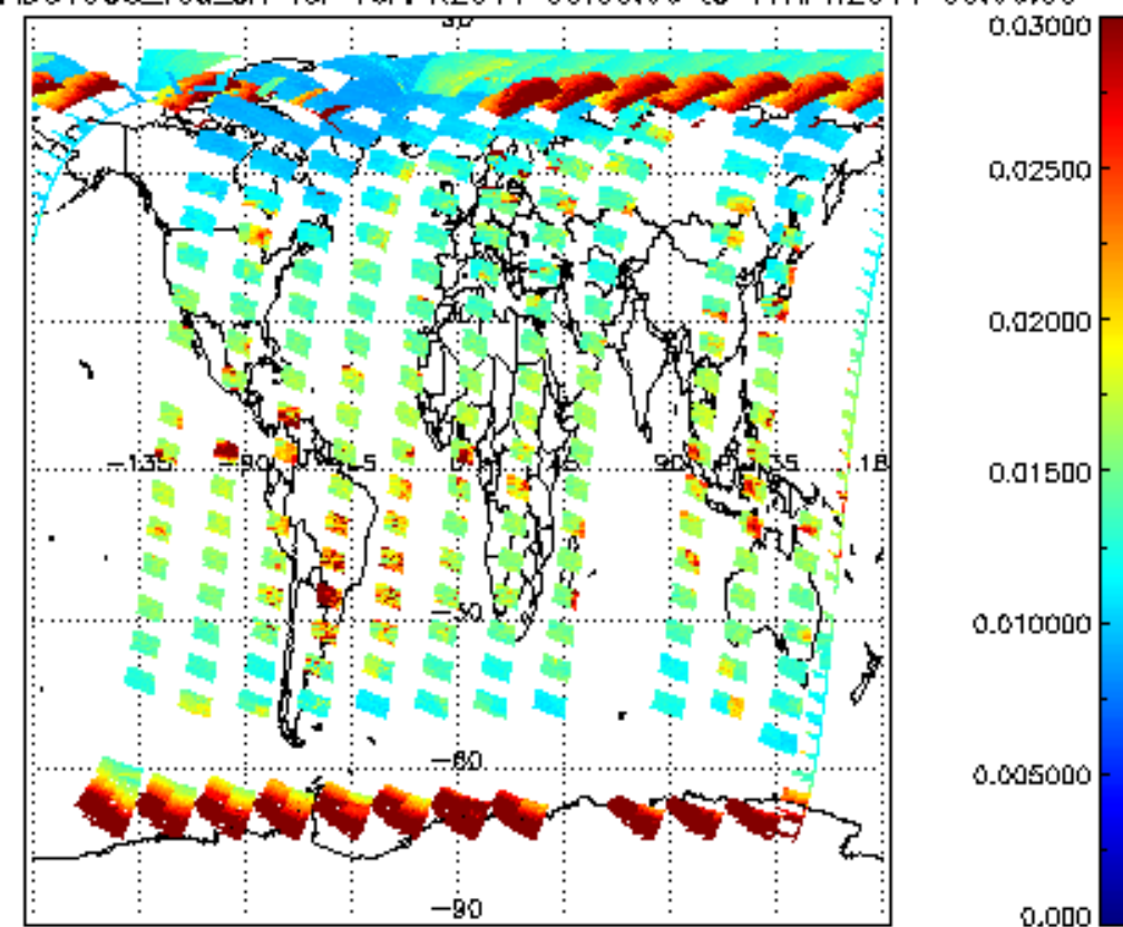
SCIOL2P_NADUV003_vcd_err for 16APR2011 00:00:00 to 17APR2011 00:00:00
