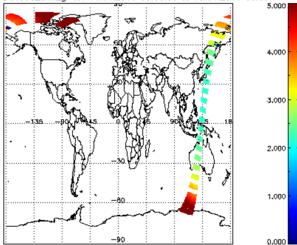
SCIOL2P_NADUV003_amf_gr for 14APR2011 00:00:00 to 15APR2011 00:00:00
