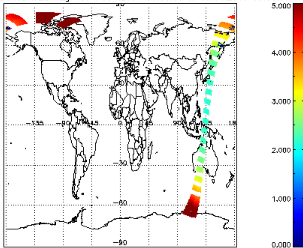
SCIOL2P_NADUV3BRO_amf_gr for 14APR2011 00:00:00 to 15APR2011 00:00:00
