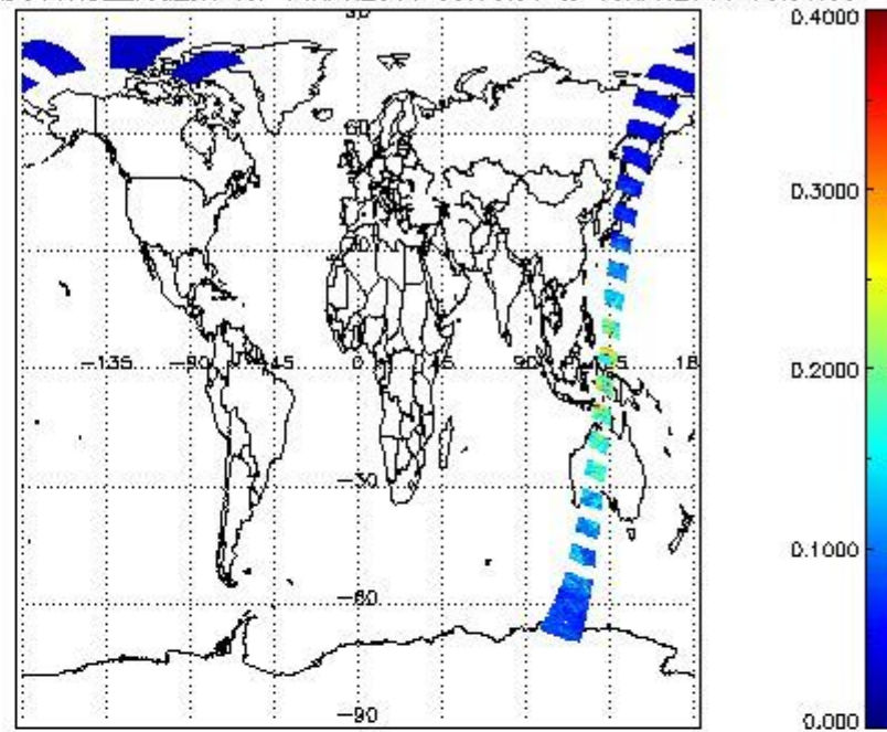
SCIOL2P_NADUV1NO2_vcd_err for 14APR2011 00:00:00 to 15APR2011 00:00:00
