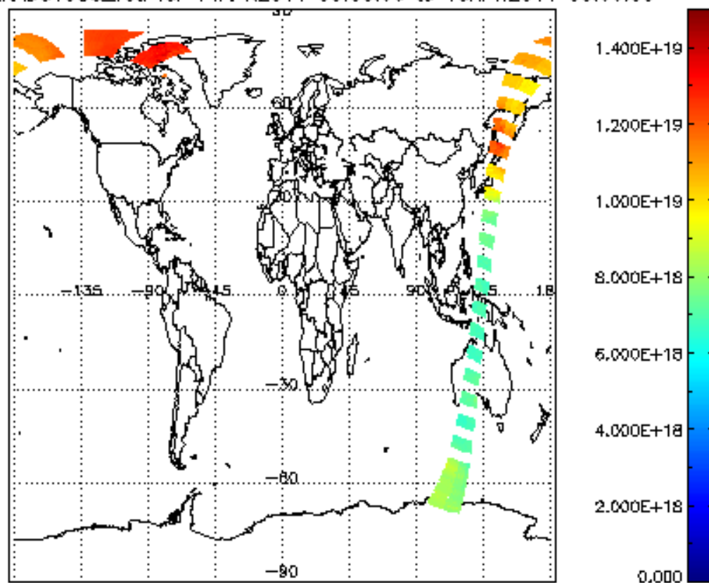
SCIOL2P_NADUV003_vcd for 14APR2011 00:00:00 to 15APR2011 00:00:00
