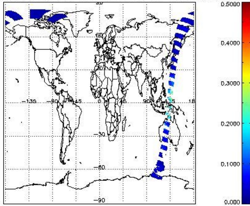
SCIOL2P_NADUV8H2O_vcd_err for 14APR2011 00:00:00 to 15APR2011 00:00:00
