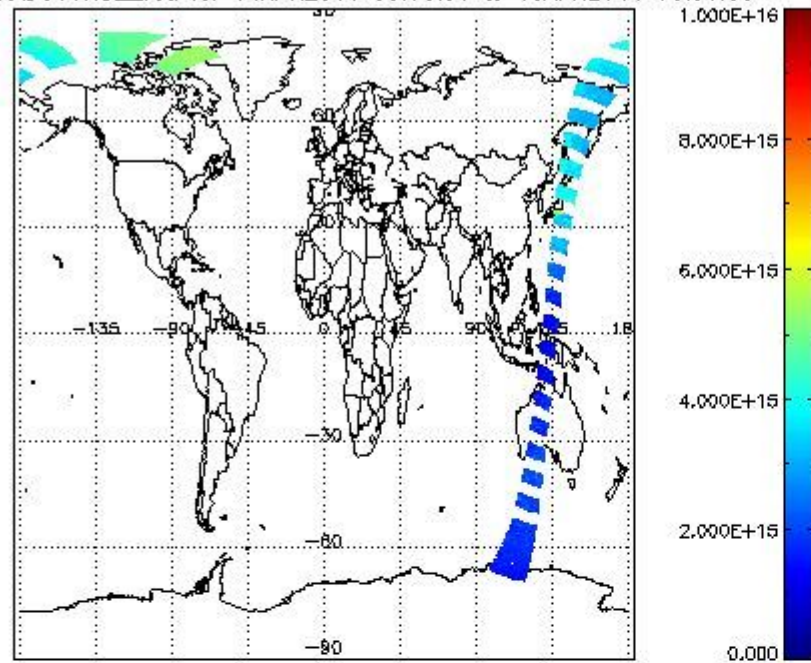
SCIOL2P_NADUV1NO2_vcd for 14APR2011 00:00:00 to 15APR2011 00:00:00
