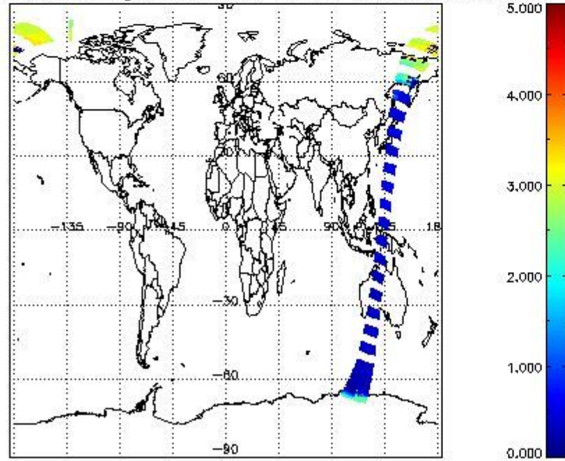
SCIOL2P_NADUV5S02_amf_gr for 14APR2011 00:00:00 to 15APR2011 00:00:00
