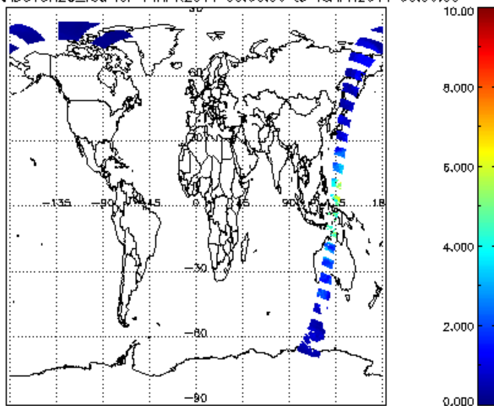
SCIOL2P_NADUV8H2O_vcd for 14APR2011 00:00:00 to 15APR2011 00:00:00
