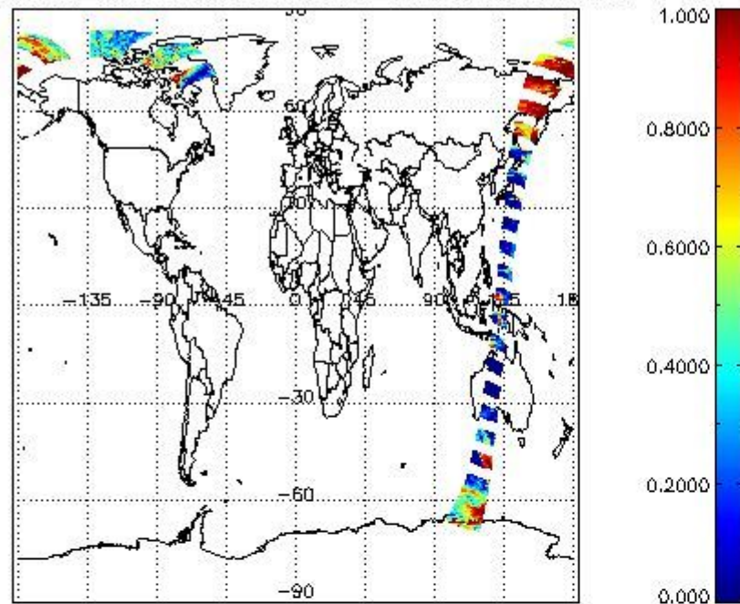
cL_frac for 14APR2011 00:00:00 to 15APR2011 00:00:00
