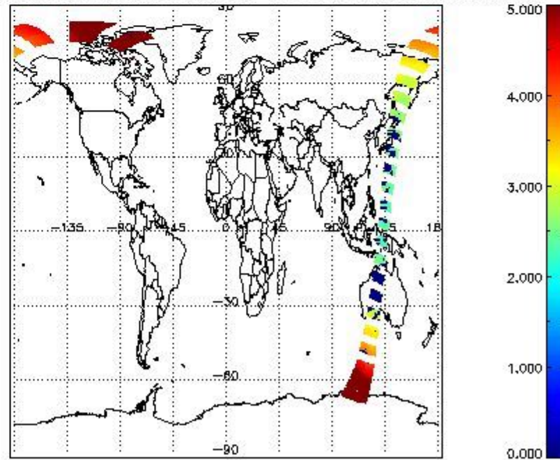
SCIOL2P_NADUV003_amf_cl for 14APR2011 00:00:00 to 15APR2011 00:00:00
