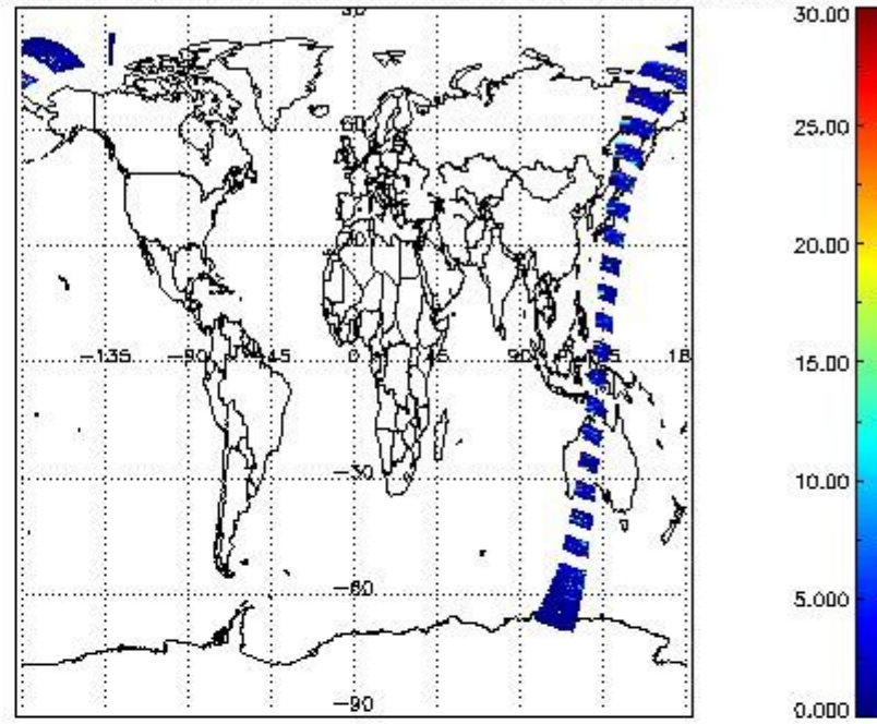
SCIOL2P_NADUV5S02_vcd_err for 14APR2011 00:00:00 to 15APR2011 00:00:00
