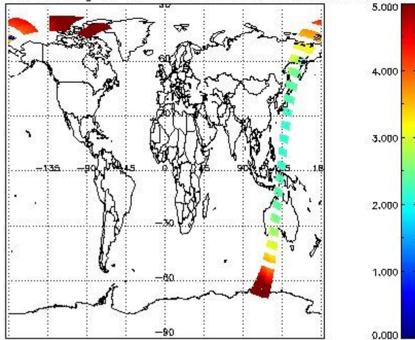
SCIOL2P_NADUV003_amf_gr for 14APR2011 00:00:00 to 15APR2011 00:00:00
