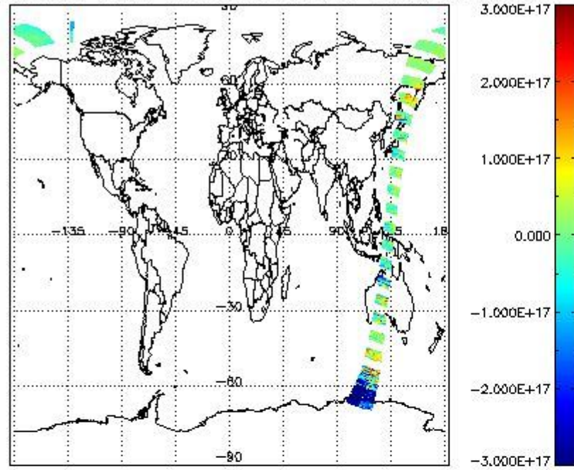
SCIOL2P_NADUV5S02_vcd for 14APR2011 00:00:00 to 15APR2011 00:00:00
