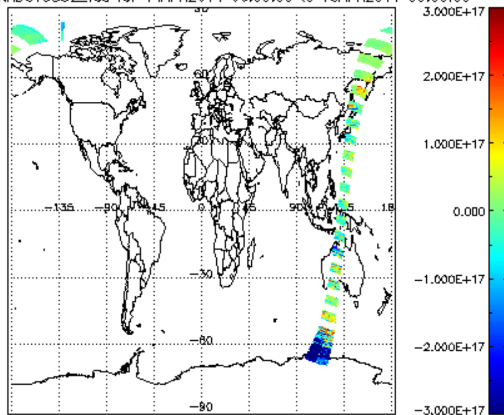
SCIOL2P_NADUV5S02_vcd for 14APR2011 00:00:00 to 15APR2011 00:00:00
