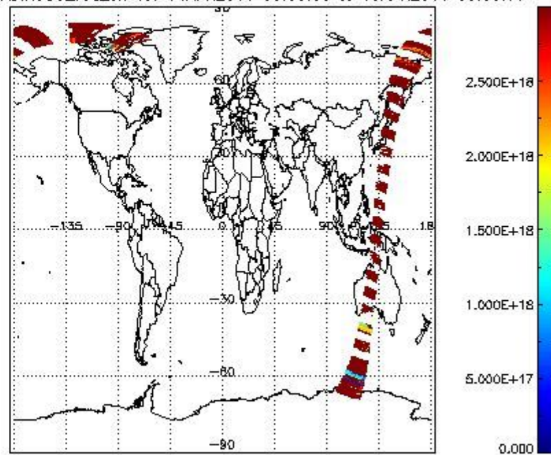
SCIDL2P_NADIR3CO_vcd_err for 14APR2011 00:00:00 to 15APR2011 00:00:00
