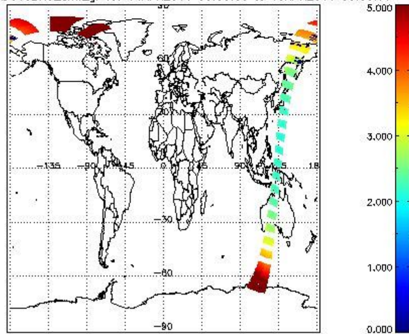
SCIOL2P_NADUV3BRO_amf_gr for 14APR2011 00:00:00 to 15APR2011 00:00:00
