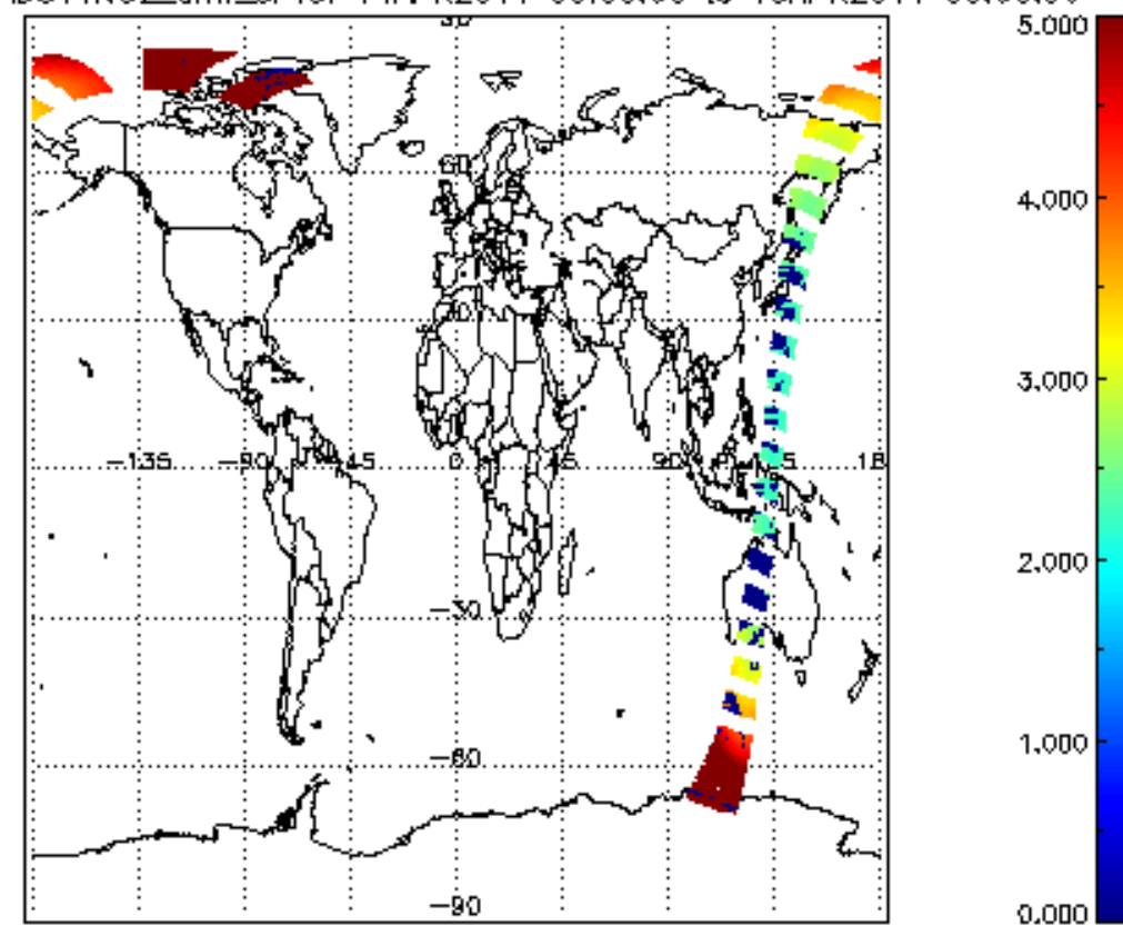
SCIOL2P_NADUV1NO2_amf_cl for 14APR2011 00:00:00 to 15APR2011 00:00:00
