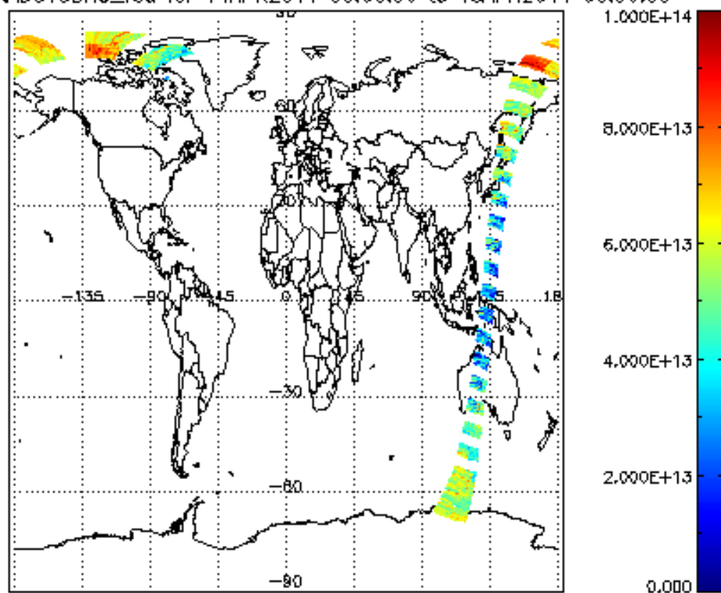
SCIOL2P_NADUV3BRO_vcd for 14APR2011 00:00:00 to 15APR2011 00:00:00
