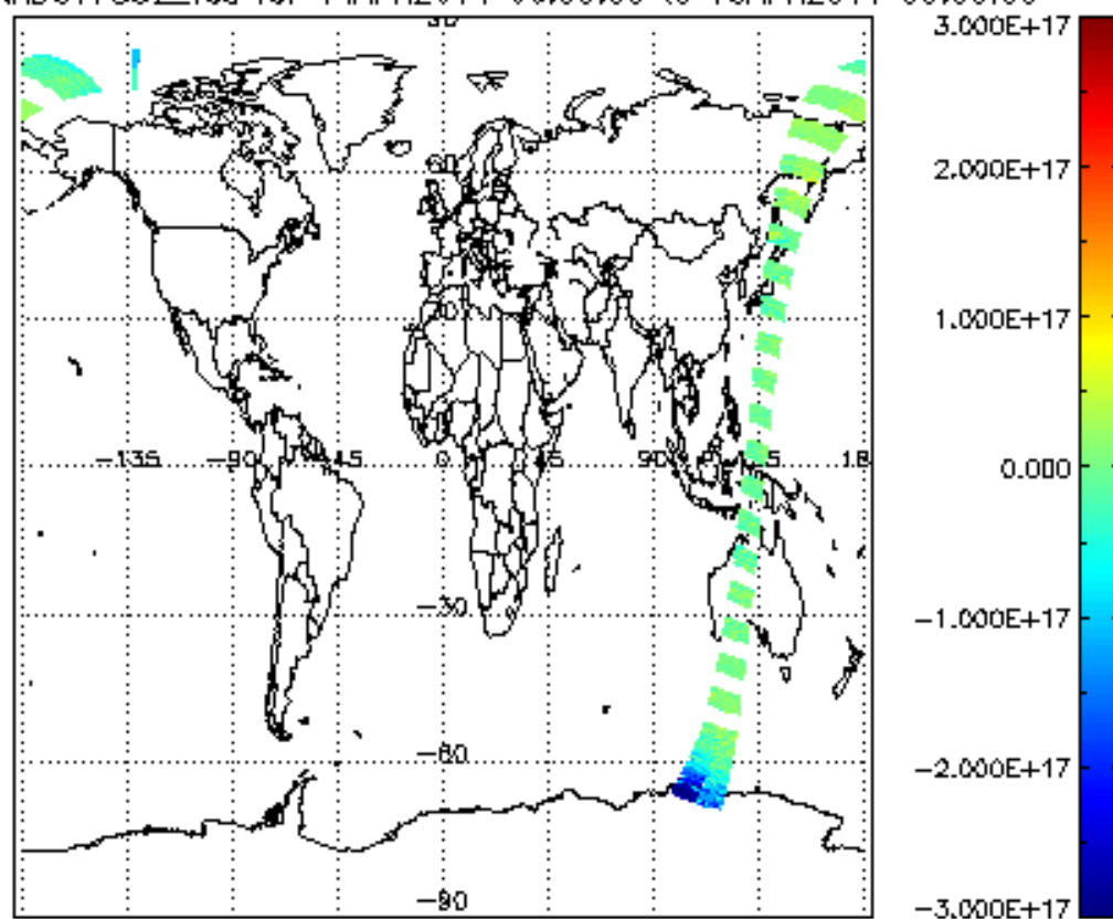
SCIOL2P_NADUV7S02_vcd for 14APR2011 00:00:00 to 15APR2011 00:00:00
