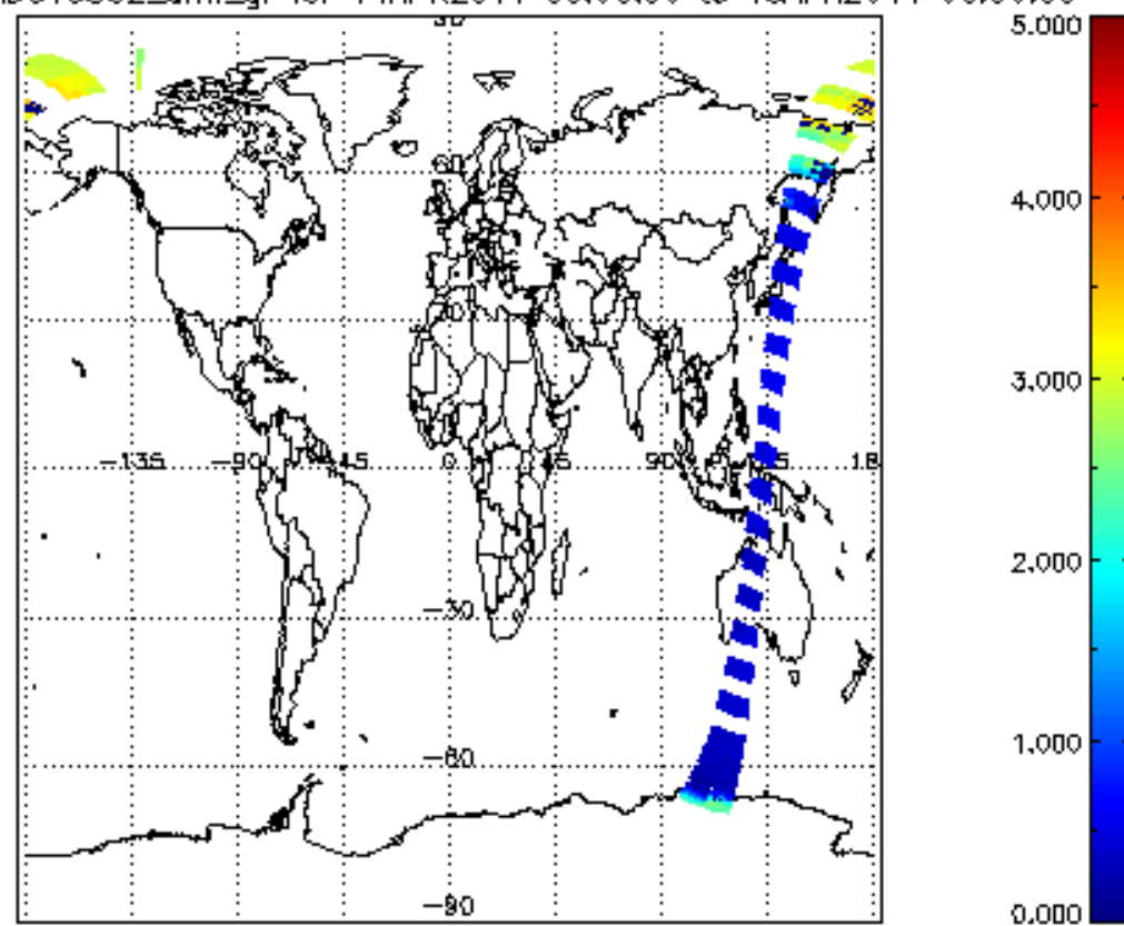
SCIOL2P_NADUV5S02_amf_gr for 14APR2011 00:00:00 to 15APR2011 00:00:00
