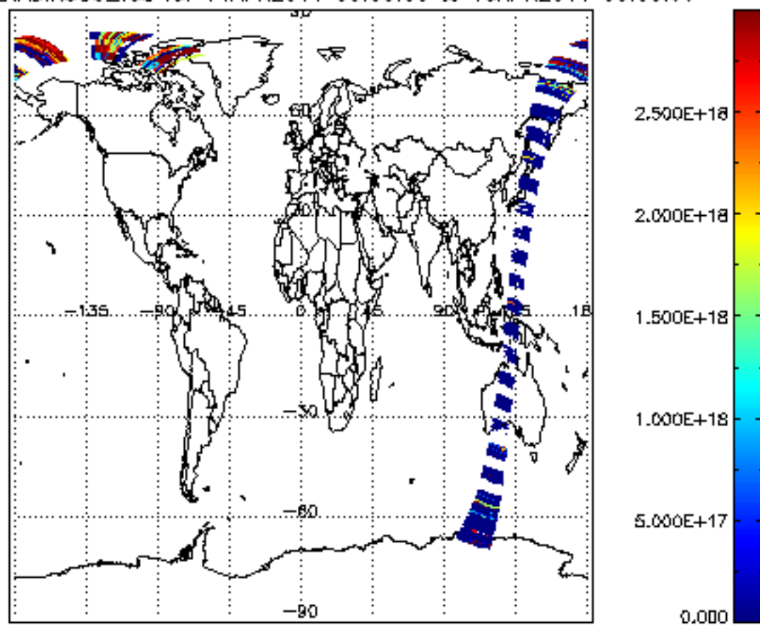
SCIOL2P_NADIR3CO_vcd for 14APR2011 00:00:00 to 15APR2011 00:00:00
