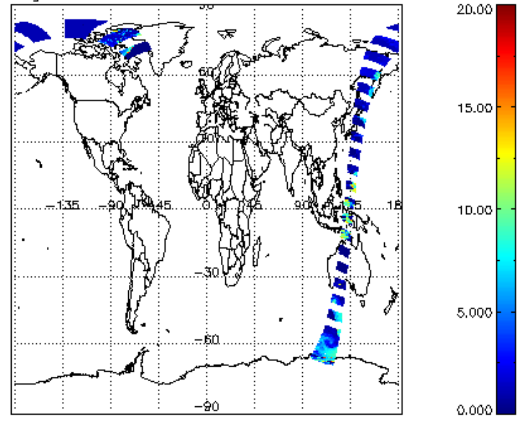
cl_top_height for 14APR2011 00:00:00 to 15APR2011 00:00:00
