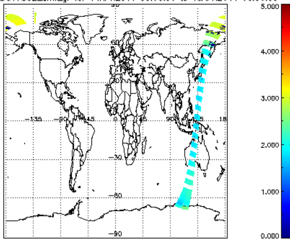
SCIOL2P_NADUV7S02_amf_gr for 14APR2011 00:00:00 to 15APR2011 00:00:00
