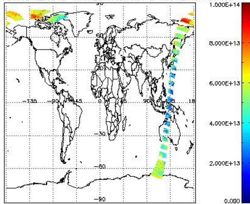
SCIOL2P_NADUV3BRO_vcd for 14APR2011 00:00:00 to 15APR2011 00:00:00
