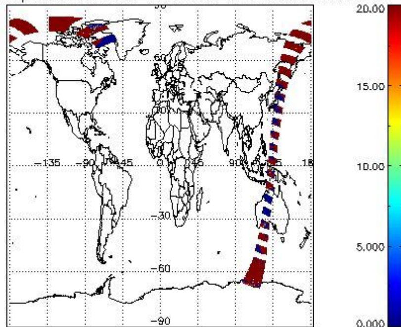
cL_opt_depth for 14APR2011 00:00:00 to 15APR2011 00:00:00
