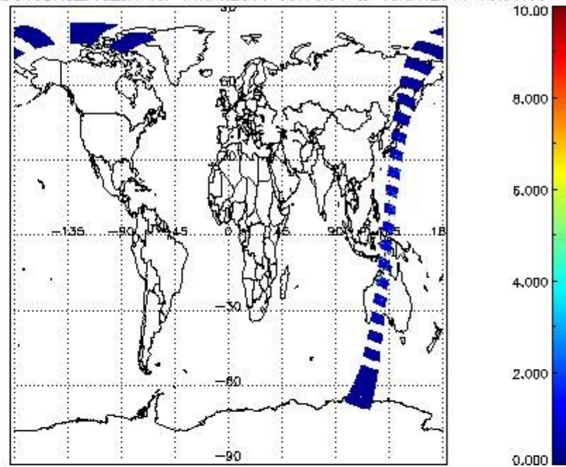
SCIOL2P_NADUV3BRO_vcd_err for 14APR2011 00:00:00 to 15APR2011 00:00:00
