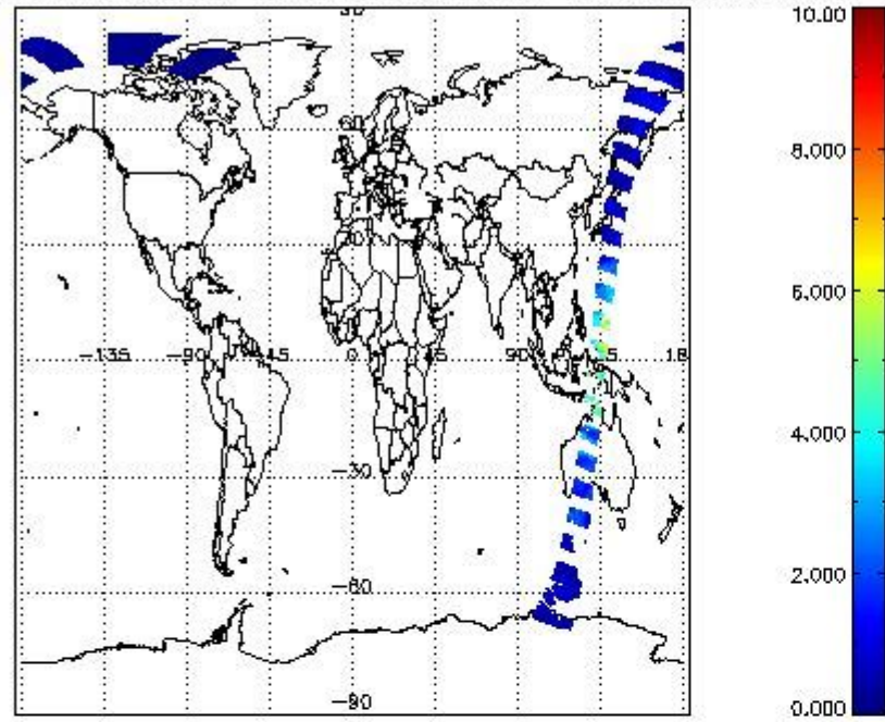
SCIOL2P_NADUV8H2O_vcd for 14APR2011 00:00:00 to 15APR2011 00:00:00
