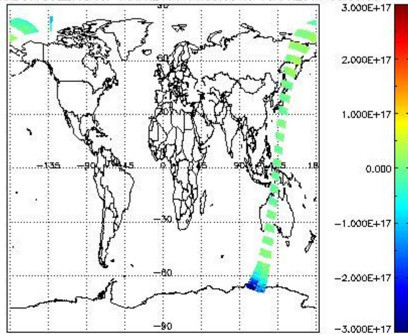
SCIOL2P_NADUV7S02_vcd for 14APR2011 00:00:00 to 15APR2011 00:00:00
