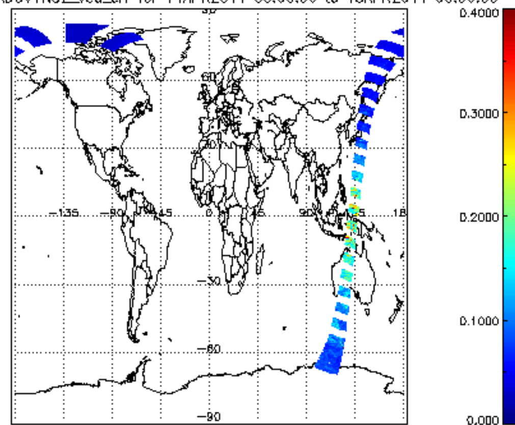
SCIOL2P_NADUV1NO2_vcd_err for 14APR2011 00:00:00 to 15APR2011 00:00:00
