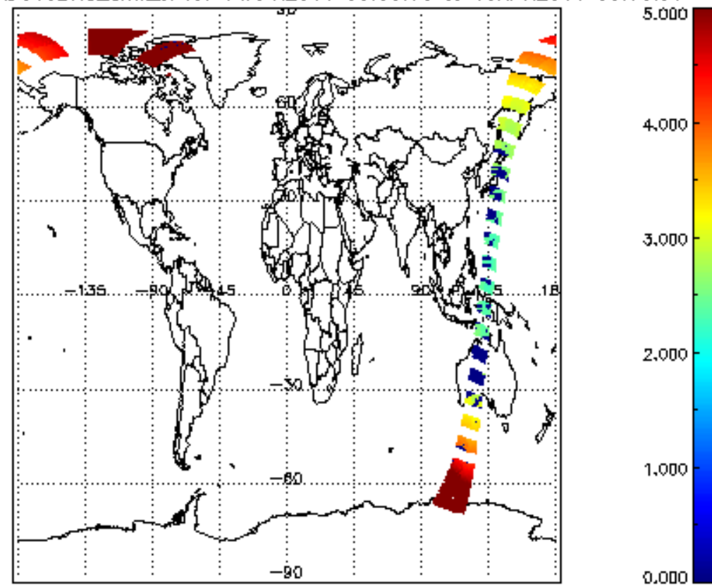
SCIOL2P_NADUV3BRO_amf_cl for 14APR2011 00:00:00 to 15APR2011 00:00:00
