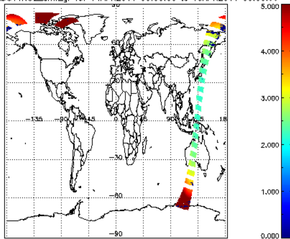
SCIOL2P_NADUV1NO2_amf_gr for 14APR2011 00:00:00 to 15APR2011 00:00:00
