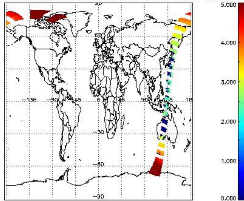
SCIOL2P_NADUV3BRO_amf_cl for 14APR2011 00:00:00 to 15APR2011 00:00:00
