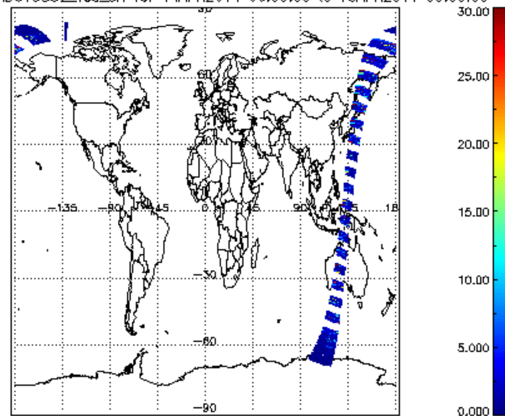
SCIOL2P_NADUV5S02_vcd_err for 14APR2011 00:00:00 to 15APR2011 00:00:00
