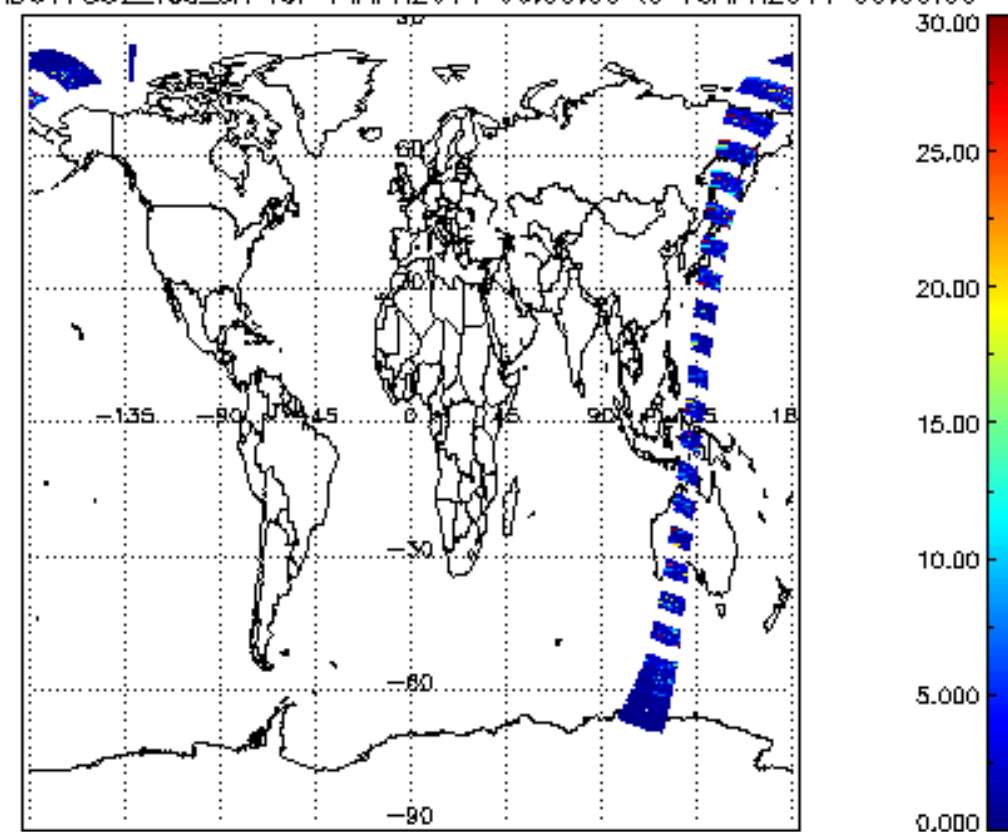
SCIOL2P_NADUV7S02_vcd_err for 14APR2011 00:00:00 to 15APR2011 00:00:00
