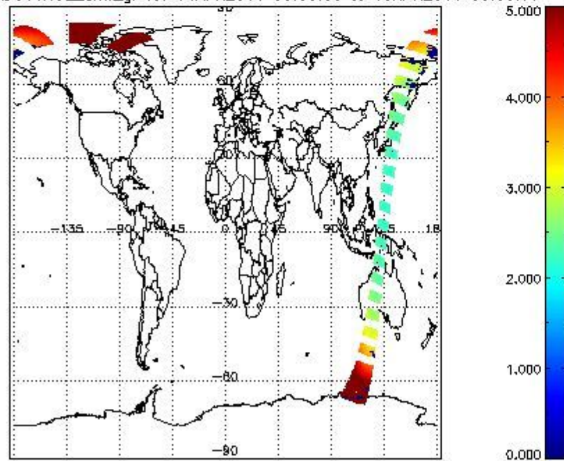
SCIOL2P_NADUV1NO2_amf_gr for 14APR2011 00:00:00 to 15APR2011 00:00:00
