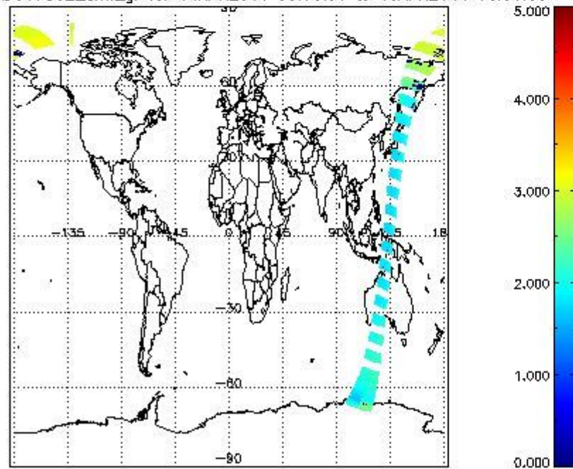
SCIOL2P_NADUV7S02_amf_gr for 14APR2011 00:00:00 to 15APR2011 00:00:00
