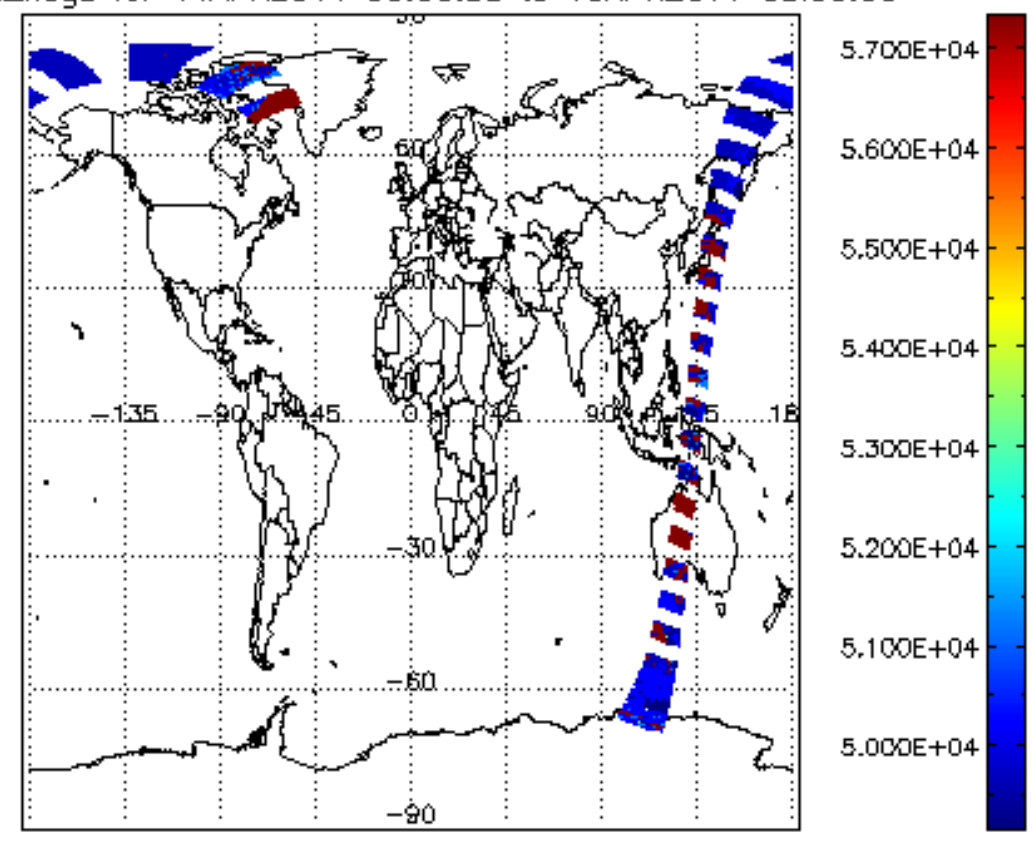
cloud_flags for 14APR2011 00:00:00 to 15APR2011 00:00:00
