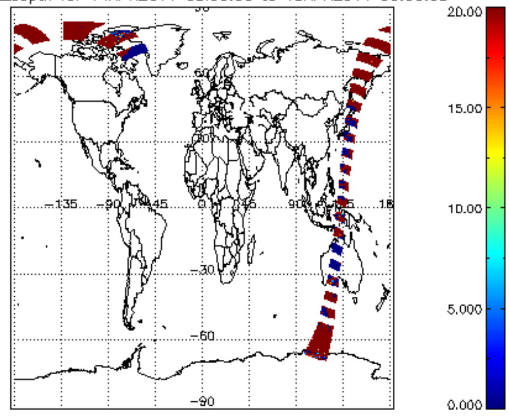
cl_opt_depth for 14APR2011 00:00:00 to 15APR2011 00:00:00
