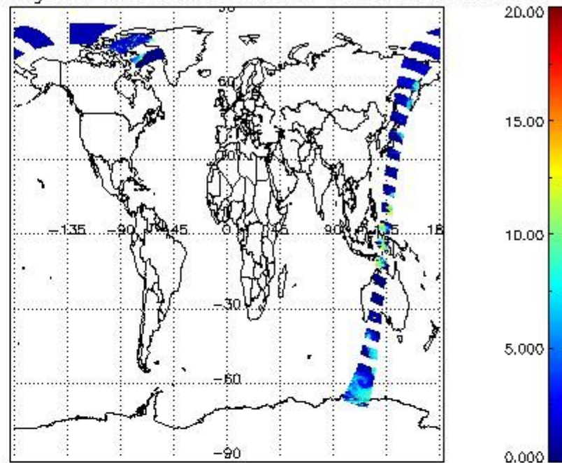
cL_top_height for 14APR2011 00:00:00 to 15APR2011 00:00:00
