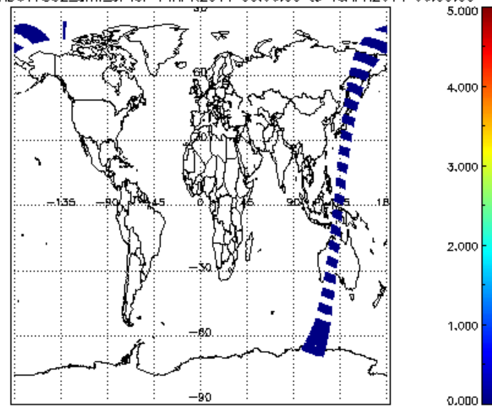
SCIOL2P_NADUV7S02_amf_cl for 14APR2011 00:00:00 to 15APR2011 00:00:00
