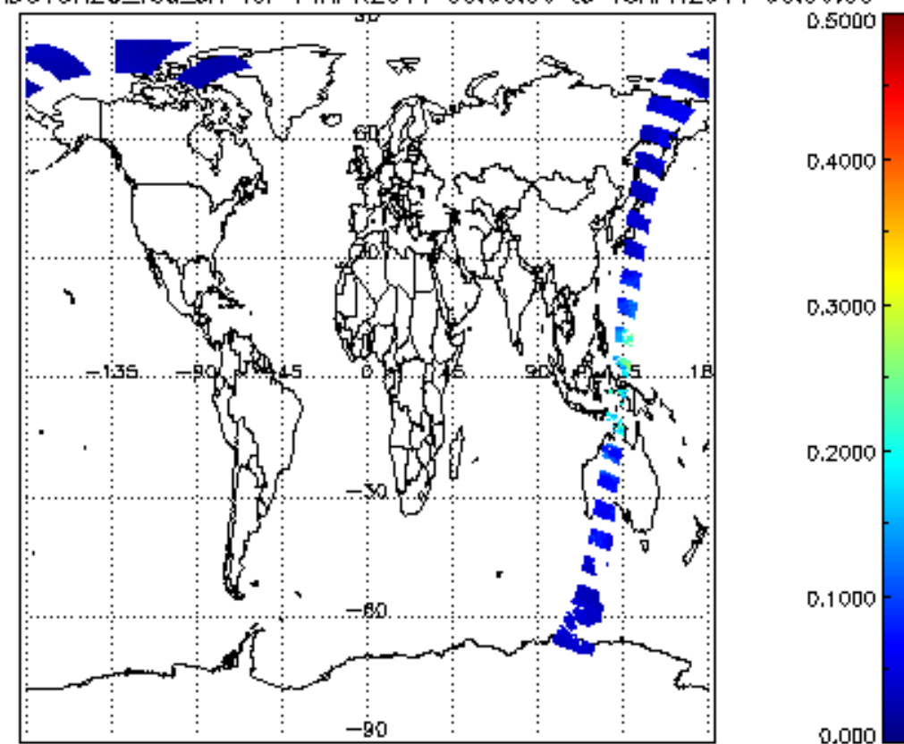
SCIOL2P_NADUV8H2O_vcd_err for 14APR2011 00:00:00 to 15APR2011 00:00:00
