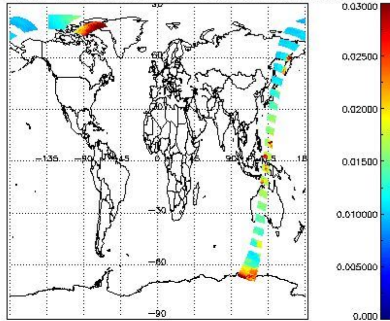
SCIOL2P_NADUV003_vcd_err for 14APR2011 00:00:00 to 15APR2011 00:00:00
