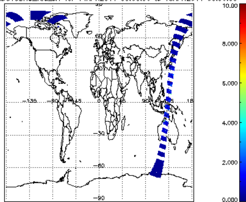
SCIOL2P_NADUV3BRO_vcd_err for 14APR2011 00:00:00 to 15APR2011 00:00:00
