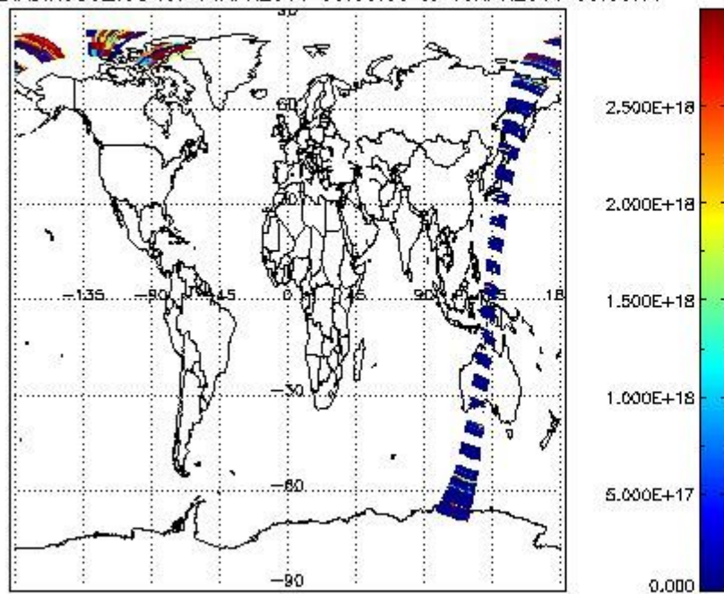
SCIDL2P_NADIR3CO_vcd for 14APR2011 00:00:00 to 15APR2011 00:00:00
