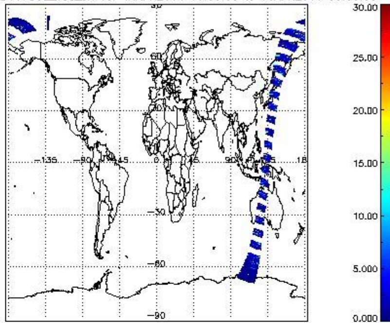
SCIOL2P_NADUV7S02_vcd_err for 14APR2011 00:00:00 to 15APR2011 00:00:00
