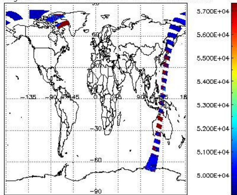
cloud_flags for 14APR2011 00:00:00 to 15APR2011 00:00:00
