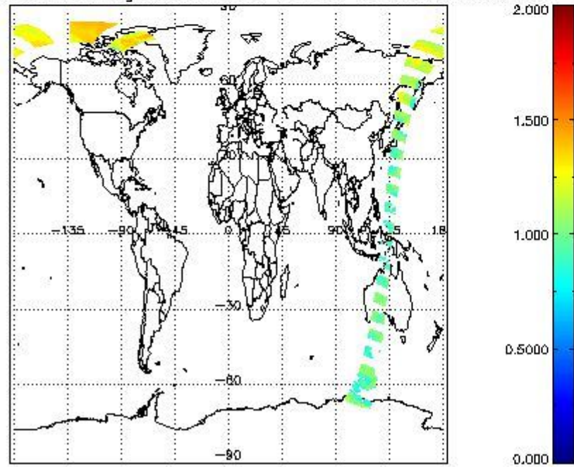
SCIOL2P_NADUV8H2O_arnf_gr for 14APR2011 00:00:00 to 15APR2011 00:00:00
