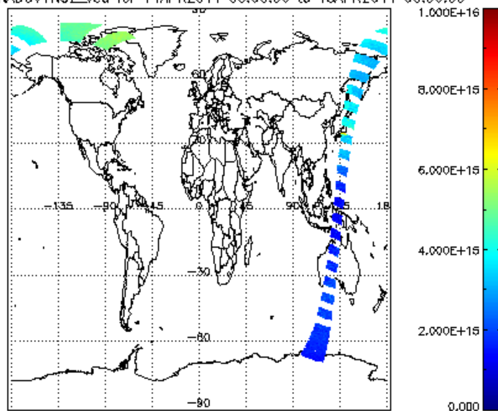
SCIOL2P_NADUV1NO2_vcd for 14APR2011 00:00:00 to 15APR2011 00:00:00
