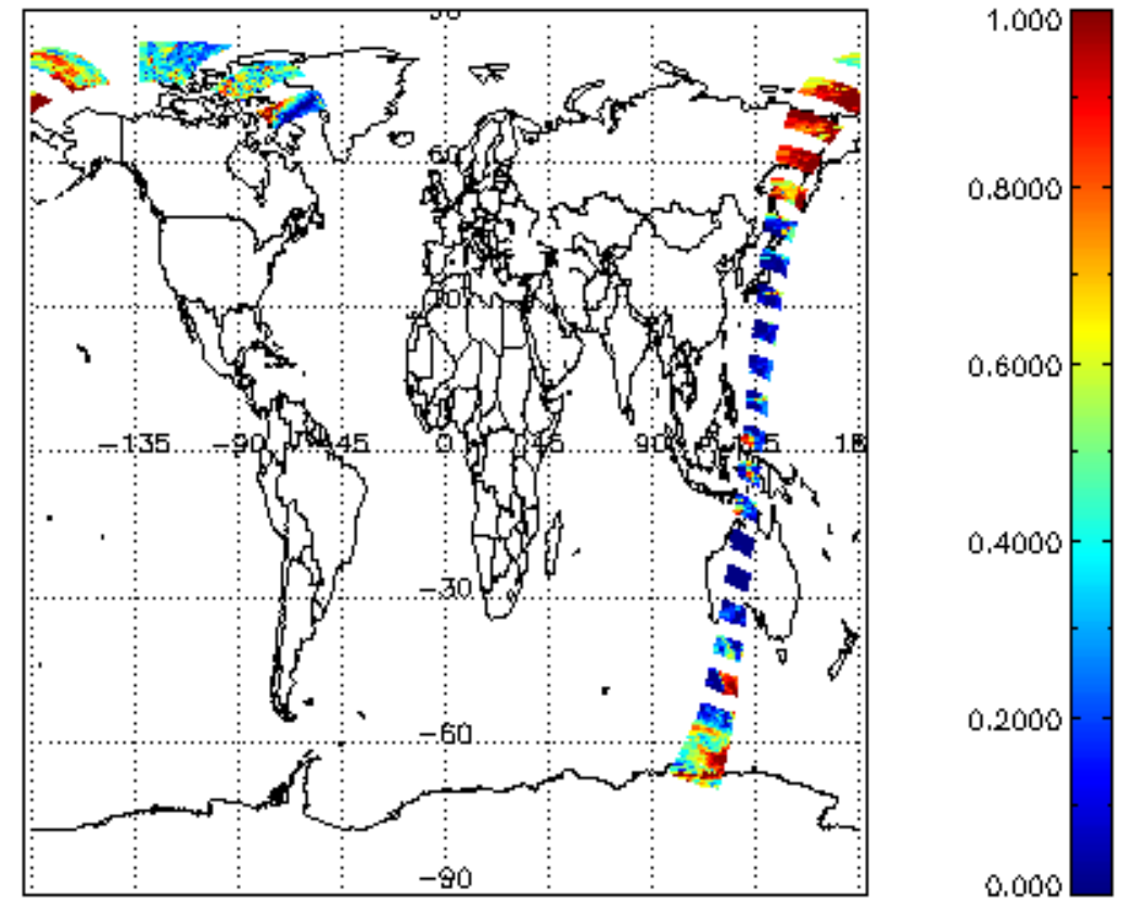
cl_frac for 14APR2011 00:00:00 to 15APR2011 00:00:00
