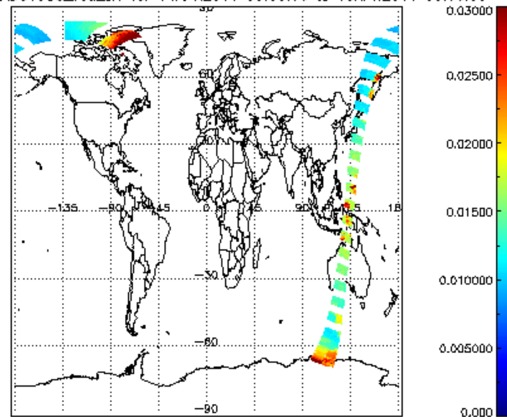
SCIOL2P_NADUV003_vcd_err for 14APR2011 00:00:00 to 15APR2011 00:00:00
