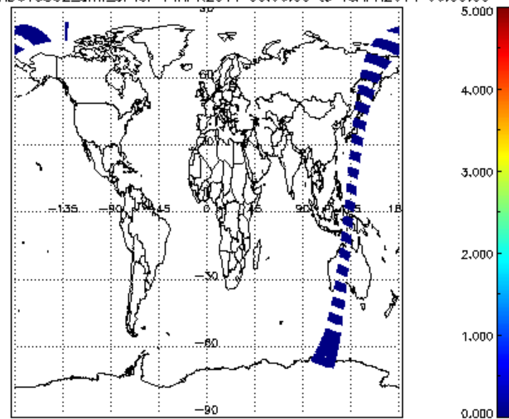
SCIOL2P_NADUV5S02_amf_cl for 14APR2011 00:00:00 to 15APR2011 00:00:00
