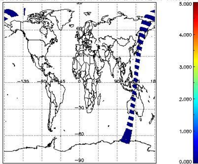
SCIOL2P_NADUV7S02_amf_cl for 14APR2011 00:00:00 to 15APR2011 00:00:00
