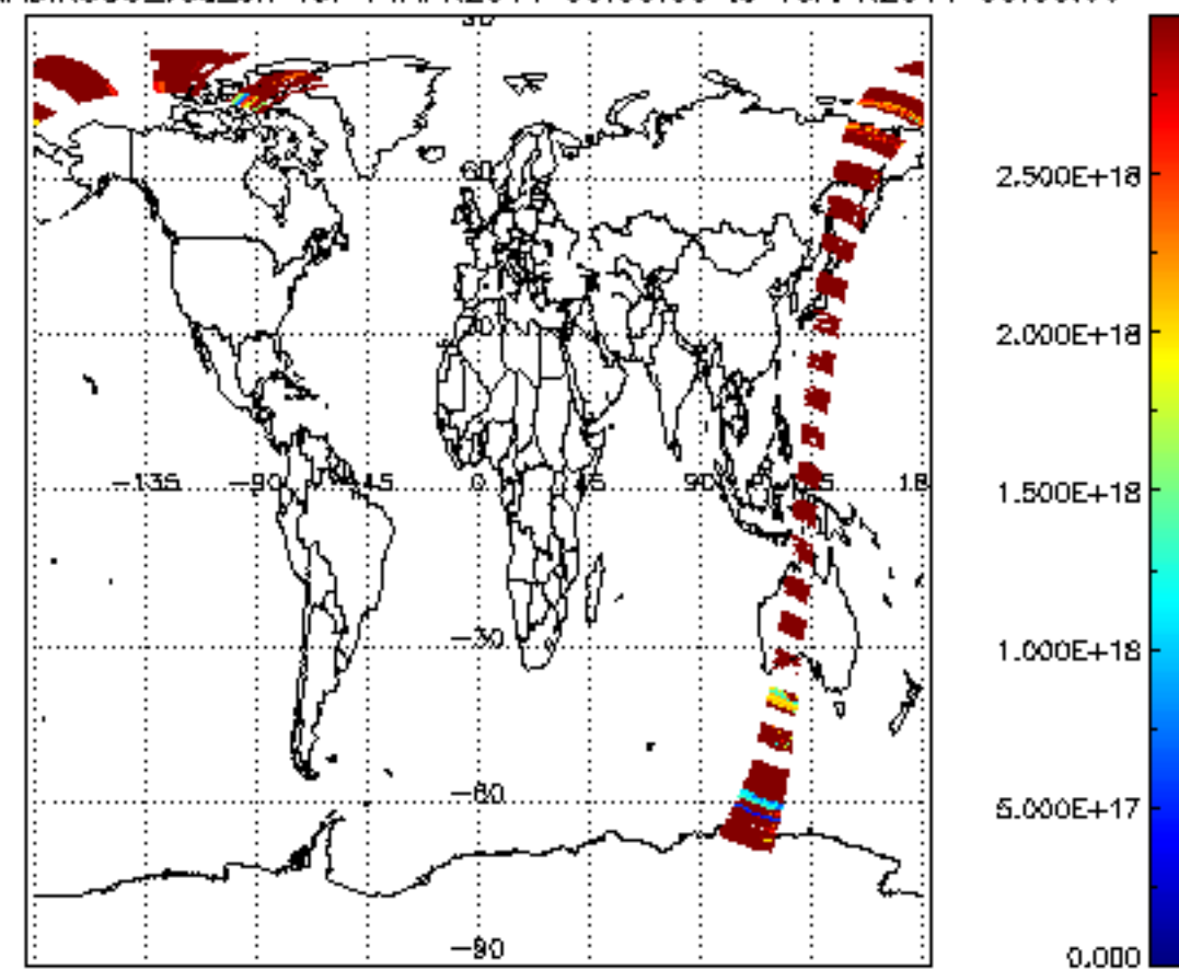
SCIOL2P_NADIR3CO_vcd_err for 14APR2011 00:00:00 to 15APR2011 00:00:00
