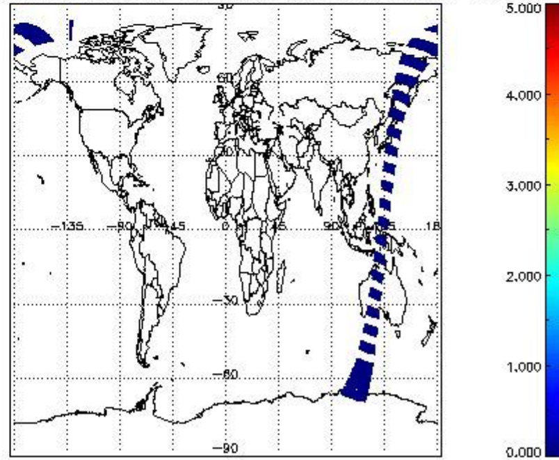
SCIOL2P_NADUV5S02_amf_cl for 14APR2011 00:00:00 to 15APR2011 00:00:00
