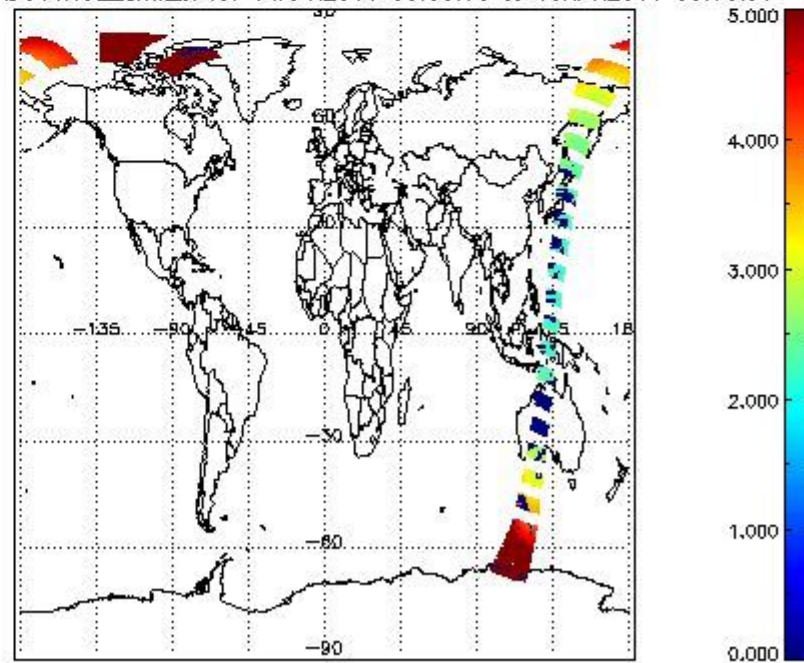
SCIOL2P_NADUV1NO2_amf_cl for 14APR2011 00:00:00 to 15APR2011 00:00:00
