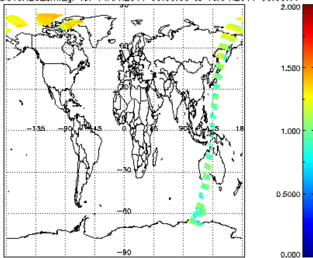
SCIOL2P_NADUV8H2O_amf_gr for 14APR2011 00:00:00 to 15APR2011 00:00:00
