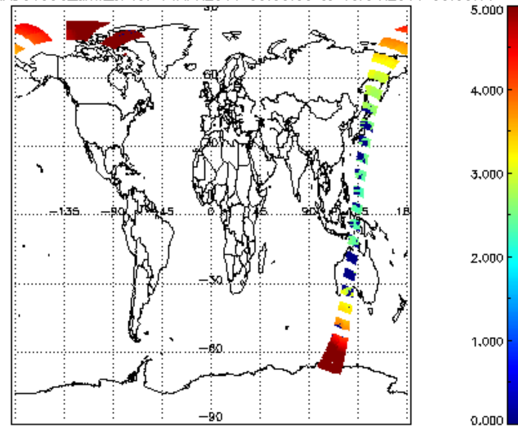
SCIOL2P_NADUV003_amf_cl for 14APR2011 00:00:00 to 15APR2011 00:00:00
