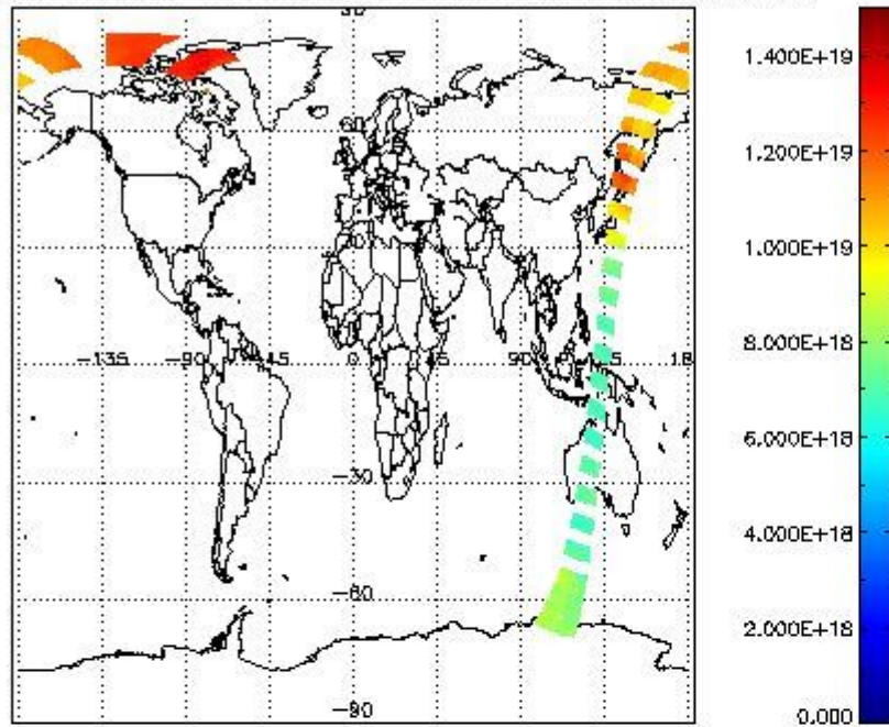
SCIOL2P_NADUV003_vcd for 14APR2011 00:00:00 to 15APR2011 00:00:00
