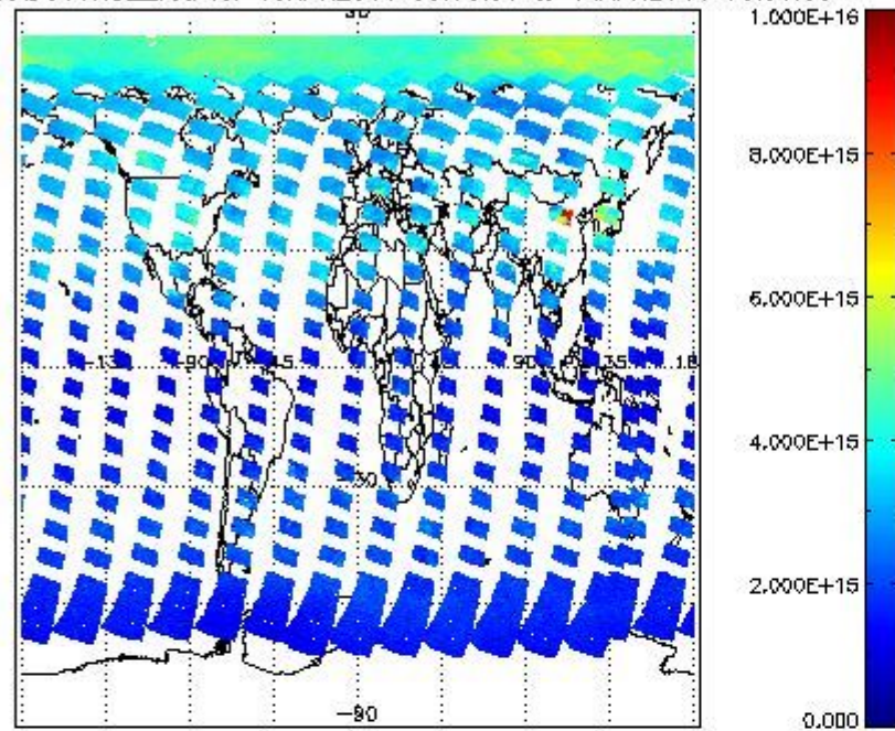
SCIOL2P_NADUV1NO2_vcd for 13APR2011 00:00:00 to 14APR2011 00:00:00
