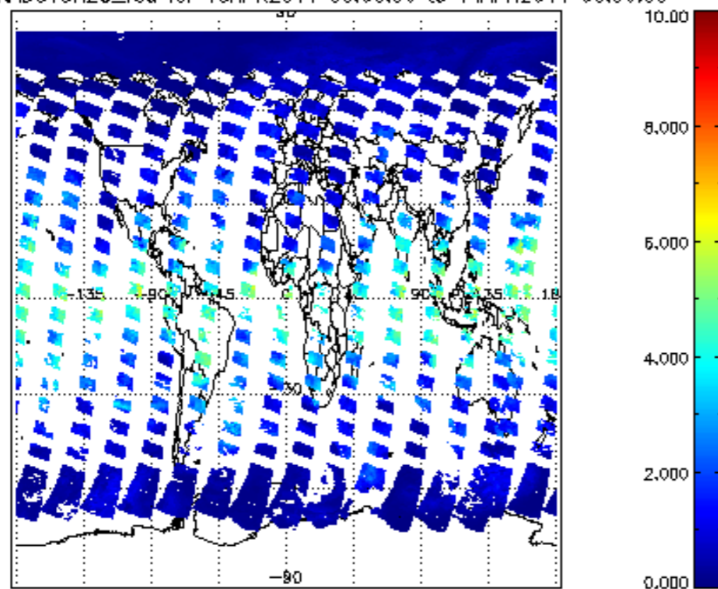
SCIOL2P_NADUV8H2O_vcd for 13APR2011 00:00:00 to 14APR2011 00:00:00
