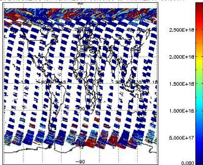
SCIDL2P_NADIR3CO_vcd for 13APR2011 00:00:00 to 14APR2011 00:00:00
