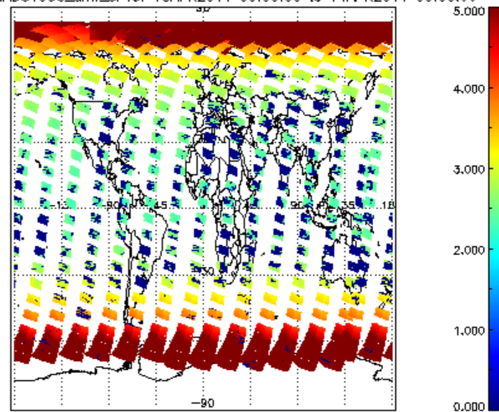
SCIOL2P_NADUV003_amf_cl for 13APR2011 00:00:00 to 14APR2011 00:00:00
