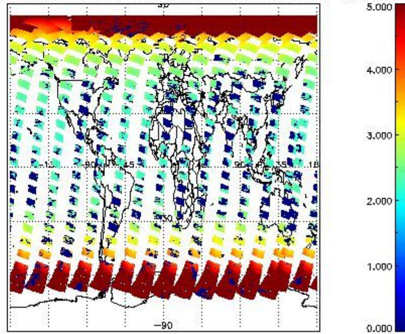
SCIOL2P_NADUV1NO2_amf_cl for 13APR2011 00:00:00 to 14APR2011 00:00:00
