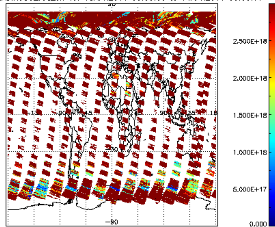
SCIOL2P_NADIR3CO_vcd_err for 13APR2011 00:00:00 to 14APR2011 00:00:00
