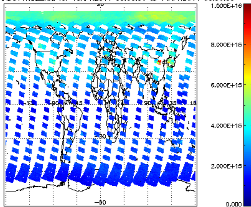
SCIOL2P_NADUV1NO2_vcd for 13APR2011 00:00:00 to 14APR2011 00:00:00
