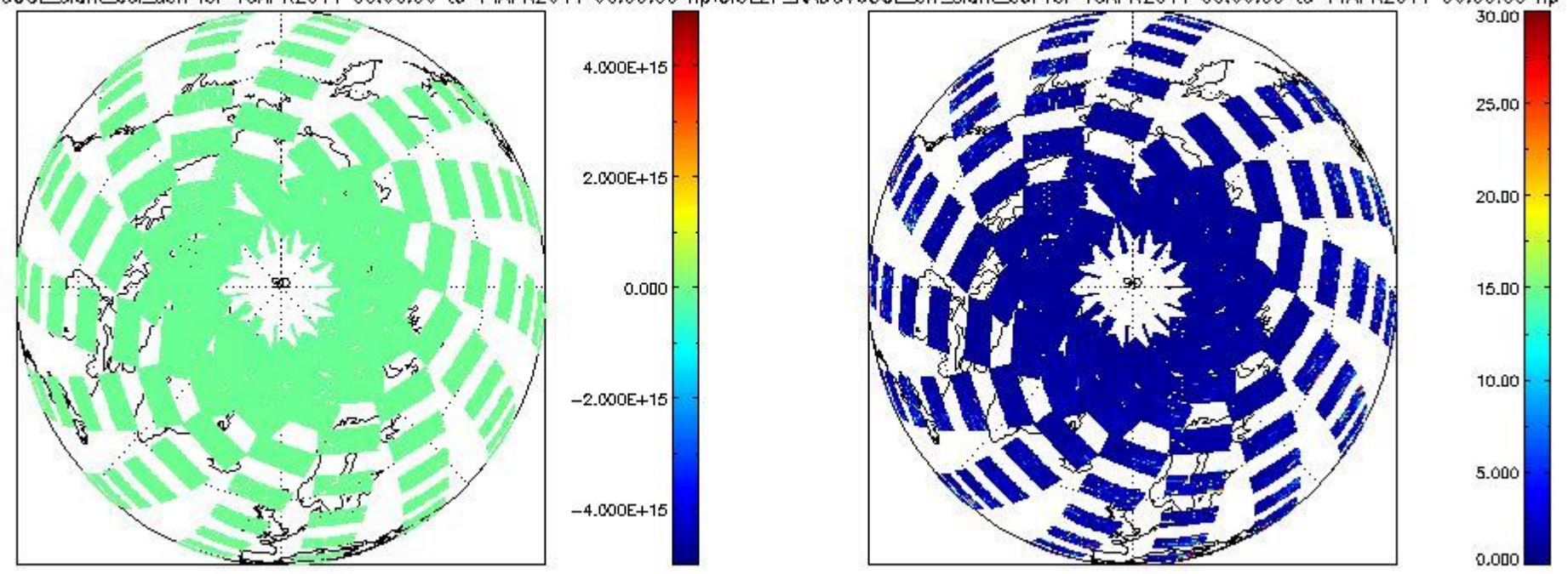
CIOL2P_NADUV60CLslant_col_den for 13APR2011 00:00:00 to 14APR2011 00:00:00 np; CIOL2P_NADUV60CLerr_slant_col for 13APR2011 00:00:00 to 14APR2011 00:00:00 np
