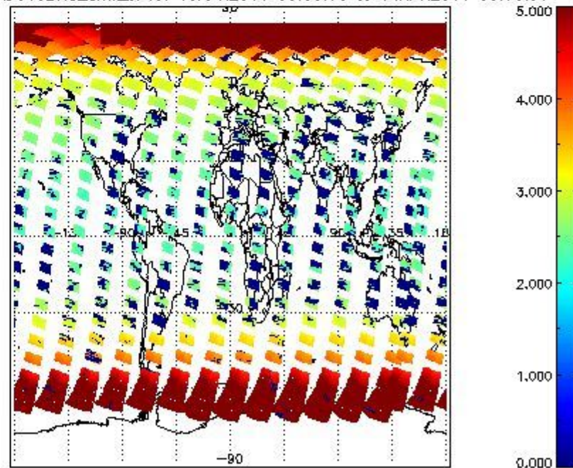
SCIOL2P_NADUV3BRO_amf_cl for 13APR2011 00:00:00 to 14APR2011 00:00:00
