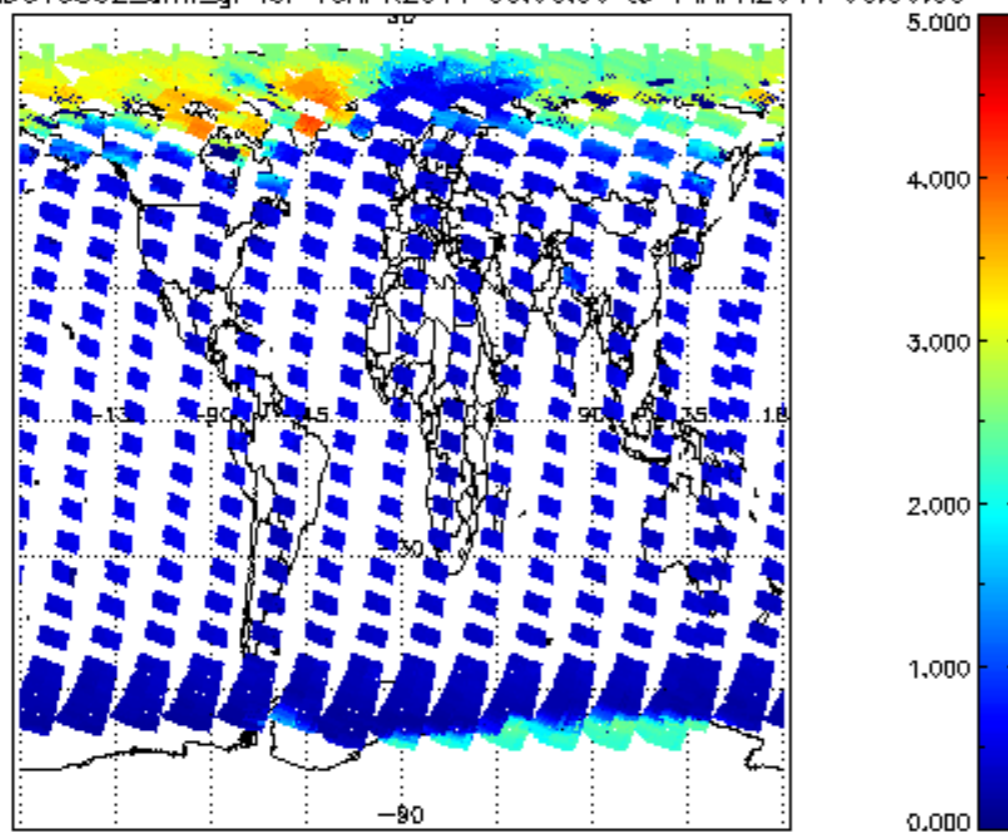
SCIOL2P_NADUV5S02_amf_gr for 13APR2011 00:00:00 to 14APR2011 00:00:00
