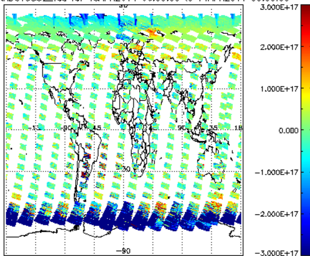
SCIOL2P_NADUV5S02_vcd for 13APR2011 00:00:00 to 14APR2011 00:00:00
