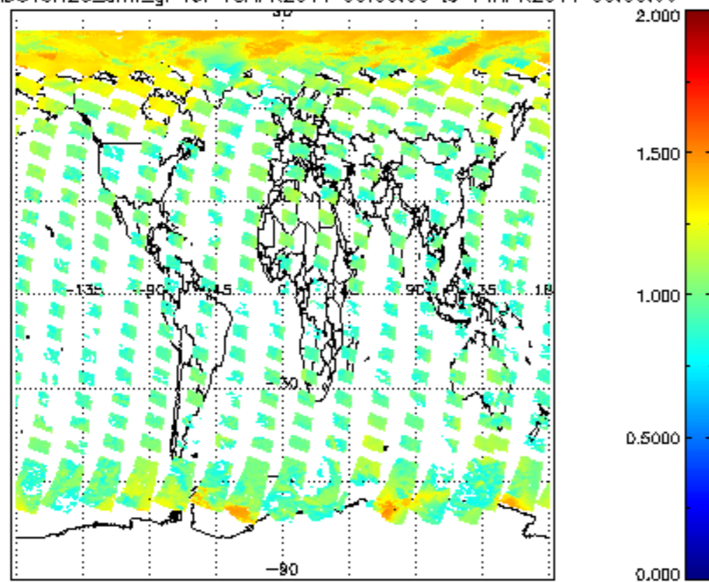
SCIOL2P_NADUV8H2O_amf_gr for 13APR2011 00:00:00 to 14APR2011 00:00:00
