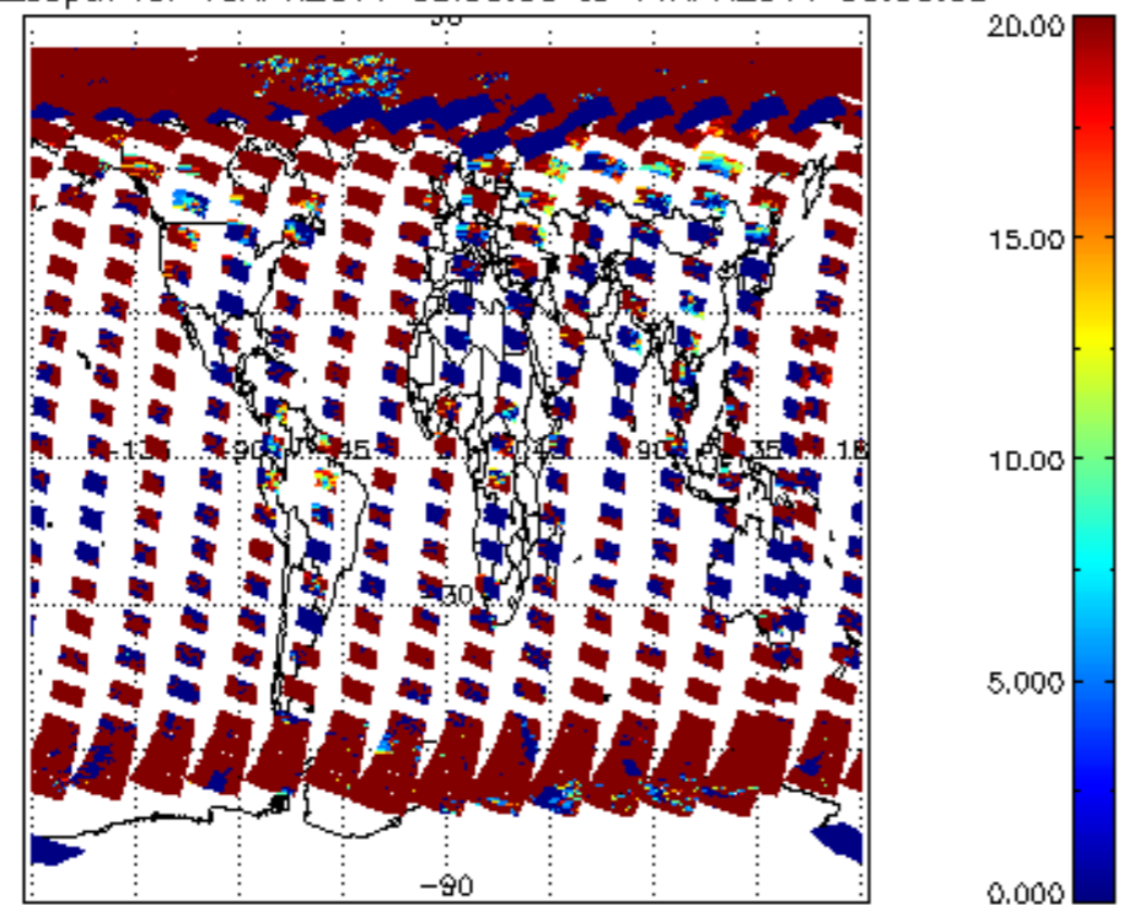
cl_opt_depth for 13APR2011 00:00:00 to 14APR2011 00:00:00
