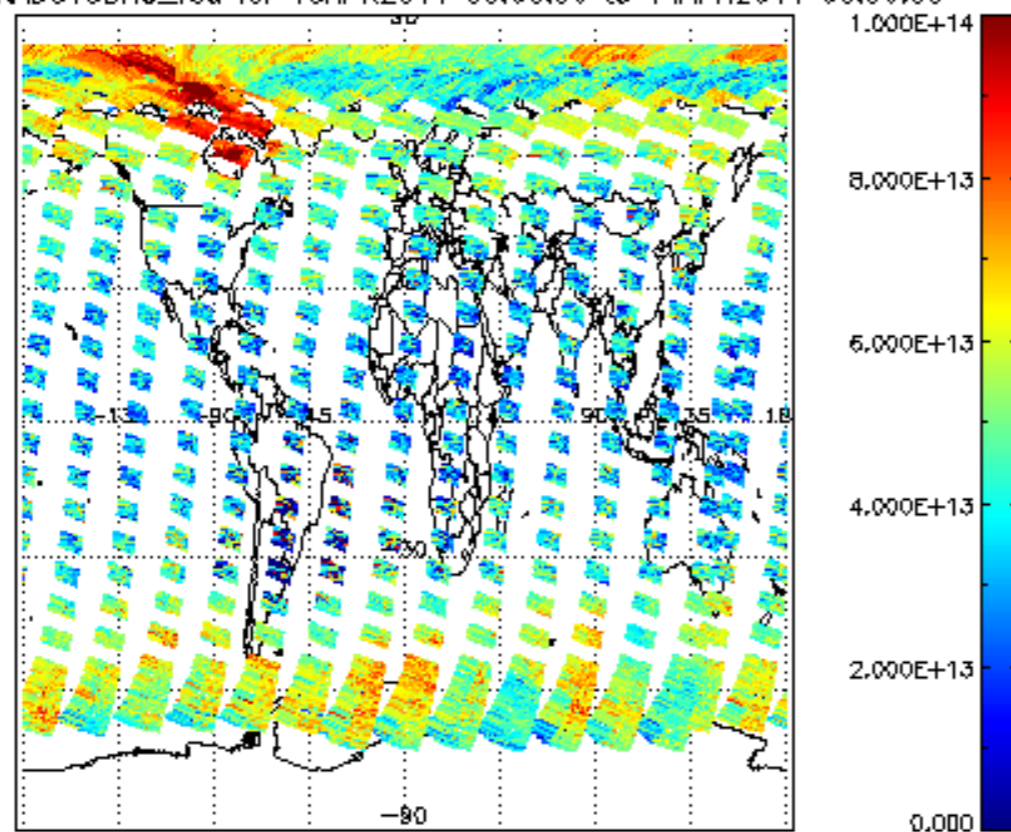
SCIOL2P_NADUV3BRO_vcd for 13APR2011 00:00:00 to 14APR2011 00:00:00
