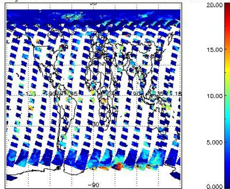
cL_top_height for 13APR2011 00:00:00 to 14APR2011 00:00:00
