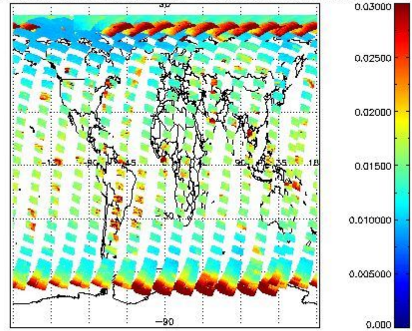
SCIOL2P_NADUV003_vcd_err for 13APR2011 00:00:00 to 14APR2011 00:00:00
