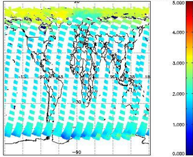
SCIOL2P_NADUV7S02_amf_gr for 13APR2011 00:00:00 to 14APR2011 00:00:00
