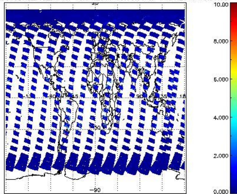
SCIOL2P_NADUV3BRO_vcd_err for 13APR2011 00:00:00 to 14APR2011 00:00:00
