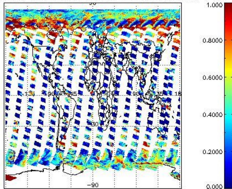
cL_frac for 13APR2011 00:00:00 to 14APR2011 00:00:00
