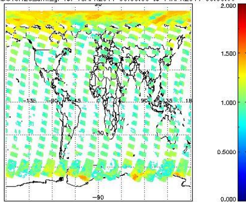
SCIOL2P_NADUV8H2O_arnf_gr for 13APR2011 00:00:00 to 14APR2011 00:00:00
