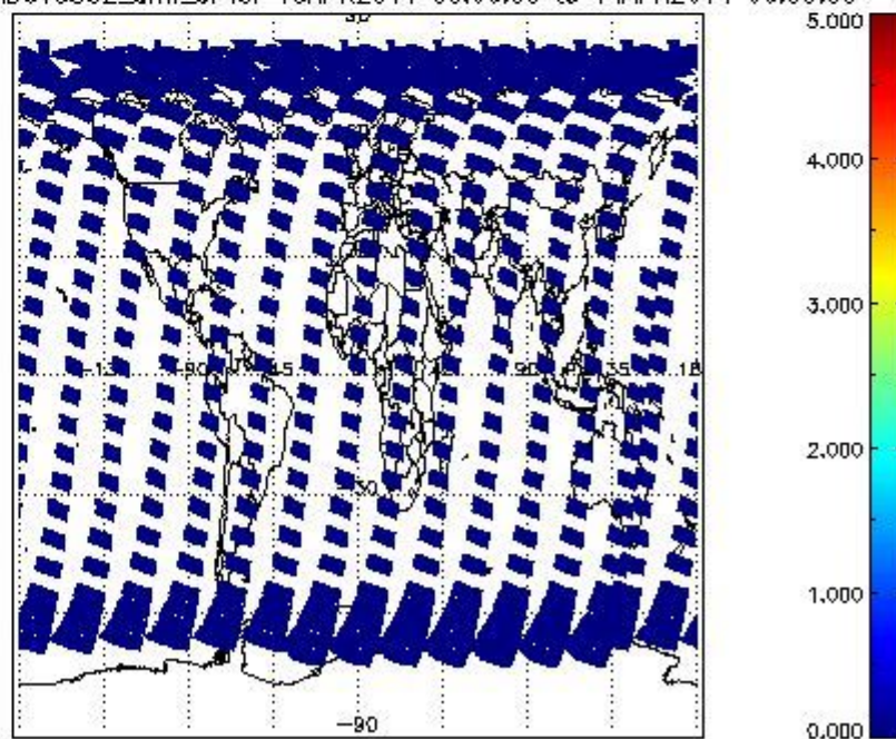
SCIOL2P_NADUV5S02_amf_cl for 13APR2011 00:00:00 to 14APR2011 00:00:00
