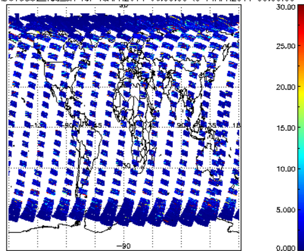
SCIOL2P_NADUV5S02_vcd_err for 13APR2011 00:00:00 to 14APR2011 00:00:00
