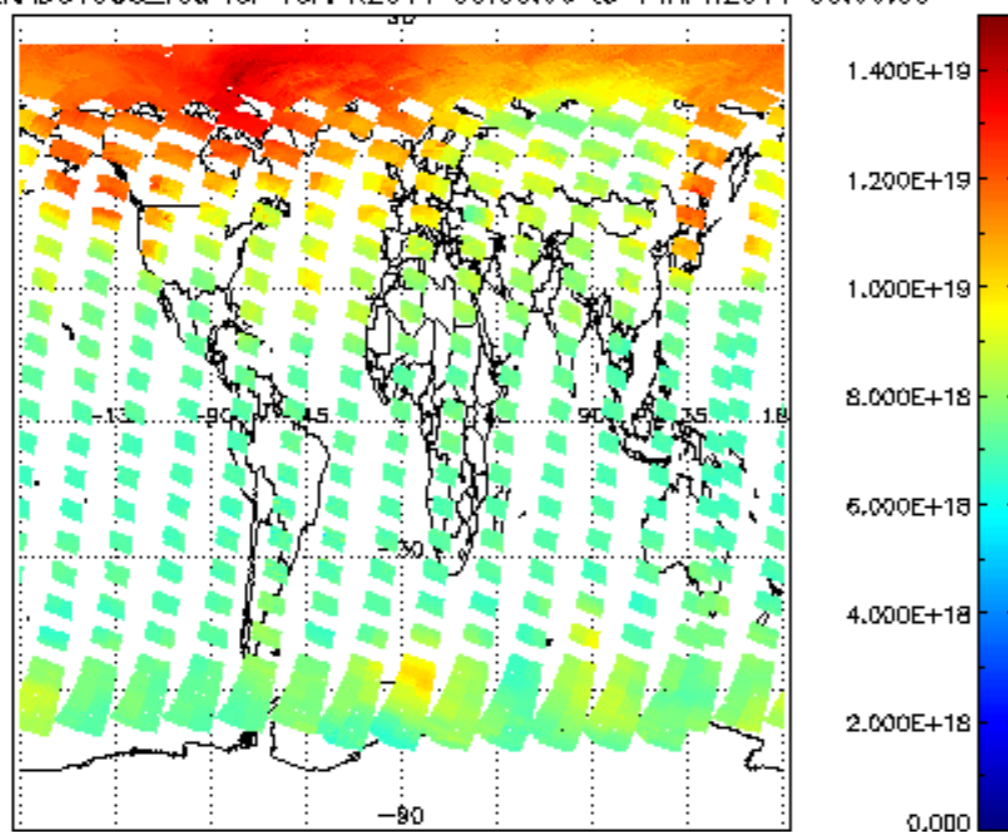
SCIOL2P_NADUV003_vcd for 13APR2011 00:00:00 to 14APR2011 00:00:00
