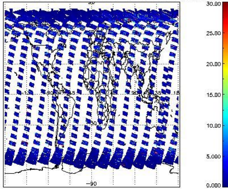
SCIOL2P_NADUV7S02_vcd_err for 13APR2011 00:00:00 to 14APR2011 00:00:00
