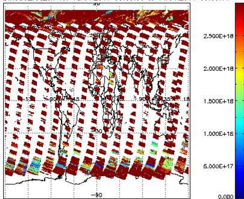
SCIDL2P_NADIR3CO_vcd_err for 13APR2011 00:00:00 to 14APR2011 00:00:00
