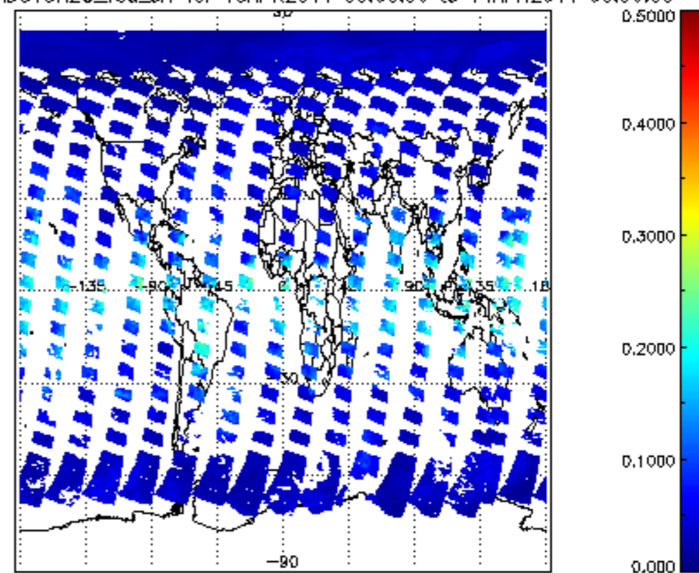
SCIOL2P_NADUV8H2O_vcd_err for 13APR2011 00:00:00 to 14APR2011 00:00:00
