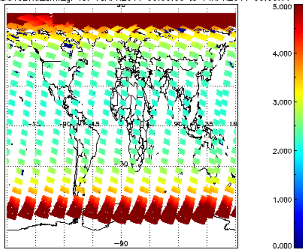
SCIOL2P_NADUV3BRO_amf_gr for 13APR2011 00:00:00 to 14APR2011 00:00:00
