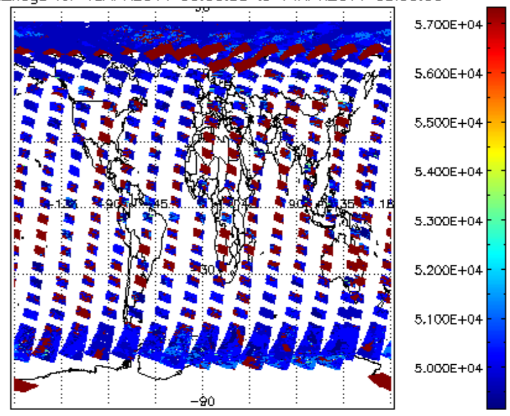
cloud_flags for 13APR2011 00:00:00 to 14APR2011 00:00:00
