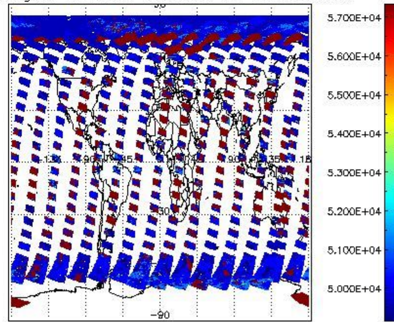
cloud_flags for 13APR2011 00:00:00 to 14APR2011 00:00:00
