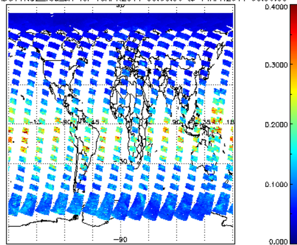
SCIOL2P_NADUV1NO2_vcd_err for 13APR2011 00:00:00 to 14APR2011 00:00:00
