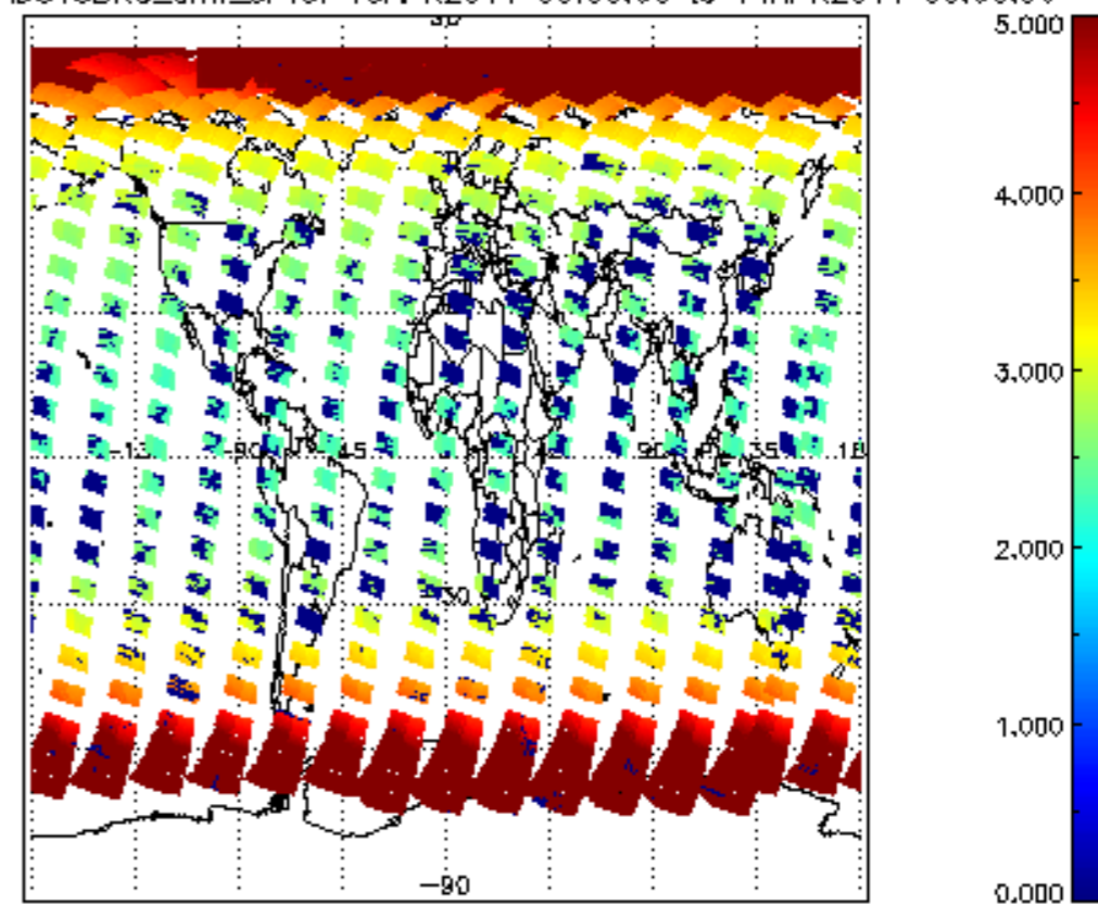
SCIOL2P_NADUV3BRO_amf_sl for 13APR2011 00:00:00 to 14APR2011 00:00:00
