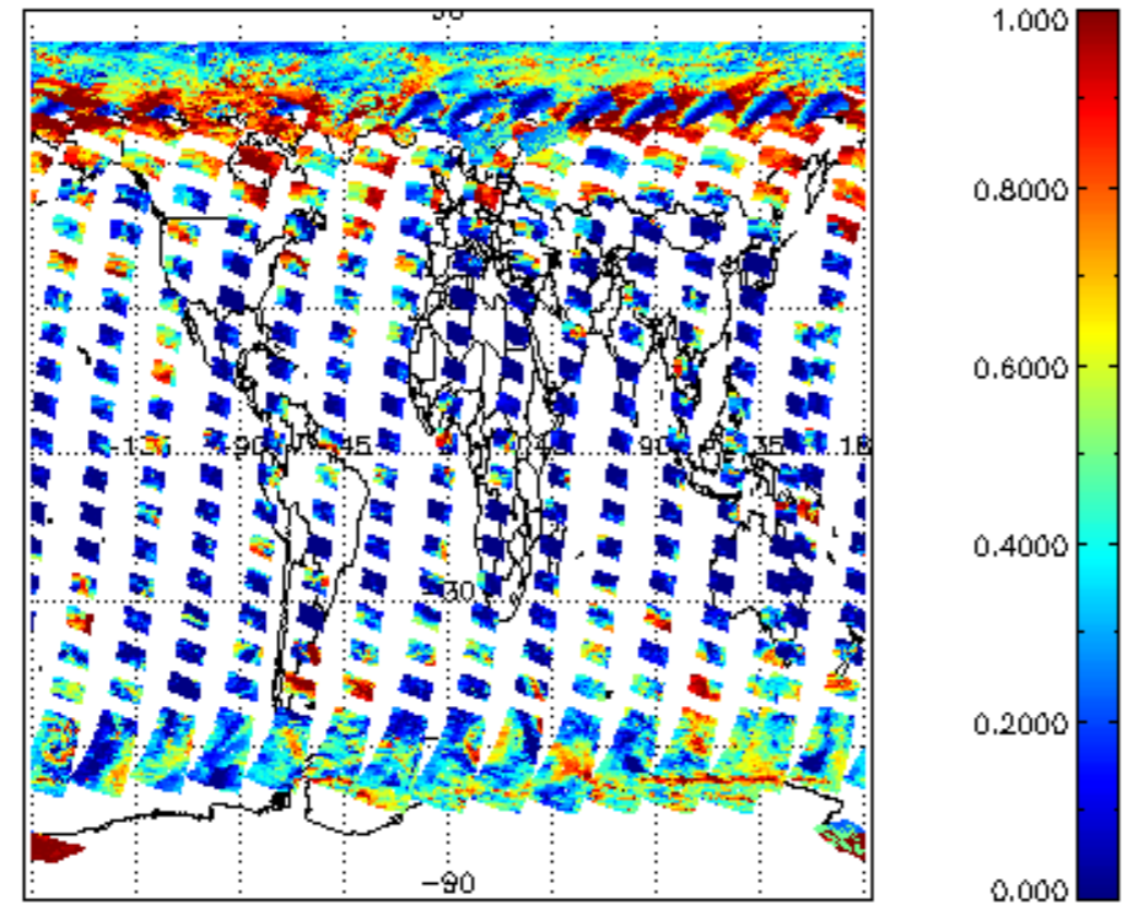
cl_frac for 13APR2011 00:00:00 to 14APR2011 00:00:00
