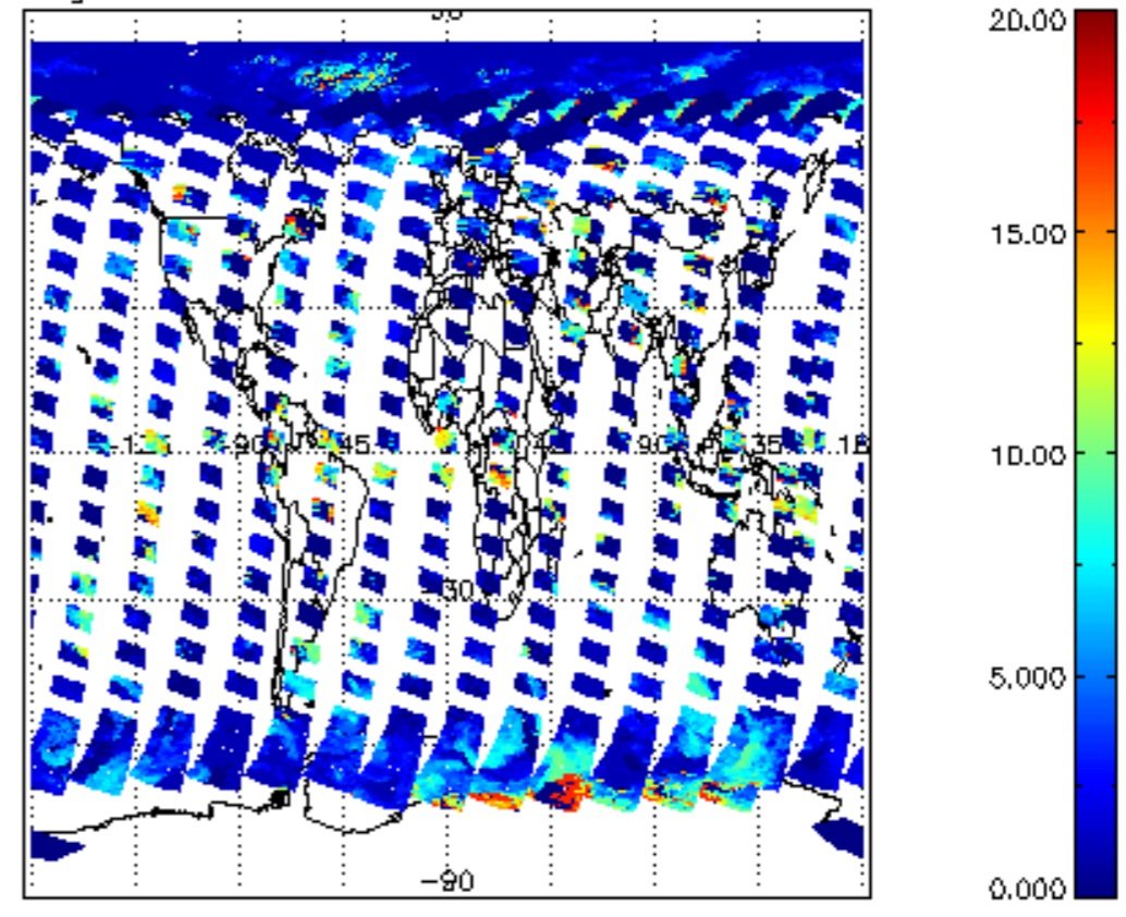
cl_top_height for 13APR2011 00:00:00 to 14APR2011 00:00:00
