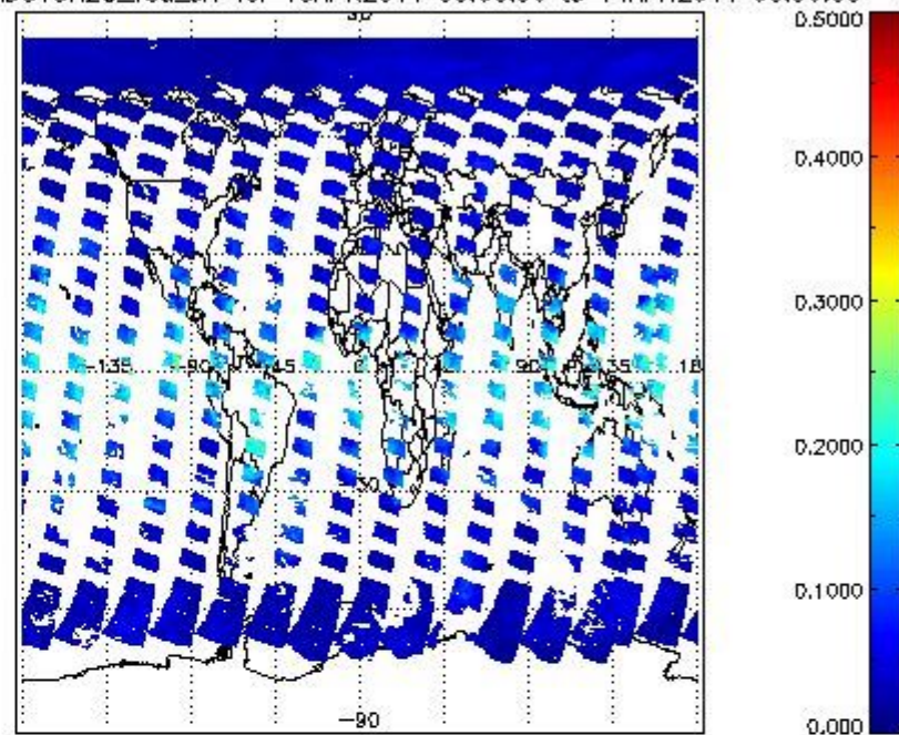
SCIOL2P_NADUV8H2O_vcd_err for 13APR2011 00:00:00 to 14APR2011 00:00:00
