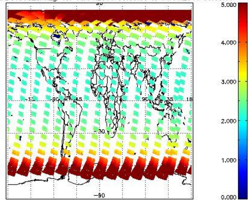
SCIOL2P_NADUV003_amf_gr for 13APR2011 00:00:00 to 14APR2011 00:00:00
