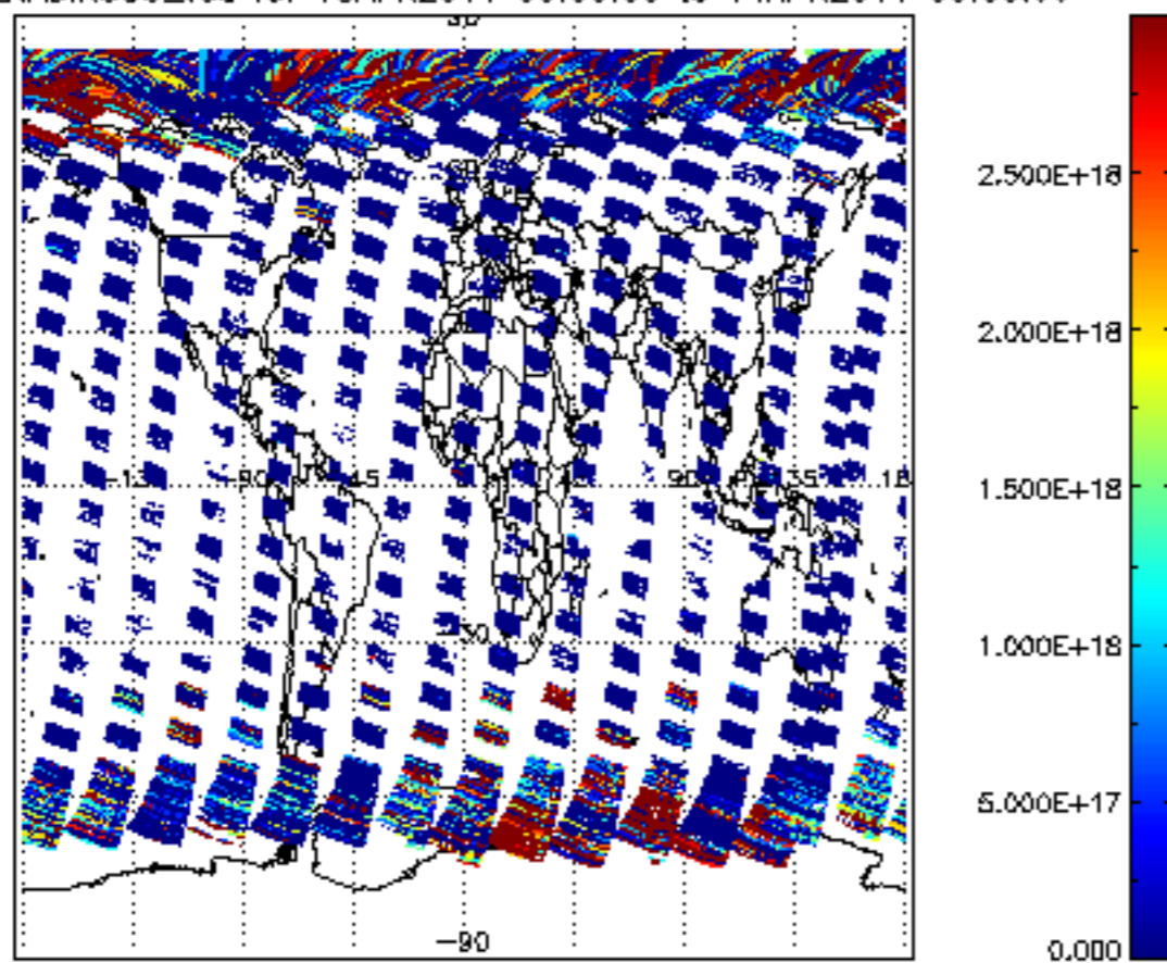
SCIOL2P_NADIR3CO_vcd for 13APR2011 00:00:00 to 14APR2011 00:00:00
