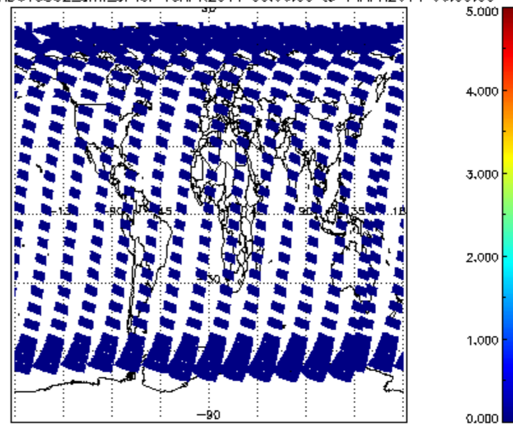
SCIOL2P_NADUV5S02_amf_cl for 13APR2011 00:00:00 to 14APR2011 00:00:00
