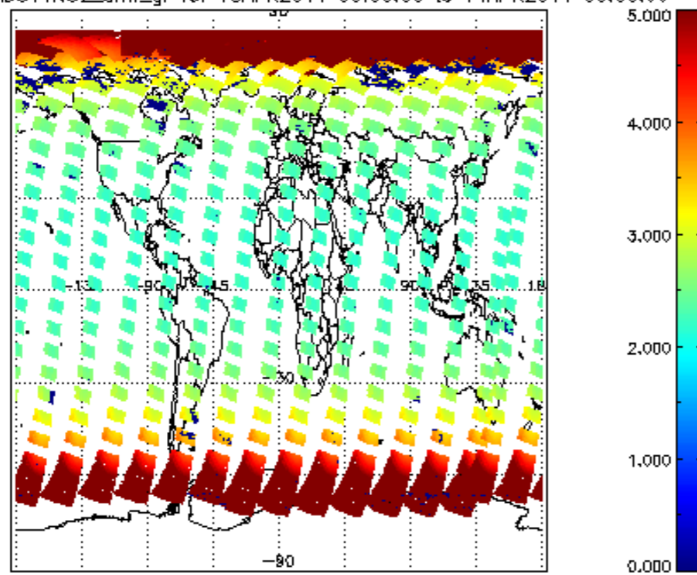
SCIOL2P_NADUV1NO2_amf_gr for 13APR2011 00:00:00 to 14APR2011 00:00:00
