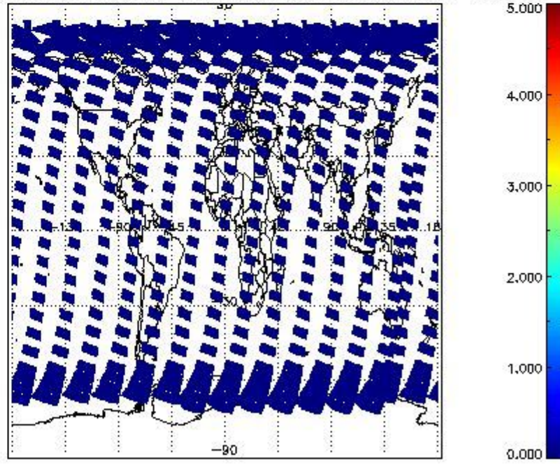
SCIOL2P_NADUV7S02_amf_cl for 13APR2011 00:00:00 to 14APR2011 00:00:00
