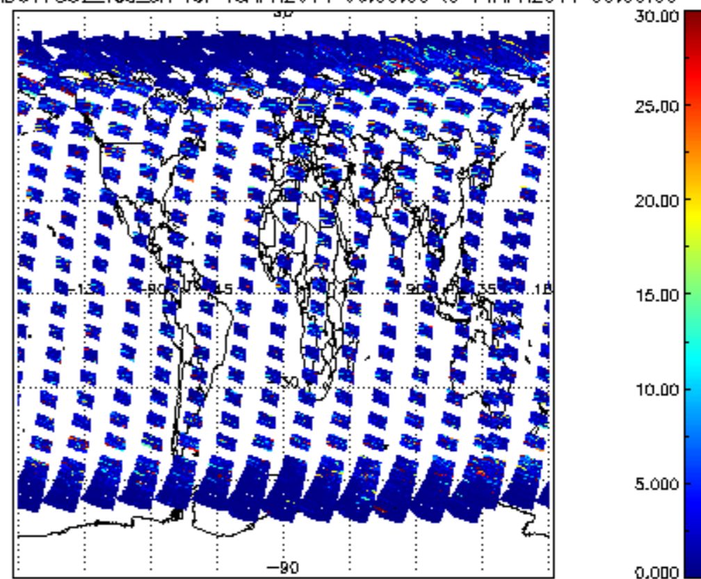
SCIOL2P_NADUV7S02_vcd_err for 13APR2011 00:00:00 to 14APR2011 00:00:00
