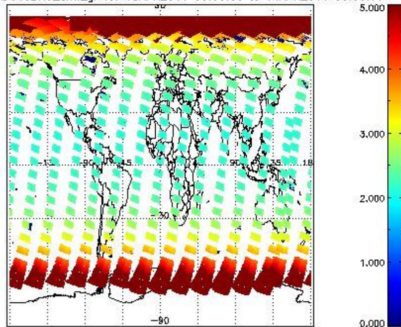
SCIOL2P_NADUV3BRO_amf_gr for 13APR2011 00:00:00 to 14APR2011 00:00:00
