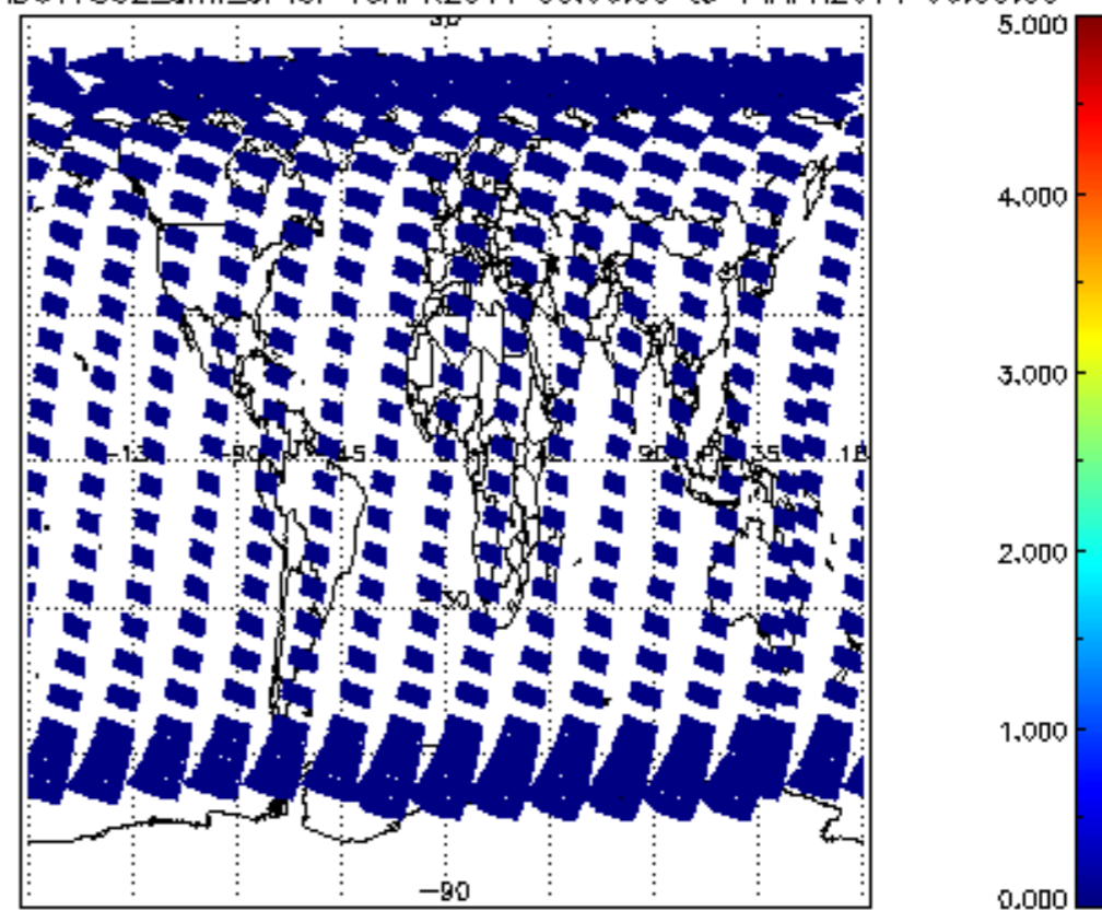
SCIOL2P_NADUV7S02_amf_cl for 13APR2011 00:00:00 to 14APR2011 00:00:00
