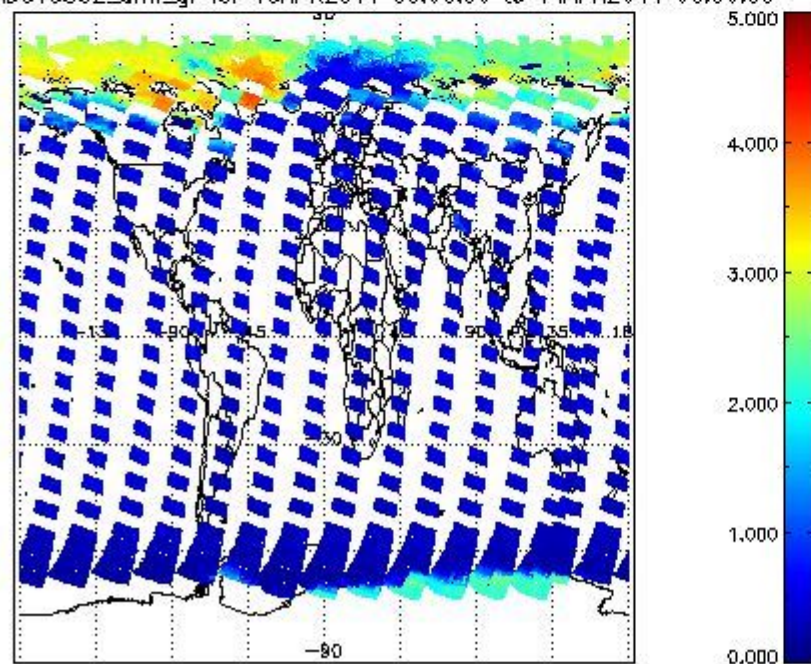
SCIOL2P_NADUV5S02_amf_gr for 13APR2011 00:00:00 to 14APR2011 00:00:00
