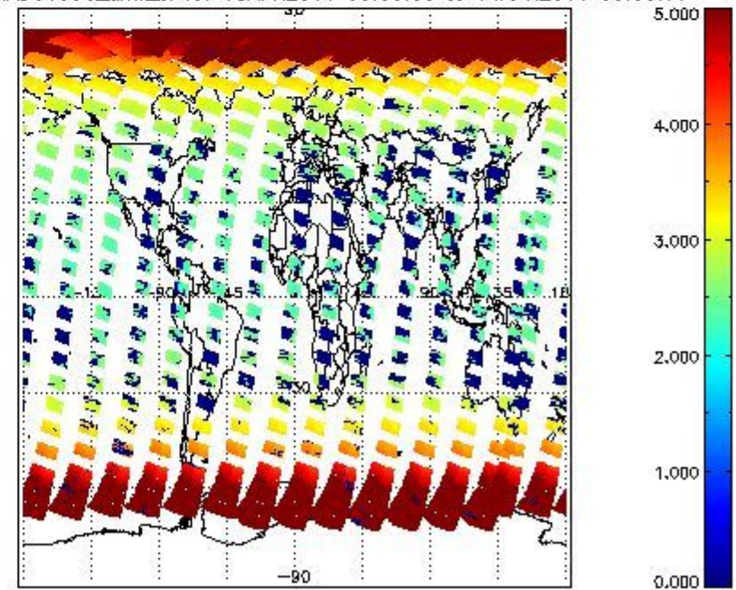
SCIOL2P_NADUV003_amf_cl for 13APR2011 00:00:00 to 14APR2011 00:00:00
