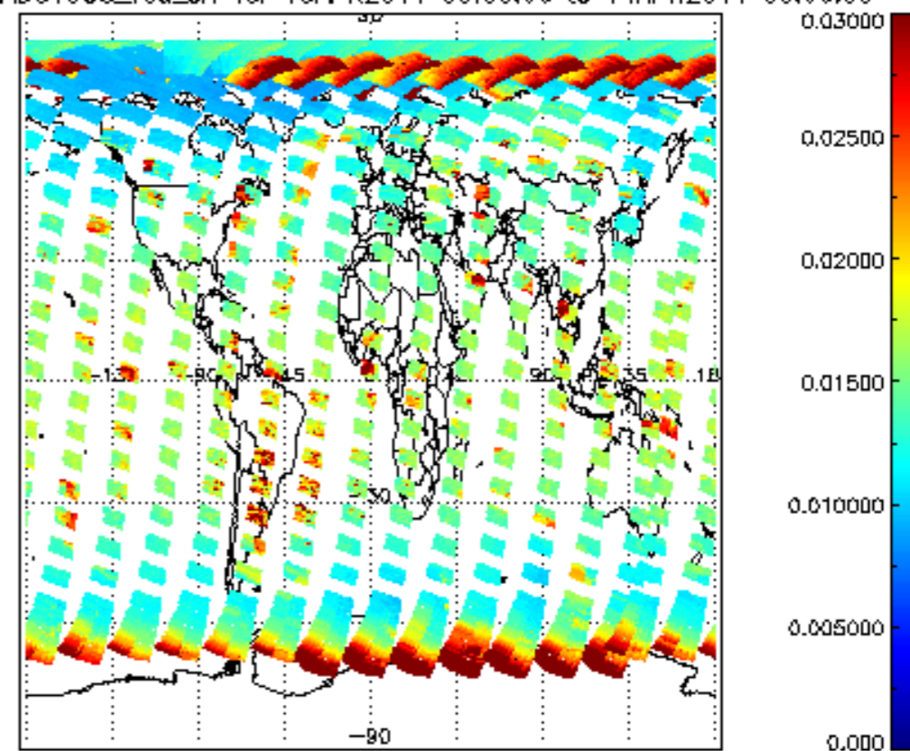
SCIOL2P_NADUV003_vcd_err for 13APR2011 00:00:00 to 14APR2011 00:00:00
