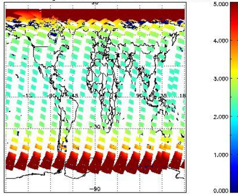
SCIOL2P_NADUV1NO2_amf_gr for 13APR2011 00:00:00 to 14APR2011 00:00:00
