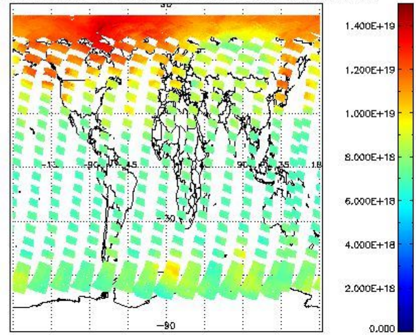
SCIOL2P_NADUV003_vcd for 13APR2011 00:00:00 to 14APR2011 00:00:00
