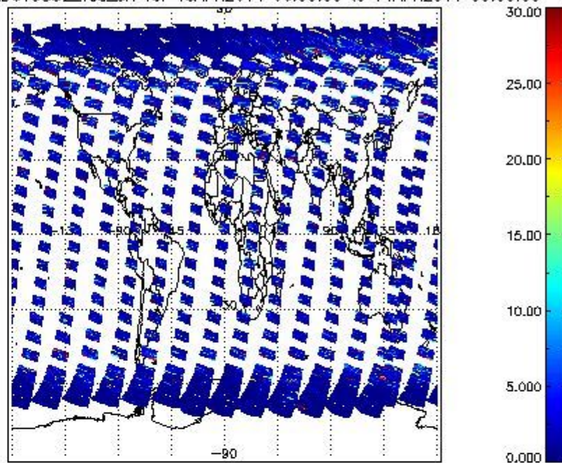
SCIOL2P_NADUV5S02_vcd_err for 13APR2011 00:00:00 to 14APR2011 00:00:00
