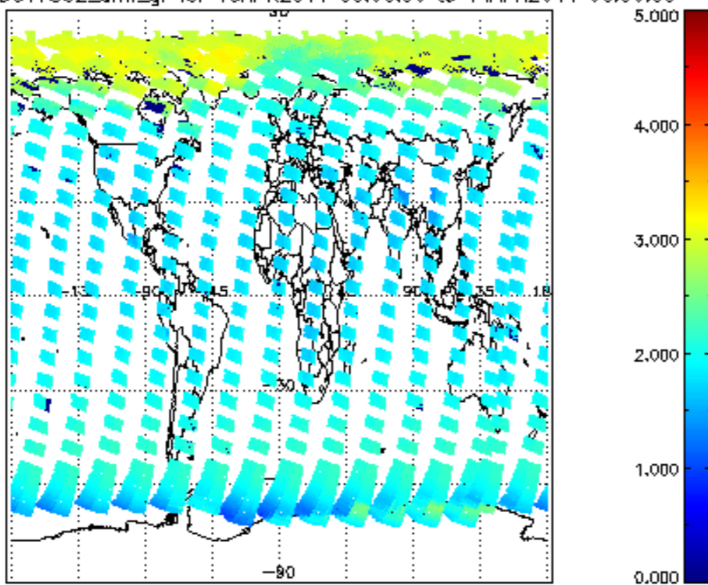
SCIOL2P_NADUV7S02_amf_gr for 13APR2011 00:00:00 to 14APR2011 00:00:00
