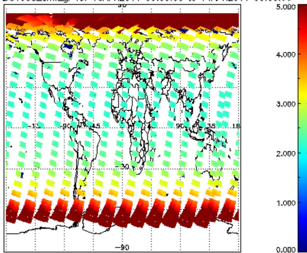
SCIOL2P_NADUV003_amf_gr for 13APR2011 00:00:00 to 14APR2011 00:00:00
