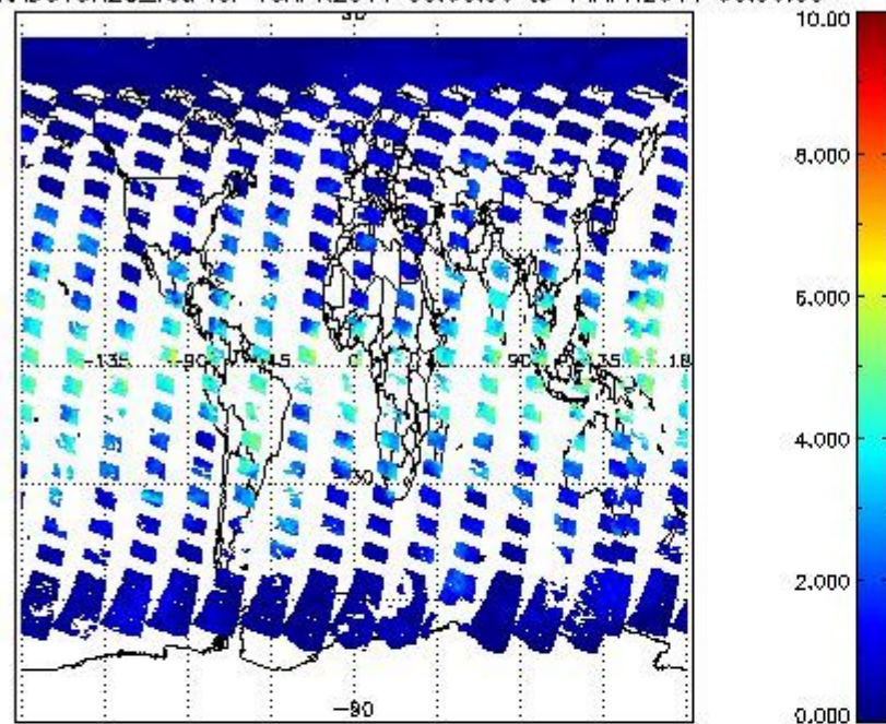
SCIOL2P_NADUV8H2O_vcd for 13APR2011 00:00:00 to 14APR2011 00:00:00
