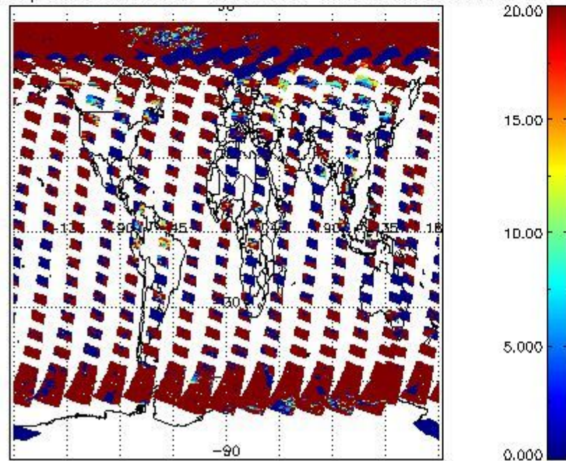
cL_opt_depth for 13APR2011 00:00:00 to 14APR2011 00:00:00
