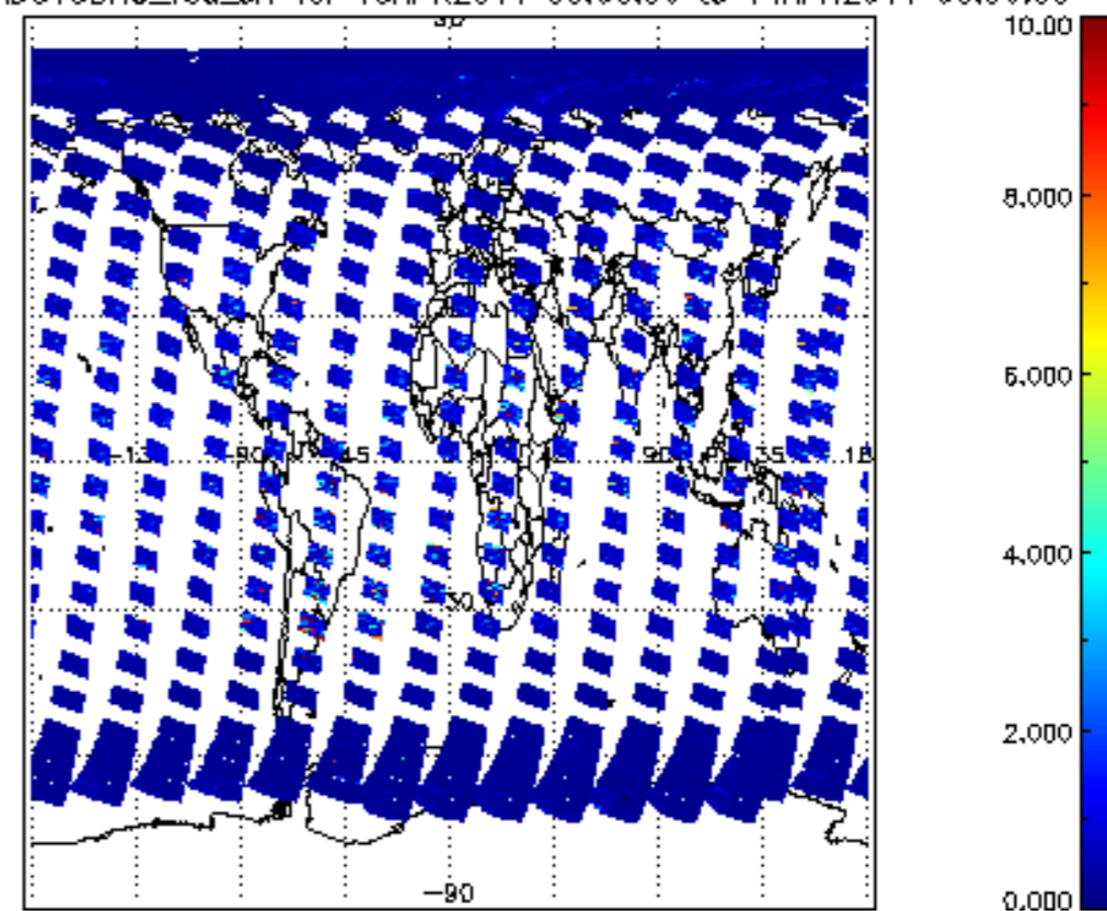
SCIOL2P_NADUV3BRO_vcd_err for 13APR2011 00:00:00 to 14APR2011 00:00:00
