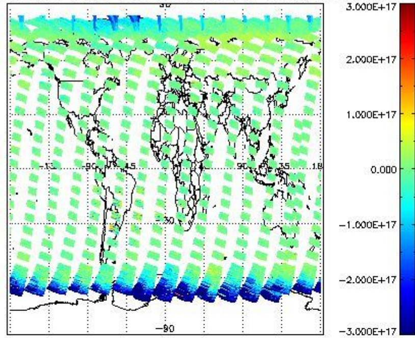
SCIOL2P_NADUV7S02_vcd for 13APR2011 00:00:00 to 14APR2011 00:00:00
