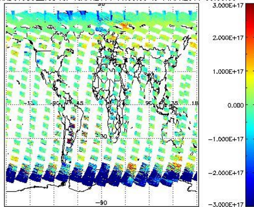
SCIOL2P_NADUV5S02_vcd for 13APR2011 00:00:00 to 14APR2011 00:00:00
