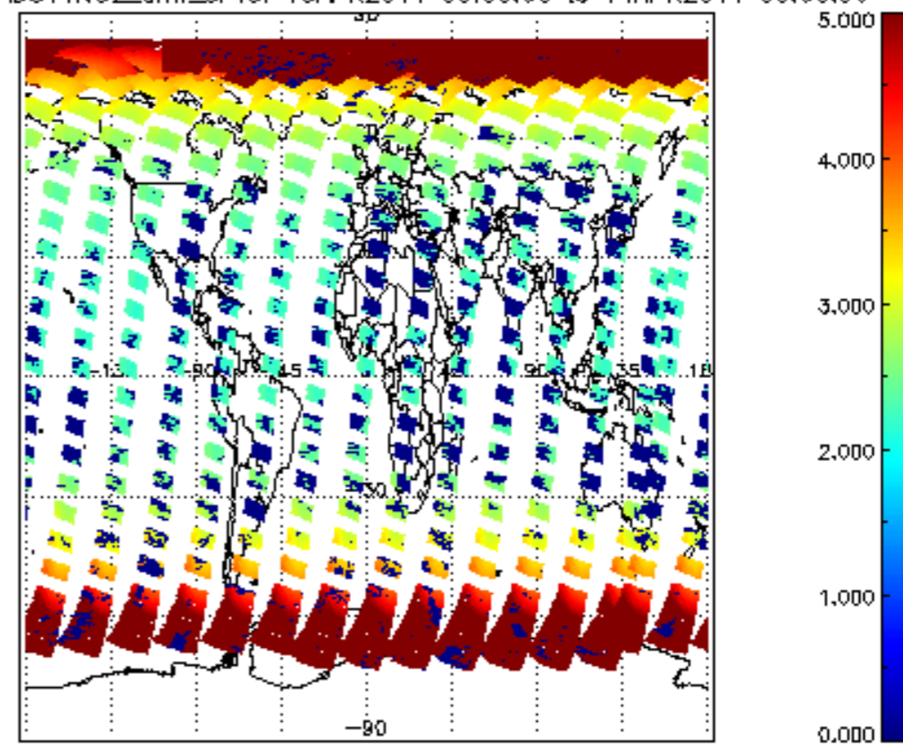
SCIOL2P_NADUV1NO2_amf_sl for 13APR2011 00:00:00 to 14APR2011 00:00:00
