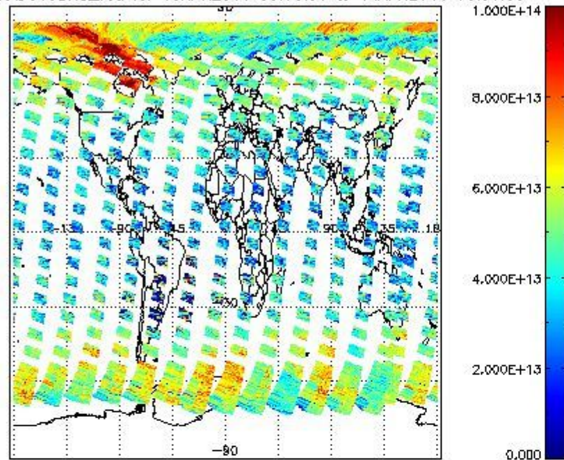
SCIOL2P_NADUV3BRO_vcd for 13APR2011 00:00:00 to 14APR2011 00:00:00
