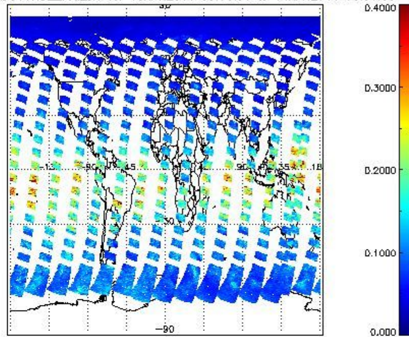
SCIOL2P_NADUV1NO2_vcd_err for 13APR2011 00:00:00 to 14APR2011 00:00:00
