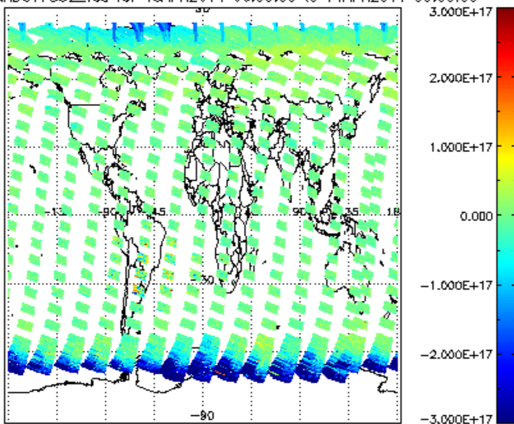
SCIOL2P_NADUV7S02_vcd for 13APR2011 00:00:00 to 14APR2011 00:00:00
