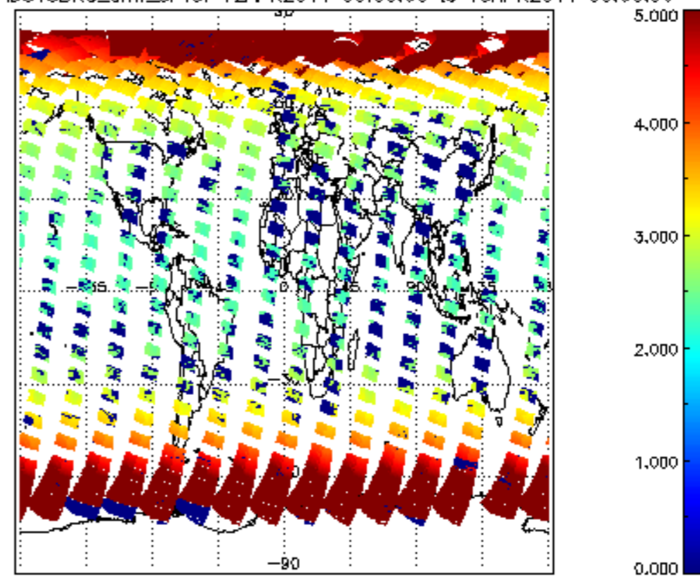
SCIOL2P_NADUV3BRO_amf_sl for 12APR2011 00:00:00 to 13APR2011 00:00:00
