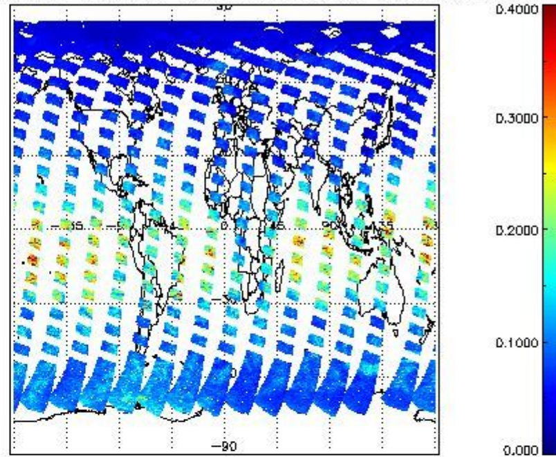
SCIOL2P_NADUV1NO2_vcd_err for 12APR2011 00:00:00 to 13APR2011 00:00:00
