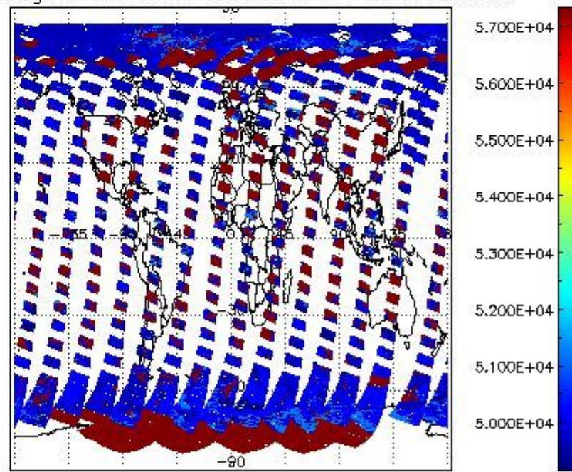
cloud_flags for 12APR2011 00:00:00 to 13APR2011 00:00:00
