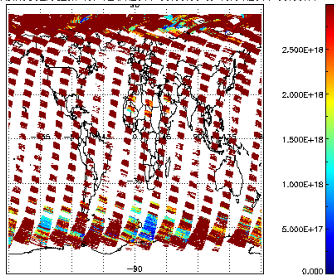
SCIOL2P_NADIR3CO_vcd_err for 12APR2011 00:00:00 to 13APR2011 00:00:00
