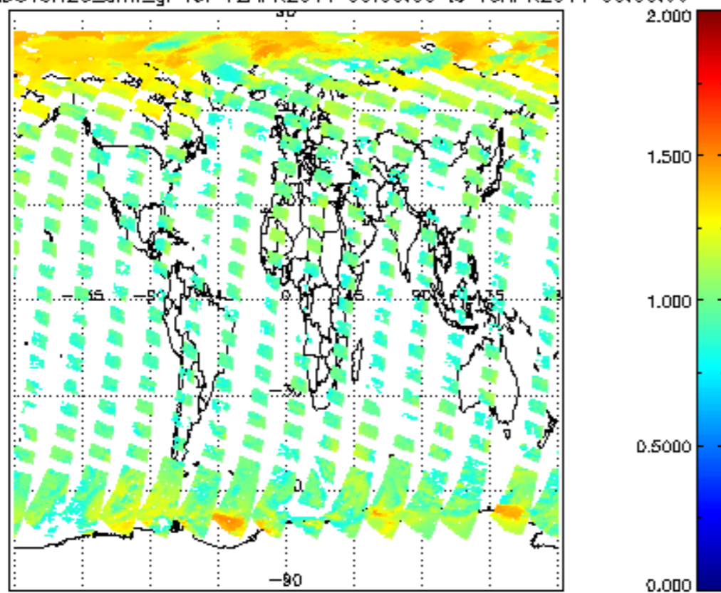
SCIOL2P_NADUV8H2O_amf_gr for 12APR2011 00:00:00 to 13APR2011 00:00:00
