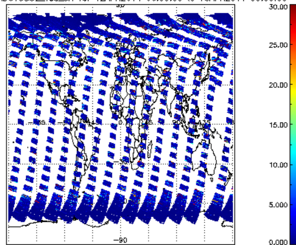
SCIOL2P_NADUV5S02_vcd_err for 12APR2011 00:00:00 to 13APR2011 00:00:00
