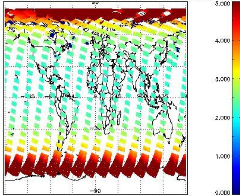
SCIOL2P_NADUV3BRO_amf_gr for 12APR2011 00:00:00 to 13APR2011 00:00:00
