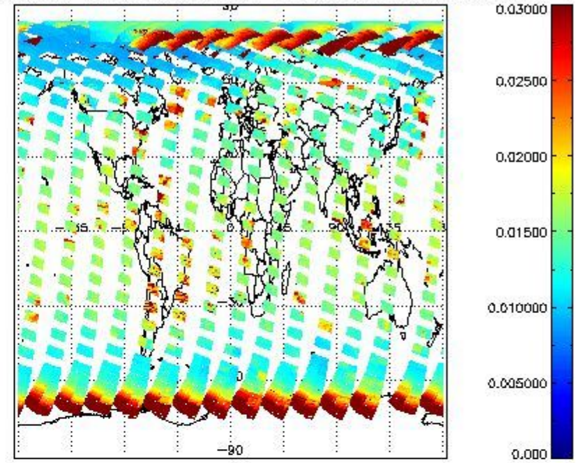
SCIOL2P_NADUV003_vcd_err for 12APR2011 00:00:00 to 13APR2011 00:00:00
