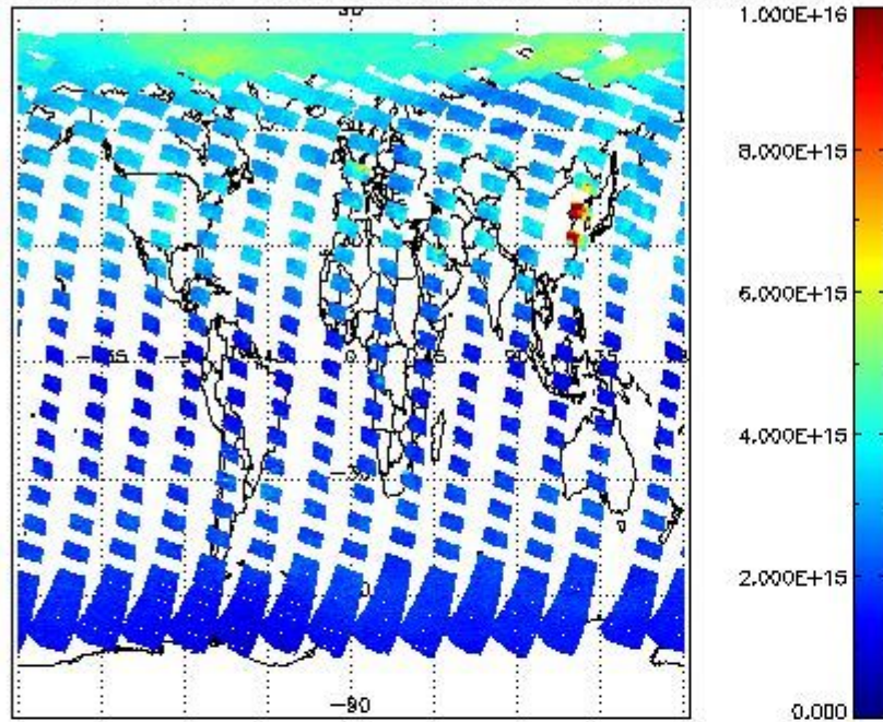
SCIOL2P_NADUV1NO2_vcd for 12APR2011 00:00:00 to 13APR2011 00:00:00
