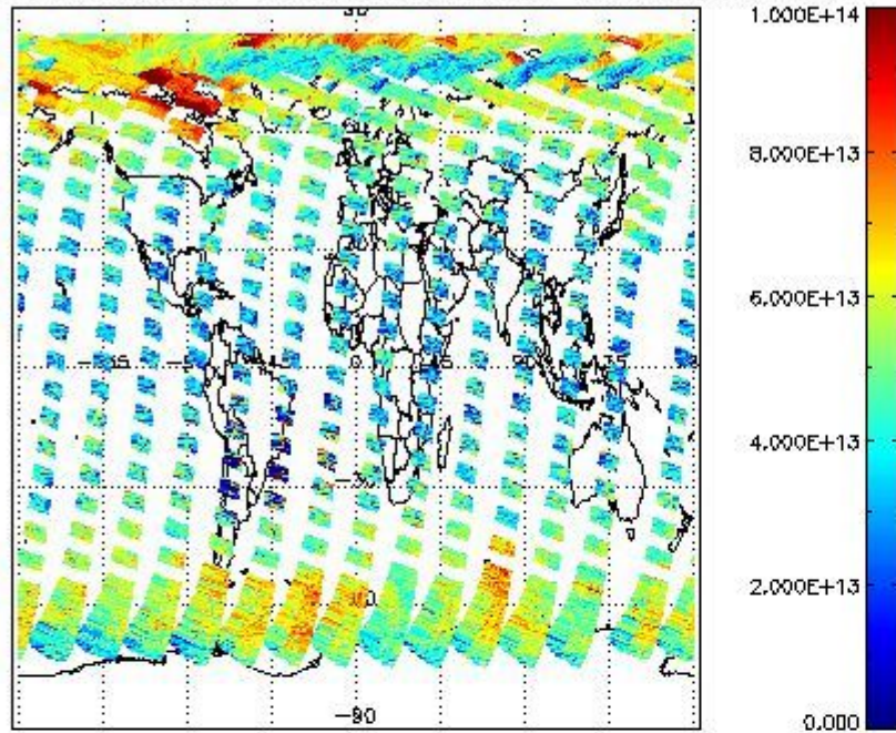
SCIOL2P_NADUV3BRO_vcd for 12APR2011 00:00:00 to 13APR2011 00:00:00
