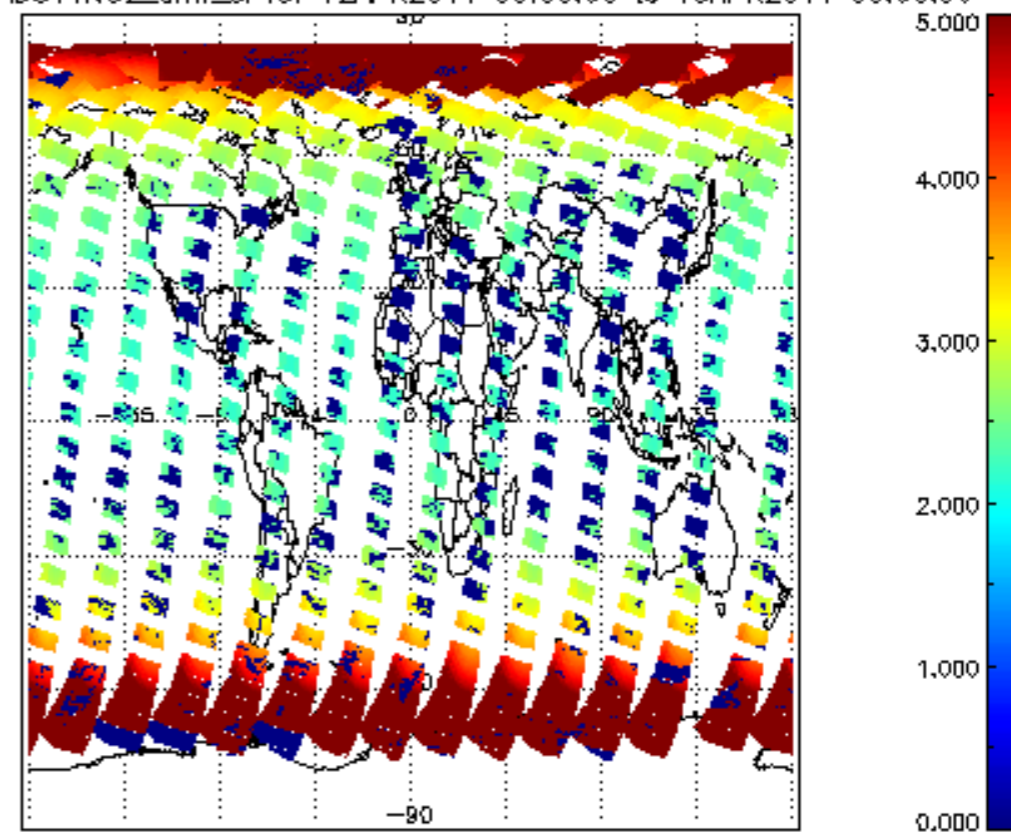
SCIOL2P_NADUV1NO2_amf_sl for 12APR2011 00:00:00 to 13APR2011 00:00:00
