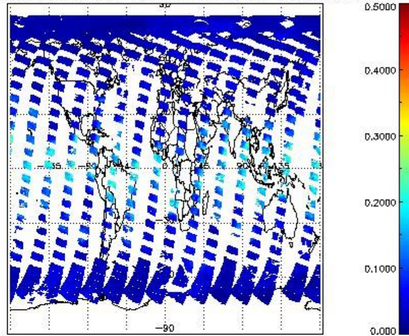
SCIOL2P_NADUV8H2O_vcd_err for 12APR2011 00:00:00 to 13APR2011 00:00:00
