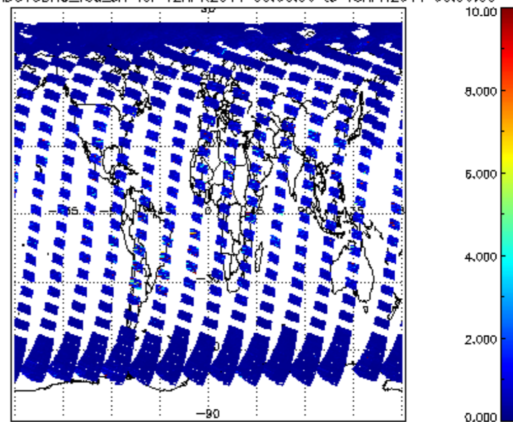
SCIOL2P_NADUV3BRO_vcd_err for 12APR2011 00:00:00 to 13APR2011 00:00:00
