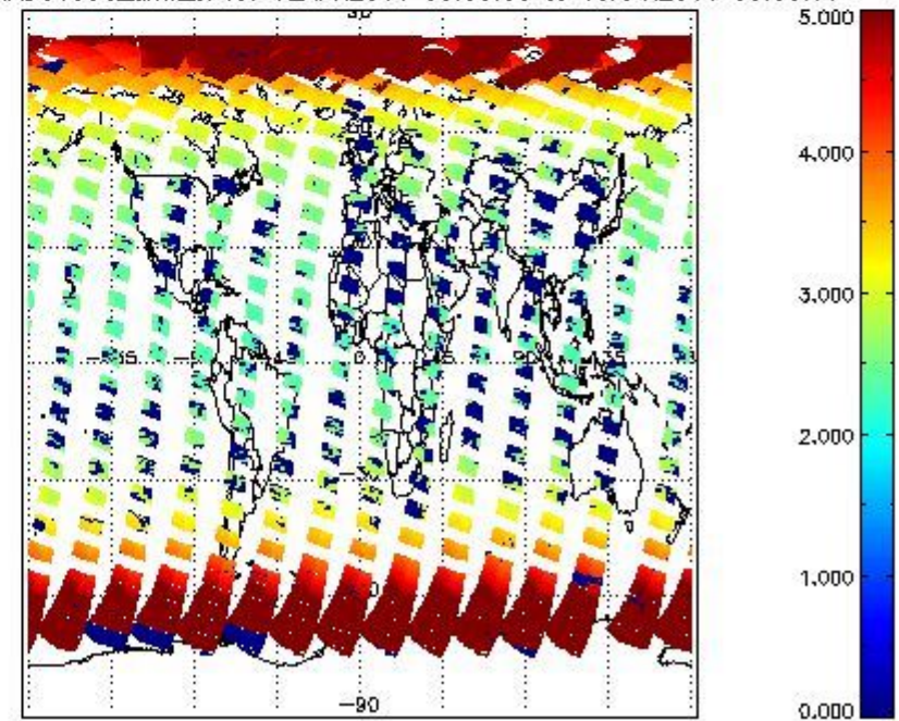
SCIOL2P_NADUV003_amf_cl for 12APR2011 00:00:00 to 13APR2011 00:00:00
