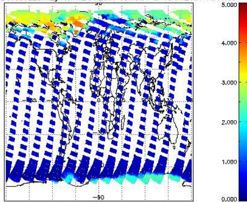
SCIOL2P_NADUV5S02_amf_gr for 12APR2011 00:00:00 to 13APR2011 00:00:00
