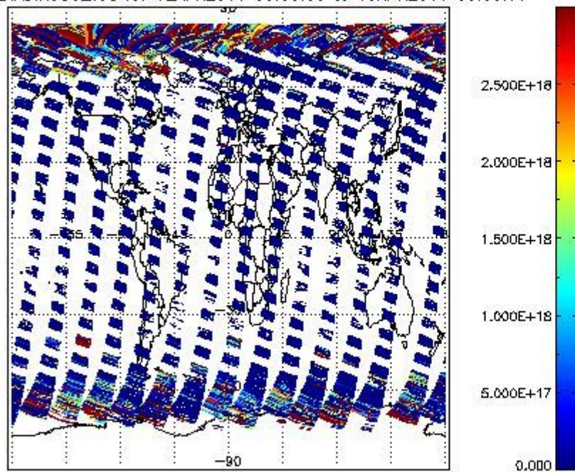
SCIDL2P_NADIR3CO_vcd for 12APR2011 00:00:00 to 13APR2011 00:00:00
