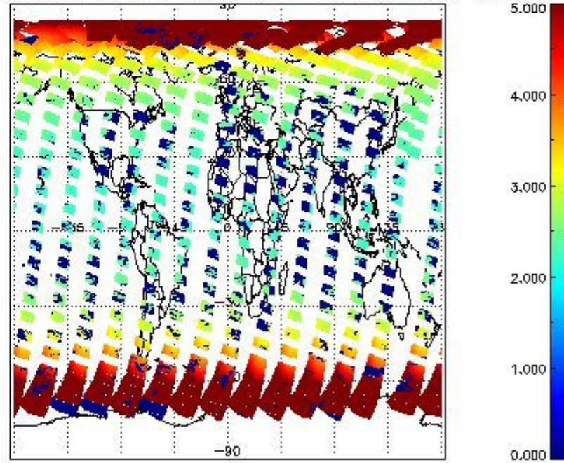
SCIOL2P_NADUV1NO2_amf_cl for 12APR2011 00:00:00 to 13APR2011 00:00:00
