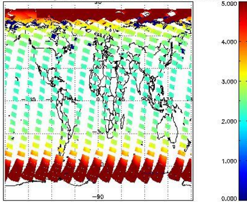
SCIOL2P_NADUV1NO2_amf_gr for 12APR2011 00:00:00 to 13APR2011 00:00:00
