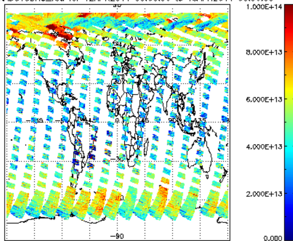
SCIOL2P_NADUV3BRO_vcd for 12APR2011 00:00:00 to 13APR2011 00:00:00
