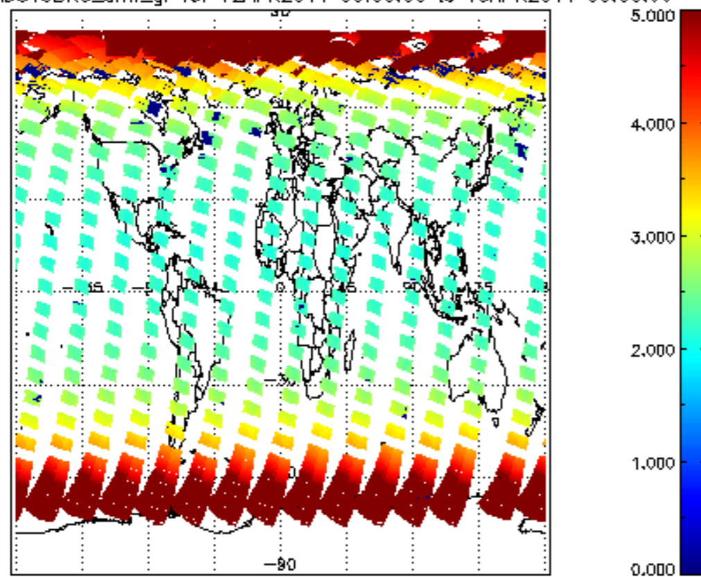
SCIOL2P_NADUV3BRO_amf_gr for 12APR2011 00:00:00 to 13APR2011 00:00:00
