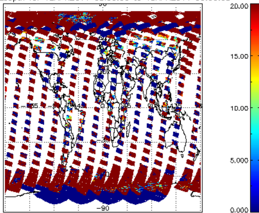
cL_opt_depth for 12APR2011 00:00:00 to 13APR2011 00:00:00
