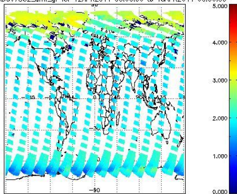
SCIOL2P_NADUV7S02_amf_gr for 12APR2011 00:00:00 to 13APR2011 00:00:00
