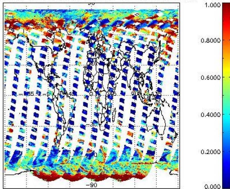
cL_frac for 12APR2011 00:00:00 to 13APR2011 00:00:00
