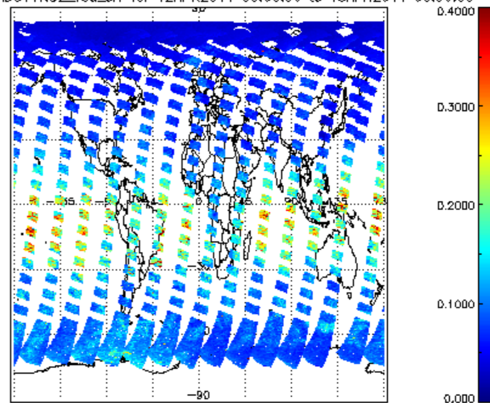
SCIOL2P_NADUV1NO2_vcd_err for 12APR2011 00:00:00 to 13APR2011 00:00:00
