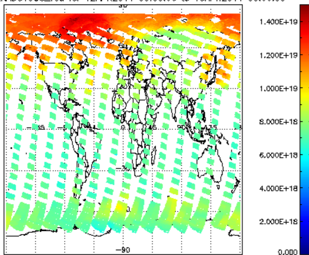
SCIOL2P_NADUV003_vcd for 12APR2011 00:00:00 to 13APR2011 00:00:00
