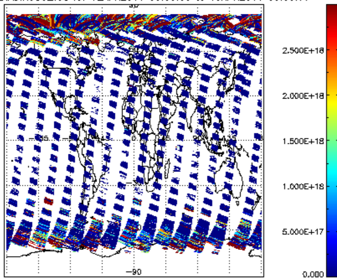
SCIOL2P_NADIR3CO_vcd for 12APR2011 00:00:00 to 13APR2011 00:00:00
