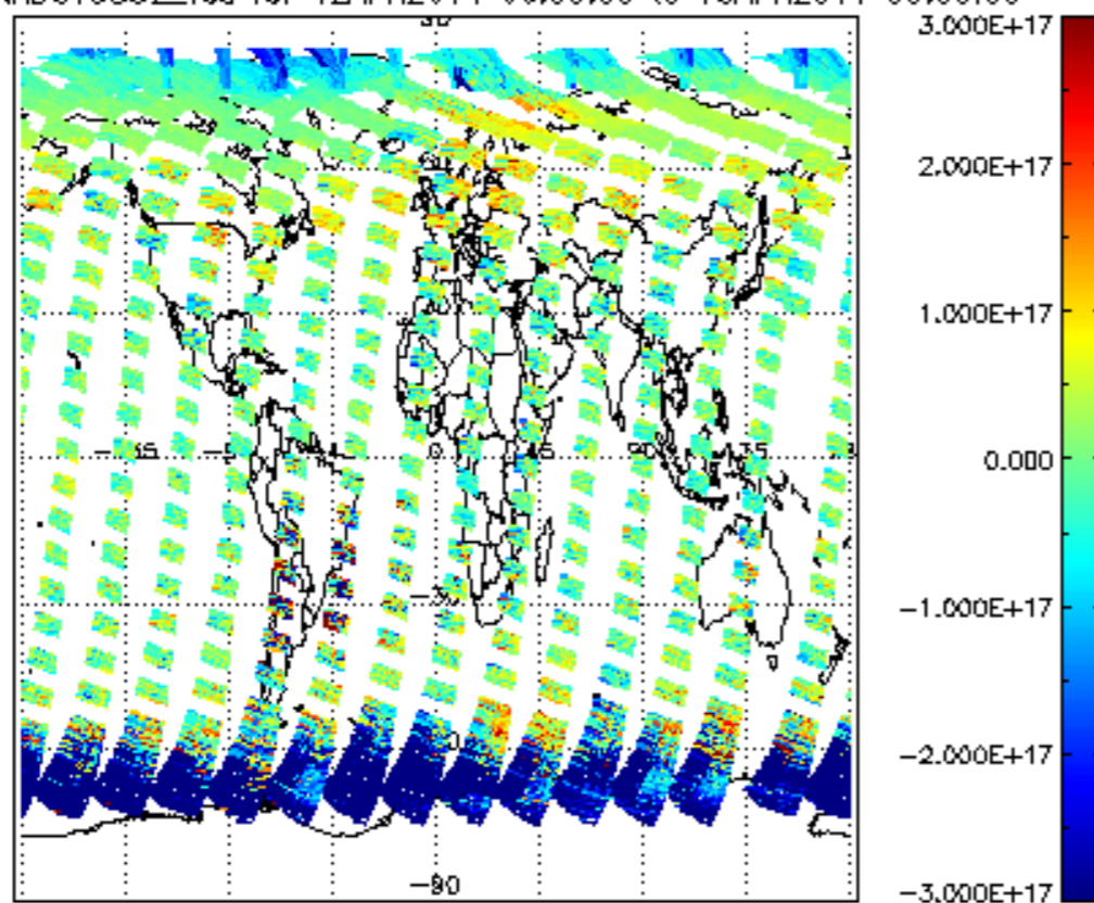
SCIOL2P_NADUV5S02_vcd for 12APR2011 00:00:00 to 13APR2011 00:00:00
