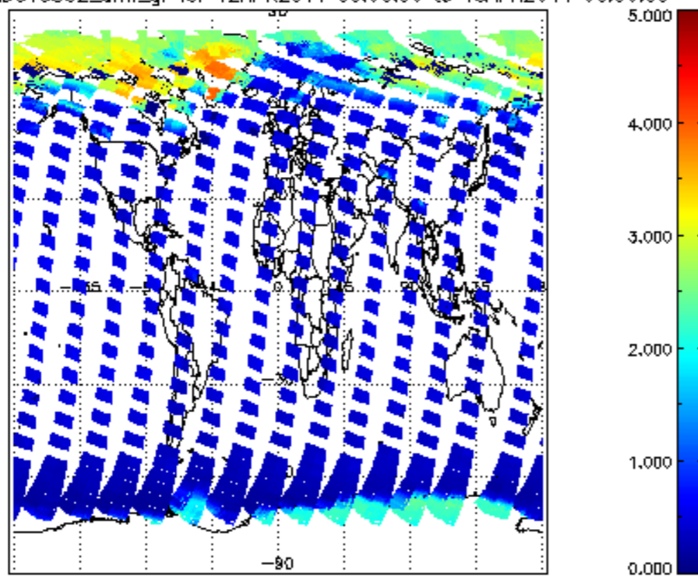
SCIOL2P_NADUV5S02_amf_gr for 12APR2011 00:00:00 to 13APR2011 00:00:00
