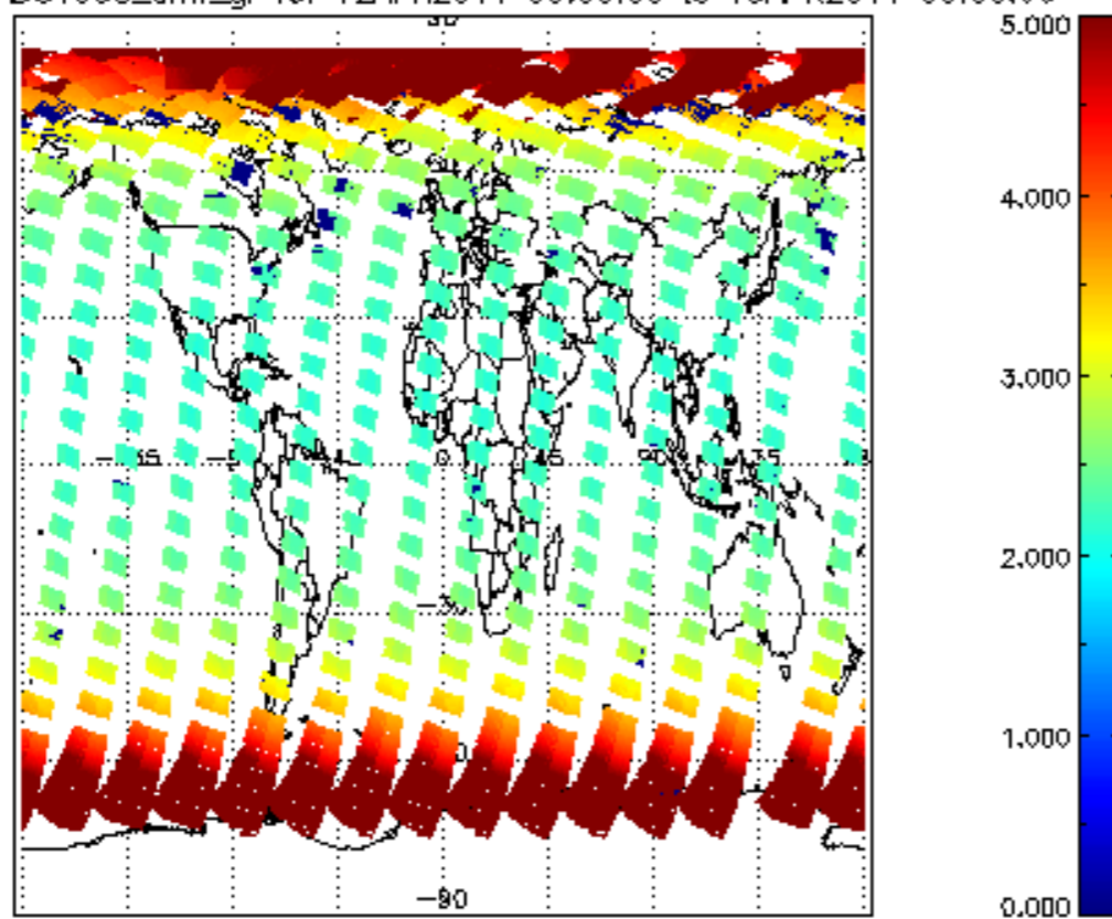
SCIOL2P_NADUV003_amf_gr for 12APR2011 00:00:00 to 13APR2011 00:00:00
