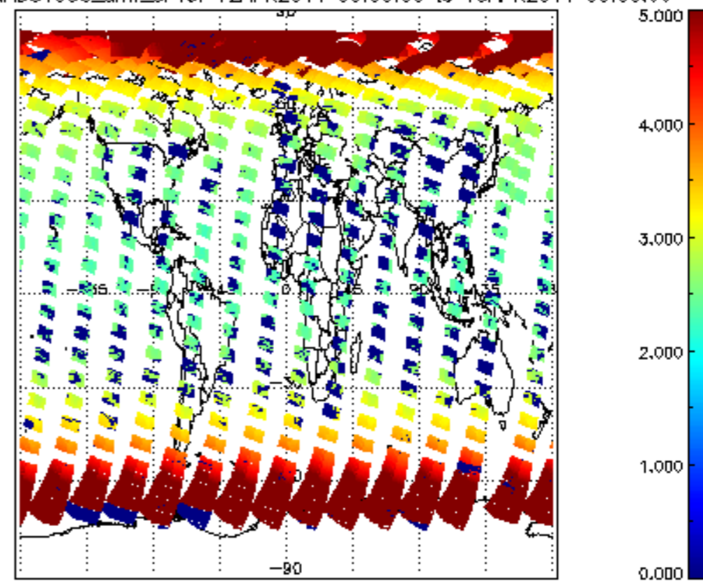
SCIOL2P_NADUV003_amf_cl for 12APR2011 00:00:00 to 13APR2011 00:00:00
