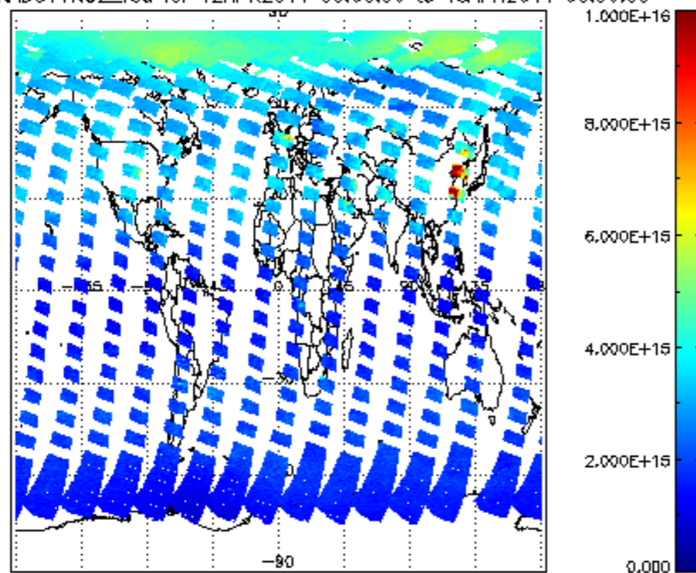
SCIOL2P_NADUV1NO2_vcd for 12APR2011 00:00:00 to 13APR2011 00:00:00
