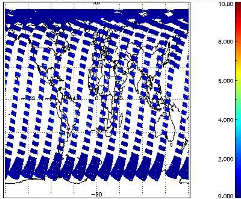
SCIOL2P_NADUV3BRO_vcd_err for 12APR2011 00:00:00 to 13APR2011 00:00:00
