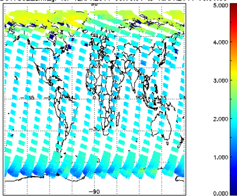
SCIOL2P_NADUV7S02_amf_gr for 12APR2011 00:00:00 to 13APR2011 00:00:00
