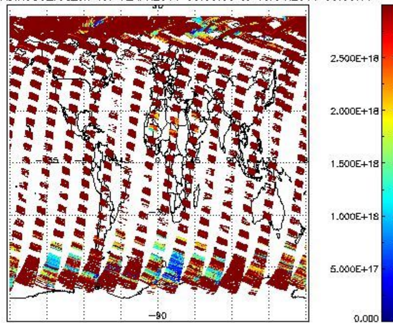
SCIDL2P_NADIR3CO_vcd_err for 12APR2011 00:00:00 to 13APR2011 00:00:00
