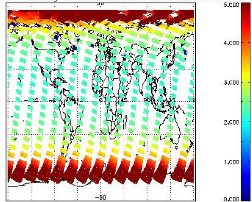
SCIOL2P_NADUV003_amf_gr for 12APR2011 00:00:00 to 13APR2011 00:00:00
