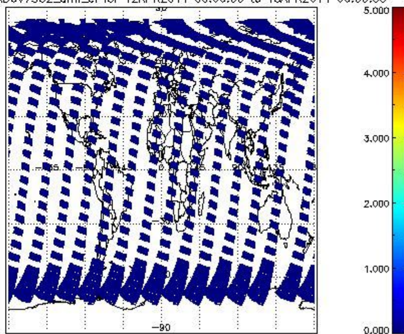
SCIOL2P_NADUV7S02_amf_cl for 12APR2011 00:00:00 to 13APR2011 00:00:00
