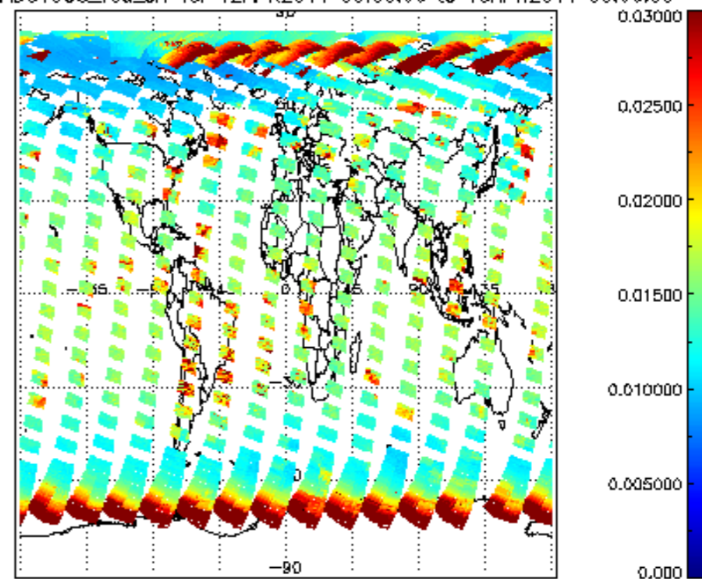
SCIOL2P_NADUV003_vcd_err for 12APR2011 00:00:00 to 13APR2011 00:00:00
