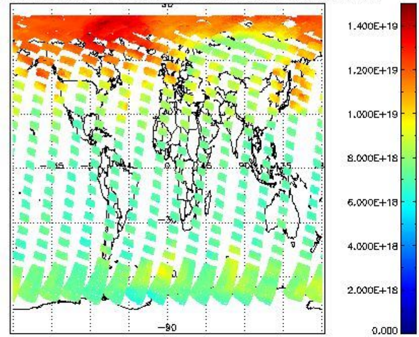
SCIOL2P_NADUV003_vcd for 12APR2011 00:00:00 to 13APR2011 00:00:00
