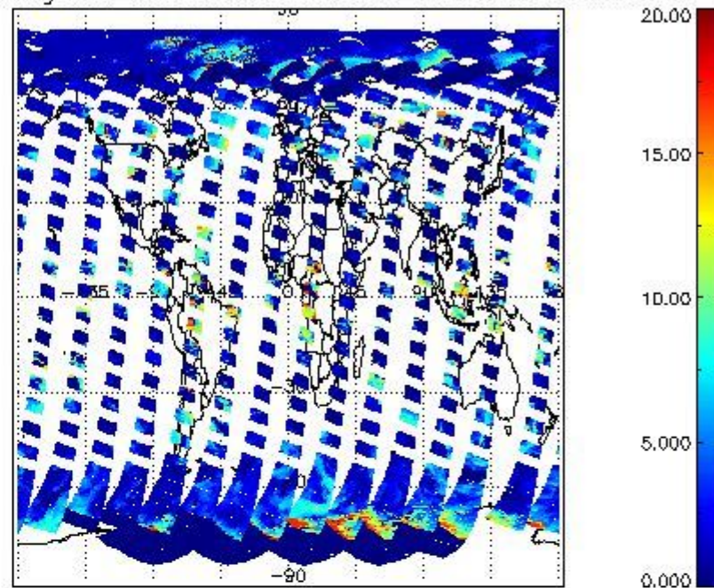
cL_top_height for 12APR2011 00:00:00 to 13APR2011 00:00:00
