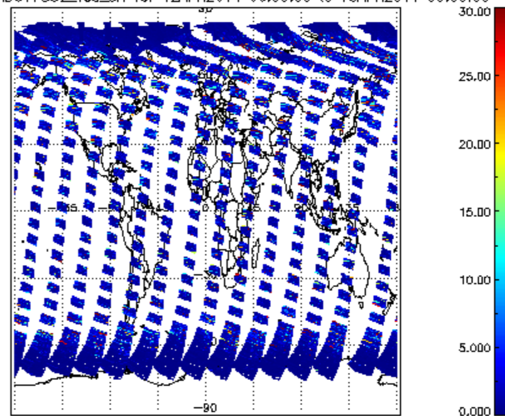
SCIOL2P_NADUV7S02_vcd_err for 12APR2011 00:00:00 to 13APR2011 00:00:00
