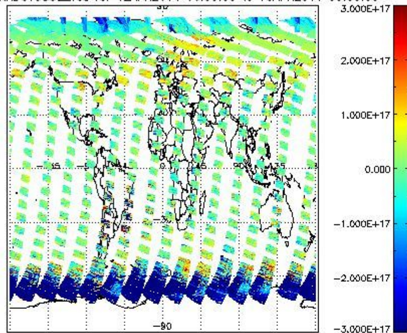
SCIOL2P_NADUV5S02_vcd for 12APR2011 00:00:00 to 13APR2011 00:00:00
