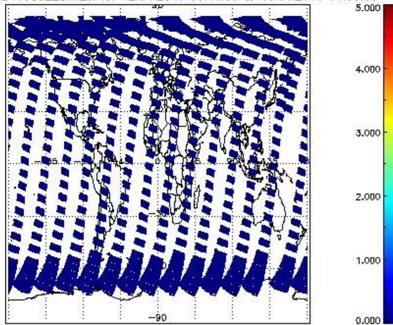
SCIOL2P_NADUV5S02_amf_cl for 12APR2011 00:00:00 to 13APR2011 00:00:00
