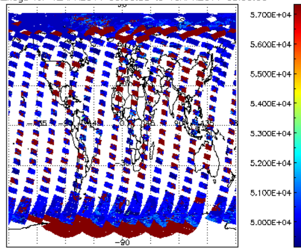
cloud_flags for 12APR2011 00:00:00 to 13APR2011 00:00:00
