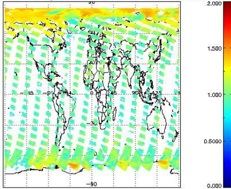
SCIOL2P_NADUV8H2O_arnf_gr for 12APR2011 00:00:00 to 13APR2011 00:00:00
