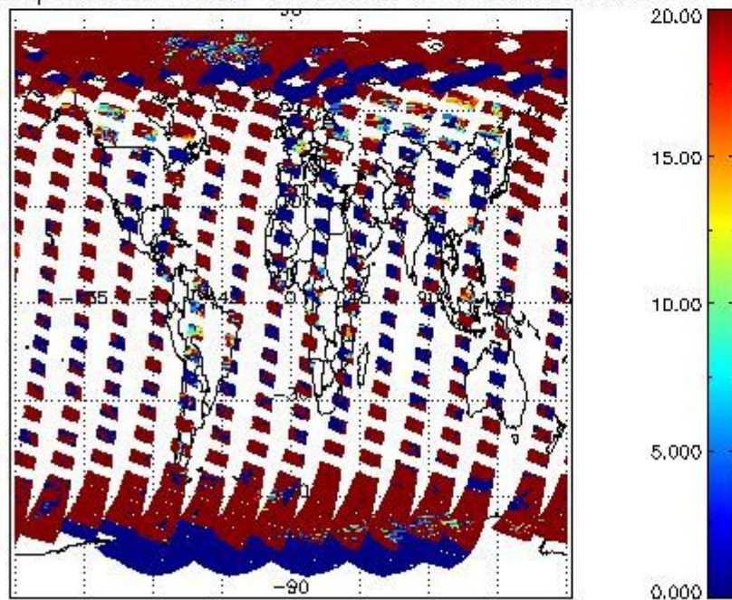
cL_opt_depth for 12APR2011 00:00:00 to 13APR2011 00:00:00
