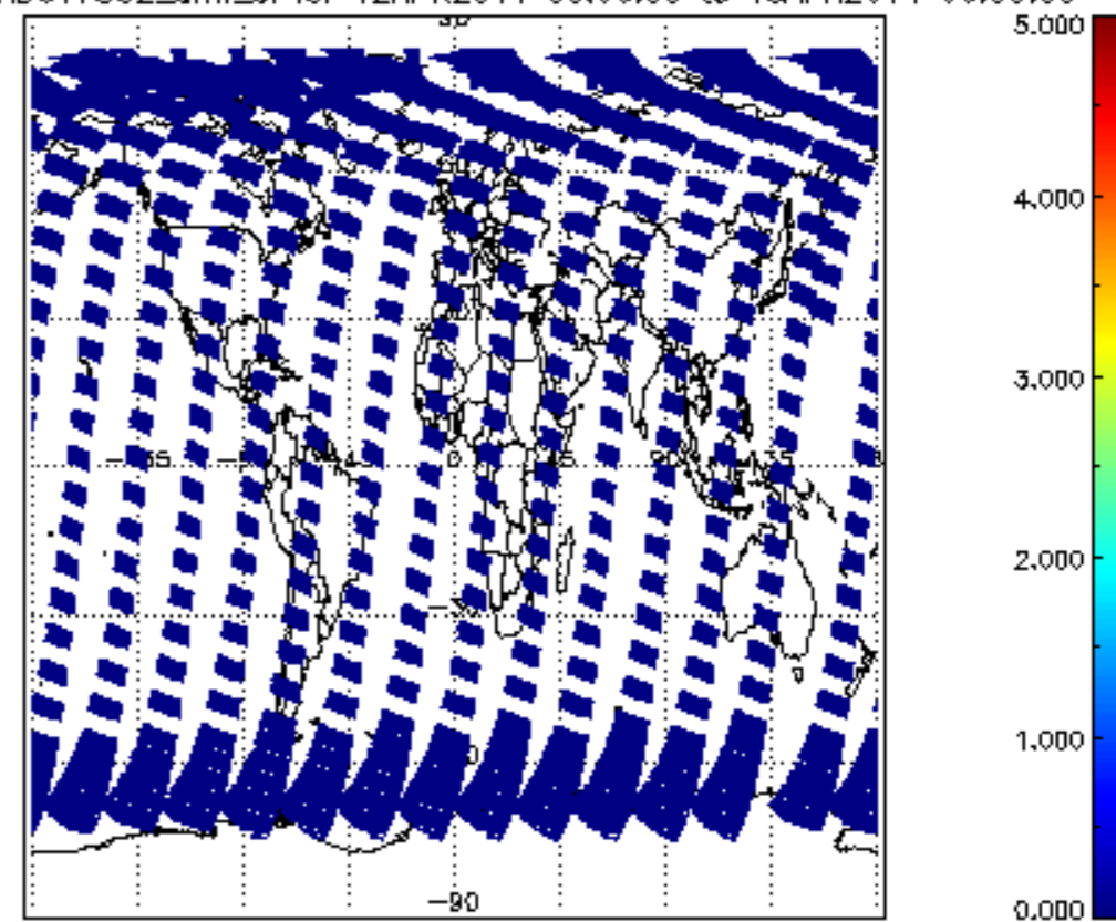
SCIOL2P_NADUV7S02_amf_cl for 12APR2011 00:00:00 to 13APR2011 00:00:00
