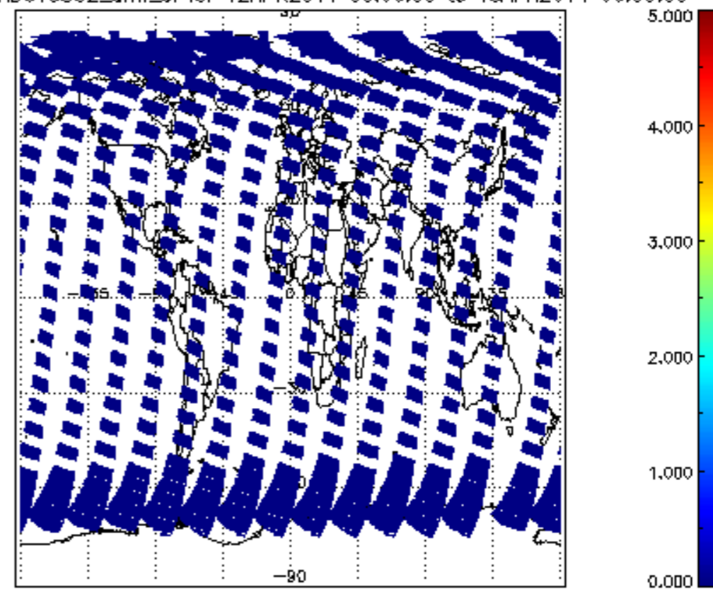
SCIOL2P_NADUV5S02_amf_cl for 12APR2011 00:00:00 to 13APR2011 00:00:00
