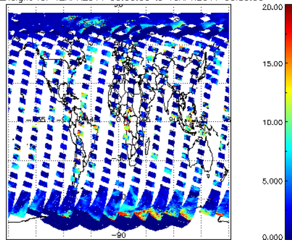
cL_top_height for 12APR2011 00:00:00 to 13APR2011 00:00:00
