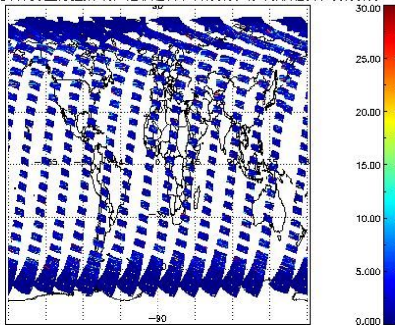
SCIOL2P_NADUV7S02_vcd_err for 12APR2011 00:00:00 to 13APR2011 00:00:00
