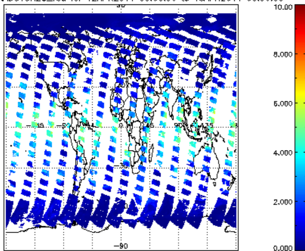
SCIOL2P_NADUV8H2O_vcd for 12APR2011 00:00:00 to 13APR2011 00:00:00
