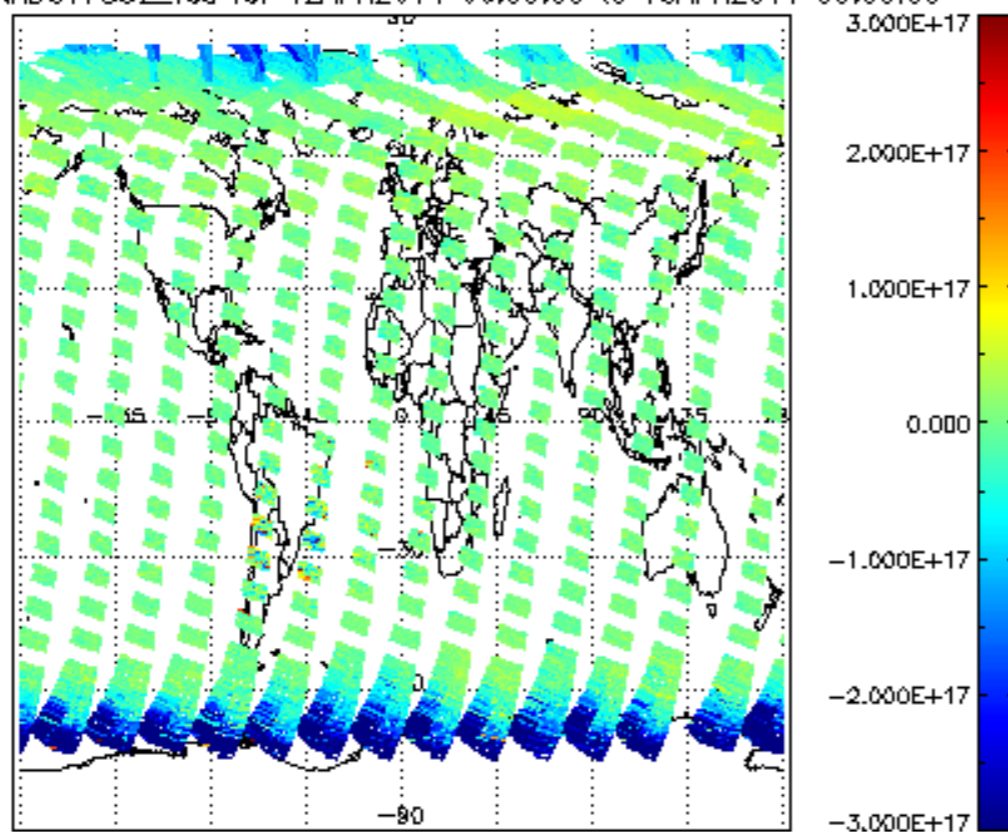
SCIOL2P_NADUV7S02_vcd for 12APR2011 00:00:00 to 13APR2011 00:00:00
