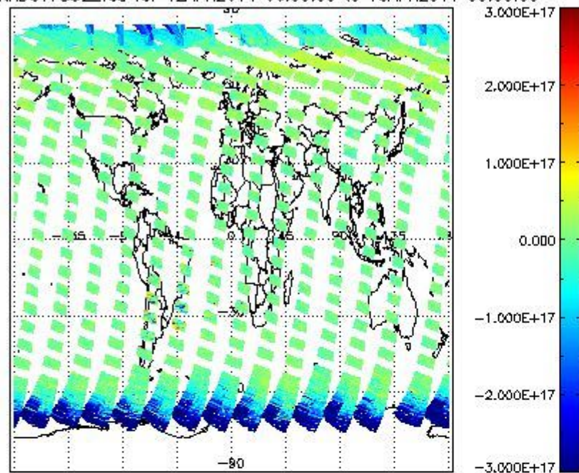
SCIOL2P_NADUV7S02_vcd for 12APR2011 00:00:00 to 13APR2011 00:00:00
