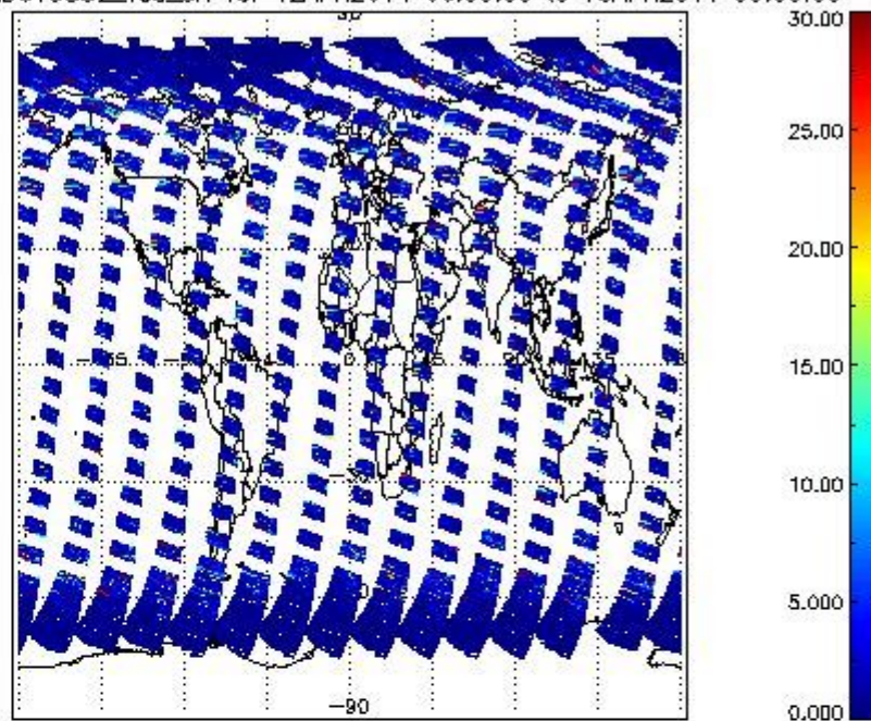
SCIOL2P_NADUV5S02_vcd_err for 12APR2011 00:00:00 to 13APR2011 00:00:00
