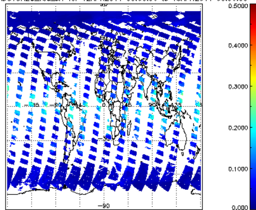
SCIOL2P_NADUV8H2O_vcd_err for 12APR2011 00:00:00 to 13APR2011 00:00:00
