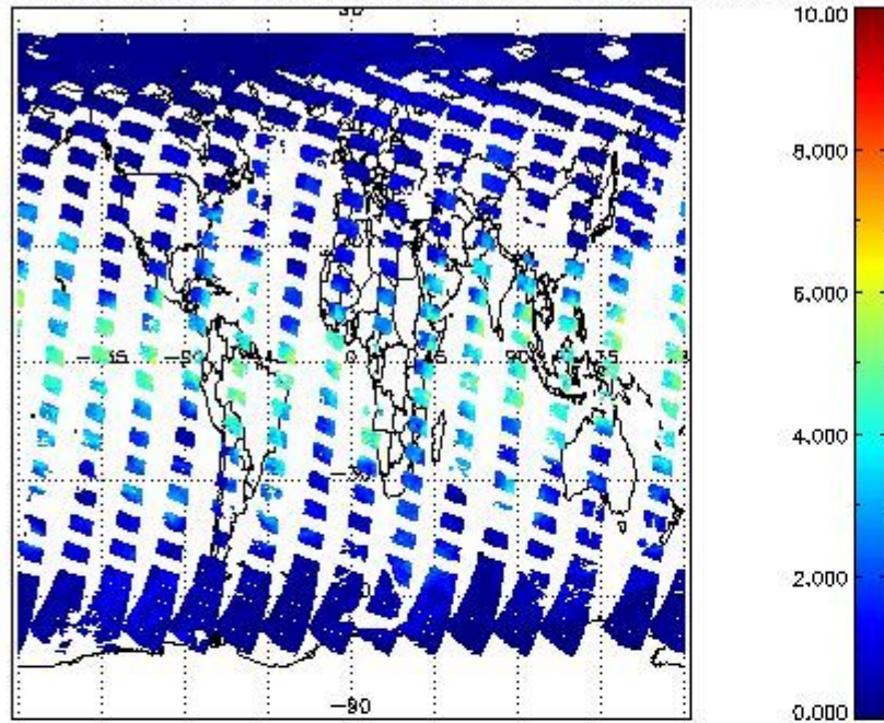
SCIOL2P_NADUV8H2O_vcd for 12APR2011 00:00:00 to 13APR2011 00:00:00
