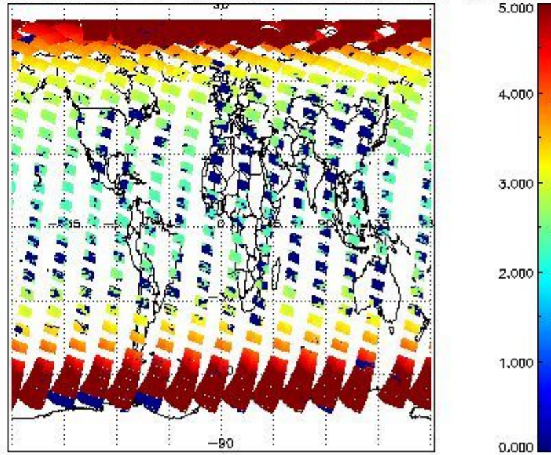
SCIOL2P_NADUV3BRO_amf_cl for 12APR2011 00:00:00 to 13APR2011 00:00:00
