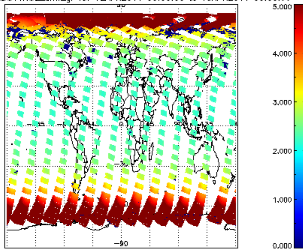
SCIOL2P_NADUV1NO2_amf_gr for 12APR2011 00:00:00 to 13APR2011 00:00:00
