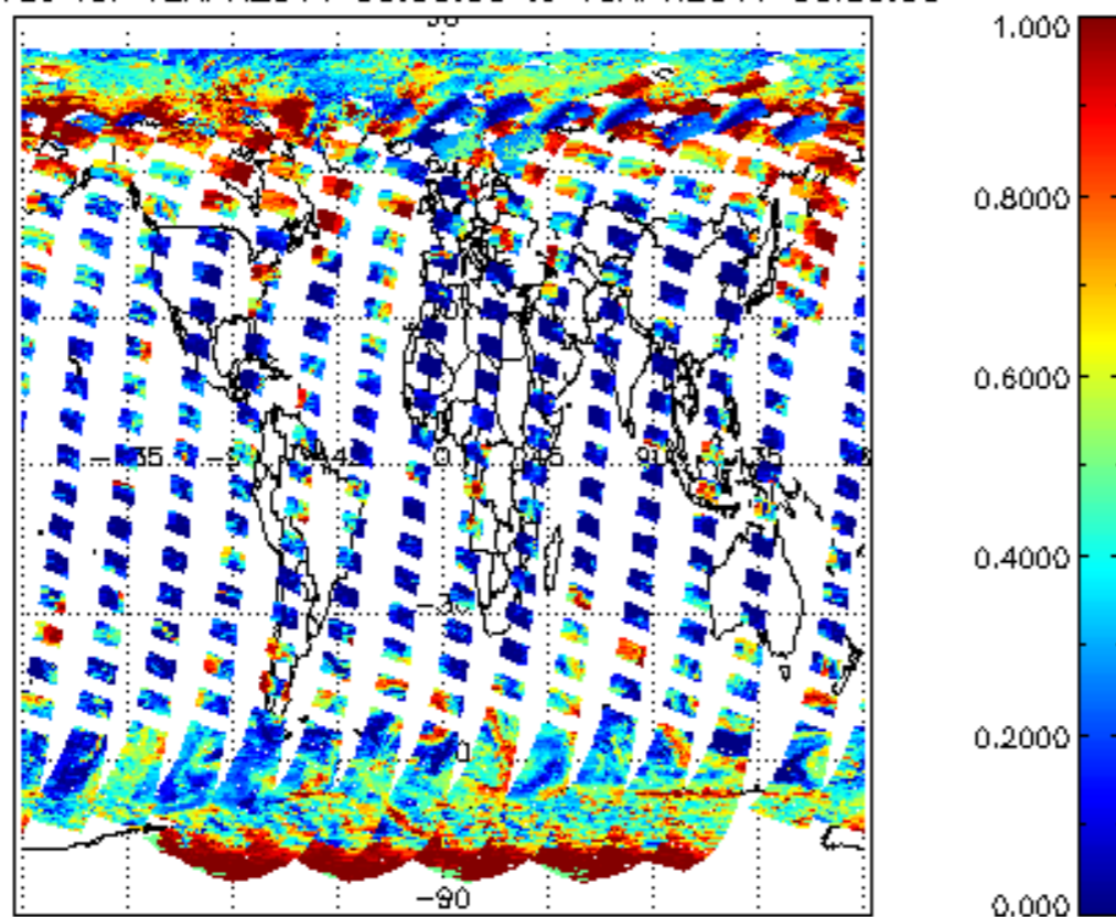
cL_frac for 12APR2011 00:00:00 to 13APR2011 00:00:00
