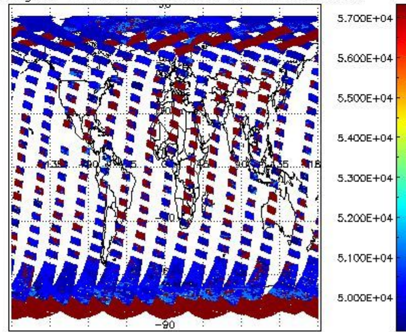
cloud_flags for 11APR2011 00:00:00 to 12APR2011 00:00:00
