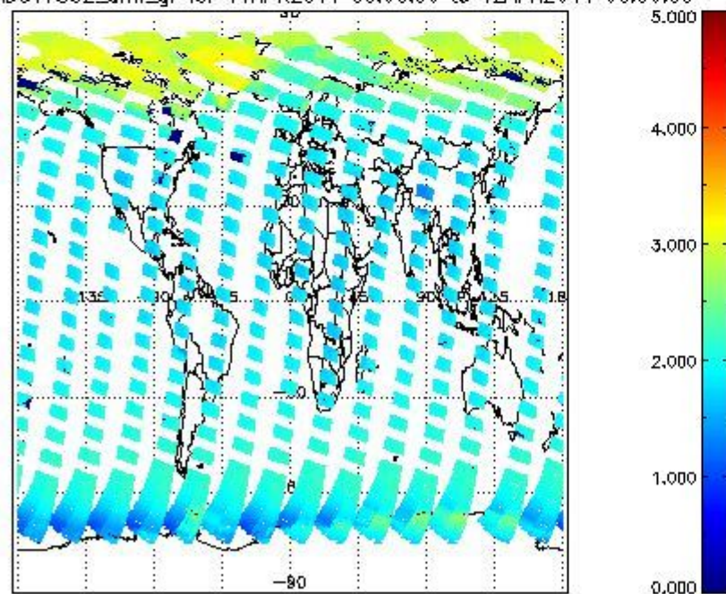
SCIOL2P_NADUV7S02_amf_gr for 11APR2011 00:00:00 to 12APR2011 00:00:00
