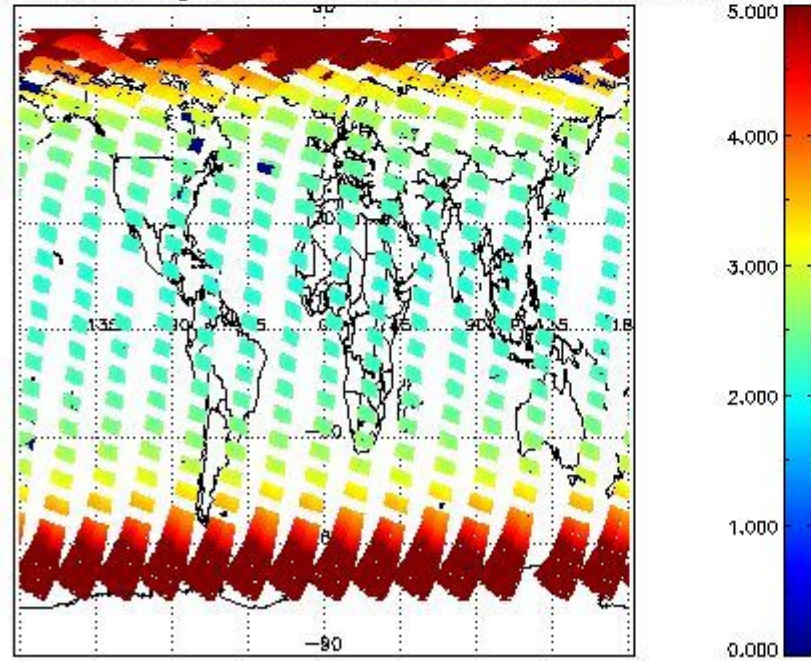
SCIOL2P_NADUV3BRO_amf_gr for 11APR2011 00:00:00 to 12APR2011 00:00:00
