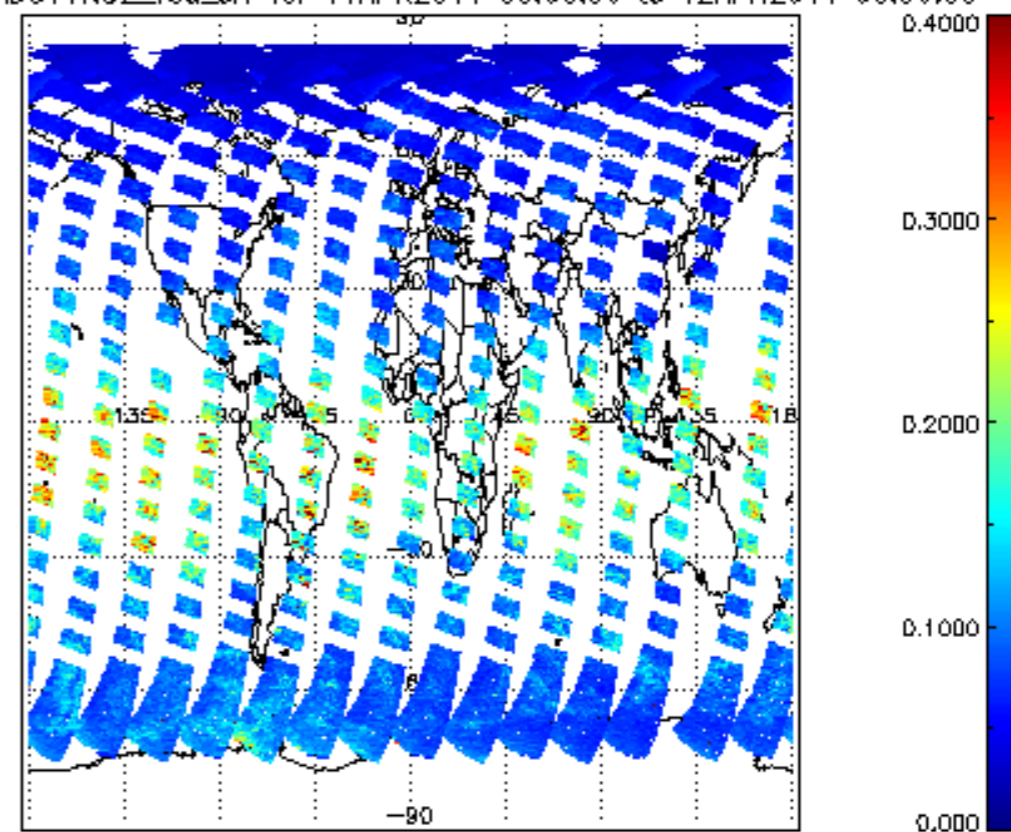
SCIOL2P_NADUV1NO2_vcd_err for 11APR2011 00:00:00 to 12APR2011 00:00:00
