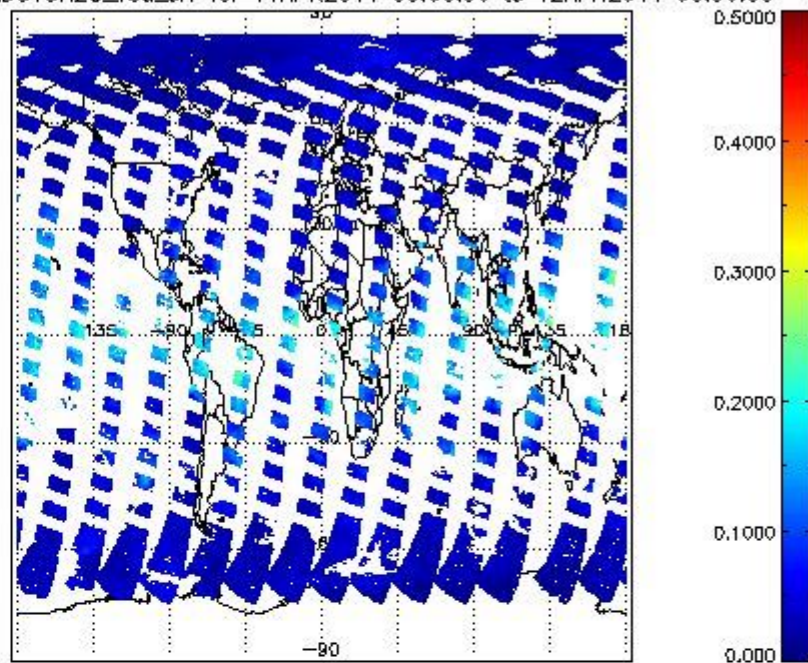
SCIOL2P_NADUV8H2O_vcd_err for 11APR2011 00:00:00 to 12APR2011 00:00:00
