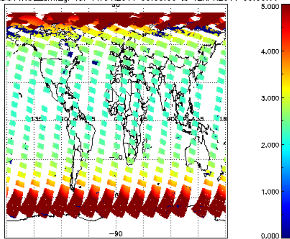
SCIOL2P_NADUV1NO2_amf_gr for 11APR2011 00:00:00 to 12APR2011 00:00:00
