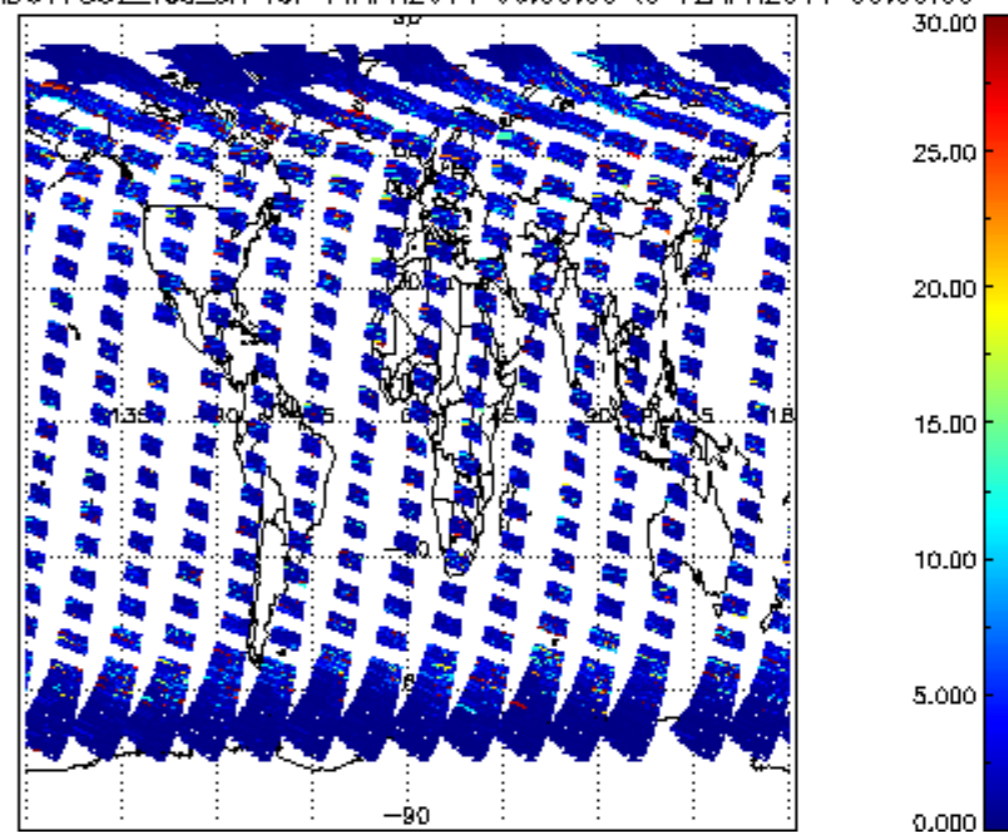
SCIOL2P_NADUV7S02_vcd_err for 11APR2011 00:00:00 to 12APR2011 00:00:00
