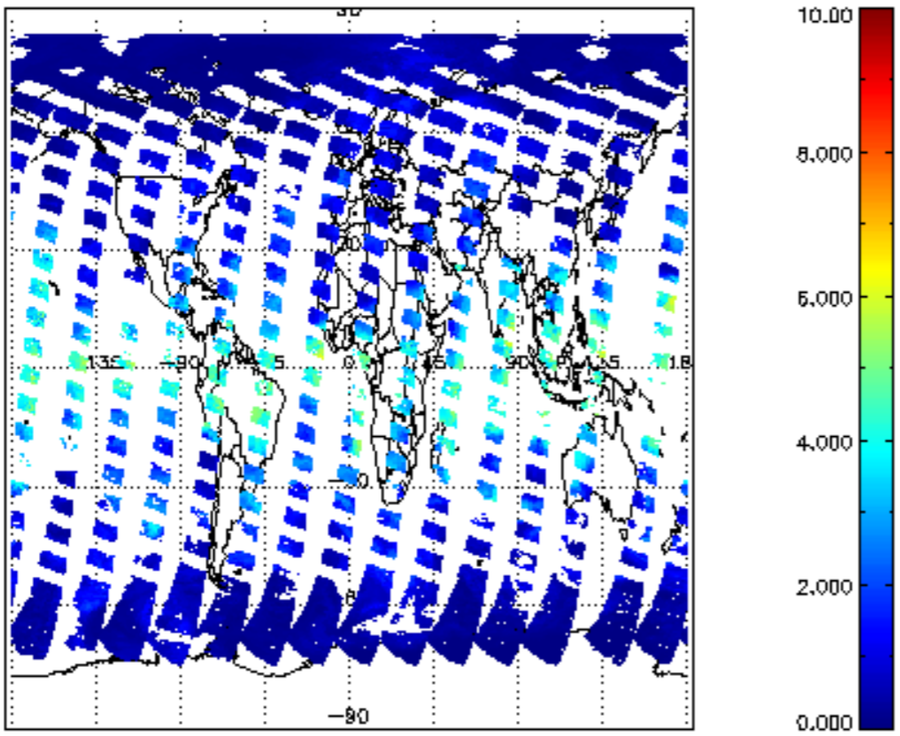
SCIOL2P_NADUV8H2O_vcd for 11APR2011 00:00:00 to 12APR2011 00:00:00
