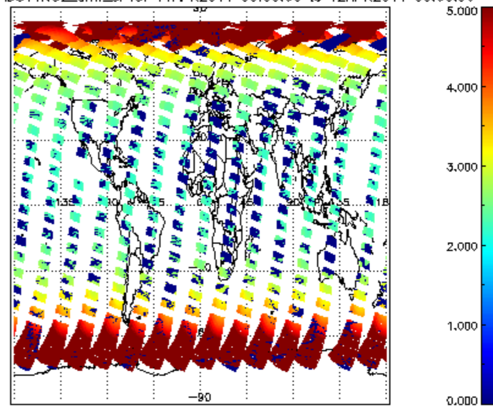
SCIOL2P_NADUV1NO2_amf_sl for 11APR2011 00:00:00 to 12APR2011 00:00:00
