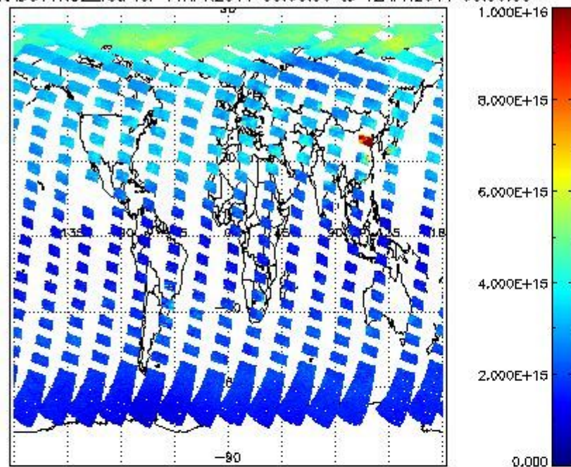
SCIOL2P_NADUV1NO2_vcd for 11APR2011 00:00:00 to 12APR2011 00:00:00
