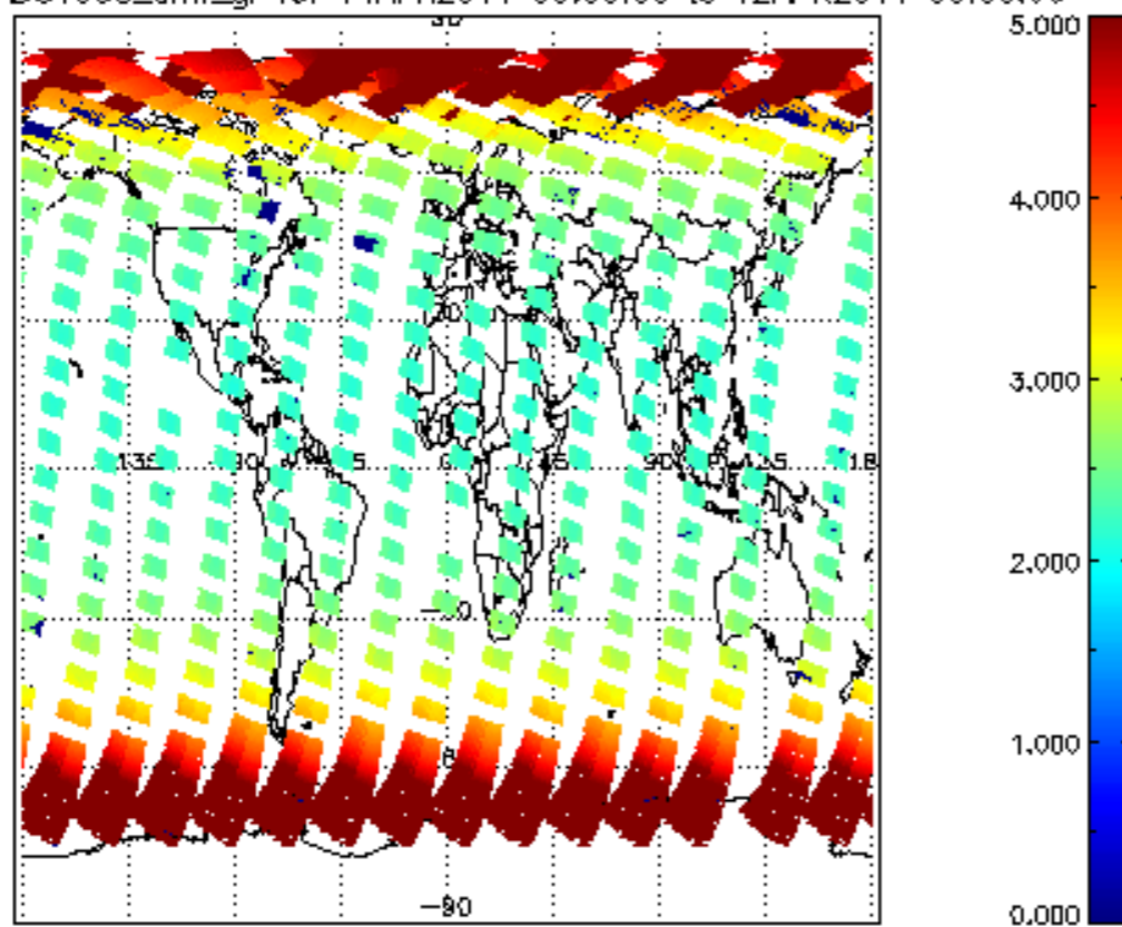
SCIOL2P_NADUV003_amf_gr for 11APR2011 00:00:00 to 12APR2011 00:00:00
