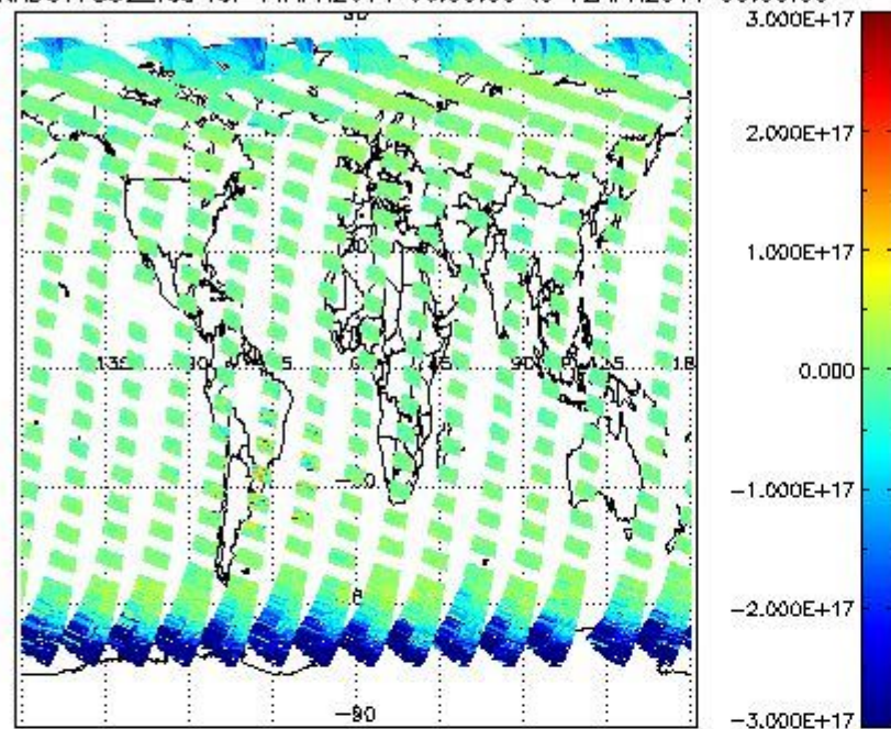
SCIOL2P_NADUV7S02_vcd for 11APR2011 00:00:00 to 12APR2011 00:00:00
