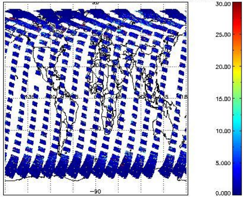
SCIOL2P_NADUV5S02_vcd_err for 11APR2011 00:00:00 to 12APR2011 00:00:00
