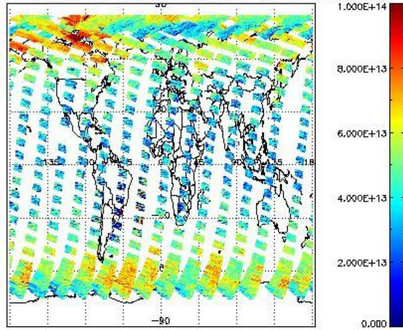
SCIOL2P_NADUV3BRO_vcd for 11APR2011 00:00:00 to 12APR2011 00:00:00
