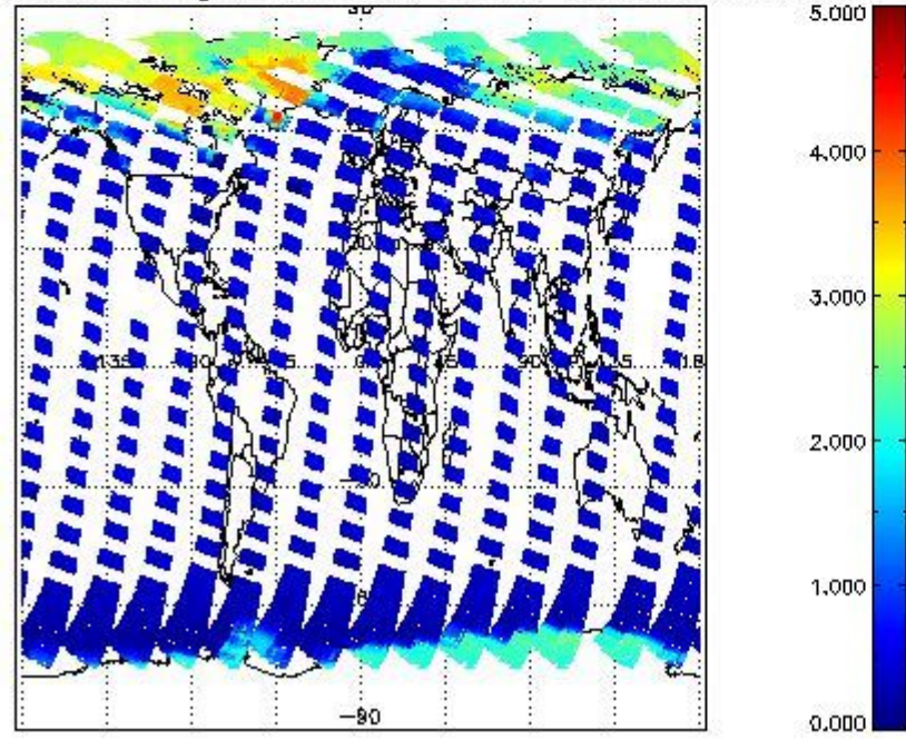
SCIOL2P_NADUV5S02_amf_gr for 11APR2011 00:00:00 to 12APR2011 00:00:00
