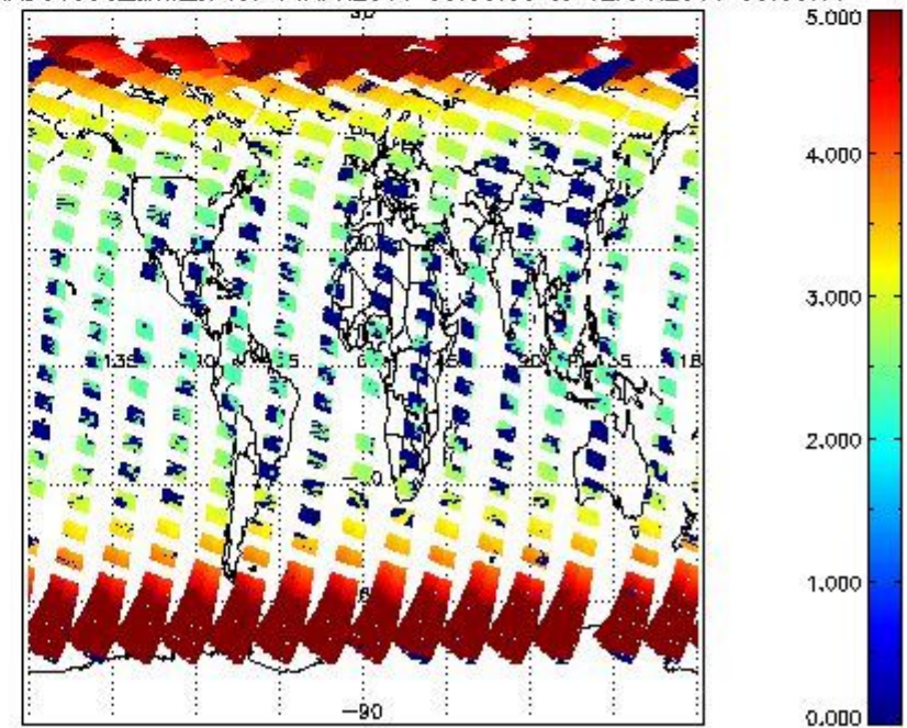
SCIOL2P_NADUV003_amf_cl for 11APR2011 00:00:00 to 12APR2011 00:00:00
