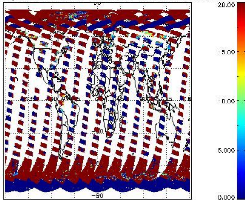
cL_opt_depth for 11APR2011 00:00:00 to 12APR2011 00:00:00
