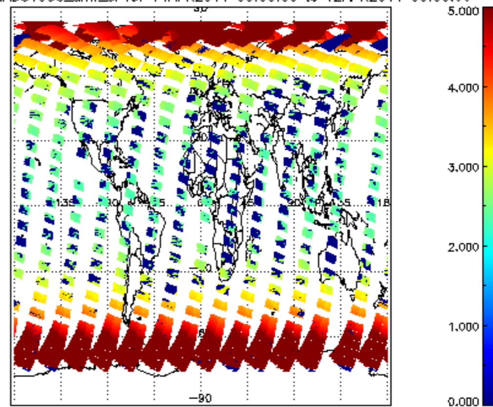
SCIOL2P_NADUV003_amf_cl for 11APR2011 00:00:00 to 12APR2011 00:00:00
