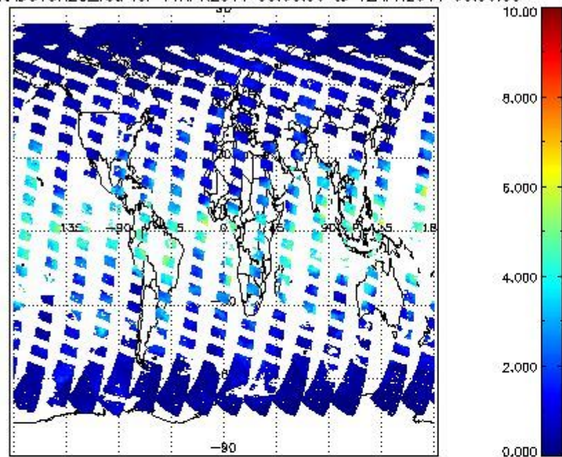
SCIOL2P_NADUV8H2O_vcd for 11APR2011 00:00:00 to 12APR2011 00:00:00
