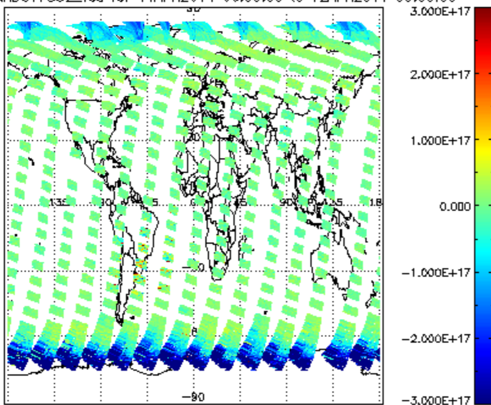
SCIOL2P_NADUV7S02_vcd for 11APR2011 00:00:00 to 12APR2011 00:00:00
