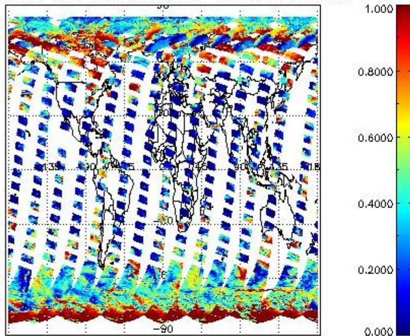
cL_frac for 11APR2011 00:00:00 to 12APR2011 00:00:00
