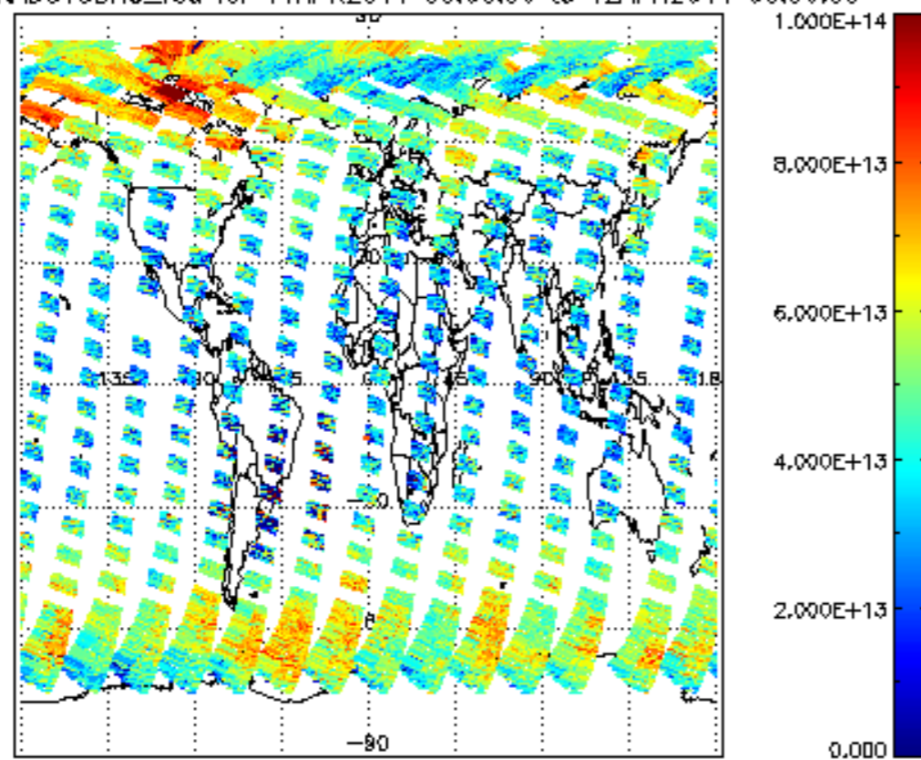
SCIOL2P_NADUV3BRO_vcd for 11APR2011 00:00:00 to 12APR2011 00:00:00
