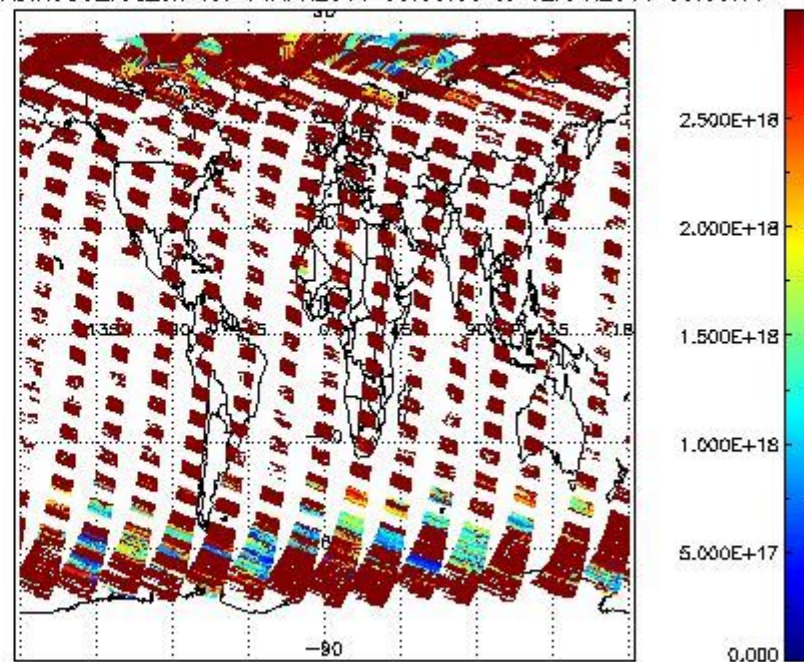
SCIDL2P_NADIR3CO_vcd_err for 11APR2011 00:00:00 to 12APR2011 00:00:00
