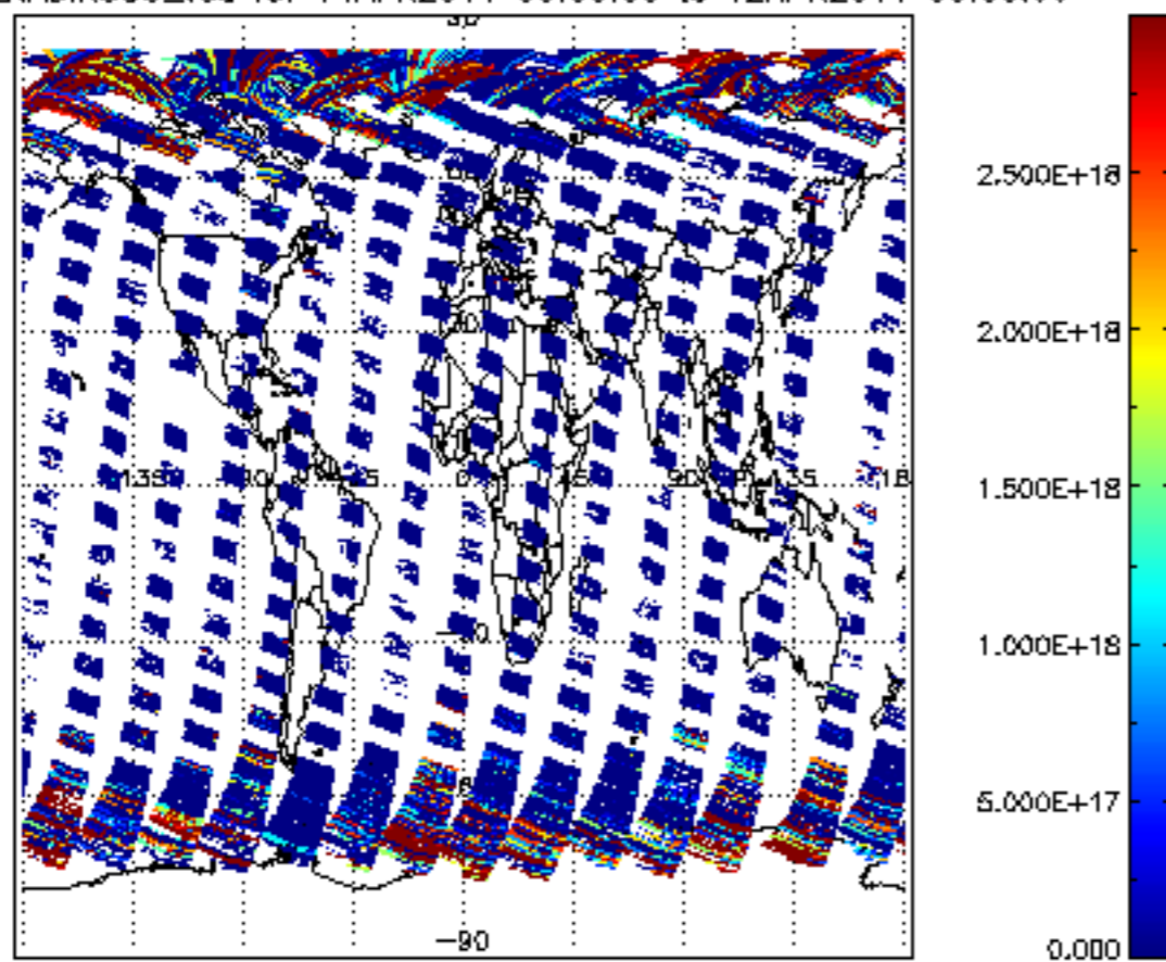
SCIOL2P_NADIR3CO_vcd for 11APR2011 00:00:00 to 12APR2011 00:00:00
