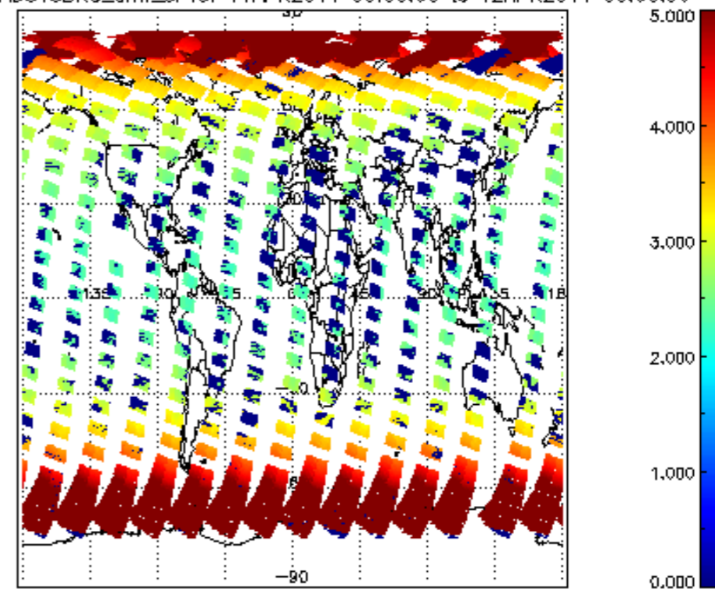
SCIOL2P_NADUV3BRO_amf_sl for 11APR2011 00:00:00 to 12APR2011 00:00:00
