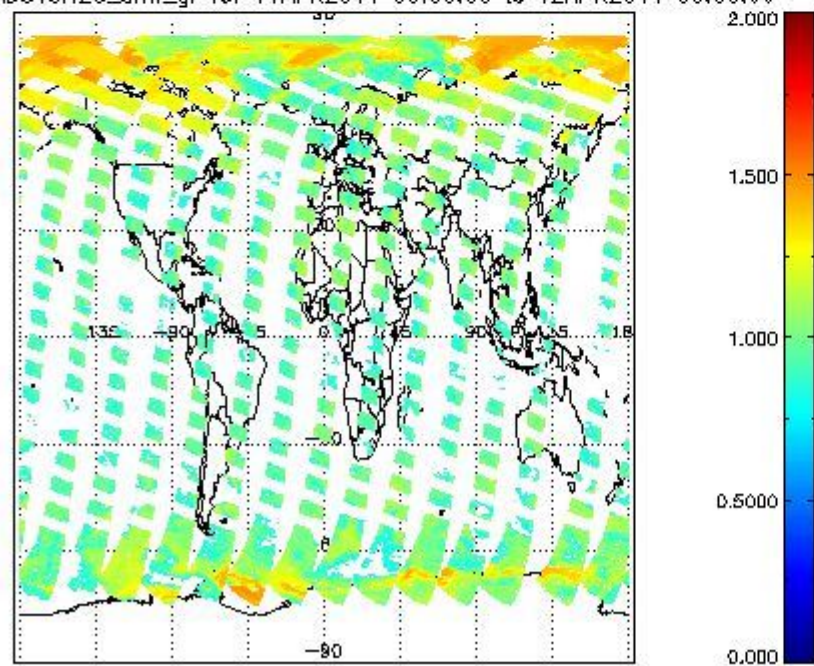
SCIOL2P_NADUV8H2O_arnf_gr for 11APR2011 00:00:00 to 12APR2011 00:00:00
