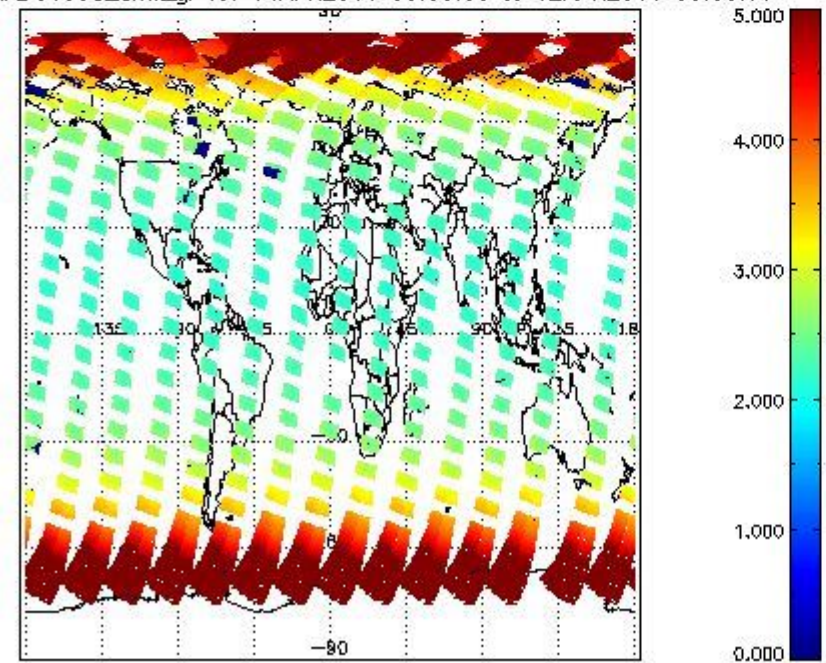
SCIOL2P_NADUV003_amf_gr for 11APR2011 00:00:00 to 12APR2011 00:00:00
