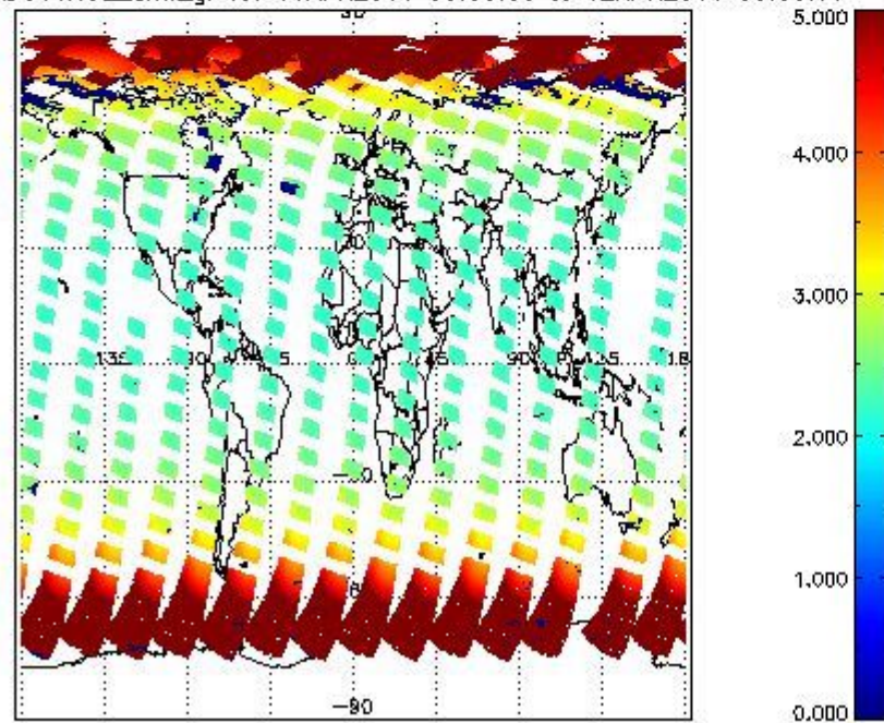
SCIOL2P_NADUV1NO2_amf_gr for 11APR2011 00:00:00 to 12APR2011 00:00:00
