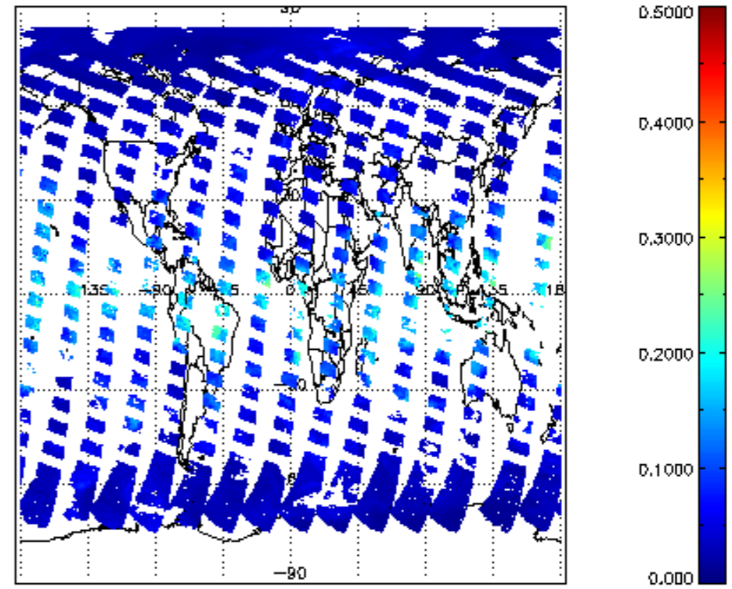
SCIOL2P_NADUV8H2O_vcd_err for 11APR2011 00:00:00 to 12APR2011 00:00:00
