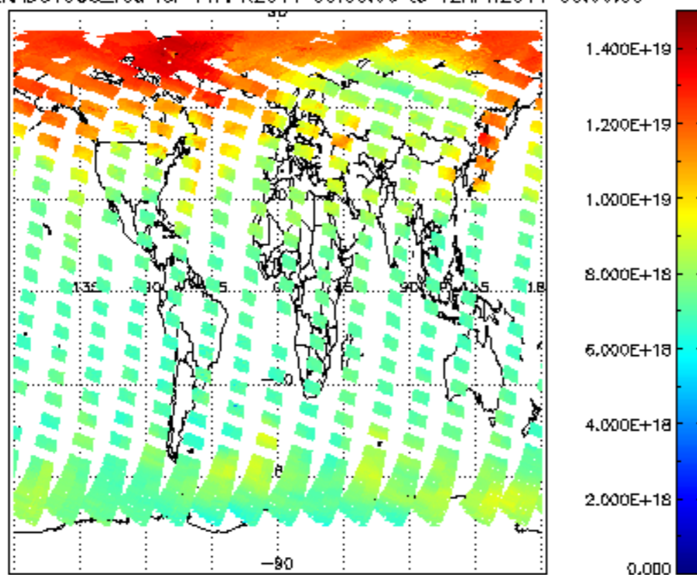
SCIOL2P_NADUV003_vcd for 11APR2011 00:00:00 to 12APR2011 00:00:00
