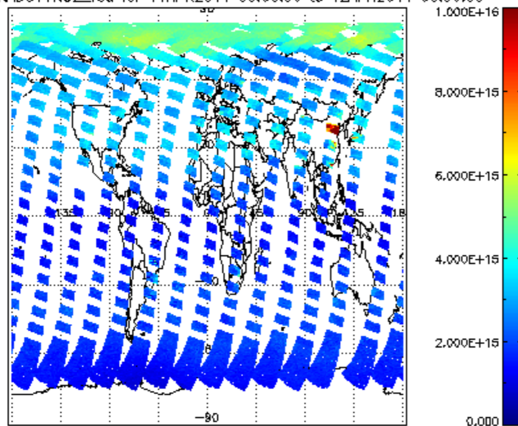
SCIOL2P_NADUV1NO2_vcd for 11APR2011 00:00:00 to 12APR2011 00:00:00
