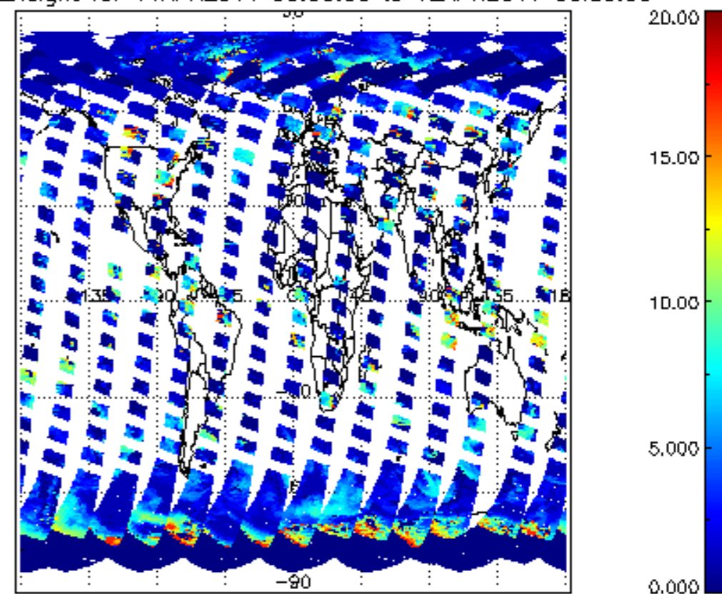
cL_top_height for 11APR2011 00:00:00 to 12APR2011 00:00:00
