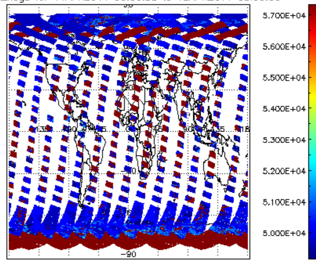
cloud_flags for 11APR2011 00:00:00 to 12APR2011 00:00:00
