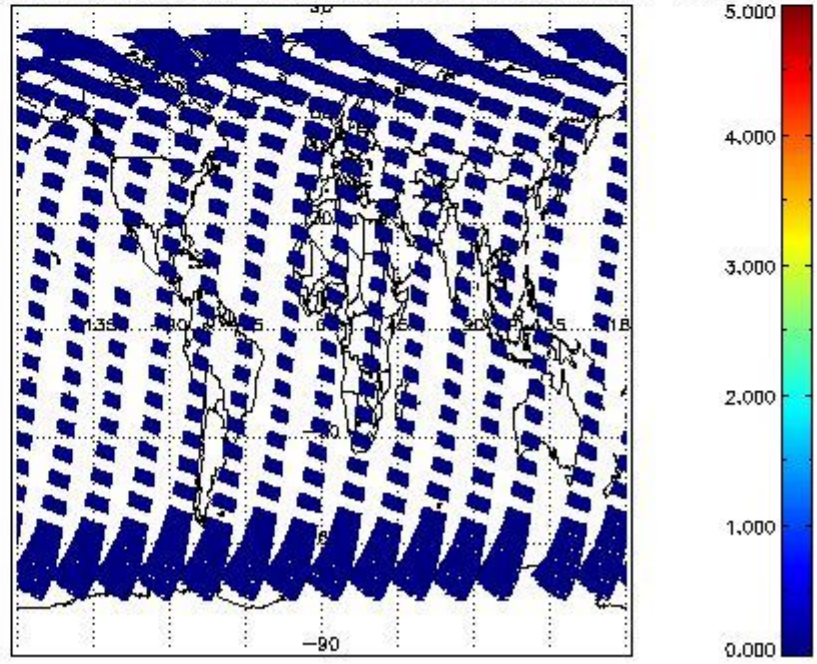
SCIOL2P_NADUV5S02_amf_cl for 11APR2011 00:00:00 to 12APR2011 00:00:00
