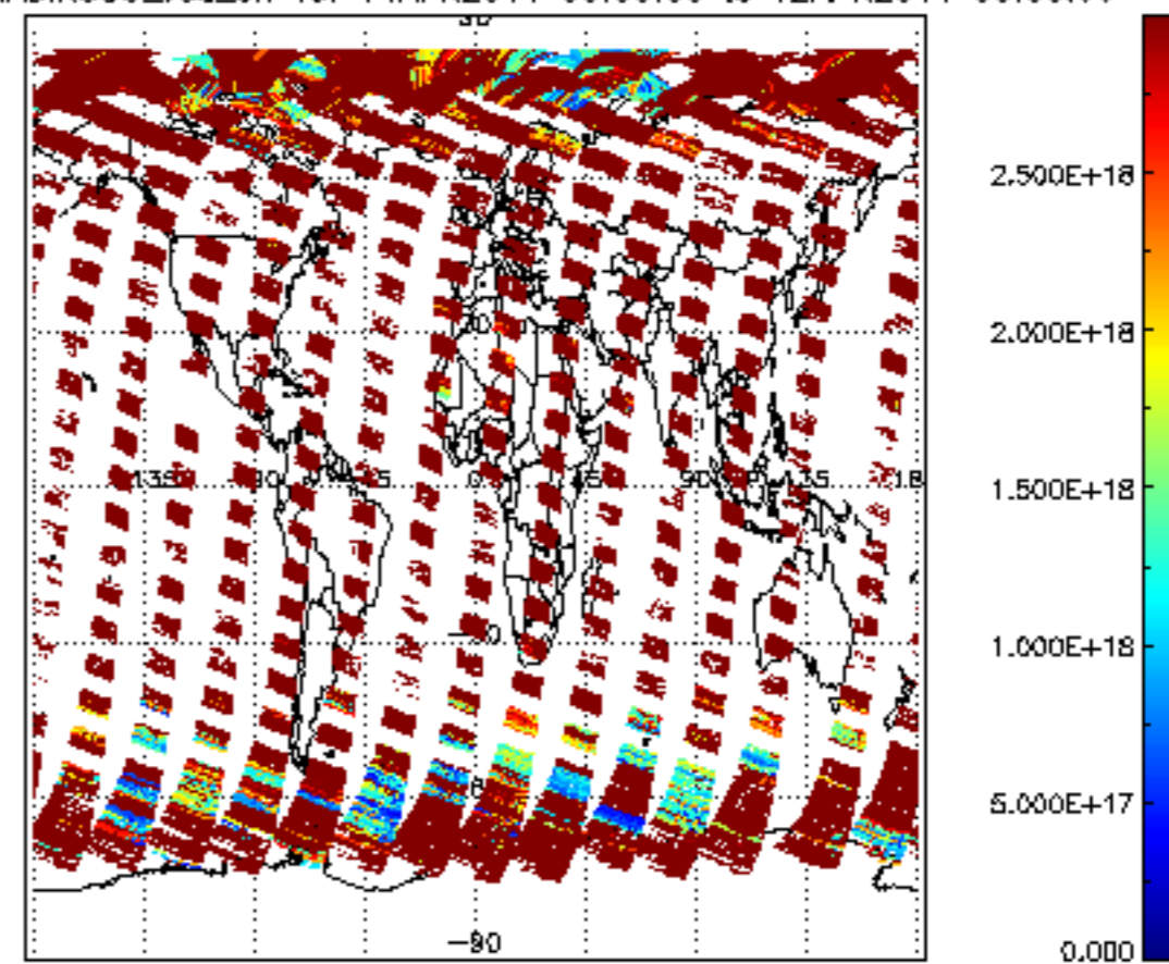
SCIOL2P_NADIR3CO_vcd_err for 11APR2011 00:00:00 to 12APR2011 00:00:00
