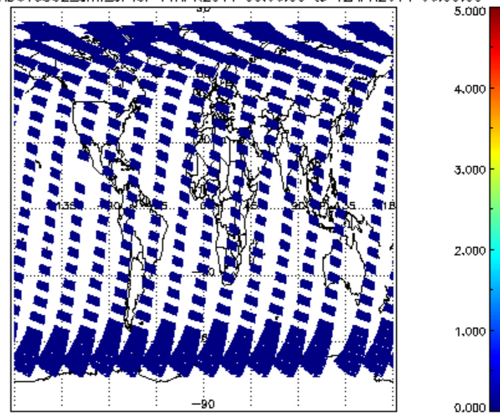
SCIOL2P_NADUV5S02_amf_cl for 11APR2011 00:00:00 to 12APR2011 00:00:00
