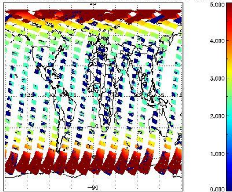
SCIOL2P_NADUV1NO2_amf_cl for 11APR2011 00:00:00 to 12APR2011 00:00:00
