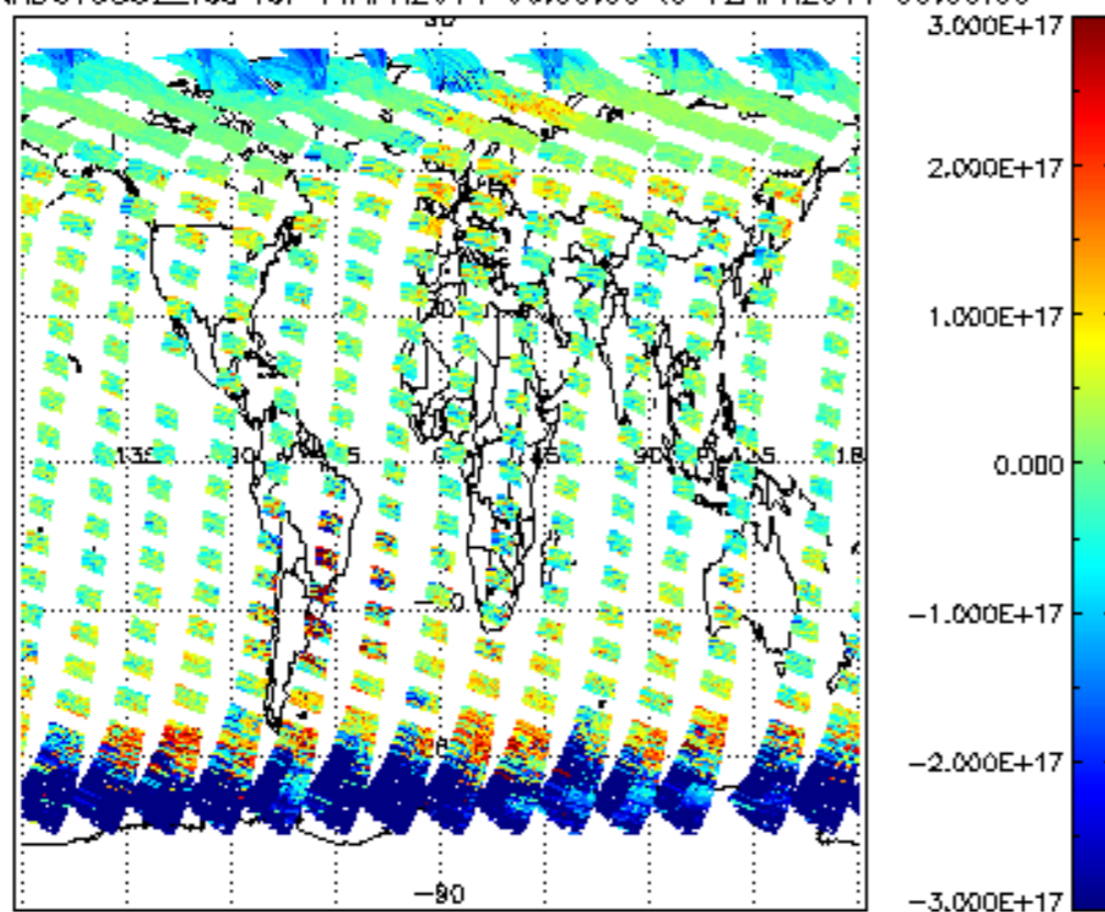
SCIOL2P_NADUV5S02_vcd for 11APR2011 00:00:00 to 12APR2011 00:00:00
