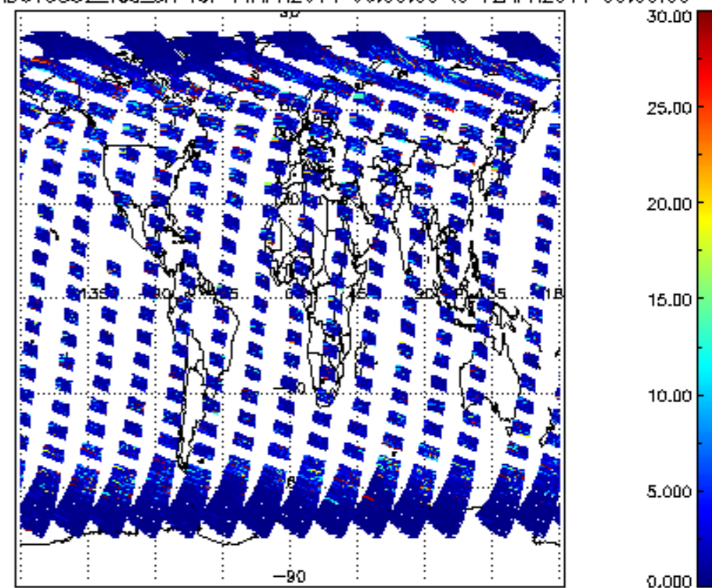
SCIOL2P_NADUV5S02_vcd_err for 11APR2011 00:00:00 to 12APR2011 00:00:00
