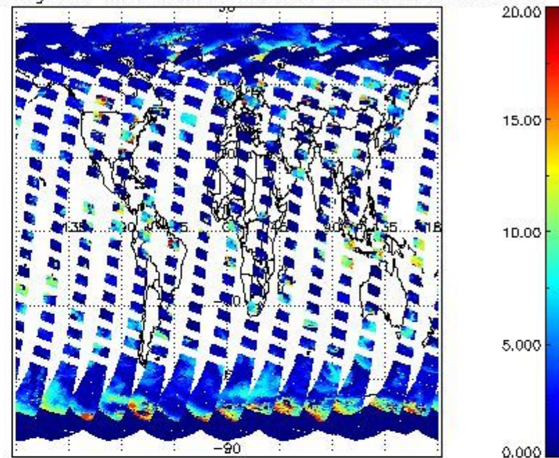
cL_top_height for 11APR2011 00:00:00 to 12APR2011 00:00:00
