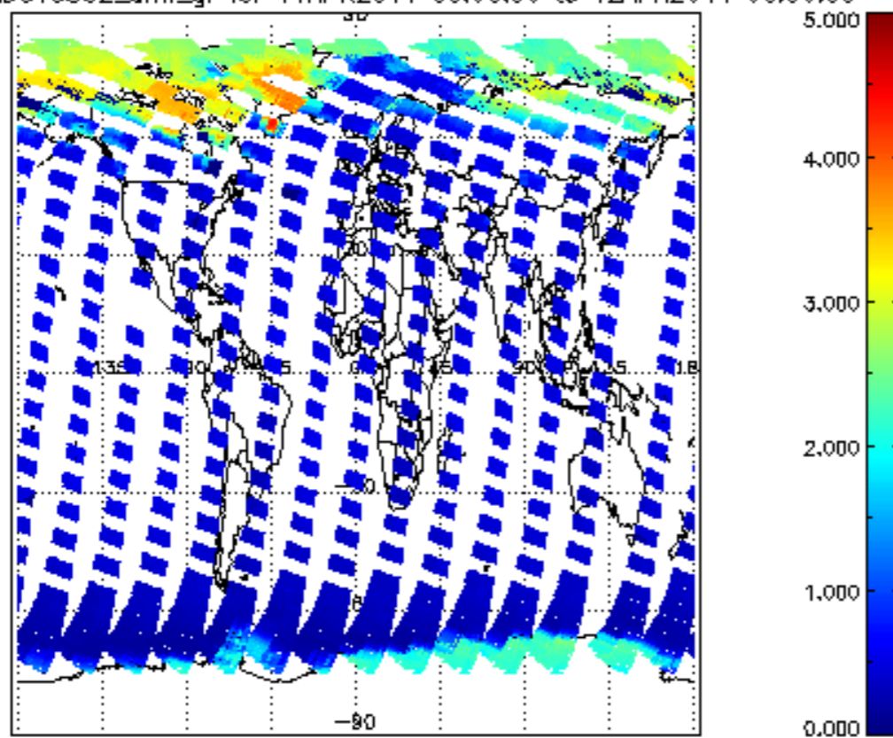
SCIOL2P_NADUV5S02_amf_gr for 11APR2011 00:00:00 to 12APR2011 00:00:00
