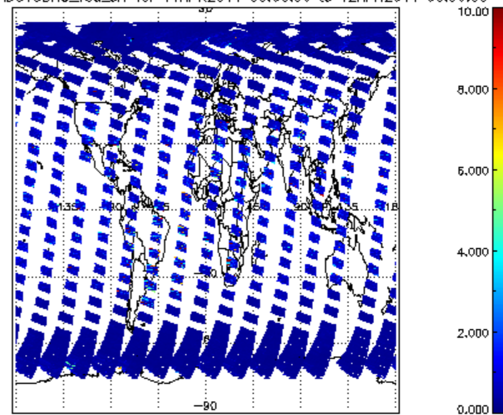
SCIOL2P_NADUV3BRO_vcd_err for 11APR2011 00:00:00 to 12APR2011 00:00:00
