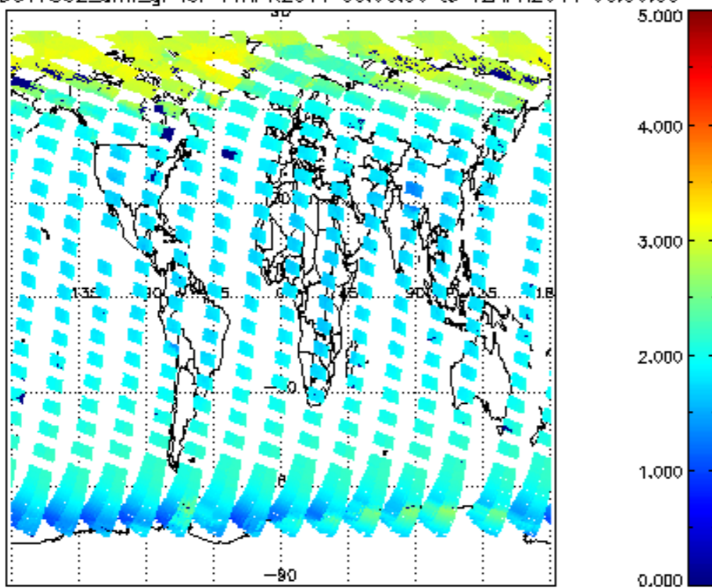
SCIOL2P_NADUV7S02_amf_gr for 11APR2011 00:00:00 to 12APR2011 00:00:00
