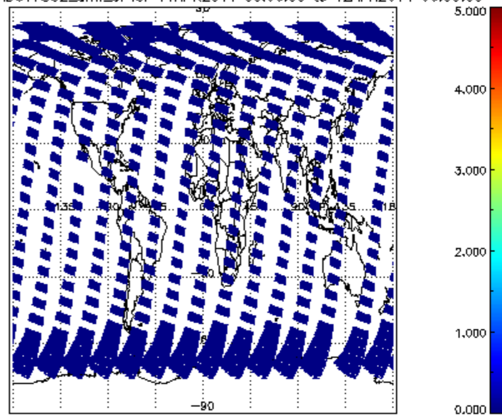
SCIOL2P_NADUV7S02_amf_cl for 11APR2011 00:00:00 to 12APR2011 00:00:00
