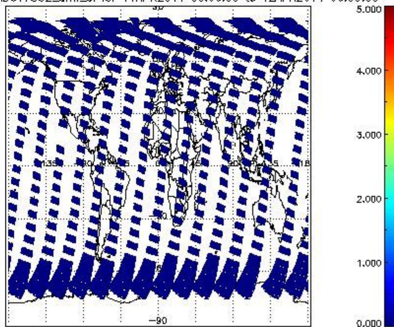
SCIOL2P_NADUV7S02_amf_cl for 11APR2011 00:00:00 to 12APR2011 00:00:00
