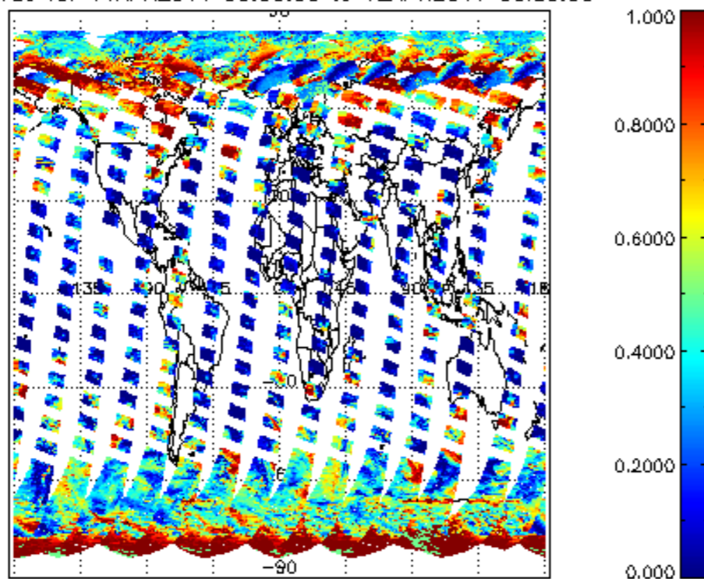
cL_frac for 11APR2011 00:00:00 to 12APR2011 00:00:00
