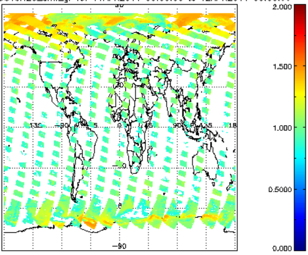
SCIOL2P_NADUV8H2O_amf_gr for 11APR2011 00:00:00 to 12APR2011 00:00:00
