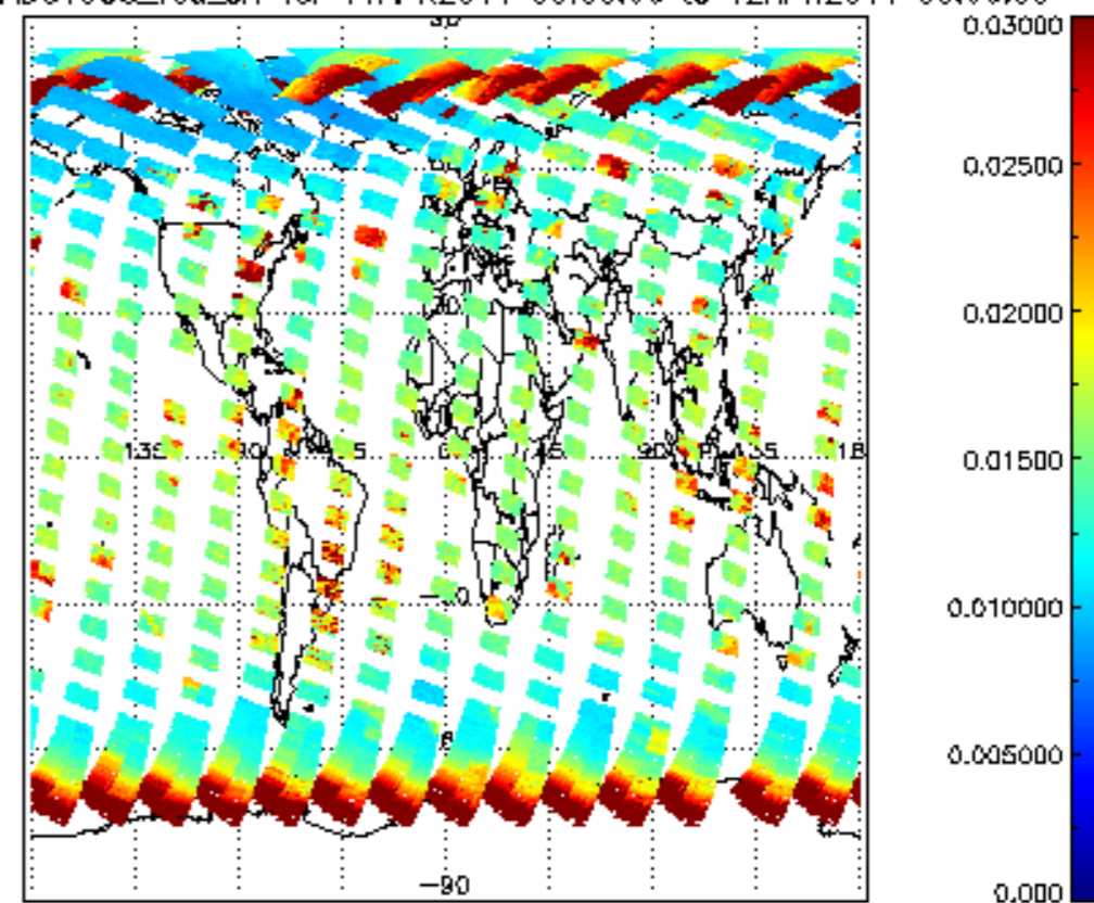
SCIOL2P_NADUV003_vcd_err for 11APR2011 00:00:00 to 12APR2011 00:00:00
