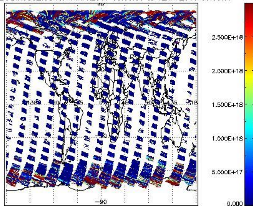
SCIDL2P_NADIR3CO_vcd for 11APR2011 00:00:00 to 12APR2011 00:00:00
