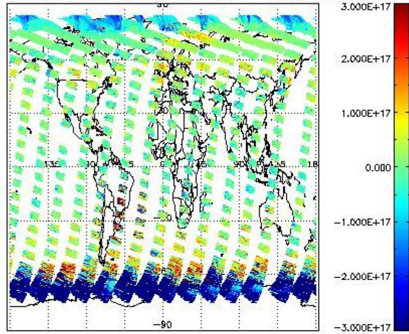
SCIOL2P_NADUV5S02_vcd for 11APR2011 00:00:00 to 12APR2011 00:00:00
