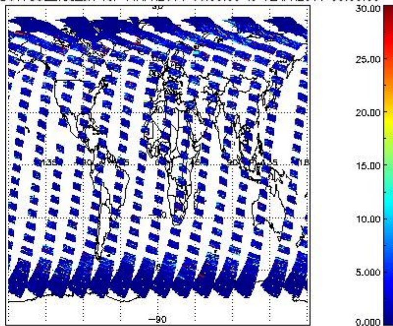
SCIOL2P_NADUV7S02_vcd_err for 11APR2011 00:00:00 to 12APR2011 00:00:00
