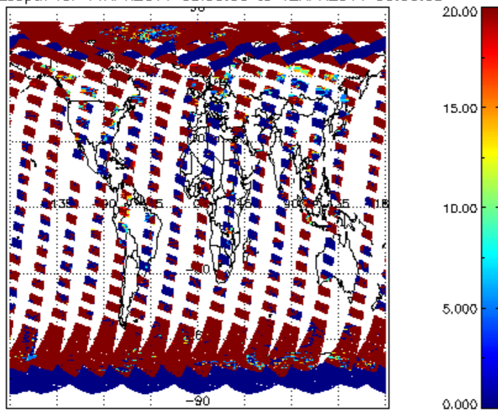
cL_opt_depth for 11APR2011 00:00:00 to 12APR2011 00:00:00
