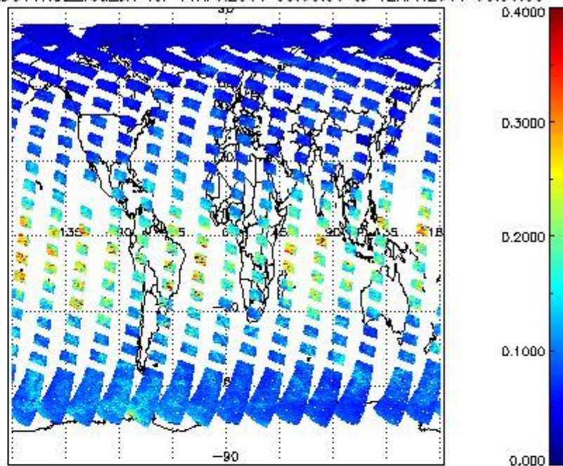
SCIOL2P_NADUV1NO2_vcd_err for 11APR2011 00:00:00 to 12APR2011 00:00:00
