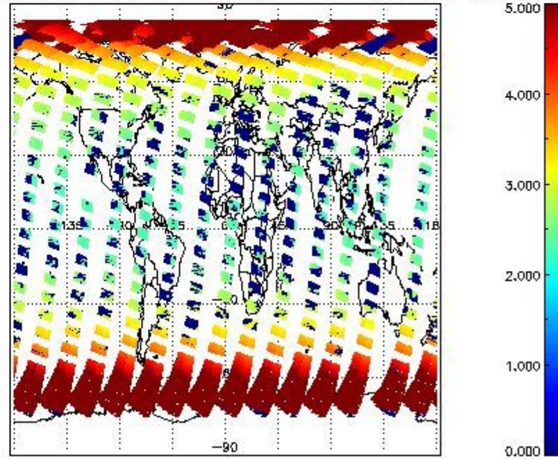
SCIOL2P_NADUV3BRO_amf_cl for 11APR2011 00:00:00 to 12APR2011 00:00:00
