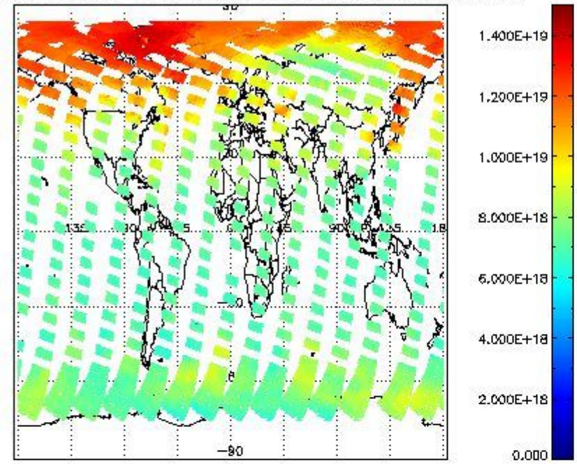
SCIOL2P_NADUV003_vcd for 11APR2011 00:00:00 to 12APR2011 00:00:00
