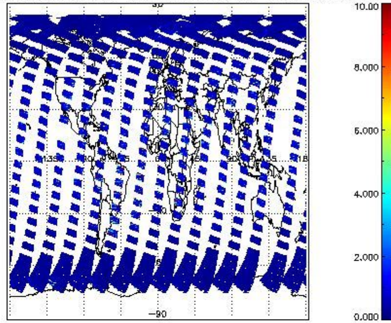
SCIOL2P_NADUV3BRO_vcd_err for 11APR2011 00:00:00 to 12APR2011 00:00:00
