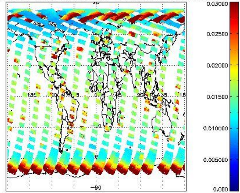
SCIOL2P_NADUV003_vcd_err for 11APR2011 00:00:00 to 12APR2011 00:00:00
