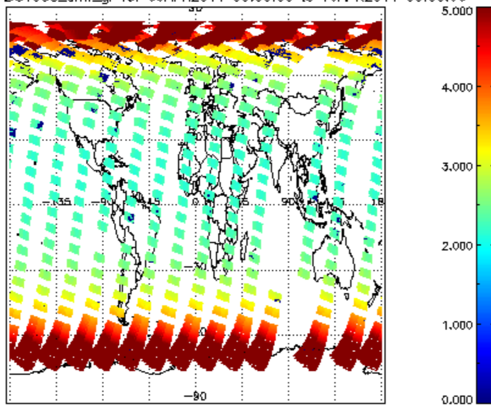
SCIOL2P_NADUV003_amf_gr for 09APR2011 00:00:00 to 10APR2011 00:00:00
