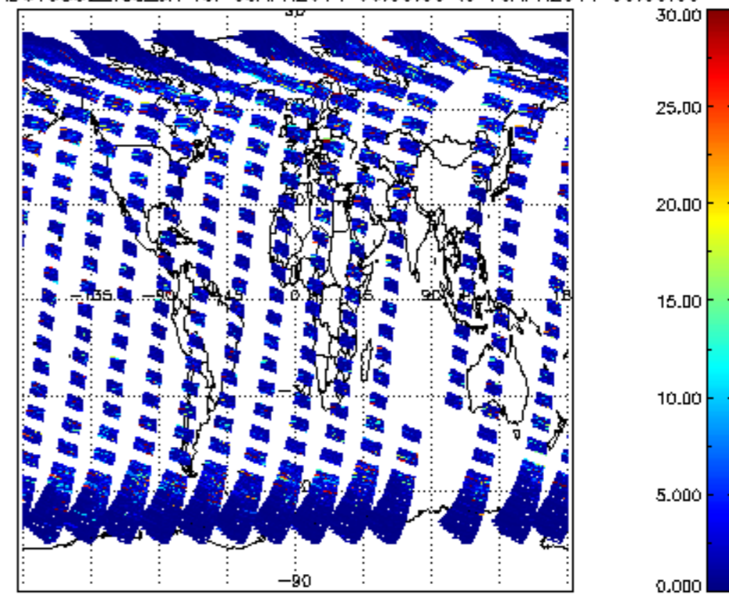
SCIOL2P_NADUV5S02_vcd_err for 09APR2011 00:00:00 to 10APR2011 00:00:00
