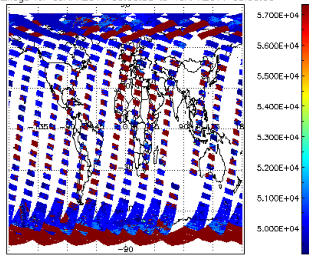
cloud_flags for 09APR2011 00:00:00 to 10APR2011 00:00:00
