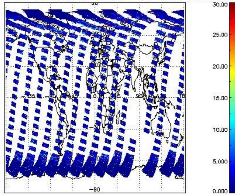
SCIOL2P_NADUV7S02_vcd_err for 09APR2011 00:00:00 to 10APR2011 00:00:00
