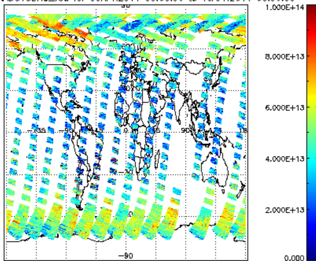
SCIOL2P_NADUV3BRO_vcd for 09APR2011 00:00:00 to 10APR2011 00:00:00
