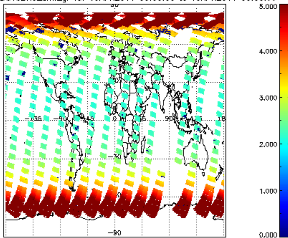
SCIOL2P_NADUV3BRO_amf_gr for 09APR2011 00:00:00 to 10APR2011 00:00:00
