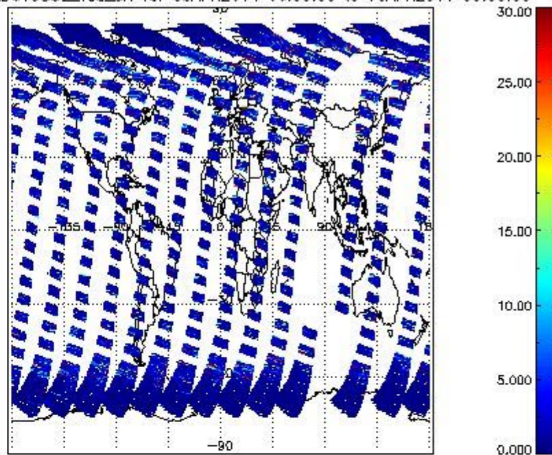
SCIOL2P_NADUV5S02_vcd_err for 09APR2011 00:00:00 to 10APR2011 00:00:00
