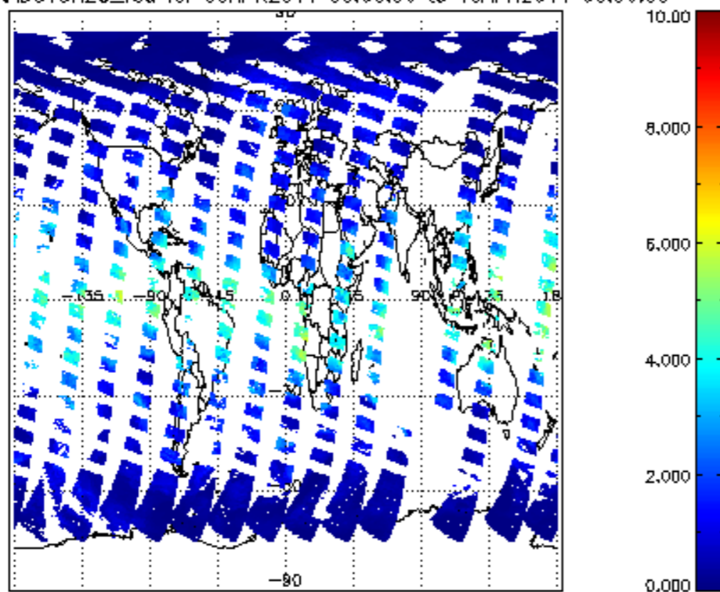
SCIOL2P_NADUV8H2O_vcd for 09APR2011 00:00:00 to 10APR2011 00:00:00
