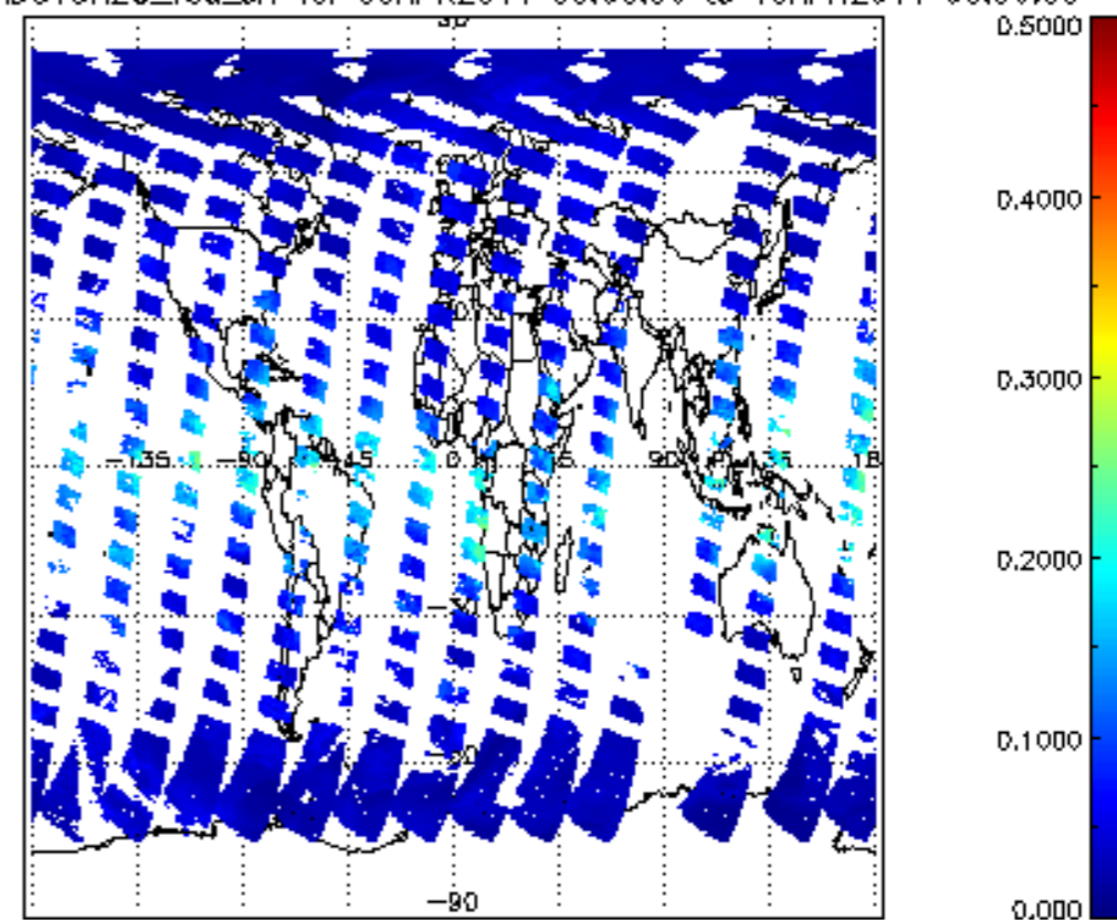
SCIOL2P_NADUV8H2O_vcd_err for 09APR2011 00:00:00 to 10APR2011 00:00:00
