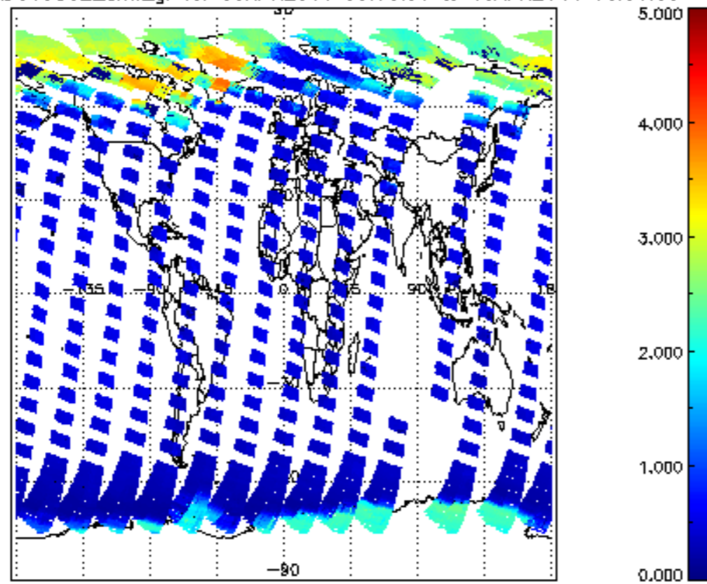
SCIOL2P_NADUV5S02_amf_gr for 09APR2011 00:00:00 to 10APR2011 00:00:00
