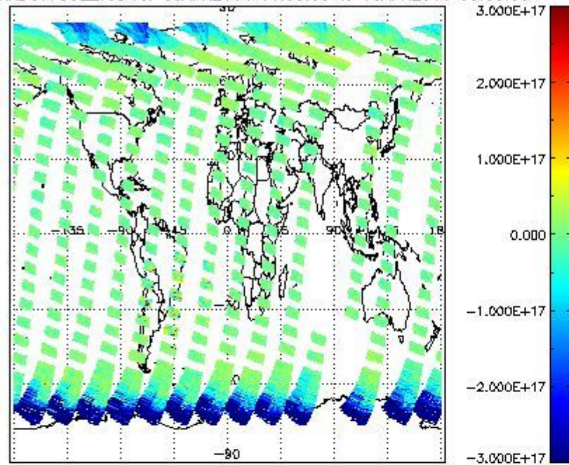
SCIOL2P_NADUV7S02_vcd for 09APR2011 00:00:00 to 10APR2011 00:00:00
