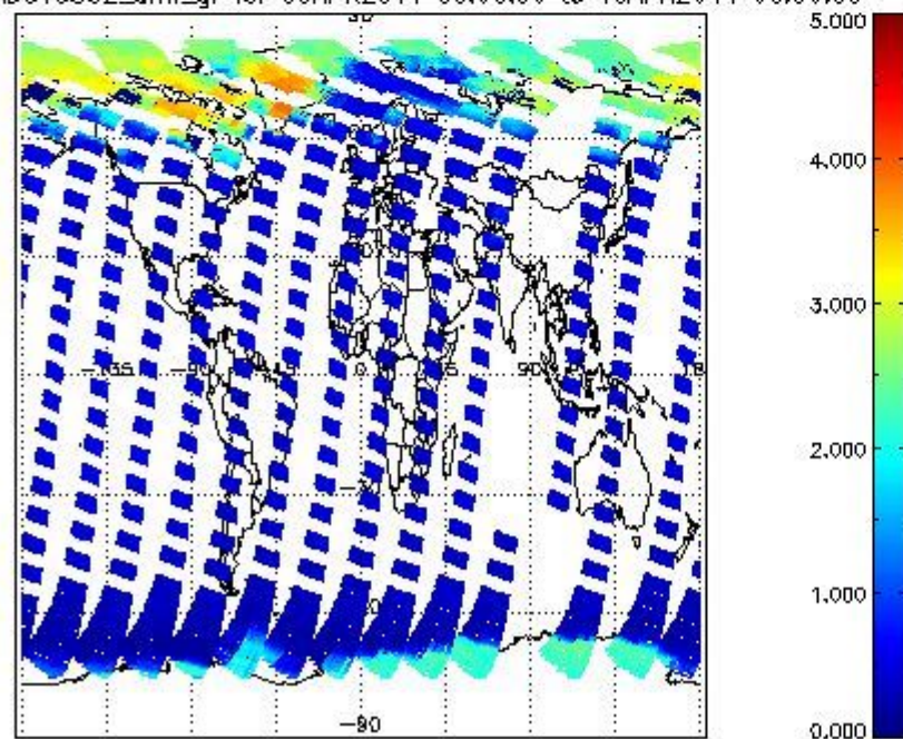
SCIOL2P_NADUV5S02_amf_gr for 09APR2011 00:00:00 to 10APR2011 00:00:00
