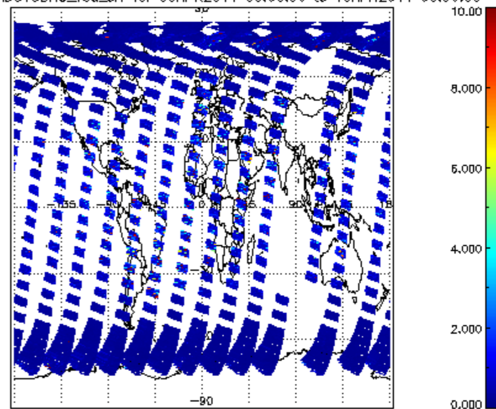
SCIOL2P_NADUV3BRO_vcd_err for 09APR2011 00:00:00 to 10APR2011 00:00:00
