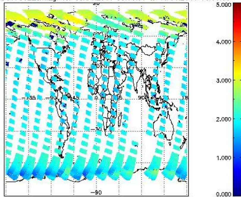
SCIOL2P_NADUV7S02_amf_gr for 09APR2011 00:00:00 to 10APR2011 00:00:00
