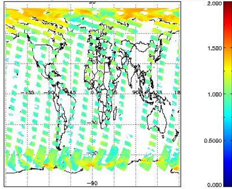
SCIOL2P_NADUV8H2O_arnf_gr for 09APR2011 00:00:00 to 10APR2011 00:00:00
