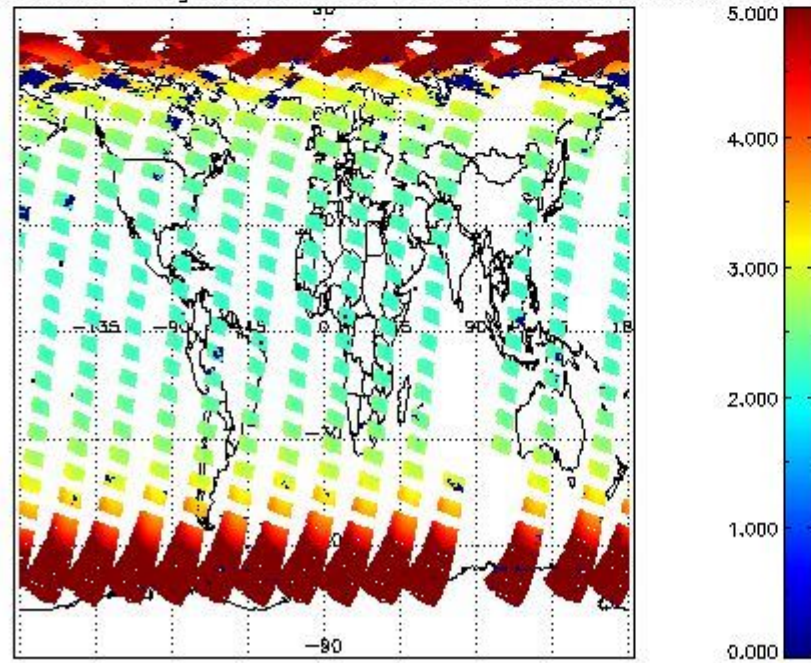
SCIOL2P_NADUV1NO2_amf_gr for 09APR2011 00:00:00 to 10APR2011 00:00:00
