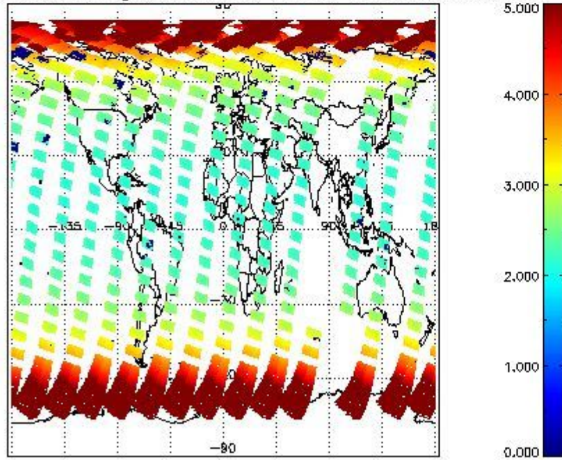
SCIOL2P_NADUV3BRO_amf_gr for 09APR2011 00:00:00 to 10APR2011 00:00:00
