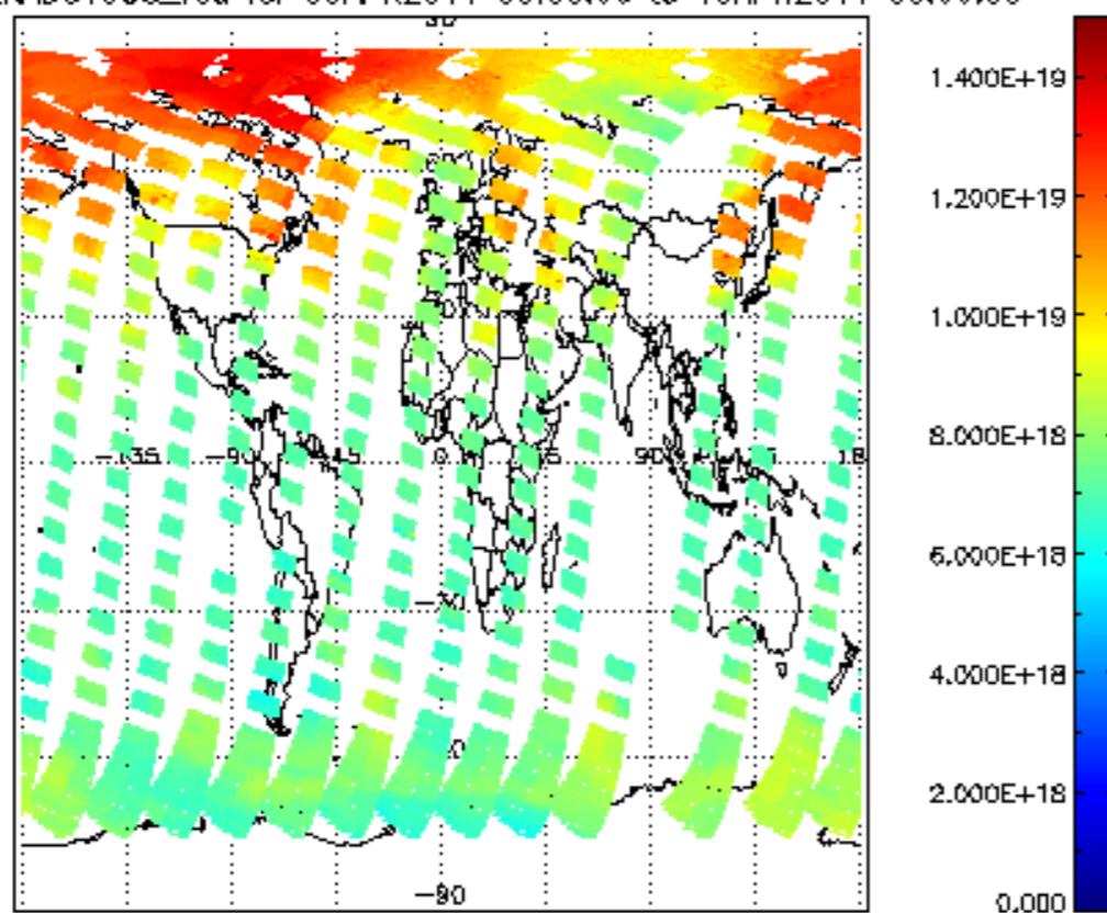
SCIOL2P_NADUV003_vcd for 09APR2011 00:00:00 to 10APR2011 00:00:00
