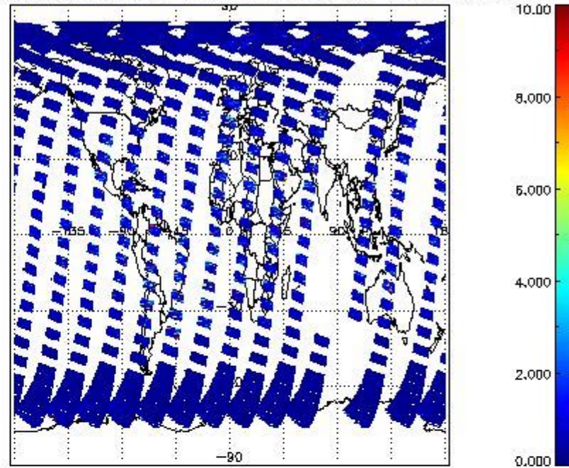
SCIOL2P_NADUV3BRO_vcd_err for 09APR2011 00:00:00 to 10APR2011 00:00:00
