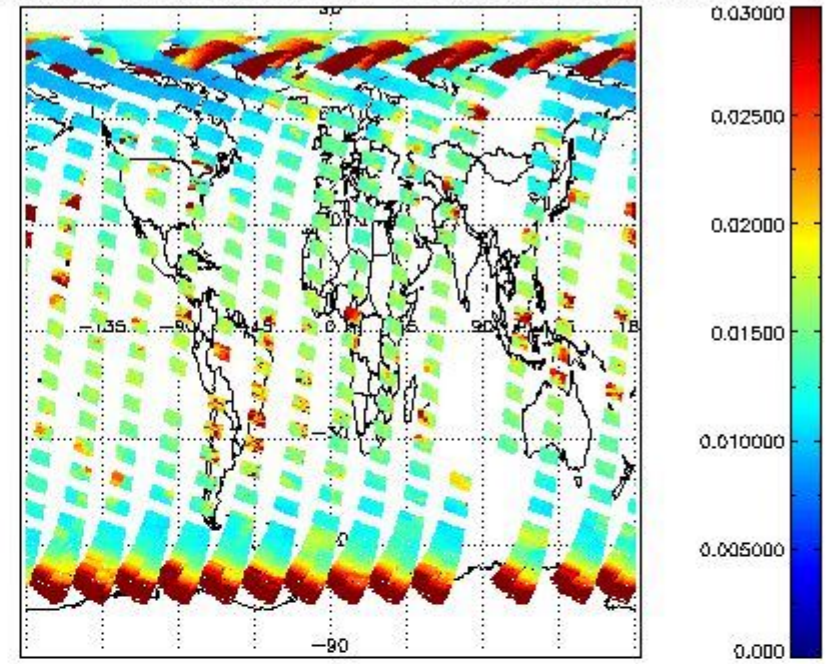
SCIOL2P_NADUV003_vcd_err for 09APR2011 00:00:00 to 10APR2011 00:00:00
