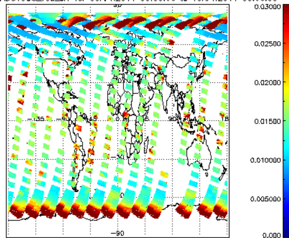
SCIOL2P_NADUV003_vcd_err for 09APR2011 00:00:00 to 10APR2011 00:00:00
