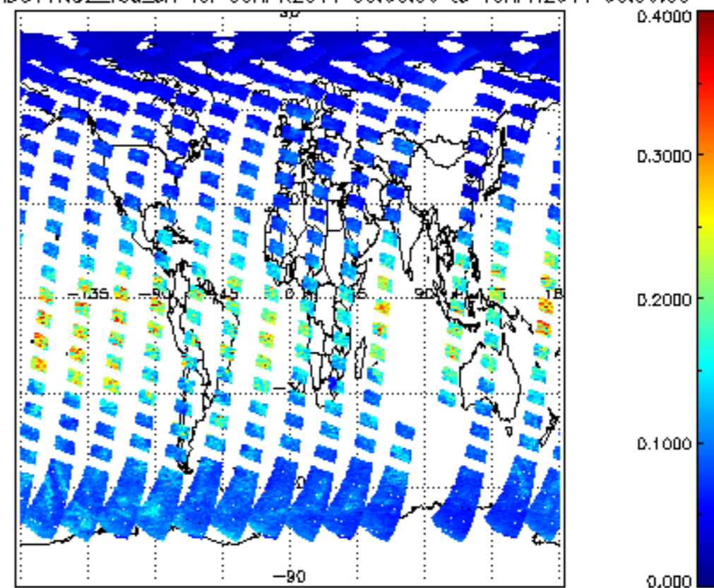
SCIOL2P_NADUV1NO2_vcd_err for 09APR2011 00:00:00 to 10APR2011 00:00:00
