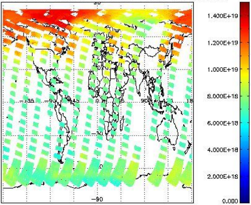
SCIOL2P_NADUV003_vcd for 09APR2011 00:00:00 to 10APR2011 00:00:00
