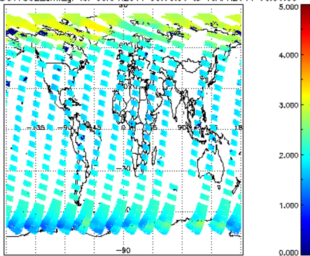
SCIOL2P_NADUV7S02_amf_gr for 09APR2011 00:00:00 to 10APR2011 00:00:00
