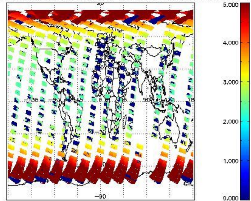
SCIOL2P_NADUV003_amf_cl for 09APR2011 00:00:00 to 10APR2011 00:00:00
