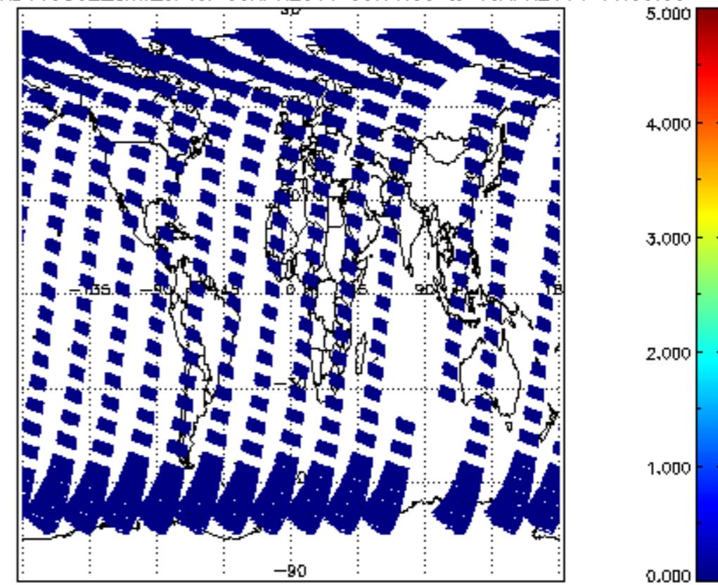
SCIOL2P_NADUV5S02_amf_cl for 09APR2011 00:00:00 to 10APR2011 00:00:00
