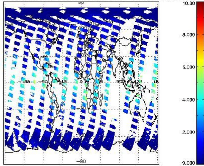
SCIOL2P_NADUV8H2O_vcd for 09APR2011 00:00:00 to 10APR2011 00:00:00
