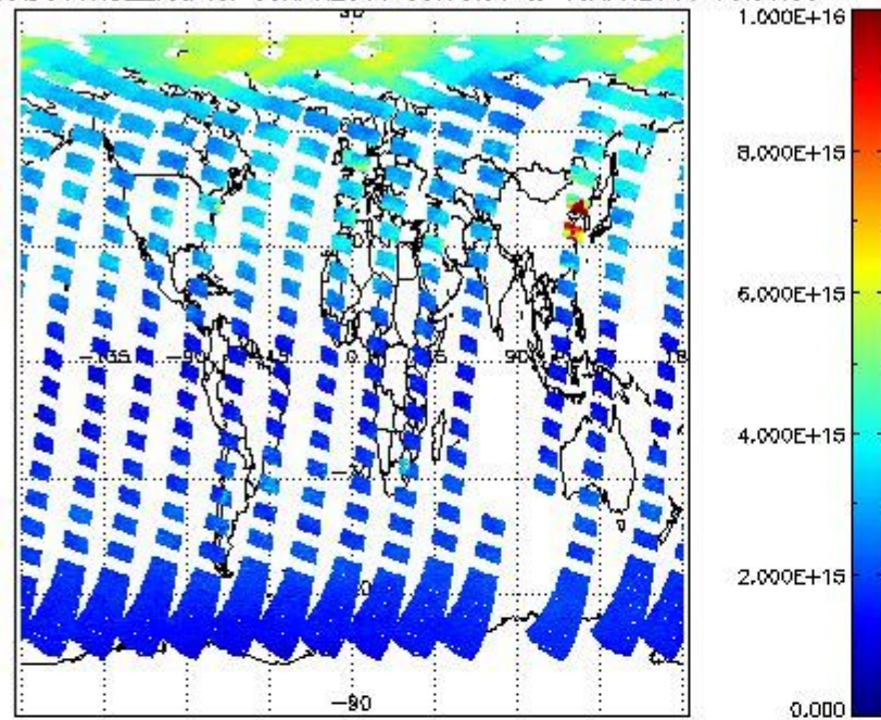
SCIOL2P_NADUV1NO2_vcd for 09APR2011 00:00:00 to 10APR2011 00:00:00
