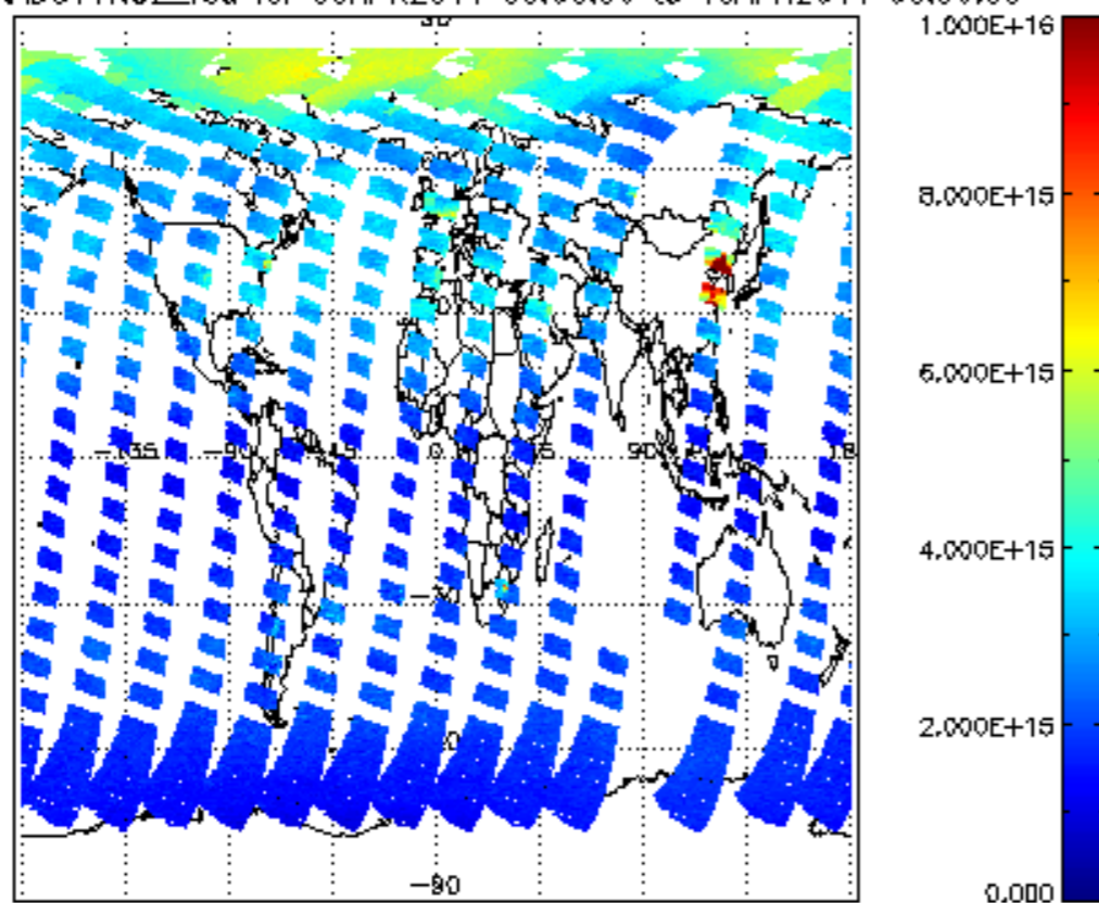
SCIOL2P_NADUV1NO2_vcd for 09APR2011 00:00:00 to 10APR2011 00:00:00
