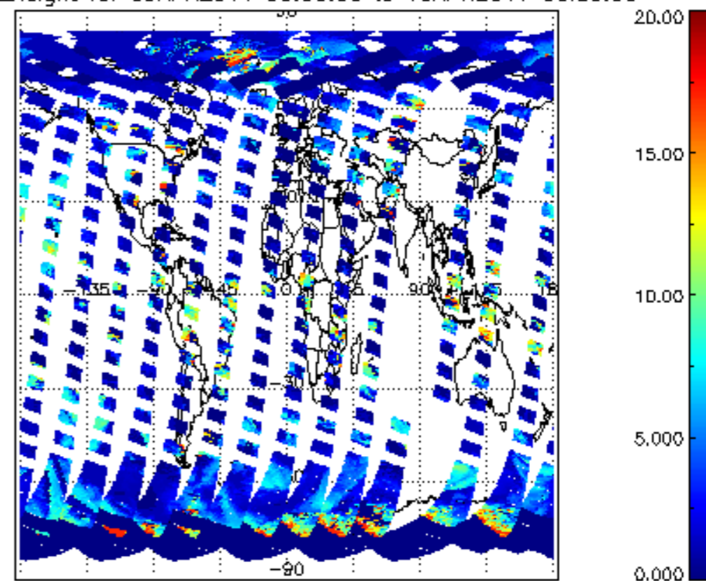
cL_top_height for 09APR2011 00:00:00 to 10APR2011 00:00:00
