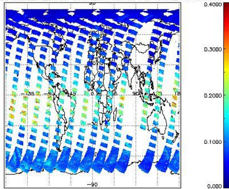
SCIOL2P_NADUV1NO2_vcd_err for 09APR2011 00:00:00 to 10APR2011 00:00:00
