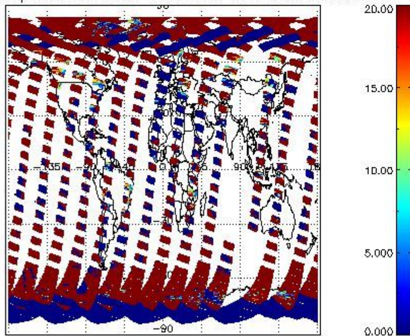
cL_opt_depth for 09APR2011 00:00:00 to 10APR2011 00:00:00
