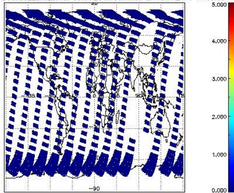
SCIOL2P_NADUV7S02_amf_cl for 09APR2011 00:00:00 to 10APR2011 00:00:00
