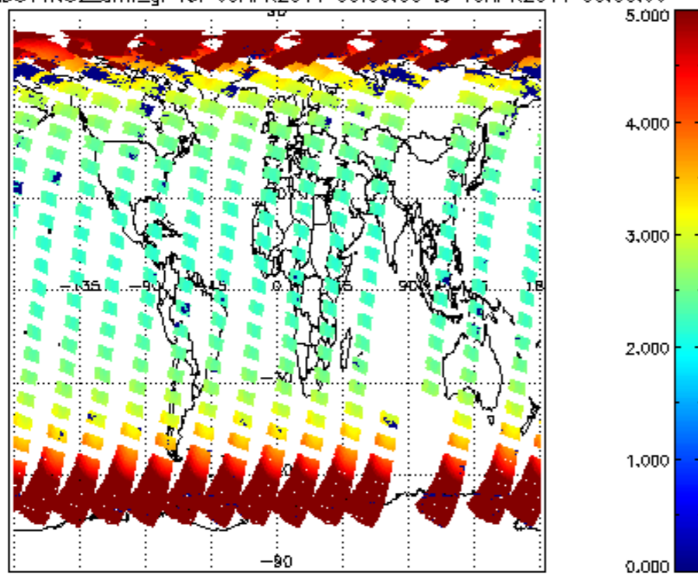
SCIOL2P_NADUV1NO2_amf_gr for 09APR2011 00:00:00 to 10APR2011 00:00:00
