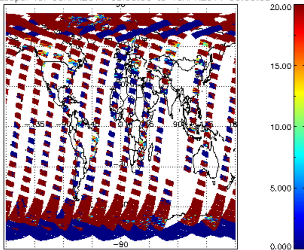
cL_opt_depth for 09APR2011 00:00:00 to 10APR2011 00:00:00
