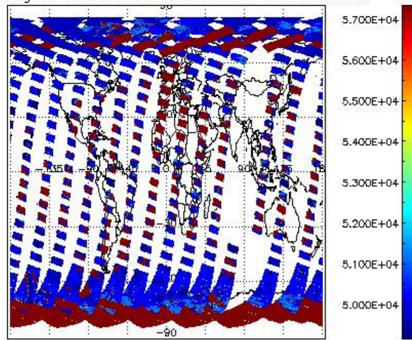
cloud_flags for 09APR2011 00:00:00 to 10APR2011 00:00:00
