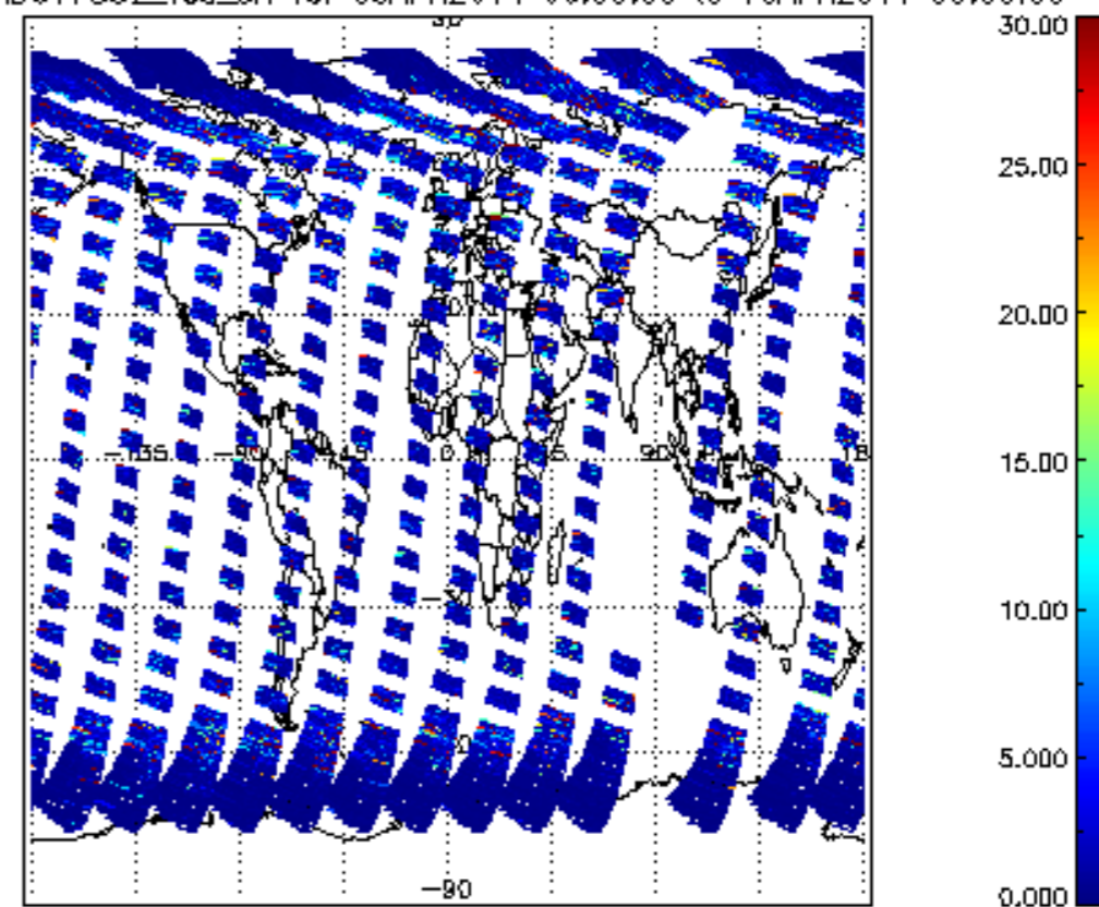
SCIOL2P_NADUV7S02_vcd_err for 09APR2011 00:00:00 to 10APR2011 00:00:00
