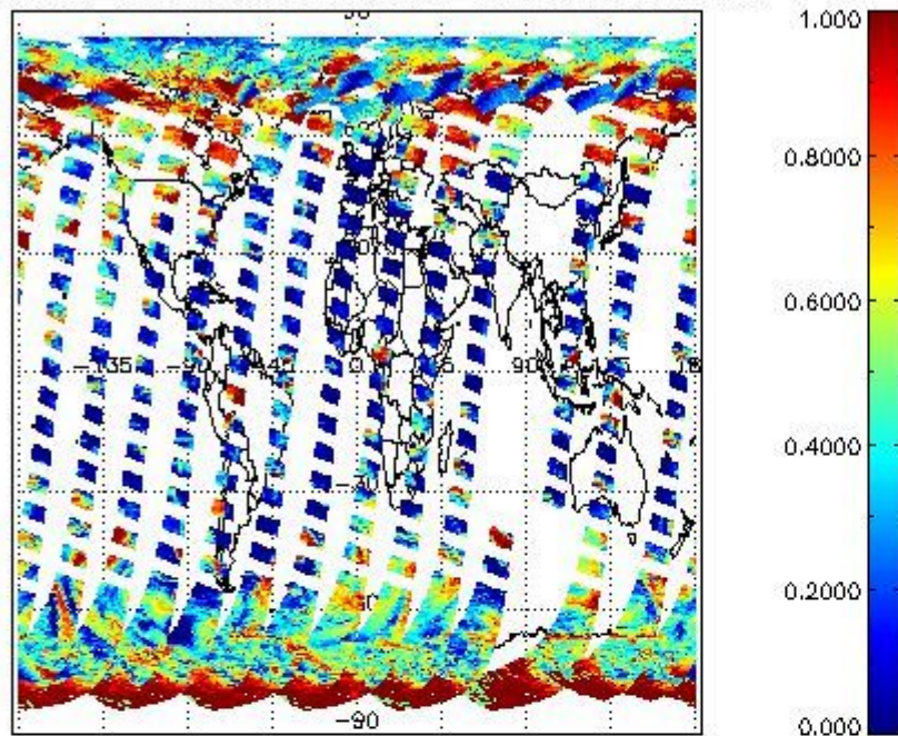
cL_frac for 09APR2011 00:00:00 to 10APR2011 00:00:00
