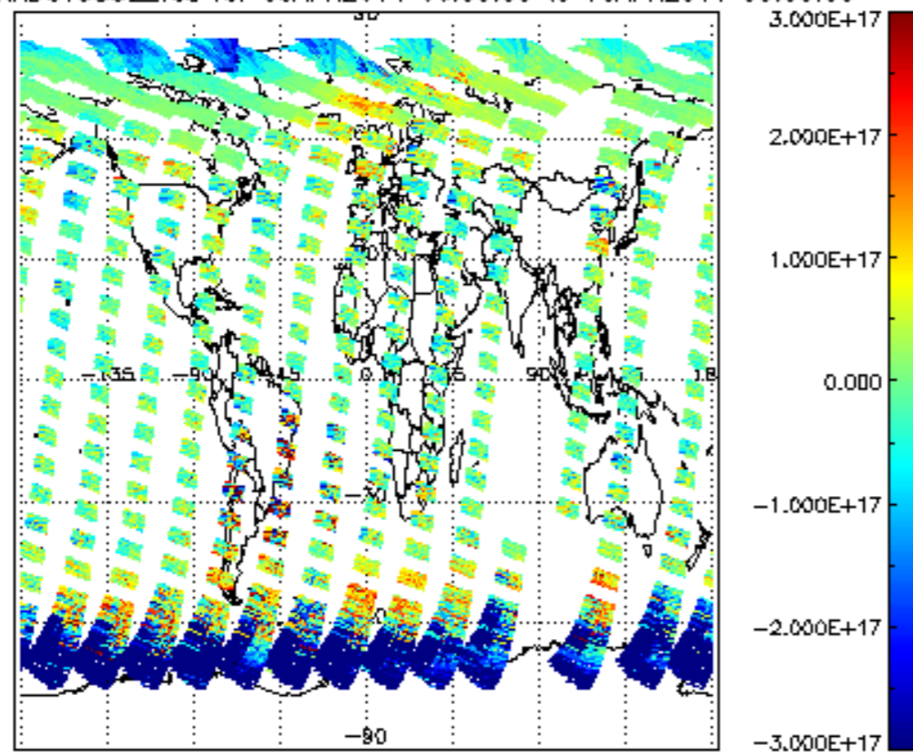
SCIOL2P_NADUV5S02_vcd for 09APR2011 00:00:00 to 10APR2011 00:00:00
