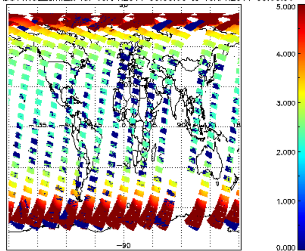
SCIOL2P_NADUV1NO2_amf_cl for 09APR2011 00:00:00 to 10APR2011 00:00:00
