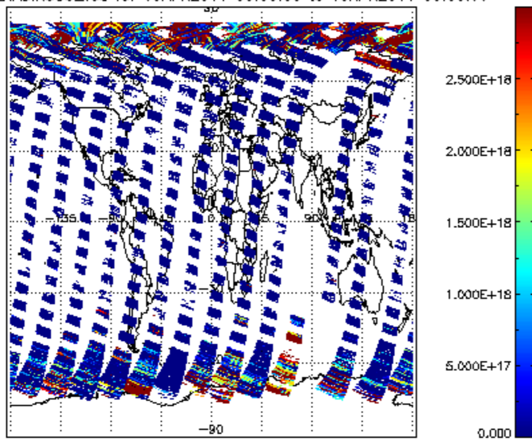
SCIOL2P_NADIR3CO_vcd for 09APR2011 00:00:00 to 10APR2011 00:00:00
