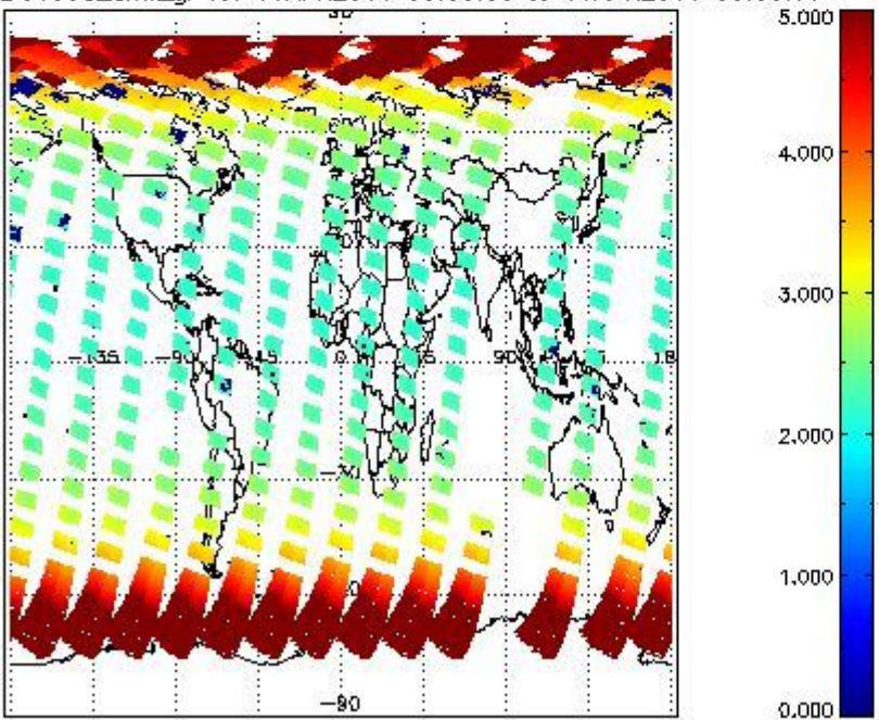
SCIOL2P_NADUV003_amf_gr for 09APR2011 00:00:00 to 10APR2011 00:00:00
