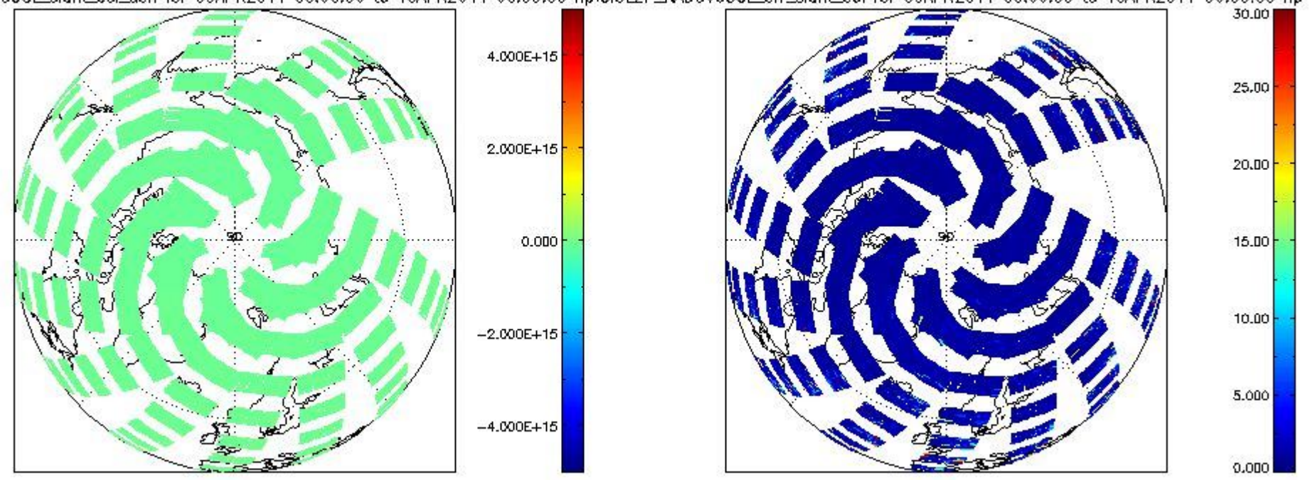
CIOL2P_NADUV60CLslant_col_den for 09APR2011 00:00:00 to 10APR2011 00:00:00 np; CIOL2P_NADUV60CLerr_slant_col for 09APR2011 00:00:00 to 10APR2011 00:00:00 np
