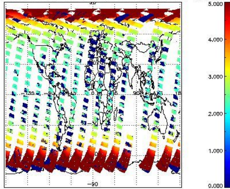
SCIOL2P_NADUV1NO2_amf_cl for 09APR2011 00:00:00 to 10APR2011 00:00:00
