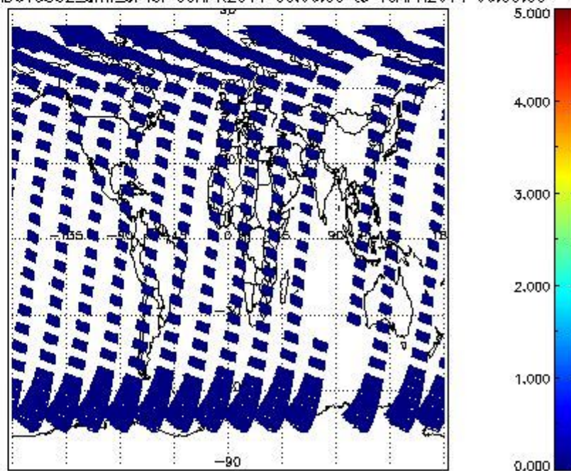
SCIOL2P_NADUV5S02_amf_cl for 09APR2011 00:00:00 to 10APR2011 00:00:00
