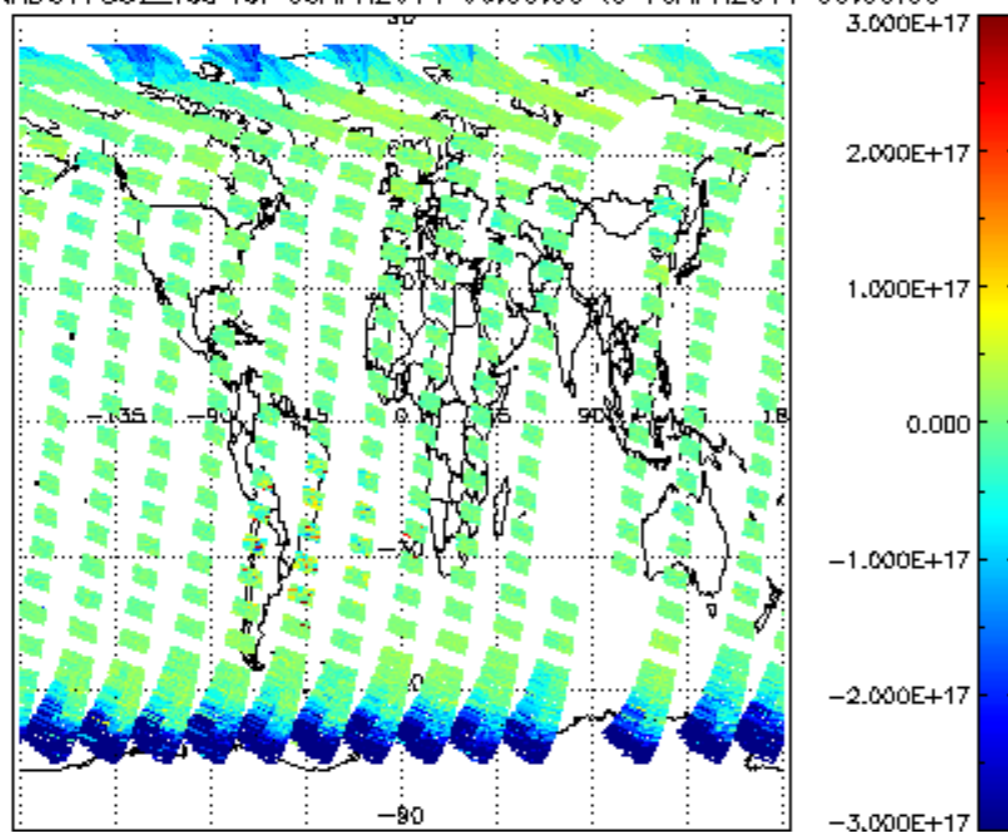
SCIOL2P_NADUV7S02_vcd for 09APR2011 00:00:00 to 10APR2011 00:00:00
