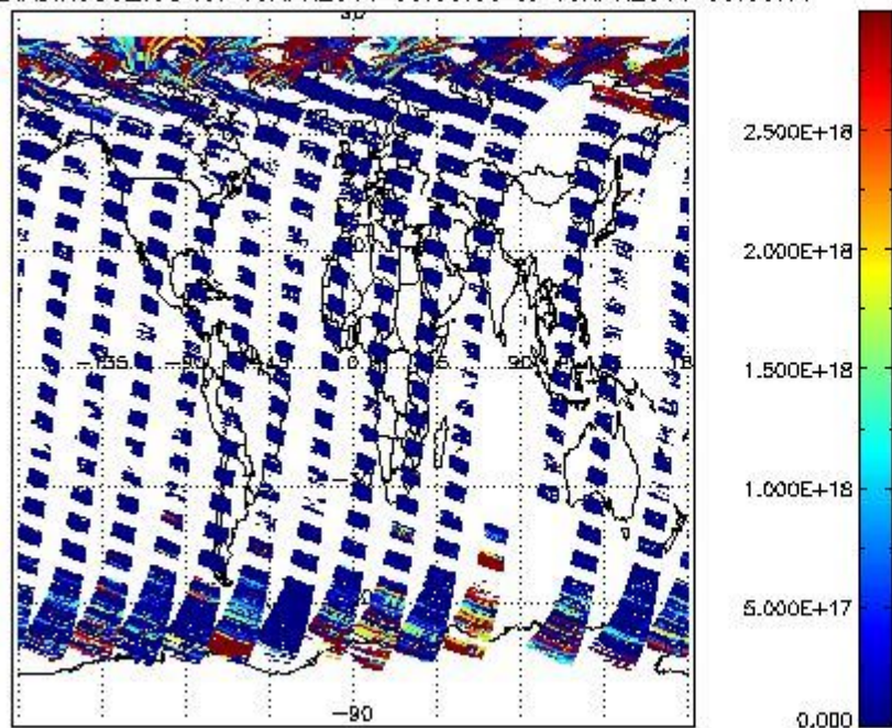
SCIDL2P_NADIR3CO_vcd for 09APR2011 00:00:00 to 10APR2011 00:00:00
