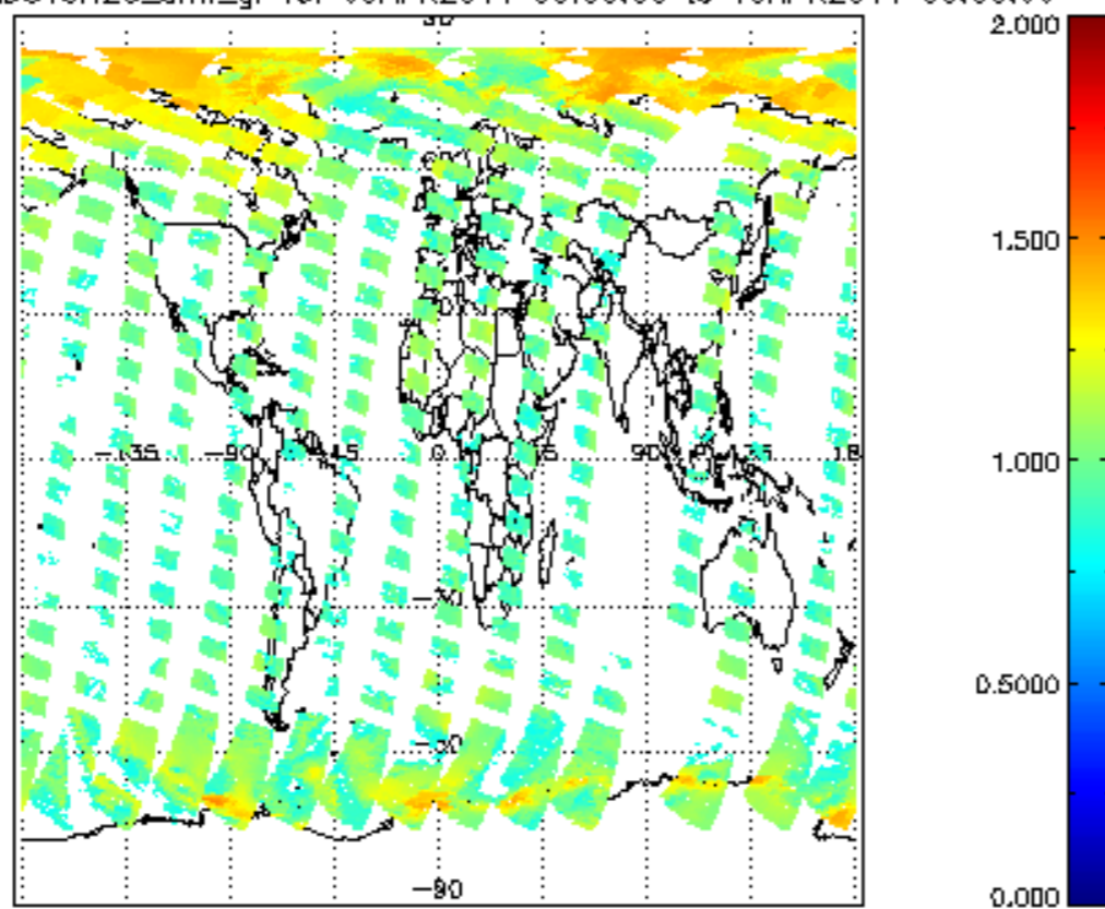
SCIOL2P_NADUV8H2O_amf_gr for 09APR2011 00:00:00 to 10APR2011 00:00:00
