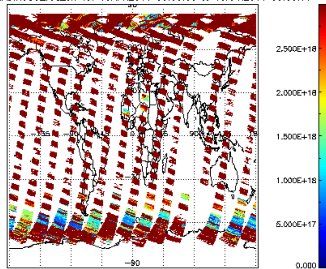
SCIOL2P_NADIR3CO_vcd_err for 09APR2011 00:00:00 to 10APR2011 00:00:00
