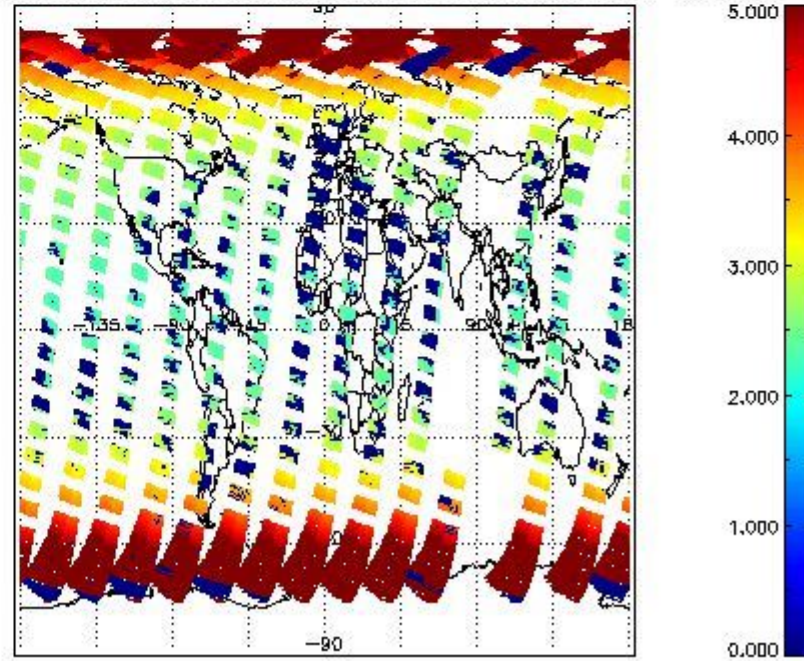
SCIOL2P_NADUV3BRO_amf_cl for 09APR2011 00:00:00 to 10APR2011 00:00:00
