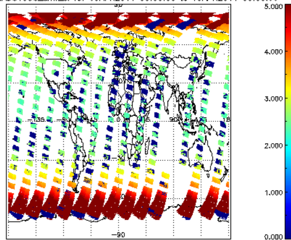
SCIOL2P_NADUV003_amf_cl for 09APR2011 00:00:00 to 10APR2011 00:00:00
