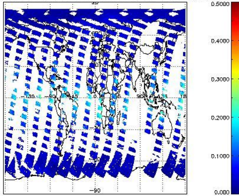
SCIOL2P_NADUV8H2O_vcd_err for 09APR2011 00:00:00 to 10APR2011 00:00:00
