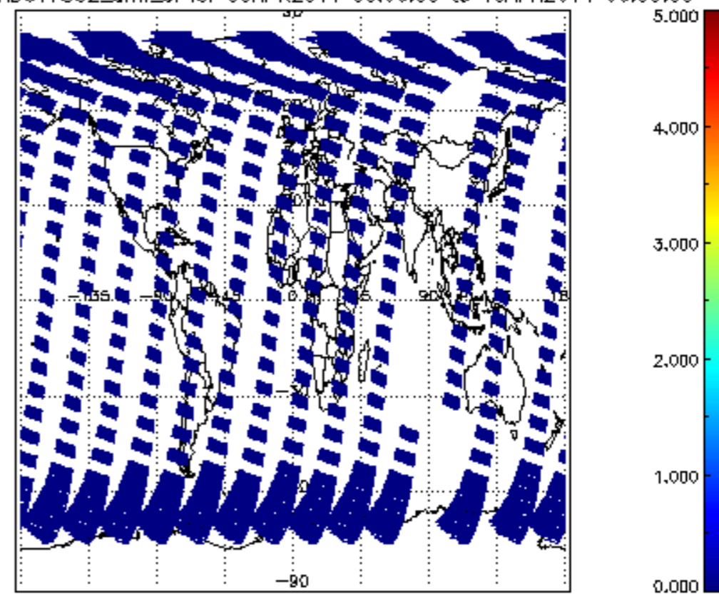
SCIOL2P_NADUV7S02_amf_cl for 09APR2011 00:00:00 to 10APR2011 00:00:00
