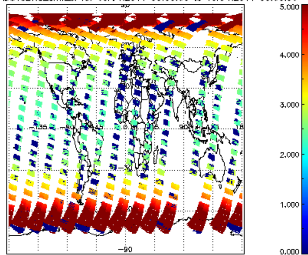
SCIOL2P_NADUV3BRO_amf_sl for 09APR2011 00:00:00 to 10APR2011 00:00:00
