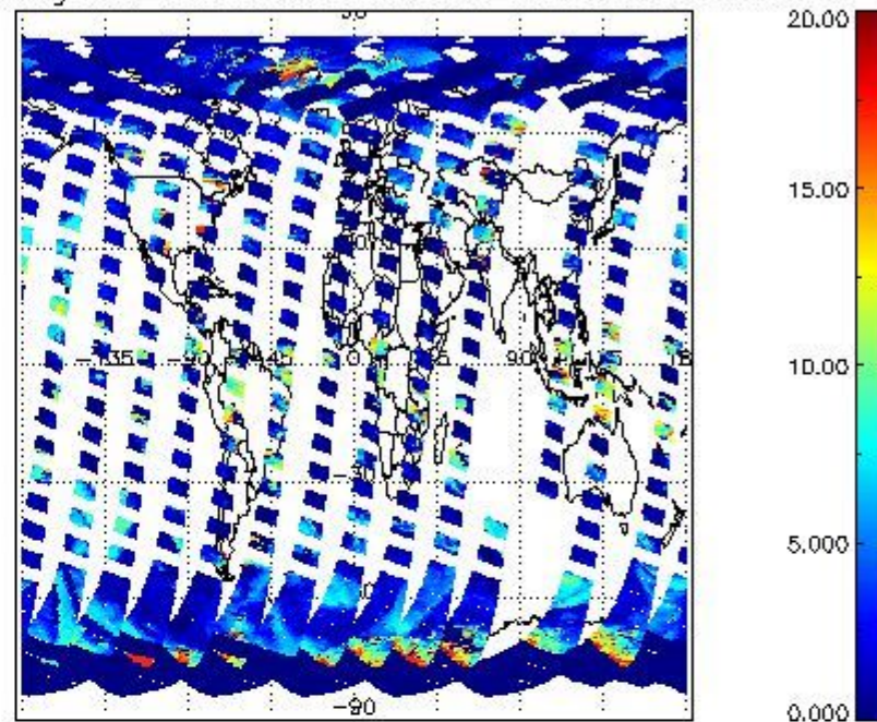
cL_top_height for 09APR2011 00:00:00 to 10APR2011 00:00:00
