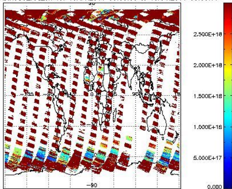
SCIDL2P_NADIR3CO_vcd_err for 09APR2011 00:00:00 to 10APR2011 00:00:00
