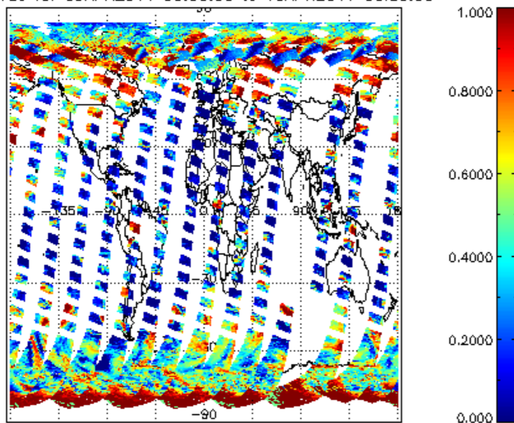
cL_frac for 09APR2011 00:00:00 to 10APR2011 00:00:00
