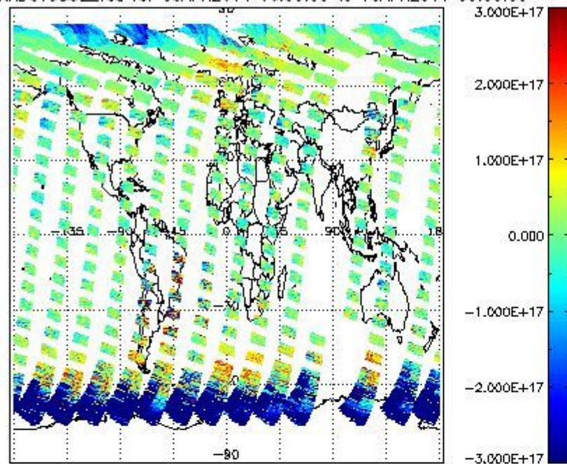
SCIOL2P_NADUV5S02_vcd for 09APR2011 00:00:00 to 10APR2011 00:00:00
