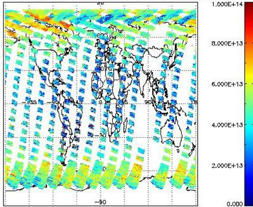
SCIOL2P_NADUV3BRO_vcd for 09APR2011 00:00:00 to 10APR2011 00:00:00
