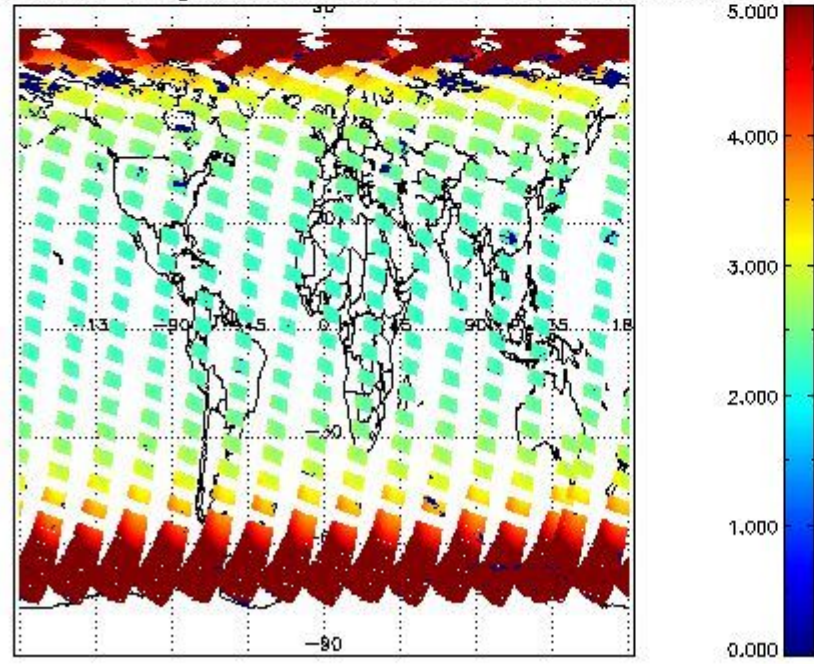
SCIOL2P_NADUV1NO2_amf_gr for 08APR2011 00:00:00 to 09APR2011 00:00:00
