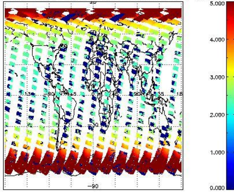
SCIOL2P_NADUV1NO2_amf_cl for 08APR2011 00:00:00 to 09APR2011 00:00:00
