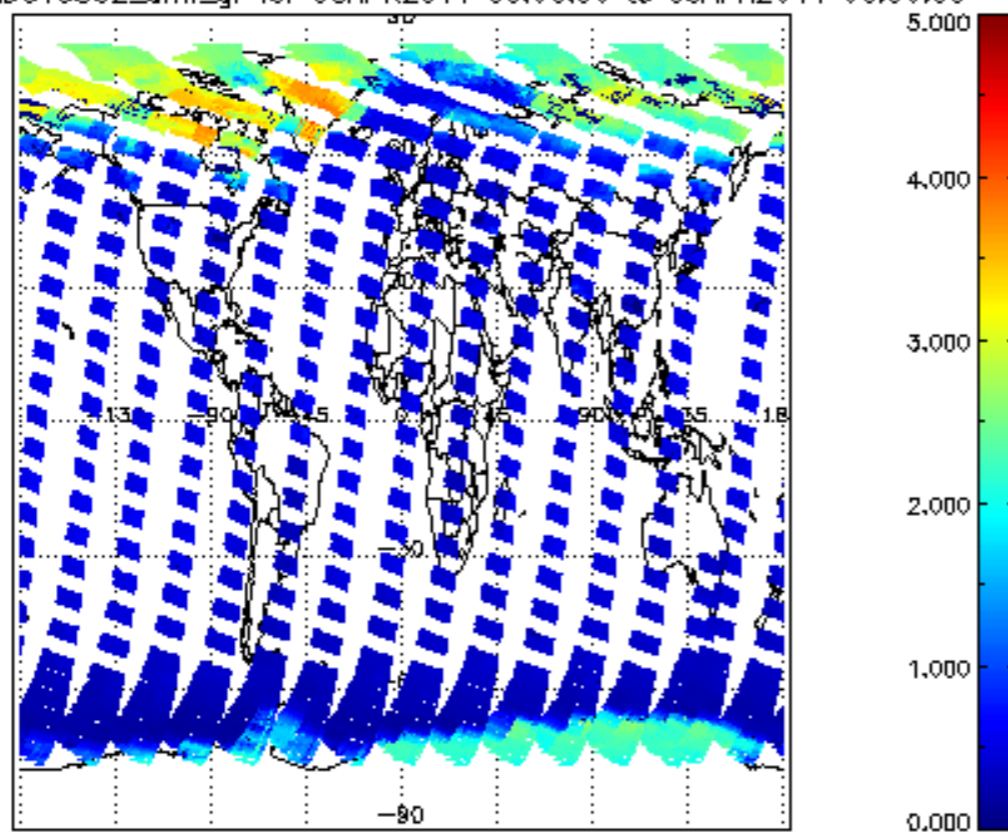
SCIOL2P_NADUV5S02_amf_gr for 08APR2011 00:00:00 to 09APR2011 00:00:00
