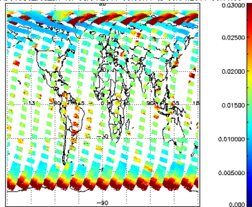
SCIOL2P_NADUV003_vcd_err for 08APR2011 00:00:00 to 09APR2011 00:00:00
