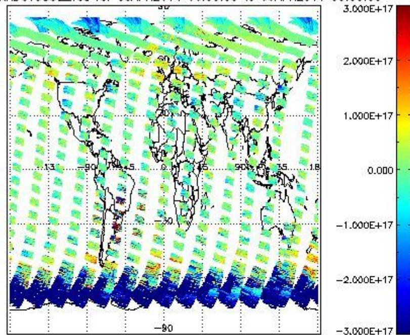
SCIOL2P_NADUV5S02_vcd for 08APR2011 00:00:00 to 09APR2011 00:00:00
