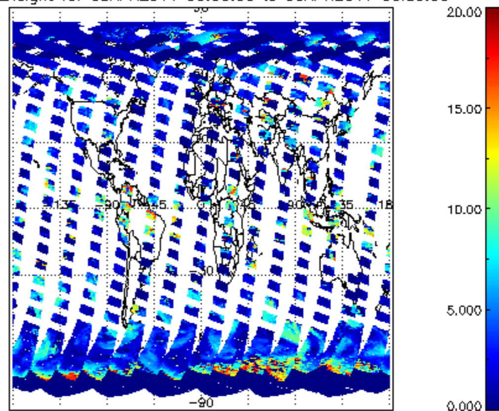
cL_top_height for 08APR2011 00:00:00 to 09APR2011 00:00:00
