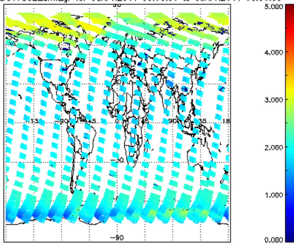
SCIOL2P_NADUV7S02_amf_gr for 08APR2011 00:00:00 to 09APR2011 00:00:00
