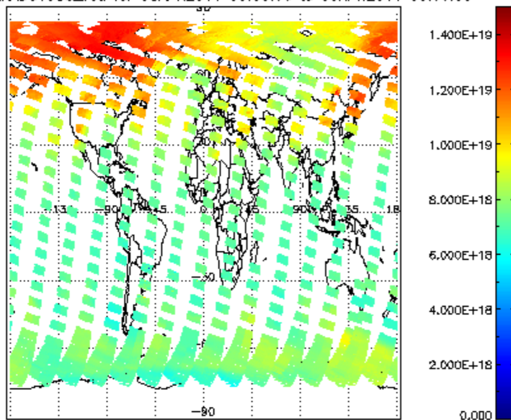
SCIOL2P_NADUV003_vcd for 08APR2011 00:00:00 to 09APR2011 00:00:00
