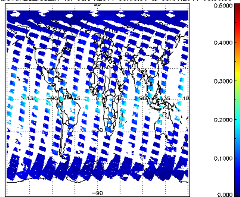
SCIOL2P_NADUV8H2O_vcd_err for 08APR2011 00:00:00 to 09APR2011 00:00:00
