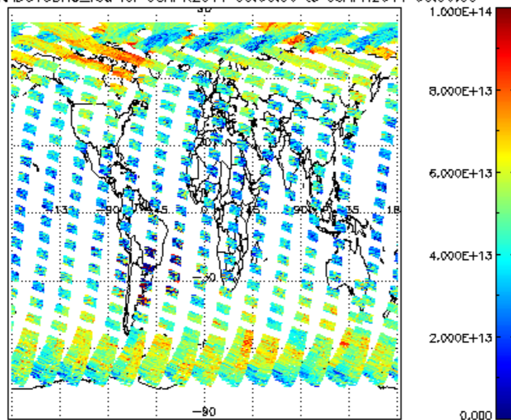
SCIOL2P_NADUV3BRO_vcd for 08APR2011 00:00:00 to 09APR2011 00:00:00
