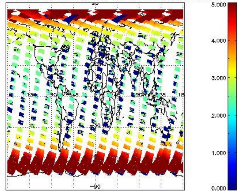
SCIOL2P_NADUV003_amf_cl for 08APR2011 00:00:00 to 09APR2011 00:00:00
