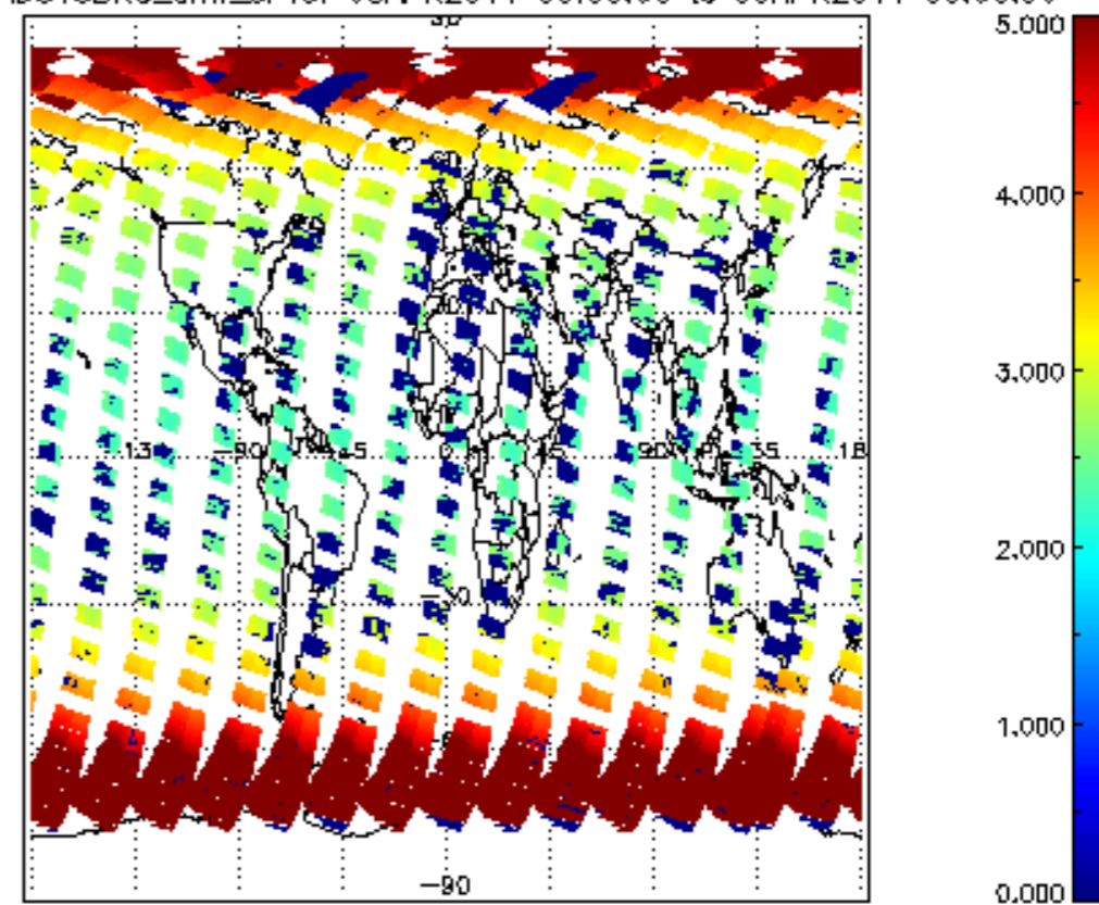
SCIOL2P_NADUV3BRO_amf_cl for 08APR2011 00:00:00 to 09APR2011 00:00:00
