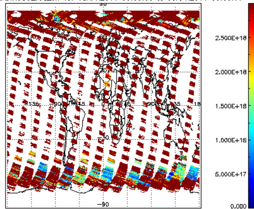
SCIOL2P_NADIR3CO_vcd_err for 08APR2011 00:00:00 to 09APR2011 00:00:00
