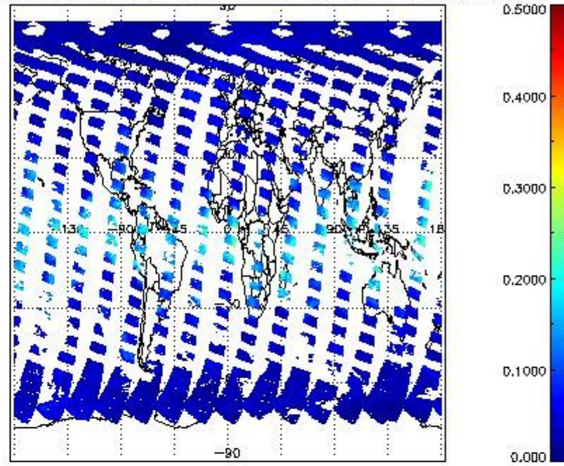
SCIOL2P_NADUV8H2O_vcd_err for 08APR2011 00:00:00 to 09APR2011 00:00:00
