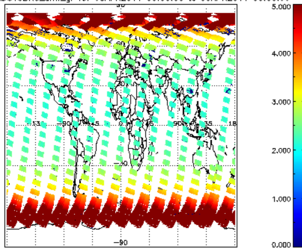
SCIOL2P_NADUV3BRO_amf_gr for 08APR2011 00:00:00 to 09APR2011 00:00:00
