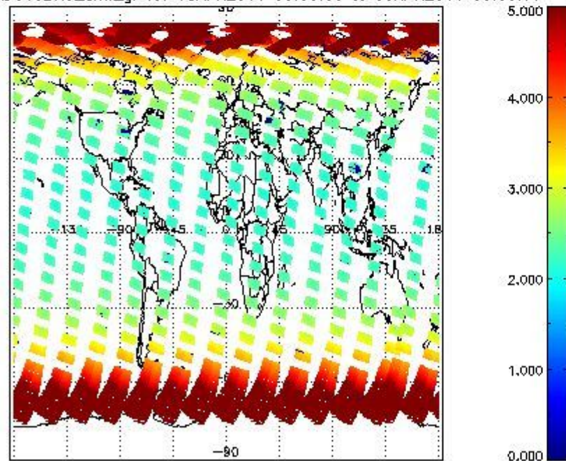
SCIOL2P_NADUV3BRO_amf_gr for 08APR2011 00:00:00 to 09APR2011 00:00:00
