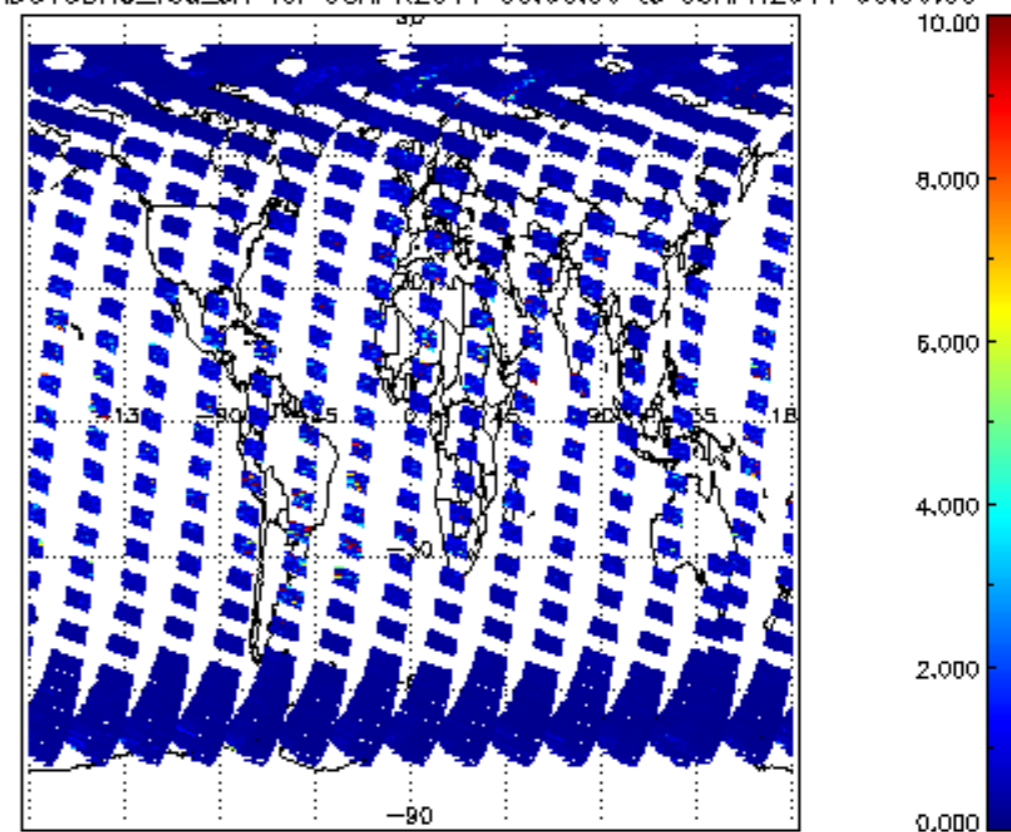
SCIOL2P_NADUV3BRO_vcd_err for 08APR2011 00:00:00 to 09APR2011 00:00:00
