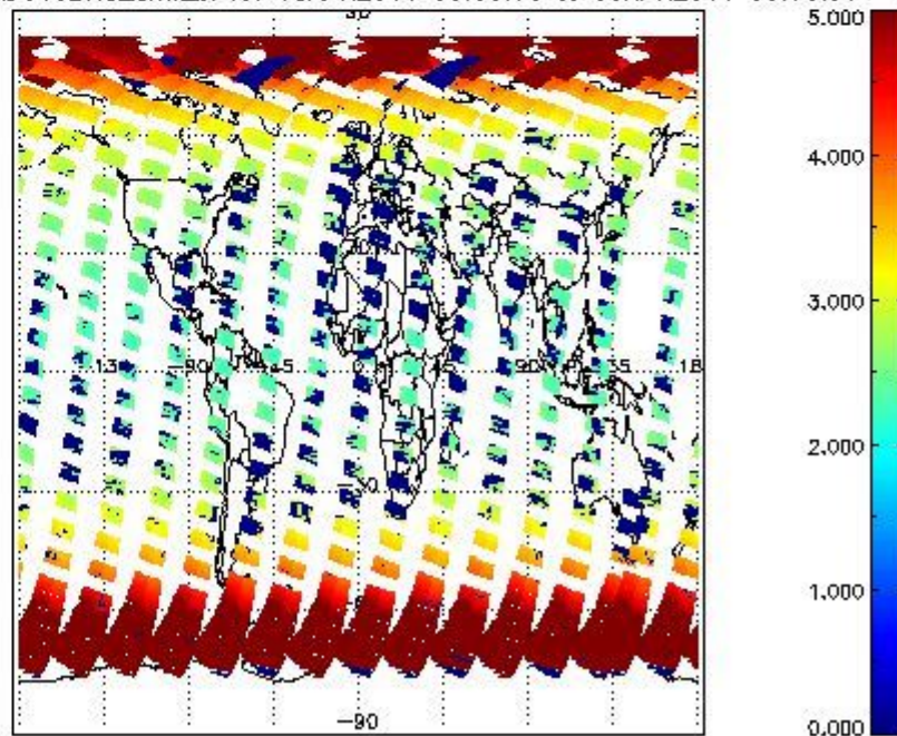
SCIOL2P_NADUV3BRO_amf_cl for 08APR2011 00:00:00 to 09APR2011 00:00:00
