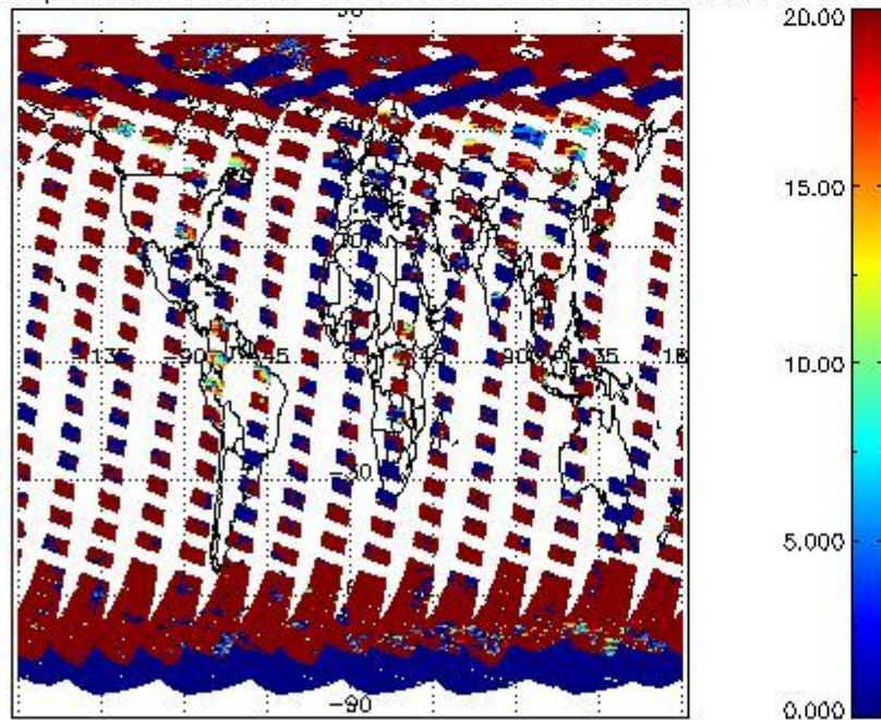
cL_opt_depth for 08APR2011 00:00:00 to 09APR2011 00:00:00
