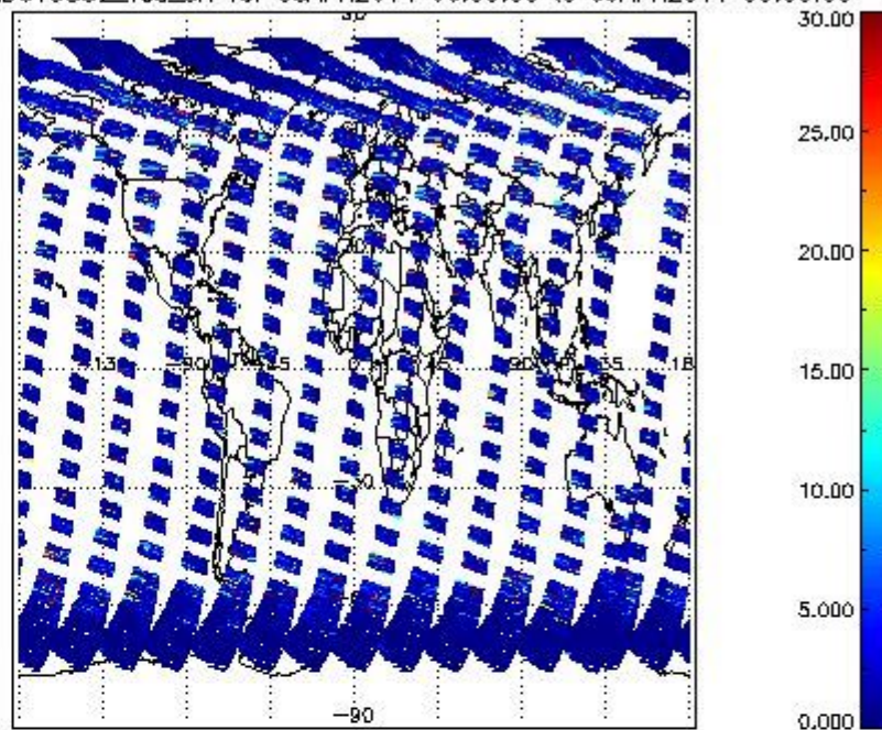
SCIOL2P_NADUV5S02_vcd_err for 08APR2011 00:00:00 to 09APR2011 00:00:00
