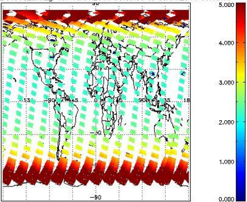
SCIOL2P_NADUV003_amf_gr for 08APR2011 00:00:00 to 09APR2011 00:00:00
