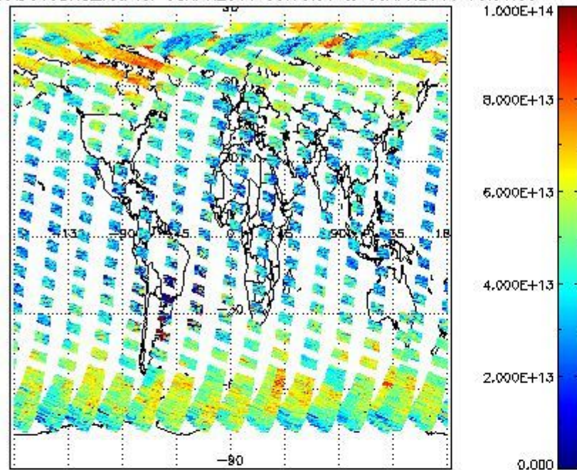
SCIOL2P_NADUV3BRO_vcd for 08APR2011 00:00:00 to 09APR2011 00:00:00
