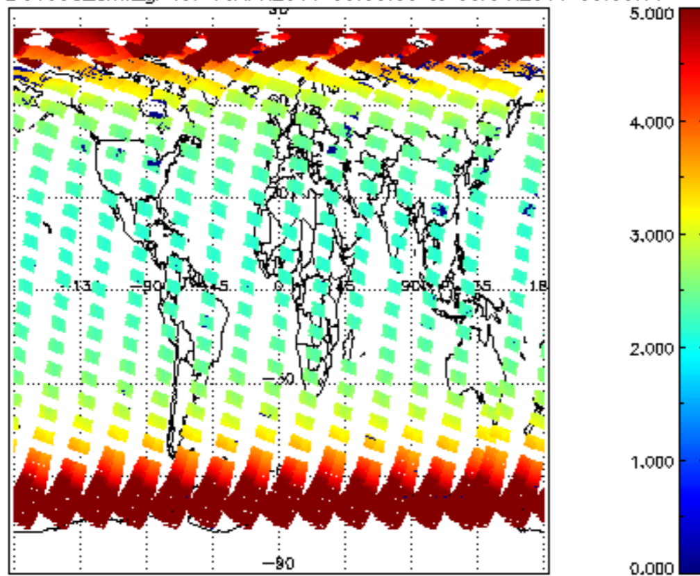
SCIOL2P_NADUV003_amf_gr for 08APR2011 00:00:00 to 09APR2011 00:00:00
