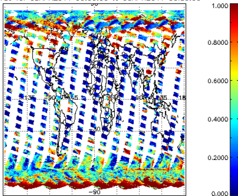
cL_frac for 08APR2011 00:00:00 to 09APR2011 00:00:00
