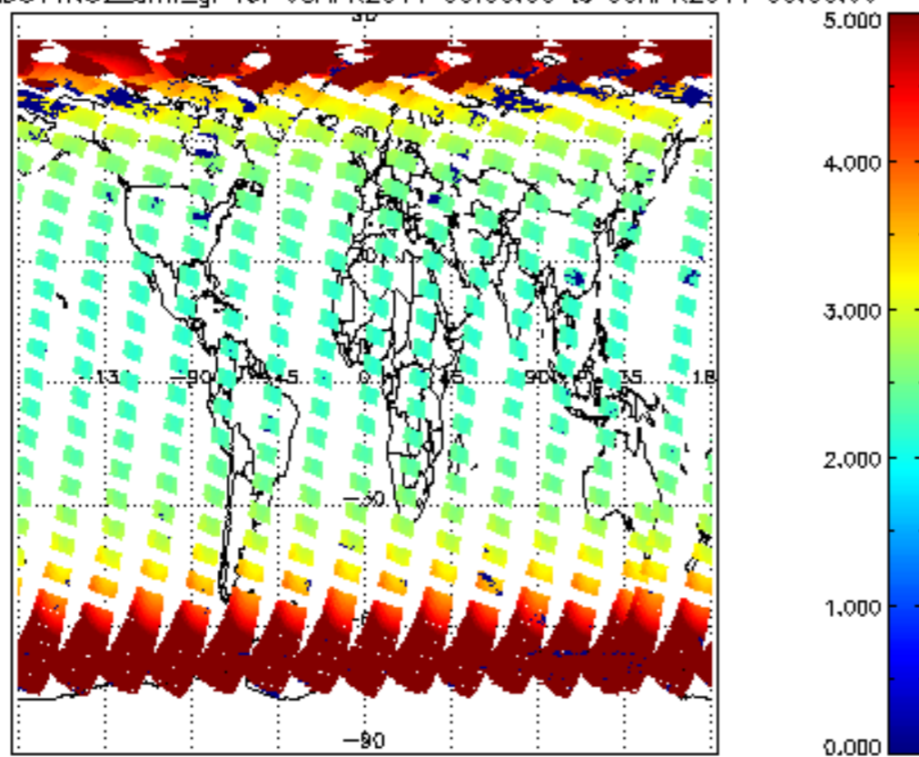
SCIOL2P_NADUV1NO2_amf_gr for 08APR2011 00:00:00 to 09APR2011 00:00:00
