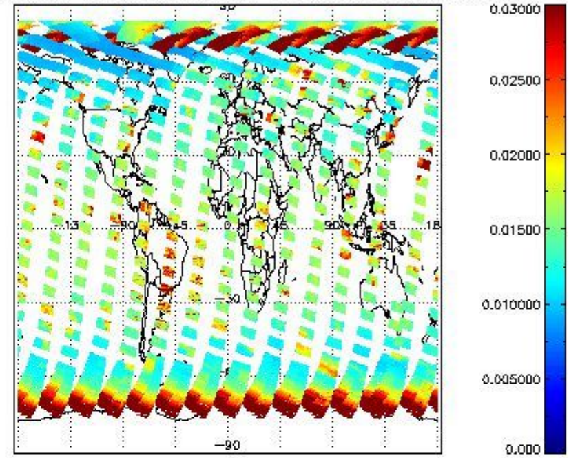
SCIOL2P_NADUV003_vcd_err for 08APR2011 00:00:00 to 09APR2011 00:00:00
