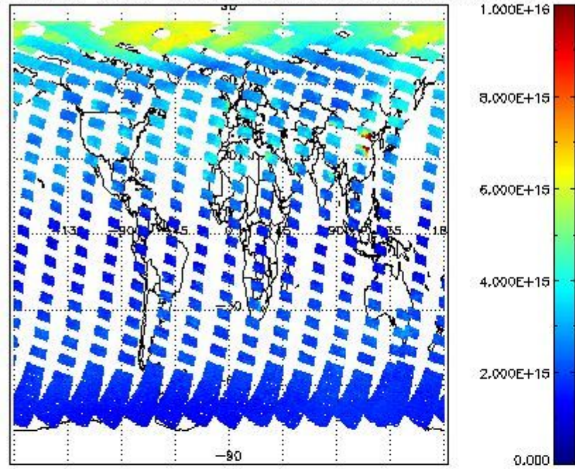
SCIOL2P_NADUV1NO2_vcd for 08APR2011 00:00:00 to 09APR2011 00:00:00
