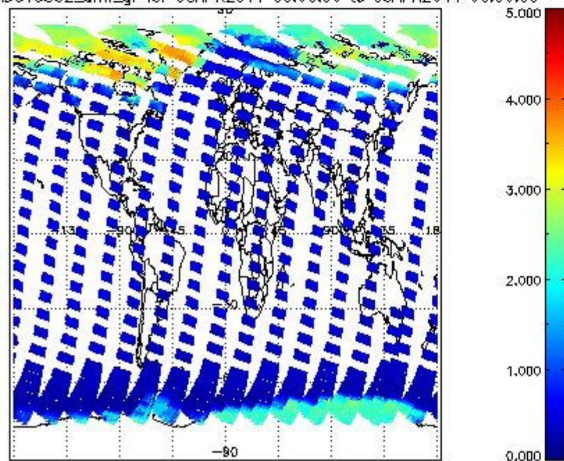
SCIOL2P_NADUV5S02_amf_gr for 08APR2011 00:00:00 to 09APR2011 00:00:00
