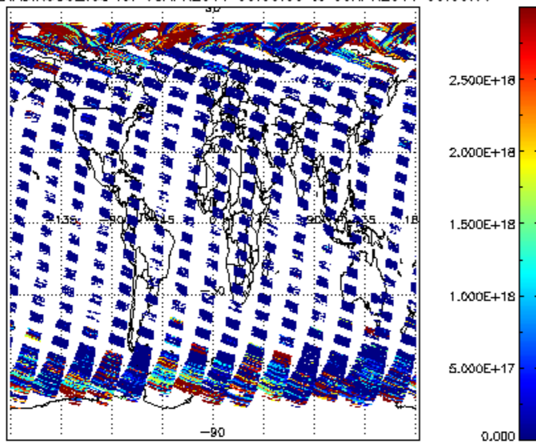
SCIOL2P_NADIR3CO_vcd for 08APR2011 00:00:00 to 09APR2011 00:00:00
