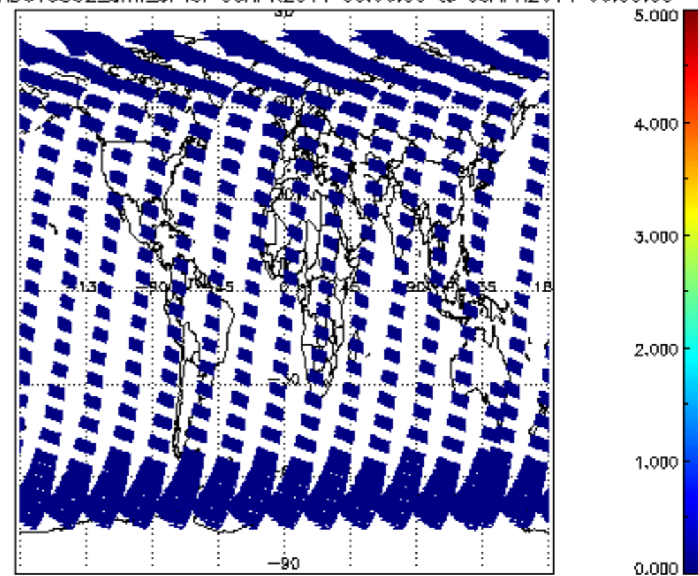
SCIOL2P_NADUV5S02_amf_cl for 08APR2011 00:00:00 to 09APR2011 00:00:00
