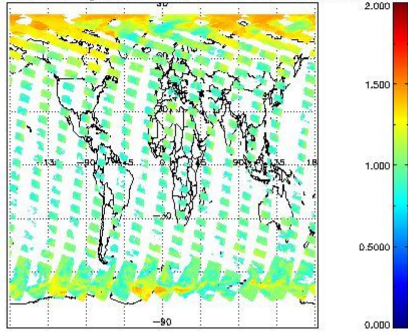
SCIOL2P_NADUV8H2O_arnf_gr for 08APR2011 00:00:00 to 09APR2011 00:00:00
