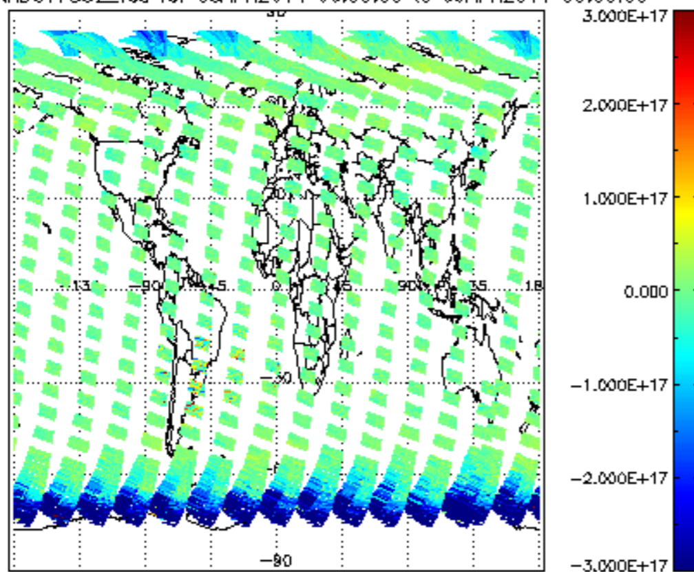
SCIOL2P_NADUV7S02_vcd for 08APR2011 00:00:00 to 09APR2011 00:00:00
