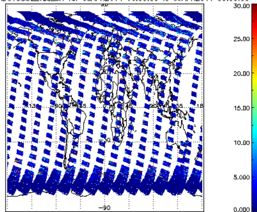
SCIOL2P_NADUV5S02_vcd_err for 08APR2011 00:00:00 to 09APR2011 00:00:00
