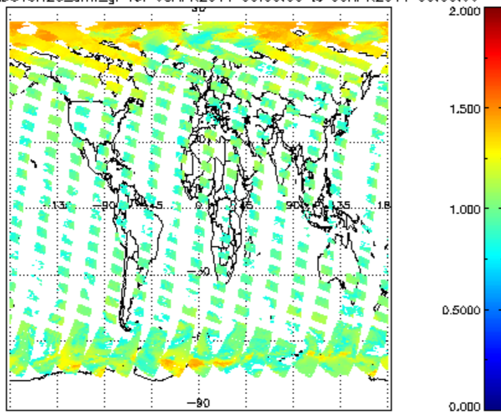
SCIOL2P_NADUV8H2O_amf_gr for 08APR2011 00:00:00 to 09APR2011 00:00:00
