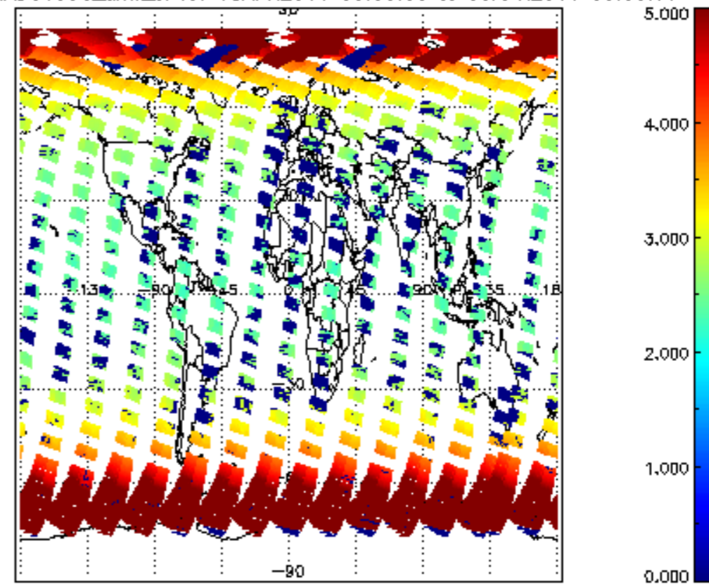
SCIOL2P_NADUV003_amf_cl for 08APR2011 00:00:00 to 09APR2011 00:00:00
