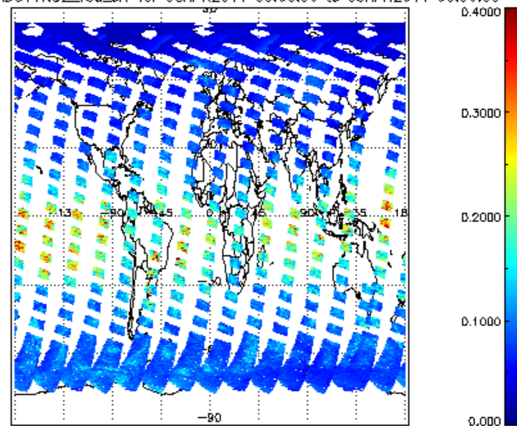
SCIOL2P_NADUV1NO2_vcd_err for 08APR2011 00:00:00 to 09APR2011 00:00:00
