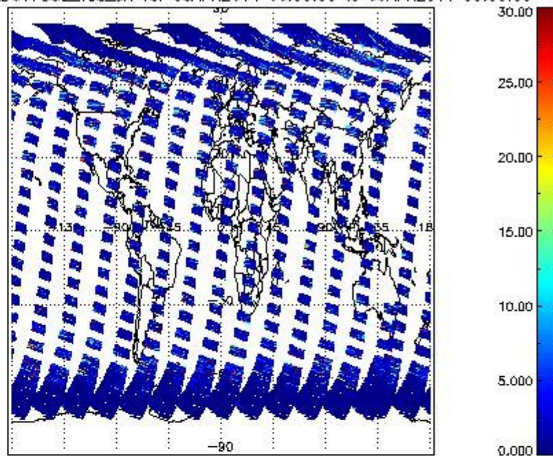
SCIOL2P_NADUV7S02_vcd_err for 08APR2011 00:00:00 to 09APR2011 00:00:00
