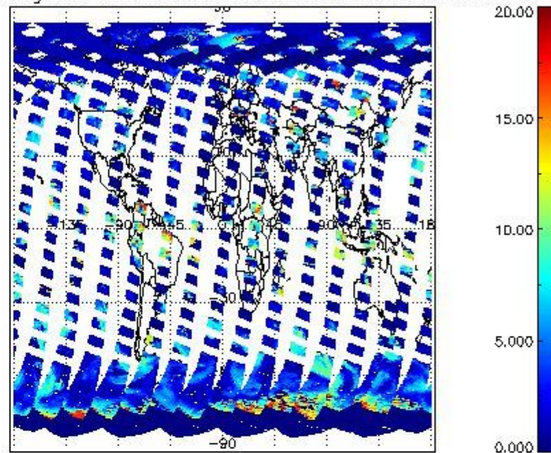
cL_top_height for 08APR2011 00:00:00 to 09APR2011 00:00:00
