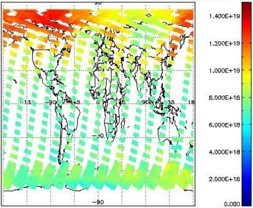
SCIOL2P_NADUV003_vcd for 08APR2011 00:00:00 to 09APR2011 00:00:00
