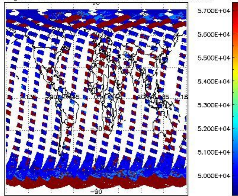
cloud_flags for 08APR2011 00:00:00 to 09APR2011 00:00:00
