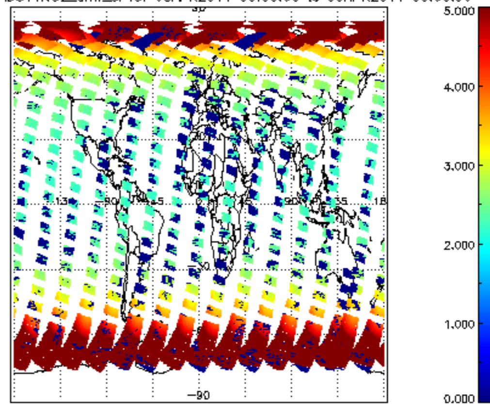
SCIOL2P_NADUV1NO2_amf_sl for 08APR2011 00:00:00 to 09APR2011 00:00:00
