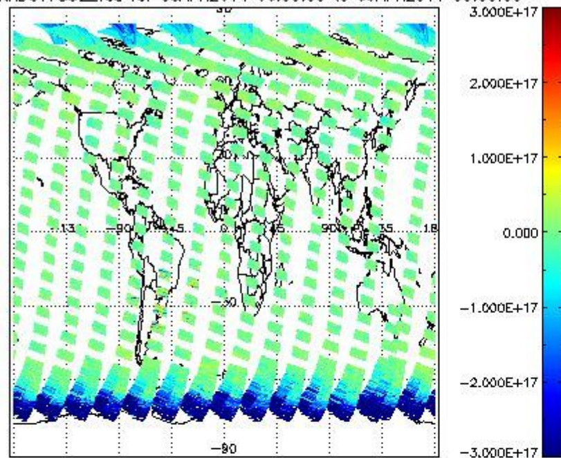
SCIOL2P_NADUV7S02_vcd for 08APR2011 00:00:00 to 09APR2011 00:00:00
