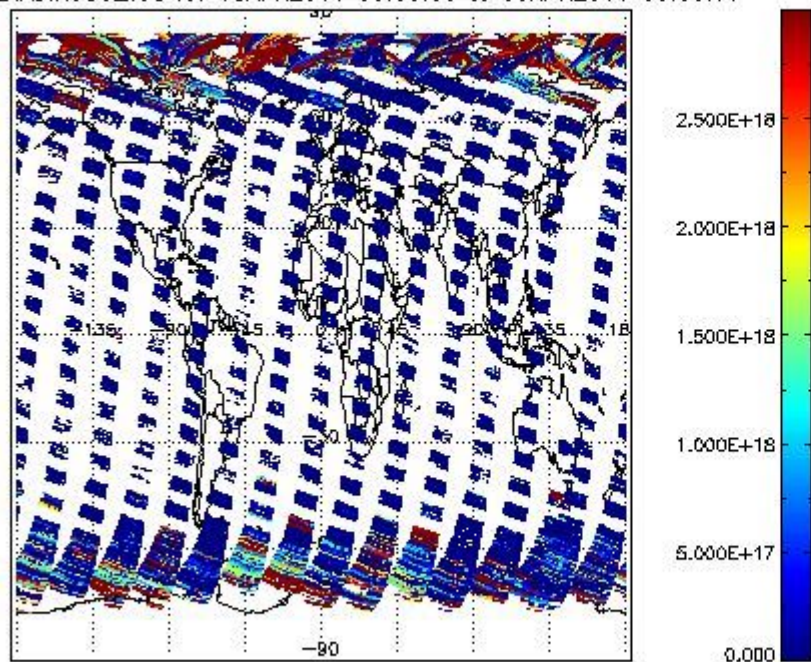
SCIOL2P_NADIR3CO_vcd for 08APR2011 00:00:00 to 09APR2011 00:00:00
