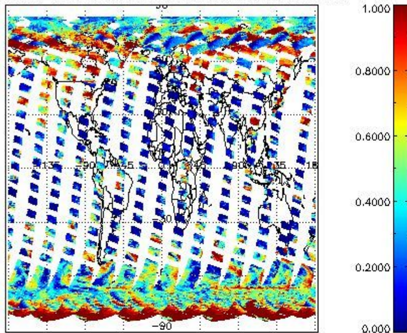
cL_frac for 08APR2011 00:00:00 to 09APR2011 00:00:00
