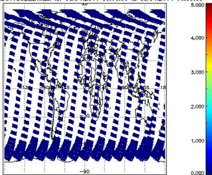
SCIOL2P_NADUV7S02_amf_cl for 08APR2011 00:00:00 to 09APR2011 00:00:00
