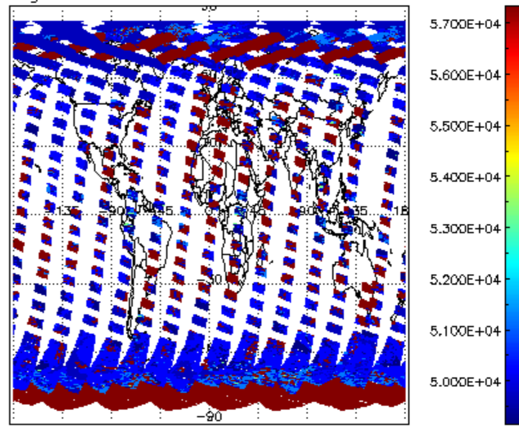
cloud_flags for 08APR2011 00:00:00 to 09APR2011 00:00:00
