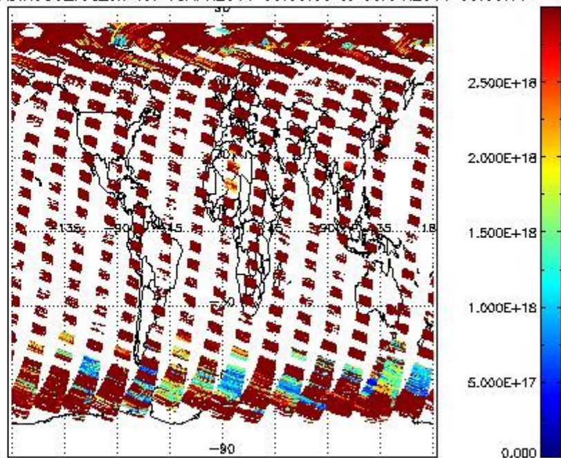
SCIOL2P_NADIR3CO_vcd_err for 08APR2011 00:00:00 to 09APR2011 00:00:00
