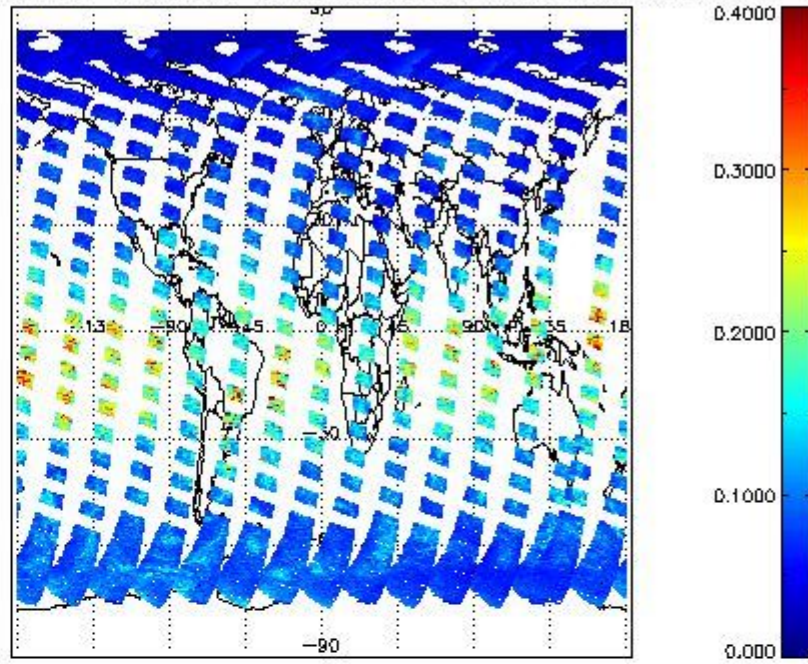
SCIOL2P_NADUV1NO2_vcd_err for 08APR2011 00:00:00 to 09APR2011 00:00:00
