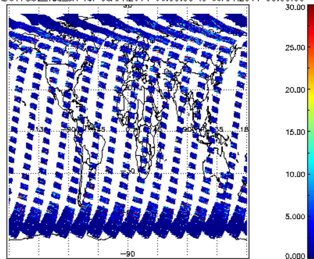
SCIOL2P_NADUV7S02_vcd_err for 08APR2011 00:00:00 to 09APR2011 00:00:00
