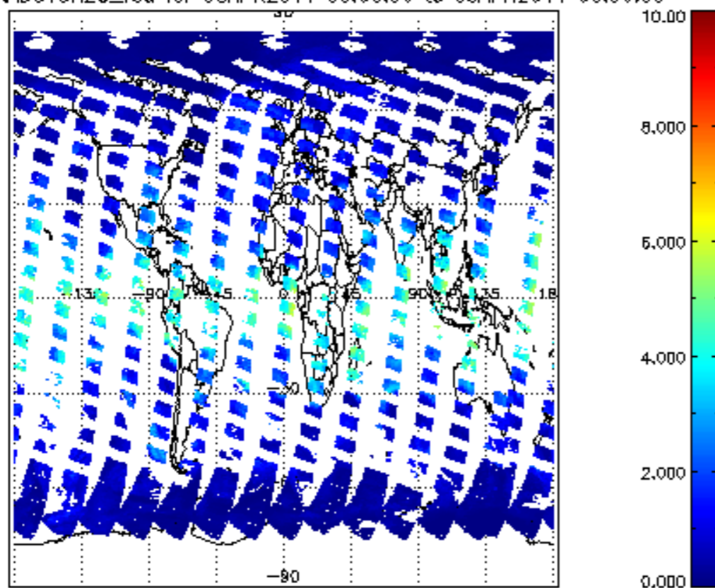
SCIOL2P_NADUV8H2O_vcd for 08APR2011 00:00:00 to 09APR2011 00:00:00
