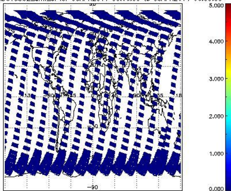
SCIOL2P_NADUV5S02_amf_cl for 08APR2011 00:00:00 to 09APR2011 00:00:00
