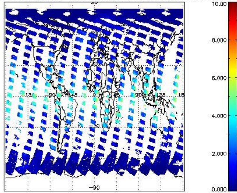
SCIOL2P_NADUV8H2O_vcd for 08APR2011 00:00:00 to 09APR2011 00:00:00
