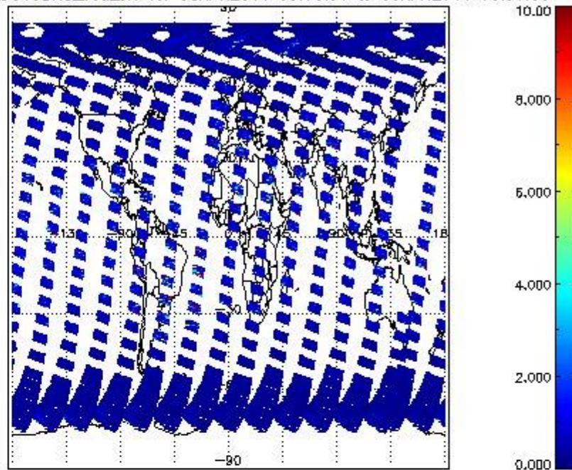
SCIOL2P_NADUV3BRO_vcd_err for 08APR2011 00:00:00 to 09APR2011 00:00:00
