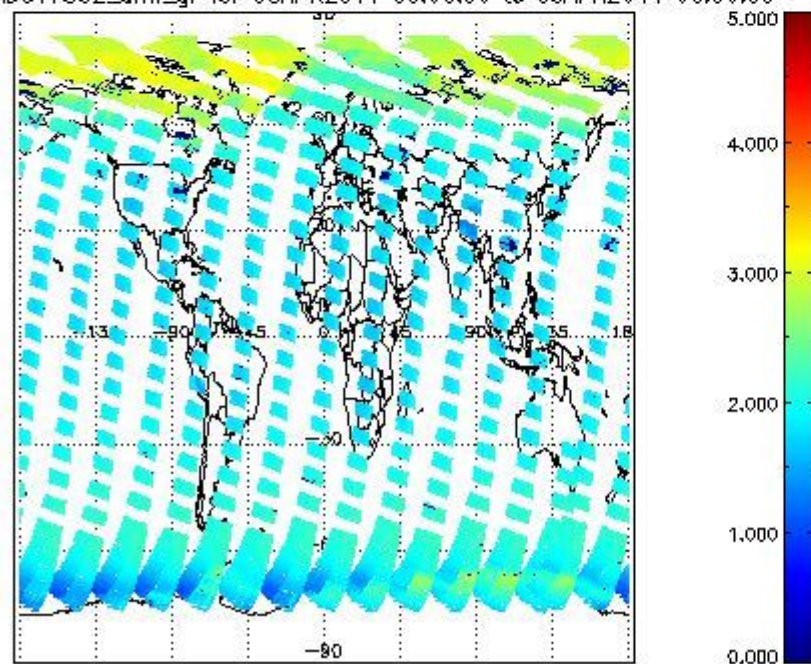
SCIOL2P_NADUV7S02_amf_gr for 08APR2011 00:00:00 to 09APR2011 00:00:00
