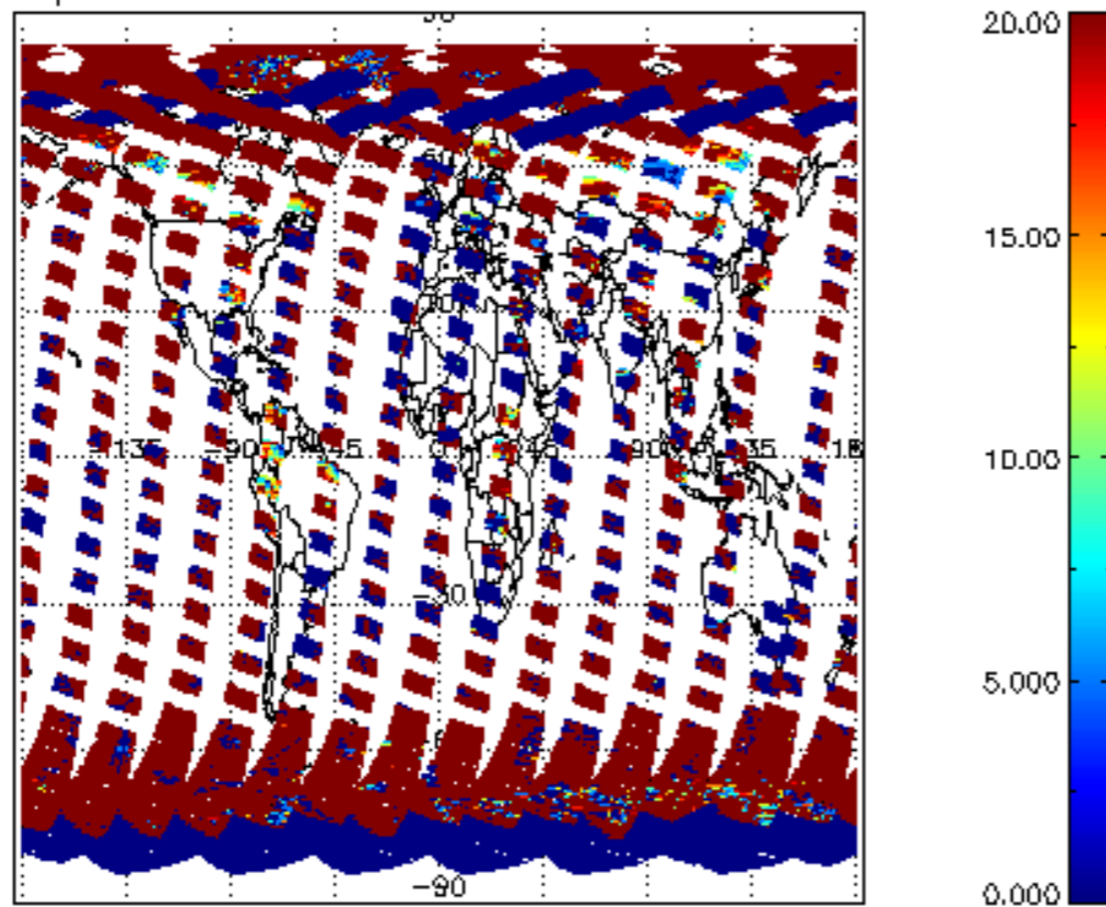
cL_opt_depth for 08APR2011 00:00:00 to 09APR2011 00:00:00
