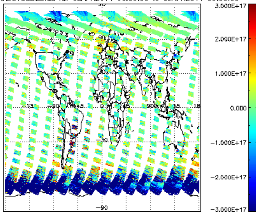
SCIOL2P_NADUV5S02_vcd for 08APR2011 00:00:00 to 09APR2011 00:00:00
