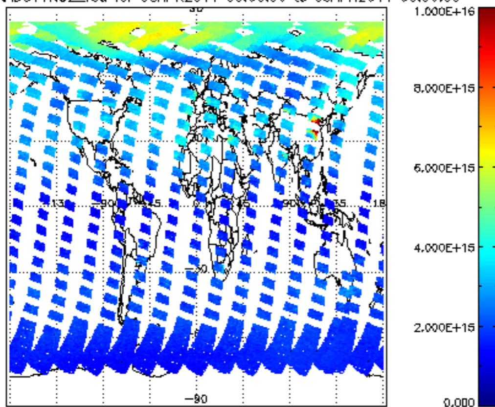
SCIOL2P_NADUV1NO2_vcd for 08APR2011 00:00:00 to 09APR2011 00:00:00
