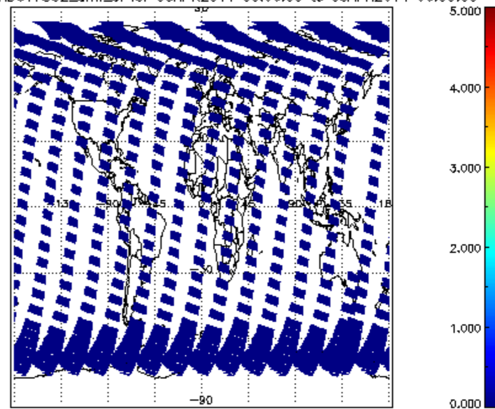
SCIOL2P_NADUV7S02_amf_cl for 08APR2011 00:00:00 to 09APR2011 00:00:00
