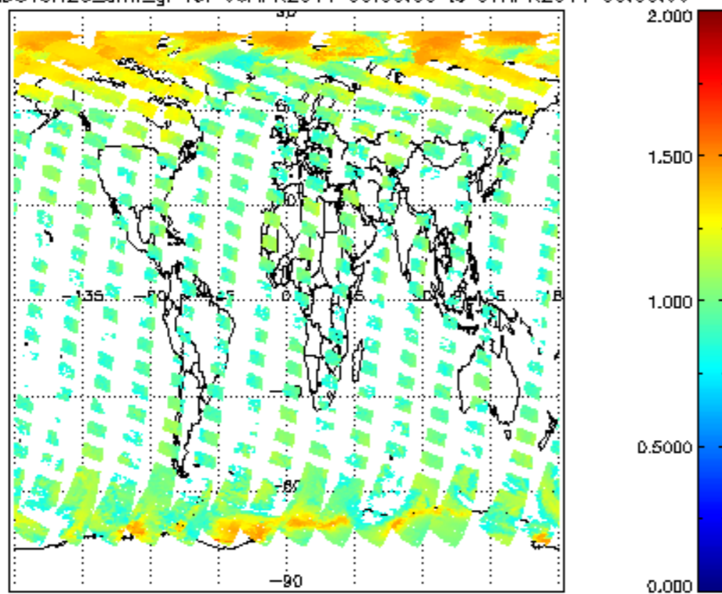
SCIOL2P_NADUV8H2O_amf_gr for 06APR2011 00:00:00 to 07APR2011 00:00:00
