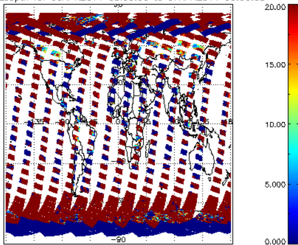
cl_opt_depth for 06APR2011 00:00:00 to 07APR2011 00:00:00
