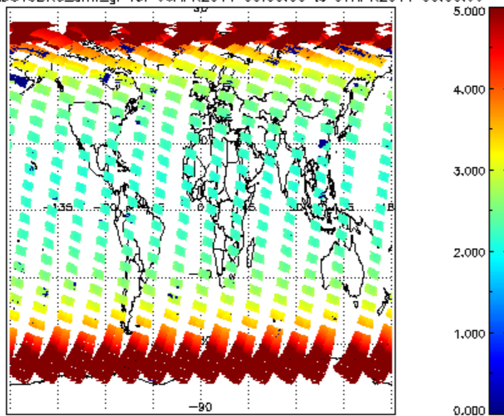
SCIOL2P_NADUV3BRO_amf_gr for 06APR2011 00:00:00 to 07APR2011 00:00:00
