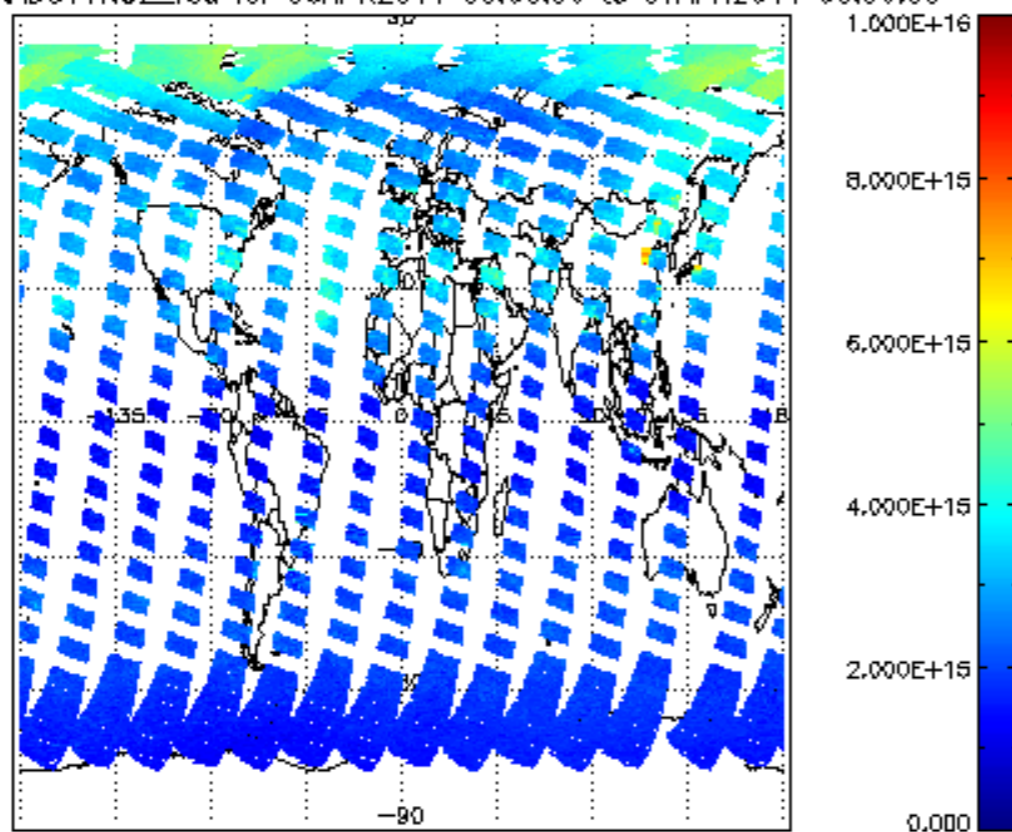
SCIOL2P_NADUV1NO2_vcd for 06APR2011 00:00:00 to 07APR2011 00:00:00
