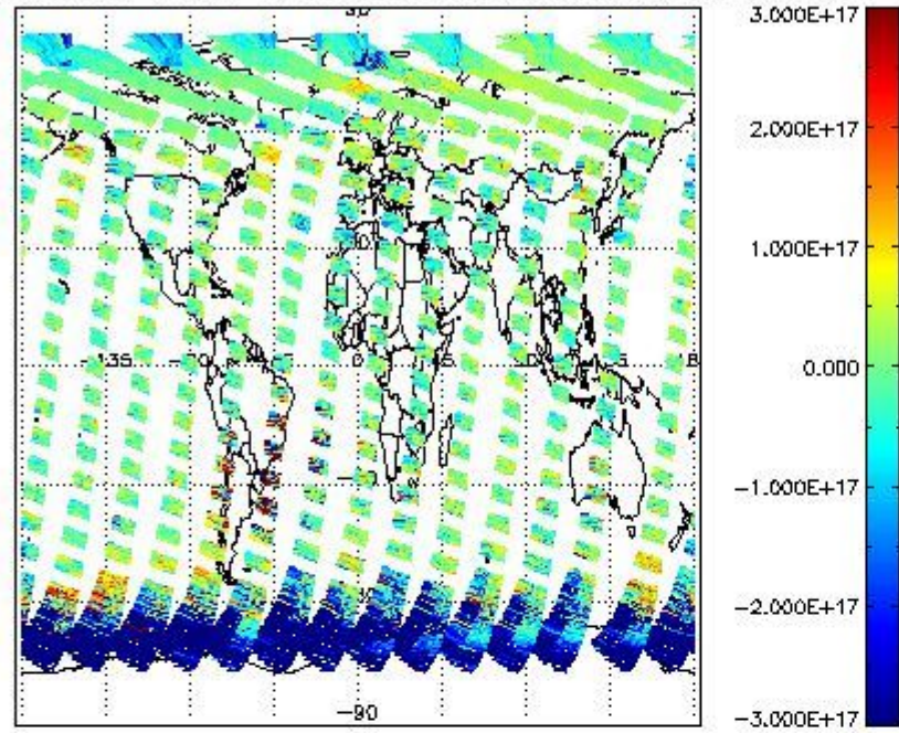
SCIOL2P_NADUV5S02_vcd for 06APR2011 00:00:00 to 07APR2011 00:00:00
