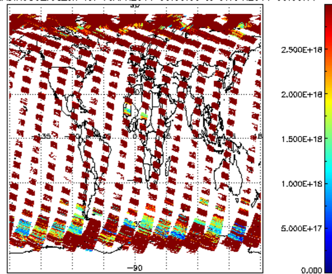
SCIOL2P_NADIR3CO_vcd_err for 06APR2011 00:00:00 to 07APR2011 00:00:00
