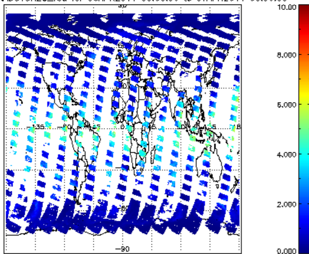
SCIOL2P_NADUV8H2O_vcd for 06APR2011 00:00:00 to 07APR2011 00:00:00
