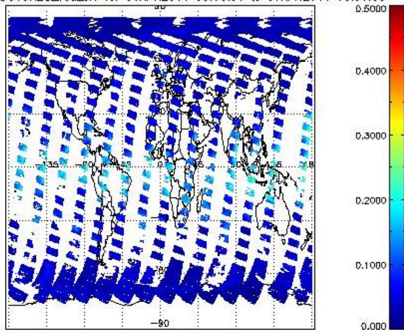
SCIOL2P_NADUV8H2O_vcd_err for 06APR2011 00:00:00 to 07APR2011 00:00:00
