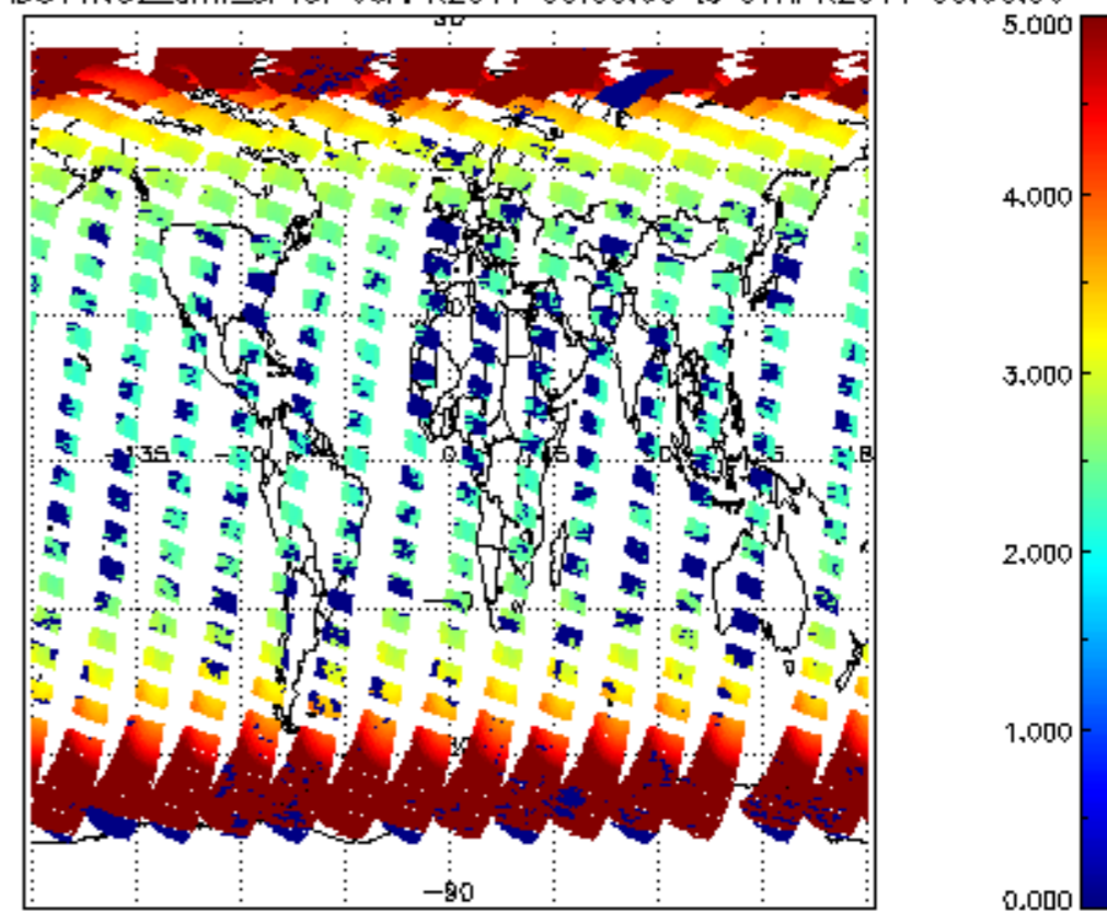
SCIOL2P_NADUV1NO2_amf_sl for 06APR2011 00:00:00 to 07APR2011 00:00:00
