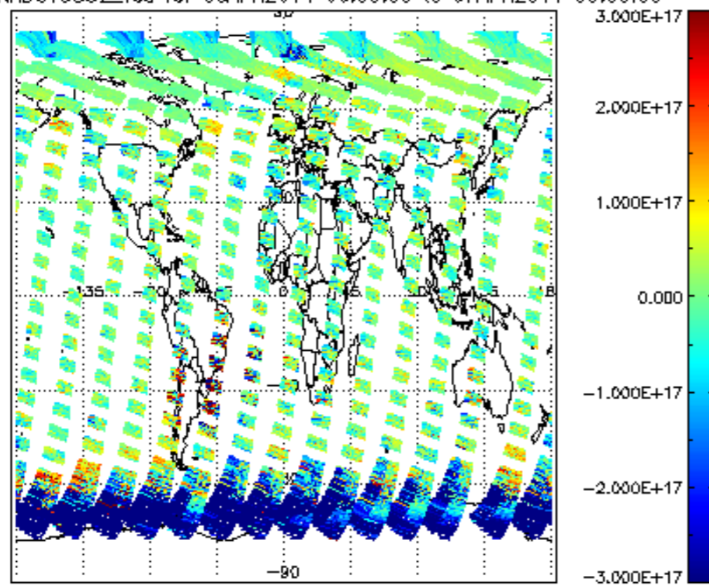
SCIOL2P_NADUV5S02_vcd for 06APR2011 00:00:00 to 07APR2011 00:00:00
