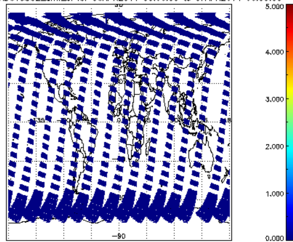
SCIOL2P_NADUV5S02_amf_cl for 06APR2011 00:00:00 to 07APR2011 00:00:00
