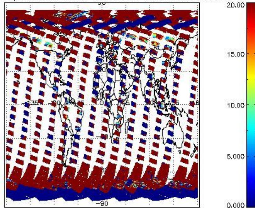
cL_opt_depth for 06APR2011 00:00:00 to 07APR2011 00:00:00
