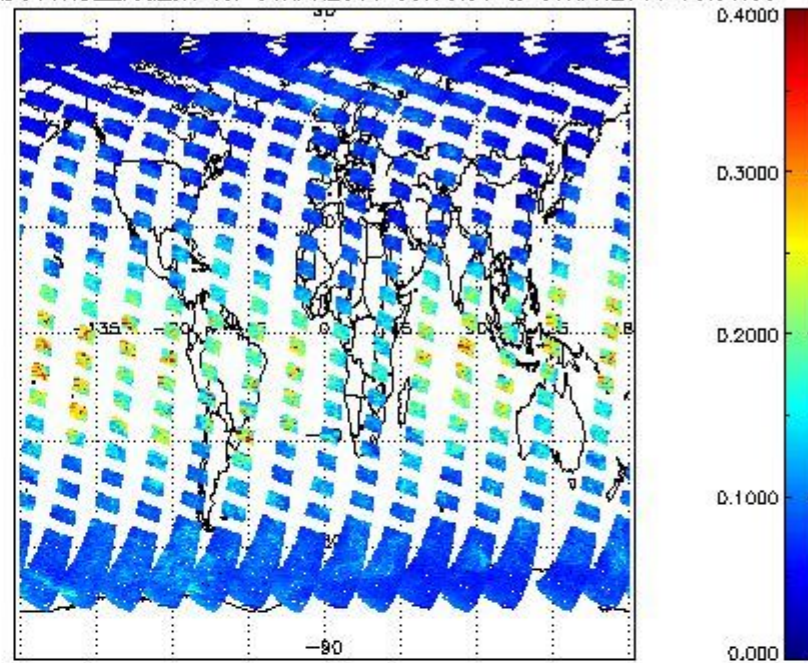
SCIOL2P_NADUV1NO2_vcd_err for 06APR2011 00:00:00 to 07APR2011 00:00:00
