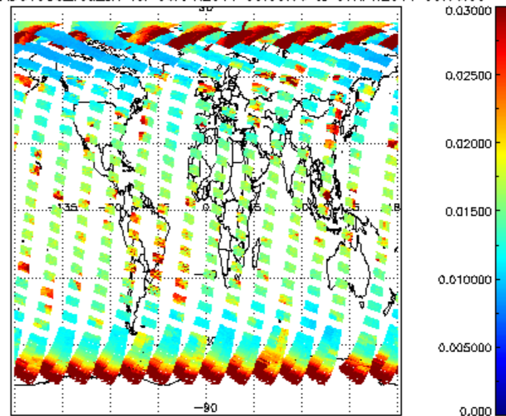
SCIOL2P_NADUV003_vcd_err for 06APR2011 00:00:00 to 07APR2011 00:00:00
