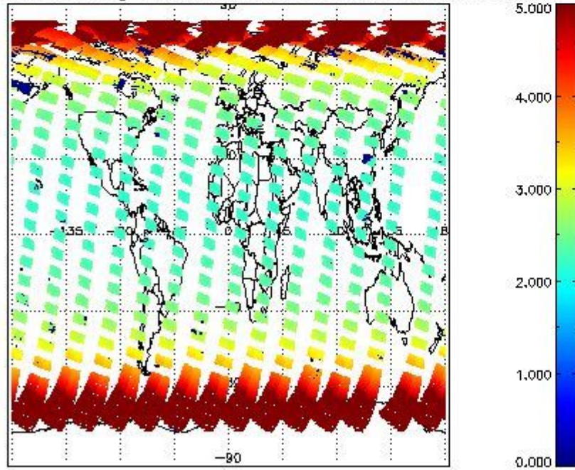
SCIOL2P_NADUV003_amf_gr for 06APR2011 00:00:00 to 07APR2011 00:00:00
