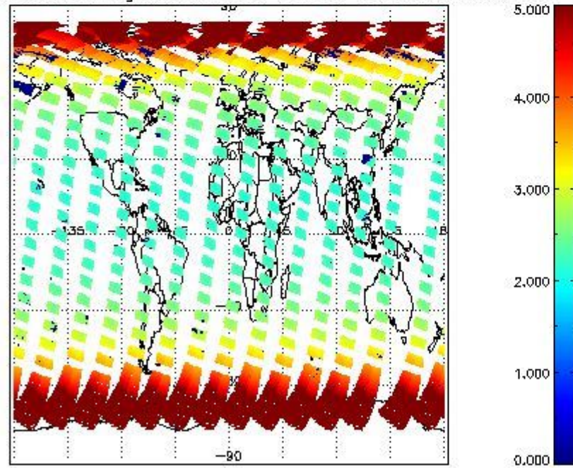
SCIOL2P_NADUV3BRO_amf_gr for 06APR2011 00:00:00 to 07APR2011 00:00:00
