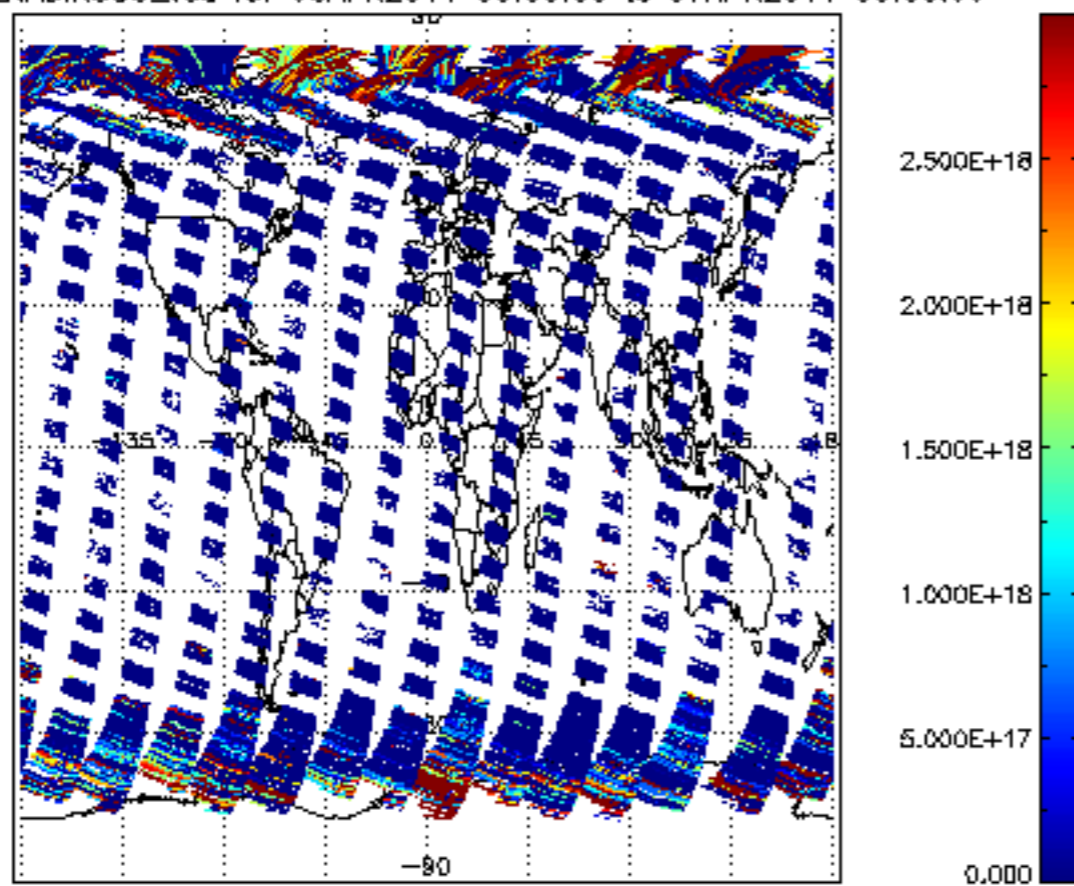
SCIOL2P_NADIR3CO_vcd for 06APR2011 00:00:00 to 07APR2011 00:00:00
