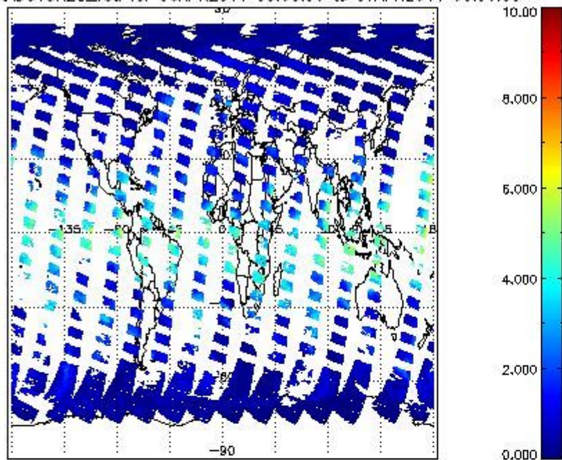
SCIOL2P_NADUV8H2O_vcd for 06APR2011 00:00:00 to 07APR2011 00:00:00
