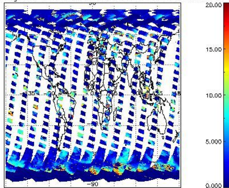
cL_top_height for 06APR2011 00:00:00 to 07APR2011 00:00:00
