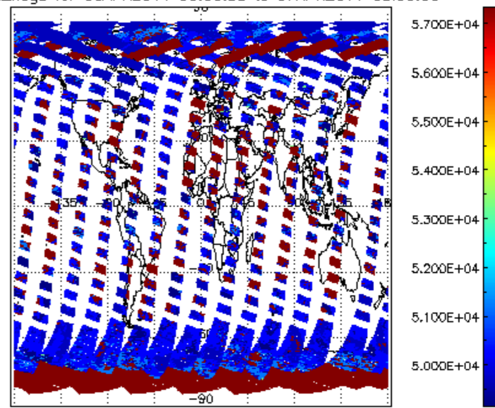
cloud_flags for 06APR2011 00:00:00 to 07APR2011 00:00:00
