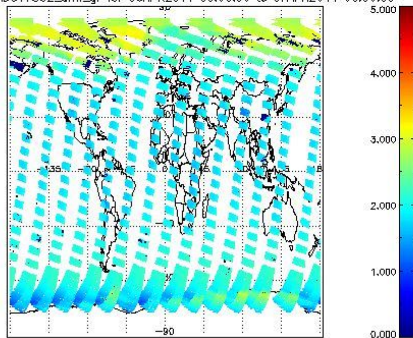
SCIOL2P_NADUV7S02_amf_gr for 06APR2011 00:00:00 to 07APR2011 00:00:00
