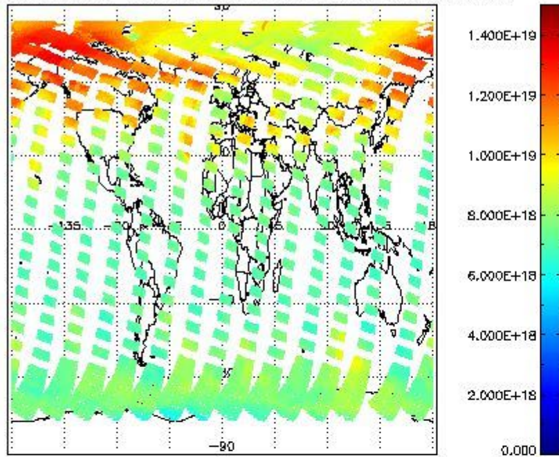
SCIOL2P_NADUV003_vcd for 06APR2011 00:00:00 to 07APR2011 00:00:00
