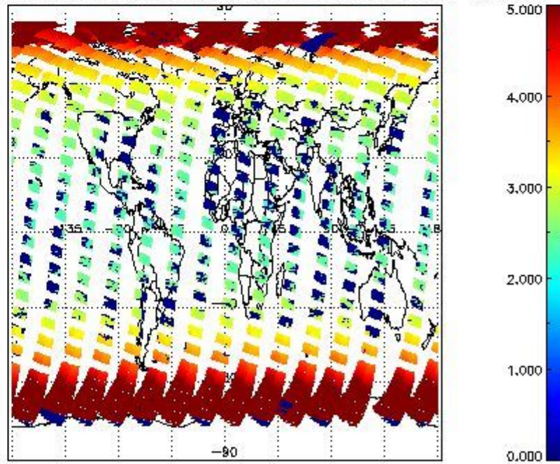
SCIOL2P_NADUV3BRO_amf_cl for 06APR2011 00:00:00 to 07APR2011 00:00:00
