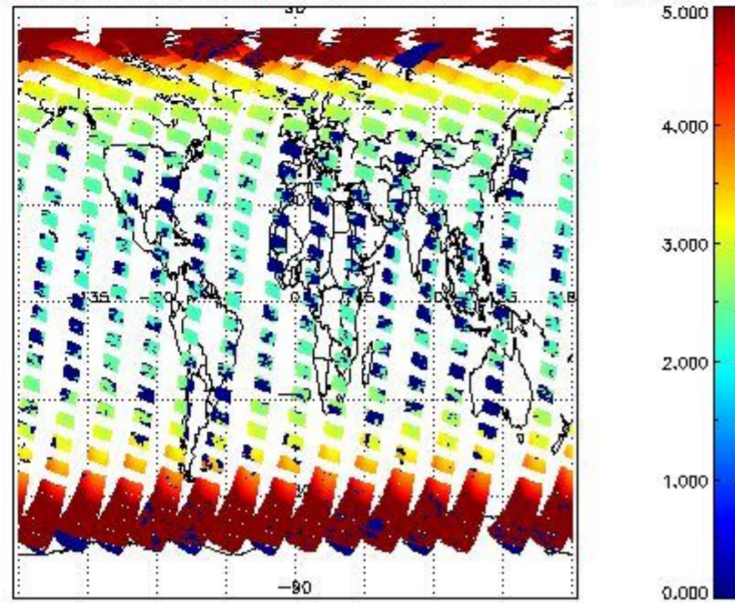
SCIOL2P_NADUV1NO2_amf_cl for 06APR2011 00:00:00 to 07APR2011 00:00:00
