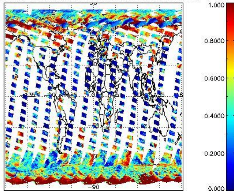
cL_frac for 06APR2011 00:00:00 to 07APR2011 00:00:00
