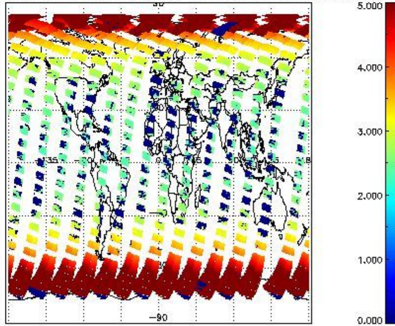
SCIOL2P_NADUV003_amf_cl for 06APR2011 00:00:00 to 07APR2011 00:00:00
