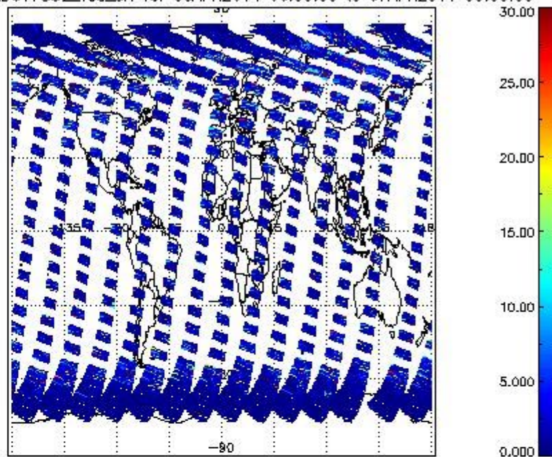
SCIOL2P_NADUV7S02_vcd_err for 06APR2011 00:00:00 to 07APR2011 00:00:00
