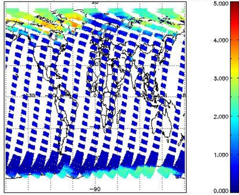
SCIOL2P_NADUV5S02_amf_gr for 06APR2011 00:00:00 to 07APR2011 00:00:00
