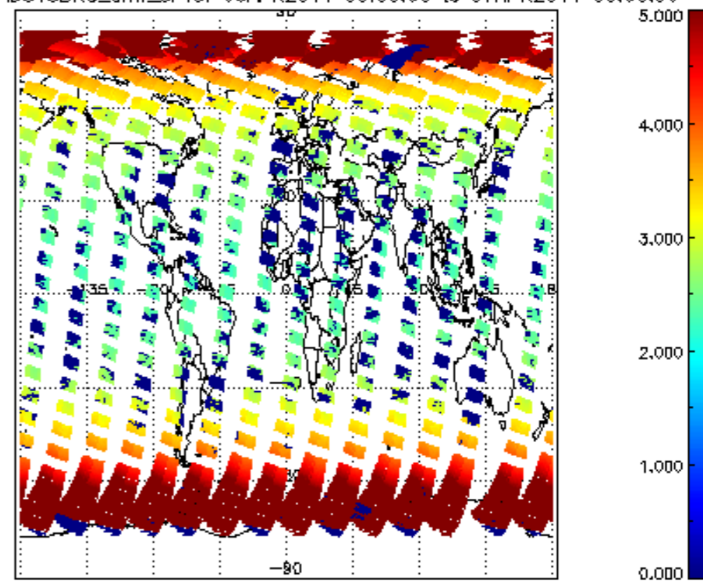
SCIOL2P_NADUV3BRO_amf_sl for 06APR2011 00:00:00 to 07APR2011 00:00:00
