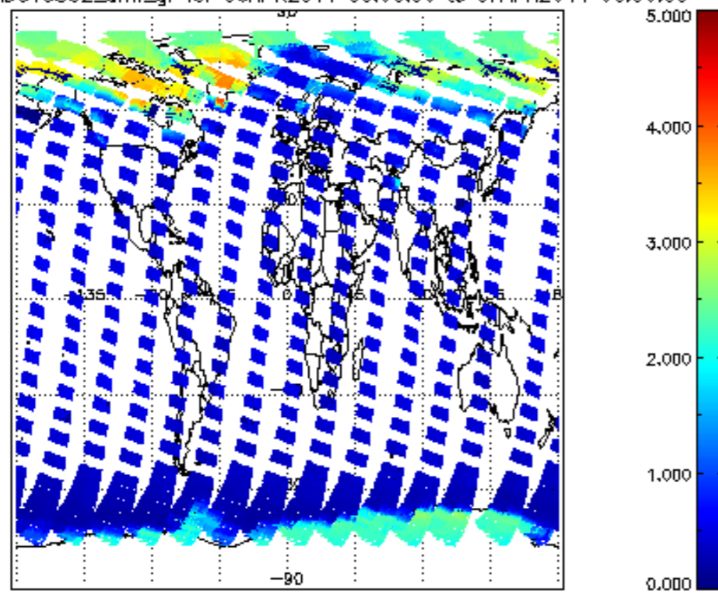
SCIOL2P_NADUV5S02_amf_gr for 06APR2011 00:00:00 to 07APR2011 00:00:00
