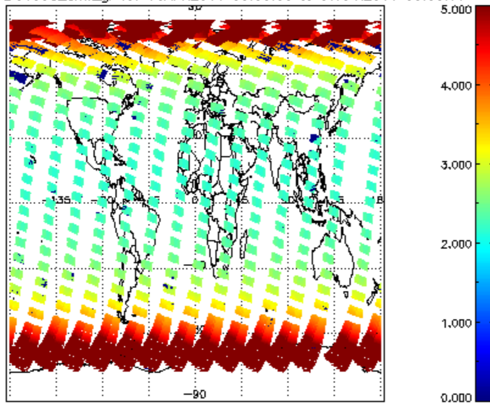
SCIOL2P_NADUV003_amf_gr for 06APR2011 00:00:00 to 07APR2011 00:00:00
