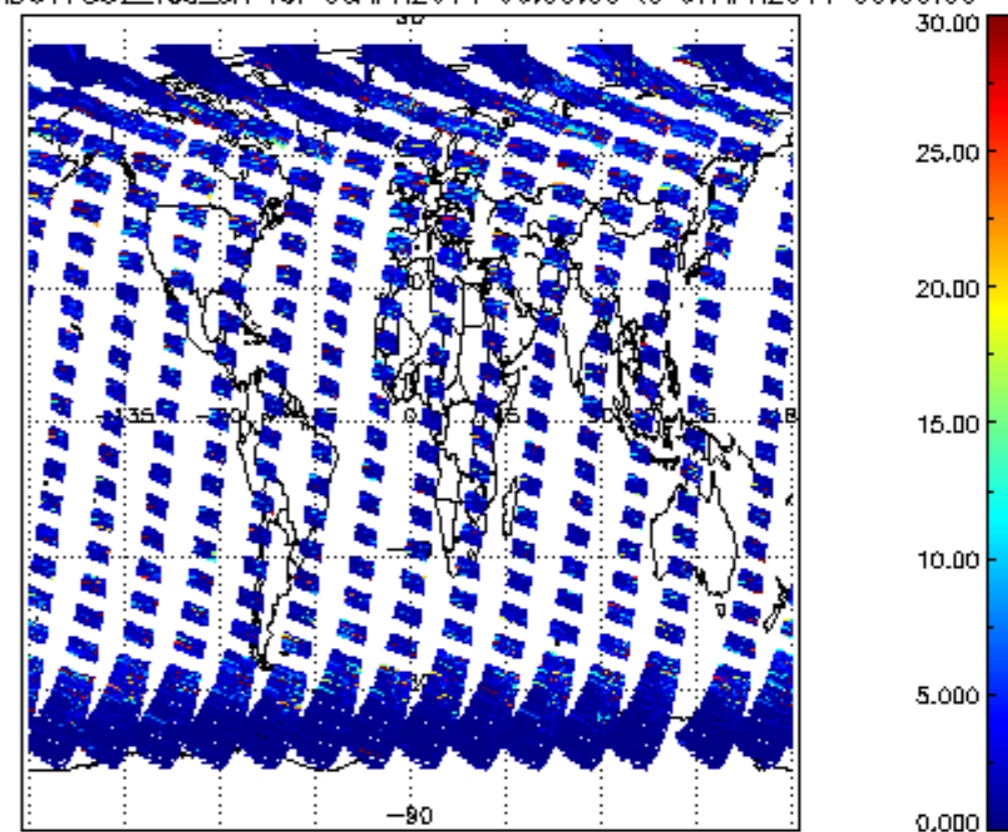
SCIOL2P_NADUV7S02_vcd_err for 06APR2011 00:00:00 to 07APR2011 00:00:00
