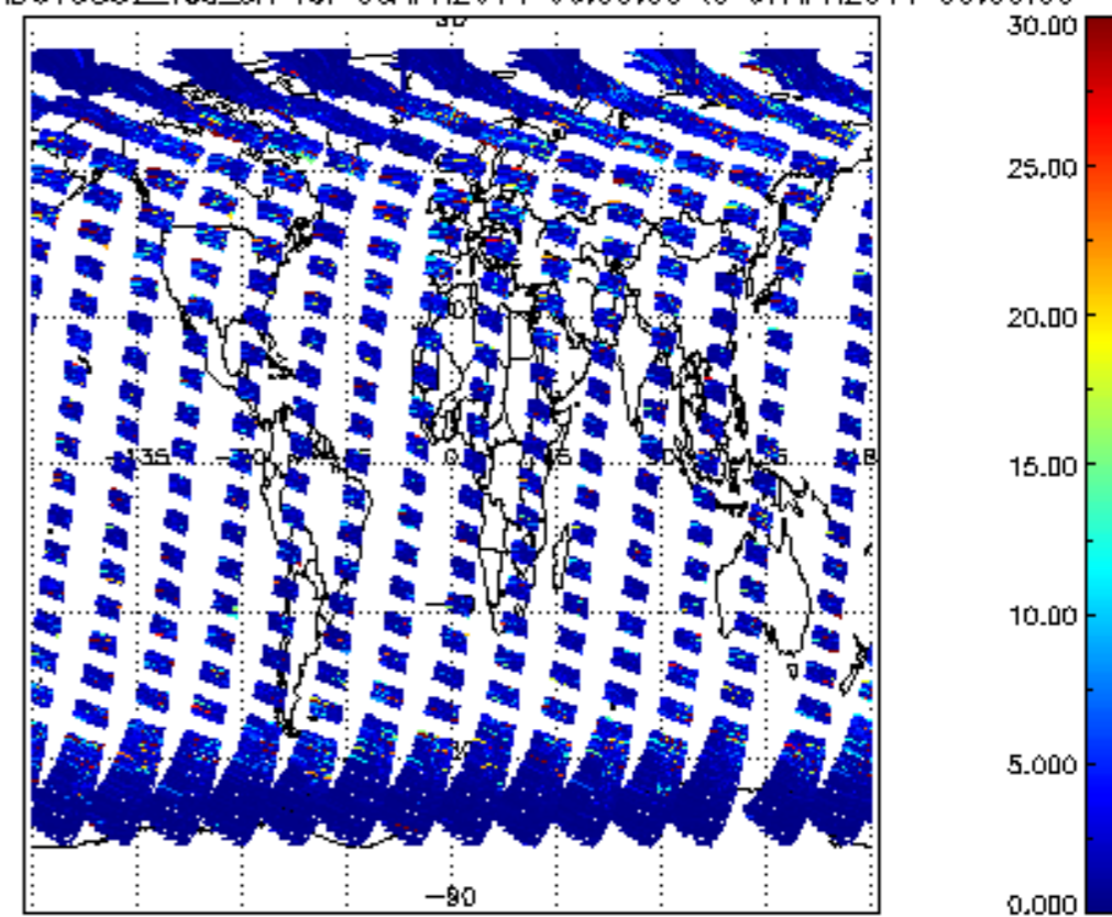
SCIOL2P_NADUV5S02_vcd_err for 06APR2011 00:00:00 to 07APR2011 00:00:00
