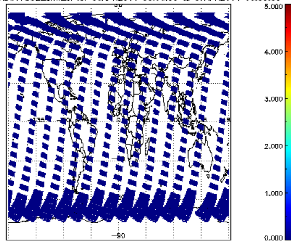
SCIOL2P_NADUV7S02_amf_cl for 06APR2011 00:00:00 to 07APR2011 00:00:00
