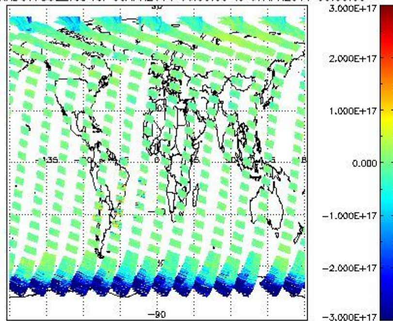
SCIOL2P_NADUV7S02_vcd for 06APR2011 00:00:00 to 07APR2011 00:00:00
