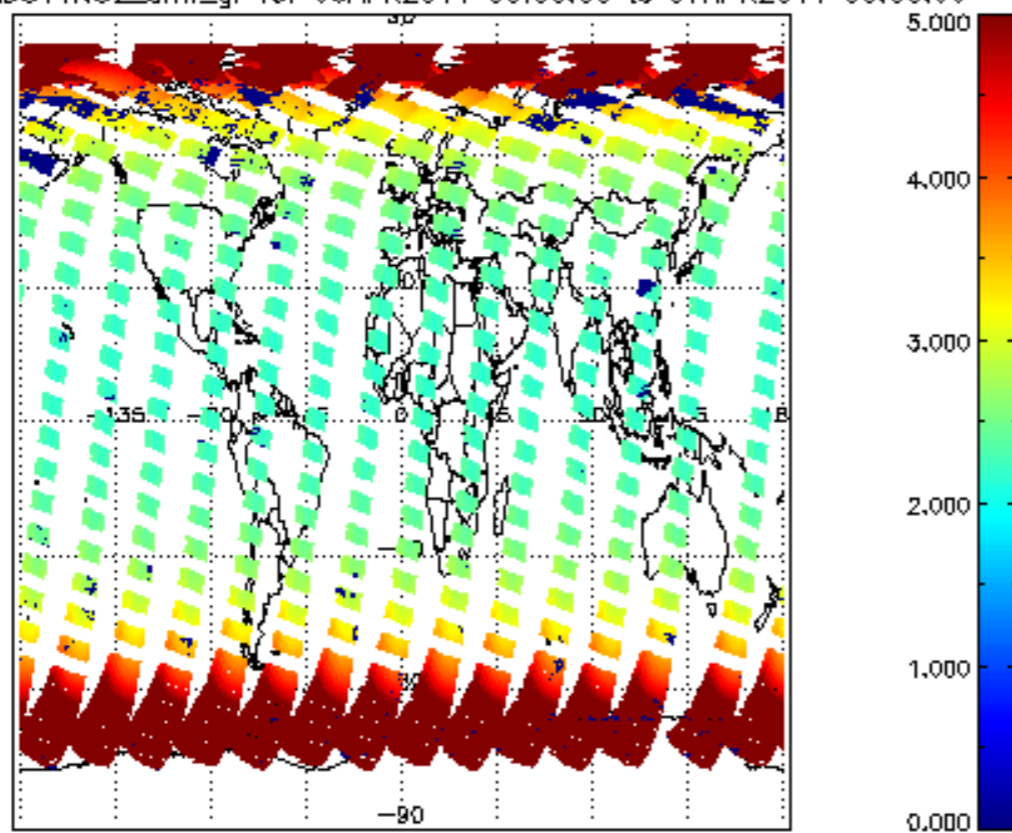
SCIOL2P_NADUV1NO2_amf_gr for 06APR2011 00:00:00 to 07APR2011 00:00:00
