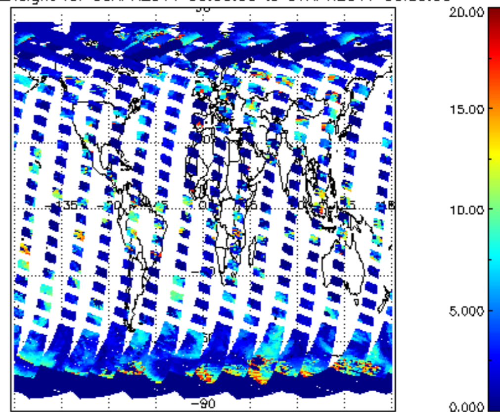
cl_top_height for 06APR2011 00:00:00 to 07APR2011 00:00:00
