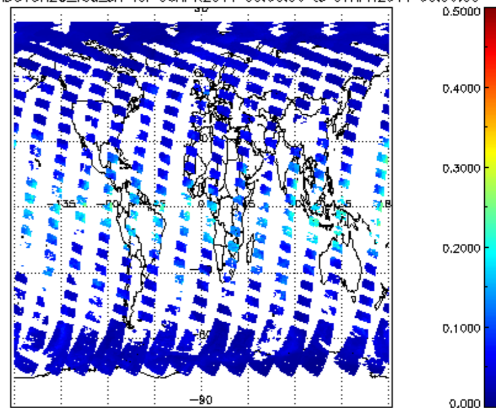
SCIOL2P_NADUV8H2O_vcd_err for 06APR2011 00:00:00 to 07APR2011 00:00:00
