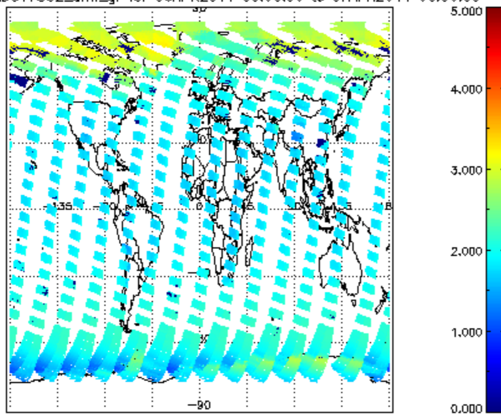
SCIOL2P_NADUV7S02_amf_gr for 06APR2011 00:00:00 to 07APR2011 00:00:00
