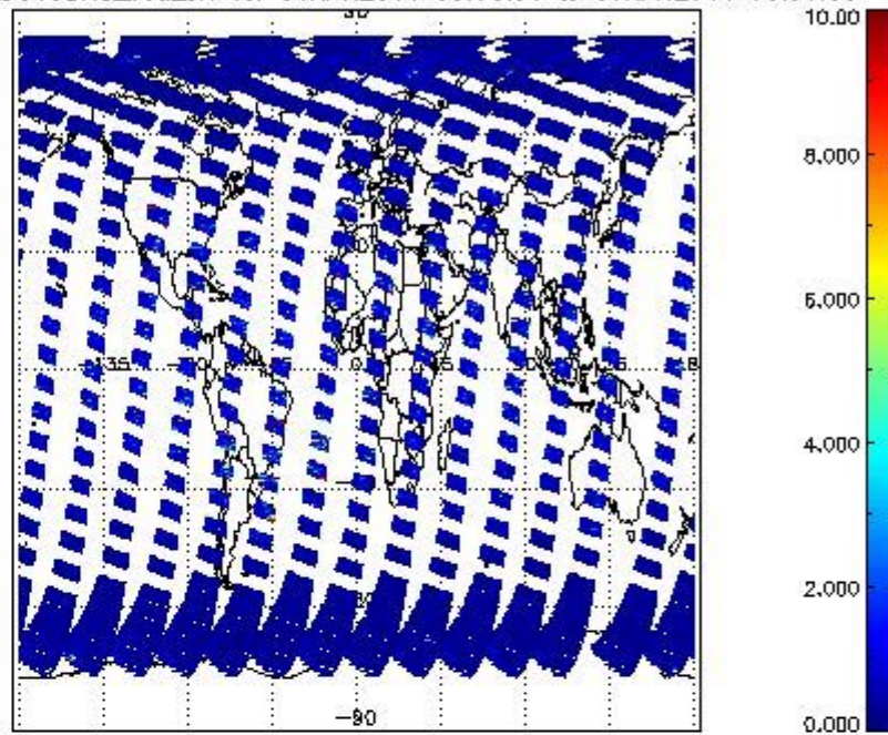
SCIOL2P_NADUV3BRO_vcd_err for 06APR2011 00:00:00 to 07APR2011 00:00:00
