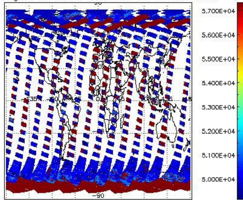
cloud_flags for 06APR2011 00:00:00 to 07APR2011 00:00:00
