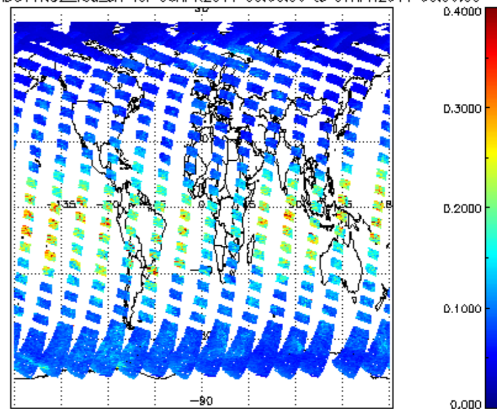
SCIOL2P_NADUV1NO2_vcd_err for 06APR2011 00:00:00 to 07APR2011 00:00:00
