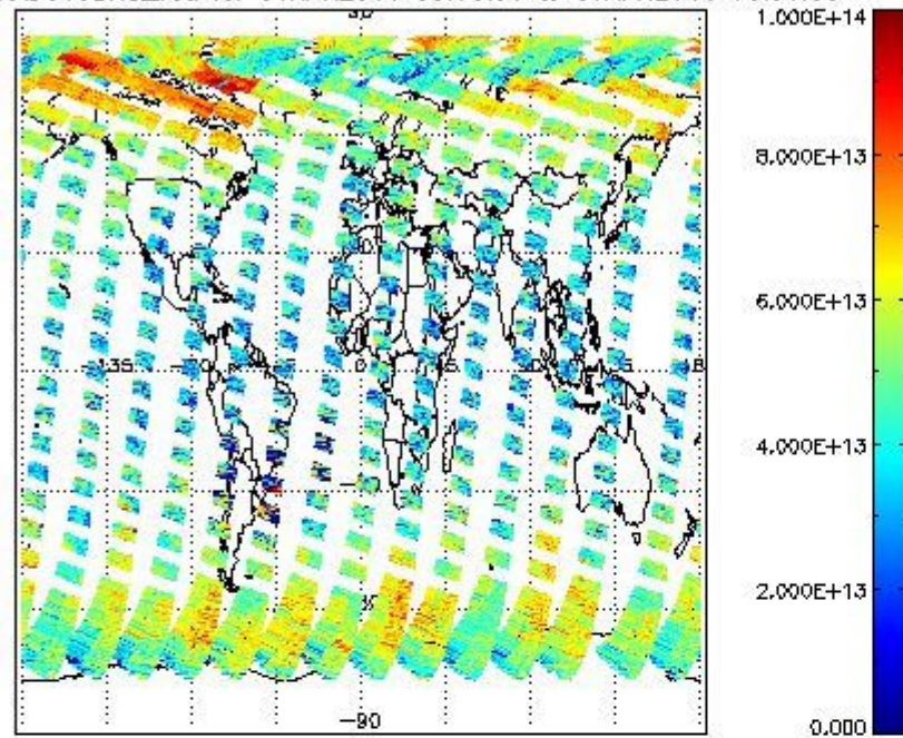
SCIOL2P_NADUV3BRO_vcd for 06APR2011 00:00:00 to 07APR2011 00:00:00
