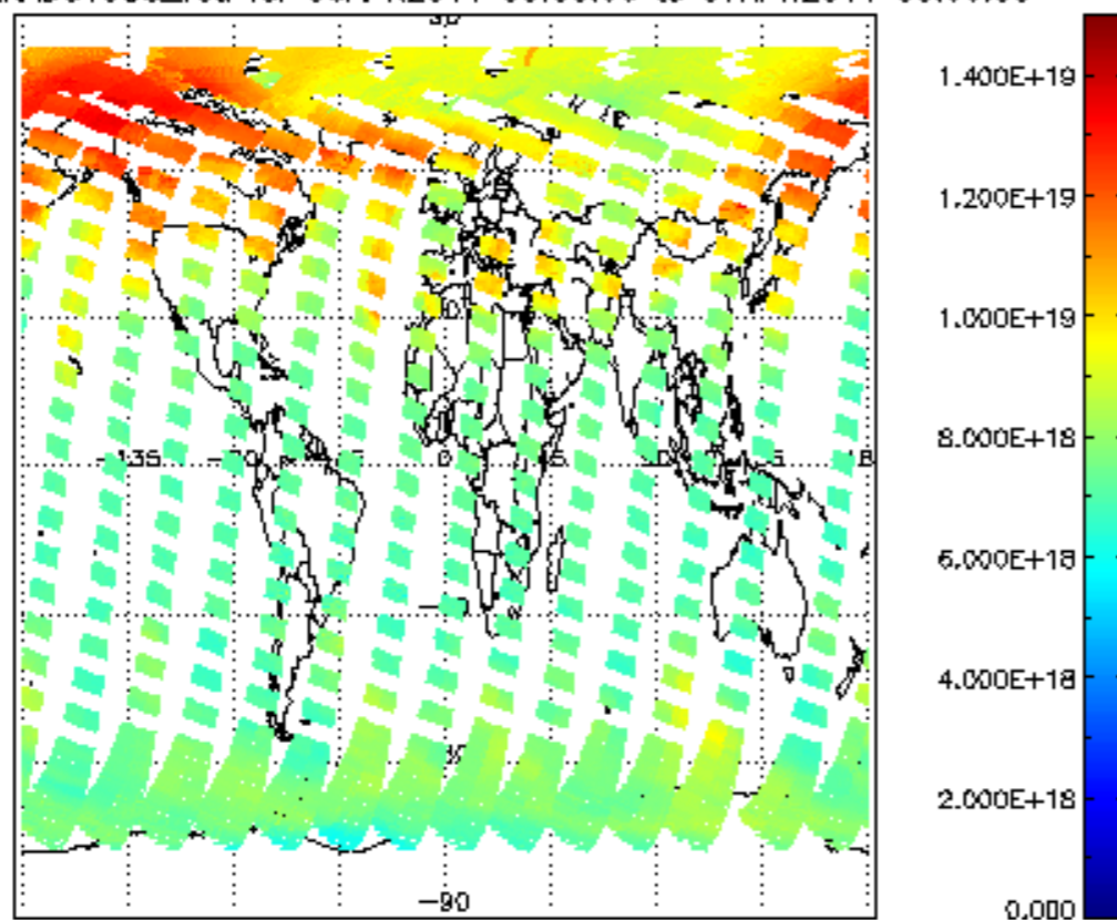
SCIOL2P_NADUV003_vcd for 06APR2011 00:00:00 to 07APR2011 00:00:00
