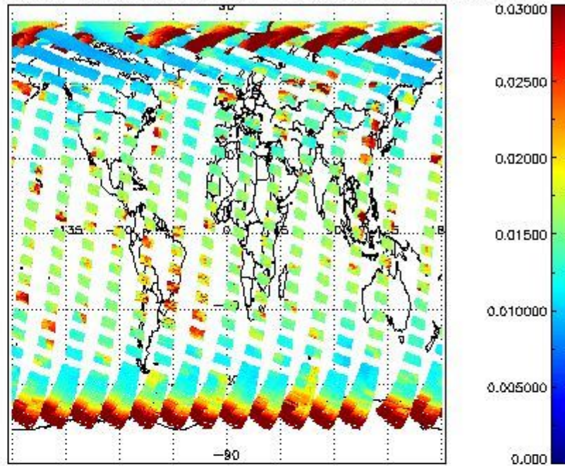
SCIOL2P_NADUV003_vcd_err for 06APR2011 00:00:00 to 07APR2011 00:00:00
