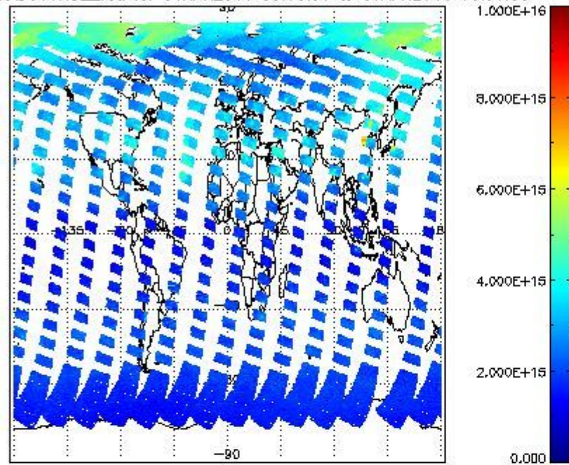
SCIOL2P_NADUV1NO2_vcd for 06APR2011 00:00:00 to 07APR2011 00:00:00
