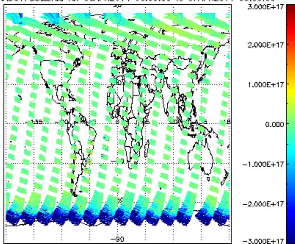
SCIOL2P_NADUV7S02_vcd for 06APR2011 00:00:00 to 07APR2011 00:00:00
