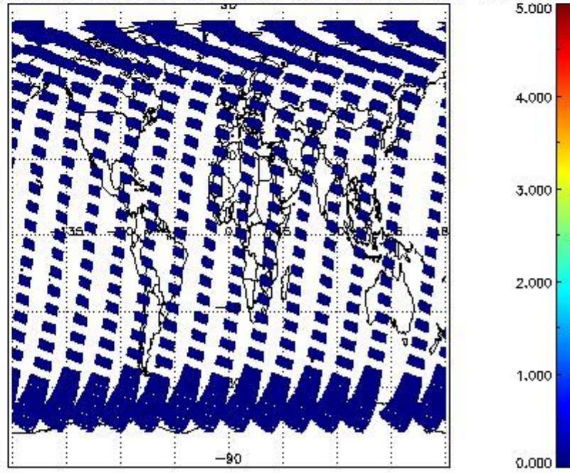
SCIOL2P_NADUV5S02_amf_cl for 06APR2011 00:00:00 to 07APR2011 00:00:00
