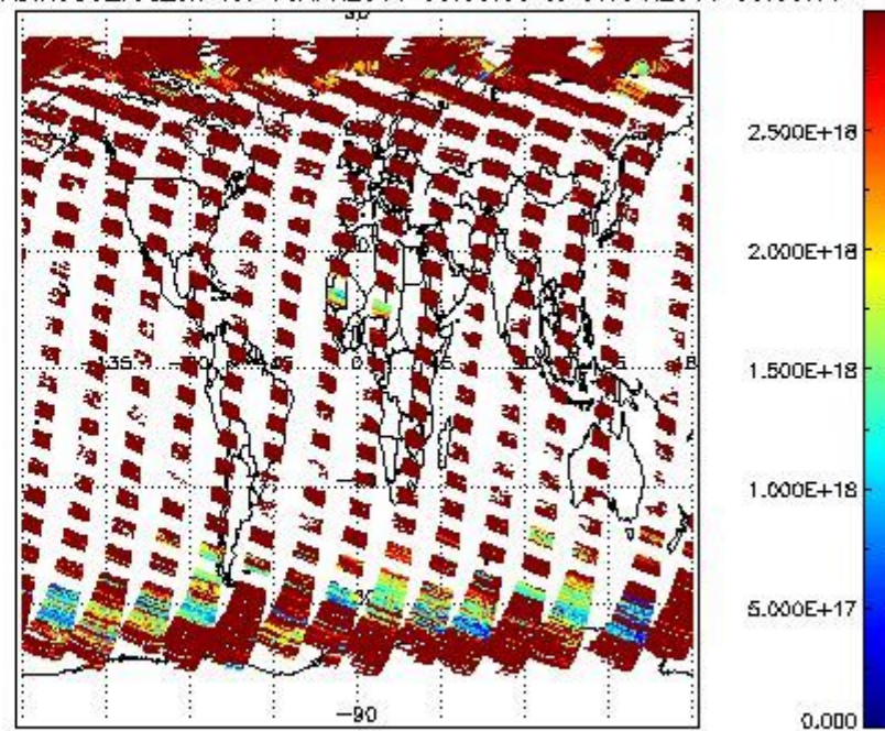
SCIDL2P_NADIR3CO_vcd_err for 06APR2011 00:00:00 to 07APR2011 00:00:00
