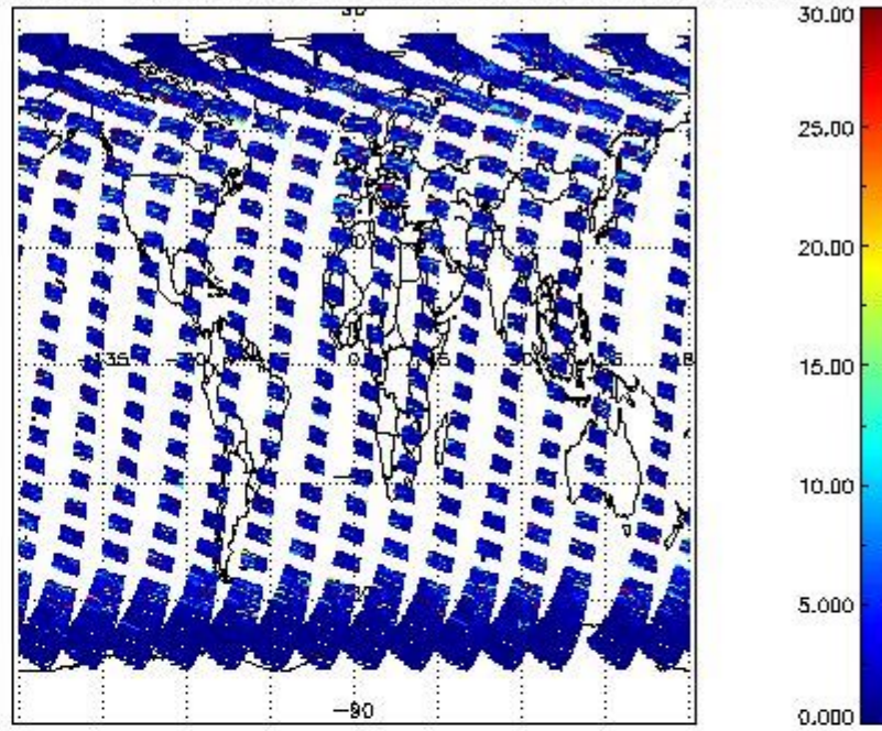
SCIOL2P_NADUV5S02_vcd_err for 06APR2011 00:00:00 to 07APR2011 00:00:00
