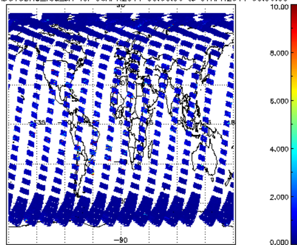
SCIOL2P_NADUV3BRO_vcd_err for 06APR2011 00:00:00 to 07APR2011 00:00:00
