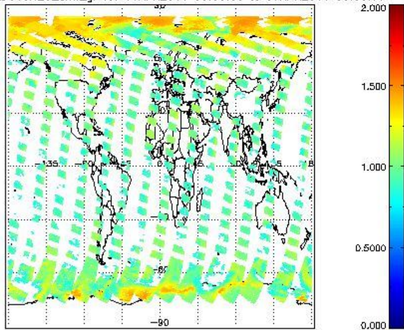
SCIOL2P_NADUV8H2O_arnf_gr for 06APR2011 00:00:00 to 07APR2011 00:00:00
