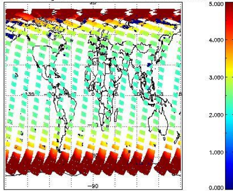
SCIOL2P_NADUV1NO2_amf_gr for 06APR2011 00:00:00 to 07APR2011 00:00:00
