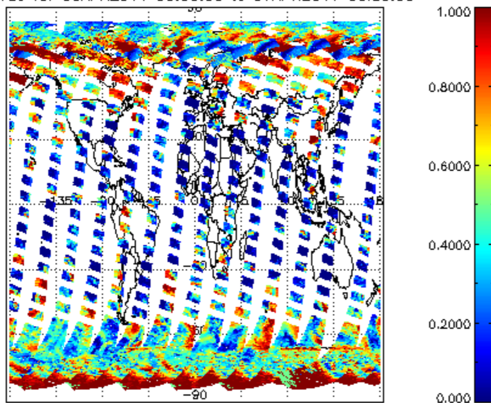
cl_frac for 06APR2011 00:00:00 to 07APR2011 00:00:00
