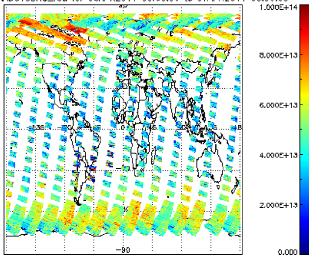
SCIOL2P_NADUV3BRO_vcd for 06APR2011 00:00:00 to 07APR2011 00:00:00
