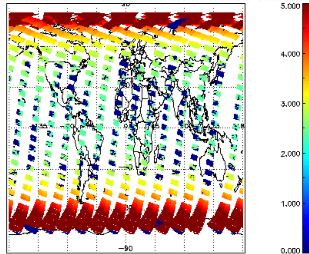
SCIOL2P_NADUV003_amf_cl for 06APR2011 00:00:00 to 07APR2011 00:00:00
