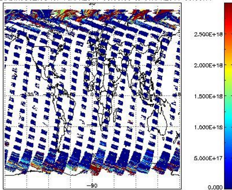
SCIDL2P_NADIR3CO_vcd for 06APR2011 00:00:00 to 07APR2011 00:00:00
