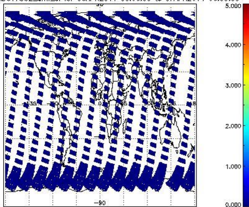
SCIOL2P_NADUV7S02_amf_cl for 06APR2011 00:00:00 to 07APR2011 00:00:00
