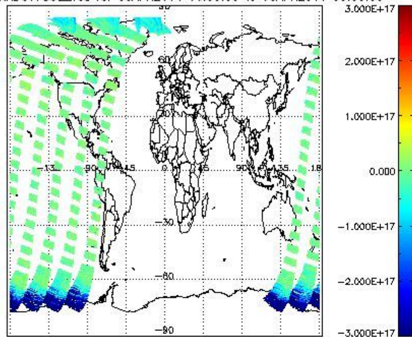
SCIOL2P_NADUV7S02_vcd for 05APR2011 00:00:00 to 06APR2011 00:00:00
