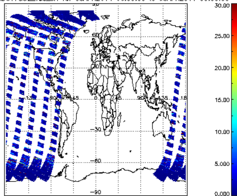
SCIOL2P_NADUV7S02_vcd_err for 05APR2011 00:00:00 to 06APR2011 00:00:00
