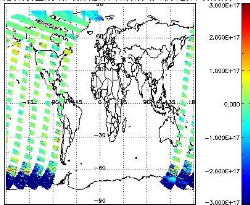
SCIOL2P_NADUV5S02_vcd for 05APR2011 00:00:00 to 06APR2011 00:00:00
