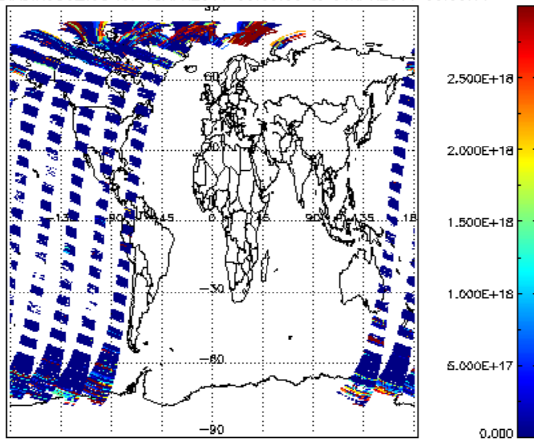
SCIOL2P_NADIR3CO_vcd for 05APR2011 00:00:00 to 06APR2011 00:00:00
