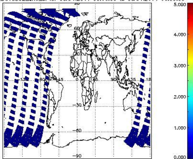
SCIOL2P_NADUV5S02_amf_cl for 05APR2011 00:00:00 to 06APR2011 00:00:00
