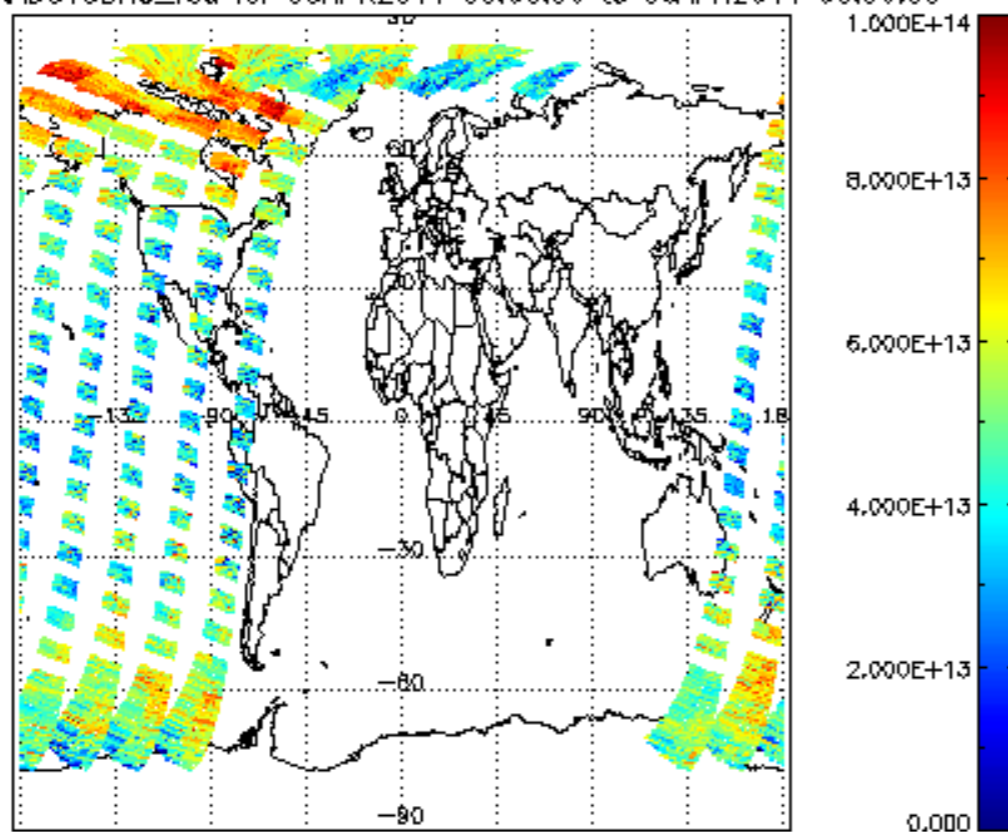
SCIOL2P_NADUV3BRO_vcd for 05APR2011 00:00:00 to 06APR2011 00:00:00
