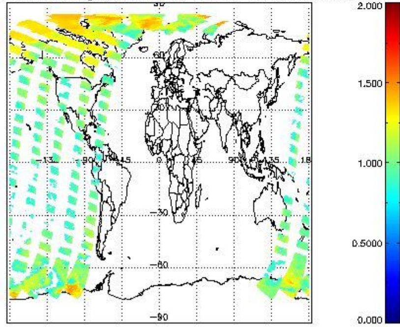
SCIOL2P_NADUV8H2O_amf_gr for 05APR2011 00:00:00 to 06APR2011 00:00:00
