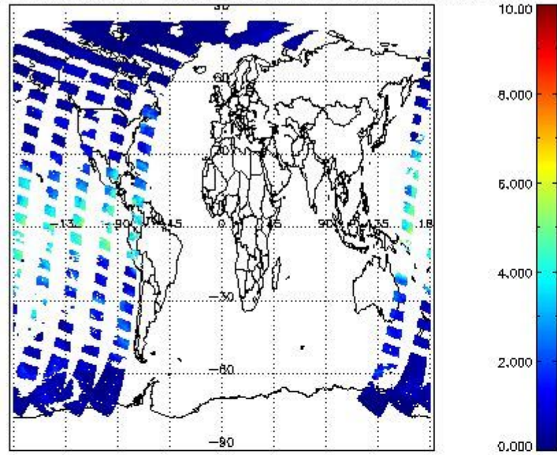
SCIOL2P_NADUV8H2O_vcd for 05APR2011 00:00:00 to 06APR2011 00:00:00
