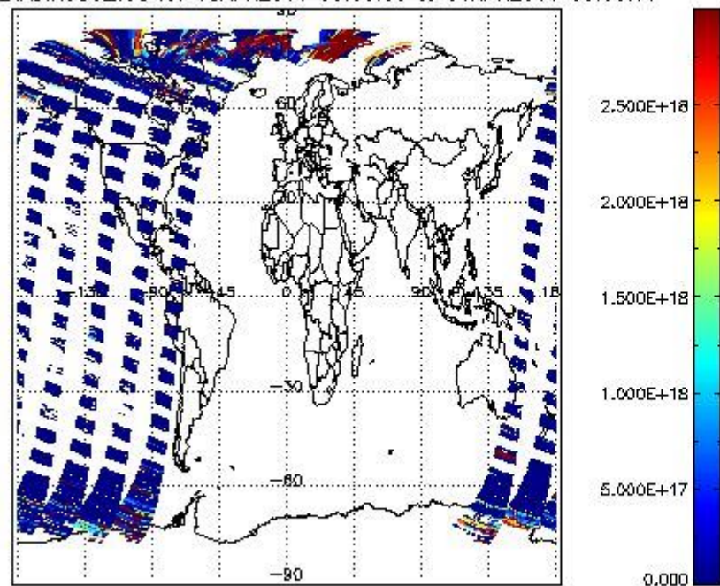
SCIO2P_NADIR3CO_vcd for 05APR2011 00:00:00 to 06APR2011 00:00:00
