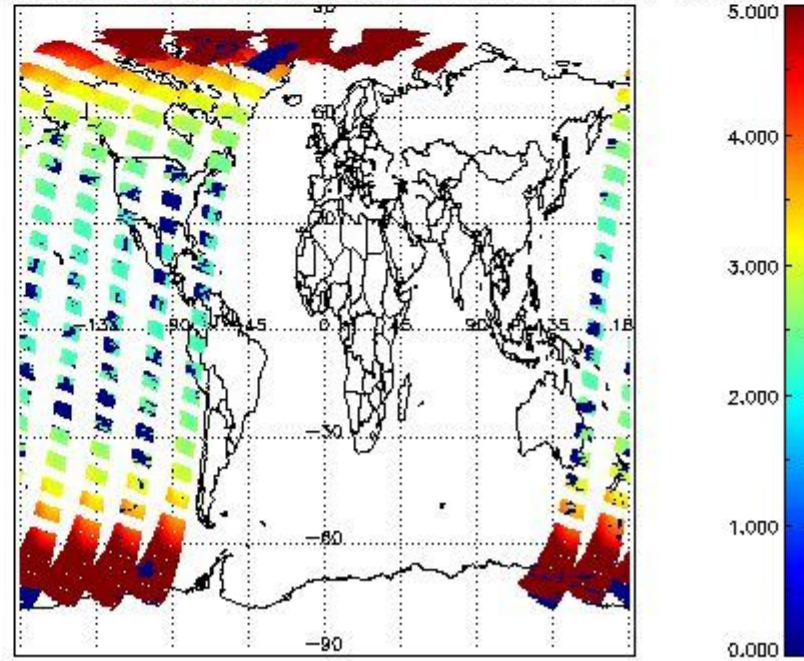
SCIOL2P_NADUV1NO2_amf_cl for 05APR2011 00:00:00 to 06APR2011 00:00:00
