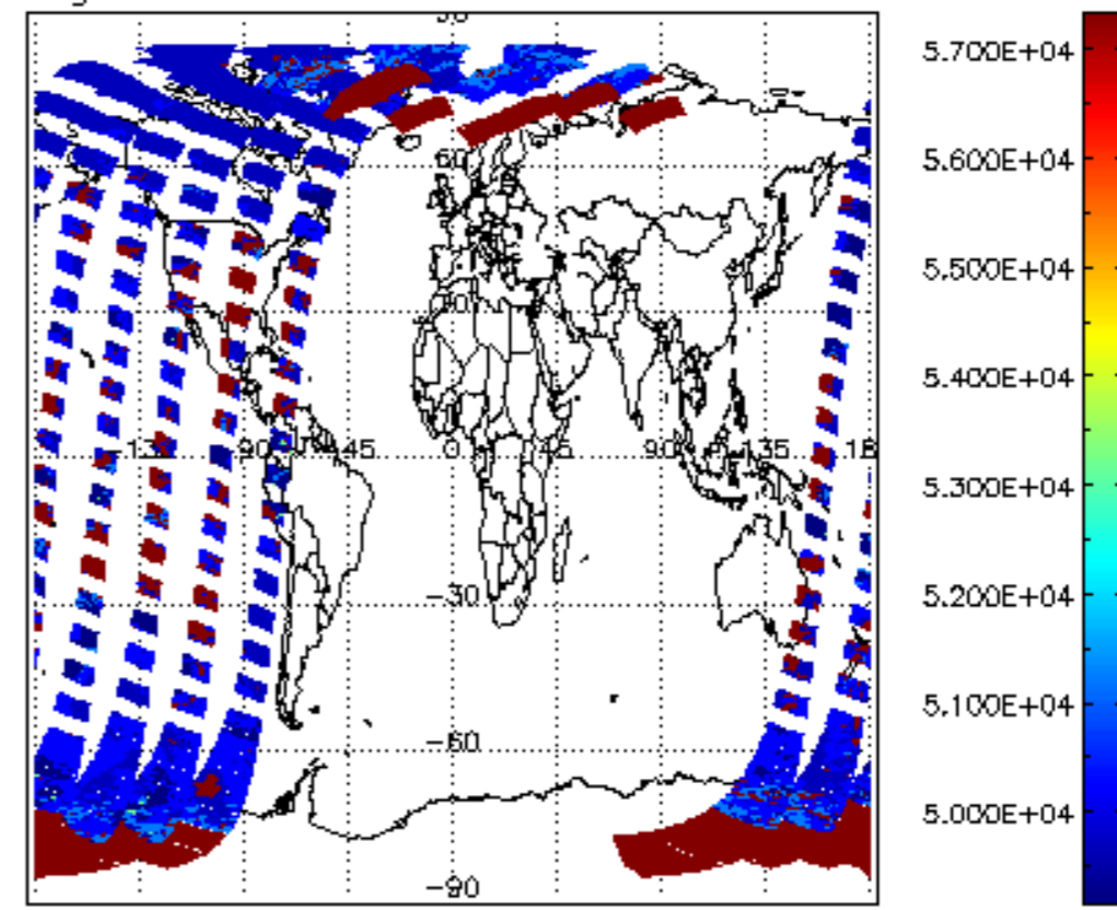
cloud_flags for 05APR2011 00:00:00 to 06APR2011 00:00:00
