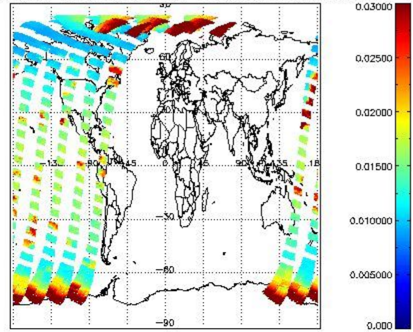
SCIOL2P_NADUV003_vcd_err for 05APR2011 00:00:00 to 06APR2011 00:00:00
