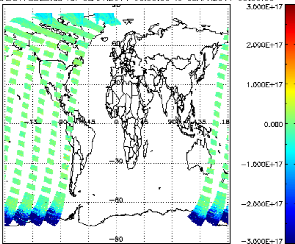
SCIOL2P_NADUV7S02_vcd for 05APR2011 00:00:00 to 06APR2011 00:00:00
