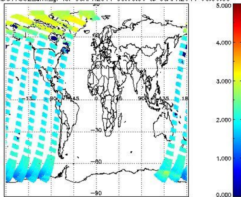
SCIOL2P_NADUV7S02_amf_gr for 05APR2011 00:00:00 to 06APR2011 00:00:00
