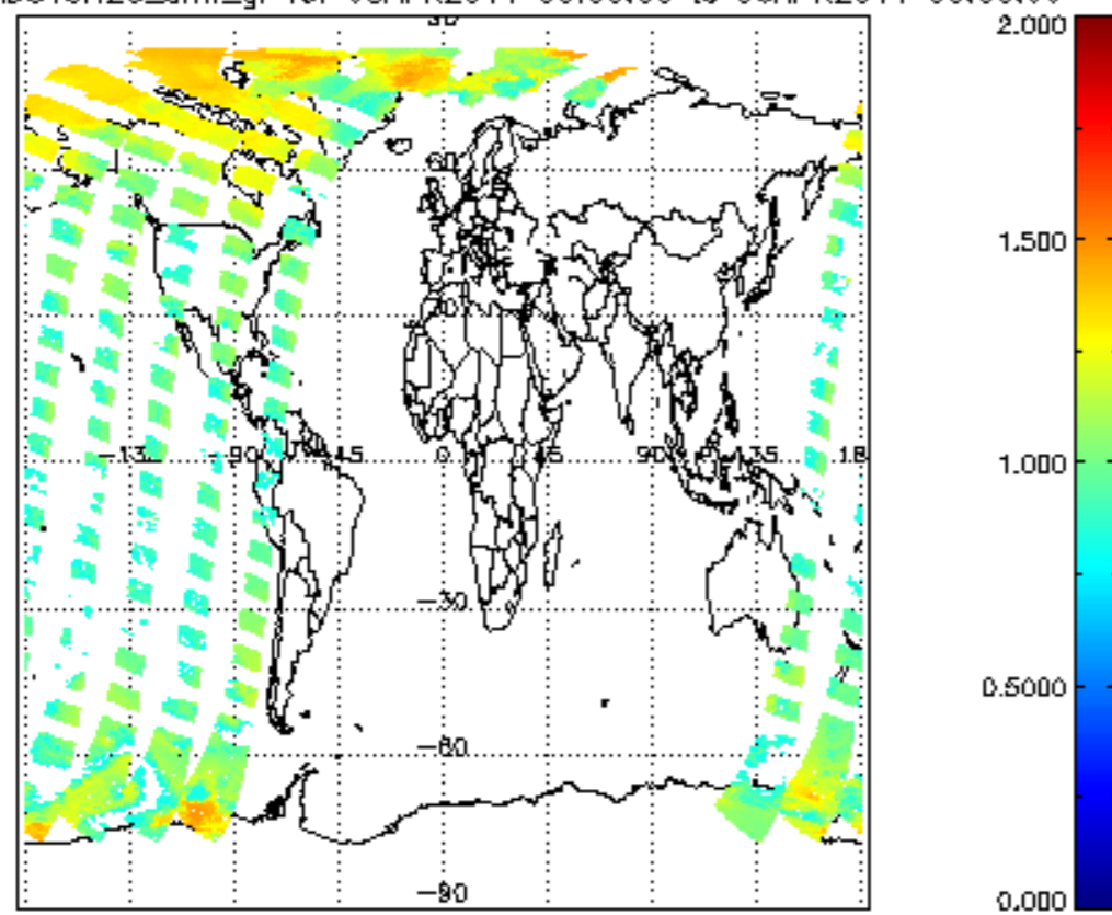
SCIOL2P_NADUV8H2O_amf_gr for 05APR2011 00:00:00 to 06APR2011 00:00:00
