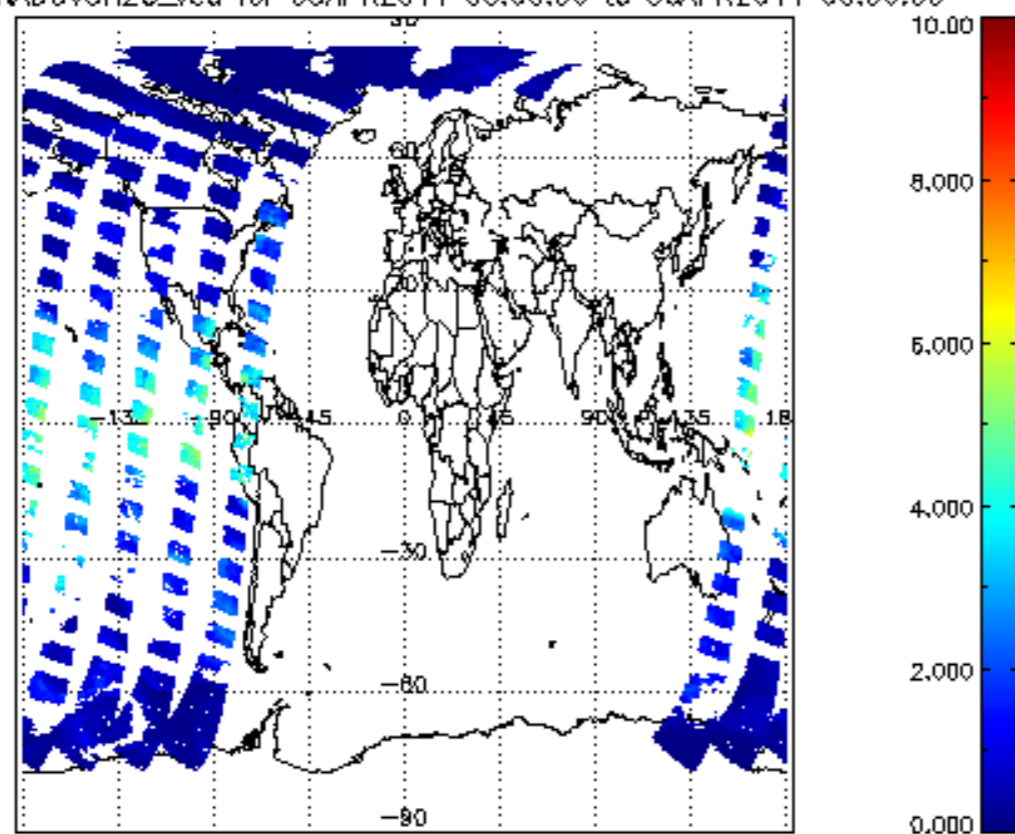
SCIOL2P_NADUV8H2O_vcd for 05APR2011 00:00:00 to 06APR2011 00:00:00
