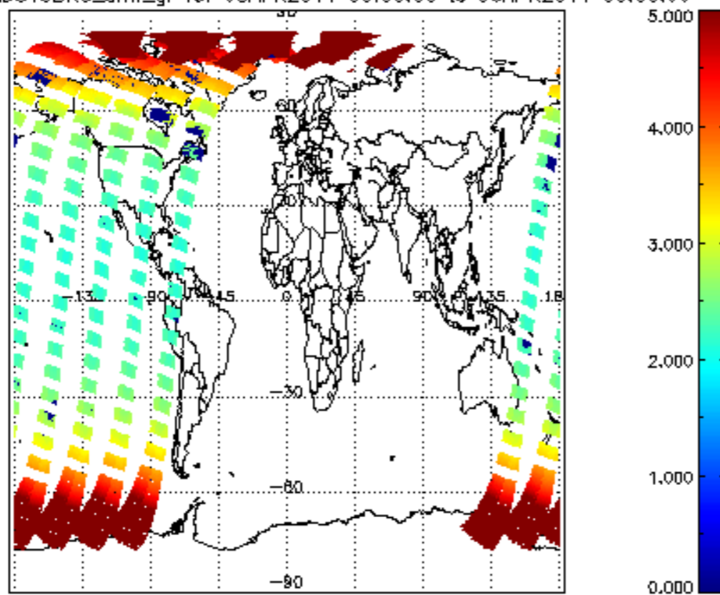
SCIOL2P_NADUV3BRO_amf_gr for 05APR2011 00:00:00 to 06APR2011 00:00:00
