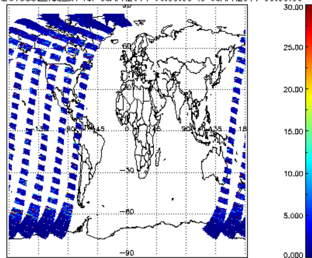
SCIOL2P_NADUV5S02_vcd_err for 05APR2011 00:00:00 to 06APR2011 00:00:00
