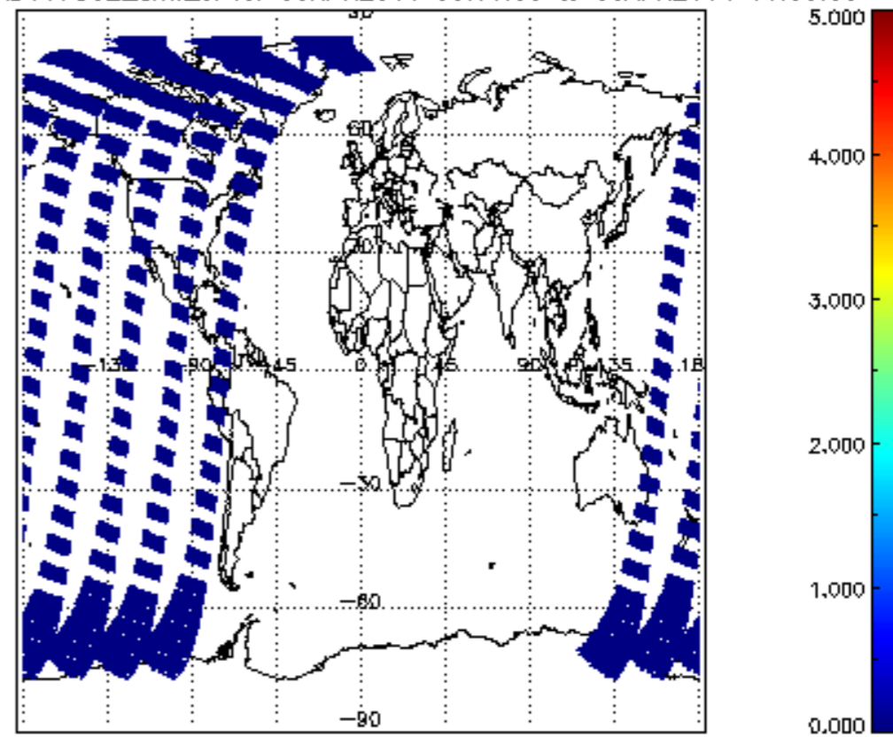
SCIOL2P_NADUV7S02_amf_cl for 05APR2011 00:00:00 to 06APR2011 00:00:00
