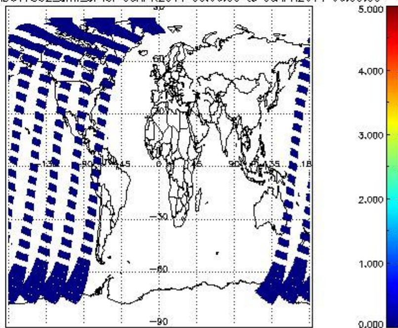
SCIOL2P_NADUV7S02_amf_cl for 05APR2011 00:00:00 to 06APR2011 00:00:00
