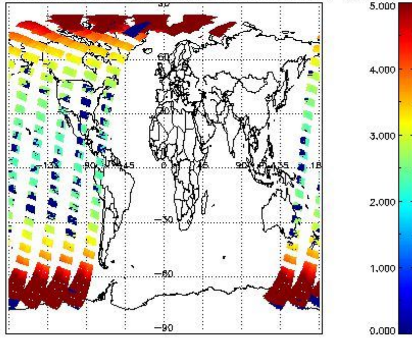
SCIOL2P_NADUV3BRO_amf_cl for 05APR2011 00:00:00 to 06APR2011 00:00:00
