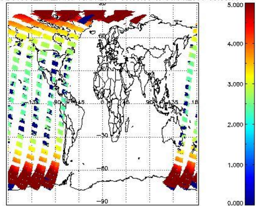
SCIOL2P_NADUV003_amf_cl for 05APR2011 00:00:00 to 06APR2011 00:00:00
