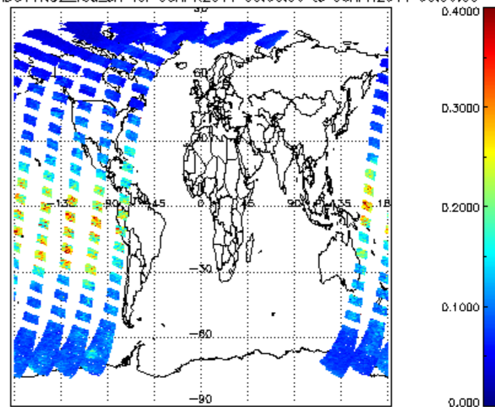
SCIOL2P_NADUV1NO2_vcd_err for 05APR2011 00:00:00 to 06APR2011 00:00:00
