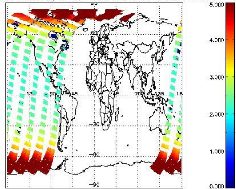
SCIOL2P_NADUV003_amf_gr for 05APR2011 00:00:00 to 06APR2011 00:00:00
