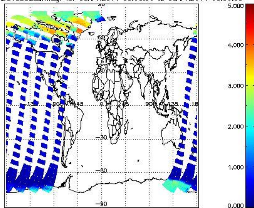
SCIOL2P_NADUV5S02_amf_gr for 05APR2011 00:00:00 to 06APR2011 00:00:00
