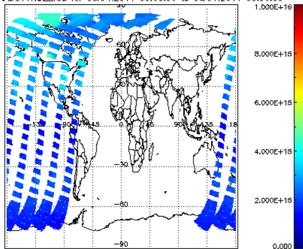
SCIOL2P_NADUV1NO2_vcd for 05APR2011 00:00:00 to 06APR2011 00:00:00
