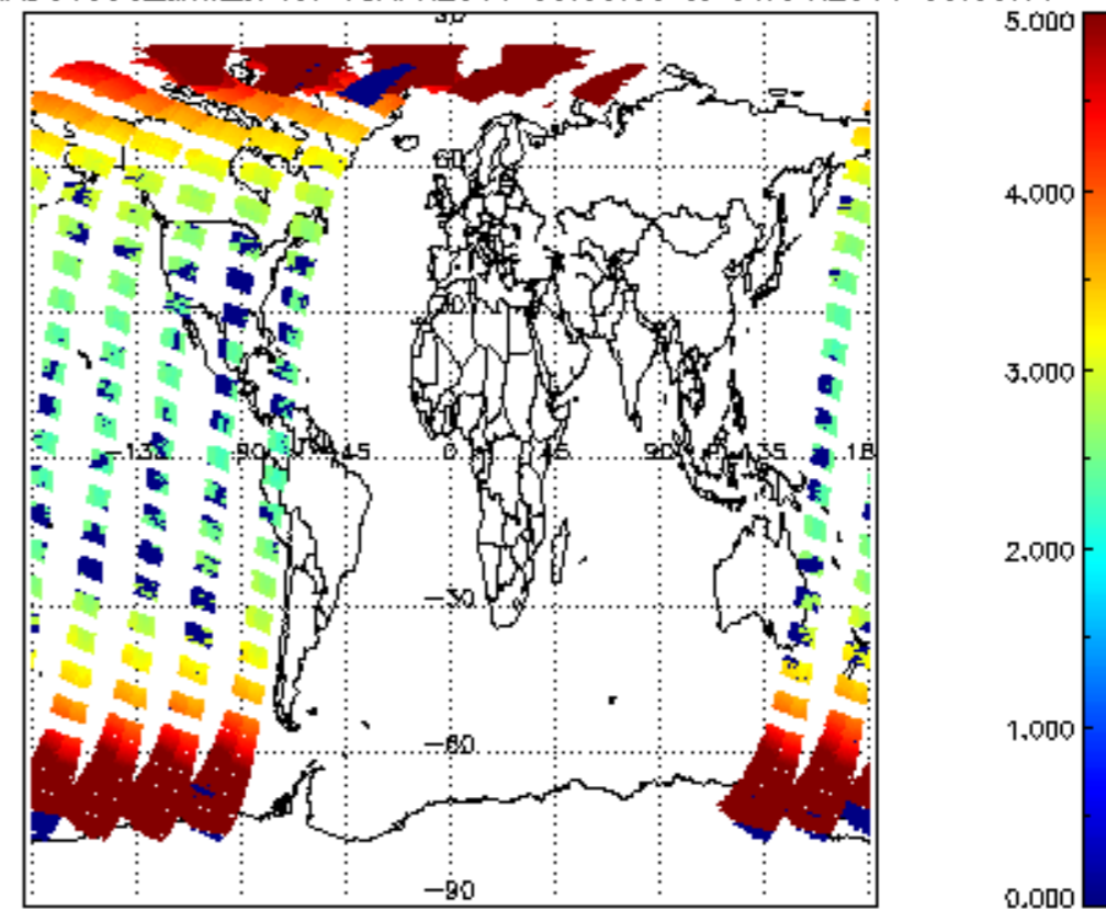
SCIOL2P_NADUV003_amf_cl for 05APR2011 00:00:00 to 06APR2011 00:00:00
