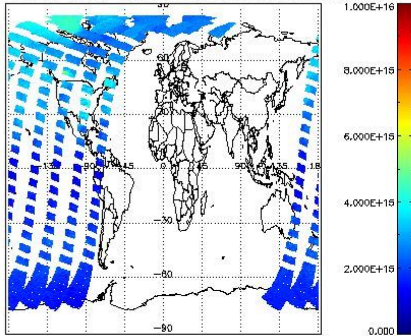
SCIOL2P_NADUV1NO2_vcd for 05APR2011 00:00:00 to 06APR2011 00:00:00
