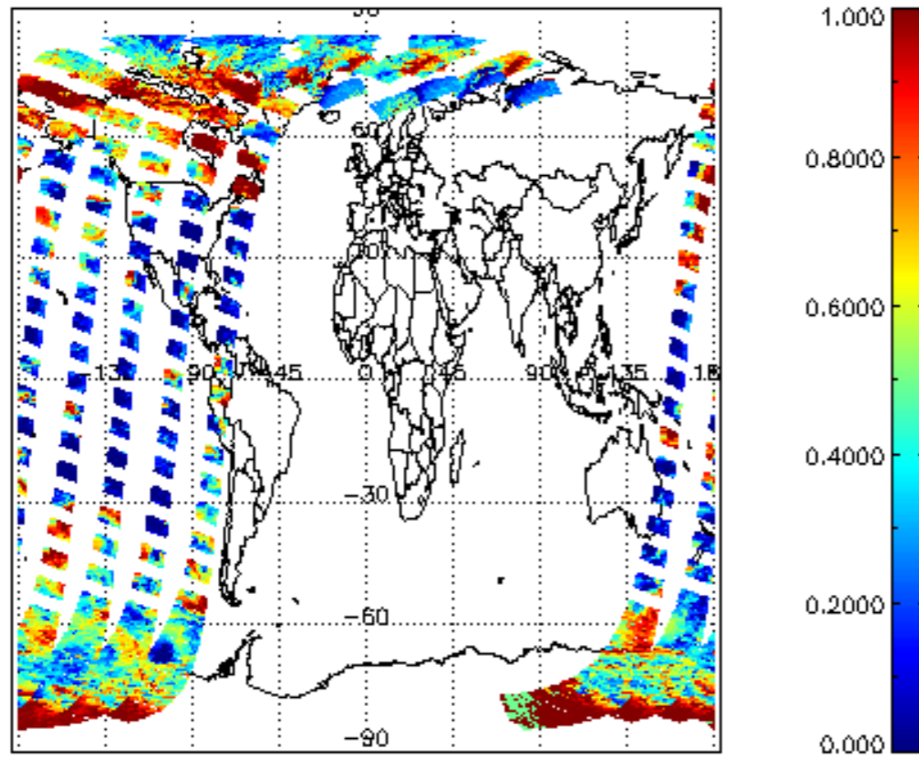
cL_frac for 05APR2011 00:00:00 to 06APR2011 00:00:00
