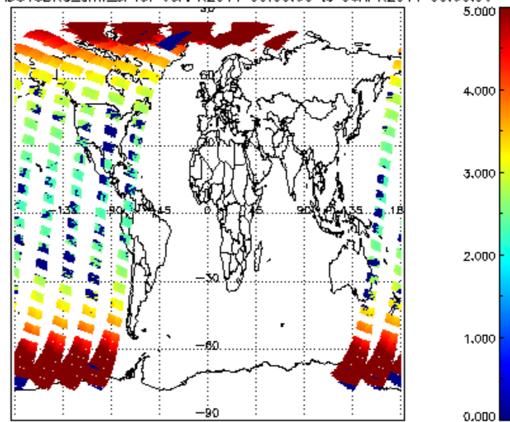
SCIOL2P_NADUV3BRO_amf_sl for 05APR2011 00:00:00 to 06APR2011 00:00:00
