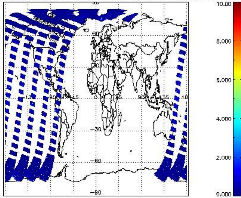
SCIOL2P_NADUV3BRO_vcd_err for 05APR2011 00:00:00 to 06APR2011 00:00:00
