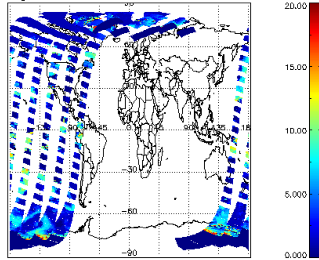
cL_top_height for 05APR2011 00:00:00 to 06APR2011 00:00:00
