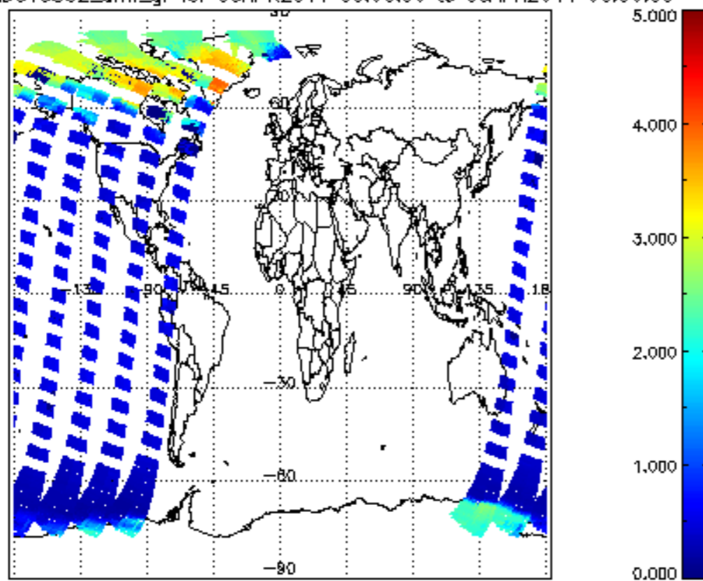
SCIOL2P_NADUV5S02_amf_gr for 05APR2011 00:00:00 to 06APR2011 00:00:00
