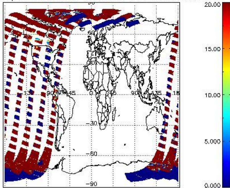
cL_opt_depth for 05APR2011 00:00:00 to 06APR2011 00:00:00
