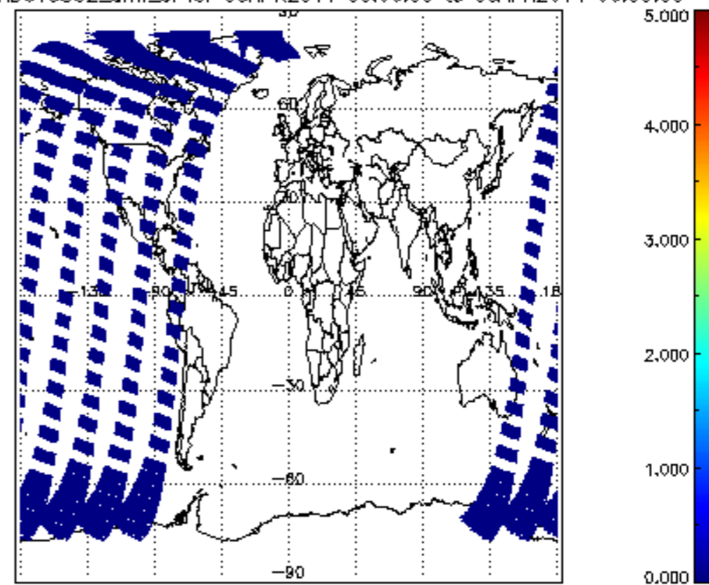
SCIOL2P_NADUV5S02_amf_cl for 05APR2011 00:00:00 to 06APR2011 00:00:00
