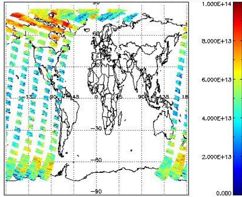
SCIOL2P_NADUV3BRO_vcd for 05APR2011 00:00:00 to 06APR2011 00:00:00
