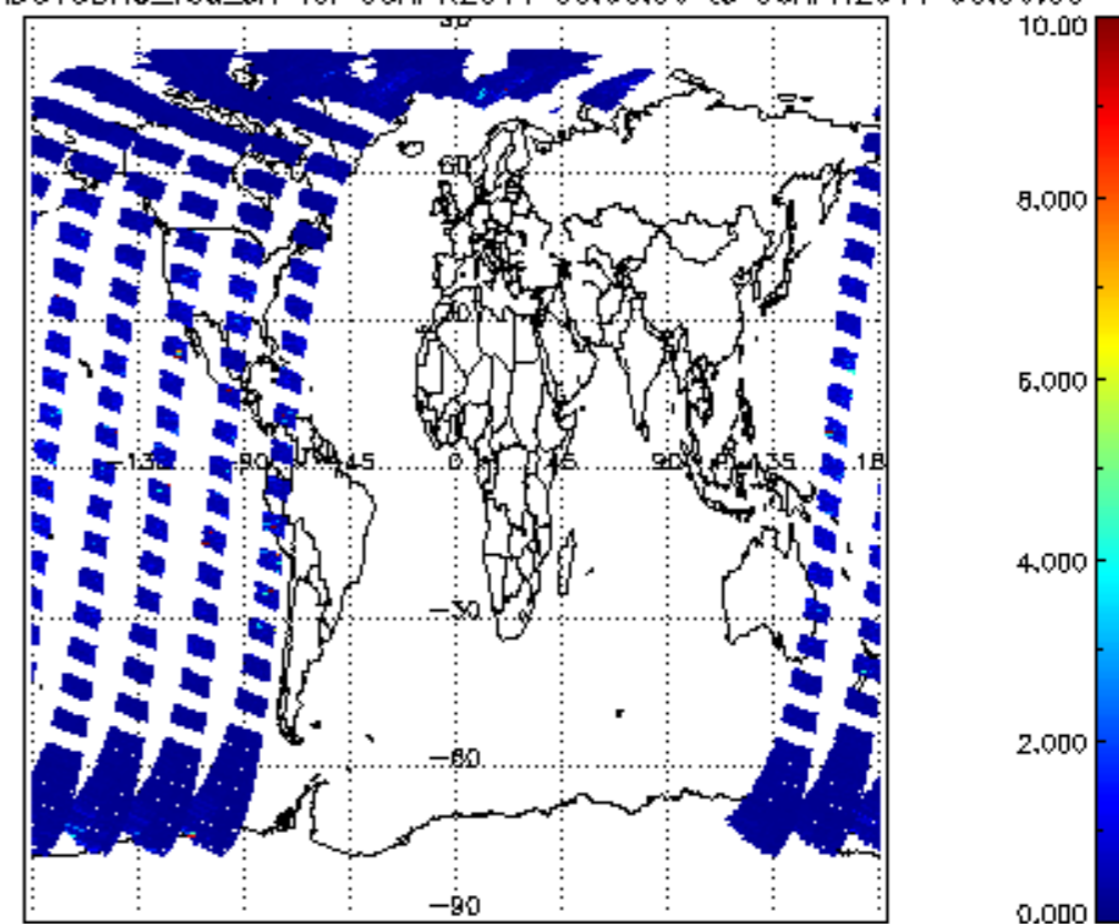
SCIOL2P_NADUV3BRO_vcd_err for 05APR2011 00:00:00 to 06APR2011 00:00:00
