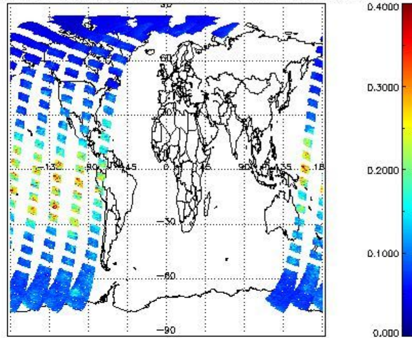
SCIOL2P_NADUV1NO2_vcd_err for 05APR2011 00:00:00 to 06APR2011 00:00:00
