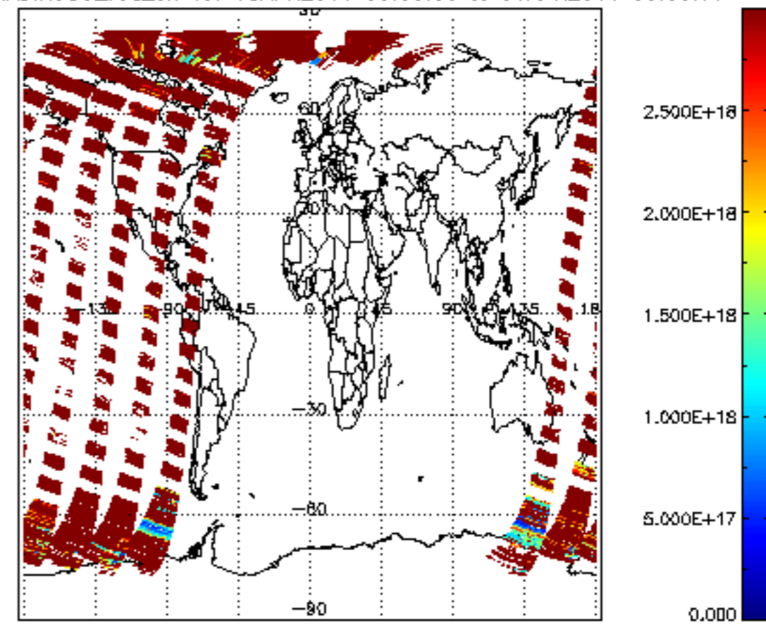
SCIOL2P_NADIR3CO_vcd_err for 05APR2011 00:00:00 to 06APR2011 00:00:00
