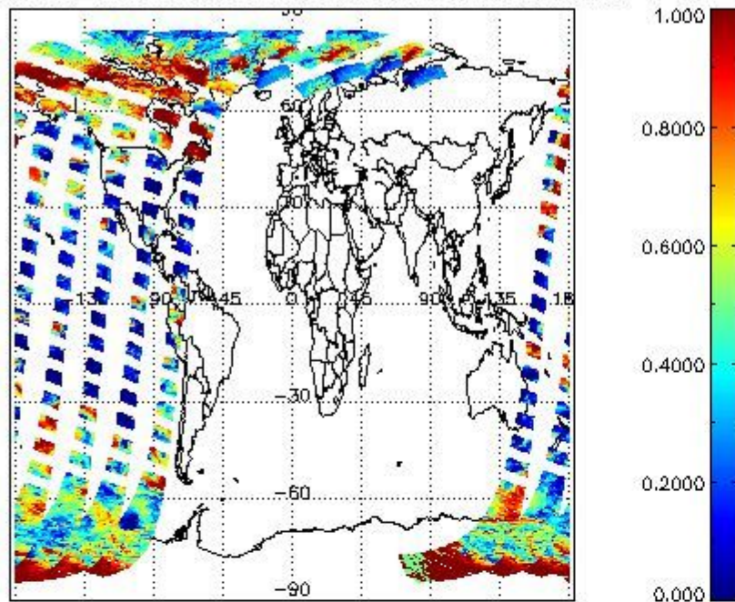
cL_frac for 05APR2011 00:00:00 to 06APR2011 00:00:00
