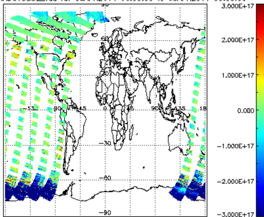
SCIOL2P_NADUV5S02_vcd for 05APR2011 00:00:00 to 06APR2011 00:00:00
