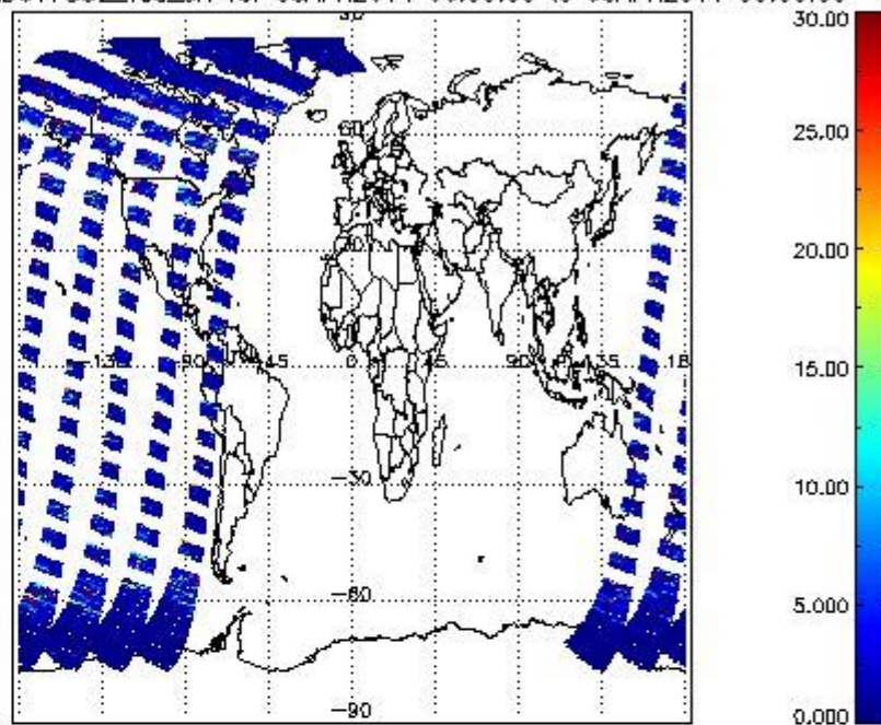
SCIOL2P_NADUV7S02_vcd_err for 05APR2011 00:00:00 to 06APR2011 00:00:00
