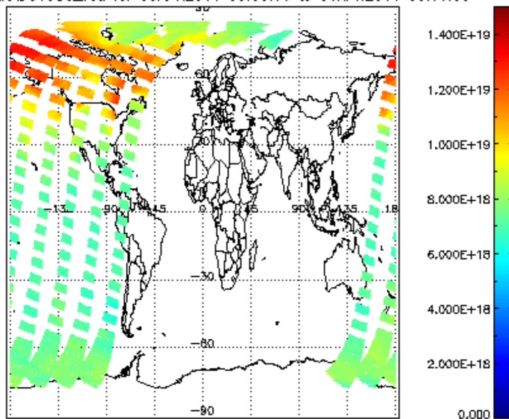
SCIOL2P_NADUV003_vcd for 05APR2011 00:00:00 to 06APR2011 00:00:00
