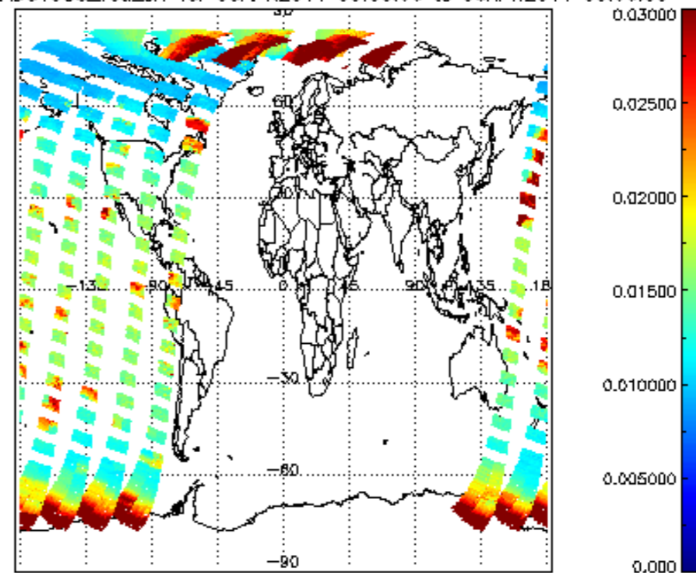
SCIOL2P_NADUV003_vcd_err for 05APR2011 00:00:00 to 06APR2011 00:00:00
