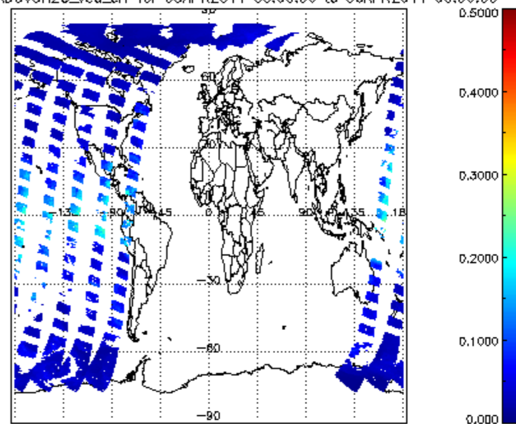
SCIOL2P_NADUV8H2O_vcd_err for 05APR2011 00:00:00 to 06APR2011 00:00:00
