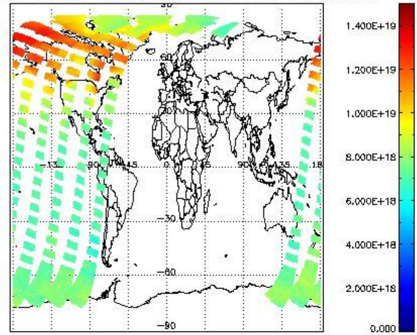
SCIOL2P_NADUV003_vcd for 05APR2011 00:00:00 to 06APR2011 00:00:00
