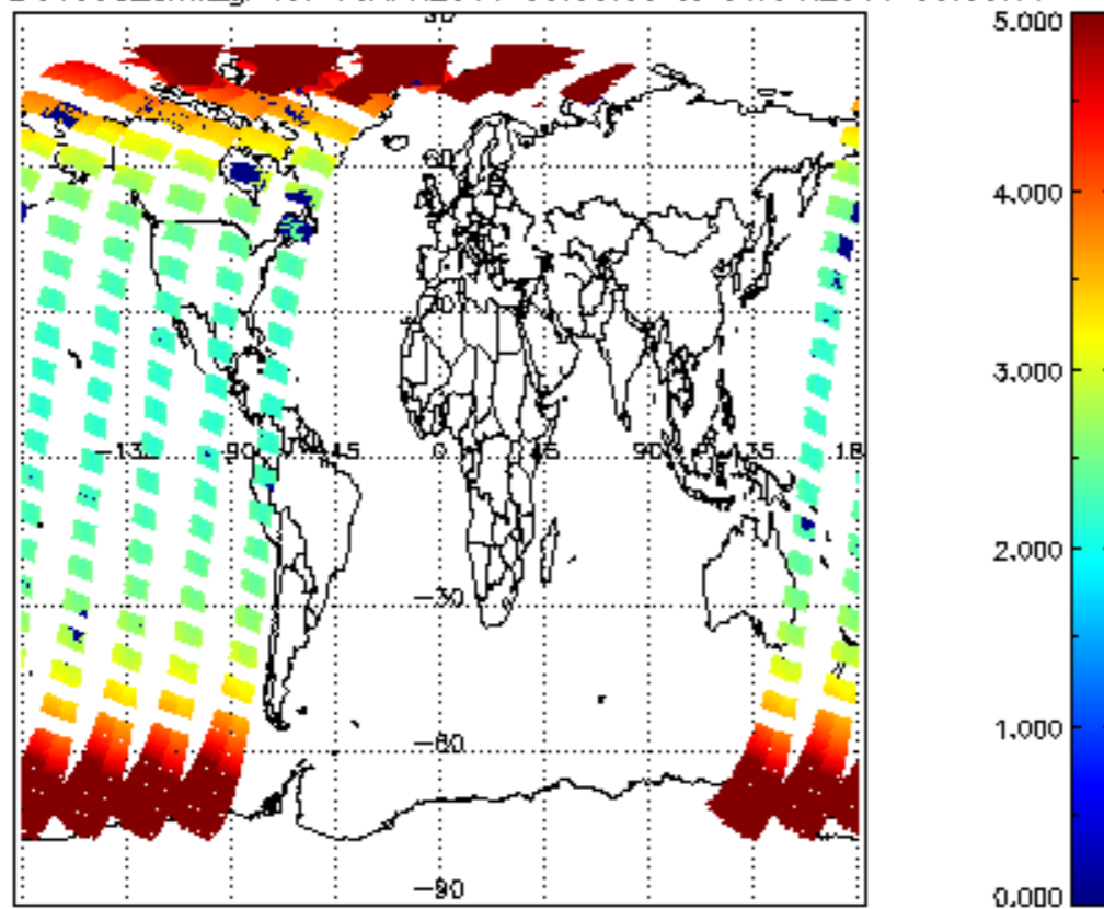
SCIOL2P_NADUV003_amf_gr for 05APR2011 00:00:00 to 06APR2011 00:00:00
