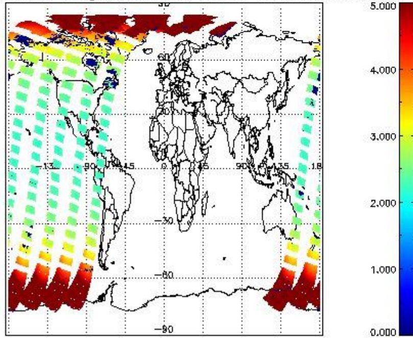
SCIOL2P_NADUV1NO2_amf_gr for 05APR2011 00:00:00 to 06APR2011 00:00:00
