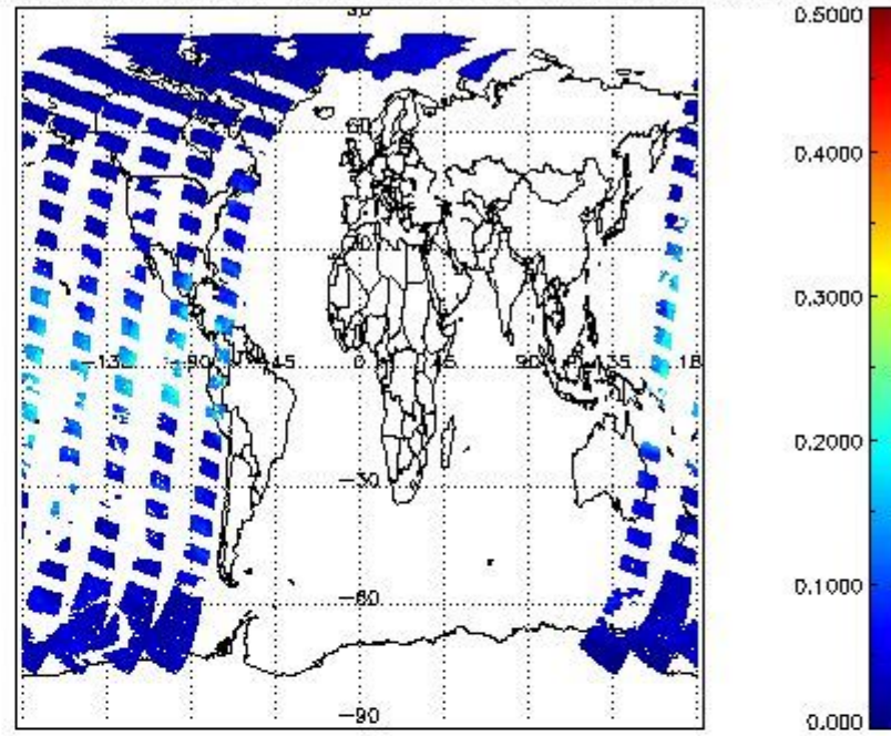
SCIOL2P_NADUV8H2O_vcd_err for 05APR2011 00:00:00 to 06APR2011 00:00:00
