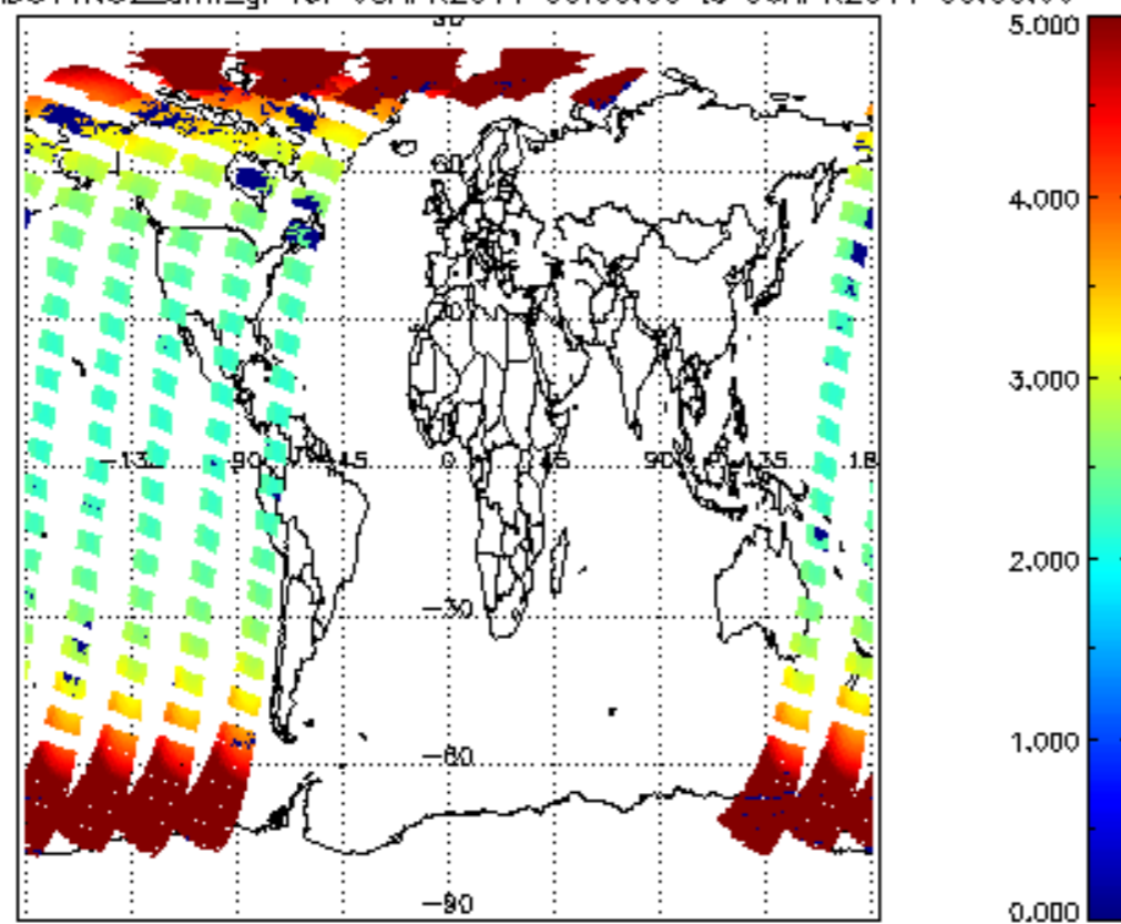
SCIOL2P_NADUV1NO2_amf_gr for 05APR2011 00:00:00 to 06APR2011 00:00:00
