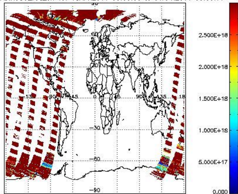
SCIO2P_NADIR3CO_vcd_err for 05APR2011 00:00:00 to 06APR2011 00:00:00
