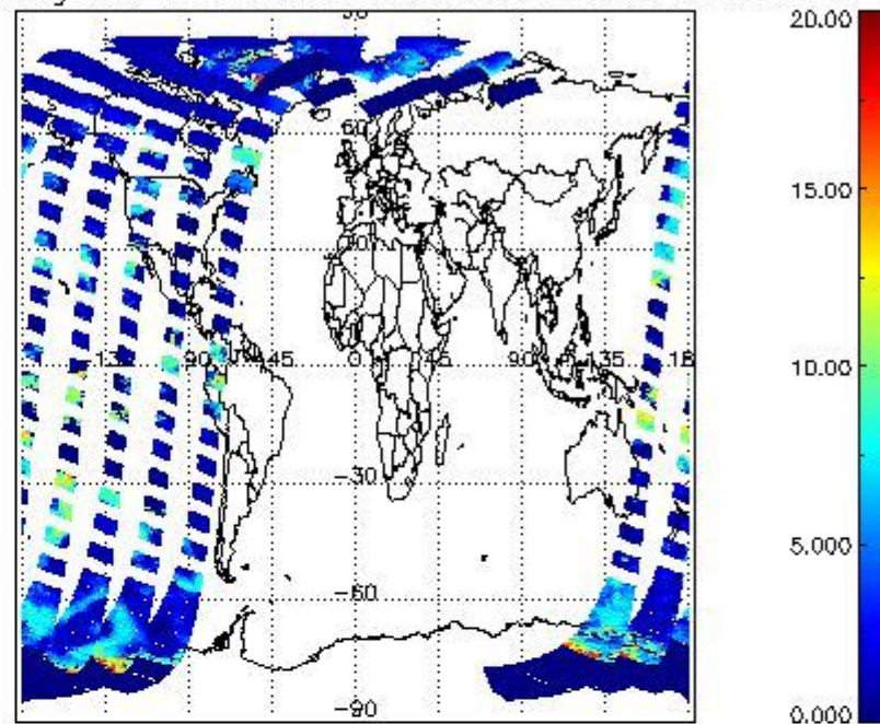
cL_top_height for 05APR2011 00:00:00 to 06APR2011 00:00:00
