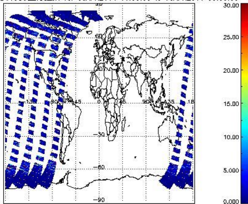
SCIOL2P_NADUV5S02_vcd_err for 05APR2011 00:00:00 to 06APR2011 00:00:00
