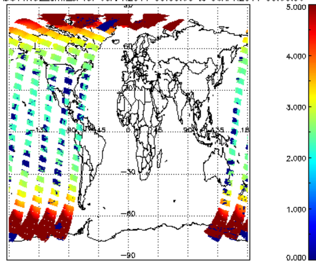
SCIOL2P_NADUV1NO2_amf_sl for 05APR2011 00:00:00 to 06APR2011 00:00:00
