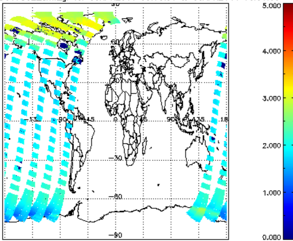
SCIOL2P_NADUV7S02_amf_gr for 05APR2011 00:00:00 to 06APR2011 00:00:00
