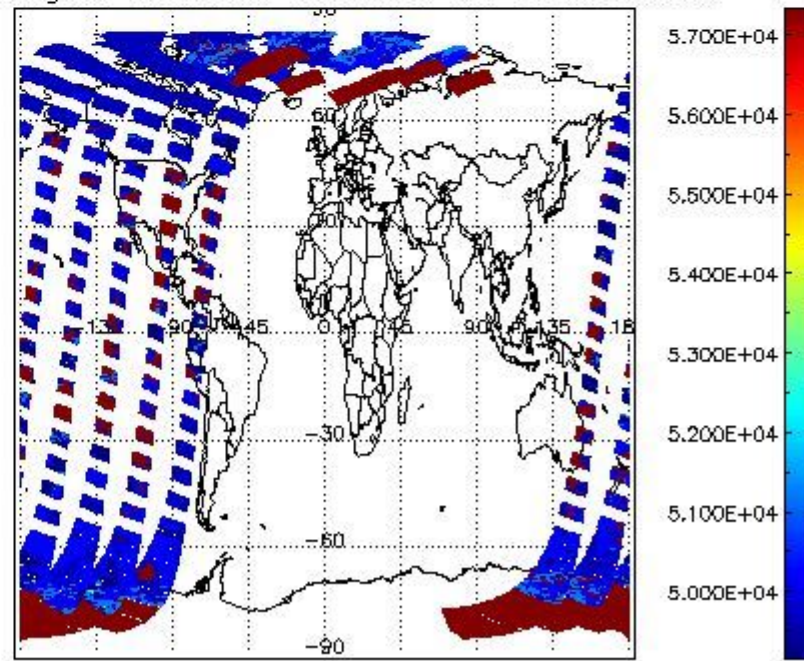
cloud_flags for 05APR2011 00:00:00 to 06APR2011 00:00:00
