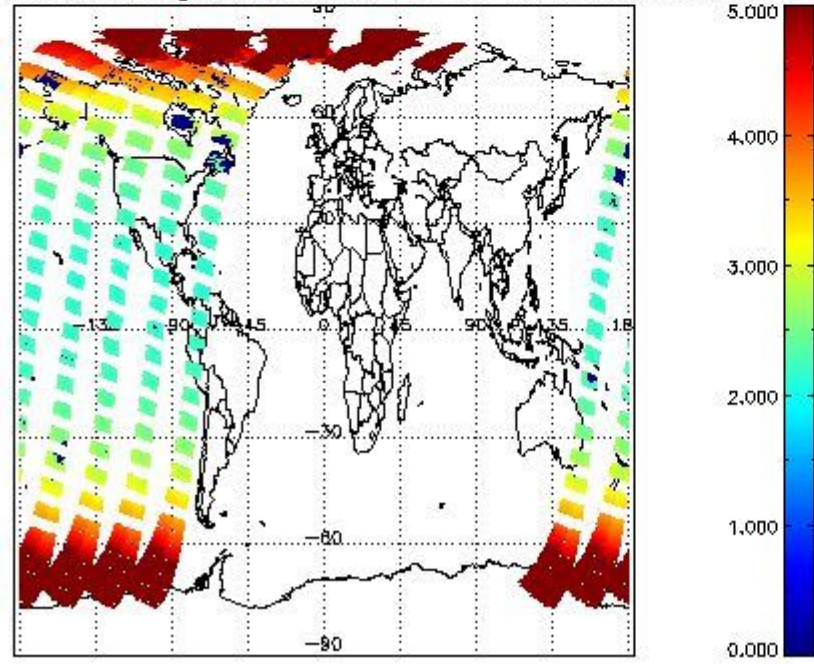
SCIOL2P_NADUV3BRO_amf_gr for 05APR2011 00:00:00 to 06APR2011 00:00:00
