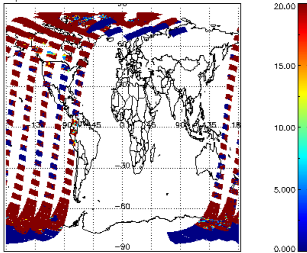
cL_opt_depth for 05APR2011 00:00:00 to 06APR2011 00:00:00
