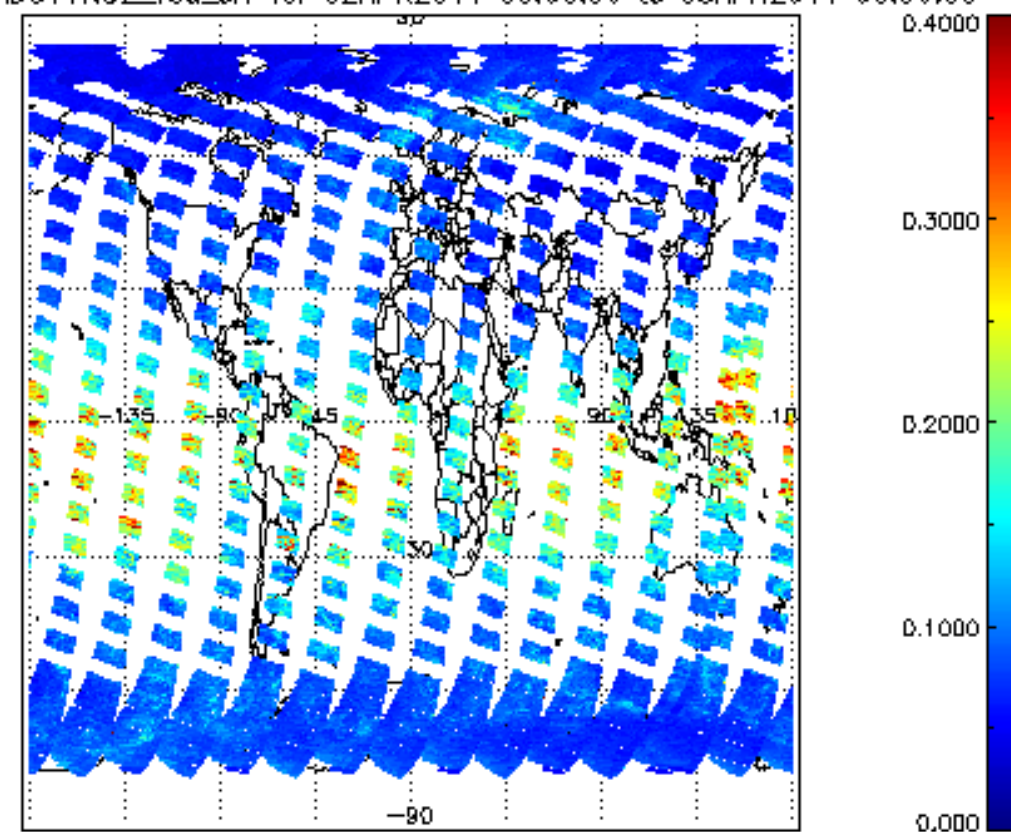
SCIOL2P_NADUV1NO2_vcd_err for 02APR2011 00:00:00 to 03APR2011 00:00:00
