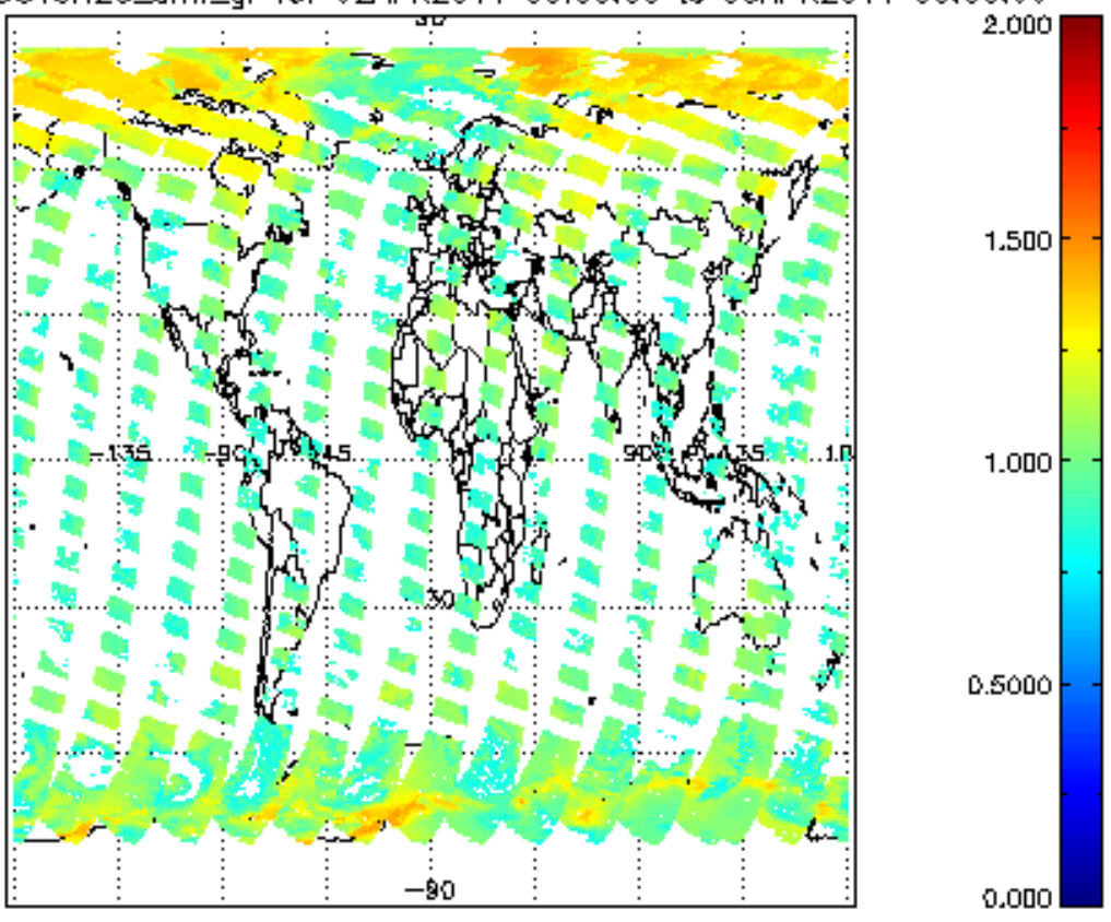
SCIOL2P_NADUV8H2O_amf_gr for 02APR2011 00:00:00 to 03APR2011 00:00:00
