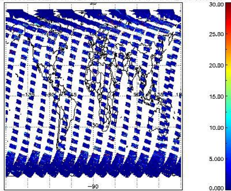
SCIOL2P_NADUV5S02_vcd_err for 02APR2011 00:00:00 to 03APR2011 00:00:00
