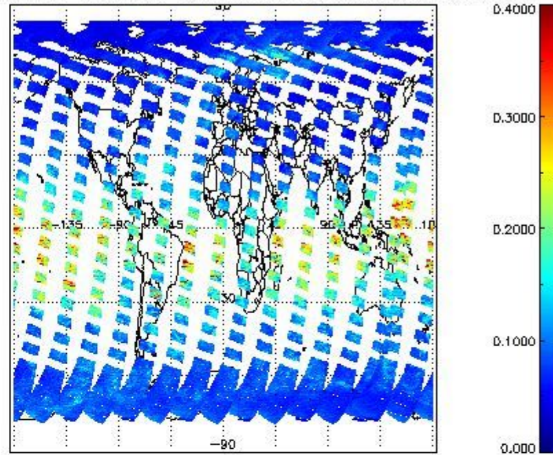
SCIOL2P_NADUV1NO2_vcd_err for 02APR2011 00:00:00 to 03APR2011 00:00:00
