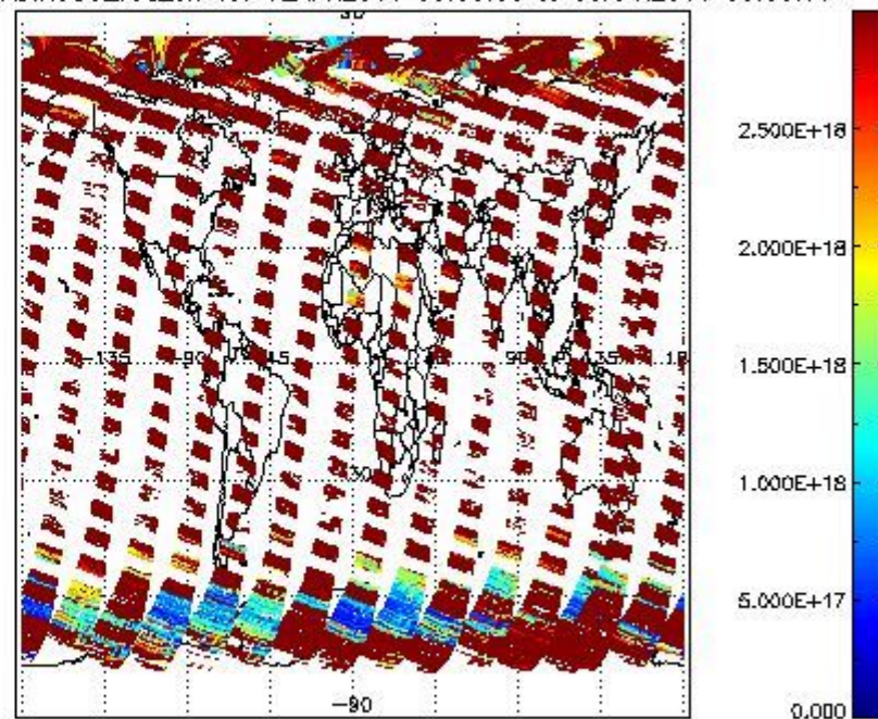
SCIDL2P_NADIR3CO_vcd_err for 02APR2011 00:00:00 to 03APR2011 00:00:00
