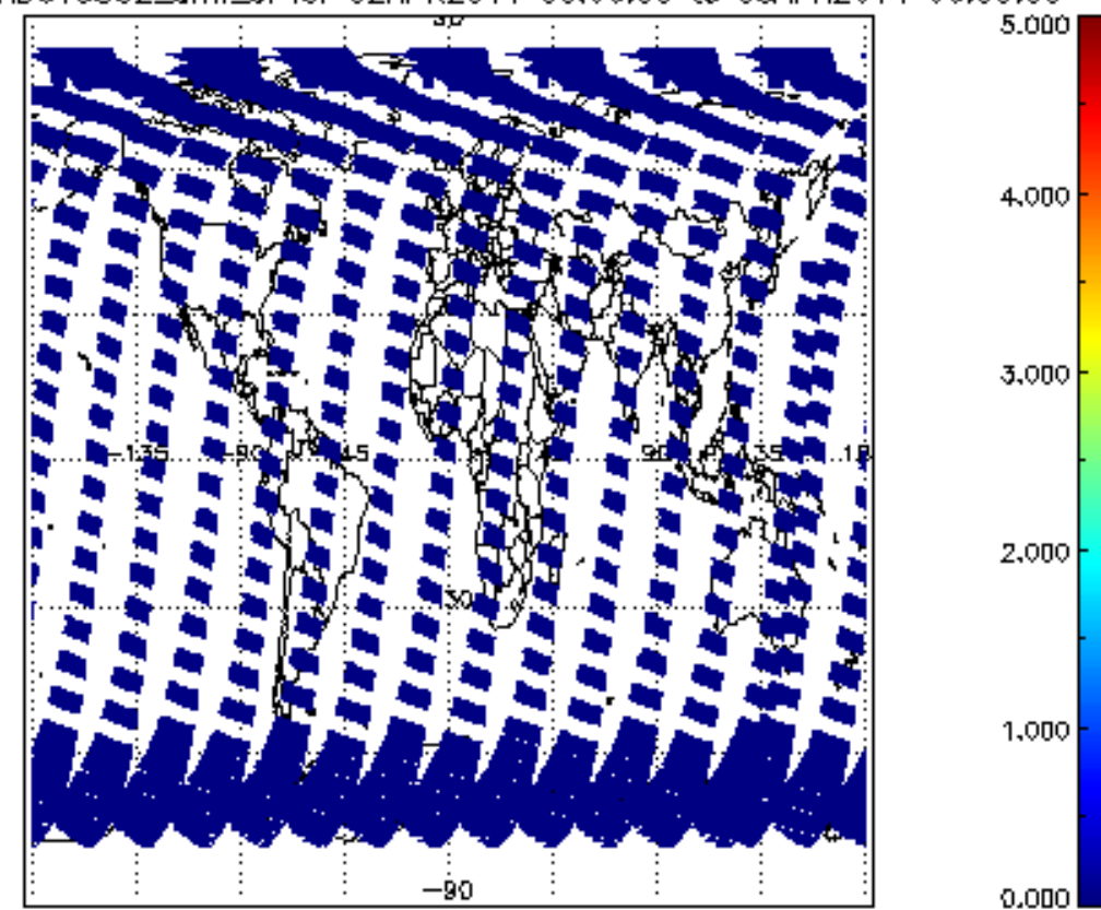
SCIOL2P_NADUV5S02_amf_cl for 02APR2011 00:00:00 to 03APR2011 00:00:00
