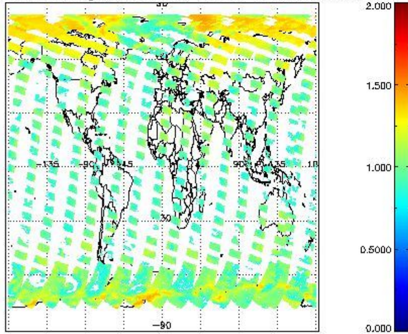
SCIOL2P_NADUV8H2O_arnf_gr for 02APR2011 00:00:00 to 03APR2011 00:00:00
