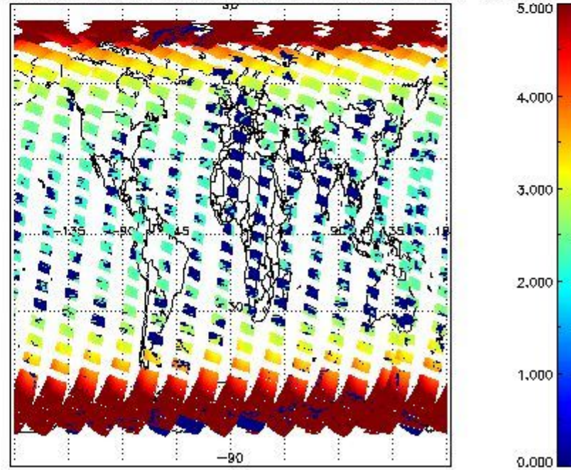
SCIOL2P_NADUV1NO2_amf_cl for 02APR2011 00:00:00 to 03APR2011 00:00:00
