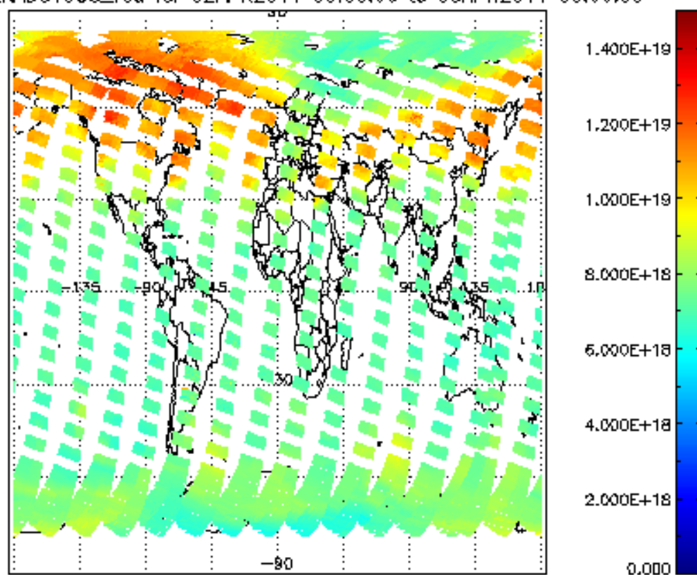
SCIOL2P_NADUV003_vcd for 02APR2011 00:00:00 to 03APR2011 00:00:00
