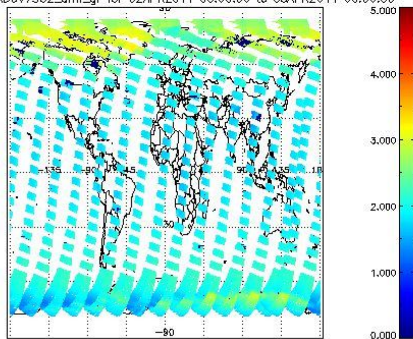
SCIOL2P_NADUV7S02_amf_gr for 02APR2011 00:00:00 to 03APR2011 00:00:00
