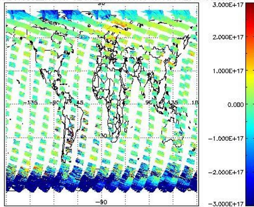
SCIOL2P_NADUV5S02_vcd for 02APR2011 00:00:00 to 03APR2011 00:00:00
