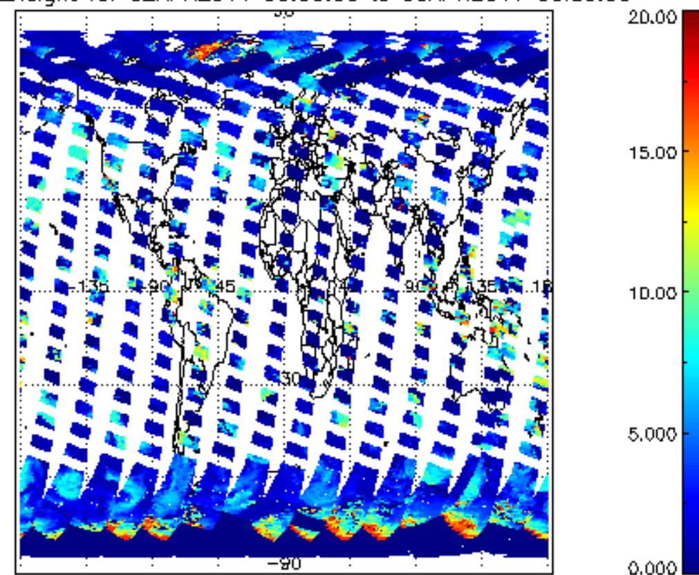
cl_top_height for 02APR2011 00:00:00 to 03APR2011 00:00:00
