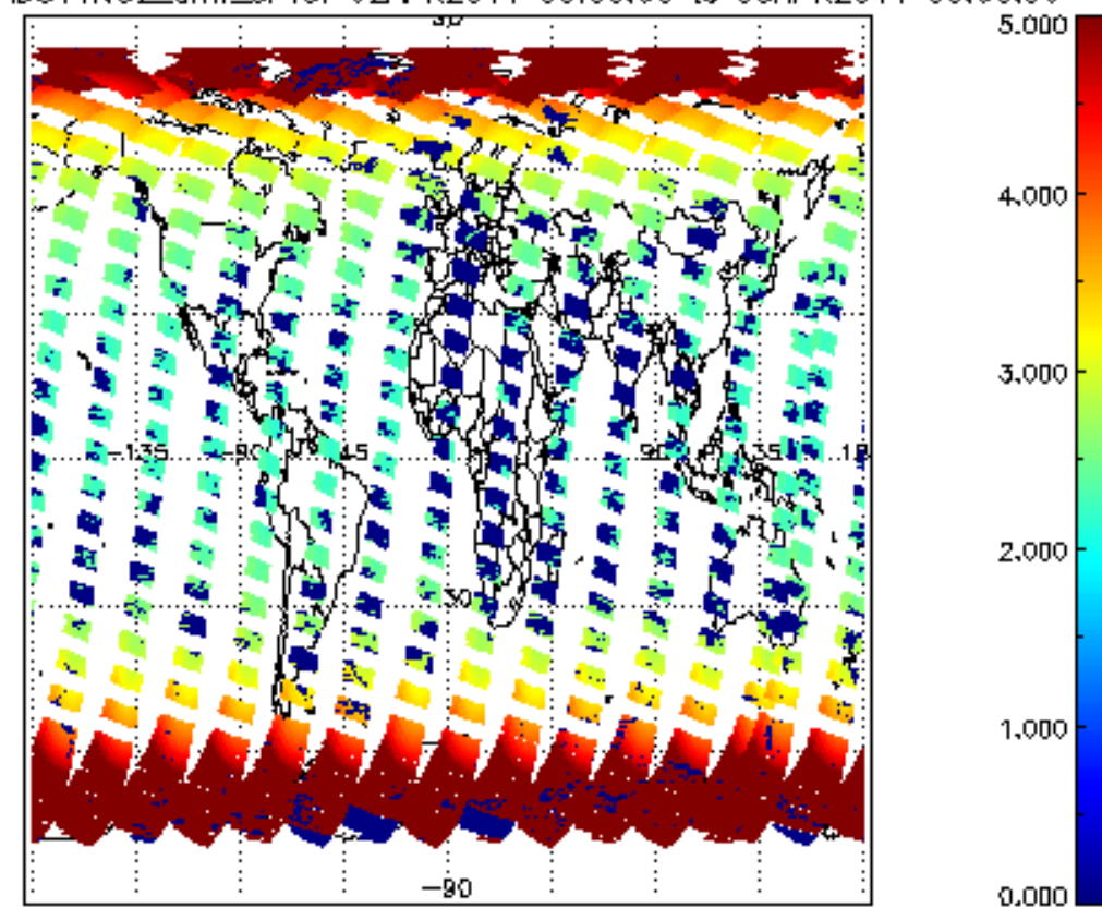
SCIOL2P_NADUV1NO2_amf_sl for 02APR2011 00:00:00 to 03APR2011 00:00:00
