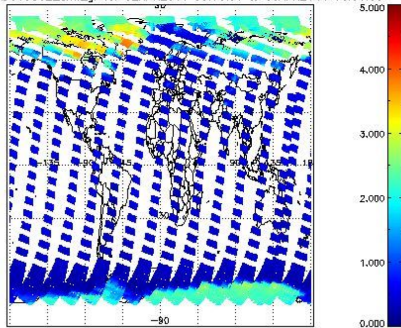
SCIOL2P_NADUV5S02_amf_gr for 02APR2011 00:00:00 to 03APR2011 00:00:00
