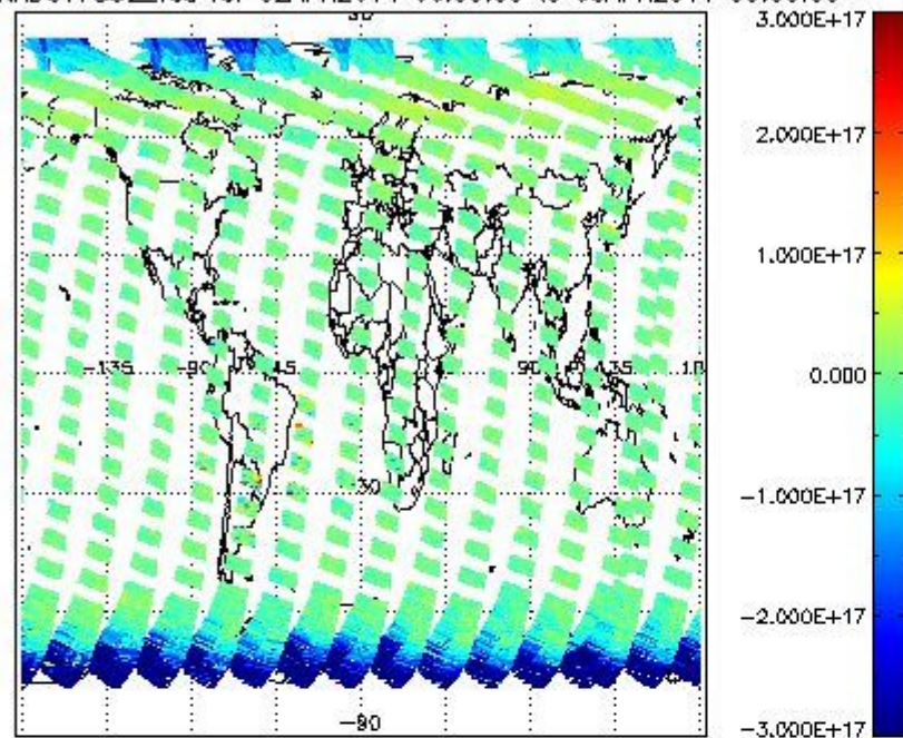
SCIOL2P_NADUV7S02_vcd for 02APR2011 00:00:00 to 03APR2011 00:00:00
