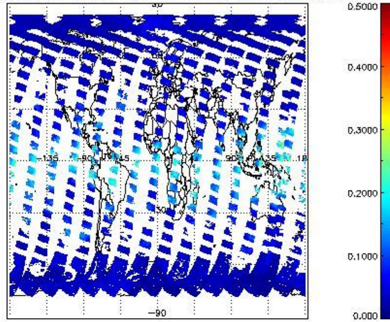
SCIOL2P_NADUV8H2O_vcd_err for 02APR2011 00:00:00 to 03APR2011 00:00:00
