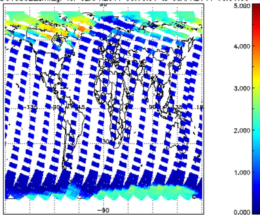
SCIOL2P_NADUV5S02_amf_gr for 02APR2011 00:00:00 to 03APR2011 00:00:00
