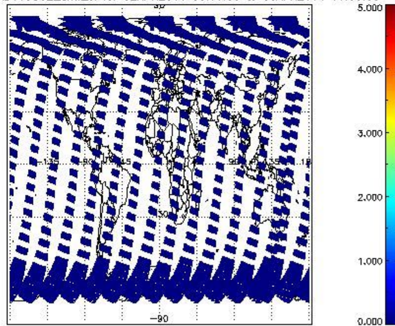
SCIOL2P_NADUV5S02_amf_cl for 02APR2011 00:00:00 to 03APR2011 00:00:00
