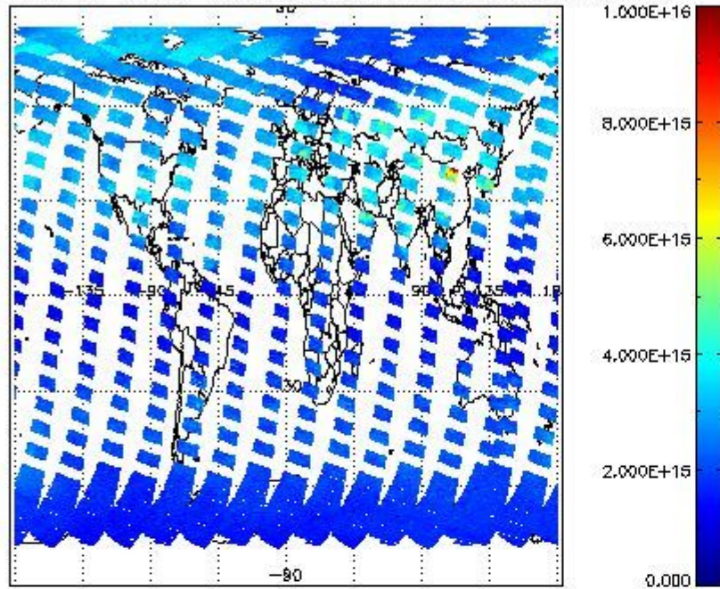
SCIOL2P_NADUV1NO2_vcd for 02APR2011 00:00:00 to 03APR2011 00:00:00
