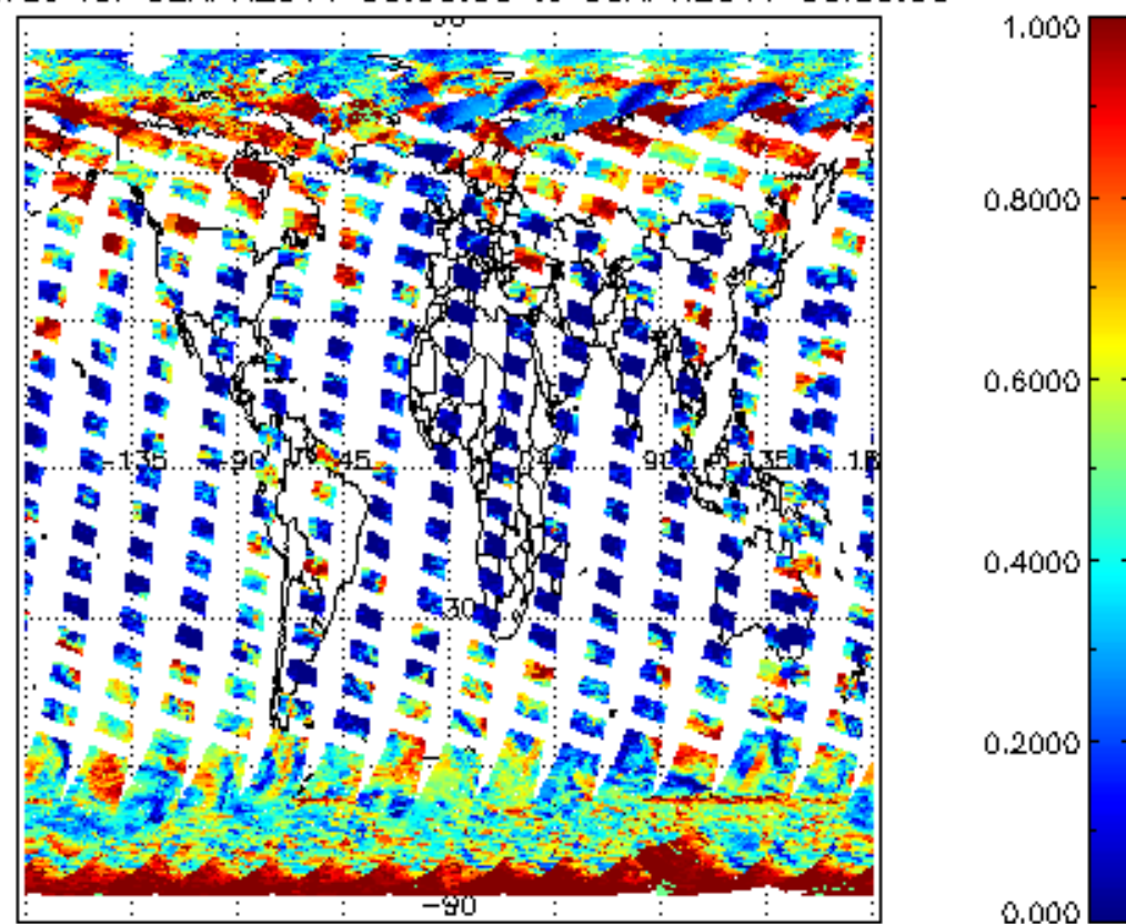
cl_frac for 02APR2011 00:00:00 to 03APR2011 00:00:00
