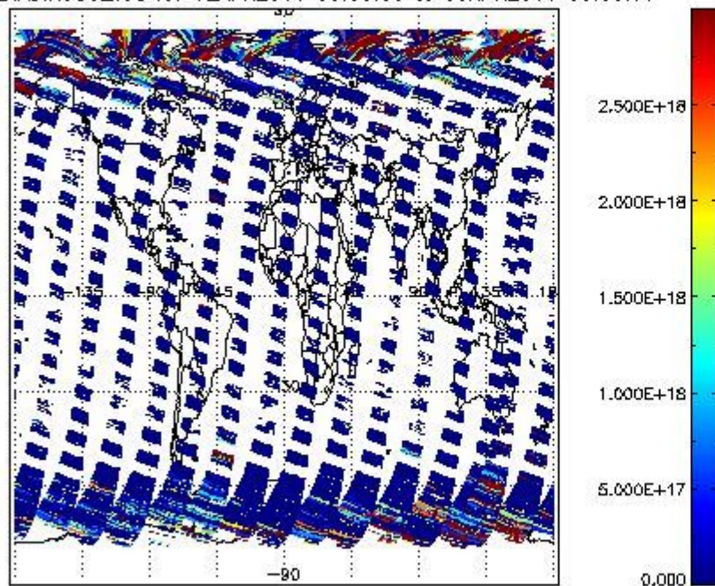
SCIDL2P_NADIR3CO_vcd for 02APR2011 00:00:00 to 03APR2011 00:00:00
