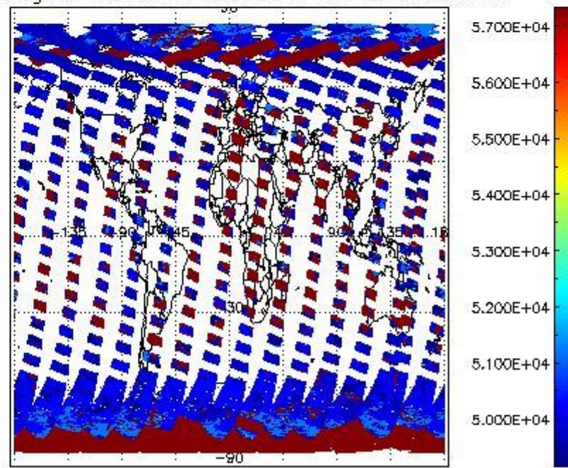
cloud_flags for 02APR2011 00:00:00 to 03APR2011 00:00:00
