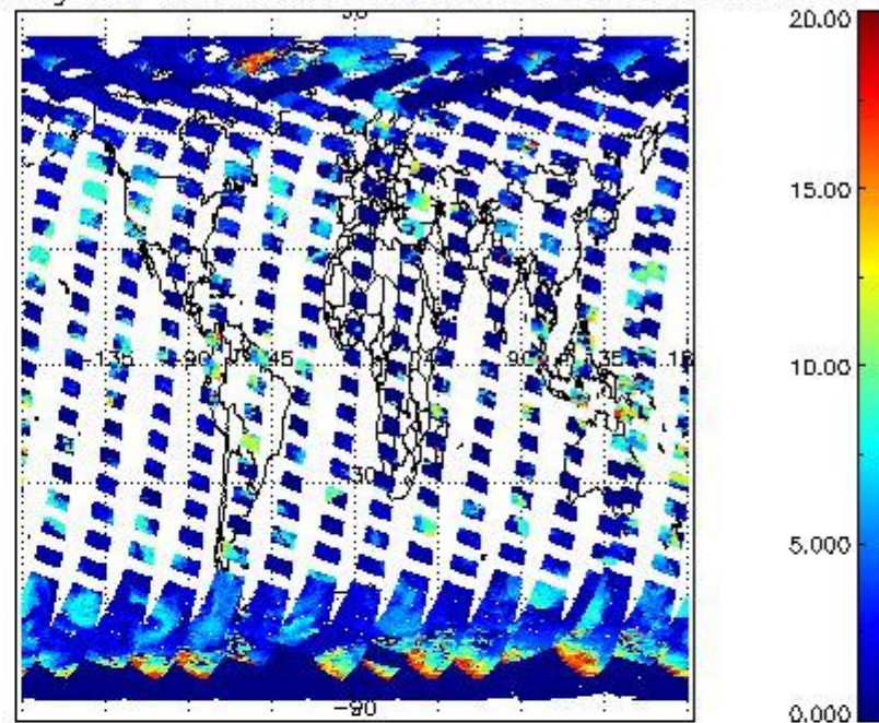
cL_top_height for 02APR2011 00:00:00 to 03APR2011 00:00:00
