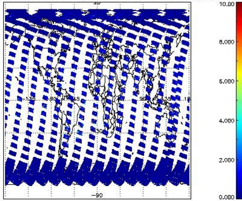
SCIOL2P_NADUV3BRO_vcd_err for 02APR2011 00:00:00 to 03APR2011 00:00:00
