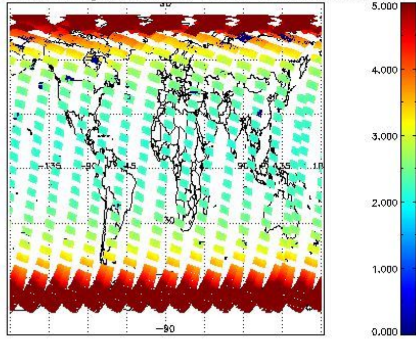
SCIOL2P_NADUV3BRO_amf_gr for 02APR2011 00:00:00 to 03APR2011 00:00:00
