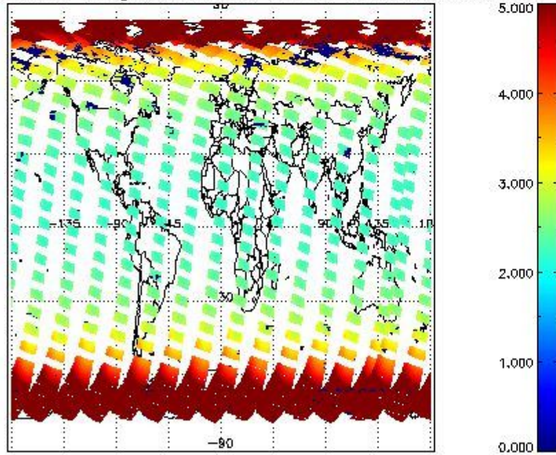
SCIOL2P_NADUV1NO2_amf_gr for 02APR2011 00:00:00 to 03APR2011 00:00:00
