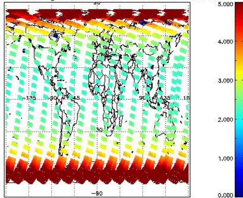
SCIOL2P_NADUV003_amf_gr for 02APR2011 00:00:00 to 03APR2011 00:00:00
