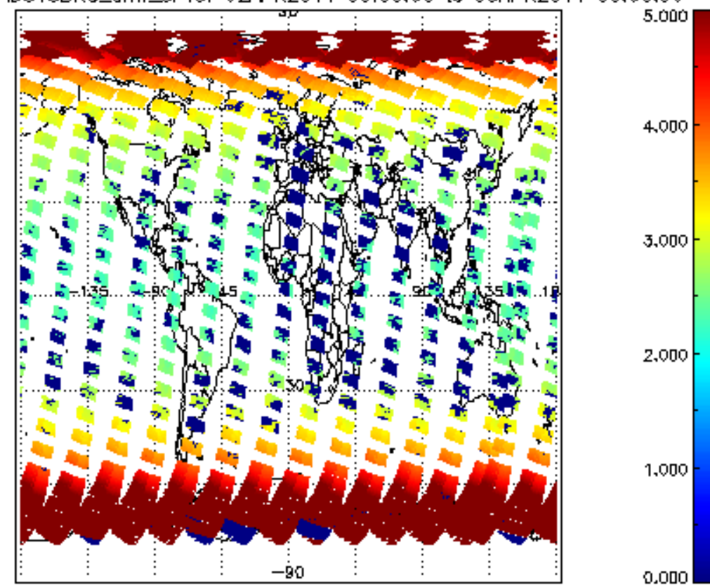
SCIOL2P_NADUV3BRO_amf_sl for 02APR2011 00:00:00 to 03APR2011 00:00:00
