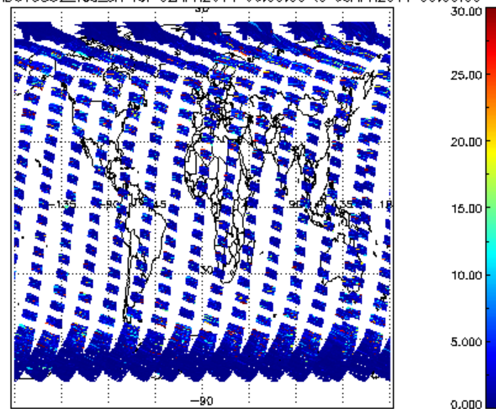
SCIOL2P_NADUV5S02_vcd_err for 02APR2011 00:00:00 to 03APR2011 00:00:00
