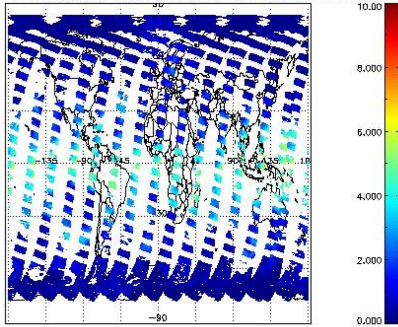
SCIOL2P_NADUV8H2O_vcd for 02APR2011 00:00:00 to 03APR2011 00:00:00
