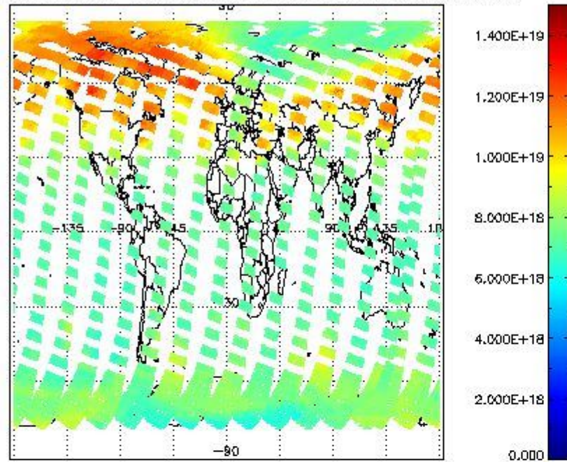
SCIOL2P_NADUV003_vcd for 02APR2011 00:00:00 to 03APR2011 00:00:00
