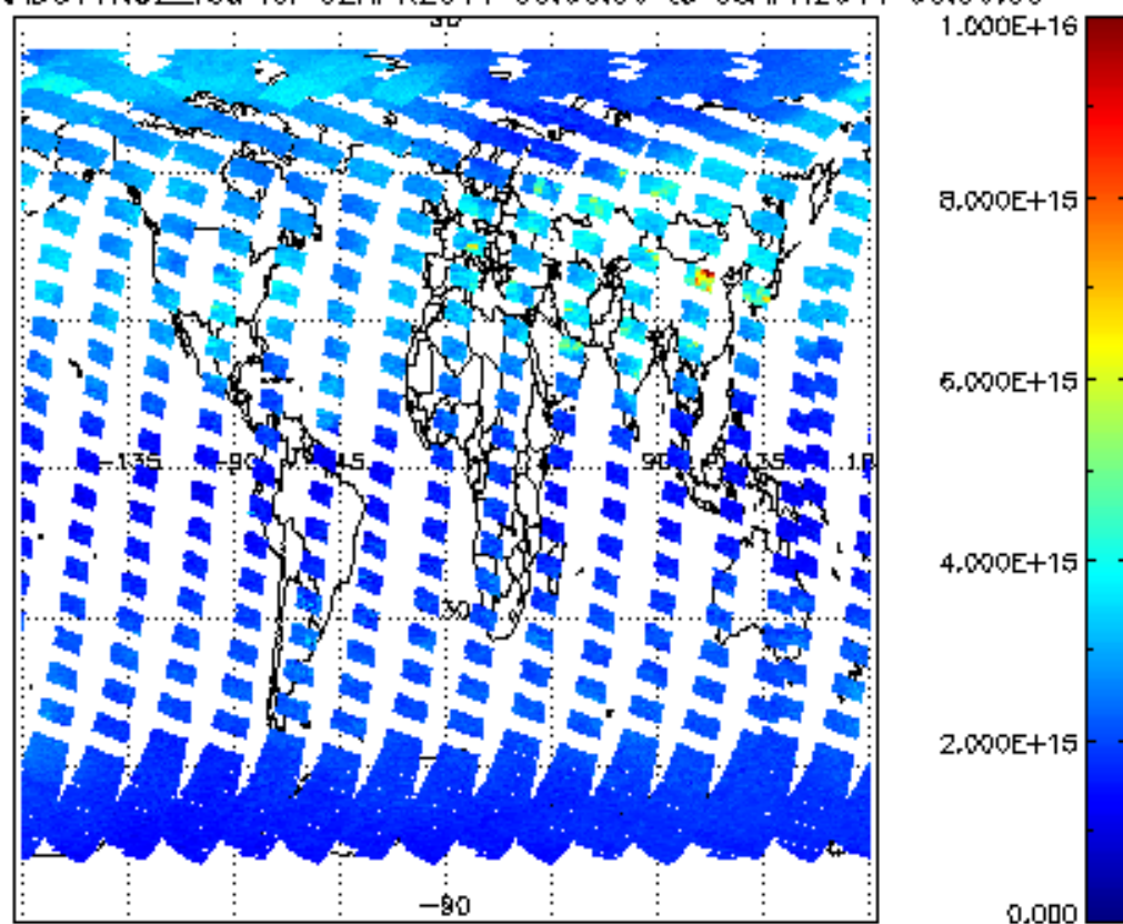
SCIOL2P_NADUV1NO2_vcd for 02APR2011 00:00:00 to 03APR2011 00:00:00
