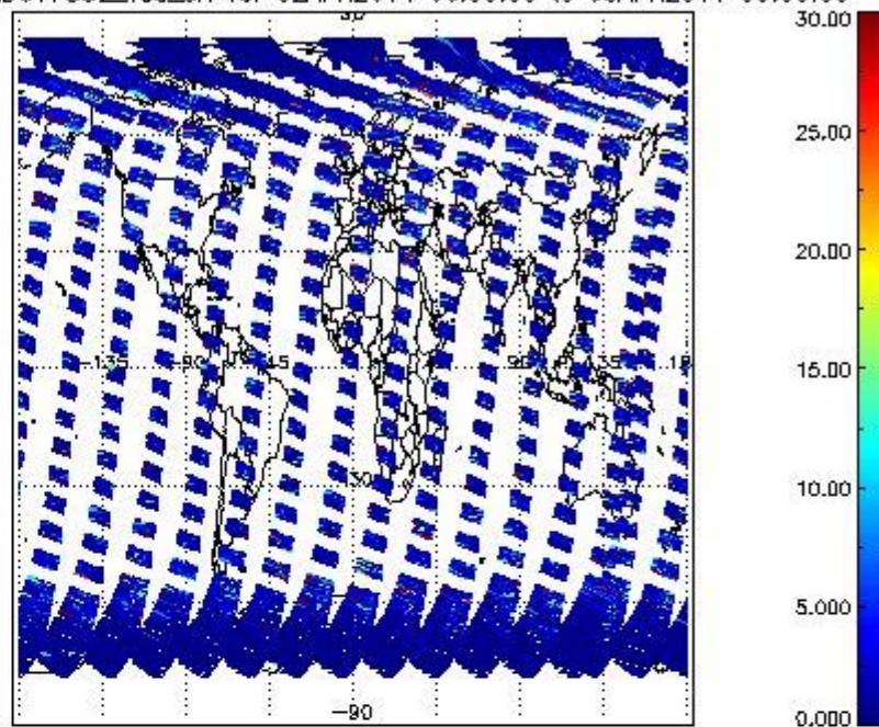
SCIOL2P_NADUV7S02_vcd_err for 02APR2011 00:00:00 to 03APR2011 00:00:00
