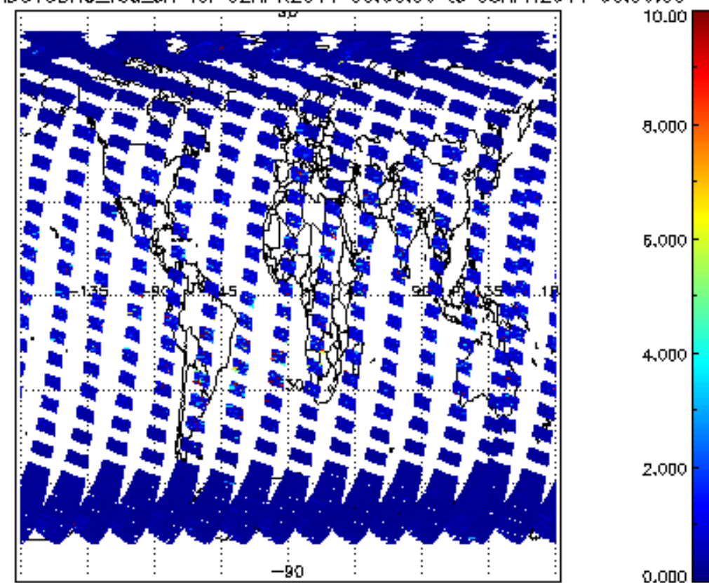
SCIOL2P_NADUV3BRO_vcd_err for 02APR2011 00:00:00 to 03APR2011 00:00:00
