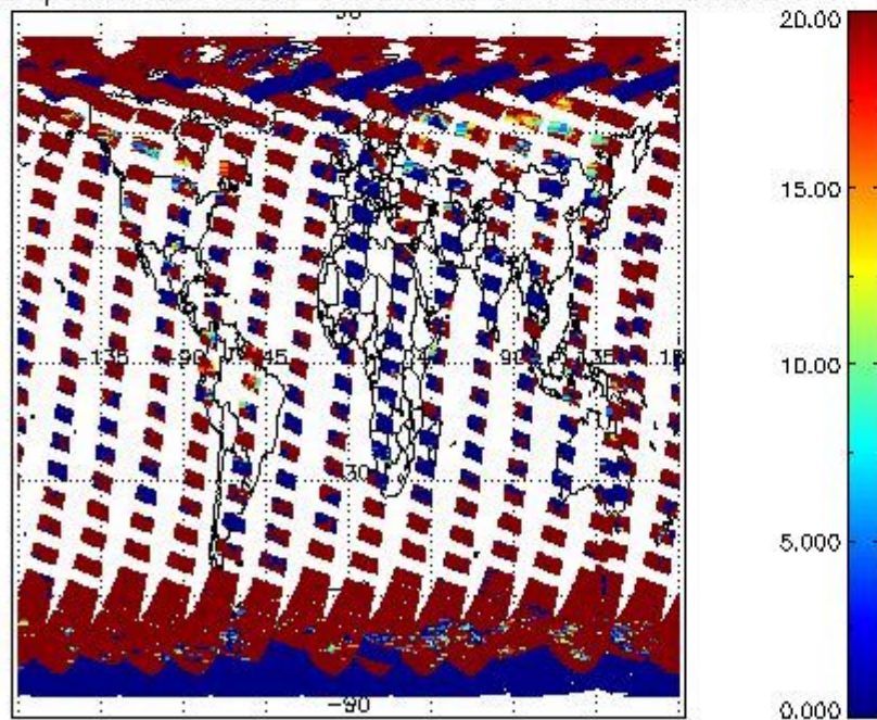
cL_opt_depth for 02APR2011 00:00:00 to 03APR2011 00:00:00
