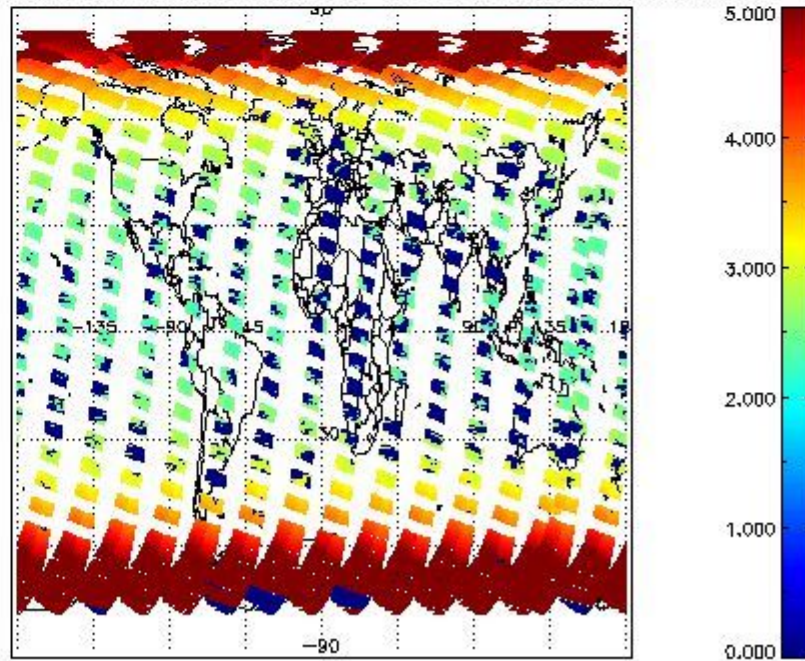
SCIOL2P_NADUV003_amf_cl for 02APR2011 00:00:00 to 03APR2011 00:00:00
