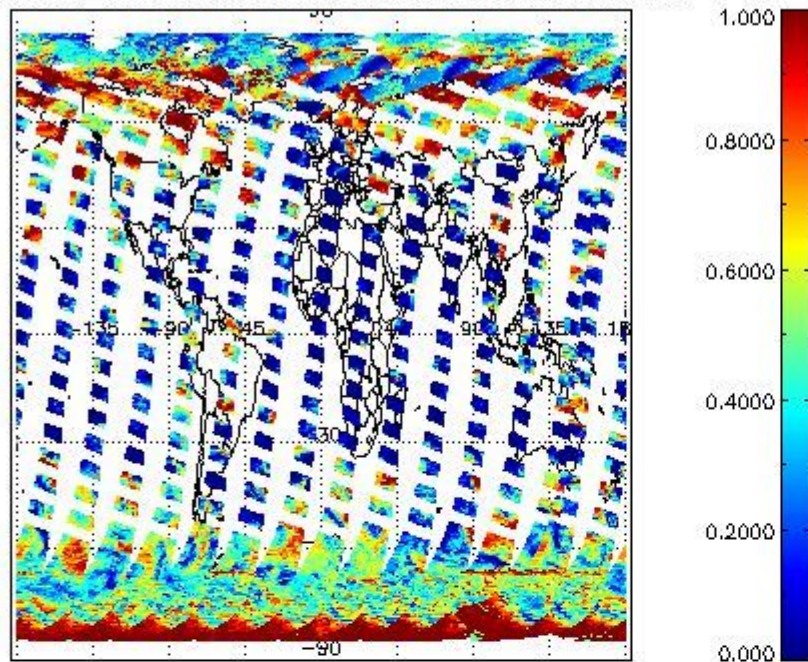
cL_frac for 02APR2011 00:00:00 to 03APR2011 00:00:00
