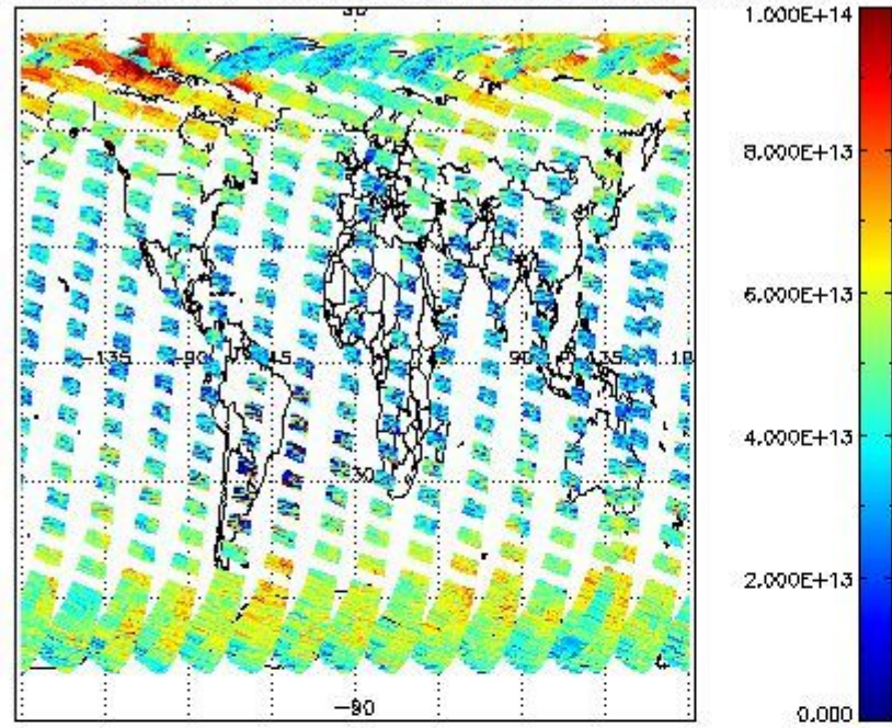
SCIOL2P_NADUV3BRO_vcd for 02APR2011 00:00:00 to 03APR2011 00:00:00
