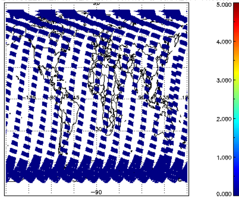
SCIOL2P_NADUV7S02_amf_cl for 02APR2011 00:00:00 to 03APR2011 00:00:00
