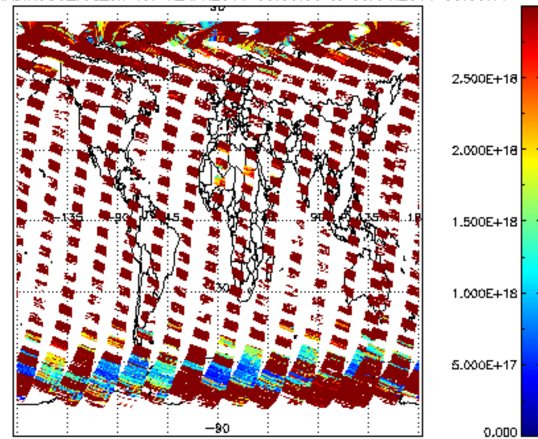
SCIOL2P_NADIR3CO_vcd_err for 02APR2011 00:00:00 to 03APR2011 00:00:00
