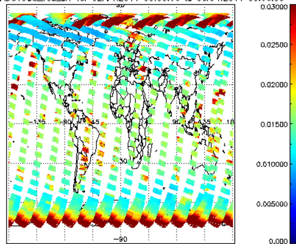
SCIOL2P_NADUV003_vcd_err for 02APR2011 00:00:00 to 03APR2011 00:00:00
