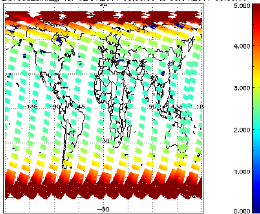
SCIOL2P_NADUV003_amf_gr for 02APR2011 00:00:00 to 03APR2011 00:00:00
