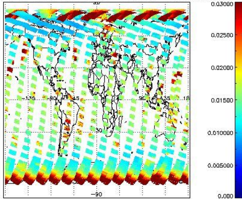
SCIOL2P_NADUV003_vcd_err for 02APR2011 00:00:00 to 03APR2011 00:00:00
