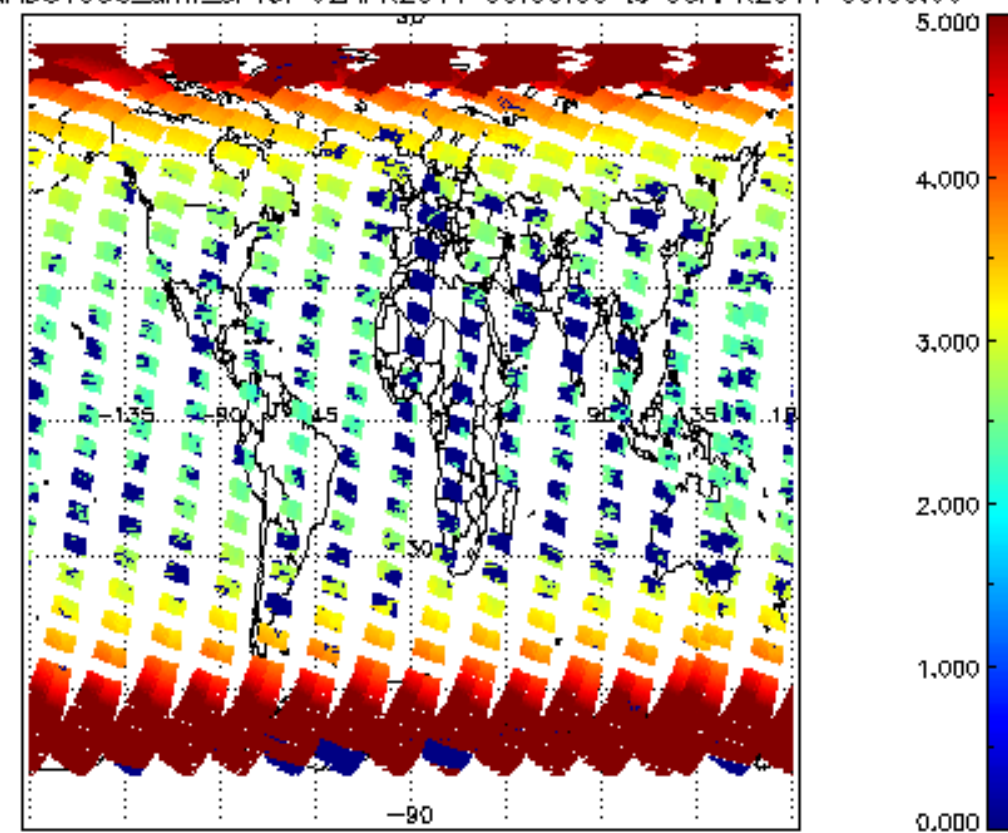
SCIOL2P_NADUV003_amf_cl for 02APR2011 00:00:00 to 03APR2011 00:00:00
