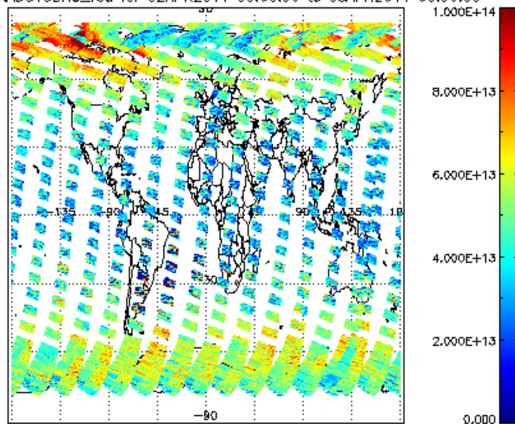
SCIOL2P_NADUV3BRO_vcd for 02APR2011 00:00:00 to 03APR2011 00:00:00
