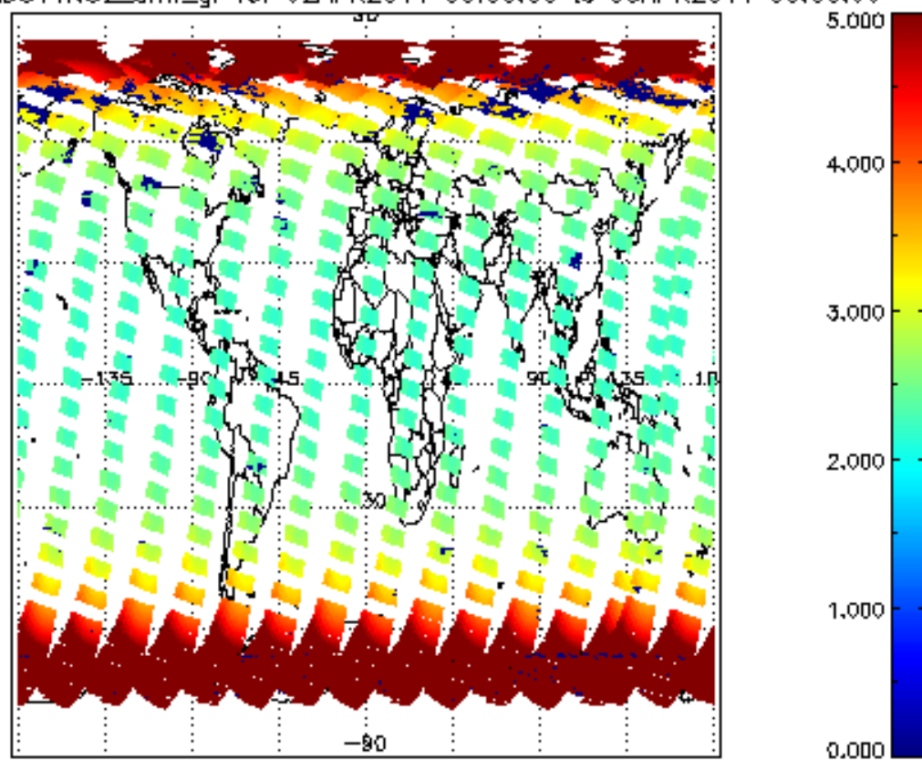
SCIOL2P_NADUV1NO2_amf_gr for 02APR2011 00:00:00 to 03APR2011 00:00:00
