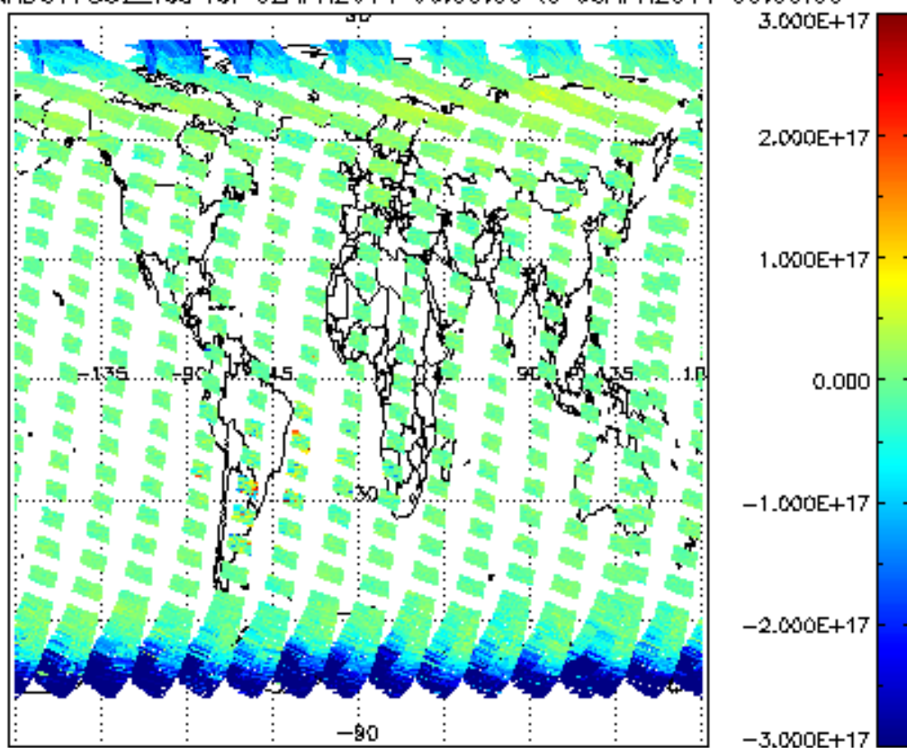
SCIOL2P_NADUV7S02_vcd for 02APR2011 00:00:00 to 03APR2011 00:00:00
