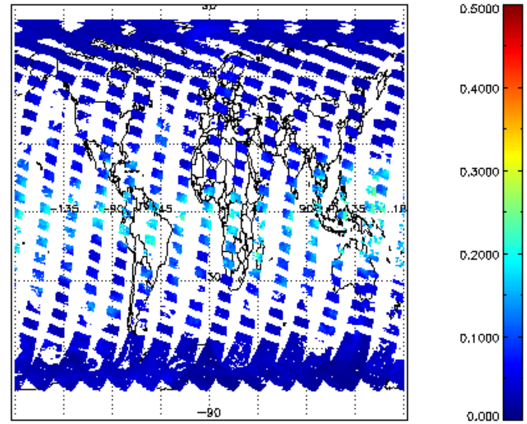
SCIOL2P_NADUV8H2O_vcd_err for 02APR2011 00:00:00 to 03APR2011 00:00:00
