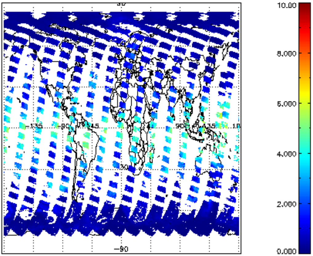
SCIOL2P_NADUV8H2O_vcd for 02APR2011 00:00:00 to 03APR2011 00:00:00
