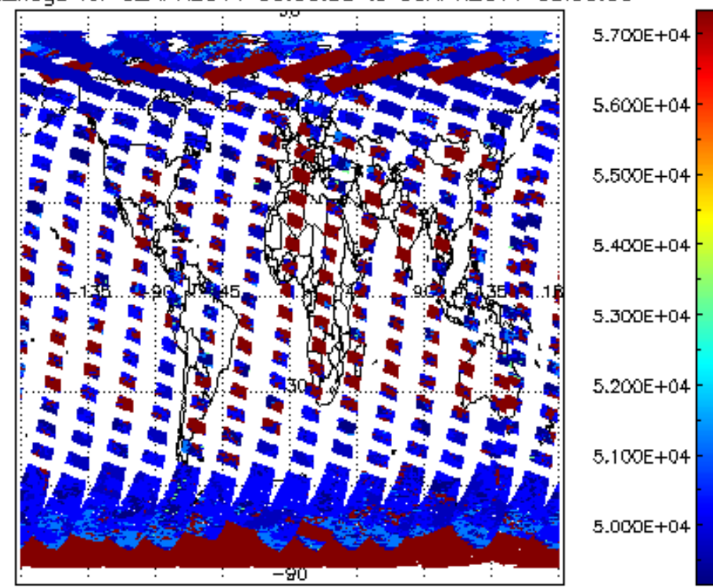
cloud_flags for 02APR2011 00:00:00 to 03APR2011 00:00:00
