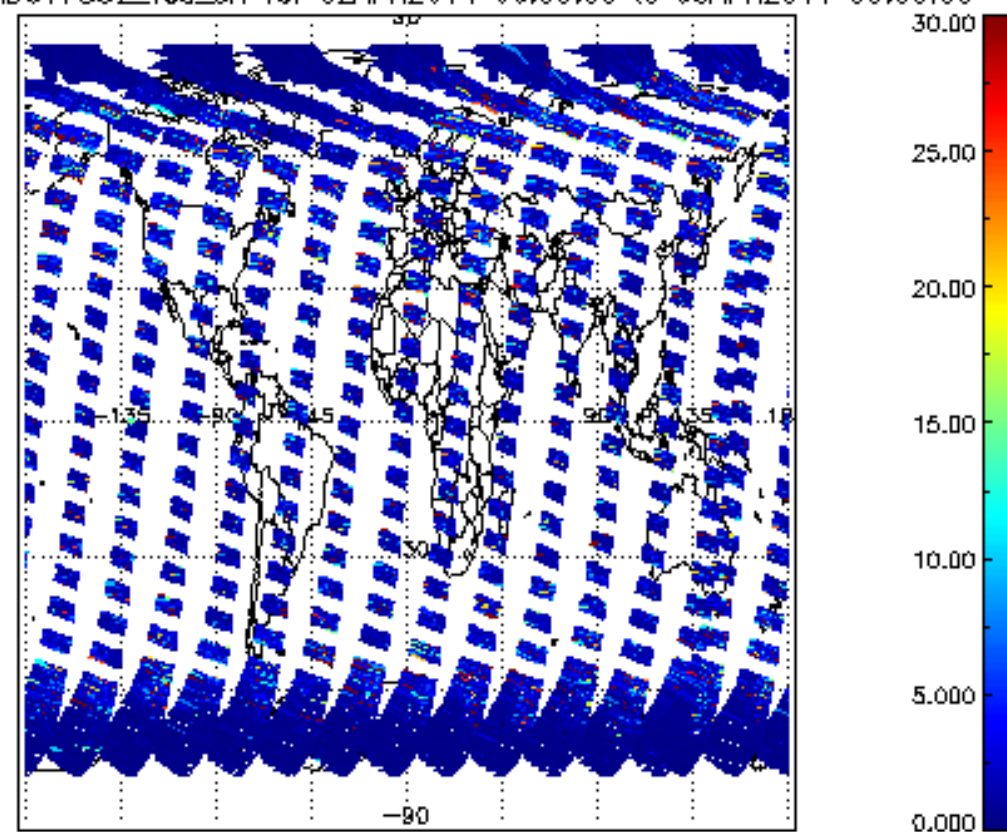
SCIOL2P_NADUV7S02_vcd_err for 02APR2011 00:00:00 to 03APR2011 00:00:00
