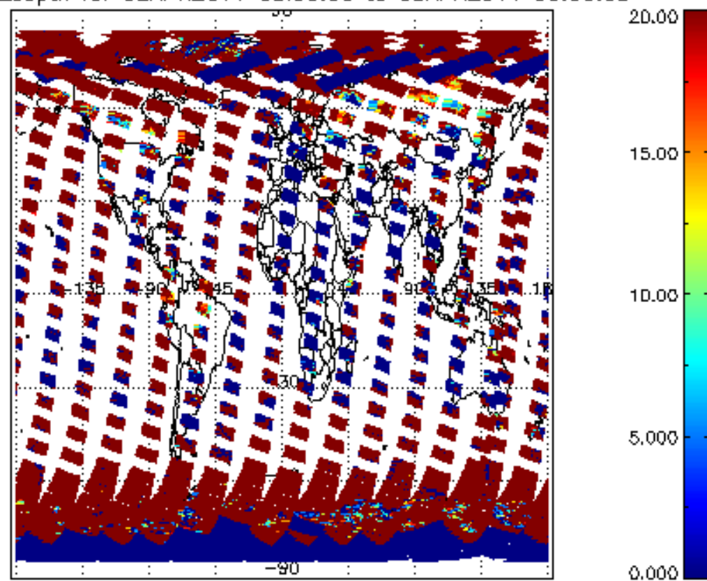
cl_opt_depth for 02APR2011 00:00:00 to 03APR2011 00:00:00
