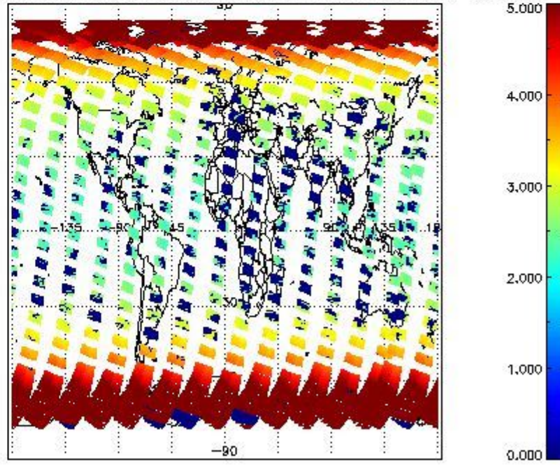
SCIOL2P_NADUV3BRO_amf_cl for 02APR2011 00:00:00 to 03APR2011 00:00:00
