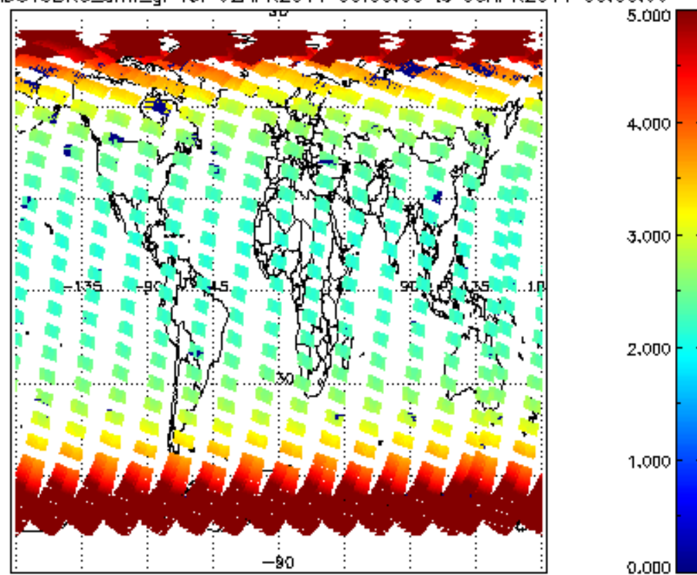
SCIOL2P_NADUV3BRO_amf_gr for 02APR2011 00:00:00 to 03APR2011 00:00:00
