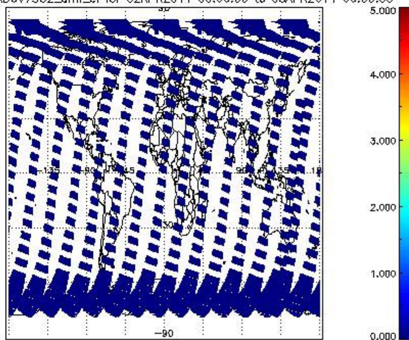
SCIOL2P_NADUV7S02_amf_cl for 02APR2011 00:00:00 to 03APR2011 00:00:00
