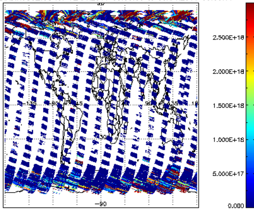
SCIOL2P_NADIR3CO_vcd for 02APR2011 00:00:00 to 03APR2011 00:00:00
