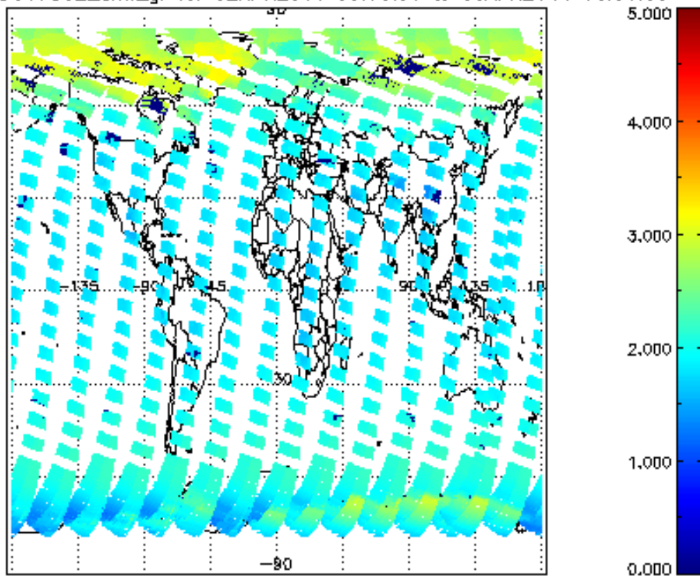
SCIOL2P_NADUV7S02_amf_gr for 02APR2011 00:00:00 to 03APR2011 00:00:00
