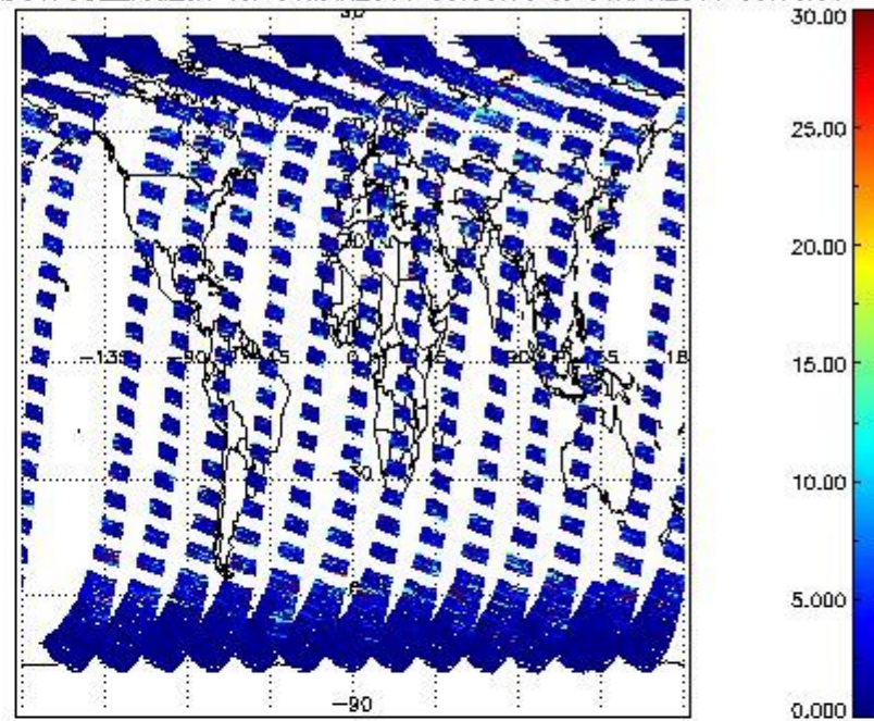
SCIOL2P_NADUV7S02_vcd_err for 31MAR2011 00:00:00 to 01APR2011 00:00:00
