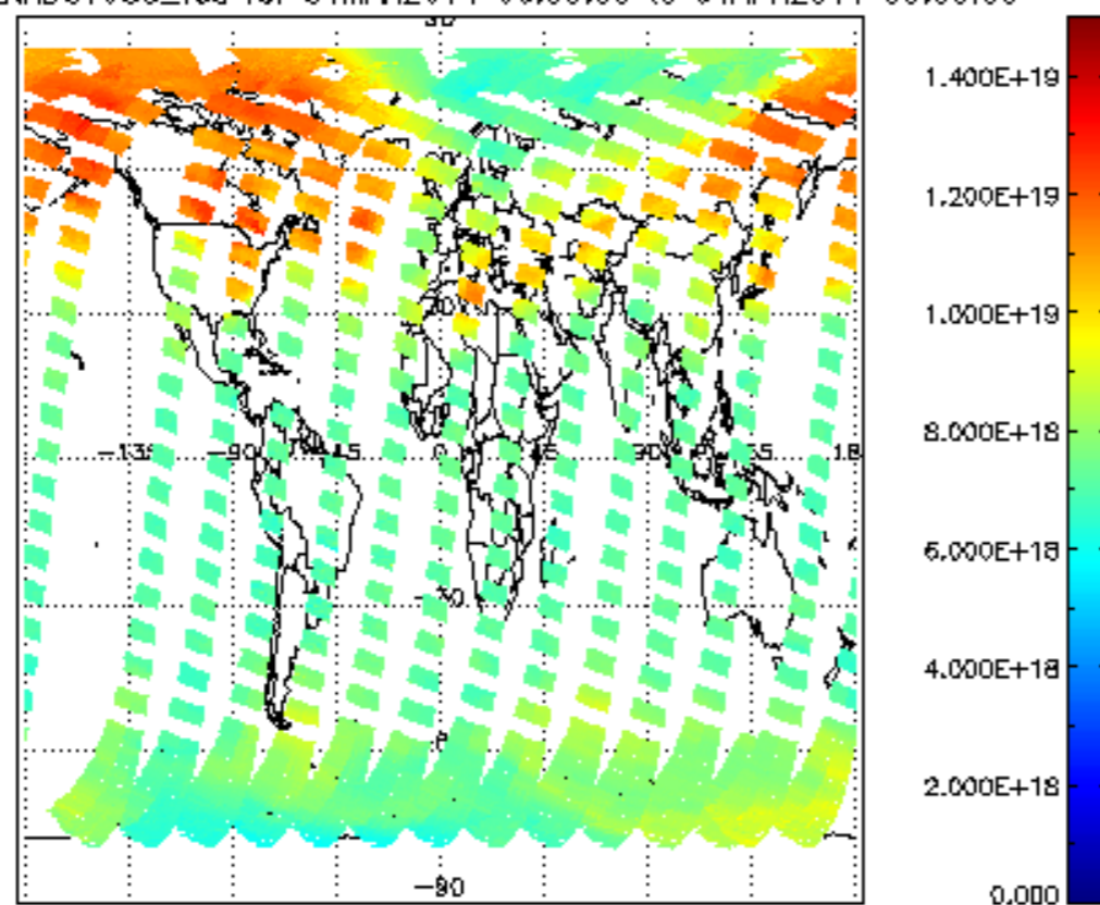
SCIOL2P_NADUV003_vcd for 31MAR2011 00:00:00 to 01APR2011 00:00:00
