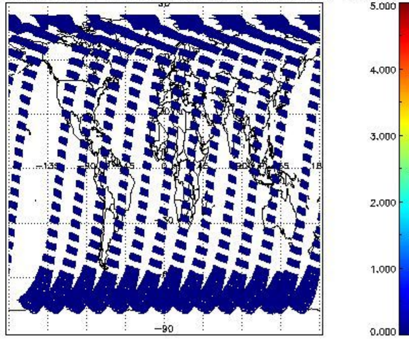
SCIOL2P_NADUV5SO2_amf_cl for 31MAR2011 00:00:00 to 01APR2011 00:00:00
