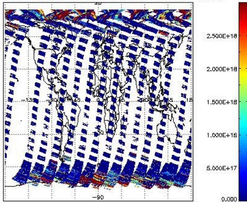
SCIDL2P_NADIR3CO_vcd for 31MAR2011 00:00:00 to 01APR2011 00:00:00
