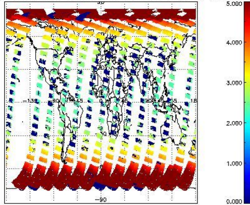
SCIOL2P_NADUV3BRO_amf_cl for 31MAR2011 00:00:00 to 01APR2011 00:00:00
