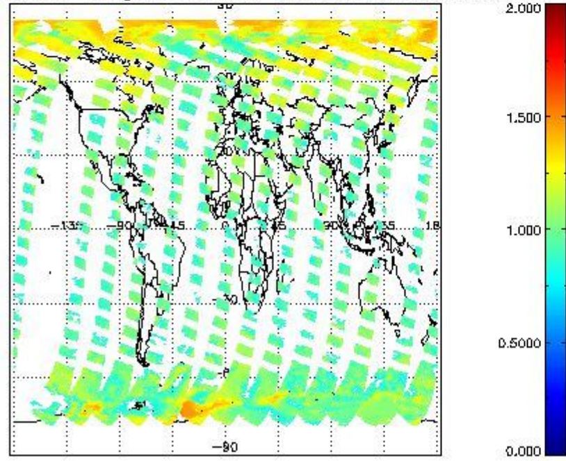
SCIOL2P_NADUV8H20_amf_gr for 31MAR2011 00:00:00 to 01APR2011 00:00:00
