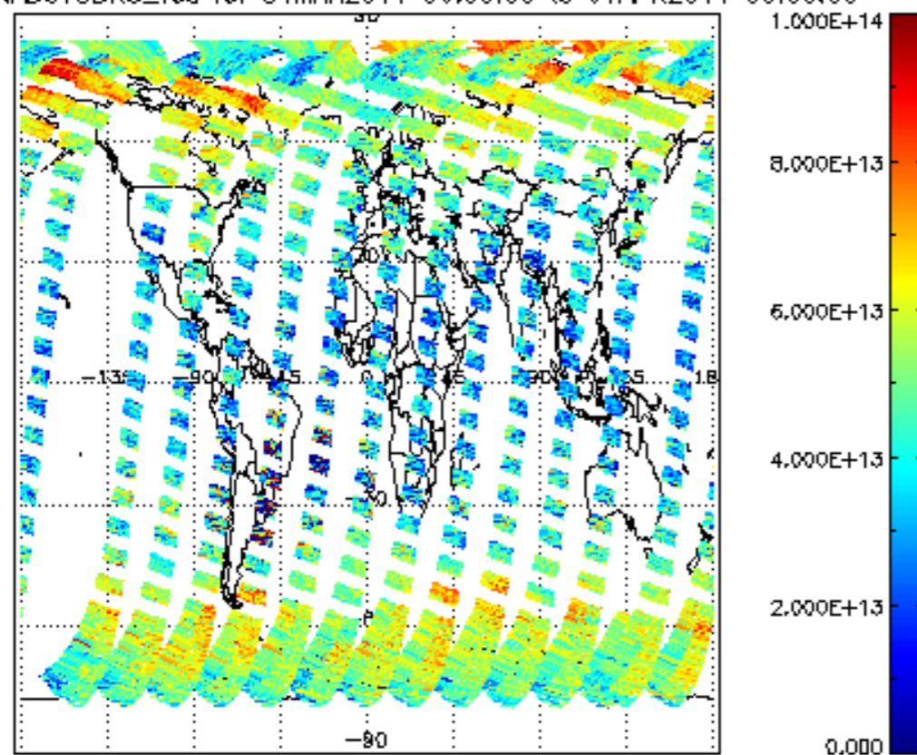
SCIOL2P_NADUV3BRO_vcd for 31MAR2011 00:00:00 to 01APR2011 00:00:00
