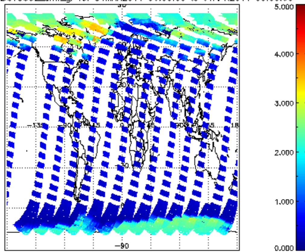
SCIOL2P_NADUV5S02_amf_gr for 31MAR2011 00:00:00 to 01APR2011 00:00:00
