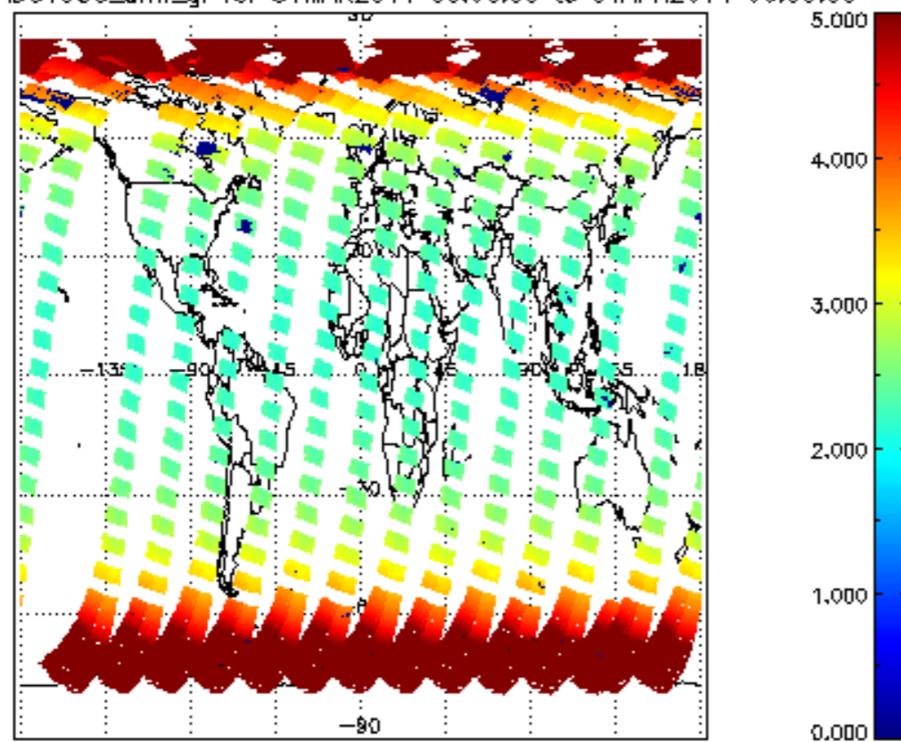
SCIOL2P_NADUV003_amf_gr for 31MAR2011 00:00:00 to 01APR2011 00:00:00
