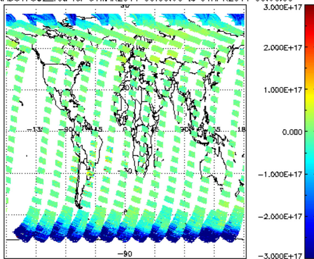
SCIOL2P_NADUV7S02_vcd for 31MAR2011 00:00:00 to 01APR2011 00:00:00
