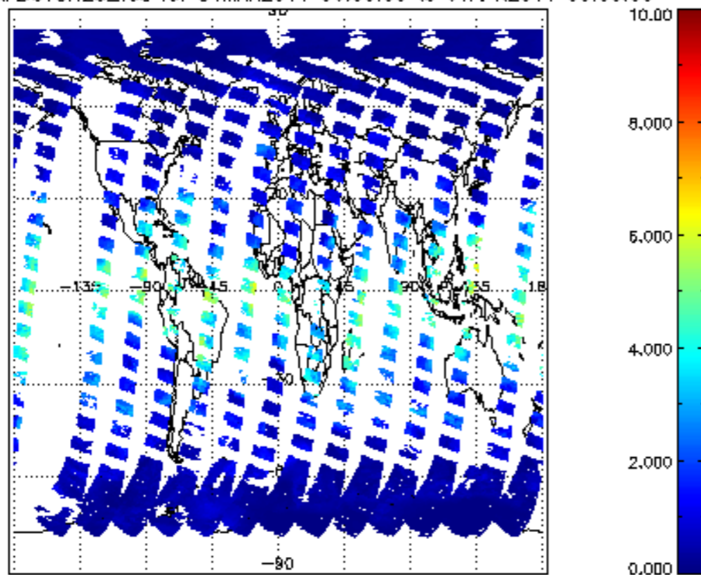
SCIOL2P_NADUV8H20_vcd for 31MAR2011 00:00:00 to 01APR2011 00:00:00
