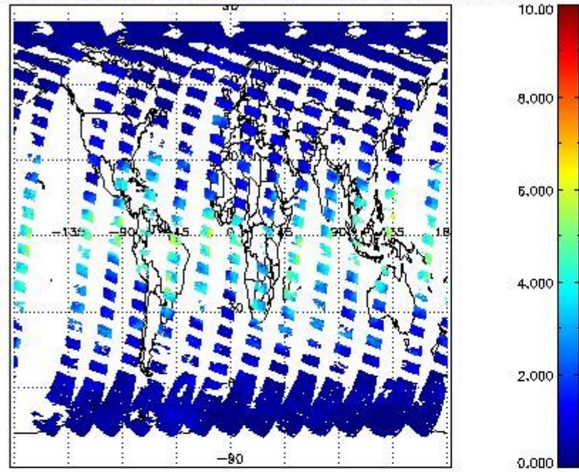
SCIOL2P_NADUVBH20_vcd for 31MAR2011 00:00:00 to 01APR2011 00:00:00
