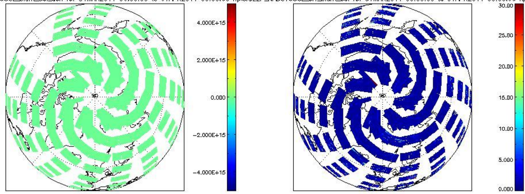
CIOL2P_NADUV60CL_slant_col_den for 31MAR2011 00:00:00 to 01APR2011 00:00:00 npCIOL2P_NADUV60CL_err_slant_col for 31MAR2011 00:00:00 to 01APR2011 00:00:00 np
