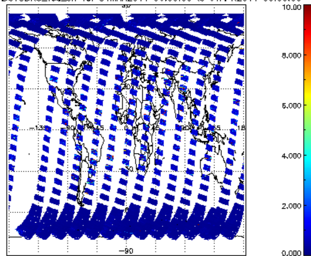
SCIOL2P_NADUV3BRO_vcd_err for 31MAR2011 00:00:00 to 01APR2011 00:00:00
