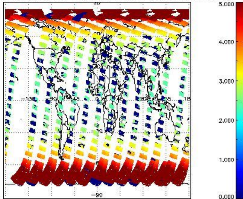
SCIOL2P_NADUV003_amf_cl for 31MAR2011 00:00:00 to 01APR2011 00:00:00
