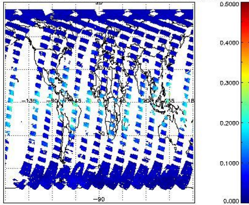
SCIOL2P_NADUVBH20_vcd_err for 31MAR2011 00:00:00 to 01APR2011 00:00:00
