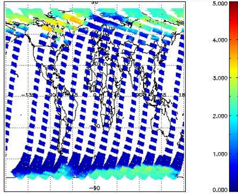
SCIOL2P_NADUV5SO2_amf_gr for 31MAR2011 00:00:00 to 01APR2011 00:00:00
