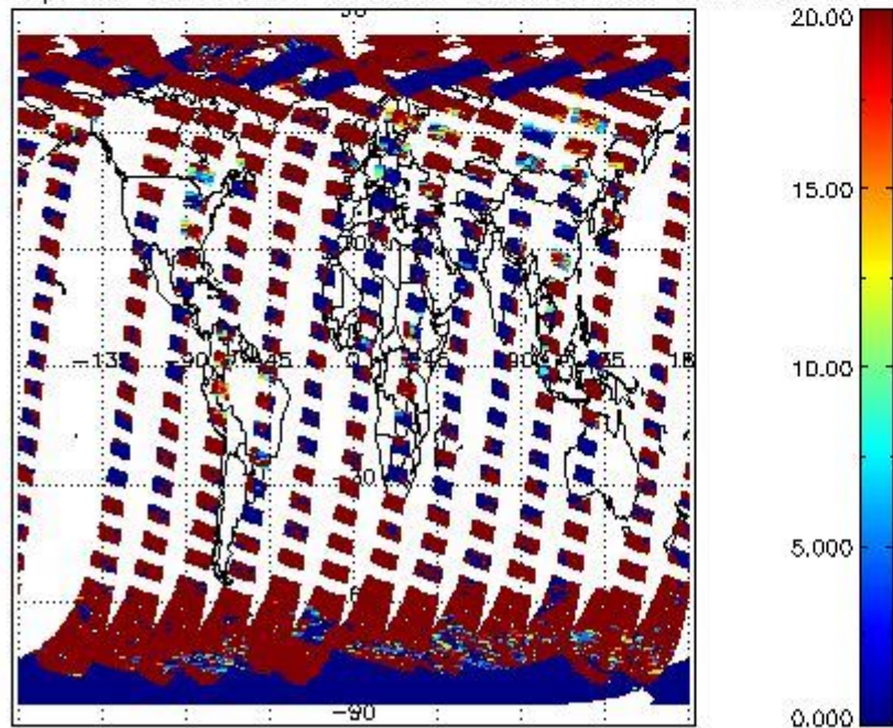
cLopt_depth for 31MAR2011 00:00:00 to 01APR2011 00:00:00
