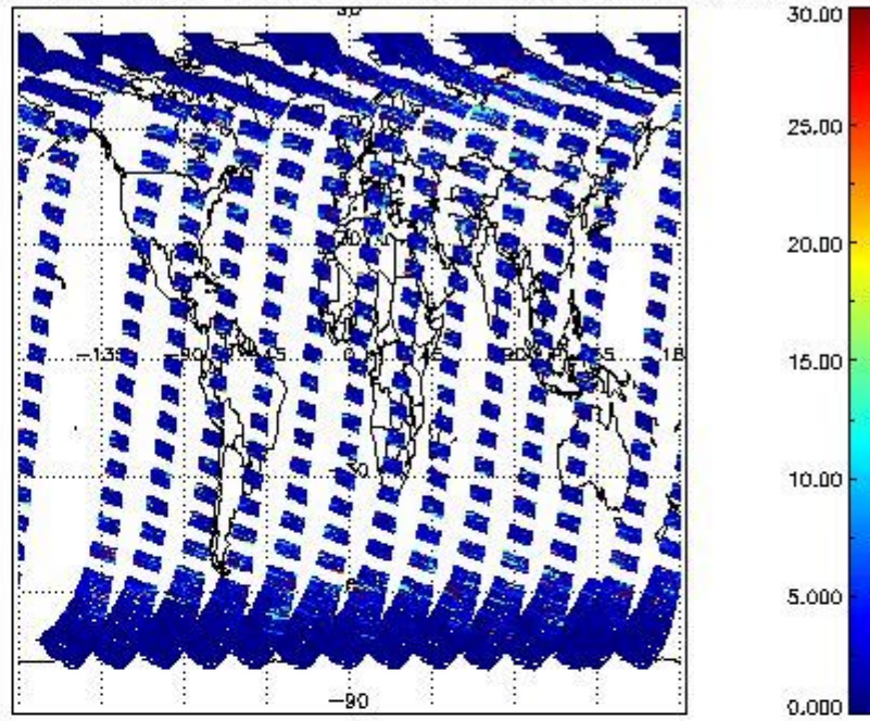
SCIOL2P_NADUV5SO2_vcd_err for 31MAR2011 00:00:00 to 01APR2011 00:00:00
