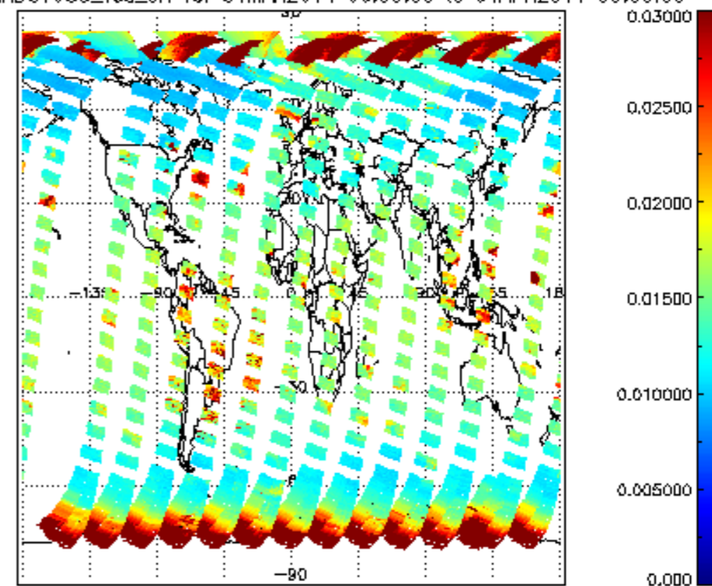
SCIOL2P_NADUV003_vcd_err for 31MAR2011 00:00:00 to 01APR2011 00:00:00
