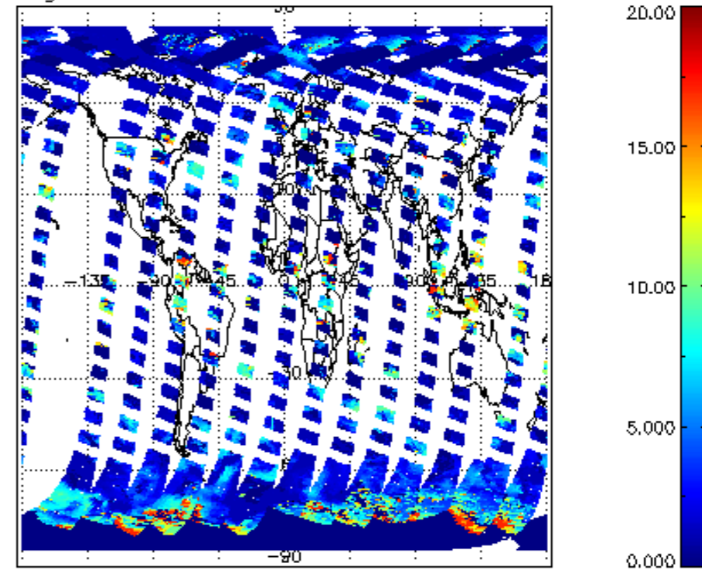
cL_top_height for 31MAR2011 00:00:00 to 01APR2011 00:00:00
