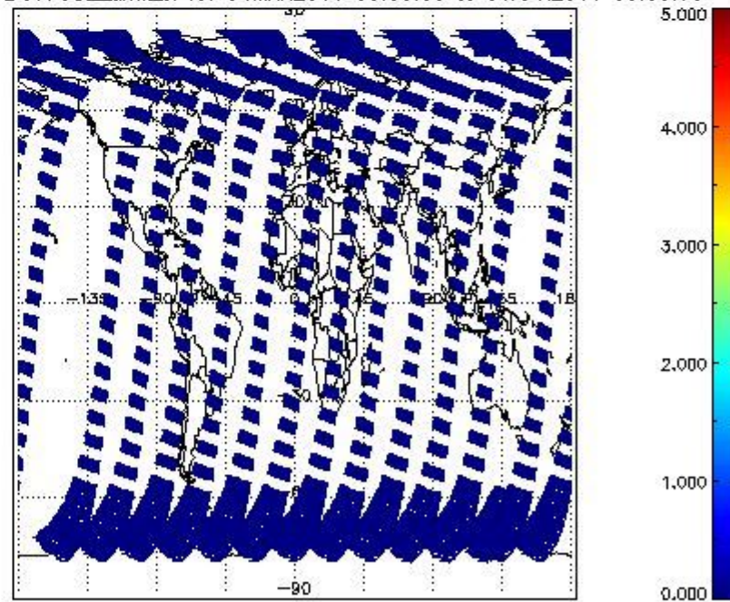
SCIOL2P_NADUV7S02_amf_cl for 31MAR2011 00:00:00 to 01APR2011 00:00:00
