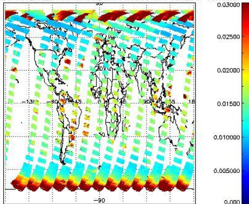
SCIOL2P_NADUV003_vcd_err for 31MAR2011 00:00:00 to 01APR2011 00:00:00
