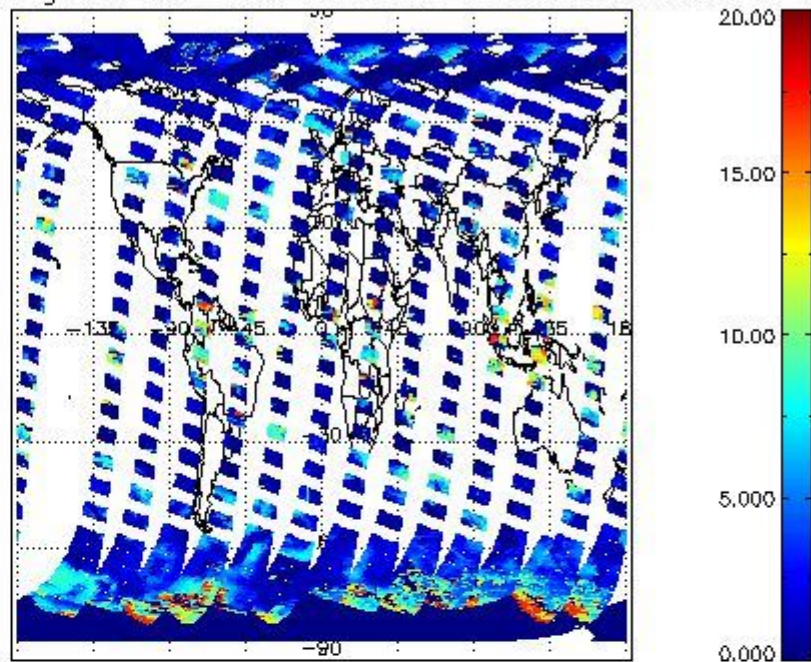
cL_top_height for 31MAR2011 00:00:00 to 01APR2011 00:00:00
