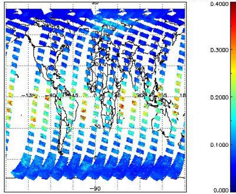
SCIOL2P_NADUV1NO2_vcd_err for 31MAR2011 00:00:00 to 01APR2011 00:00:00
