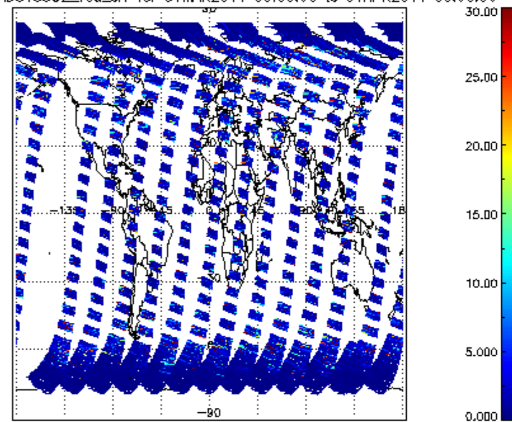
SCIOL2P_NADUV5S02_vcd_err for 31MAR2011 00:00:00 to 01APR2011 00:00:00
