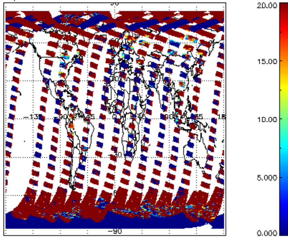
cL_opt_depth for 31MAR2011 00:00:00 to 01APR2011 00:00:00
