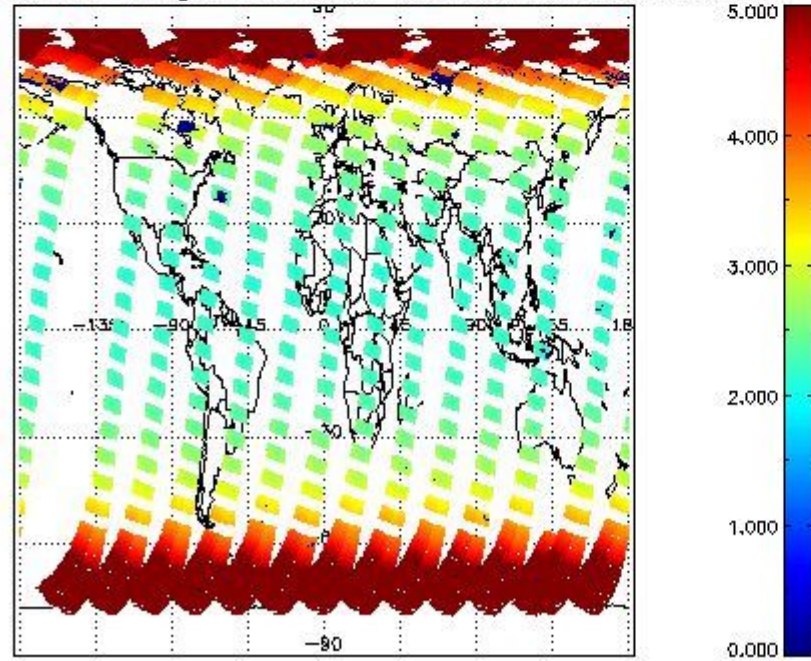
SCIOL2P_NADUV3BRO_amf_gr for 31MAR2011 00:00:00 to 01APR2011 00:00:00
