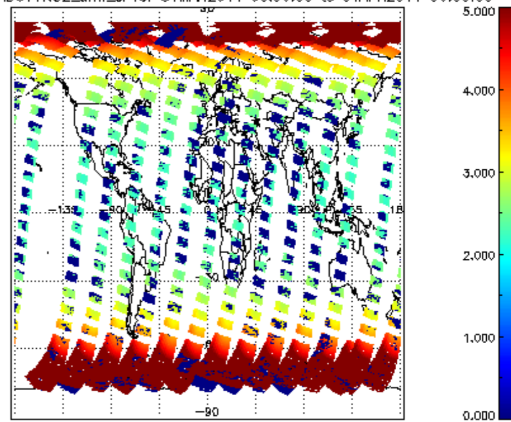
SCIOL2P_NADUV1NO2_amf_cl for 31MAR2011 00:00:00 to 01APR2011 00:00:00
