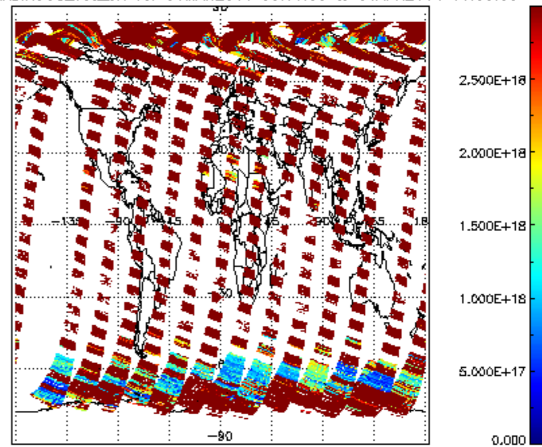
SCIOL2P_NADIR3CO_vcdLerr for 31MAR2011 00:00:00 to 01APR2011 00:00:00
