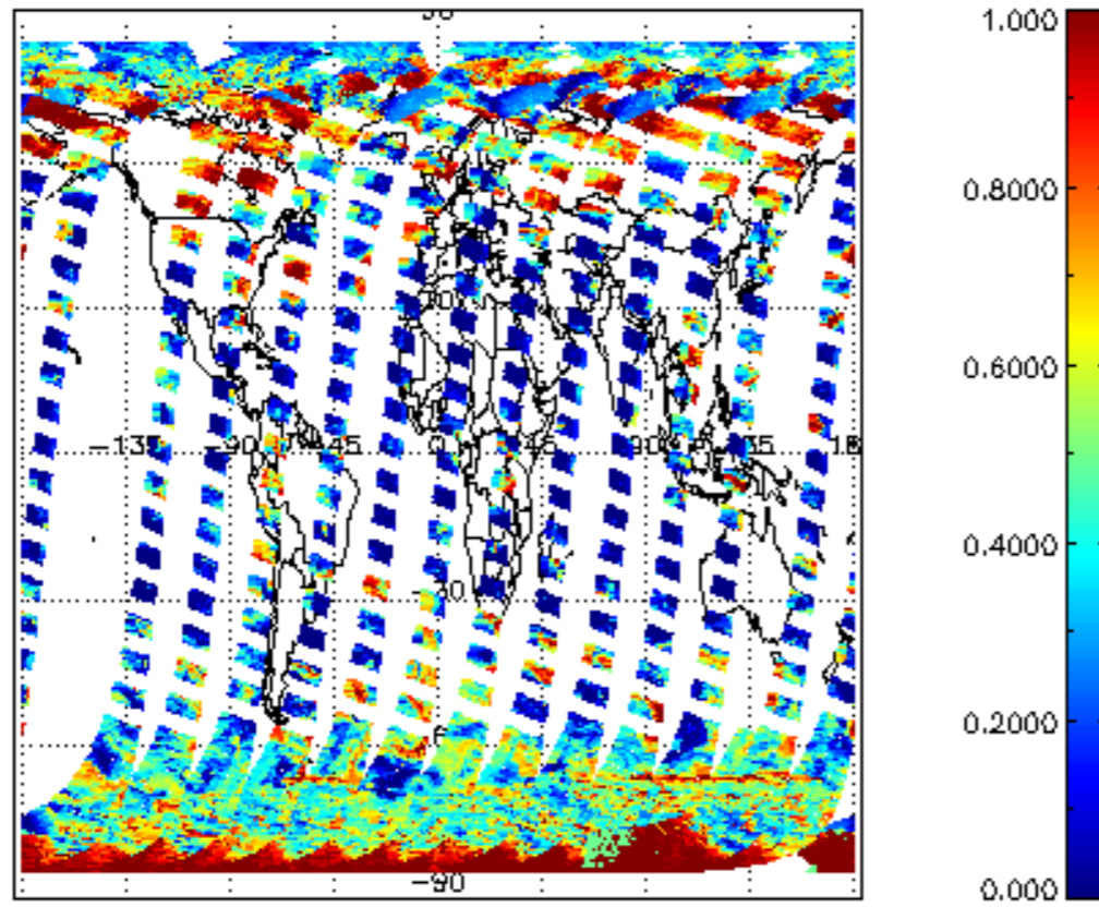
cL_frac for 31MAR2011 00:00:00 to 01APR2011 00:00:00
