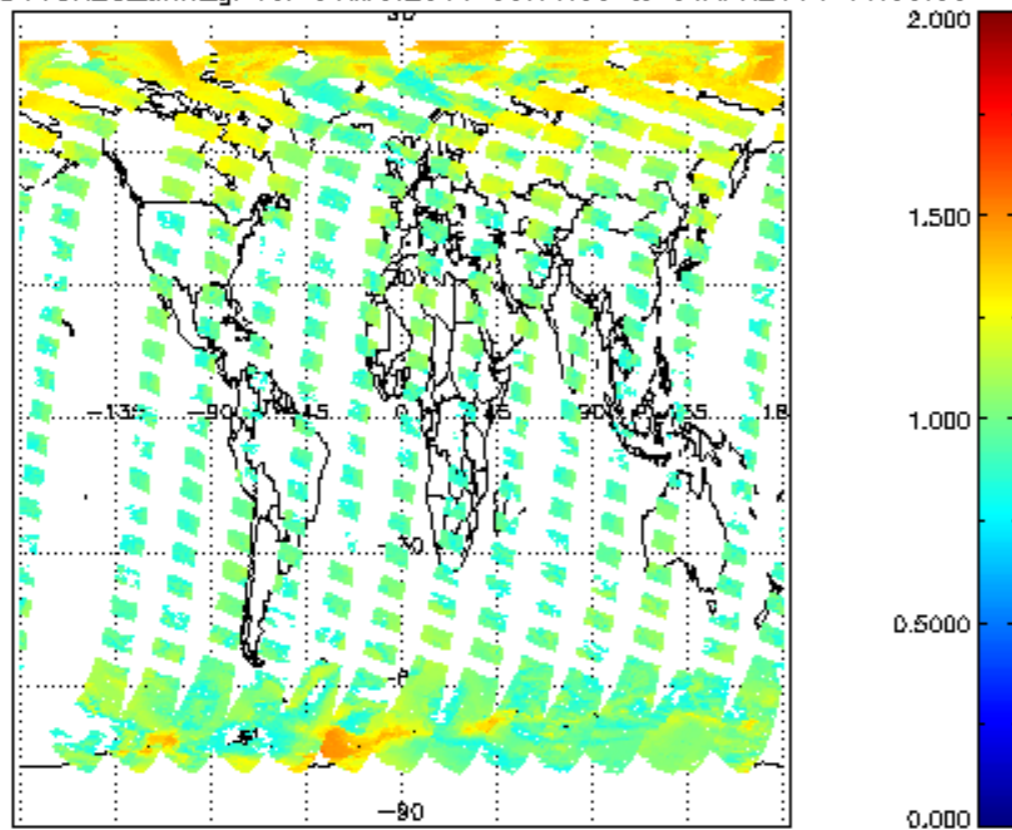
SCIOL2P_NADUV8H20_amf_gr for 31MAR2011 00:00:00 to 01APR2011 00:00:00
