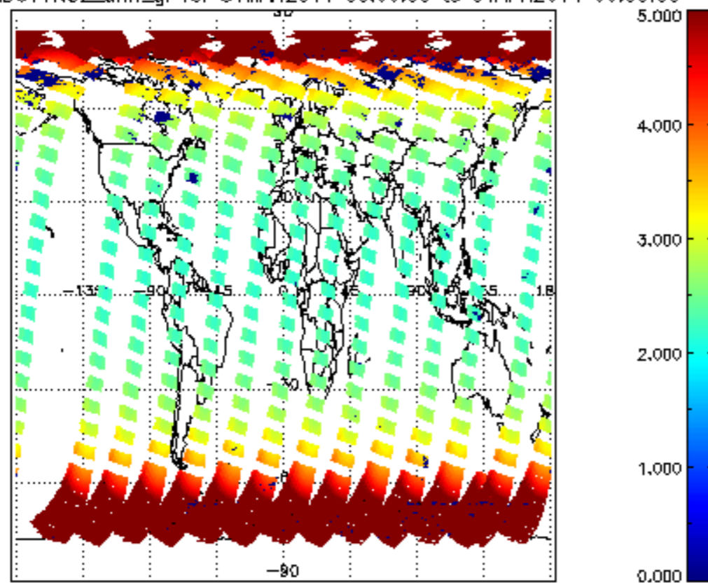
SCIOL2P_NADUV1NO2_amf_gr for 31MAR2011 00:00:00 to 01APR2011 00:00:00
