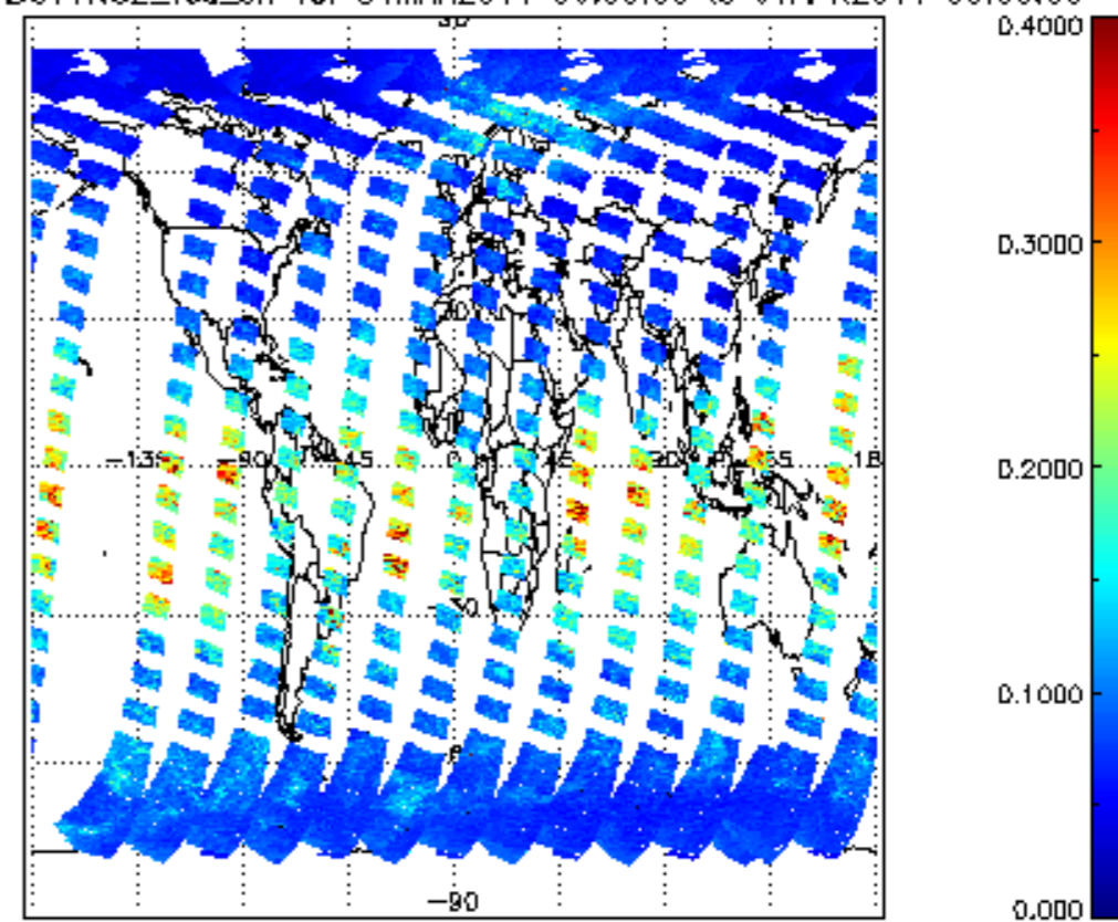
SCIOL2P_NADUV1NO2_vcd_err for 31MAR2011 00:00:00 to 01APR2011 00:00:00
