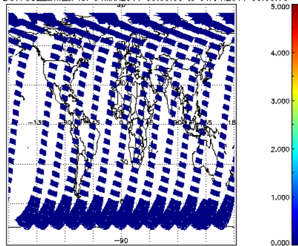
SCIOL2P_NADUV7S02_amf_cl for 31MAR2011 00:00:00 to 01APR2011 00:00:00
