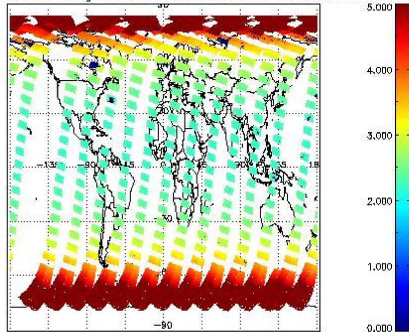
SCIOL2P_NADUV003_amf_gr for 31MAR2011 00:00:00 to 01APR2011 00:00:00
