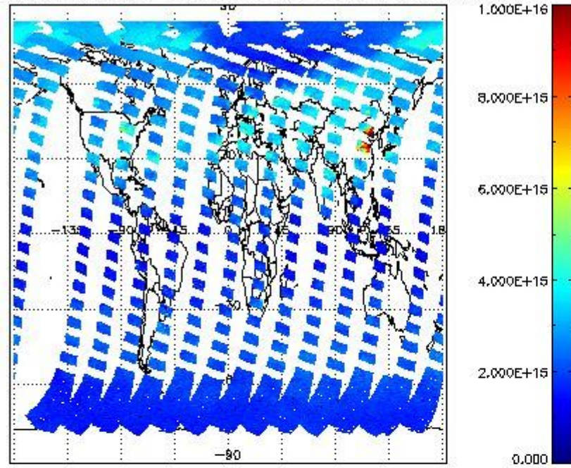
SCIOL2P_NADUV1NO2_vcd for 31MAR2011 00:00:00 to 01APR2011 00:00:00
