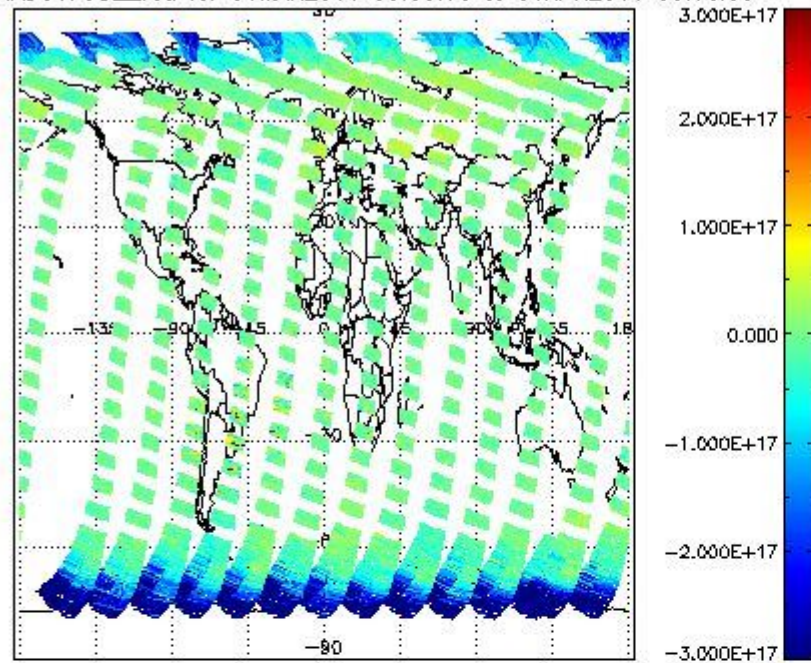
SCIOL2P_NADUV7S02_vcd for 31MAR2011 00:00:00 to 01APR2011 00:00:00
