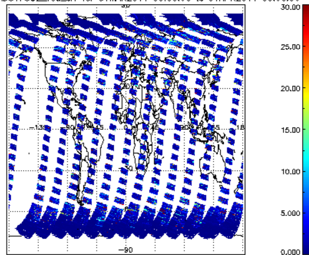
SCIOL2P_NADUV7S02_vcd_err for 31MAR2011 00:00:00 to 01APR2011 00:00:00
