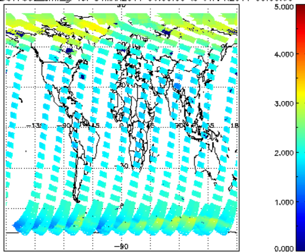
SCIOL2P_NADUV7S02_amf_gr for 31MAR2011 00:00:00 to 01APR2011 00:00:00
