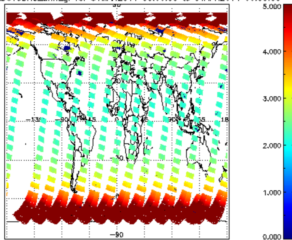
SCIOL2P_NADUV3BRO_amf_gr for 31MAR2011 00:00:00 to 01APR2011 00:00:00
