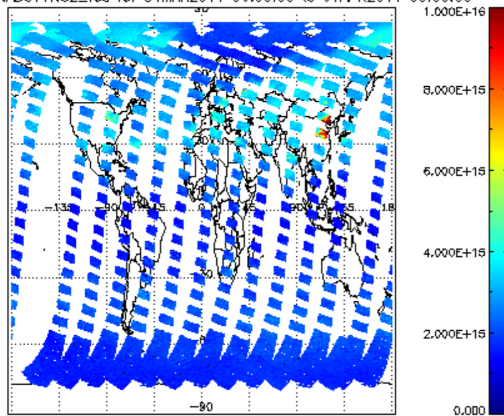
SCIOL2P_NADUV1NO2_vcd for 31MAR2011 00:00:00 to 01APR2011 00:00:00
