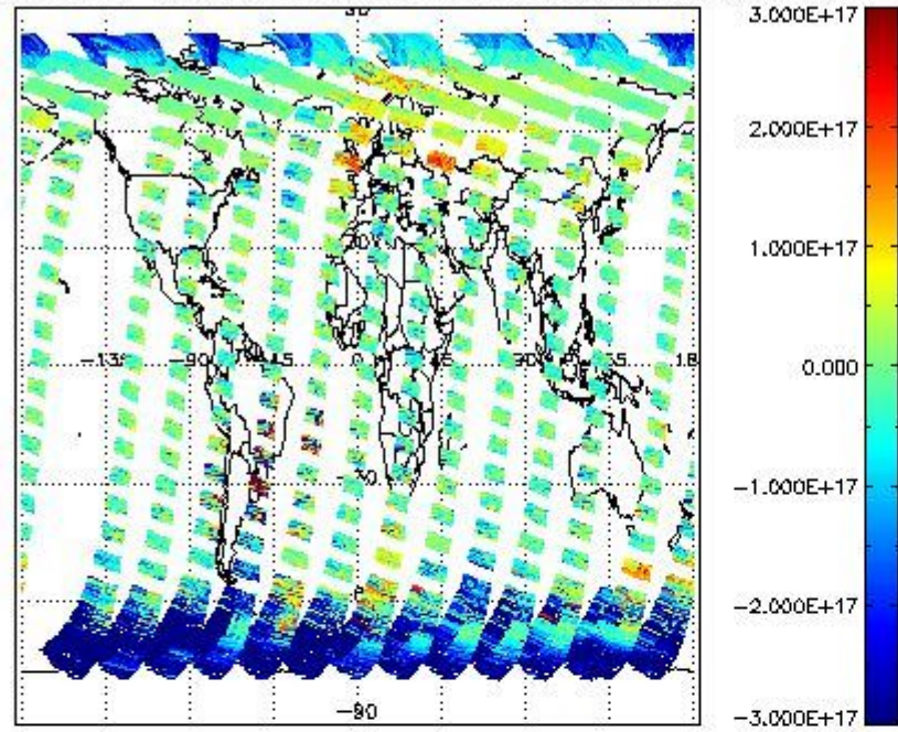
SCIOL2P_NADUV5SO2_vcd for 31MAR2011 00:00:00 to 01APR2011 00:00:00
