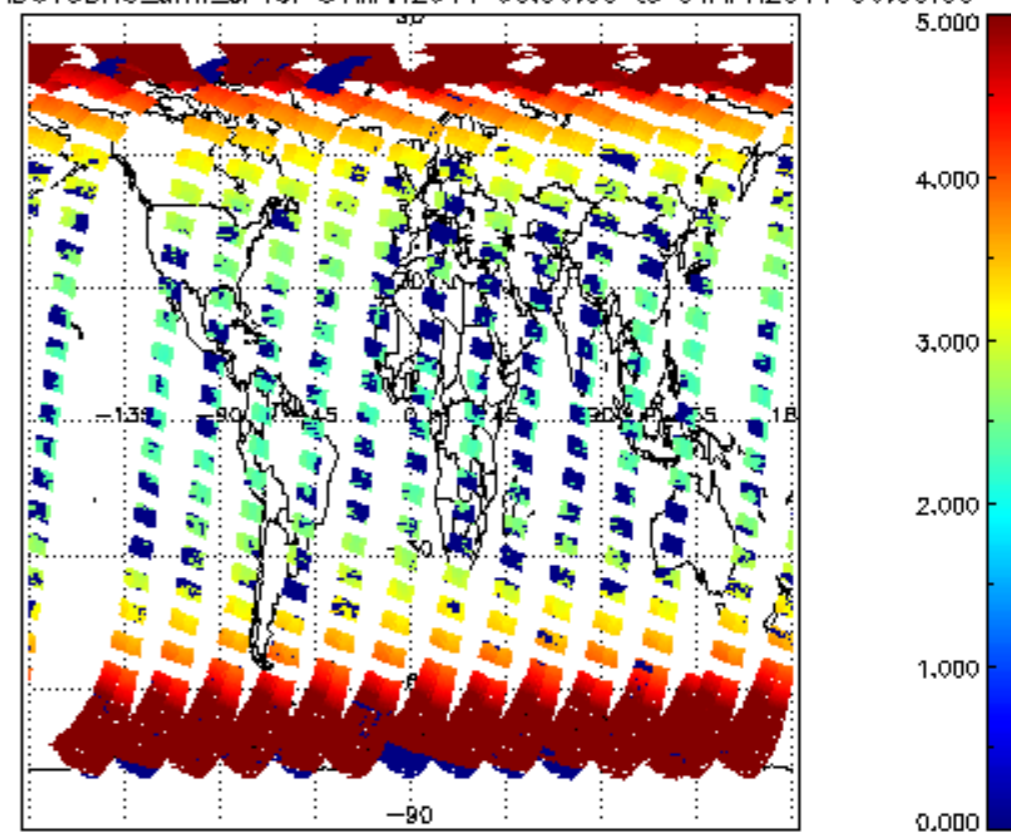
SCIOL2P_NADUV3BRO_amf_cl for 31MAR2011 00:00:00 to 01APR2011 00:00:00
