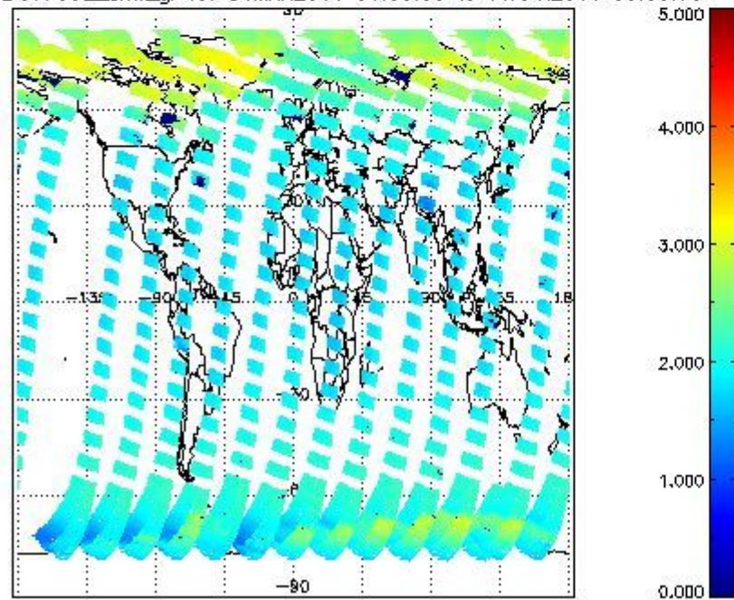
SCIOL2P_NADUV7S02_amf_gr for 31MAR2011 00:00:00 to 01APR2011 00:00:00
