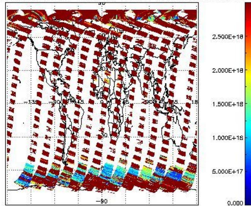
SCIDL2P_NADIR3CO_vcd_err for 31MAR2011 00:00:00 to 01APR2011 00:00:00
