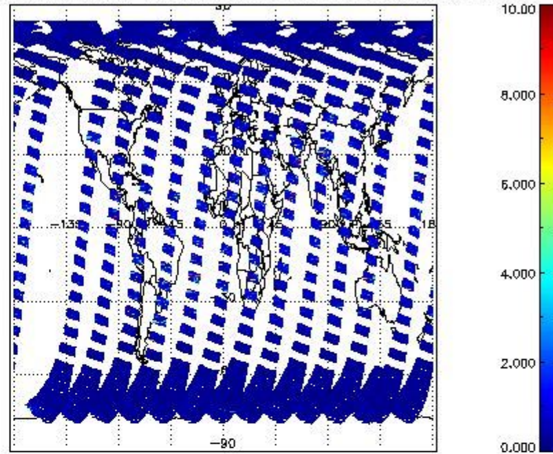
SCIOL2P_NADUV3BRO_vcd_err for 31MAR2011 00:00:00 to 01APR2011 00:00:00
