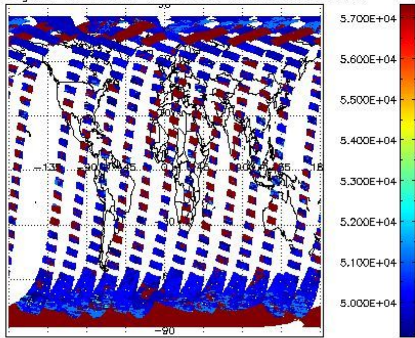
cloud_flags for 31MAR2011 00:00:00 to 01APR2011 00:00:00
