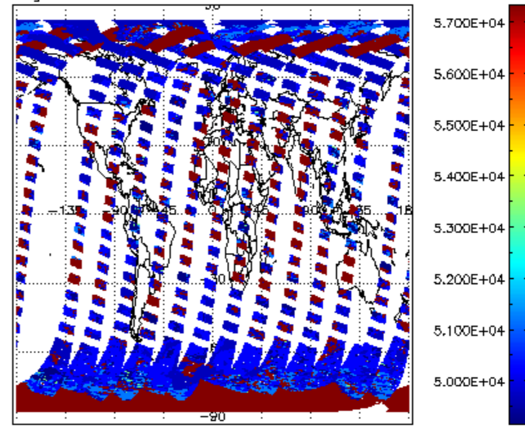
cloud_flags for 31MAR2011 00:00:00 to 01APR2011 00:00:00
