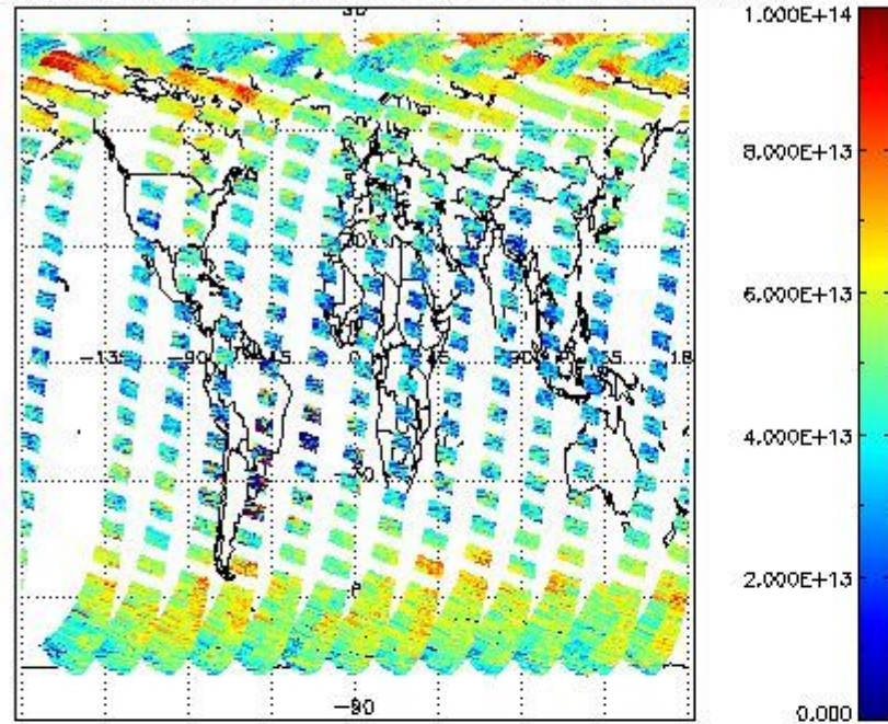
SCIOL2P_NADUV3BRO_vcd for 31MAR2011 00:00:00 to 01APR2011 00:00:00
