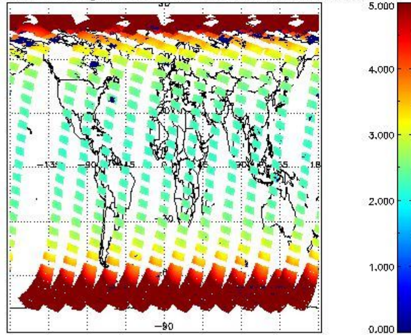
SCIOL2P_NADUV1NO2_amf_gr for 31MAR2011 00:00:00 to 01APR2011 00:00:00
