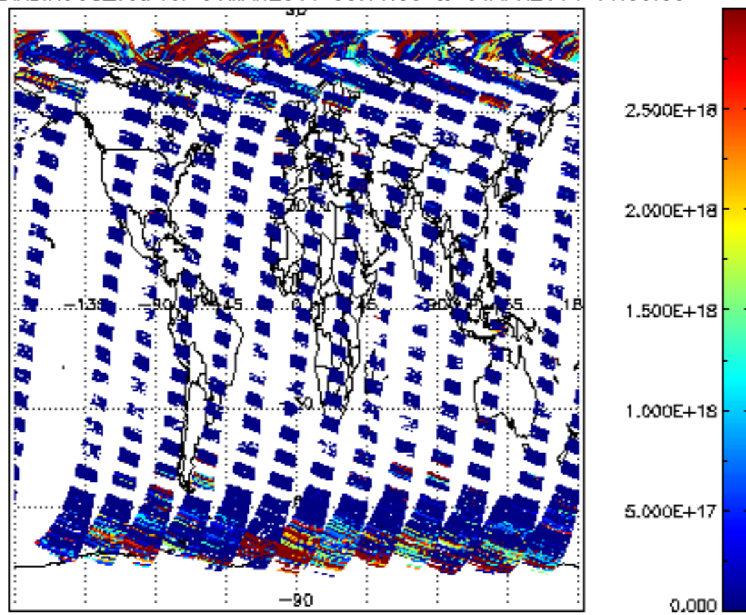
SCIOL2P_NADIR3CO_vcd for 31MAR2011 00:00:00 to 01APR2011 00:00:00
