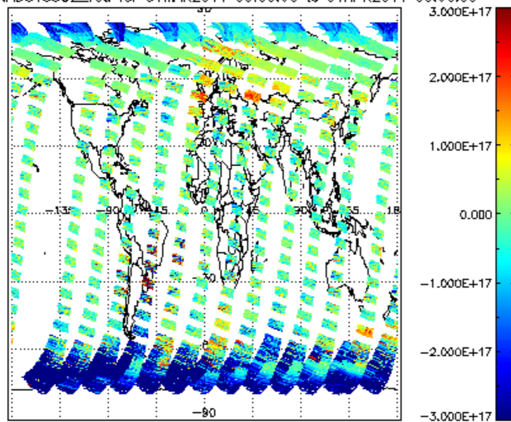
SCIOL2P_NADUV5S02_vcd for 31MAR2011 00:00:00 to 01APR2011 00:00:00
