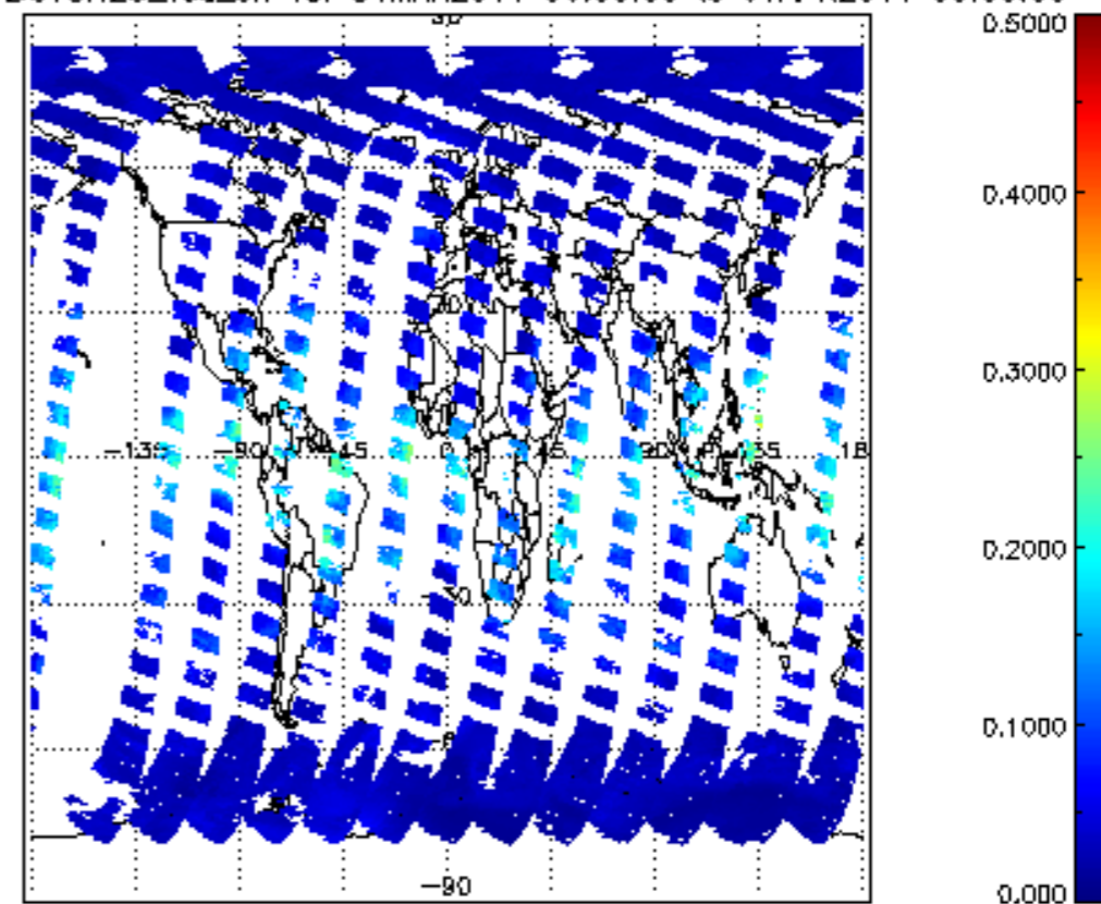
SCIOL2P_NADUV8H20_vcd_err for 31MAR2011 00:00:00 to 01APR2011 00:00:00
