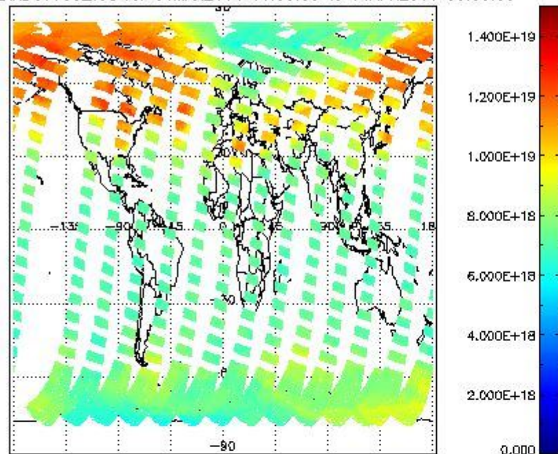
SCIOL2P_NADUV003_vcd for 31MAR2011 00:00:00 to 01APR2011 00:00:00
