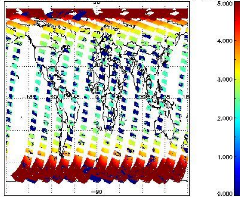
SCIOL2P_NADUV1NO2_amf_cl for 31MAR2011 00:00:00 to 01APR2011 00:00:00
