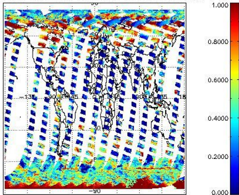
cLfrac for 31MAR2011 00:00:00 to 01APR2011 00:00:00
