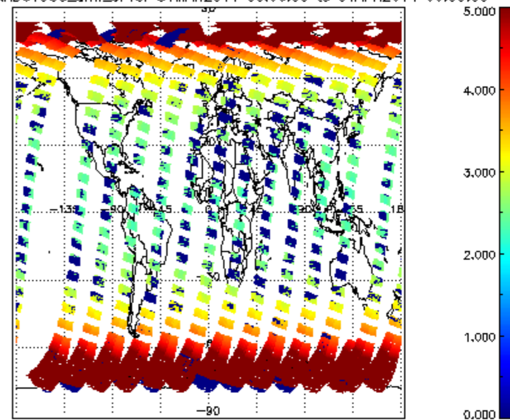
SCIOL2P_NADUV003_amf_cl for 31MAR2011 00:00:00 to 01APR2011 00:00:00
