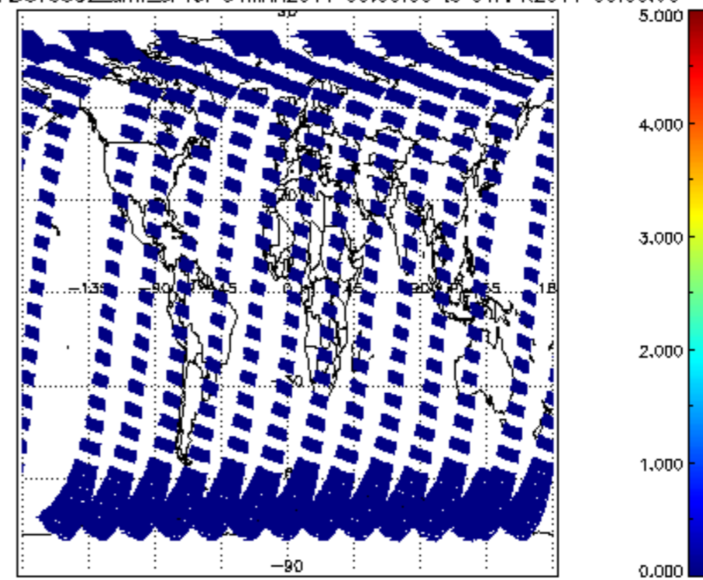
SCIOL2P_NADUV5S02_amf_cl for 31MAR2011 00:00:00 to 01APR2011 00:00:00
