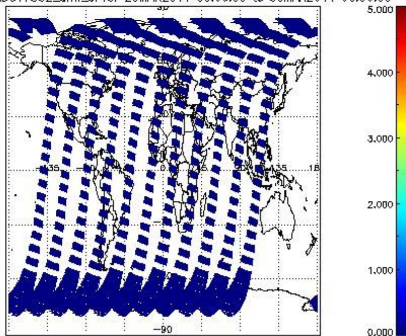
SCIOL2P_NADUV7S02_amf_cl for 29MAR2011 00:00:00 to 30MAR2011 00:00:00
