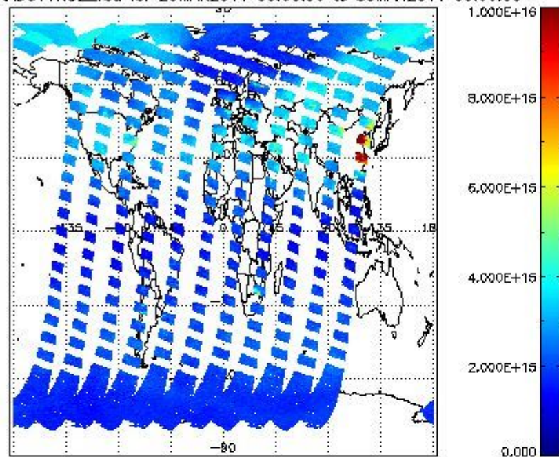
SCIOL2P_NADUV1NO2_vcd for 29MAR2011 00:00:00 to 30MAR2011 00:00:00
