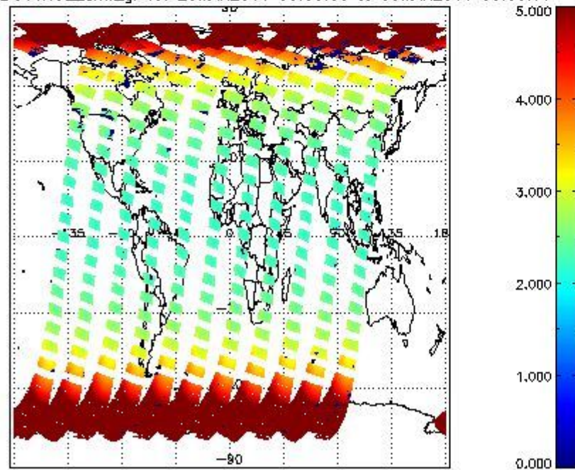
SCIOL2P_NADUV1NO2_amf_gr for 29MAR2011 00:00:00 to 30MAR2011 00:00:00
