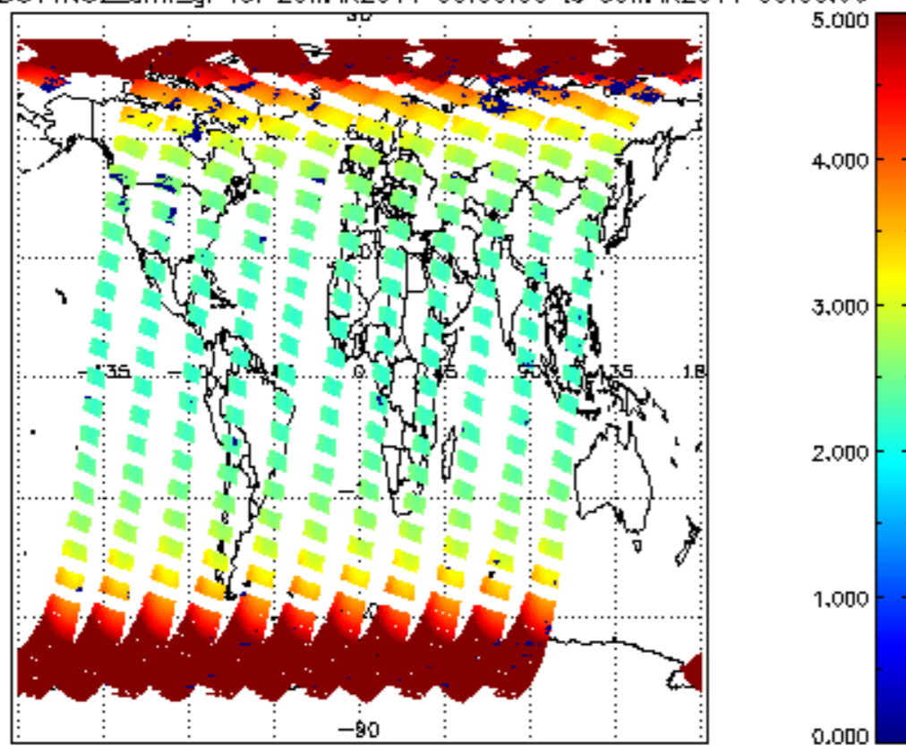
SCIOL2P_NADUV1NO2_amf_gr for 29MAR2011 00:00:00 to 30MAR2011 00:00:00
