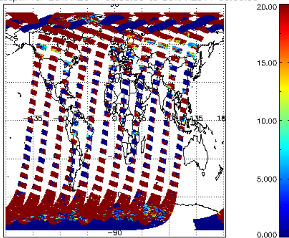
cL_opt_depth for 29MAR2011 00:00:00 to 30MAR2011 00:00:00
