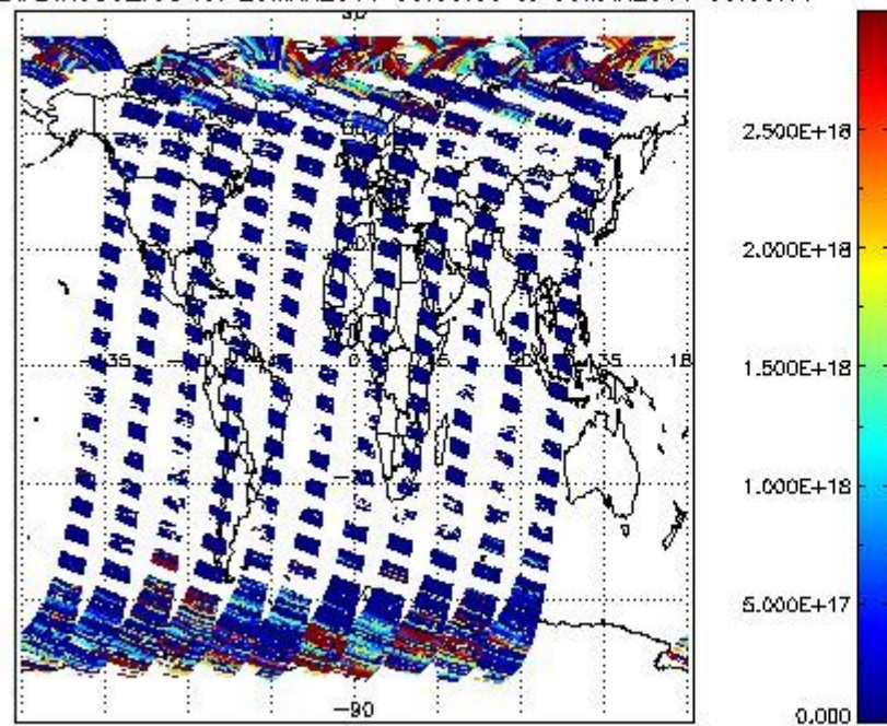
SCIDL2P_NADIR3CO_vcd for 29MAR2011 00:00:00 to 30MAR2011 00:00:00
