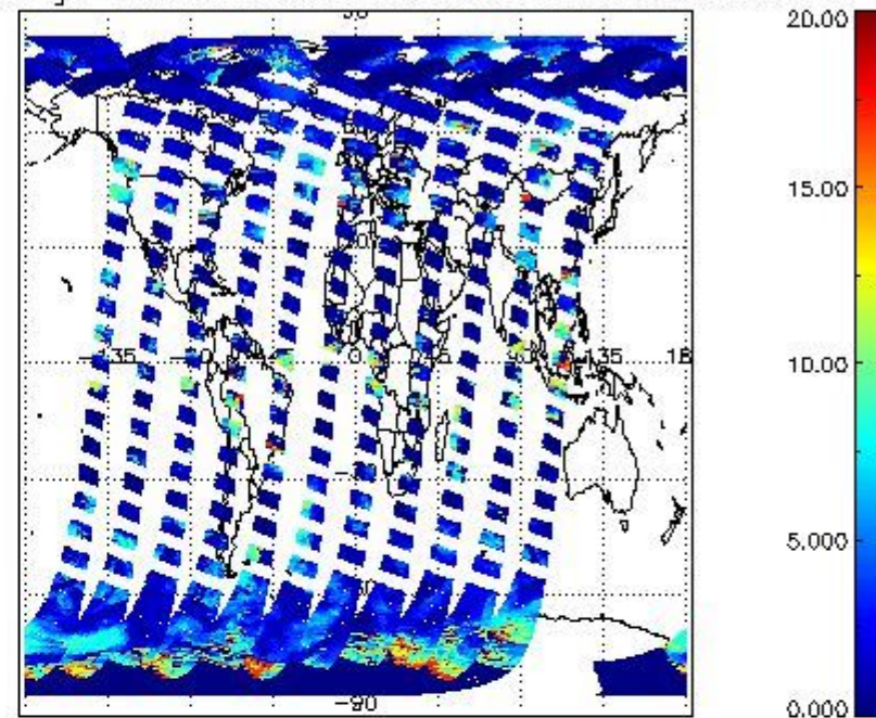
cL_top_height for 29MAR2011 00:00:00 to 30MAR2011 00:00:00
