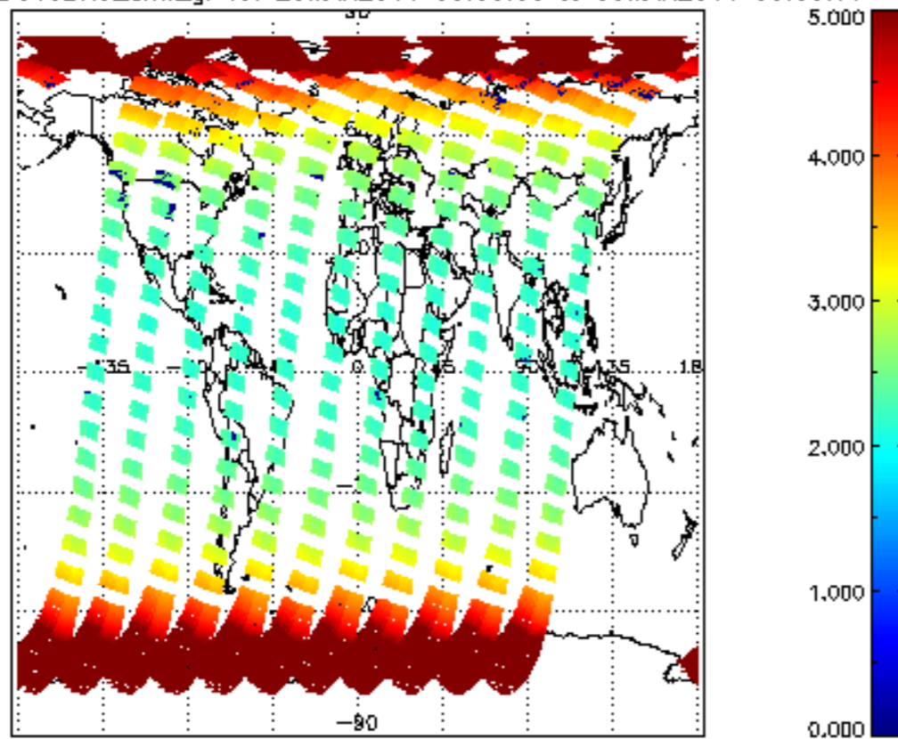
SCIOL2P_NADUV3BRO_amf_gr for 29MAR2011 00:00:00 to 30MAR2011 00:00:00
