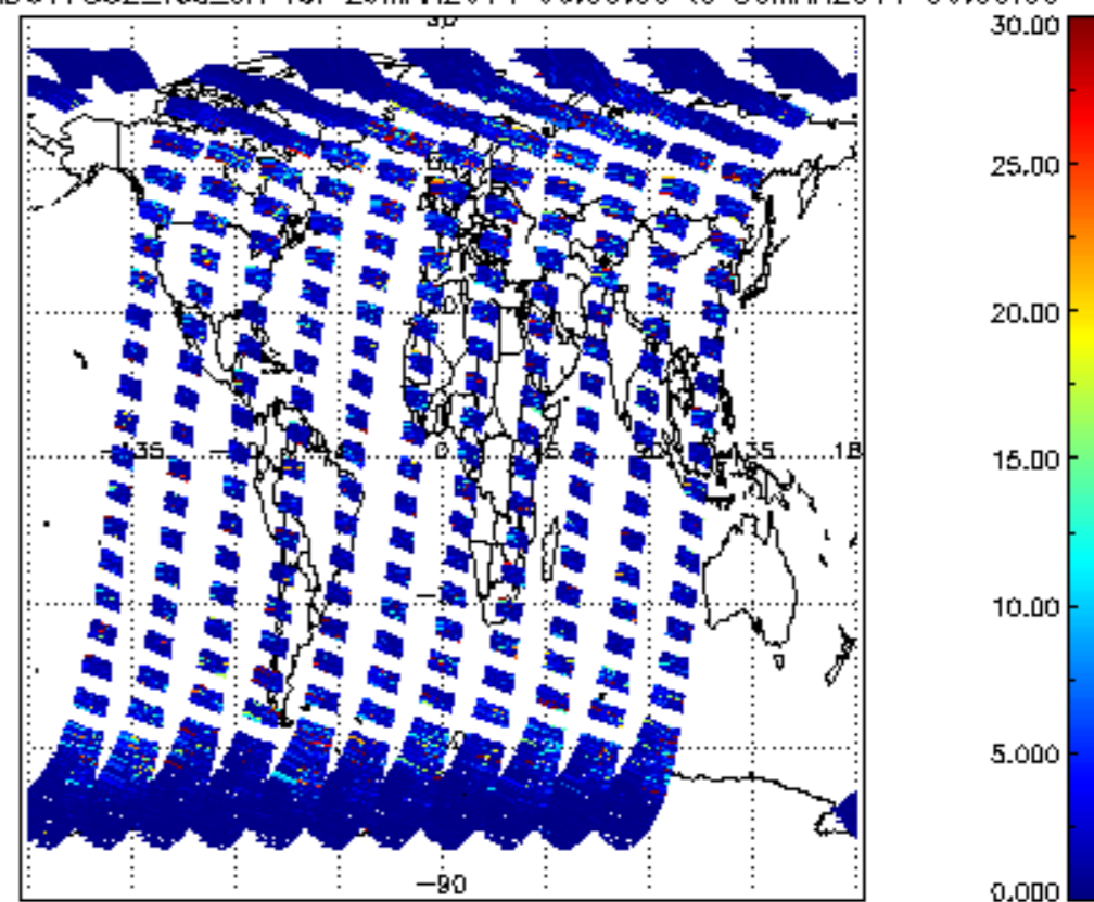
SCIOL2P_NADUV7S02_vcd_err for 29MAR2011 00:00:00 to 30MAR2011 00:00:00
