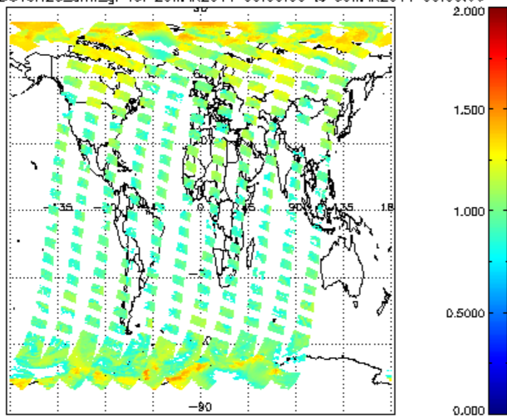
SCIOL2P_NADUV8H20_arnf_gr for 29MAR2011 00:00:00 to 30MAR2011 00:00:00
