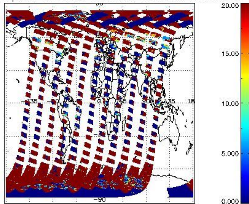
cL_opt_depth for 29MAR2011 00:00:00 to 30MAR2011 00:00:00
