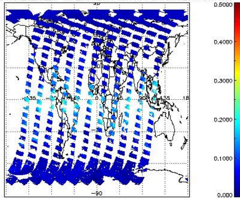
SCIOL2P_NADUV8H2O_vcd_err for 29MAR2011 00:00:00 to 30MAR2011 00:00:00
