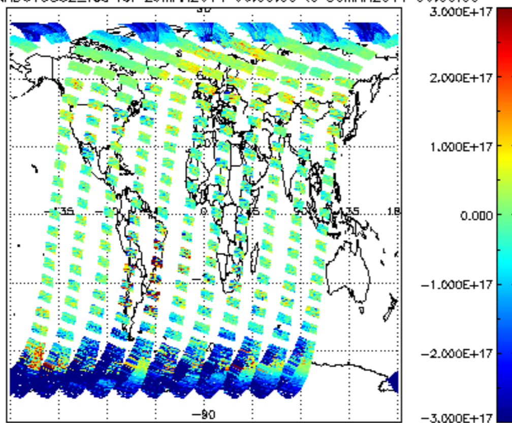
SCIOL2P_NADUV5S02_vcd for 29MAR2011 00:00:00 to 30MAR2011 00:00:00
