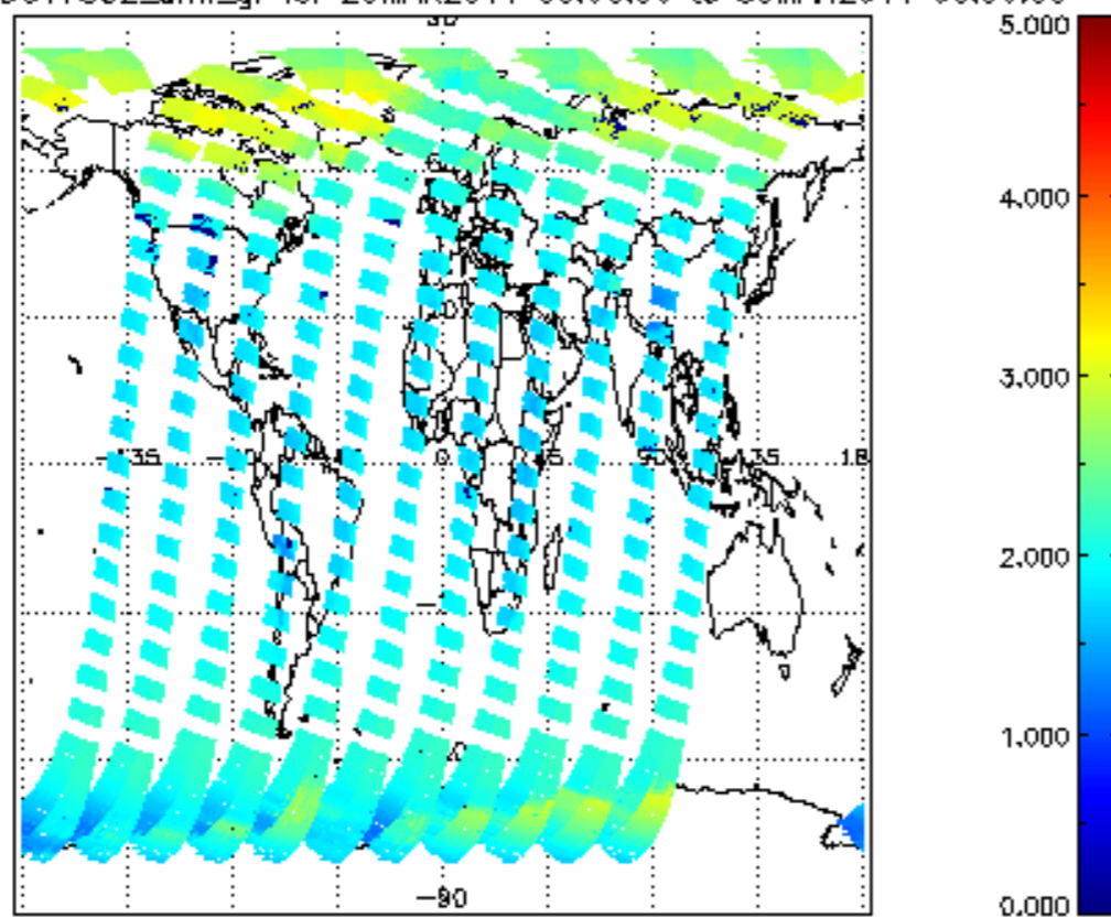
SCIOL2P_NADUV7S02_amf_gr for 29MAR2011 00:00:00 to 30MAR2011 00:00:00
