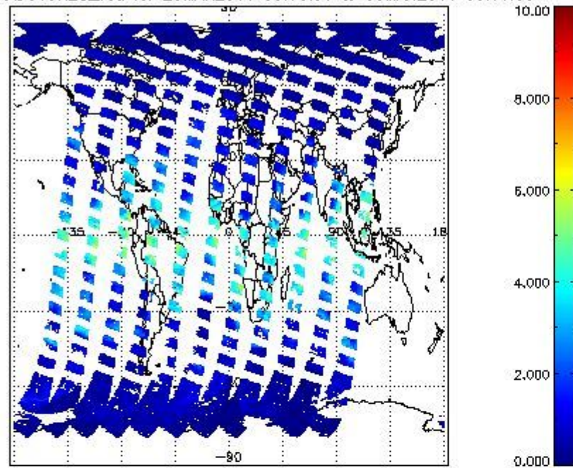
SCIOL2P_NADUV8H2O_vcd for 29MAR2011 00:00:00 to 30MAR2011 00:00:00
