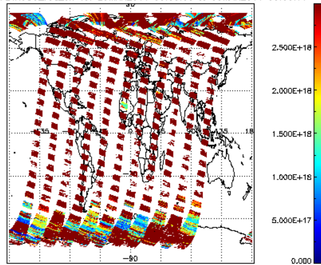
SCIOL2P_NADIR3CO_vcd_err for 29MAR2011 00:00:00 to 30MAR2011 00:00:00
