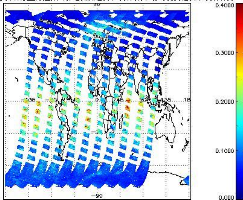
SCIOL2P_NADUV1NO2_vcd_err for 29MAR2011 00:00:00 to 30MAR2011 00:00:00
