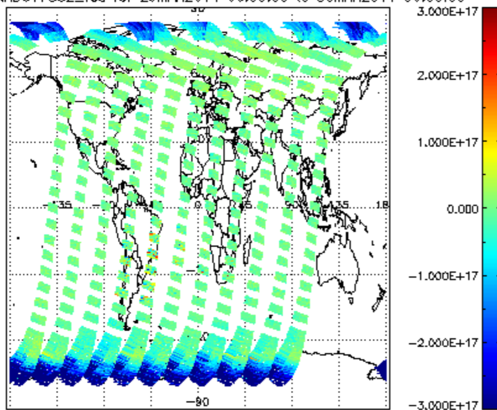
SCIOL2P_NADUV7S02_vcd for 29MAR2011 00:00:00 to 30MAR2011 00:00:00
