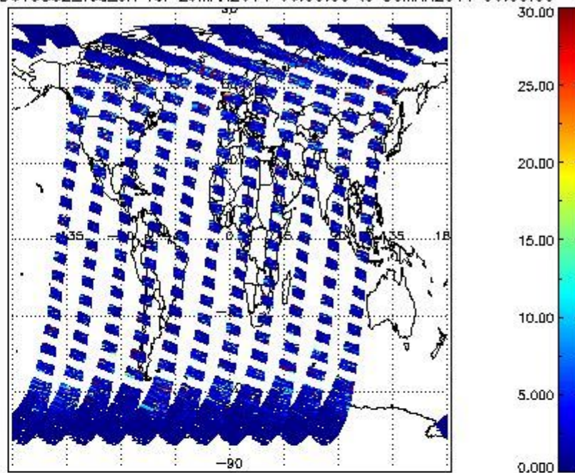
SCIOL2P_NADUV5SO2_vcd_err for 29MAR2011 00:00:00 to 30MAR2011 00:00:00
