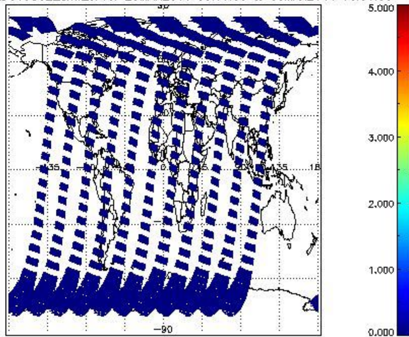
SCIOL2P_NADUV5SO2_amf_cl for 29MAR2011 00:00:00 to 30MAR2011 00:00:00
