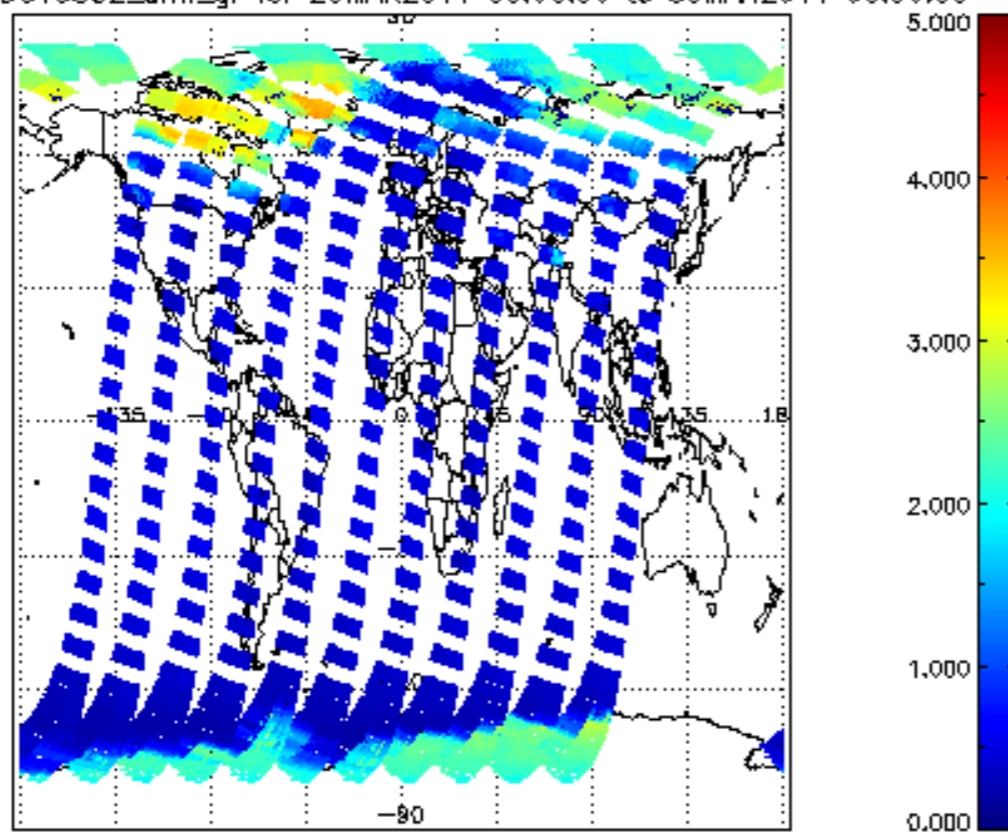
SCIOL2P_NADUV5S02_amf_gr for 29MAR2011 00:00:00 to 30MAR2011 00:00:00
