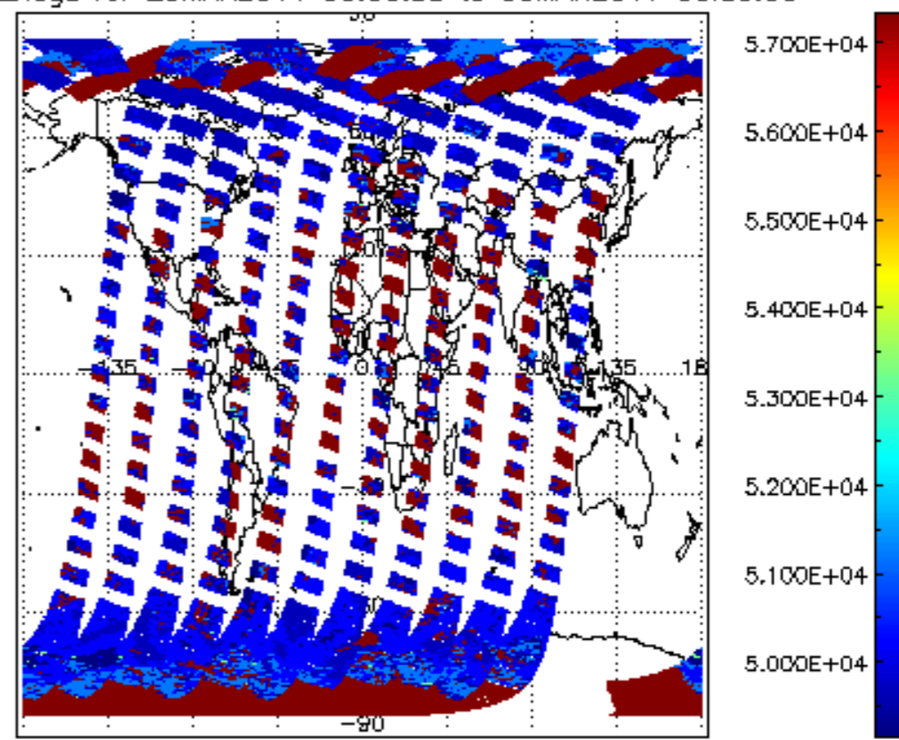
cloud_flags for 29MAR2011 00:00:00 to 30MAR2011 00:00:00
