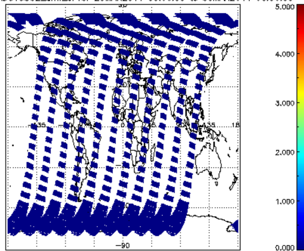
SCIOL2P_NADUV5S02_amf_cl for 29MAR2011 00:00:00 to 30MAR2011 00:00:00
