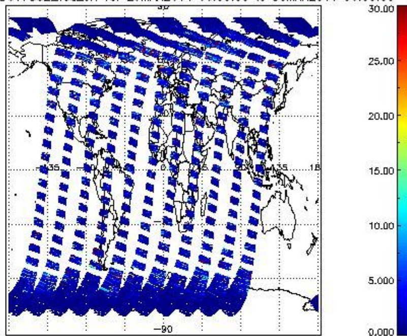
SCIOL2P_NADUV7S02_vcd_err for 29MAR2011 00:00:00 to 30MAR2011 00:00:00
