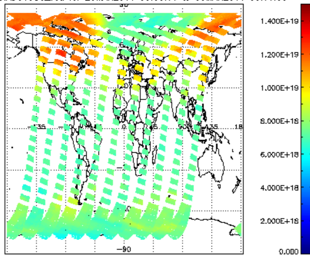
SCIOL2P_NADUV003_vcd for 29MAR2011 00:00:00 to 30MAR2011 00:00:00
