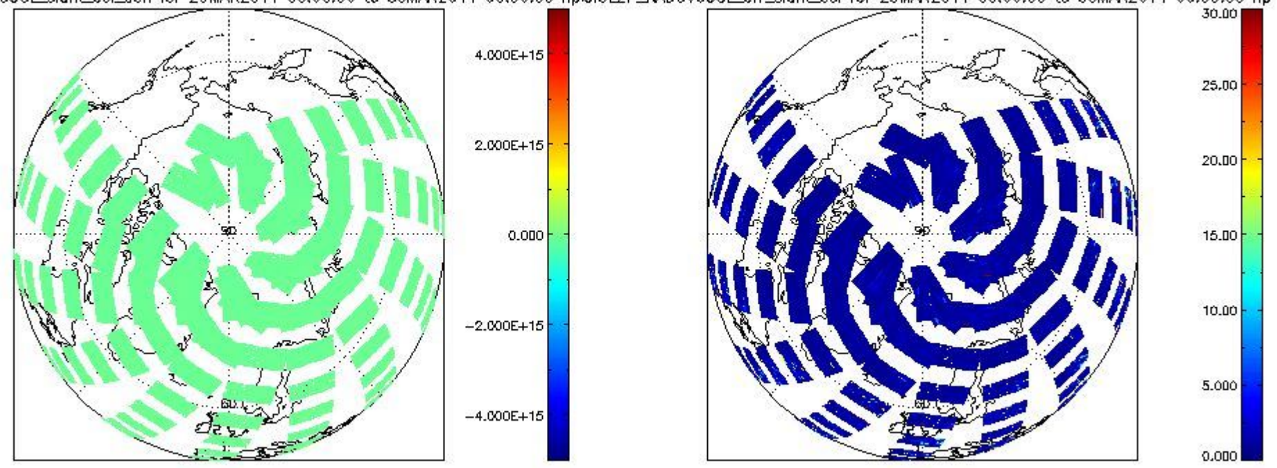
CIOL2P_NADUV6OCL_slant_col_den for 29MAR2011 00:00:00 to 30MAR2011 00:00:00 np CIOL2P_NADUV6OCL_err_slant_col for 29MAR2011 00:00:00 to 30MAR2011 00:00:00 np
