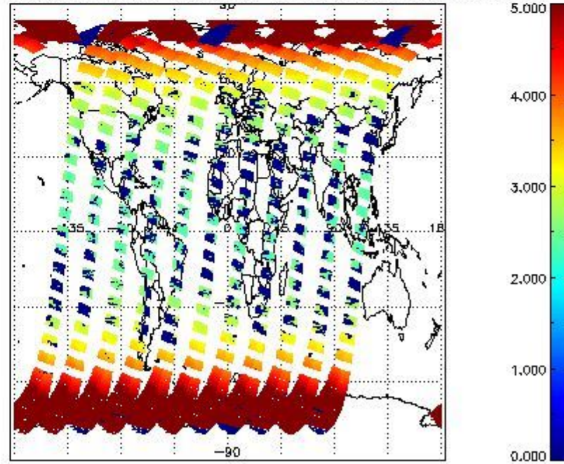
SCIOL2P_NADUV003_amf_cl for 29MAR2011 00:00:00 to 30MAR2011 00:00:00
