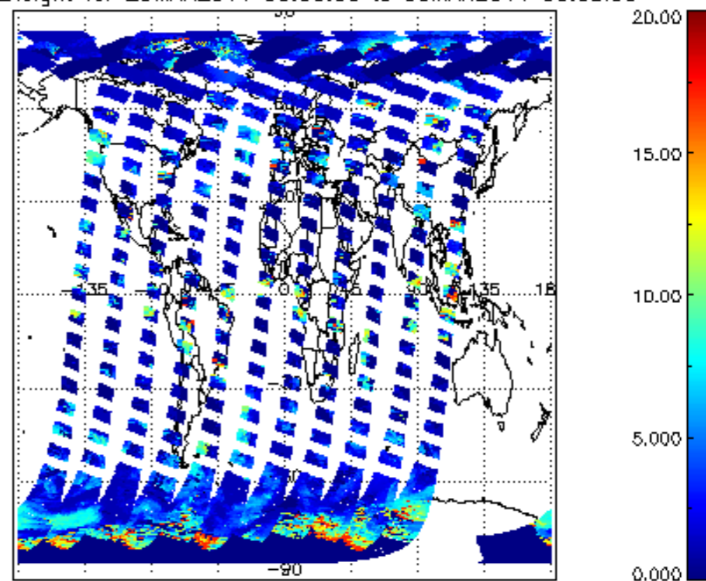
cL_top_height for 29MAR2011 00:00:00 to 30MAR2011 00:00:00
