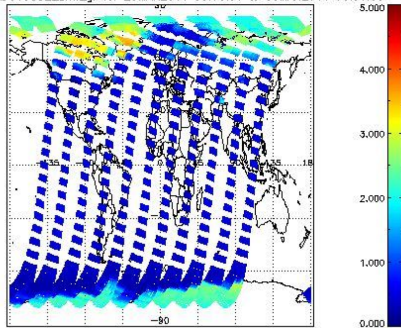
SCIOL2P_NADUV5SO2_amf_gr for 29MAR2011 00:00:00 to 30MAR2011 00:00:00
