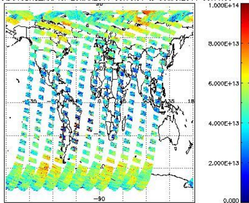
SCIOL2P_NADUV3BRO_vcd for 29MAR2011 00:00:00 to 30MAR2011 00:00:00
