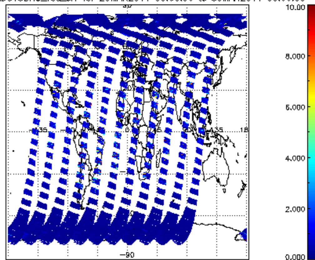
SCIOL2P_NADUV3BRO_vcd_err for 29MAR2011 00:00:00 to 30MAR2011 00:00:00
