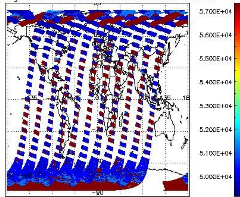
cloud_flags for 29MAR2011 00:00:00 to 30MAR2011 00:00:00
