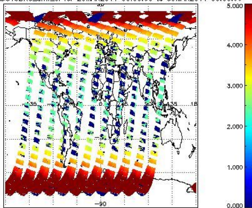
SCIOL2P_NADUV3BRO_amf_cl for 29MAR2011 00:00:00 to 30MAR2011 00:00:00
