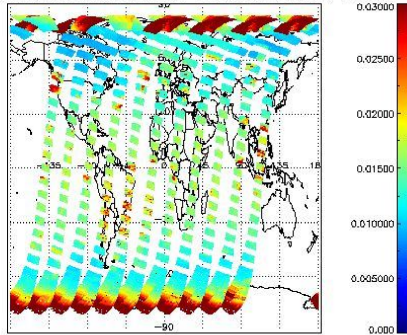
SCIOL2P_NADUV003_vcd_err for 29MAR2011 00:00:00 to 30MAR2011 00:00:00
