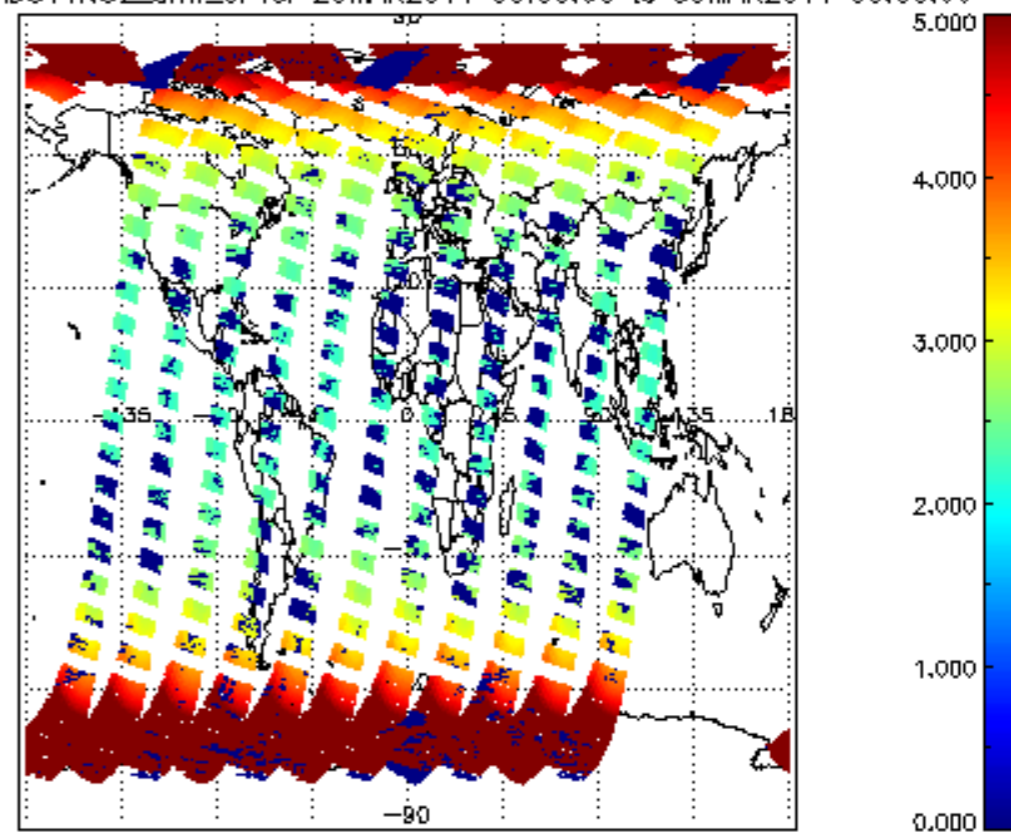
SCIOL2P_NADUV1NO2_amf_cl for 29MAR2011 00:00:00 to 30MAR2011 00:00:00
