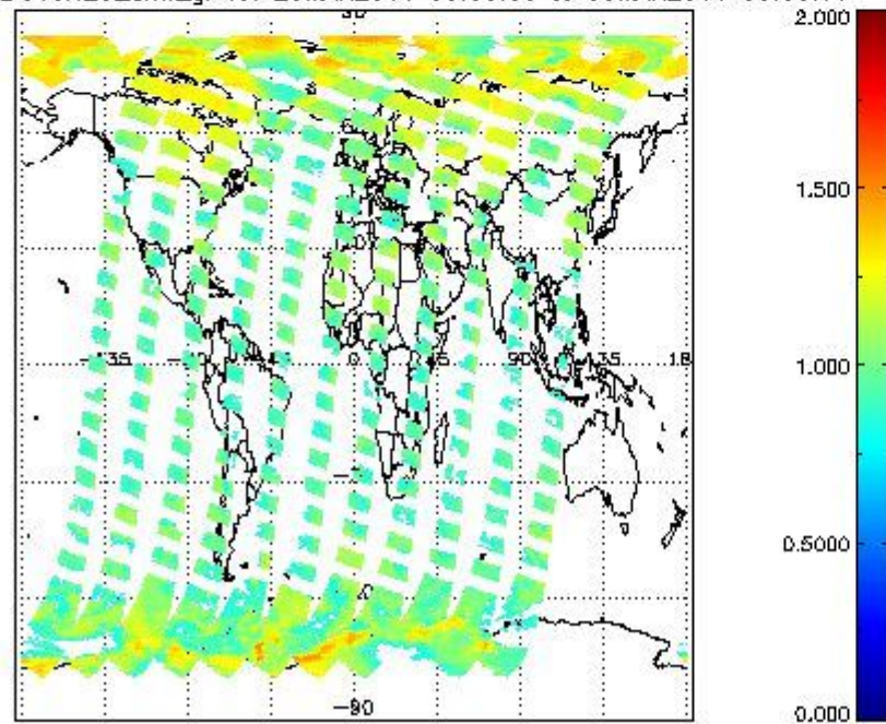
SCIOL2P_NADUV8H2O_arnf_gr for 29MAR2011 00:00:00 to 30MAR2011 00:00:00
