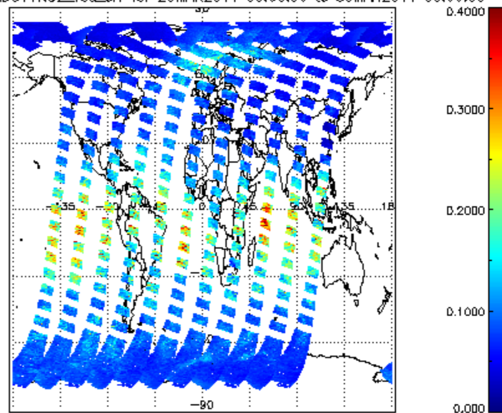
SCIOL2P_NADUV1NO2_vcdLerr for 29MAR2011 00:00:00 to 30MAR2011 00:00:00
