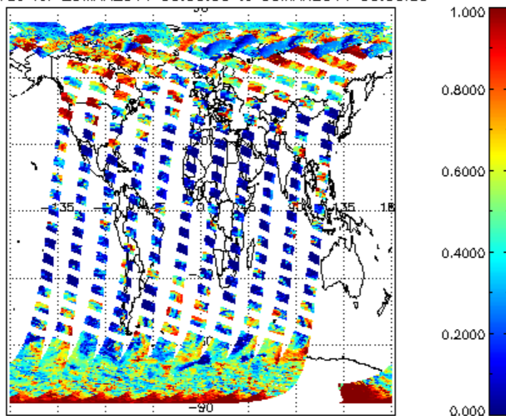
cL_frac for 29MAR2011 00:00:00 to 30MAR2011 00:00:00
