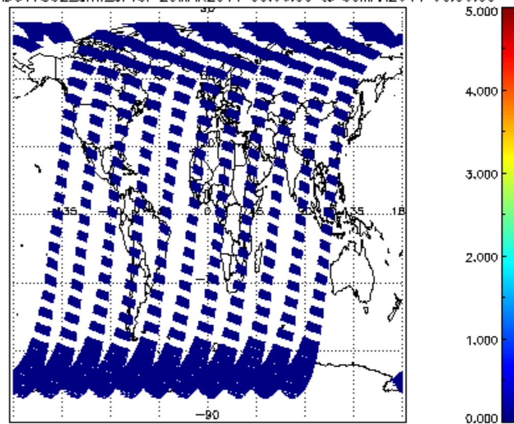
SCIOL2P_NADUV7S02_amf_cl for 29MAR2011 00:00:00 to 30MAR2011 00:00:00
