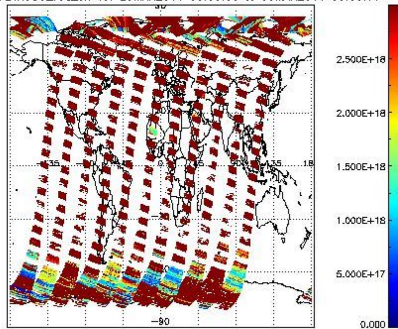
SCIDL2P_NADIR3CO_vcd_err for 29MAR2011 00:00:00 to 30MAR2011 00:00:00
