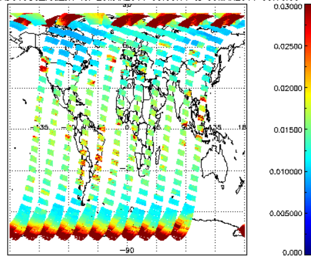
SCIOL2P_NADUV003_vcd_err for 29MAR2011 00:00:00 to 30MAR2011 00:00:00
