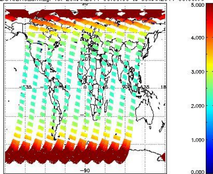
SCIOL2P_NADUV3BRO_amf_gr for 29MAR2011 00:00:00 to 30MAR2011 00:00:00
