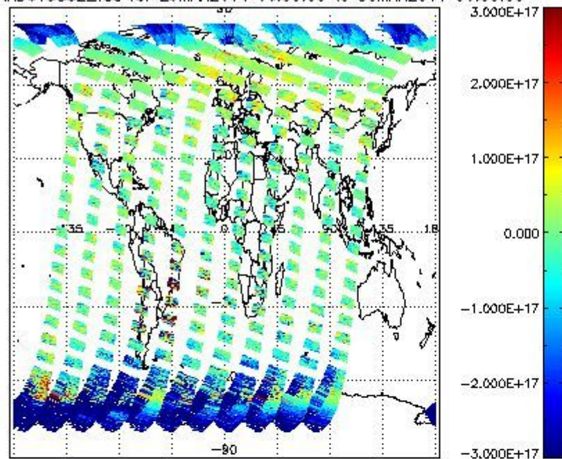
SCIOL2P_NADUV5SO2_vcd for 29MAR2011 00:00:00 to 30MAR2011 00:00:00
