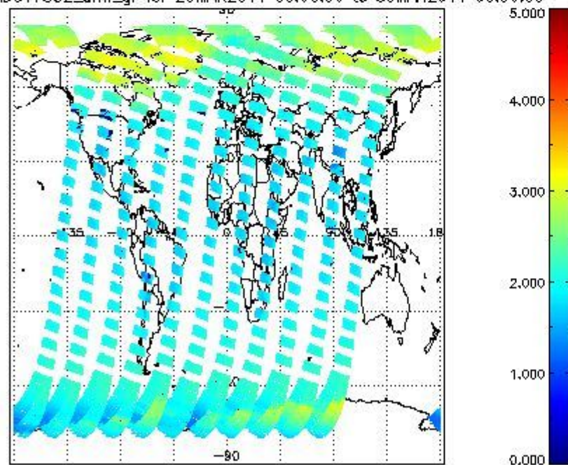
SCIOL2P_NADUV7S02_amf_gr for 29MAR2011 00:00:00 to 30MAR2011 00:00:00
