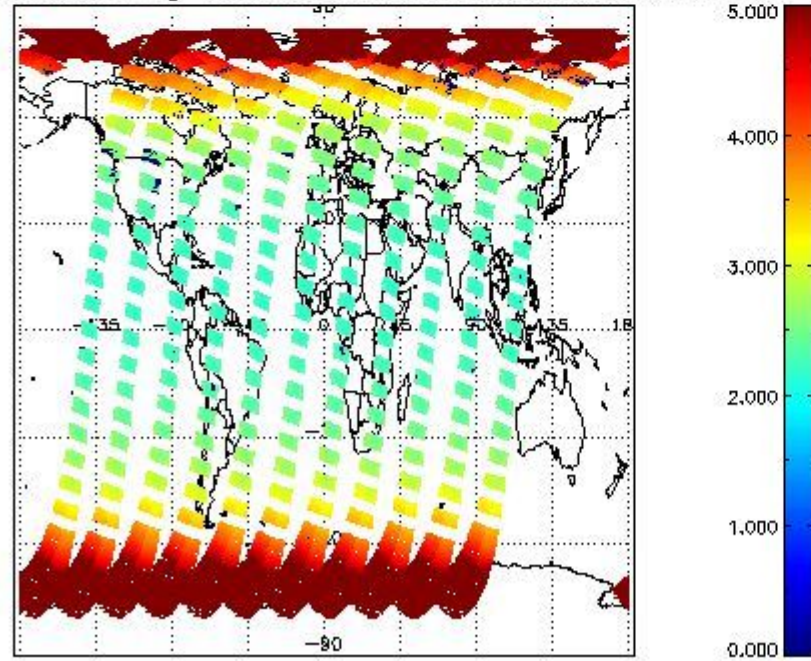
SCIOL2P_NADUV003_amf_gr for 29MAR2011 00:00:00 to 30MAR2011 00:00:00
