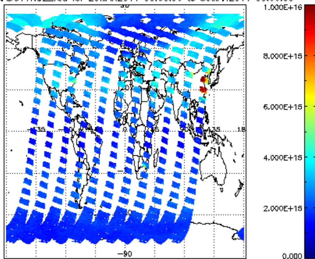
SCIOL2P_NADUV1NO2_vcd for 29MAR2011 00:00:00 to 30MAR2011 00:00:00
