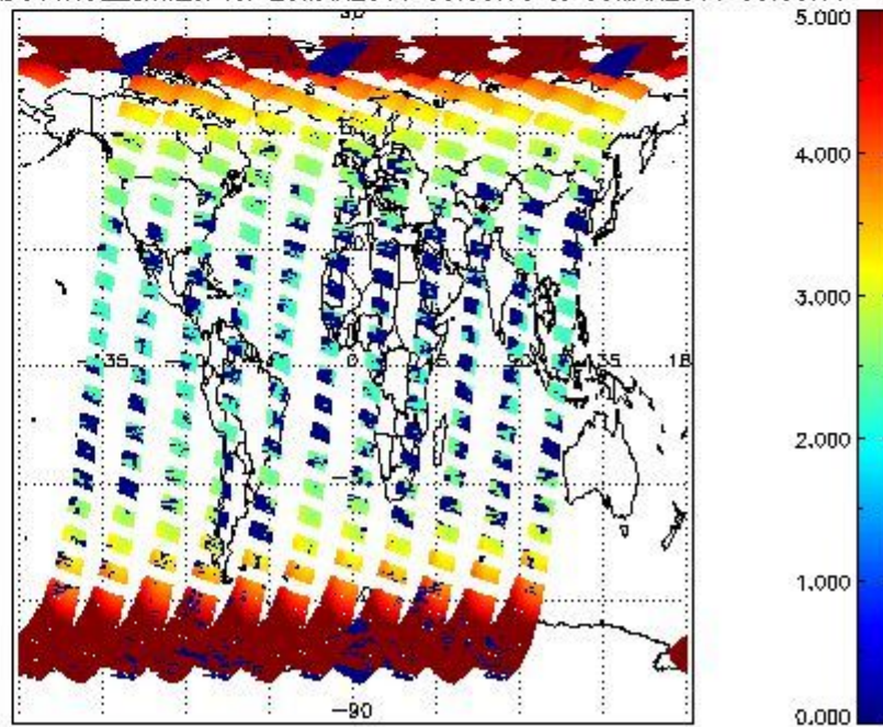
SCIOL2P_NADUV1NO2_amf_cl for 29MAR2011 00:00:00 to 30MAR2011 00:00:00
