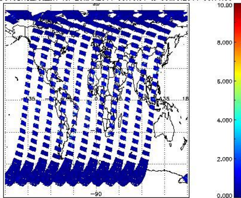
SCIOL2P_NADUV3BRO_vcd_err for 29MAR2011 00:00:00 to 30MAR2011 00:00:00
