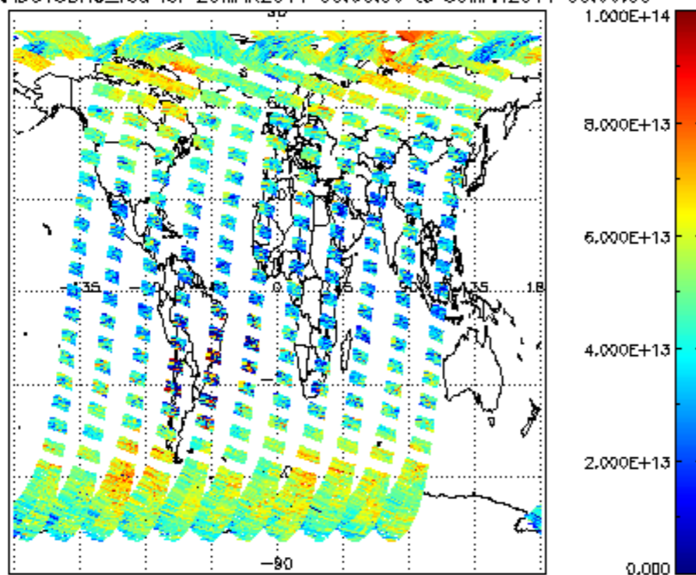
SCIOL2P_NADUV3BRO_vcd for 29MAR2011 00:00:00 to 30MAR2011 00:00:00
