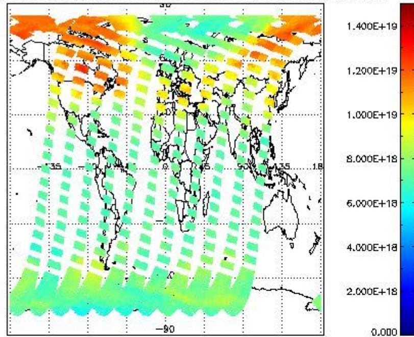
SCIOL2P_NADUV003_vcd for 29MAR2011 00:00:00 to 30MAR2011 00:00:00
