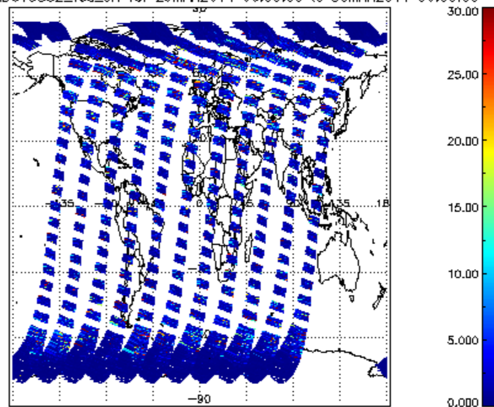
SCIOL2P_NADUV5S02_vcd_err for 29MAR2011 00:00:00 to 30MAR2011 00:00:00
