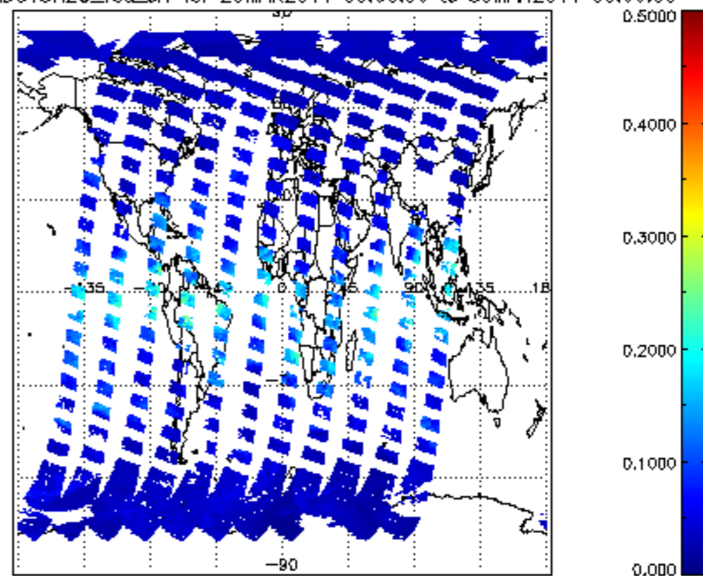
SCIOL2P_NADUV8H20_vcd_err for 29MAR2011 00:00:00 to 30MAR2011 00:00:00
