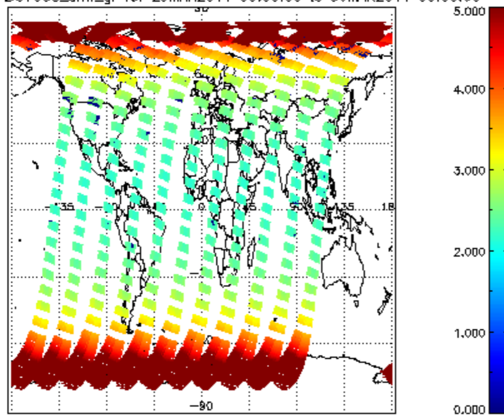
SCIOL2P_NADUV003_arnf_gr for 29MAR2011 00:00:00 to 30MAR2011 00:00:00
