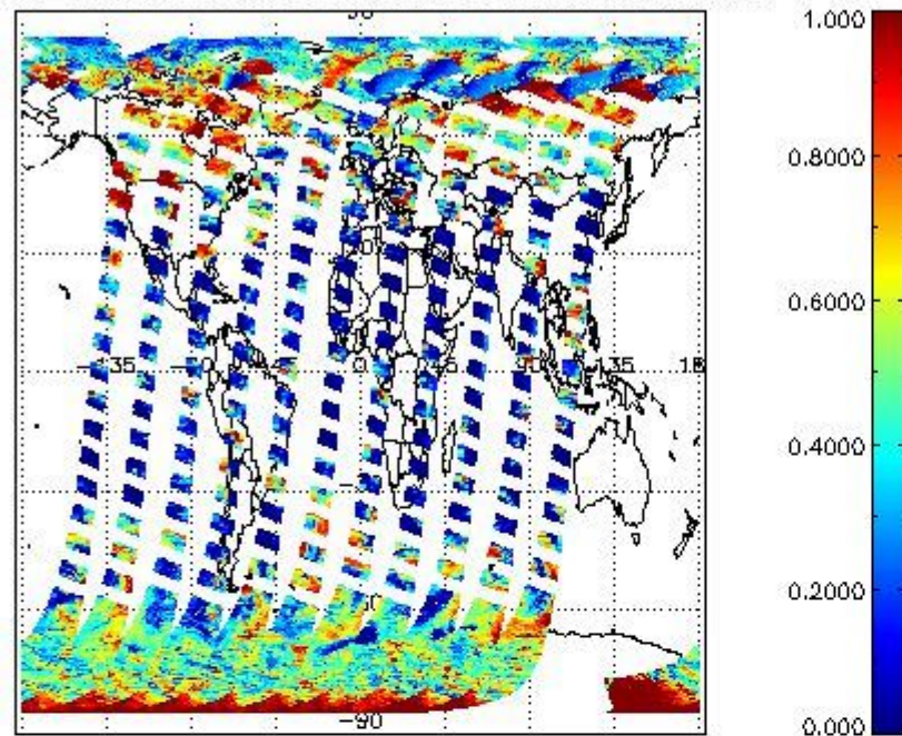
cL_frac for 29MAR2011 00:00:00 to 30MAR2011 00:00:00
