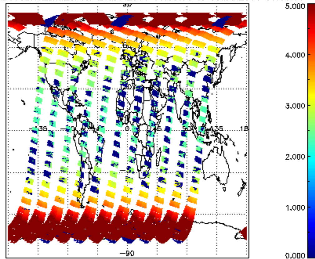
SCIOL2P_NADUV3BRO_amf_cl for 29MAR2011 00:00:00 to 30MAR2011 00:00:00
