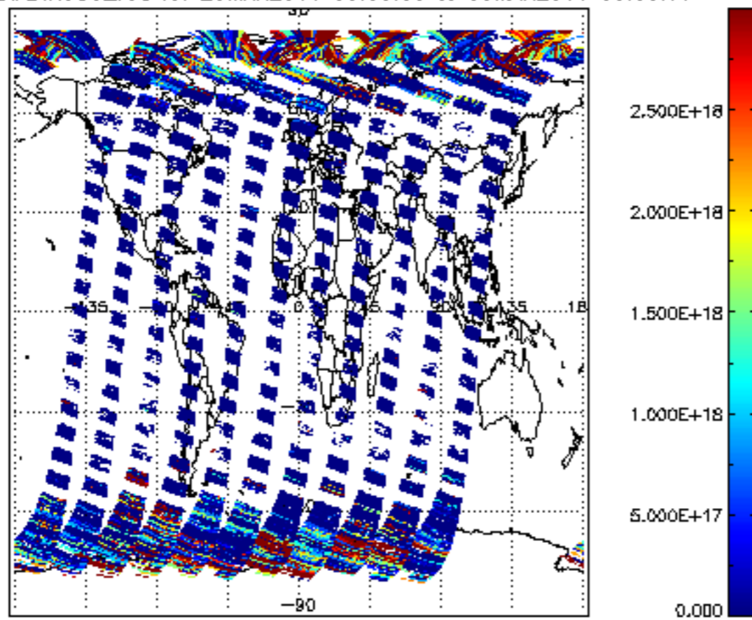
SCIOL2P_NADIR3CO_vcd for 29MAR2011 00:00:00 to 30MAR2011 00:00:00
