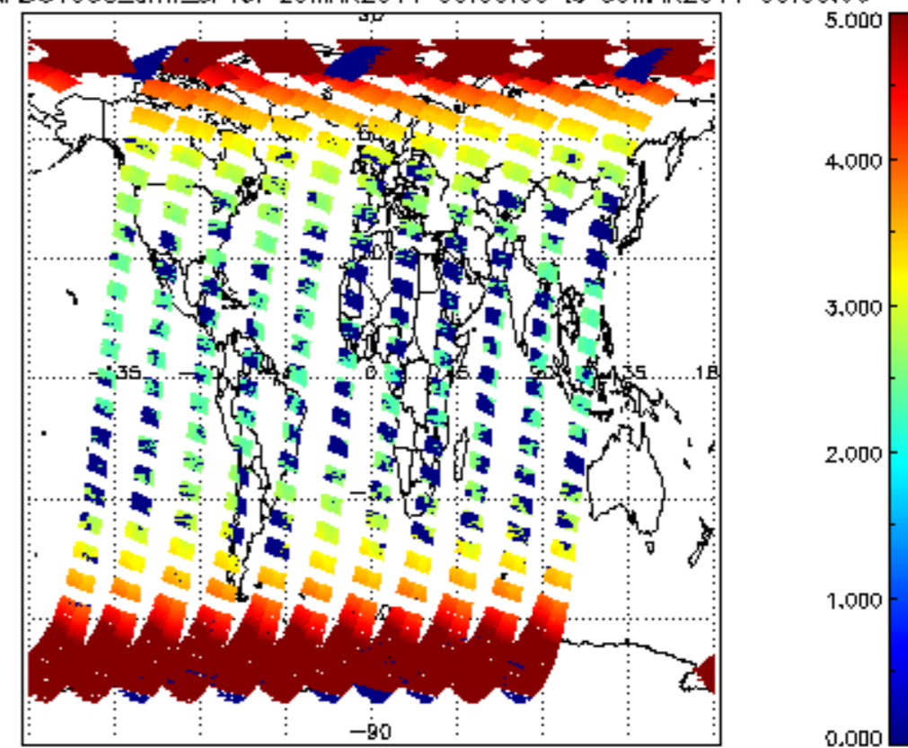
SCIOL2P_NADUV003_arnf_cl for 29MAR2011 00:00:00 to 30MAR2011 00:00:00
