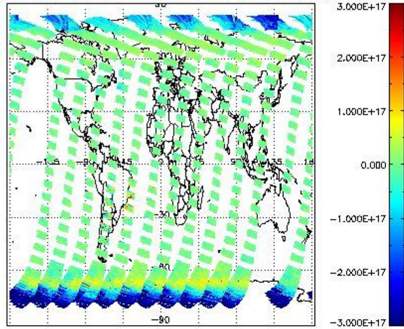
SCIOL2P_NADUV7S02_vcd for 27MAR2011 00:00:00 to 28MAR2011 00:00:00
