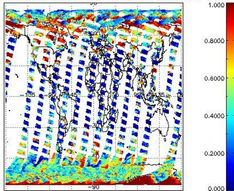
cL_frac for 27MAR2011 00:00:00 to 28MAR2011 00:00:00
