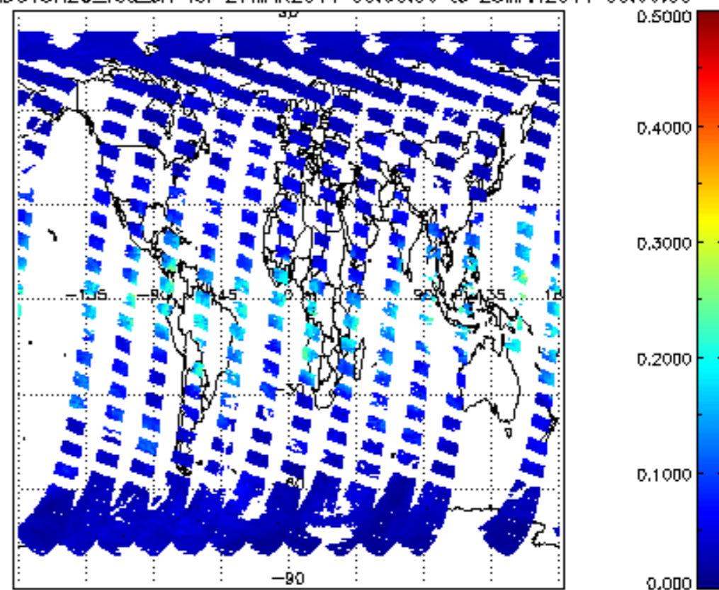
SCIOL2P_NADUV8H20_vcd_err for 27MAR2011 00:00:00 to 28MAR2011 00:00:00
