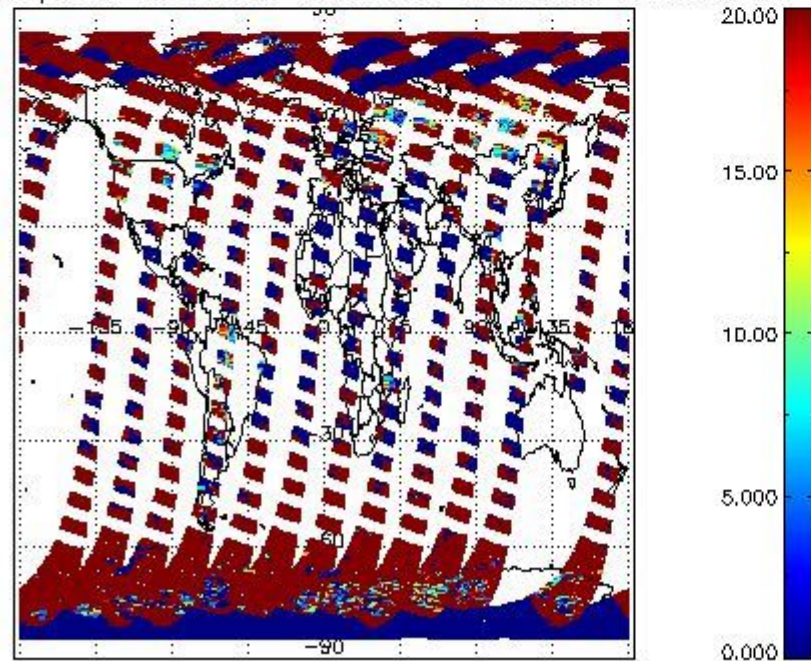
cL_opt_depth for 27MAR2011 00:00:00 to 28MAR2011 00:00:00
