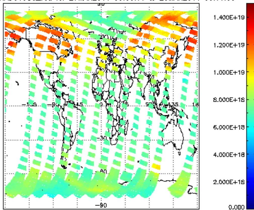
SCIOL2P_NADUV003_vcd for 27MAR2011 00:00:00 to 28MAR2011 00:00:00
