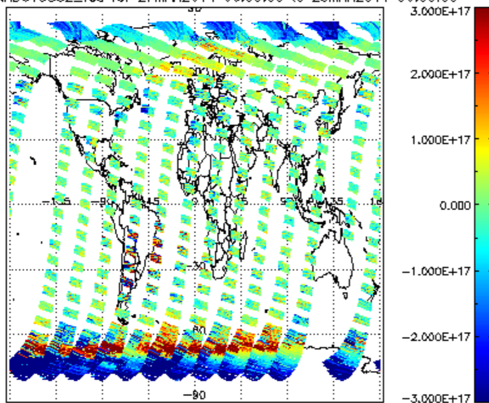
SCIOL2P_NADUV5S02_vcd for 27MAR2011 00:00:00 to 28MAR2011 00:00:00
