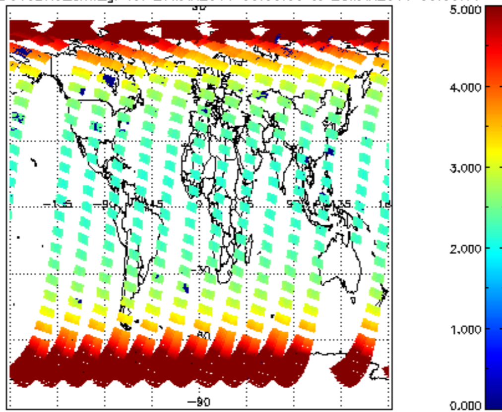
SCIOL2P_NADUV3BRO_amf_gr for 27MAR2011 00:00:00 to 28MAR2011 00:00:00
