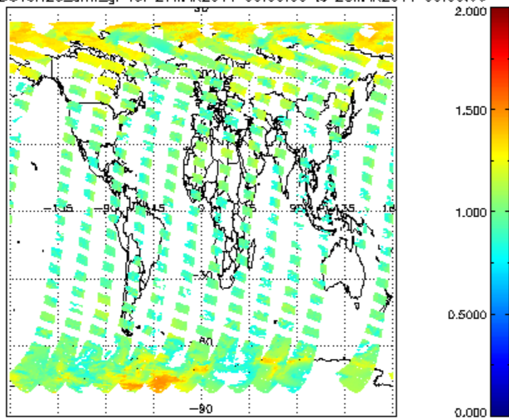
SCIOL2P_NADUV8H20_arnf_gr for 27MAR2011 00:00:00 to 28MAR2011 00:00:00
