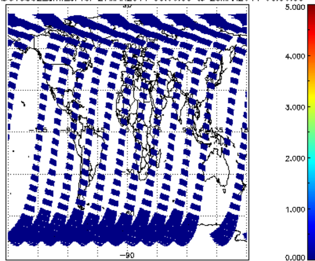
SCIOL2P_NADUV5S02_amf_cl for 27MAR2011 00:00:00 to 28MAR2011 00:00:00
