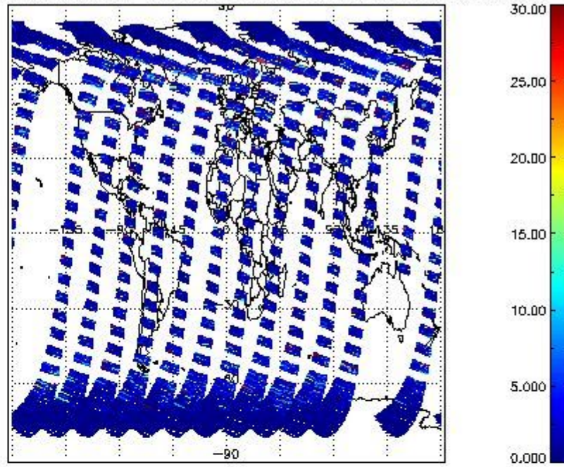
SCIOL2P_NADUV7S02_vcd_err for 27MAR2011 00:00:00 to 28MAR2011 00:00:00
