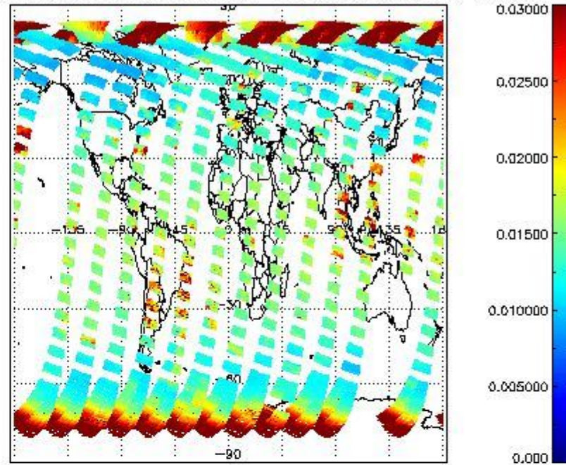
SCIOL2P_NADUV003_vcd_err for 27MAR2011 00:00:00 to 28MAR2011 00:00:00
