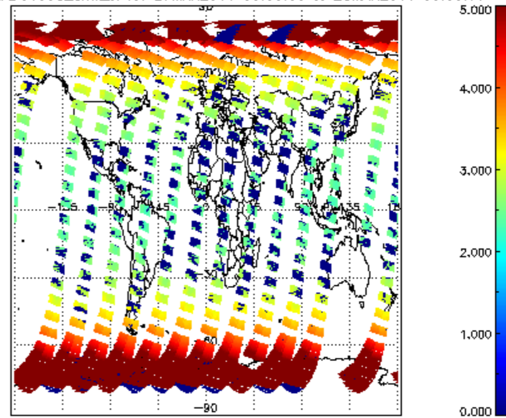
SCIOL2P_NADUV003_arnf_cl for 27MAR2011 00:00:00 to 28MAR2011 00:00:00
