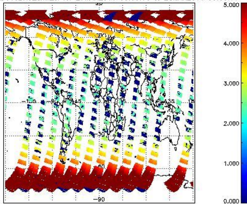
SCIOL2P_NADUV3BRO_amf_cl for 27MAR2011 00:00:00 to 28MAR2011 00:00:00
