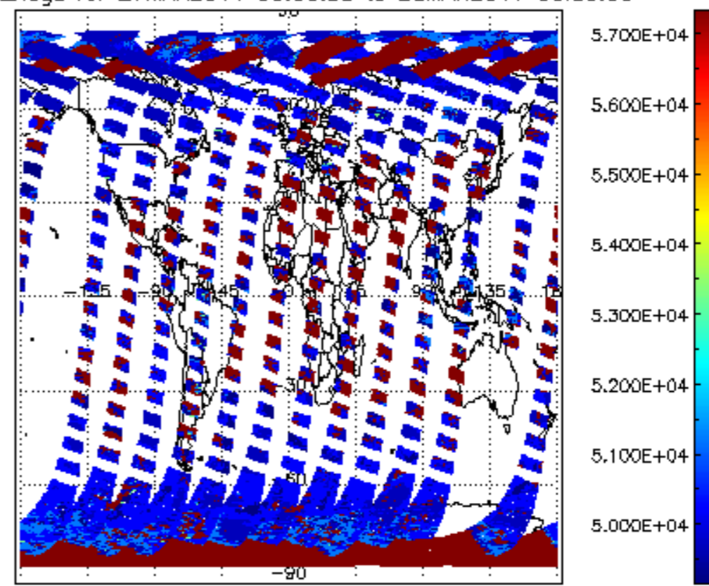
cloud_flags for 27MAR2011 00:00:00 to 28MAR2011 00:00:00
