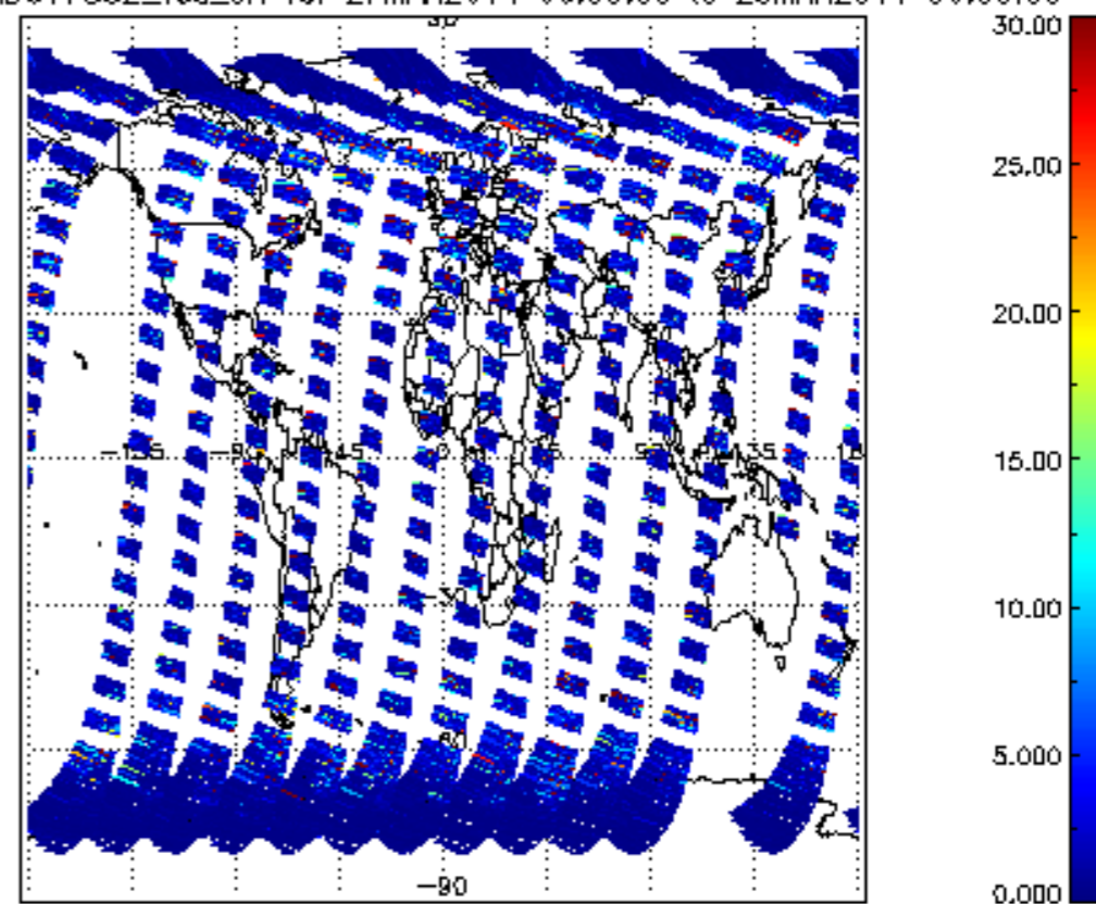
SCIOL2P_NADUV7S02_vcd_err for 27MAR2011 00:00:00 to 28MAR2011 00:00:00
