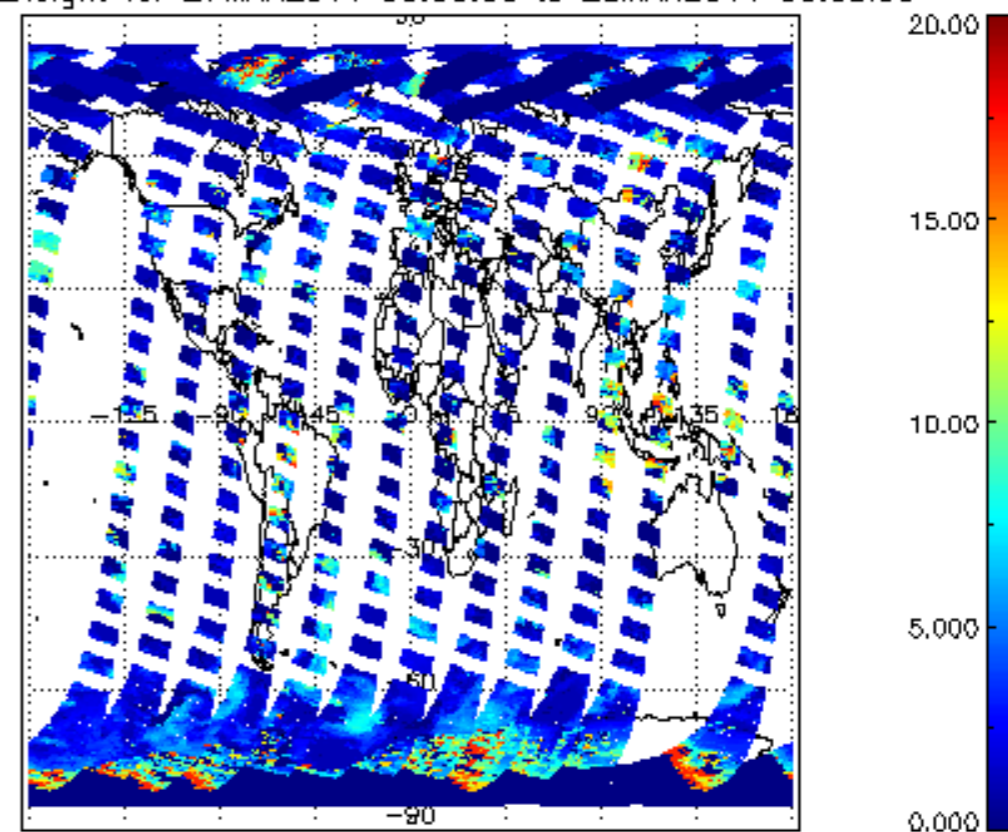
cL_top_height for 27MAR2011 00:00:00 to 28MAR2011 00:00:00
