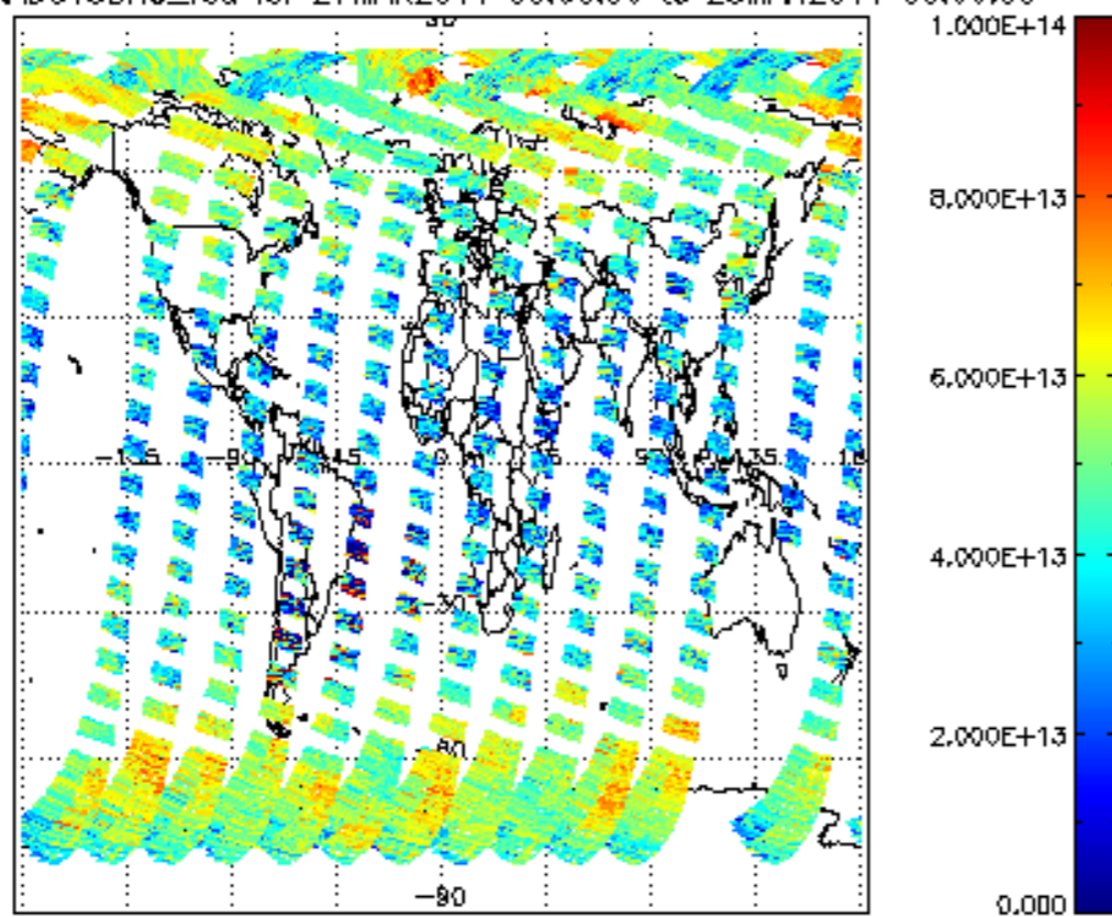
SCIOL2P_NADUV3BRO_vcd for 27MAR2011 00:00:00 to 28MAR2011 00:00:00
