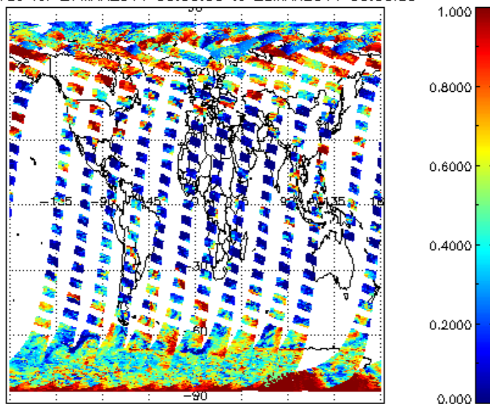
cL_frac for 27MAR2011 00:00:00 to 28MAR2011 00:00:00
