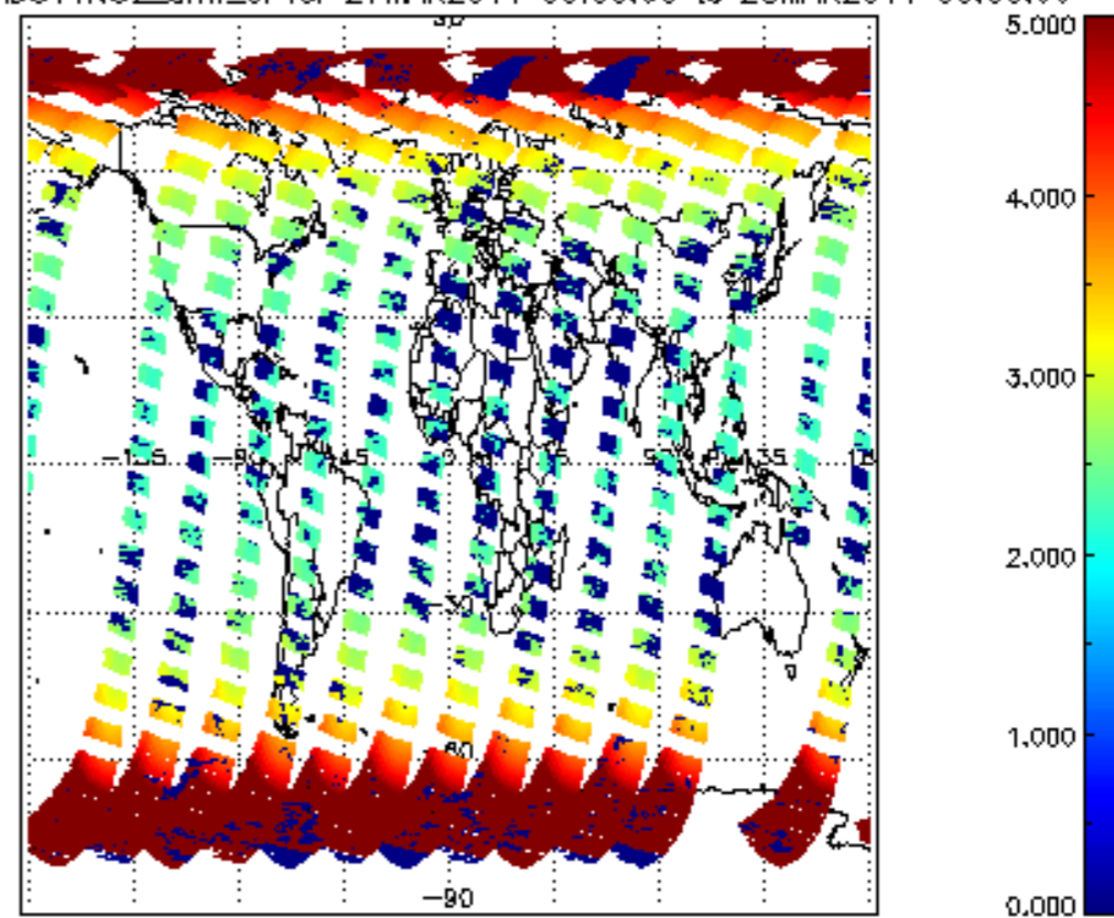
SCIOL2P_NADUV1NO2_amf_cl for 27MAR2011 00:00:00 to 28MAR2011 00:00:00
