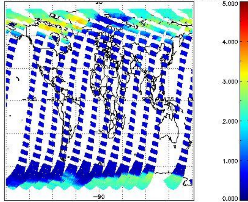
SCIOL2P_NADUV5SO2_amf_gr for 27MAR2011 00:00:00 to 28MAR2011 00:00:00
