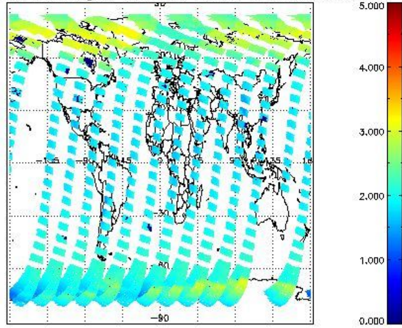
SCIOL2P_NADUV7S02_amf_gr for 27MAR2011 00:00:00 to 28MAR2011 00:00:00
