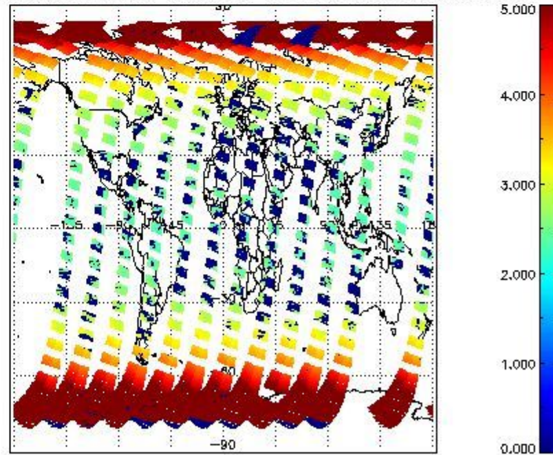
SCIOL2P_NADUV003_amf_cl for 27MAR2011 00:00:00 to 28MAR2011 00:00:00
