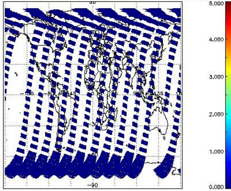
SCIOL2P_NADUV7S02_amf_cl for 27MAR2011 00:00:00 to 28MAR2011 00:00:00
