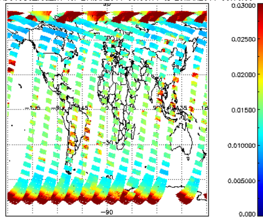
SCIOL2P_NADUV003_vcd_err for 27MAR2011 00:00:00 to 28MAR2011 00:00:00
