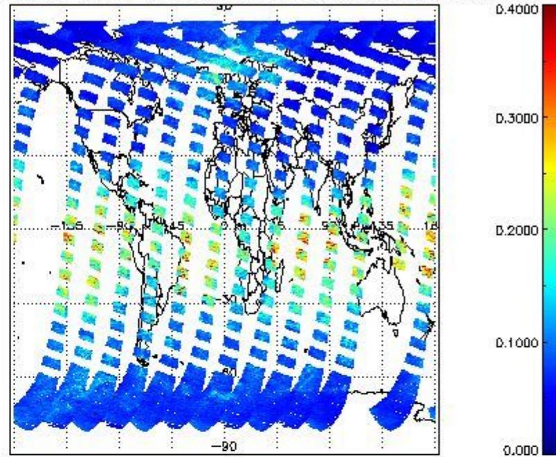
SCIOL2P_NADUV1NO2_vcd_err for 27MAR2011 00:00:00 to 26MAR2011 00:00:00
