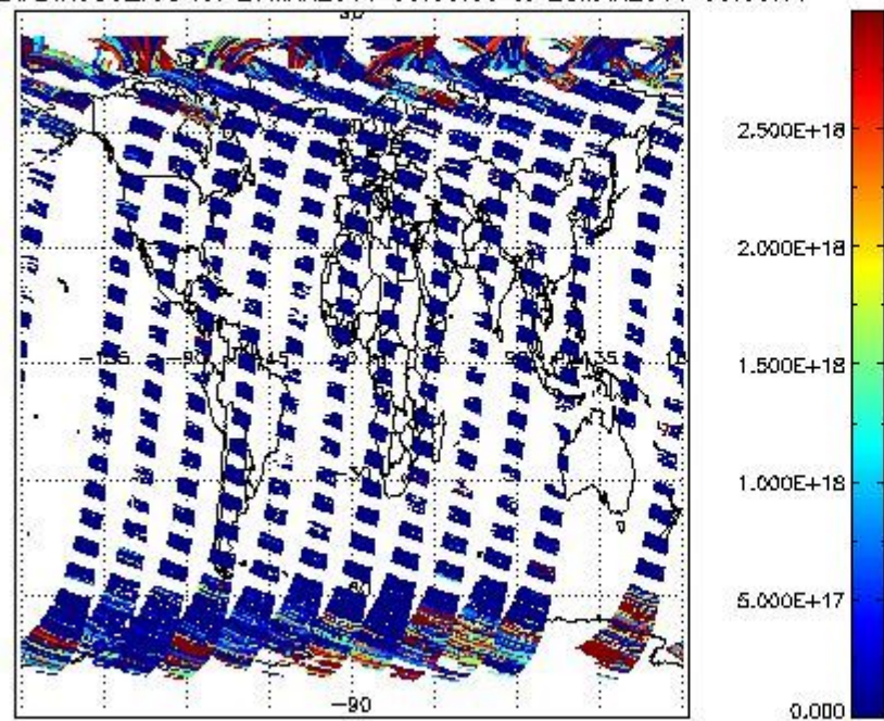
SCIO2P_NADIR3CO_vcd for 27MAR2011 00:00:00 to 28MAR2011 00:00:00
