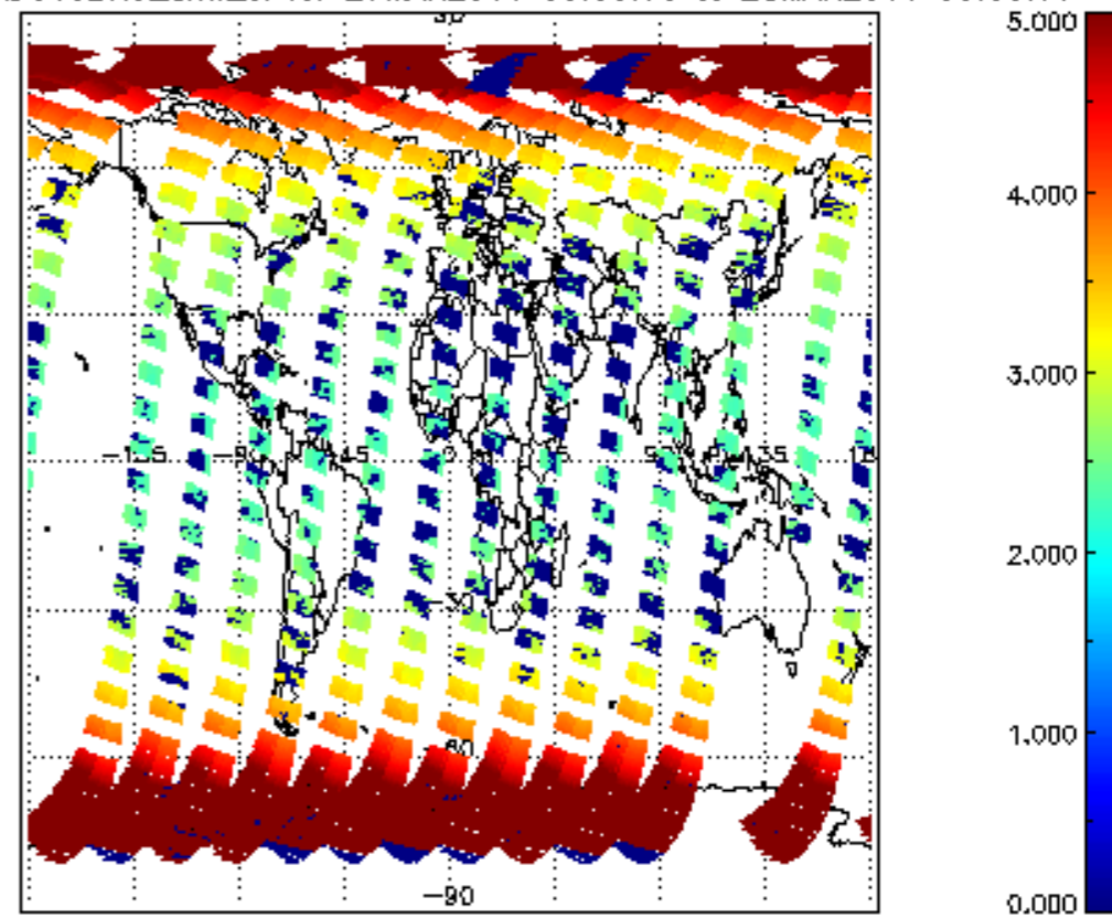
SCIOL2P_NADUV3BRO_amf_cl for 27MAR2011 00:00:00 to 28MAR2011 00:00:00
