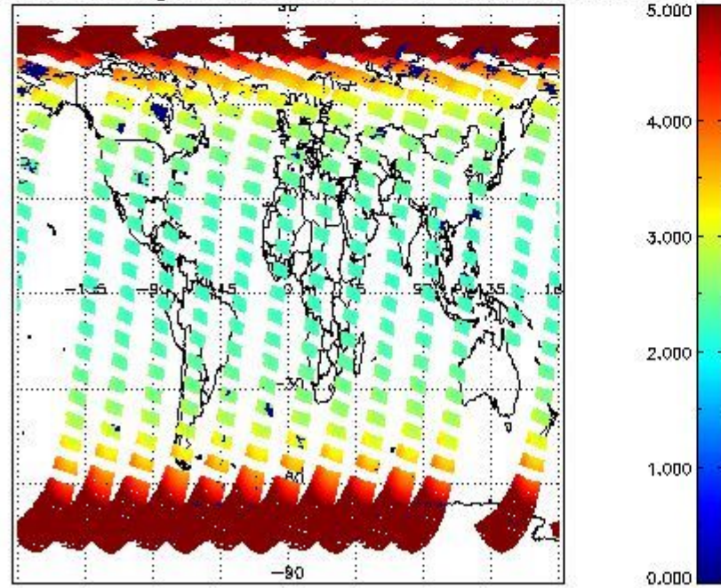
SCIOL2P_NADUV1NO2_amf_gr for 27MAR2011 00:00:00 to 28MAR2011 00:00:00
