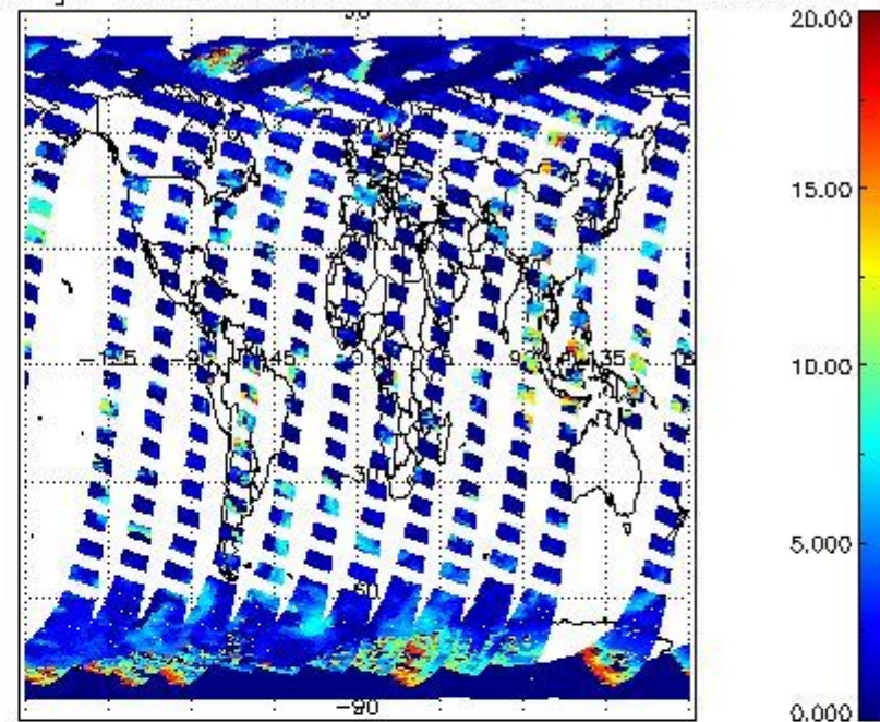
cL_top_height for 27MAR2011 00:00:00 to 28MAR2011 00:00:00
