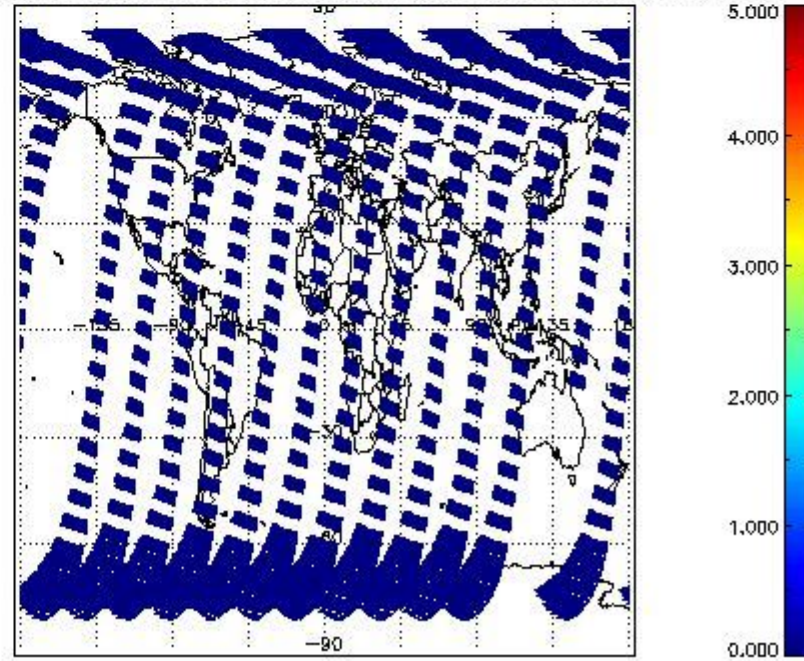
SCIOL2P_NADUV5SO2_amf_cl for 27MAR2011 00:00:00 to 28MAR2011 00:00:00
