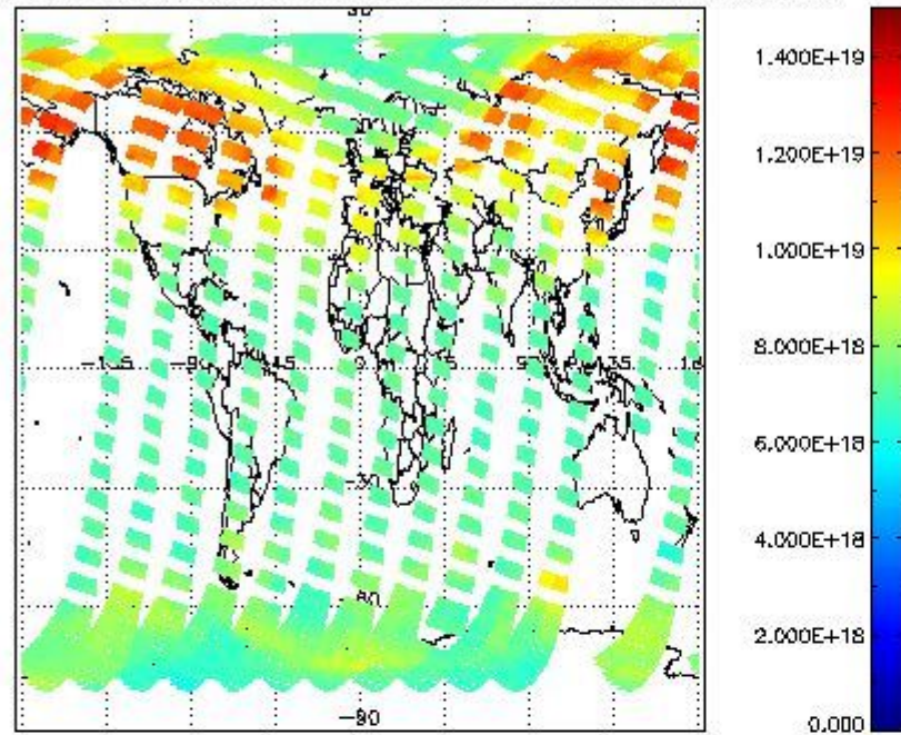
SCIOL2P_NADUV003_vcd for 27MAR2011 00:00:00 to 28MAR2011 00:00:00
