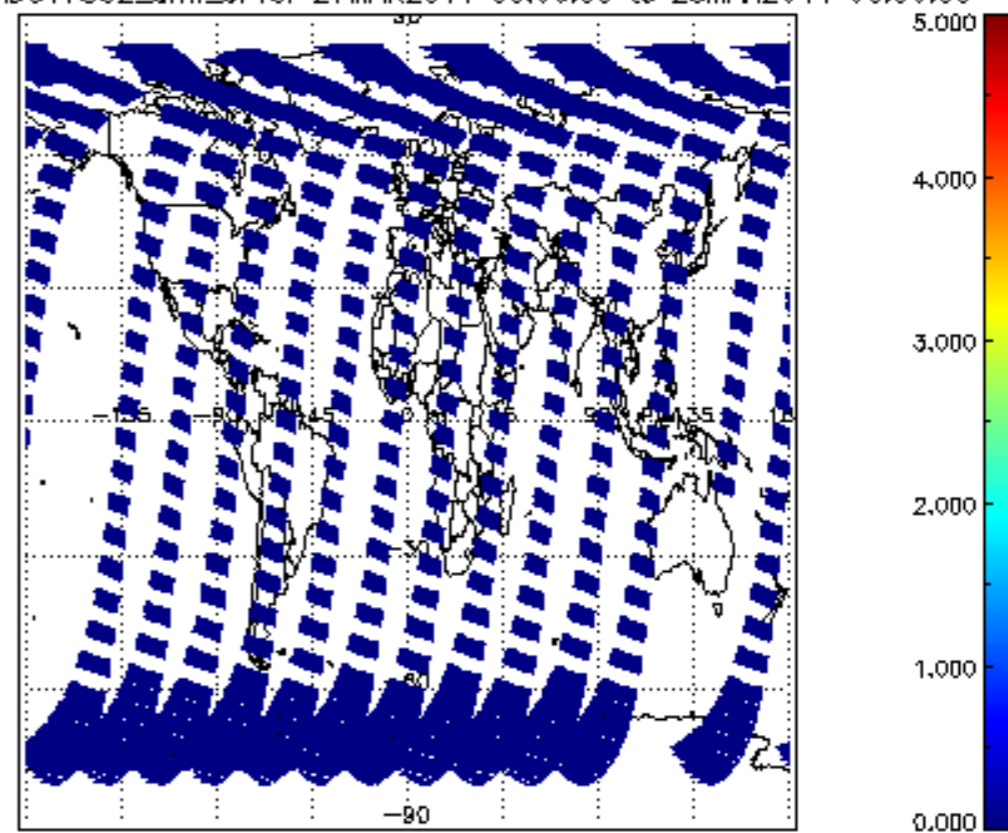
SCIOL2P_NADUV7S02_amf_cl for 27MAR2011 00:00:00 to 28MAR2011 00:00:00
