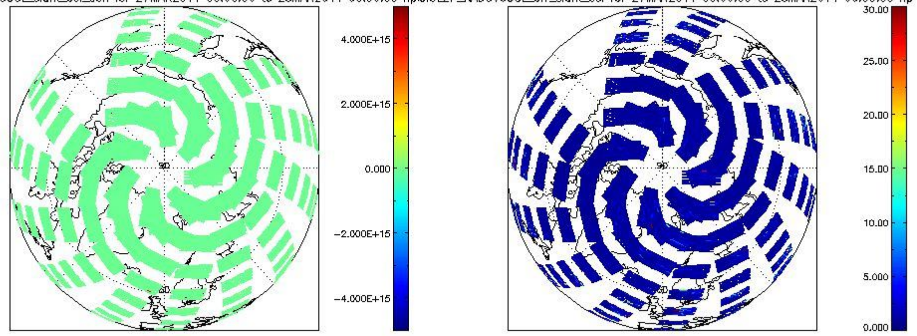
CIOL2P_NADUV6OCL_slant_col_den for 27MAR2011 00:00:00 to 28MAR2011 00:00:00 np CIOL2P_NADUV6OCL_err_slant_col for 27MAR2011 00:00:00 to 28MAR2011 00:00:00 np
