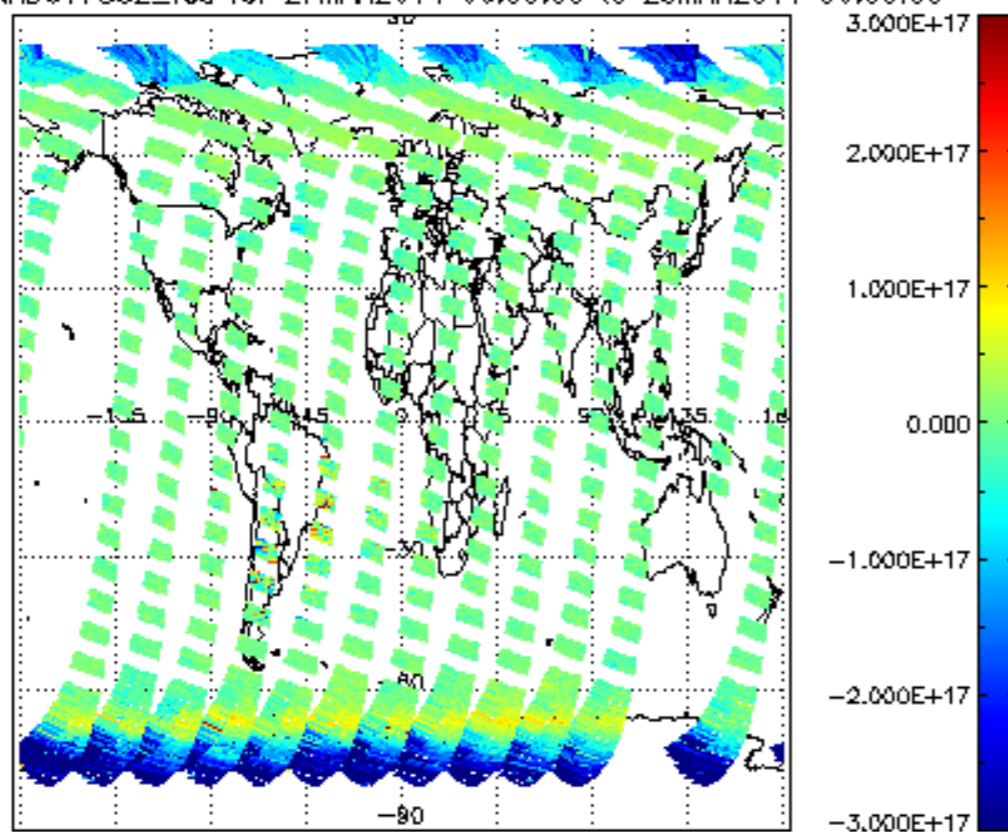
SCIOL2P_NADUV7S02_vcd for 27MAR2011 00:00:00 to 28MAR2011 00:00:00
