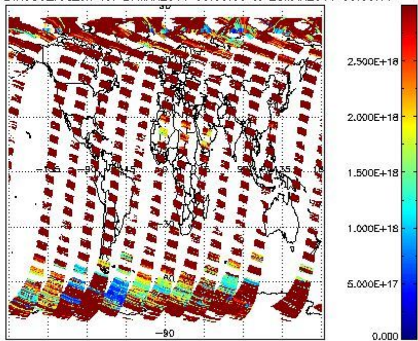
SCIO2P_NADIR3CO_vcd_err for 27MAR2011 00:00:00 to 28MAR2011 00:00:00
