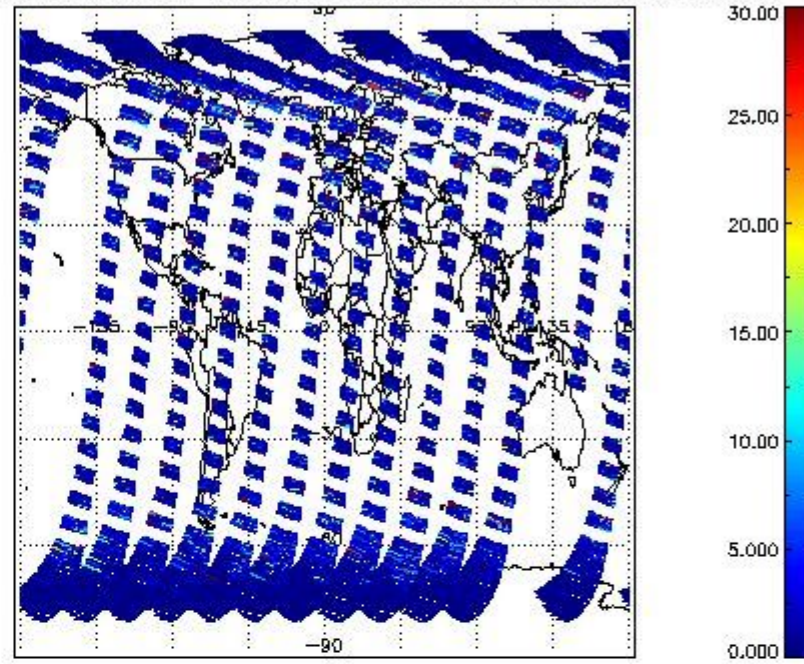
SCIOL2P_NADUV5SO2_vcd_err for 27MAR2011 00:00:00 to 28MAR2011 00:00:00
