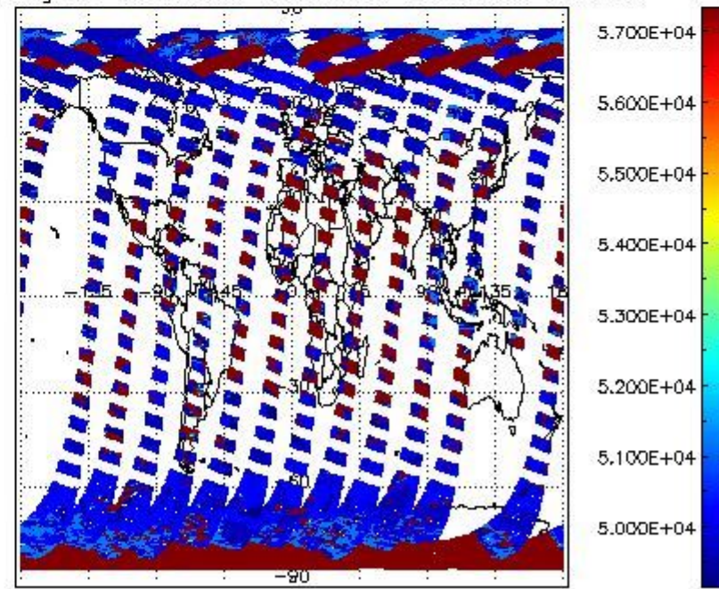
cloud_flags for 27MAR2011 00:00:00 to 28MAR2011 00:00:00
