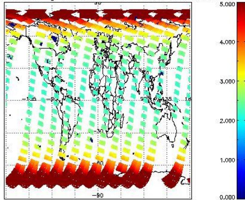
SCIOL2P_NADUV003_amf_gr for 27MAR2011 00:00:00 to 28MAR2011 00:00:00
