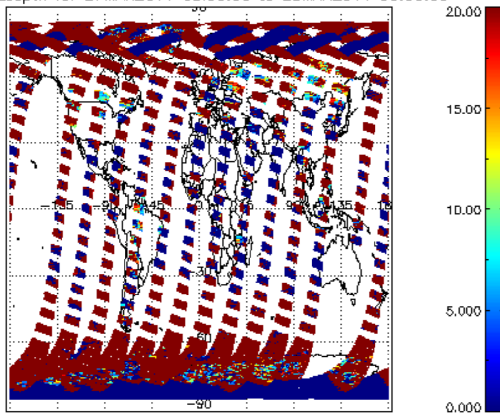
cL_opt_depth for 27MAR2011 00:00:00 to 28MAR2011 00:00:00
