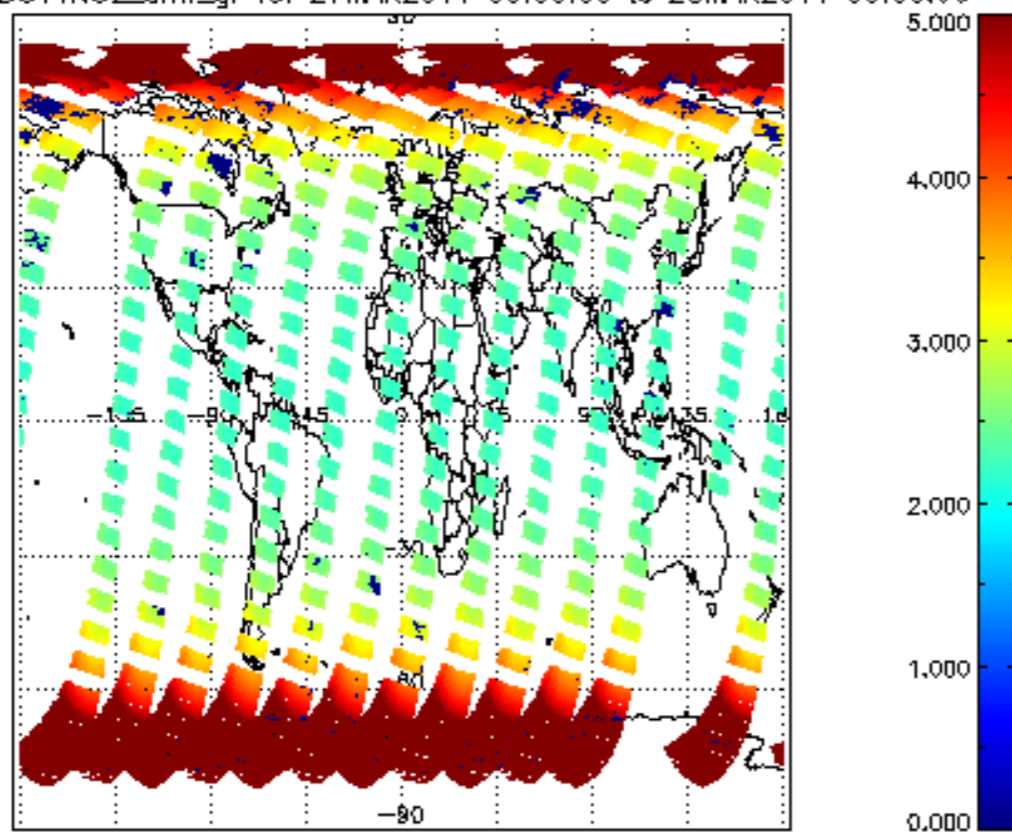
SCIOL2P_NADUV1NO2_amf_gr for 27MAR2011 00:00:00 to 28MAR2011 00:00:00
