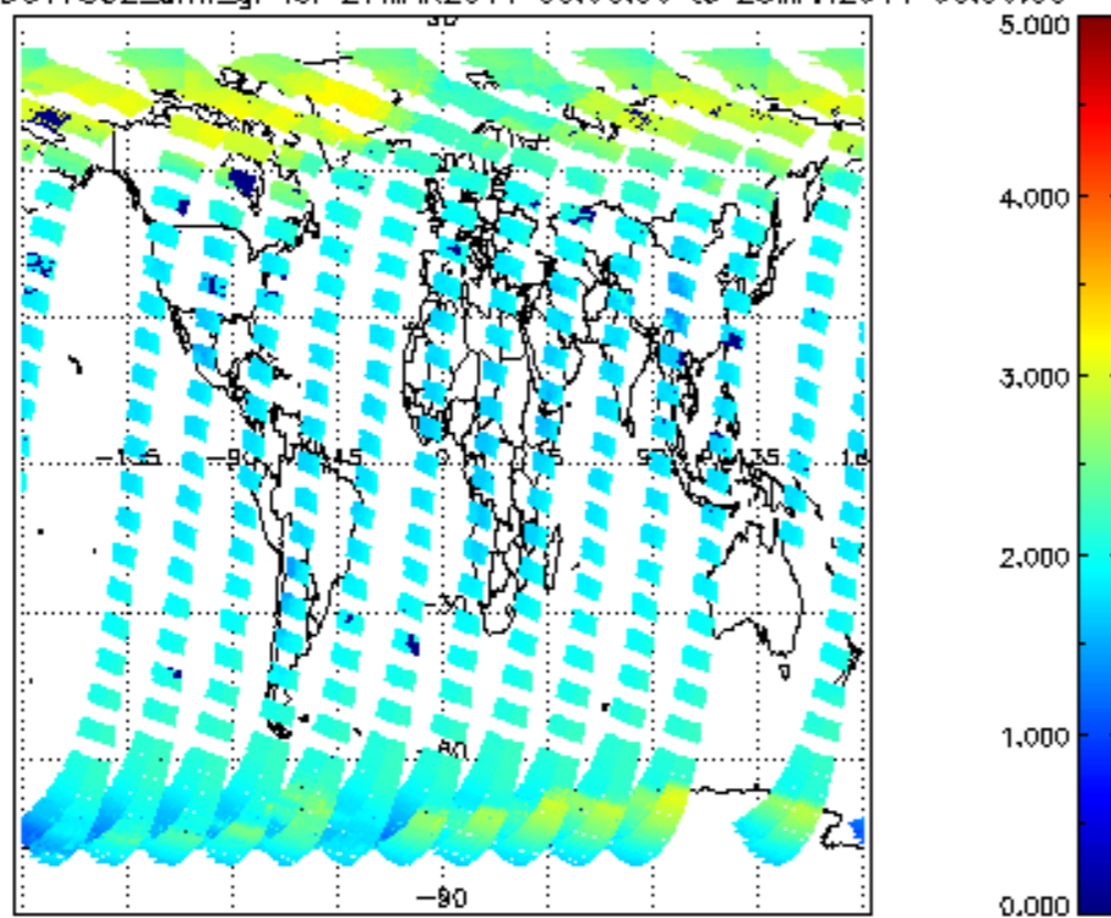
SCIOL2P_NADUV7S02_amf_gr for 27MAR2011 00:00:00 to 28MAR2011 00:00:00
