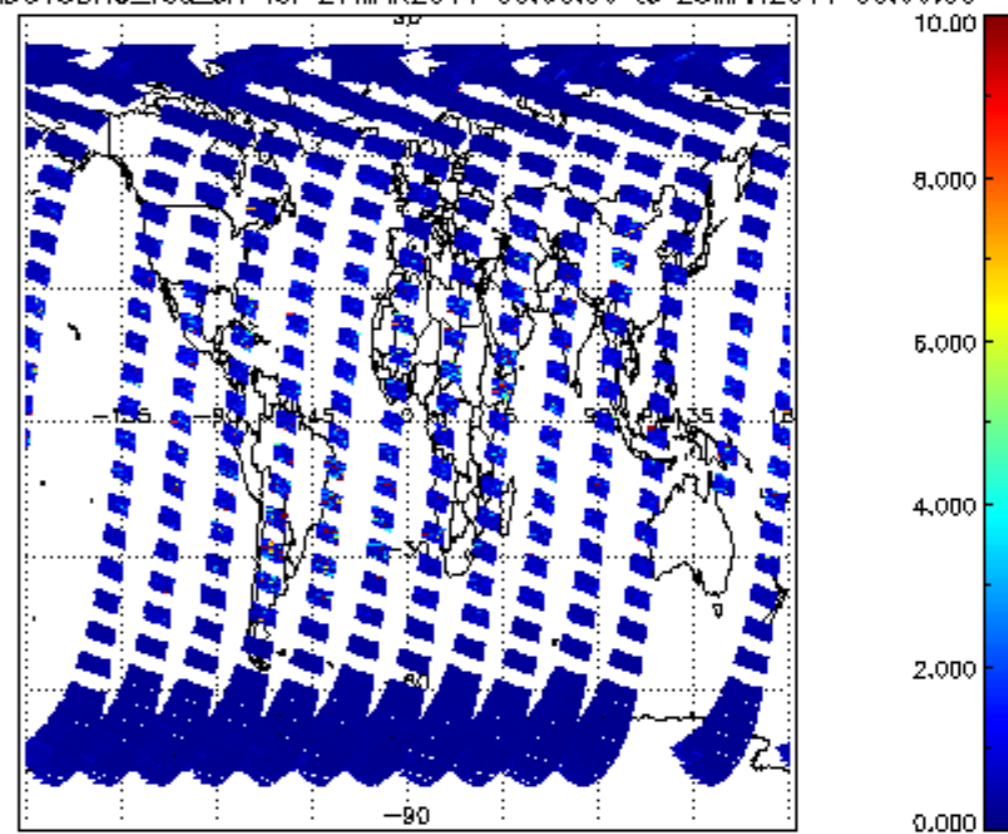
SCIOL2P_NADUV3BRO_vcd_err for 27MAR2011 00:00:00 to 28MAR2011 00:00:00
