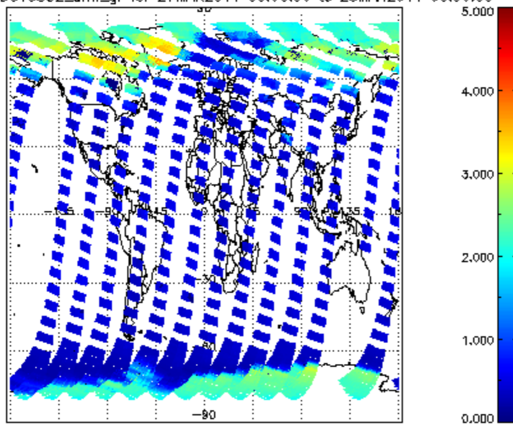
SCIOL2P_NADUV5S02_amf_gr for 27MAR2011 00:00:00 to 28MAR2011 00:00:00
