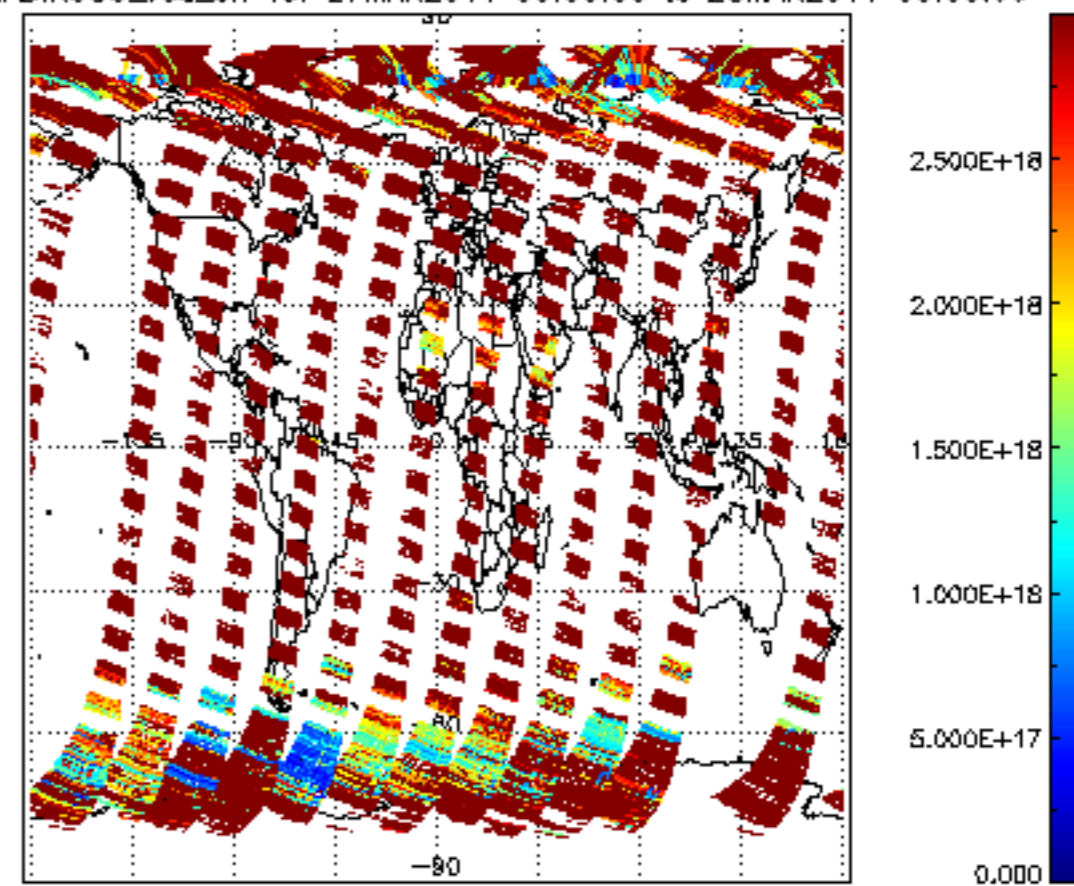
SCIOL2P_NADIR3CO_vcd_err for 27MAR2011 00:00:00 to 28MAR2011 00:00:00
