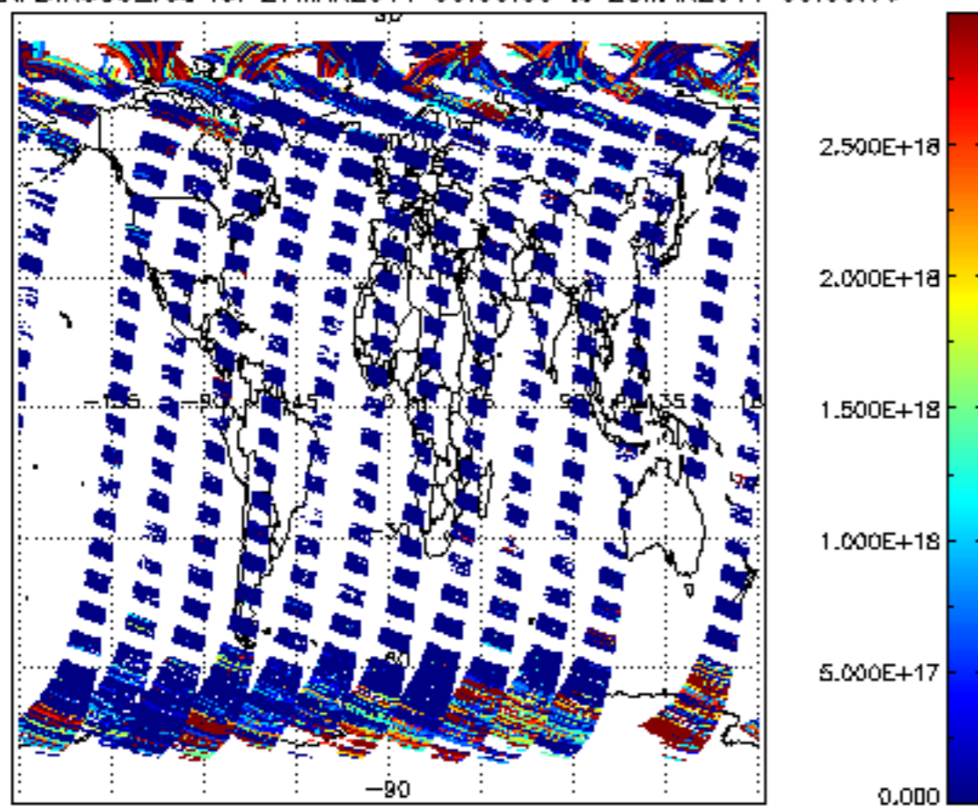
SCIOL2P_NADIR3CO_vcd for 27MAR2011 00:00:00 to 28MAR2011 00:00:00
