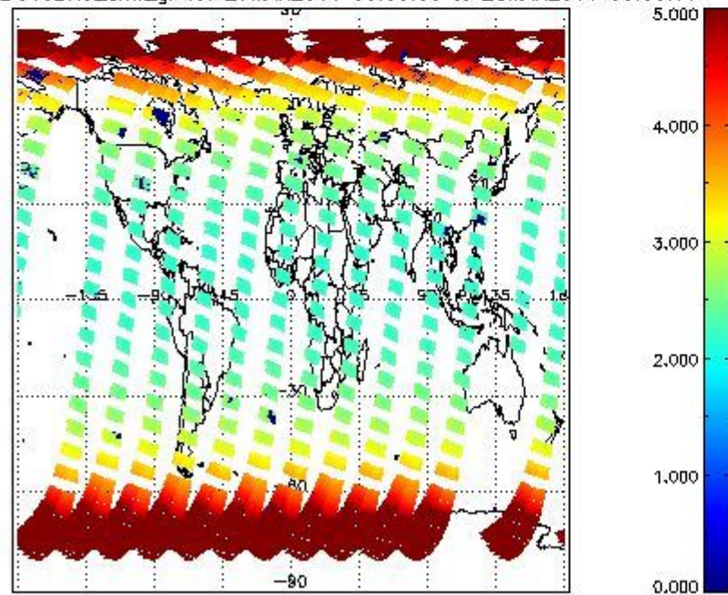
SCIOL2P_NADUV3BRO_amf_gr for 27MAR2011 00:00:00 to 28MAR2011 00:00:00
