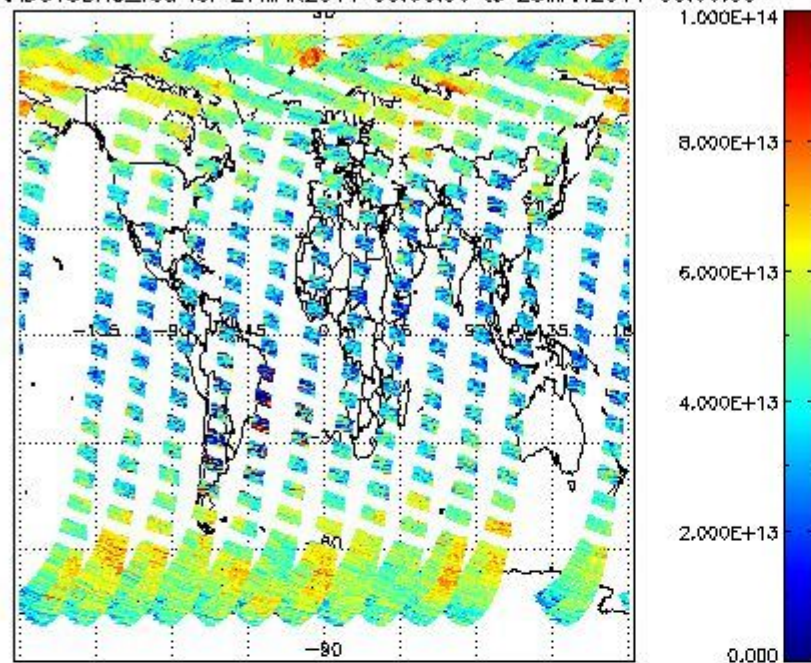
SCIOL2P_NADUV3BRO_vcd for 27MAR2011 00:00:00 to 26MAR2011 00:00:00
