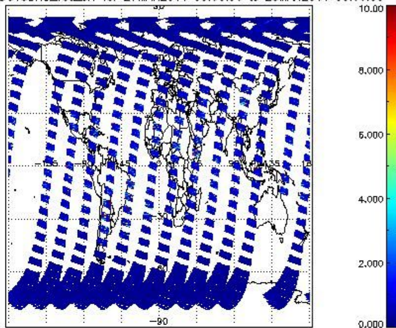
SCIOL2P_NADUV3BRO_vcd_err for 27MAR2011 00:00:00 to 26MAR2011 00:00:00
