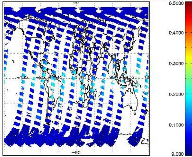
SCIOL2P_NADUV8H2O_vcd_err for 27MAR2011 00:00:00 to 28MAR2011 00:00:00
