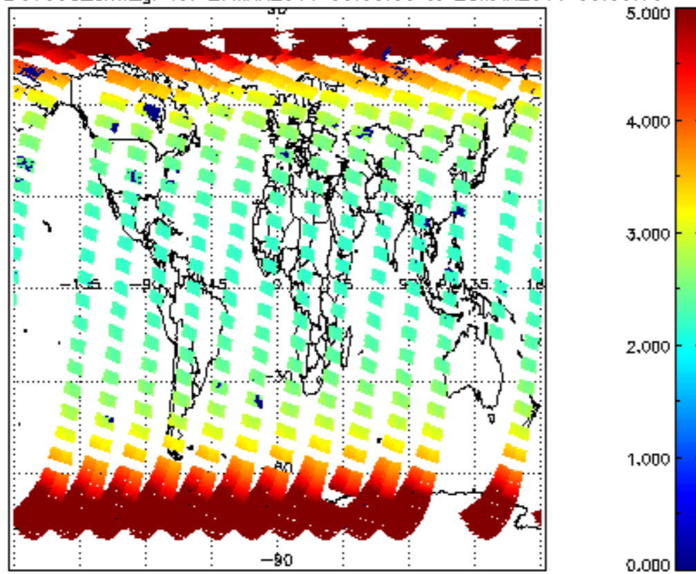
SCIOL2P_NADUV003_arnf_gr for 27MAR2011 00:00:00 to 28MAR2011 00:00:00
