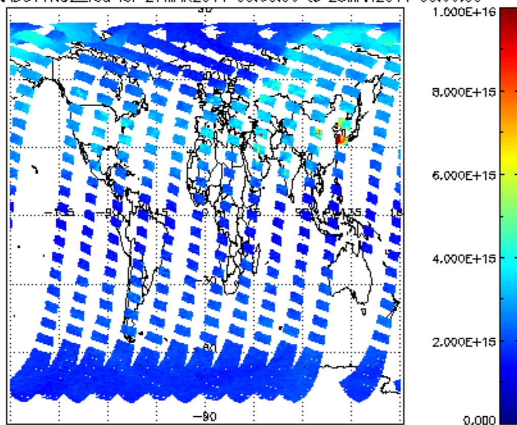
SCIOL2P_NADUV1NO2_vcd for 27MAR2011 00:00:00 to 28MAR2011 00:00:00
