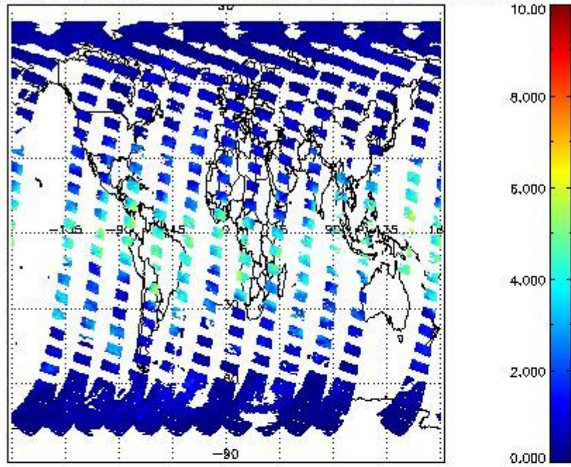
SCIOL2P_NADUV8H2O_vcd for 27MAR2011 00:00:00 to 28MAR2011 00:00:00
