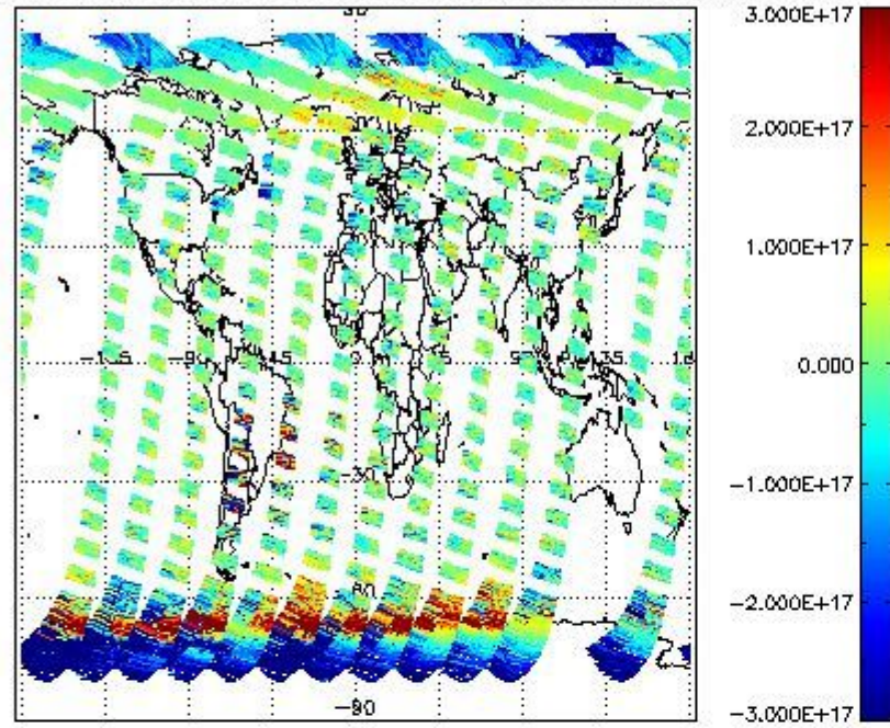
SCIOL2P_NADUV5SO2_vcd for 27MAR2011 00:00:00 to 28MAR2011 00:00:00
