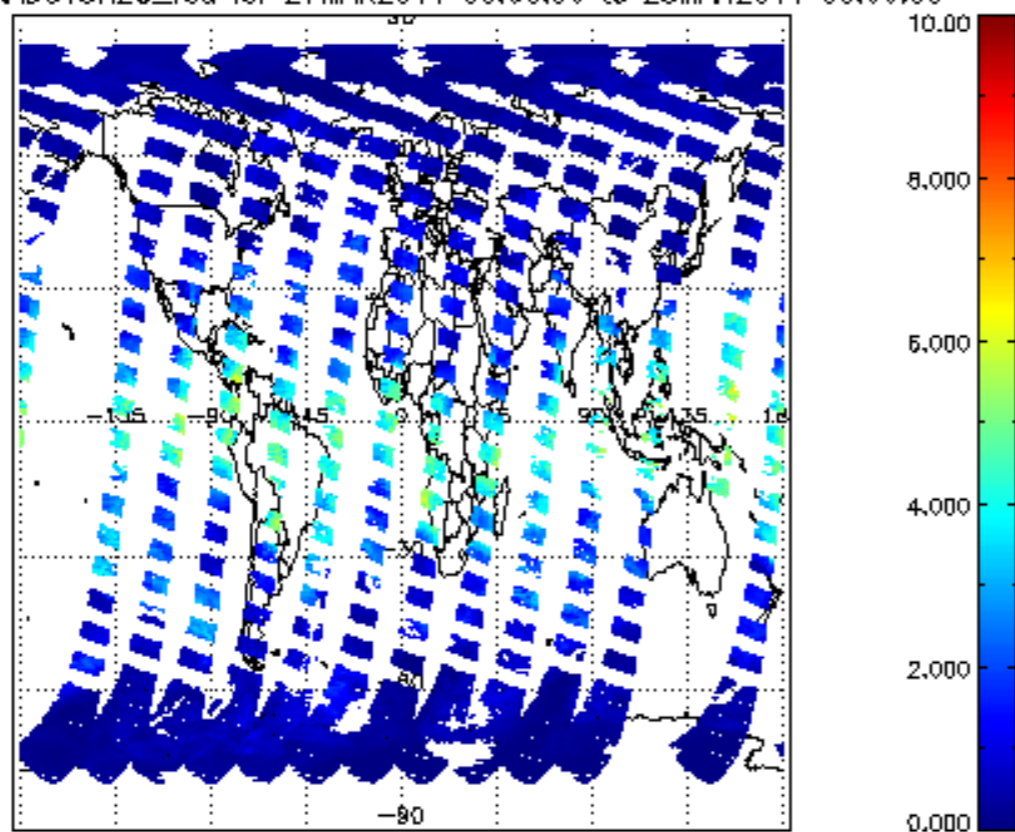
SCIOL2P_NADUV8H20_vcd for 27MAR2011 00:00:00 to 28MAR2011 00:00:00
