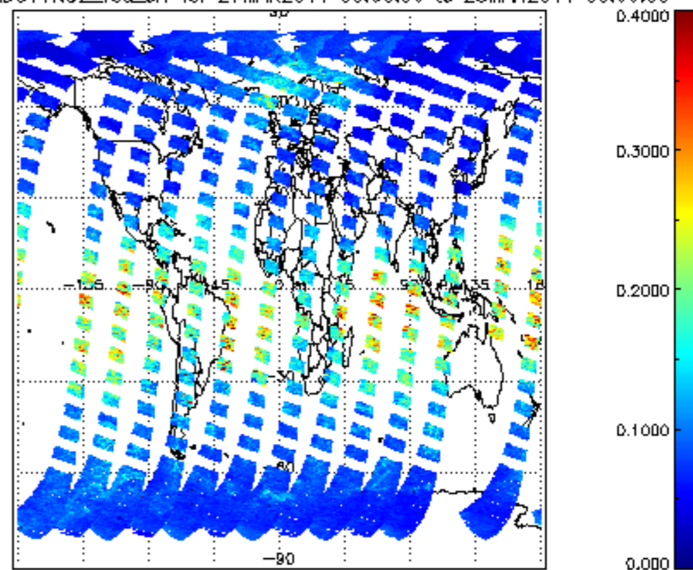
SCIOL2P_NADUV1NO2_vcd_err for 27MAR2011 00:00:00 to 28MAR2011 00:00:00
