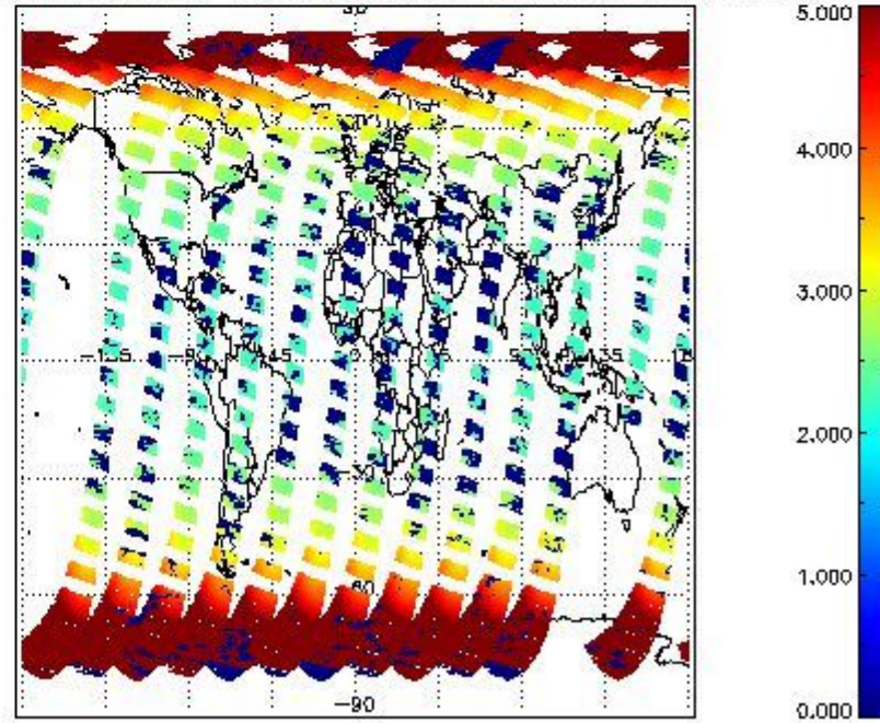
SCIOL2P_NADUV1NO2_amf_cl for 27MAR2011 00:00:00 to 28MAR2011 00:00:00
