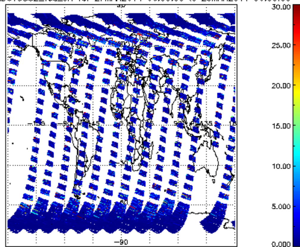
SCIOL2P_NADUV5S02_vcd_err for 27MAR2011 00:00:00 to 28MAR2011 00:00:00
