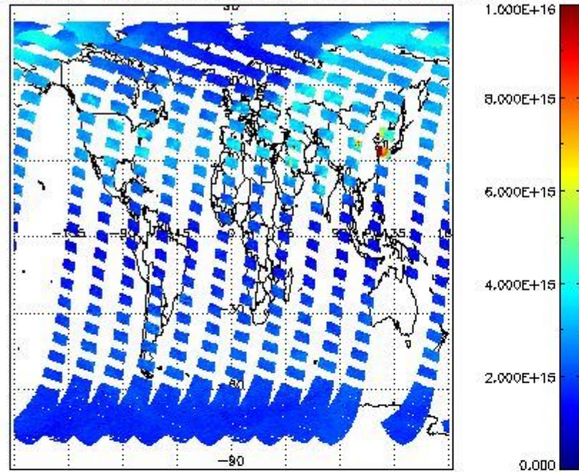
SCIOL2P_NADUV1NO2_vcd for 27MAR2011 00:00:00 to 26MAR2011 00:00:00
