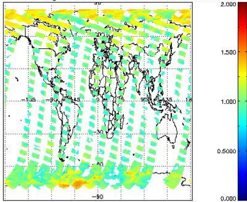
SCIOL2P_NADUV8H2O_amf_gr for 27MAR2011 00:00:00 to 28MAR2011 00:00:00
