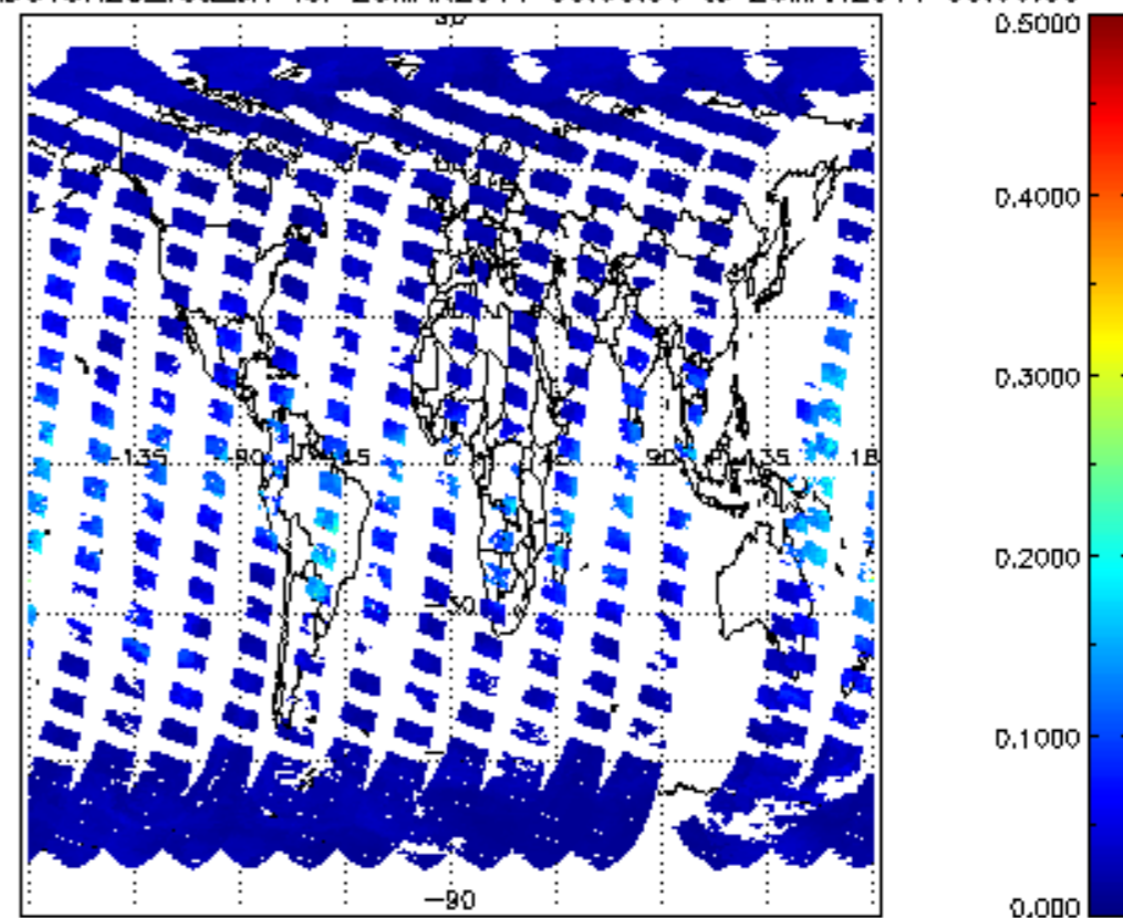
SCIOL2P_NADUV8H2O_vcd_err for 25MAR2011 00:00:00 to 26MAR2011 00:00:00
