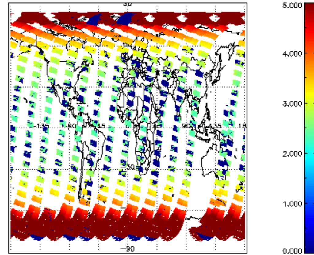
SCIOL2P_NADUV003_arnf_cl for 25MAR2011 00:00:00 to 26MAR2011 00:00:00
