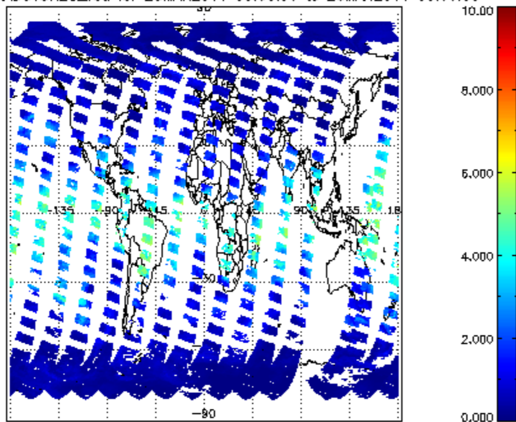
SCIOL2P_NADUV8H2O_vcd for 25MAR2011 00:00:00 to 26MAR2011 00:00:00
