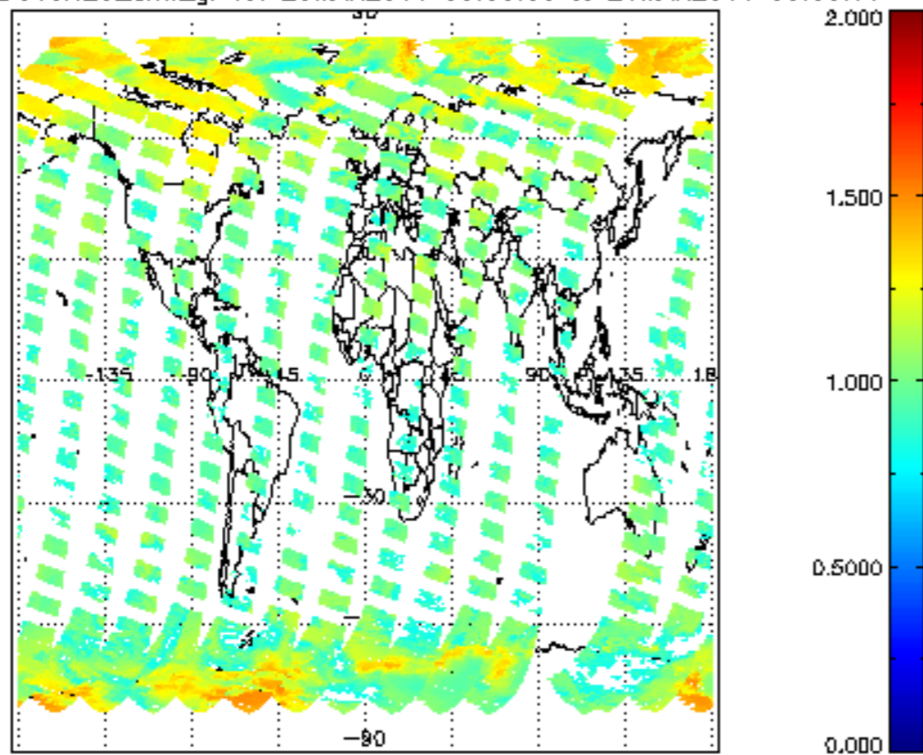
SCIOL2P_NADUV8H2O_arnf_gr for 25MAR2011 00:00:00 to 26MAR2011 00:00:00
