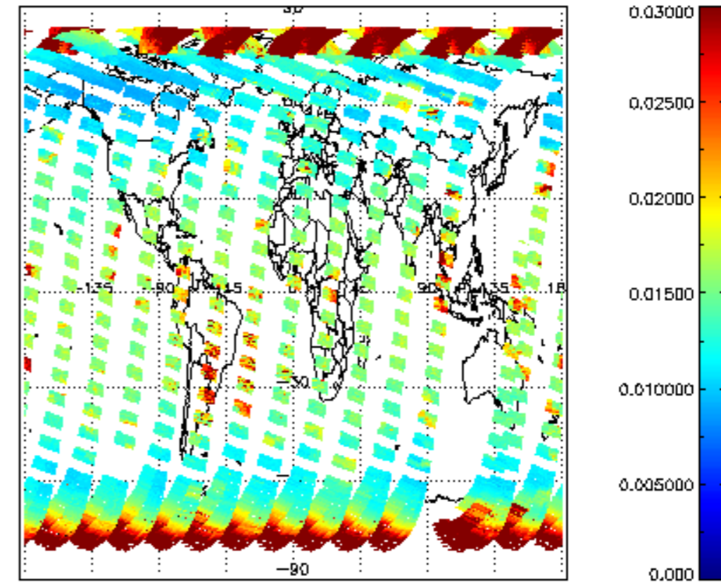
SCIOL2P_NADUV003_vcd_err for 25MAR2011 00:00:00 to 26MAR2011 00:00:00
