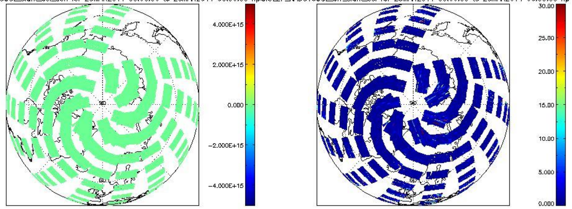
CIOL2P_NADUV6OCLslant_col_den for 25MAR2011 00:00:00 to 26MAR2011 00:00:00 np CIOL2P_NADUV6OCLerr_slant_col for 25MAR2011 00:00:00 to 26MAR2011 00:00:00 np
