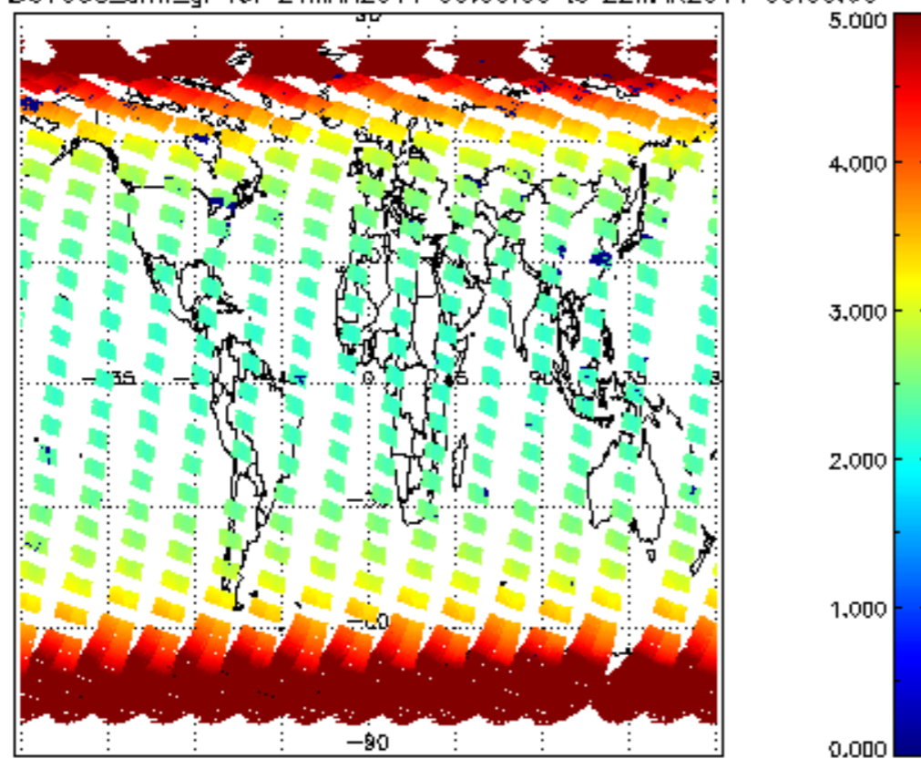
SCIOL2P_NADUV003_arnf_gr for 21MAR2011 00:00:00 to 22MAR2011 00:00:00
