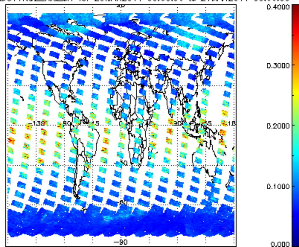
SCIOL2P_NADUV1NO2_vcd_Lerr for 20MAR2011 00:00:00 to 21MAR2011 00:00:00
