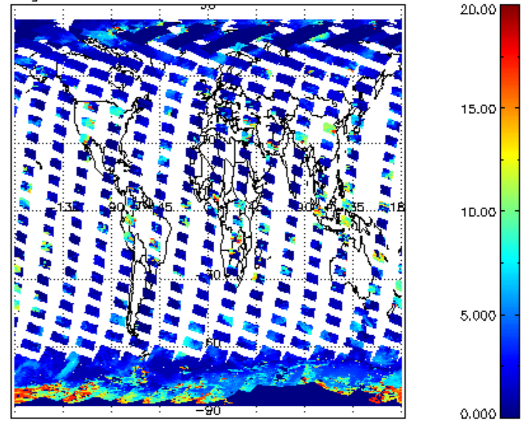
cL_top_height for 20MAR2011 00:00:00 to 21MAR2011 00:00:00
