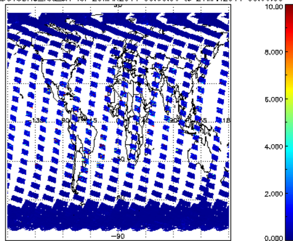
SCIOL2P_NADUV3BRO_vcd_err for 20MAR2011 00:00:00 to 21MAR2011 00:00:00
