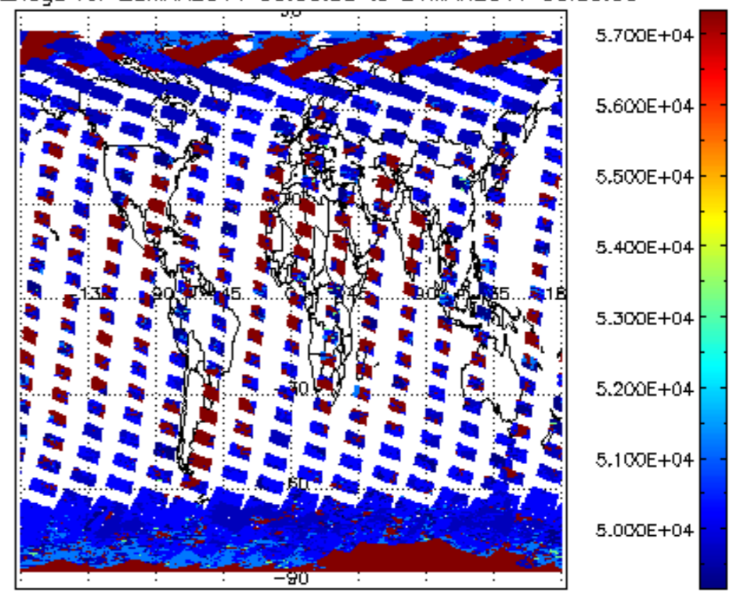
cloud_flags for 20MAR2011 00:00:00 to 21MAR2011 00:00:00
