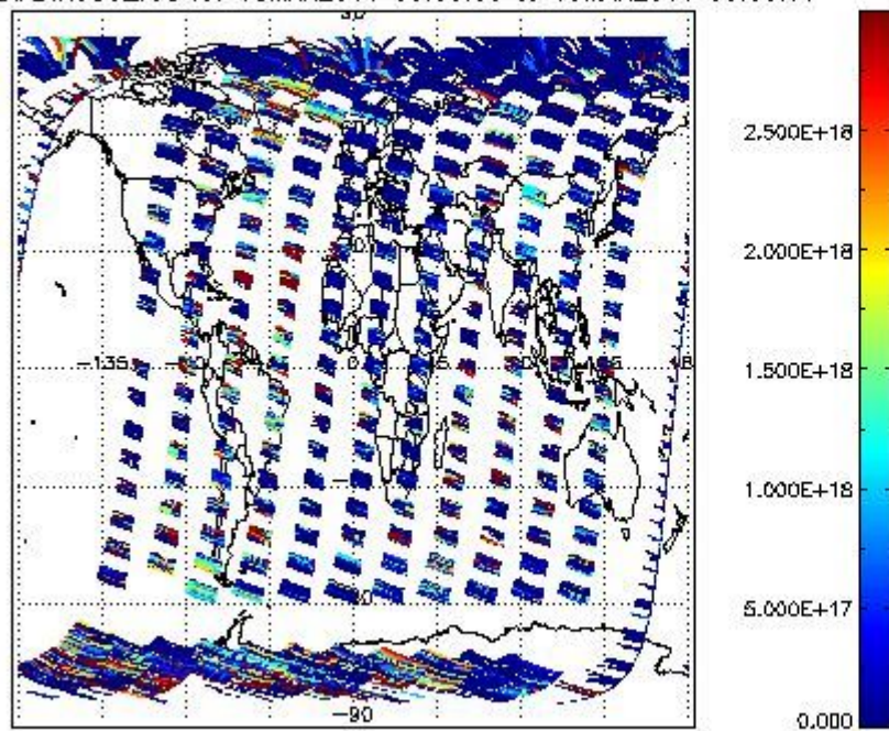
SCIDL2P_NADIR3CO_vcd for 18MAR2011 00:00:00 to 19MAR2011 00:00:00
