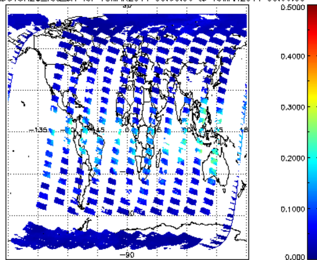
SCIOL2P_NADUV8H2O_vcd_err for 18MAR2011 00:00:00 to 19MAR2011 00:00:00
