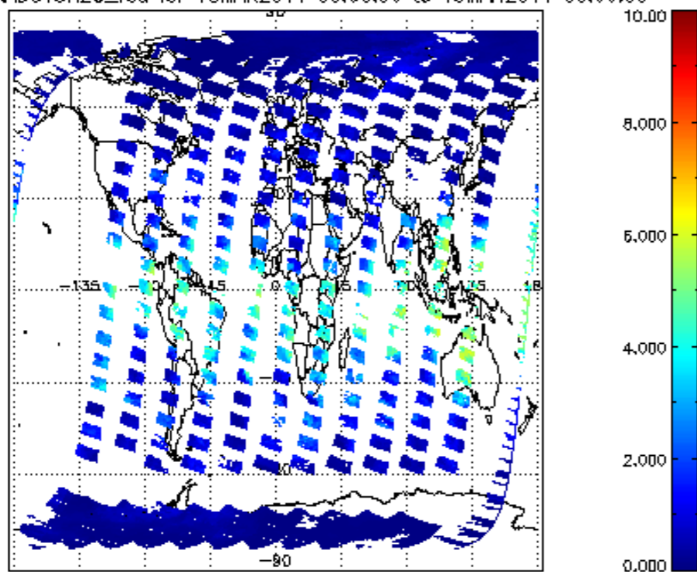
SCIOL2P_NADUV8H2O_vcd for 18MAR2011 00:00:00 to 19MAR2011 00:00:00
