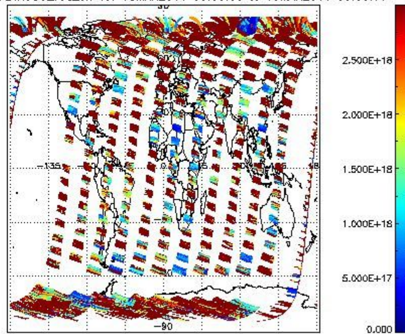
SCIDL2P_NADIR3CO_vcd_err for 18MAR2011 00:00:00 to 19MAR2011 00:00:00
