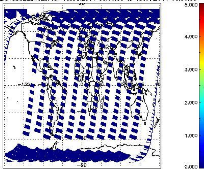
SCIOL2P_NADUV5S02_amf_cl for 18MAR2011 00:00:00 to 19MAR2011 00:00:00
