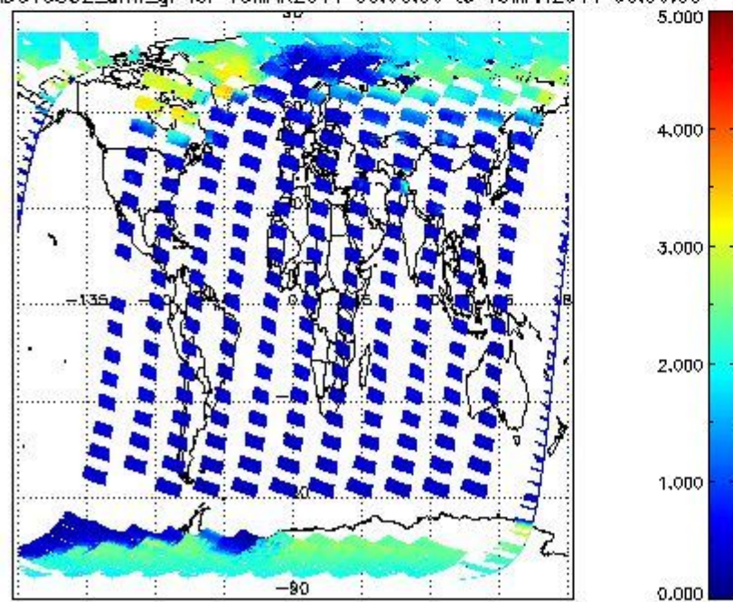
SCIOL2P_NADUV5S02_amf_gr for 18MAR2011 00:00:00 to 19MAR2011 00:00:00
