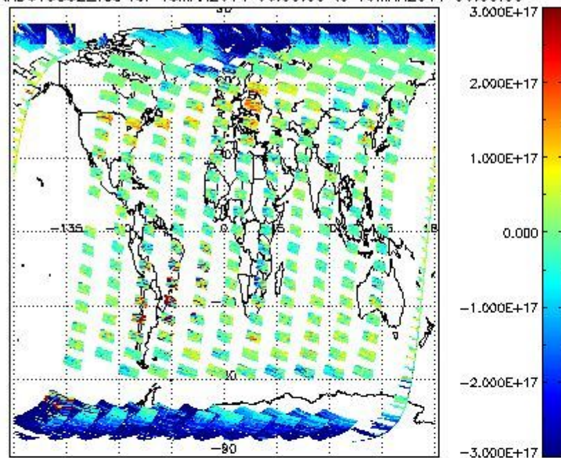
SCIOL2P_NADUV5S02_vcd for 18MAR2011 00:00:00 to 19MAR2011 00:00:00
