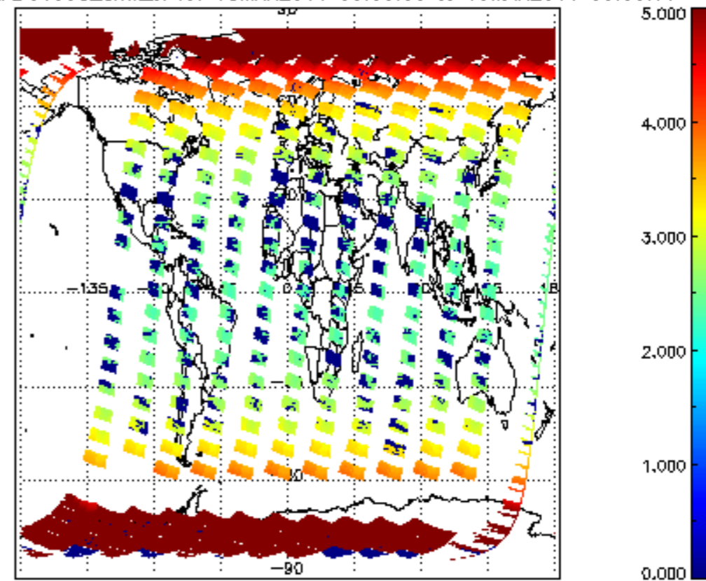
SCIOL2P_NADUV003_arnf_cl for 18MAR2011 00:00:00 to 19MAR2011 00:00:00
