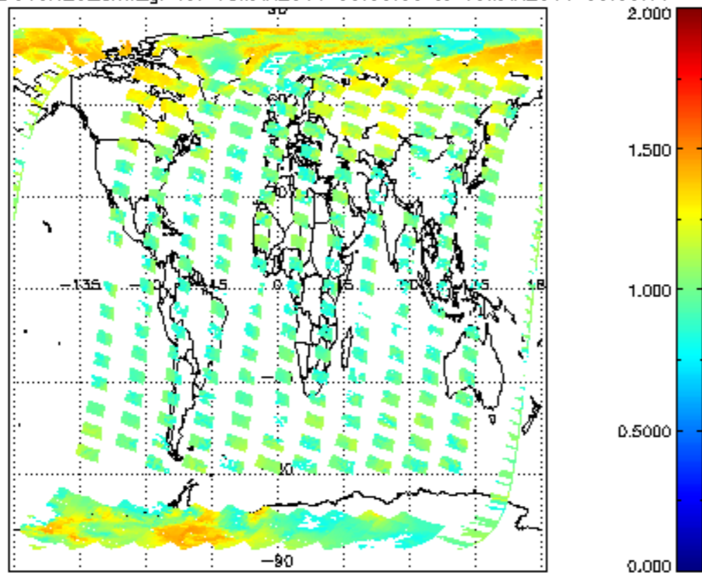
SCIOL2P_NADUV8H2O_arnf_gr for 18MAR2011 00:00:00 to 19MAR2011 00:00:00
