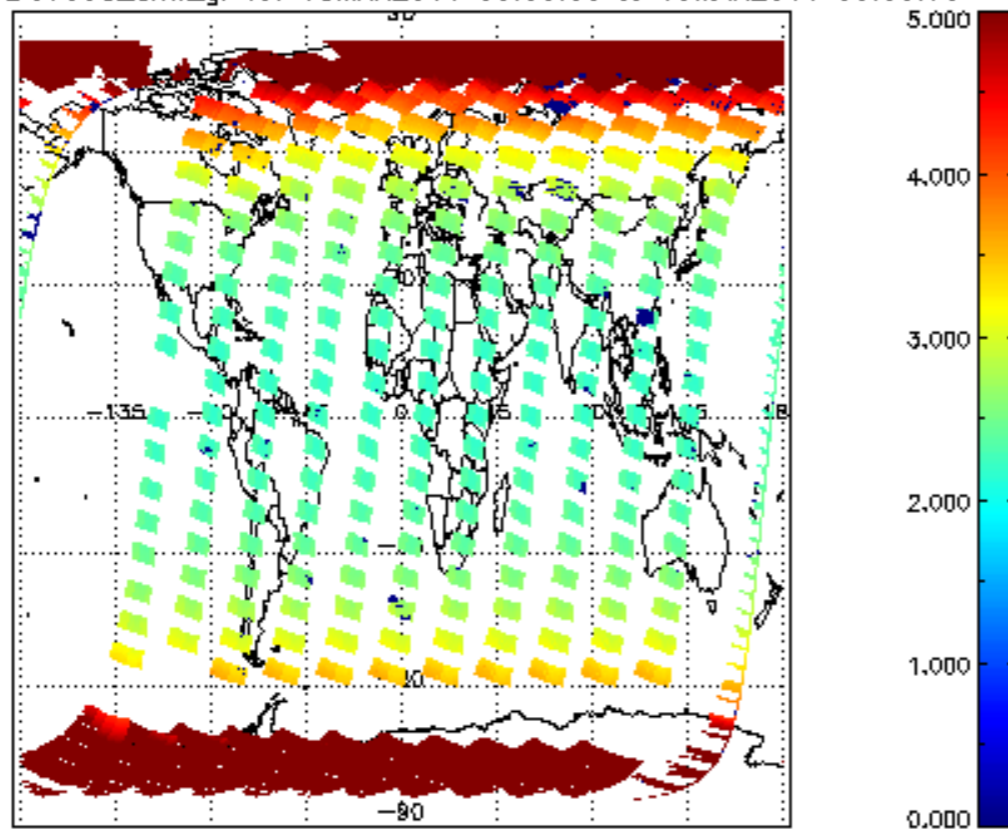
SCIOL2P_NADUV003_arnf_gr for 18MAR2011 00:00:00 to 19MAR2011 00:00:00
