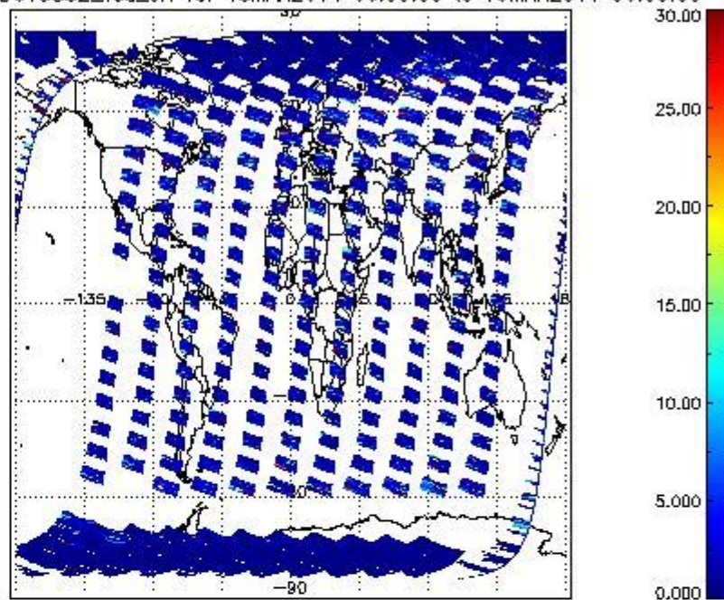
SCIOL2P_NADUV5S02_vcd_err for 18MAR2011 00:00:00 to 19MAR2011 00:00:00
