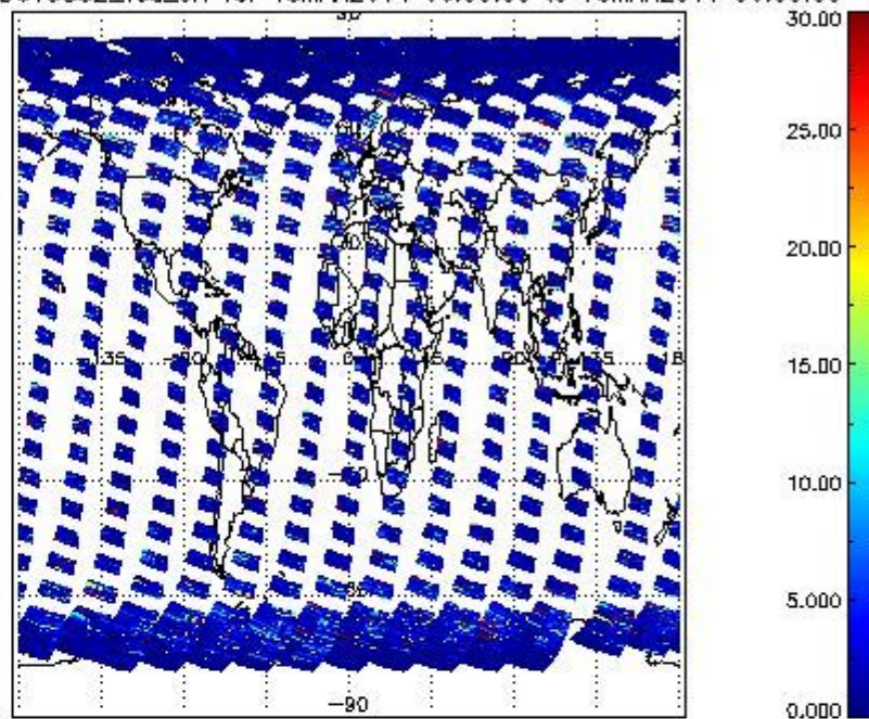
SCIOL2P_NADUV5SO2_vcd_err for 15MAR2011 00:00:00 to 16MAR2011 00:00:00
