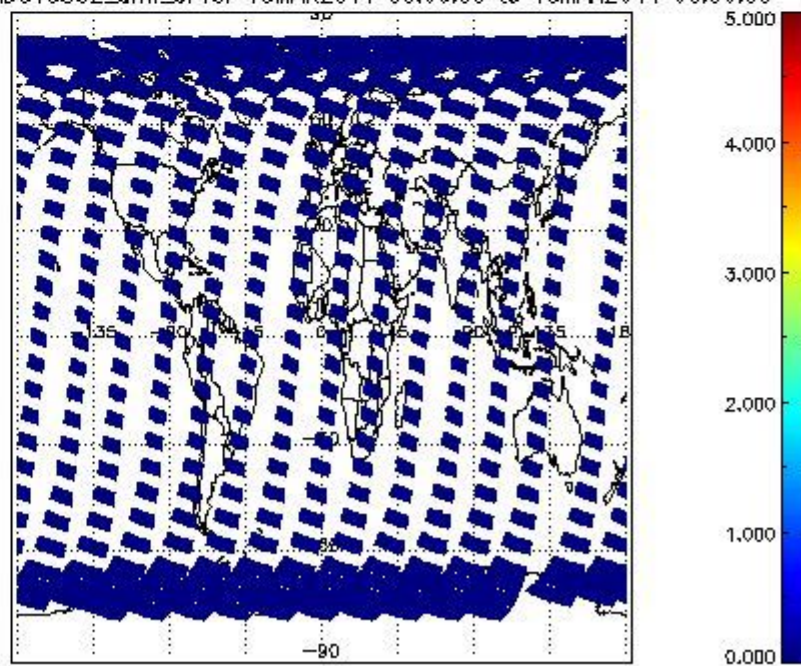
SCIOL2P_NADUV5SO2_amf_cl for 15MAR2011 00:00:00 to 16MAR2011 00:00:00
