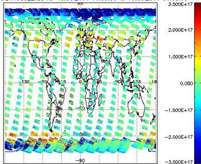
SCIOL2P_NADUV5SO2_vcd for 15MAR2011 00:00:00 to 16MAR2011 00:00:00
