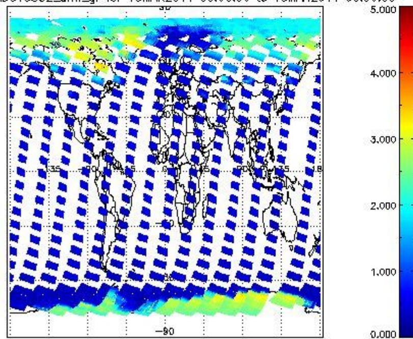
SCIOL2P_NADUV5SO2_amf_gr for 15MAR2011 00:00:00 to 16MAR2011 00:00:00
