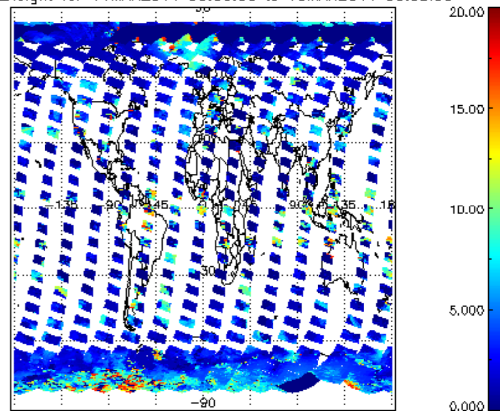
cL_top_height for 14MAR2011 00:00:00 to 15MAR2011 00:00:00
