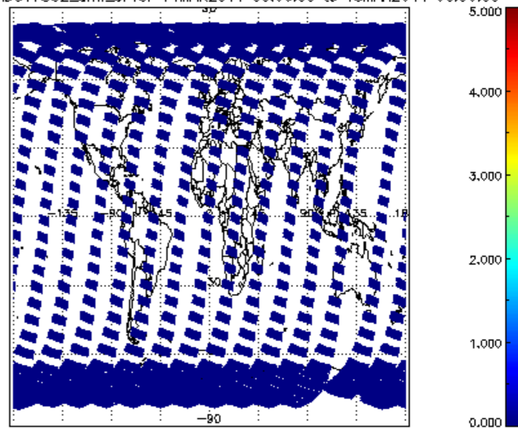
SCIOL2P_NADUV7S02_amf_cl for 14MAR2011 00:00:00 to 15MAR2011 00:00:00
