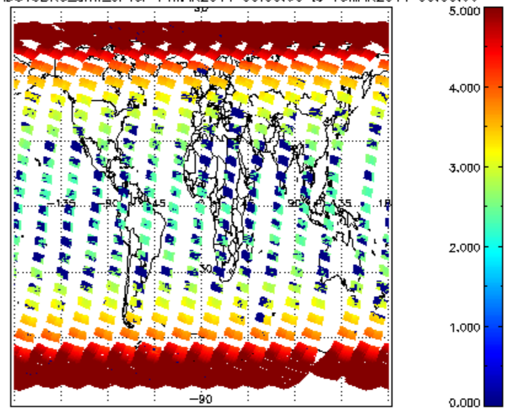
SCIOL2P_NADUV3BRO_arnf_cl for 14MAR2011 00:00:00 to 15MAR2011 00:00:00
