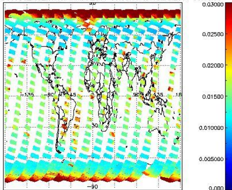
SCIOL2P_NADUV003_vcd_err for 14MAR2011 00:00:00 to 15MAR2011 00:00:00
