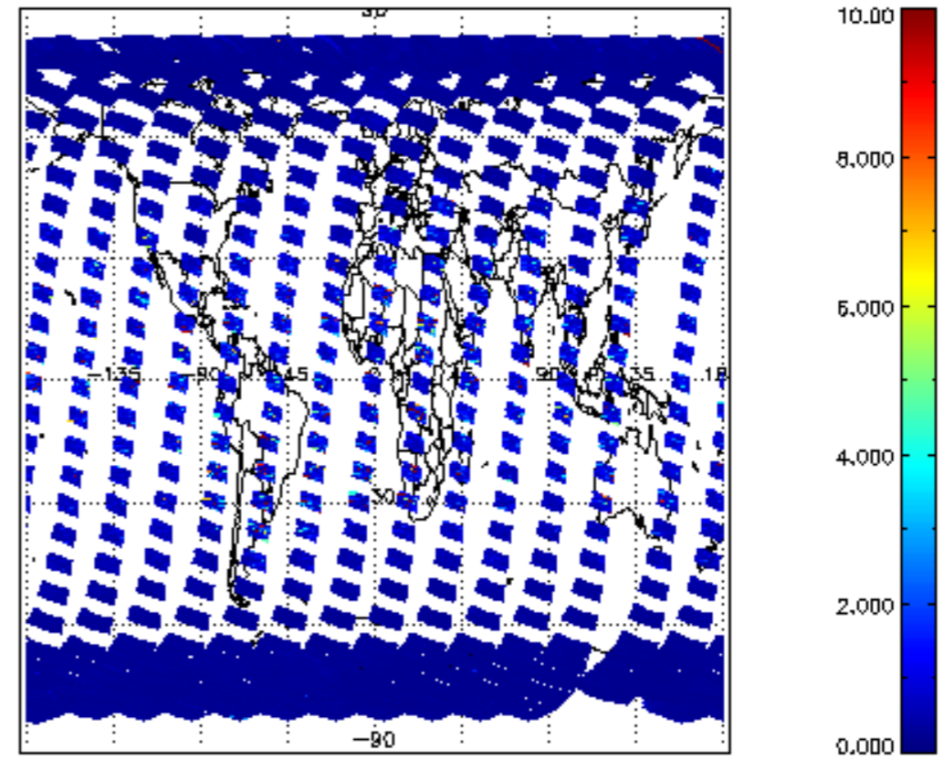
SCIOL2P_NADUV3BRO_vcd_Lerr for 14MAR2011 00:00:00 to 15MAR2011 00:00:00
