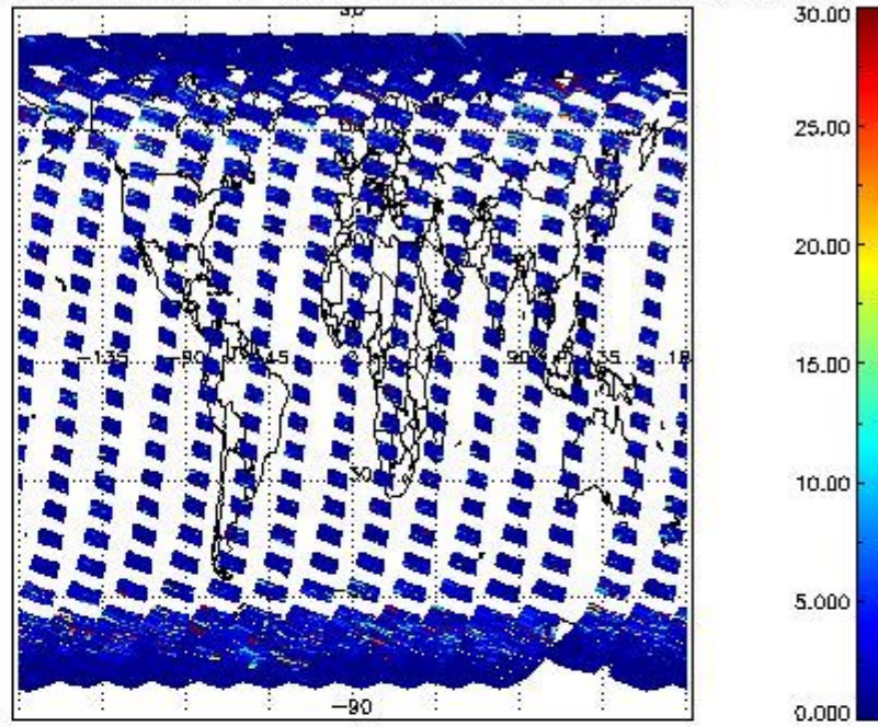
SCIOL2P_NADUV5SO2_vcd_err for 14MAR2011 00:00:00 to 15MAR2011 00:00:00
