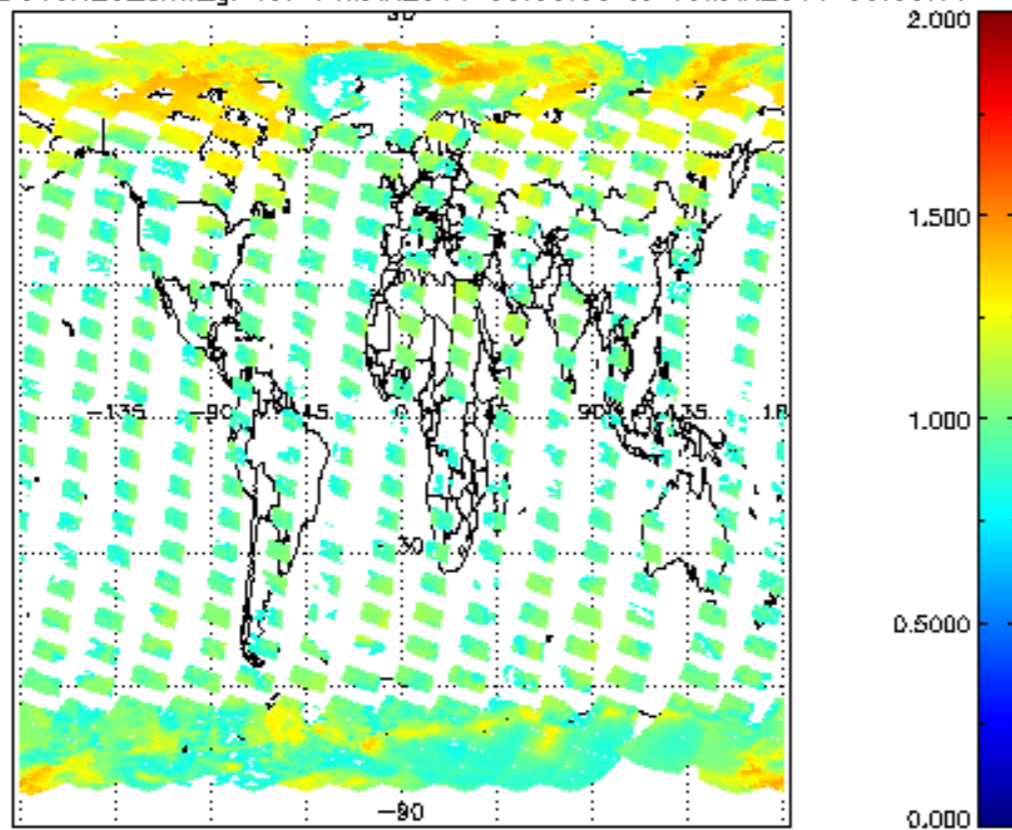
SCIOL2P_NADUV8H2O_arnf_gr for 14MAR2011 00:00:00 to 15MAR2011 00:00:00
