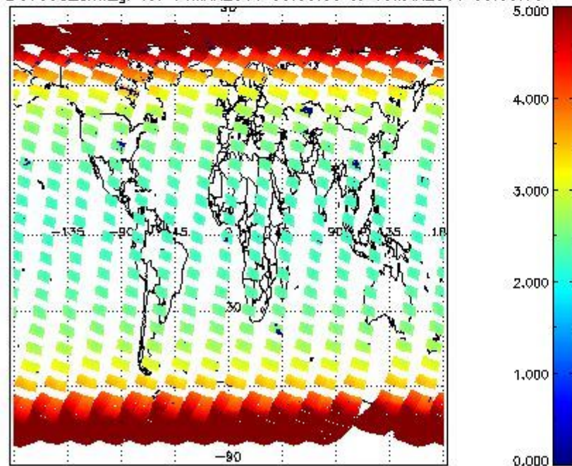
SCIOL2P_NADUV003_amf_gr for 14MAR2011 00:00:00 to 15MAR2011 00:00:00
