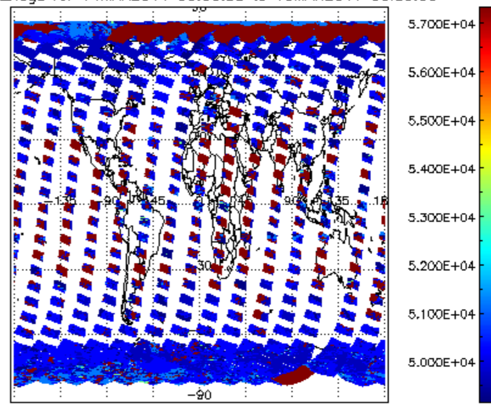
cloud_flags for 14MAR2011 00:00:00 to 15MAR2011 00:00:00
