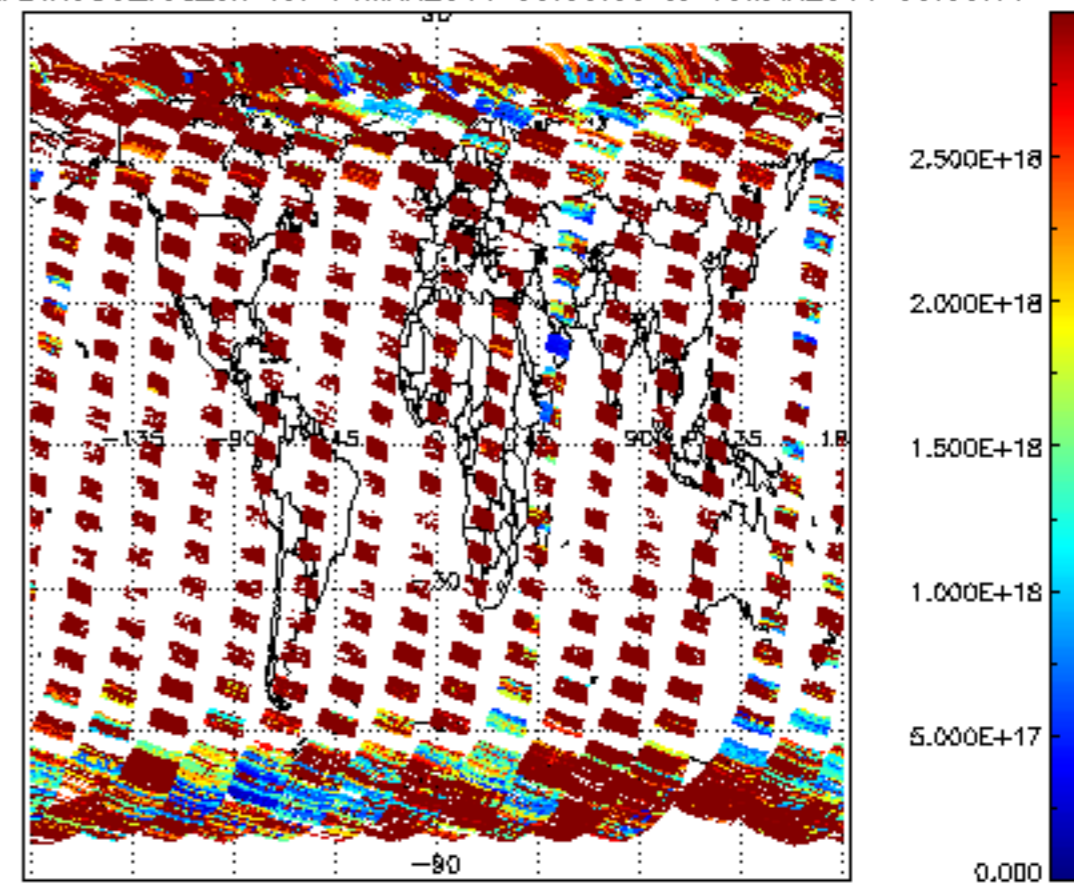
SCIOL2P_NADIR3CO_vcd_err for 14MAR2011 00:00:00 to 15MAR2011 00:00:00
