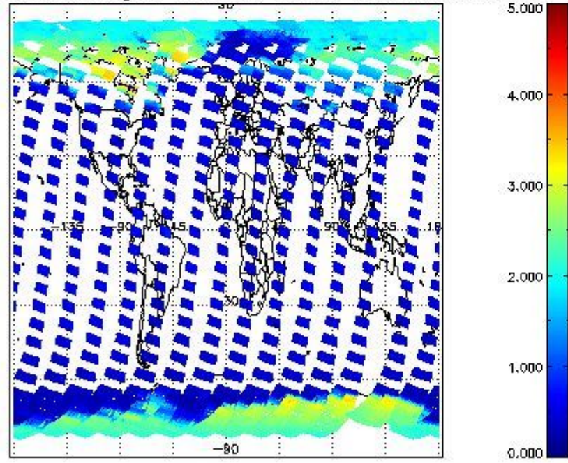
SCIOL2P_NADUV5SO2_amf_gr for 14MAR2011 00:00:00 to 15MAR2011 00:00:00
