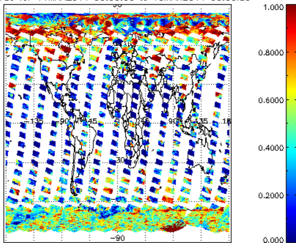
cL_frac for 14MAR2011 00:00:00 to 15MAR2011 00:00:00
