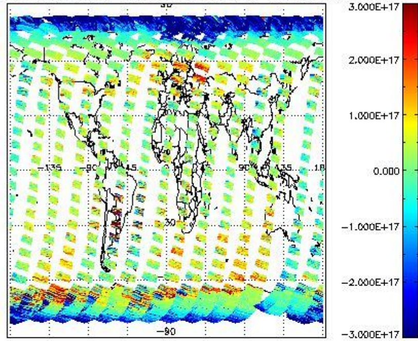
SCIOL2P_NADUV5SO2_vcd for 14MAR2011 00:00:00 to 15MAR2011 00:00:00
