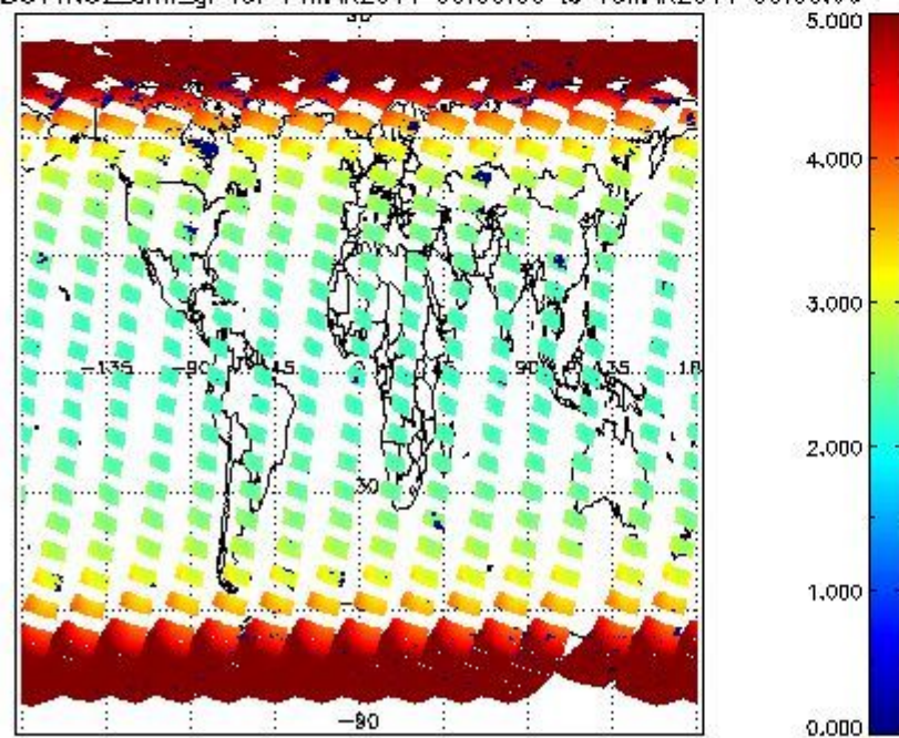
SCIOL2P_NADUV1NO2_amf_gr for 14MAR2011 00:00:00 to 15MAR2011 00:00:00
