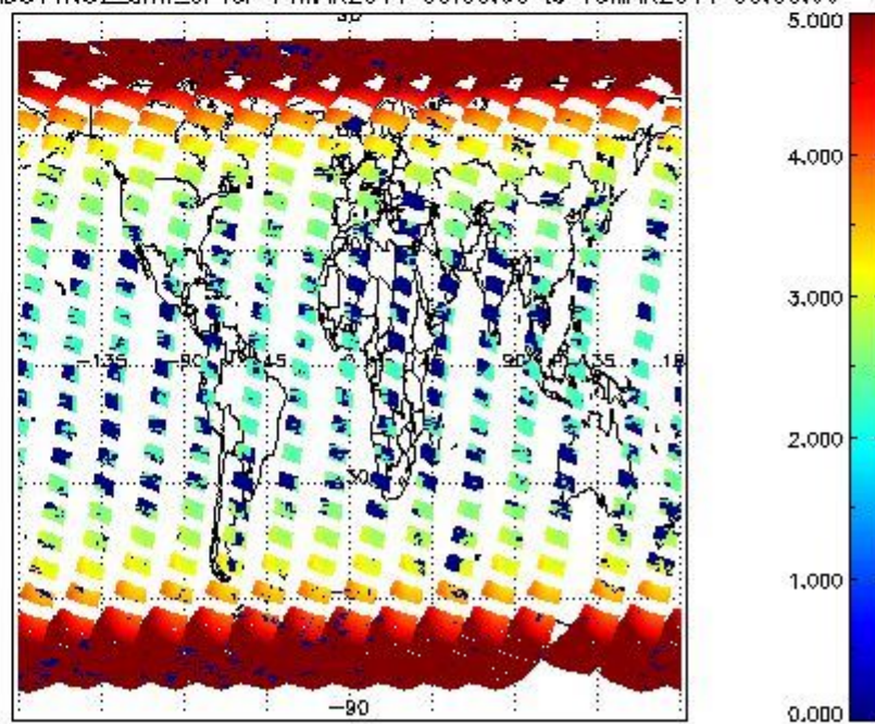
SCIOL2P_NADUV1NO2_amf_cl for 14MAR2011 00:00:00 to 15MAR2011 00:00:00
