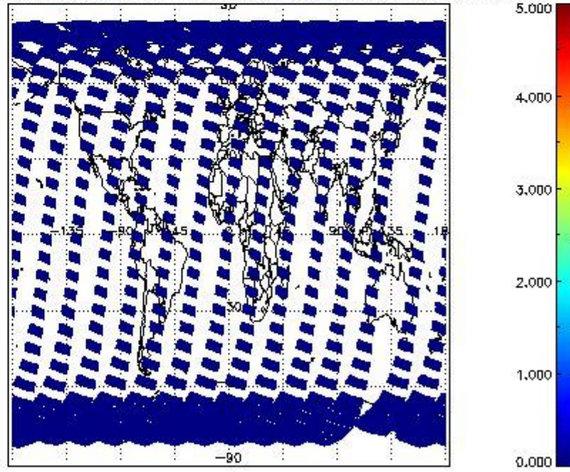
SCIOL2P_NADUV5SO2_amf_cl for 14MAR2011 00:00:00 to 15MAR2011 00:00:00
