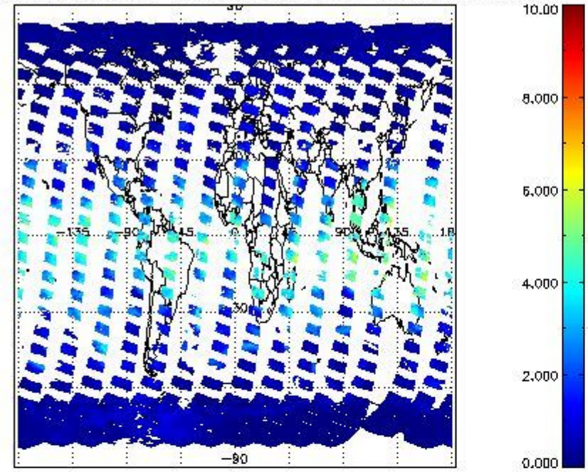
SCIOL2P_NADUV8H2O_vcd for 14MAR2011 00:00:00 to 15MAR2011 00:00:00
