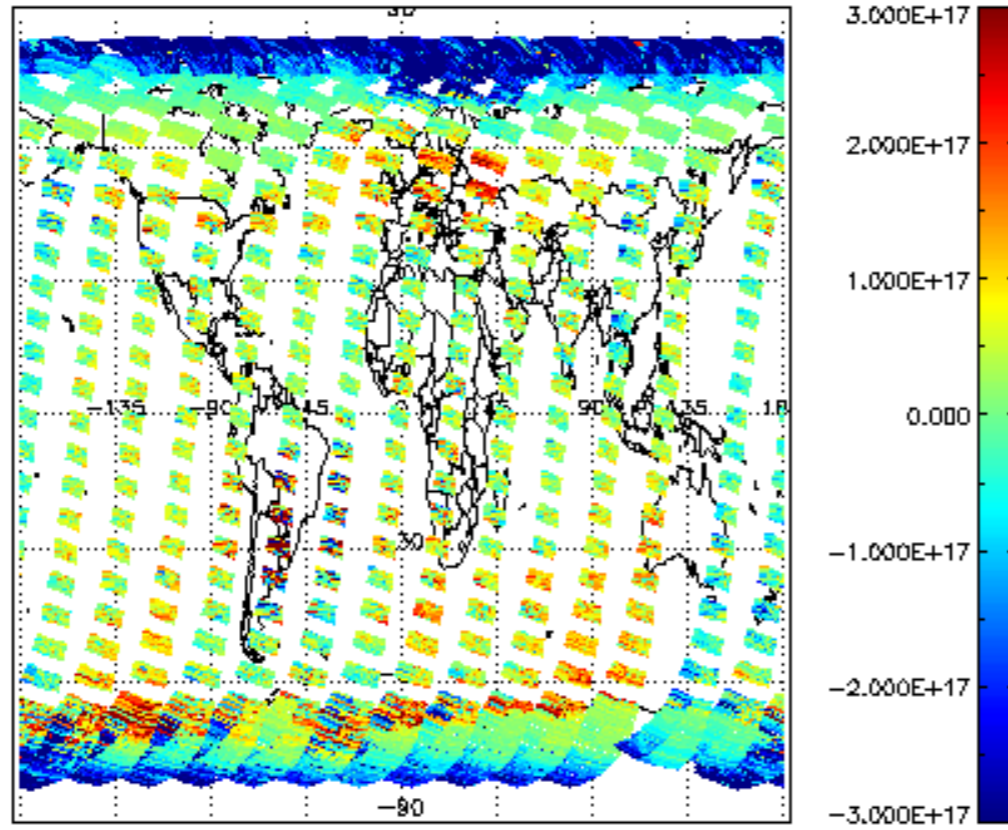
SCIOL2P_NADUV5S02_vcd for 14MAR2011 00:00:00 to 15MAR2011 00:00:00
