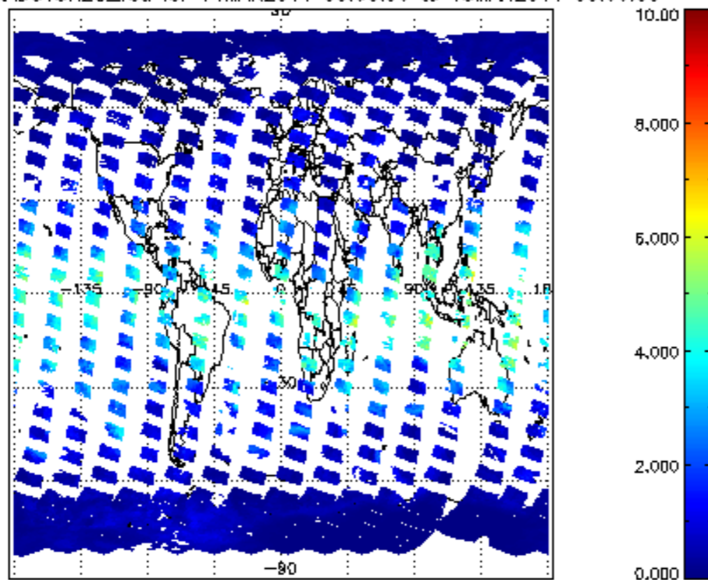
SCIOL2P_NADUV8H2O_vcd for 14MAR2011 00:00:00 to 15MAR2011 00:00:00
