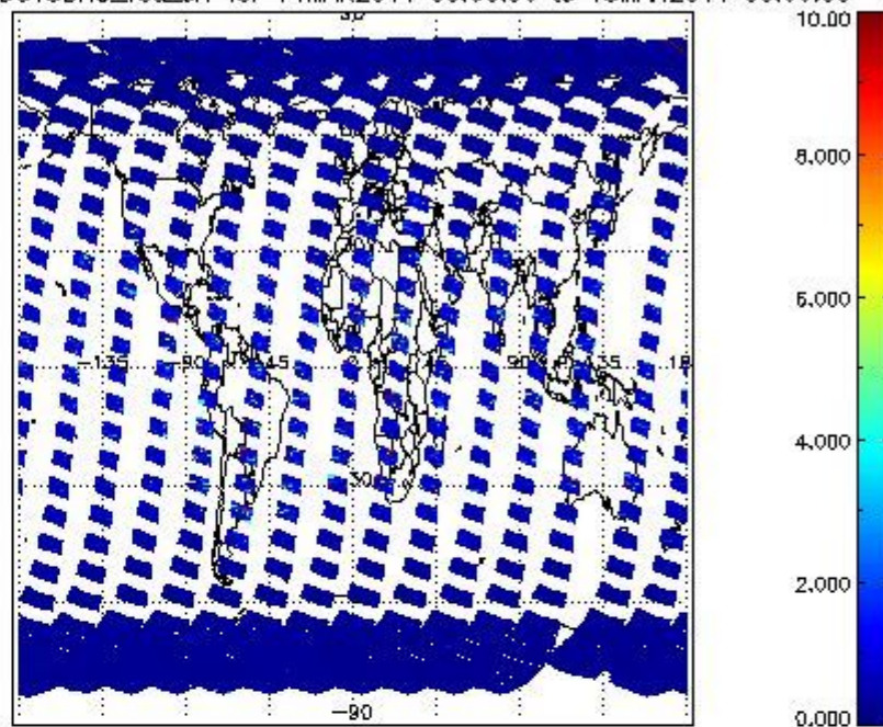
SCIOL2P_NADUV3BRO_vcd_err for 14MAR2011 00:00:00 to 15MAR2011 00:00:00
