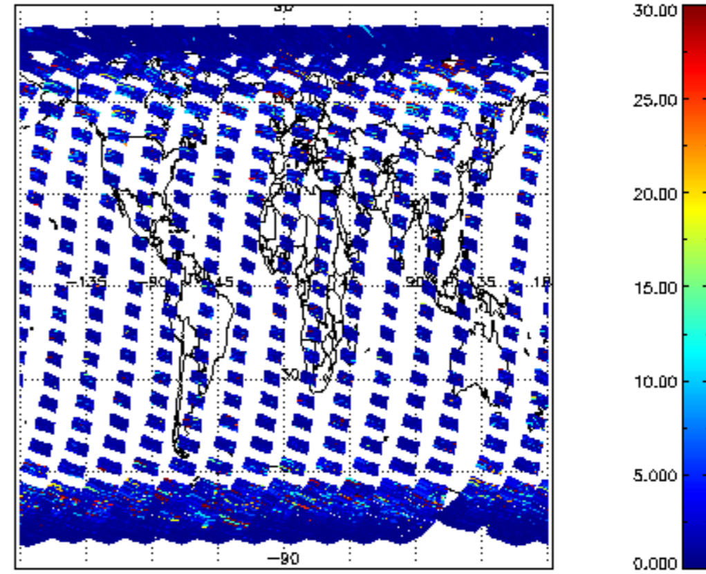
SCIOL2P_NADUV5S02_vcd_err for 14MAR2011 00:00:00 to 15MAR2011 00:00:00
