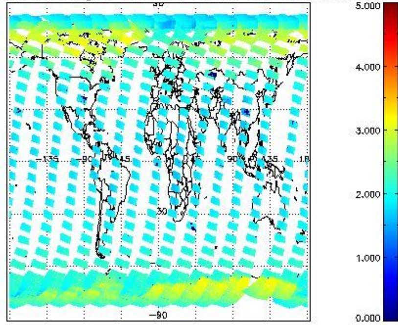
SCIOL2P_NADUV7S02_amf_gr for 14MAR2011 00:00:00 to 15MAR2011 00:00:00
