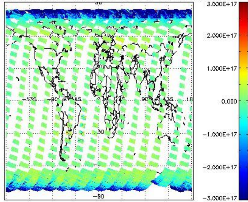
SCIOL2P_NADUV7S02_vcd for 14MAR2011 00:00:00 to 15MAR2011 00:00:00
