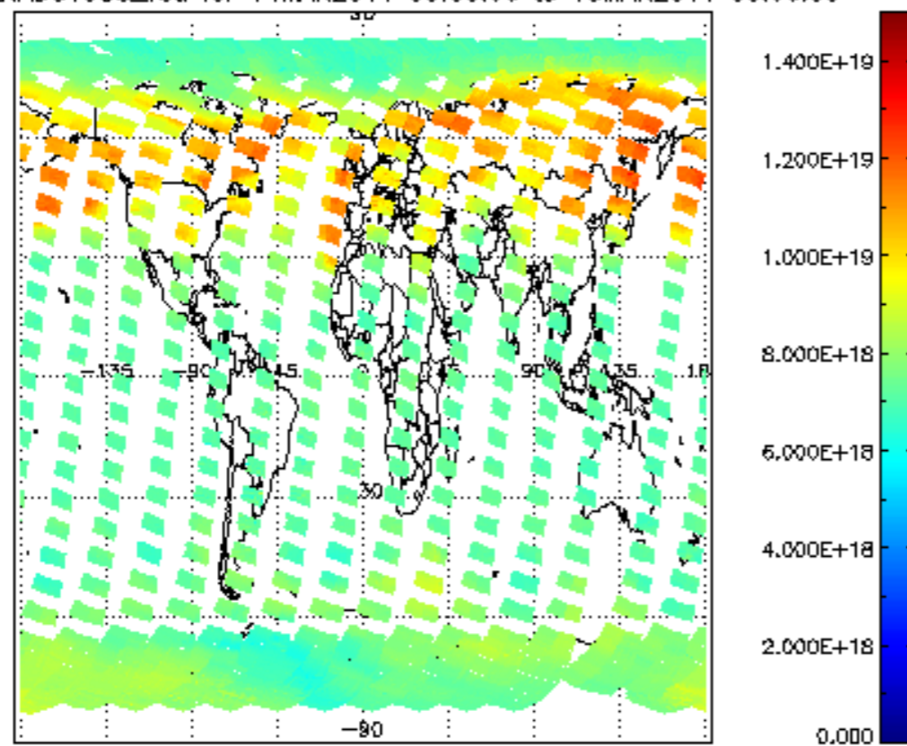
SCIOL2P_NADUV003_vcd for 14MAR2011 00:00:00 to 15MAR2011 00:00:00
