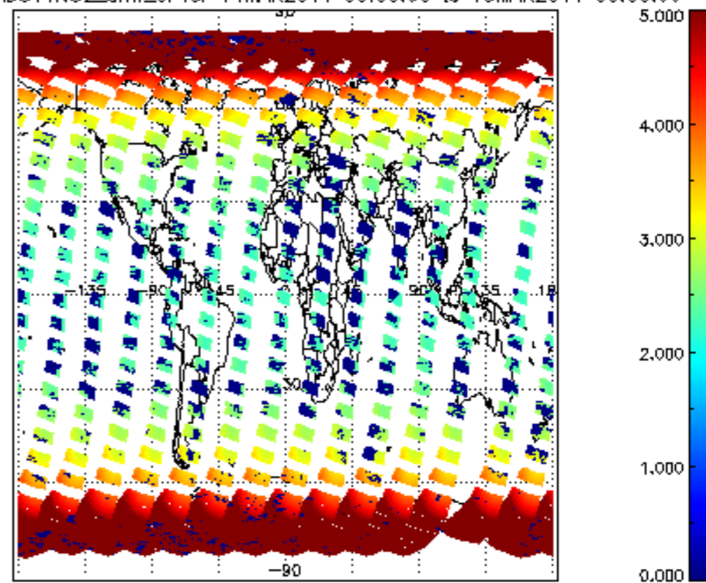
SCIOL2P_NADUV1NO2_amf_cl for 14MAR2011 00:00:00 to 15MAR2011 00:00:00
