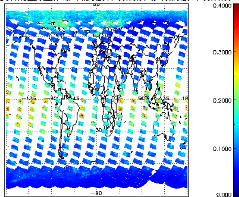
SCIOL2P_NADUV1NO2_vcd_err for 14MAR2011 00:00:00 to 15MAR2011 00:00:00
