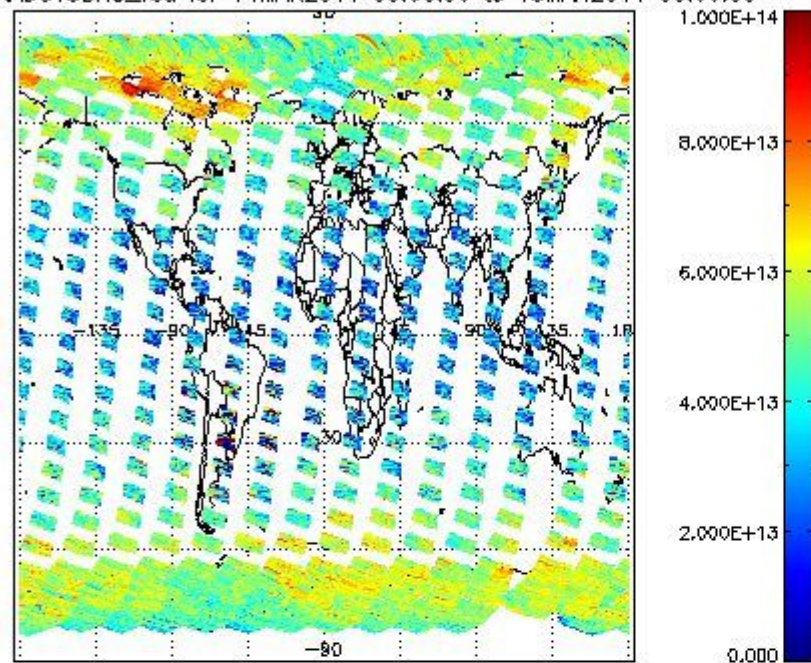
SCIOL2P_NADUV3BRO_vcd for 14MAR2011 00:00:00 to 15MAR2011 00:00:00
