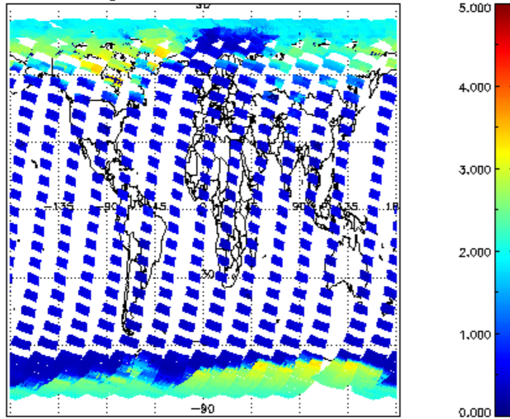
SCIOL2P_NADUV5S02_amf_gr for 14MAR2011 00:00:00 to 15MAR2011 00:00:00
