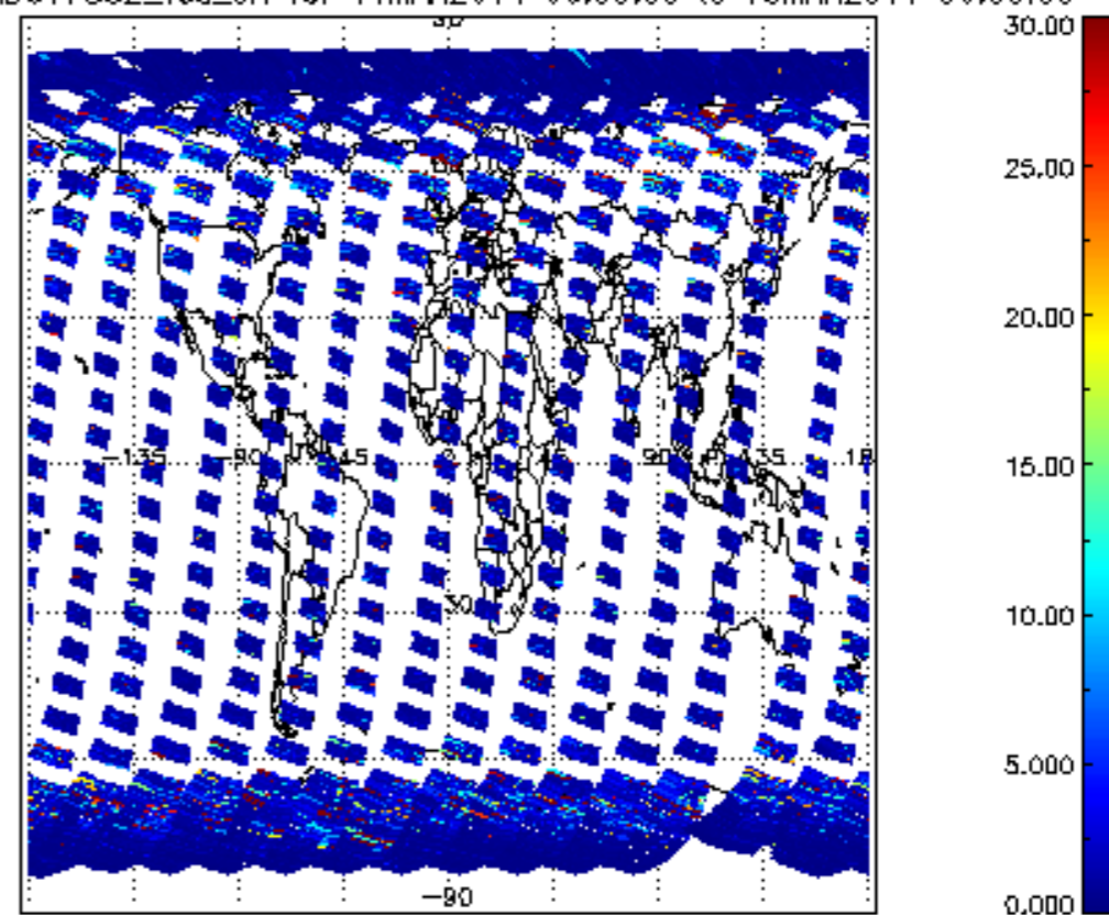
SCIOL2P_NADUV7S02_vcd_err for 14MAR2011 00:00:00 to 15MAR2011 00:00:00
