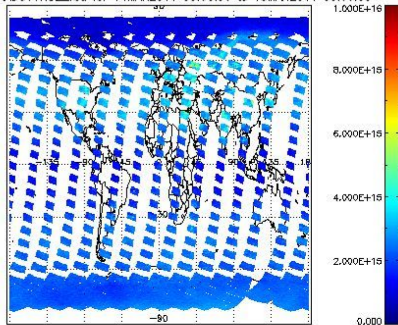
SCIOL2P_NADUV1NO2_vcd for 14MAR2011 00:00:00 to 15MAR2011 00:00:00
