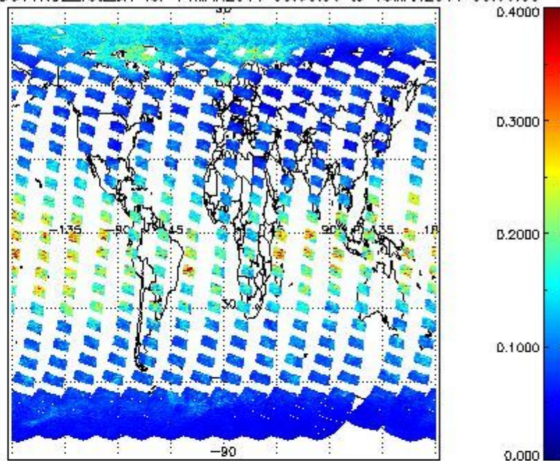
SCIOL2P_NADUV1NO2_vcd_err for 14MAR2011 00:00:00 to 15MAR2011 00:00:00
