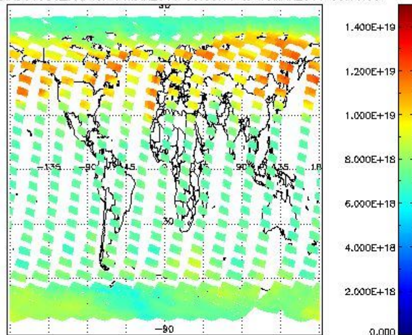
SCIOL2P_NADUV003_vcd for 14MAR2011 00:00:00 to 15MAR2011 00:00:00
