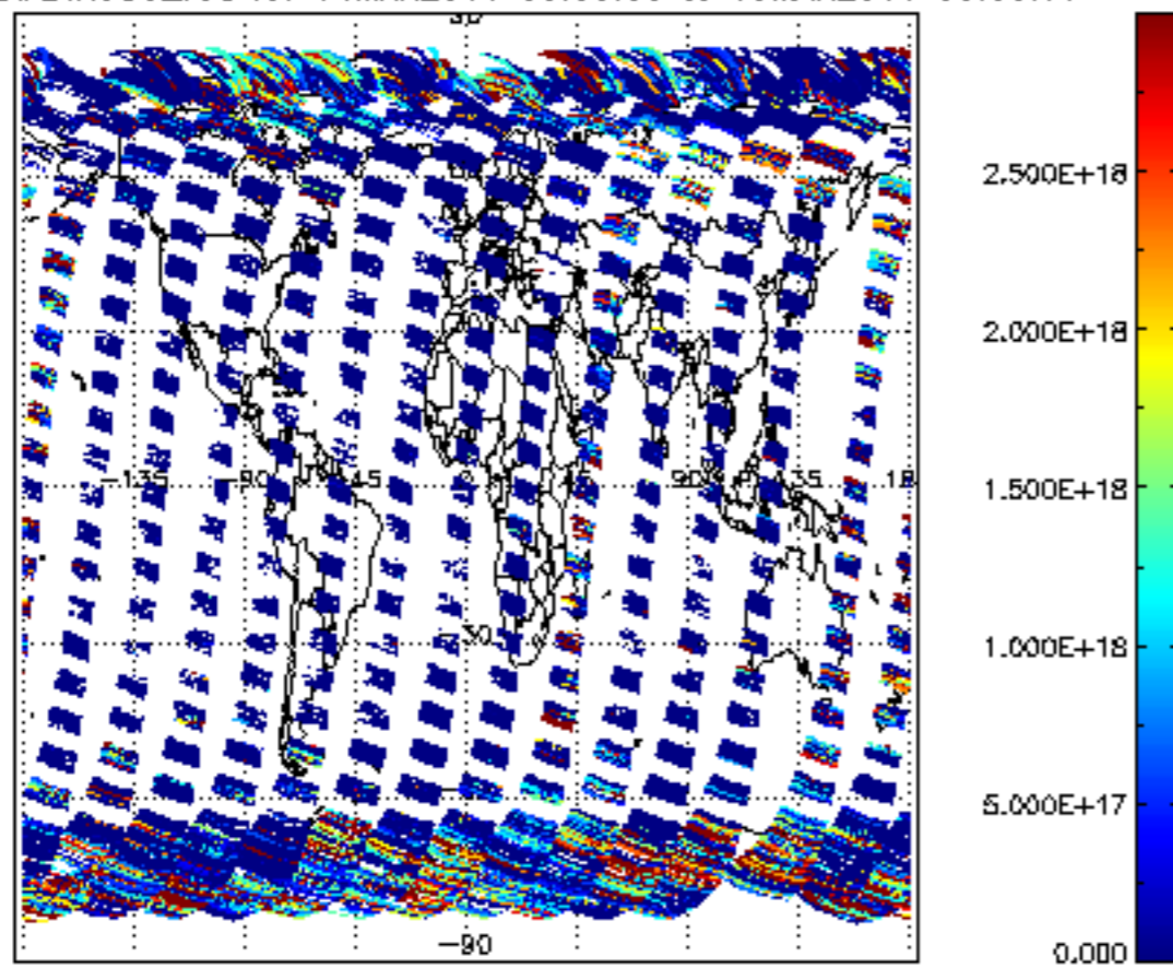
SCIOL2P_NADIR3CO_vcd for 14MAR2011 00:00:00 to 15MAR2011 00:00:00
