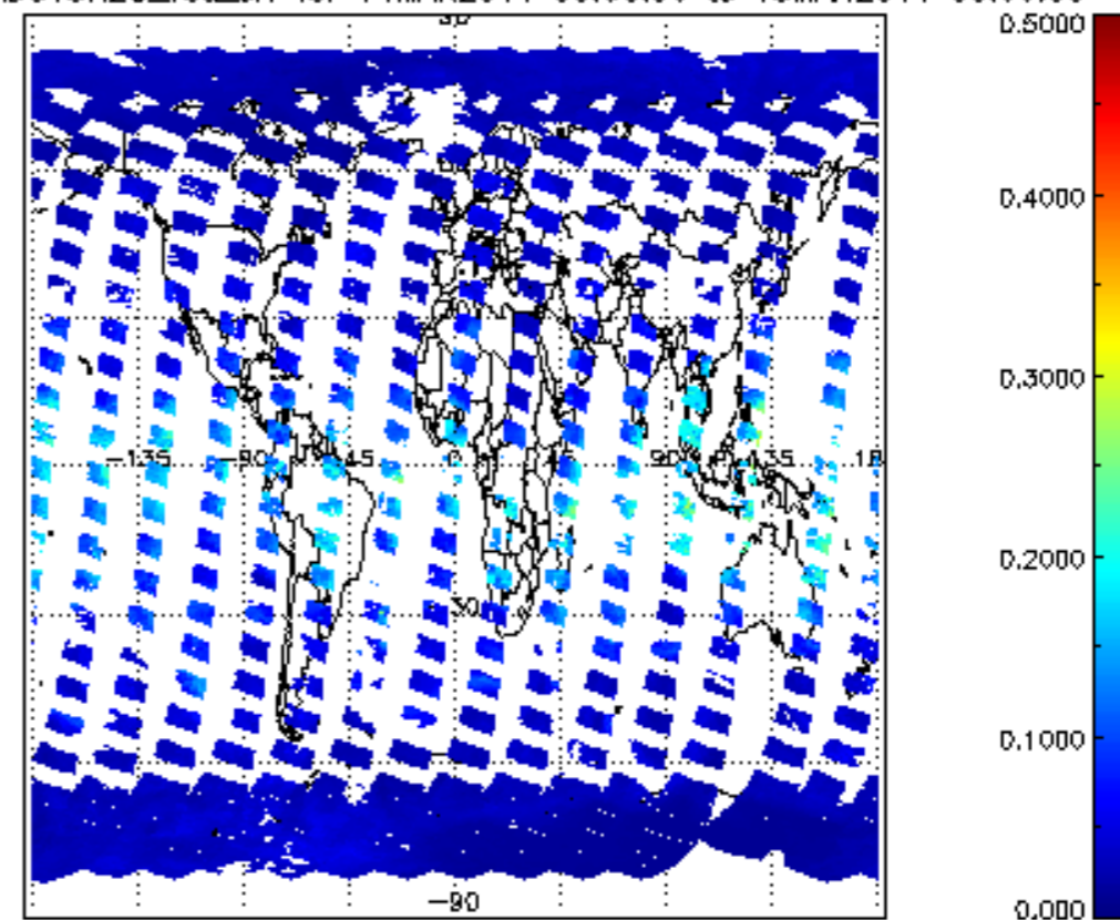
SCIOL2P_NADUV8H2O_vcd_Lerr for 14MAR2011 00:00:00 to 15MAR2011 00:00:00
