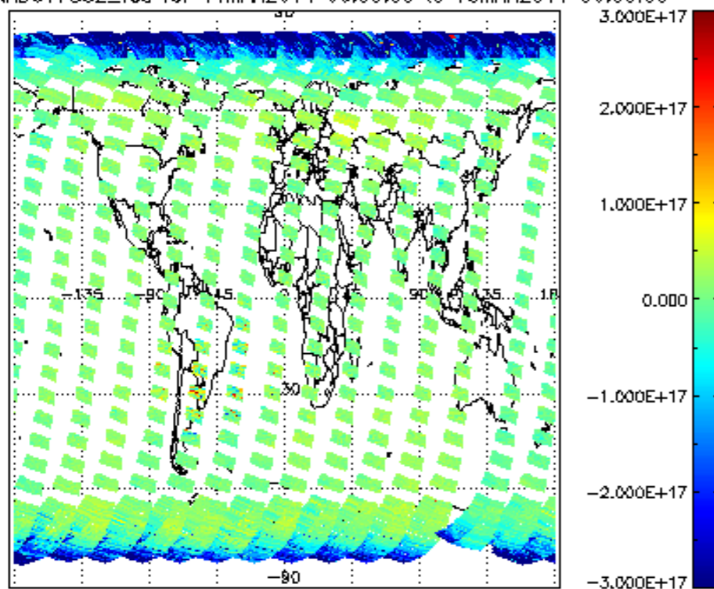
SCIOL2P_NADUV7S02_vcd for 14MAR2011 00:00:00 to 15MAR2011 00:00:00
