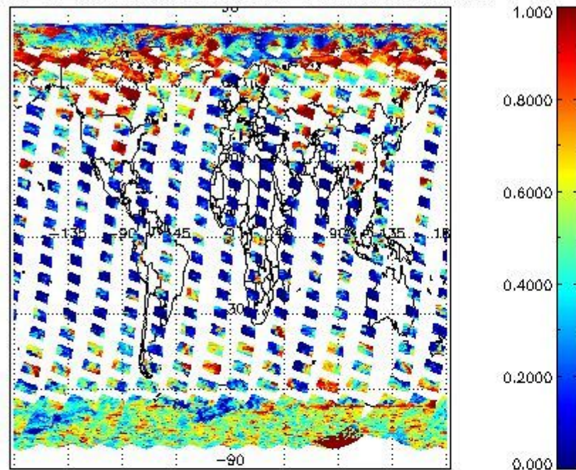
cL_frac for 14MAR2011 00:00:00 to 15MAR2011 00:00:00
