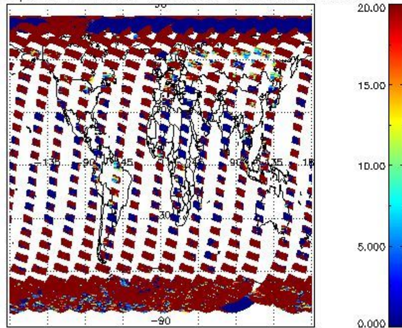
cL_opt_depth for 14MAR2011 00:00:00 to 15MAR2011 00:00:00
