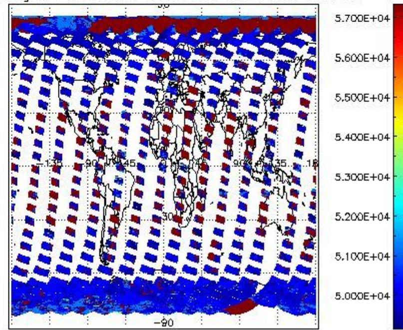
cloud_flags for 14MAR2011 00:00:00 to 15MAR2011 00:00:00
