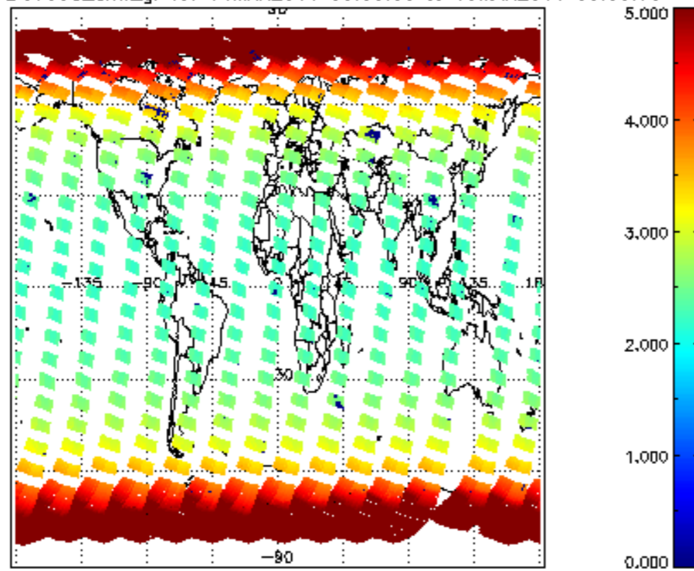
SCIOL2P_NADUV003_amf_gr for 14MAR2011 00:00:00 to 15MAR2011 00:00:00
