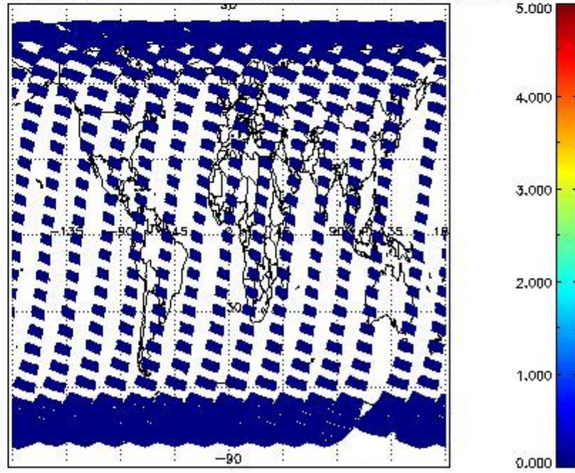
SCIOL2P_NADUV7S02_amf_cl for 14MAR2011 00:00:00 to 15MAR2011 00:00:00
