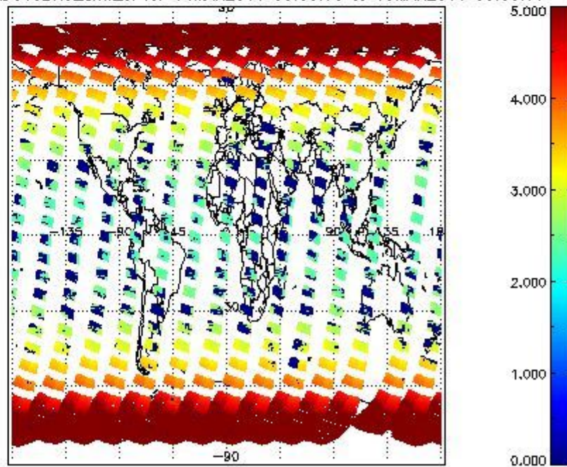
SCIOL2P_NADUV3BRO_amf_cl for 14MAR2011 00:00:00 to 15MAR2011 00:00:00
