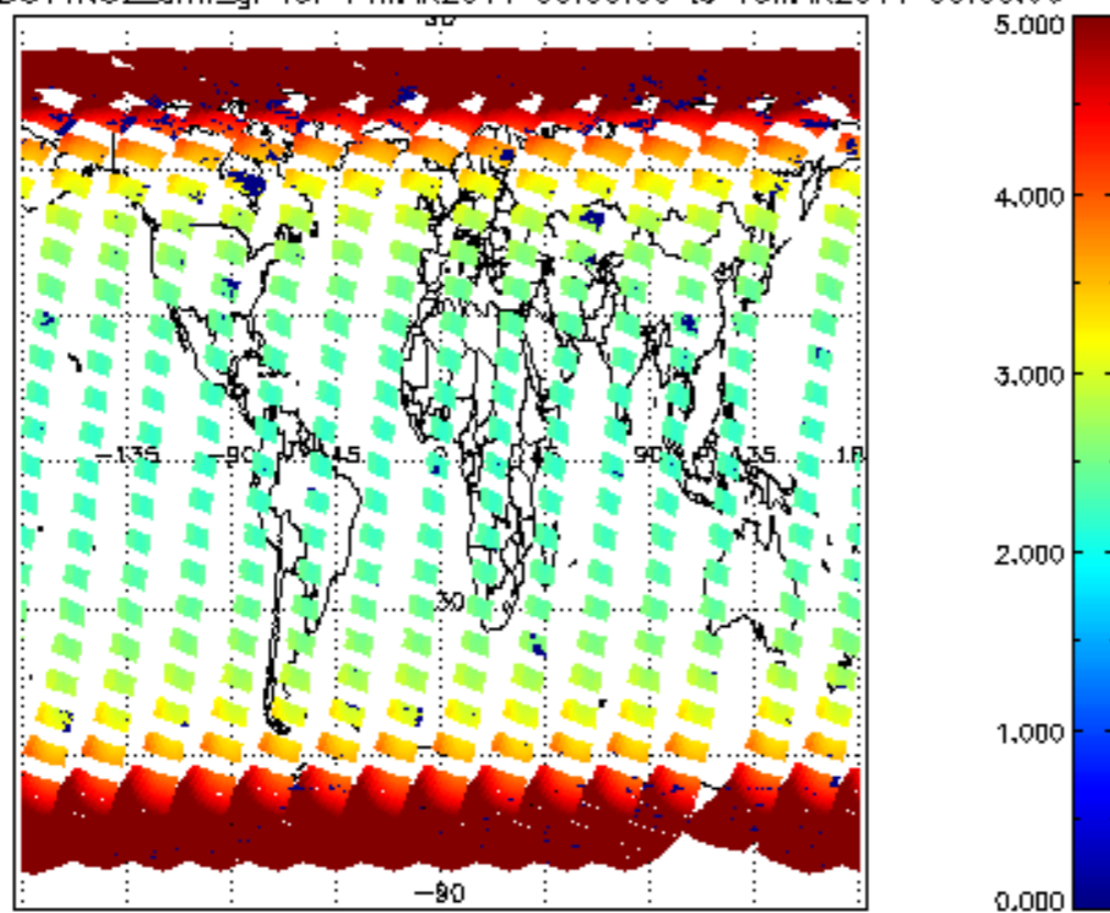
SCIOL2P_NADUV1NO2_amf_gr for 14MAR2011 00:00:00 to 15MAR2011 00:00:00
