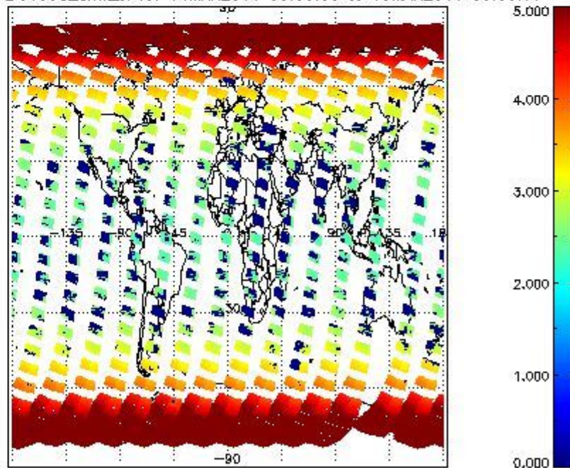
SCIOL2P_NADUV003_amf_cl for 14MAR2011 00:00:00 to 15MAR2011 00:00:00
