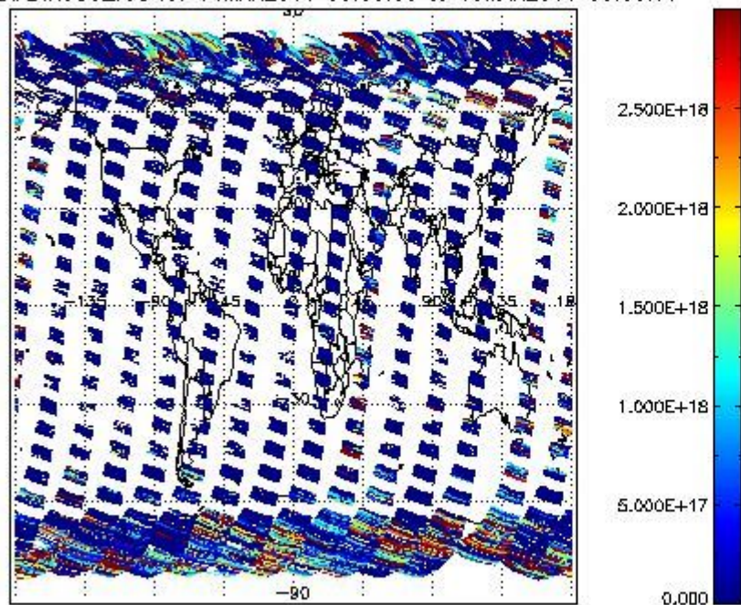
SCIDL2P_NADIR3CO_vcd for 14MAR2011 00:00:00 to 15MAR2011 00:00:00
