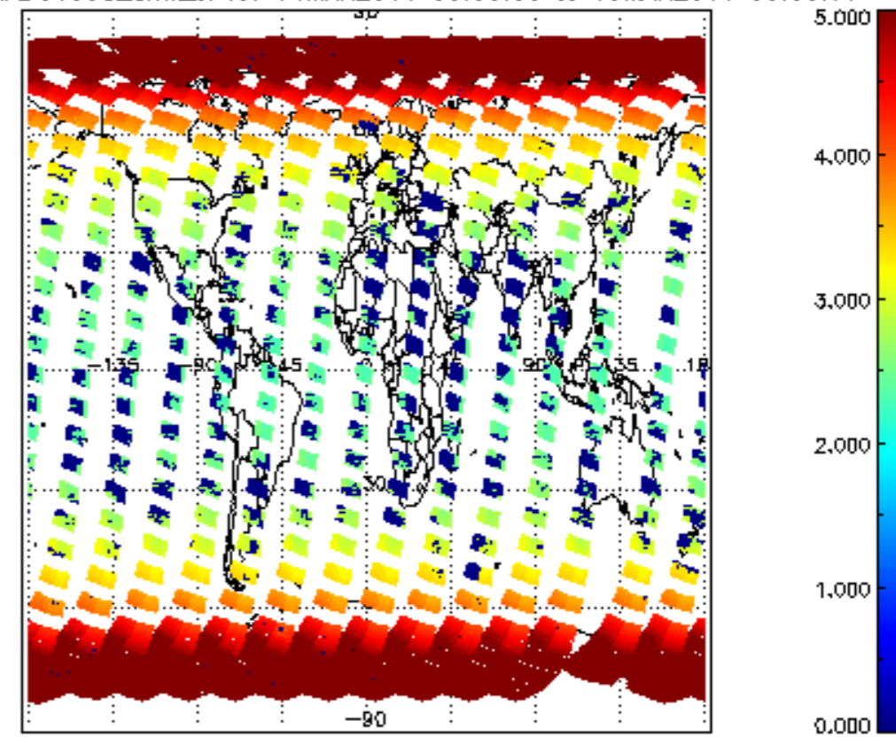
SCIOL2P_NADUV003_amf_cl for 14MAR2011 00:00:00 to 15MAR2011 00:00:00
