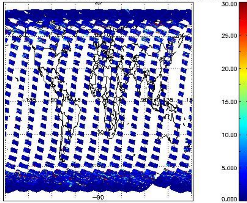
SCIOL2P_NADUV7S02_vcd_err for 14MAR2011 00:00:00 to 15MAR2011 00:00:00
