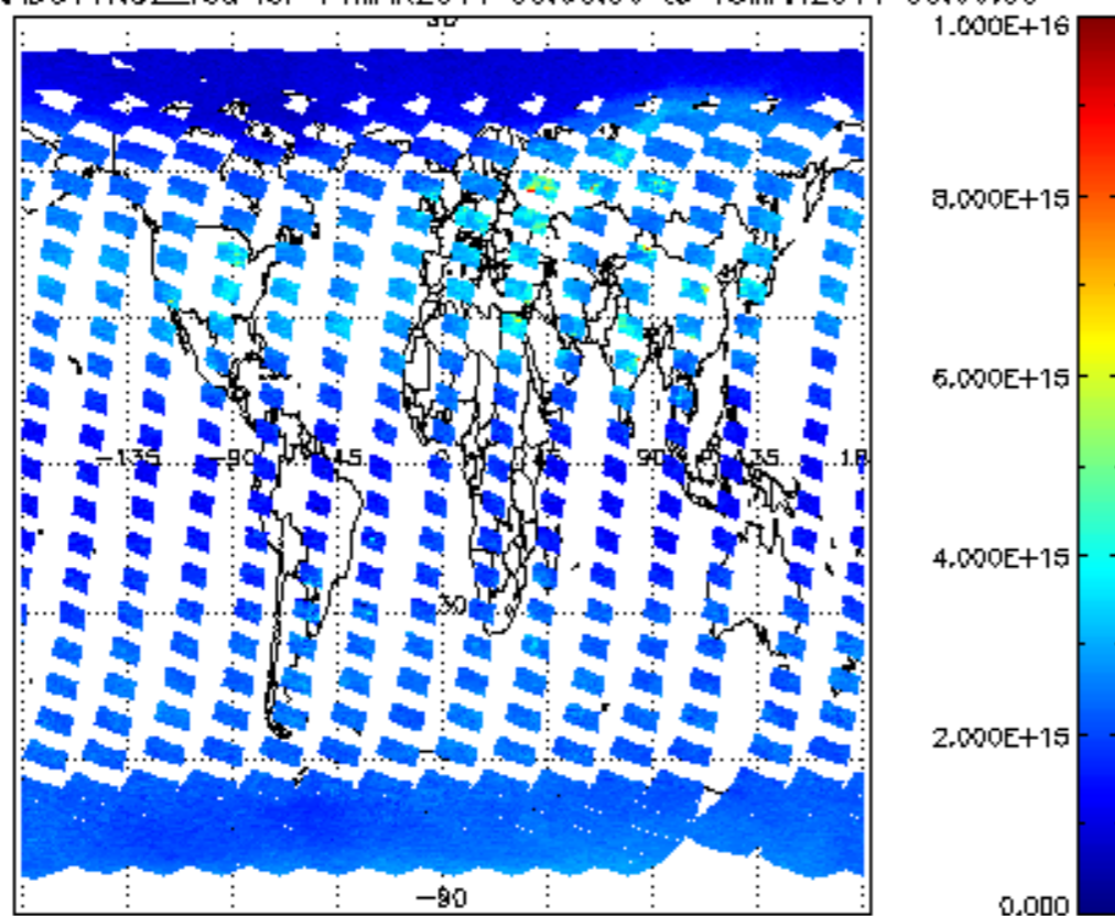
SCIOL2P_NADUV1NO2_vcd for 14MAR2011 00:00:00 to 15MAR2011 00:00:00
