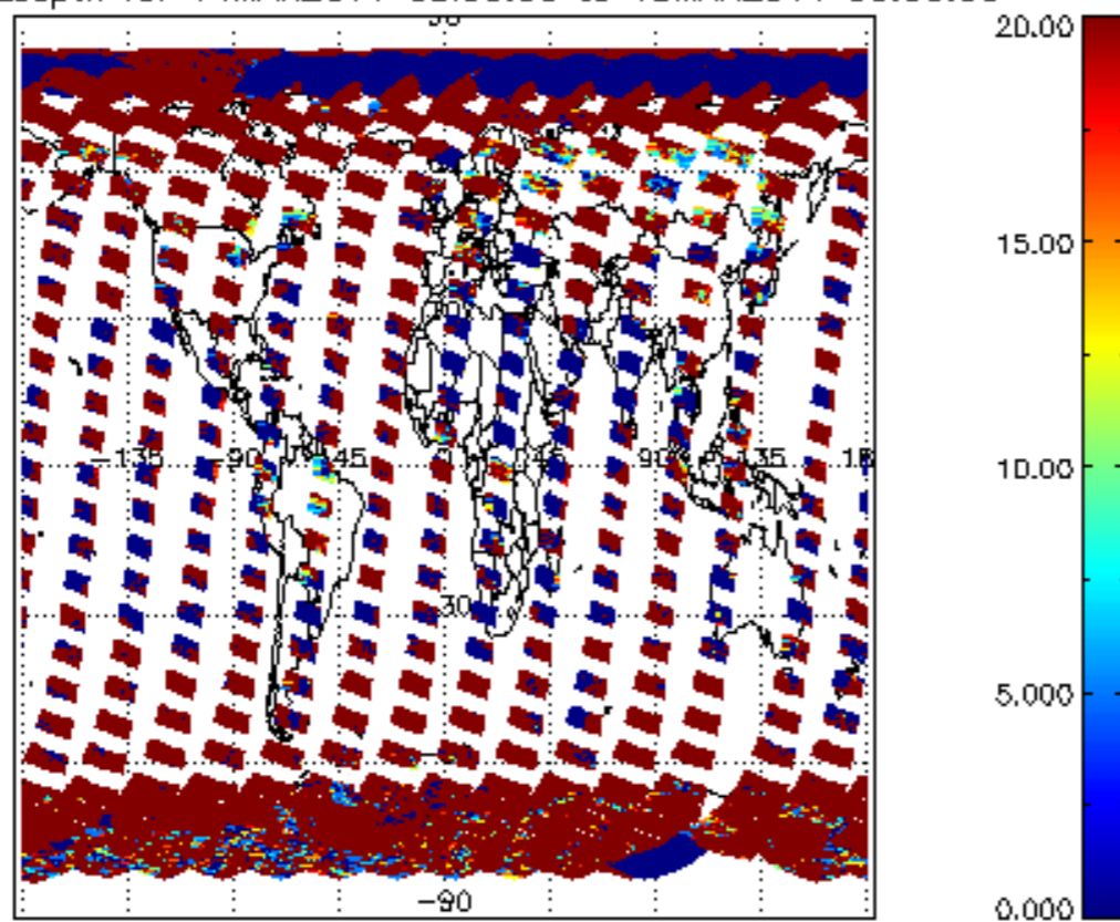
cL_opt_depth for 14MAR2011 00:00:00 to 15MAR2011 00:00:00
