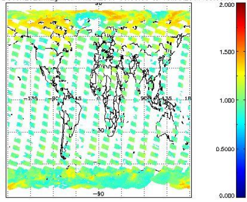
SCIOL2P_NADUV8H2O_arnf_gr for 14MAR2011 00:00:00 to 15MAR2011 00:00:00
