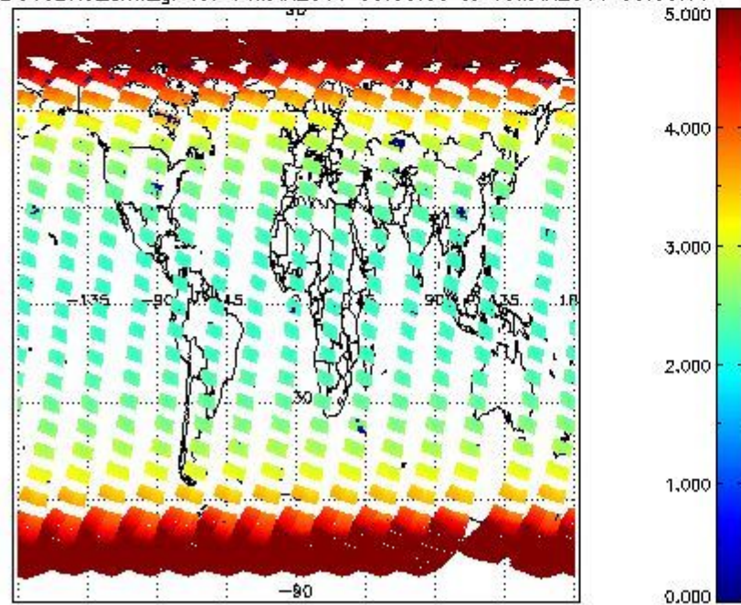
SCIOL2P_NADUV3BRO_amf_gr for 14MAR2011 00:00:00 to 15MAR2011 00:00:00
