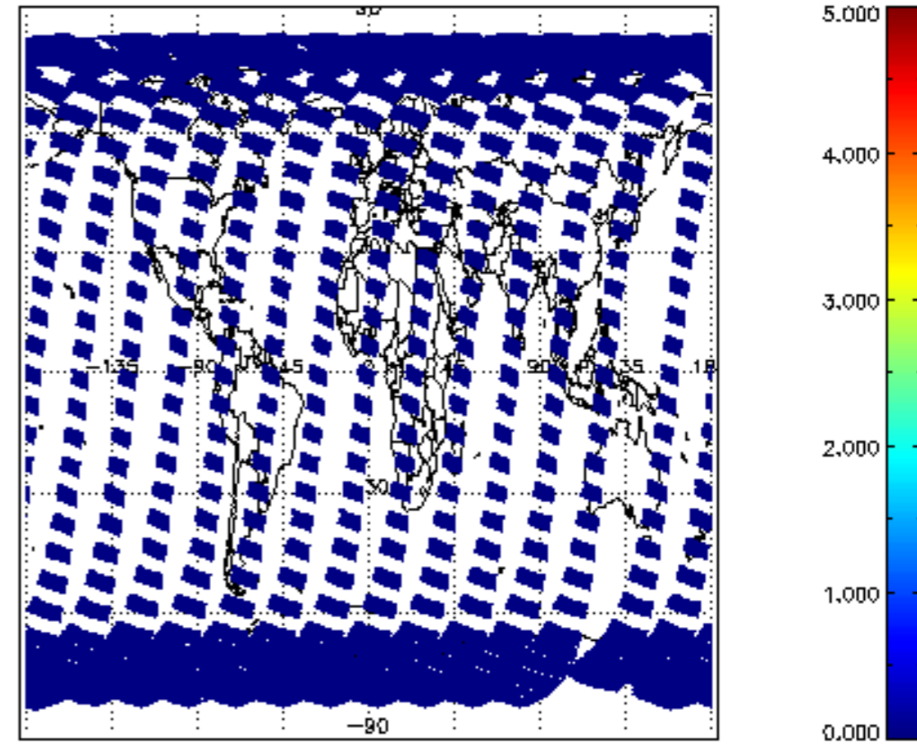
SCIOL2P_NADUV5S02_amf_cl for 14MAR2011 00:00:00 to 15MAR2011 00:00:00
