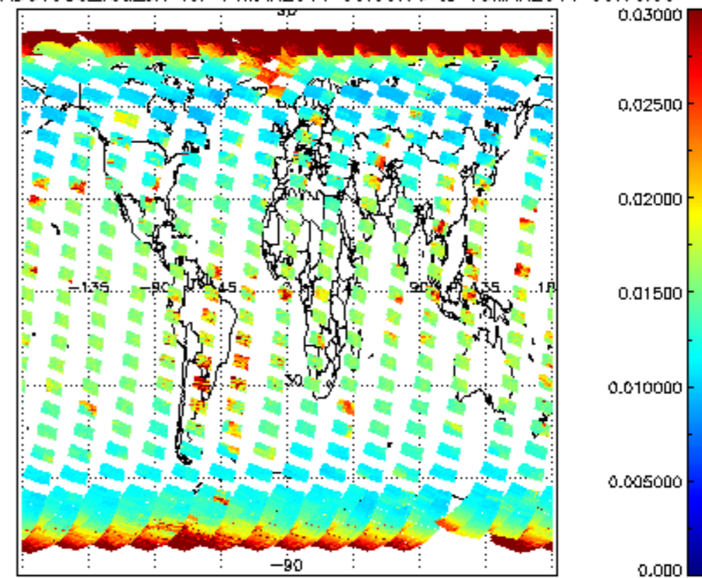
SCIOL2P_NADUV003_vcd_err for 14MAR2011 00:00:00 to 15MAR2011 00:00:00
