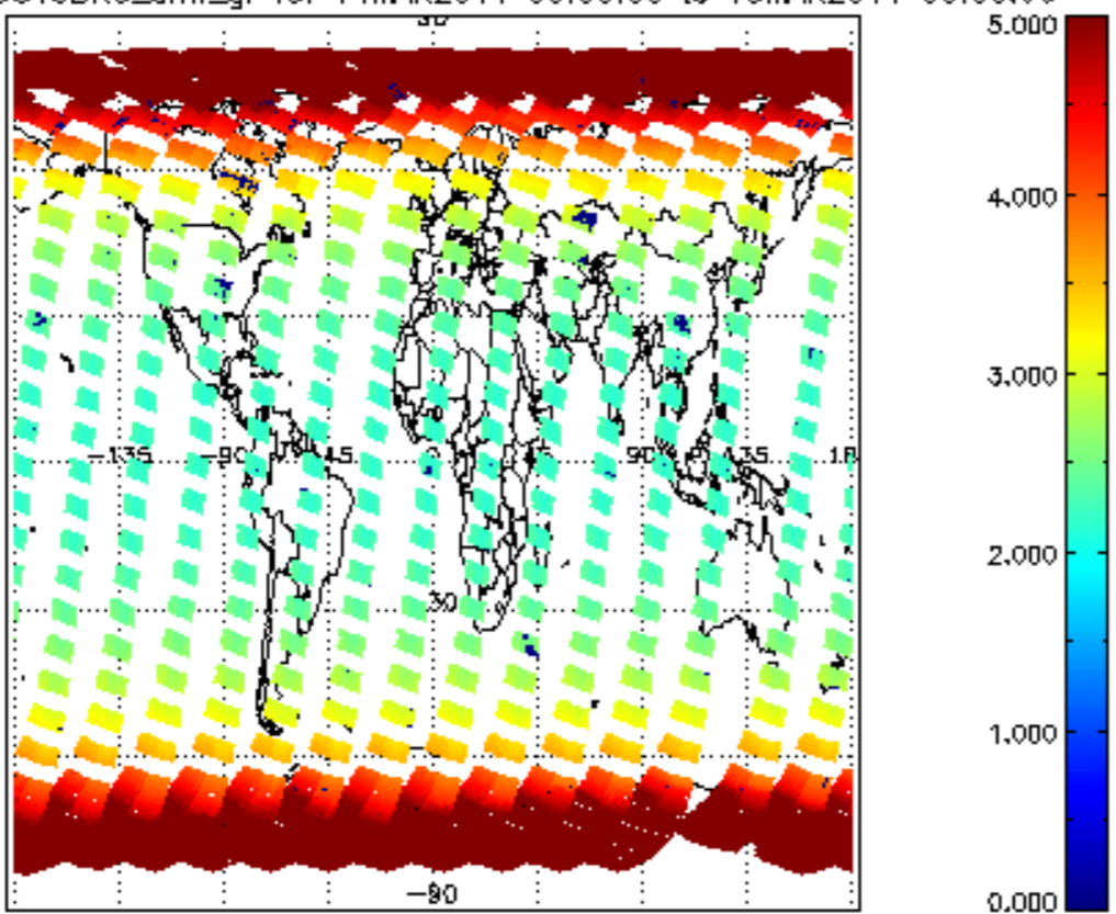
SCIOL2P_NADUV3BRO_arnf_gr for 14MAR2011 00:00:00 to 15MAR2011 00:00:00
