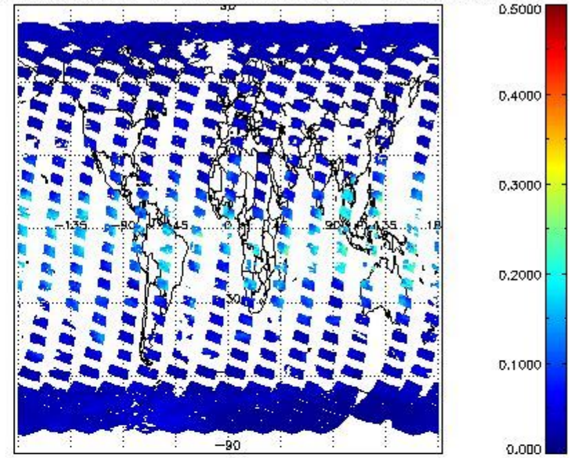
SCIOL2P_NADUV8H2O_vcd_err for 14MAR2011 00:00:00 to 15MAR2011 00:00:00
