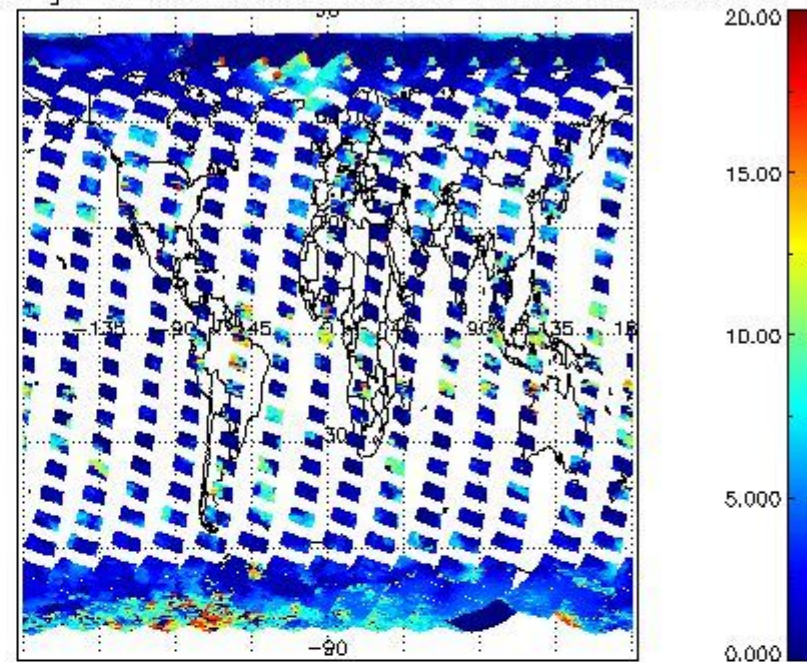
cL_top_height for 14MAR2011 00:00:00 to 15MAR2011 00:00:00
