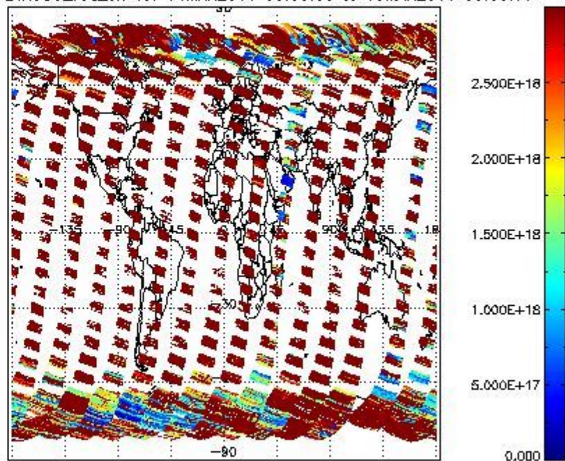
SCIDL2P_NADIR3CO_vcd_err for 14MAR2011 00:00:00 to 15MAR2011 00:00:00
