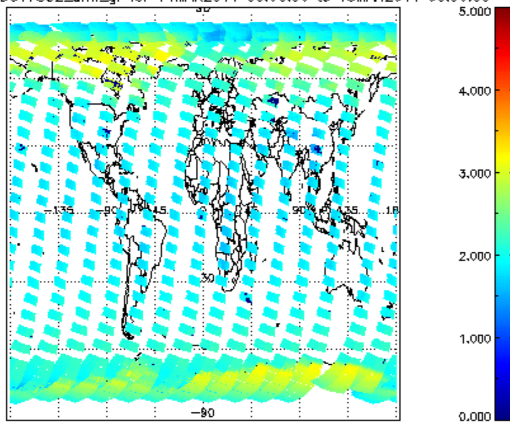
SCIOL2P_NADUV7S02_amf_gr for 14MAR2011 00:00:00 to 15MAR2011 00:00:00
