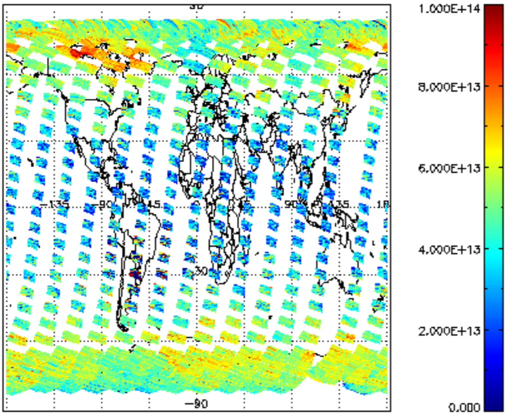
SCIOL2P_NADUV3BRO_vcd for 14MAR2011 00:00:00 to 15MAR2011 00:00:00
