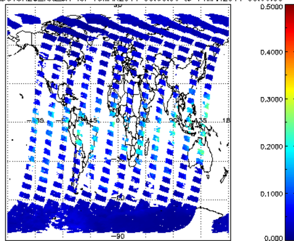
SCIOL2P_NADUV8H20_vcd_Lerr for 13MAR2011 00:00:00 to 14MAR2011 00:00:00
