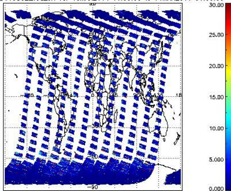
SCIOL2P_NADUV5SO2_vcd_err for 13MAR2011 00:00:00 to 14MAR2011 00:00:00
