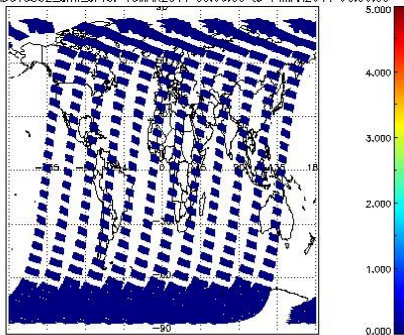
SCIOL2P_NADUV5SO2_amf_cl for 13MAR2011 00:00:00 to 14MAR2011 00:00:00
