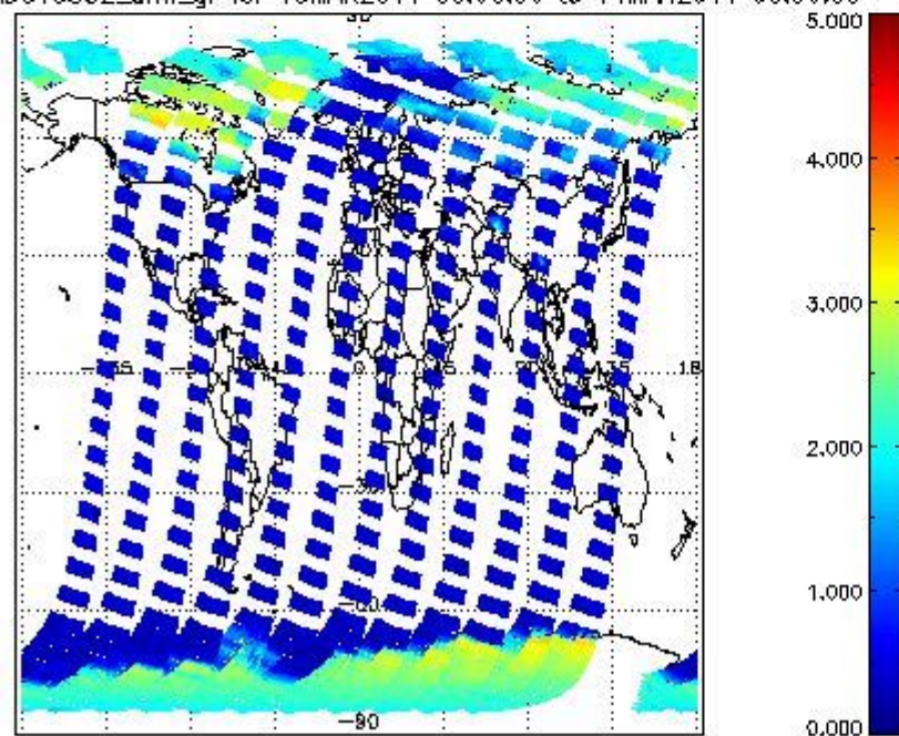
SCIOL2P_NADUV5SO2_amf_gr for 13MAR2011 00:00:00 to 14MAR2011 00:00:00
