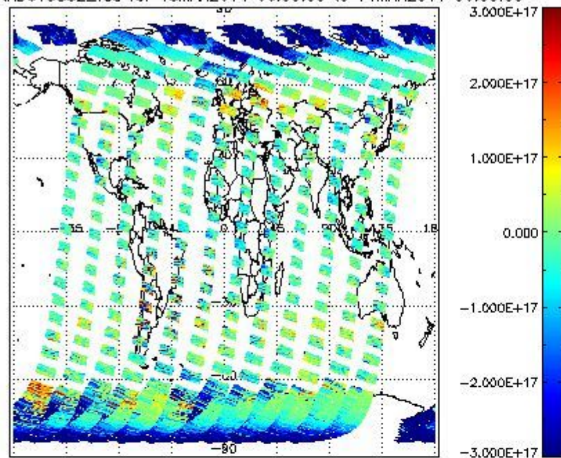
SCIOL2P_NADUV5SO2_vcd for 13MAR2011 00:00:00 to 14MAR2011 00:00:00
