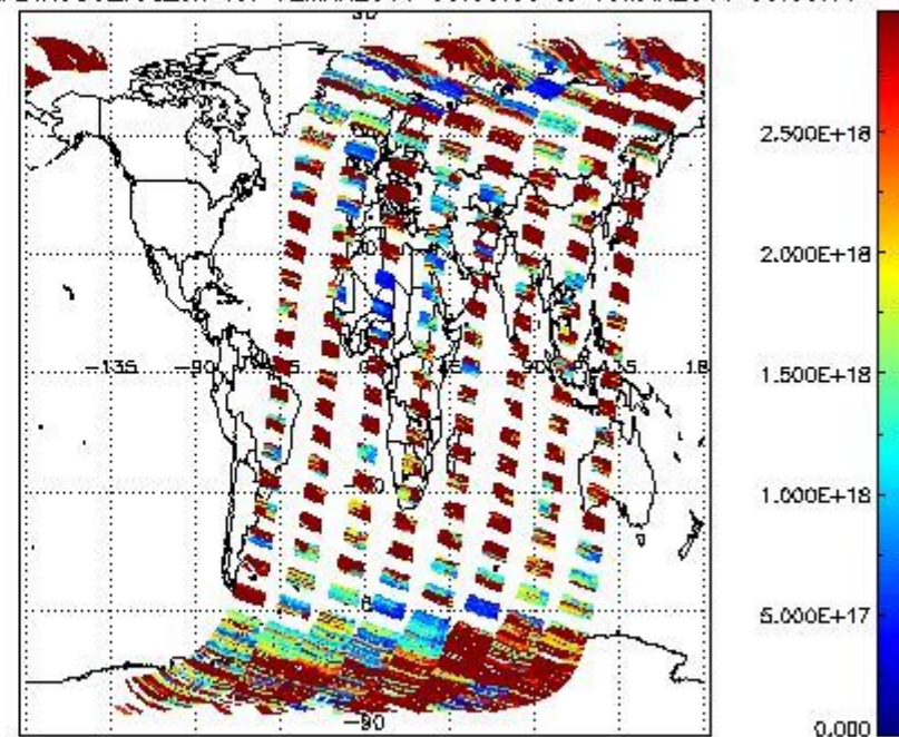
SCIDL2P_NADIR3CO_vcd_err for 12MAR2011 00:00:00 to 13MAR2011 00:00:00
