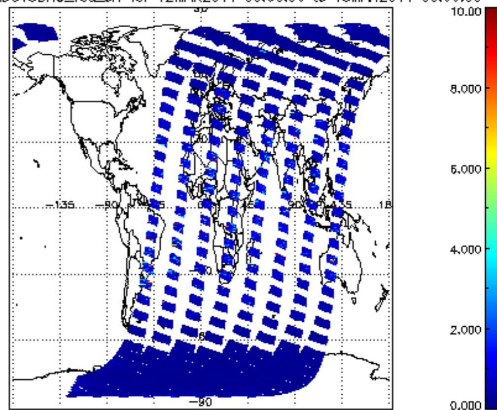
SCIOL2P_NADUV3BRO_vcd_err for 12MAR2011 00:00:00 to 13MAR2011 00:00:00
