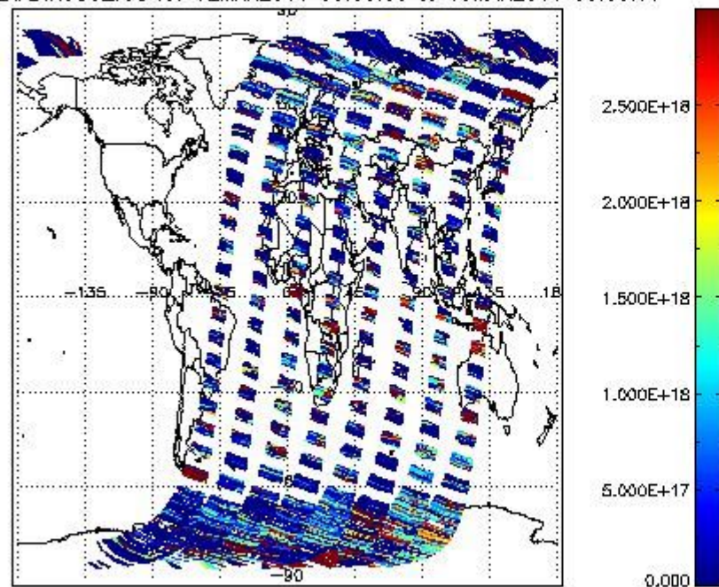
SCIDL2P_NADIR3CO_vcd for 12MAR2011 00:00:00 to 13MAR2011 00:00:00
