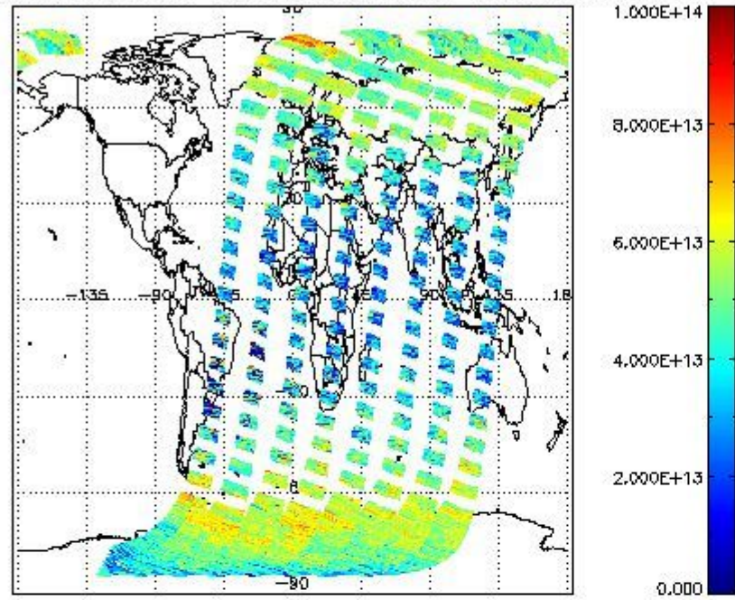
SCIOL2P_NADUV3BRO_vcd for 12MAR2011 00:00:00 to 13MAR2011 00:00:00
