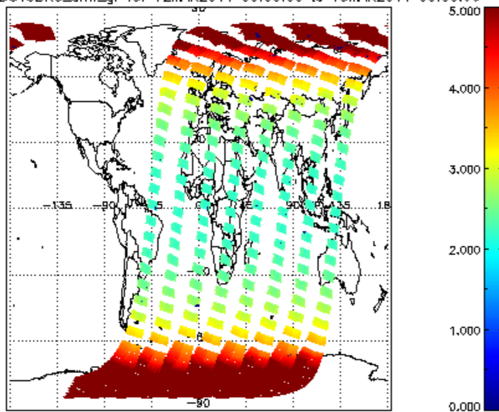
SCIOL2P_NADUV3BRO_amf_gr for 12MAR2011 00:00:00 to 13MAR2011 00:00:00
