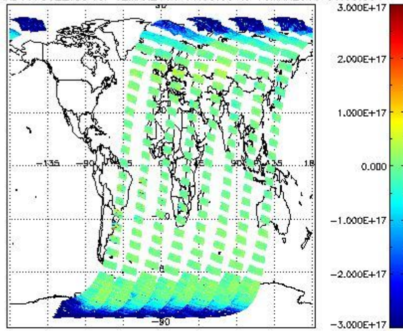
SCIOL2P_NADUV7S02_vcd for 12MAR2011 00:00:00 to 13MAR2011 00:00:00
