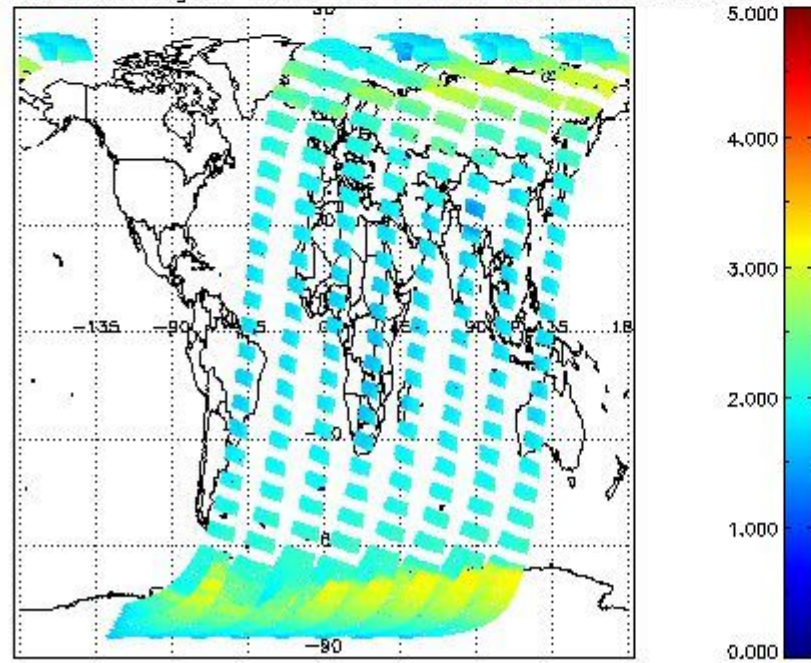
SCIOL2P_NADUV7S02_amf_gr for 12MAR2011 00:00:00 to 13MAR2011 00:00:00
