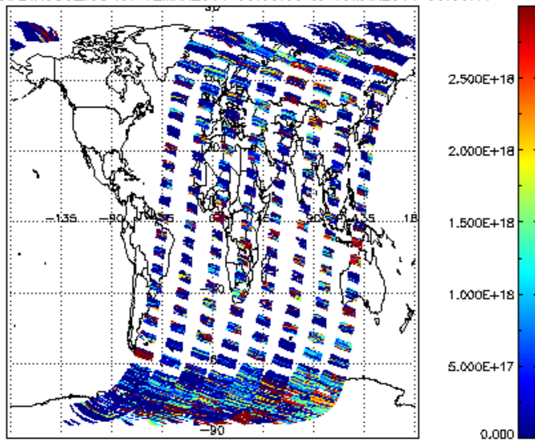
SCIOL2P_NADIR3CO_vcd for 12MAR2011 00:00:00 to 13MAR2011 00:00:00
