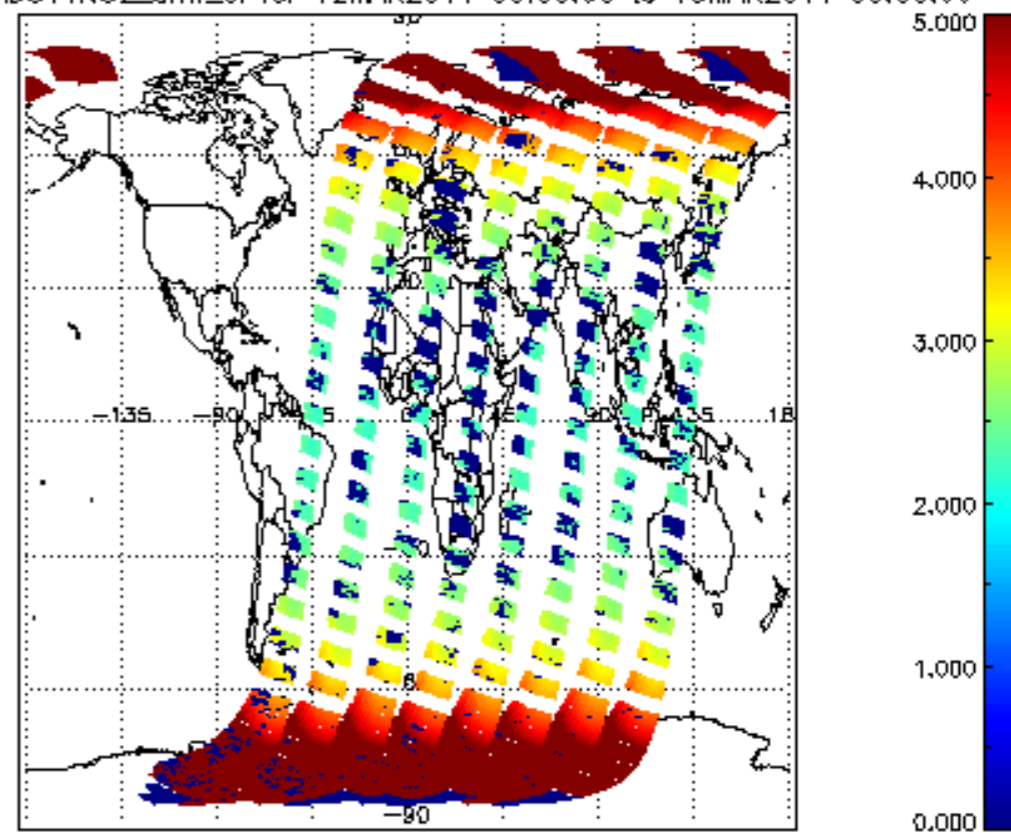
SCIOL2P_NADUV1NO2_amf_cl for 12MAR2011 00:00:00 to 13MAR2011 00:00:00
