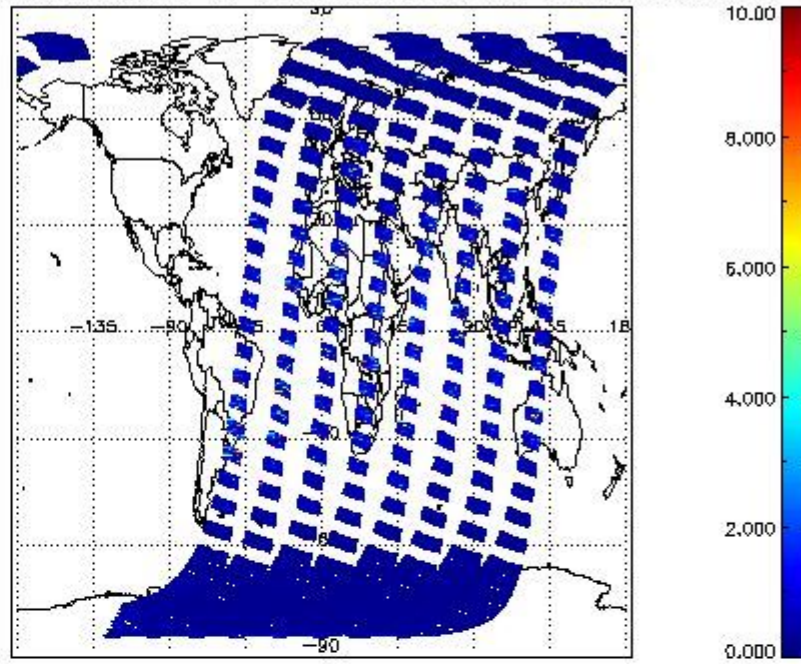
SCIOL2P_NADUV3BRO_vcd_err for 12MAR2011 00:00:00 to 13MAR2011 00:00:00
