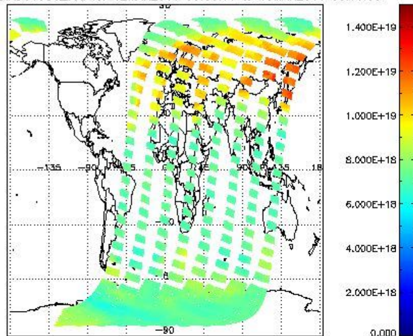
SCIOL2P_NADUV003_vcd for 12MAR2011 00:00:00 to 13MAR2011 00:00:00
