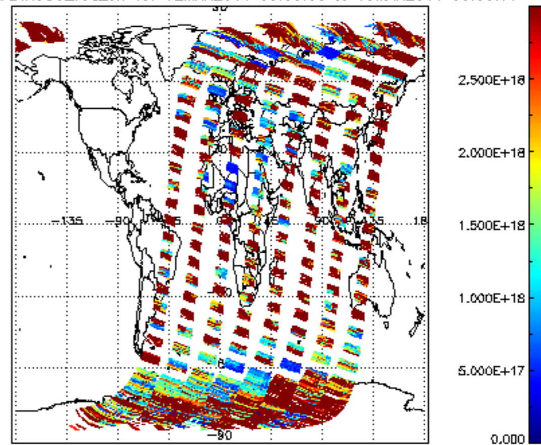
SCIOL2P_NADIR3CO_vcd_err for 12MAR2011 00:00:00 to 13MAR2011 00:00:00
