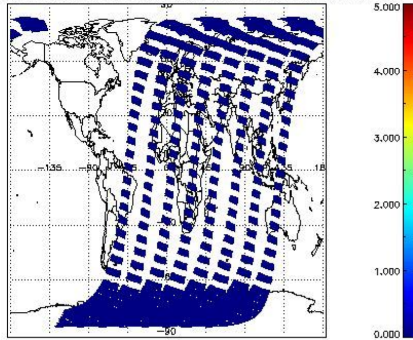
SCIOL2P_NADUV7S02_amf_cl for 12MAR2011 00:00:00 to 13MAR2011 00:00:00
