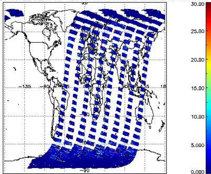
SCIOL2P_NADUV5S02_vcd_err for 12MAR2011 00:00:00 to 13MAR2011 00:00:00
