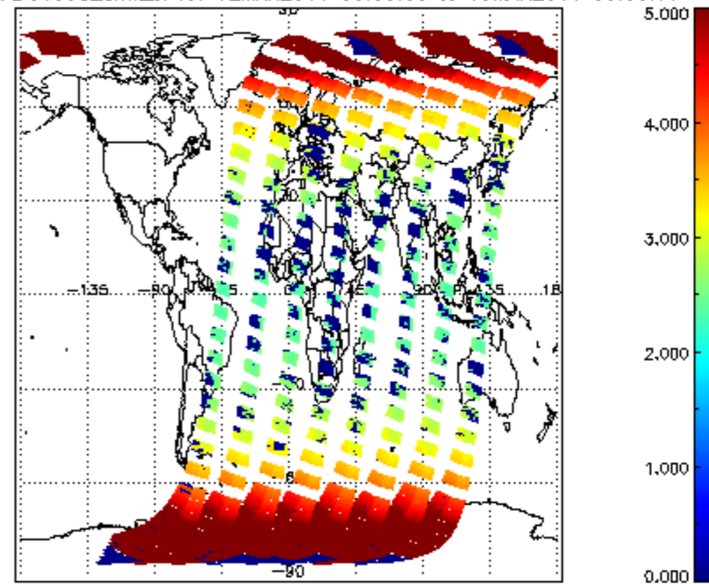
SCIOL2P_NADUV003_arnf_cl for 12MAR2011 00:00:00 to 13MAR2011 00:00:00
