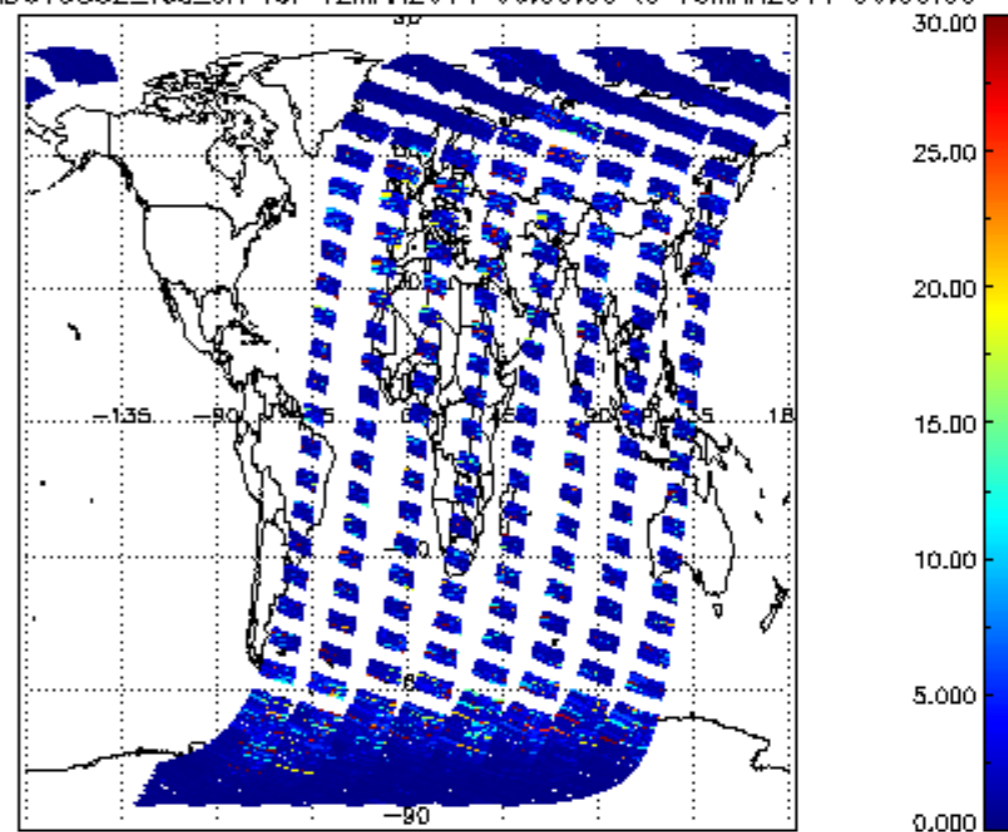
SCIOL2P_NADUV5S02_vcd_err for 12MAR2011 00:00:00 to 13MAR2011 00:00:00
