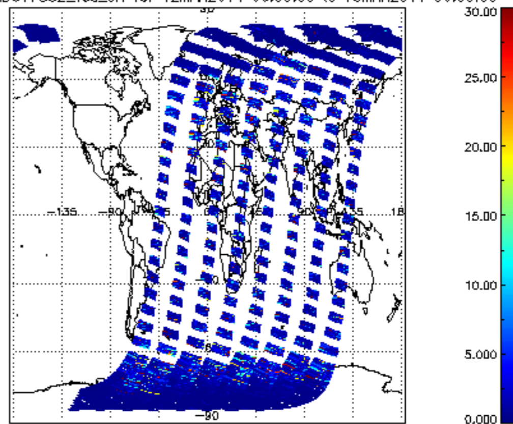
SCIOL2P_NADUV7S02_vcd_err for 12MAR2011 00:00:00 to 13MAR2011 00:00:00
