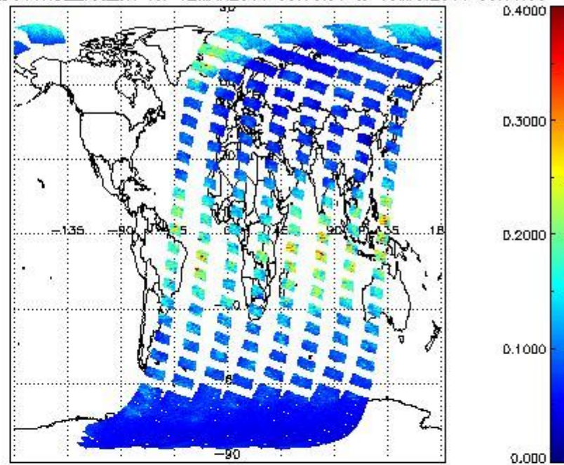
SCIOL2P_NADUV1NO2_vcd_err for 12MAR2011 00:00:00 to 13MAR2011 00:00:00
