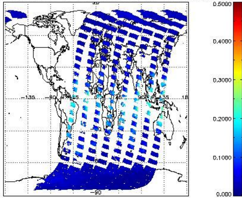
SCIOL2P_NADUV8H2O_vcd_err for 12MAR2011 00:00:00 to 13MAR2011 00:00:00
