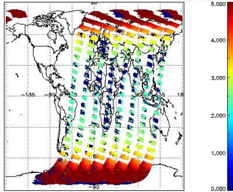
SCIOL2P_NADUV1NO2_amf_cl for 12MAR2011 00:00:00 to 13MAR2011 00:00:00
