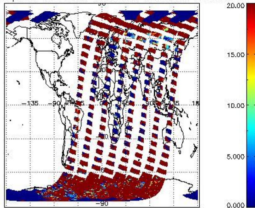
cL_opt_depth for 12MAR2011 00:00:00 to 13MAR2011 00:00:00
