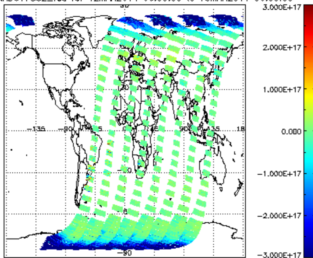
SCIOL2P_NADUV7S02_vcd for 12MAR2011 00:00:00 to 13MAR2011 00:00:00
