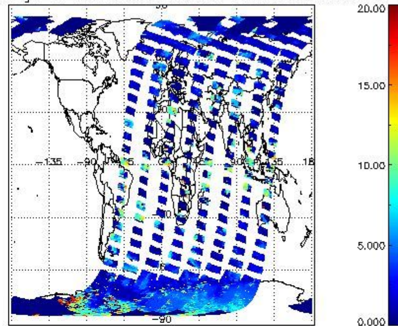
cL_top_height for 12MAR2011 00:00:00 to 13MAR2011 00:00:00
