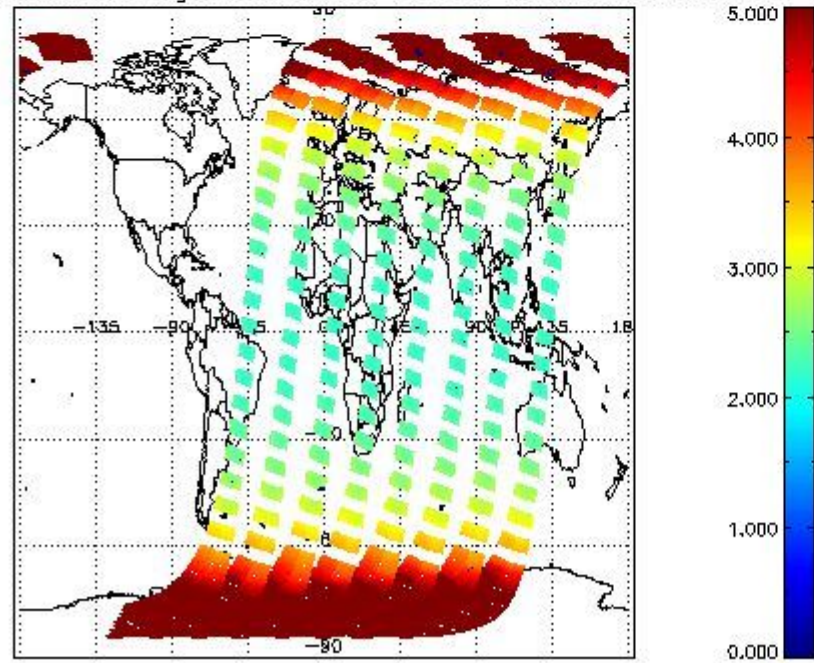
SCIOL2P_NADUV3BRO_amf_gr for 12MAR2011 00:00:00 to 13MAR2011 00:00:00
