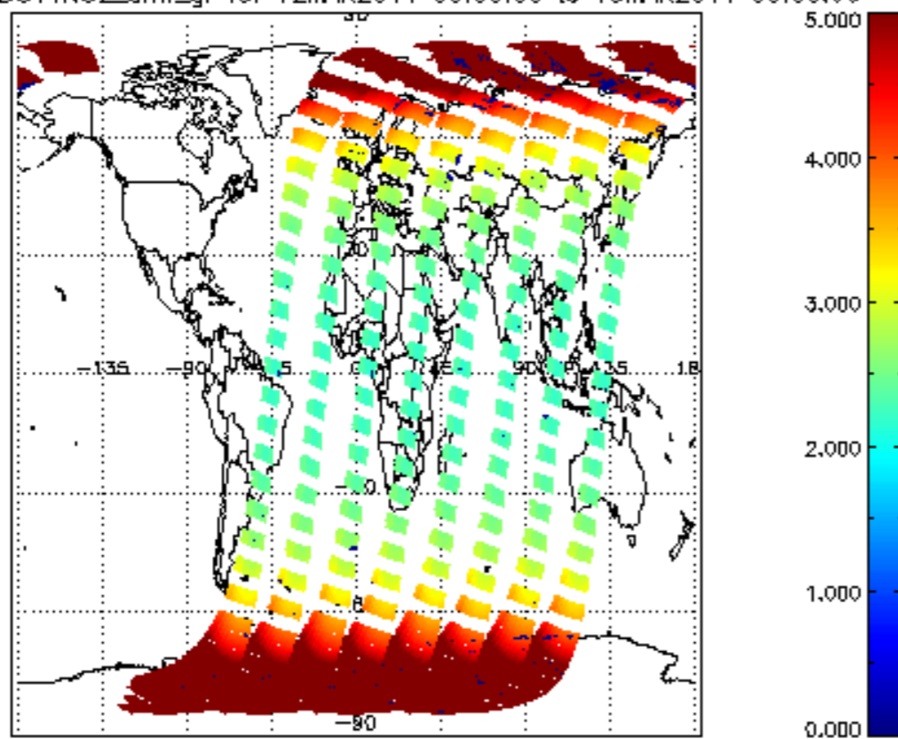
SCIOL2P_NADUV1NO2_amf_gr for 12MAR2011 00:00:00 to 13MAR2011 00:00:00
