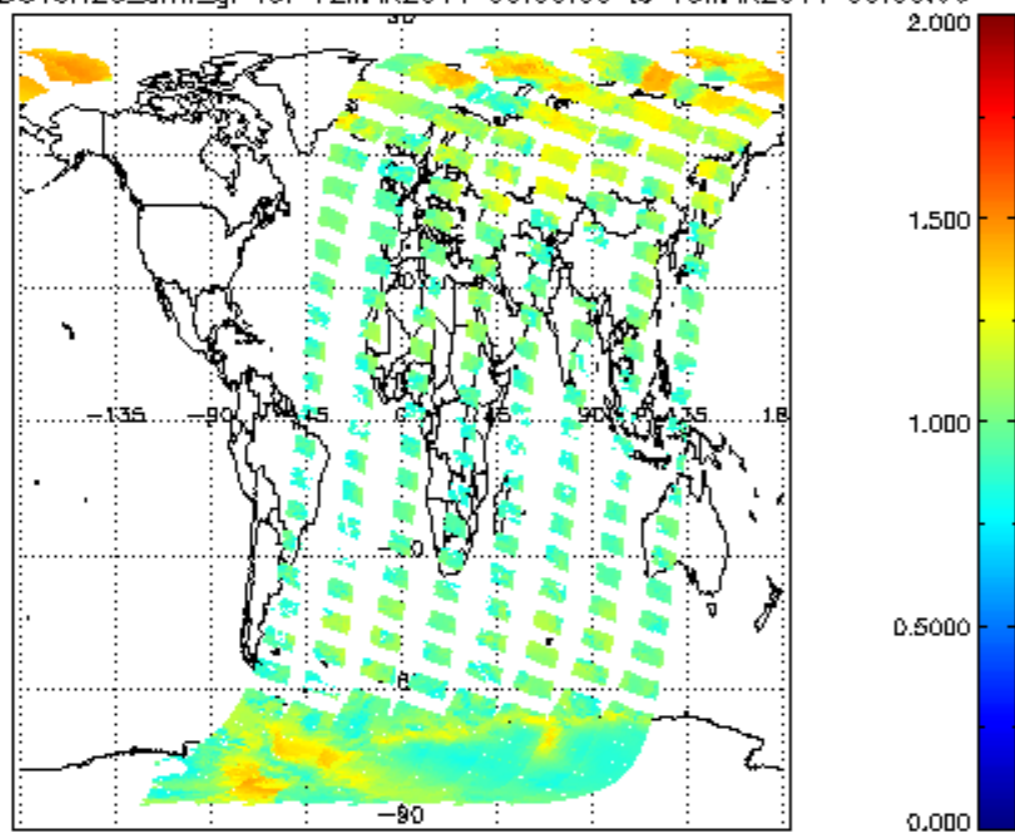
SCIOL2P_NADUV8H20_arnf_gr for 12MAR2011 00:00:00 to 13MAR2011 00:00:00
