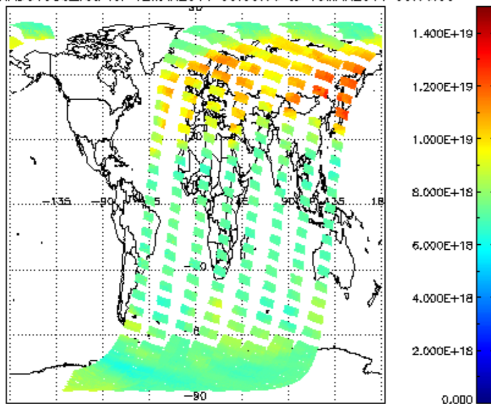
SCIOL2P_NADUV003_vcd for 12MAR2011 00:00:00 to 13MAR2011 00:00:00
