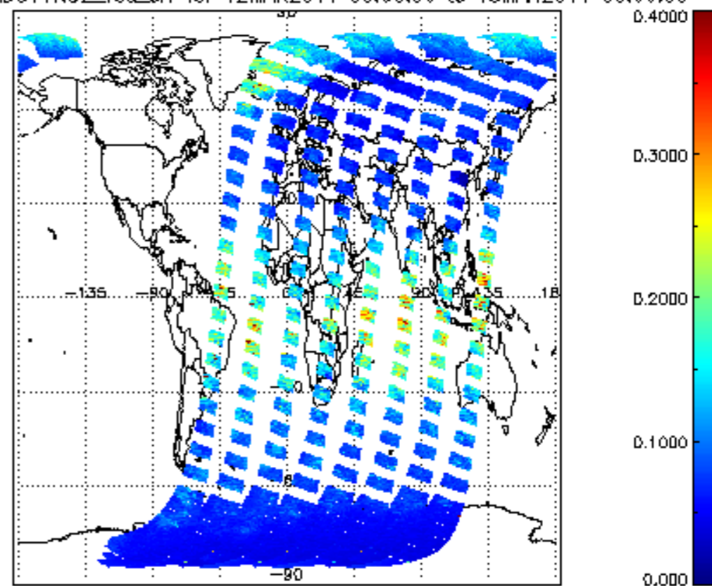
SCIOL2P_NADUV1NO2_vcd_err for 12MAR2011 00:00:00 to 13MAR2011 00:00:00
