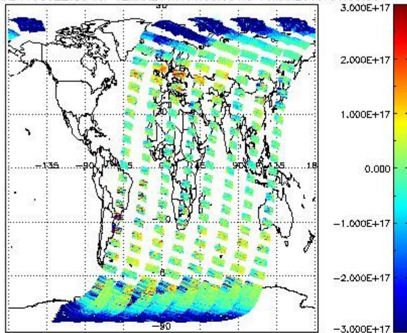
SCIOL2P_NADUV5S02_vcd for 12MAR2011 00:00:00 to 13MAR2011 00:00:00
