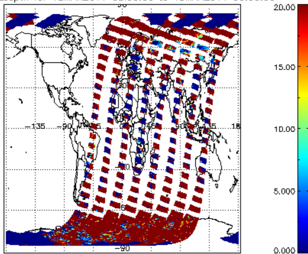
cL_opt_depth for 12MAR2011 00:00:00 to 13MAR2011 00:00:00
