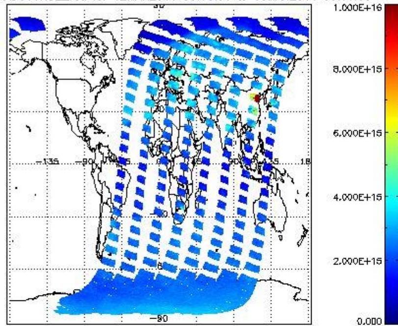
SCIOL2P_NADUV1NO2_vcd for 12MAR2011 00:00:00 to 13MAR2011 00:00:00
