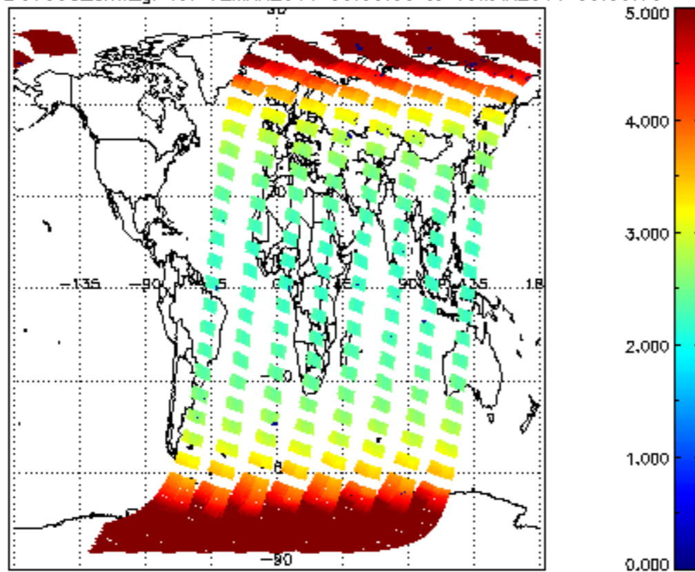
SCIOL2P_NADUV003_arnf_gr for 12MAR2011 00:00:00 to 13MAR2011 00:00:00
