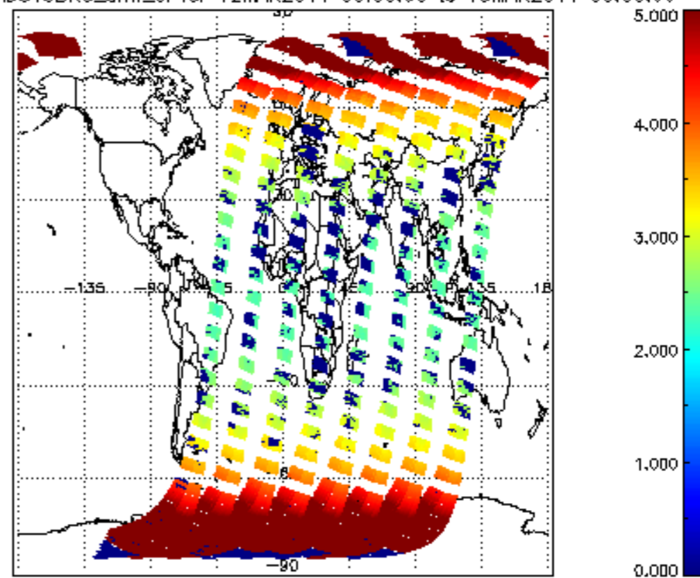
SCIOL2P_NADUV3BRO_amf_cl for 12MAR2011 00:00:00 to 13MAR2011 00:00:00
