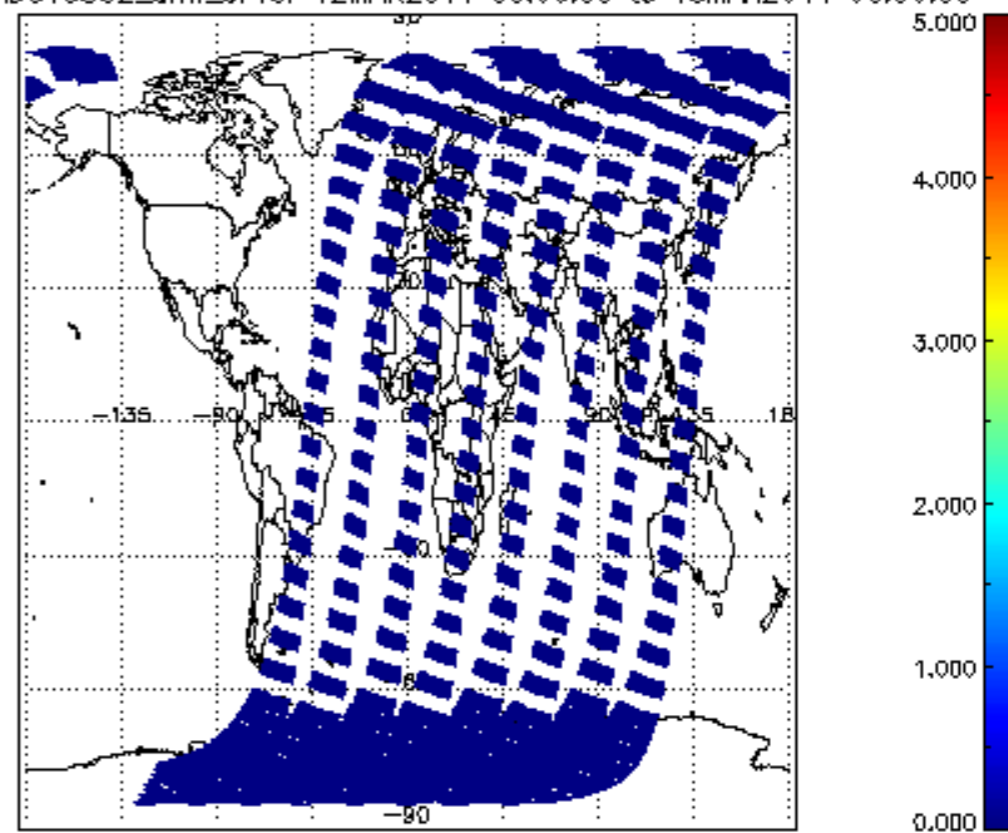
SCIOL2P_NADUV5S02_amf_cl for 12MAR2011 00:00:00 to 13MAR2011 00:00:00
