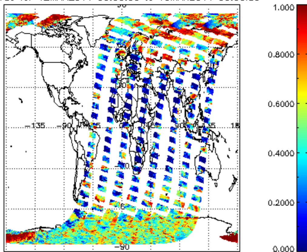
cL_frac for 12MAR2011 00:00:00 to 13MAR2011 00:00:00
