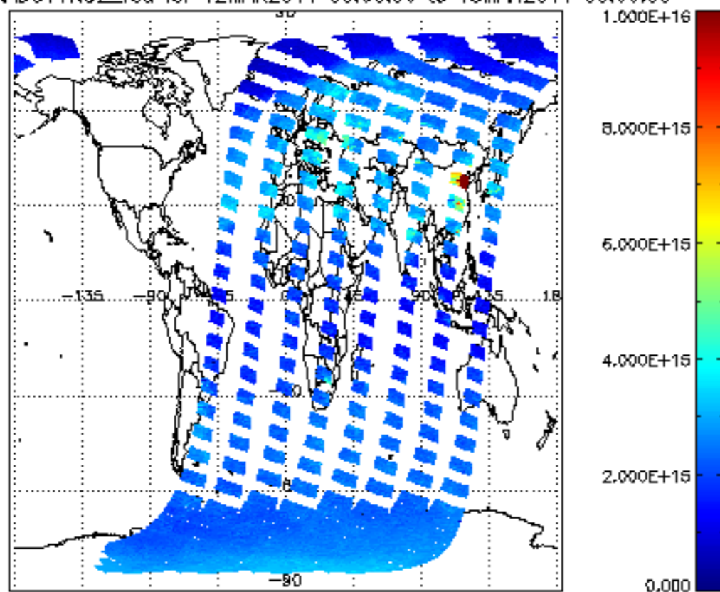
SCIOL2P_NADUV1NO2_vcd for 12MAR2011 00:00:00 to 13MAR2011 00:00:00
