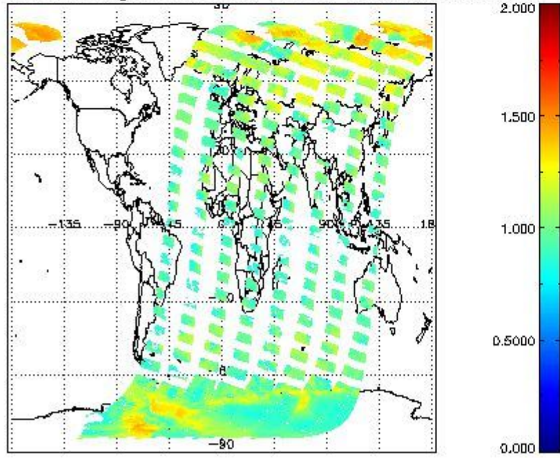
SCIOL2P_NADUV8H2O_amf_gr for 12MAR2011 00:00:00 to 13MAR2011 00:00:00
