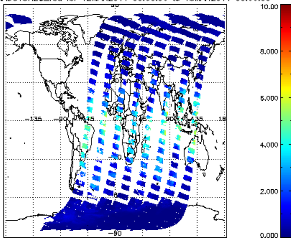
SCIOL2P_NADUV8H20_vcd for 12MAR2011 00:00:00 to 13MAR2011 00:00:00
