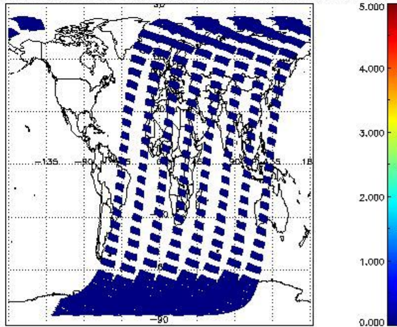
SCIOL2P_NADUV5S02_amf_cl for 12MAR2011 00:00:00 to 13MAR2011 00:00:00
