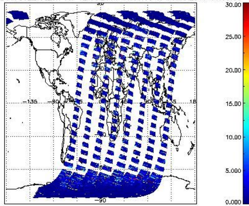
SCIOL2P_NADUV7S02_vcd_err for 12MAR2011 00:00:00 to 13MAR2011 00:00:00
