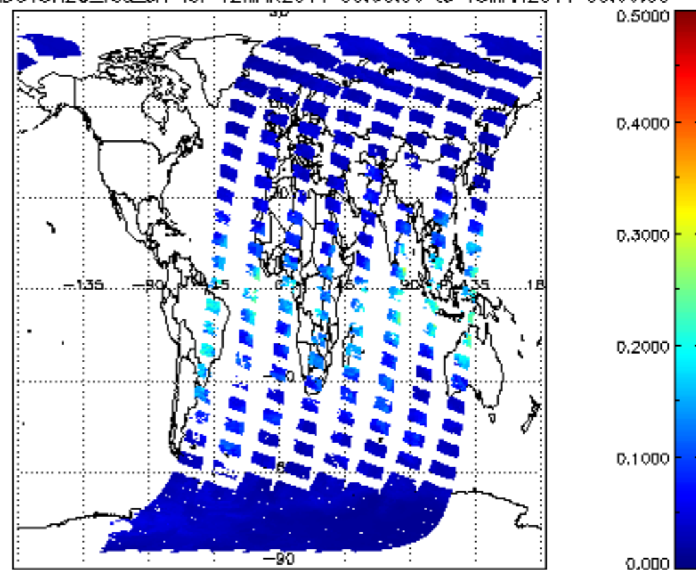
SCIOL2P_NADUV8H20_vcd_err for 12MAR2011 00:00:00 to 13MAR2011 00:00:00
