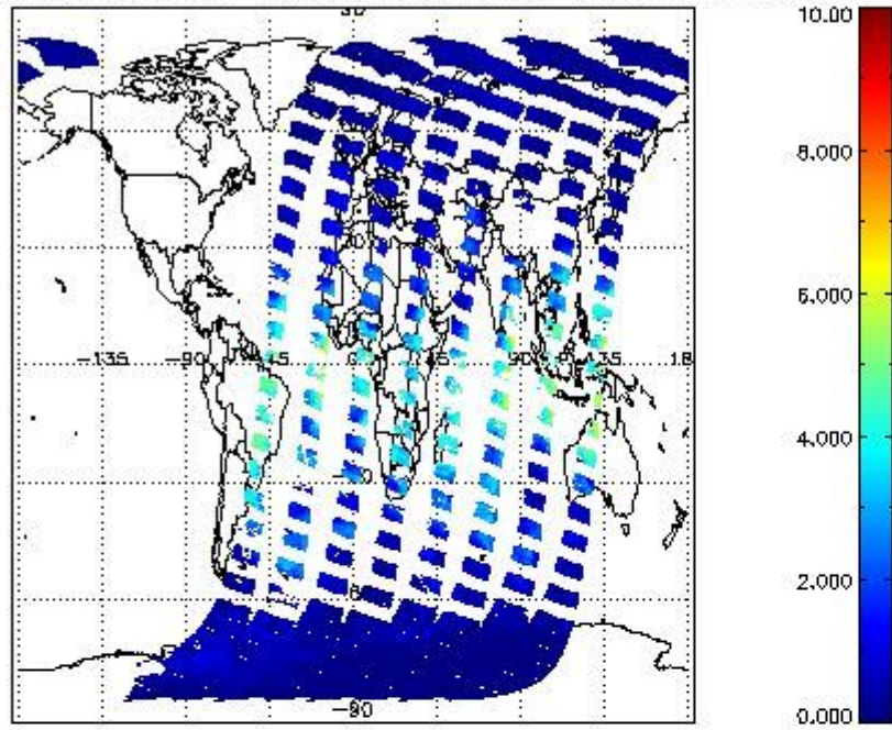
SCIOL2P_NADUV8H2O_vcd for 12MAR2011 00:00:00 to 13MAR2011 00:00:00
