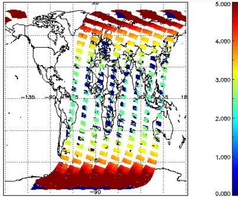
SCIOL2P_NADUV3BRO_amf_cl for 12MAR2011 00:00:00 to 13MAR2011 00:00:00
