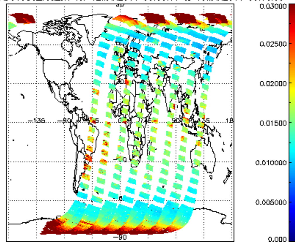
SCIOL2P_NADUV003_vcd_err for 12MAR2011 00:00:00 to 13MAR2011 00:00:00
