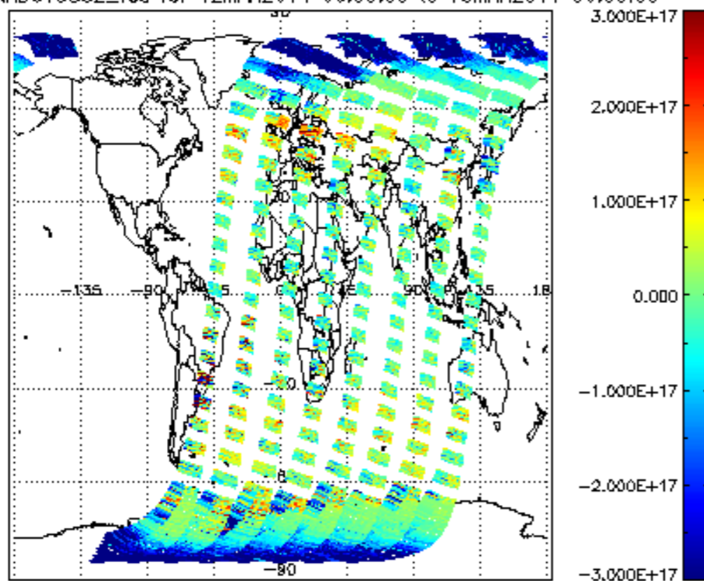
SCIOL2P_NADUV5S02_vcd for 12MAR2011 00:00:00 to 13MAR2011 00:00:00
