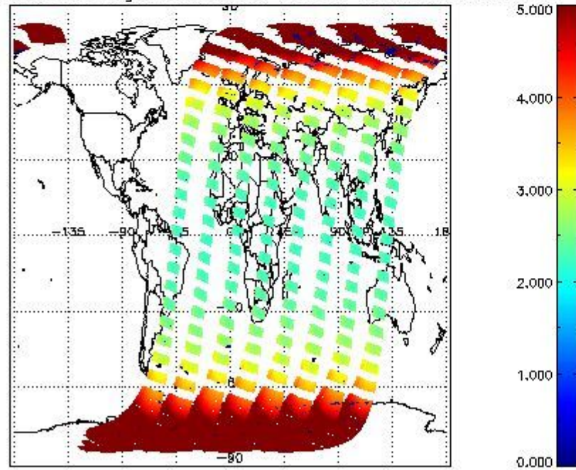
SCIOL2P_NADUV1NO2_amf_gr for 12MAR2011 00:00:00 to 13MAR2011 00:00:00
