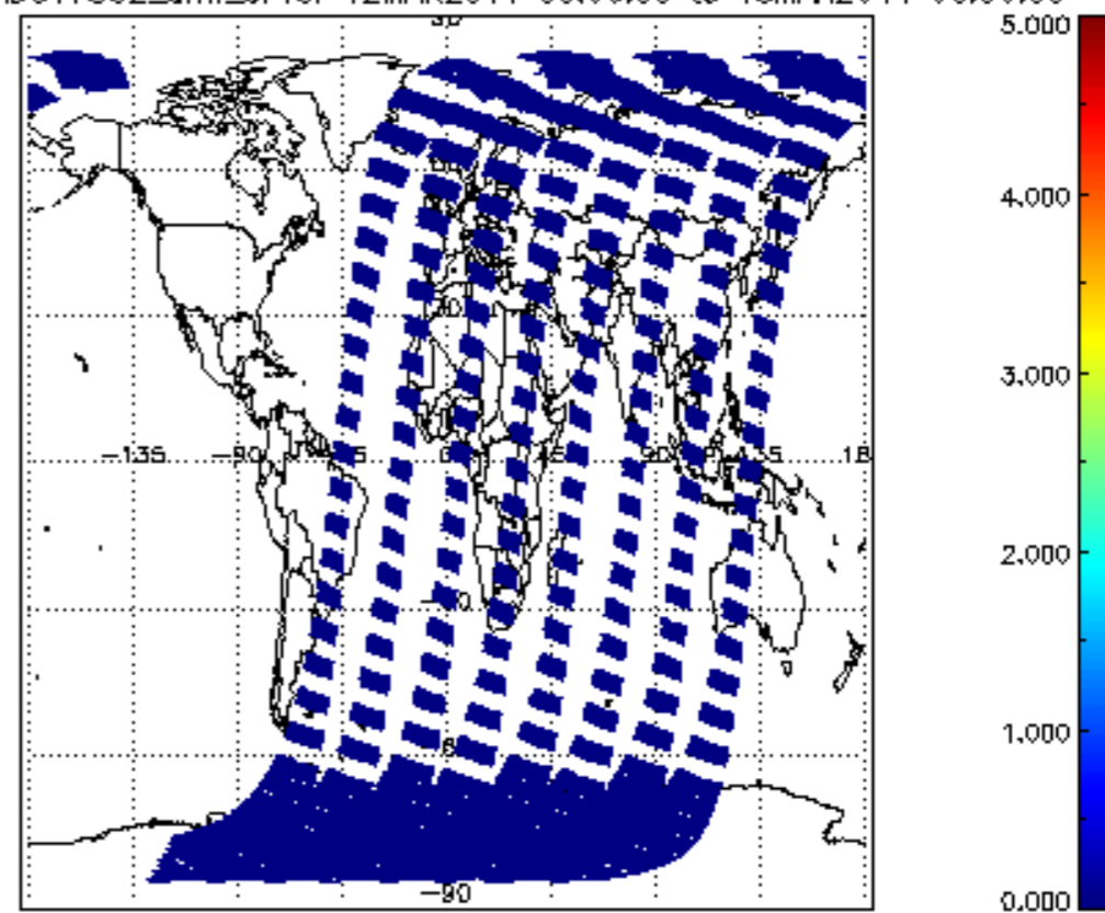
SCIOL2P_NADUV7S02_amf_cl for 12MAR2011 00:00:00 to 13MAR2011 00:00:00
