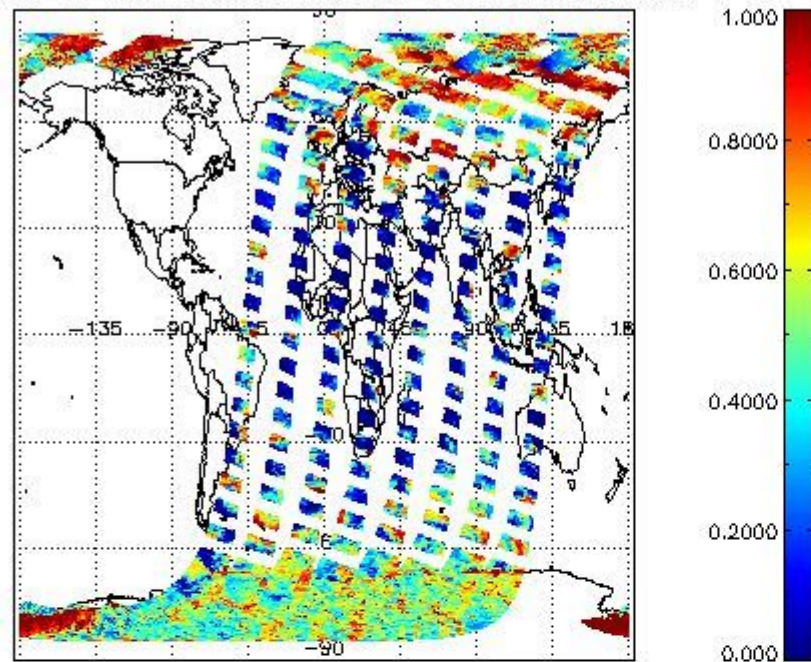
cL_frac for 12MAR2011 00:00:00 to 13MAR2011 00:00:00
