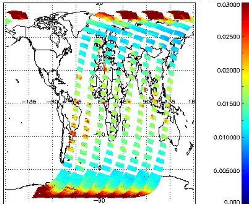
SCIOL2P_NADUV003_vcd_err for 12MAR2011 00:00:00 to 13MAR2011 00:00:00
