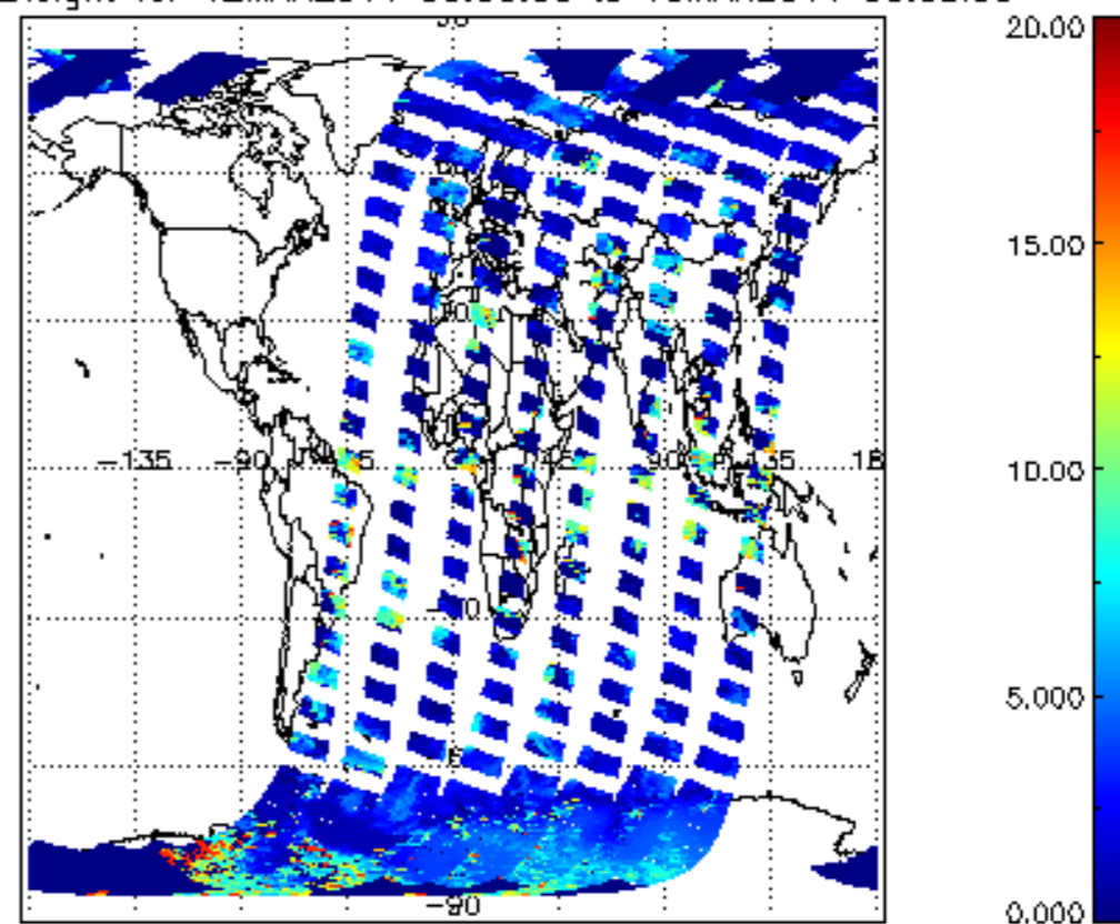
cL_top_height for 12MAR2011 00:00:00 to 13MAR2011 00:00:00
