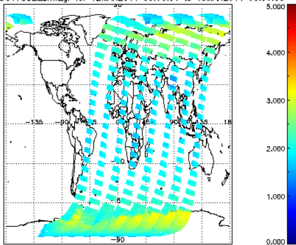
SCIOL2P_NADUV7S02_amf_gr for 12MAR2011 00:00:00 to 13MAR2011 00:00:00
