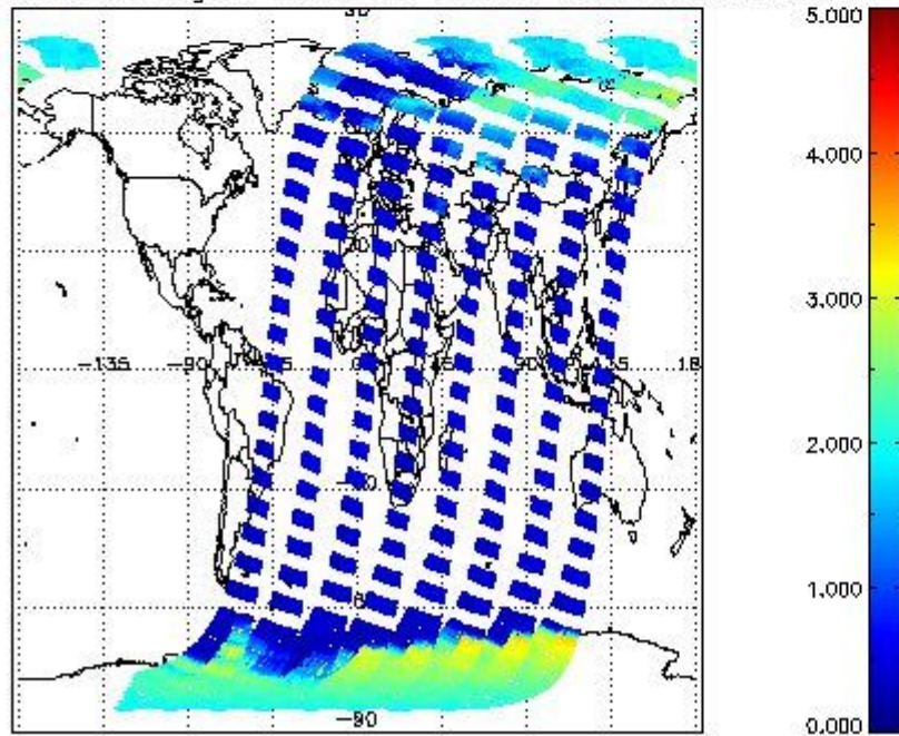
SCIOL2P_NADUV5S02_amf_gr for 12MAR2011 00:00:00 to 13MAR2011 00:00:00
