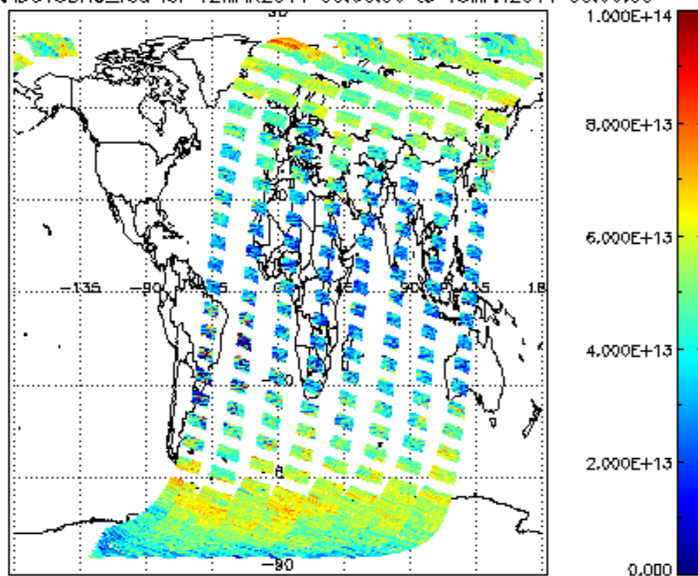
SCIOL2P_NADUV3BRO_vcd for 12MAR2011 00:00:00 to 13MAR2011 00:00:00
