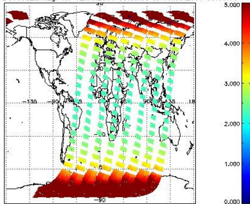
SCIOL2P_NADUV003_amf_gr for 12MAR2011 00:00:00 to 13MAR2011 00:00:00
