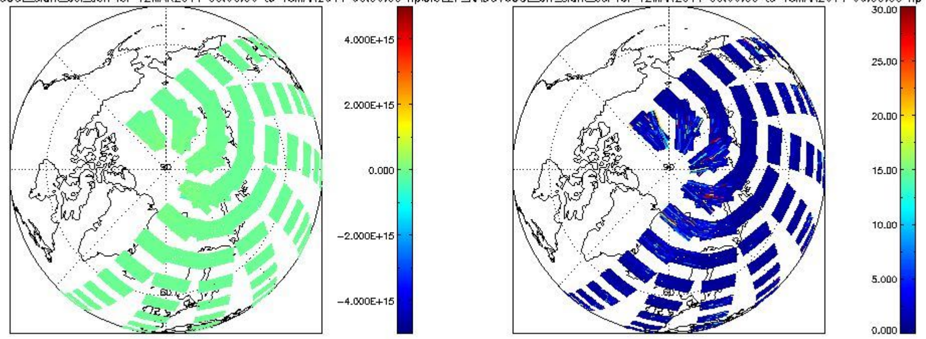
CIOL2P_NADUV6OCL_slant_col_den for 12MAR2011 00:00:00 to 13MAR2011 00:00:00 np CIOL2P_NADUV6OCL_err_slant_col for 12MAR2011 00:00:00 to 13MAR2011 00:00:00 np
