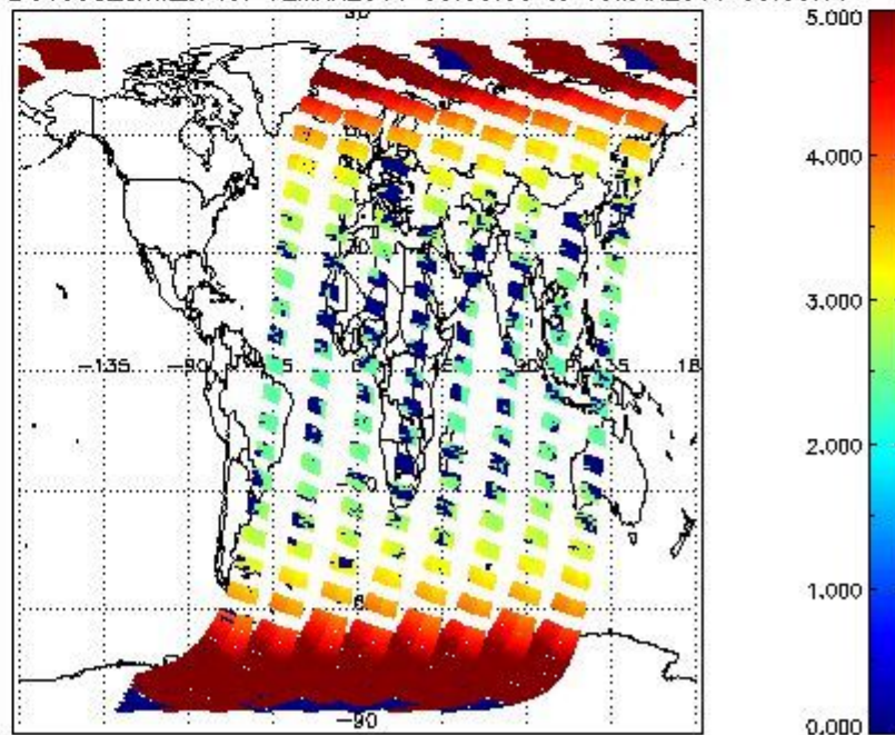
SCIOL2P_NADUV003_amf_cl for 12MAR2011 00:00:00 to 13MAR2011 00:00:00
