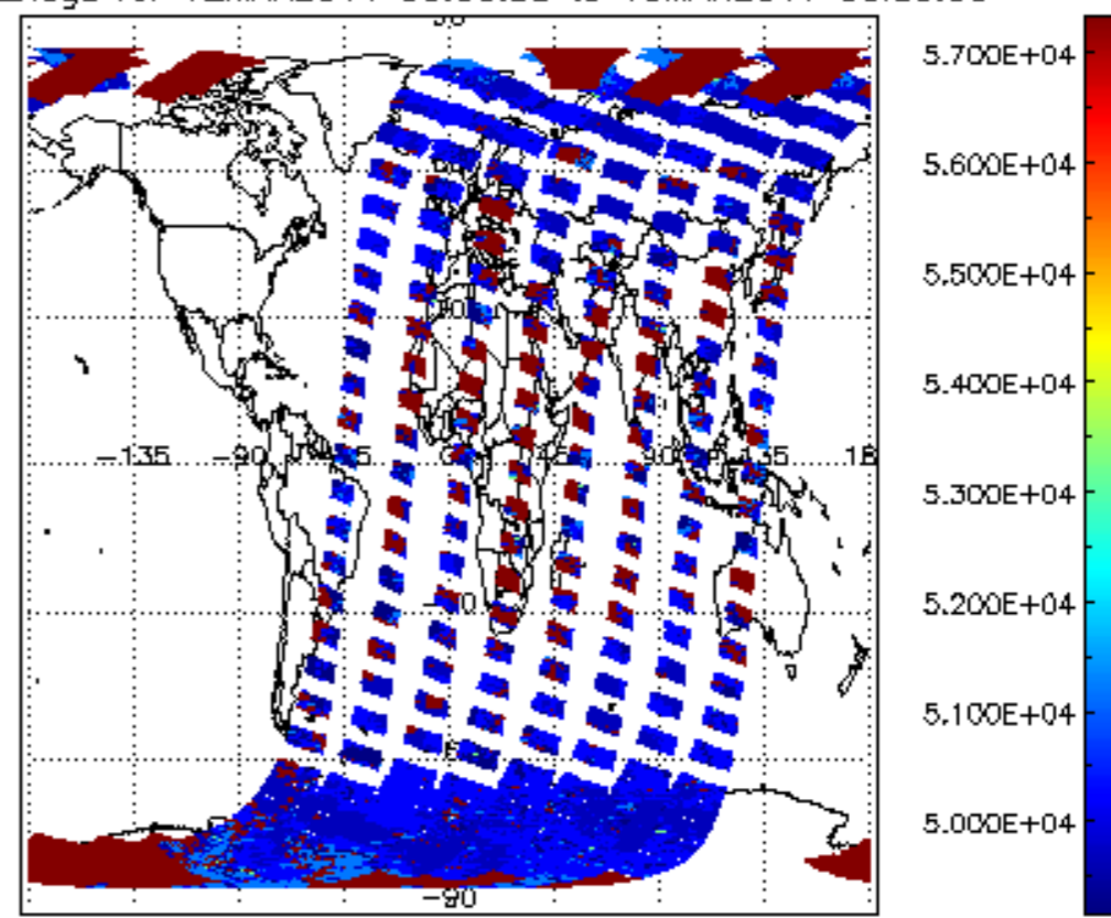
cloud_flags for 12MAR2011 00:00:00 to 13MAR2011 00:00:00
