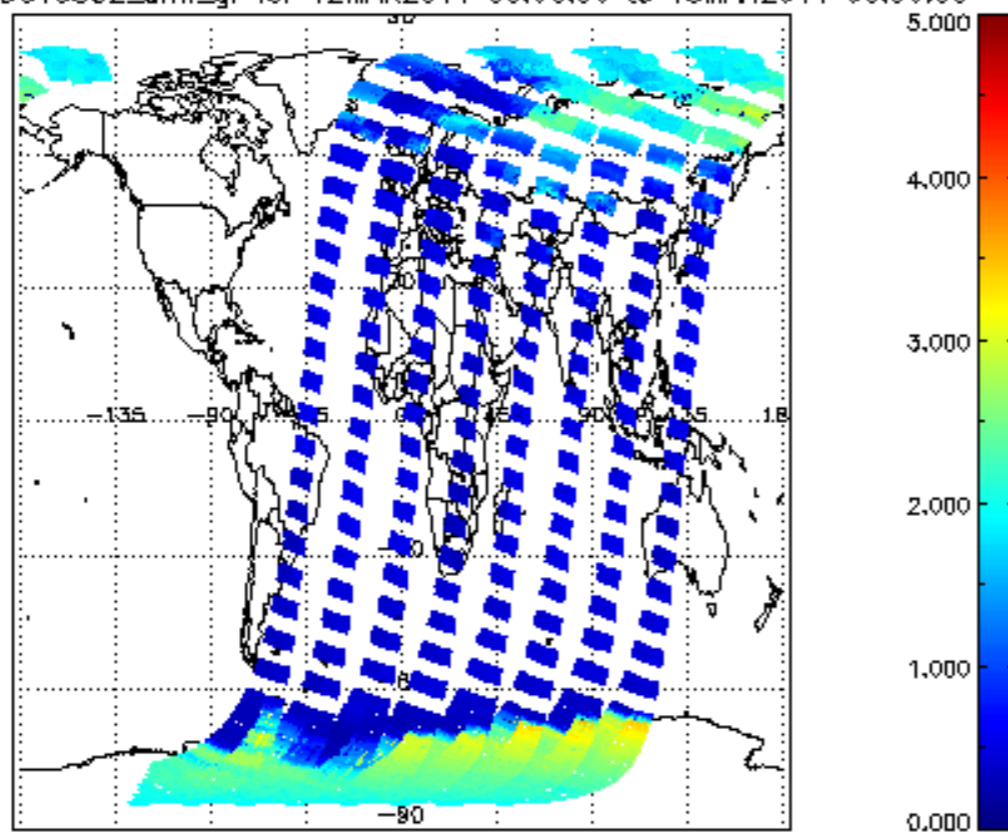
SCIOL2P_NADUV5S02_amf_gr for 12MAR2011 00:00:00 to 13MAR2011 00:00:00
