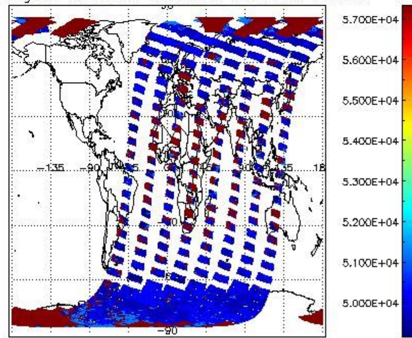
cloud_flags for 12MAR2011 00:00:00 to 13MAR2011 00:00:00
