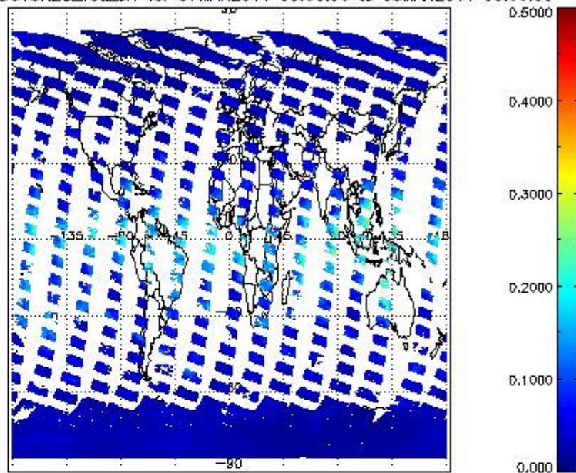
SCIOL2P_NADUV8H2O_vcd_err for 07MAR2011 00:00:00 to 08MAR2011 00:00:00
