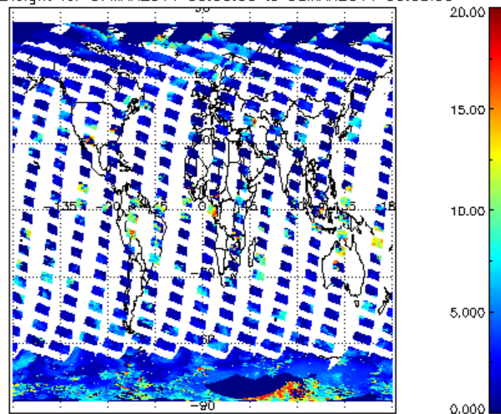
cL_top_height for 07MAR2011 00:00:00 to 08MAR2011 00:00:00
