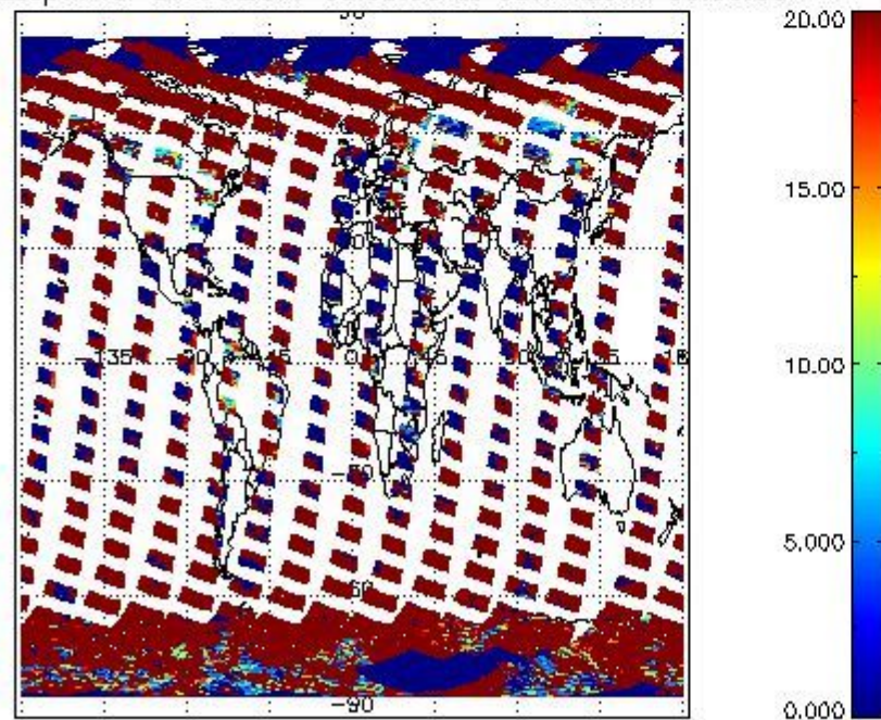
cL_opt_depth for 07MAR2011 00:00:00 to 08MAR2011 00:00:00
