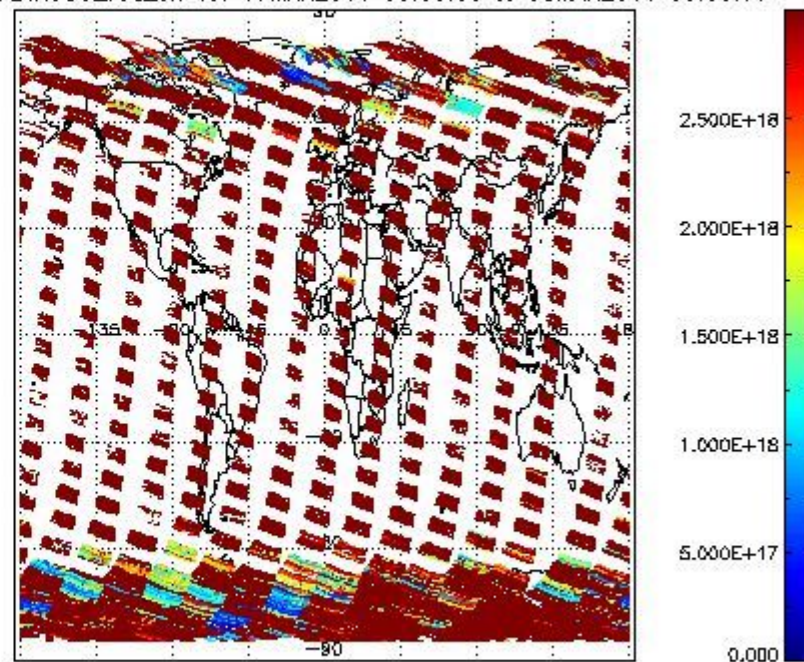
SCIDL2P_NADIR3CO_vcd_err for 07MAR2011 00:00:00 to 08MAR2011 00:00:00
