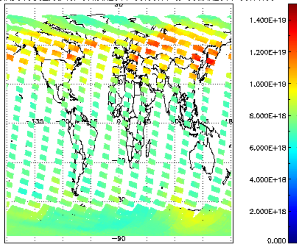
SCIOL2P_NADUV003_vcd for 07MAR2011 00:00:00 to 08MAR2011 00:00:00
