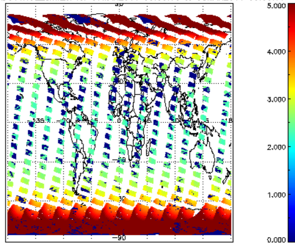
SCIOL2P_NADUV1NO2_amf_cl for 07MAR2011 00:00:00 to 08MAR2011 00:00:00
