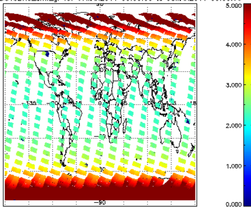
SCIOL2P_NADUV3BRO_arnf_gr for 07MAR2011 00:00:00 to 08MAR2011 00:00:00
