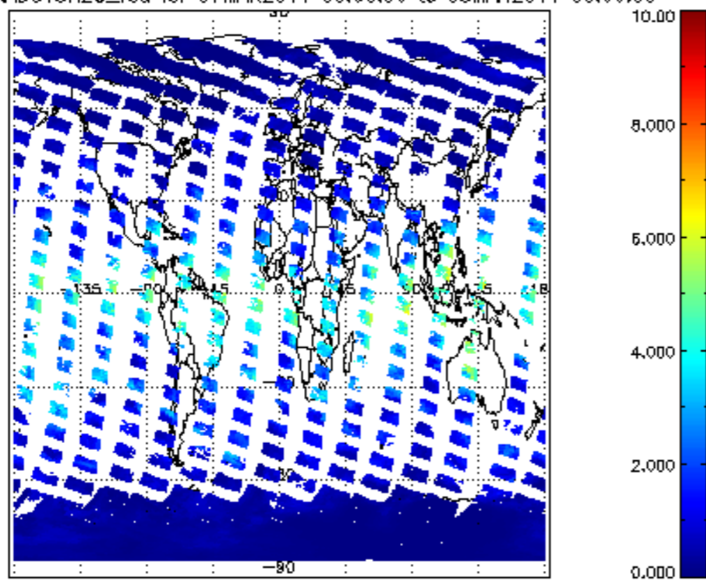
SCIOL2P_NADUV8H20_vcd for 07MAR2011 00:00:00 to 08MAR2011 00:00:00
