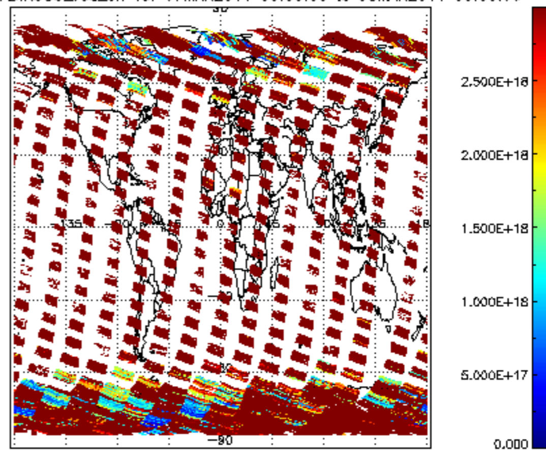
SCIOL2P_NADIR3CO_vcd_err for 07MAR2011 00:00:00 to 08MAR2011 00:00:00
