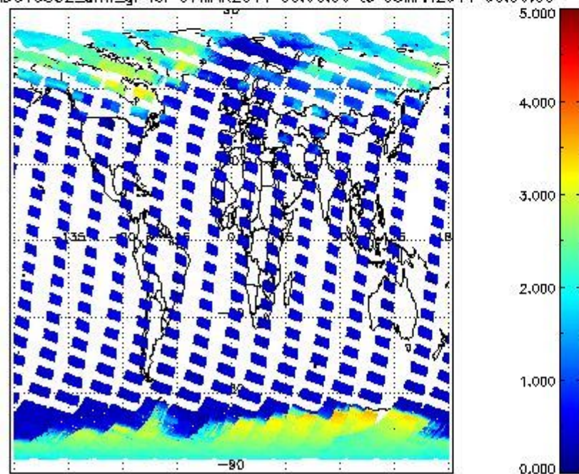
SCIOL2P_NADUV5SO2_amf_gr for 07MAR2011 00:00:00 to 08MAR2011 00:00:00
