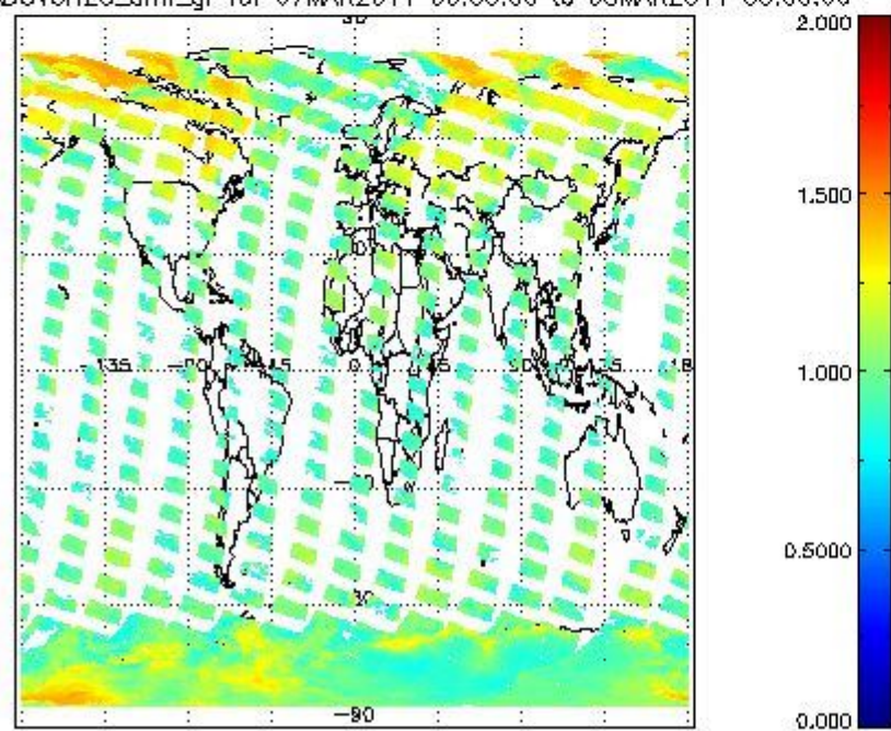
SCIOL2P_NADUV8H2O_arnf_gr for 07MAR2011 00:00:00 to 08MAR2011 00:00:00
