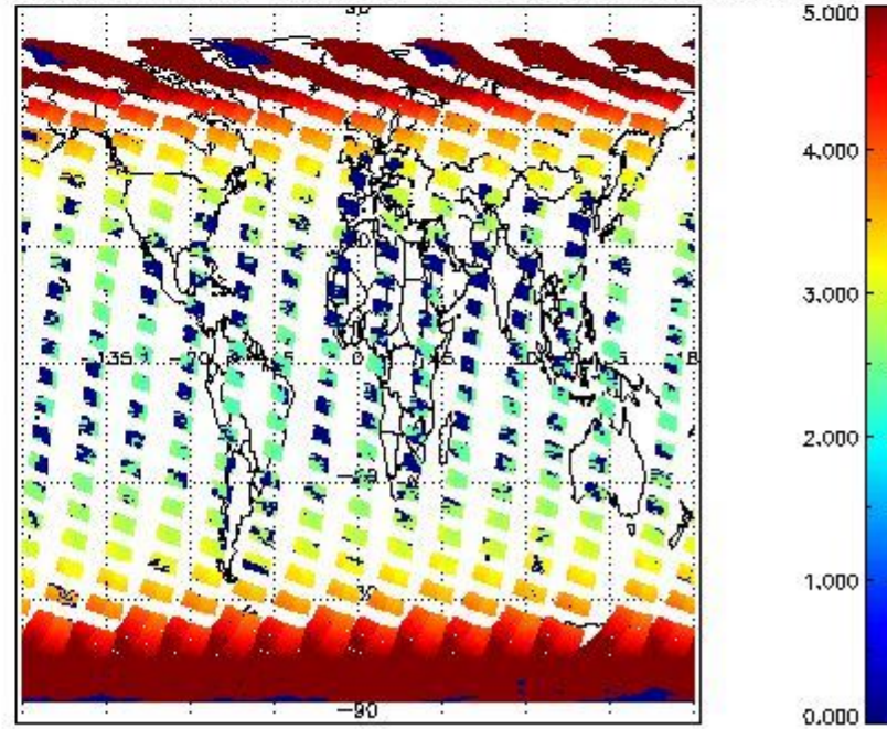
SCIOL2P_NADUV003_amf_cl for 07MAR2011 00:00:00 to 08MAR2011 00:00:00
