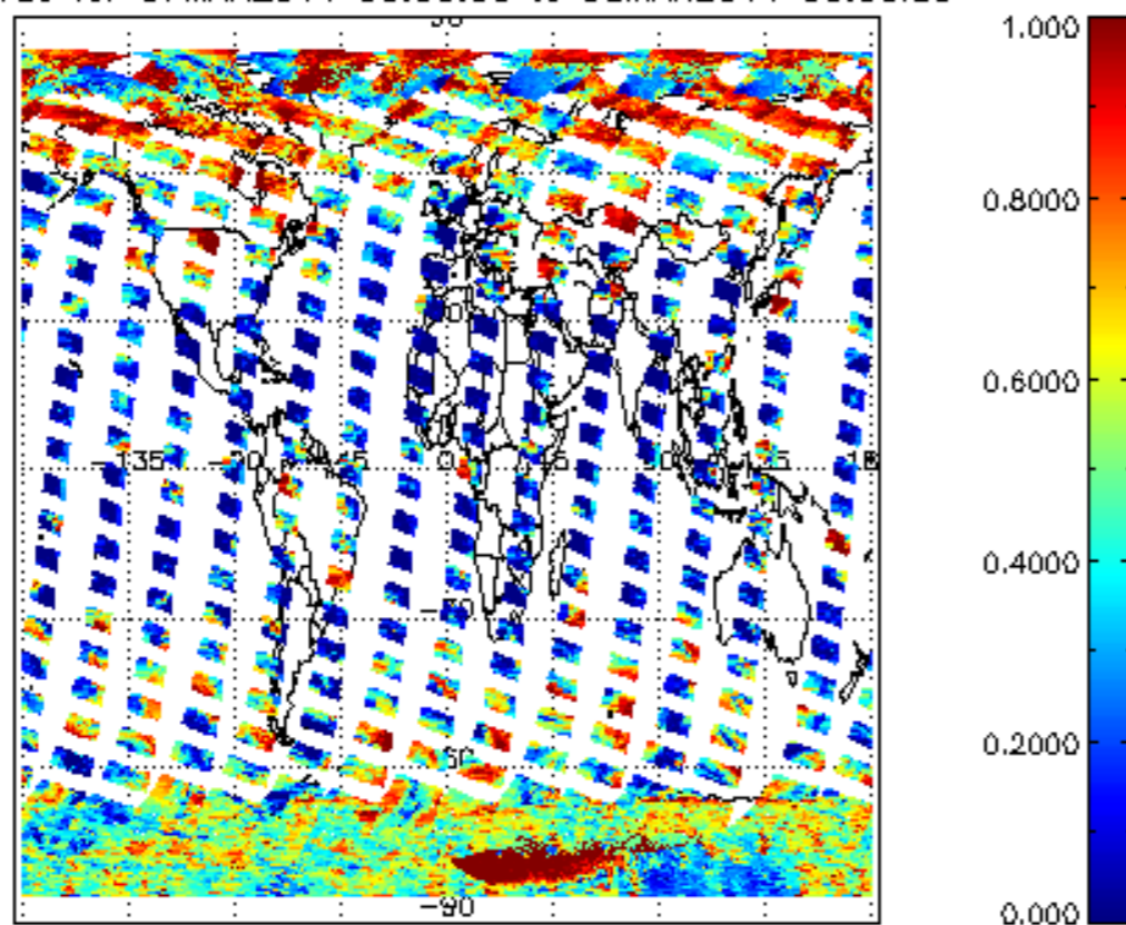
cL_frac for 07MAR2011 00:00:00 to 08MAR2011 00:00:00
