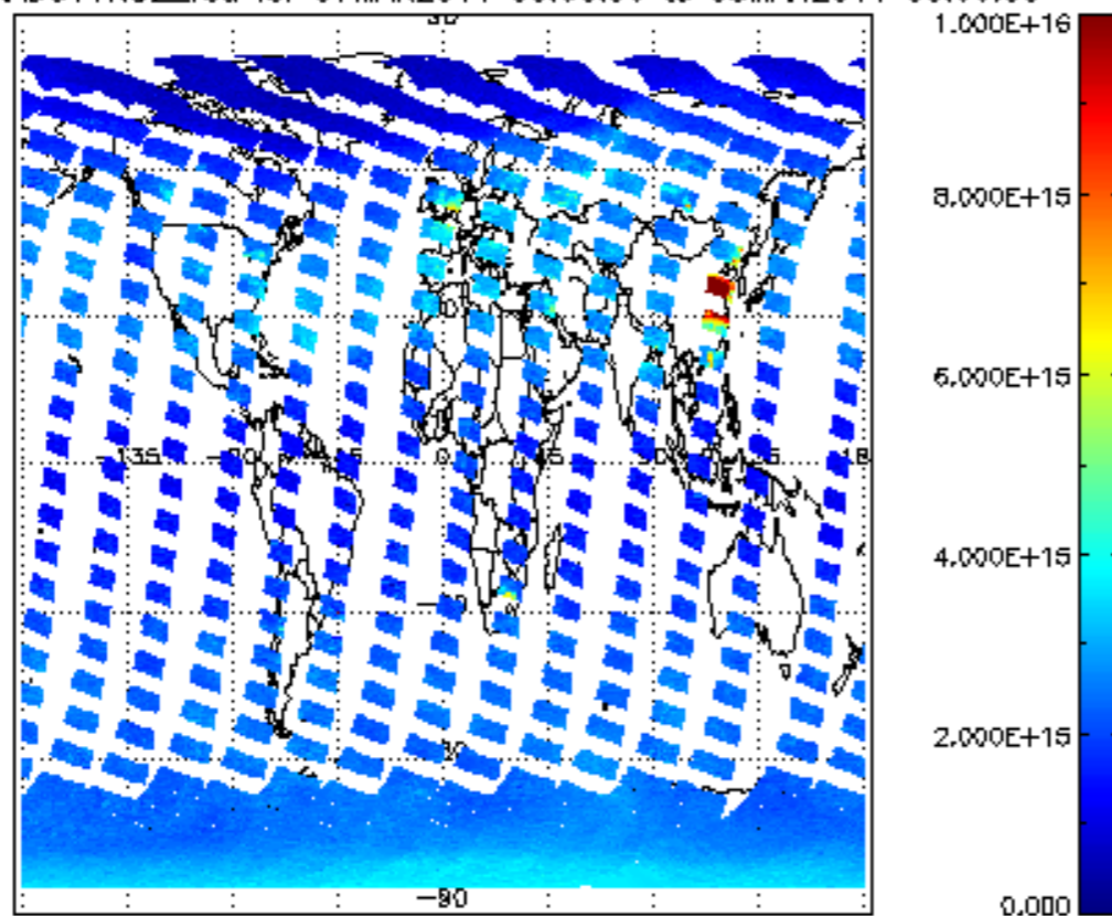
SCIOL2P_NADUV1NO2_vcd for 07MAR2011 00:00:00 to 08MAR2011 00:00:00
