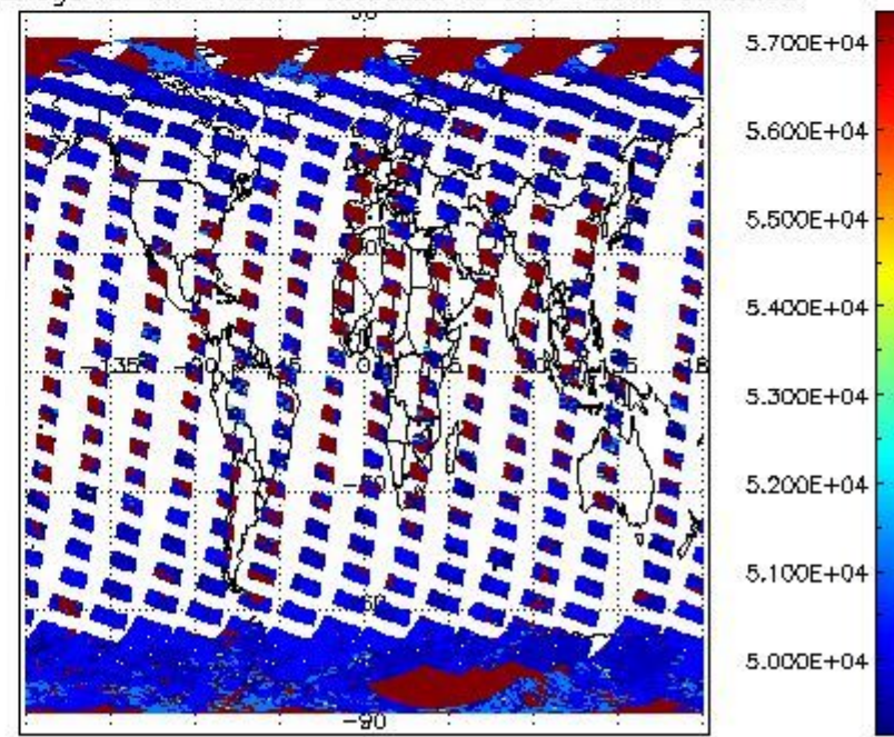
cloud_flags for 07MAR2011 00:00:00 to 08MAR2011 00:00:00
