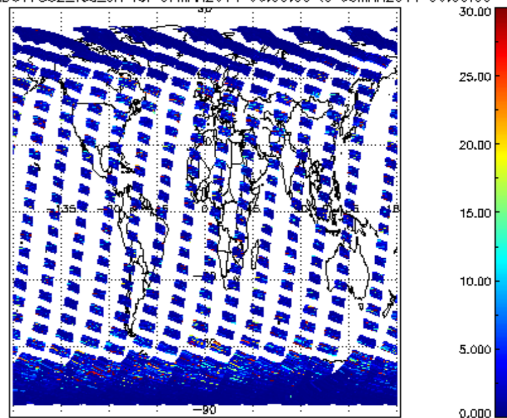
SCIOL2P_NADUV7S02_vcd_err for 07MAR2011 00:00:00 to 08MAR2011 00:00:00
