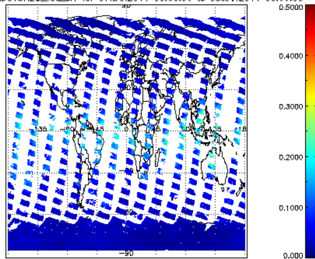
SCIOL2P_NADUV8H20_vcd_Lerr for 07MAR2011 00:00:00 to 08MAR2011 00:00:00
