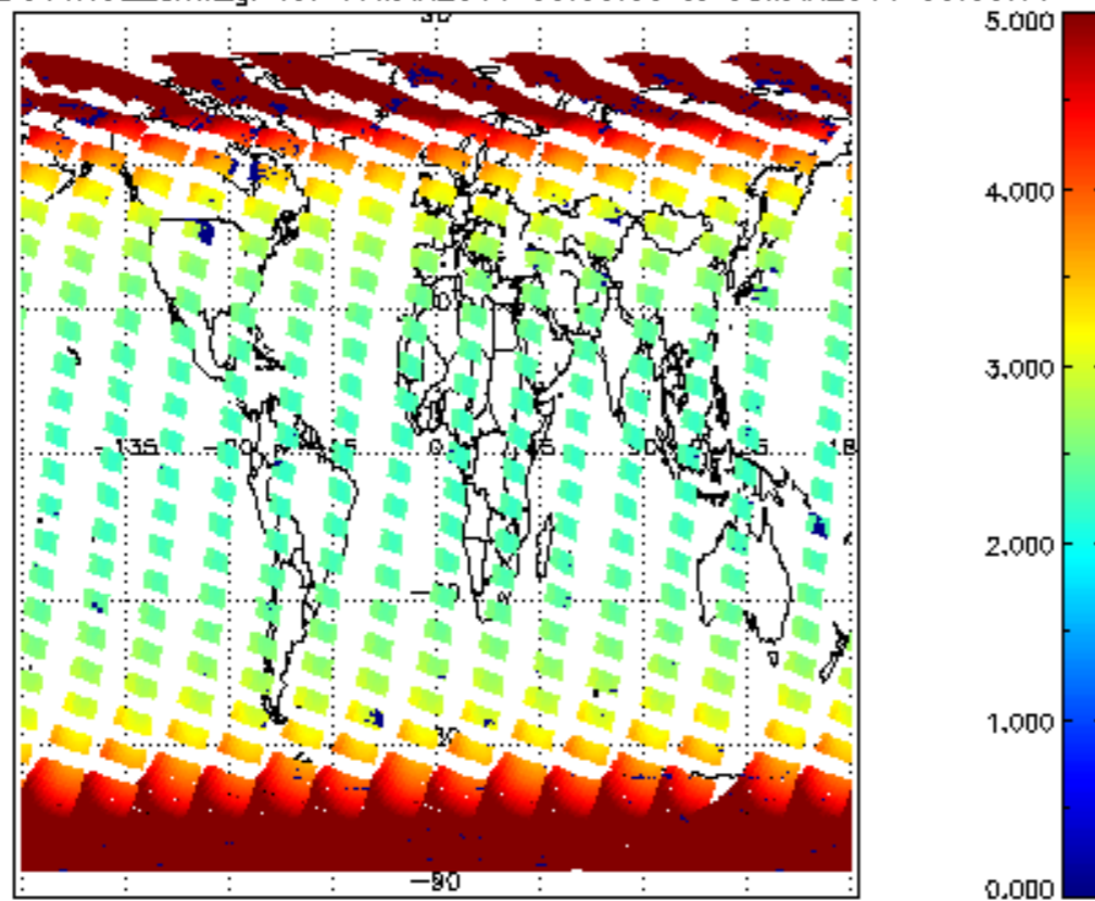
SCIOL2P_NADUV1NO2_amf_gr for 07MAR2011 00:00:00 to 08MAR2011 00:00:00
