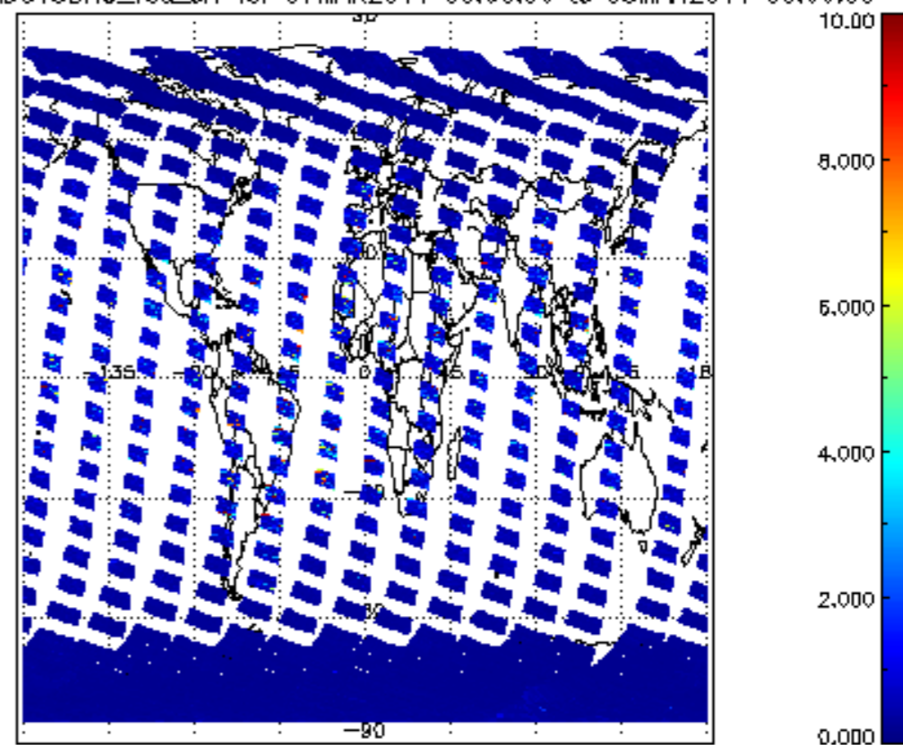
SCIOL2P_NADUV3BRO_vcd_err for 07MAR2011 00:00:00 to 08MAR2011 00:00:00
