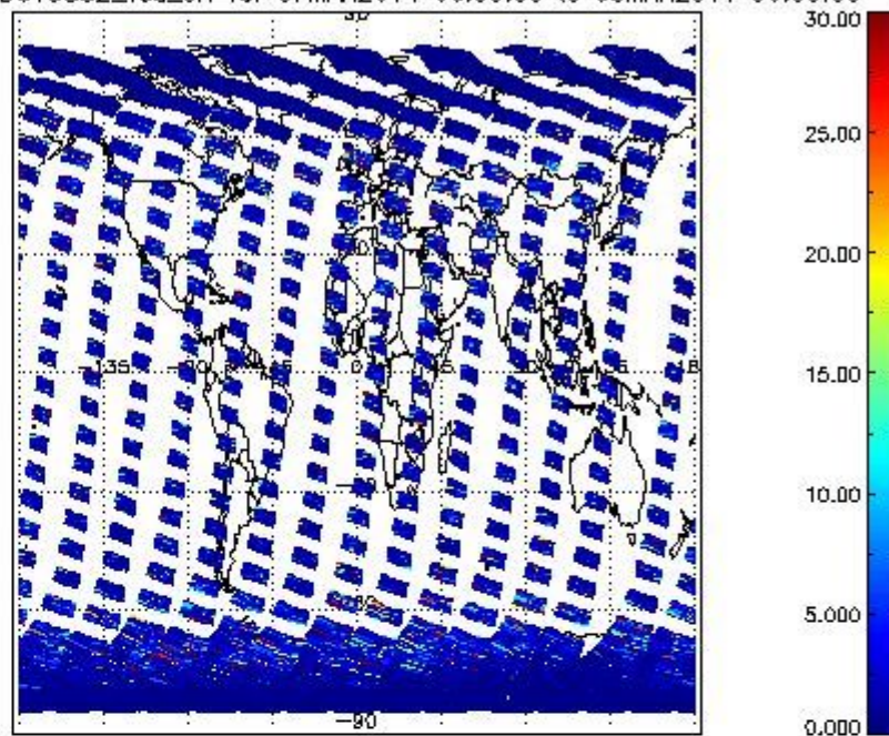
SCIOL2P_NADUV5SO2_vcd_err for 07MAR2011 00:00:00 to 08MAR2011 00:00:00
