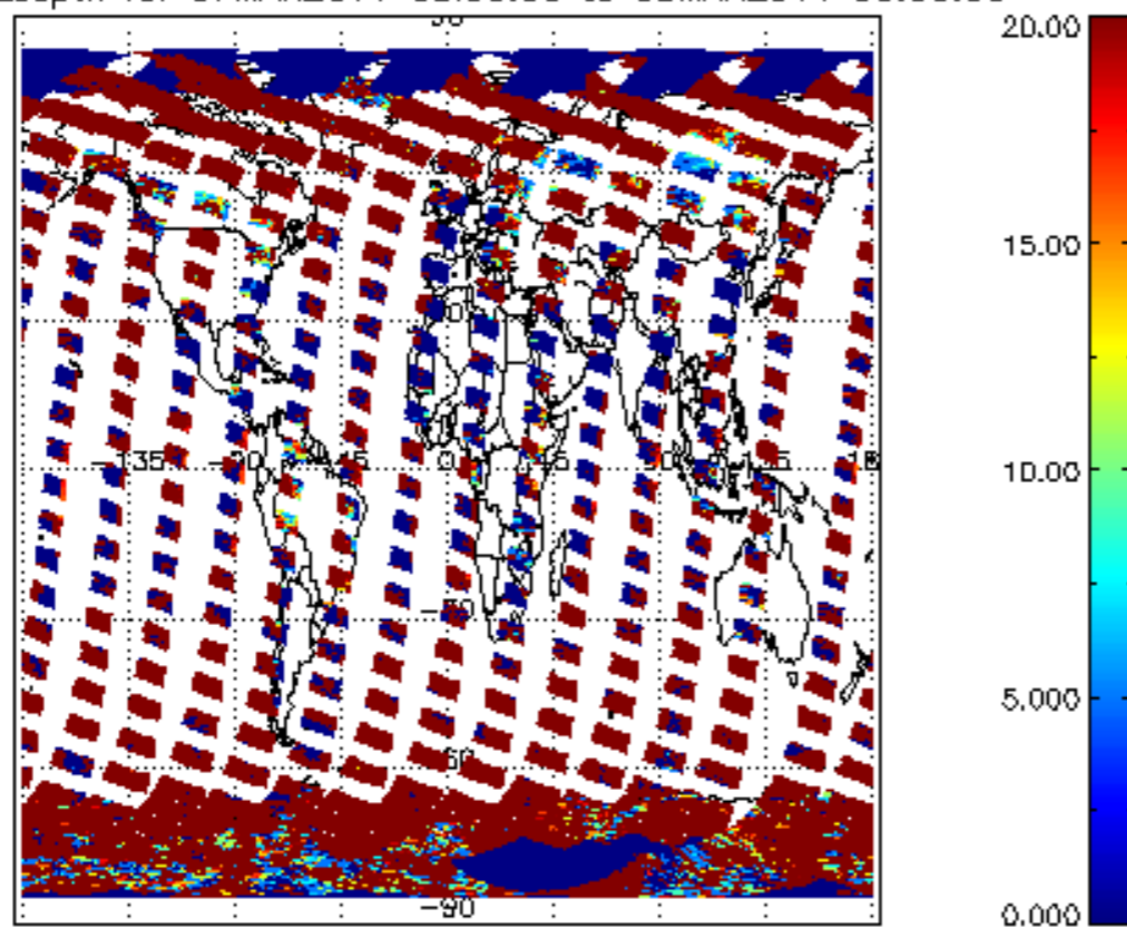
cL_opt_depth for 07MAR2011 00:00:00 to 08MAR2011 00:00:00
