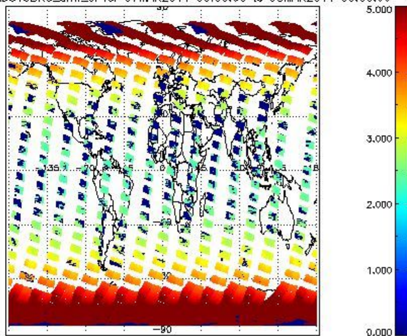
SCIOL2P_NADUV3BRO_amf_cl for 07MAR2011 00:00:00 to 08MAR2011 00:00:00
