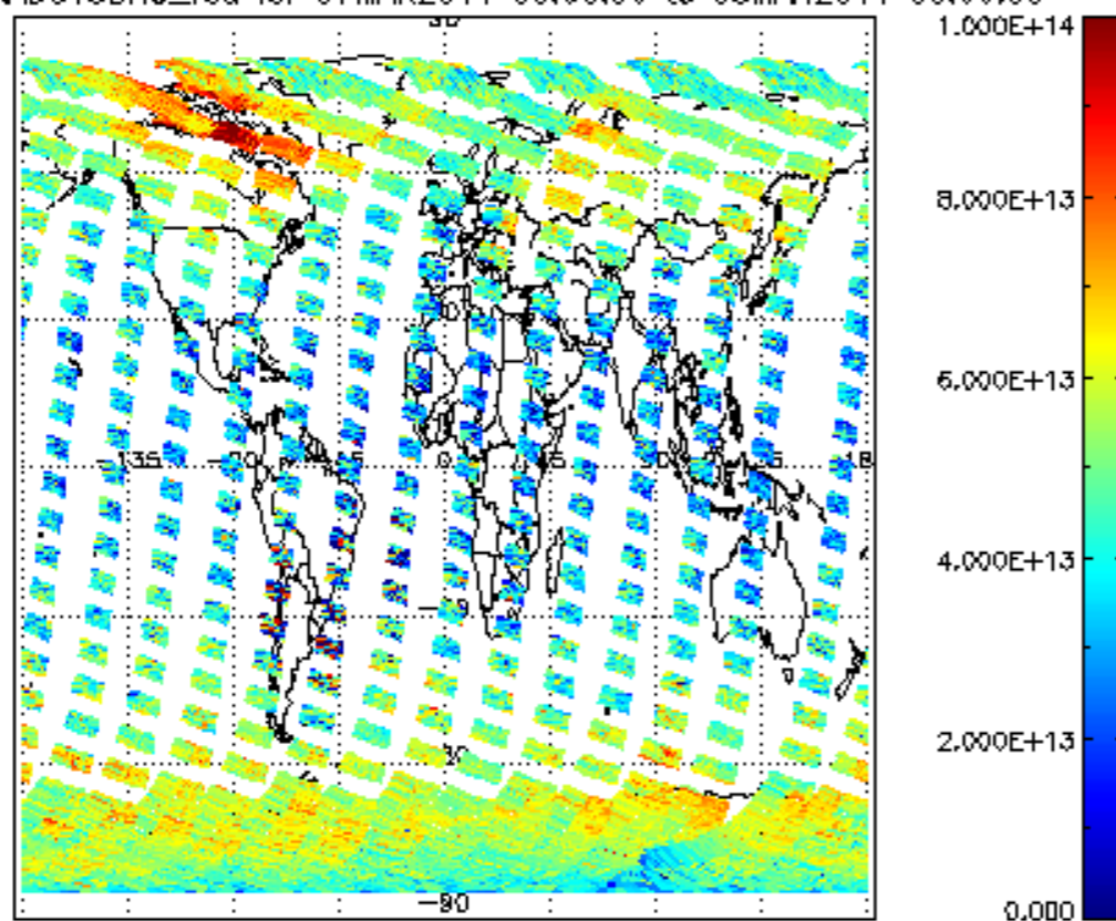
SCIOL2P_NADUV3BRO_vcd for 07MAR2011 00:00:00 to 08MAR2011 00:00:00
