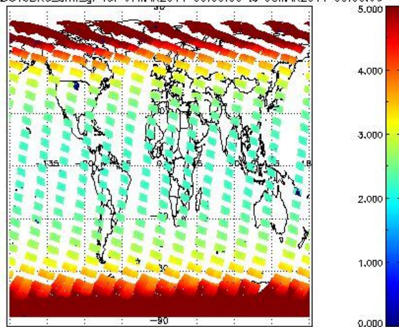
SCIOL2P_NADUV3BRO_amf_gr for 07MAR2011 00:00:00 to 08MAR2011 00:00:00
