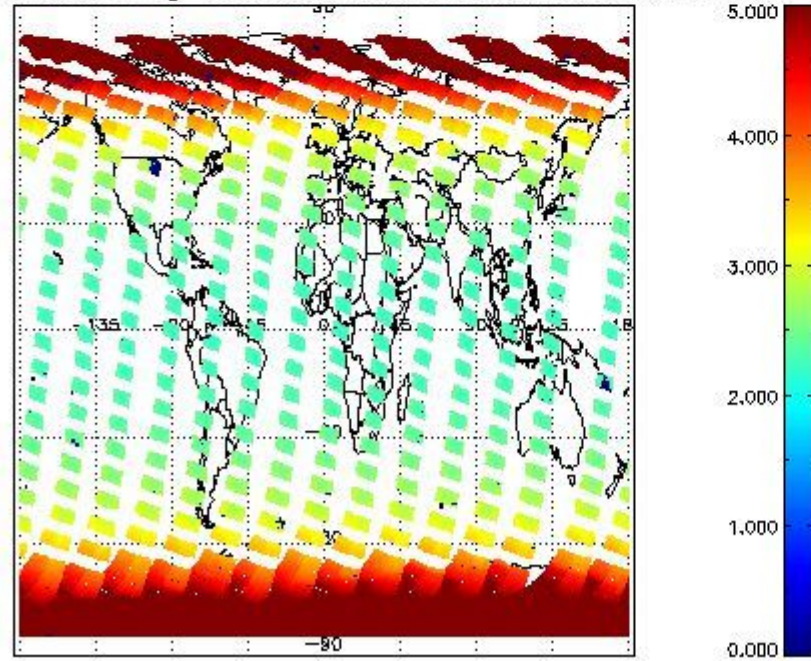
SCIOL2P_NADUV003_amf_gr for 07MAR2011 00:00:00 to 08MAR2011 00:00:00
