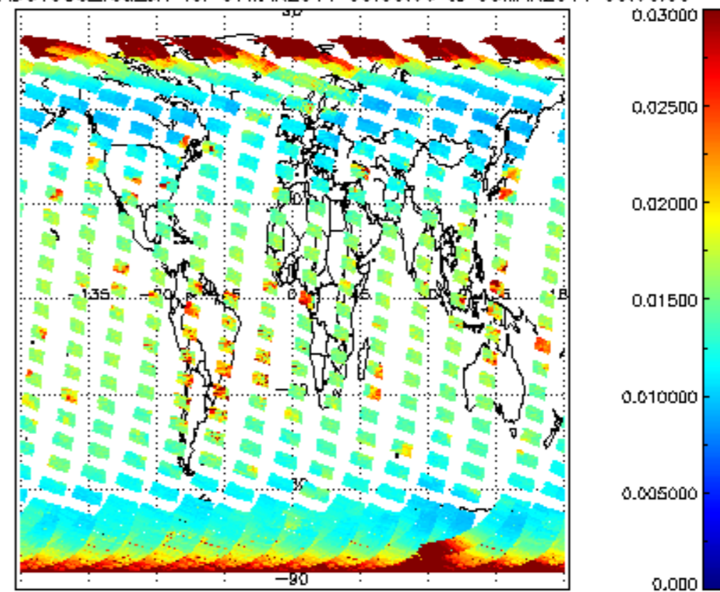
SCIOL2P_NADUV003_vcd_err for 07MAR2011 00:00:00 to 08MAR2011 00:00:00
