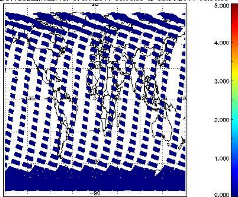
SCIOL2P_NADUV7S02_amf_cl for 07MAR2011 00:00:00 to 08MAR2011 00:00:00
