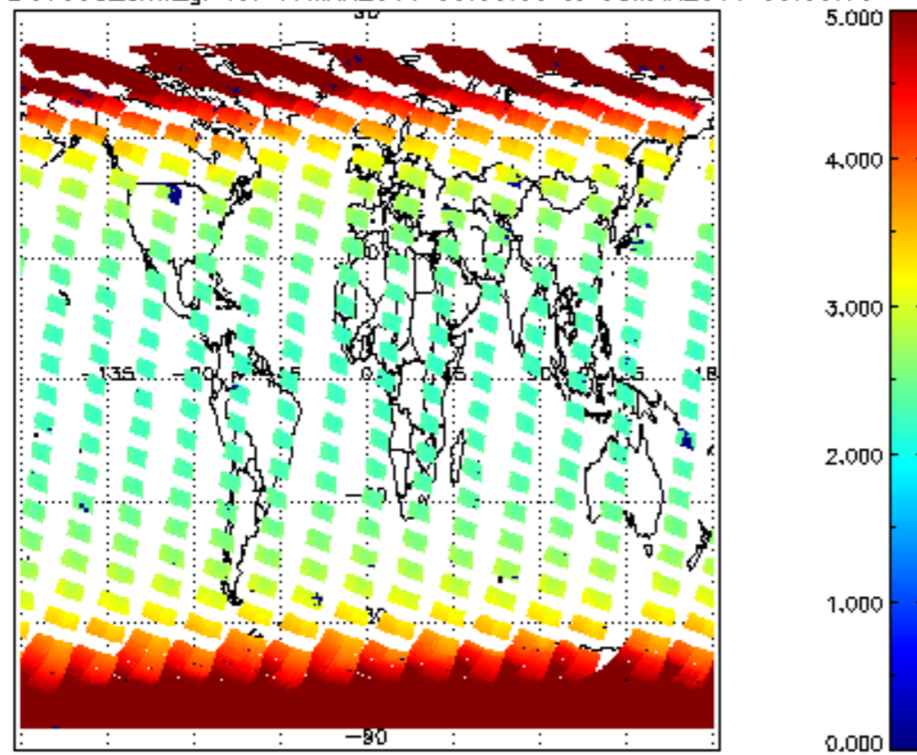
SCIOL2P_NADUV003_arnf_gr for 07MAR2011 00:00:00 to 08MAR2011 00:00:00
