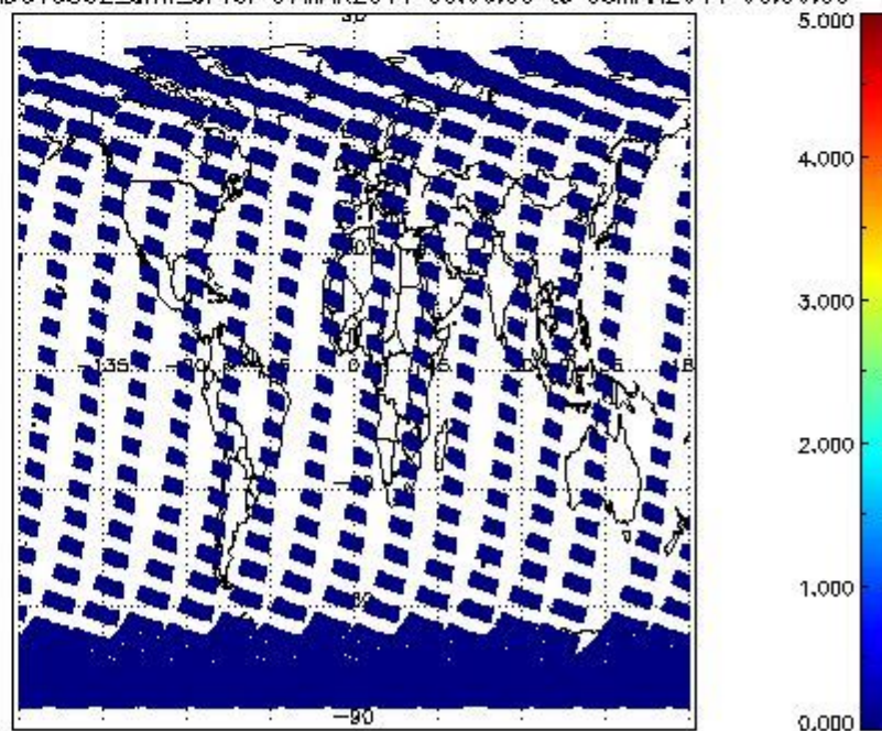
SCIOL2P_NADUV5SO2_amf_cl for 07MAR2011 00:00:00 to 08MAR2011 00:00:00
