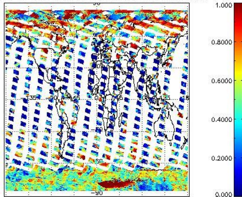
cL_frac for 07MAR2011 00:00:00 to 08MAR2011 00:00:00
