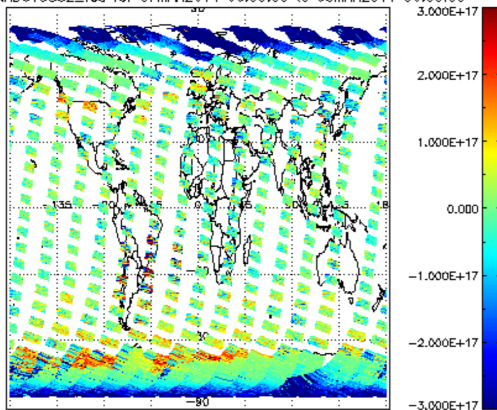
SCIOL2P_NADUV5S02_vcd for 07MAR2011 00:00:00 to 08MAR2011 00:00:00
