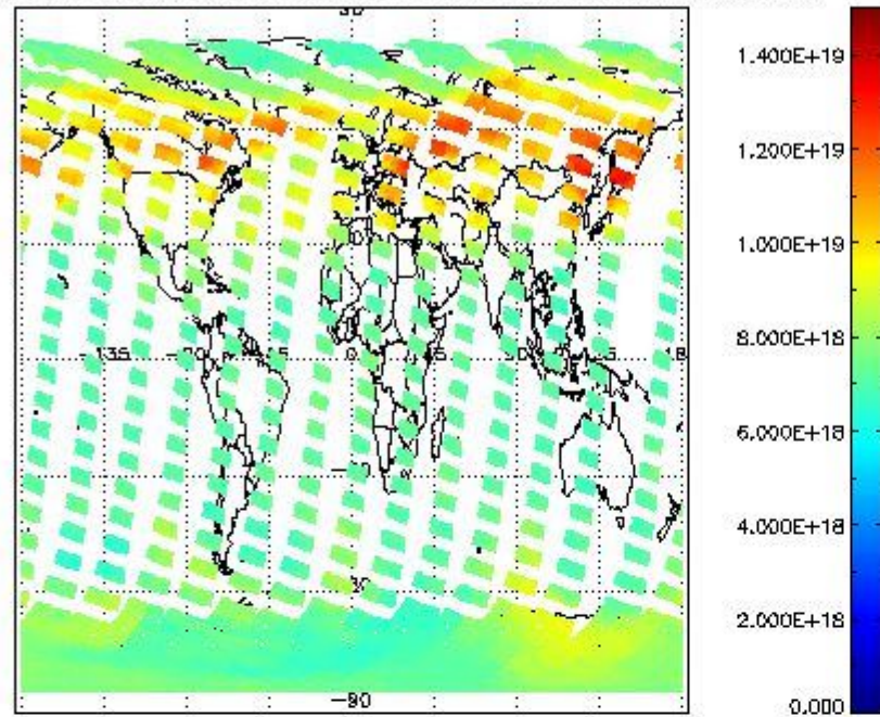
SCIOL2P_NADUV003_vcd for 07MAR2011 00:00:00 to 08MAR2011 00:00:00
