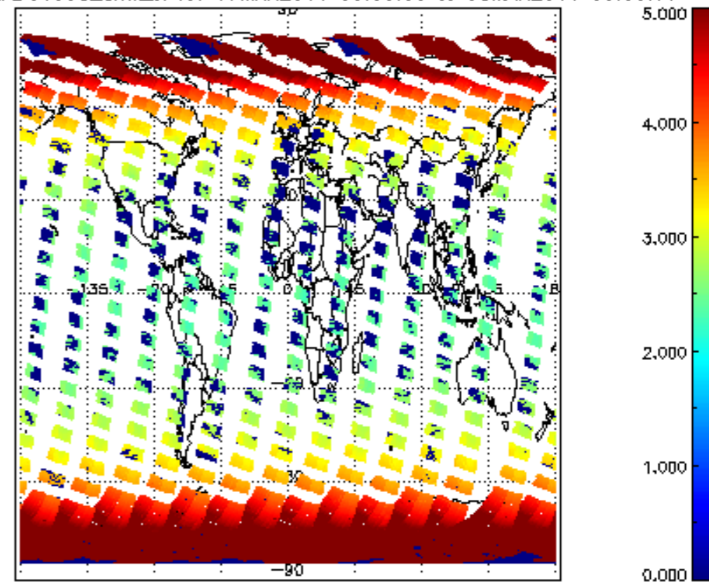
SCIOL2P_NADUV003_arnf_cl for 07MAR2011 00:00:00 to 08MAR2011 00:00:00
