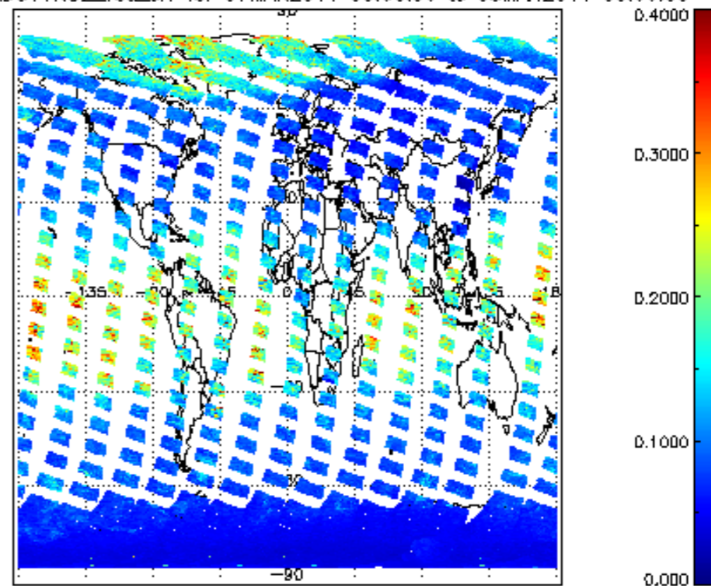
SCIOL2P_NADUV1NO2_vcd_err for 07MAR2011 00:00:00 to 08MAR2011 00:00:00
