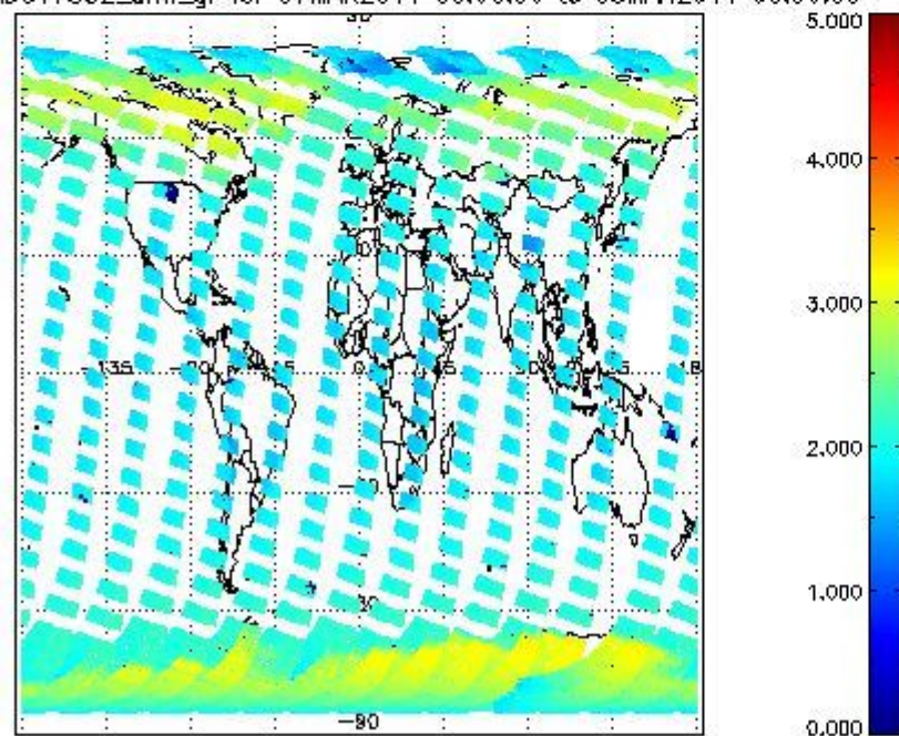
SCIOL2P_NADUV7S02_amf_gr for 07MAR2011 00:00:00 to 08MAR2011 00:00:00
