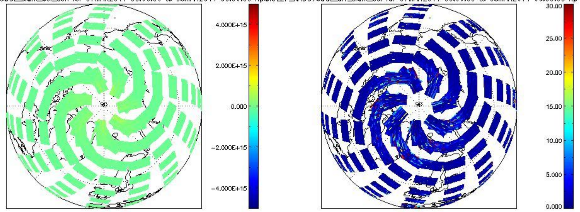
CIOL2P_NADUV6OCLslant_col_den for 07MAR2011 00:00:00 to 08MAR2011 00:00:00 npCIOL2P_NADUV6OCLarr_slant_col for 07MAR2011 00:00:00 to 08MAR2011 00:00:00 np
