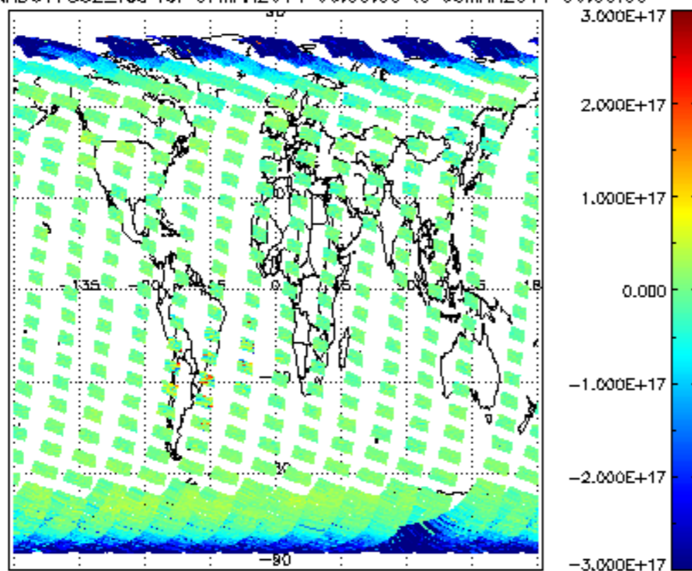
SCIOL2P_NADUV7S02_vcd for 07MAR2011 00:00:00 to 08MAR2011 00:00:00
