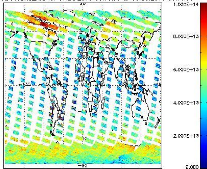
SCIOL2P_NADUV3BRO_vcd for 07MAR2011 00:00:00 to 08MAR2011 00:00:00
