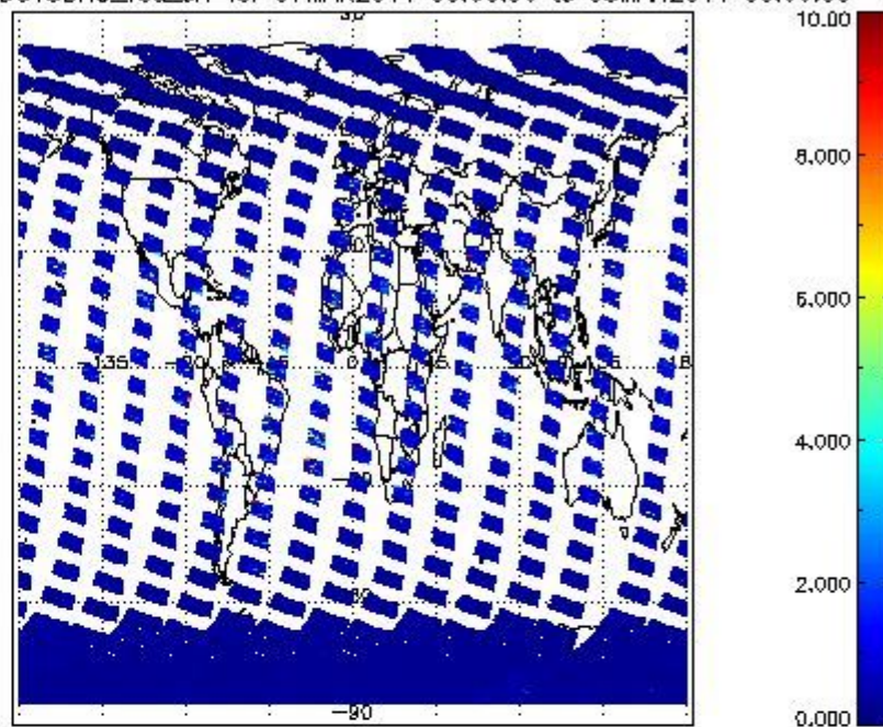
SCIOL2P_NADUV3BRO_vcd_err for 07MAR2011 00:00:00 to 08MAR2011 00:00:00
