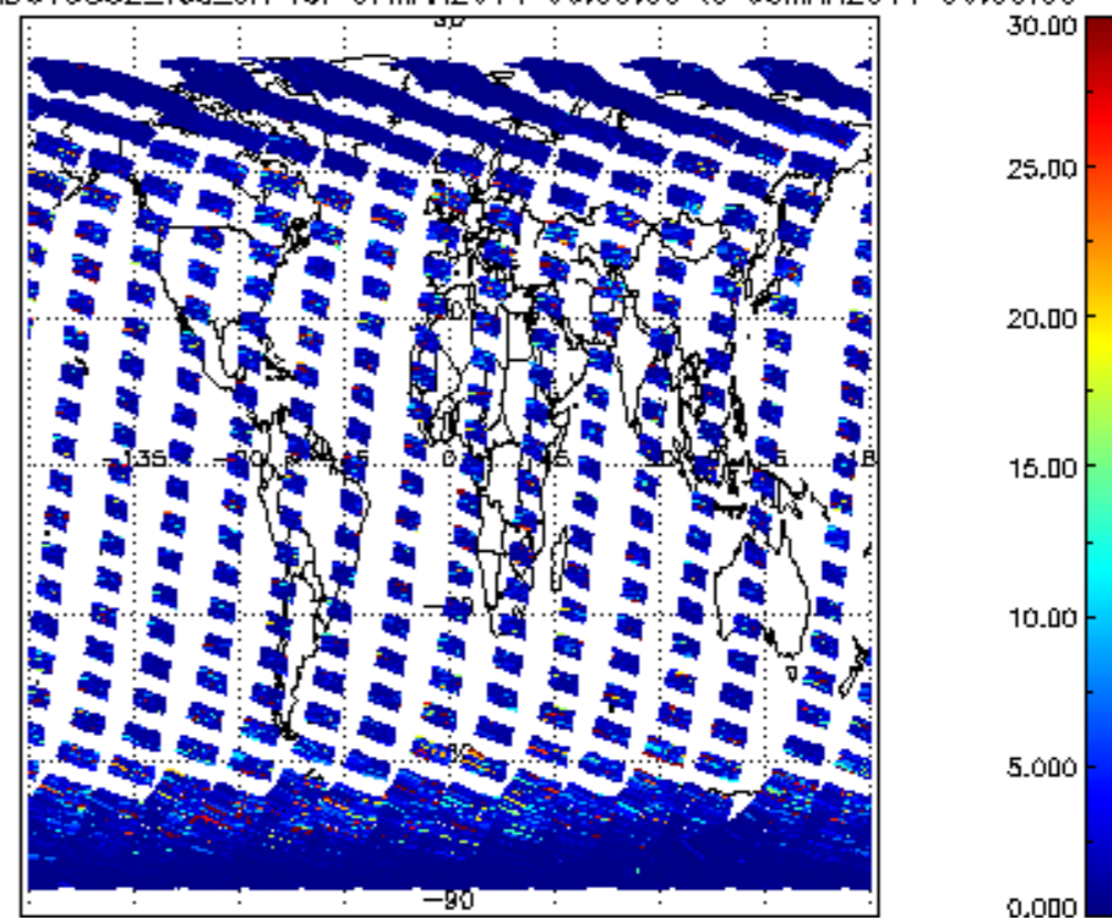
SCIOL2P_NADUV5S02_vcd_err for 07MAR2011 00:00:00 to 08MAR2011 00:00:00
