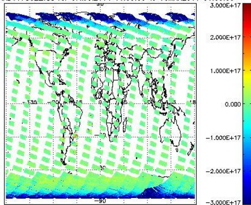
SCIOL2P_NADUV7S02_vcd for 07MAR2011 00:00:00 to 08MAR2011 00:00:00
