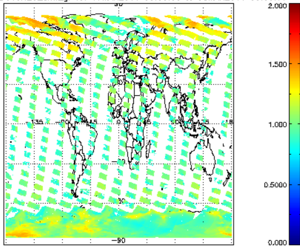
SCIOL2P_NADUV8H20_arnf_gr for 07MAR2011 00:00:00 to 08MAR2011 00:00:00
