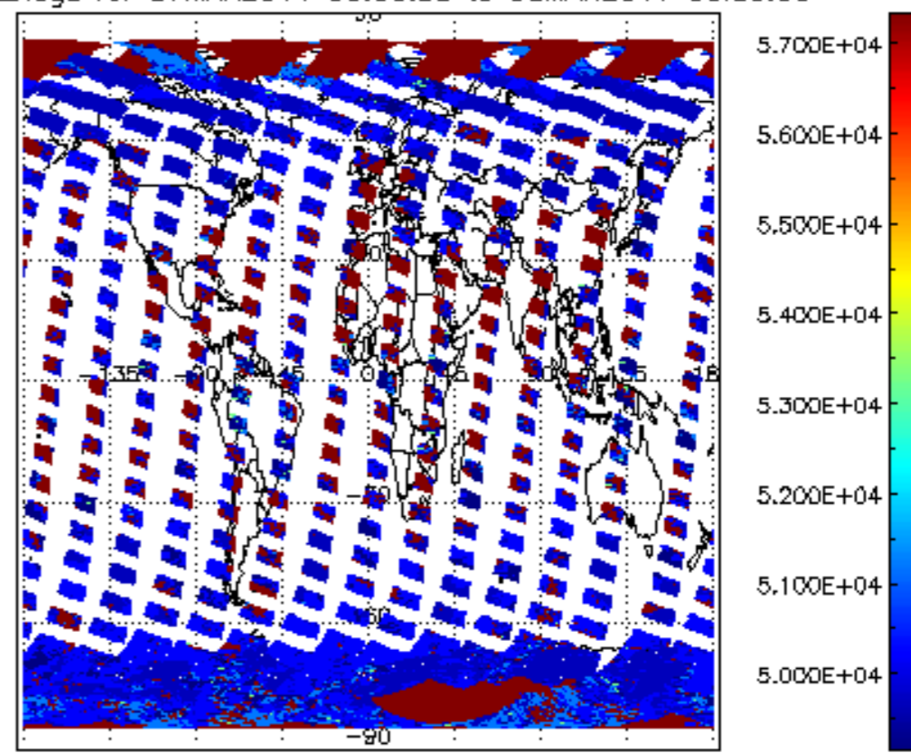
cloud_flags for 07MAR2011 00:00:00 to 08MAR2011 00:00:00
