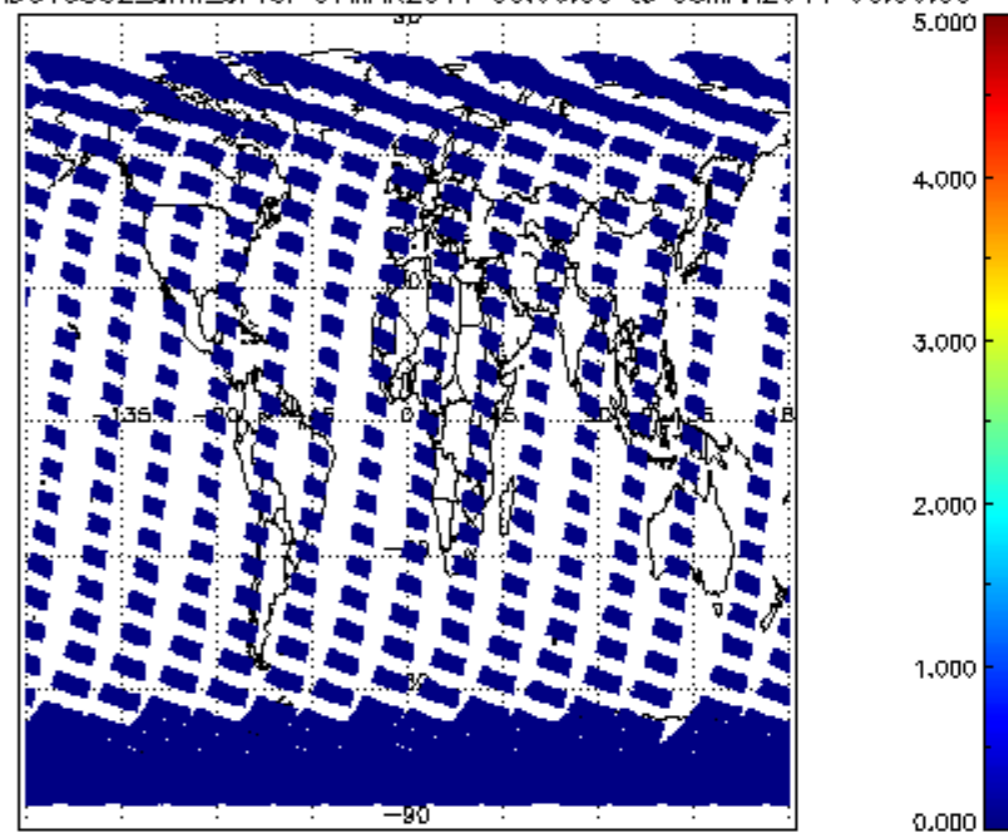
SCIOL2P_NADUV5S02_amf_cl for 07MAR2011 00:00:00 to 08MAR2011 00:00:00
