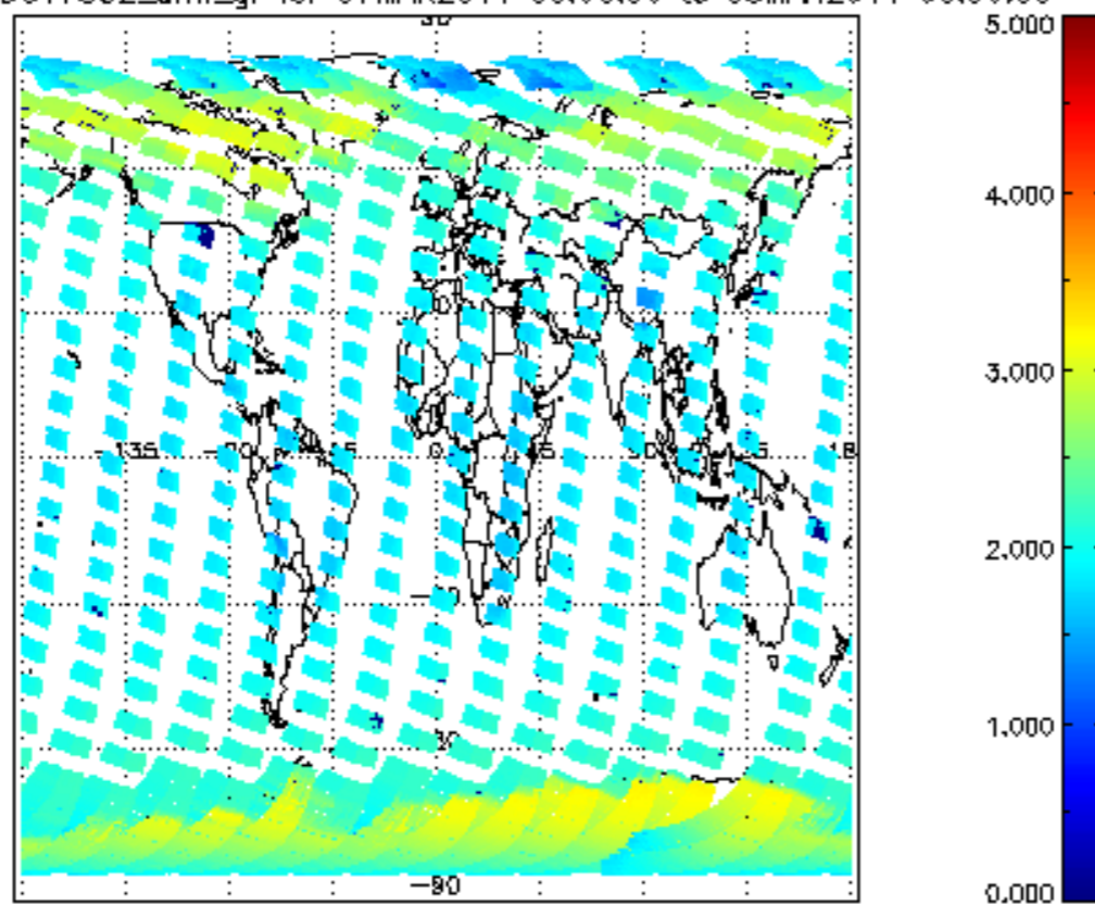
SCIOL2P_NADUV7S02_amf_gr for 07MAR2011 00:00:00 to 08MAR2011 00:00:00
