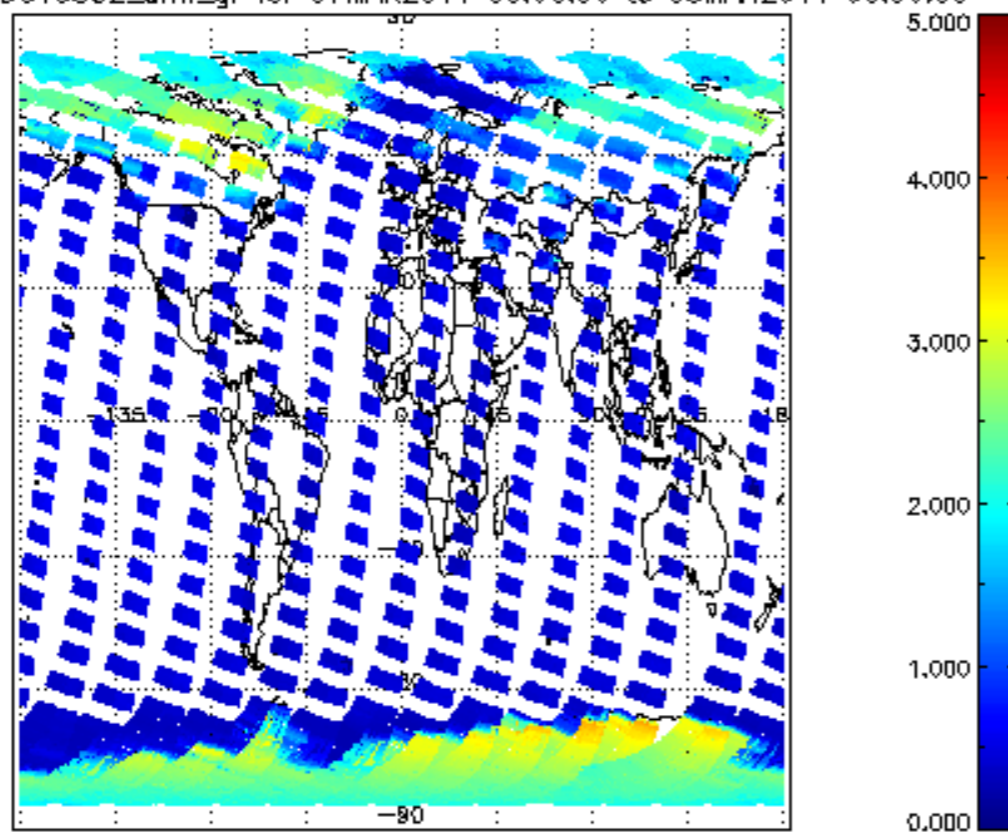
SCIOL2P_NADUV5S02_amf_gr for 07MAR2011 00:00:00 to 08MAR2011 00:00:00
