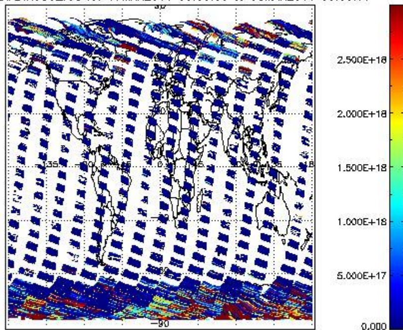
SCIDL2P_NADIR3CO_vcd for 07MAR2011 00:00:00 to 08MAR2011 00:00:00
