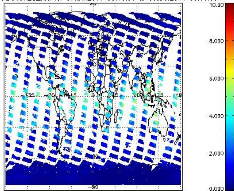
SCIOL2P_NADUV8H2O_vcd for 07MAR2011 00:00:00 to 08MAR2011 00:00:00
