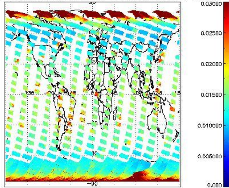
SCIOL2P_NADUV003_vcd_err for 07MAR2011 00:00:00 to 08MAR2011 00:00:00
