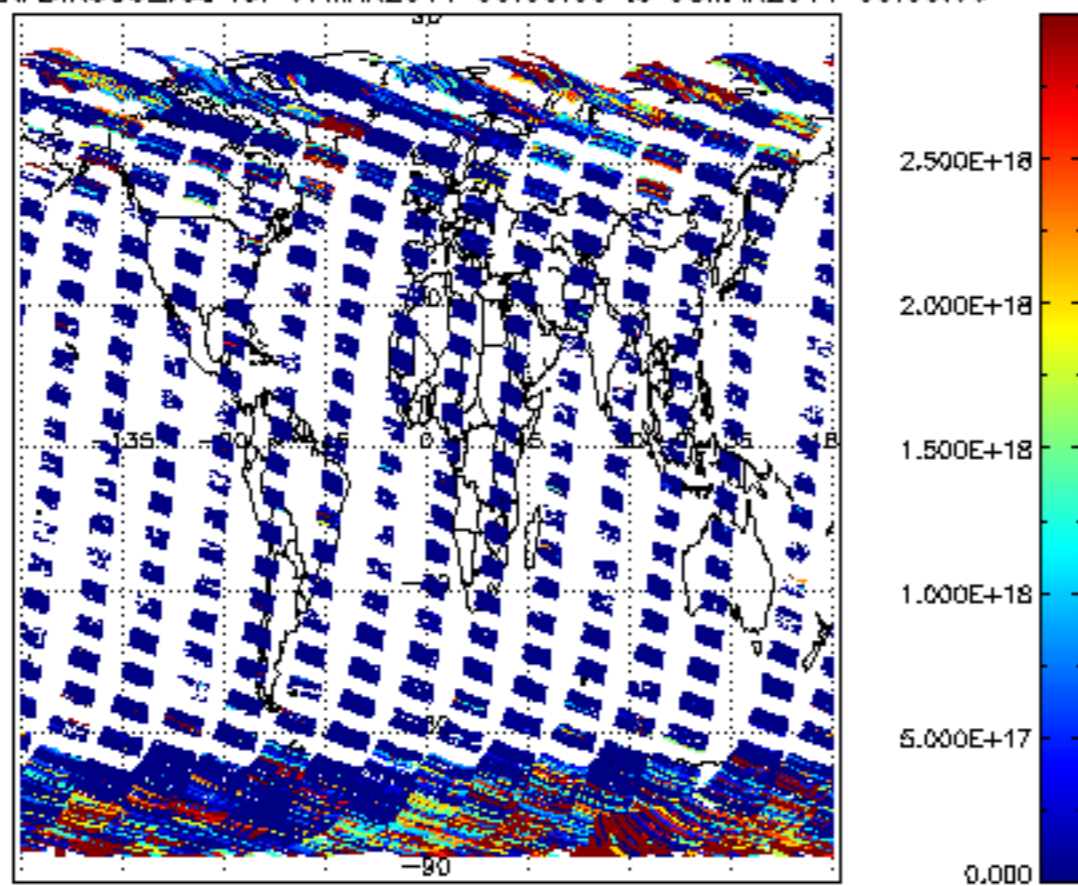
SCIOL2P_NADIR3CO_vcd for 07MAR2011 00:00:00 to 08MAR2011 00:00:00
