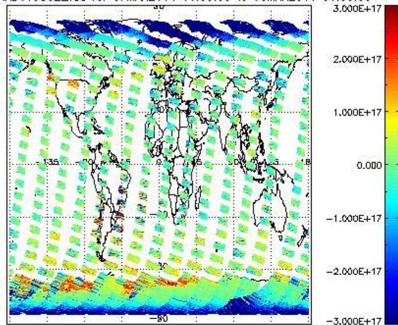
SCIOL2P_NADUV5SO2_vcd for 07MAR2011 00:00:00 to 08MAR2011 00:00:00
