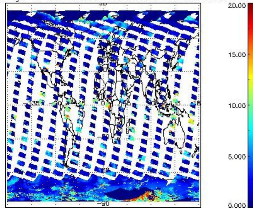
cL_top_height for 07MAR2011 00:00:00 to 08MAR2011 00:00:00
