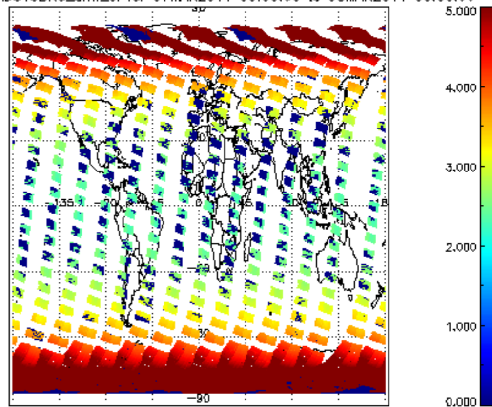
SCIOL2P_NADUV3BRO_arnf_cl for 07MAR2011 00:00:00 to 08MAR2011 00:00:00
