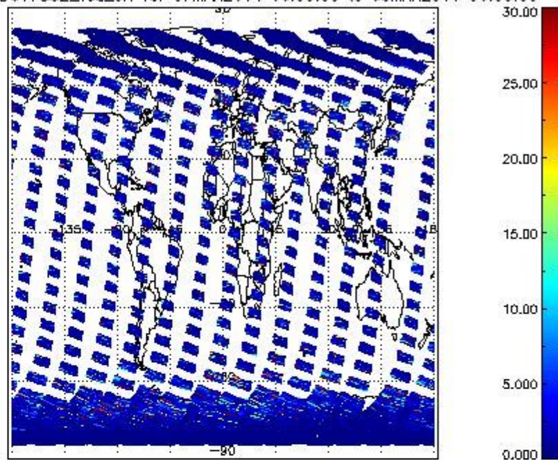
SCIOL2P_NADUV7S02_vcd_err for 07MAR2011 00:00:00 to 08MAR2011 00:00:00
