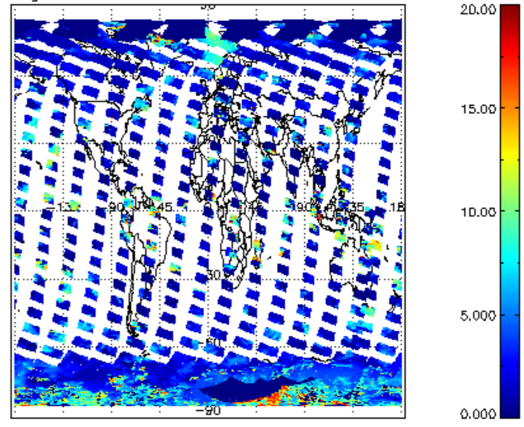
cL_top_height for 06MAR2011 00:00:00 to 07MAR2011 00:00:00
