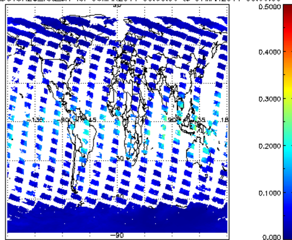
SCIOL2P_NADUV8H2O_vcd_Lerr for 06MAR2011 00:00:00 to 07MAR2011 00:00:00
