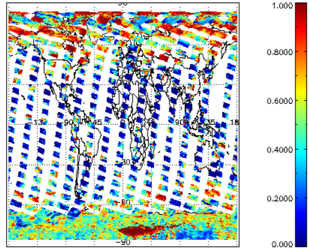
cL_frac for 06MAR2011 00:00:00 to 07MAR2011 00:00:00
