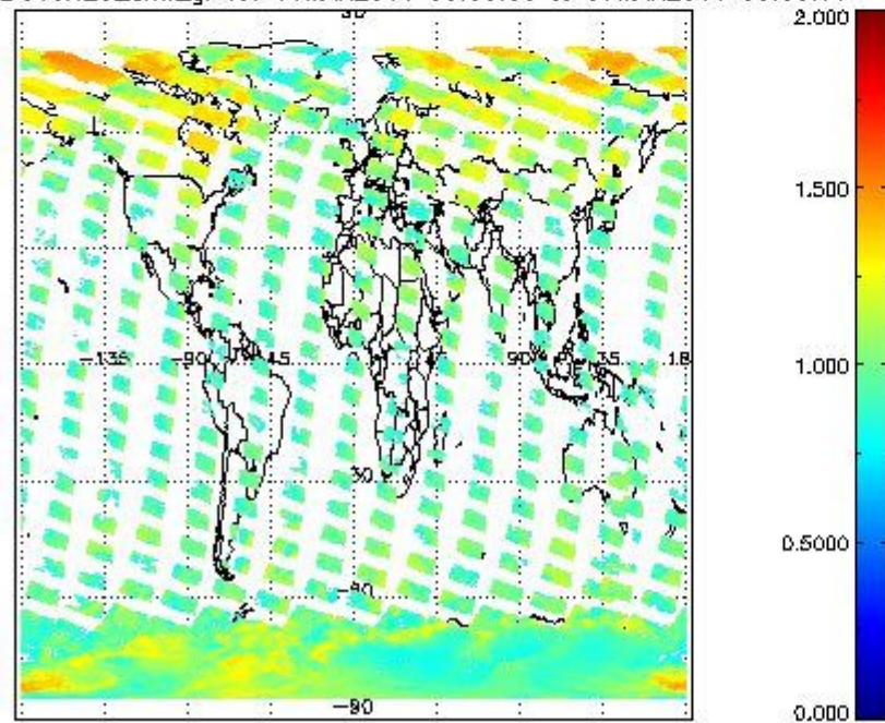
SCIOL2P_NADUV8H2O_amb_gr for 06MAR2011 00:00:00 to 07MAR2011 00:00:00
