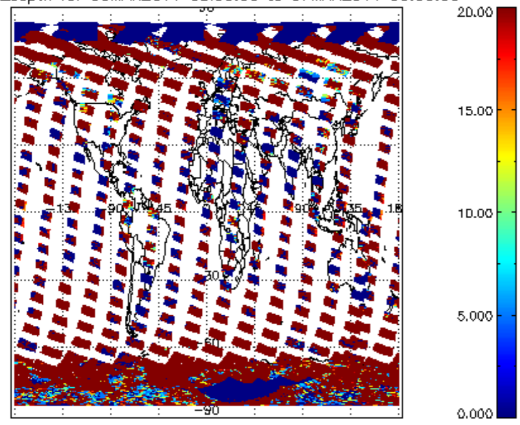
cL_opt_depth for 06MAR2011 00:00:00 to 07MAR2011 00:00:00
