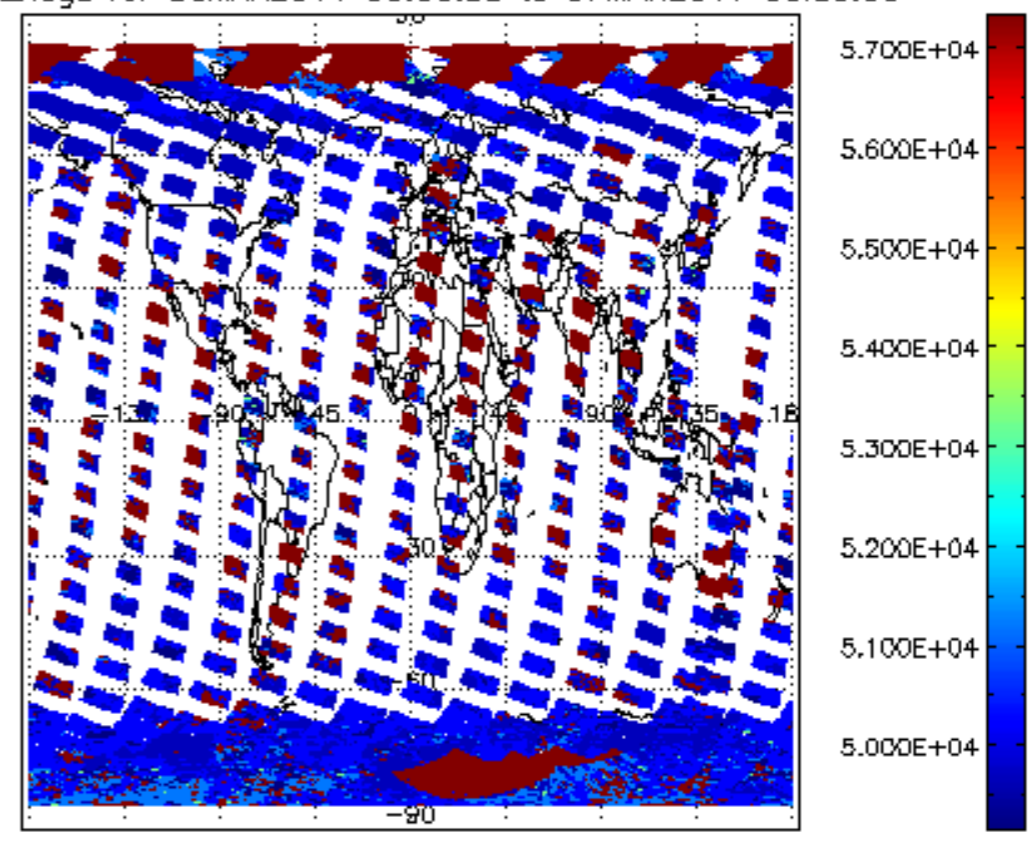
cloud_flags for 06MAR2011 00:00:00 to 07MAR2011 00:00:00
