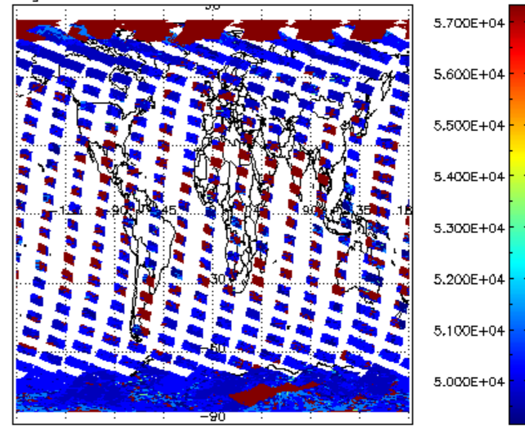
cloud_flags for 03MAR2011 00:00:00 to 04MAR2011 00:00:00
