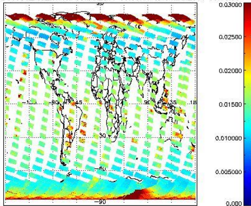
SCIOL2P_NADUV003_vcd_err for 03MAR2011 00:00:00 to 04MAR2011 00:00:00
