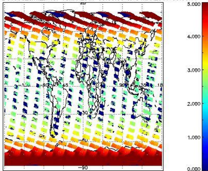
SCIOL2P_NADUV003_amf_cl for 03MAR2011 00:00:00 to 04MAR2011 00:00:00
