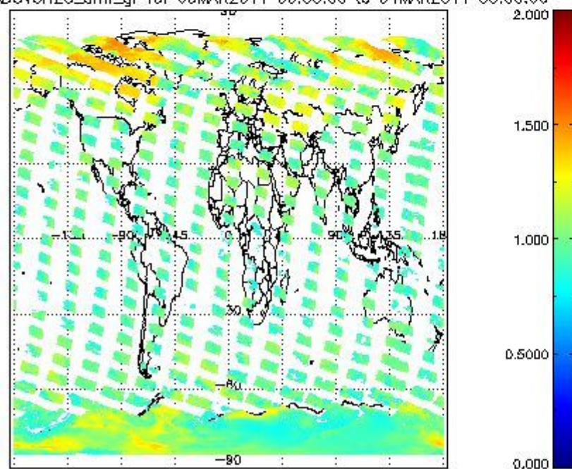
SCIOL2P_NADUV8H2O_arnf_gr for 03MAR2011 00:00:00 to 04MAR2011 00:00:00
