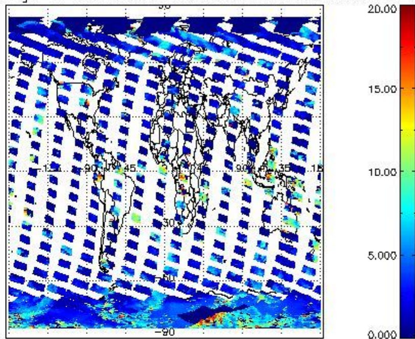
cL_top_height for 03MAR2011 00:00:00 to 04MAR2011 00:00:00
