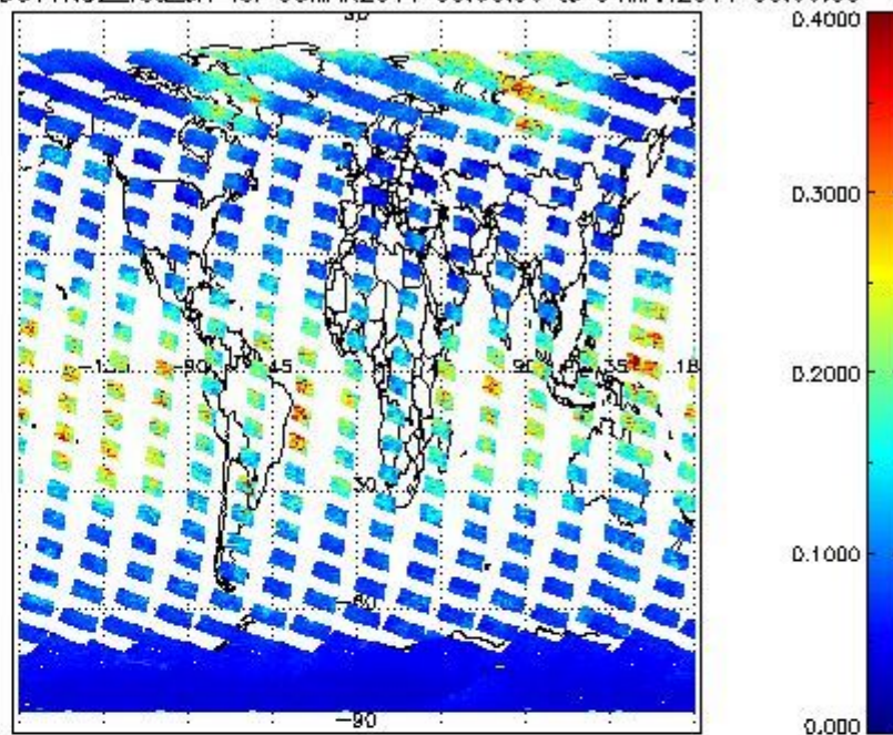
SCIOL2P_NADUV1NO2_vcd_err for 03MAR2011 00:00:00 to 04MAR2011 00:00:00
