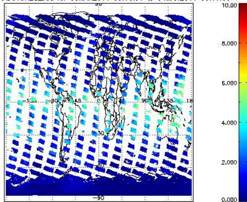
SCIOL2P_NADUV8H2O_vcd for 03MAR2011 00:00:00 to 04MAR2011 00:00:00
