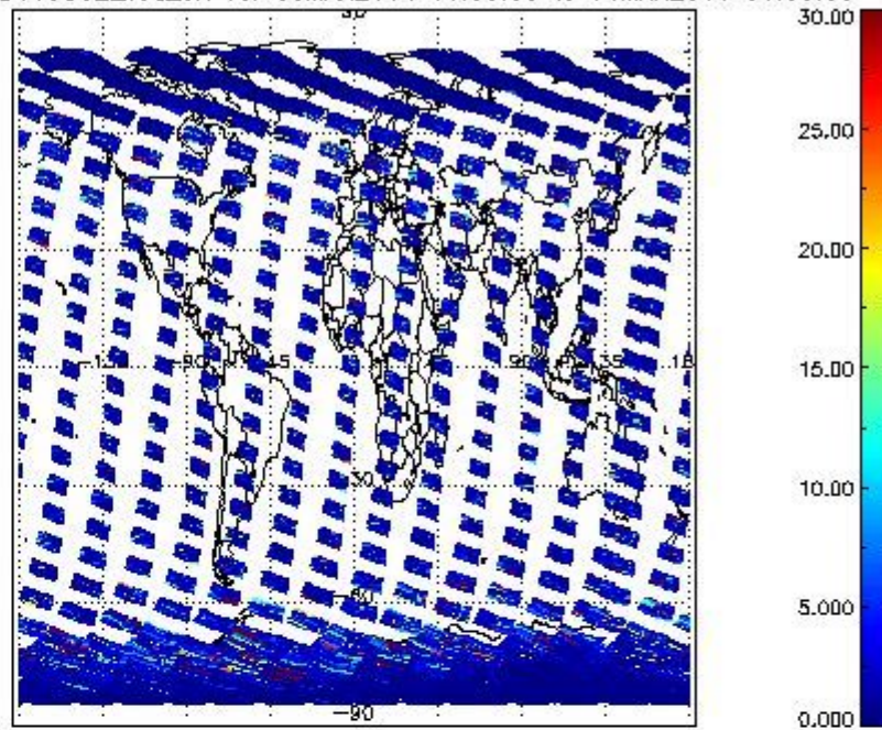
SCIOL2P_NADUV5SO2_vcd_err for 03MAR2011 00:00:00 to 04MAR2011 00:00:00
