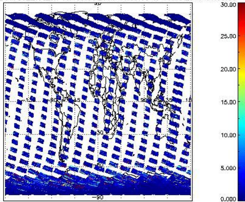
SCIOL2P_NADUV7S02_vcd_err for 03MAR2011 00:00:00 to 04MAR2011 00:00:00
