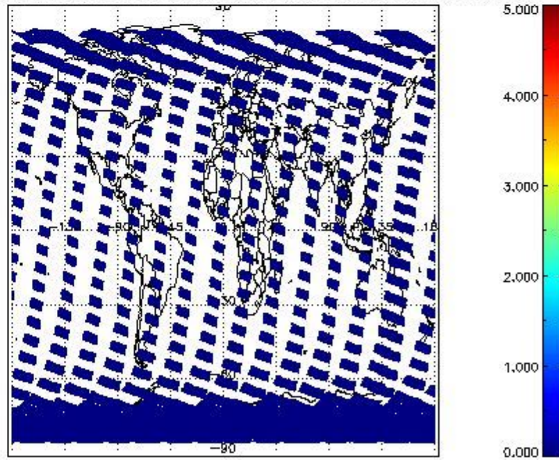
SCIOL2P_NADUV7S02_amf_cl for 03MAR2011 00:00:00 to 04MAR2011 00:00:00
