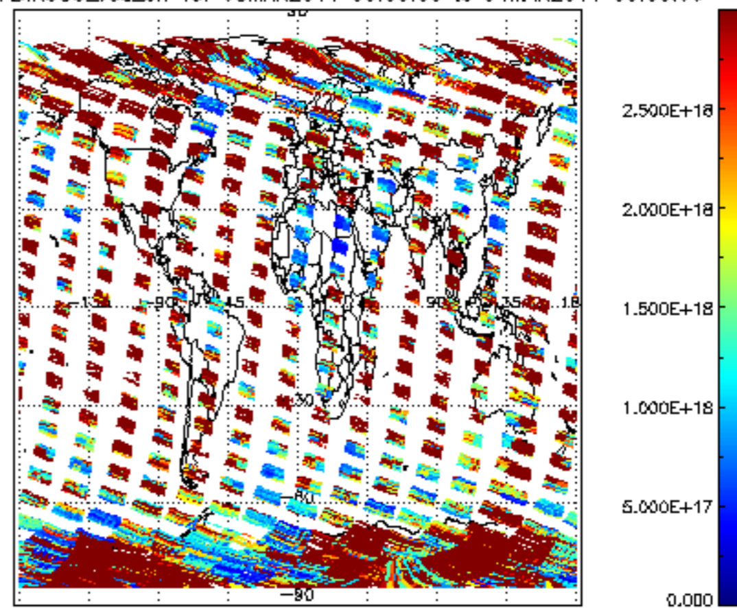
SCIOL2P_NADIR3CO_vcd_err for 03MAR2011 00:00:00 to 04MAR2011 00:00:00
