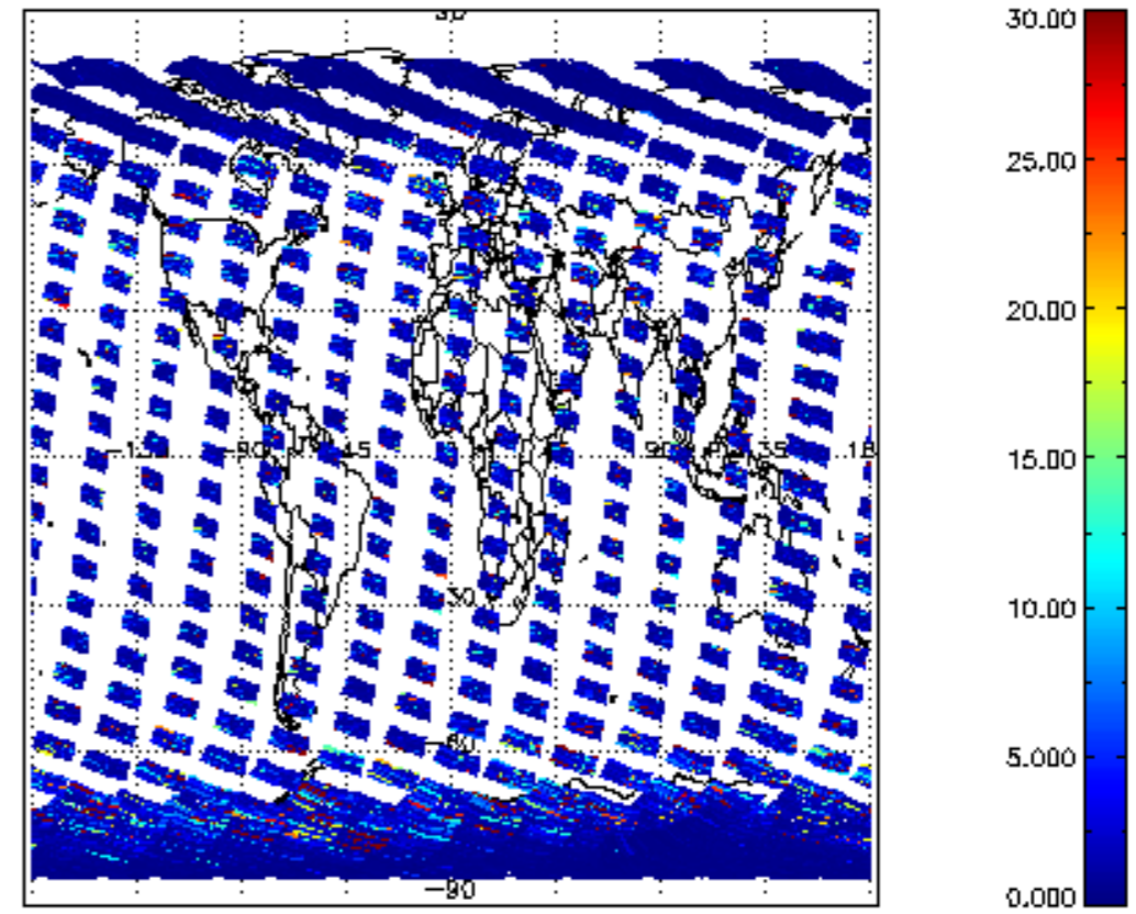
SCIOL2P_NADUV7S02_vcd_err for 03MAR2011 00:00:00 to 04MAR2011 00:00:00
