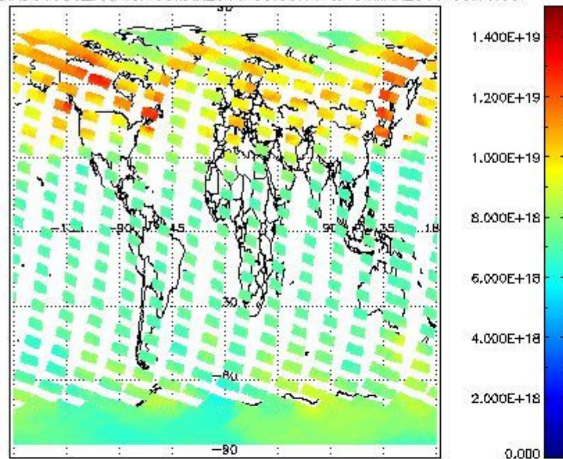
SCIOL2P_NADUV003_vcd for 03MAR2011 00:00:00 to 04MAR2011 00:00:00
