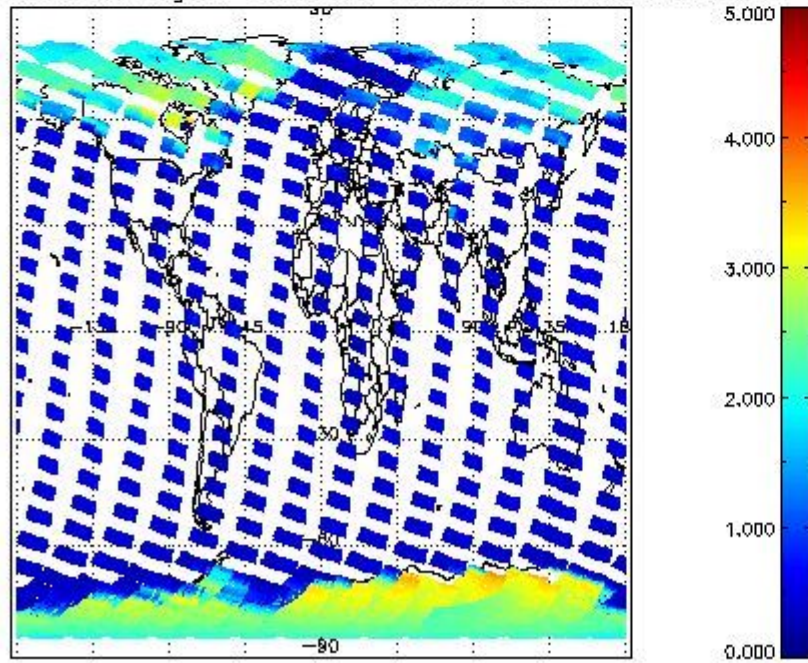
SCIOL2P_NADUV5SO2_amf_gr for 03MAR2011 00:00:00 to 04MAR2011 00:00:00
