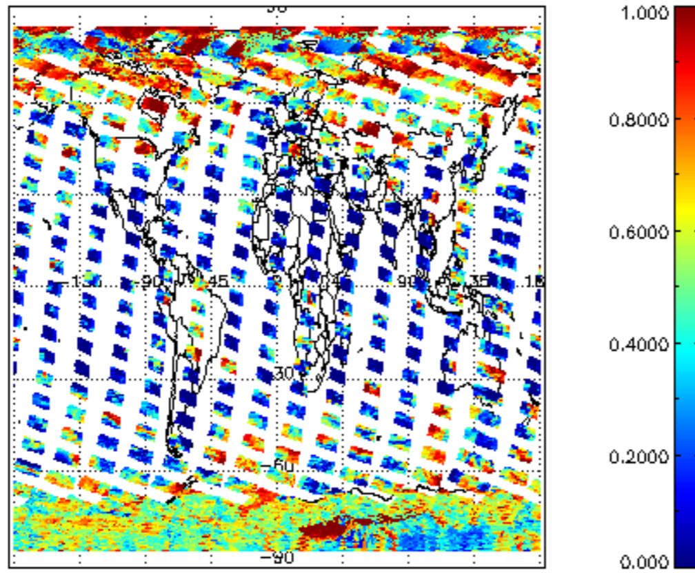
cL_frac for 03MAR2011 00:00:00 to 04MAR2011 00:00:00
