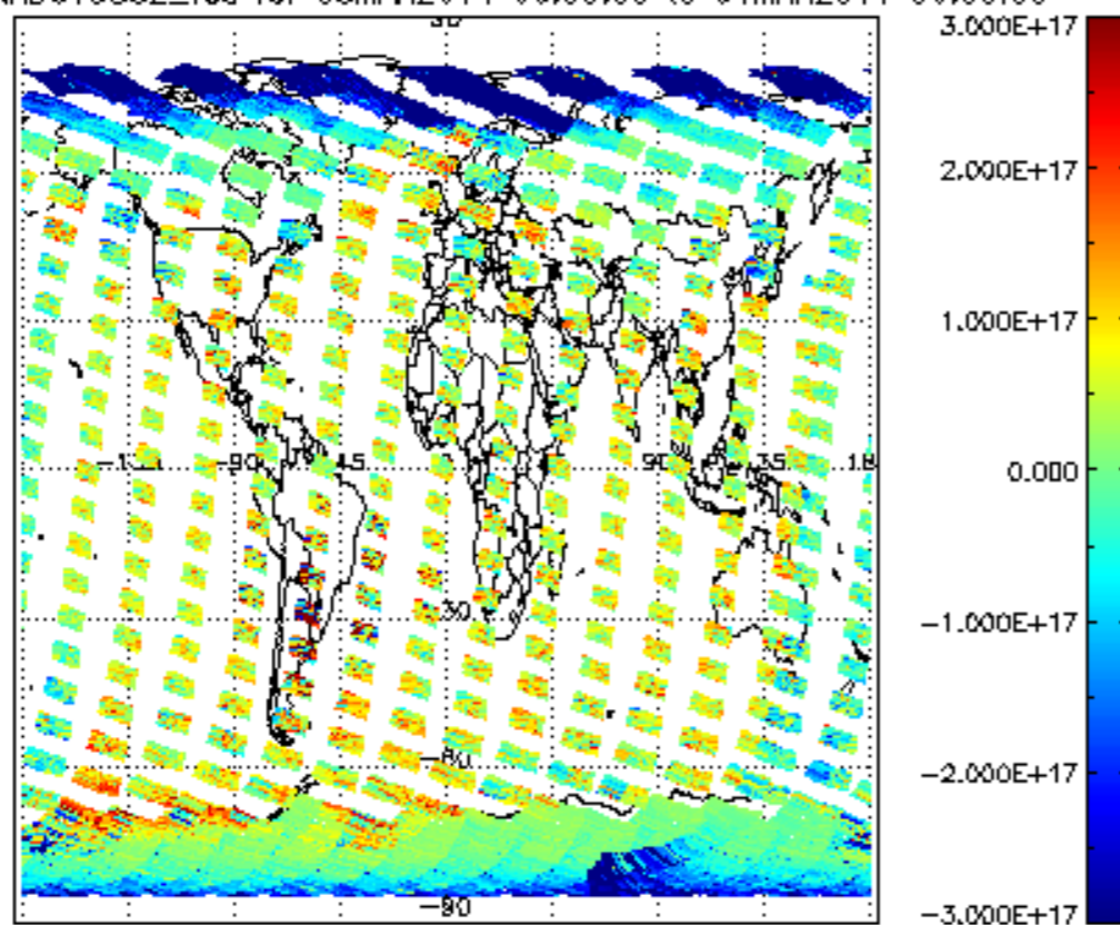
SCIOL2P_NADUV5S02_vcd for 03MAR2011 00:00:00 to 04MAR2011 00:00:00
