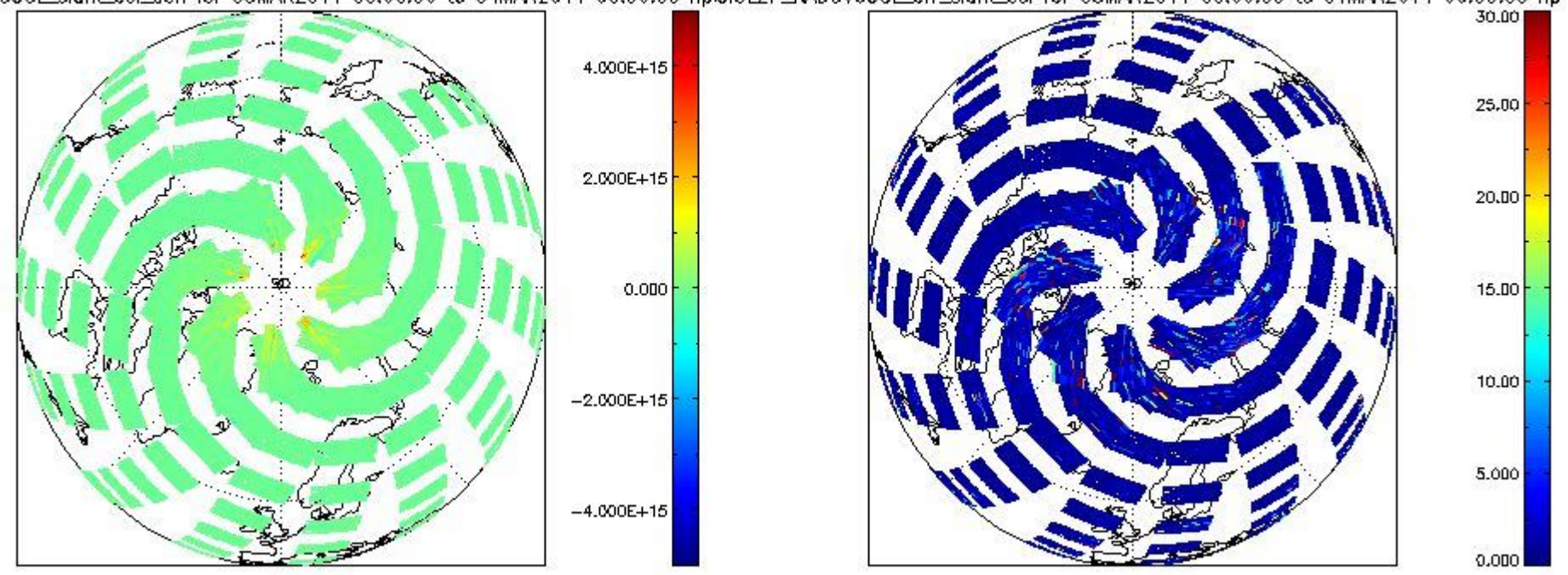
CIOL2P_NADUV6OCL_slant_col_den for 03MAR2011 00:00:00 to 04MAR2011 00:00:00 np CIOL2P_NADUV6OCL_err_slant_col for 03MAR2011 00:00:00 to 04MAR2011 00:00:00 np
