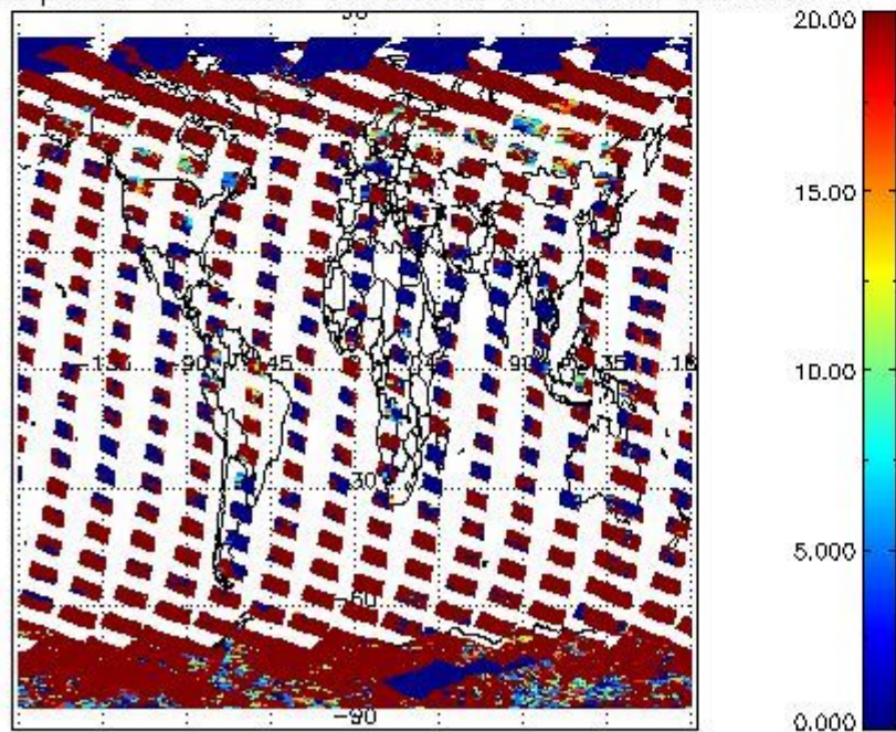
cL_opt_depth for 03MAR2011 00:00:00 to 04MAR2011 00:00:00
