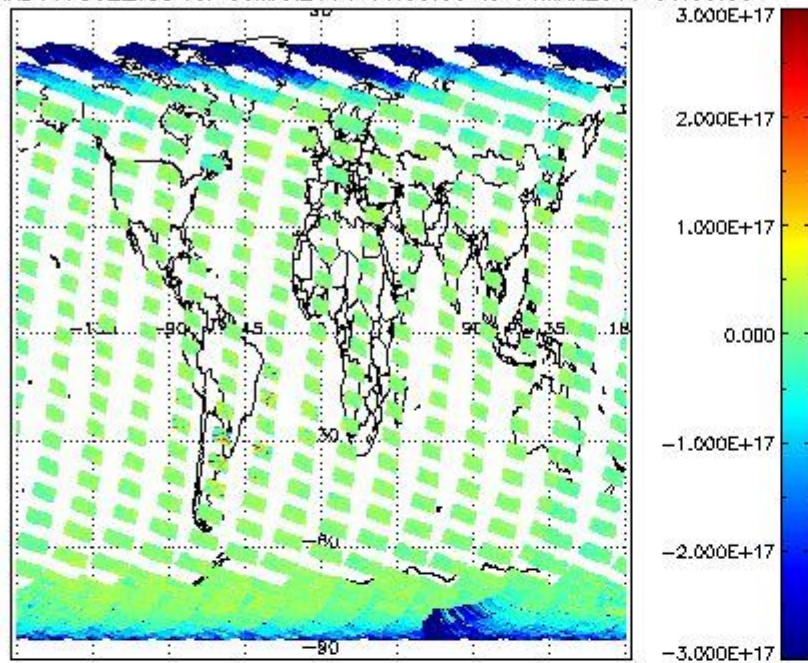
SCIOL2P_NADUV7S02_vcd for 03MAR2011 00:00:00 to 04MAR2011 00:00:00
