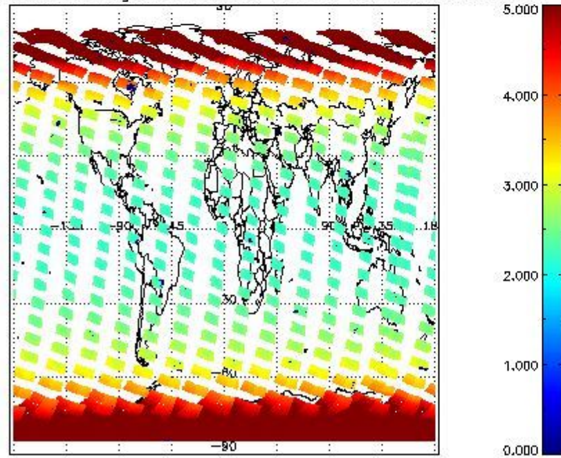
SCIOL2P_NADUV3BRO_amf_gr for 03MAR2011 00:00:00 to 04MAR2011 00:00:00
