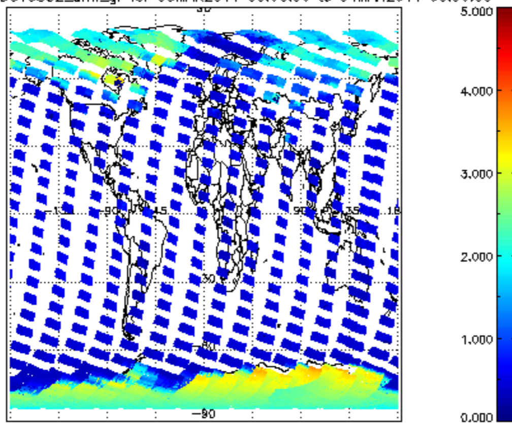
SCIOL2P_NADUV5S02_amf_gr for 03MAR2011 00:00:00 to 04MAR2011 00:00:00
