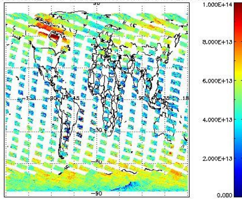
SCIOL2P_NADUV3BRO_vcd for 03MAR2011 00:00:00 to 04MAR2011 00:00:00
