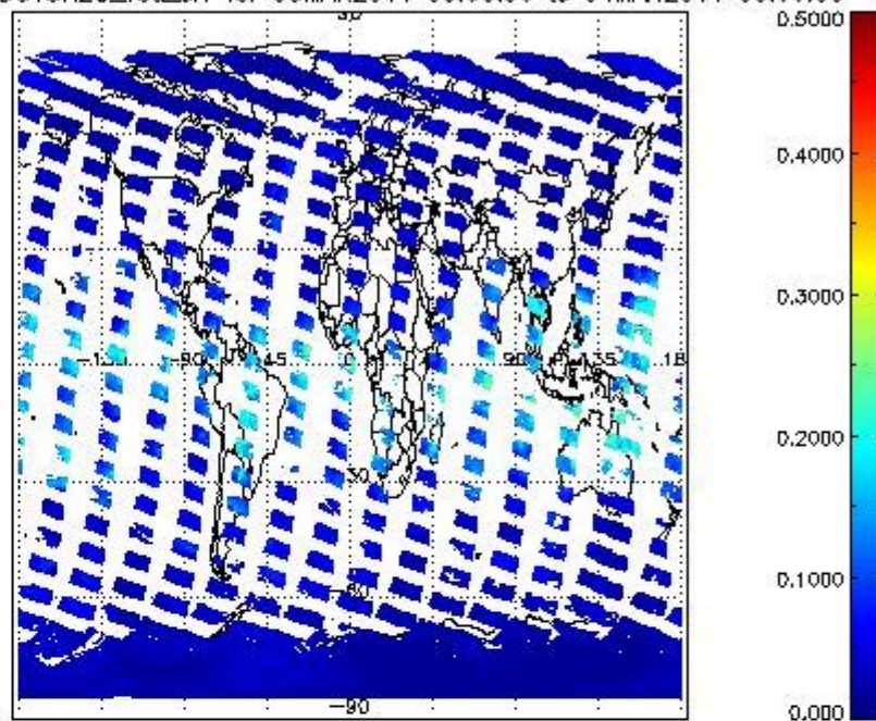
SCIOL2P_NADUV8H2O_vcd_err for 03MAR2011 00:00:00 to 04MAR2011 00:00:00
