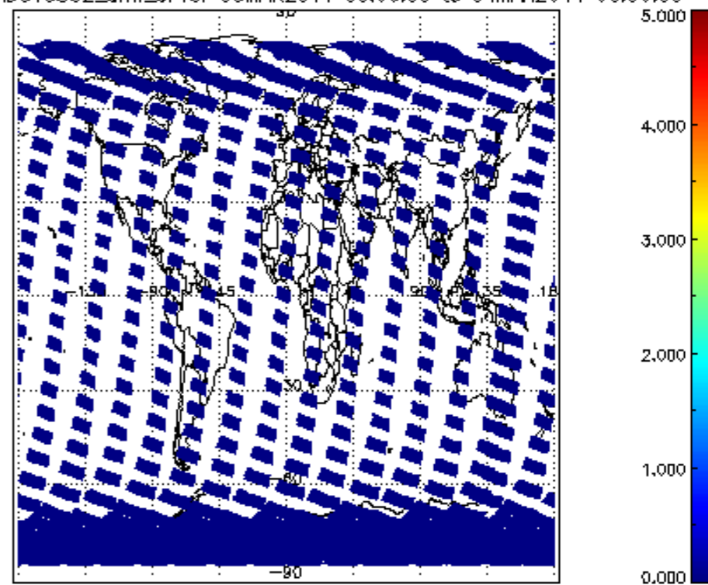
SCIOL2P_NADUV5S02_amf_cl for 03MAR2011 00:00:00 to 04MAR2011 00:00:00
