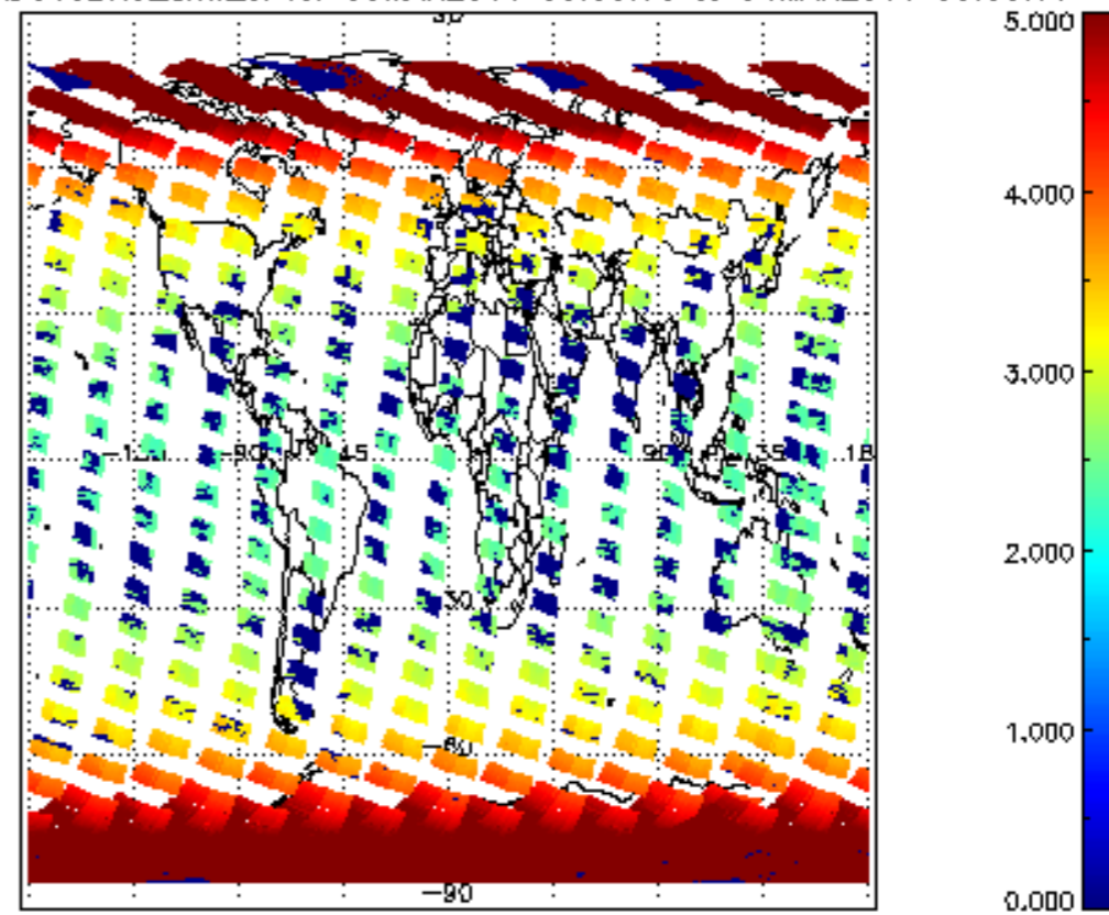
SCIOL2P_NADUV3BRO_amf_cl for 03MAR2011 00:00:00 to 04MAR2011 00:00:00
