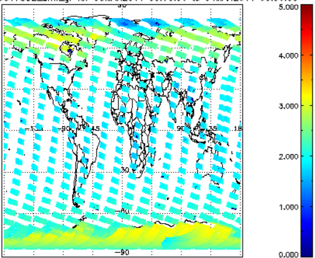
SCIOL2P_NADUV7S02_amf_gr for 03MAR2011 00:00:00 to 04MAR2011 00:00:00
