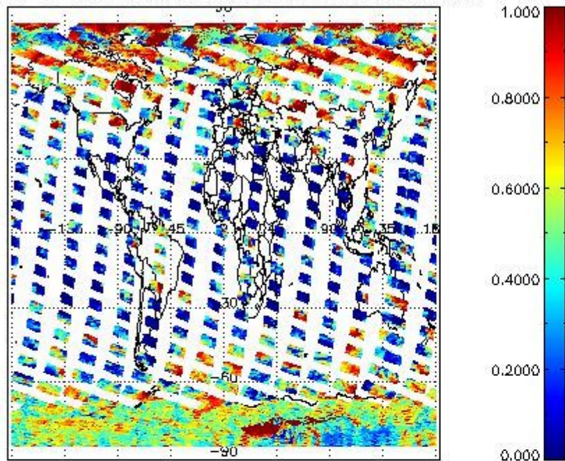
cL_frac for 03MAR2011 00:00:00 to 04MAR2011 00:00:00
