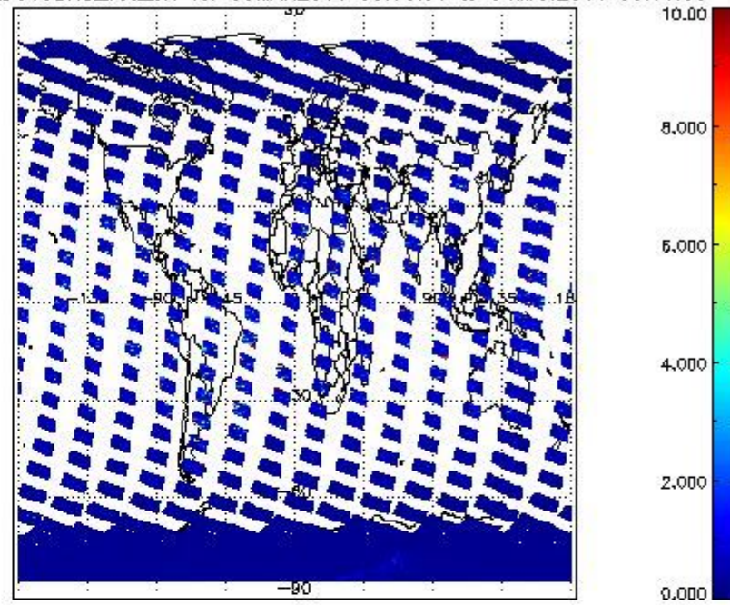
SCIOL2P_NADUV3BRO_vcd_err for 03MAR2011 00:00:00 to 04MAR2011 00:00:00
