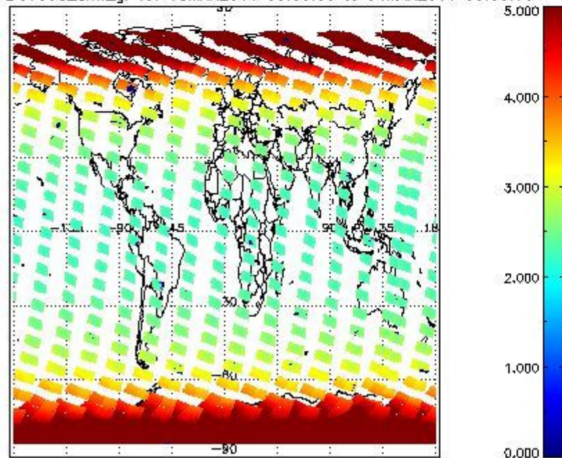
SCIOL2P_NADUV003_amf_gr for 03MAR2011 00:00:00 to 04MAR2011 00:00:00
