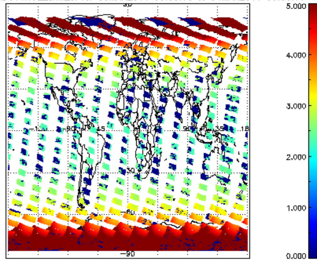
SCIOL2P_NADUV1NO2_amf_cl for 03MAR2011 00:00:00 to 04MAR2011 00:00:00
