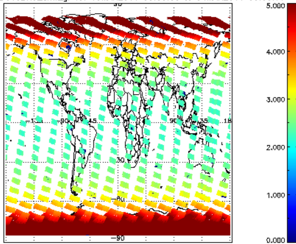
SCIOL2P_NADUV3BRO_amf_gr for 03MAR2011 00:00:00 to 04MAR2011 00:00:00
