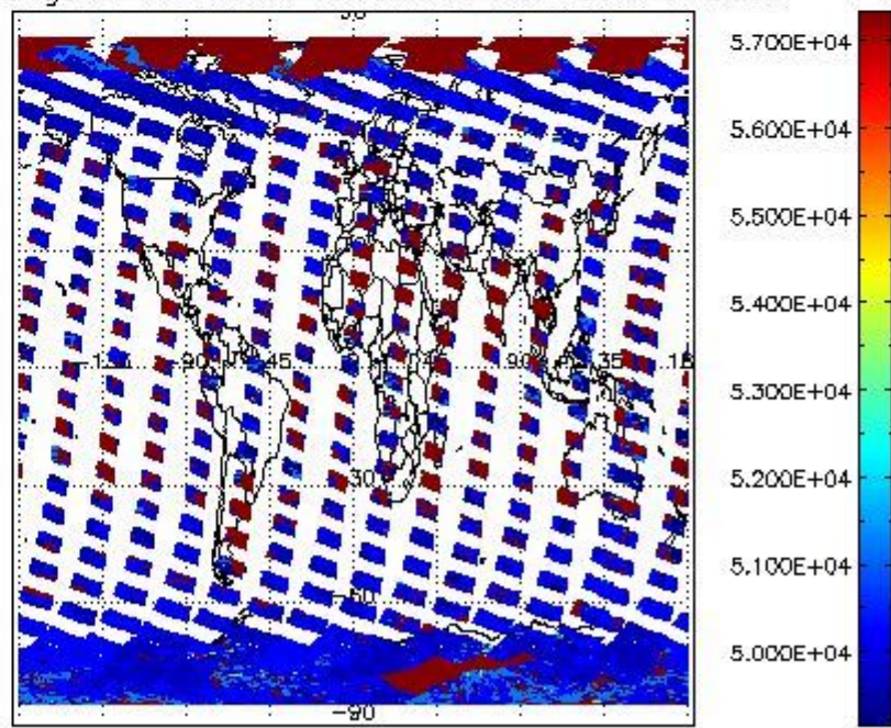
cloud_flags for 03MAR2011 00:00:00 to 04MAR2011 00:00:00
