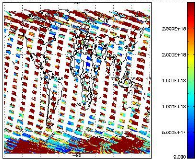
SCIDL2P_NADIR3CO_vcd_err for 03MAR2011 00:00:00 to 04MAR2011 00:00:00
