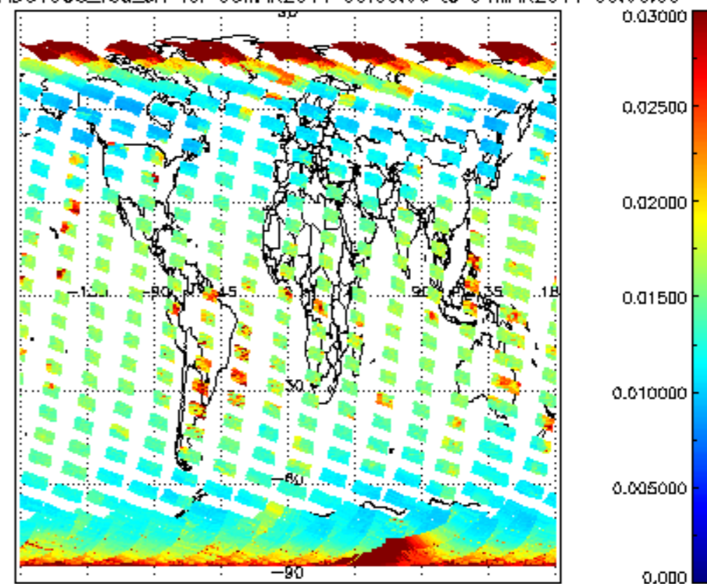
SCIOL2P_NADUV003_vcd_err for 03MAR2011 00:00:00 to 04MAR2011 00:00:00
