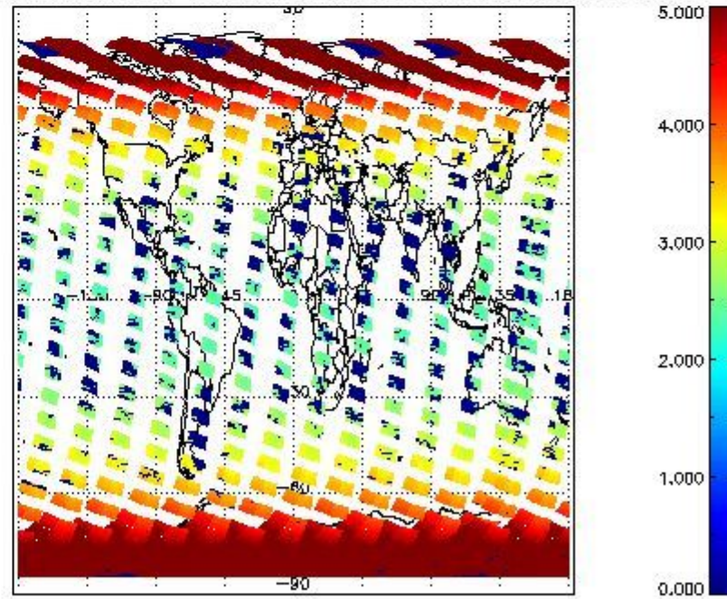
SCIOL2P_NADUV3BRO_amf_cl for 03MAR2011 00:00:00 to 04MAR2011 00:00:00
