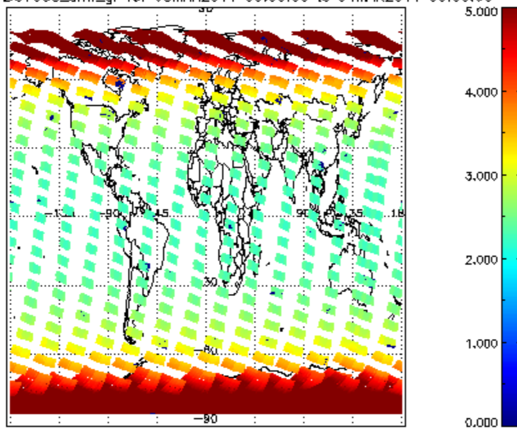
SCIOL2P_NADUV003_arnf_gr for 03MAR2011 00:00:00 to 04MAR2011 00:00:00
