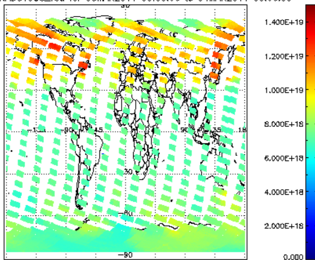
SCIOL2P_NADUV003_vcd for 03MAR2011 00:00:00 to 04MAR2011 00:00:00
