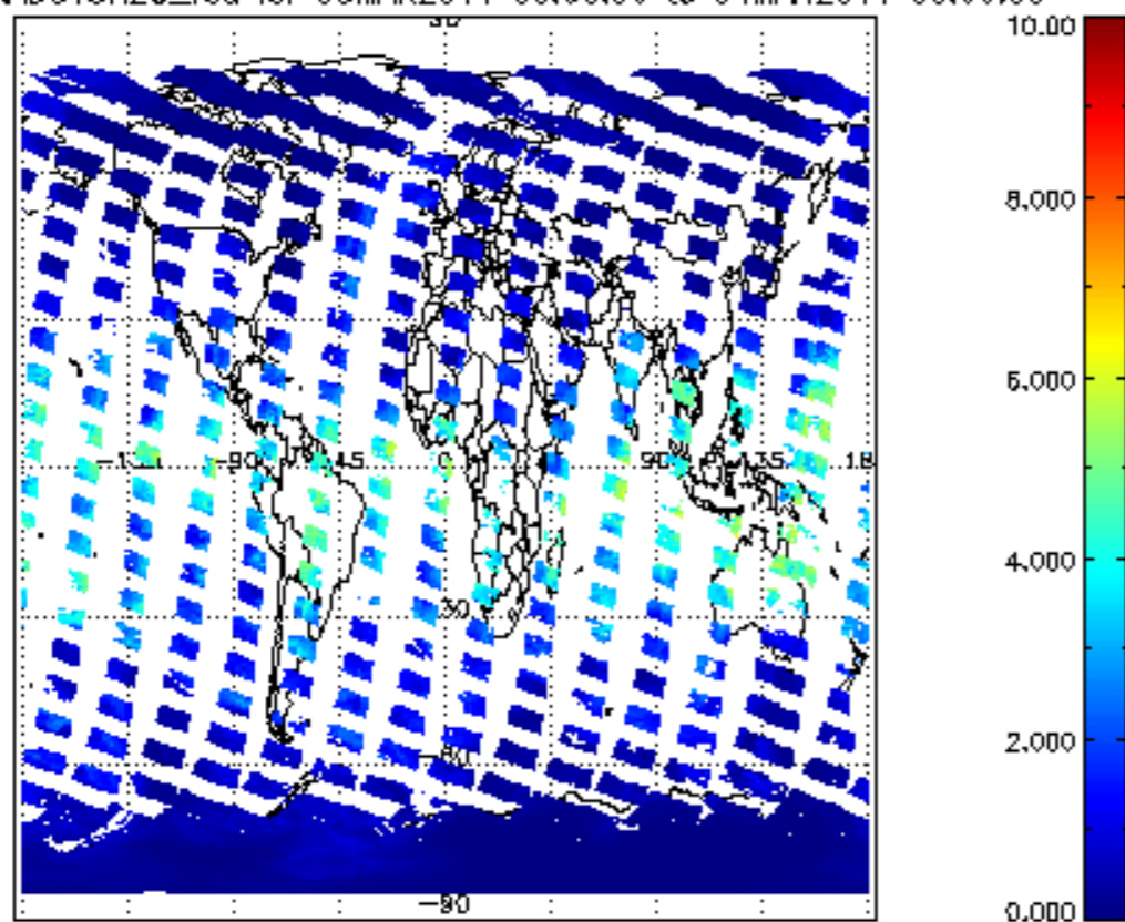
SCIOL2P_NADUV8H20_vcd for 03MAR2011 00:00:00 to 04MAR2011 00:00:00
