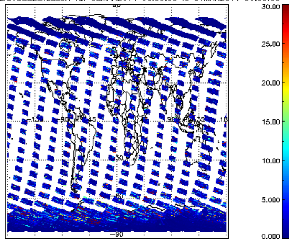
SCIOL2P_NADUV5S02_vcd_err for 03MAR2011 00:00:00 to 04MAR2011 00:00:00
