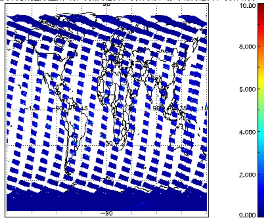
SCIOL2P_NADUV3BRO_vcd_err for 03MAR2011 00:00:00 to 04MAR2011 00:00:00
