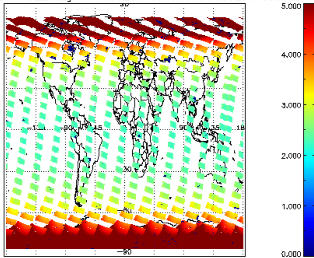
SCIOL2P_NADUV1NO2_amf_gr for 03MAR2011 00:00:00 to 04MAR2011 00:00:00
