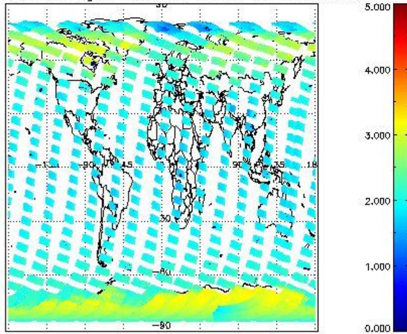
SCIOL2P_NADUV7S02_amf_gr for 03MAR2011 00:00:00 to 04MAR2011 00:00:00
