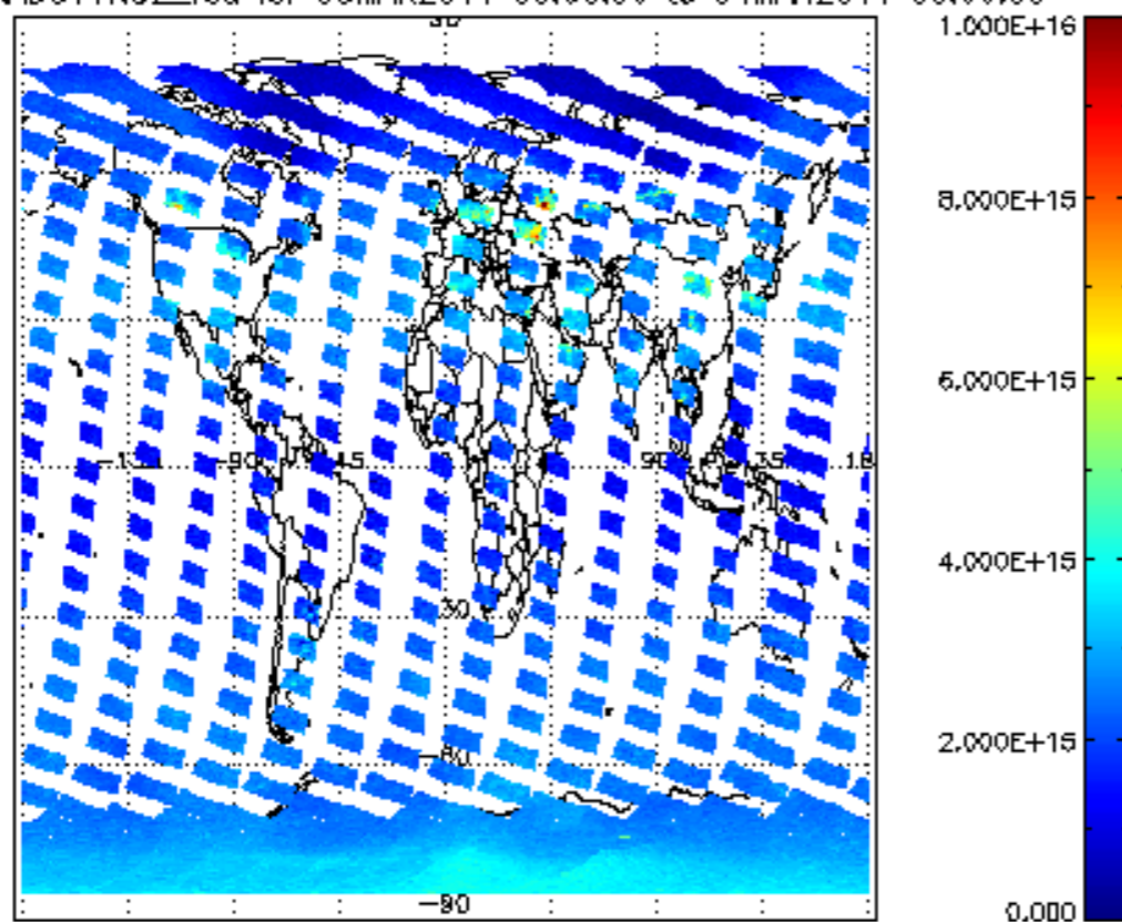
SCIOL2P_NADUV1NO2_vcd for 03MAR2011 00:00:00 to 04MAR2011 00:00:00
