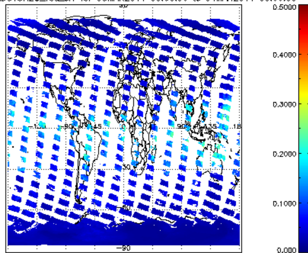
SCIOL2P_NADUV8H20_vcd_err for 03MAR2011 00:00:00 to 04MAR2011 00:00:00
