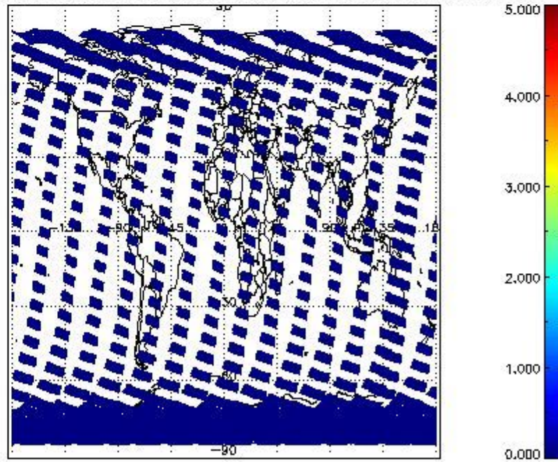
SCIOL2P_NADUV5SO2_amf_cl for 03MAR2011 00:00:00 to 04MAR2011 00:00:00
