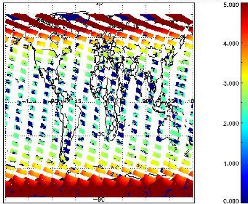
SCIOL2P_NADUV1NO2_amf_cl for 03MAR2011 00:00:00 to 04MAR2011 00:00:00
