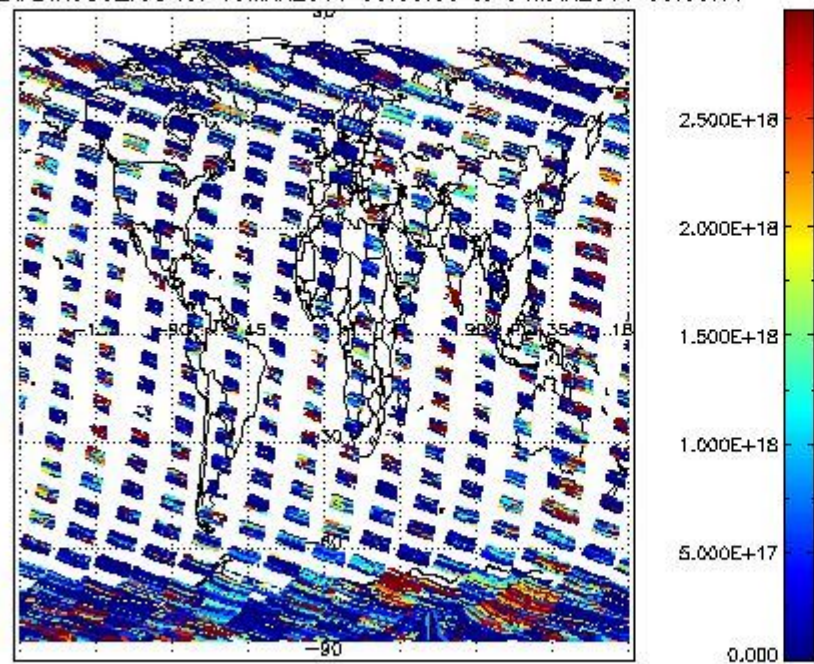
SCIDL2P_NADIR3CO_vcd for 03MAR2011 00:00:00 to 04MAR2011 00:00:00
