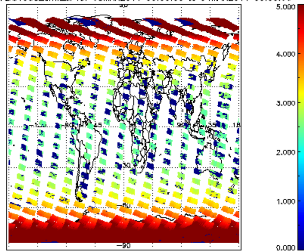
SCIOL2P_NADUV003_arnf_cl for 03MAR2011 00:00:00 to 04MAR2011 00:00:00
