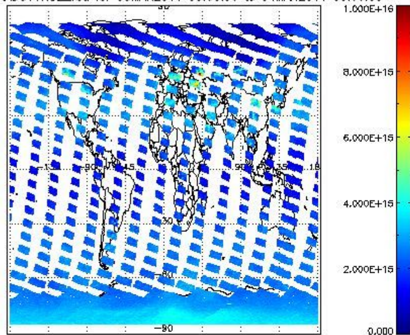
SCIOL2P_NADUV1NO2_vcd for 03MAR2011 00:00:00 to 04MAR2011 00:00:00
