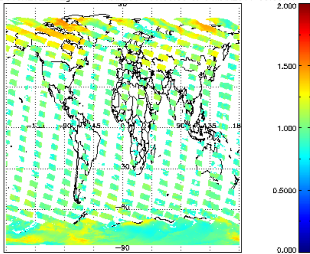
SCIOL2P_NADUV8H20_arnf_gr for 03MAR2011 00:00:00 to 04MAR2011 00:00:00
