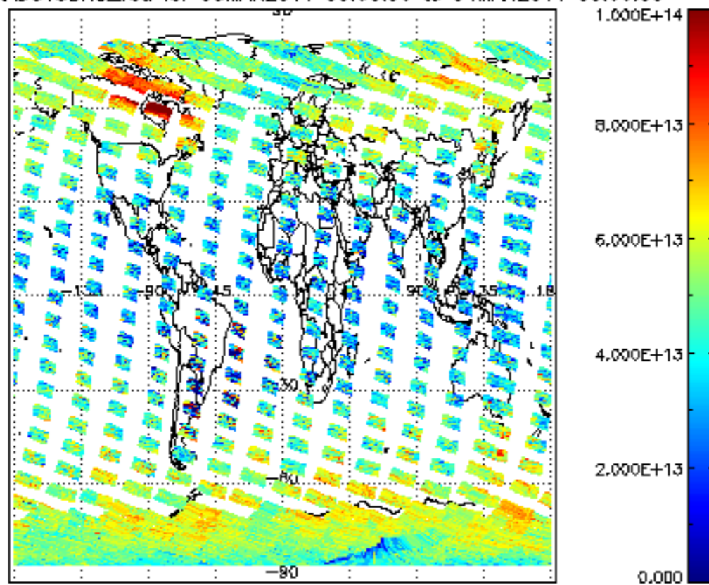
SCIOL2P_NADUV3BRO_vcd for 03MAR2011 00:00:00 to 04MAR2011 00:00:00
