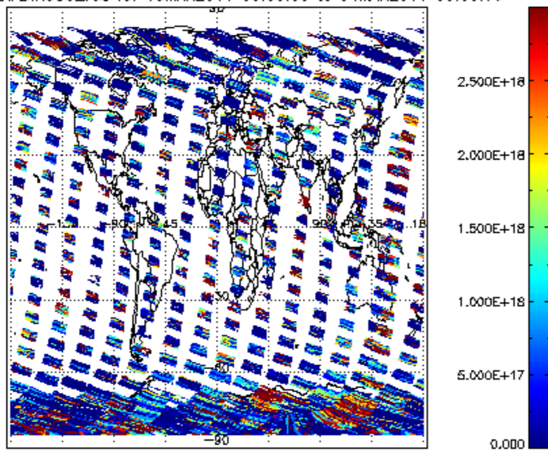
SCIOL2P_NADIR3CO_vcd for 03MAR2011 00:00:00 to 04MAR2011 00:00:00
