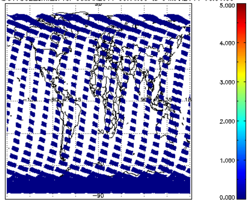
SCIOL2P_NADUV7S02_amf_cl for 03MAR2011 00:00:00 to 04MAR2011 00:00:00
