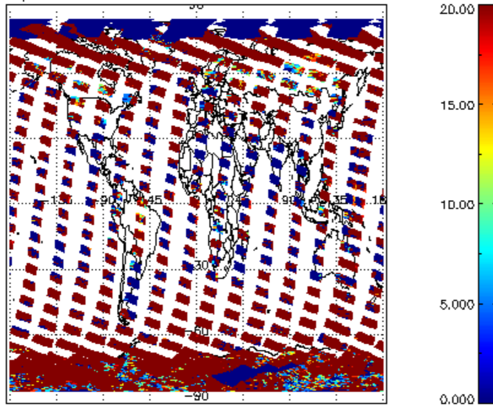
cL_opt_depth for 03MAR2011 00:00:00 to 04MAR2011 00:00:00
