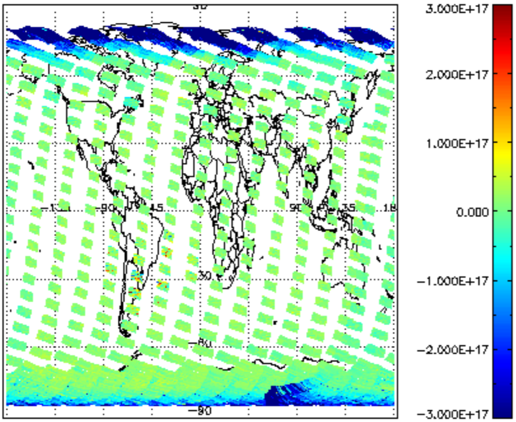
SCIOL2P_NADUV7S02_vcd for 03MAR2011 00:00:00 to 04MAR2011 00:00:00
