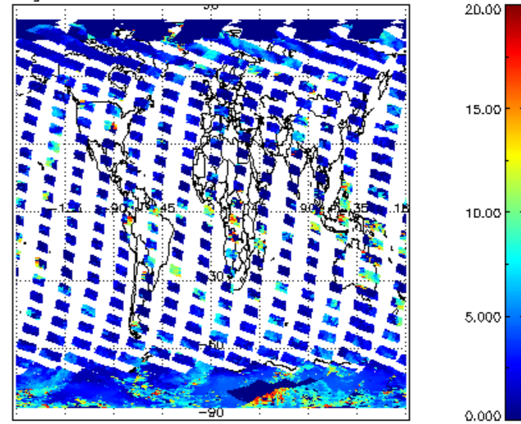
cL_top_height for 03MAR2011 00:00:00 to 04MAR2011 00:00:00
