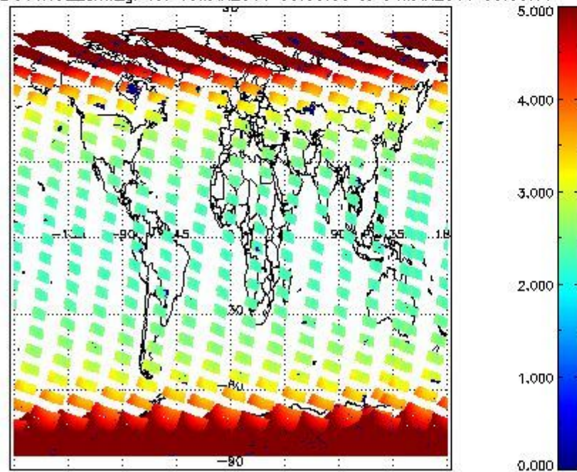
SCIOL2P_NADUV1NO2_amf_gr for 03MAR2011 00:00:00 to 04MAR2011 00:00:00
