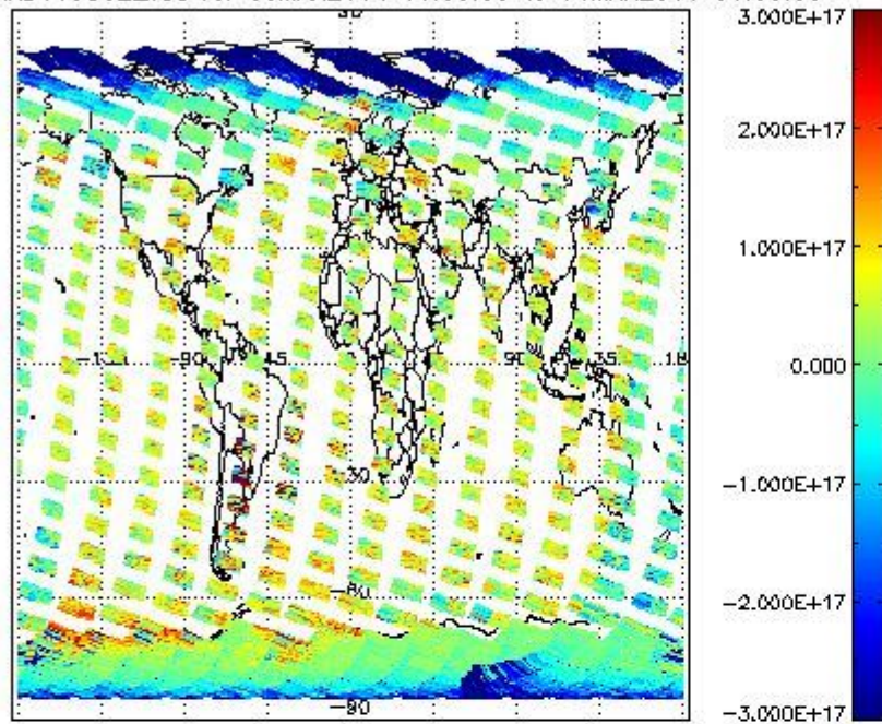
SCIOL2P_NADUV5SO2_vcd for 03MAR2011 00:00:00 to 04MAR2011 00:00:00
