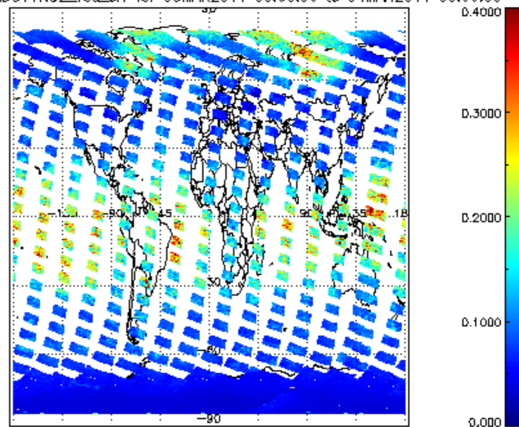
SCIOL2P_NADUV1NO2_vcd_Lerr for 03MAR2011 00:00:00 to 04MAR2011 00:00:00
