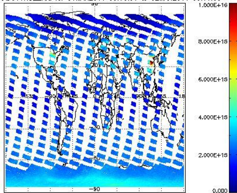
SCIOL2P_NADUV1NO2_vcd for 01MAR2011 00:00:00 to 02MAR2011 00:00:00
