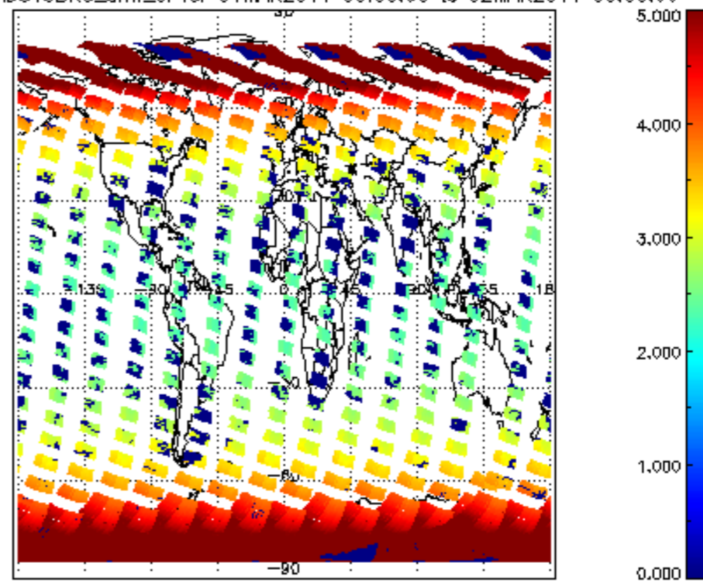
SCIOL2P_NADUV3BRO_amf_cl for 01MAR2011 00:00:00 to 02MAR2011 00:00:00
