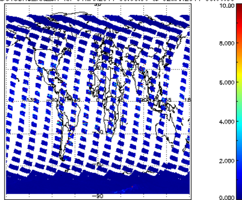
SCIOL2P_NADUV3BRO_vcd_err for 01MAR2011 00:00:00 to 02MAR2011 00:00:00
