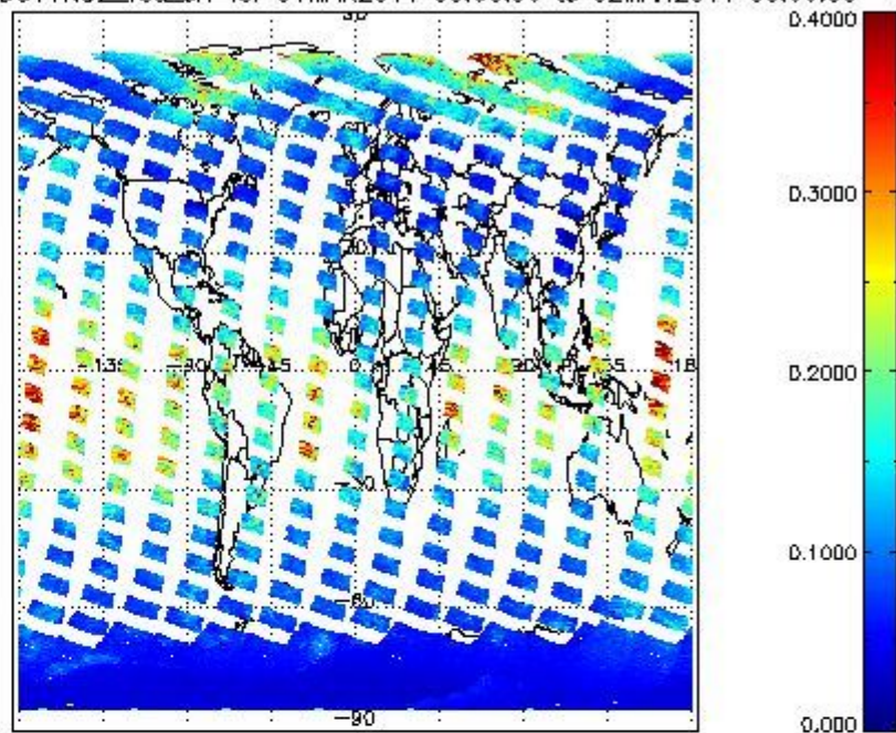
SCIOL2P_NADUV1NO2_vcd_err for 01MAR2011 00:00:00 to 02MAR2011 00:00:00
