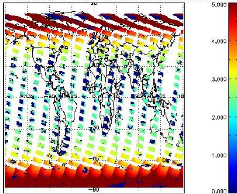
SCIOL2P_NADUV1NO2_amf_cl for 01MAR2011 00:00:00 to 02MAR2011 00:00:00
