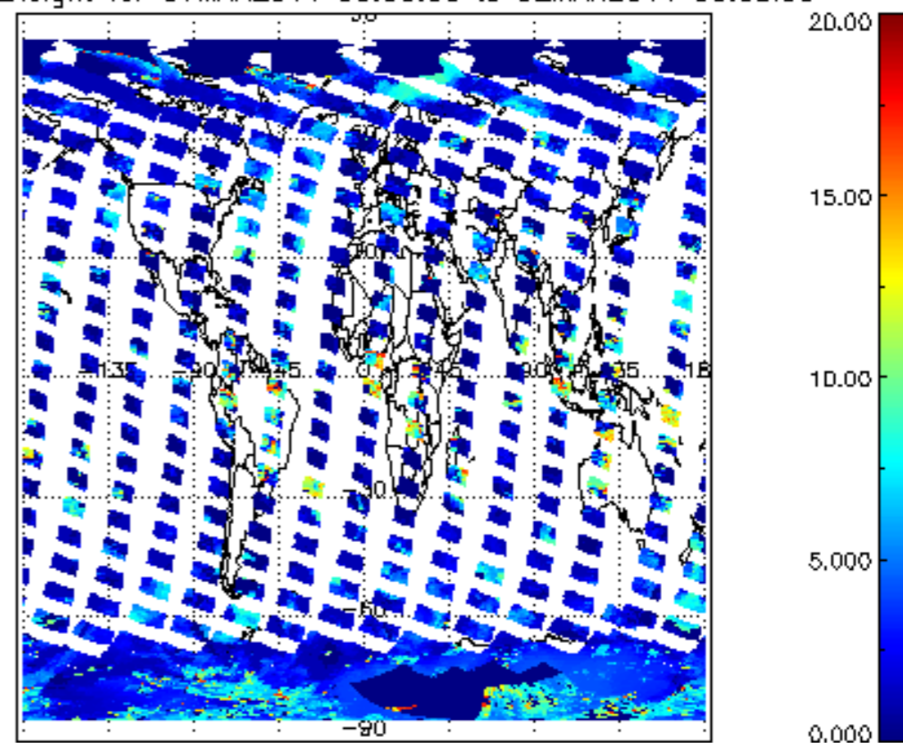
cL_top_height for 01MAR2011 00:00:00 to 02MAR2011 00:00:00
