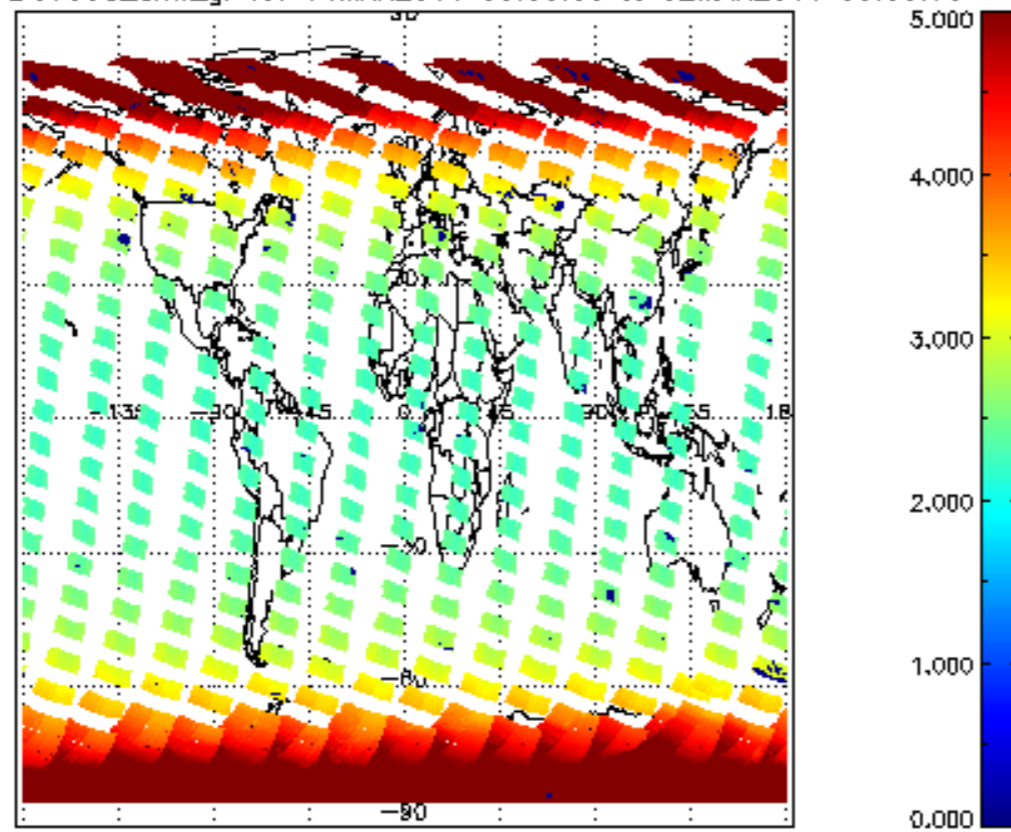
SCIOL2P_NADUV003_arnf_gr for 01MAR2011 00:00:00 to 02MAR2011 00:00:00
