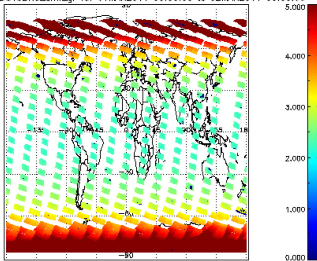
SCIOL2P_NADUV3BRO_amf_gr for 01MAR2011 00:00:00 to 02MAR2011 00:00:00
