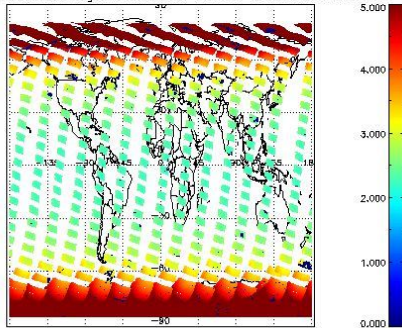
SCIOL2P_NADUV1NO2_amf_gr for 01MAR2011 00:00:00 to 02MAR2011 00:00:00
