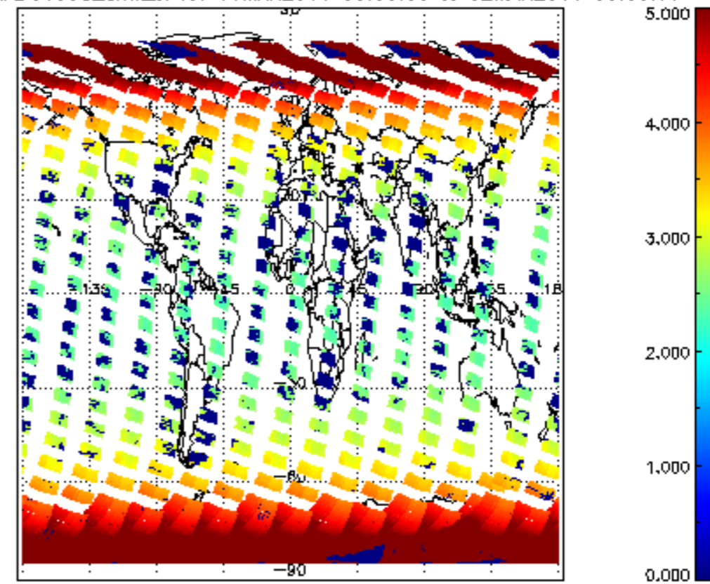
SCIOL2P_NADUV003_arnf_cl for 01MAR2011 00:00:00 to 02MAR2011 00:00:00
