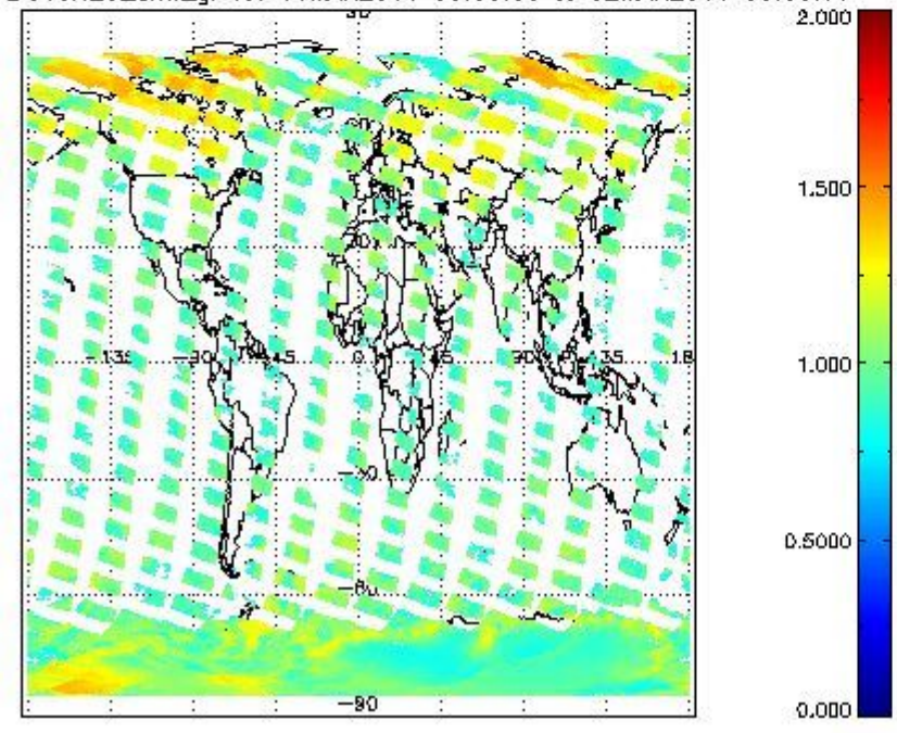
SCIOL2P_NADUV8H2O_arnf_gr for 01MAR2011 00:00:00 to 02MAR2011 00:00:00
