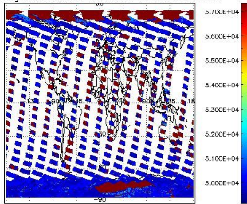
cloud_flags for 26FEB2011 00:00:00 to 27FEB2011 00:00:00
