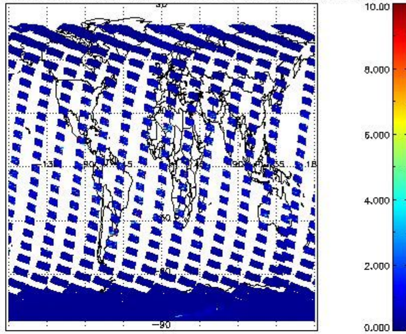
SCIOL2P_NADUV3BRO_vcd_err for 26FEB2011 00:00:00 to 27FEB2011 00:00:00
