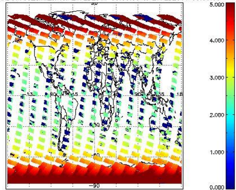
SCIOL2P_NADUV003_amf_cl for 26FEB2011 00:00:00 to 27FEB2011 00:00:00
