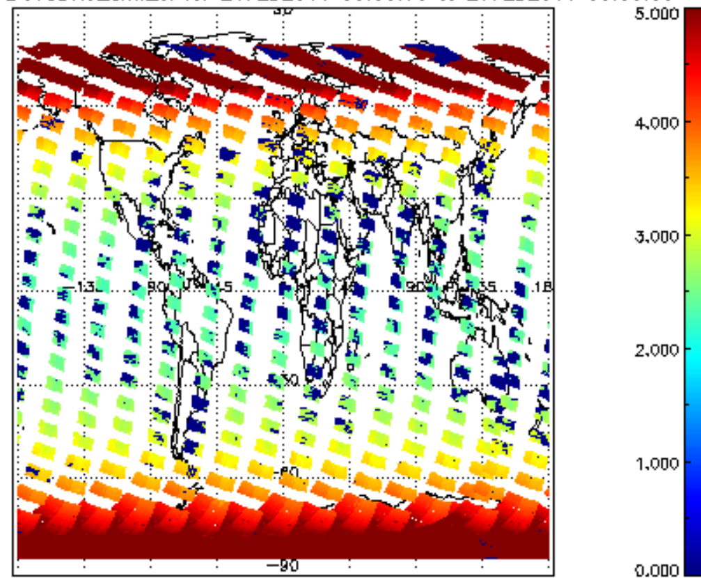
SCIOL2P_NADUV3BRO_amf_cl for 26FEB2011 00:00:00 to 27FEB2011 00:00:00
