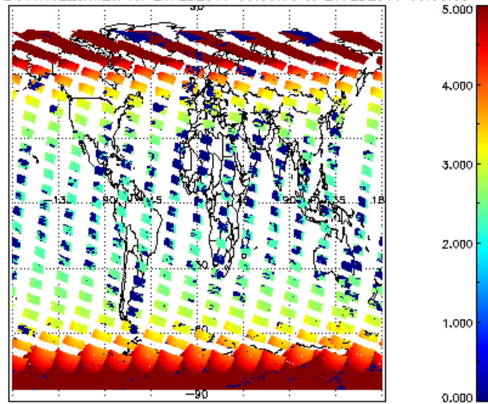
SCIOL2P_NADUV1N02_amf_cl for 26FEB2011 00:00:00 to 27FEB2011 00:00:00
