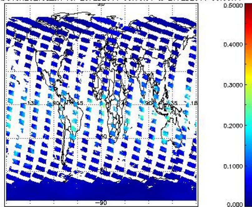
SCIOL2P_NADUV8H2O_vcd_err for 26FEB2011 00:00:00 to 27FEB2011 00:00:00
