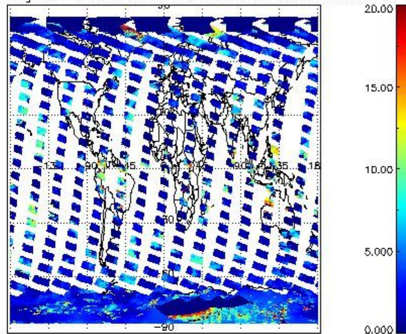
cL_top_height for 26FEB2011 00:00:00 to 27FEB2011 00:00:00
