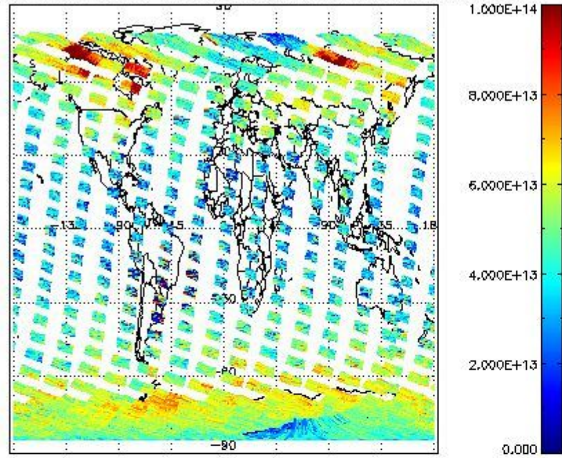
SCIOL2P_NADUV3BRO_vcd for 26FEB2011 00:00:00 to 27FEB2011 00:00:00
