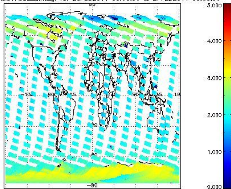
SCIOL2P_NADUV7S02_amf_gr for 26FEB2011 00:00:00 to 27FEB2011 00:00:00
