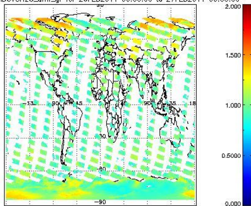
SCIOL2P_NADUV8H2O_amf_gr for 26FEB2011 00:00:00 to 27FEB2011 00:00:00
