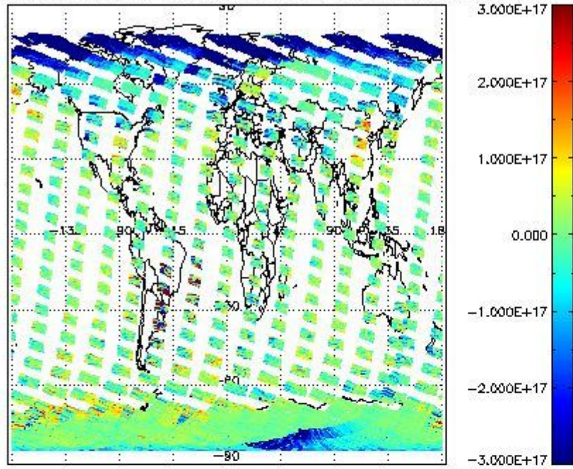
SCIOL2P_NADUV5S02_vcd for 26FEB2011 00:00:00 to 27FEB2011 00:00:00
