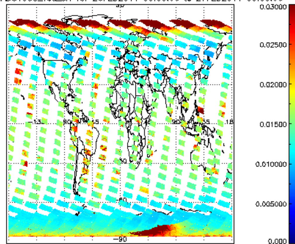
SCIOL2P_NADUV003_vcd_err for 26FEB2011 00:00:00 to 27FEB2011 00:00:00
