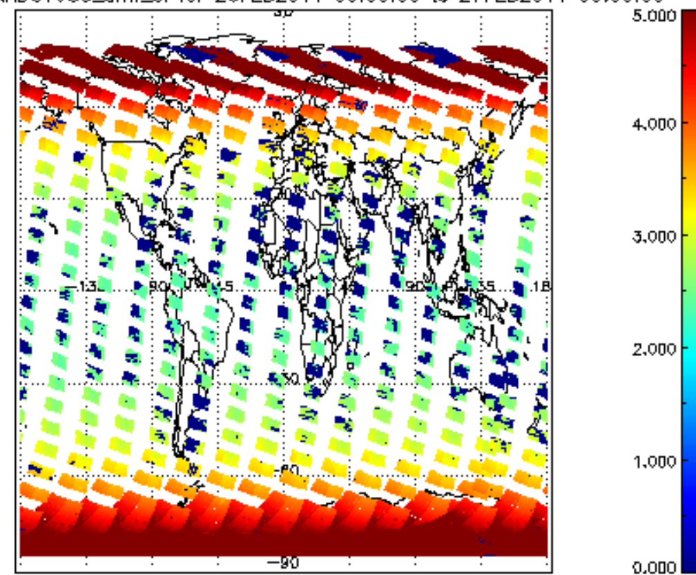
SCIOL2P_NADUV003_amf_cl for 26FEB2011 00:00:00 to 27FEB2011 00:00:00
