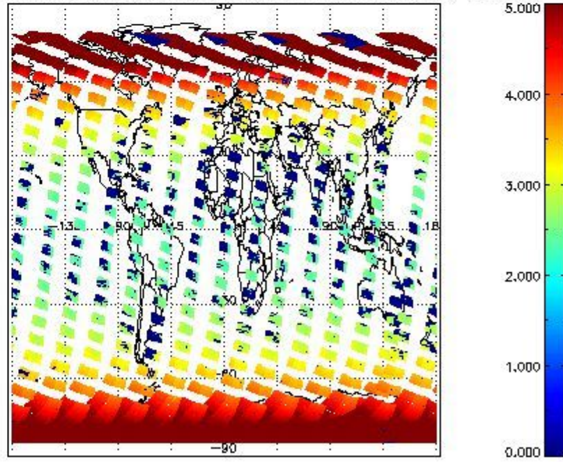
SCIOL2P_NADUV3BRO_amf_cl for 26FEB2011 00:00:00 to 27FEB2011 00:00:00
