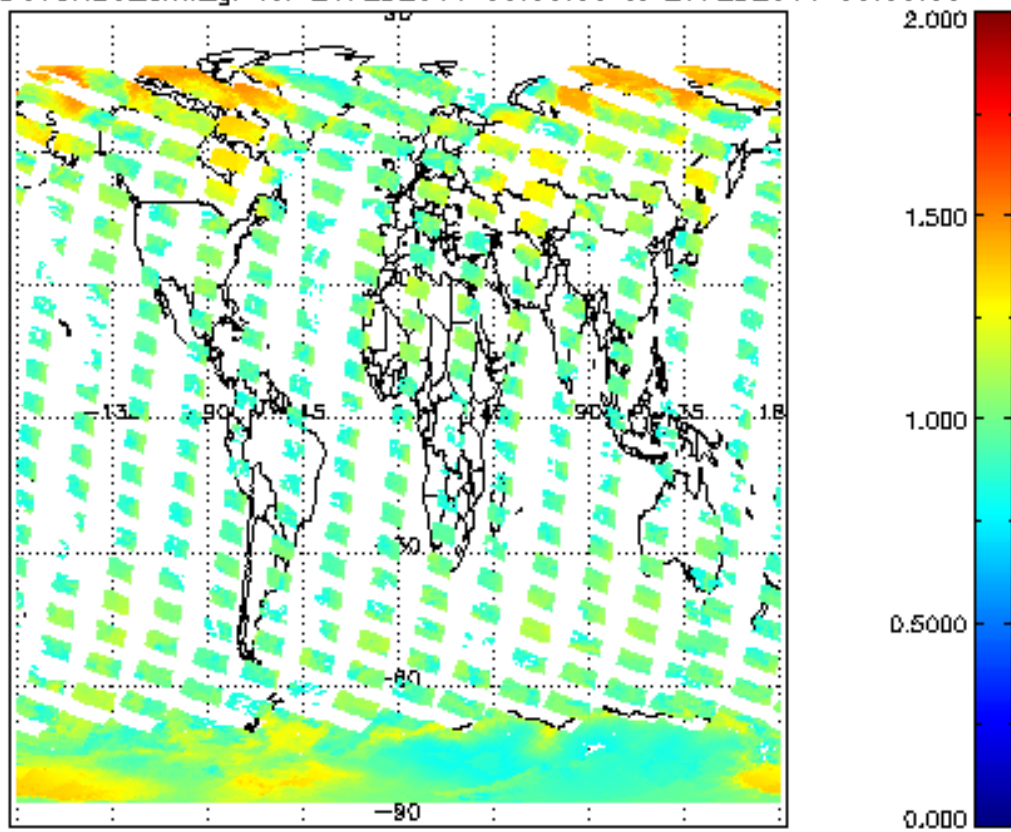
SCIOL2P_NADUV8H2O_amf_gr for 26FEB2011 00:00:00 to 27FEB2011 00:00:00
