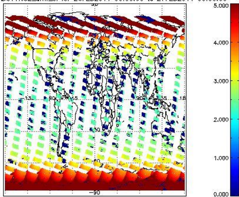
SCIOL2P_NADUV1N02_amf_cl for 26FEB2011 00:00:00 to 27FEB2011 00:00:00
