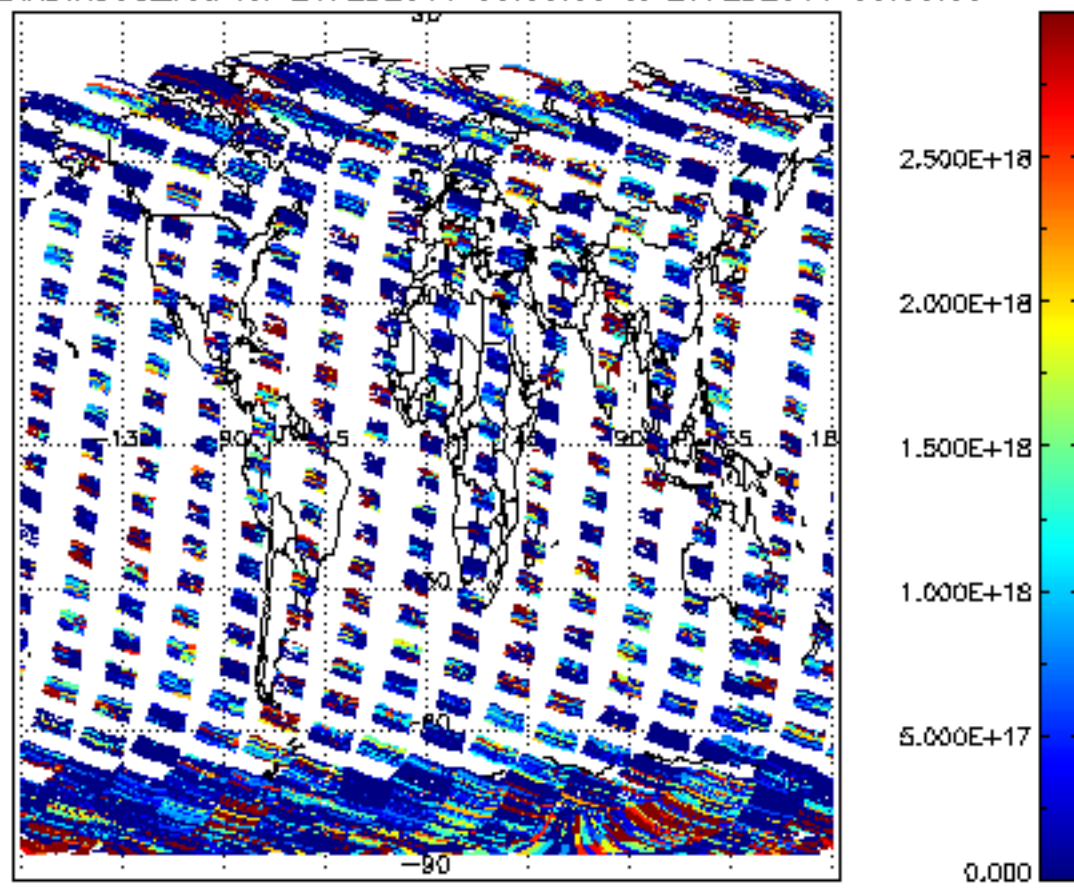
SCIOL2P_NADIR3CO_vcd for 26FEB2011 00:00:00 to 27FEB2011 00:00:00
