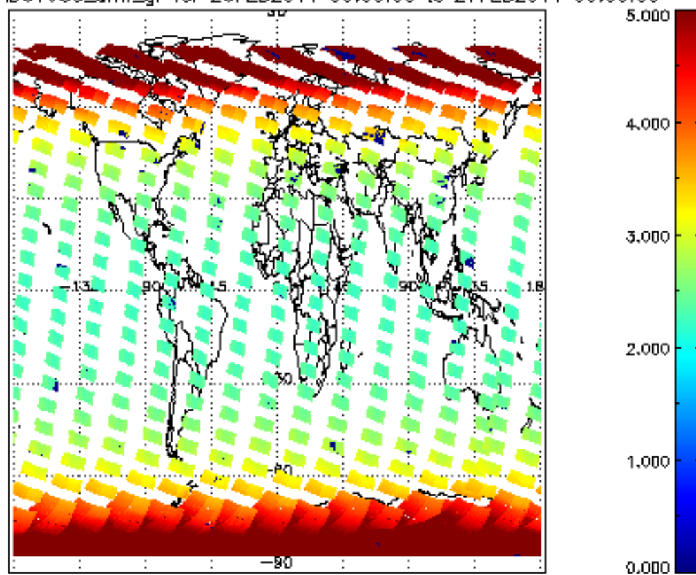
SCIOL2P_NADUV003_amf_gr for 26FEB2011 00:00:00 to 27FEB2011 00:00:00
