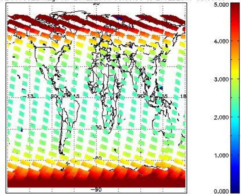
SCIOL2P_NADUV003_amf_gr for 26FEB2011 00:00:00 to 27FEB2011 00:00:00
