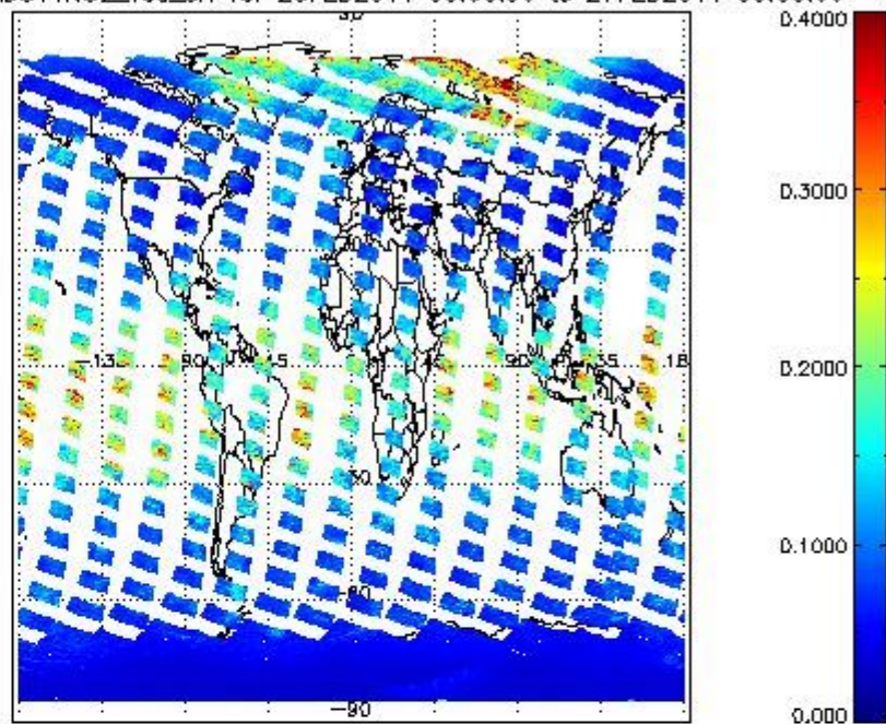
SCIOL2P_NADUV1N02_vcd_err for 26FEB2011 00:00:00 to 27FEB2011 00:00:00
