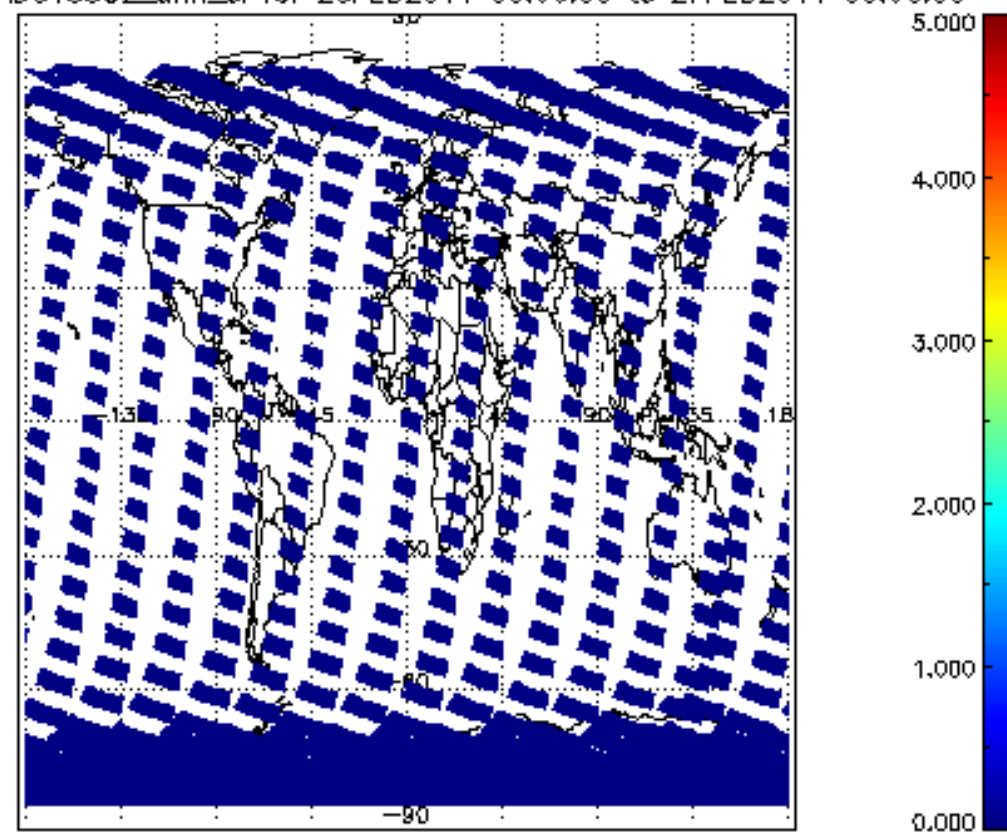
SCIOL2P_NADUV5S02_amf_cl for 26FEB2011 00:00:00 to 27FEB2011 00:00:00
