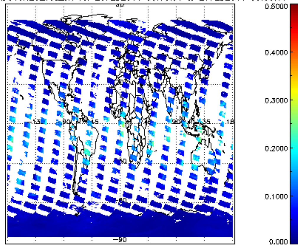
SCIOL2P_NADUV8H2O_vcd_err for 26FEB2011 00:00:00 to 27FEB2011 00:00:00
