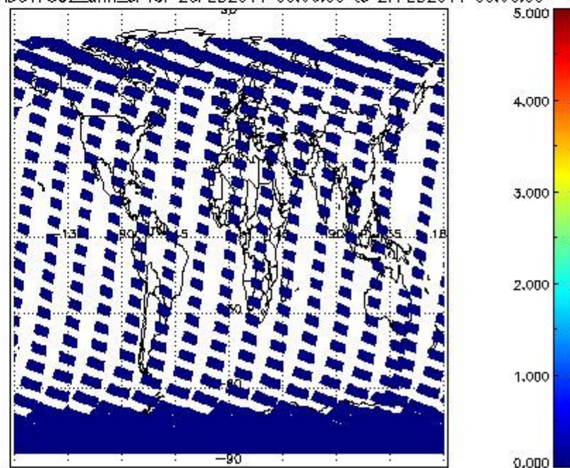
SCIOL2P_NADUV7S02_amf_cl for 26FEB2011 00:00:00 to 27FEB2011 00:00:00
