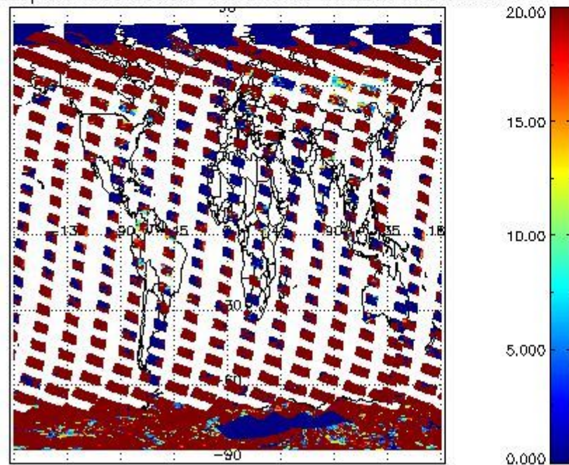
cL_opt_depth for 26FEB2011 00:00:00 to 27FEB2011 00:00:00
