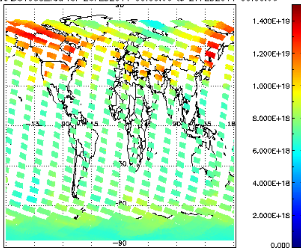
SCIOL2P_NADUV003_vcd for 26FEB2011 00:00:00 to 27FEB2011 00:00:00
