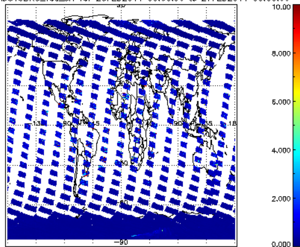
SCIOL2P_NADUV3BRO_vcd_err for 26FEB2011 00:00:00 to 27FEB2011 00:00:00
