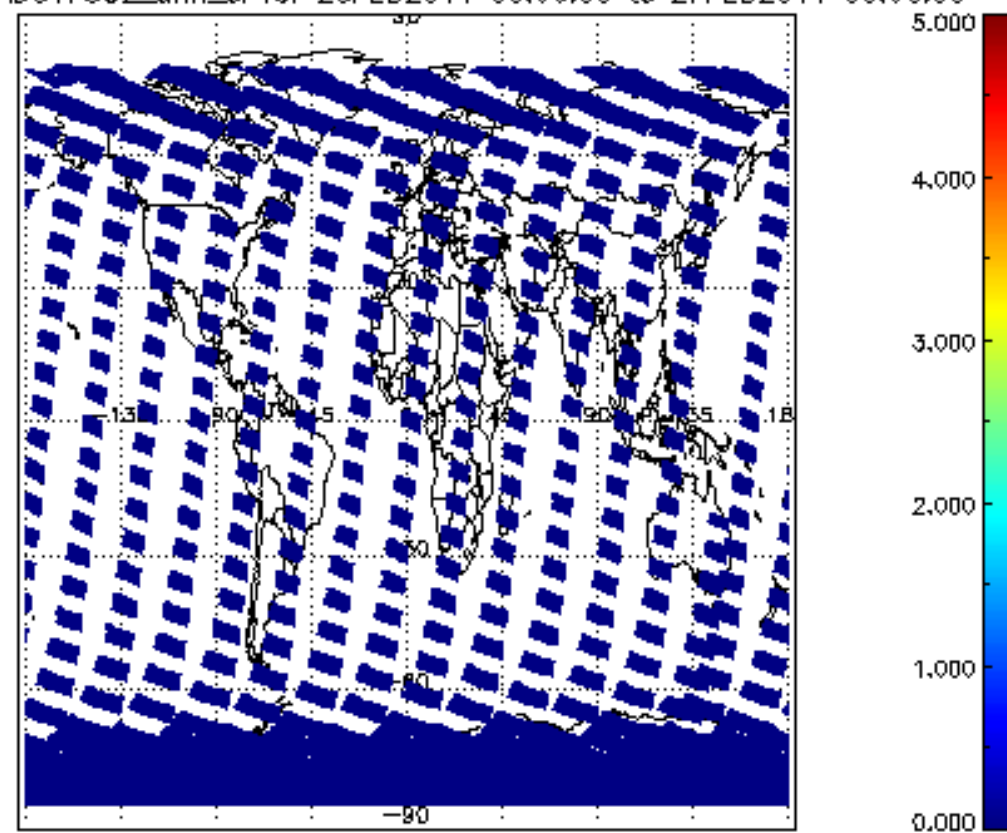
SCIOL2P_NADUV7S02_amf_cl for 26FEB2011 00:00:00 to 27FEB2011 00:00:00
