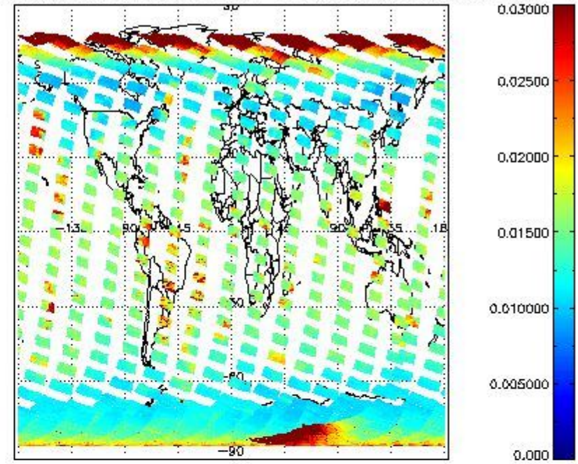
SCIOL2P_NADUV003_vcd_err for 26FEB2011 00:00:00 to 27FEB2011 00:00:00
