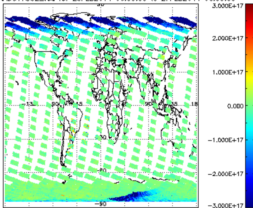
SCIOL2P_NADUV7S02_vcd for 26FEB2011 00:00:00 to 27FEB2011 00:00:00
