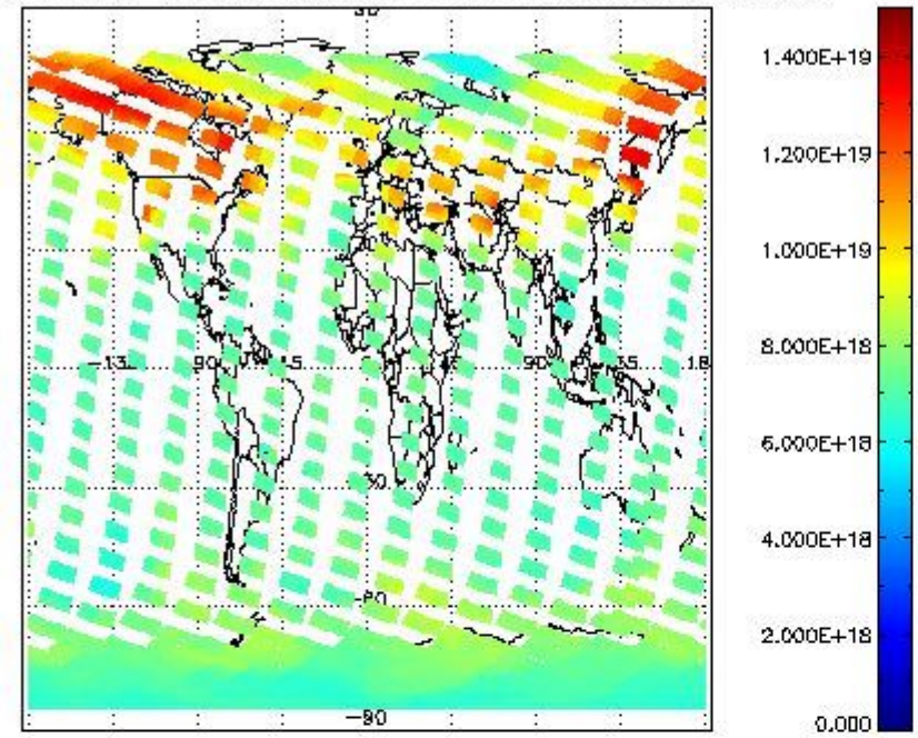
SCIOL2P_NADUV003_vcd for 26FEB2011 00:00:00 to 27FEB2011 00:00:00
