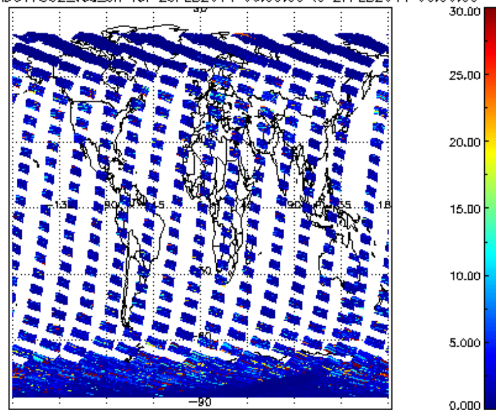
SCIOL2P_NADUV7S02_vcd_err for 26FEB2011 00:00:00 to 27FEB2011 00:00:00
