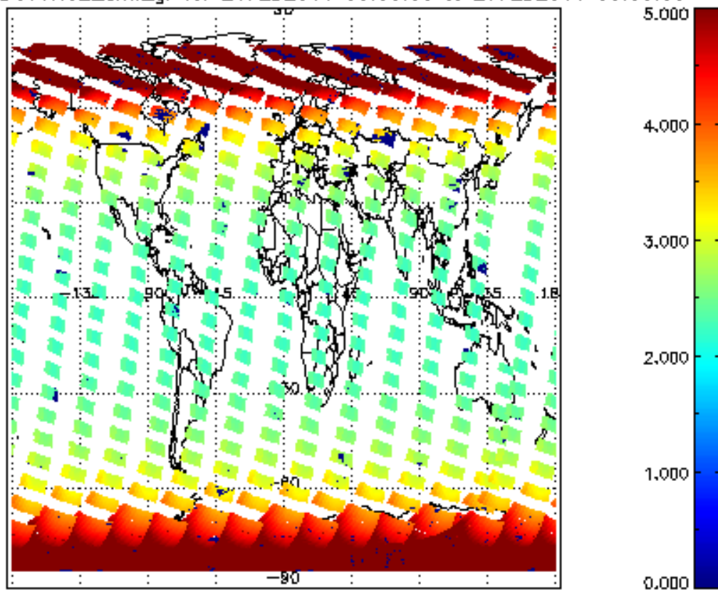
SCIOL2P_NADUV1N02_amf_gr for 26FEB2011 00:00:00 to 27FEB2011 00:00:00
