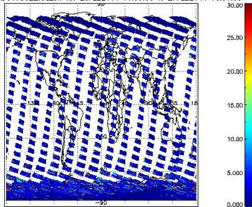
SCIOL2P_NADUV7S02_vcd_err for 26FEB2011 00:00:00 to 27FEB2011 00:00:00
