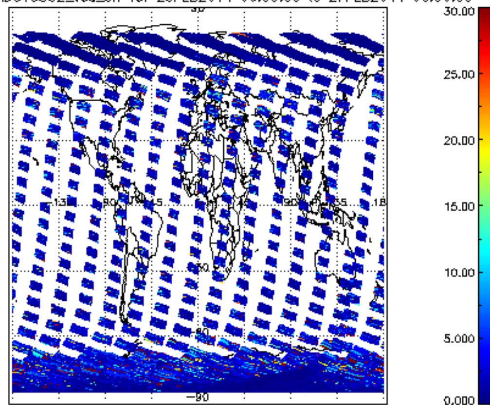
SCIOL2P_NADUV5S02_vcd_err for 26FEB2011 00:00:00 to 27FEB2011 00:00:00
