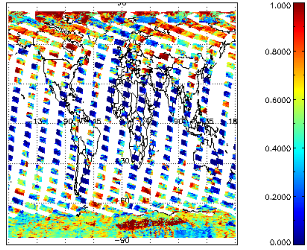
cl_frac for 26FEB2011 00:00:00 to 27FEB2011 00:00:00
