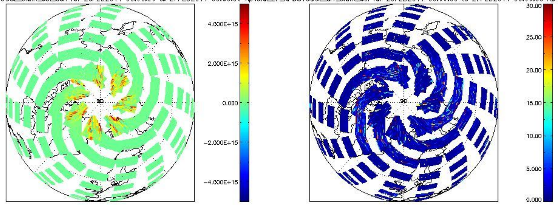
CIOL2P_NADUV6OCL_slant_col_den for 26FEB2011 00:00:00 to 27FEB2011 00:00:00 np; CIOL2P_NADUV6OCL_err_slant_col for 26FEB2011 00:00:00 to 27FEB2011 00:00:00 np
