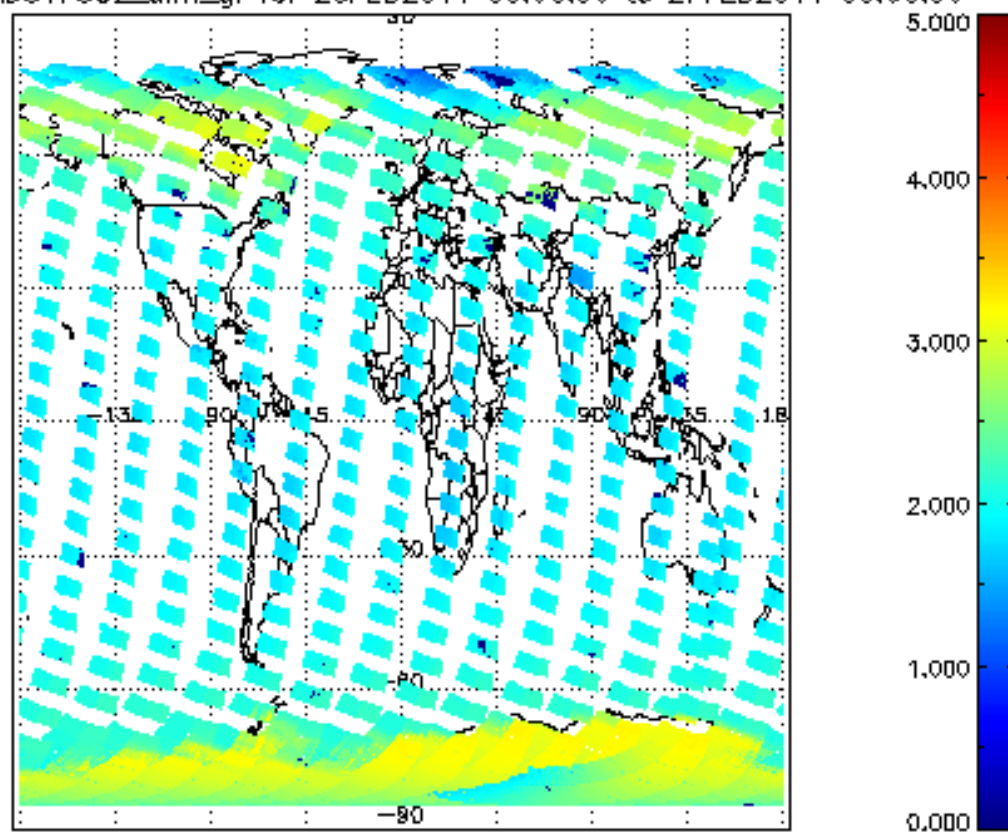
SCIOL2P_NADUV7S02_amf_gr for 26FEB2011 00:00:00 to 27FEB2011 00:00:00
