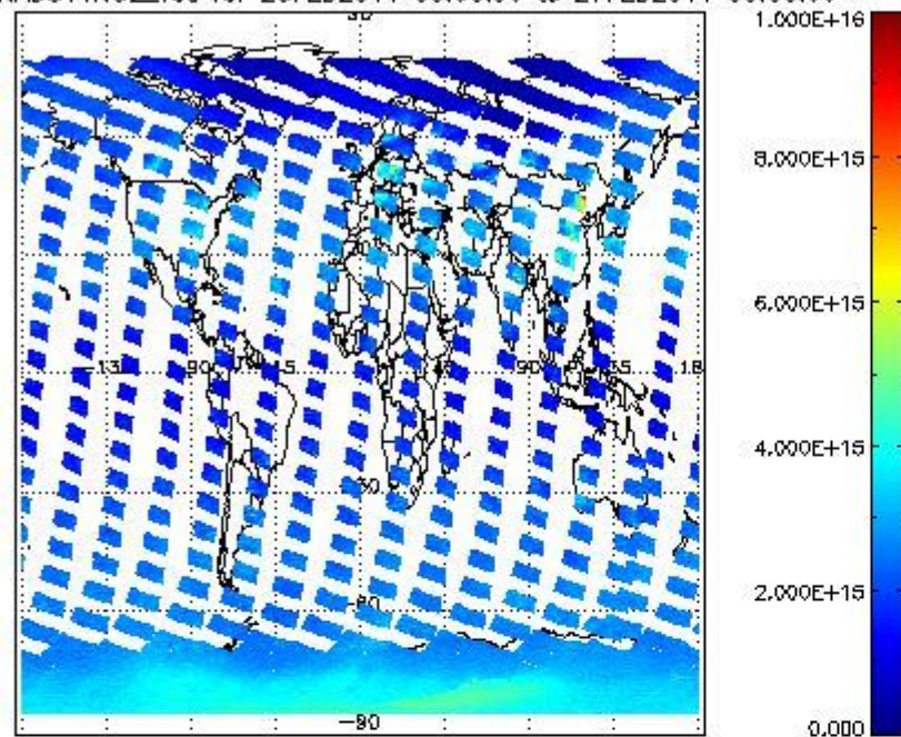
SCIOL2P_NADUV1N02_vcd for 26FEB2011 00:00:00 to 27FEB2011 00:00:00
