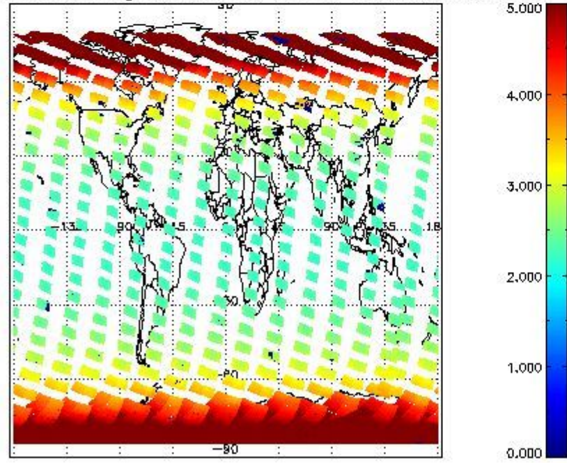
SCIOL2P_NADUV3BRO_amf_gr for 26FEB2011 00:00:00 to 27FEB2011 00:00:00
