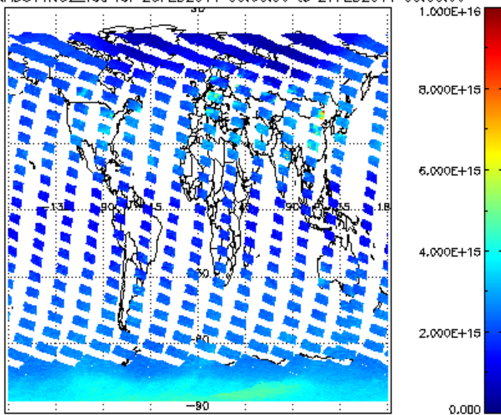
SCIOL2P_NADUV1N02_vcd for 26FEB2011 00:00:00 to 27FEB2011 00:00:00
