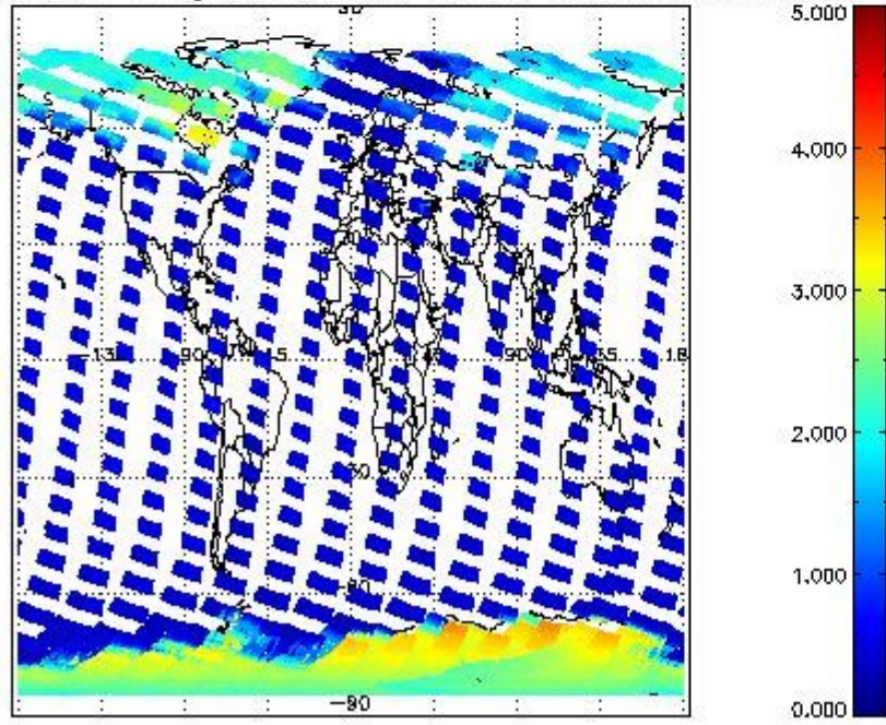
SCIOL2P_NADUV5S02_amf_gr for 26FEB2011 00:00:00 to 27FEB2011 00:00:00
