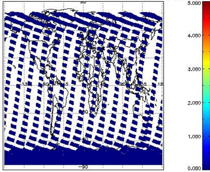
SCIOL2P_NADUV5S02_amf_cl for 26FEB2011 00:00:00 to 27FEB2011 00:00:00
