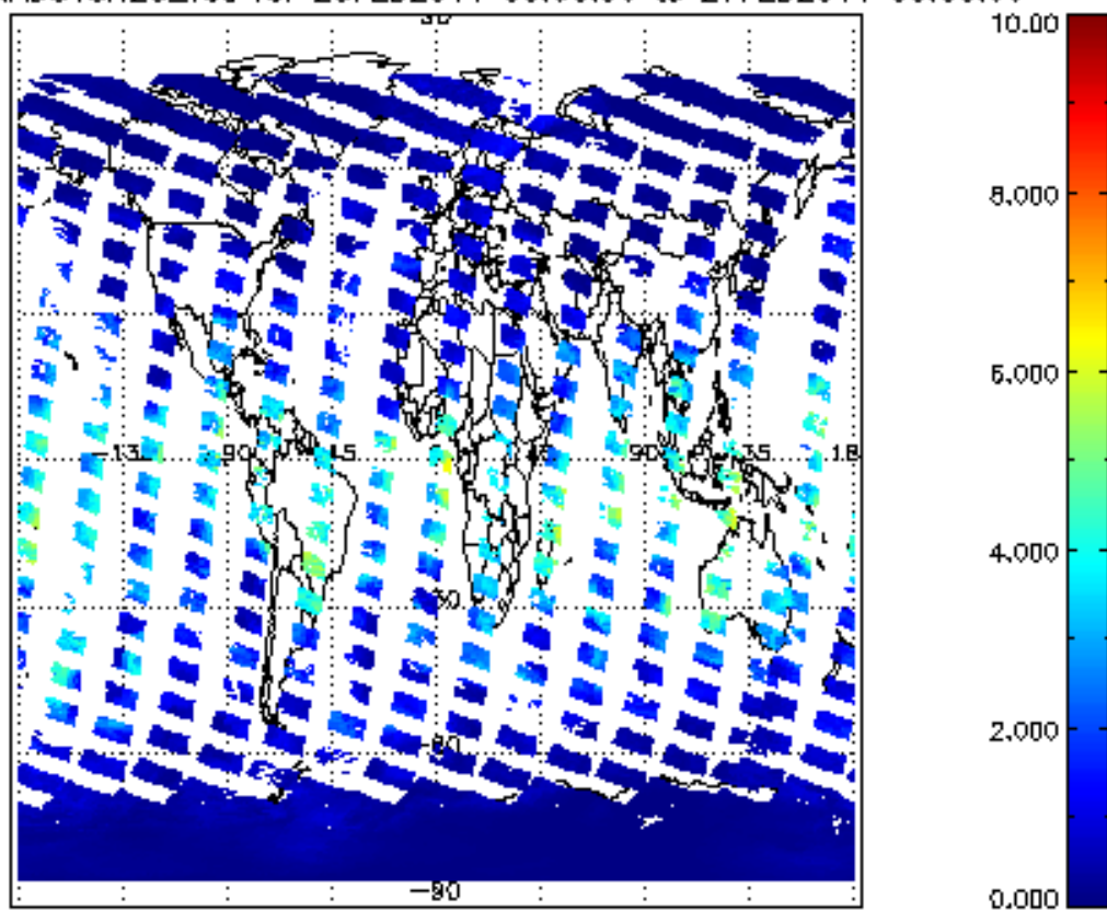
SCIOL2P_NADUV8H2O_vcd for 26FEB2011 00:00:00 to 27FEB2011 00:00:00
