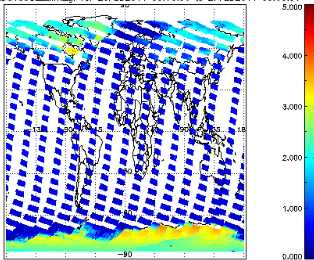
SCIOL2P_NADUV5S02_amf_gr for 26FEB2011 00:00:00 to 27FEB2011 00:00:00
