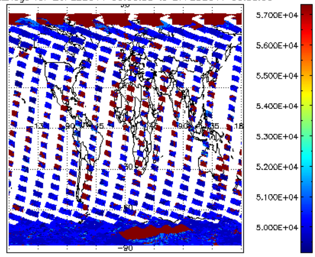
cloud_flags for 26FEB2011 00:00:00 to 27FEB2011 00:00:00
