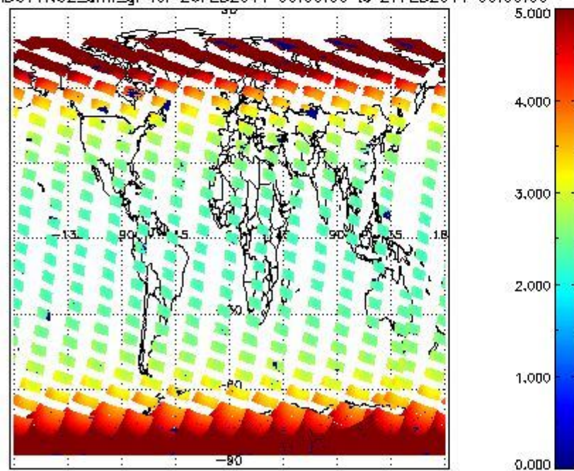
SCIOL2P_NADUV1N02_amf_gr for 26FEB2011 00:00:00 to 27FEB2011 00:00:00
