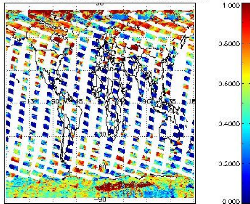
cL_frac for 26FEB2011 00:00:00 to 27FEB2011 00:00:00
