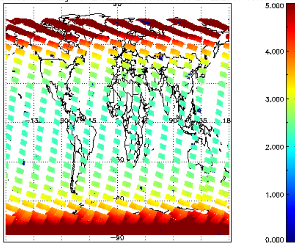
SCIOL2P_NADUV3BRO_amf_gr for 26FEB2011 00:00:00 to 27FEB2011 00:00:00
