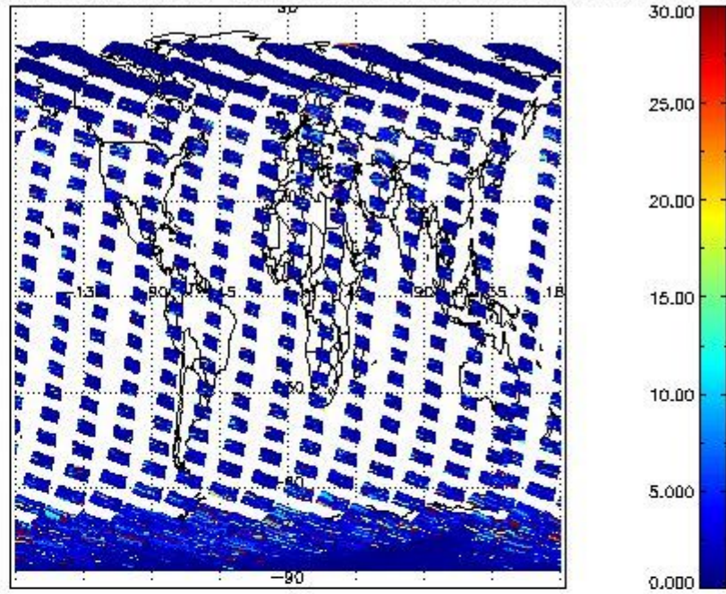
SCIOL2P_NADUV5S02_vcd_err for 26FEB2011 00:00:00 to 27FEB2011 00:00:00
