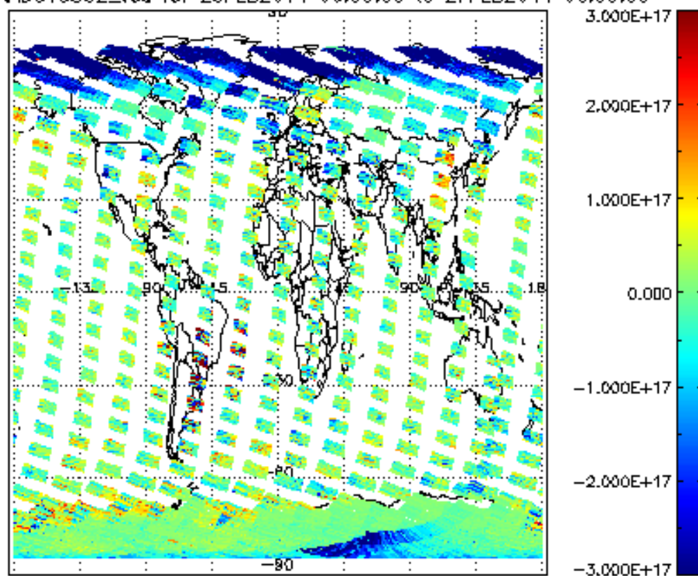
SCIOL2P_NADUV5S02_vcd for 26FEB2011 00:00:00 to 27FEB2011 00:00:00
