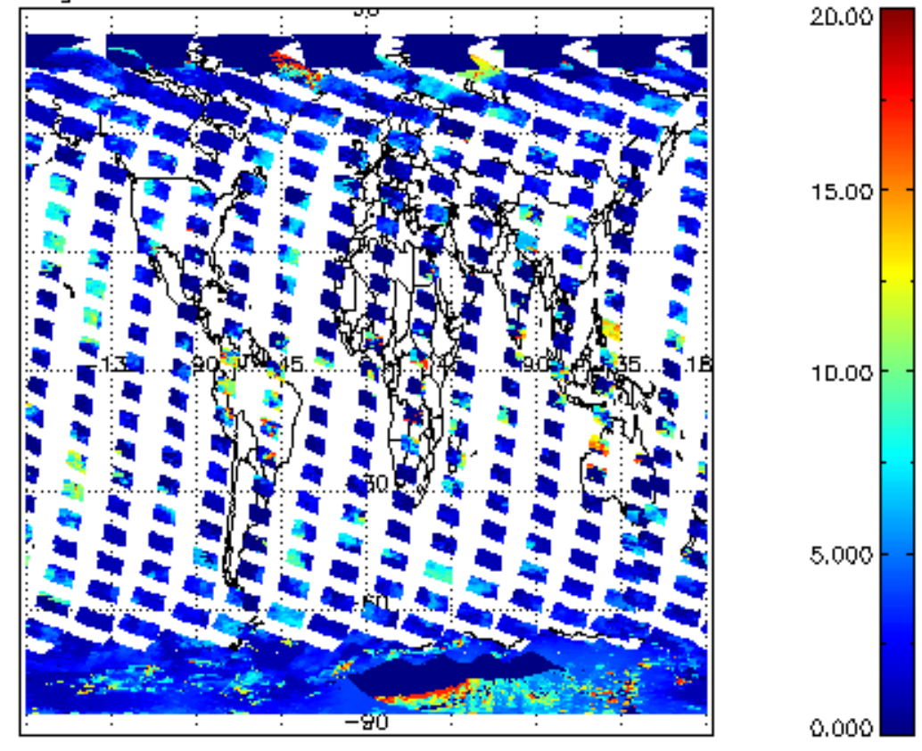
cl_top_height for 26FEB2011 00:00:00 to 27FEB2011 00:00:00
