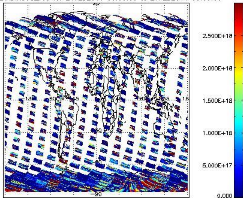
SCIDL2P_NADIR3CO_vcd for 26FEB2011 00:00:00 to 27FEB2011 00:00:00
