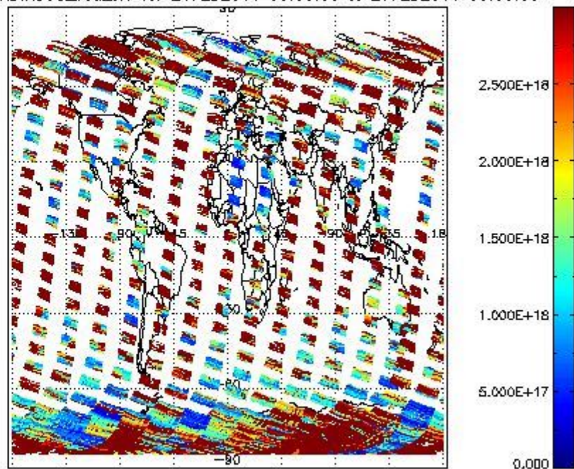
SCIDL2P_NADIR3CO_vcd_err for 26FEB2011 00:00:00 to 27FEB2011 00:00:00
