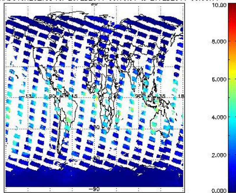
SCIOL2P_NADUV8H2O_vcd for 26FEB2011 00:00:00 to 27FEB2011 00:00:00
