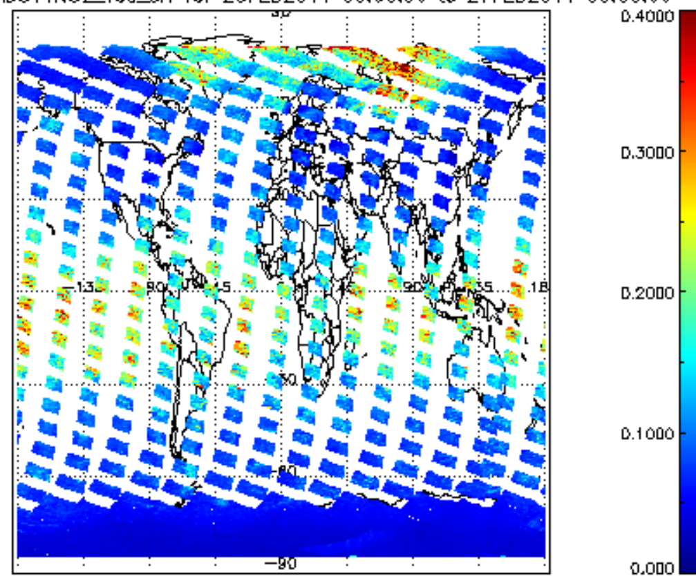
SCIOL2P_NADUV1N02_vcd_err for 26FEB2011 00:00:00 to 27FEB2011 00:00:00
