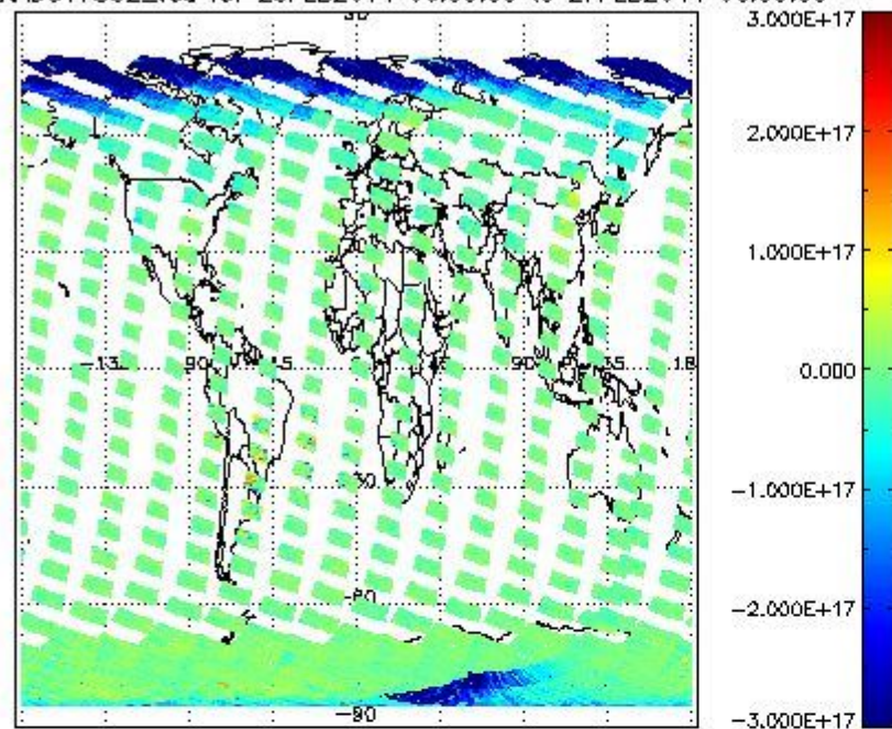
SCIOL2P_NADUV7S02_vcd for 26FEB2011 00:00:00 to 27FEB2011 00:00:00
