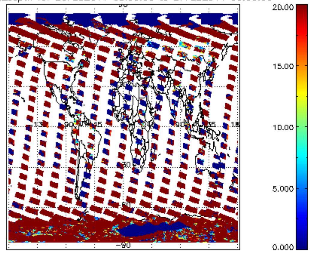
cl_opt_depth for 26FEB2011 00:00:00 to 27FEB2011 00:00:00
