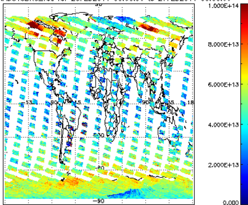
SCIOL2P_NADUV3BRO_vcd for 26FEB2011 00:00:00 to 27FEB2011 00:00:00
