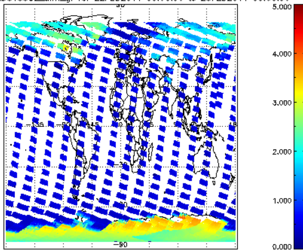
SCIOL2P_NADUV5S02_amf_gr for 22FEB2011 00:00:00 to 23FEB2011 00:00:00
