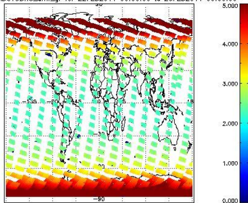
SCIOL2P_NADUV3BRO_amf_gr for 22FEB2011 00:00:00 to 23FEB2011 00:00:00
