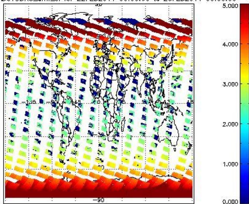
SCIOL2P_NADUV3BRO_amf_cl for 22FEB2011 00:00:00 to 23FEB2011 00:00:00
