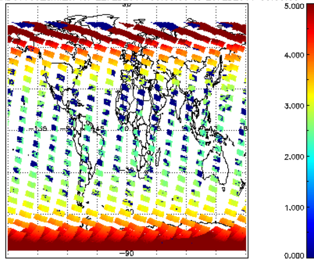
SCIOL2P_NADUV003_amf_cl for 22FEB2011 00:00:00 to 23FEB2011 00:00:00
