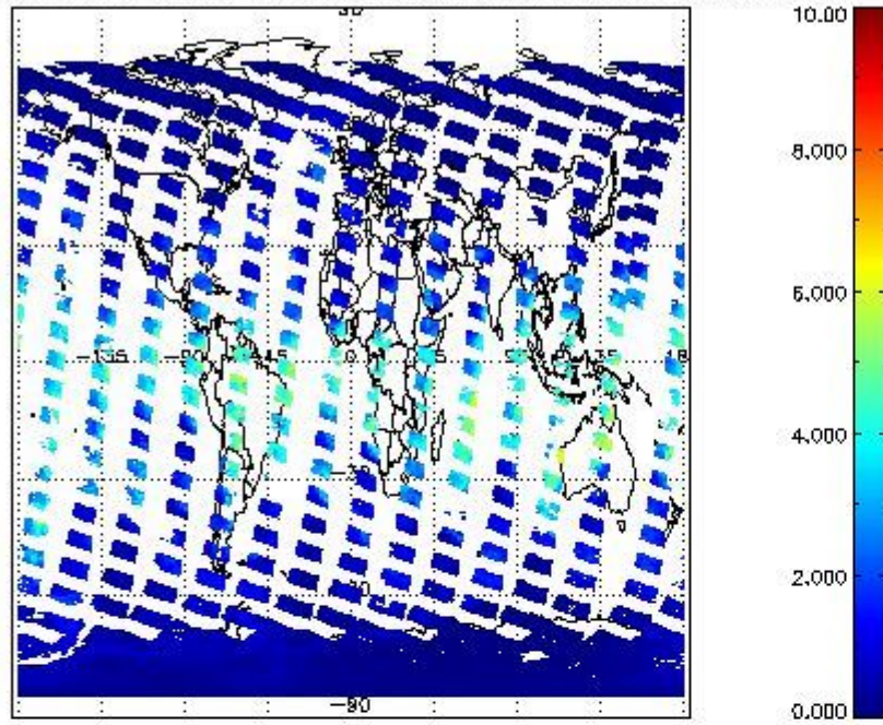
SCIOL2P_NADUV8H2O_vcd for 22FEB2011 00:00:00 to 23FEB2011 00:00:00
