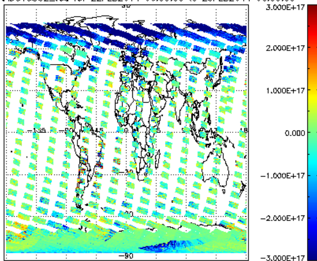
SCIOL2P_NADUV5S02_vcd for 22FEB2011 00:00:00 to 23FEB2011 00:00:00
