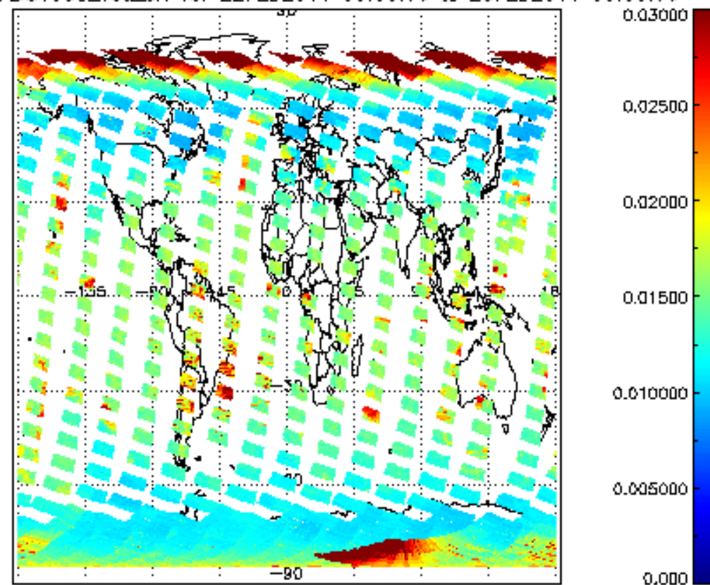
SCIOL2P_NADUV003_vcdLerr for 22FEB2011 00:00:00 to 23FEB2011 00:00:00
