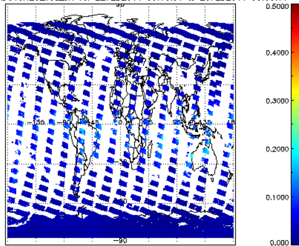
SCIOL2P_NADUV8H20_vcd_err for 22FEB2011 00:00:00 to 23FEB2011 00:00:00
