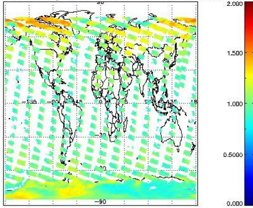
SCIOL2P_NADUV8H2O_amf_gr for 22FEB2011 00:00:00 to 23FEB2011 00:00:00
