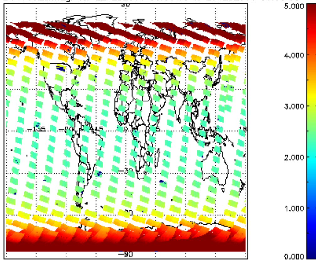
SCIOL2P_NADUV003_amf_gr for 22FEB2011 00:00:00 to 23FEB2011 00:00:00
