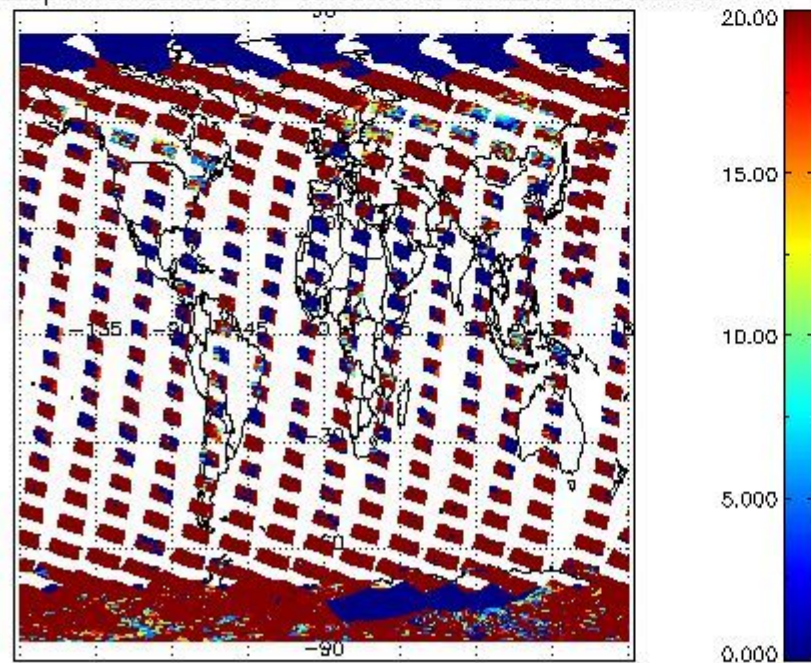
cL_opt_depth for 22FEB2011 00:00:00 to 23FEB2011 00:00:00
