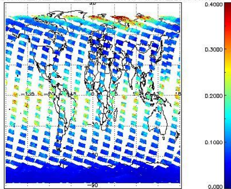
SCIOL2P_NADUV1N02_vcd_err for 22FEB2011 00:00:00 to 23FEB2011 00:00:00
