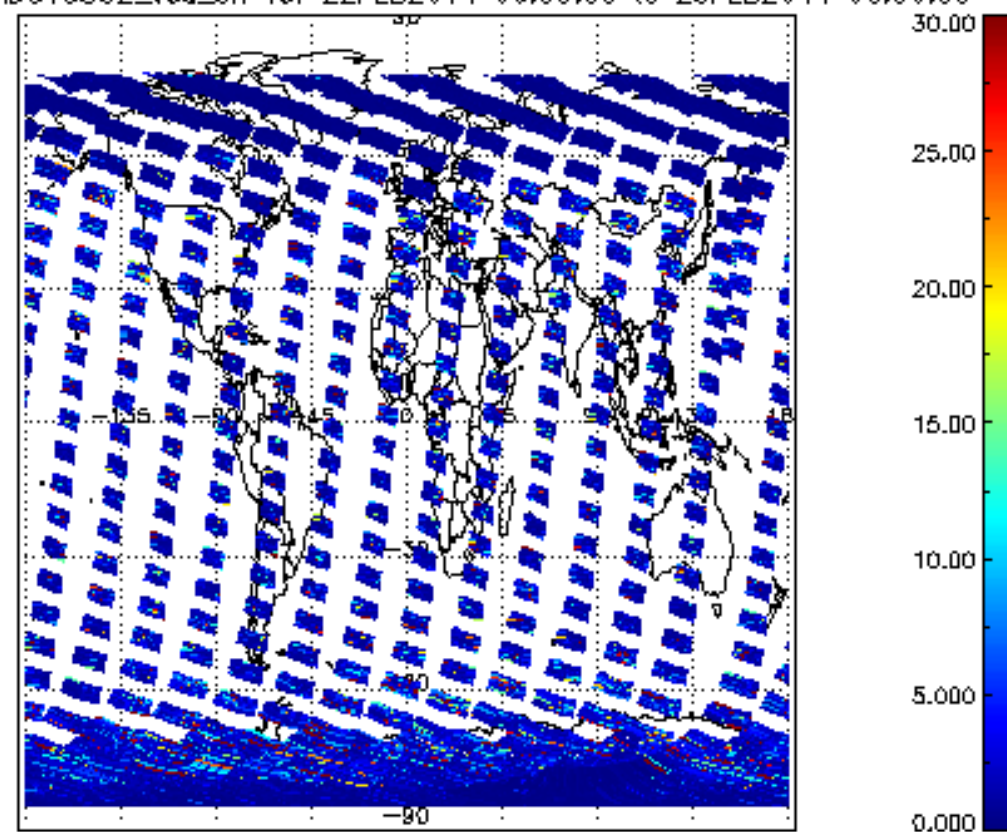
SCIOL2P_NADUV5S02_vcd_err for 22FEB2011 00:00:00 to 23FEB2011 00:00:00
