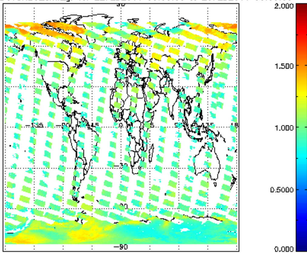
SCIOL2P_NADUV8H20_amf_gr for 22FEB2011 00:00:00 to 23FEB2011 00:00:00
