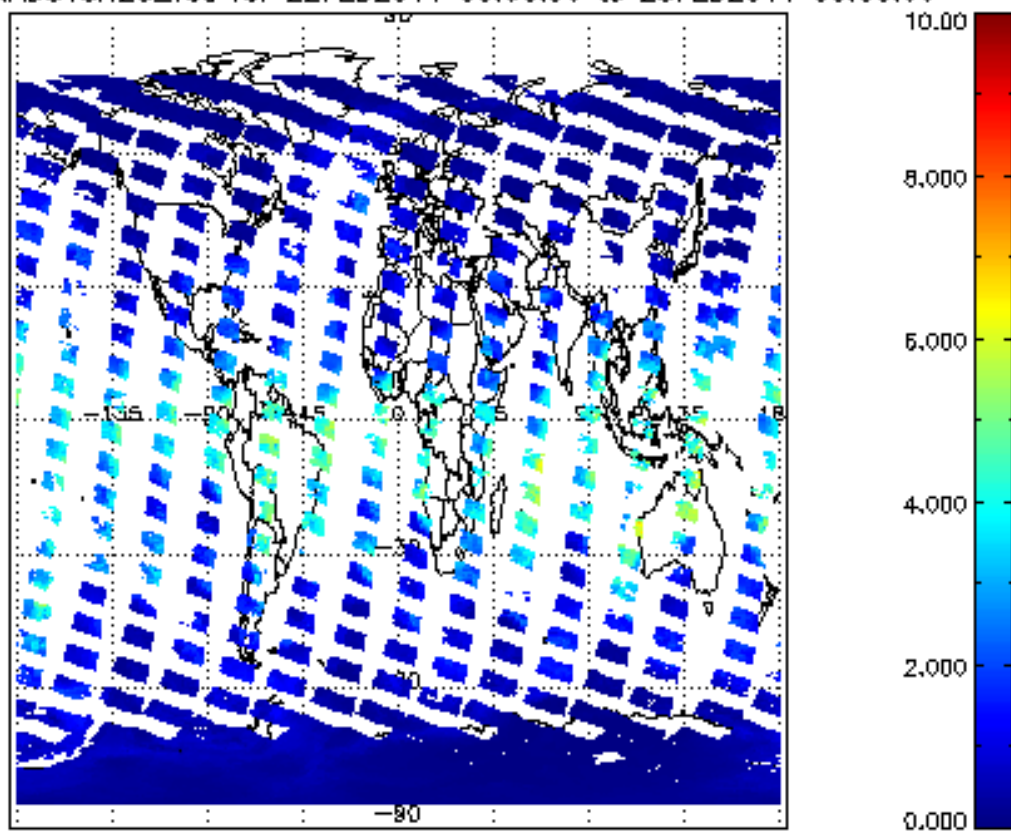
SCIOL2P_NADUV8H20_vcd for 22FEB2011 00:00:00 to 23FEB2011 00:00:00
