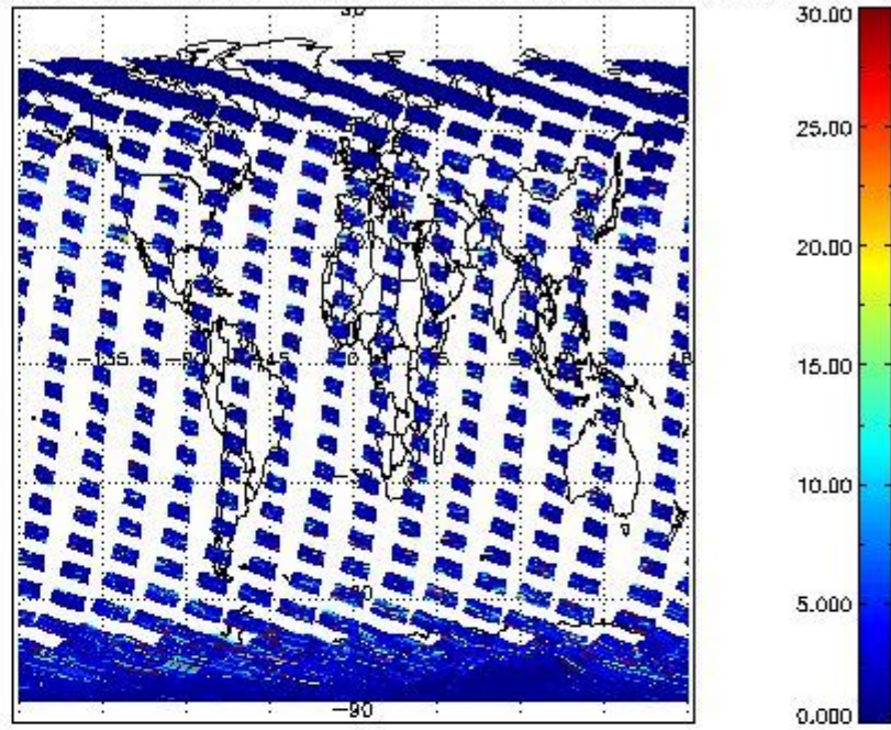
SCIOL2P_NADUV5SO2_vcd_err for 22FEB2011 00:00:00 to 23FEB2011 00:00:00
