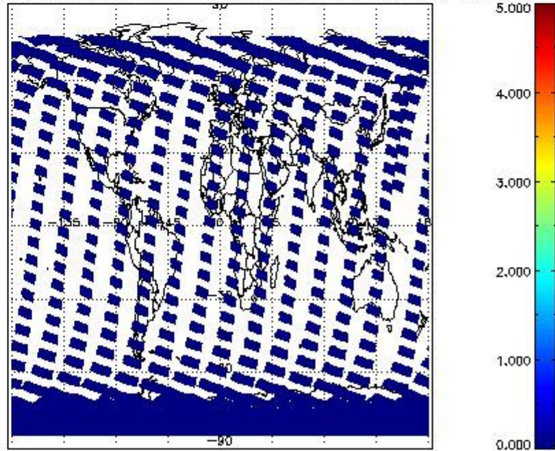
SCIOL2P_NADUV5SO2_amf_cl for 22FEB2011 00:00:00 to 23FEB2011 00:00:00
