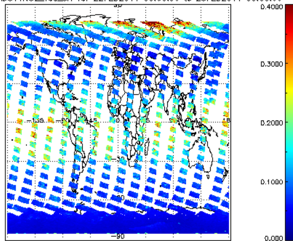
SCIOL2P_NADUV1N02_vcd_err for 22FEB2011 00:00:00 to 23FEB2011 00:00:00
