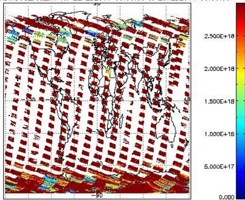
SCIO2P_NADIR3CO_vcd_err for 22FEB2011 00:00:00 to 23FEB2011 00:00:00
