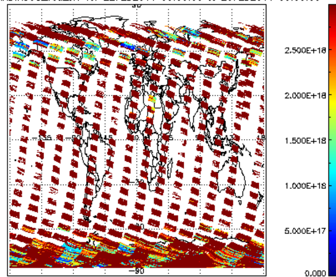
SCIOL2P_NADIR3CO_vcd_err for 22FEB2011 00:00:00 to 23FEB2011 00:00:00
