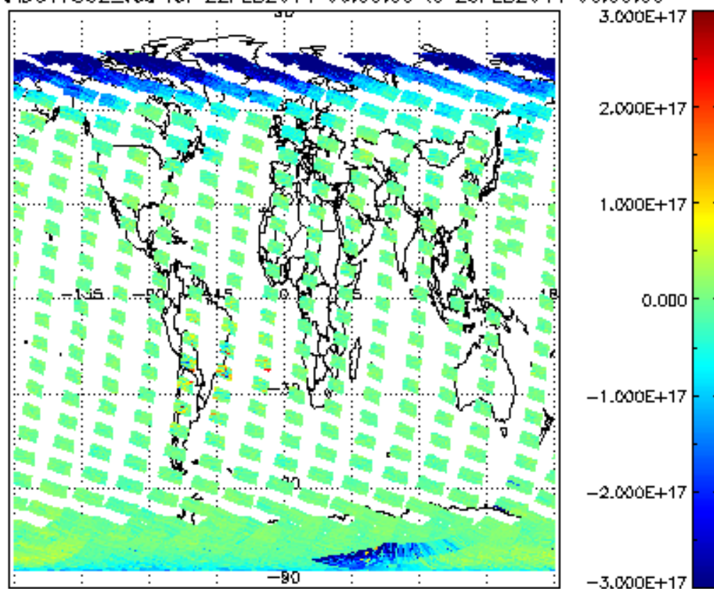
SCIOL2P_NADUV7S02_vcd for 22FEB2011 00:00:00 to 23FEB2011 00:00:00
