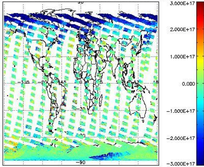
SCIOL2P_NADUV5SO2_vcd for 22FEB2011 00:00:00 to 23FEB2011 00:00:00
