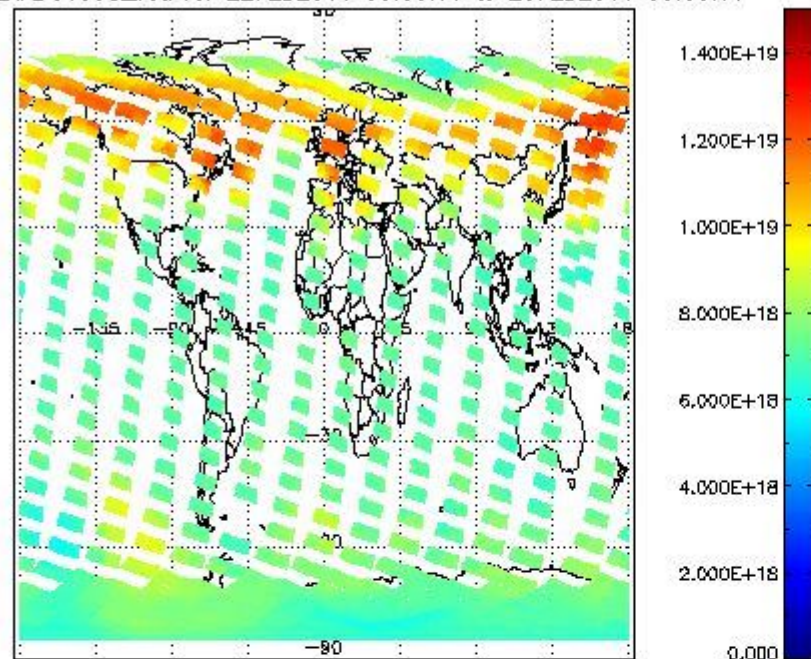
SCIOL2P_NADUV003_vcd for 22FEB2011 00:00:00 to 23FEB2011 00:00:00
