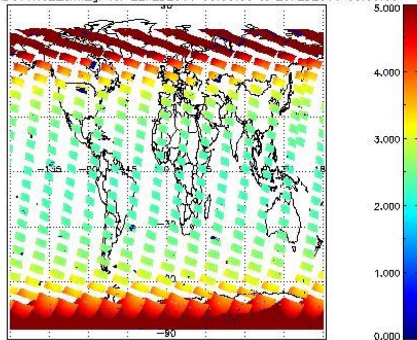
SCIOL2P_NADUV1N02_amf_gr for 22FEB2011 00:00:00 to 23FEB2011 00:00:00
