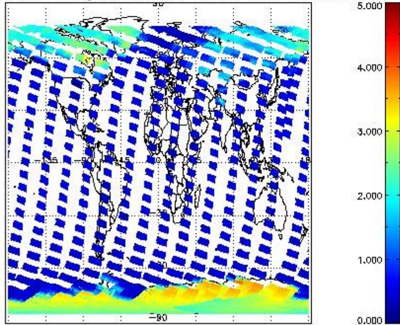
SCIOL2P_NADUV5SO2_amf_gr for 22FEB2011 00:00:00 to 23FEB2011 00:00:00
