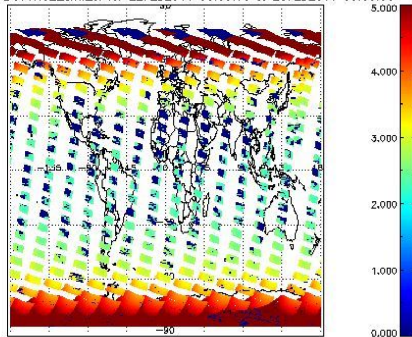
SCIOL2P_NADUV1N02_amf_cl for 22FEB2011 00:00:00 to 23FEB2011 00:00:00
