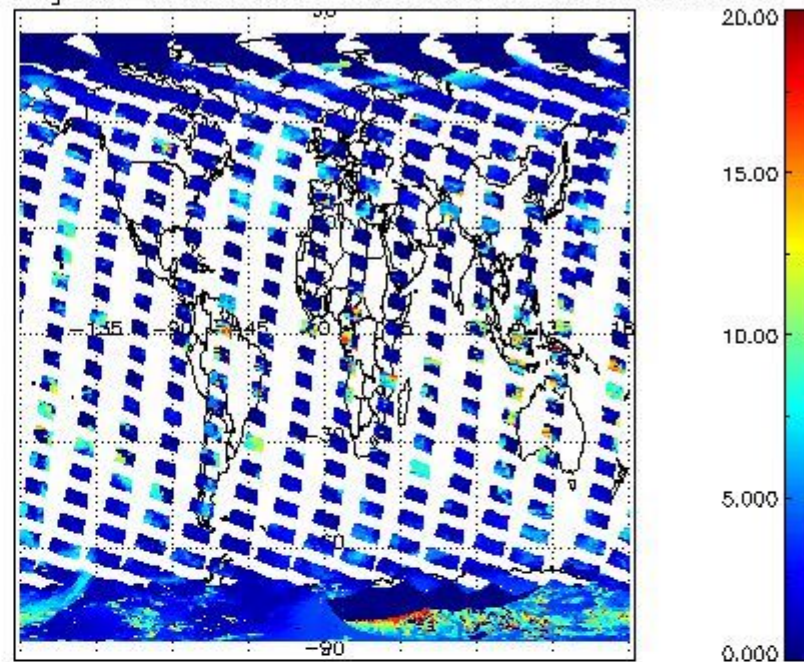
cL_top_height for 22FEB2011 00:00:00 to 23FEB2011 00:00:00
