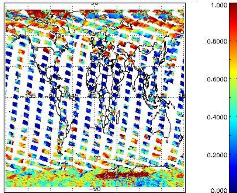
cL_frac for 22FEB2011 00:00:00 to 23FEB2011 00:00:00
