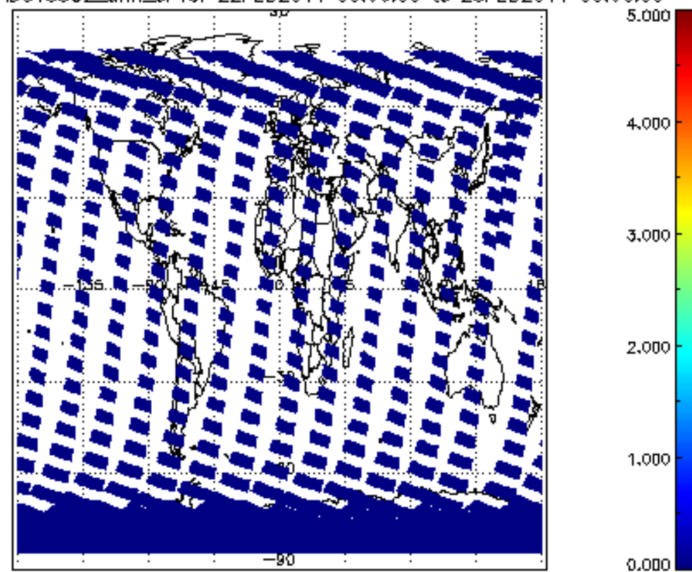
SCIOL2P_NADUV5S02_amf_cl for 22FEB2011 00:00:00 to 23FEB2011 00:00:00
