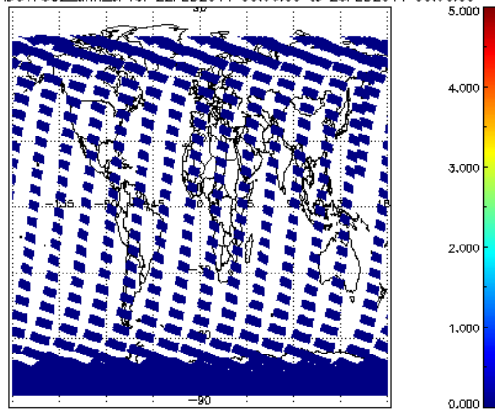
SCIOL2P_NADUV7S02_amf_cl for 22FEB2011 00:00:00 to 23FEB2011 00:00:00
