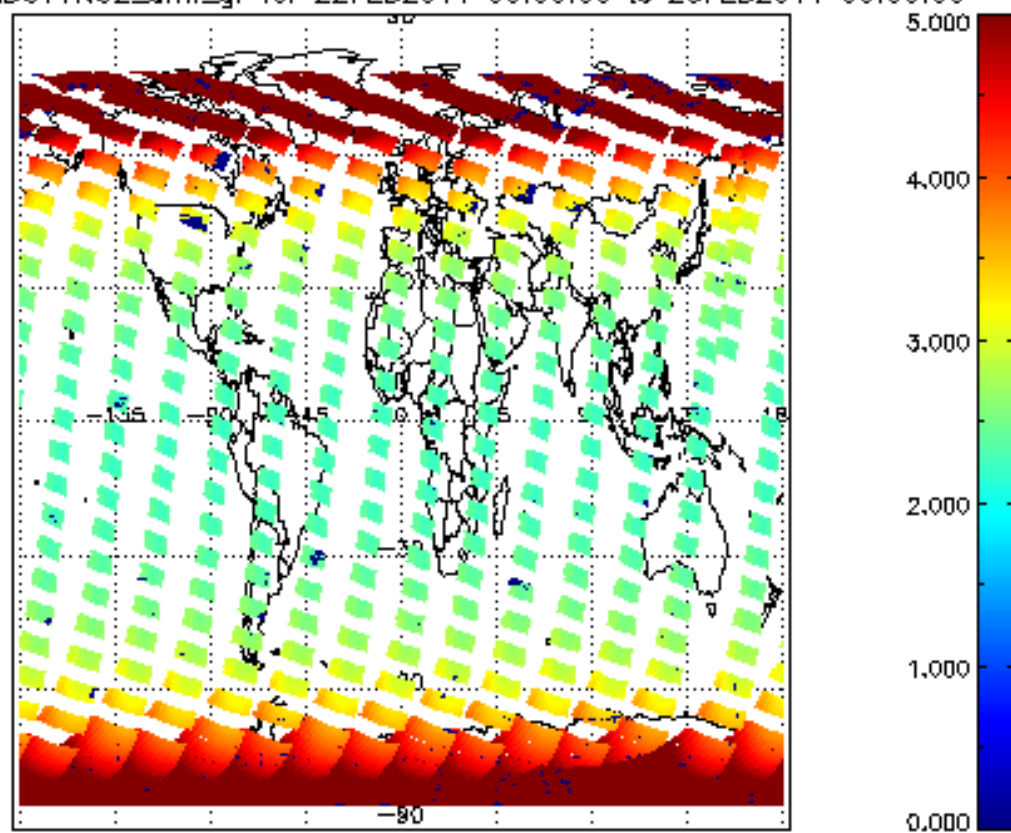
SCIOL2P_NADUV1N02_amf_gr for 22FEB2011 00:00:00 to 23FEB2011 00:00:00
