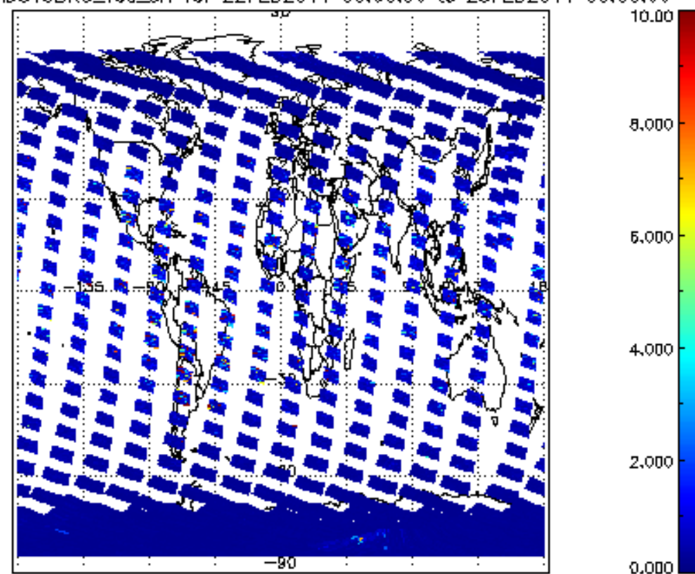
SCIOL2P_NADUV3BRO_vcd_err for 22FEB2011 00:00:00 to 23FEB2011 00:00:00
