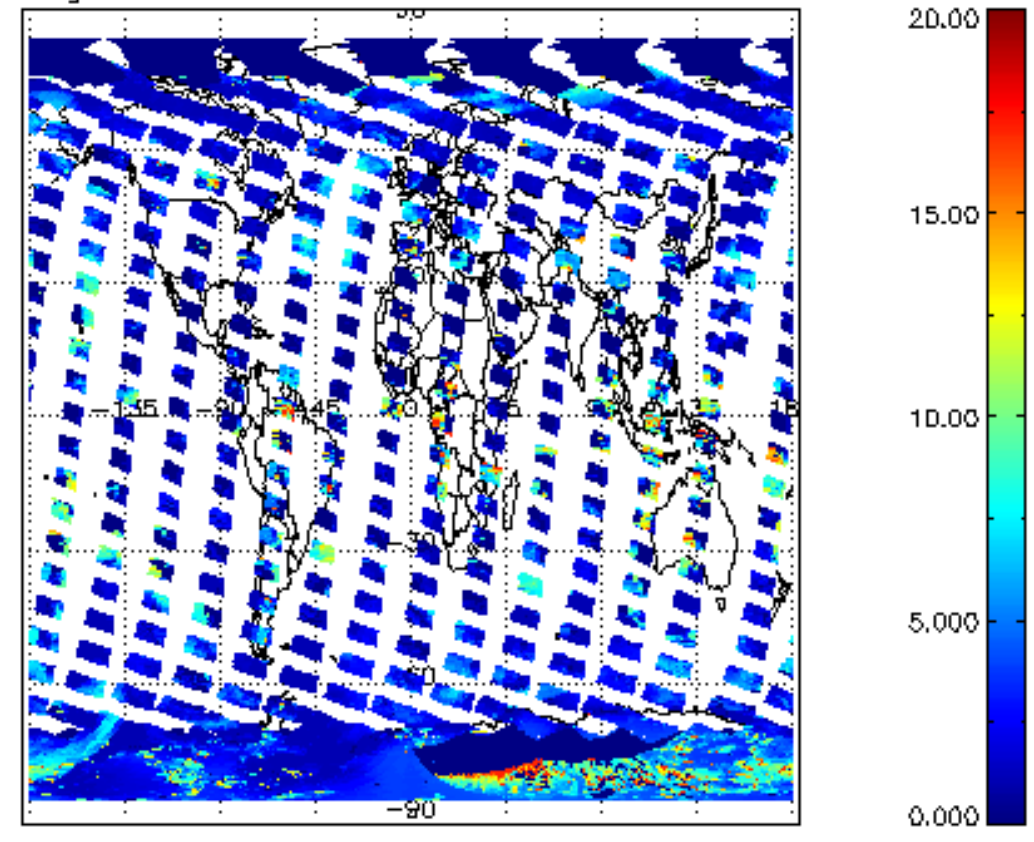
cl_top_height for 22FEB2011 00:00:00 to 23FEB2011 00:00:00
