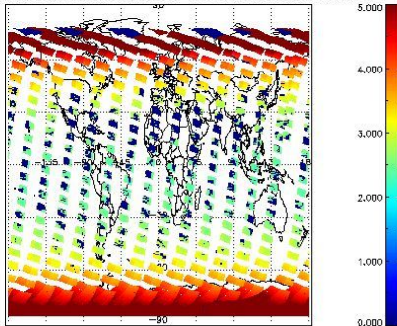
SCIOL2P_NADUV003_amf_cl for 22FEB2011 00:00:00 to 23FEB2011 00:00:00
