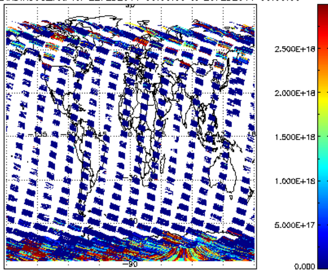
SCIOL2P_NADIR3CO_vcd for 22FEB2011 00:00:00 to 23FEB2011 00:00:00
