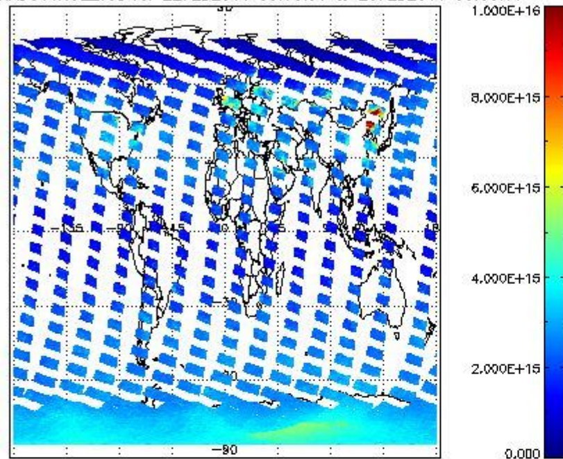
SCIOL2P_NADUV1N02_vcd for 22FEB2011 00:00:00 to 23FEB2011 00:00:00
