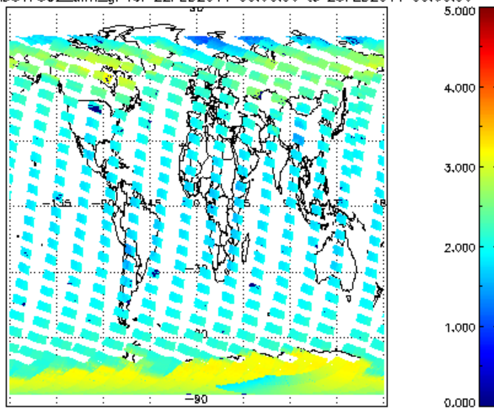
SCIOL2P_NADUV7S02_amf_gr for 22FEB2011 00:00:00 to 23FEB2011 00:00:00
