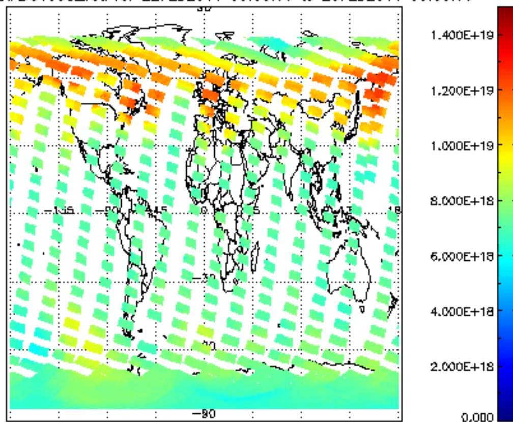
SCIOL2P_NADUV003_vcd for 22FEB2011 00:00:00 to 23FEB2011 00:00:00
