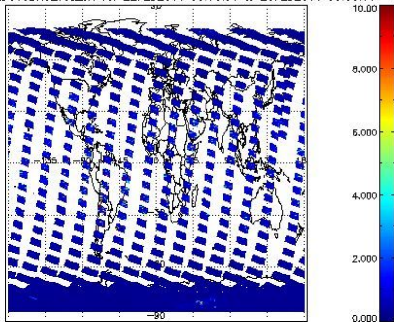
SCIOL2P_NADUV3BRO_vcd_err for 22FEB2011 00:00:00 to 23FEB2011 00:00:00
