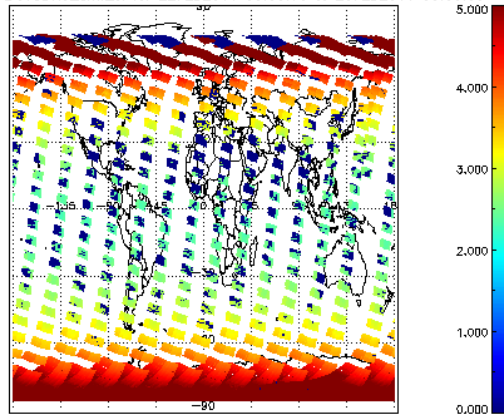
SCIOL2P_NADUV3BRO_amf_cl for 22FEB2011 00:00:00 to 23FEB2011 00:00:00
