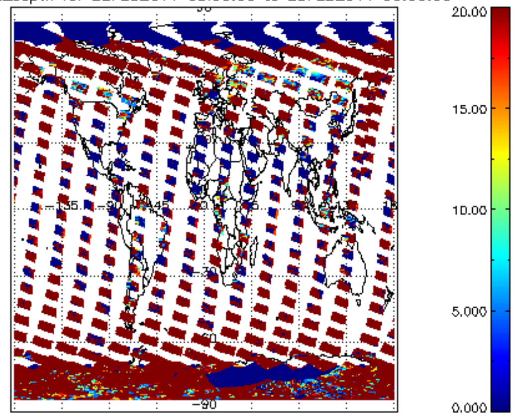
cl_opt_depth for 22FEB2011 00:00:00 to 23FEB2011 00:00:00
