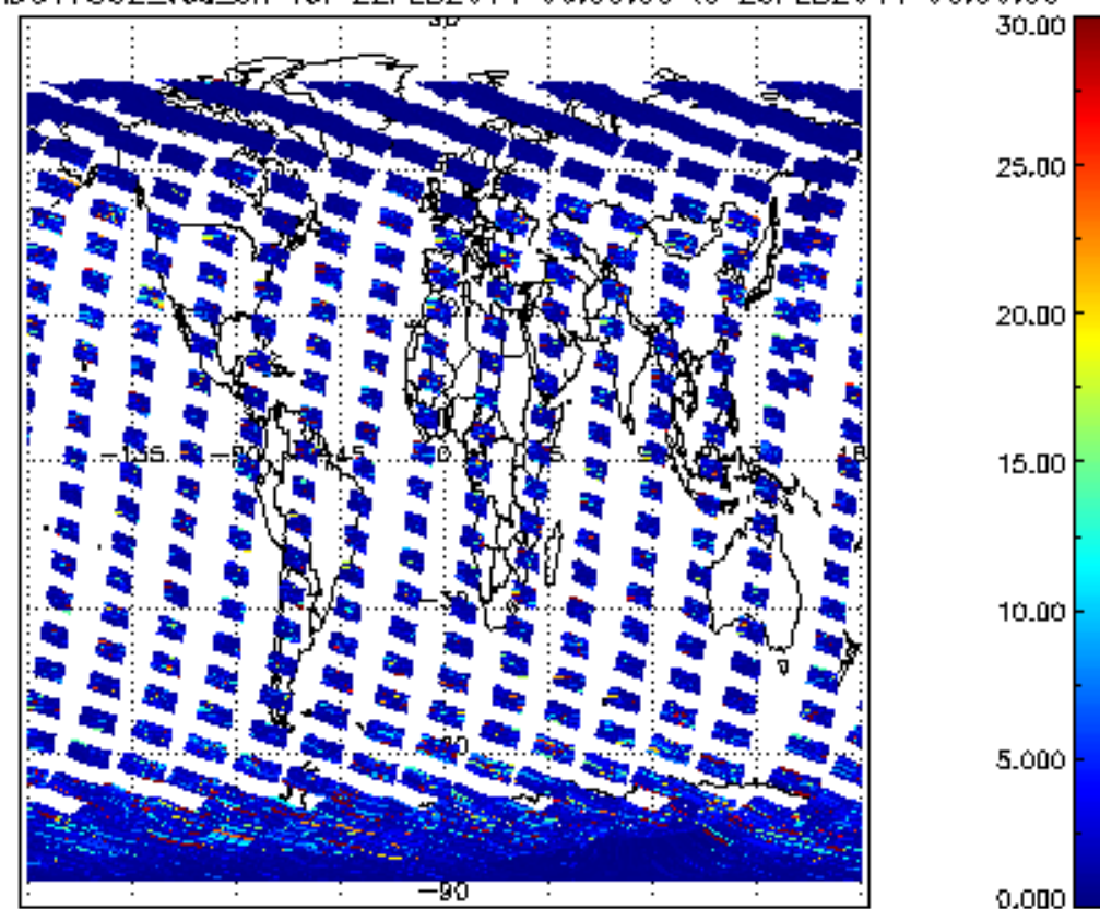
SCIOL2P_NADUV7S02_vcd_err for 22FEB2011 00:00:00 to 23FEB2011 00:00:00
