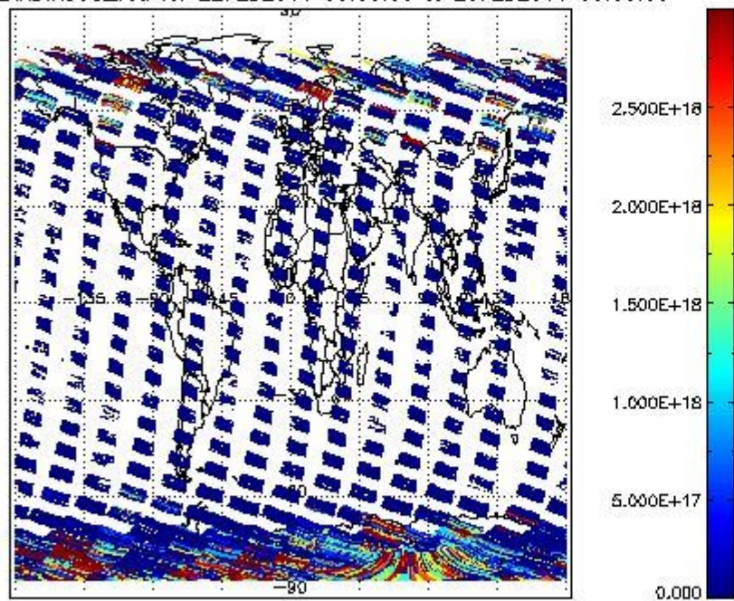
SCIO2P_NADIR3CO_vcd for 22FEB2011 00:00:00 to 23FEB2011 00:00:00
