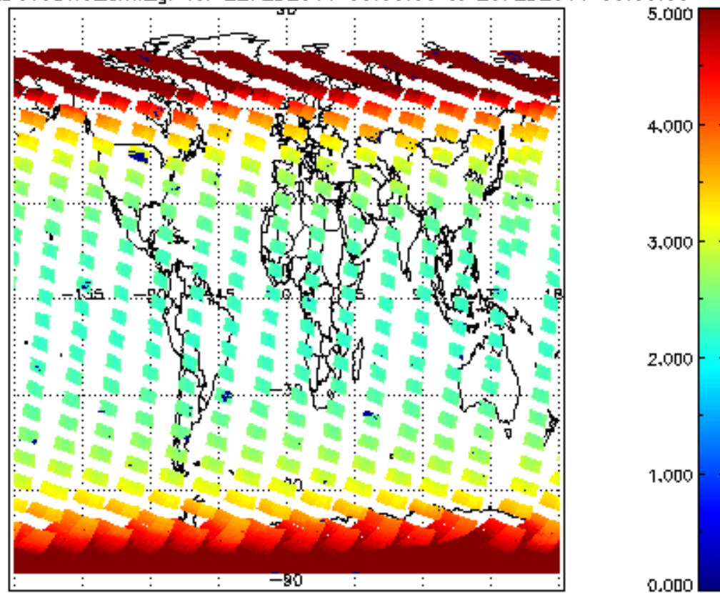
SCIOL2P_NADUV3BRO_amf_gr for 22FEB2011 00:00:00 to 23FEB2011 00:00:00
