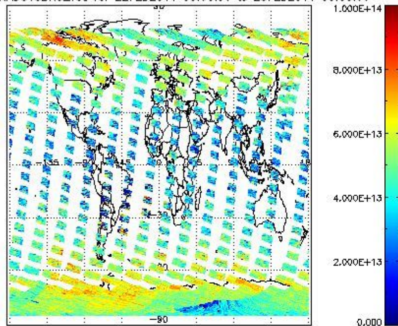
SCIOL2P_NADUV3BRO_vcd for 22FEB2011 00:00:00 to 23FEB2011 00:00:00
