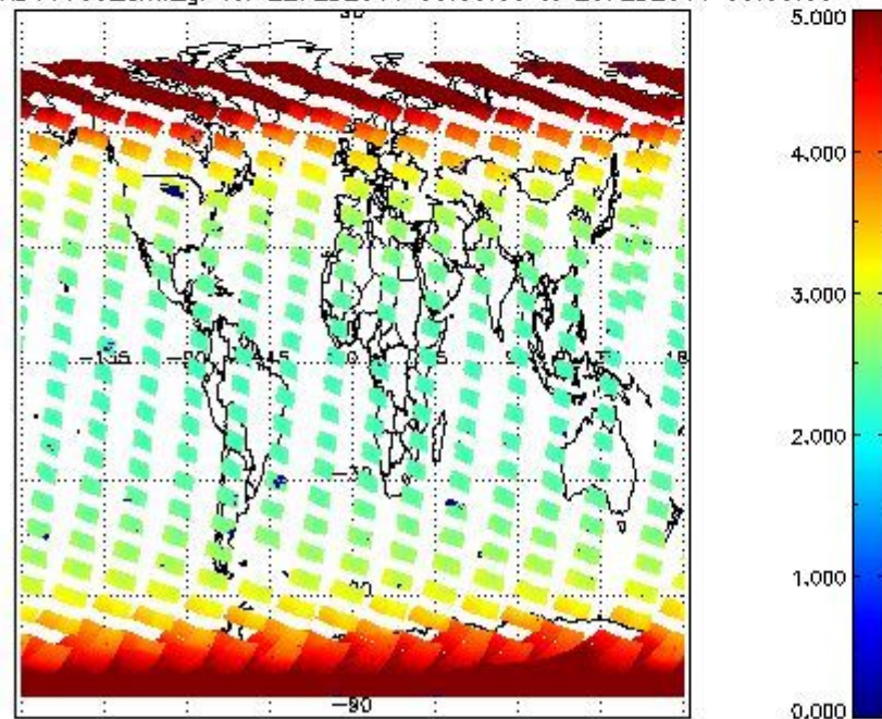
SCIOL2P_NADUV003_amf_gr for 22FEB2011 00:00:00 to 23FEB2011 00:00:00
