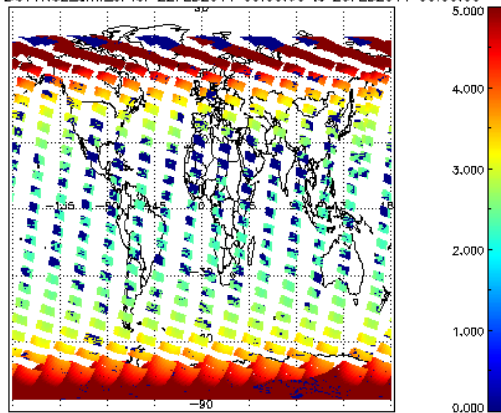
SCIOL2P_NADUV1N02_amf_cl for 22FEB2011 00:00:00 to 23FEB2011 00:00:00
