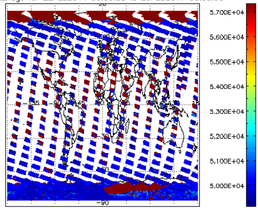
cloud_flags for 22FEB2011 00:00:00 to 23FEB2011 00:00:00
