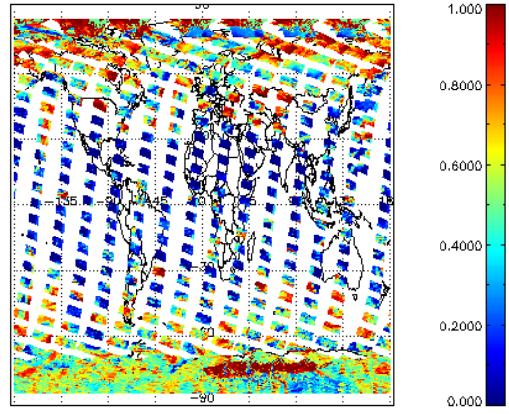
cl_frac for 22FEB2011 00:00:00 to 23FEB2011 00:00:00
