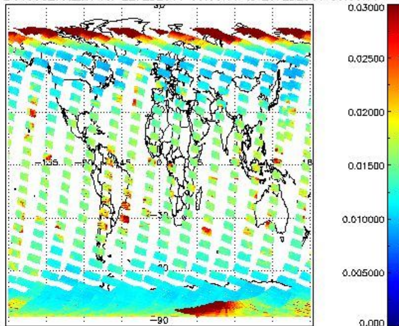
SCIOL2P_NADUV003_vcd_err for 22FEB2011 00:00:00 to 23FEB2011 00:00:00
