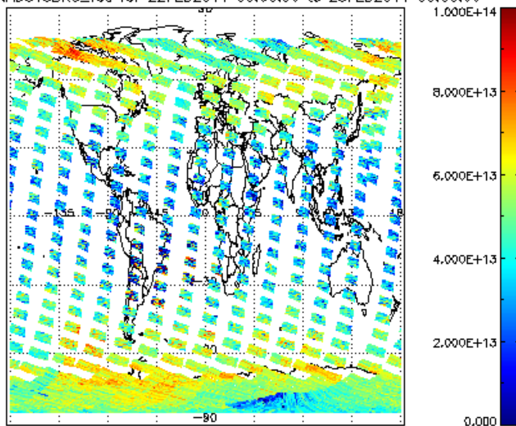
SCIOL2P_NADUV3BRO_vcd for 22FEB2011 00:00:00 to 23FEB2011 00:00:00
