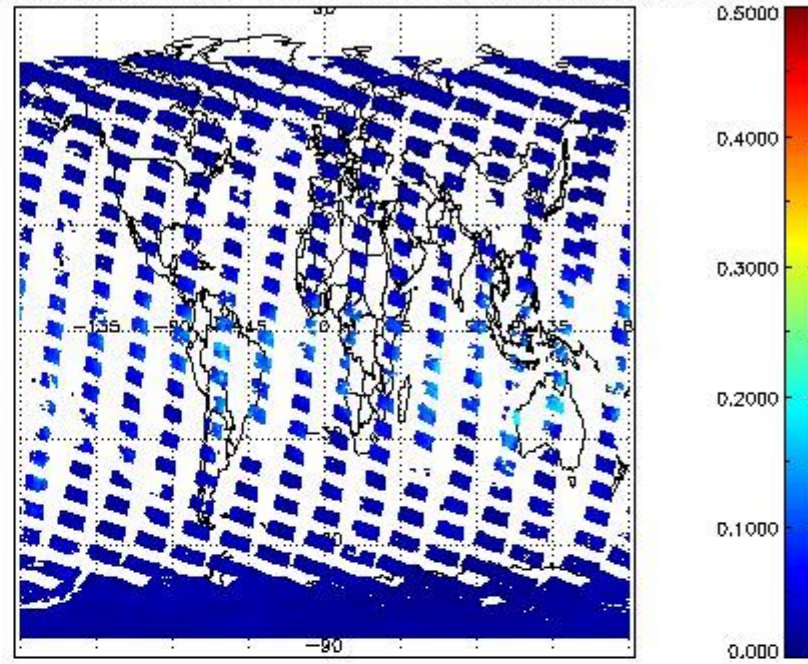
SCIOL2P_NADUV8H2O_vcd_err for 22FEB2011 00:00:00 to 23FEB2011 00:00:00
