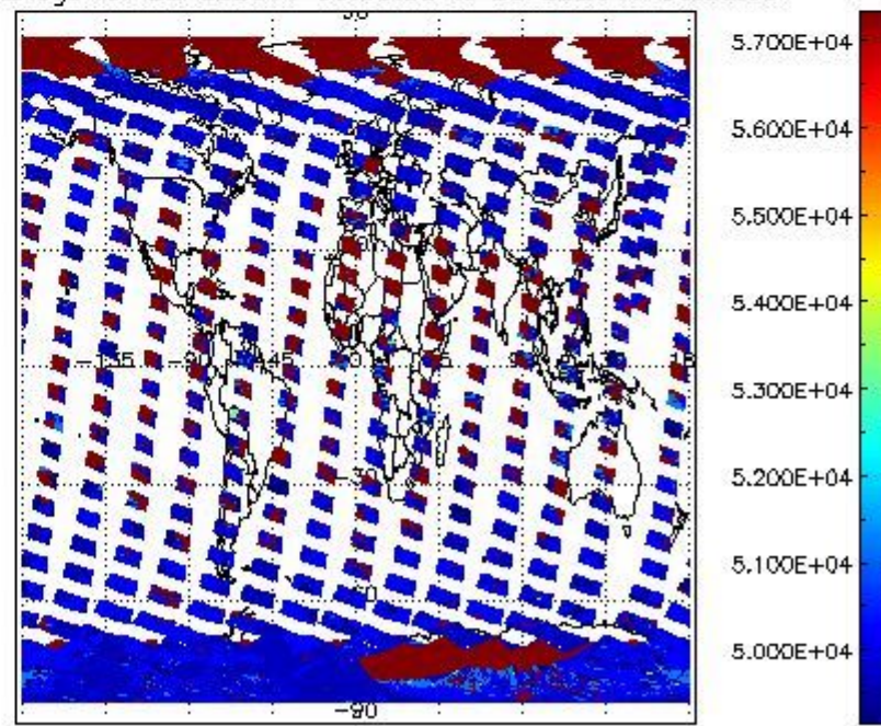
cloud_flags for 22FEB2011 00:00:00 to 23FEB2011 00:00:00
