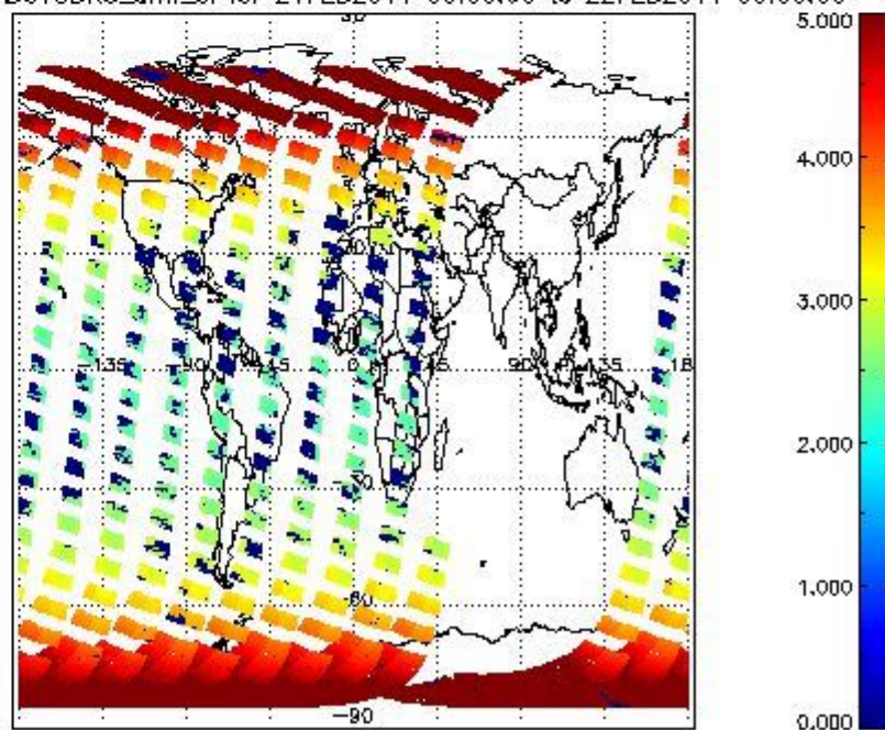
SCIOL2P_NADUV3BRO_amf_cl for 21FEB2011 00:00:00 to 22FEB2011 00:00:00
