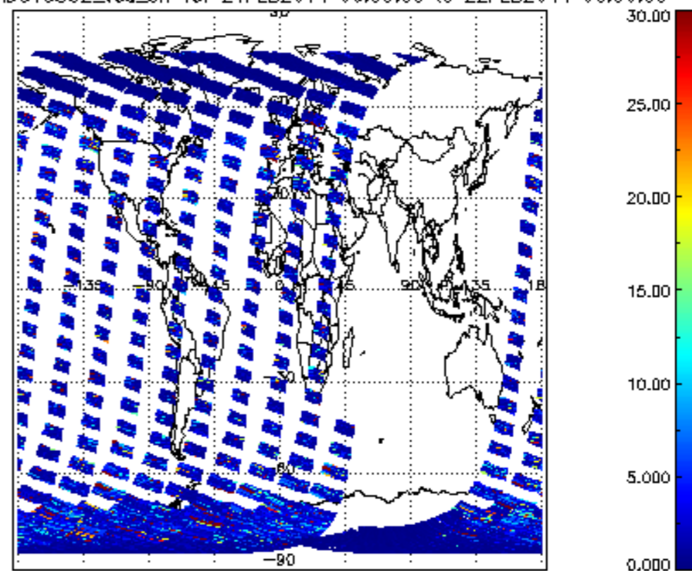
SCIOL2P_NADUV5S02_vcd_err for 21FEB2011 00:00:00 to 22FEB2011 00:00:00
