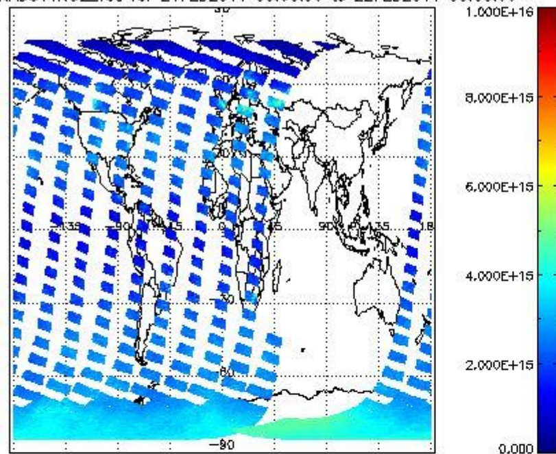
SCIOL2P_NADUV1N02_vcd for 21FEB2011 00:00:00 to 22FEB2011 00:00:00
