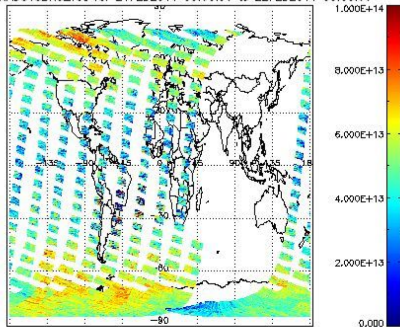
SCIOL2P_NADUV3BRO_vcd for 21FEB2011 00:00:00 to 22FEB2011 00:00:00
