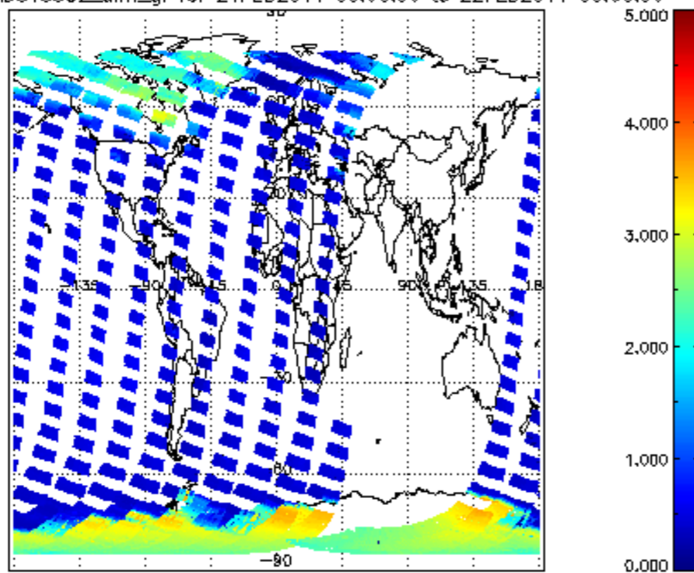
SCIOL2P_NADUV5S02_amf_gr for 21FEB2011 00:00:00 to 22FEB2011 00:00:00
