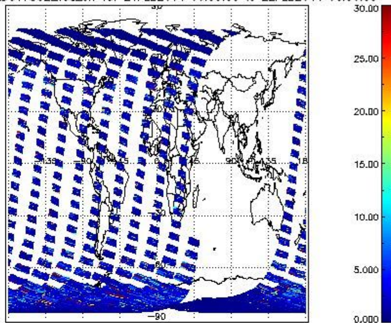
SCIOL2P_NADUV7S02_vcd_err for 21FEB2011 00:00:00 to 22FEB2011 00:00:00
