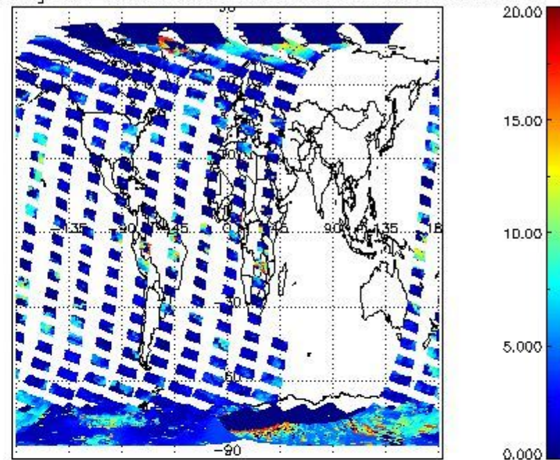
cL_top_height for 21FEB2011 00:00:00 to 22FEB2011 00:00:00
