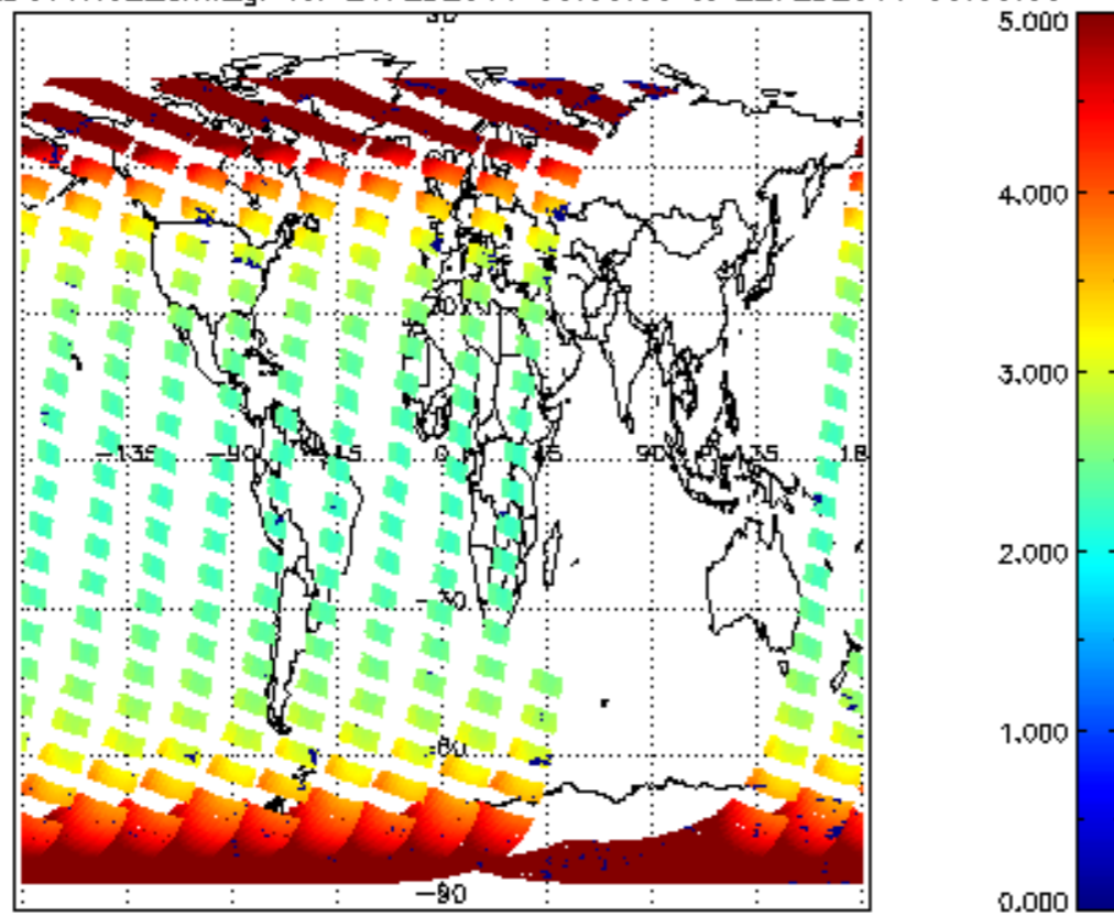
SCIOL2P_NADUV1N02_amf_gr for 21FEB2011 00:00:00 to 22FEB2011 00:00:00
