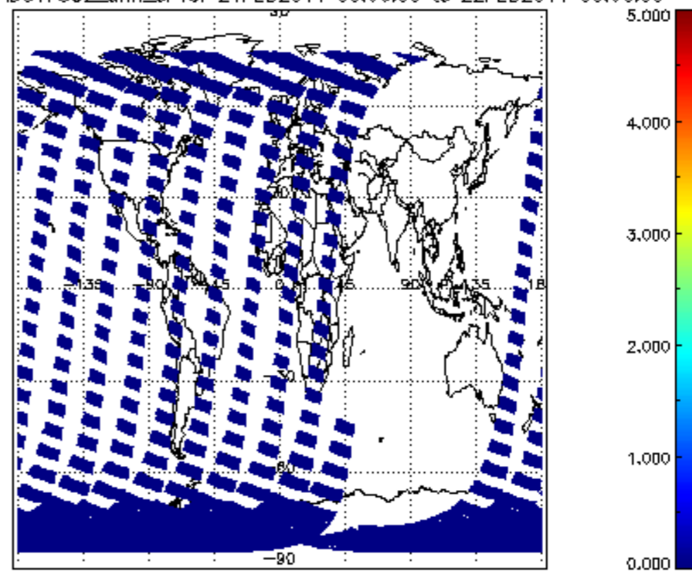
SCIOL2P_NADUV7S02_amf_cl for 21FEB2011 00:00:00 to 22FEB2011 00:00:00
