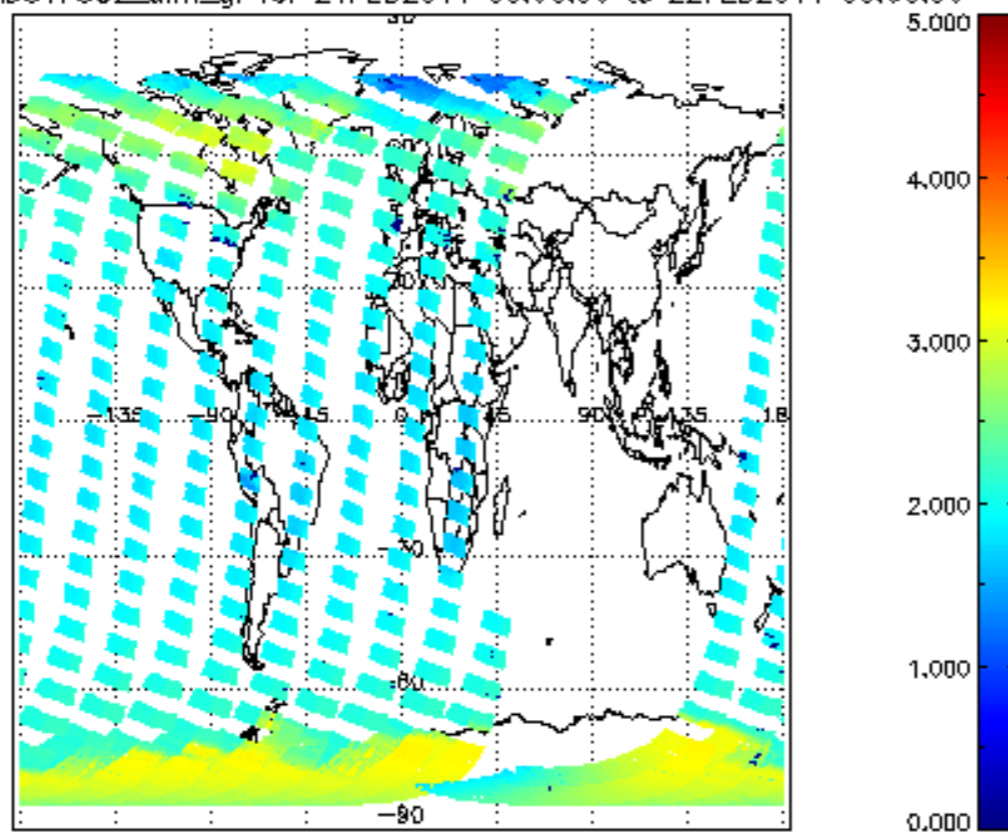
SCIOL2P_NADUV7S02_amf_gr for 21FEB2011 00:00:00 to 22FEB2011 00:00:00
