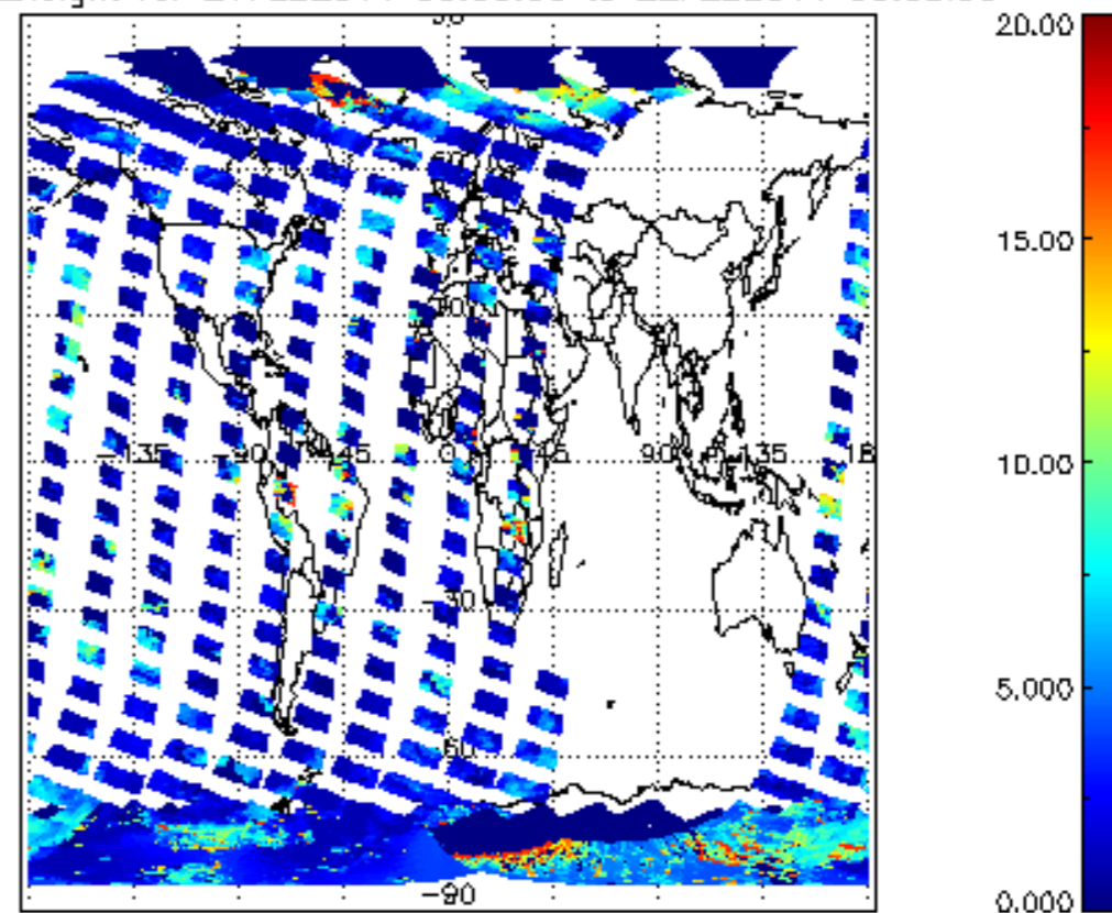
cI_top_height for 21FEB2011 00:00:00 to 22FEB2011 00:00:00
