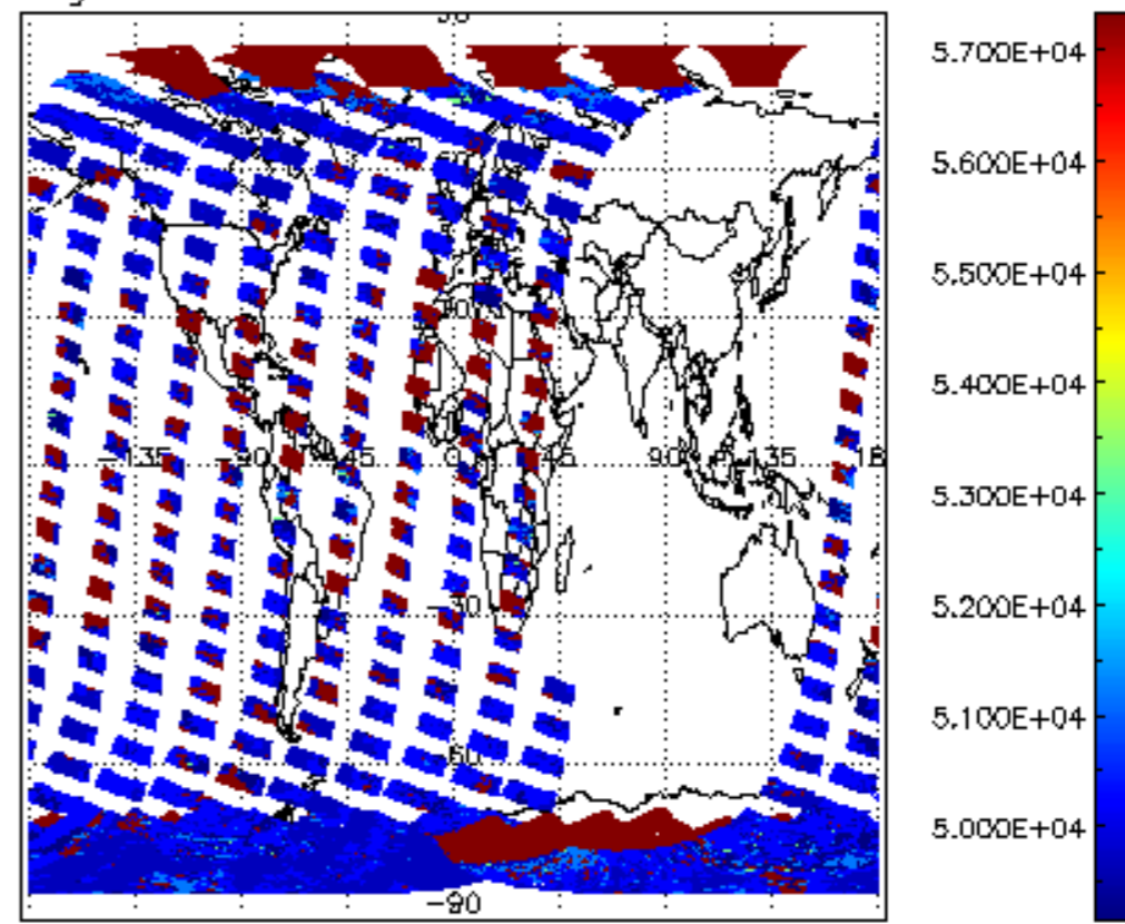
cloud_flags for 21FEB2011 00:00:00 to 22FEB2011 00:00:00
