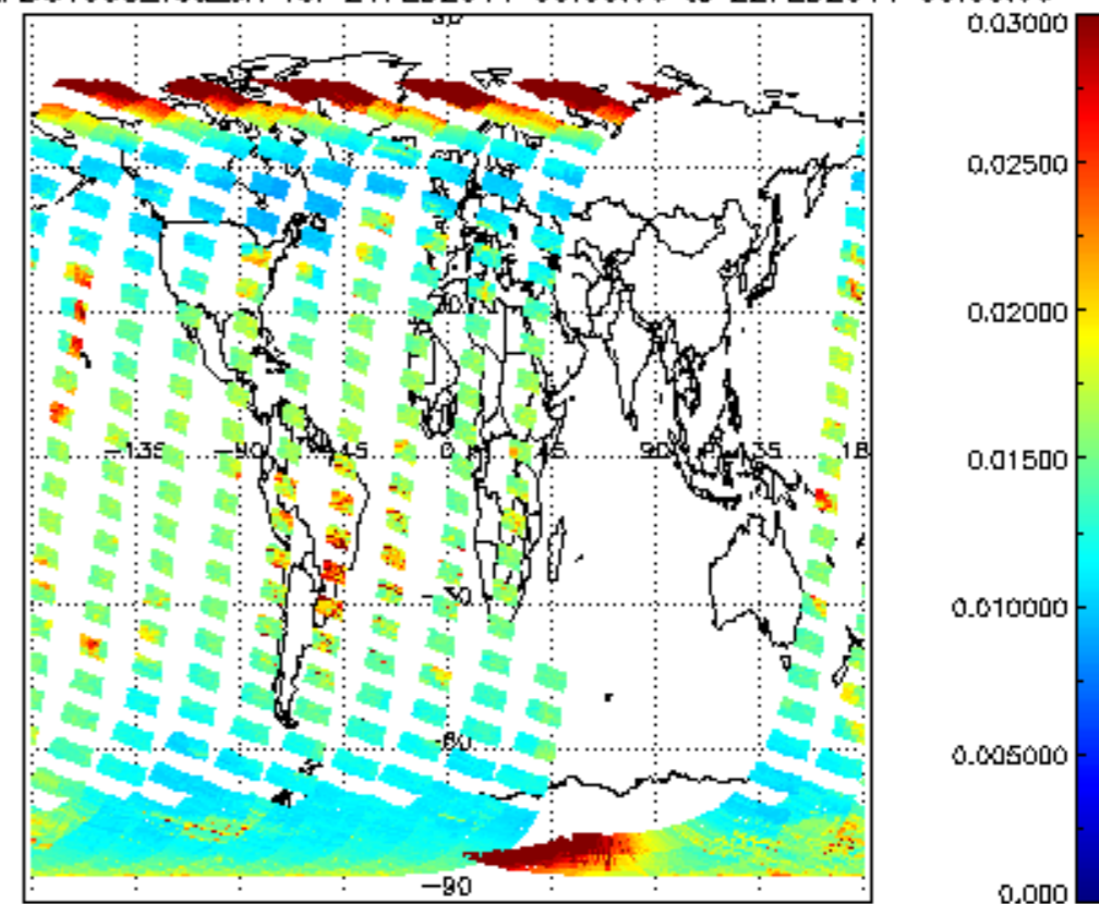
SCIOL2P_NADUV003_vcd_err for 21FEB2011 00:00:00 to 22FEB2011 00:00:00
