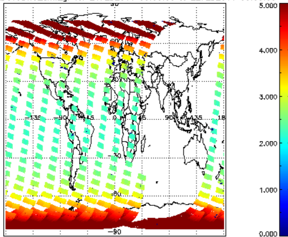
SCIOL2P_NADUV3BRO_amf_gr for 21FEB2011 00:00:00 to 22FEB2011 00:00:00
