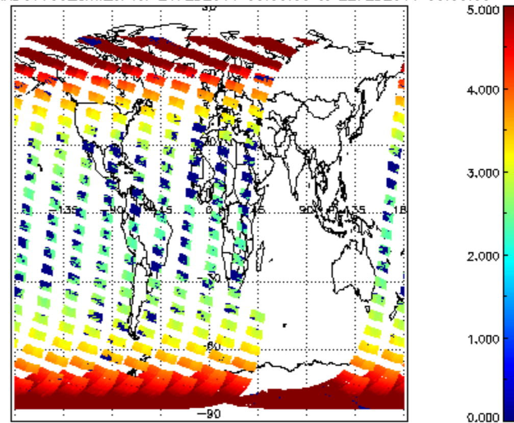
SCIOL2P_NADUV003_amf_cl for 21FEB2011 00:00:00 to 22FEB2011 00:00:00
