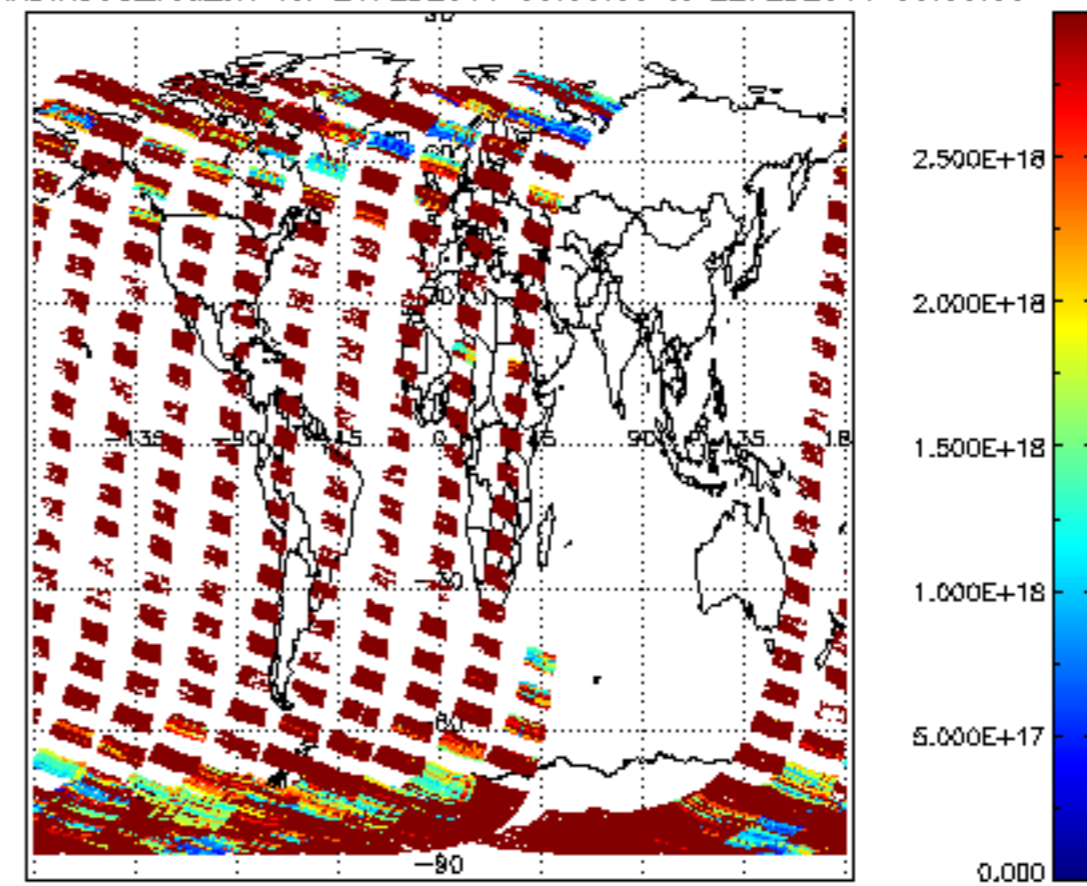
SCIOL2P_NADIR3CO_vcd_err for 21FEB2011 00:00:00 to 22FEB2011 00:00:00
