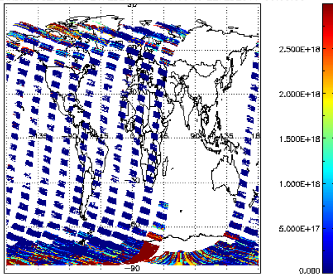
SCIOL2P_NADIR3CO_vcd for 21FEB2011 00:00:00 to 22FEB2011 00:00:00
