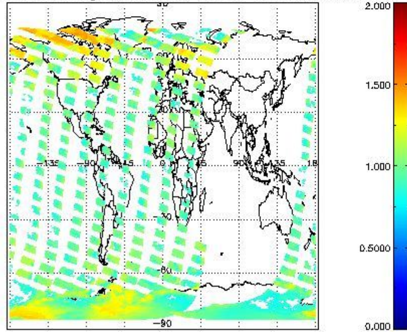
SCIOL2P_NADUV8H2O_amf_gr for 21FEB2011 00:00:00 to 22FEB2011 00:00:00
