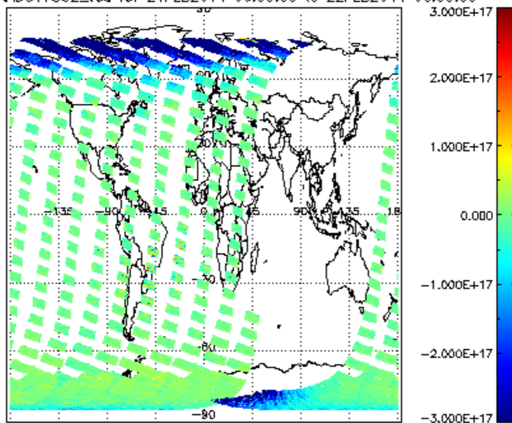
SCIOL2P_NADUV7S02_vcd for 21FEB2011 00:00:00 to 22FEB2011 00:00:00
