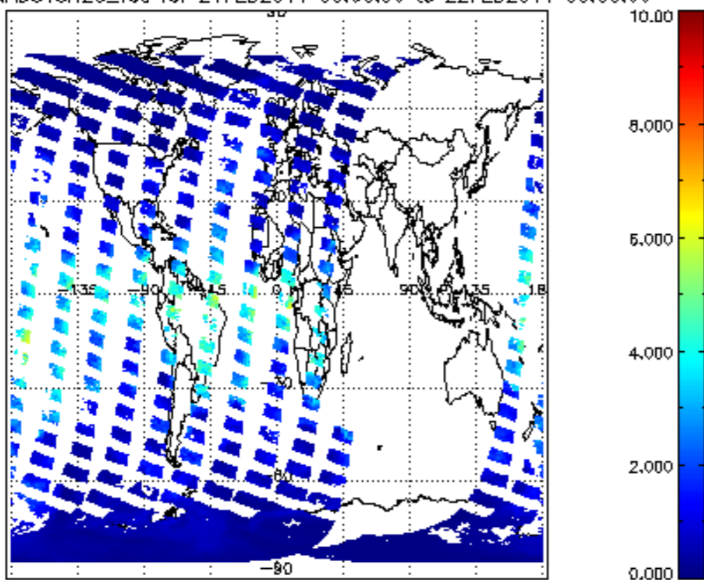
SCIOL2P_NADUV8H2O_vcd for 21FEB2011 00:00:00 to 22FEB2011 00:00:00
