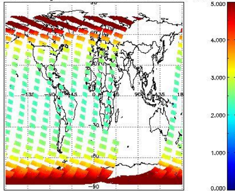
SCIOL2P_NADUV003_amf_gr for 21FEB2011 00:00:00 to 22FEB2011 00:00:00
