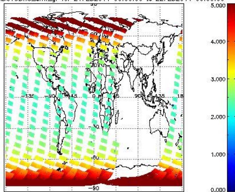
SCIOL2P_NADUV3BRO_amf_gr for 21FEB2011 00:00:00 to 22FEB2011 00:00:00
