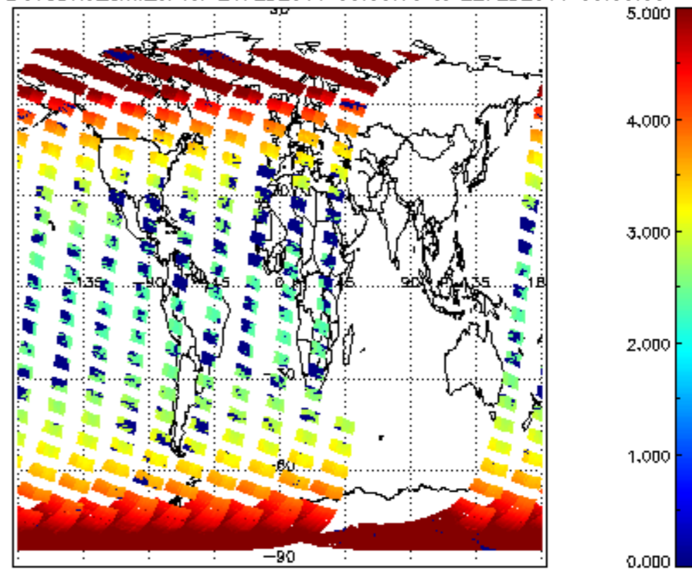
SCIOL2P_NADUV3BRO_amf_cl for 21FEB2011 00:00:00 to 22FEB2011 00:00:00
