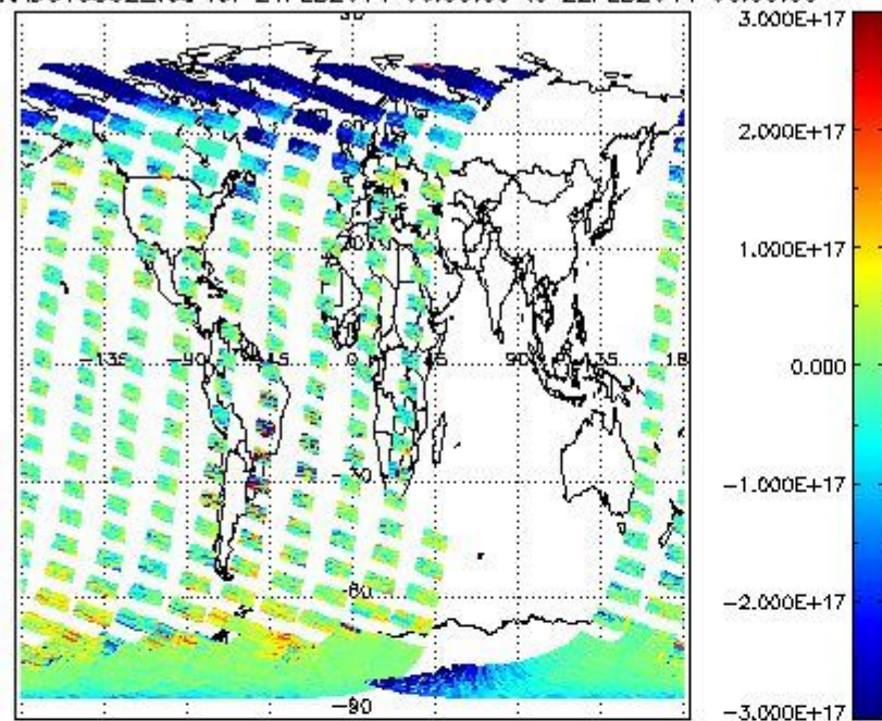
SCIOL2P_NADUV5S02_vcd for 21FEB2011 00:00:00 to 22FEB2011 00:00:00
