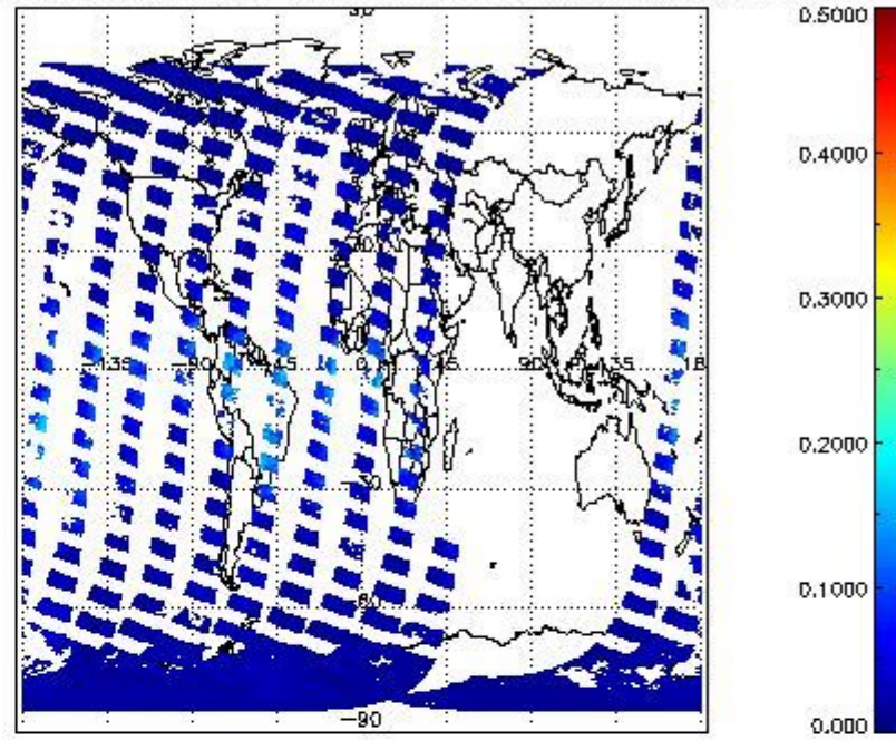
SCIOL2P_NADUV8H2O_vcd_err for 21FEB2011 00:00:00 to 22FEB2011 00:00:00
