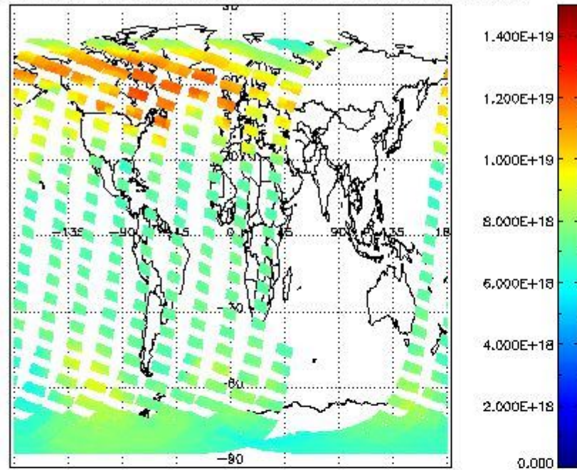
SCIOL2P_NADUV003_vcd for 21FEB2011 00:00:00 to 22FEB2011 00:00:00
