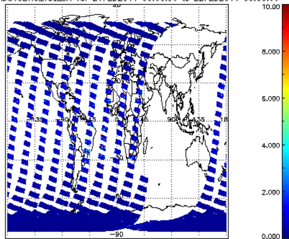
SCIOL2P_NADUV3BRO_vcd_err for 21FEB2011 00:00:00 to 22FEB2011 00:00:00
