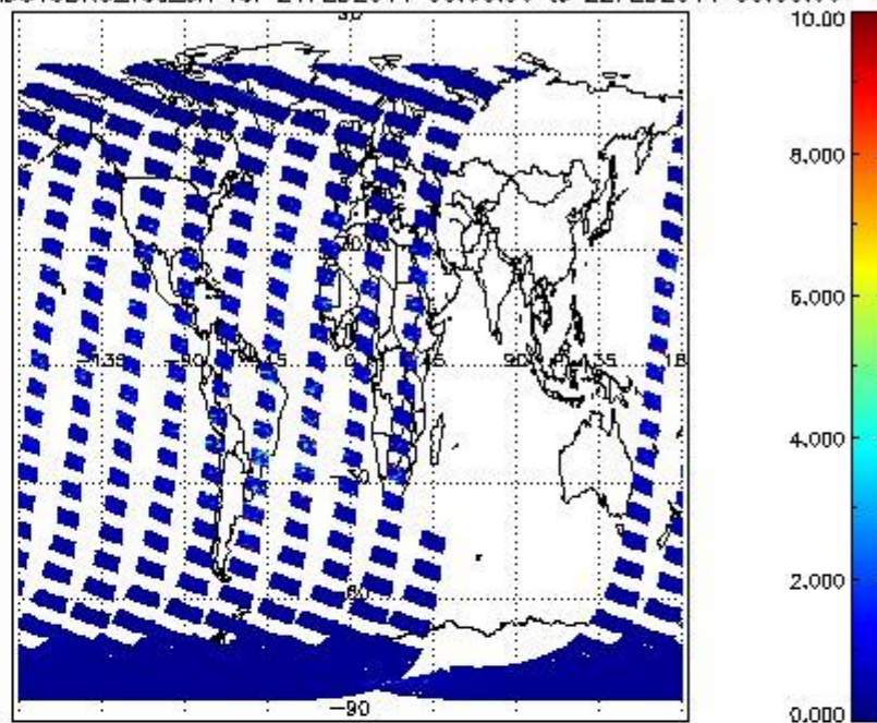
SCIOL2P_NADUV3BRO_vcd_err for 21FEB2011 00:00:00 to 22FEB2011 00:00:00
