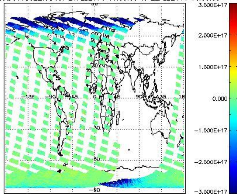
SCIOL2P_NADUV7S02_vcd for 21FEB2011 00:00:00 to 22FEB2011 00:00:00
