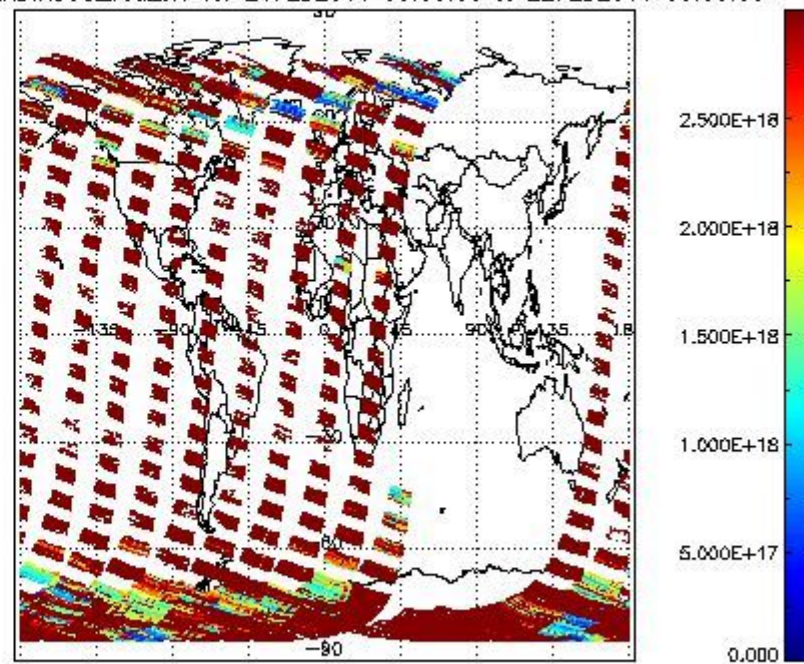
SCIDL2P_NADIR3CO_vcd_err for 21FEB2011 00:00:00 to 22FEB2011 00:00:00
