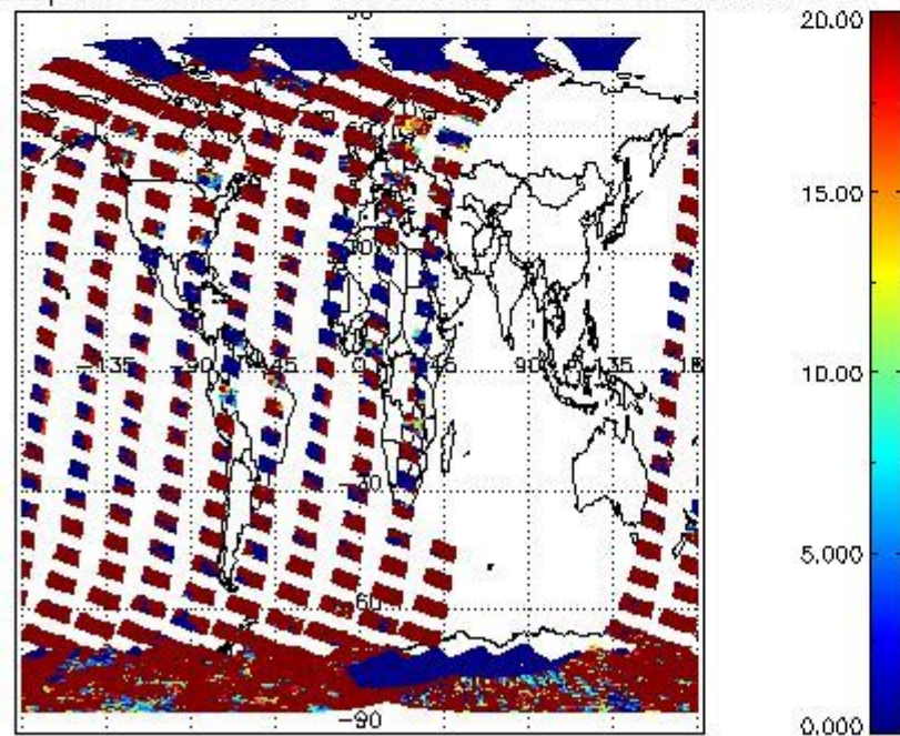
cL_opt_depth for 21FEB2011 00:00:00 to 22FEB2011 00:00:00
