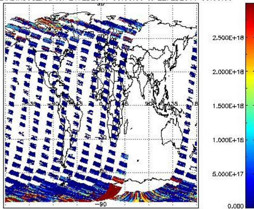
SCIDL2P_NADIR3CO_vcd for 21FEB2011 00:00:00 to 22FEB2011 00:00:00
