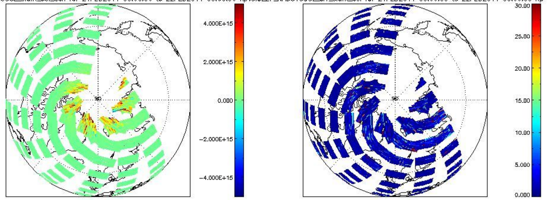
CIOL2P_NADUV6OCLslant_col_den for 21FEB2011 00:00:00 to 22FEB2011 00:00:00 np; CIOL2P_NADUV6OCLerr_slant_col for 21FEB2011 00:00:00 to 22FEB2011 00:00:00 np
