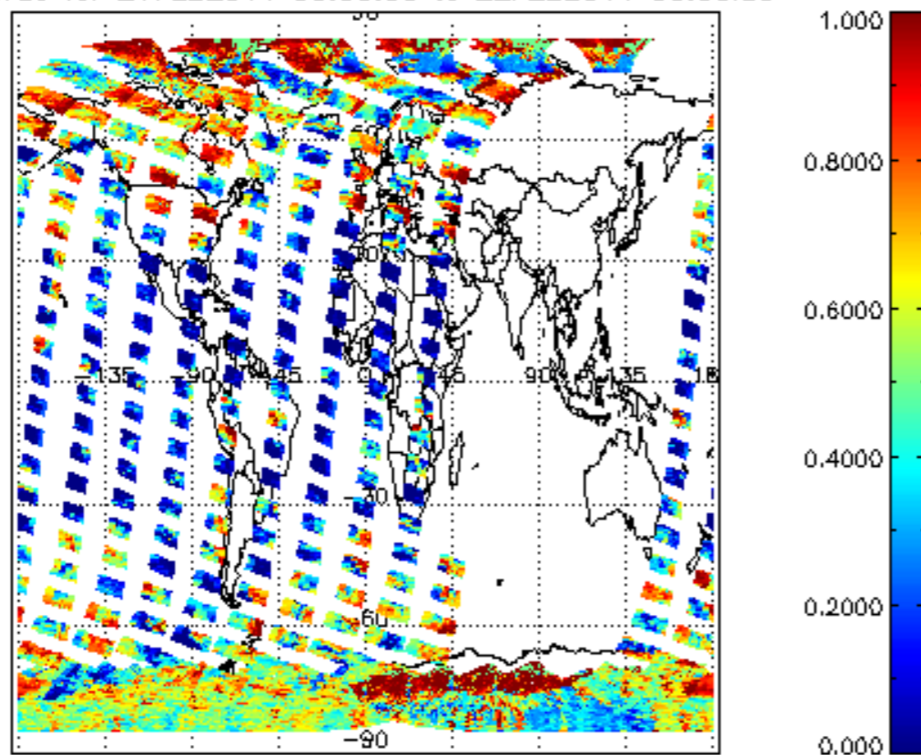
cI_frac for 21FEB2011 00:00:00 to 22FEB2011 00:00:00
