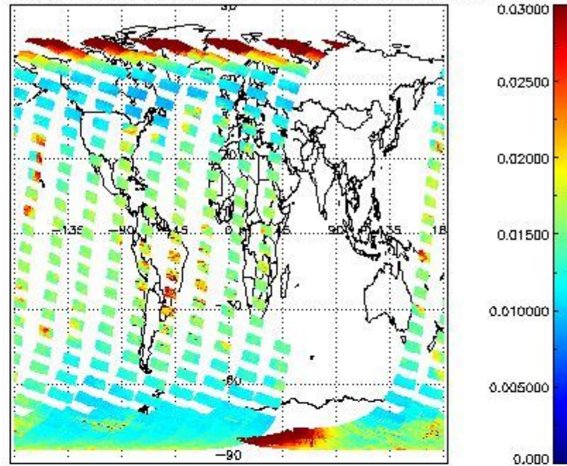
SCIOL2P_NADUV003_vcd_err for 21FEB2011 00:00:00 to 22FEB2011 00:00:00
