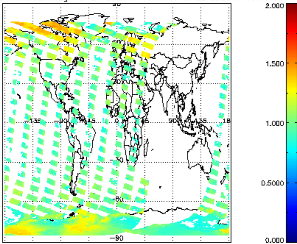
SCIOL2P_NADUV8H2O_amf_gr for 21FEB2011 00:00:00 to 22FEB2011 00:00:00
