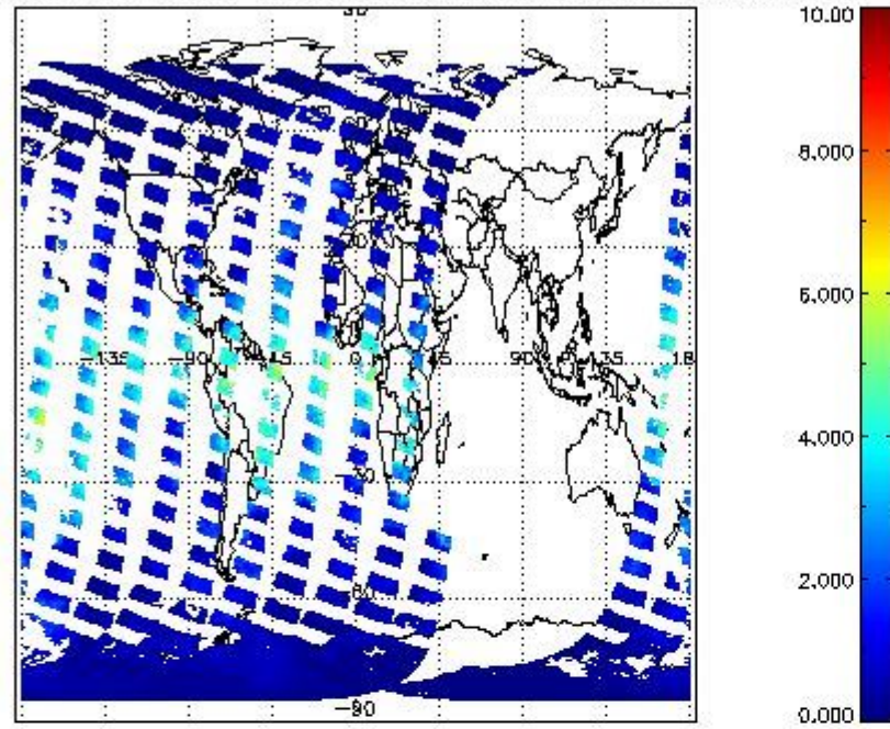
SCIOL2P_NADUV8H2O_vcd for 21FEB2011 00:00:00 to 22FEB2011 00:00:00
