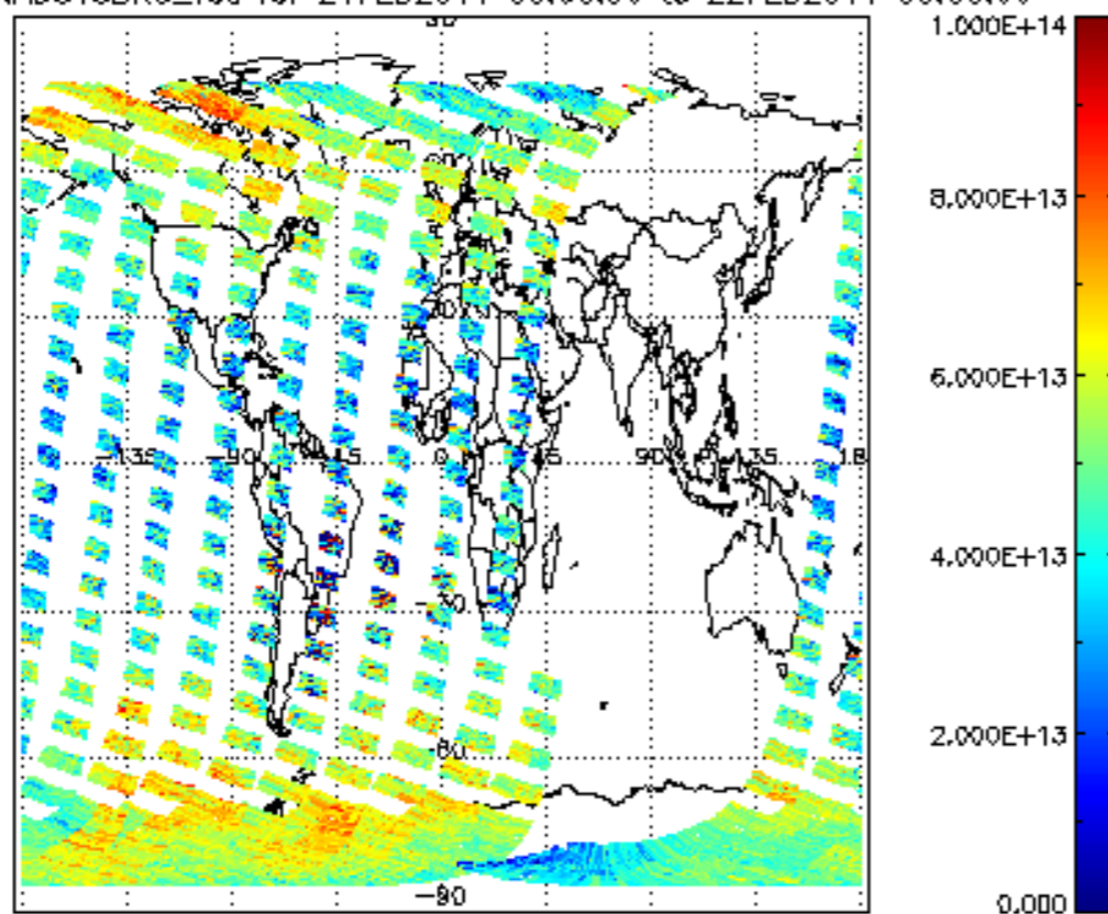
SCIOL2P_NADUV3BRO_vcd for 21FEB2011 00:00:00 to 22FEB2011 00:00:00
