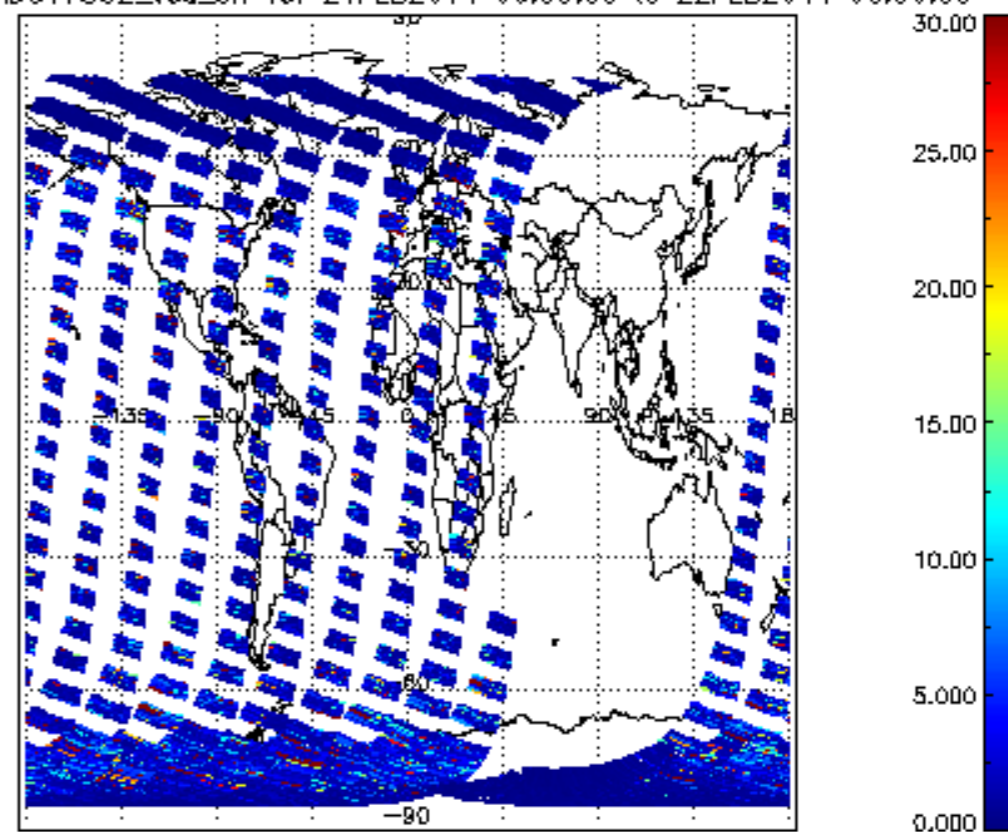
SCIOL2P_NADUV7S02_vcd_err for 21FEB2011 00:00:00 to 22FEB2011 00:00:00
