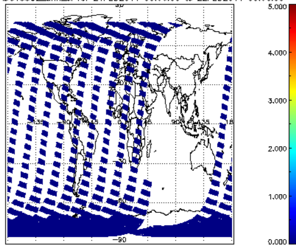
SCIOL2P_NADUV5S02_amf_cl for 21FEB2011 00:00:00 to 22FEB2011 00:00:00
