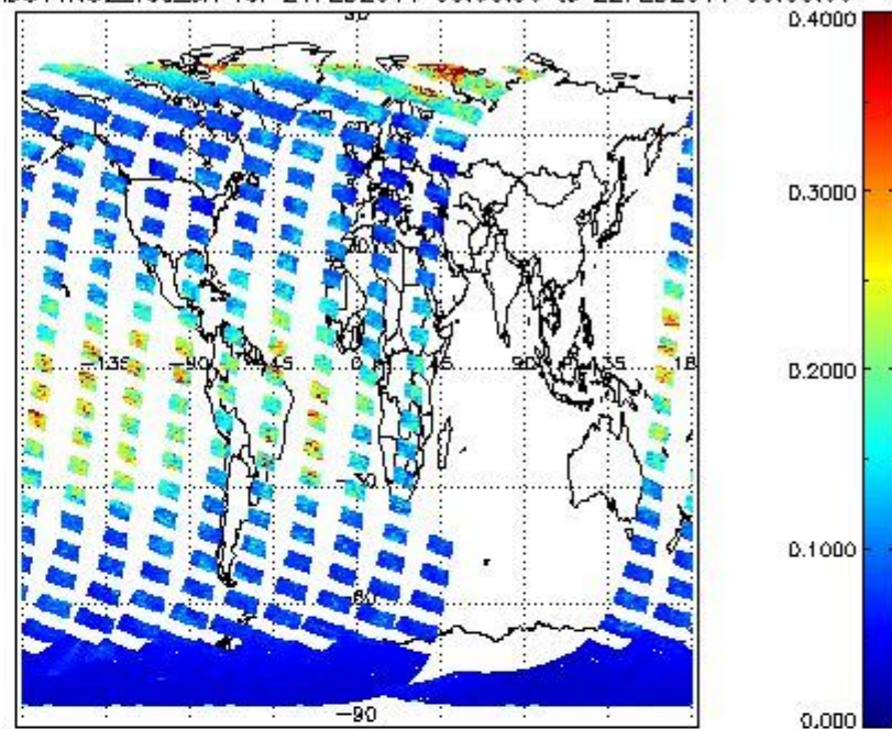
SCIOL2P_NADUV1N02_vcd_err for 21FEB2011 00:00:00 to 22FEB2011 00:00:00
