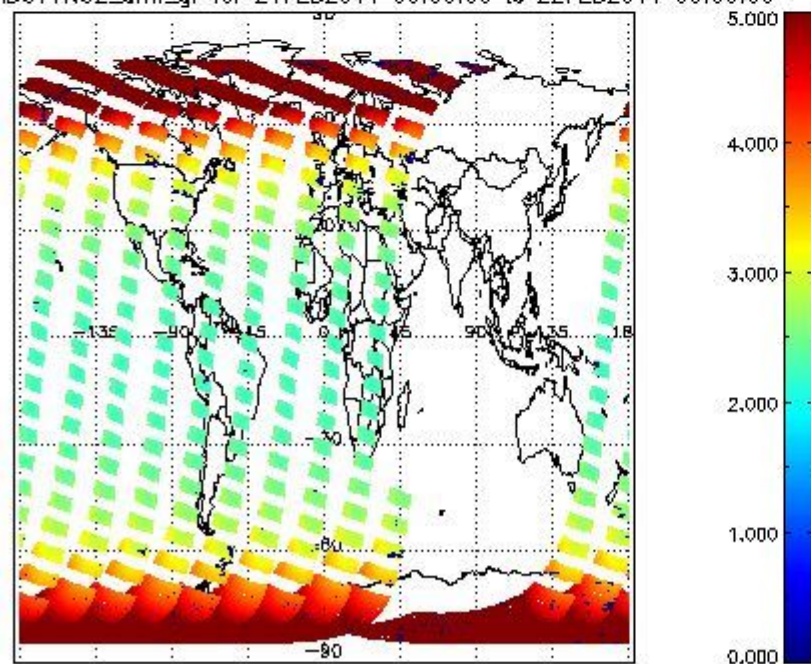
SCIOL2P_NADUV1N02_amf_gr for 21FEB2011 00:00:00 to 22FEB2011 00:00:00
