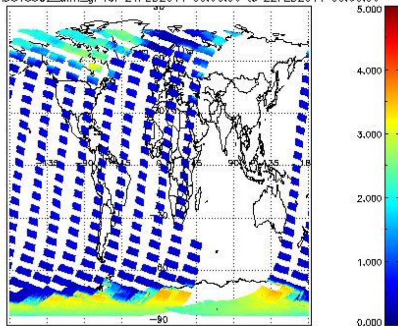
SCIOL2P_NADUV5S02_amf_gr for 21FEB2011 00:00:00 to 22FEB2011 00:00:00
