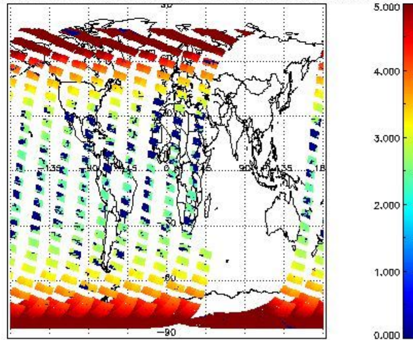
SCIOL2P_NADUV003_amf_cl for 21FEB2011 00:00:00 to 22FEB2011 00:00:00
