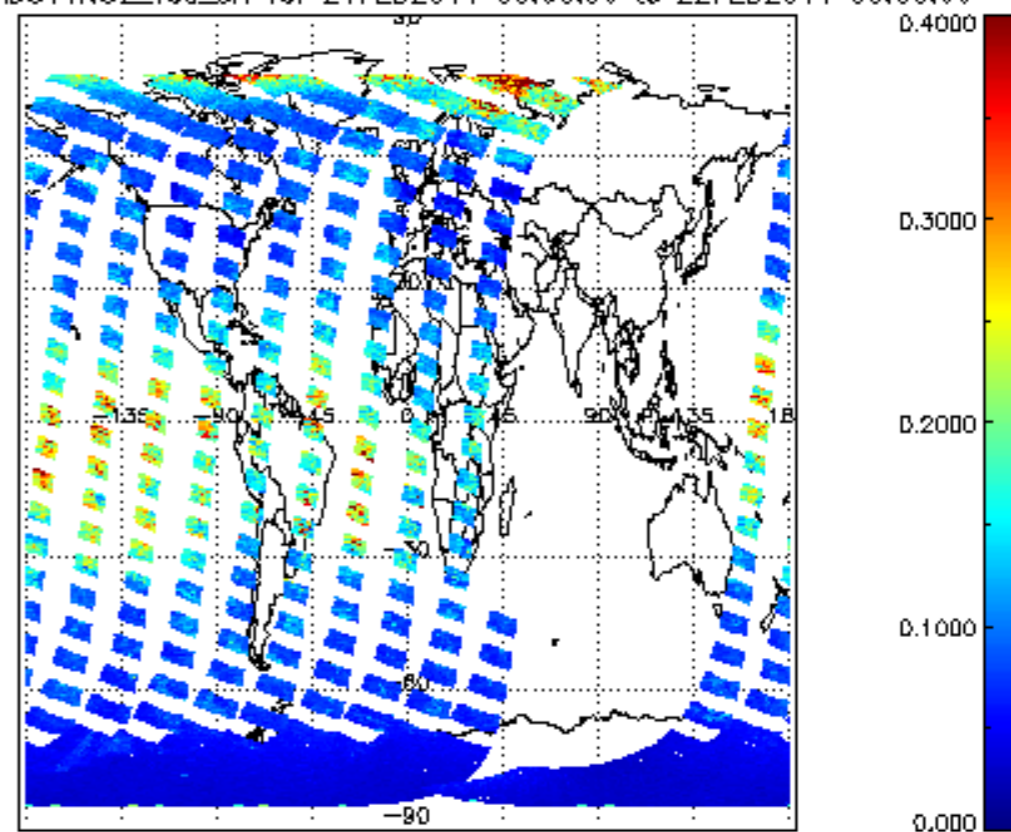
SCIOL2P_NADUV1N02_vcd_err for 21FEB2011 00:00:00 to 22FEB2011 00:00:00
