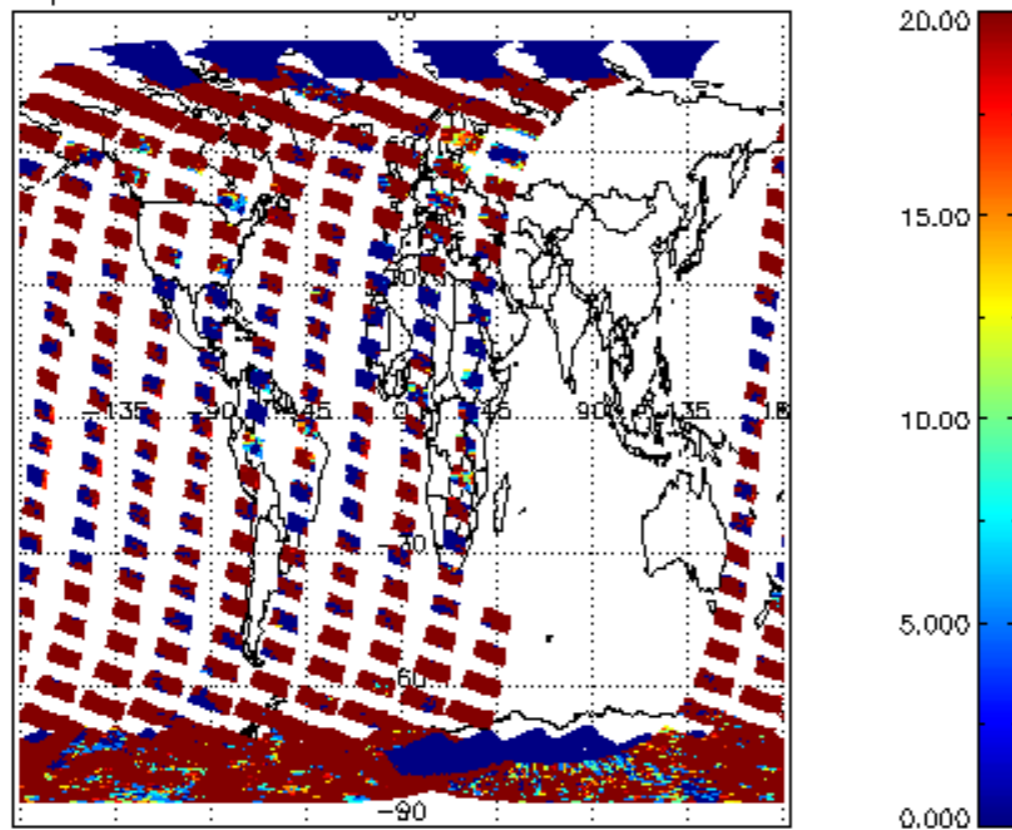
cI_opt_depth for 21FEB2011 00:00:00 to 22FEB2011 00:00:00
