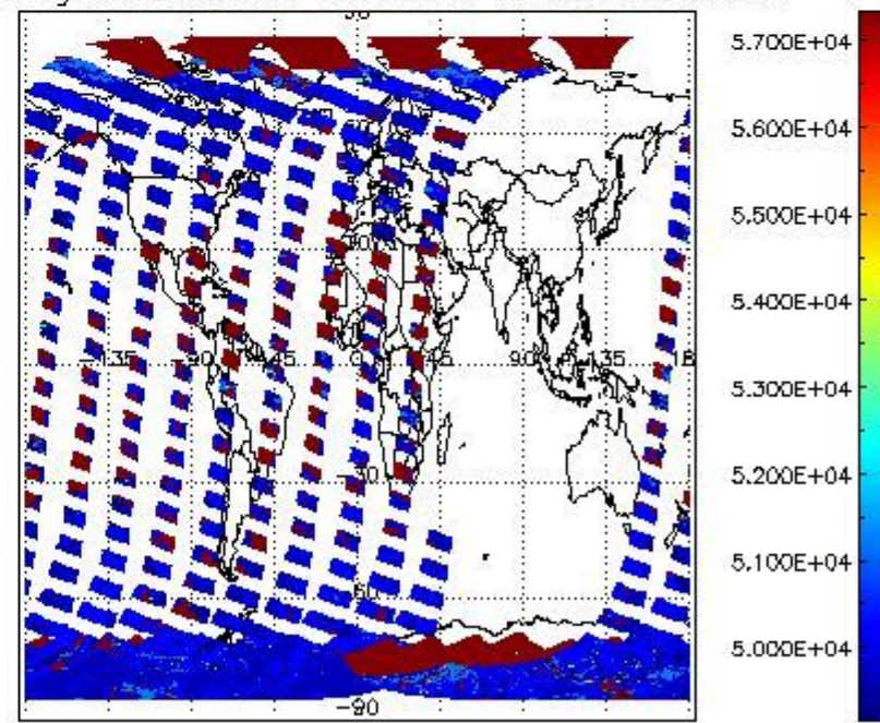
cloud_flags for 21FEB2011 00:00:00 to 22FEB2011 00:00:00
