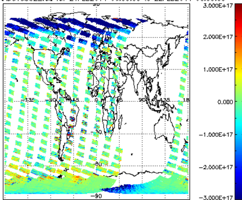
SCIOL2P_NADUV5S02_vcd for 21FEB2011 00:00:00 to 22FEB2011 00:00:00
