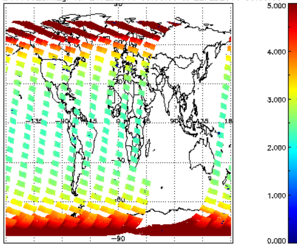
SCIOL2P_NADUV003_amf_gr for 21FEB2011 00:00:00 to 22FEB2011 00:00:00
