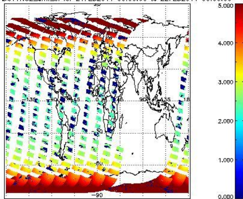
SCIOL2P_NADUV1N02_amf_cl for 21FEB2011 00:00:00 to 22FEB2011 00:00:00
