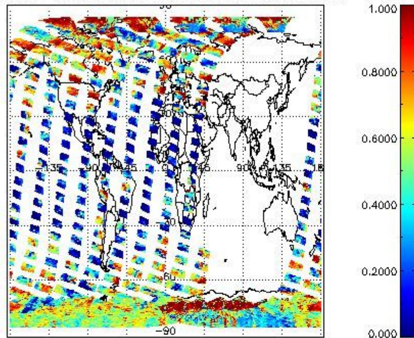
cL_frac for 21FEB2011 00:00:00 to 22FEB2011 00:00:00
