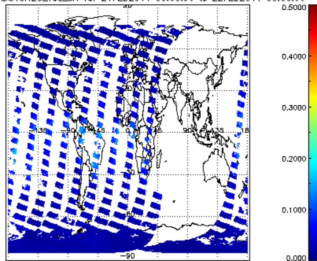
SCIOL2P_NADUV8H2O_vcd_err for 21FEB2011 00:00:00 to 22FEB2011 00:00:00
