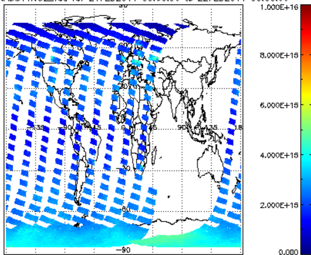
SCIOL2P_NADUV1N02_vcd for 21FEB2011 00:00:00 to 22FEB2011 00:00:00
