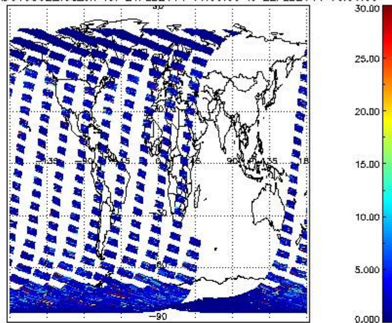
SCIOL2P_NADUV5S02_vcd_err for 21FEB2011 00:00:00 to 22FEB2011 00:00:00
