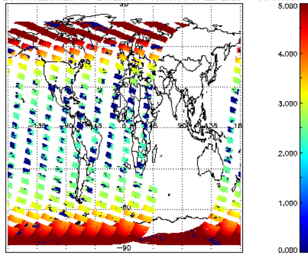
SCIOL2P_NADUV1N02_amf_cl for 21FEB2011 00:00:00 to 22FEB2011 00:00:00
