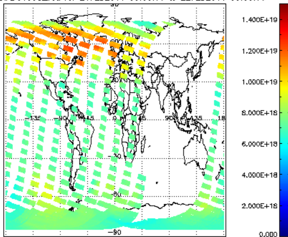
SCIOL2P_NADUV003_vcd for 21FEB2011 00:00:00 to 22FEB2011 00:00:00
