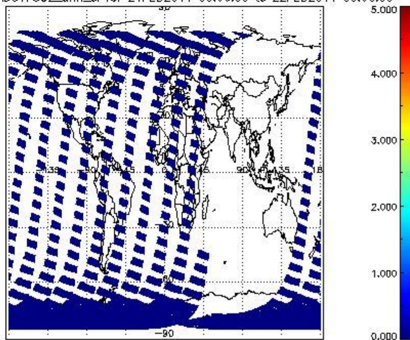
SCIOL2P_NADUV7S02_amf_cl for 21FEB2011 00:00:00 to 22FEB2011 00:00:00
