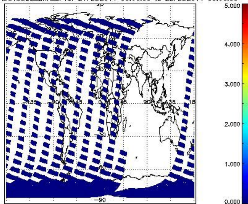
SCIOL2P_NADUV5S02_amf_cl for 21FEB2011 00:00:00 to 22FEB2011 00:00:00
