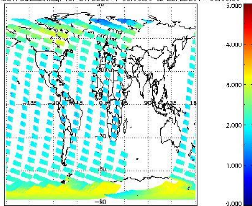
SCIOL2P_NADUV7S02_amf_gr for 21FEB2011 00:00:00 to 22FEB2011 00:00:00
