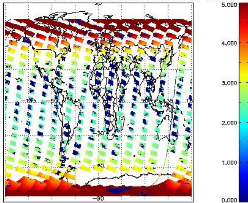
SCIOL2P_NADUV1N02_amf_cl for 17FEB2011 00:00:00 to 18FEB2011 00:00:00
