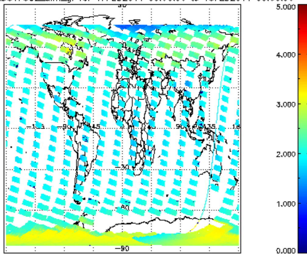
SCIOL2P_NADUV7S02_amf_gr for 17FEB2011 00:00:00 to 18FEB2011 00:00:00
