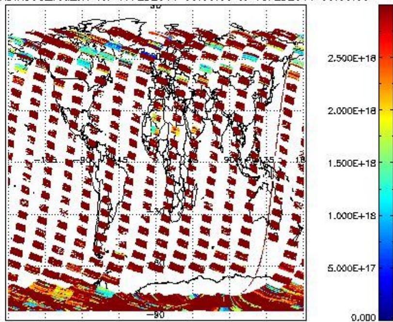
SCIO2P_NADIR3CO_vcd_err for 17FEB2011 00:00:00 to 18FEB2011 00:00:00
