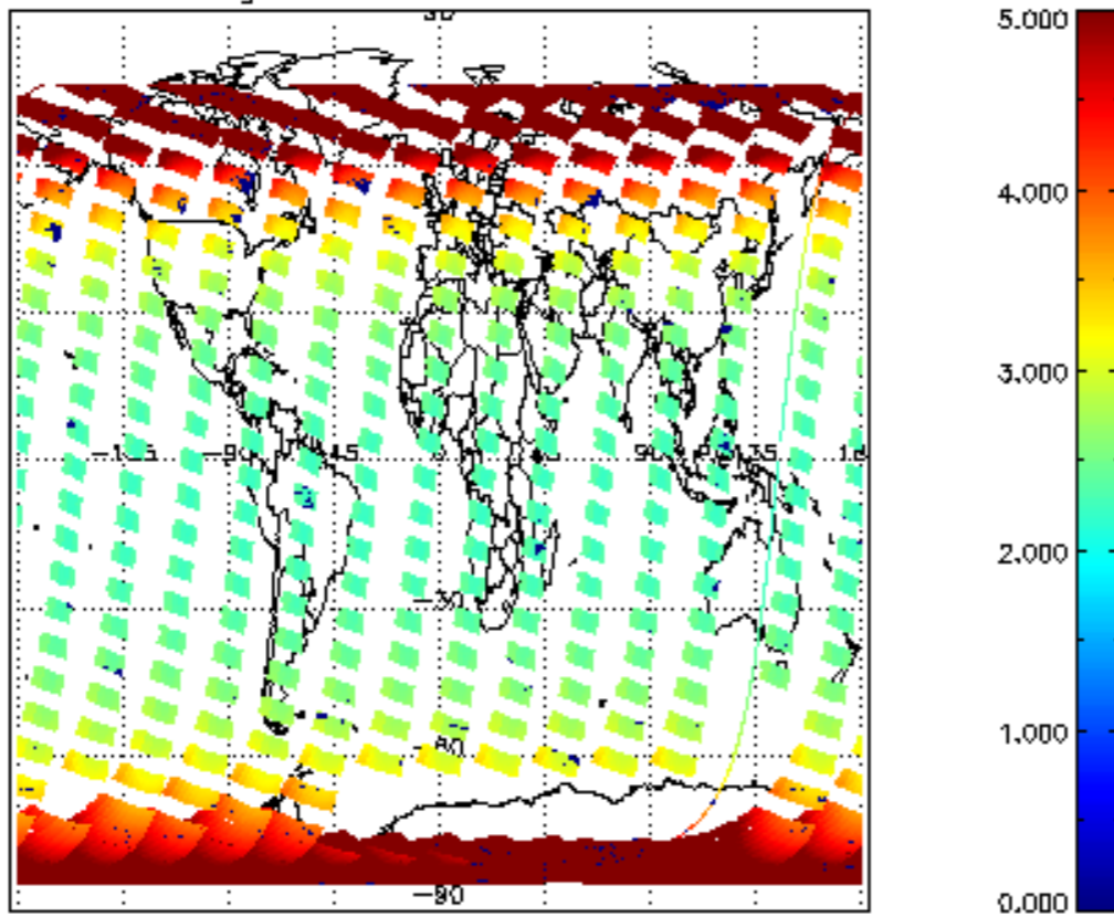
SCIOL2P_NADUV1N02_amf_gr for 17FEB2011 00:00:00 to 18FEB2011 00:00:00
