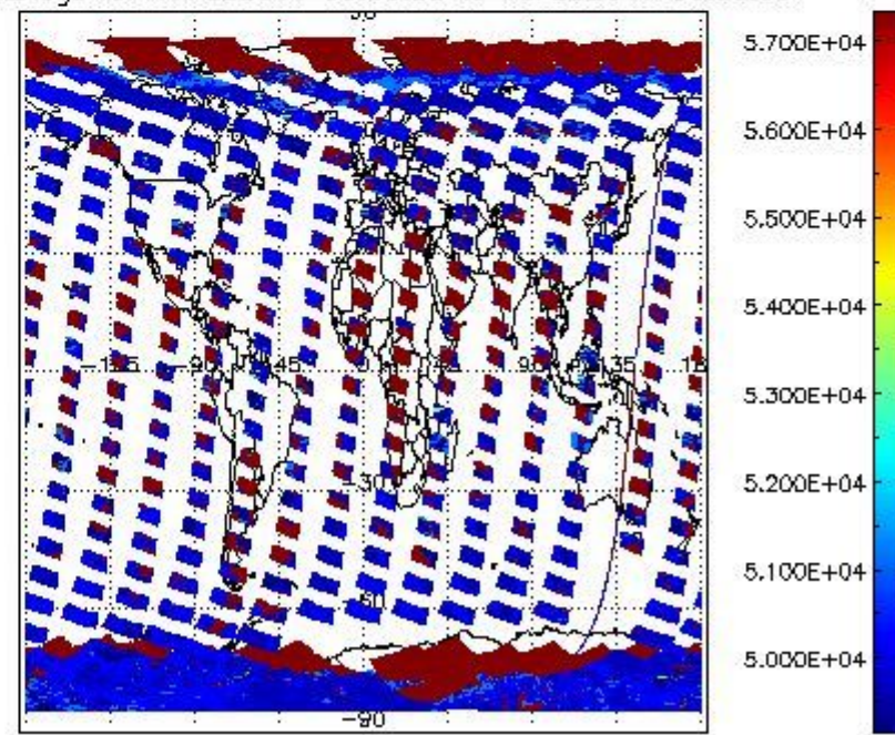
cloud_flags for 17FEB2011 00:00:00 to 18FEB2011 00:00:00
