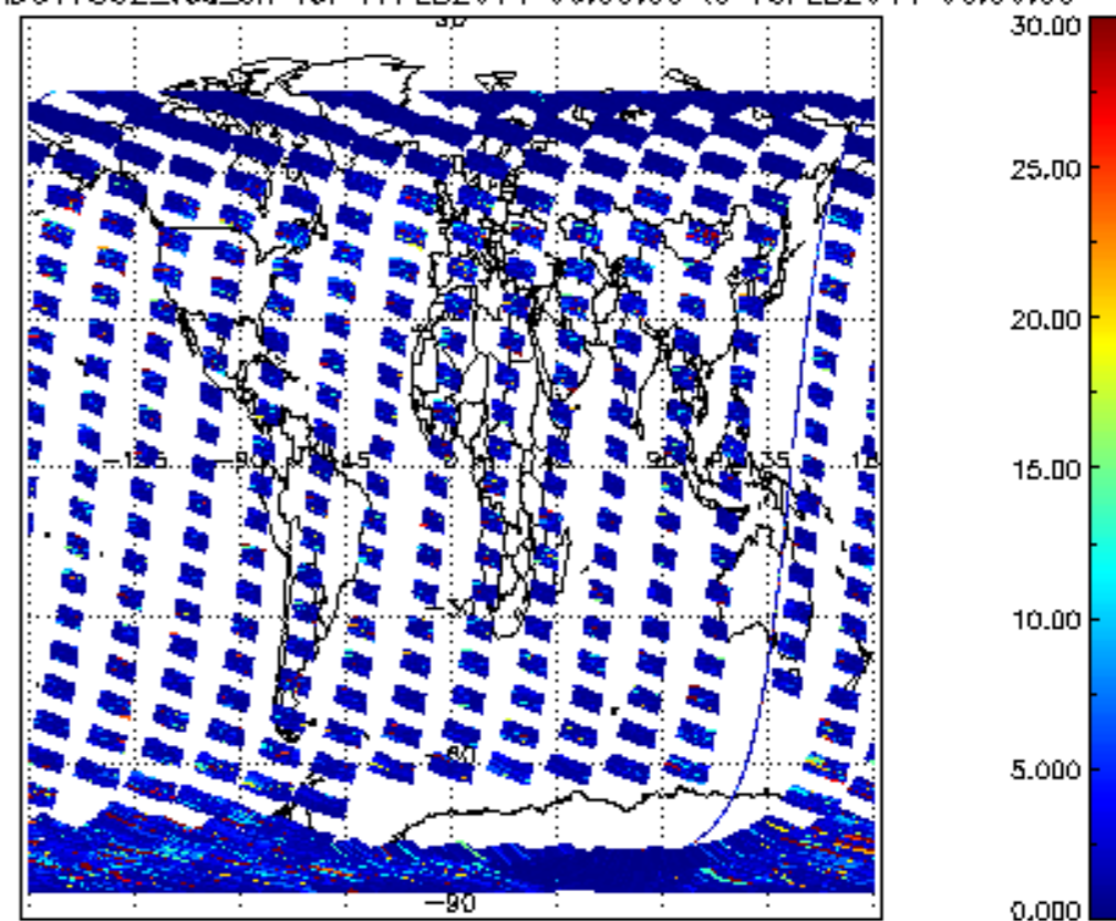
SCIOL2P_NADUV7S02_vcd_err for 17FEB2011 00:00:00 to 18FEB2011 00:00:00
