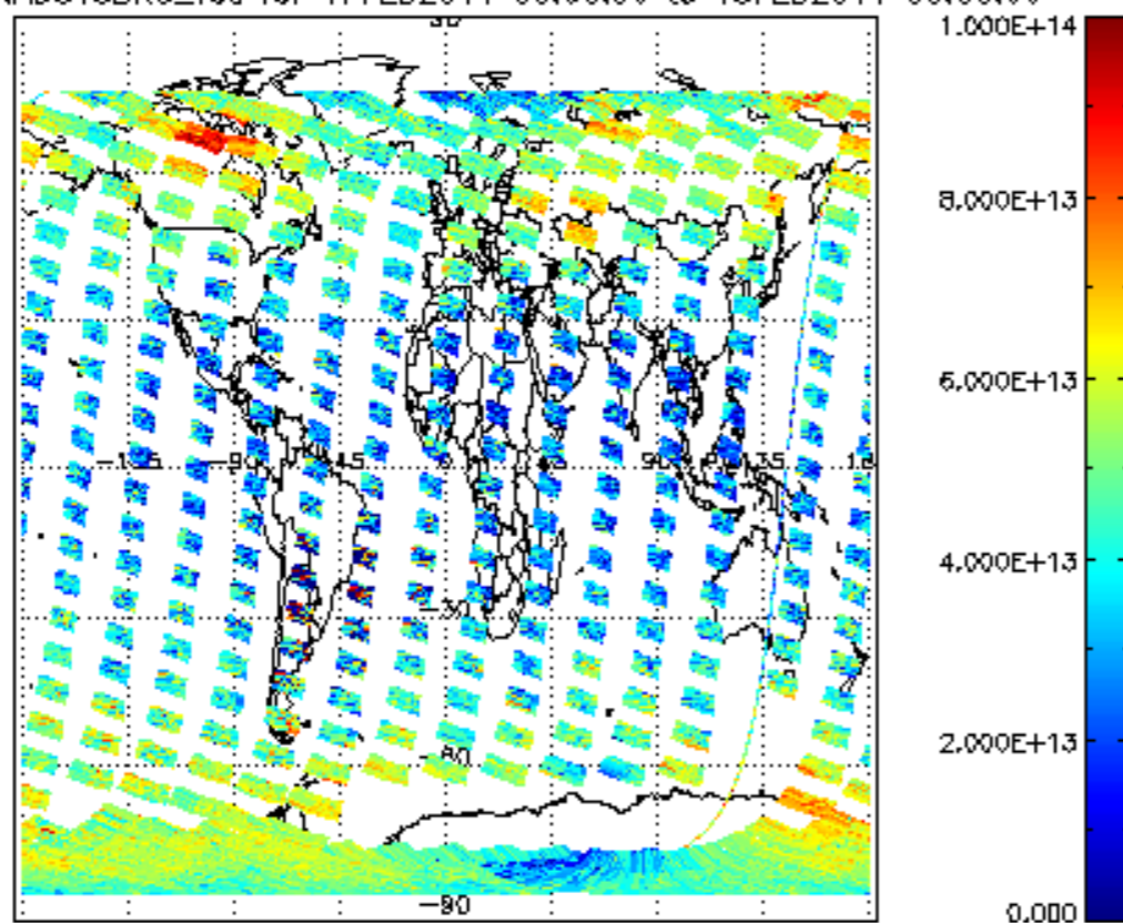
SCIOL2P_NADUV3BRO_vcd for 17FEB2011 00:00:00 to 18FEB2011 00:00:00
