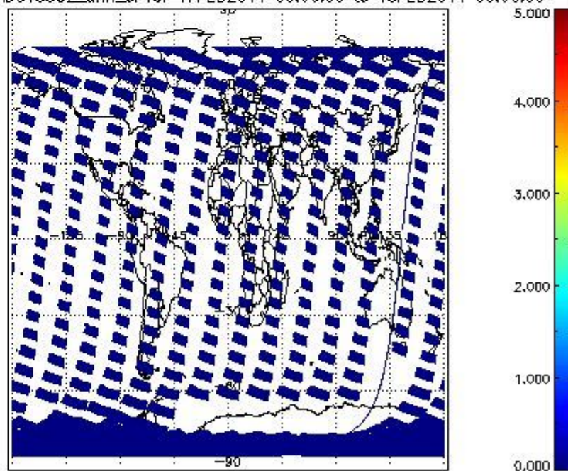
SCIOL2P_NADUV5S02_amf_cl for 17FEB2011 00:00:00 to 18FEB2011 00:00:00
