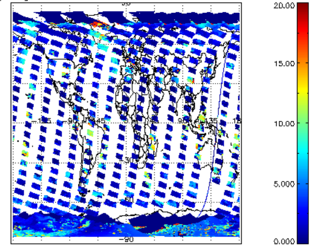
cl_top_height for 17FEB2011 00:00:00 to 18FEB2011 00:00:00
