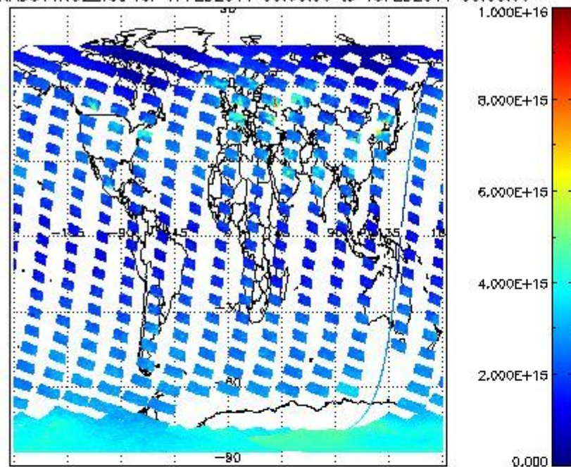
SCIOL2P_NADUV1N02_vcd for 17FEB2011 00:00:00 to 18FEB2011 00:00:00
