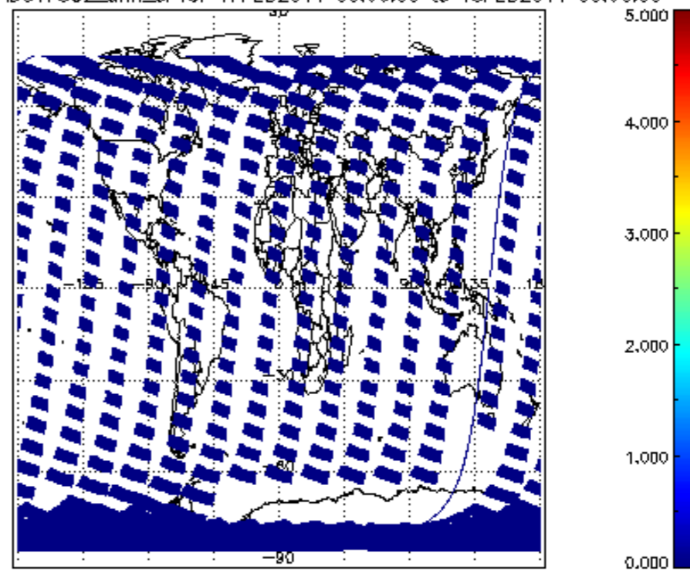
SCIOL2P_NADUV7S02_amf_cl for 17FEB2011 00:00:00 to 18FEB2011 00:00:00
