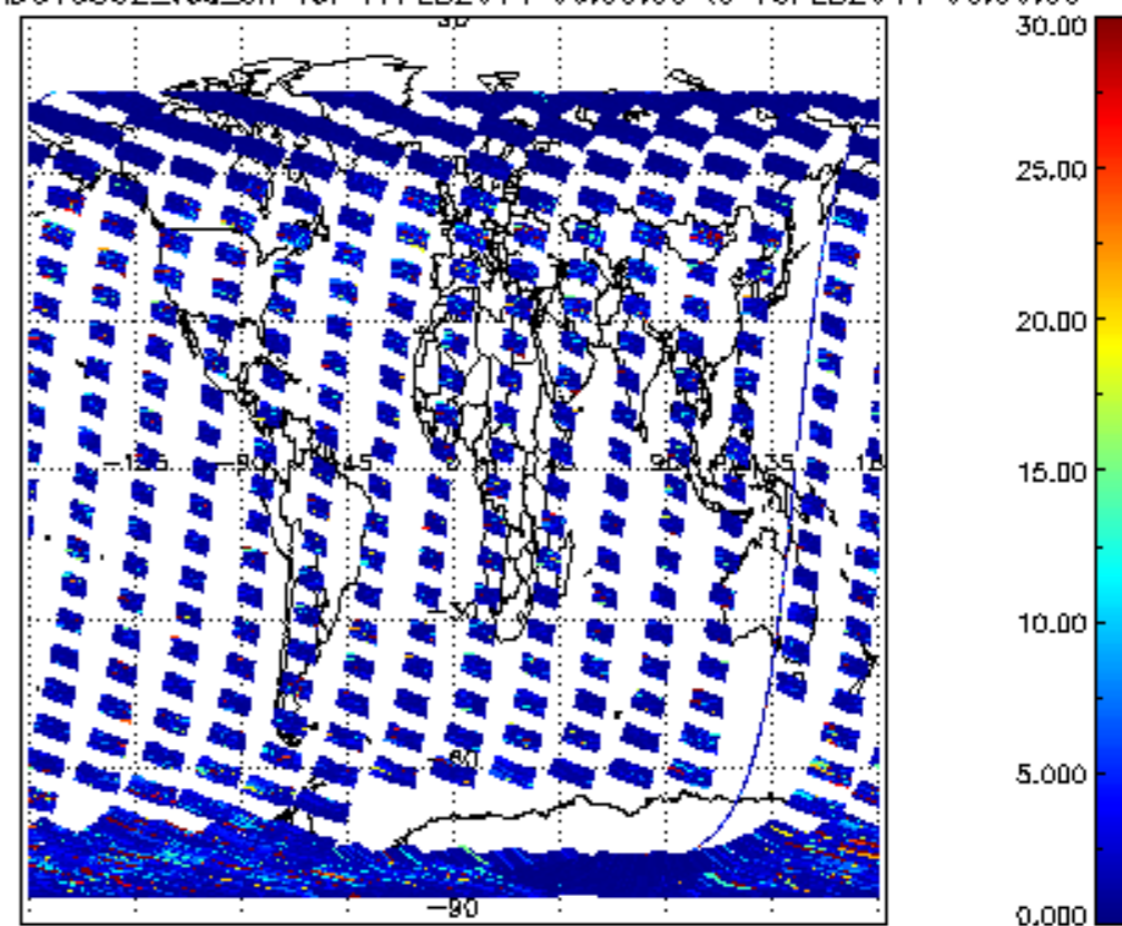
SCIOL2P_NADUV5S02_vcd_err for 17FEB2011 00:00:00 to 18FEB2011 00:00:00
