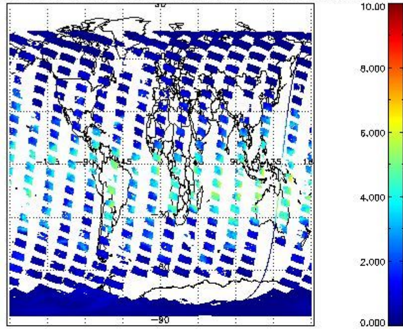
SCIOL2P_NADUV8H2O_vcd for 17FEB2011 00:00:00 to 18FEB2011 00:00:00
