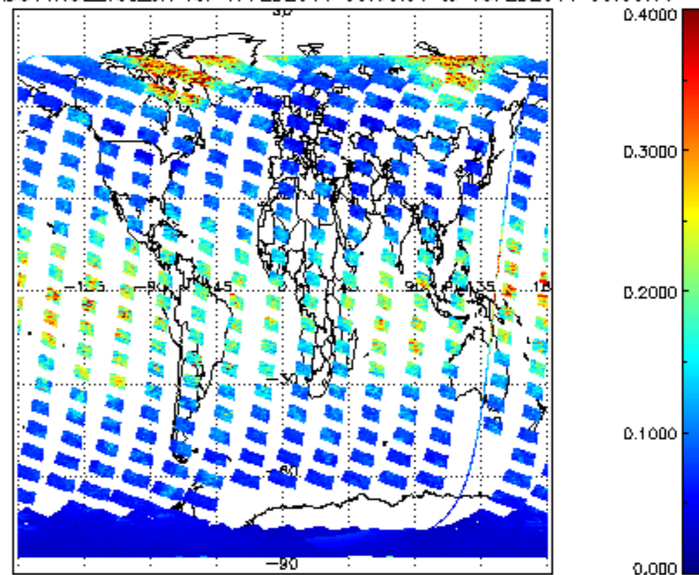
SCIOL2P_NADUV1N02_vcd_err for 17FEB2011 00:00:00 to 18FEB2011 00:00:00
