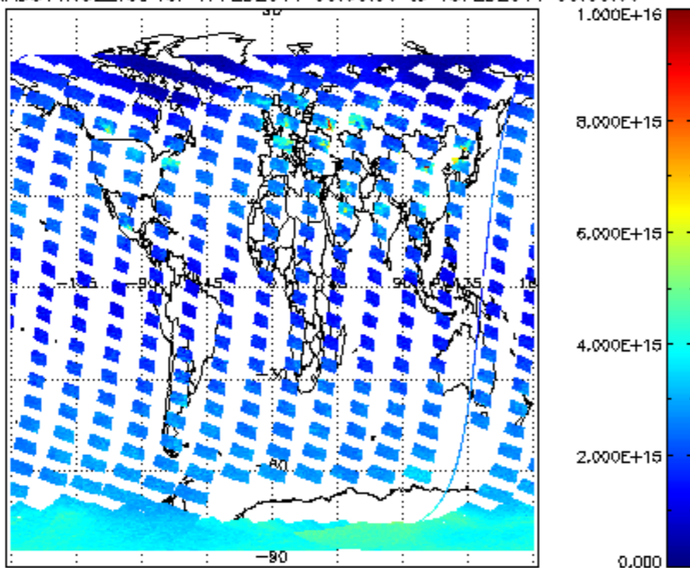
SCIOL2P_NADUV1N02_vcd for 17FEB2011 00:00:00 to 18FEB2011 00:00:00
