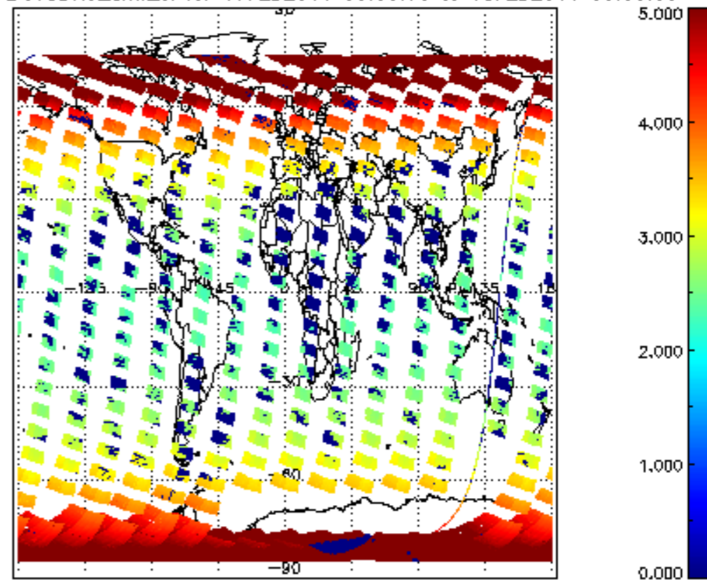
SCIOL2P_NADUV3BRO_amf_cl for 17FEB2011 00:00:00 to 18FEB2011 00:00:00
