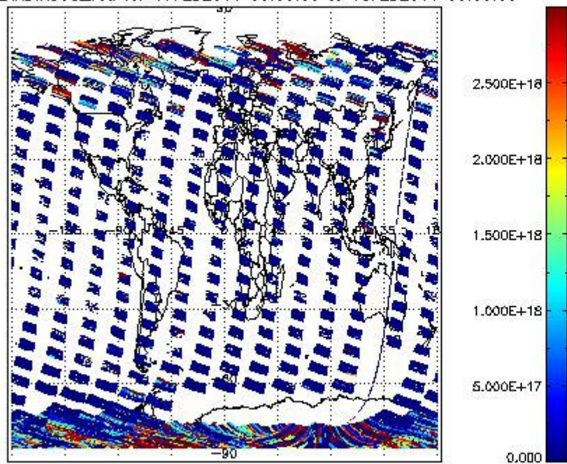
SCIO2P_NADIR3CO_vcd for 17FEB2011 00:00:00 to 18FEB2011 00:00:00
