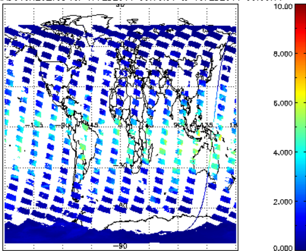
SCIOL2P_NADUV8H2O_vcd for 17FEB2011 00:00:00 to 18FEB2011 00:00:00
