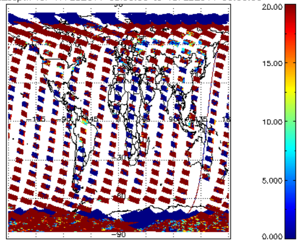
cl_opt_depth for 17FEB2011 00:00:00 to 18FEB2011 00:00:00
