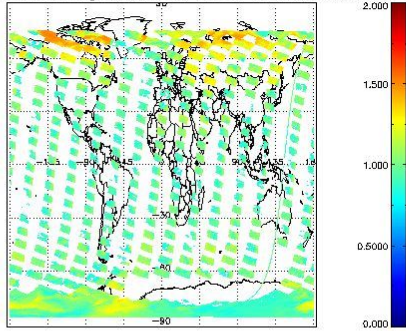
SCIOL2P_NADUV8H2O_amf_gr for 17FEB2011 00:00:00 to 18FEB2011 00:00:00
