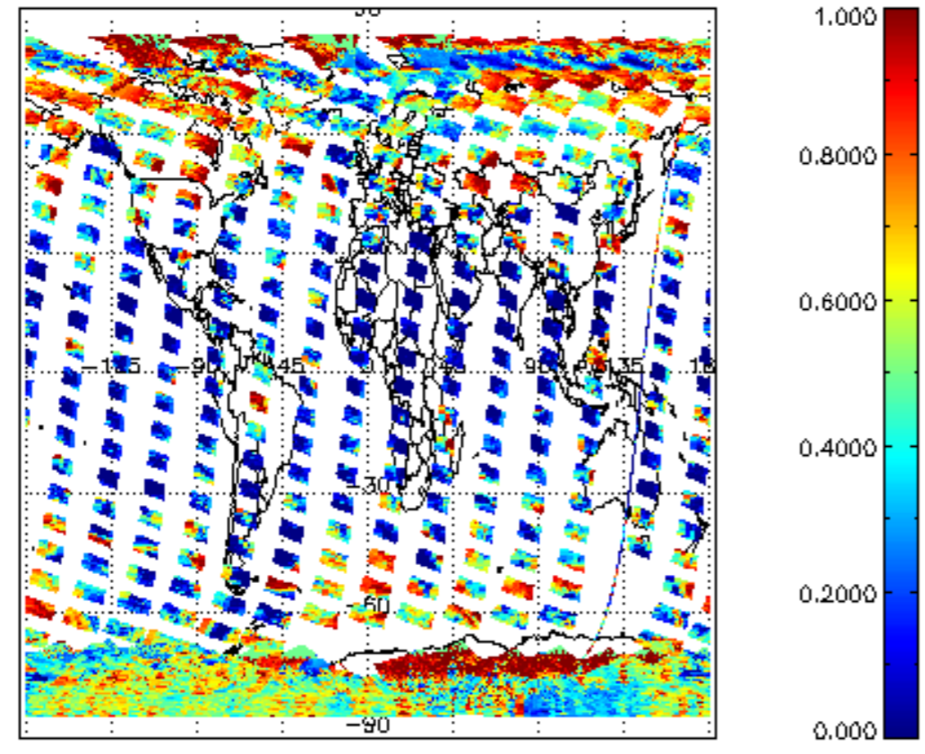
cl_frac for 17FEB2011 00:00:00 to 18FEB2011 00:00:00
