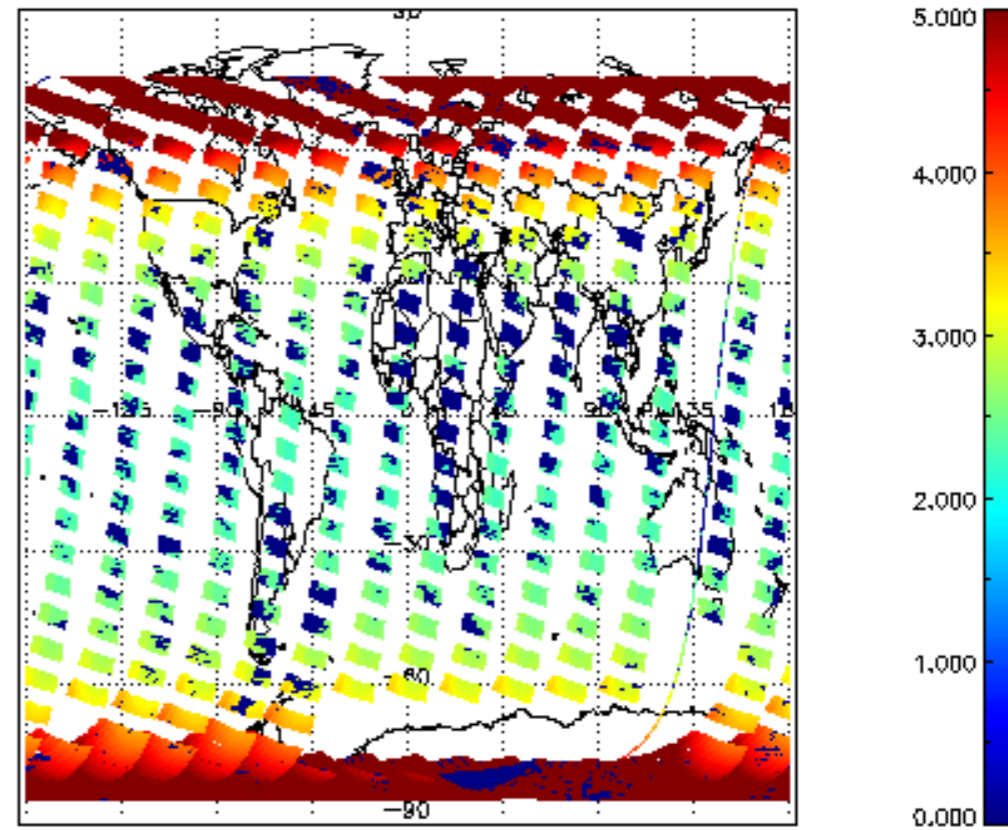
SCIOL2P_NADUV1N02_amf_cl for 17FEB2011 00:00:00 to 18FEB2011 00:00:00
