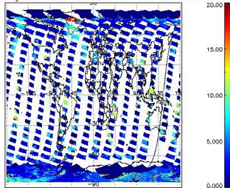
cL_top_height for 17FEB2011 00:00:00 to 18FEB2011 00:00:00
