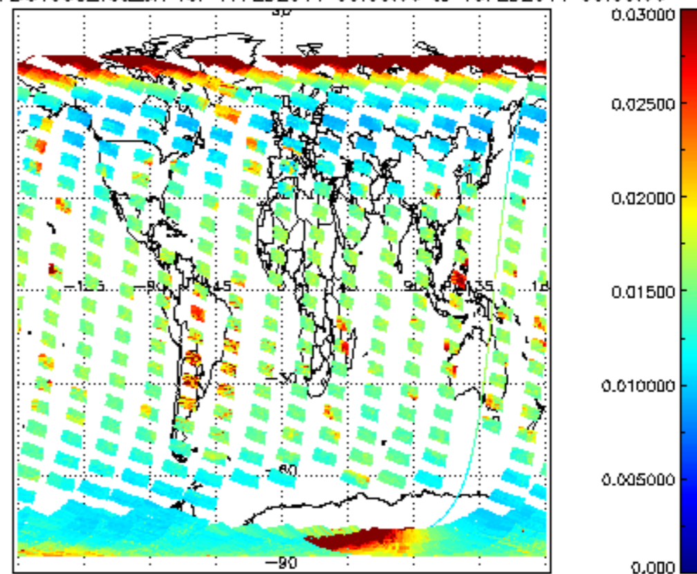
SCIOL2P_NADUV003_vcd_err for 17FEB2011 00:00:00 to 18FEB2011 00:00:00
