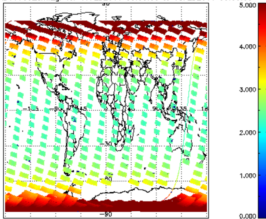
SCIOL2P_NADUV003_amf_gr for 17FEB2011 00:00:00 to 18FEB2011 00:00:00
