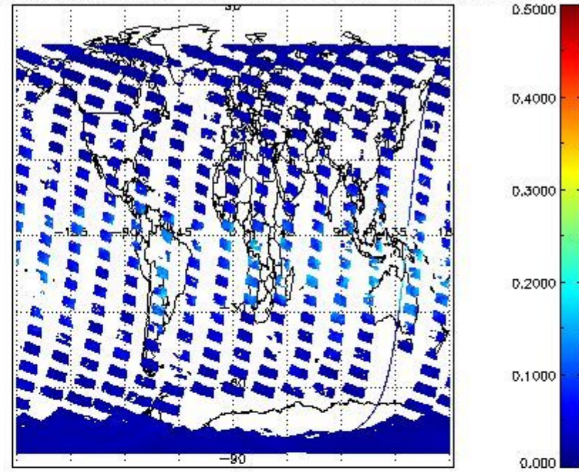
SCIOL2P_NADUV8H2O_vcd_err for 17FEB2011 00:00:00 to 18FEB2011 00:00:00
