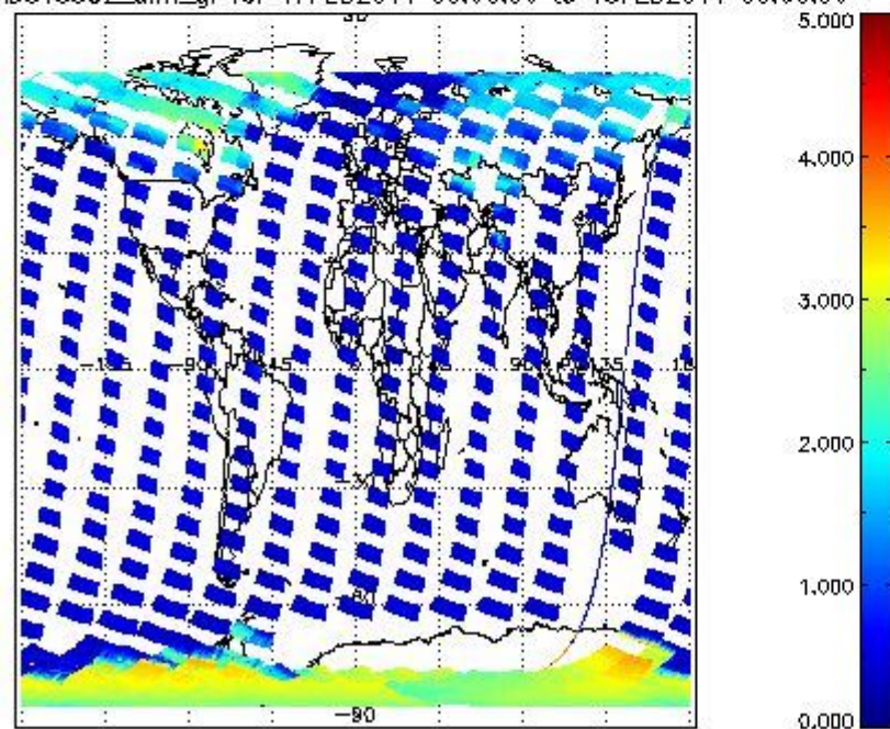
SCIOL2P_NADUV5S02_amf_gr for 17FEB2011 00:00:00 to 18FEB2011 00:00:00
