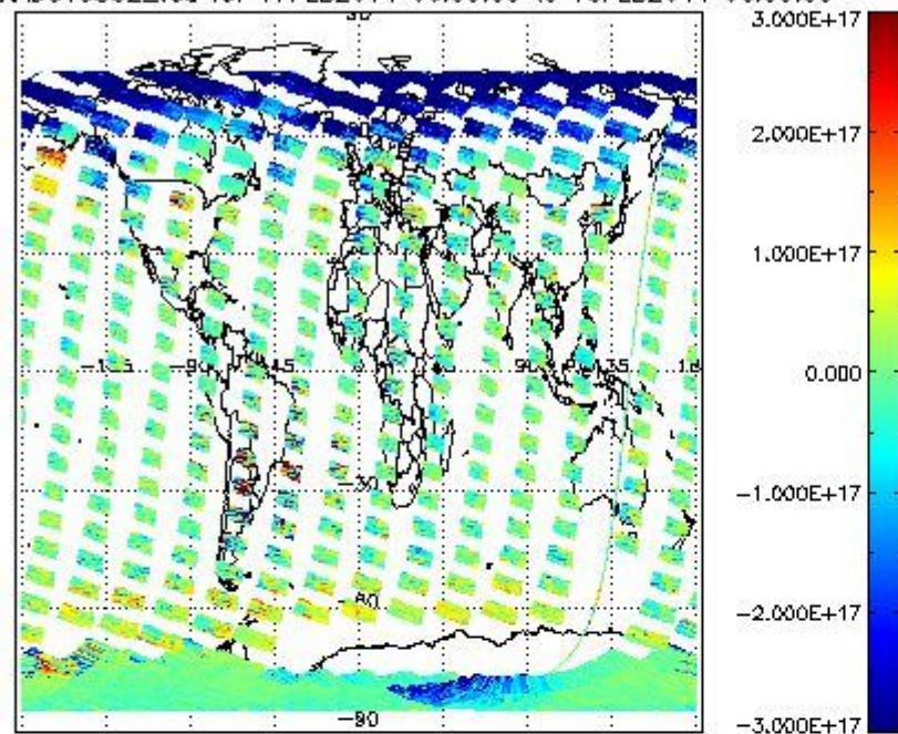
SCIOL2P_NADUV5S02_vcd for 17FEB2011 00:00:00 to 18FEB2011 00:00:00
