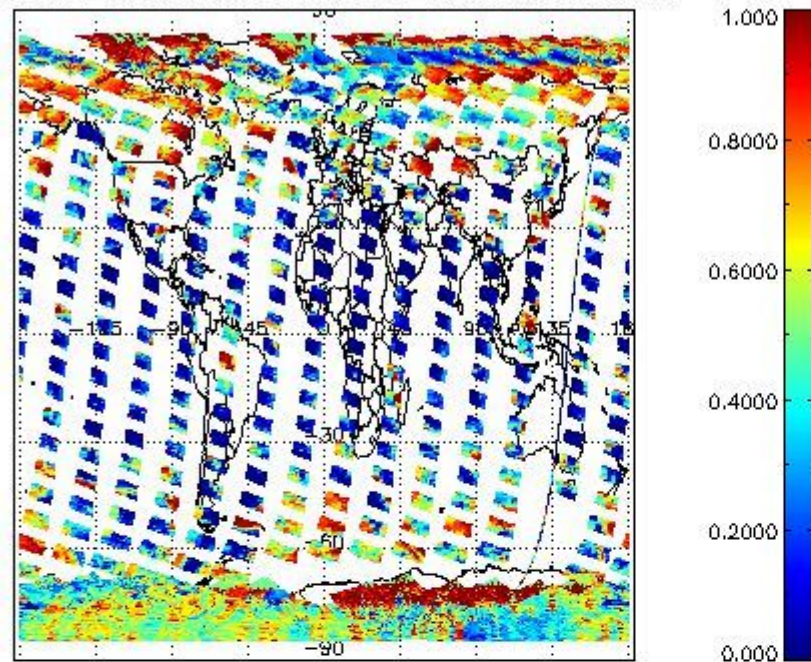
cL_frac for 17FEB2011 00:00:00 to 18FEB2011 00:00:00
