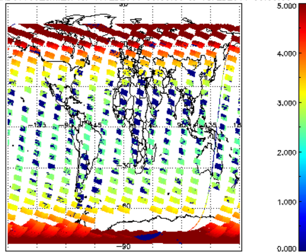
SCIOL2P_NADUV003_amf_cl for 17FEB2011 00:00:00 to 18FEB2011 00:00:00
