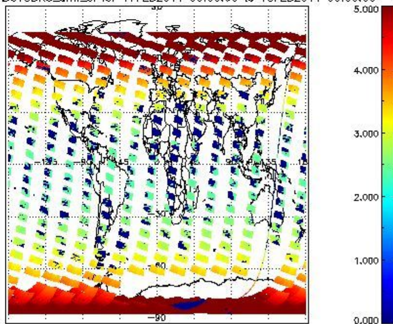
SCIOL2P_NADUV3BRO_amf_cl for 17FEB2011 00:00:00 to 18FEB2011 00:00:00
