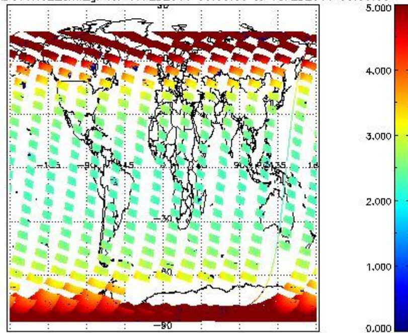
SCIOL2P_NADUV1N02_amf_gr for 17FEB2011 00:00:00 to 18FEB2011 00:00:00
