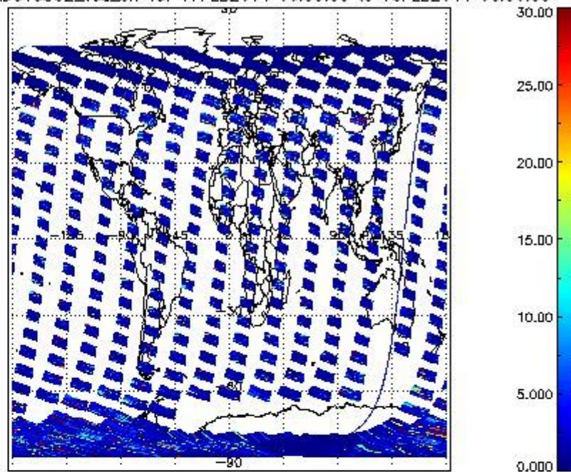
SCIOL2P_NADUV5S02_vcd_err for 17FEB2011 00:00:00 to 18FEB2011 00:00:00
