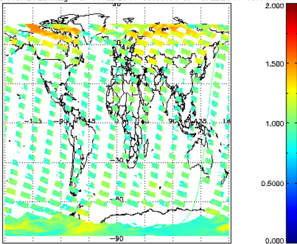
SCIOL2P_NADUV8H2O_amf_gr for 17FEB2011 00:00:00 to 18FEB2011 00:00:00
