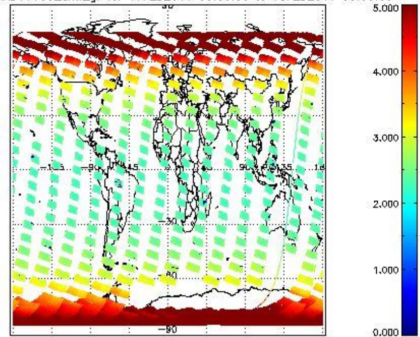
SCIOL2P_NADUV003_amf_gr for 17FEB2011 00:00:00 to 18FEB2011 00:00:00
