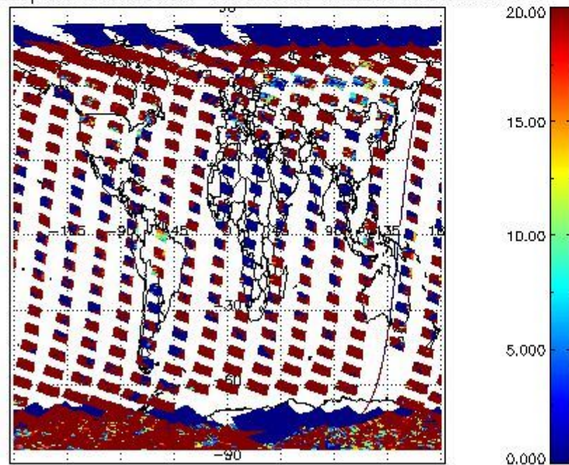
cL_opt_depth for 17FEB2011 00:00:00 to 18FEB2011 00:00:00
