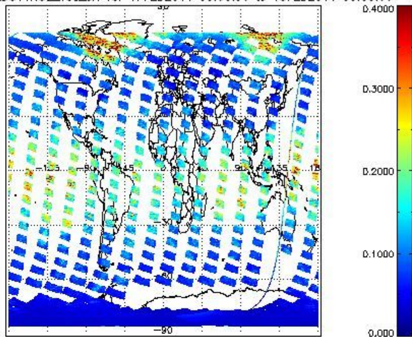
SCIOL2P_NADUV1N02_vcd_err for 17FEB2011 00:00:00 to 18FEB2011 00:00:00
