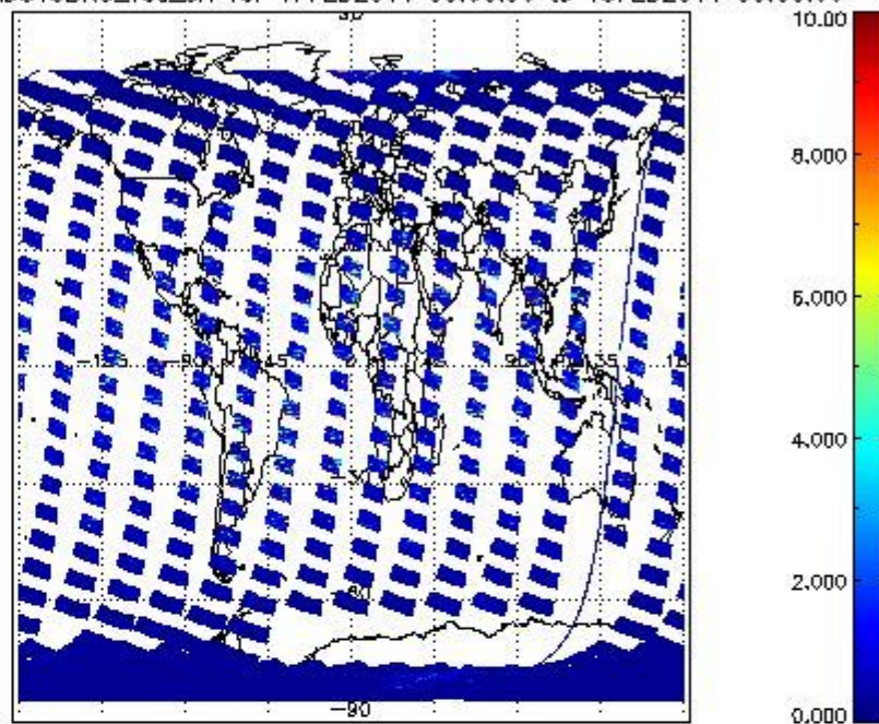
SCIOL2P_NADUV3BRO_vcd_err for 17FEB2011 00:00:00 to 18FEB2011 00:00:00
