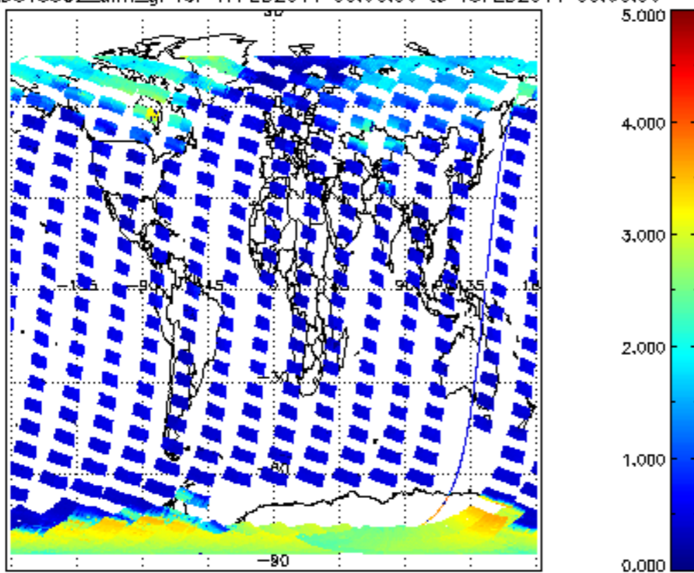
SCIOL2P_NADUV5S02_amf_gr for 17FEB2011 00:00:00 to 18FEB2011 00:00:00
