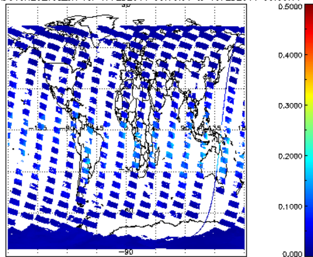
SCIOL2P_NADUV8H2O_vcd_err for 17FEB2011 00:00:00 to 18FEB2011 00:00:00
