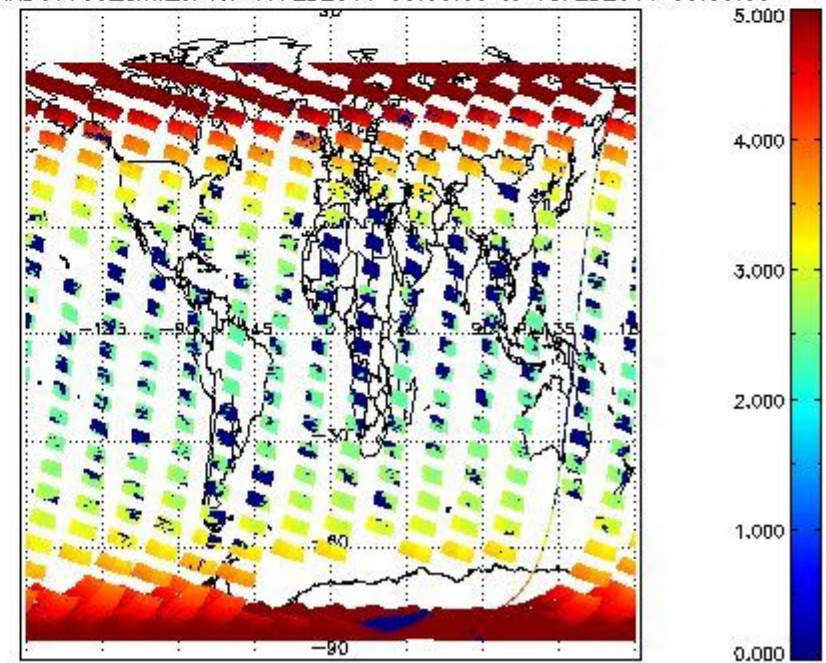
SCIOL2P_NADUV003_amf_cl for 17FEB2011 00:00:00 to 18FEB2011 00:00:00
