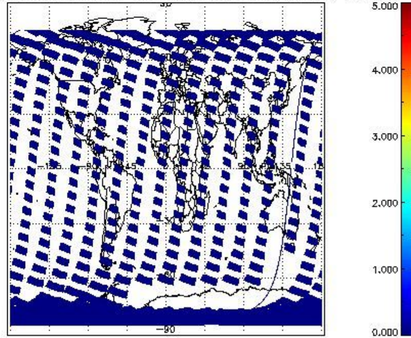
SCIOL2P_NADUV7S02_amf_cl for 17FEB2011 00:00:00 to 18FEB2011 00:00:00
