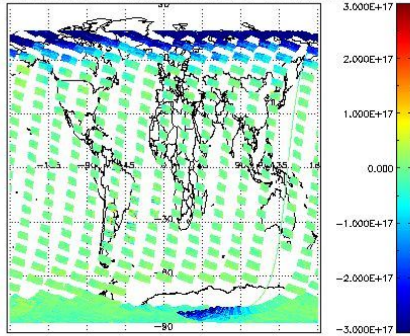
SCIOL2P_NADUV7S02_vcd for 17FEB2011 00:00:00 to 18FEB2011 00:00:00
