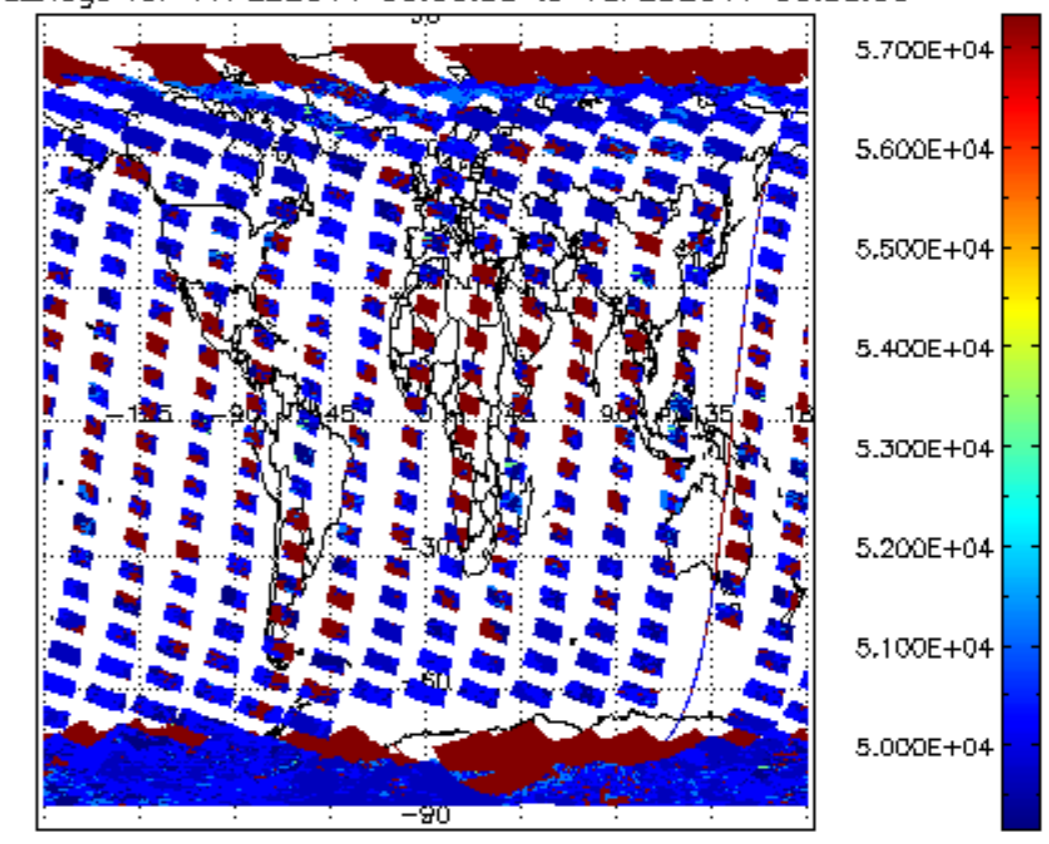
cloud_flags for 17FEB2011 00:00:00 to 18FEB2011 00:00:00
