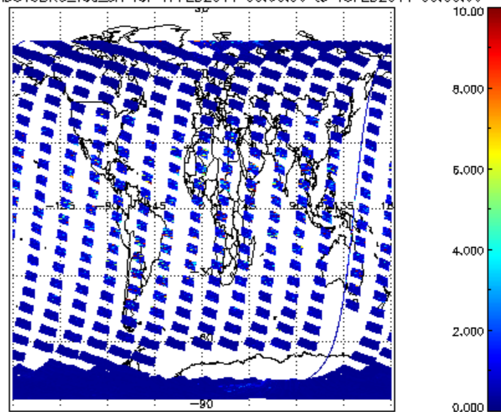
SCIOL2P_NADUV3BRO_vcd_err for 17FEB2011 00:00:00 to 18FEB2011 00:00:00
