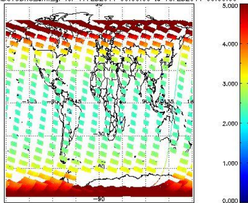
SCIOL2P_NADUV3BRO_amf_gr for 17FEB2011 00:00:00 to 18FEB2011 00:00:00
