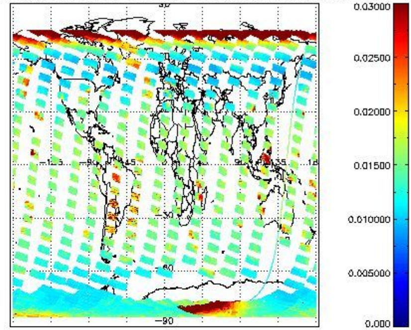
SCIOL2P_NADUV003_vcd_err for 17FEB2011 00:00:00 to 18FEB2011 00:00:00
