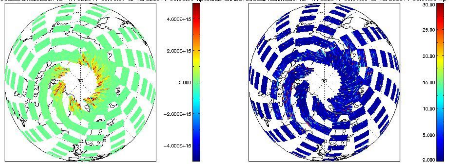
CIOL2P_NADUV6OCLslant_col_den for 17FEB2011 00:00:00 to 18FEB2011 00:00:00 np; CIOL2P_NADUV6OCLarr_slant_col for 17FEB2011 00:00:00 to 18FEB2011 00:00:00 np
