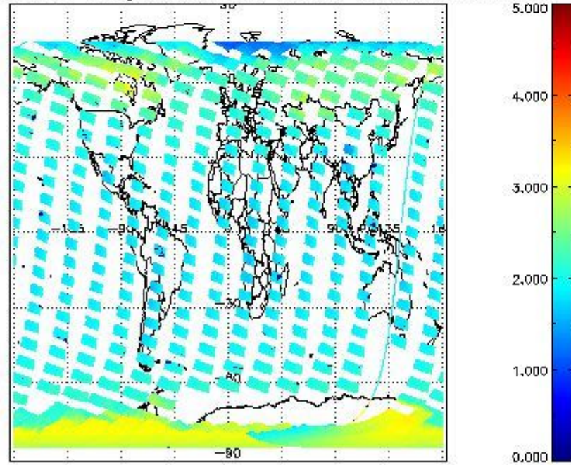
SCIOL2P_NADUV7S02_amf_gr for 17FEB2011 00:00:00 to 18FEB2011 00:00:00
