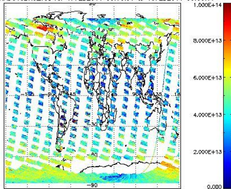
SCIOL2P_NADUV3BRO_vcd for 17FEB2011 00:00:00 to 18FEB2011 00:00:00
