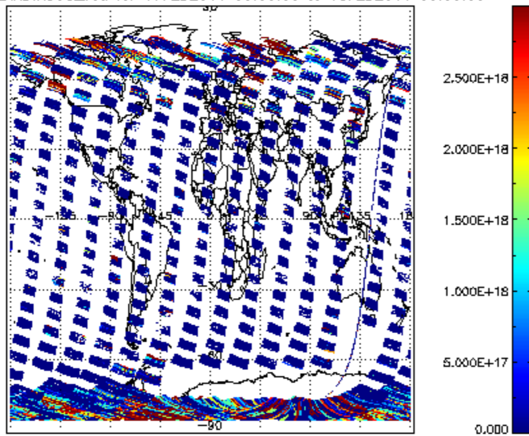
SCIOL2P_NADIR3CO_vcd for 17FEB2011 00:00:00 to 18FEB2011 00:00:00
