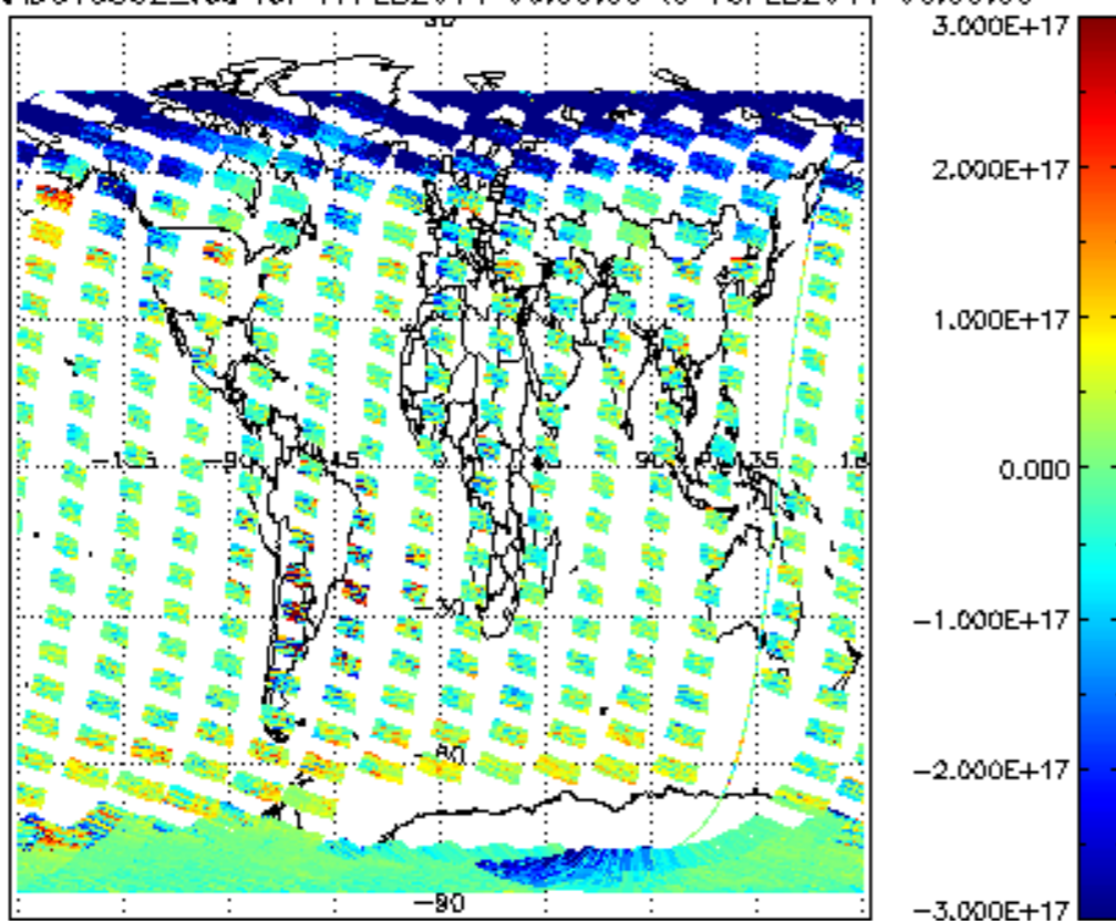
SCIOL2P_NADUV5S02_vcd for 17FEB2011 00:00:00 to 18FEB2011 00:00:00
