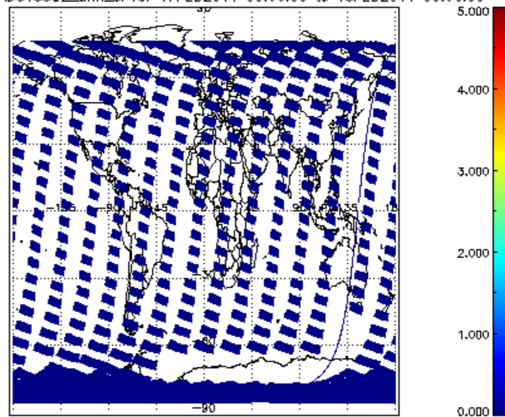
SCIOL2P_NADUV5S02_amf_cl for 17FEB2011 00:00:00 to 18FEB2011 00:00:00
