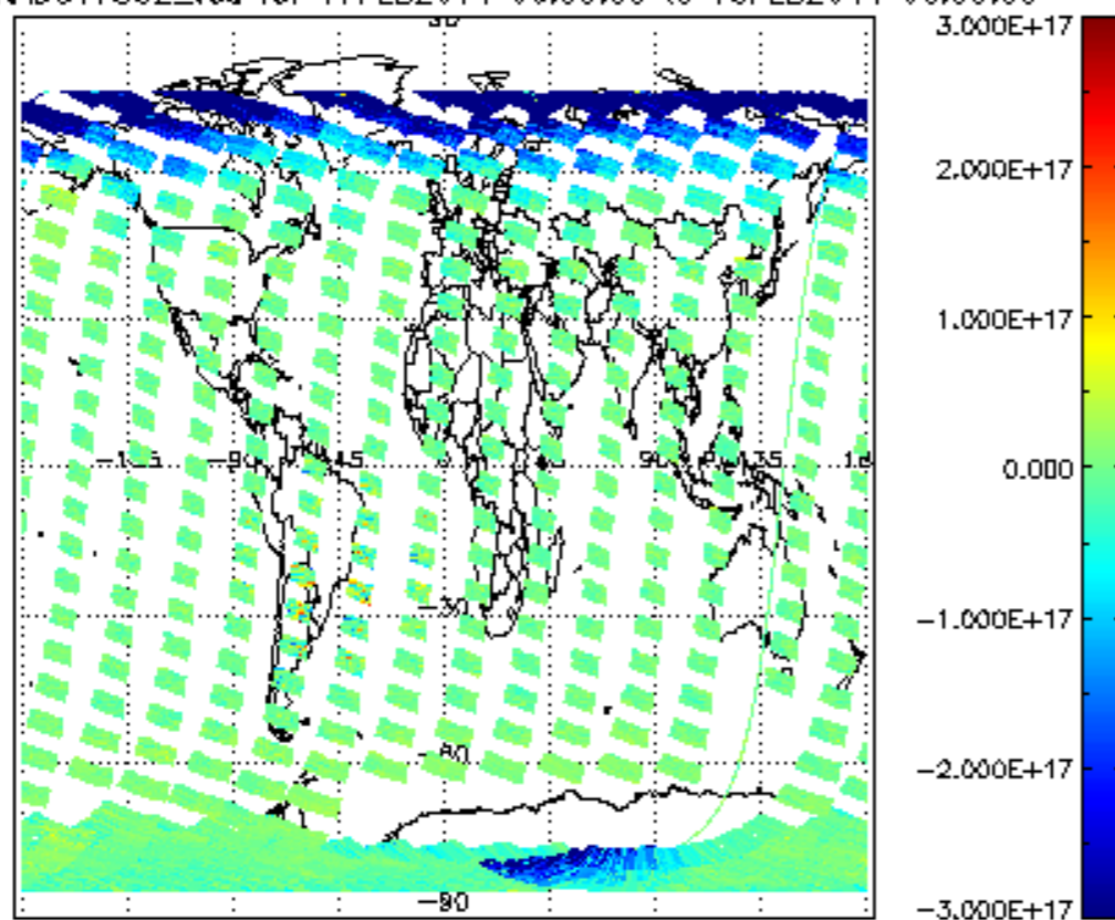
SCIOL2P_NADUV7S02_vcd for 17FEB2011 00:00:00 to 18FEB2011 00:00:00
