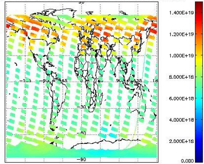
SCIOL2P_NADUV003_vcd for 17FEB2011 00:00:00 to 18FEB2011 00:00:00
