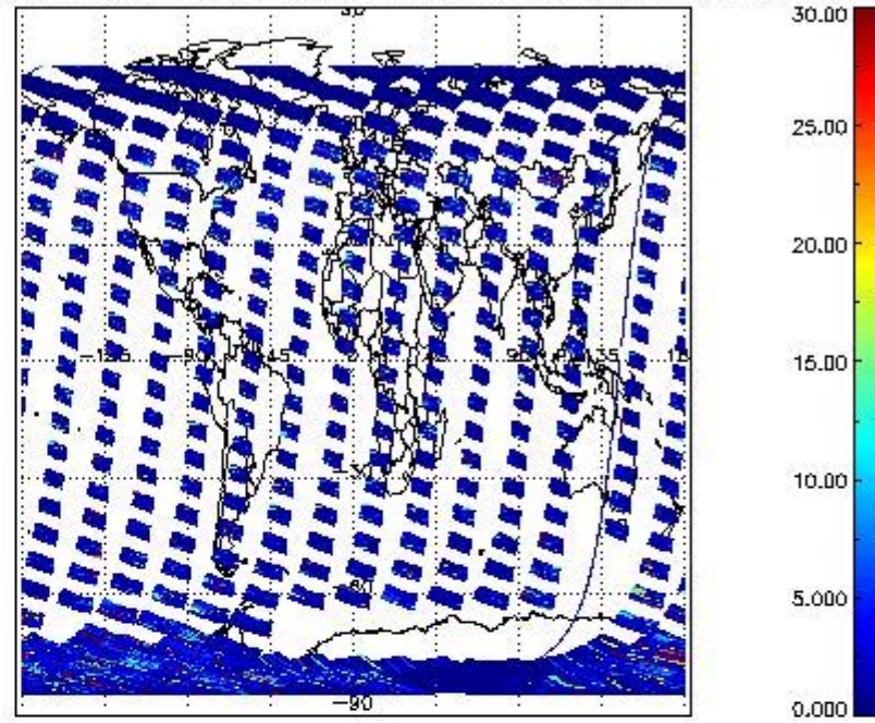
SCIOL2P_NADUV7S02_vcd_err for 17FEB2011 00:00:00 to 18FEB2011 00:00:00
