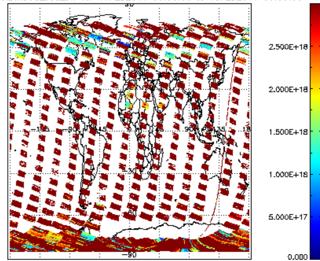
SCIOL2P_NADIR3CO_vcd_Lerr for 17FEB2011 00:00:00 to 18FEB2011 00:00:00
