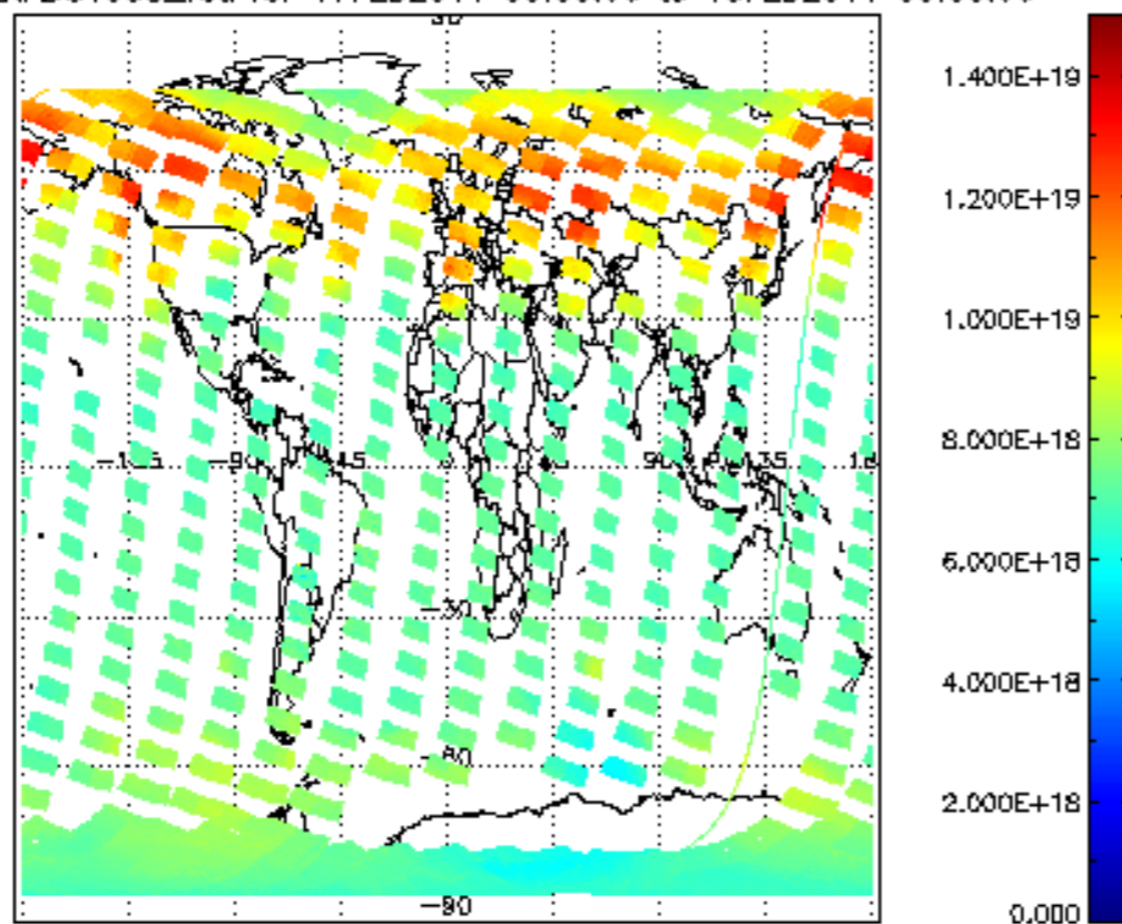
SCIOL2P_NADUV003_vcd for 17FEB2011 00:00:00 to 18FEB2011 00:00:00
