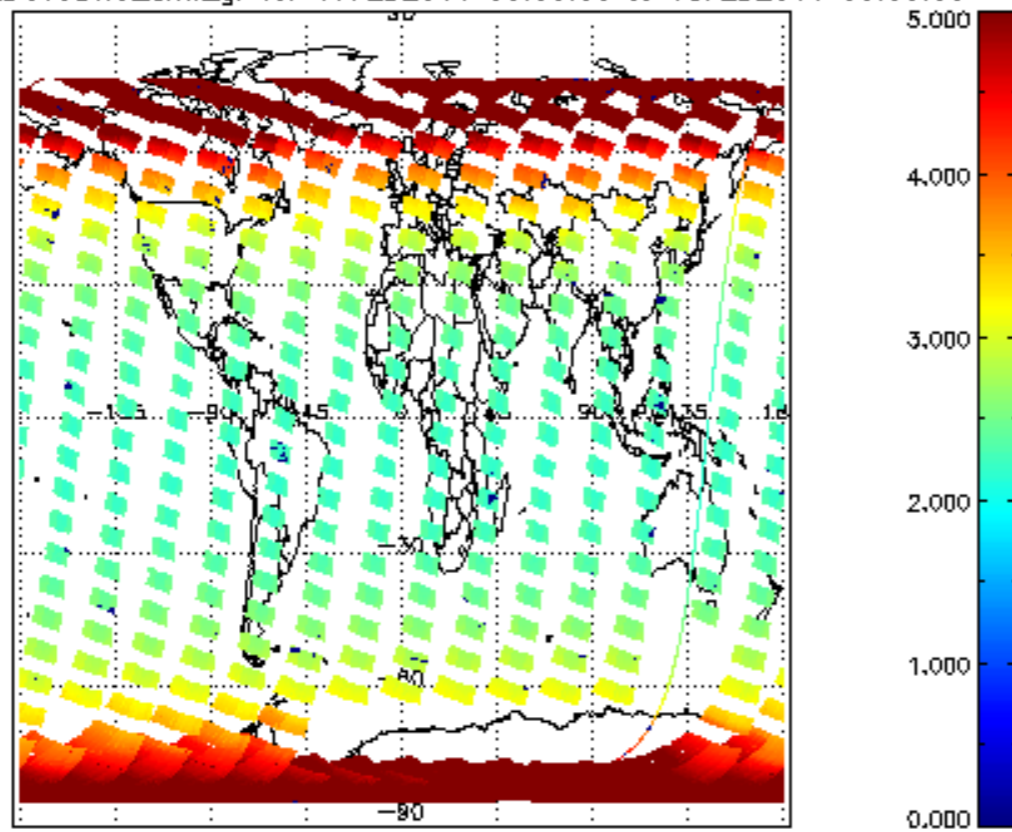
SCIOL2P_NADUV3BRO_amf_gr for 17FEB2011 00:00:00 to 18FEB2011 00:00:00
