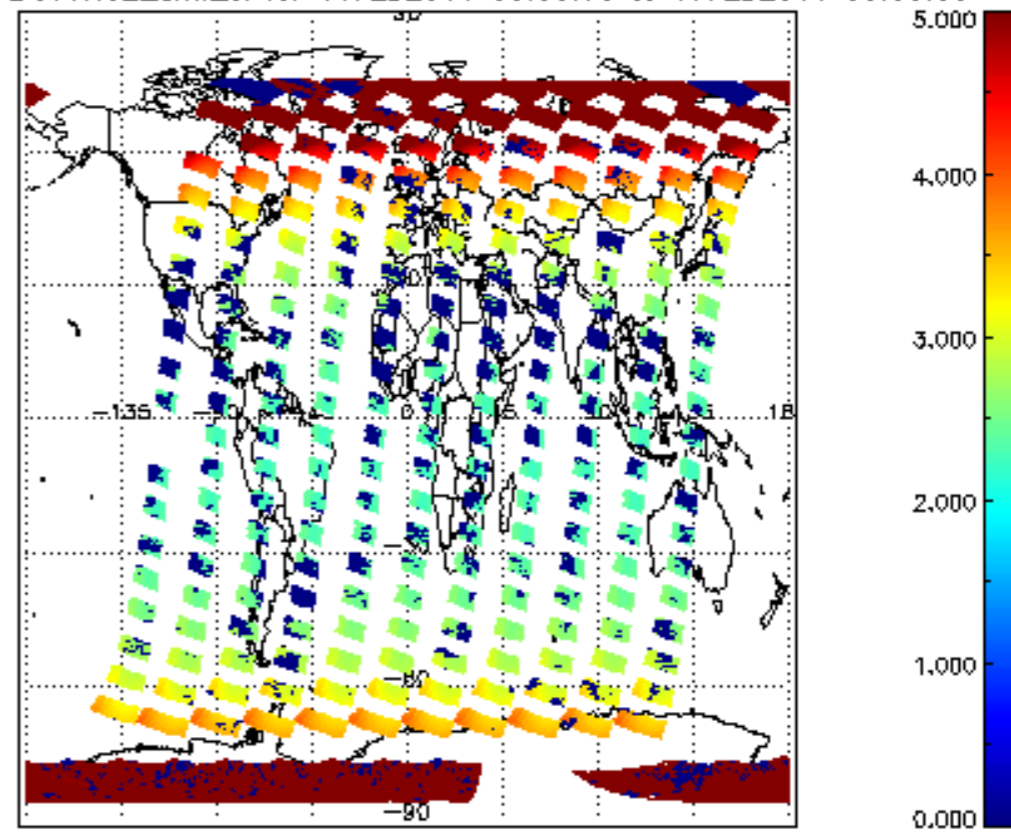
SCIOL2P_NADUV1N02_amf_cl for 16FEB2011 00:00:00 to 17FEB2011 00:00:00
