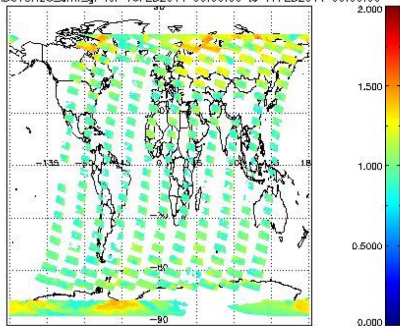
SCIOL2P_NADUV8H2O_amf_gr for 16FEB2011 00:00:00 to 17FEB2011 00:00:00
