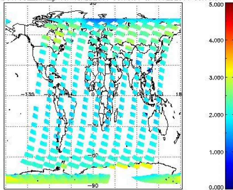
SCIOL2P_NADUV7S02_amf_gr for 16FEB2011 00:00:00 to 17FEB2011 00:00:00
