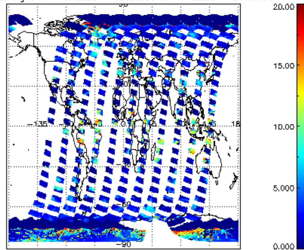
cL_top_height for 16FEB2011 00:00:00 to 17FEB2011 00:00:00
