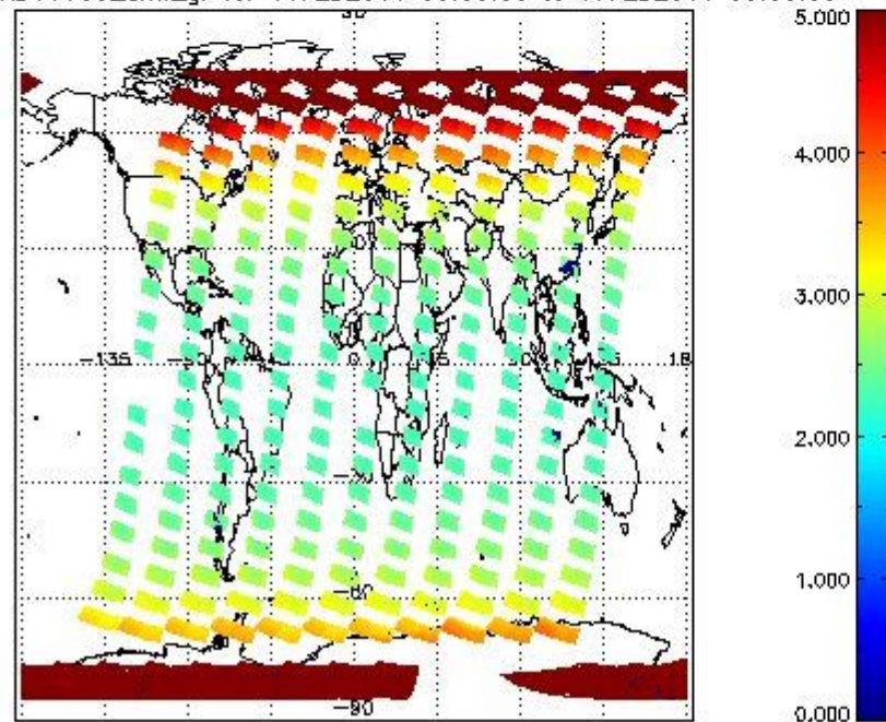
SCIOL2P_NADUV003_amf_gr for 16FEB2011 00:00:00 to 17FEB2011 00:00:00
