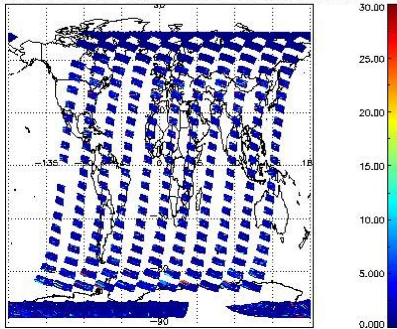
SCIOL2P_NADUV7S02_vcd_err for 16FEB2011 00:00:00 to 17FEB2011 00:00:00
