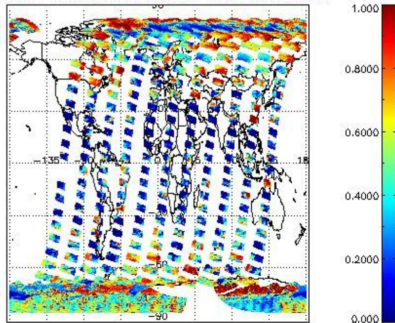
cL_frae for 16FEB2011 00:00:00 to 17FEB2011 00:00:00
