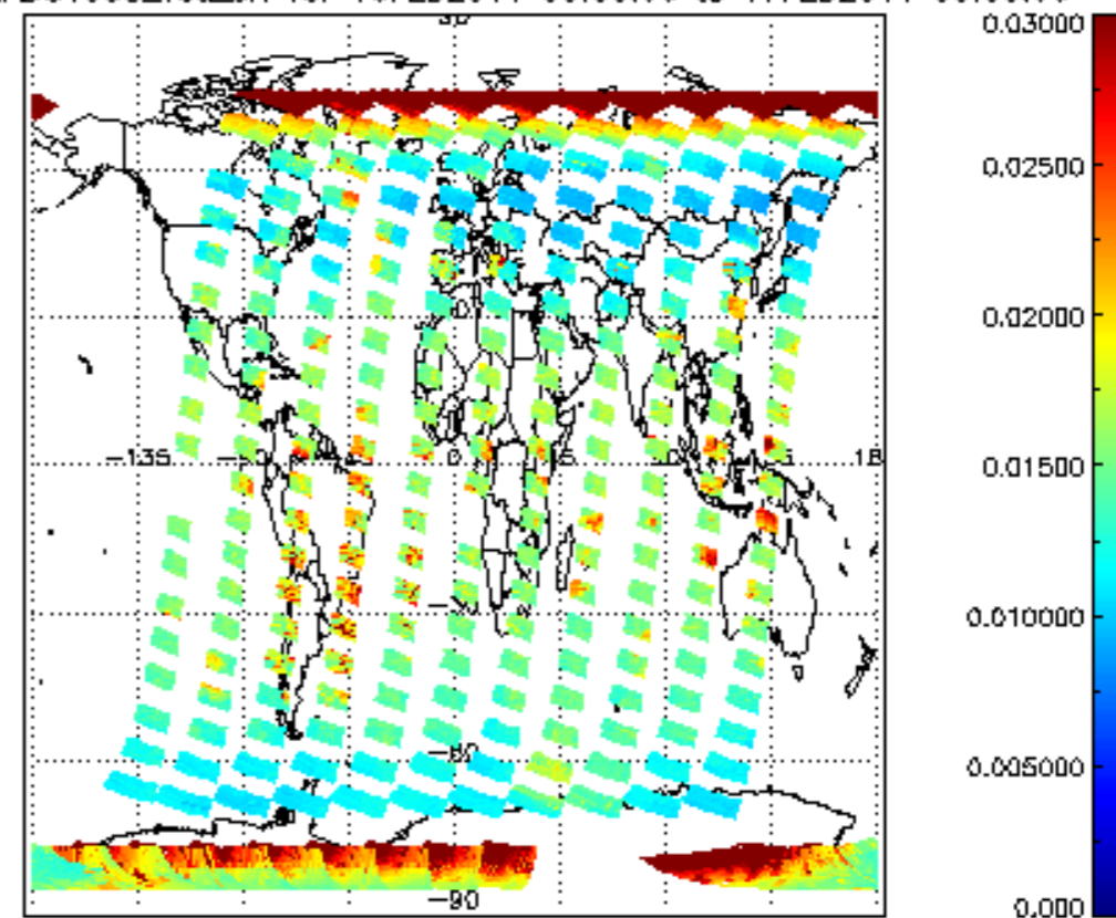
SCIOL2P_NADUV003_vcd_err for 16FEB2011 00:00:00 to 17FEB2011 00:00:00
