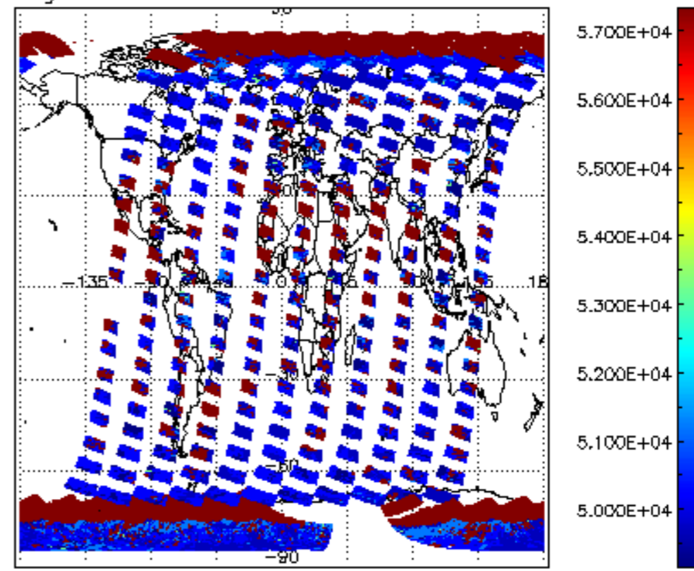
cloud_flags for 16FEB2011 00:00:00 to 17FEB2011 00:00:00
