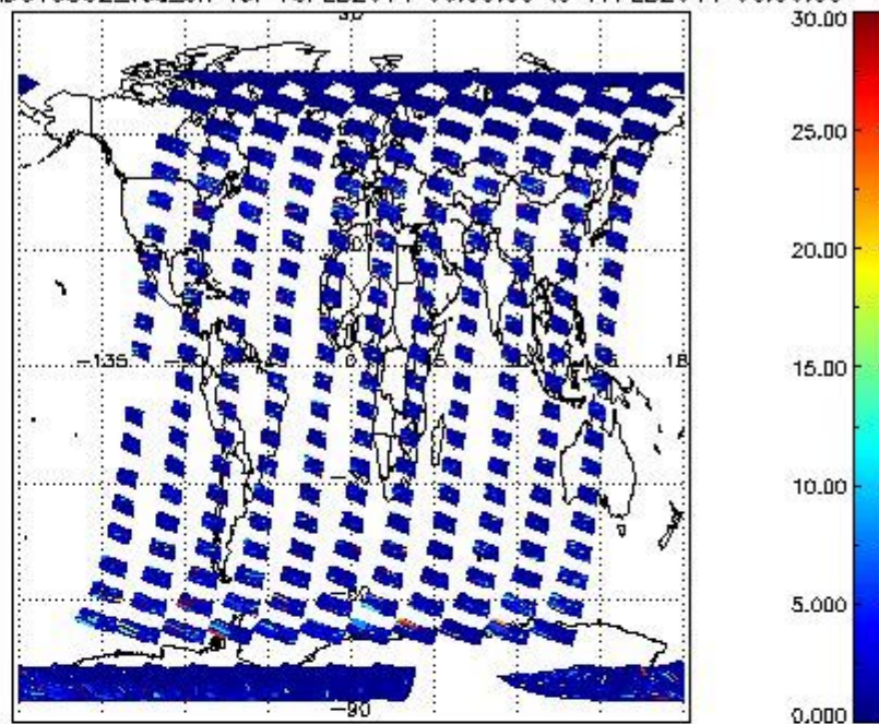
SCIOL2P_NADUV5S02_vcd_err for 16FEB2011 00:00:00 to 17FEB2011 00:00:00
