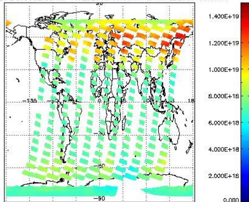
SCIOL2P_NADUV003_vcd for 16FEB2011 00:00:00 to 17FEB2011 00:00:00
