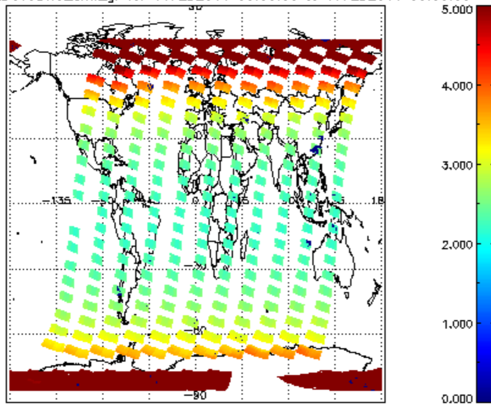
SCIOL2P_NADUV3BRO_amf_gr for 16FEB2011 00:00:00 to 17FEB2011 00:00:00
