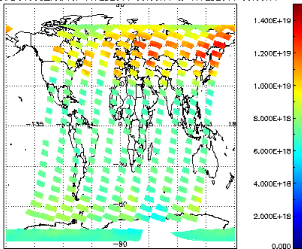
SCIOL2P_NADUV003_vcd for 16FEB2011 00:00:00 to 17FEB2011 00:00:00
