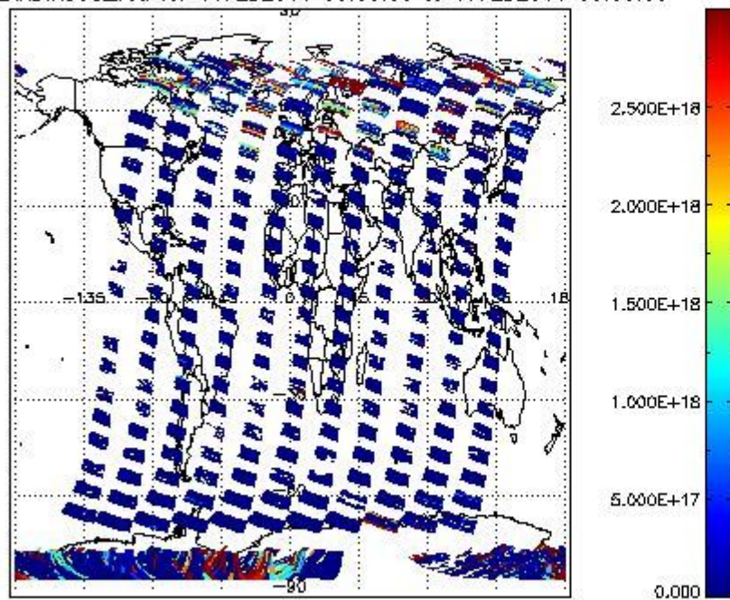
SCIDL2P_NADIR3CO_vcd for 16FEB2011 00:00:00 to 17FEB2011 00:00:00
