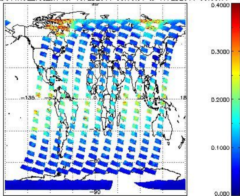
SCIOL2P_NADUV1N02_vcd_err for 16FEB2011 00:00:00 to 17FEB2011 00:00:00
