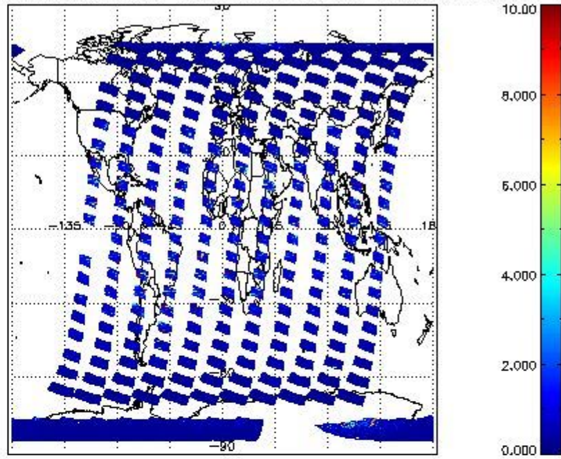
SCIOL2P_NADUV3BRO_vcd_err for 16FEB2011 00:00:00 to 17FEB2011 00:00:00
