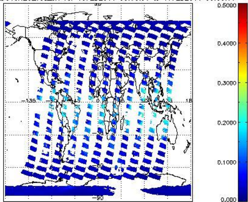
SCIOL2P_NADUV8H2O_vcd_err for 16FEB2011 00:00:00 to 17FEB2011 00:00:00
