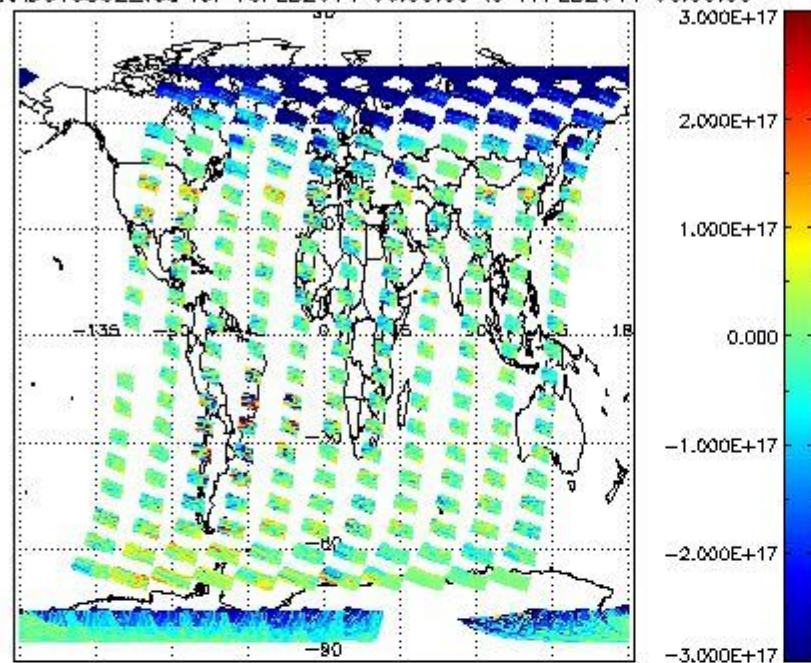
SCIOL2P_NADUV5S02_vcd for 16FEB2011 00:00:00 to 17FEB2011 00:00:00
