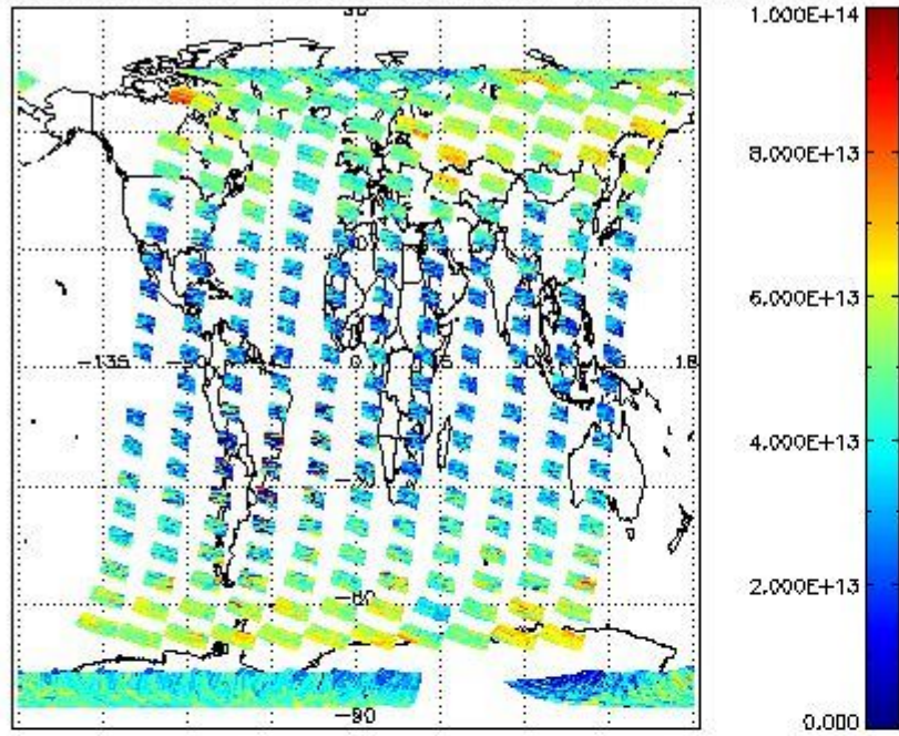
SCIOL2P_NADUV3BRO_vcd for 16FEB2011 00:00:00 to 17FEB2011 00:00:00
