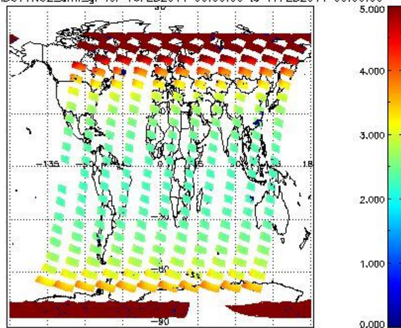
SCIOL2P_NADUV1N02_amf_gr for 16FEB2011 00:00:00 to 17FEB2011 00:00:00
