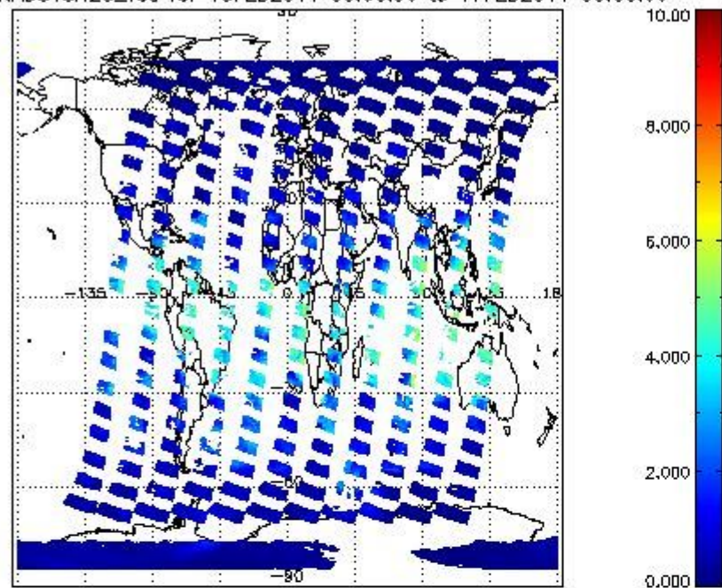
SCIOL2P_NADUV8H2O_vcd for 16FEB2011 00:00:00 to 17FEB2011 00:00:00
