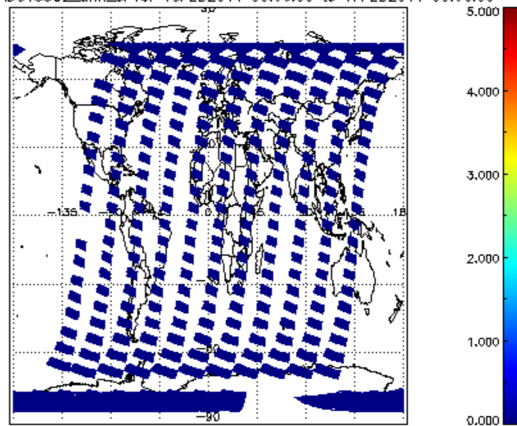
SCIOL2P_NADUV5S02_amf_cl for 16FEB2011 00:00:00 to 17FEB2011 00:00:00
