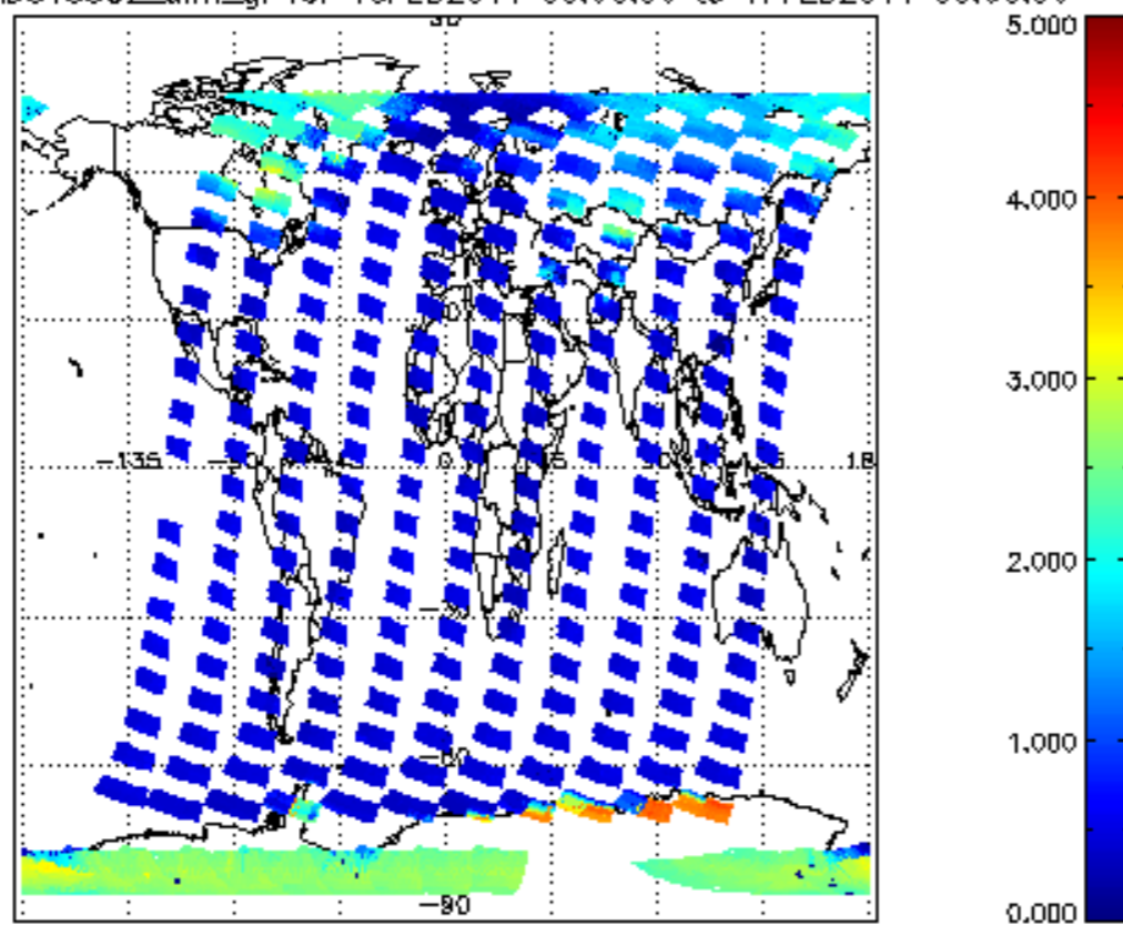
SCIOL2P_NADUV5S02_amf_gr for 16FEB2011 00:00:00 to 17FEB2011 00:00:00
