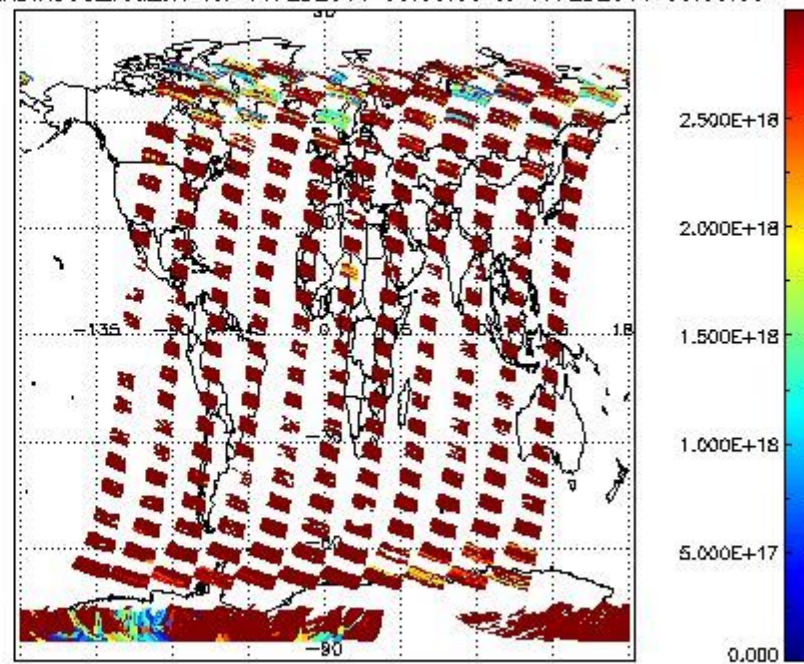
SCIDL2P_NADIR3CO_vcd_err for 16FEB2011 00:00:00 to 17FEB2011 00:00:00
