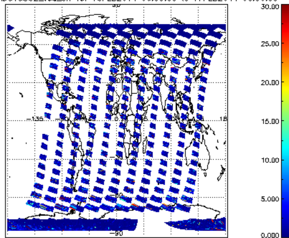
SCIOL2P_NADUV5S02_vcd_err for 16FEB2011 00:00:00 to 17FEB2011 00:00:00
