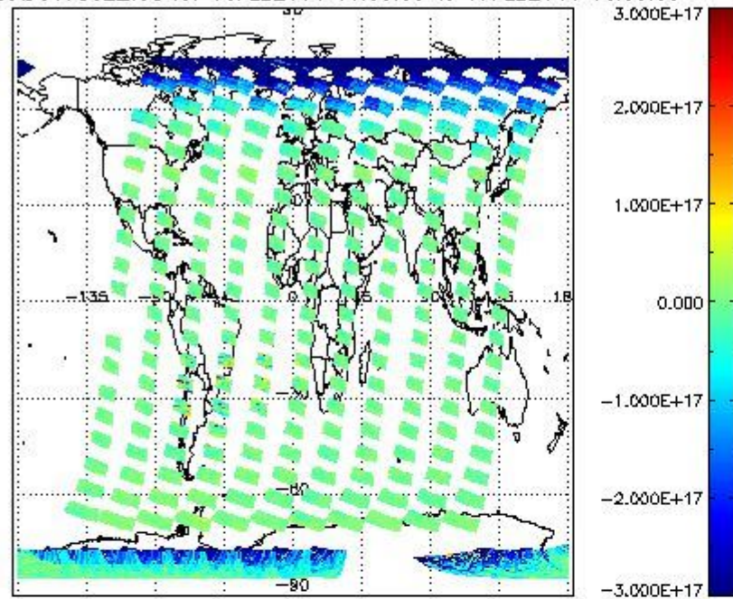
SCIOL2P_NADUV7S02_vcd for 16FEB2011 00:00:00 to 17FEB2011 00:00:00
