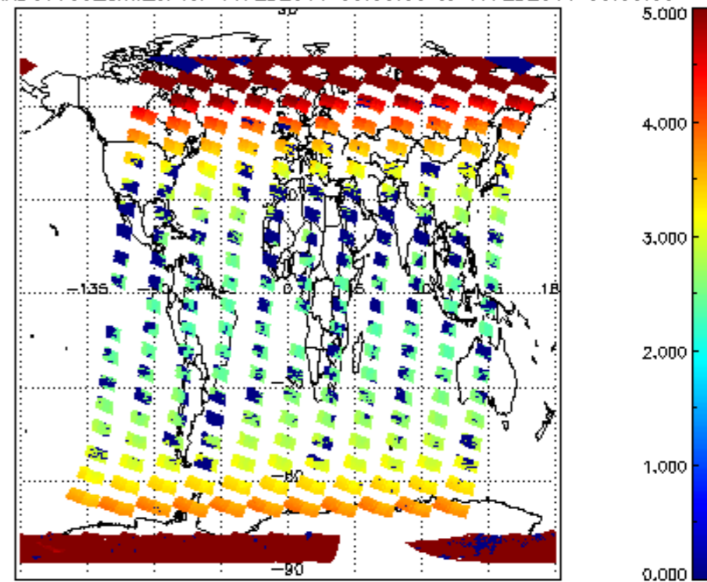
SCIOL2P_NADUV003_amf_cl for 16FEB2011 00:00:00 to 17FEB2011 00:00:00
