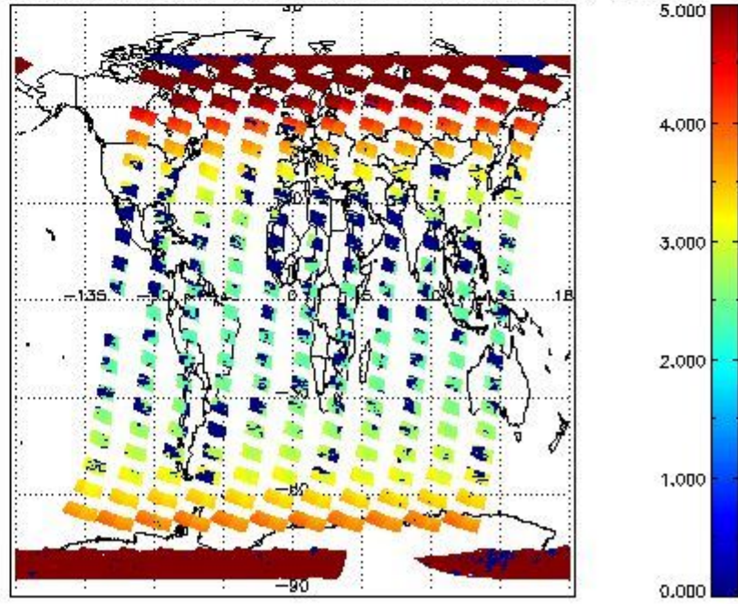
SCIOL2P_NADUV3BRO_amf_cl for 16FEB2011 00:00:00 to 17FEB2011 00:00:00
