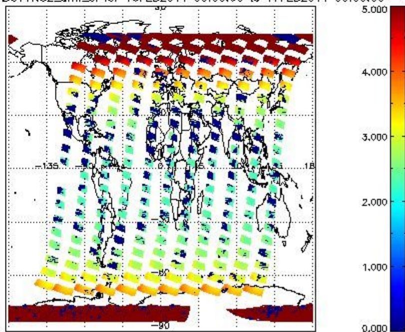
SCIOL2P_NADUV1N02_amf_cl for 16FEB2011 00:00:00 to 17FEB2011 00:00:00
