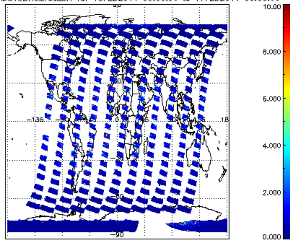
SCIOL2P_NADUV3BRO_vcd_err for 16FEB2011 00:00:00 to 17FEB2011 00:00:00
