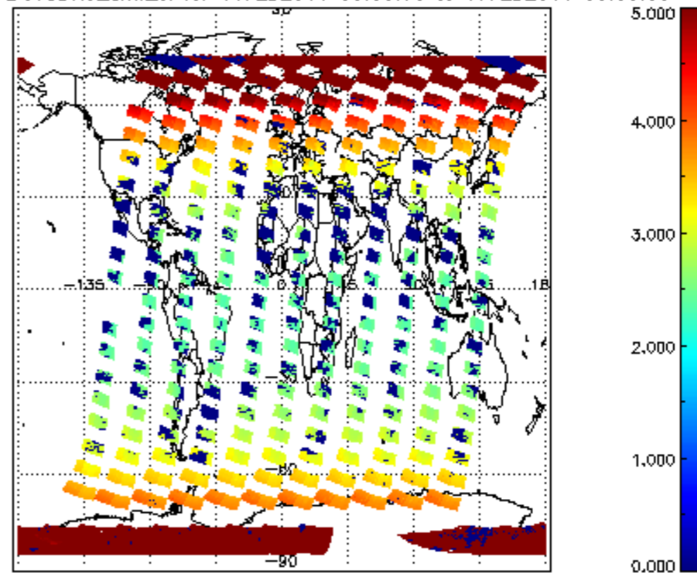
SCIOL2P_NADUV3BRO_amf_cl for 16FEB2011 00:00:00 to 17FEB2011 00:00:00
