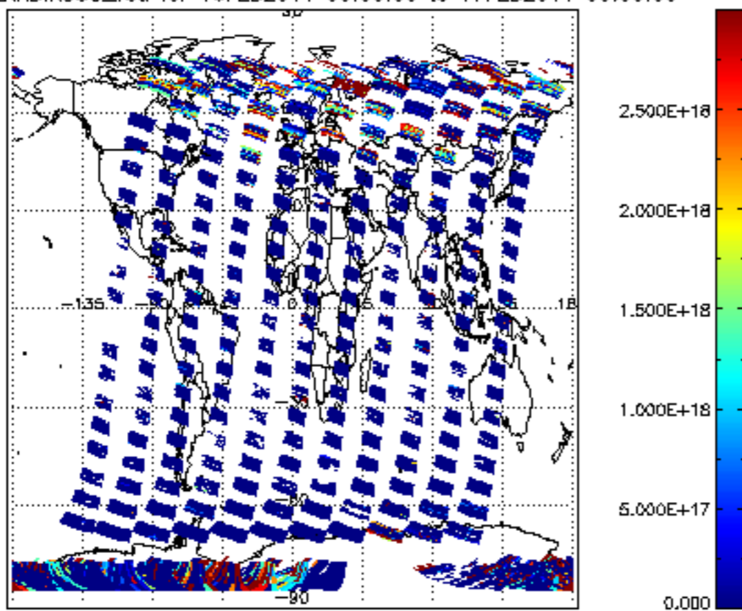
SCIOL2P_NADIR3CO_vcd for 16FEB2011 00:00:00 to 17FEB2011 00:00:00
