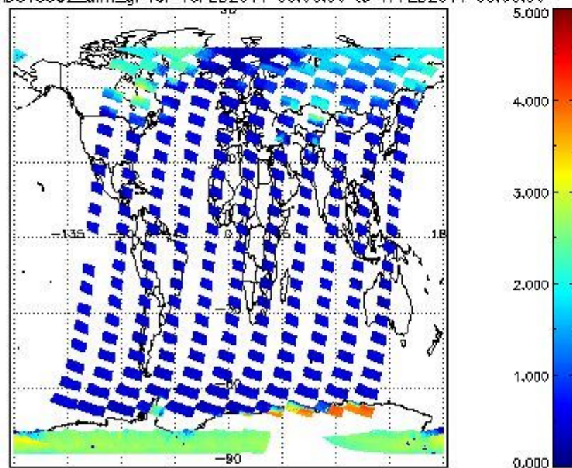
SCIOL2P_NADUV5S02_amf_gr for 16FEB2011 00:00:00 to 17FEB2011 00:00:00
