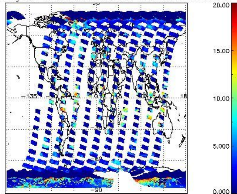
cL_top_height for 16FEB2011 00:00:00 to 17FEB2011 00:00:00
