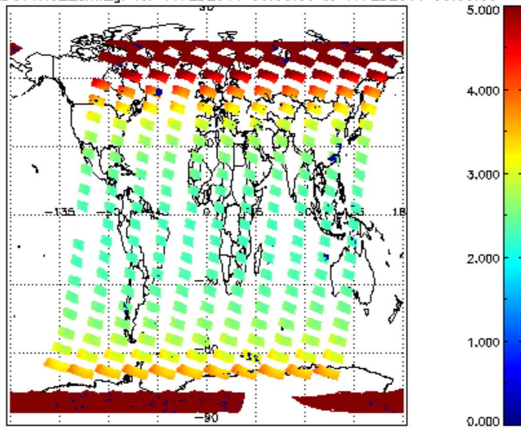
SCIOL2P_NADUV1N02_amf_gr for 16FEB2011 00:00:00 to 17FEB2011 00:00:00
