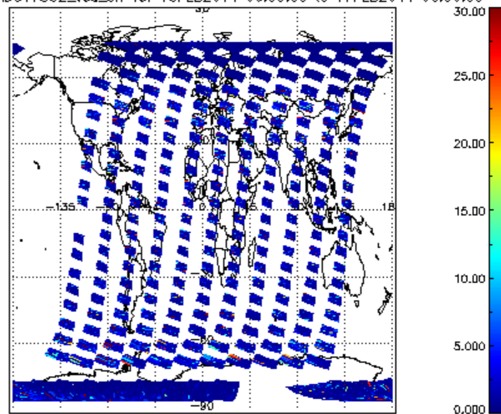
SCIOL2P_NADUV7S02_vcd_err for 16FEB2011 00:00:00 to 17FEB2011 00:00:00
