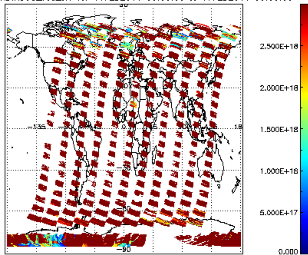
SCIOL2P_NADIR3CO_vcd_err for 16FEB2011 00:00:00 to 17FEB2011 00:00:00
