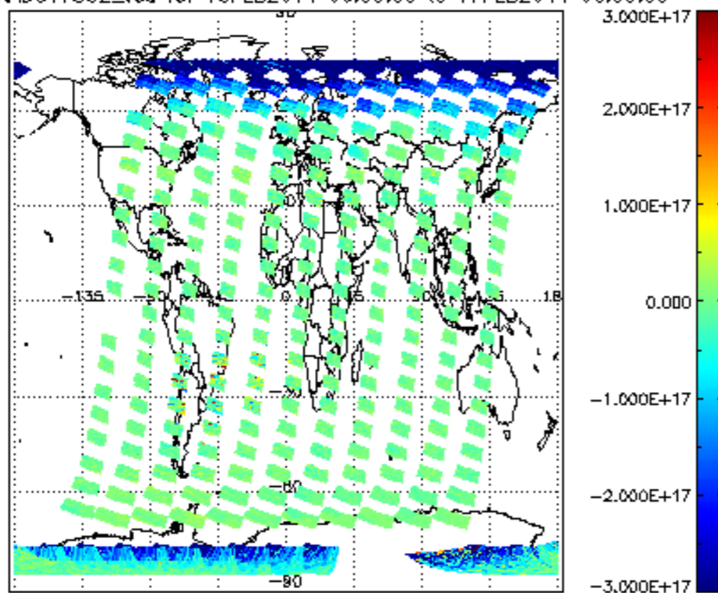
SCIOL2P_NADUV7S02_vcd for 16FEB2011 00:00:00 to 17FEB2011 00:00:00
