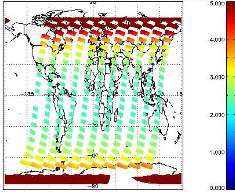
SCIOL2P_NADUV3BRO_amf_gr for 16FEB2011 00:00:00 to 17FEB2011 00:00:00
