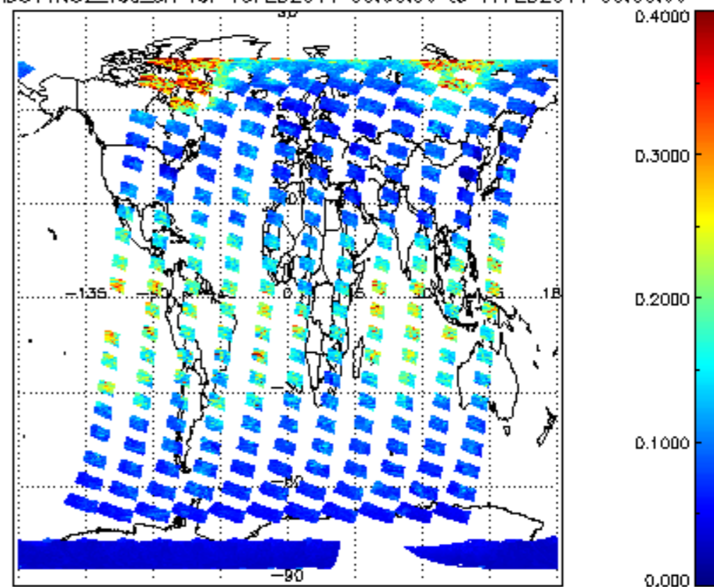
SCIOL2P_NADUV1N02_vcd_err for 16FEB2011 00:00:00 to 17FEB2011 00:00:00
