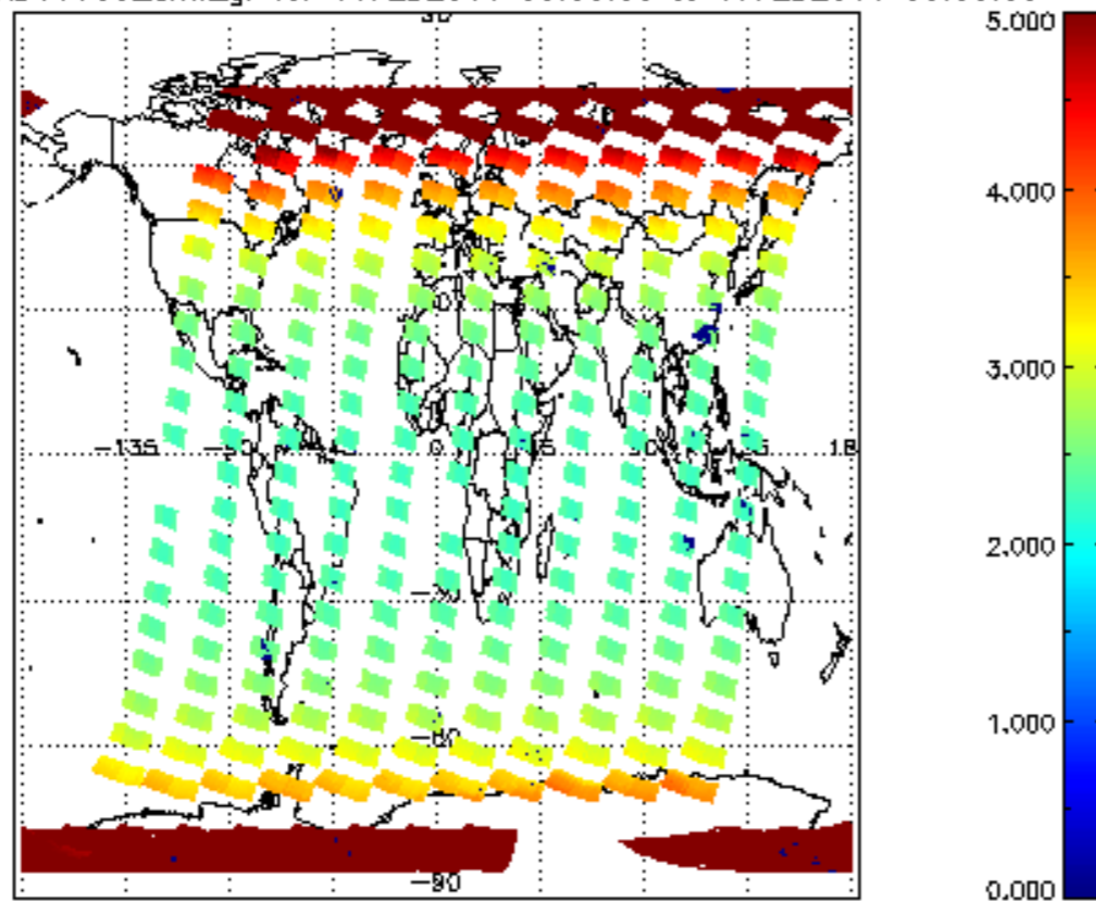
SCIOL2P_NADUV003_amf_gr for 16FEB2011 00:00:00 to 17FEB2011 00:00:00
