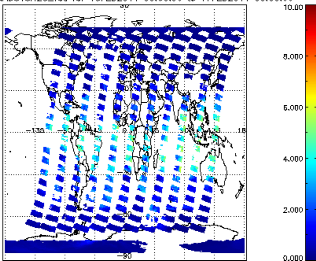
SCIOL2P_NADUV8H2O_vcd for 16FEB2011 00:00:00 to 17FEB2011 00:00:00
