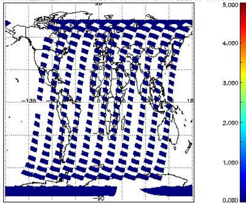
SCIOL2P_NADUV7S02_amf_cl for 16FEB2011 00:00:00 to 17FEB2011 00:00:00
