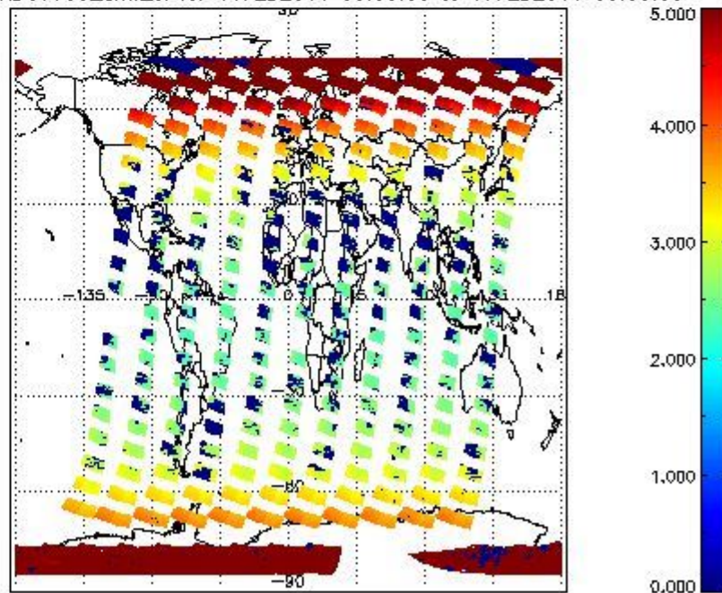
SCIOL2P_NADUV003_amf_cl for 16FEB2011 00:00:00 to 17FEB2011 00:00:00
