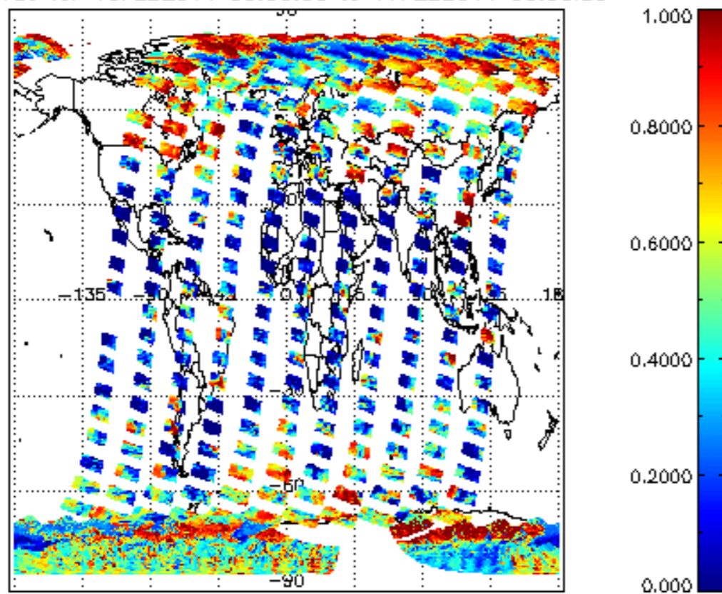
cL_frac for 16FEB2011 00:00:00 to 17FEB2011 00:00:00
