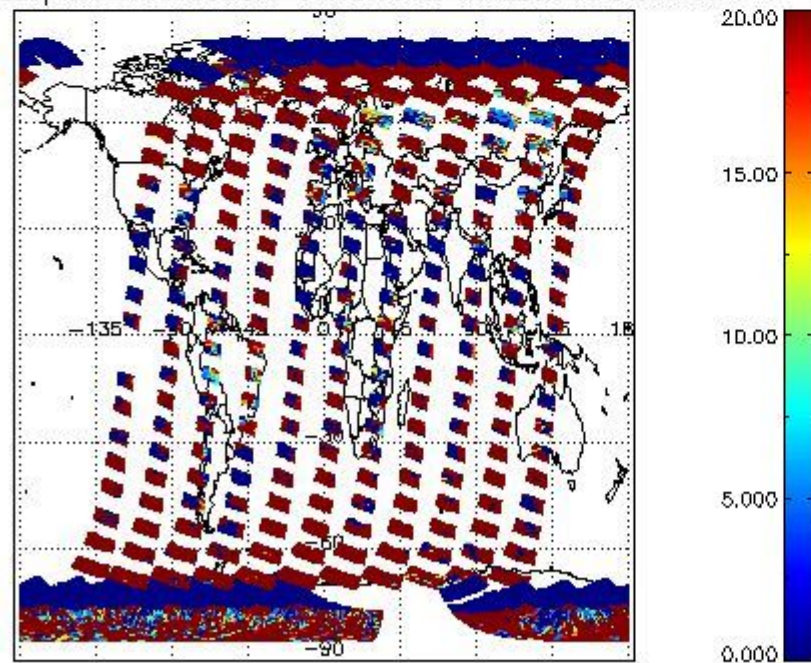
cL_opt_depth for 16FEB2011 00:00:00 to 17FEB2011 00:00:00
