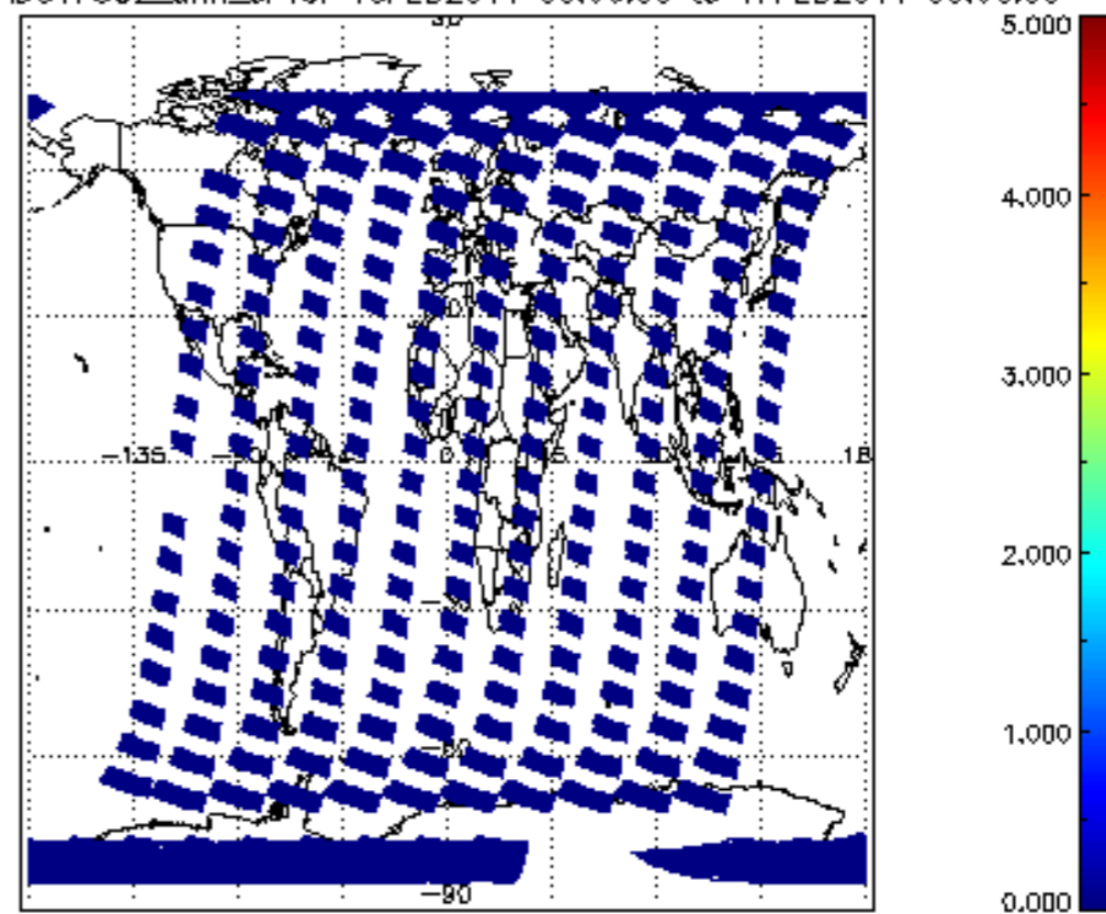
SCIOL2P_NADUV7S02_amf_cl for 16FEB2011 00:00:00 to 17FEB2011 00:00:00
