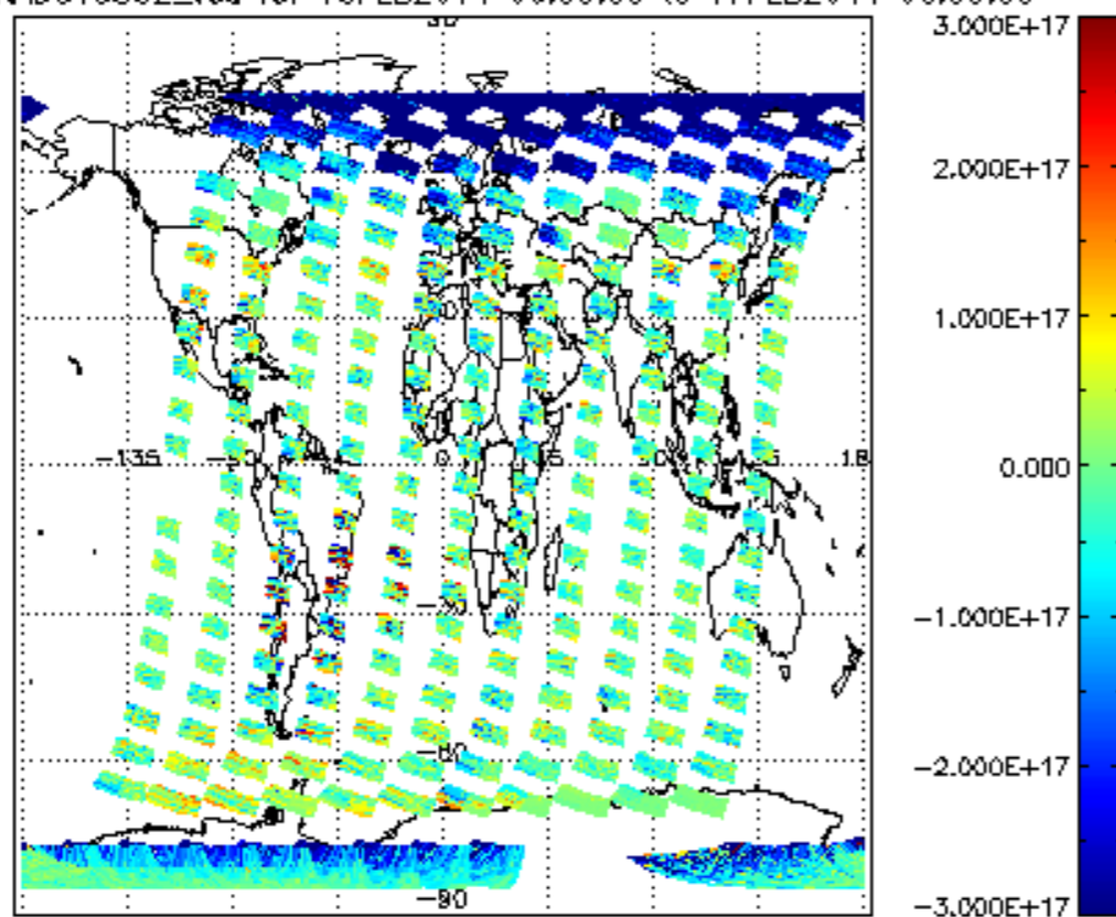
SCIOL2P_NADUV5S02_vcd for 16FEB2011 00:00:00 to 17FEB2011 00:00:00
