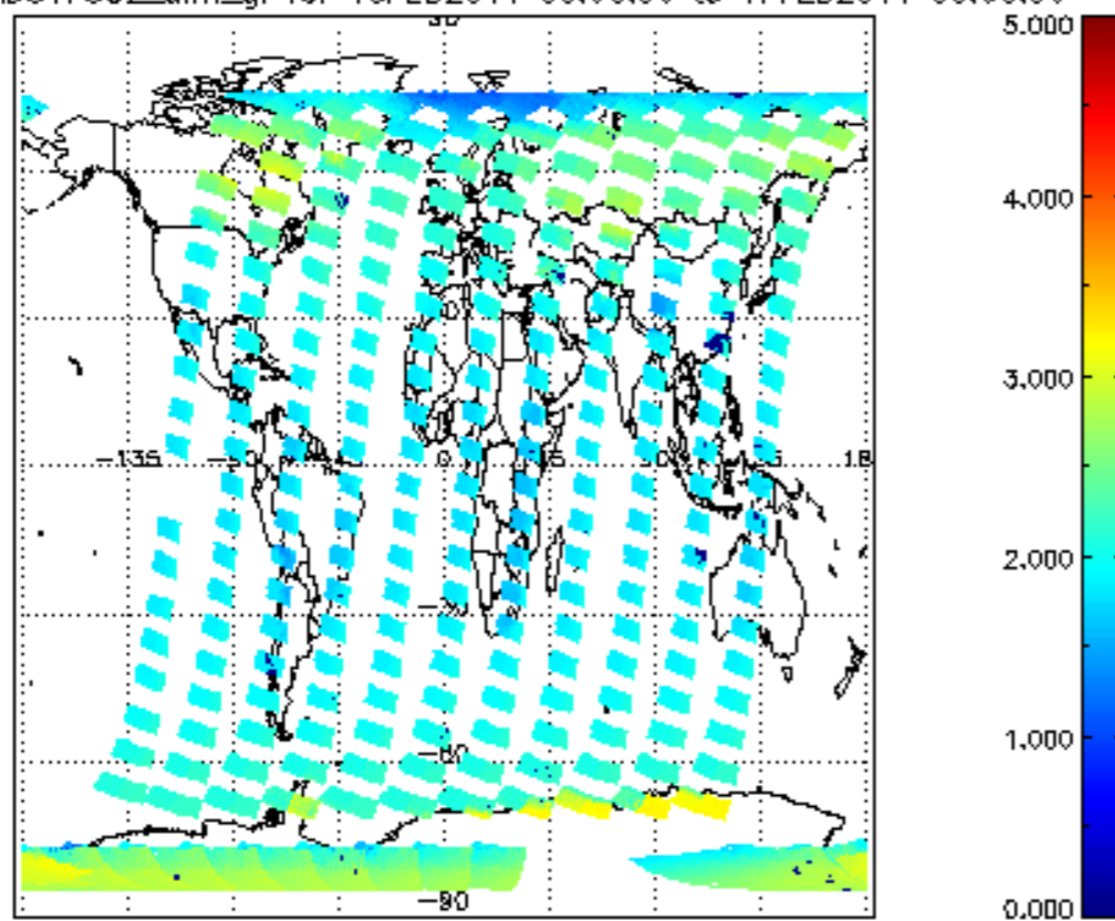
SCIOL2P_NADUV7S02_amf_gr for 16FEB2011 00:00:00 to 17FEB2011 00:00:00
