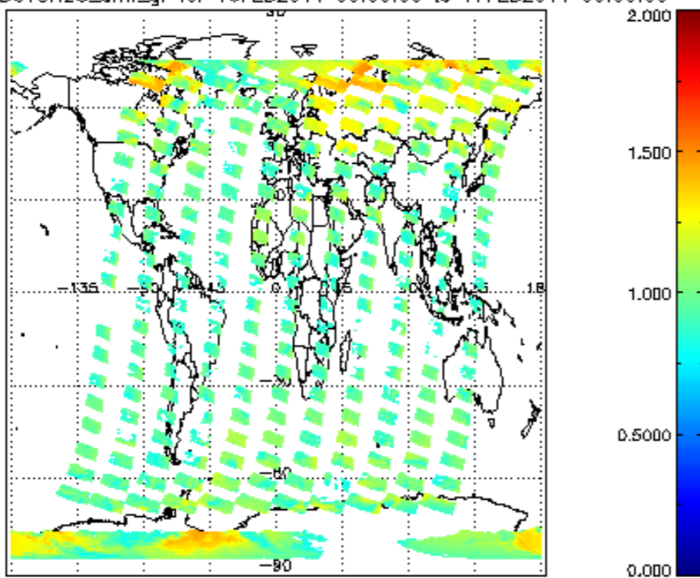
SCIOL2P_NADUV8H2O_amf_gr for 16FEB2011 00:00:00 to 17FEB2011 00:00:00
