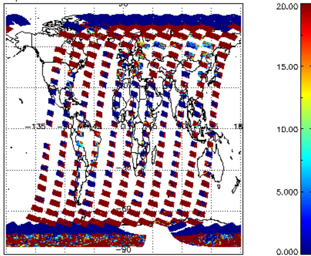
cL_opt_depth for 16FEB2011 00:00:00 to 17FEB2011 00:00:00
