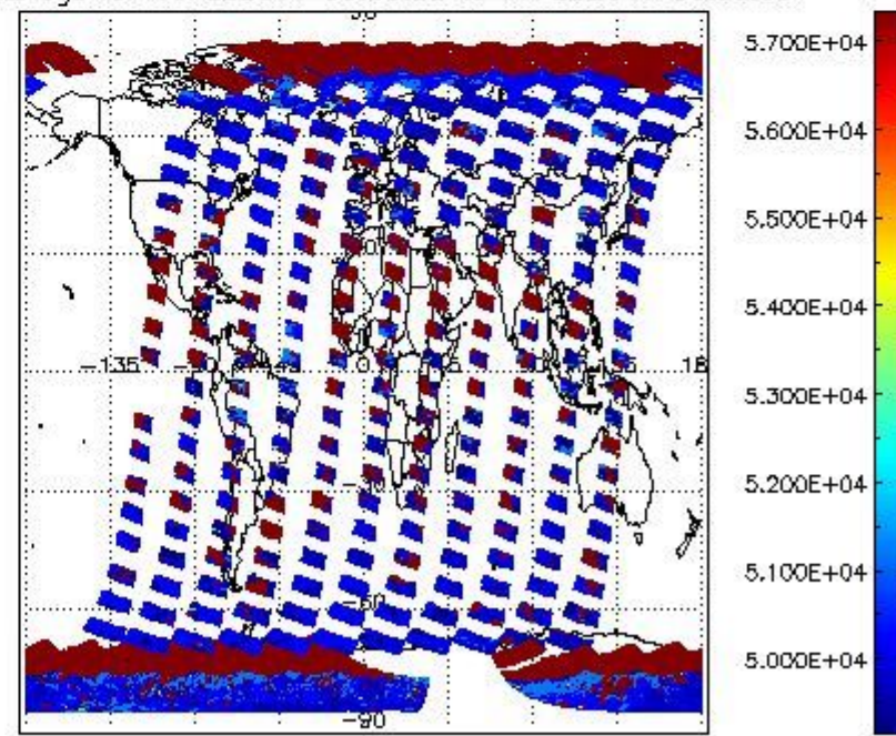
cloud_flags for 16FEB2011 00:00:00 to 17FEB2011 00:00:00
