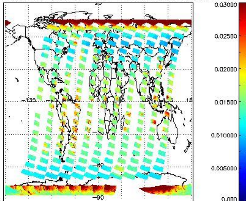
SCIOL2P_NADUV003_vcd_err for 16FEB2011 00:00:00 to 17FEB2011 00:00:00
