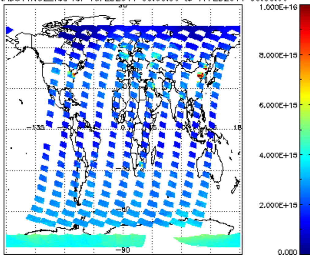
SCIOL2P_NADUV1N02_vcd for 16FEB2011 00:00:00 to 17FEB2011 00:00:00
