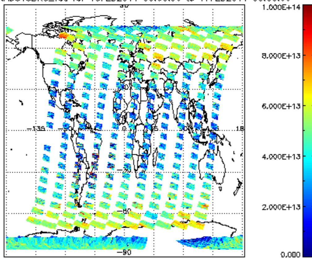
SCIOL2P_NADUV3BRO_vcd for 16FEB2011 00:00:00 to 17FEB2011 00:00:00
