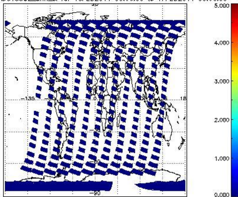
SCIOL2P_NADUV5S02_amf_cl for 16FEB2011 00:00:00 to 17FEB2011 00:00:00
