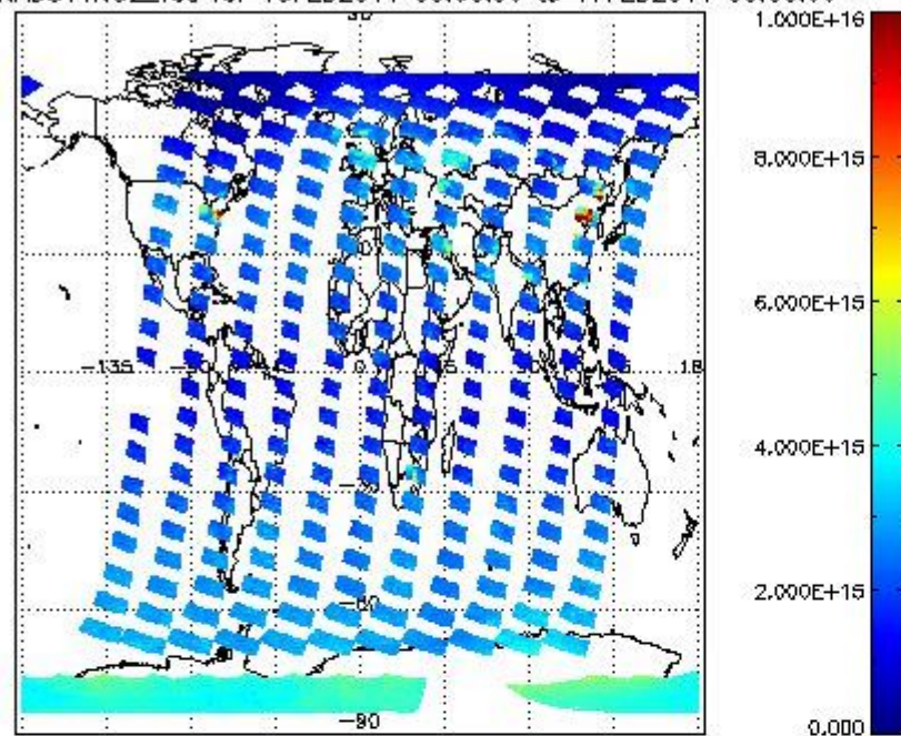
SCIOL2P_NADUV1N02_vcd for 16FEB2011 00:00:00 to 17FEB2011 00:00:00
