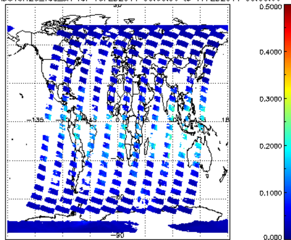
SCIOL2P_NADUV8H2O_vcd_err for 16FEB2011 00:00:00 to 17FEB2011 00:00:00
