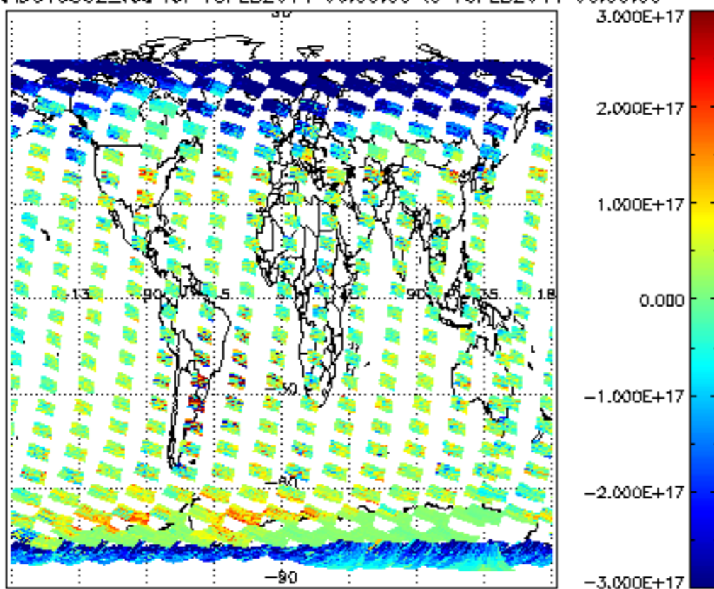
SCIOL2P_NADUV5S02_vcd for 15FEB2011 00:00:00 to 16FEB2011 00:00:00
