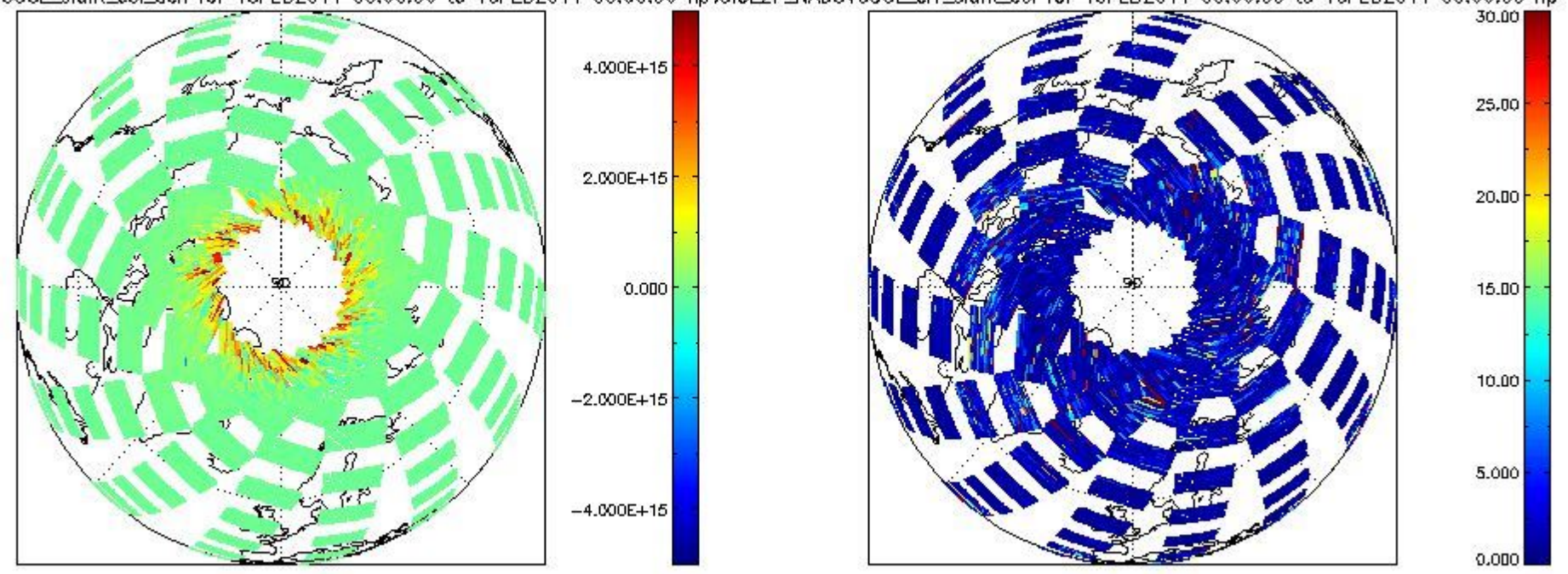
CIOL2P_NADUV60CL_slant_col_den for 15FEB2011 00:00:00 to 16FEB2011 00:00:00 np; CIOL2P_NADUV60CL_err_slant_col for 15FEB2011 00:00:00 to 16FEB2011 00:00:00 np
