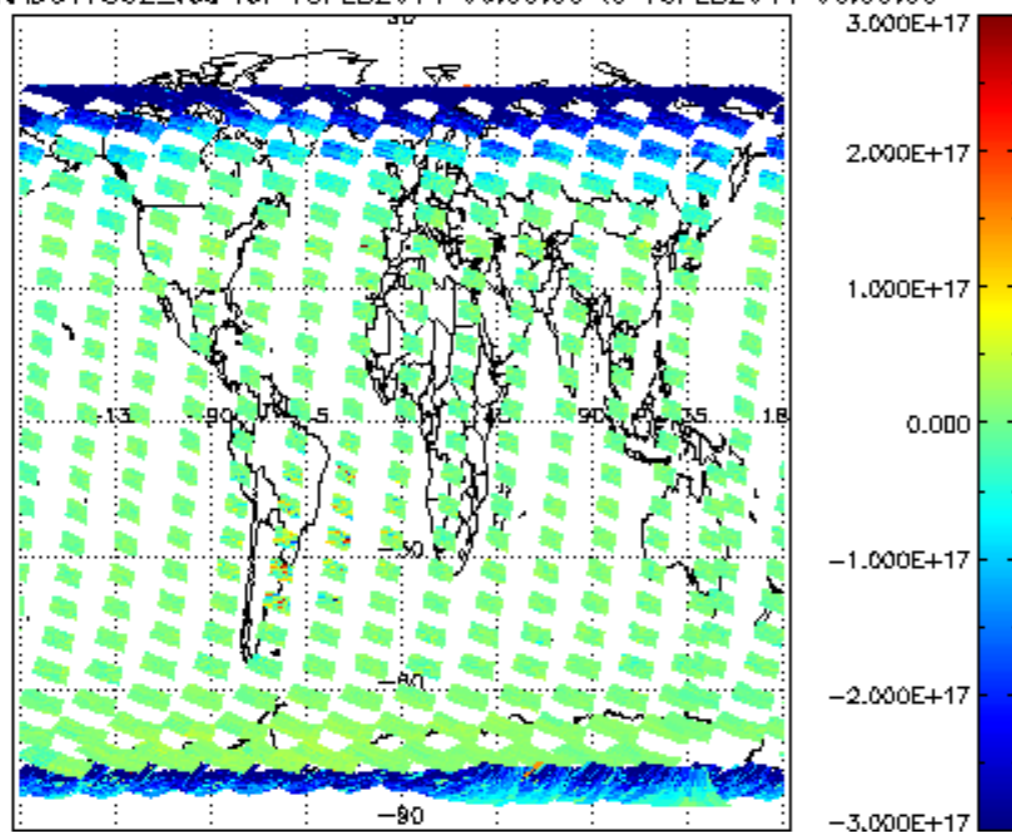
SCIOL2P_NADUV7S02_vcd for 15FEB2011 00:00:00 to 16FEB2011 00:00:00
