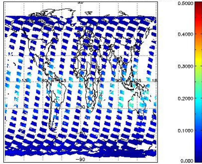
SCIOL2P_NADUV8H2O_vcd_err for 15FEB2011 00:00:00 to 16FEB2011 00:00:00
