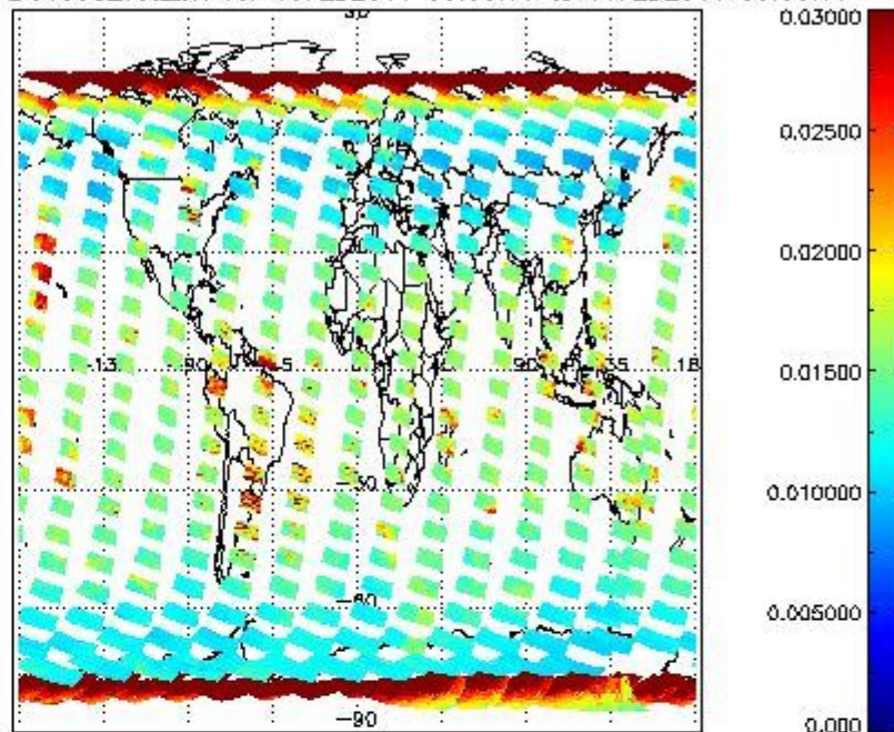
SCIOL2P_NADUV003_vcd_err for 15FEB2011 00:00:00 to 16FEB2011 00:00:00
