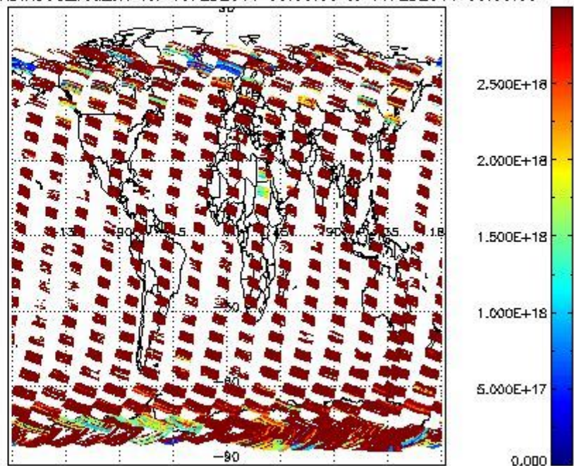
SCIDL2P_NADIR3CO_vcd_err for 15FEB2011 00:00:00 to 16FEB2011 00:00:00
