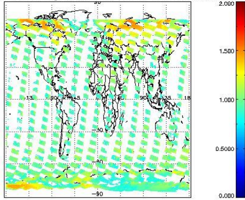
SCIOL2P_NADUV8H2O_amf_gr for 15FEB2011 00:00:00 to 16FEB2011 00:00:00
