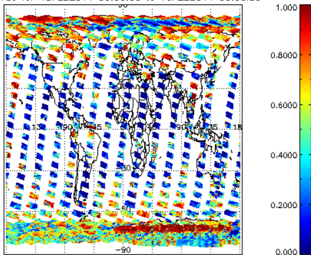
cI_frac for 15FEB2011 00:00:00 to 16FEB2011 00:00:00
