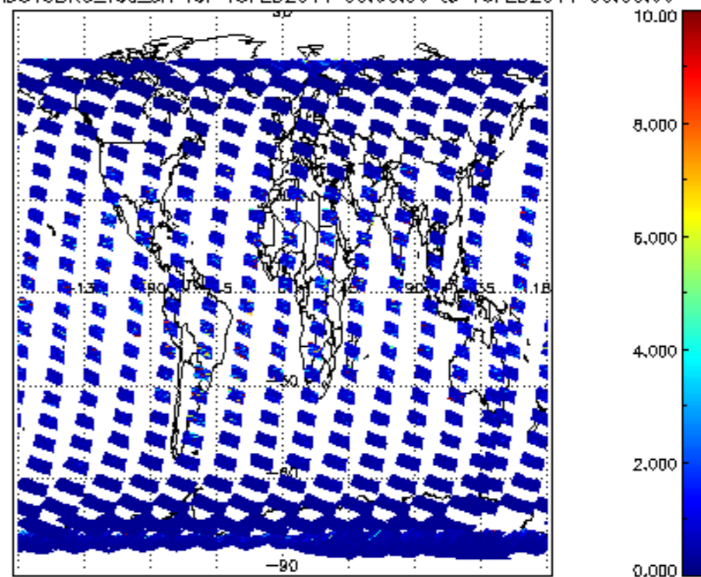
SCIOL2P_NADUV3BRO_vcd_err for 15FEB2011 00:00:00 to 16FEB2011 00:00:00
