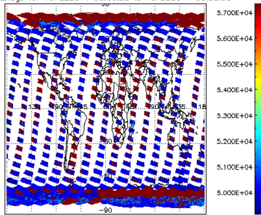
cloud_flags for 15FEB2011 00:00:00 to 16FEB2011 00:00:00
