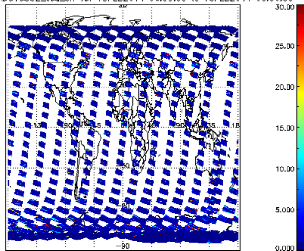
SCIOL2P_NADUV5S02_vcd_err for 15FEB2011 00:00:00 to 16FEB2011 00:00:00
