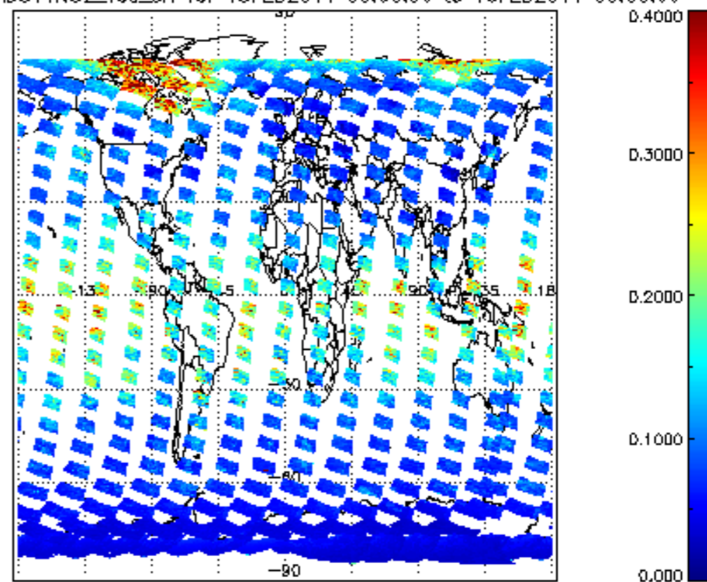
SCIOL2P_NADUV1N02_vcd_err for 15FEB2011 00:00:00 to 16FEB2011 00:00:00
