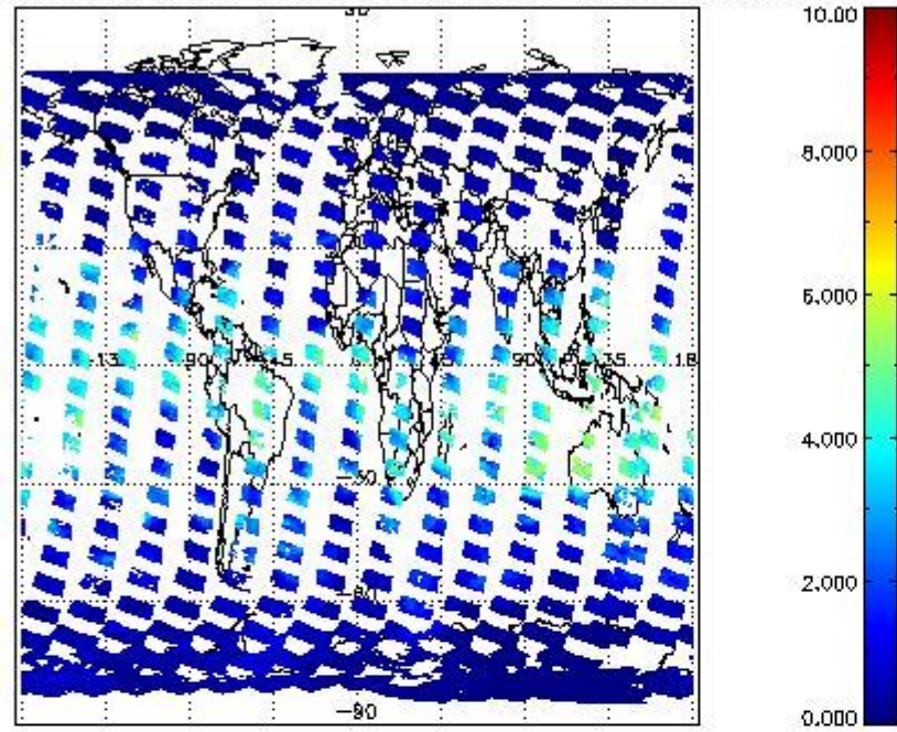
SCIOL2P_NADUV8H2O_vcd for 15FEB2011 00:00:00 to 16FEB2011 00:00:00
