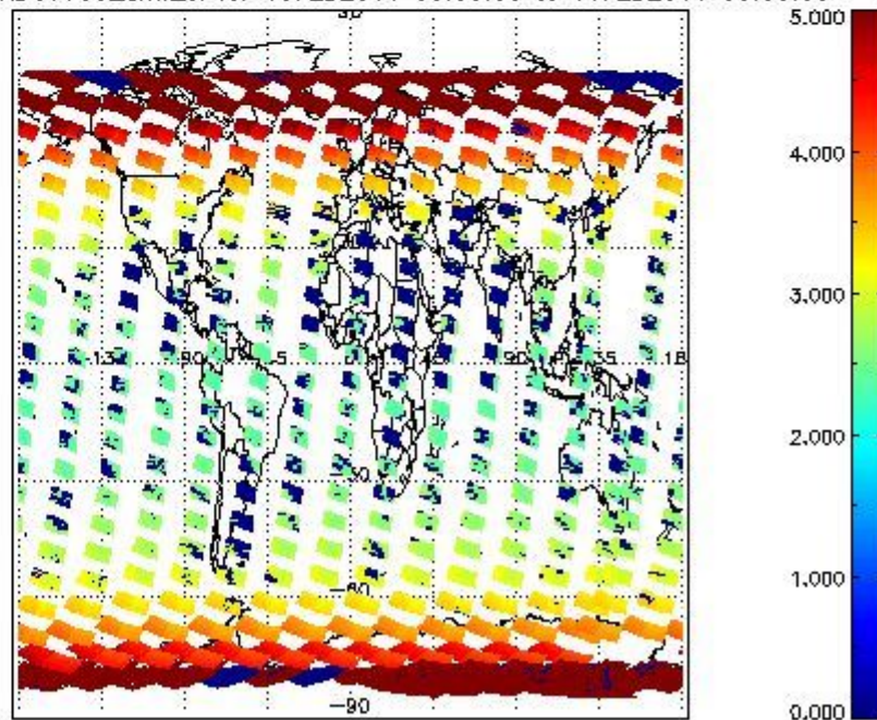
SCIOL2P_NADUV003_amf_cl for 15FEB2011 00:00:00 to 16FEB2011 00:00:00
