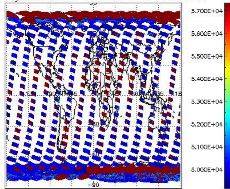
cloud_flags for 15FEB2011 00:00:00 to 16FEB2011 00:00:00
