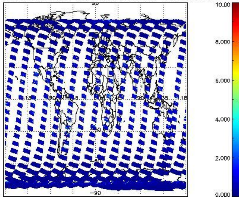
SCIOL2P_NADUV3BRO_vcd_err for 15FEB2011 00:00:00 to 16FEB2011 00:00:00
