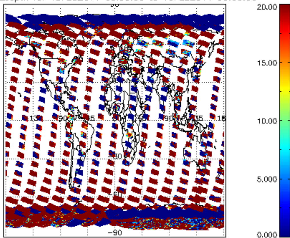
cI_opt_depth for 15FEB2011 00:00:00 to 16FEB2011 00:00:00
