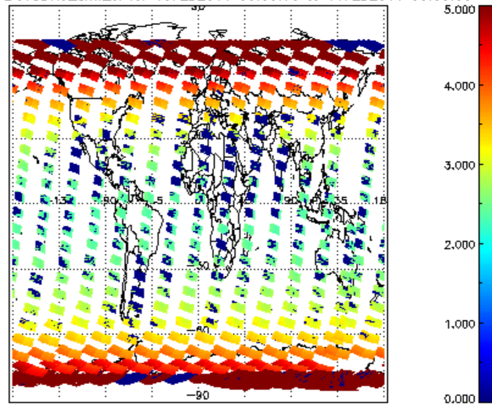
SCIOL2P_NADUV3BRO_amf_cl for 15FEB2011 00:00:00 to 16FEB2011 00:00:00
