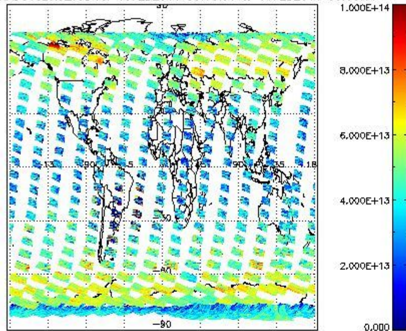
SCIOL2P_NADUV3BRO_vcd for 15FEB2011 00:00:00 to 16FEB2011 00:00:00
