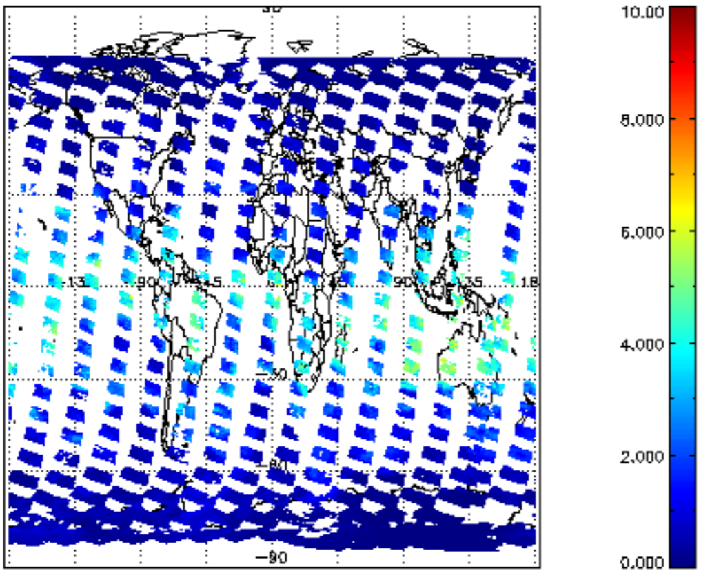
SCIOL2P_NADUV8H20_vcd for 15FEB2011 00:00:00 to 16FEB2011 00:00:00
