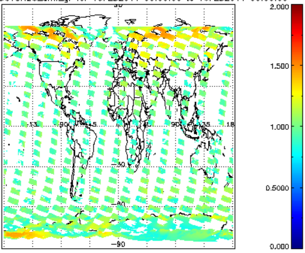
SCIOL2P_NADUV8H20_amf_gr for 15FEB2011 00:00:00 to 16FEB2011 00:00:00
