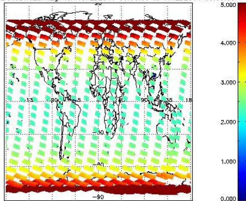
SCIOL2P_NADUV3BRO_amf_gr for 15FEB2011 00:00:00 to 16FEB2011 00:00:00
