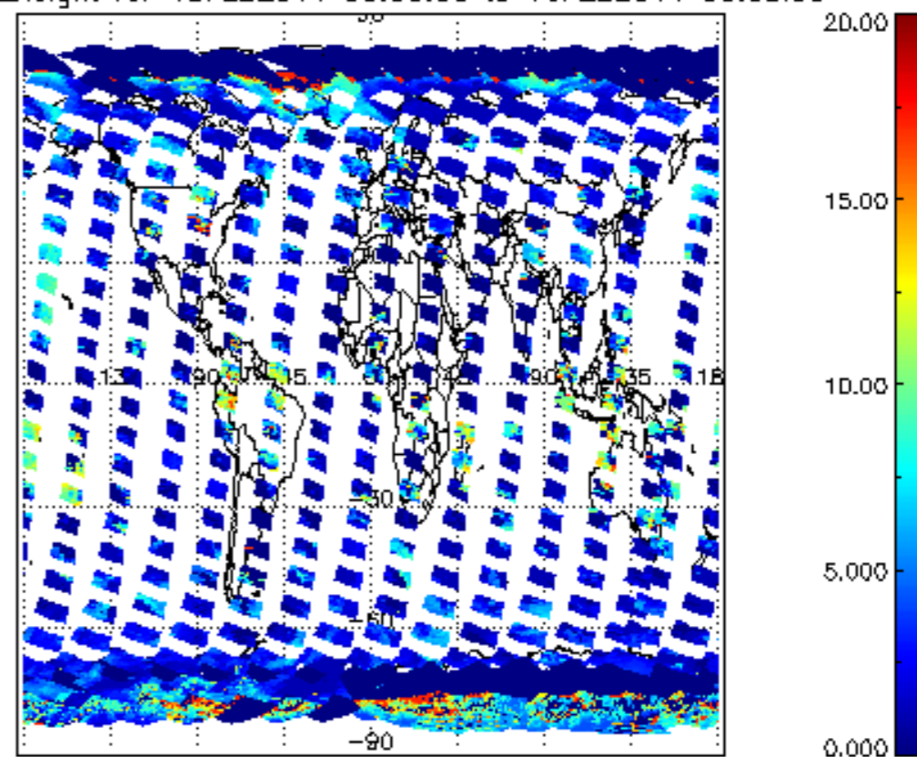
cI_top_height for 15FEB2011 00:00:00 to 16FEB2011 00:00:00
