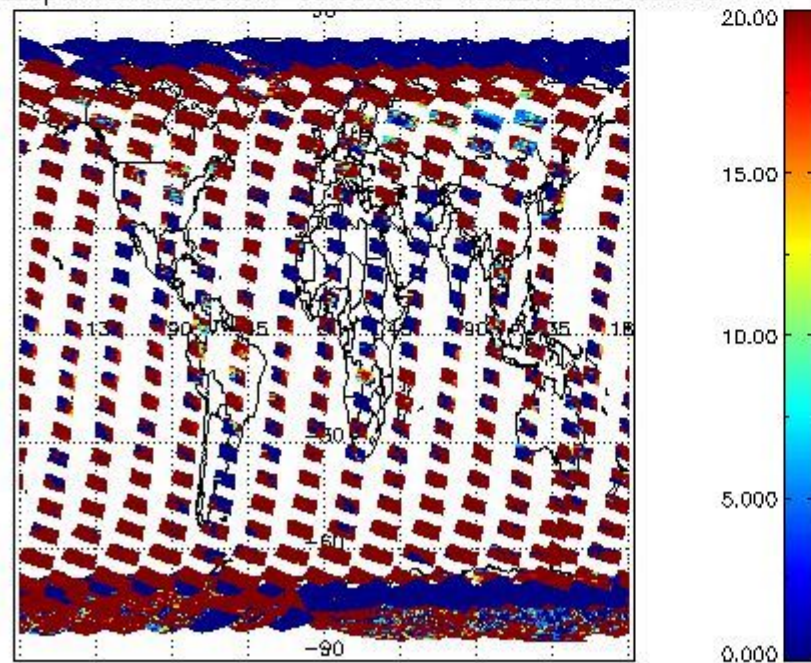
cL_opt_depth for 15FEB2011 00:00:00 to 16FEB2011 00:00:00
