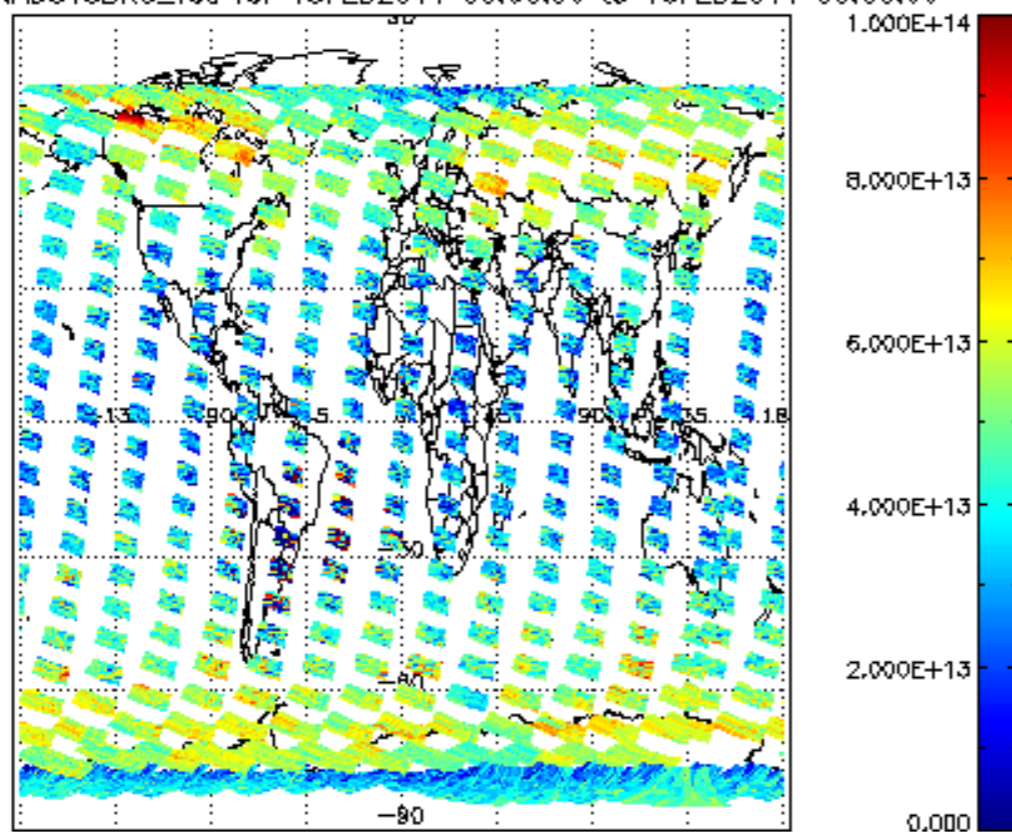
SCIOL2P_NADUV3BRO_vcd for 15FEB2011 00:00:00 to 16FEB2011 00:00:00
