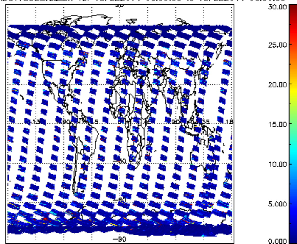
SCIOL2P_NADUV7S02_vcd_err for 15FEB2011 00:00:00 to 16FEB2011 00:00:00
