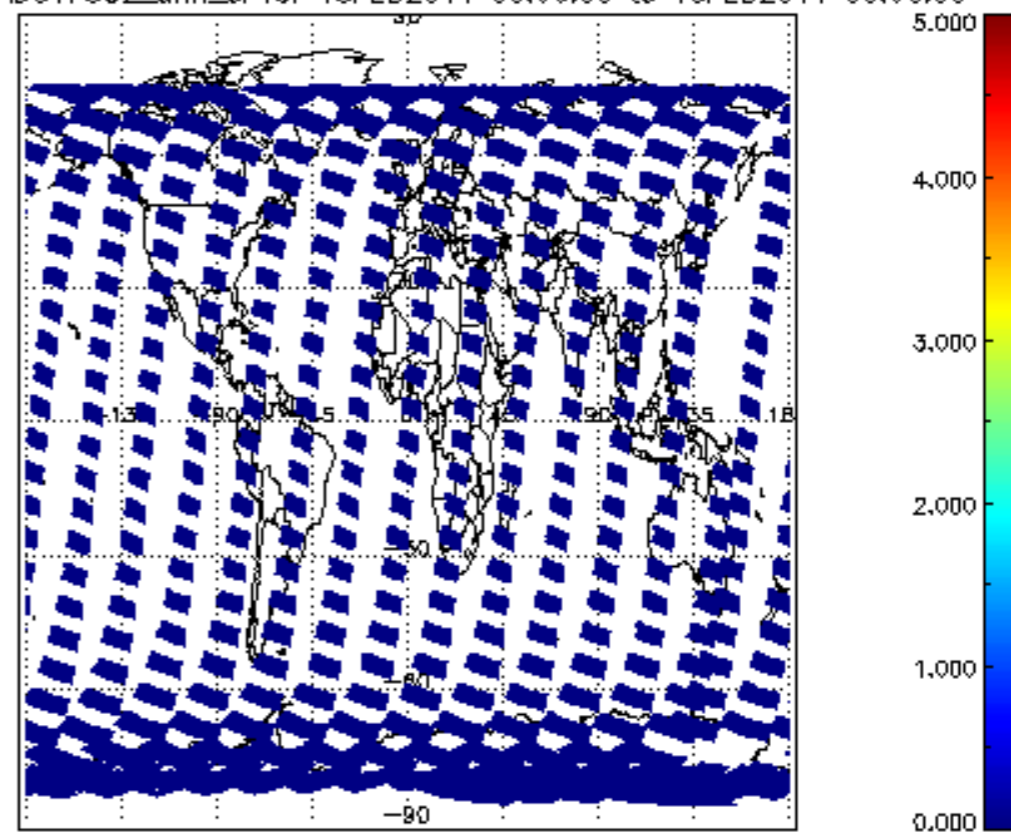
SCIOL2P_NADUV7S02_amf_cl for 15FEB2011 00:00:00 to 16FEB2011 00:00:00
