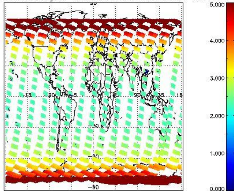
SCIOL2P_NADUV003_amf_gr for 15FEB2011 00:00:00 to 16FEB2011 00:00:00
