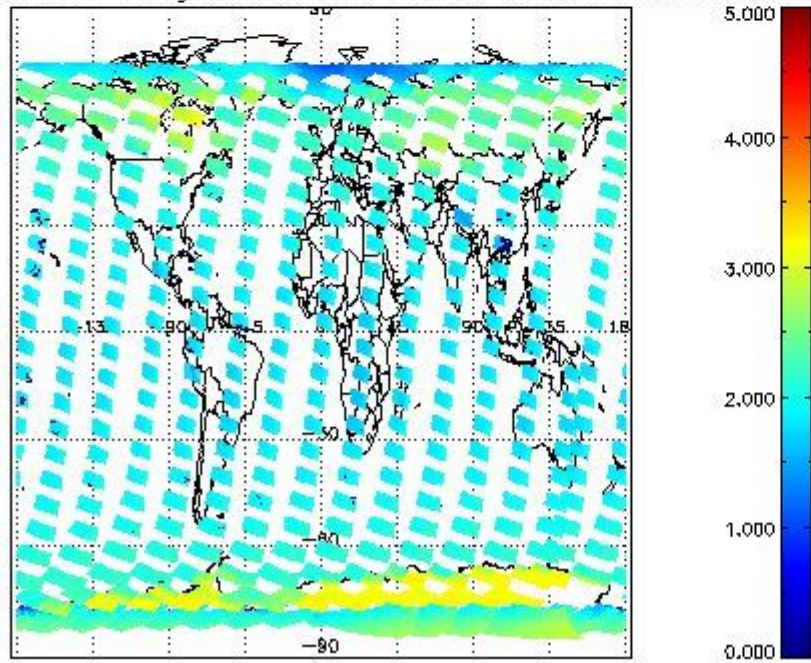
SCIOL2P_NADUV7S02_amf_gr for 15FEB2011 00:00:00 to 16FEB2011 00:00:00
