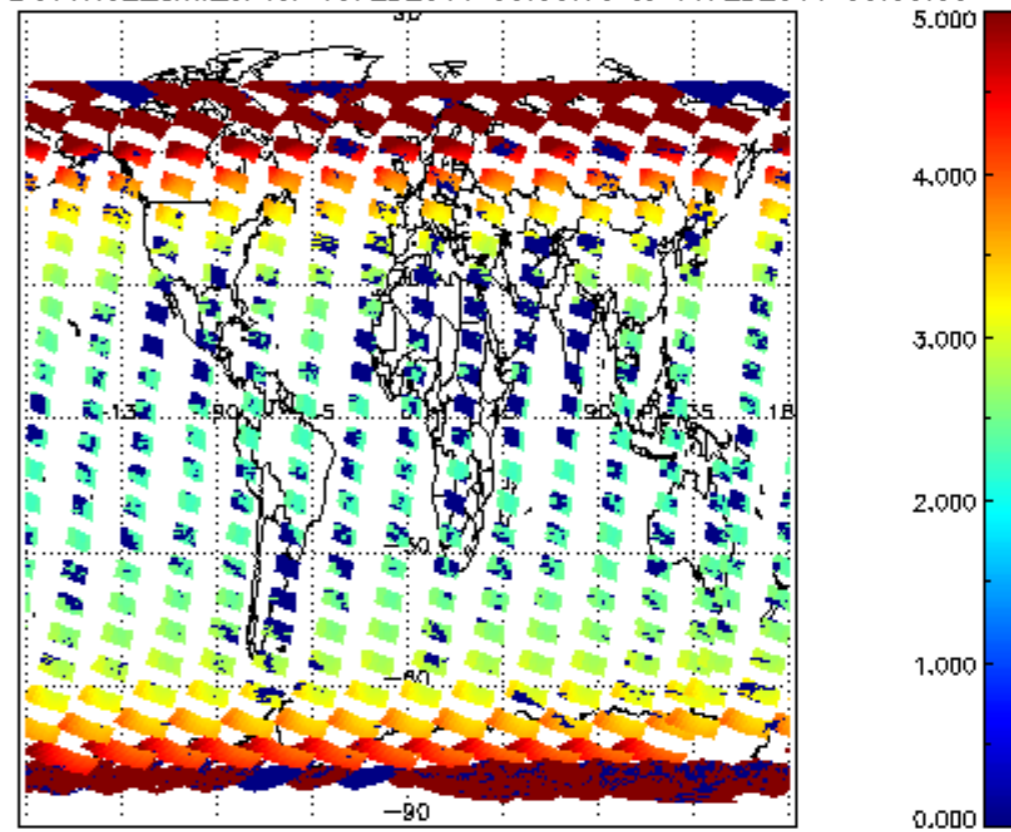
SCIOL2P_NADUV1N02_amf_cl for 15FEB2011 00:00:00 to 16FEB2011 00:00:00
