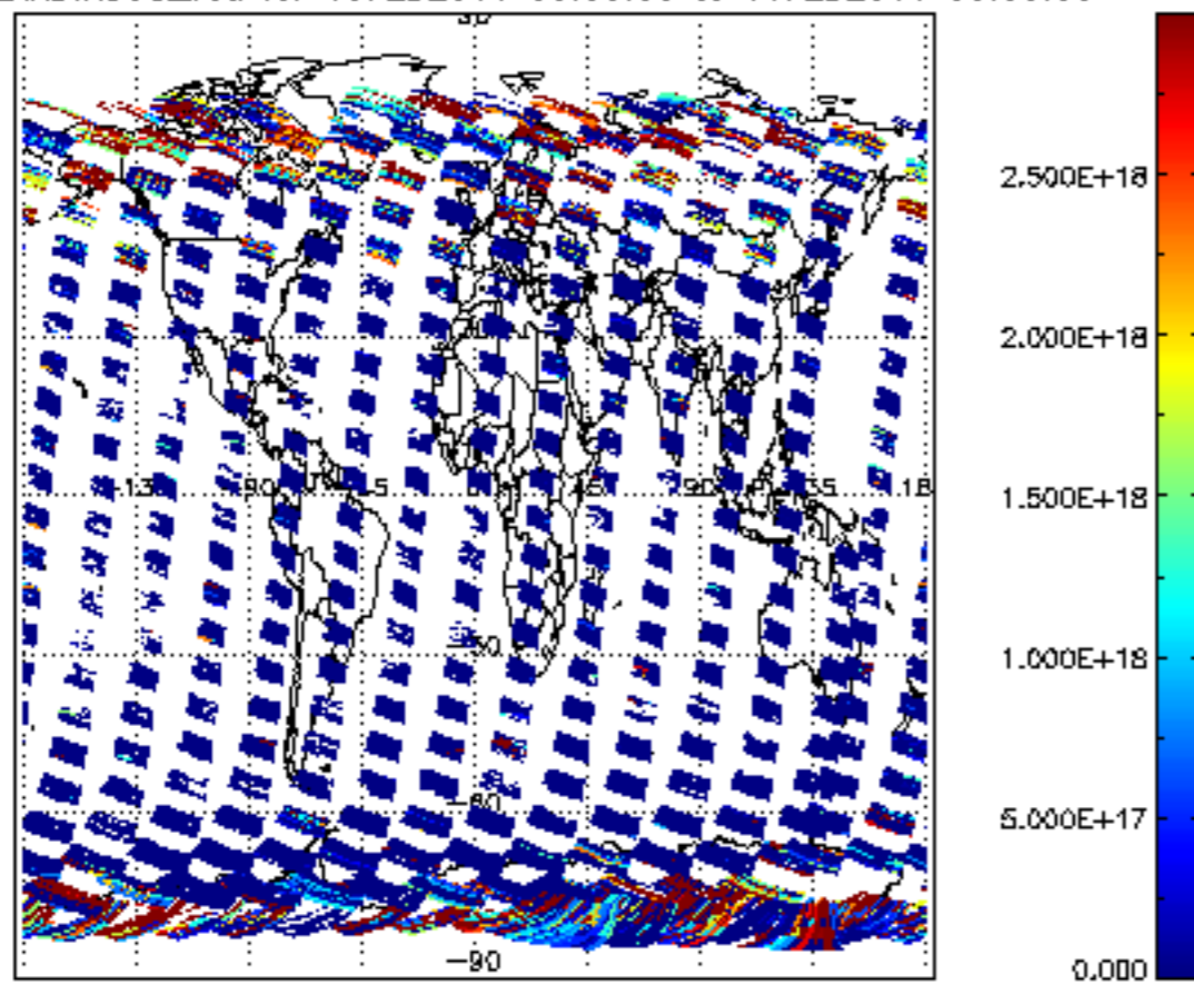
SCIOL2P_NADIR3CO_vcd for 15FEB2011 00:00:00 to 16FEB2011 00:00:00
