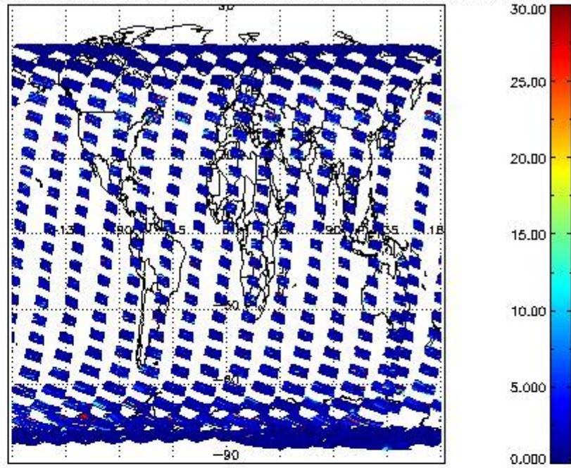
SCIOL2P_NADUV7S02_vcd_err for 15FEB2011 00:00:00 to 16FEB2011 00:00:00
