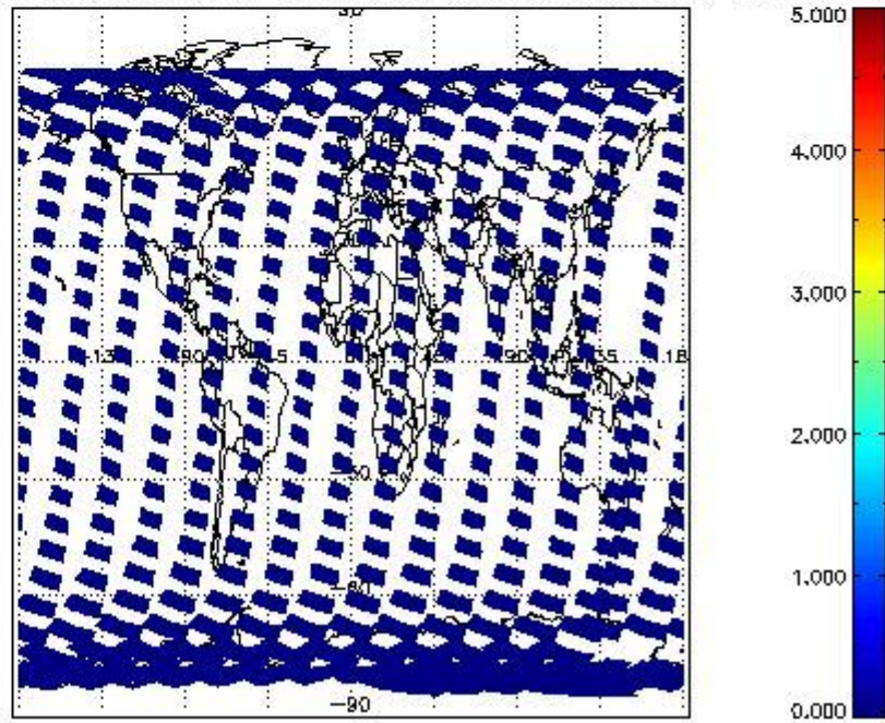
SCIOL2P_NADUV7S02_amf_cl for 15FEB2011 00:00:00 to 16FEB2011 00:00:00
