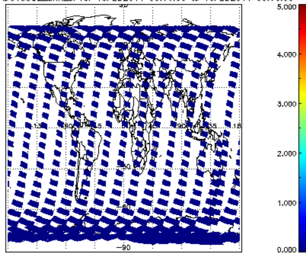
SCIOL2P_NADUV5S02_amf_cl for 15FEB2011 00:00:00 to 16FEB2011 00:00:00
