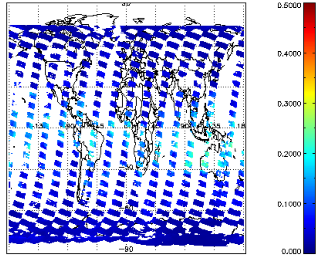
SCIOL2P_NADUV8H20_vcd_err for 15FEB2011 00:00:00 to 16FEB2011 00:00:00
