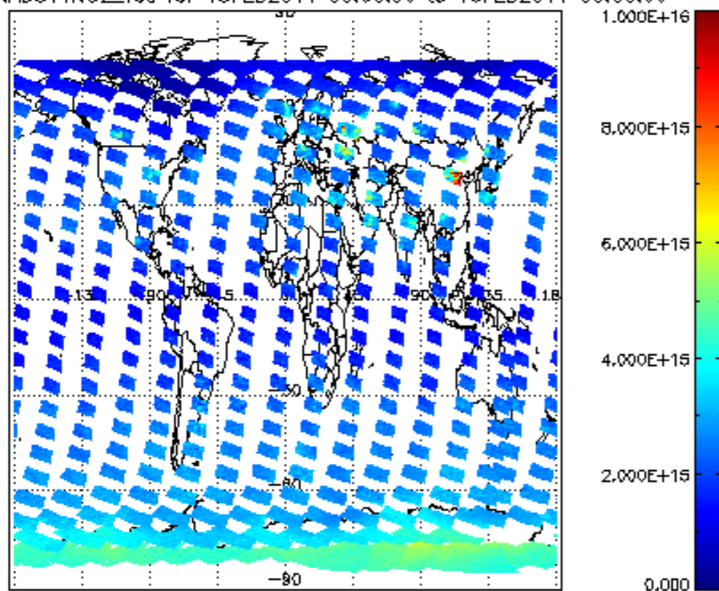
SCIOL2P_NADUV1N02_vcd for 15FEB2011 00:00:00 to 16FEB2011 00:00:00
