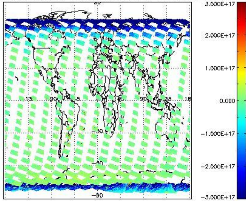
SCIOL2P_NADUV7S02_vcd for 15FEB2011 00:00:00 to 16FEB2011 00:00:00
