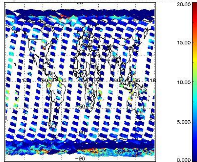
cL_top_height for 15FEB2011 00:00:00 to 16FEB2011 00:00:00
