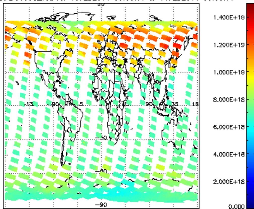
SCIOL2P_NADUV003_vcd for 15FEB2011 00:00:00 to 16FEB2011 00:00:00
