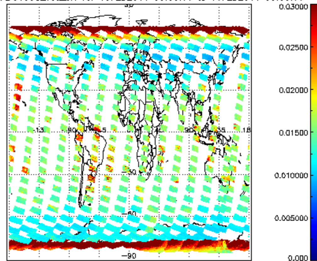
SCIOL2P_NADUV003_vcd_err for 15FEB2011 00:00:00 to 16FEB2011 00:00:00
