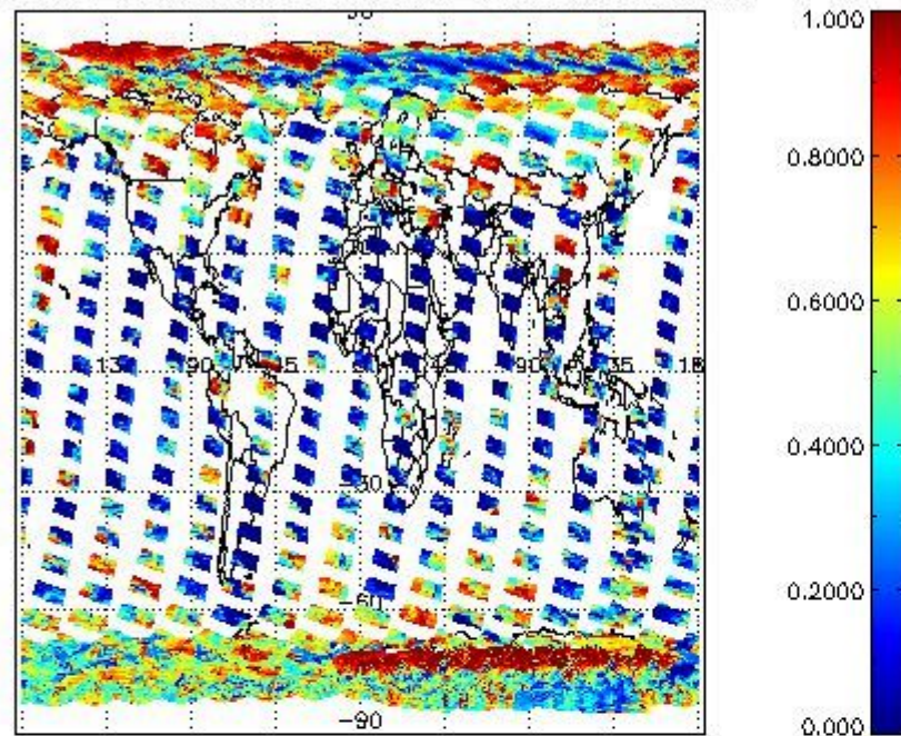
cL_frac for 15FEB2011 00:00:00 to 16FEB2011 00:00:00
