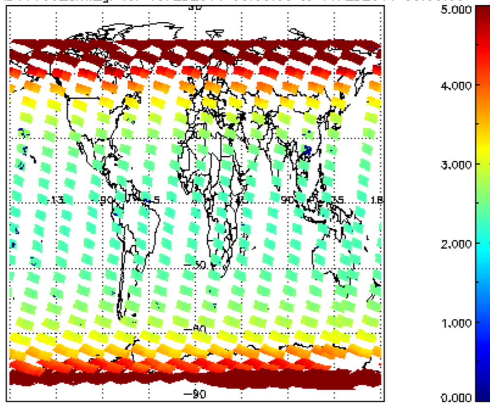
SCIOL2P_NADUV003_amf_gr for 15FEB2011 00:00:00 to 16FEB2011 00:00:00
