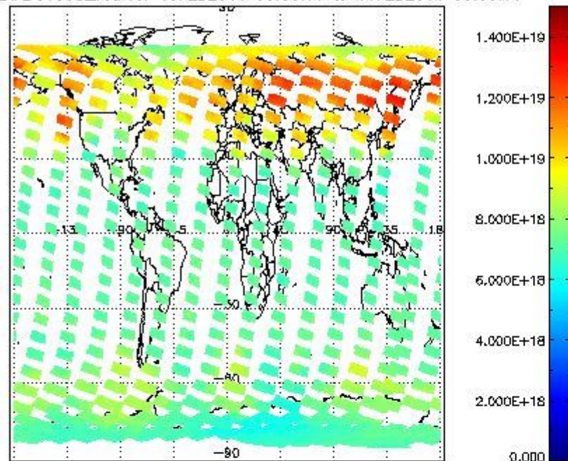
SCIOL2P_NADUV003_vcd for 15FEB2011 00:00:00 to 16FEB2011 00:00:00
