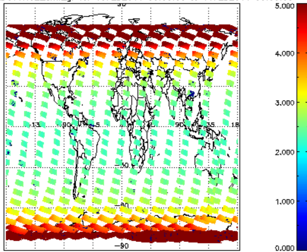
SCIOL2P_NADUV1N02_amf_gr for 15FEB2011 00:00:00 to 16FEB2011 00:00:00
