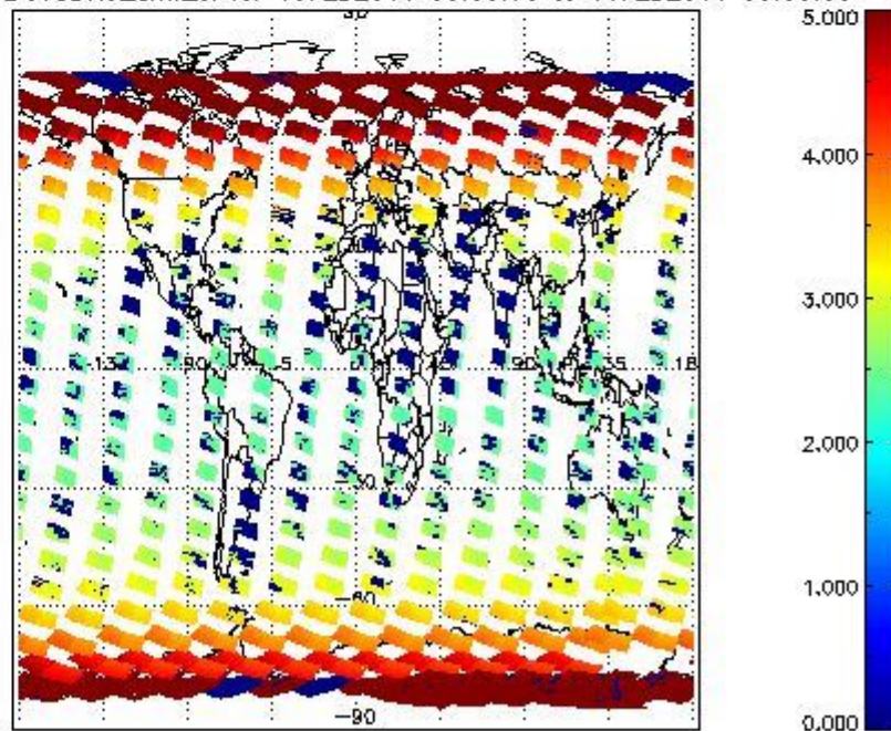
SCIOL2P_NADUV3BRO_amf_cl for 15FEB2011 00:00:00 to 16FEB2011 00:00:00
