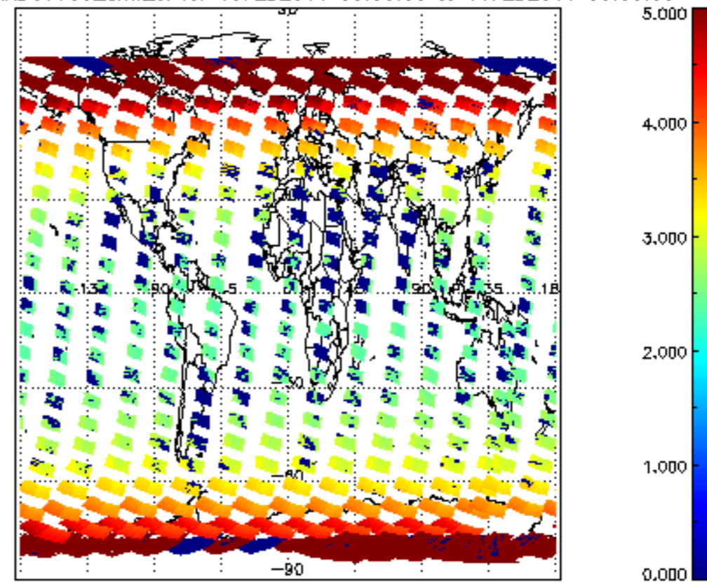
SCIOL2P_NADUV003_amf_cl for 15FEB2011 00:00:00 to 16FEB2011 00:00:00
