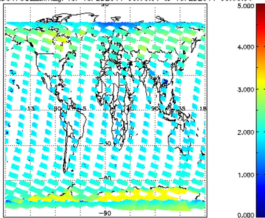
SCIOL2P_NADUV7S02_amf_gr for 15FEB2011 00:00:00 to 16FEB2011 00:00:00
