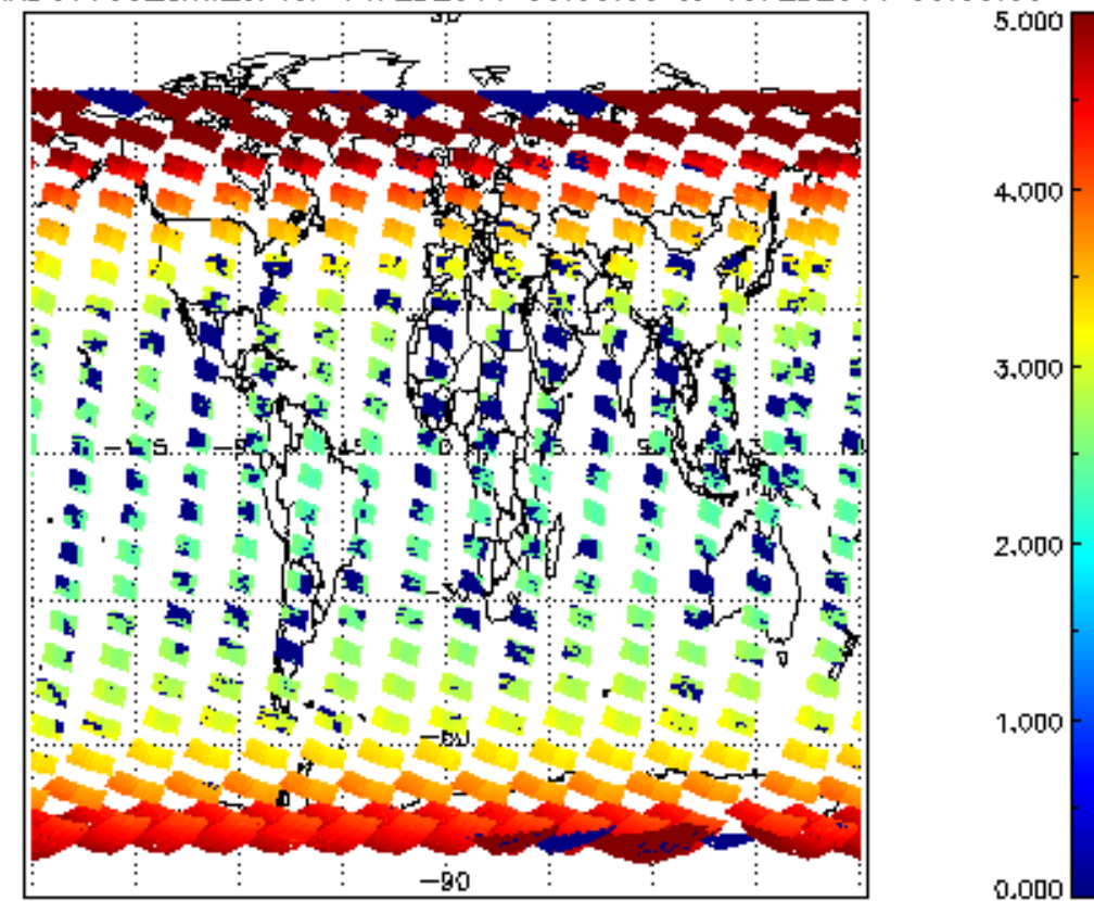
SCIOL2P_NADUV003_amf_cl for 14FEB2011 00:00:00 to 15FEB2011 00:00:00
