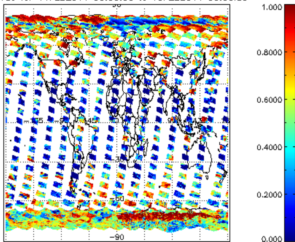
cI_frac for 14FEB2011 00:00:00 to 15FEB2011 00:00:00
