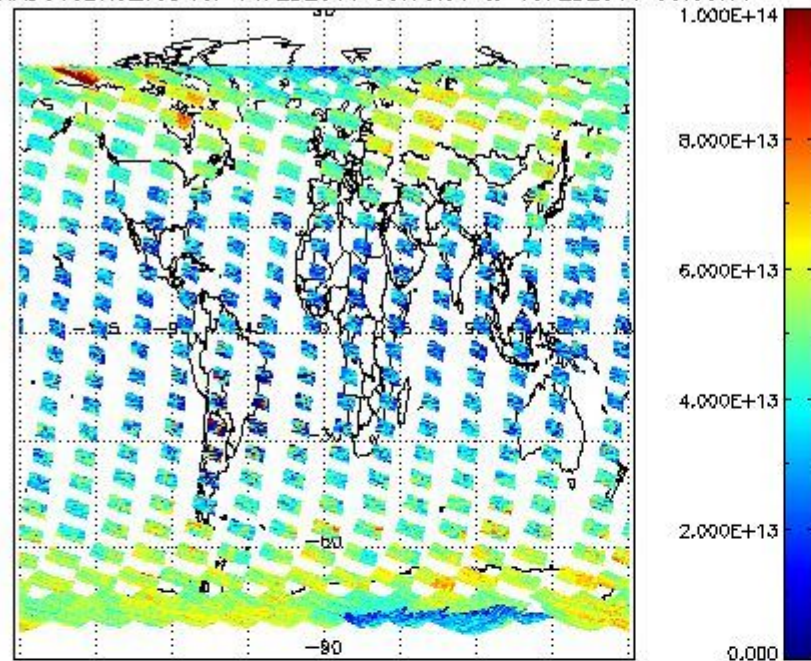
SCIOL2P_NADUV3BRO_vcd for 14FEB2011 00:00:00 to 15FEB2011 00:00:00
