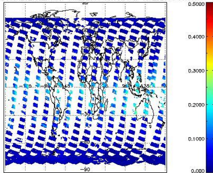
SCIOL2P_NADUV8H2O_vcd_err for 14FEB2011 00:00:00 to 15FEB2011 00:00:00
