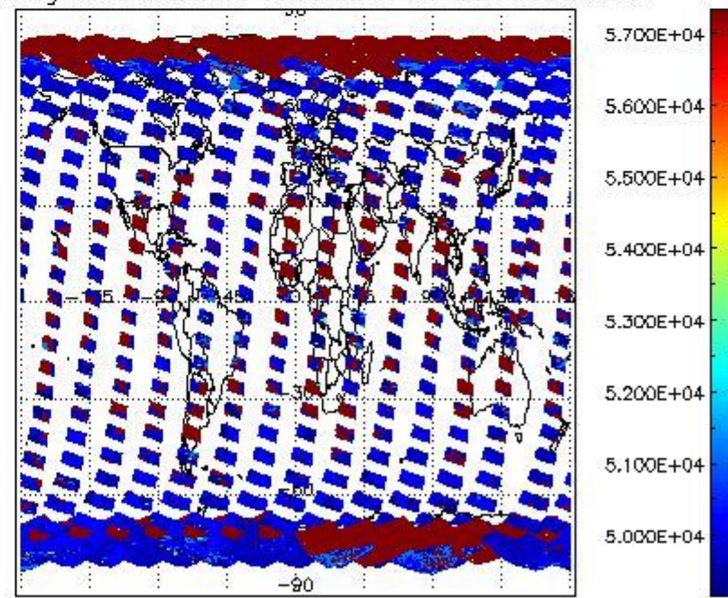
cloud_flags for 14FEB2011 00:00:00 to 15FEB2011 00:00:00
