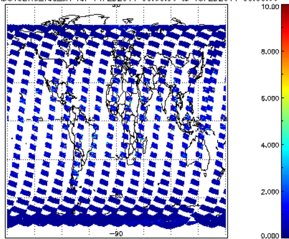
SCIOL2P_NADUV3BRO_vcd_err for 14FEB2011 00:00:00 to 15FEB2011 00:00:00
