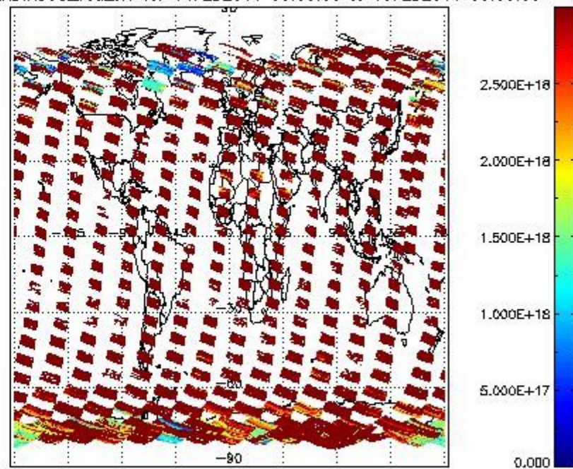
SCIDL2P_NADIR3CO_vcd_err for 14FEB2011 00:00:00 to 15FEB2011 00:00:00
