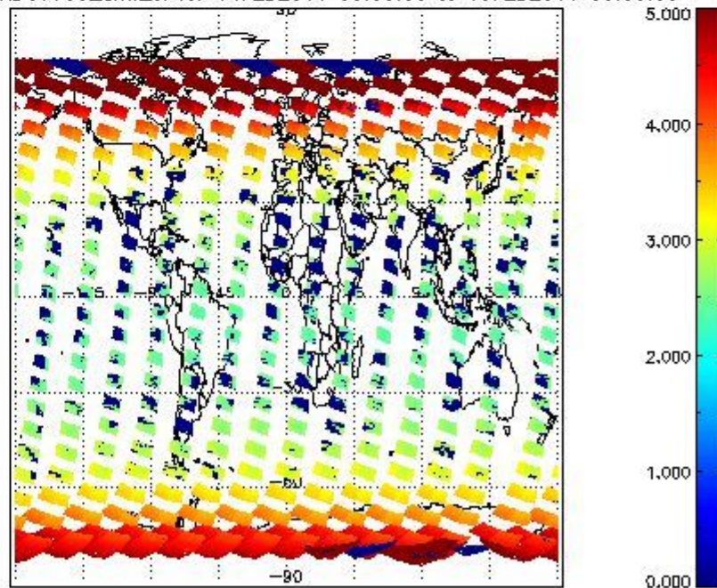
SCIOL2P_NADUV003_amf_cl for 14FEB2011 00:00:00 to 15FEB2011 00:00:00
