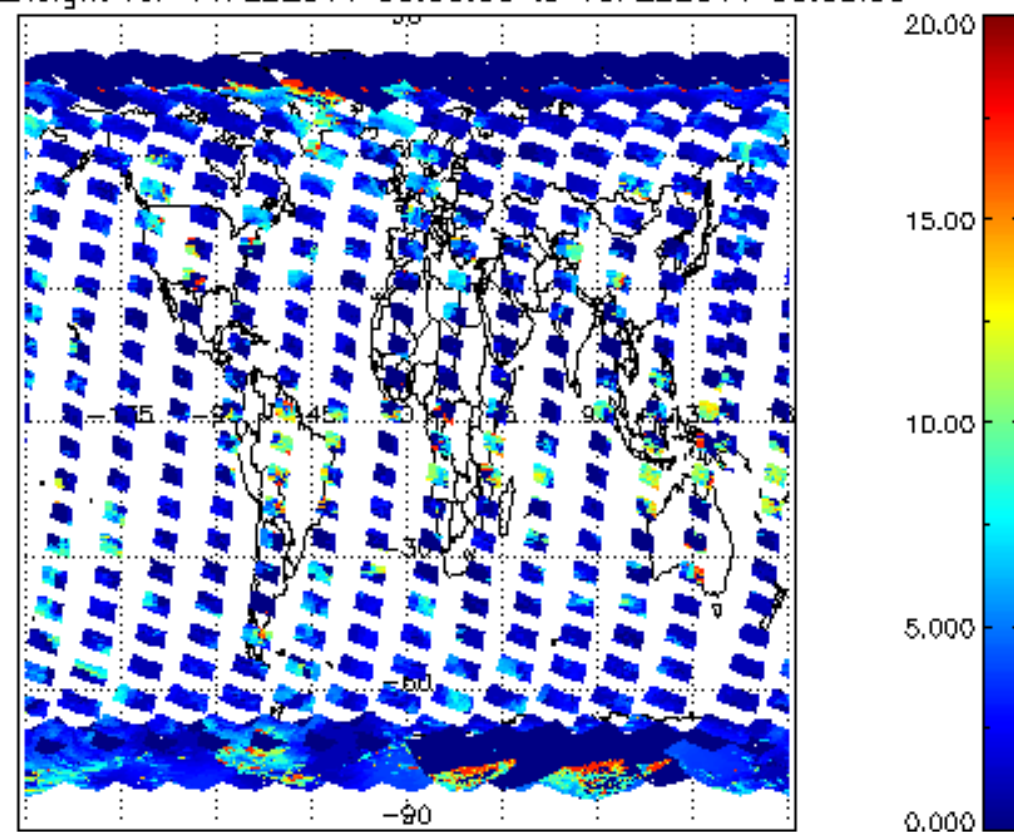
cI_top_height for 14FEB2011 00:00:00 to 15FEB2011 00:00:00
