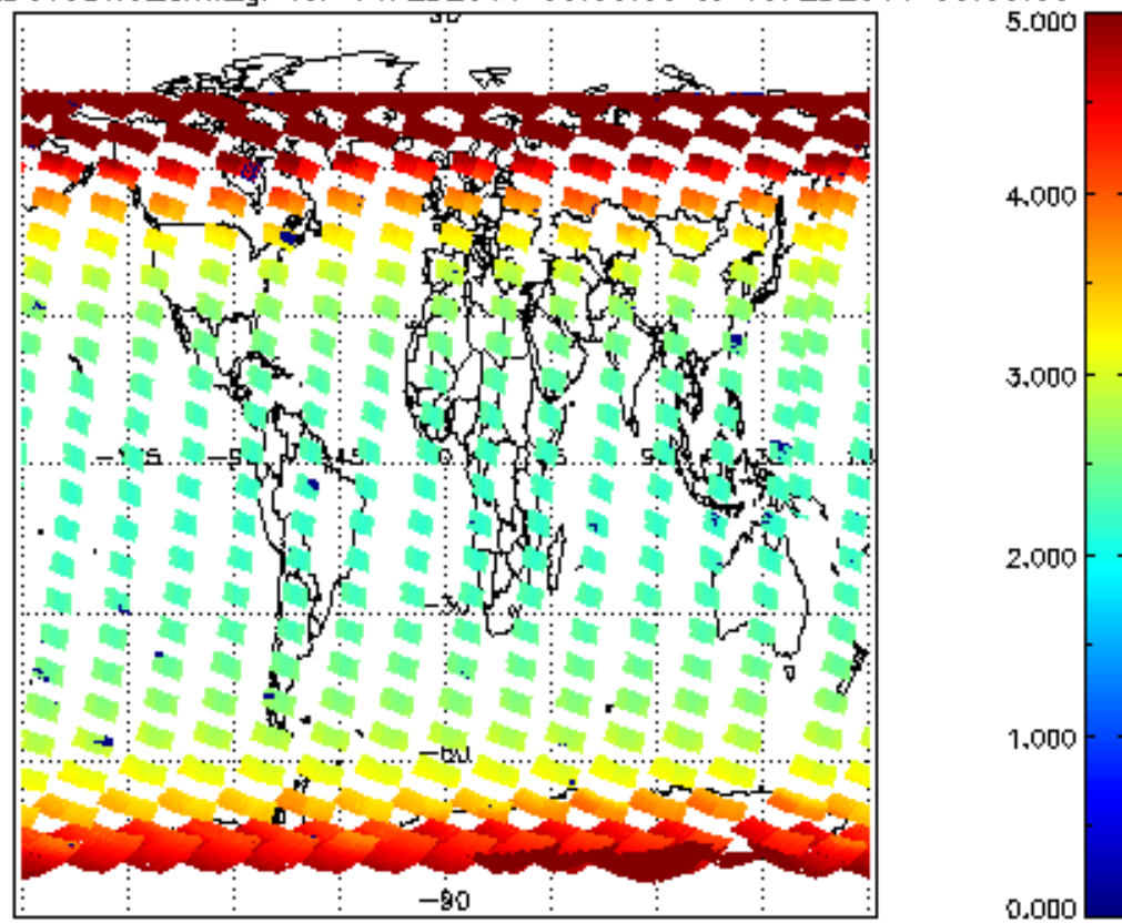
SCIOL2P_NADUV3BRO_amf_gr for 14FEB2011 00:00:00 to 15FEB2011 00:00:00
