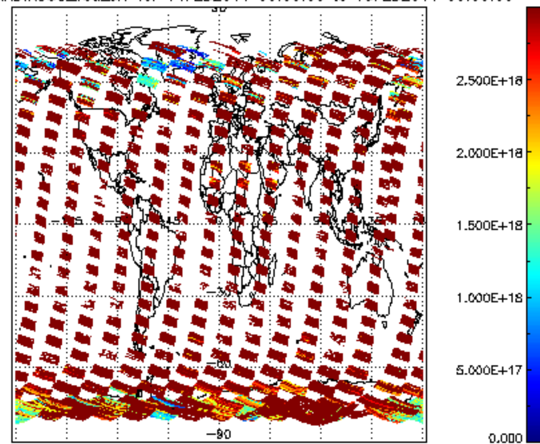
SCIOL2P_NADIR3CO_vcd_err for 14FEB2011 00:00:00 to 15FEB2011 00:00:00
