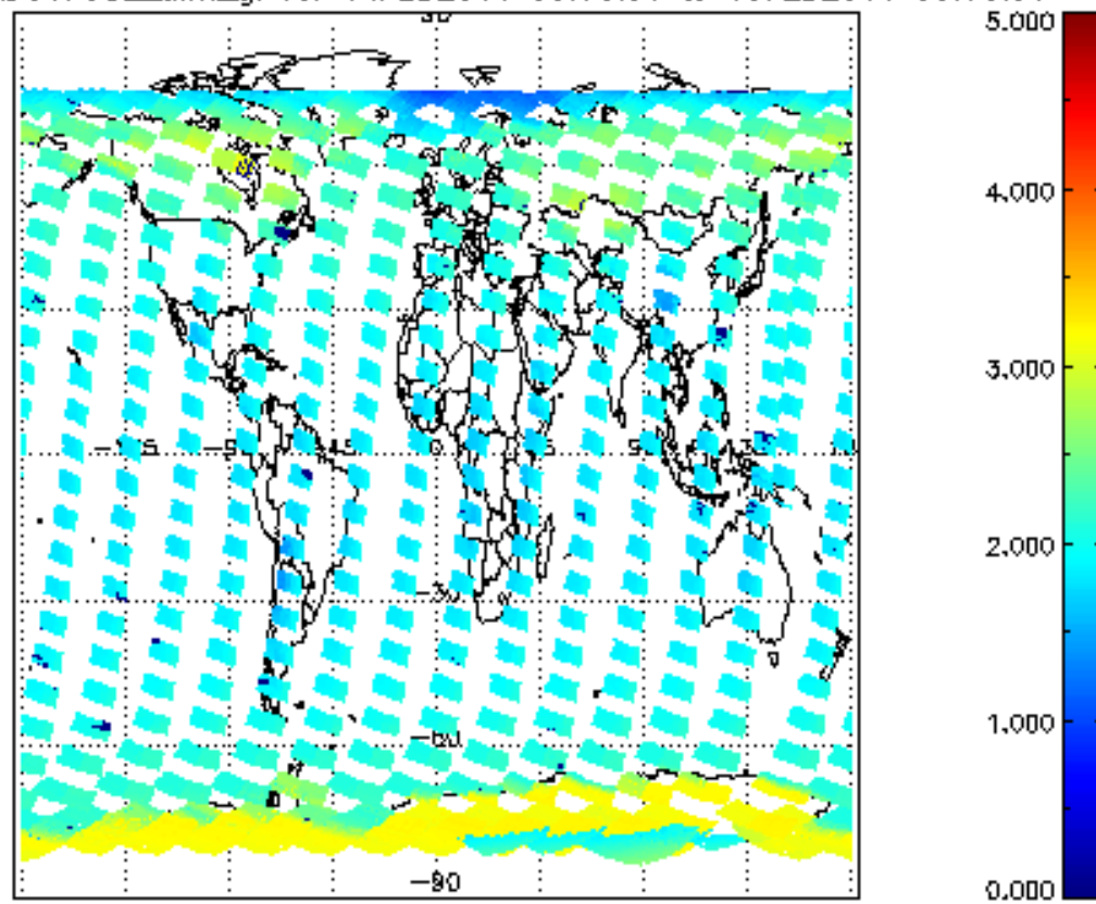
SCIOL2P_NADUV7S02_amf_gr for 14FEB2011 00:00:00 to 15FEB2011 00:00:00
