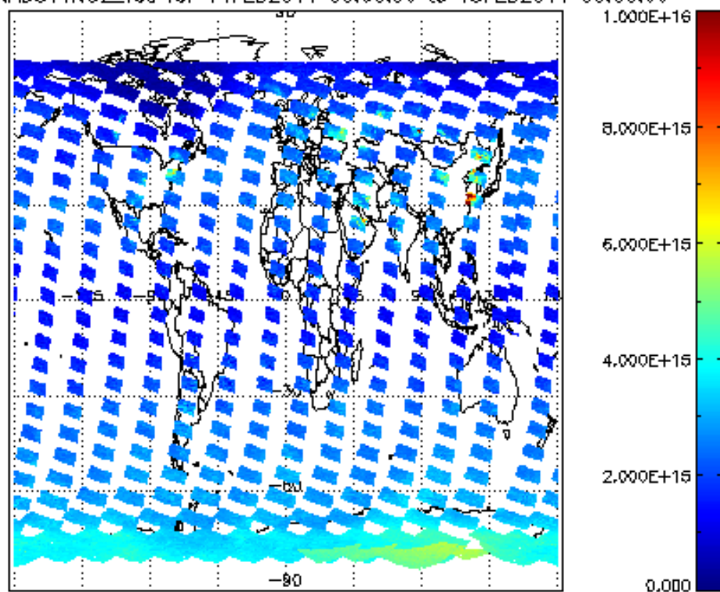
SCIOL2P_NADUV1N02_vcd for 14FEB2011 00:00:00 to 15FEB2011 00:00:00
