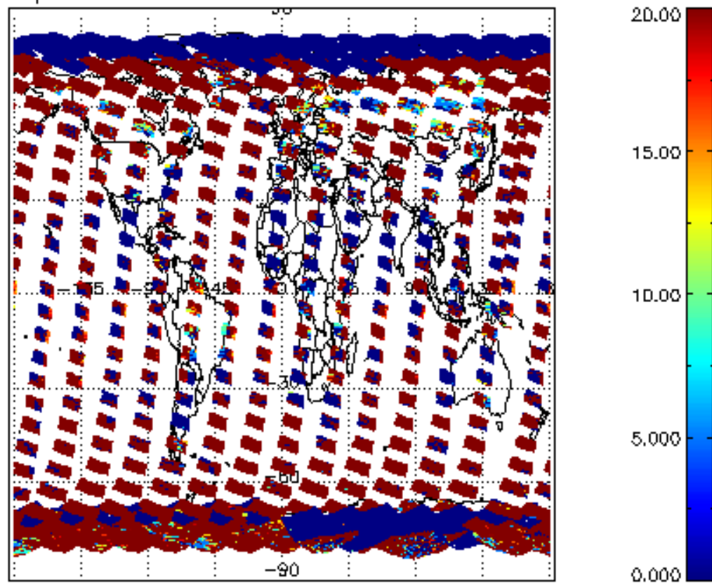
cI_opt_depth for 14FEB2011 00:00:00 to 15FEB2011 00:00:00
