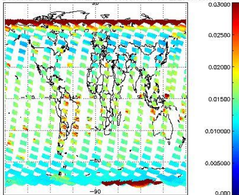
SCIOL2P_NADUV003_vcd_err for 14FEB2011 00:00:00 to 15FEB2011 00:00:00
