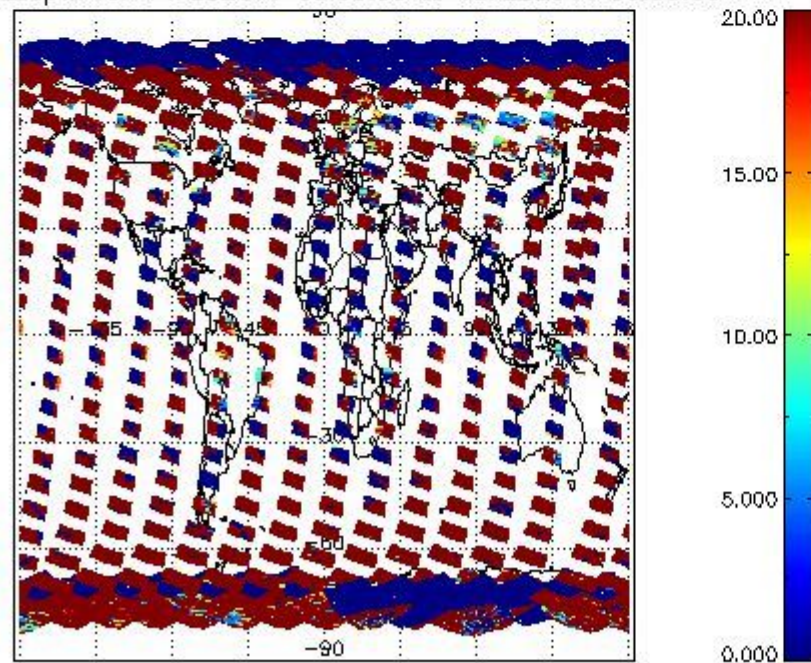
cL_opt_depth for 14FEB2011 00:00:00 to 15FEB2011 00:00:00
