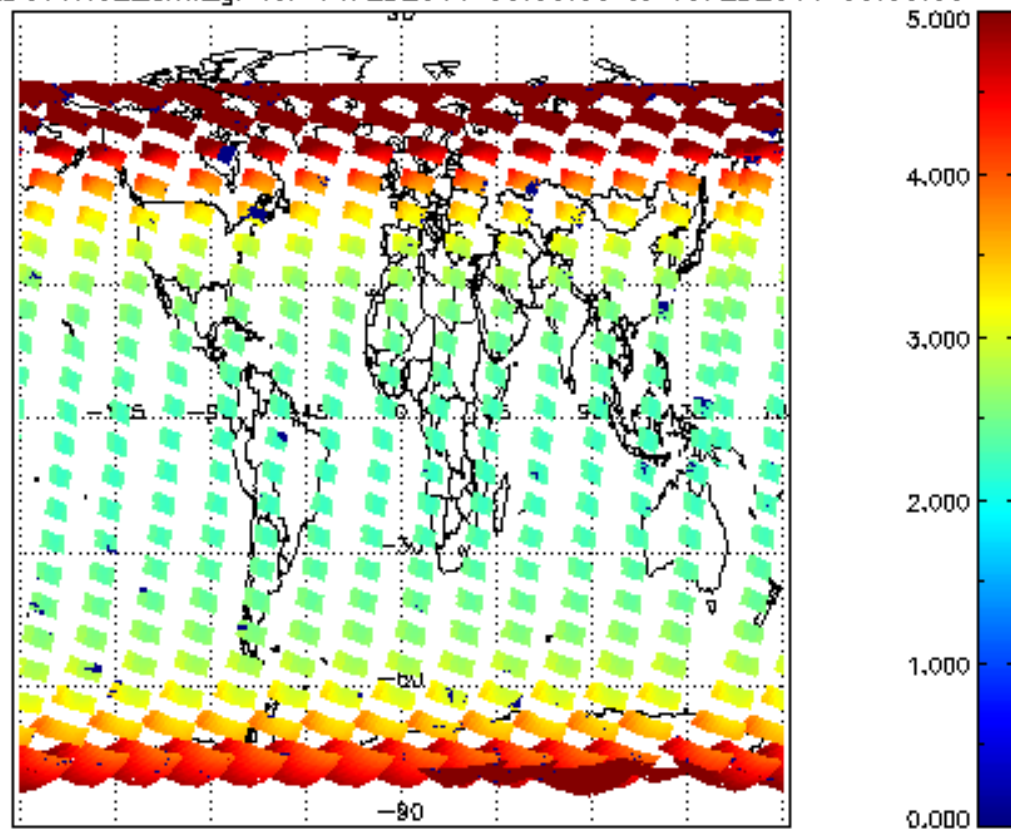
SCIOL2P_NADUV1N02_amf_gr for 14FEB2011 00:00:00 to 15FEB2011 00:00:00
