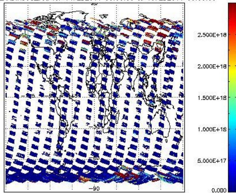
SCIDL2P_NADIR3CO_vcd for 14FEB2011 00:00:00 to 15FEB2011 00:00:00
