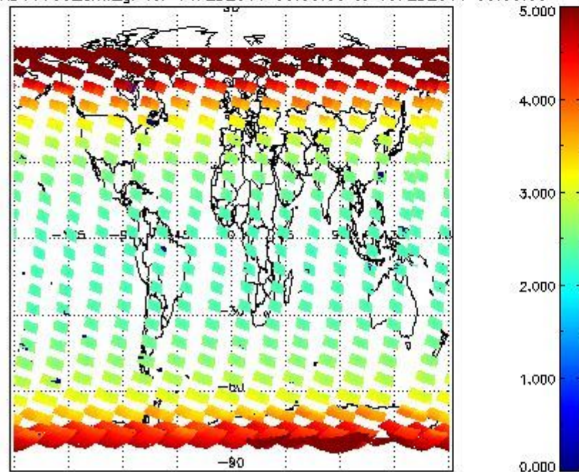
SCIOL2P_NADUV003_amf_gr for 14FEB2011 00:00:00 to 15FEB2011 00:00:00
