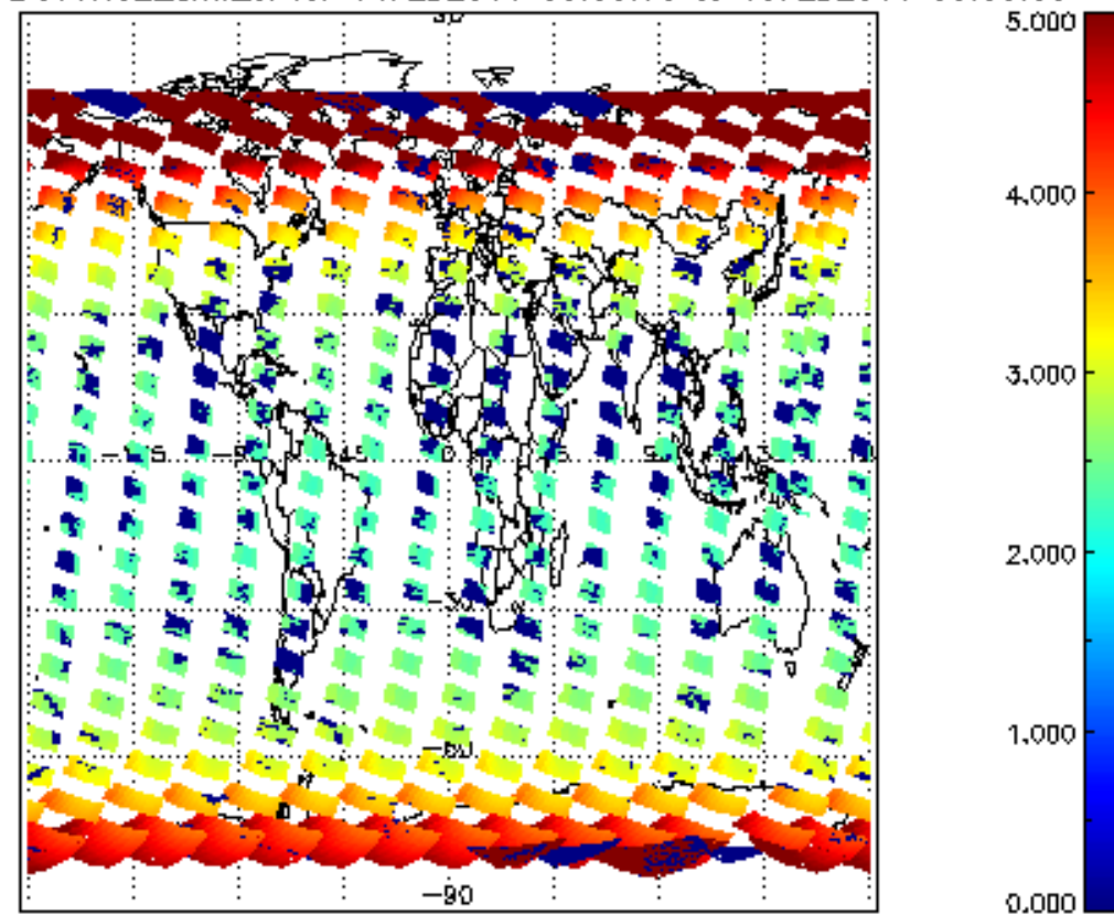
SCIOL2P_NADUV1N02_amf_cl for 14FEB2011 00:00:00 to 15FEB2011 00:00:00
