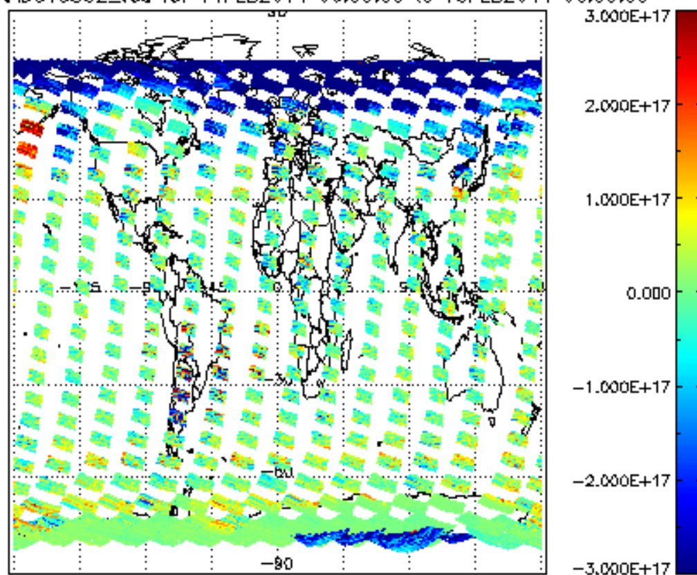
SCIOL2P_NADUV5S02_vcd for 14FEB2011 00:00:00 to 15FEB2011 00:00:00
