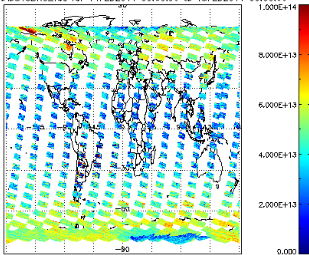
SCIOL2P_NADUV3BRO_vcd for 14FEB2011 00:00:00 to 15FEB2011 00:00:00
