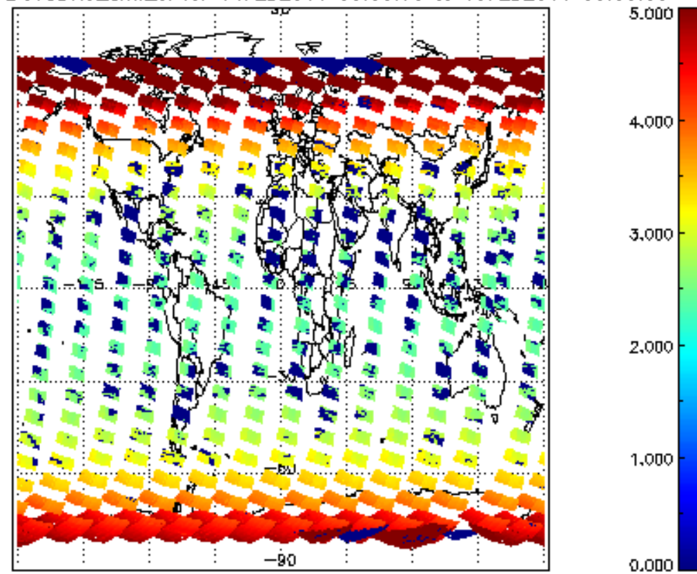
SCIOL2P_NADUV3BRO_amf_cl for 14FEB2011 00:00:00 to 15FEB2011 00:00:00
