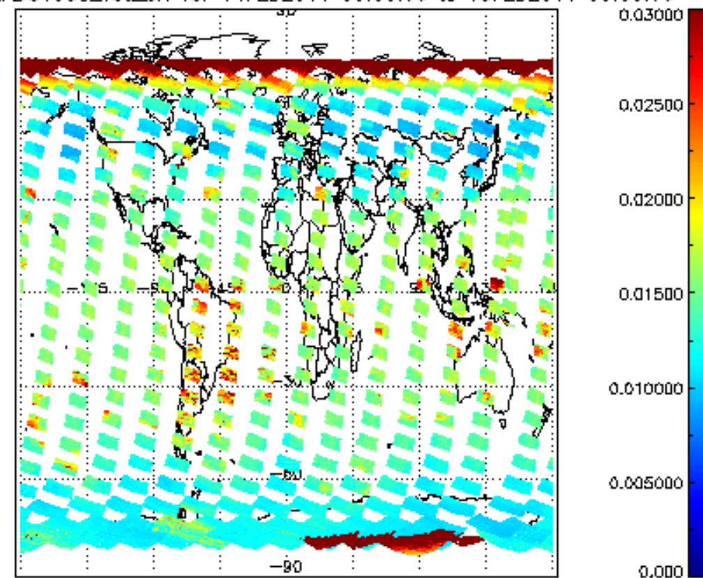
SCIOL2P_NADUV003_vcd_err for 14FEB2011 00:00:00 to 15FEB2011 00:00:00
