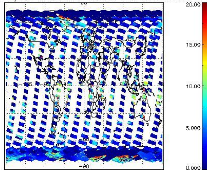
cL_top_height for 14FEB2011 00:00:00 to 15FEB2011 00:00:00
