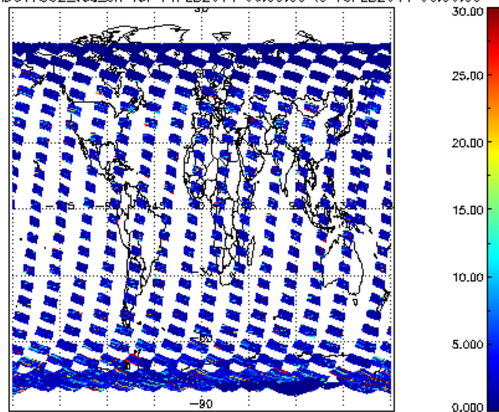
SCIOL2P_NADUV7S02_vcd_err for 14FEB2011 00:00:00 to 15FEB2011 00:00:00
