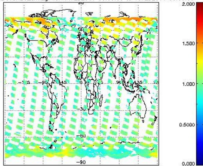
SCIOL2P_NADUV8H2O_amf_gr for 14FEB2011 00:00:00 to 15FEB2011 00:00:00
