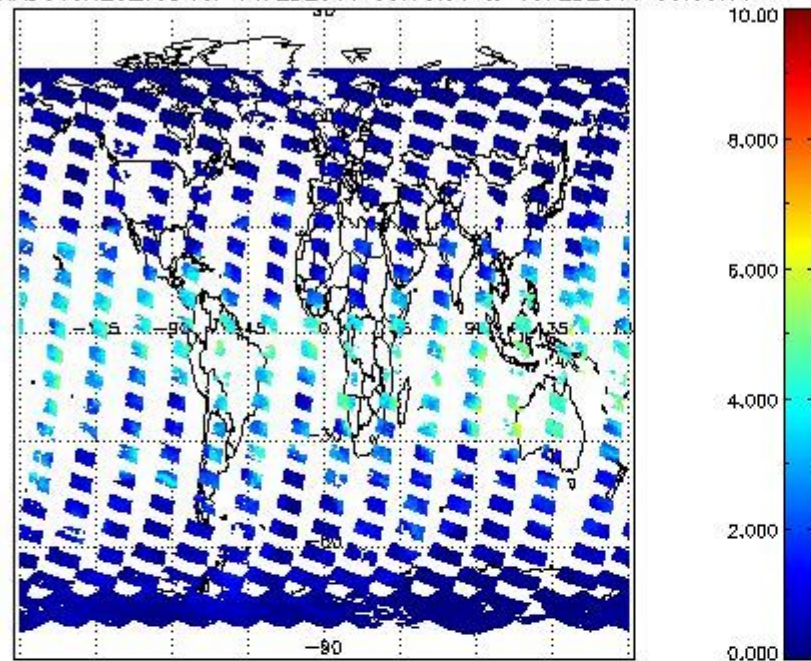
SCIOL2P_NADUV8H2O_vcd for 14FEB2011 00:00:00 to 15FEB2011 00:00:00
