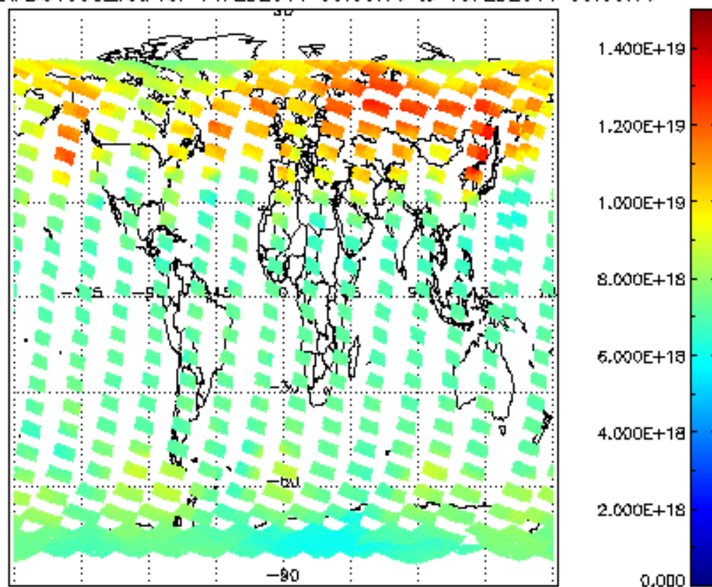
SCIOL2P_NADUV003_vcd for 14FEB2011 00:00:00 to 15FEB2011 00:00:00
