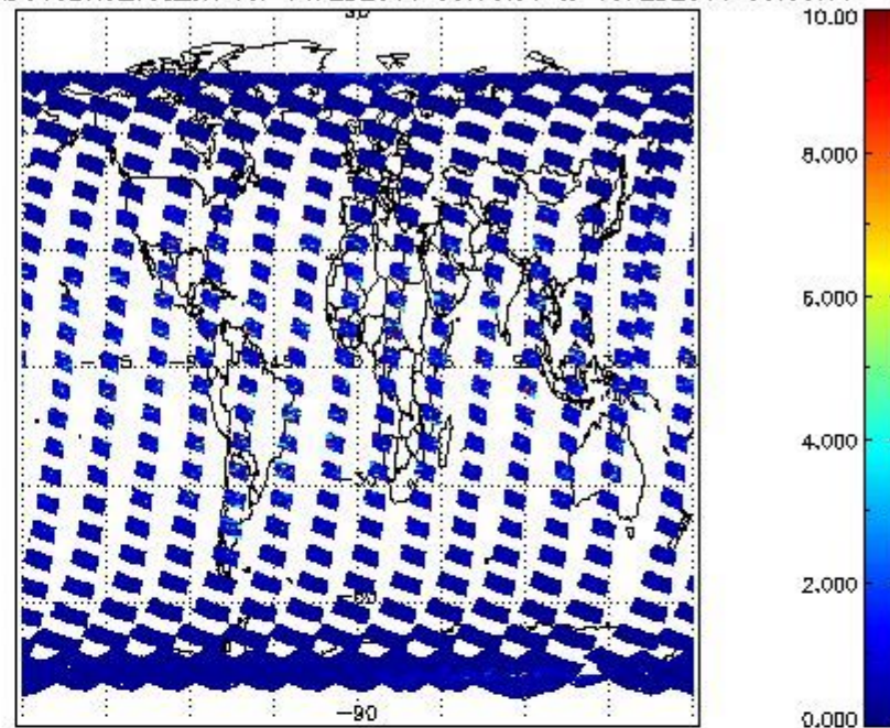
SCIOL2P_NADUV3BRO_vcd_err for 14FEB2011 00:00:00 to 15FEB2011 00:00:00
