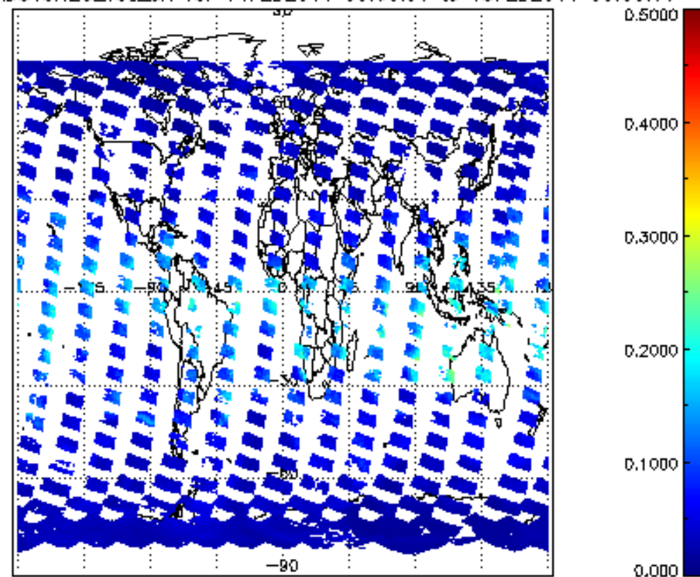
SCIOL2P_NADUV8H2O_vcd_err for 14FEB2011 00:00:00 to 15FEB2011 00:00:00
