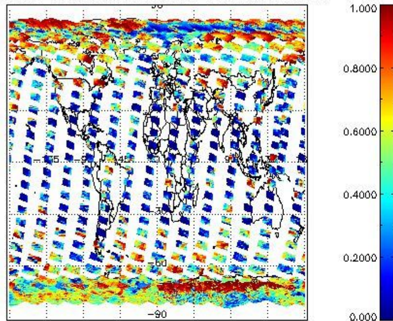
cL_frac for 14FEB2011 00:00:00 to 15FEB2011 00:00:00
