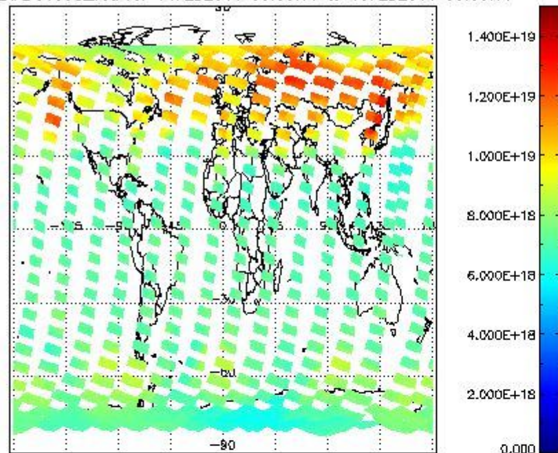
SCIOL2P_NADUV003_vcd for 14FEB2011 00:00:00 to 15FEB2011 00:00:00
