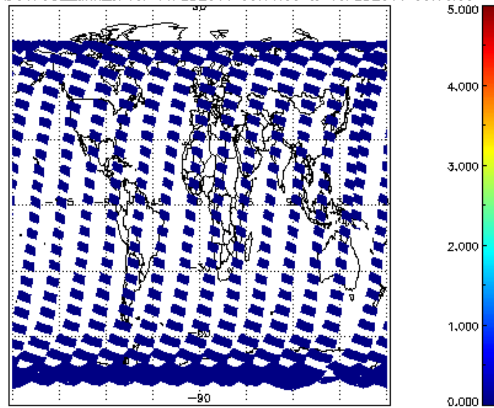
SCIOL2P_NADUV7S02_amf_cl for 14FEB2011 00:00:00 to 15FEB2011 00:00:00
