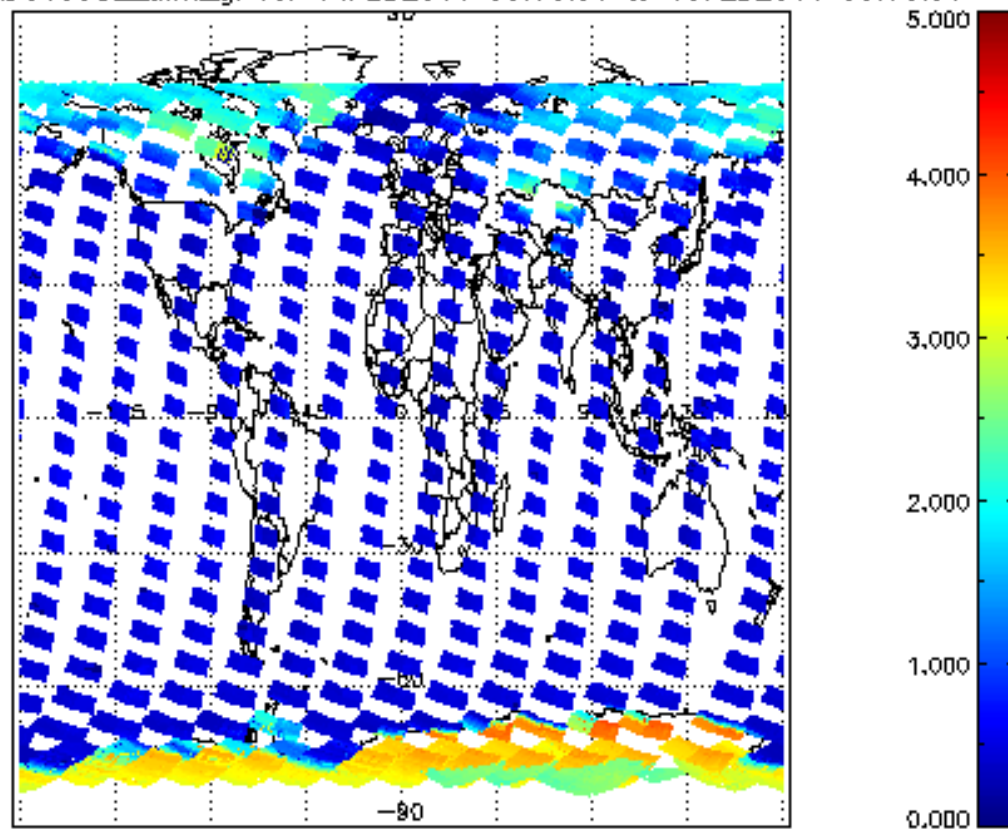
SCIOL2P_NADUV5S02_amf_gr for 14FEB2011 00:00:00 to 15FEB2011 00:00:00
