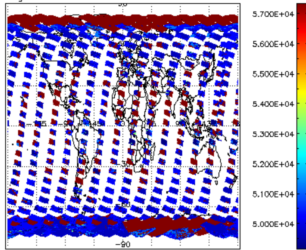
cloud_flags for 14FEB2011 00:00:00 to 15FEB2011 00:00:00
