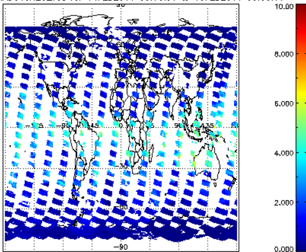
SCIOL2P_NADUV8H2O_vcd for 14FEB2011 00:00:00 to 15FEB2011 00:00:00
