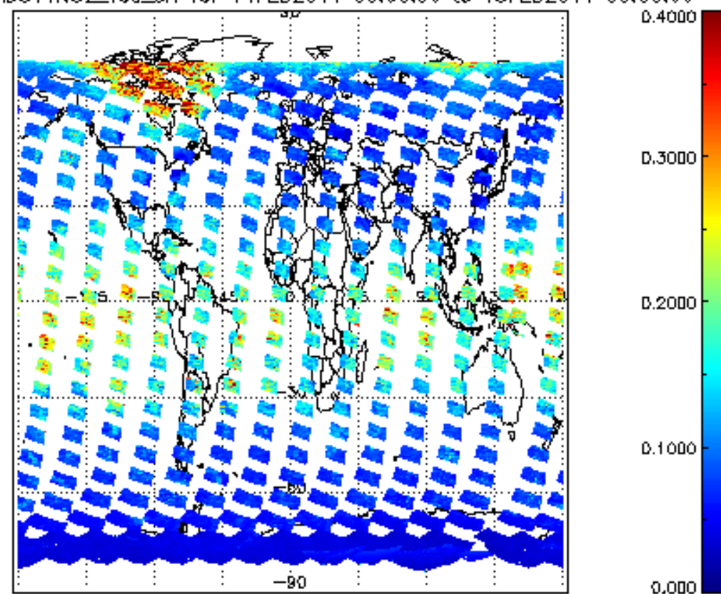
SCIOL2P_NADUV1N02_vcd_err for 14FEB2011 00:00:00 to 15FEB2011 00:00:00
