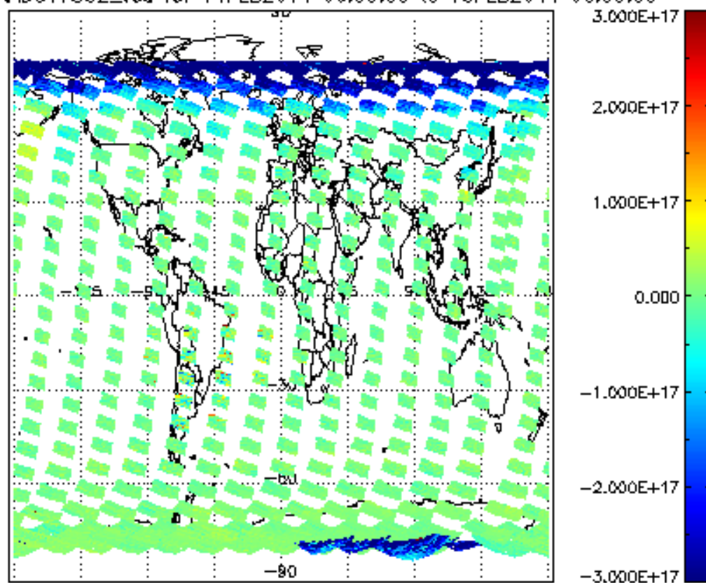
SCIOL2P_NADUV7S02_vcd for 14FEB2011 00:00:00 to 15FEB2011 00:00:00
