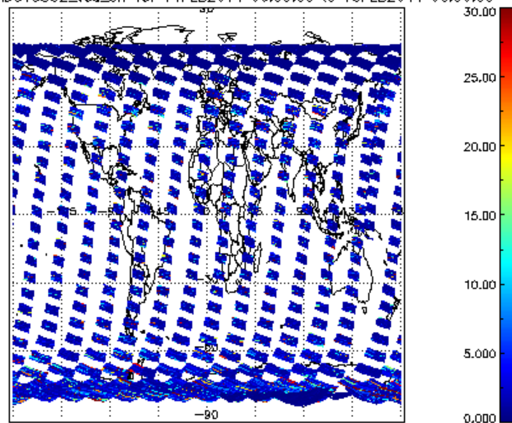
SCIOL2P_NADUV5S02_vcd_err for 14FEB2011 00:00:00 to 15FEB2011 00:00:00
