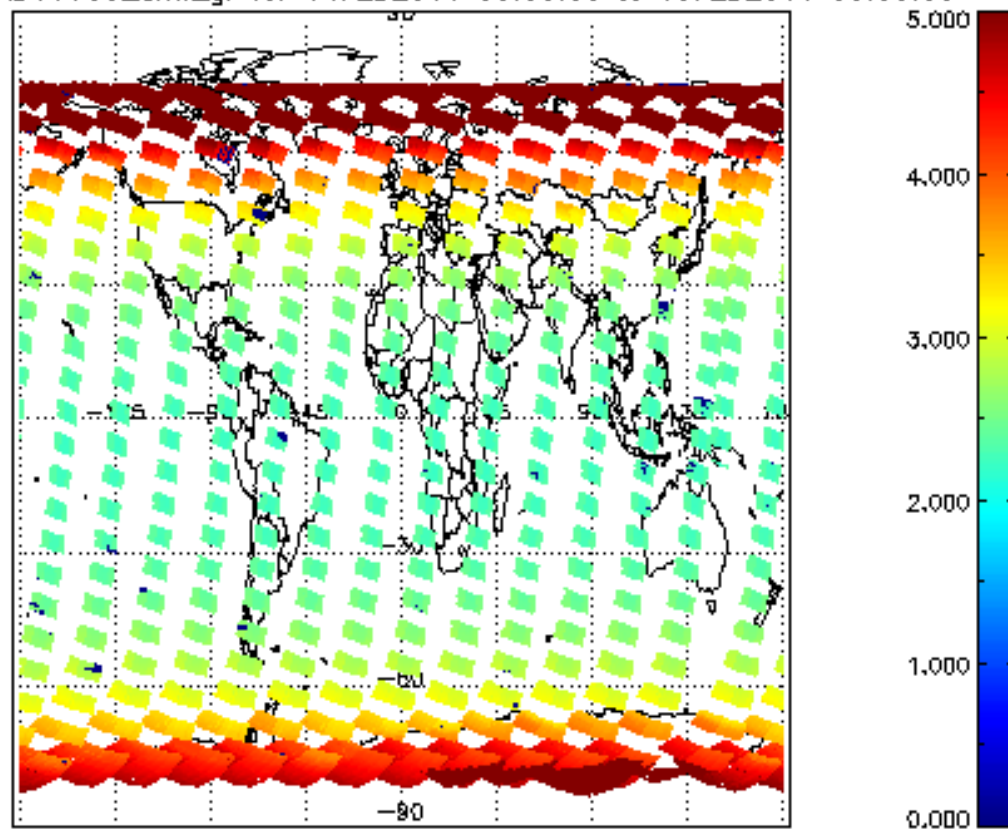
SCIOL2P_NADUV003_amf_gr for 14FEB2011 00:00:00 to 15FEB2011 00:00:00
