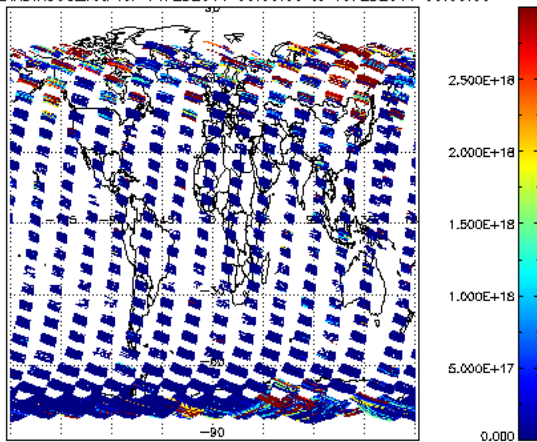
SCIOL2P_NADIR3CO_vcd for 14FEB2011 00:00:00 to 15FEB2011 00:00:00
