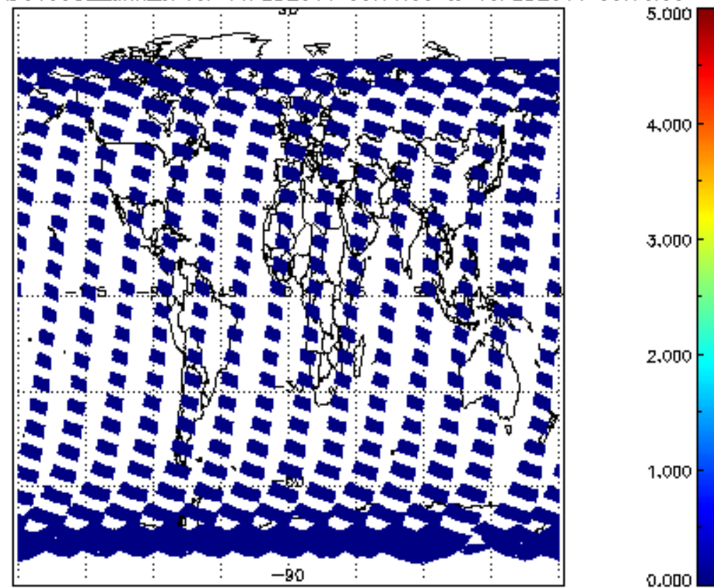
SCIOL2P_NADUV5S02_amf_cl for 14FEB2011 00:00:00 to 15FEB2011 00:00:00
