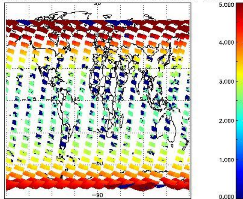
SCIOL2P_NADUV3BRO_amf_cl for 14FEB2011 00:00:00 to 15FEB2011 00:00:00
