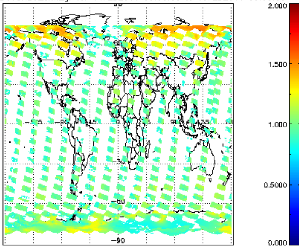
SCIOL2P_NADUV8H2O_amf_gr for 14FEB2011 00:00:00 to 15FEB2011 00:00:00
