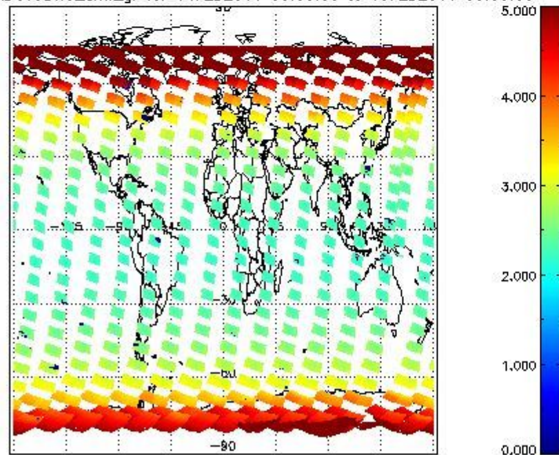
SCIOL2P_NADUV3BRO_amf_gr for 14FEB2011 00:00:00 to 15FEB2011 00:00:00
