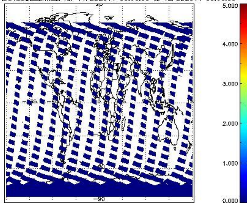
SCIOL2P_NADUV5S02_amf_cl for 11FEB2011 00:00:00 to 12FEB2011 00:00:00
