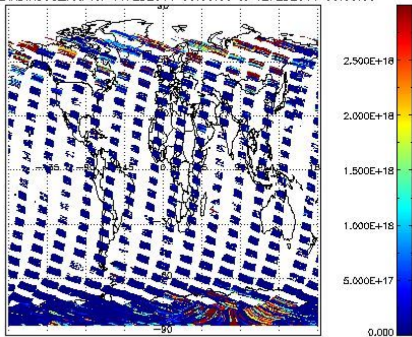
SCIDL2P_NADIR3CO_vcd for 11FEB2011 00:00:00 to 12FEB2011 00:00:00
