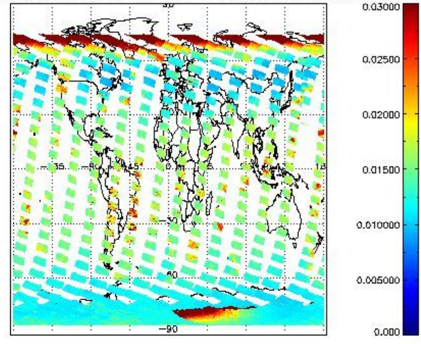
SCIOL2P_NADUV003_vcd_err for 11FEB2011 00:00:00 to 12FEB2011 00:00:00
