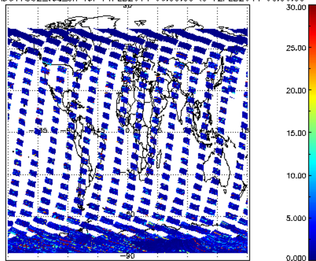
SCIOL2P_NADUV7S02_vcd_err for 11FEB2011 00:00:00 to 12FEB2011 00:00:00
