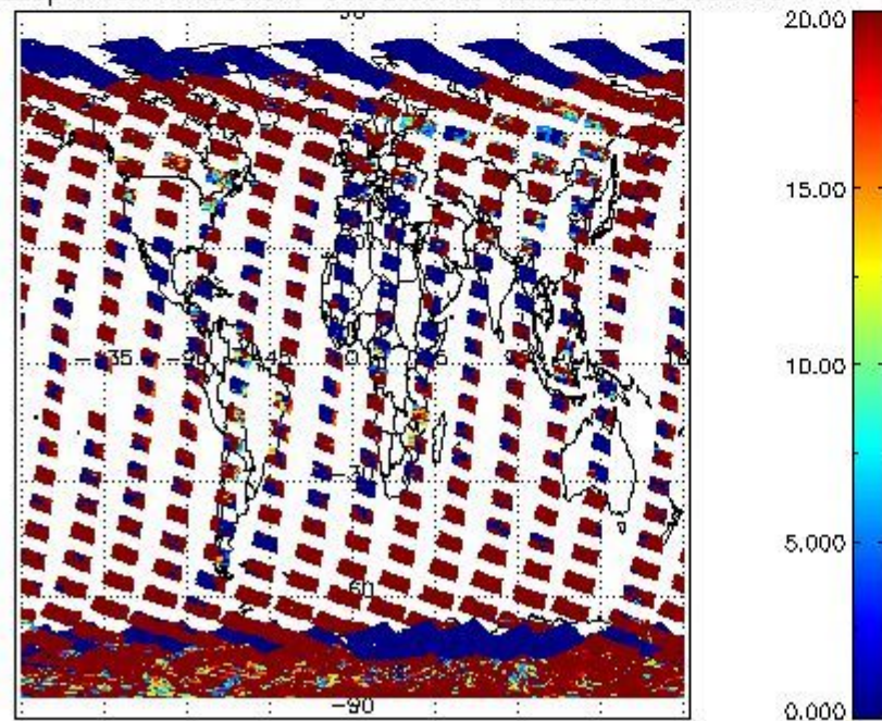
cL_opt_depth for 11FEB2011 00:00:00 to 12FEB2011 00:00:00
