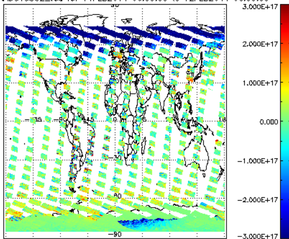
SCIOL2P_NADUV5S02_vcd for 11FEB2011 00:00:00 to 12FEB2011 00:00:00
