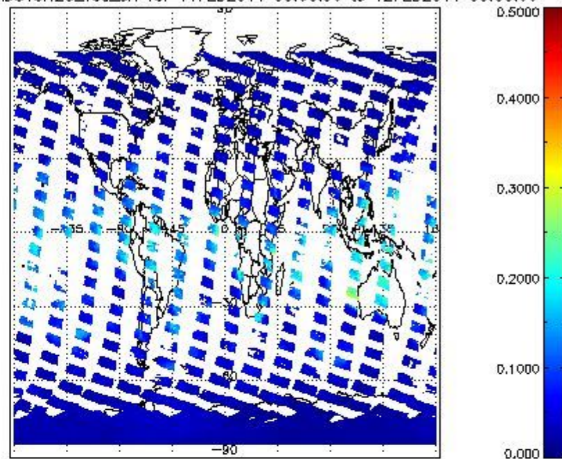
SCIOL2P_NADUV8H2O_vcd_err for 11FEB2011 00:00:00 to 12FEB2011 00:00:00
