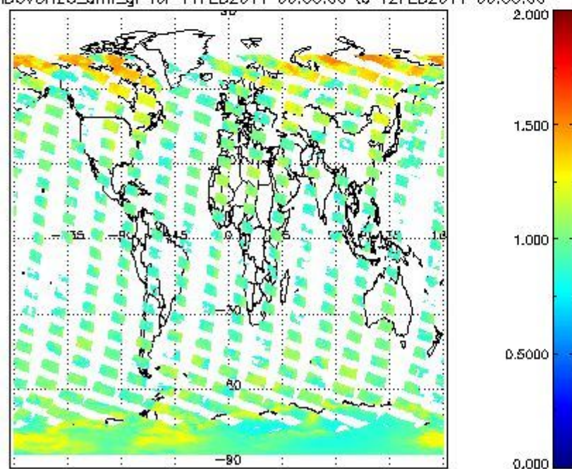
SCIOL2P_NADUV8H2O_amf_gr for 11FEB2011 00:00:00 to 12FEB2011 00:00:00
