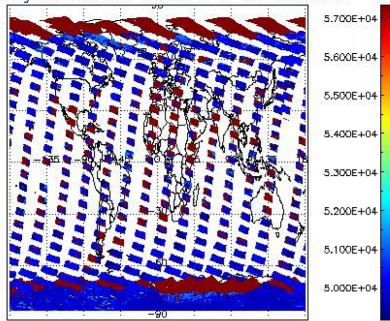
cloud_flags for 11FEB2011 00:00:00 to 12FEB2011 00:00:00
