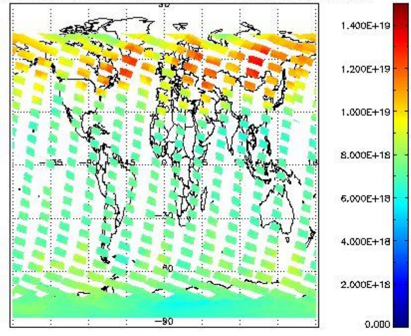
SCIOL2P_NADUV003_vcd for 11FEB2011 00:00:00 to 12FEB2011 00:00:00
