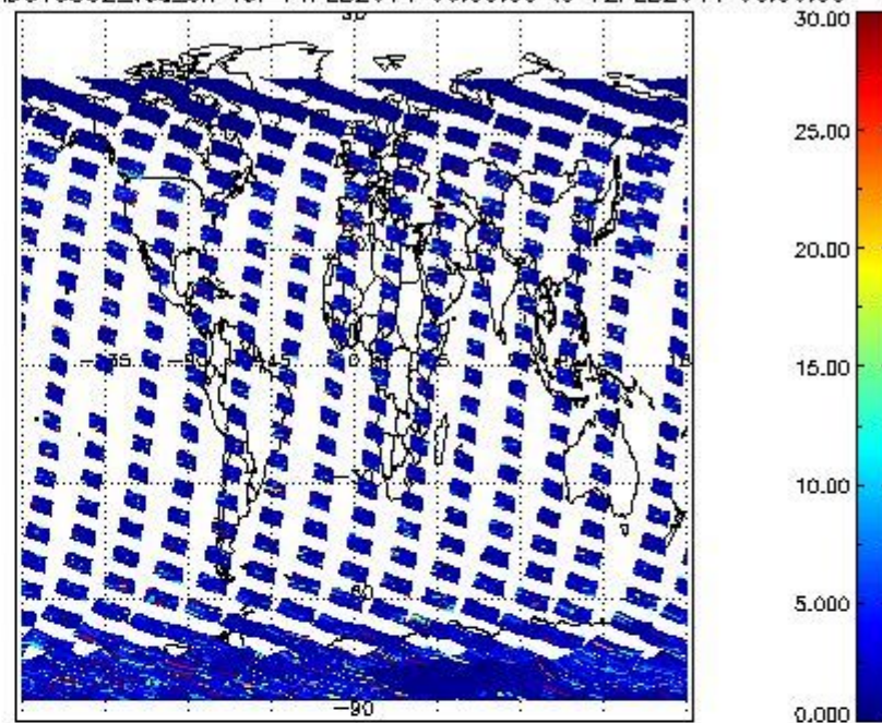
SCIOL2P_NADUV5S02_vcd_err for 11FEB2011 00:00:00 to 12FEB2011 00:00:00
