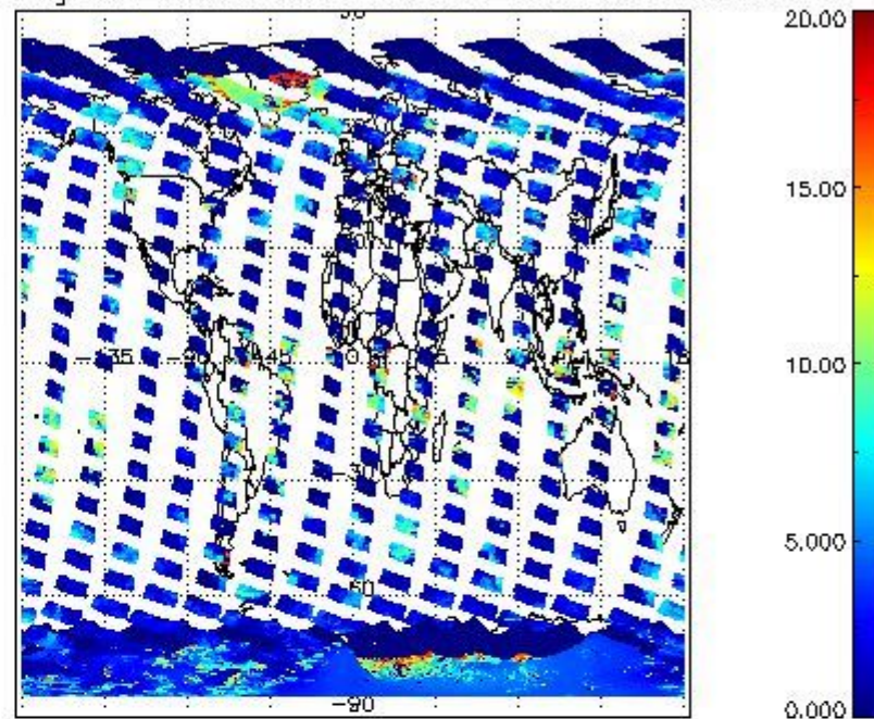
cL_top_height for 11FEB2011 00:00:00 to 12FEB2011 00:00:00
