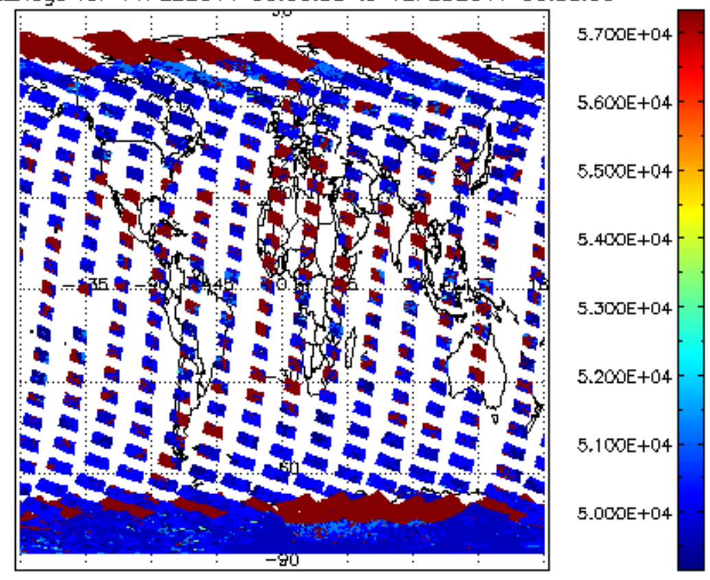
cloud_flags for 11FEB2011 00:00:00 to 12FEB2011 00:00:00
