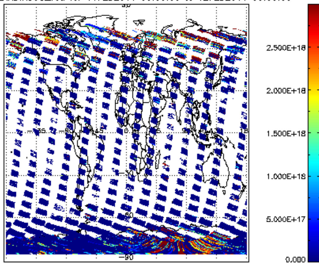
SCIOL2P_NADIR3CO_vcd for 11FEB2011 00:00:00 to 12FEB2011 00:00:00
