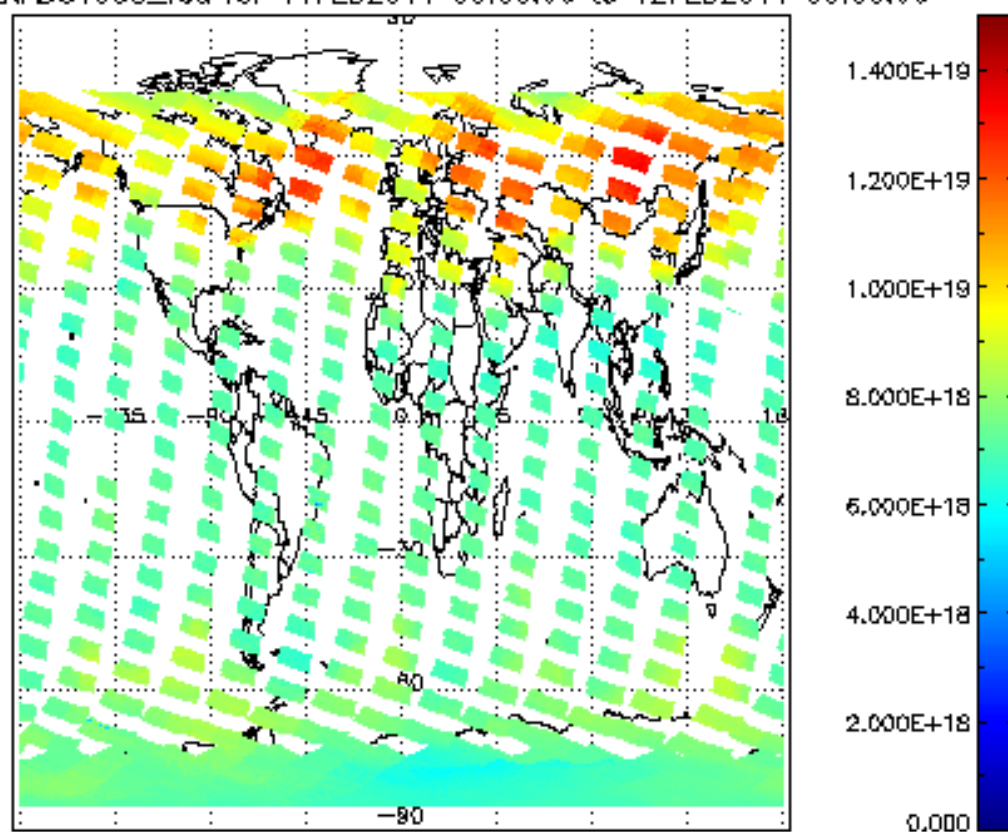
SCIOL2P_NADUV003_vcd for 11FEB2011 00:00:00 to 12FEB2011 00:00:00
