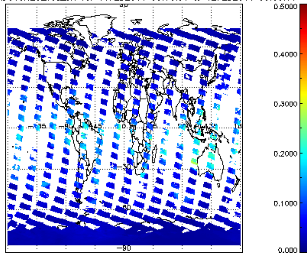
SCIOL2P_NADUV8H2O_vcd_err for 11FEB2011 00:00:00 to 12FEB2011 00:00:00
