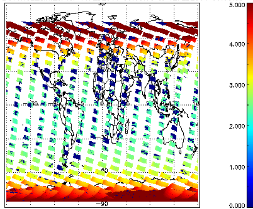
SCIOL2P_NADUV1N02_amf_cl for 11FEB2011 00:00:00 to 12FEB2011 00:00:00
