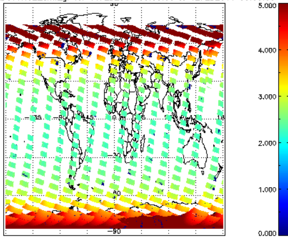
SCIOL2P_NADUV1N02_amf_gr for 11FEB2011 00:00:00 to 12FEB2011 00:00:00
