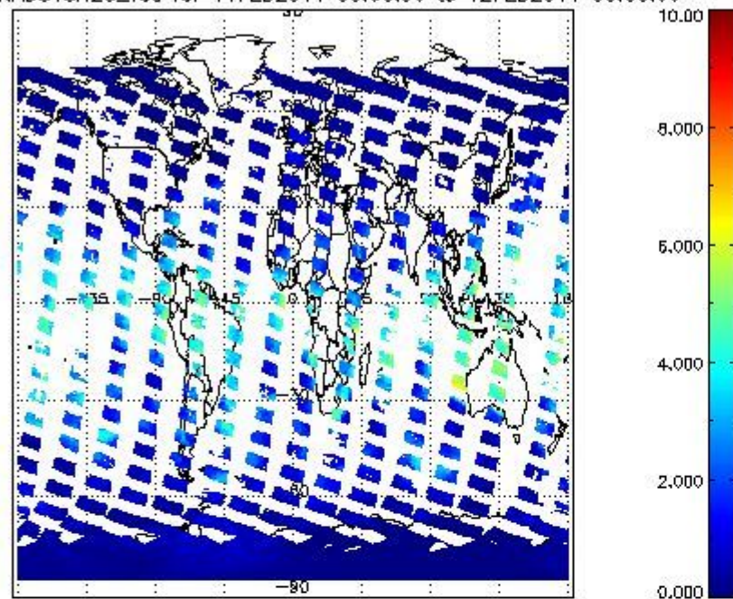
SCIOL2P_NADUV8H2O_vcd for 11FEB2011 00:00:00 to 12FEB2011 00:00:00
