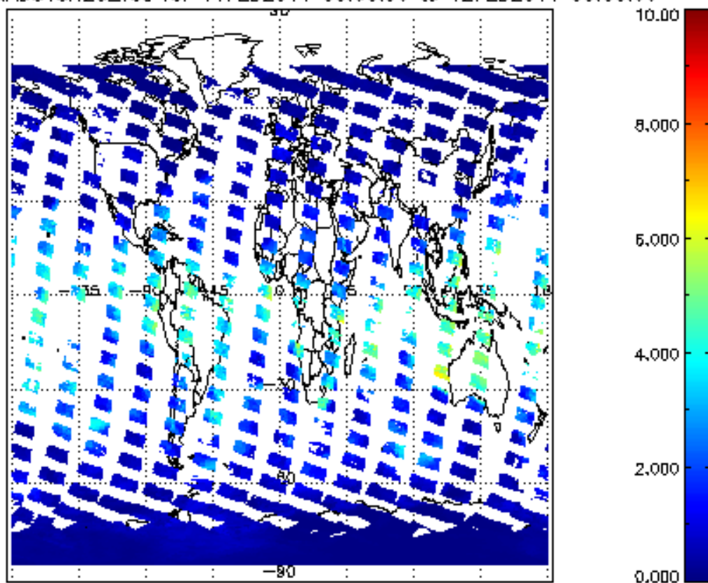
SCIOL2P_NADUV8H2O_vcd for 11FEB2011 00:00:00 to 12FEB2011 00:00:00
