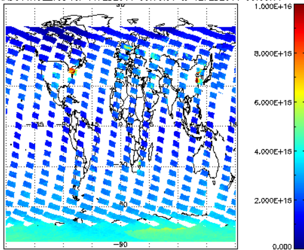
SCIOL2P_NADUV1N02_vcd for 11FEB2011 00:00:00 to 12FEB2011 00:00:00
