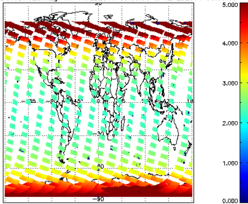
SCIOL2P_NADUV3BRO_amf_gr for 11FEB2011 00:00:00 to 12FEB2011 00:00:00
