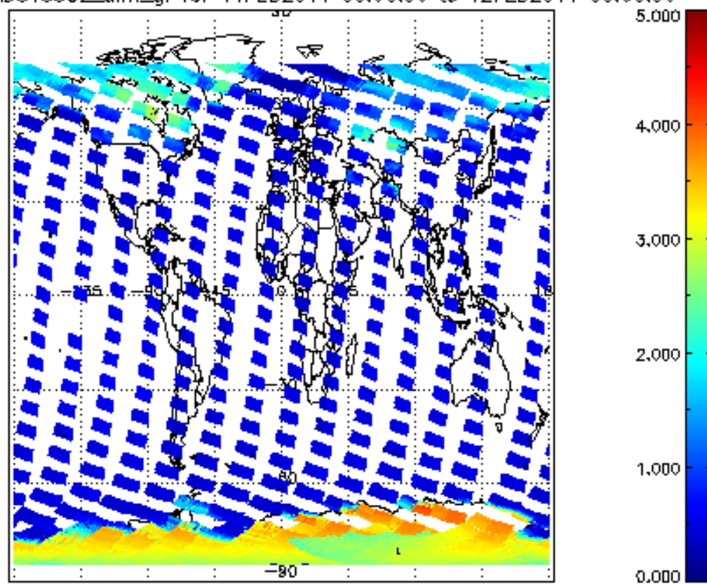
SCIOL2P_NADUV5S02_amf_gr for 11FEB2011 00:00:00 to 12FEB2011 00:00:00
