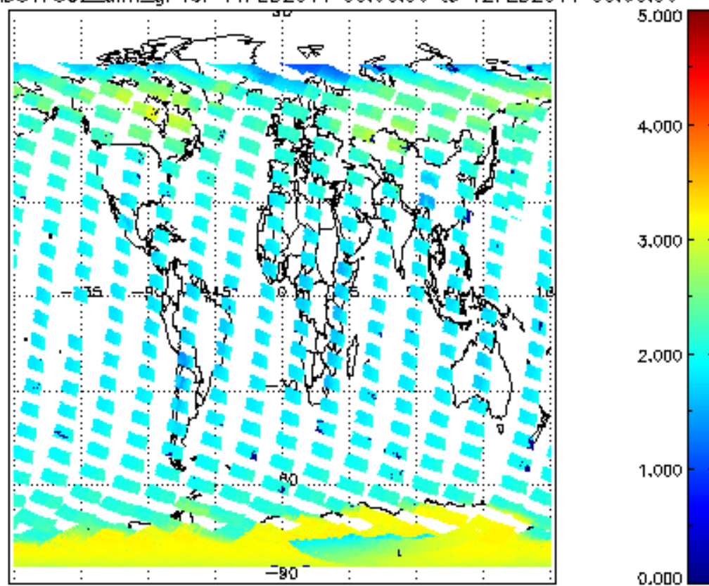
SCIOL2P_NADUV7S02_amf_gr for 11FEB2011 00:00:00 to 12FEB2011 00:00:00
