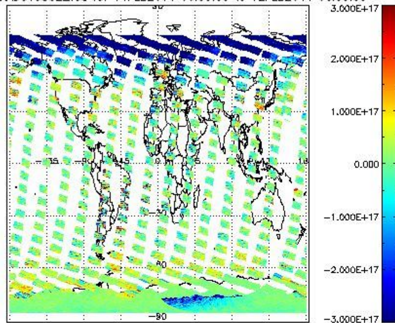
SCIOL2P_NADUV5S02_vcd for 11FEB2011 00:00:00 to 12FEB2011 00:00:00
