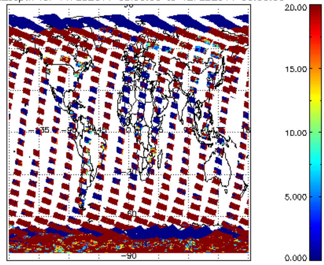
cL_opt_depth for 11FEB2011 00:00:00 to 12FEB2011 00:00:00
