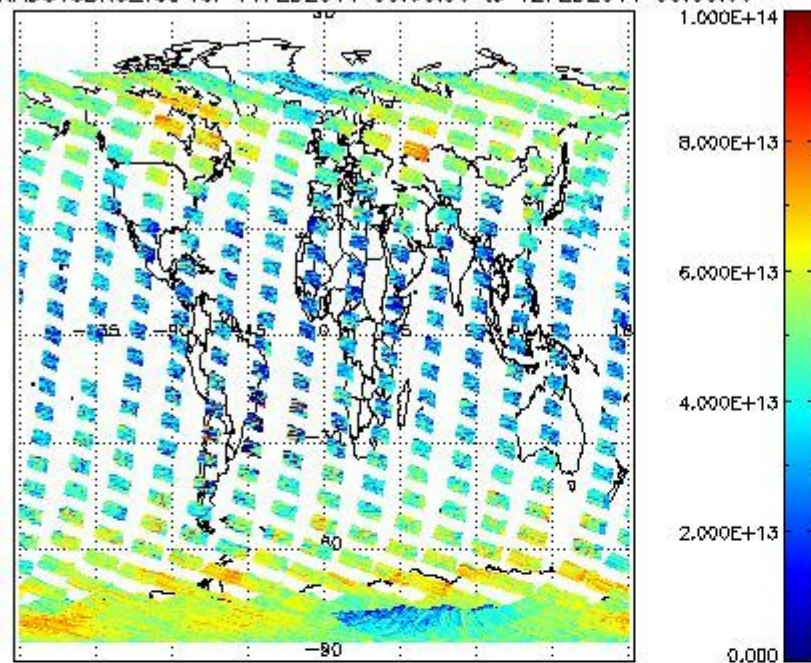
SCIOL2P_NADUV3BRO_vcd for 11FEB2011 00:00:00 to 12FEB2011 00:00:00
