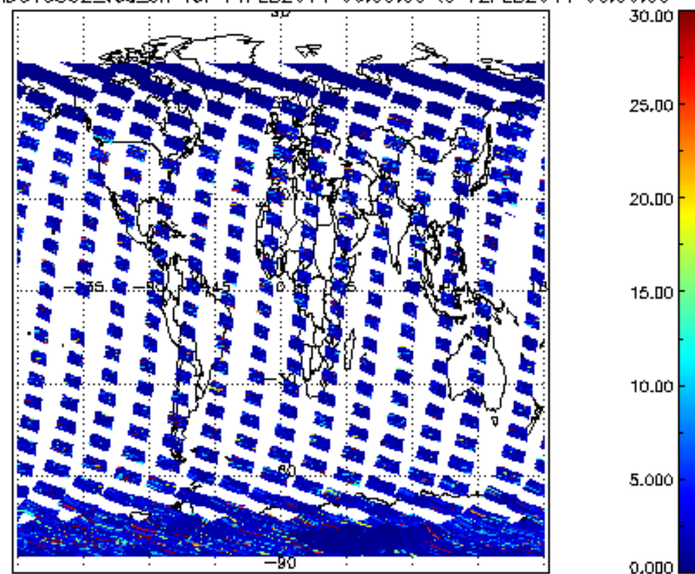
SCIOL2P_NADUV5S02_vcd_err for 11FEB2011 00:00:00 to 12FEB2011 00:00:00
