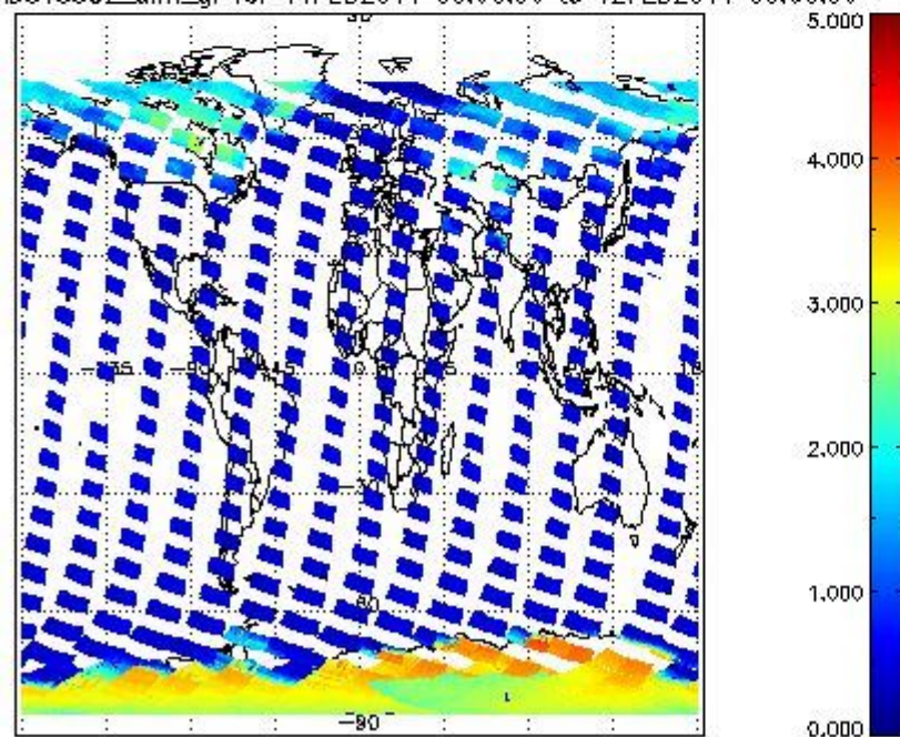
SCIOL2P_NADUV5S02_amf_gr for 11FEB2011 00:00:00 to 12FEB2011 00:00:00
