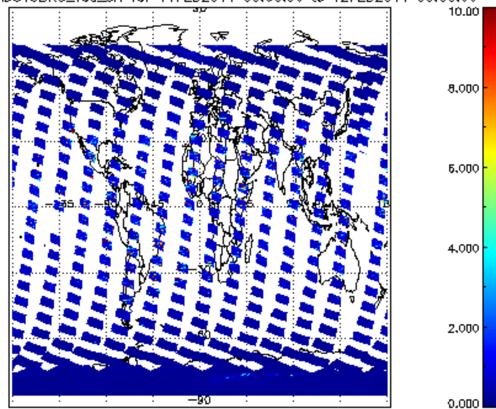
SCIOL2P_NADUV3BRO_vcd_err for 11FEB2011 00:00:00 to 12FEB2011 00:00:00
