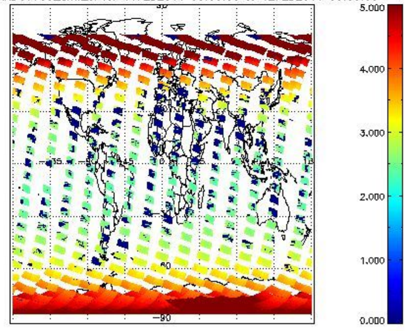
SCIOL2P_NADUV003_amf_cl for 11FEB2011 00:00:00 to 12FEB2011 00:00:00
