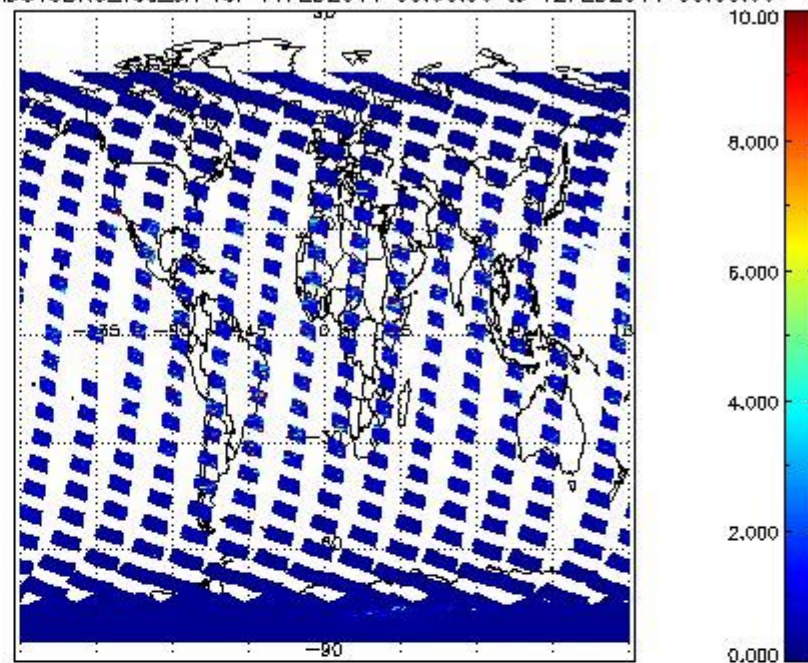
SCIOL2P_NADUV3BRO_vcd_err for 11FEB2011 00:00:00 to 12FEB2011 00:00:00
