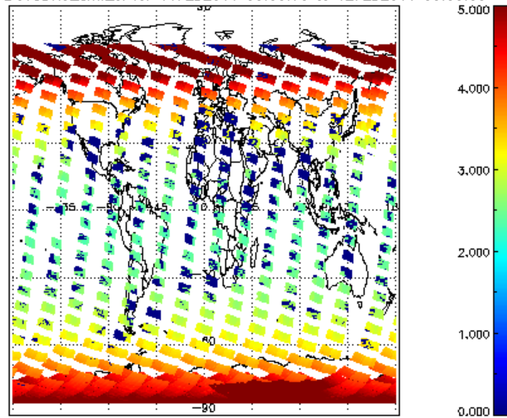
SCIOL2P_NADUV3BRO_amf_cl for 11FEB2011 00:00:00 to 12FEB2011 00:00:00
