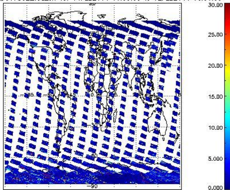
SCIOL2P_NADUV7S02_vcd_err for 11FEB2011 00:00:00 to 12FEB2011 00:00:00
