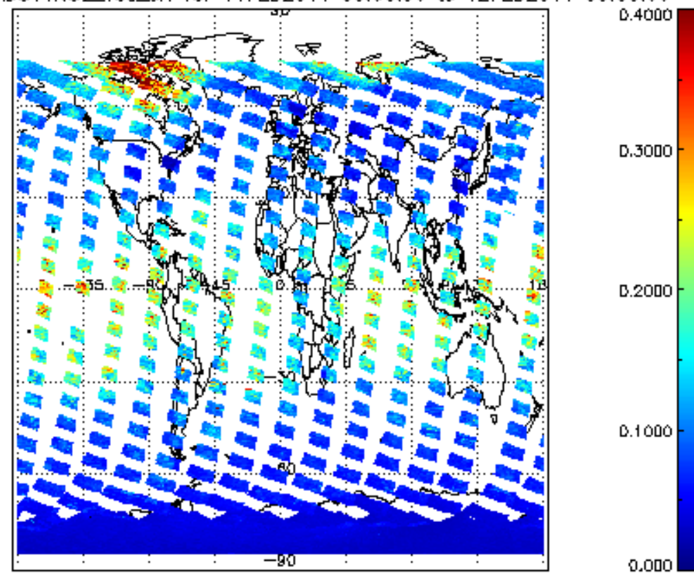
SCIOL2P_NADUV1N02_vcd_err for 11FEB2011 00:00:00 to 12FEB2011 00:00:00
