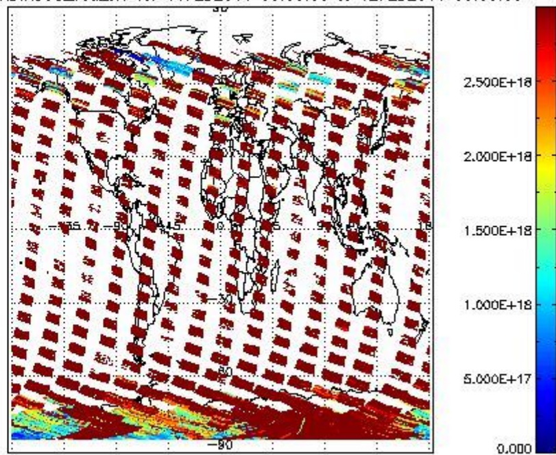
SCIDL2P_NADIR3CO_vcd_err for 11FEB2011 00:00:00 to 12FEB2011 00:00:00
