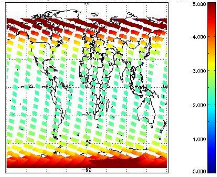
SCIOL2P_NADUV003_amf_gr for 11FEB2011 00:00:00 to 12FEB2011 00:00:00
