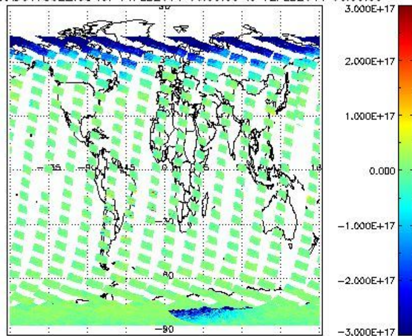
SCIOL2P_NADUV7S02_vcd for 11FEB2011 00:00:00 to 12FEB2011 00:00:00
