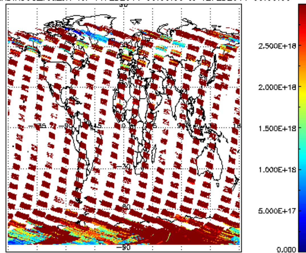
SCIOL2P_NADIR3CO_vcd_err for 11FEB2011 00:00:00 to 12FEB2011 00:00:00
