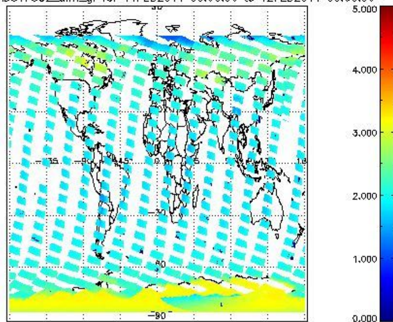
SCIOL2P_NADUV7S02_amf_gr for 11FEB2011 00:00:00 to 12FEB2011 00:00:00
