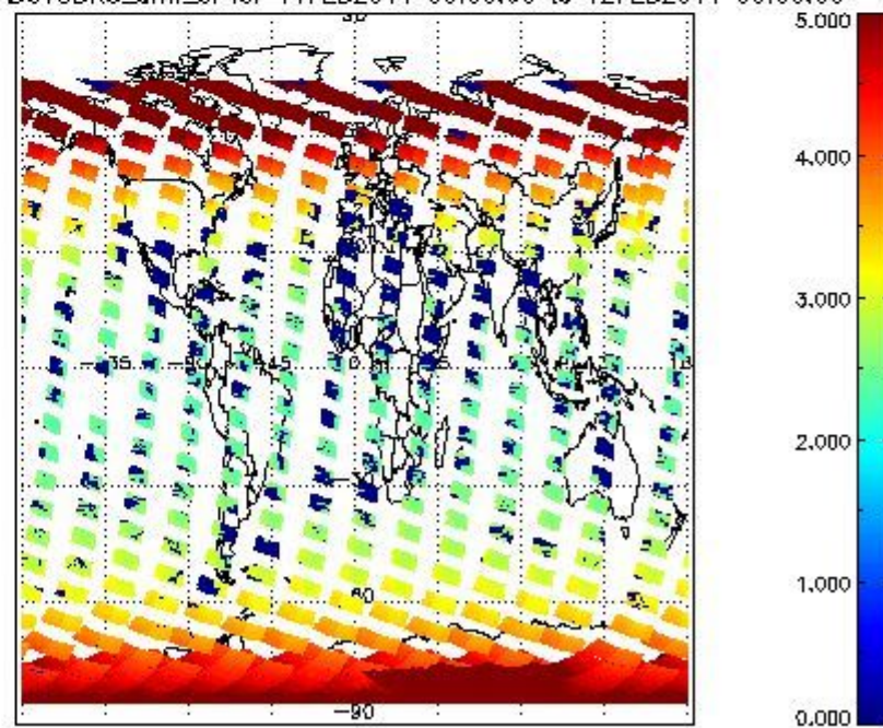
SCIOL2P_NADUV3BRO_amf_cl for 11FEB2011 00:00:00 to 12FEB2011 00:00:00
