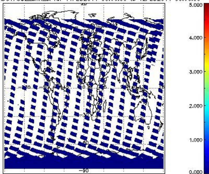
SCIOL2P_NADUV7S02_amf_cl for 11FEB2011 00:00:00 to 12FEB2011 00:00:00
