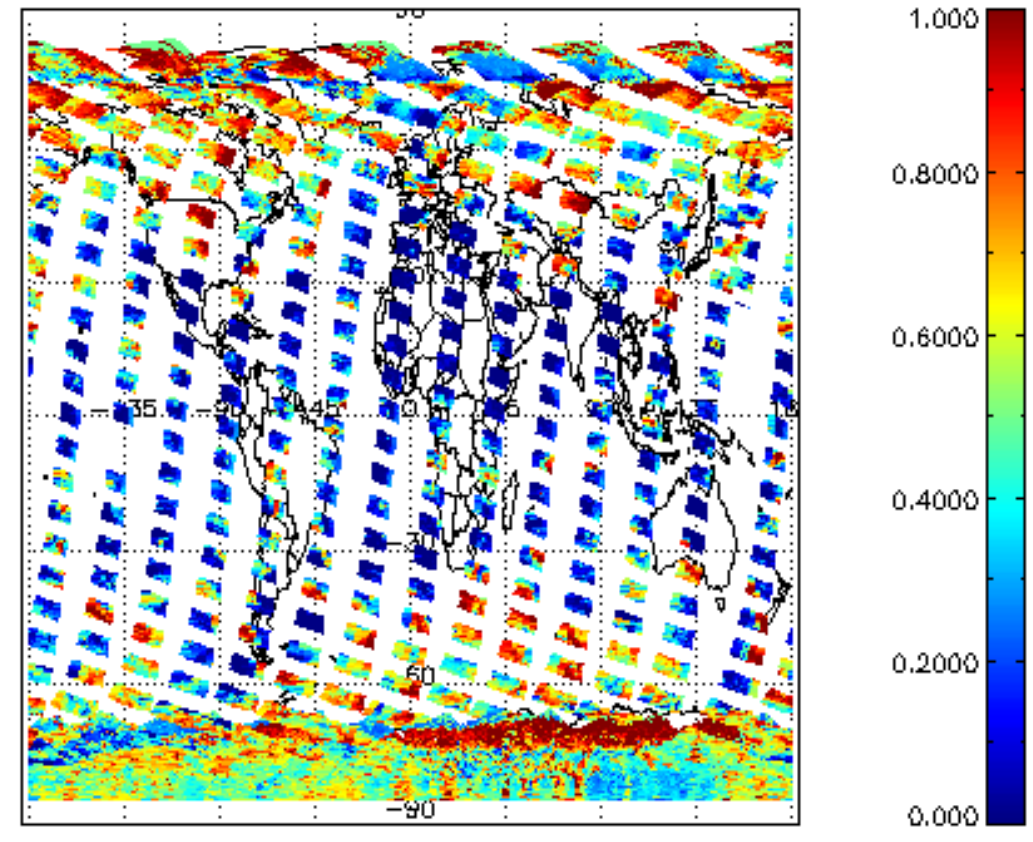
cL_frac for 11FEB2011 00:00:00 to 12FEB2011 00:00:00
