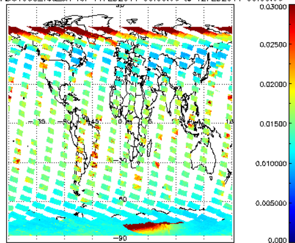
SCIOL2P_NADUV003_vcd_err for 11FEB2011 00:00:00 to 12FEB2011 00:00:00
