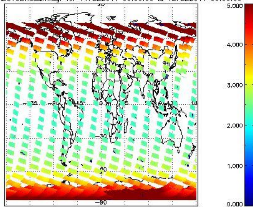
SCIOL2P_NADUV3BRO_amf_gr for 11FEB2011 00:00:00 to 12FEB2011 00:00:00
