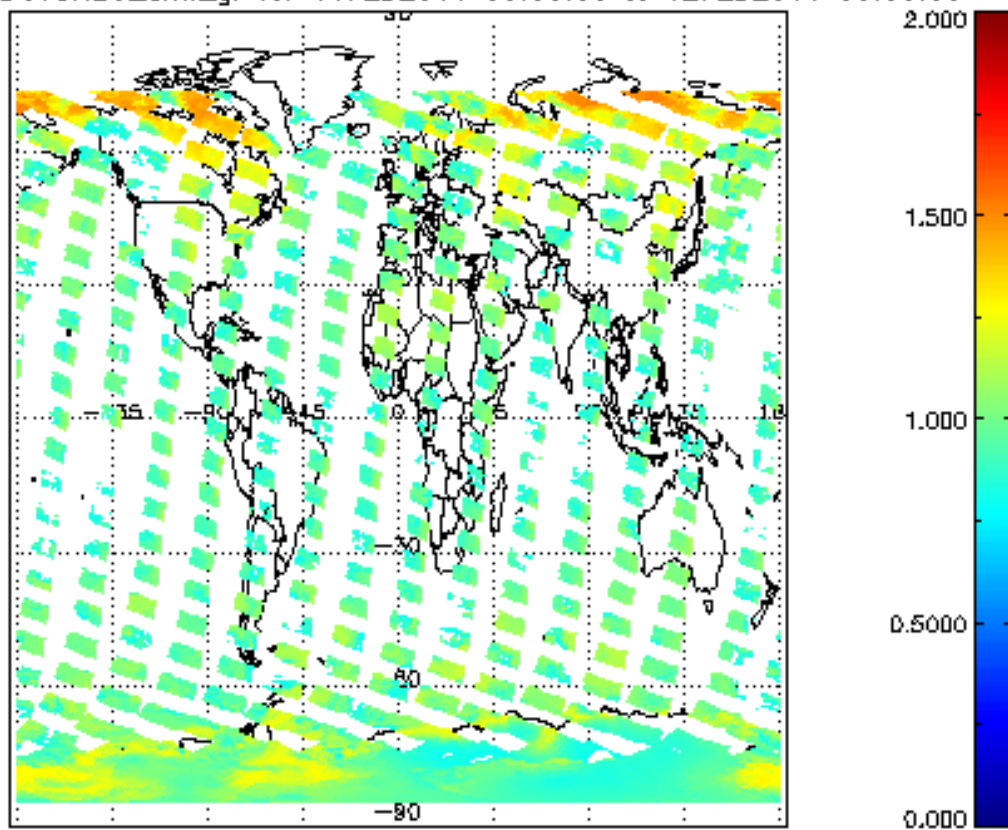
SCIOL2P_NADUV8H2O_amf_gr for 11FEB2011 00:00:00 to 12FEB2011 00:00:00
