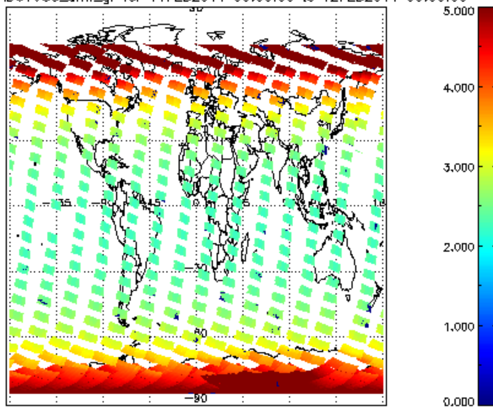
SCIOL2P_NADUV003_amf_gr for 11FEB2011 00:00:00 to 12FEB2011 00:00:00
