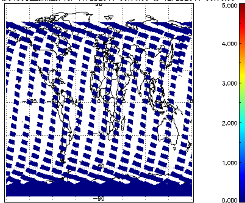
SCIOL2P_NADUV5S02_amf_cl for 11FEB2011 00:00:00 to 12FEB2011 00:00:00
