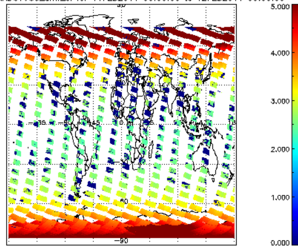
SCIOL2P_NADUV003_amf_cl for 11FEB2011 00:00:00 to 12FEB2011 00:00:00
