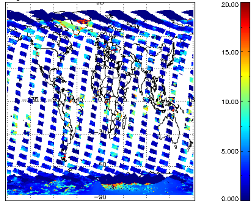
cL_top_height for 11FEB2011 00:00:00 to 12FEB2011 00:00:00
