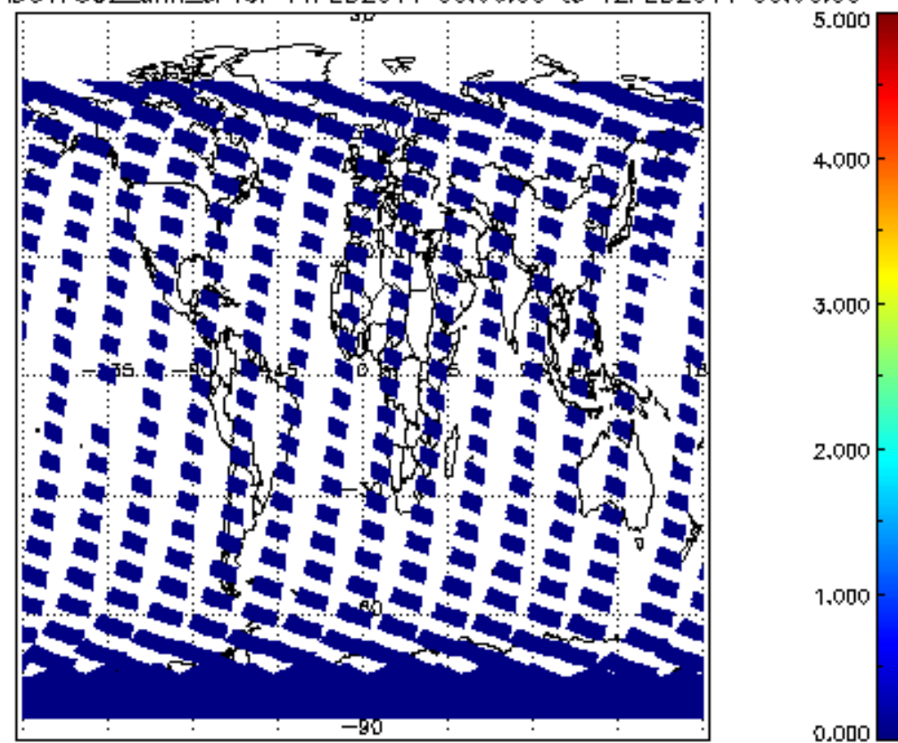
SCIOL2P_NADUV7S02_amf_cl for 11FEB2011 00:00:00 to 12FEB2011 00:00:00
