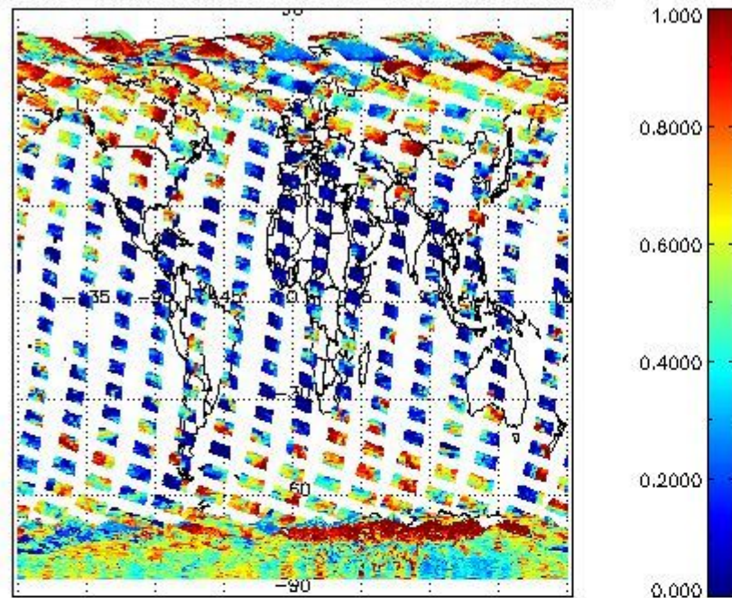
cL_frac for 11FEB2011 00:00:00 to 12FEB2011 00:00:00
