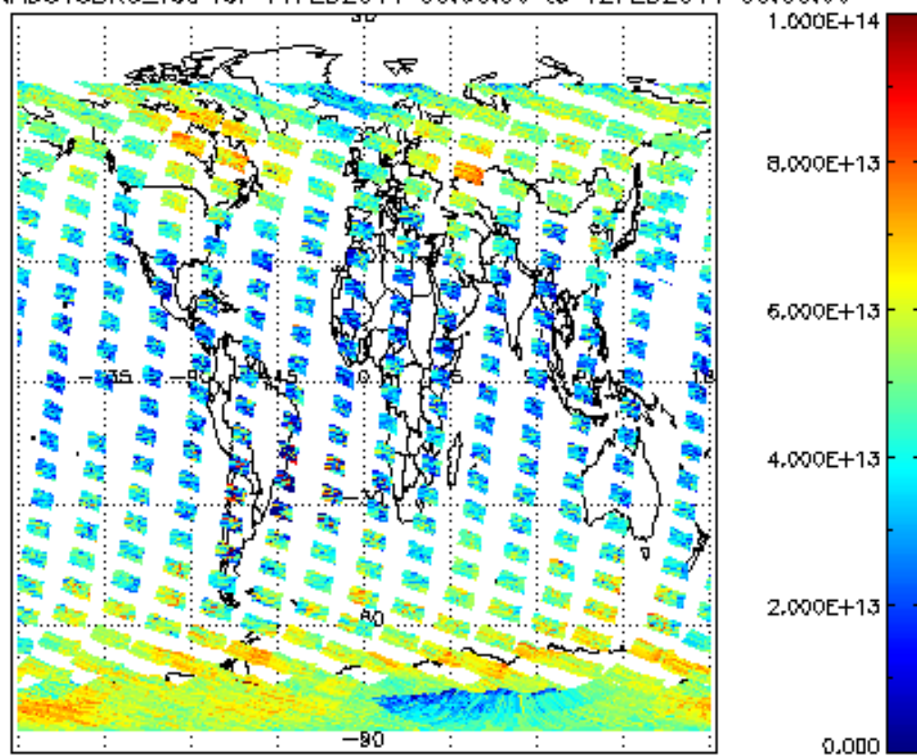
SCIOL2P_NADUV3BRO_vcd for 11FEB2011 00:00:00 to 12FEB2011 00:00:00
