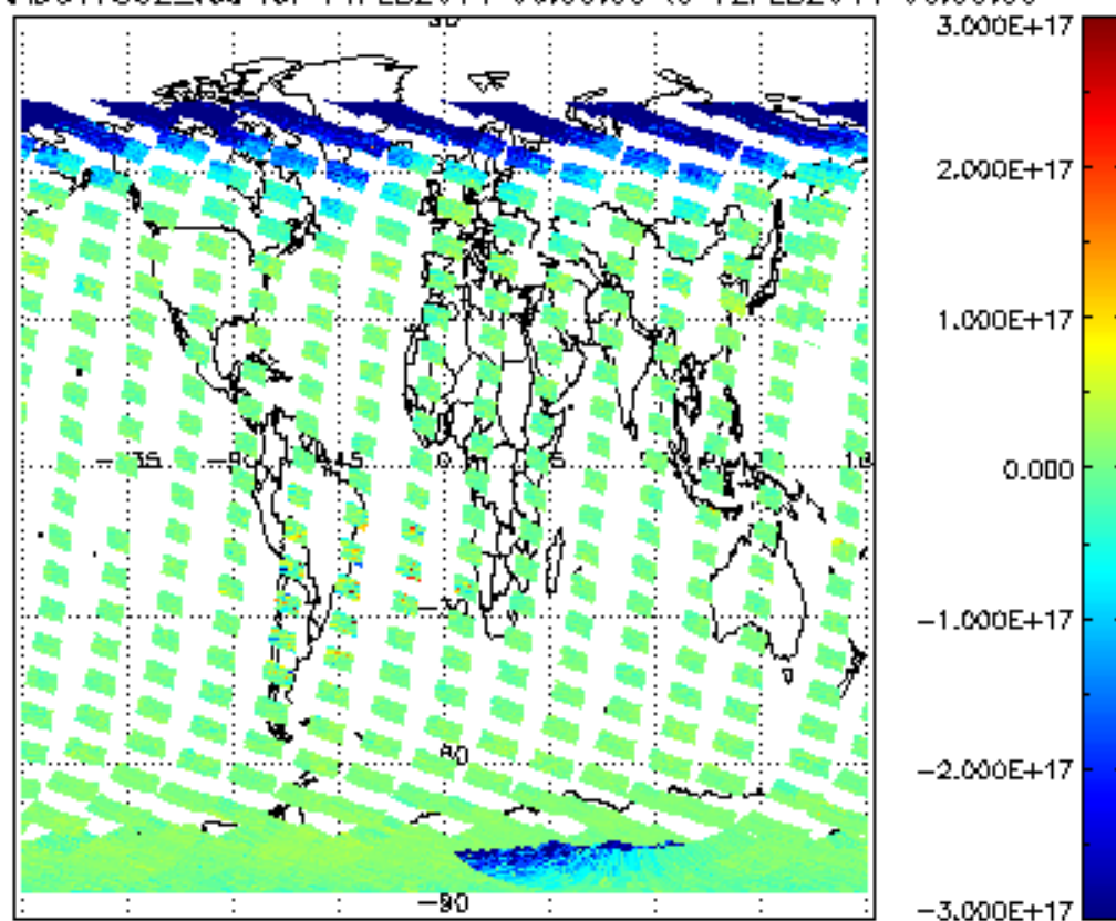
SCIOL2P_NADUV7S02_vcd for 11FEB2011 00:00:00 to 12FEB2011 00:00:00
