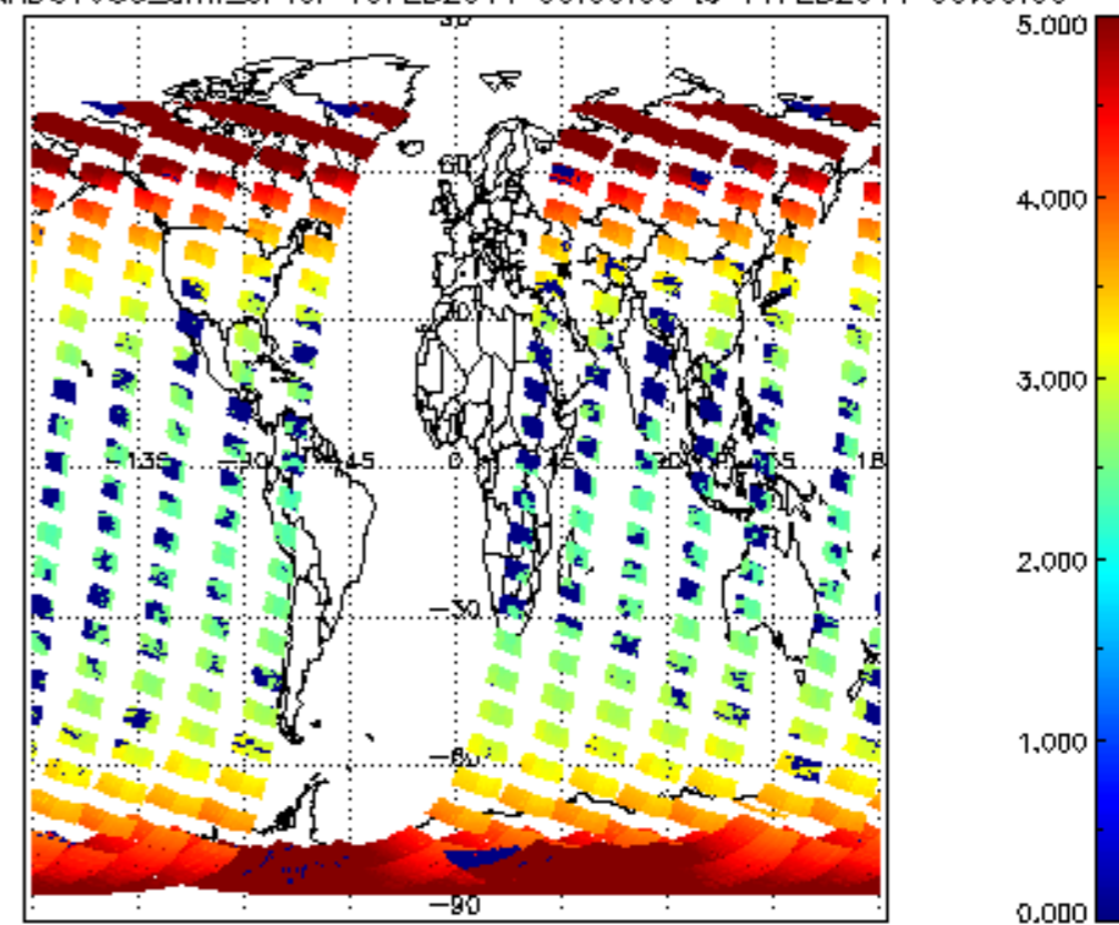
SCIOL2P_NADUV003_amf_cl for 10FEB2011 00:00:00 to 11FEB2011 00:00:00
