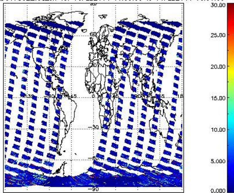
SCIOL2P_NADUV7S02_vcd_err for 10FEB2011 00:00:00 to 11FEB2011 00:00:00
