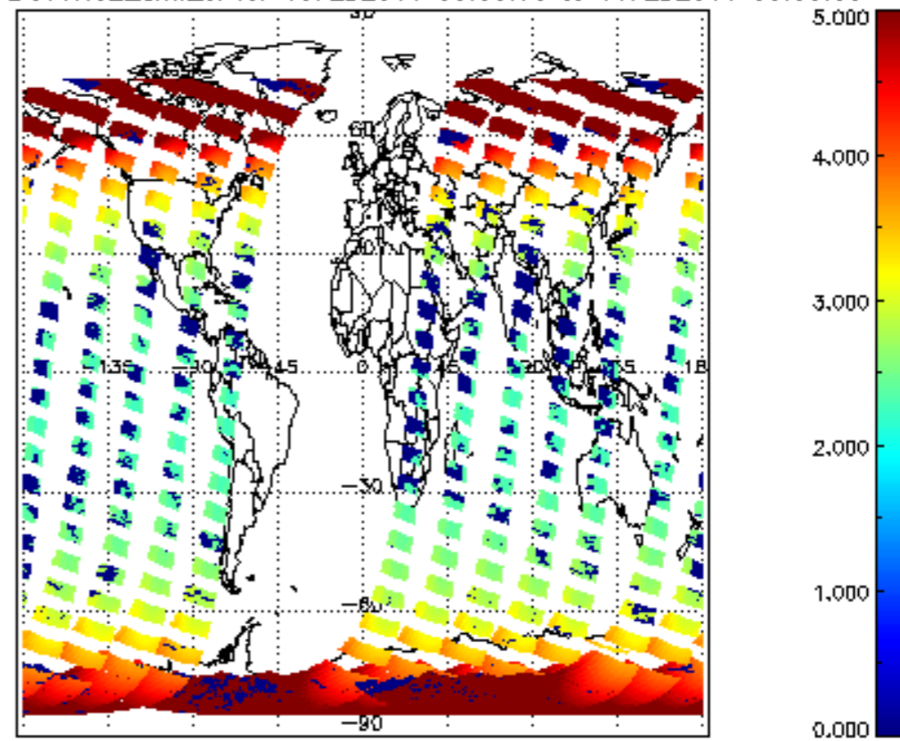
SCIOL2P_NADUV1N02_amf_cl for 10FEB2011 00:00:00 to 11FEB2011 00:00:00
