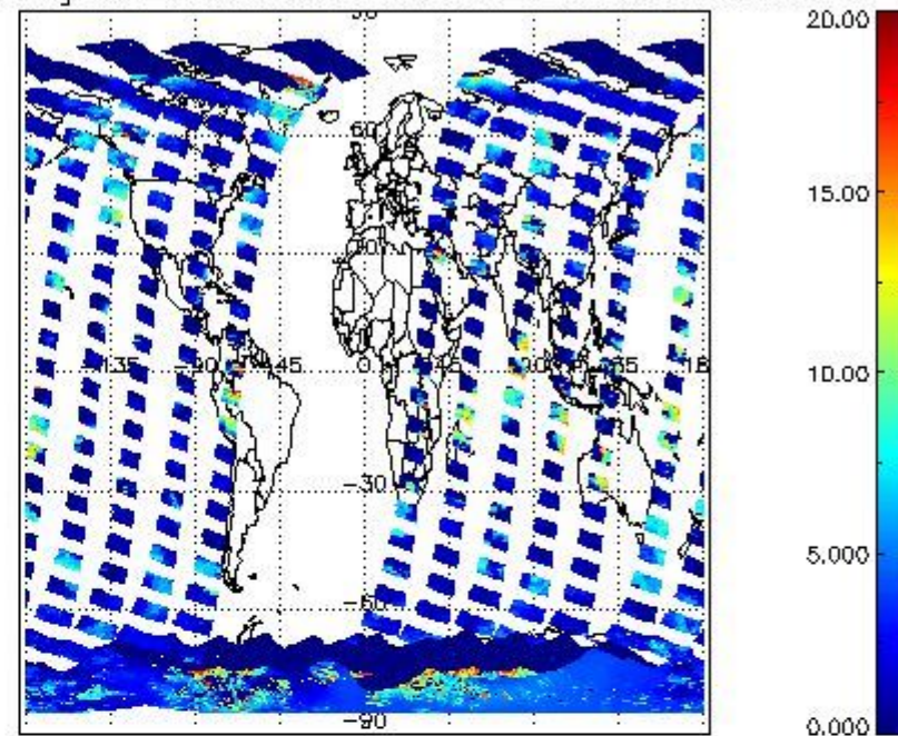
cL_top_height for 10FEB2011 00:00:00 to 11FEB2011 00:00:00
