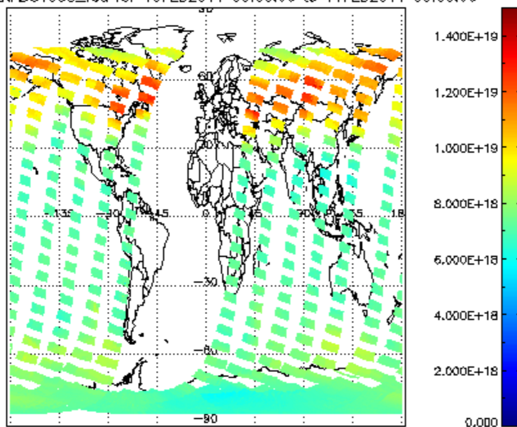
SCIOL2P_NADUV003_vcd for 10FEB2011 00:00:00 to 11FEB2011 00:00:00
