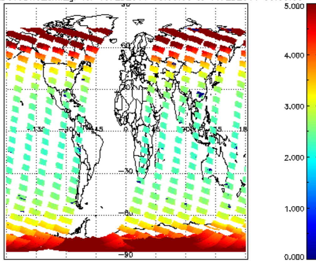
SCIOL2P_NADUV3BRO_amf_gr for 10FEB2011 00:00:00 to 11FEB2011 00:00:00
