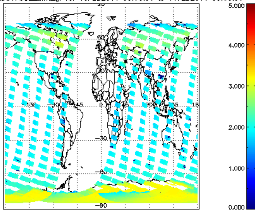
SCIOL2P_NADUV7S02_amf_gr for 10FEB2011 00:00:00 to 11FEB2011 00:00:00
