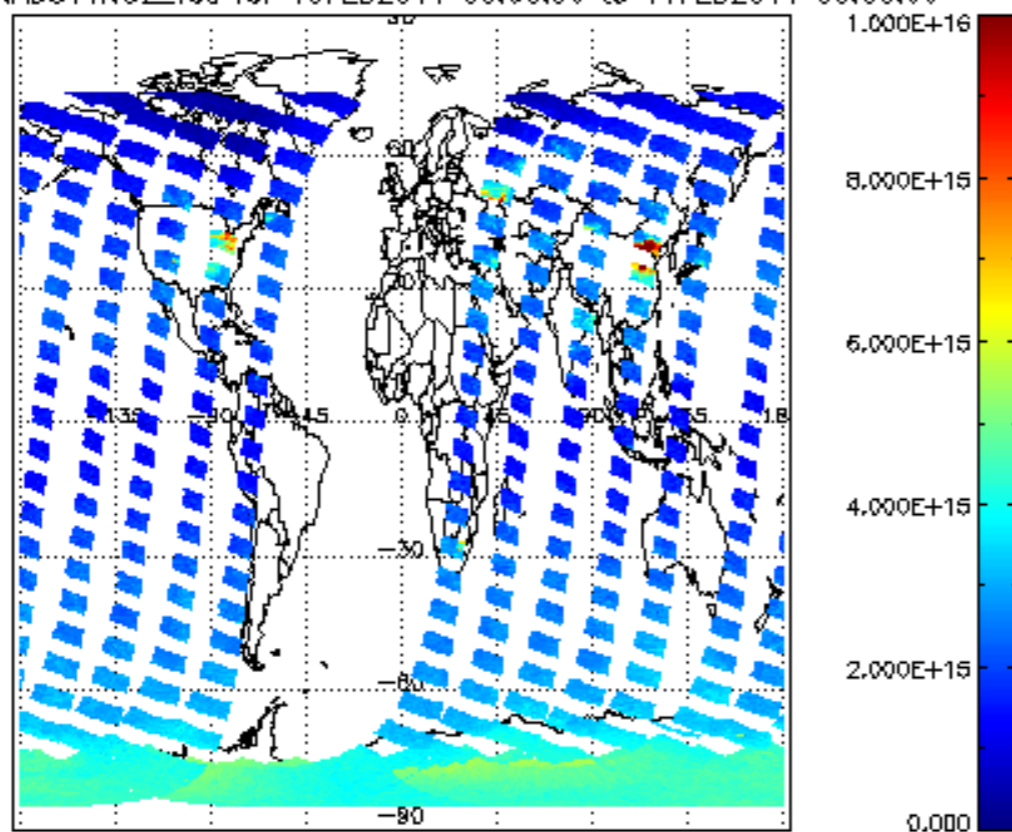
SCIOL2P_NADUV1N02_vcd for 10FEB2011 00:00:00 to 11FEB2011 00:00:00
