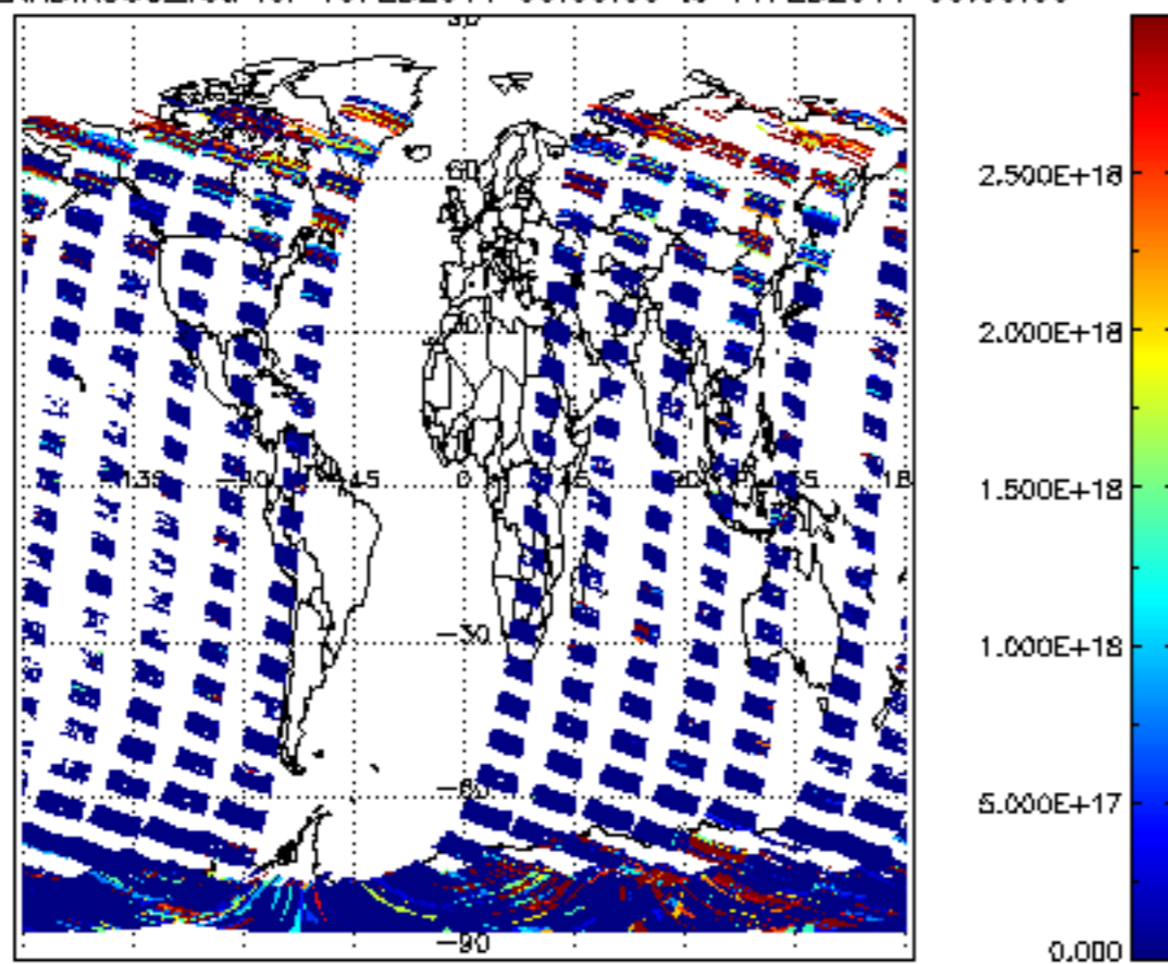
SCIOL2P_NADIR3CO_vcd for 10FEB2011 00:00:00 to 11FEB2011 00:00:00
