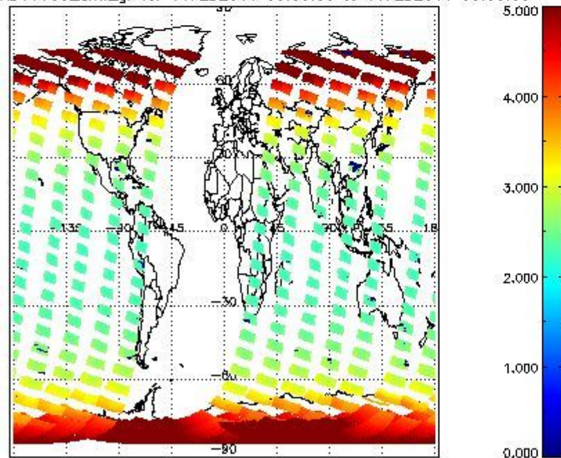
SCIOL2P_NADUV003_amf_gr for 10FEB2011 00:00:00 to 11FEB2011 00:00:00
