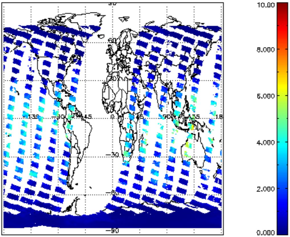
SCIOL2P_NADUV8H2O_vcd for 10FEB2011 00:00:00 to 11FEB2011 00:00:00
