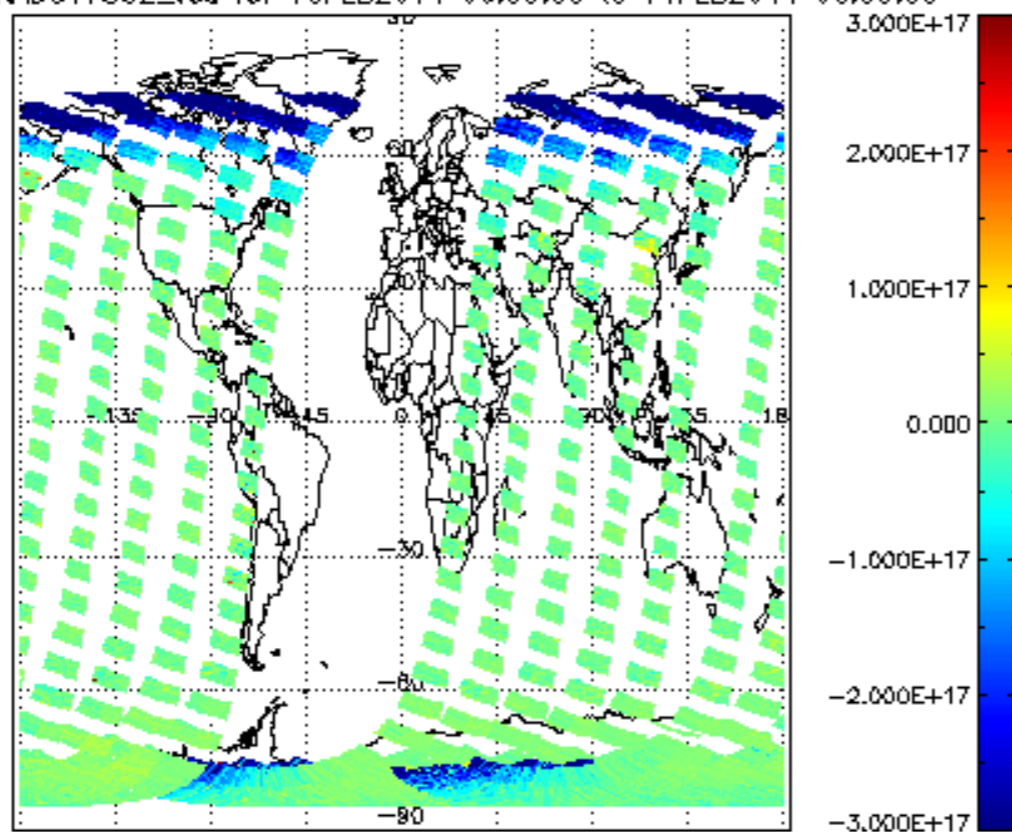
SCIOL2P_NADUV7S02_vcd for 10FEB2011 00:00:00 to 11FEB2011 00:00:00
