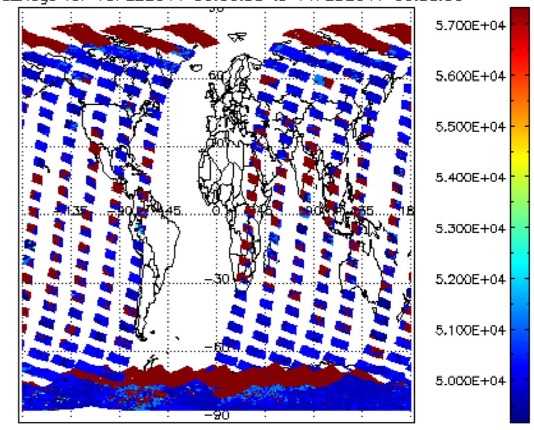
cloud_flags for 10FEB2011 00:00:00 to 11FEB2011 00:00:00
