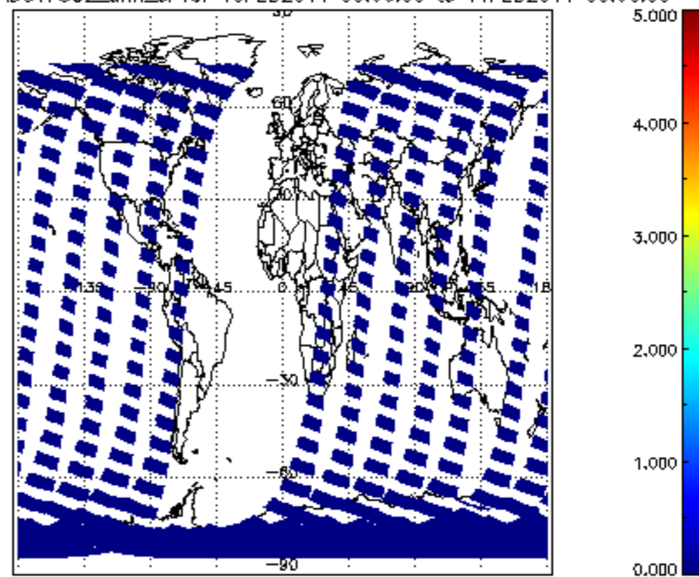
SCIOL2P_NADUV7S02_amf_cl for 10FEB2011 00:00:00 to 11FEB2011 00:00:00
