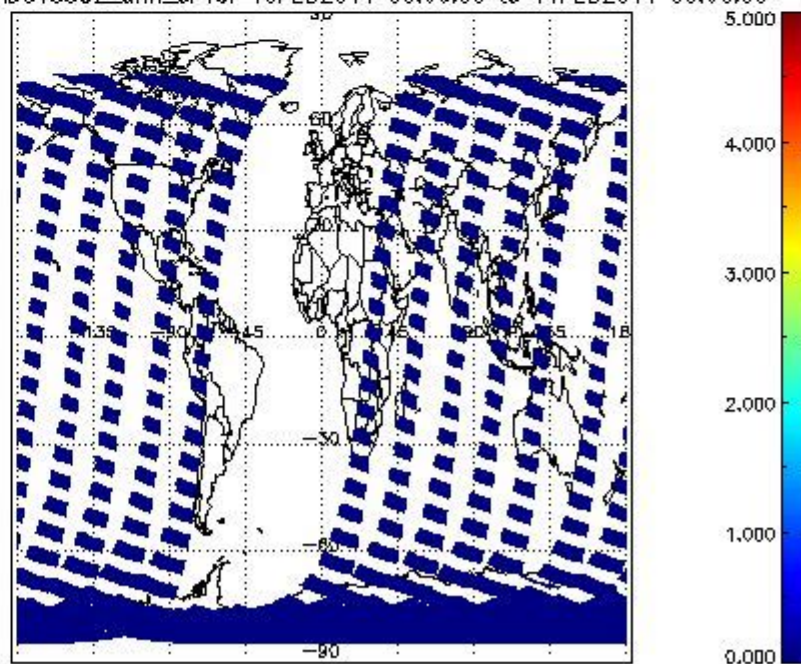
SCIOL2P_NADUV5SO2_amf_cl for 10FEB2011 00:00:00 to 11FEB2011 00:00:00
