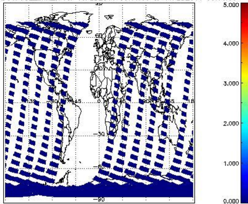
SCIOL2P_NADUV7S02_amf_cl for 10FEB2011 00:00:00 to 11FEB2011 00:00:00
