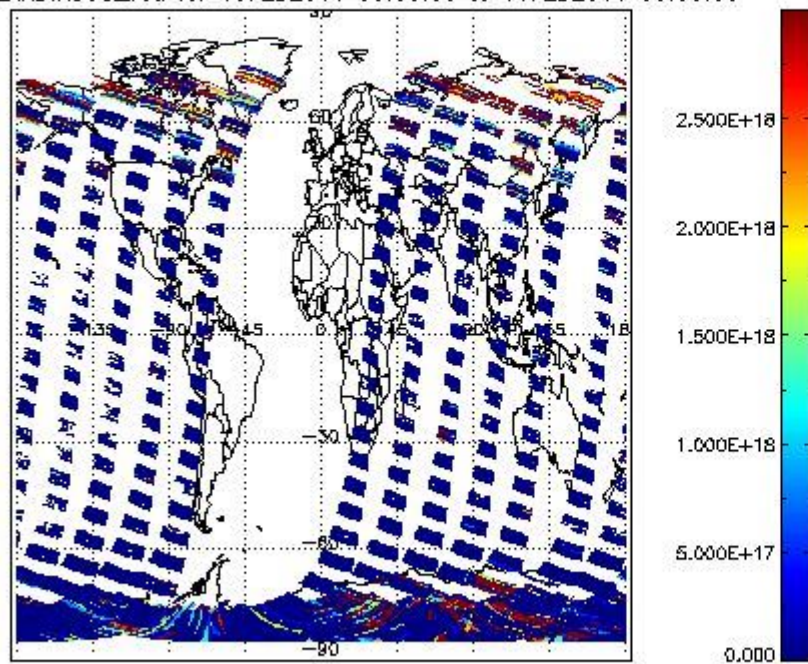
SCIDL2P_NADIR3CO_vcd for 10FEB2011 00:00:00 to 11FEB2011 00:00:00
