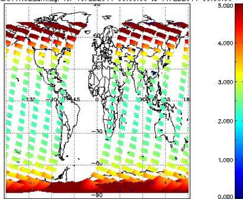
SCIOL2P_NADUV1N02_amf_gr for 10FEB2011 00:00:00 to 11FEB2011 00:00:00
