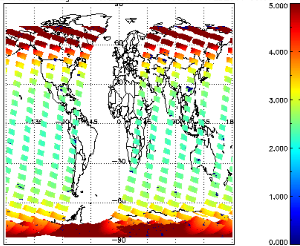
SCIOL2P_NADUV1N02_amf_gr for 10FEB2011 00:00:00 to 11FEB2011 00:00:00
