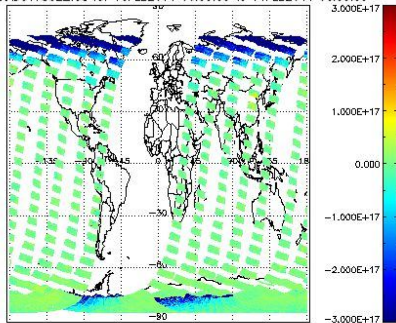
SCIOL2P_NADUV7S02_vcd for 10FEB2011 00:00:00 to 11FEB2011 00:00:00
