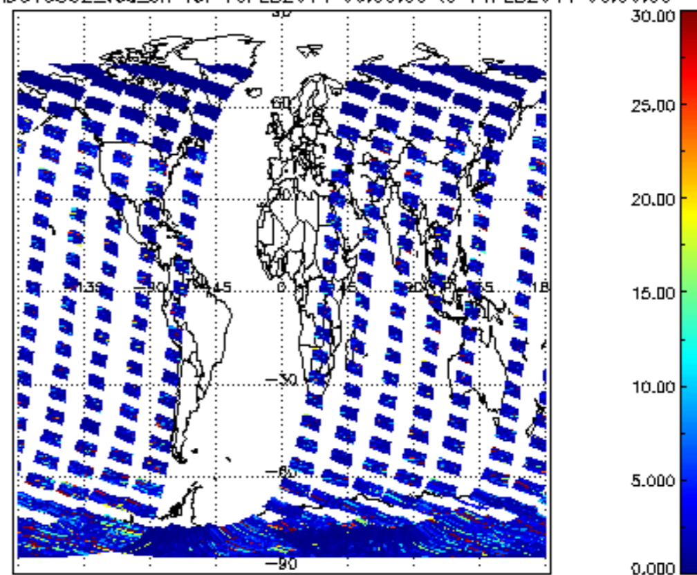
SCIOL2P_NADUV5S02_vcd_err for 10FEB2011 00:00:00 to 11FEB2011 00:00:00
