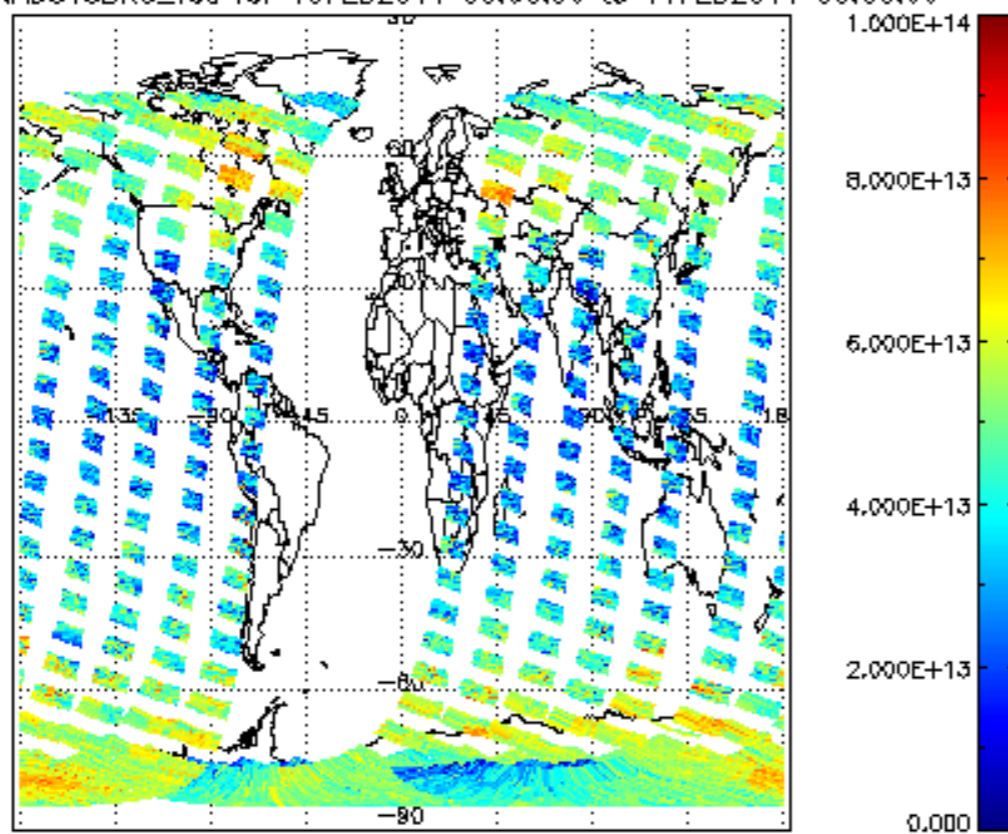
SCIOL2P_NADUV3BRO_vcd for 10FEB2011 00:00:00 to 11FEB2011 00:00:00
