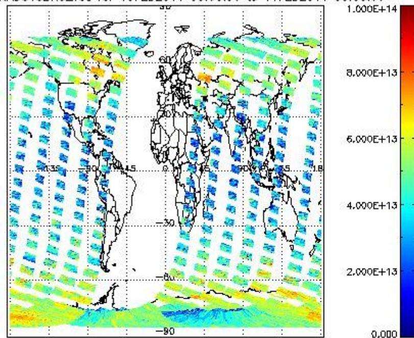
SCIOL2P_NADUV3BRO_vcd for 10FEB2011 00:00:00 to 11FEB2011 00:00:00
