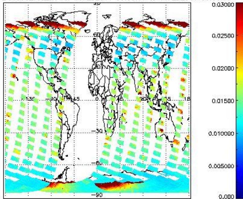
SCIOL2P_NADUV003_vcd_err for 10FEB2011 00:00:00 to 11FEB2011 00:00:00
