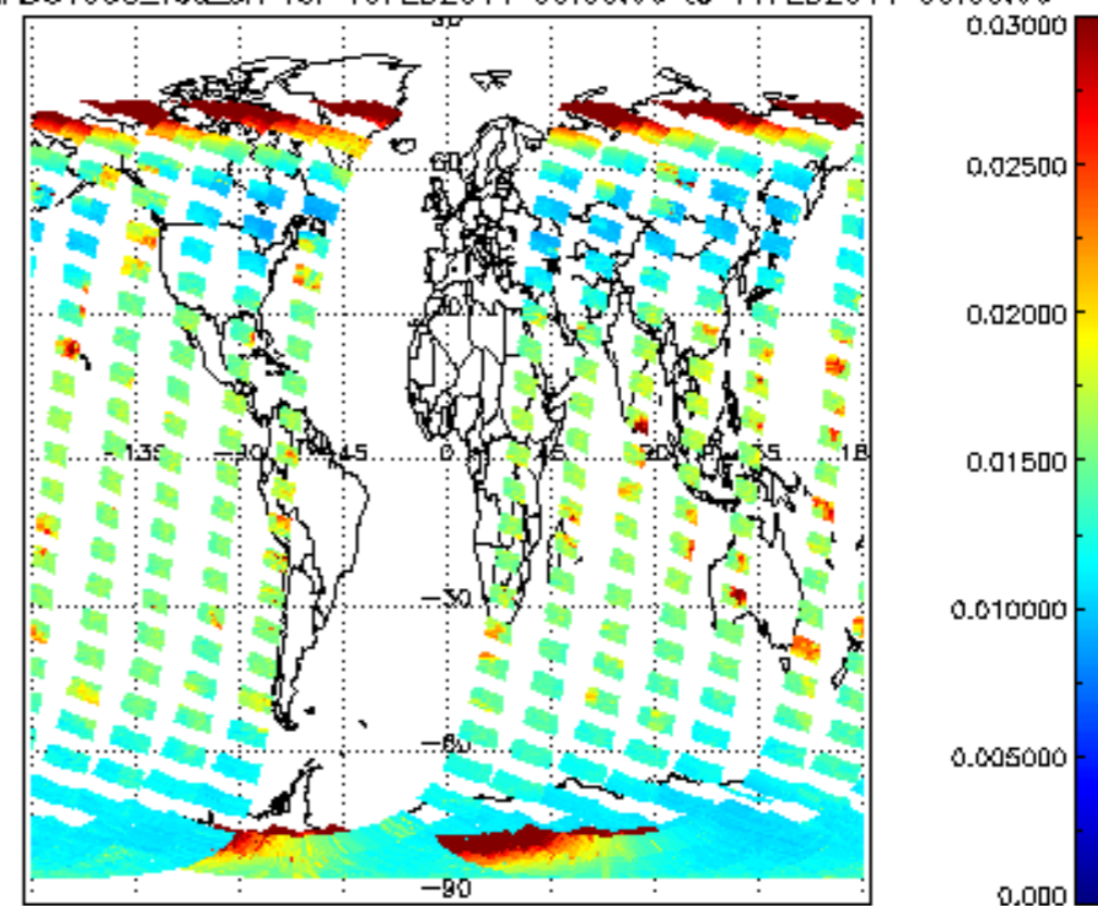
SCIOL2P_NADUV003_vcd_err for 10FEB2011 00:00:00 to 11FEB2011 00:00:00
