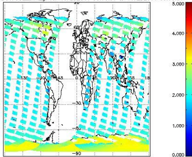
SCIOL2P_NADUV7S02_amf_gr for 10FEB2011 00:00:00 to 11FEB2011 00:00:00
