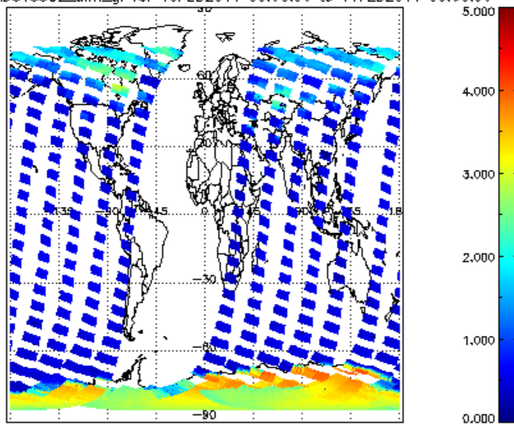
SCIOL2P_NADUV5S02_amf_gr for 10FEB2011 00:00:00 to 11FEB2011 00:00:00
