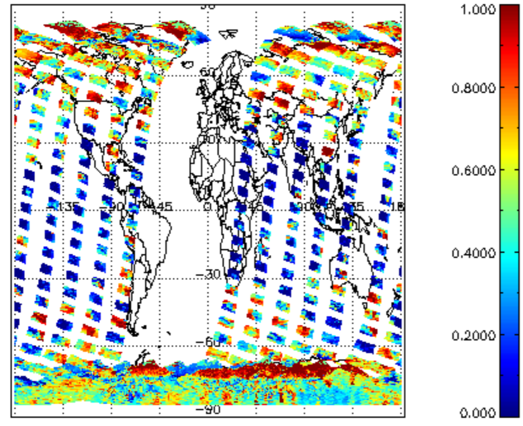
cl_frac for 10FEB2011 00:00:00 to 11FEB2011 00:00:00
