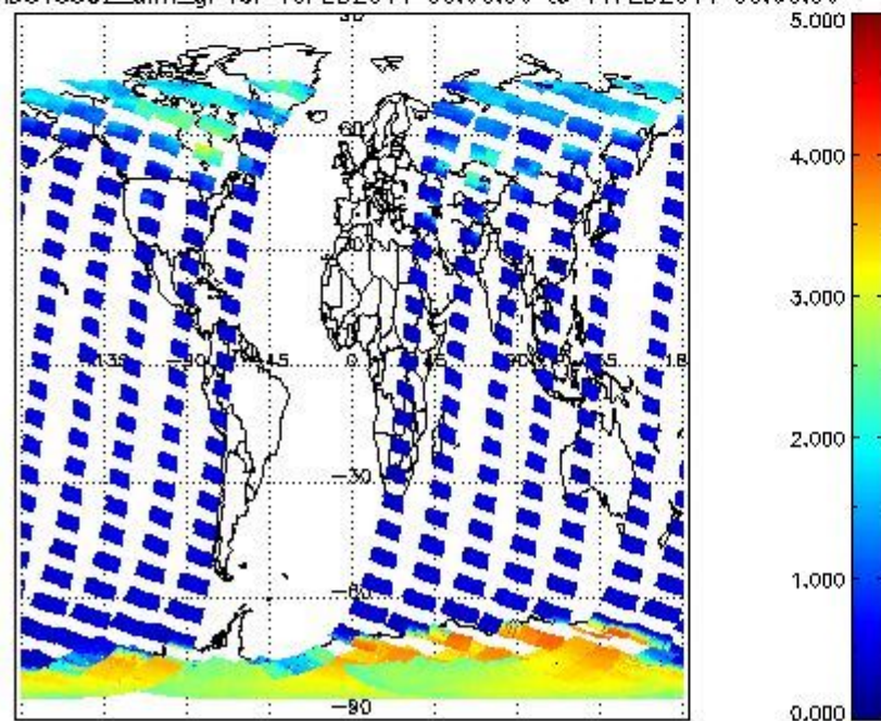
SCIOL2P_NADUV5SO2_amf_gr for 10FEB2011 00:00:00 to 11FEB2011 00:00:00
