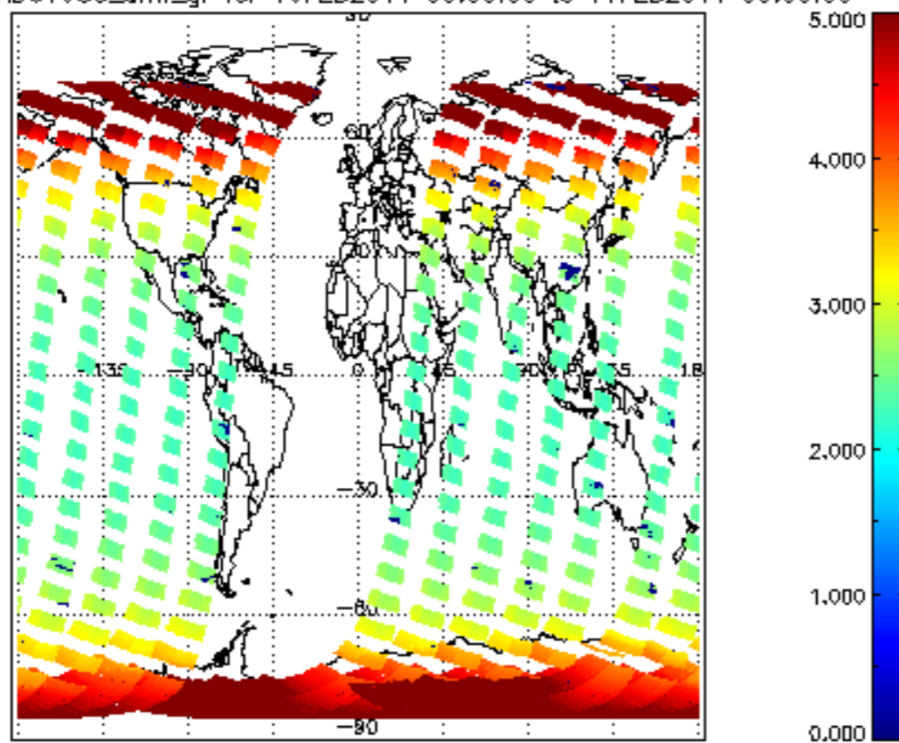
SCIOL2P_NADUV003_amf_gr for 10FEB2011 00:00:00 to 11FEB2011 00:00:00
