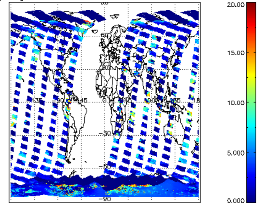
cl_top_height for 10FEB2011 00:00:00 to 11FEB2011 00:00:00
