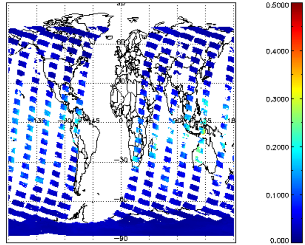
SCIOL2P_NADUV8H2O_vcd_err for 10FEB2011 00:00:00 to 11FEB2011 00:00:00
