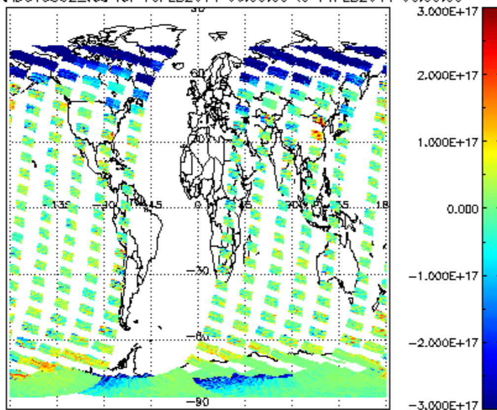
SCIOL2P_NADUV5S02_vcd for 10FEB2011 00:00:00 to 11FEB2011 00:00:00
