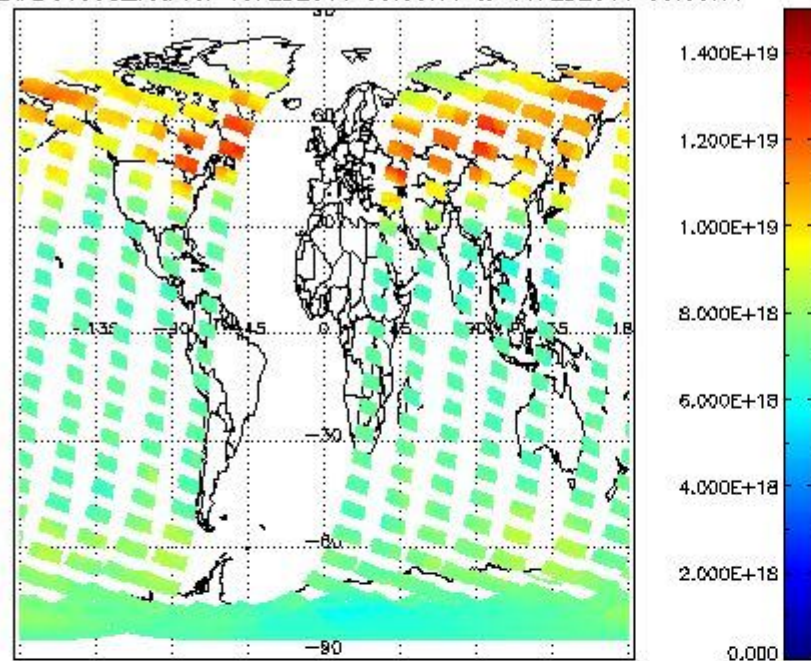
SCIOL2P_NADUV003_vcd for 10FEB2011 00:00:00 to 11FEB2011 00:00:00
