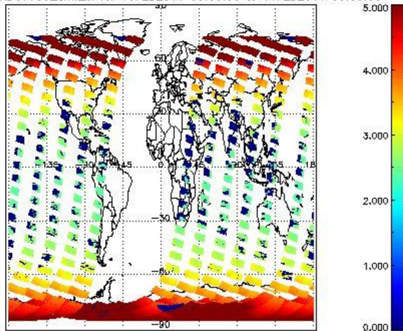
SCIOL2P_NADUV003_amf_cl for 10FEB2011 00:00:00 to 11FEB2011 00:00:00
