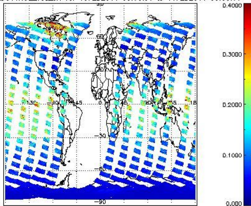
SCIOL2P_NADUV1N02_vcd_err for 10FEB2011 00:00:00 to 11FEB2011 00:00:00
