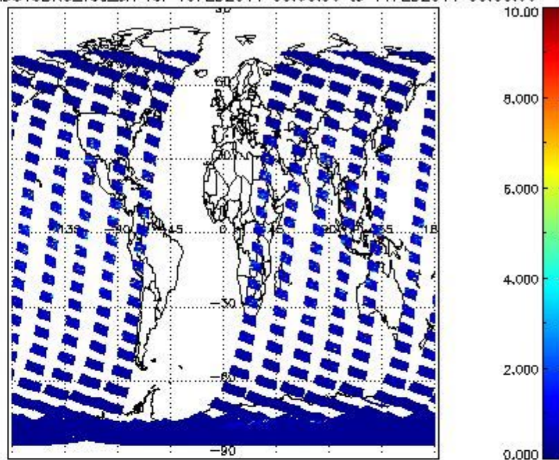
SCIOL2P_NADUV3BRO_vcd_err for 10FEB2011 00:00:00 to 11FEB2011 00:00:00
