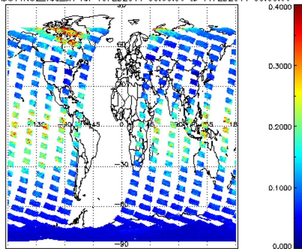
SCIOL2P_NADUV1N02_vcd_err for 10FEB2011 00:00:00 to 11FEB2011 00:00:00
