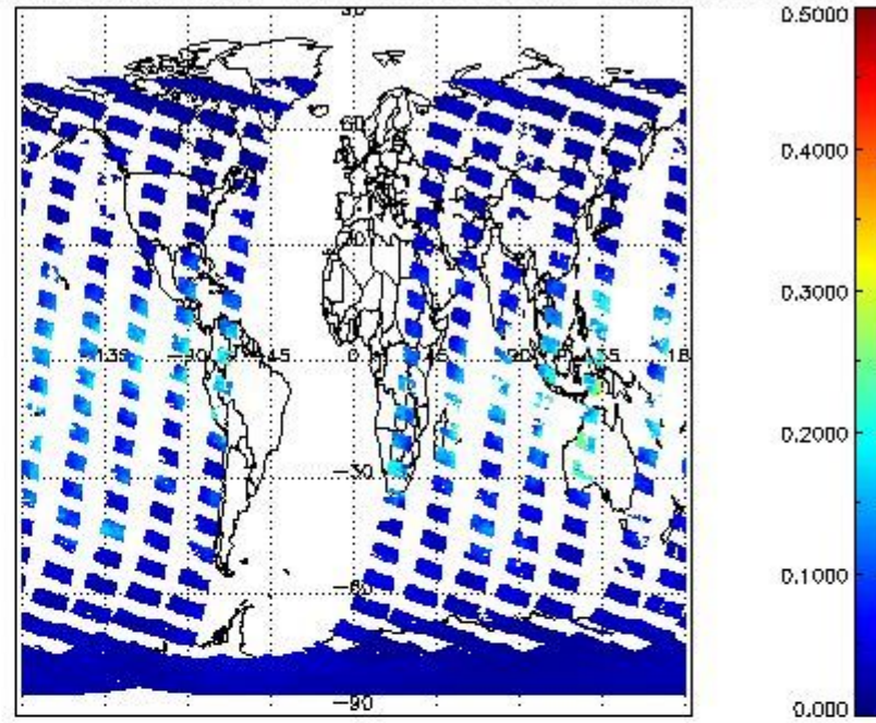
SCIOL2P_NADUV8H2O_vcd_err for 10FEB2011 00:00:00 to 11FEB2011 00:00:00
