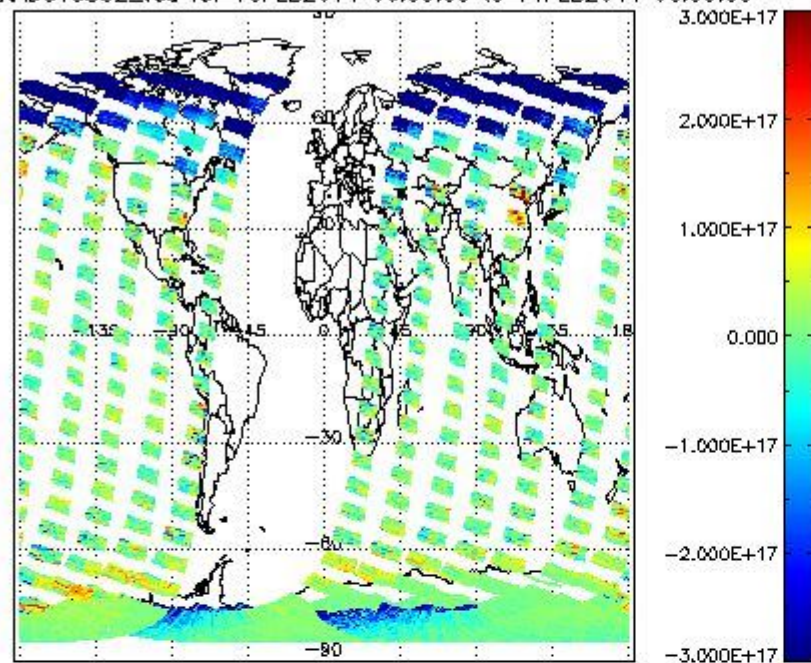
SCIOL2P_NADUV5SO2_vcd for 10FEB2011 00:00:00 to 11FEB2011 00:00:00
