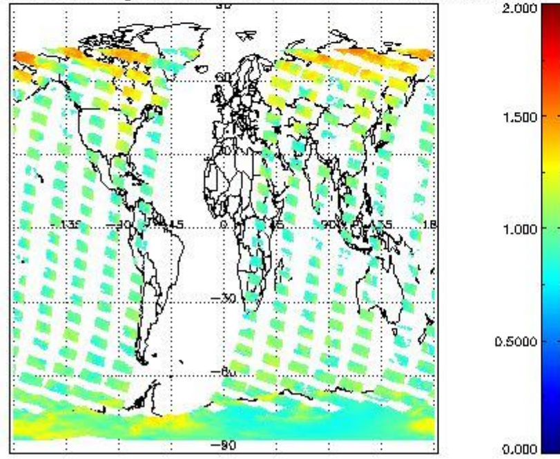
SCIOL2P_NADUV8H2O_amf_gr for 10FEB2011 00:00:00 to 11FEB2011 00:00:00
