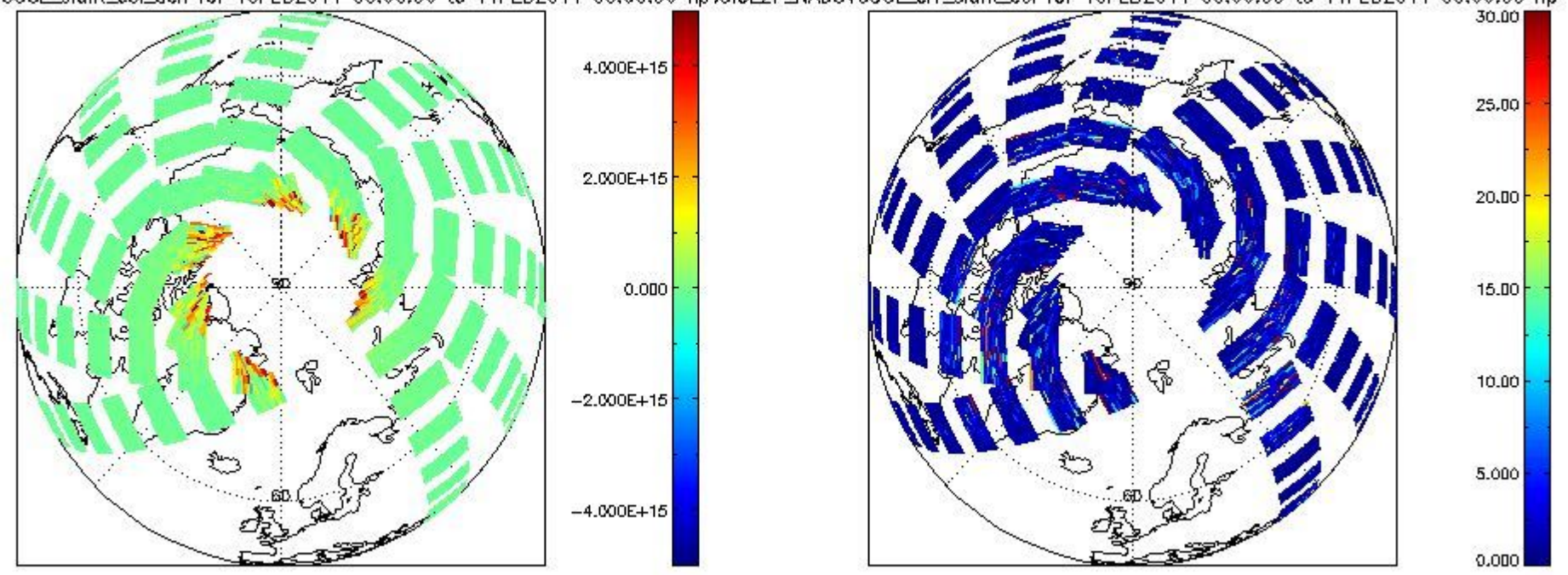
CIOL2P_NADUV60CLslant_col_den for 10FEB2011 00:00:00 to 11FEB2011 00:00:00 np; CIOL2P_NADUV60CLarr_slant_col for 10FEB2011 00:00:00 to 11FEB2011 00:00:00 np
