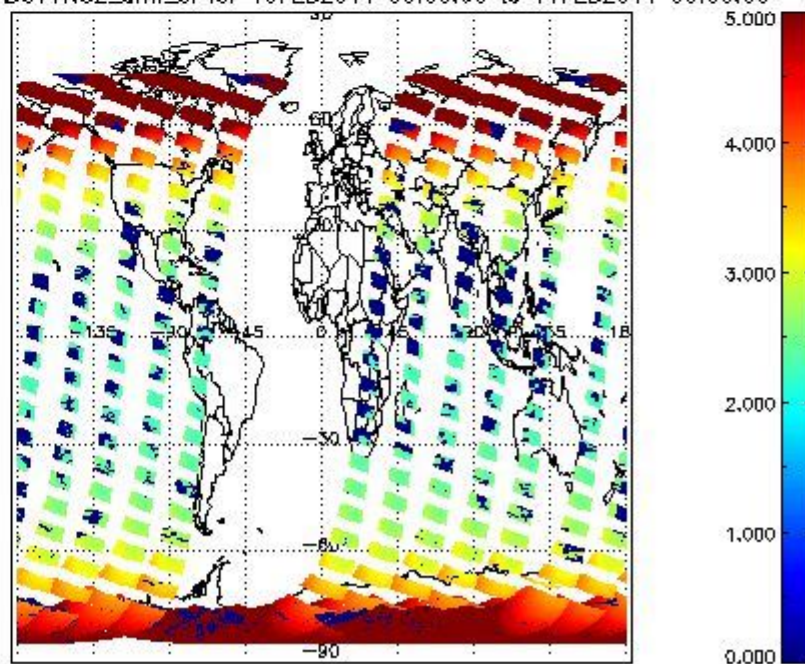
SCIOL2P_NADUV1N02_amf_cl for 10FEB2011 00:00:00 to 11FEB2011 00:00:00
