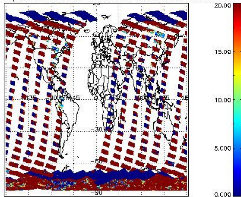
cL_opt_depth for 10FEB2011 00:00:00 to 11FEB2011 00:00:00
