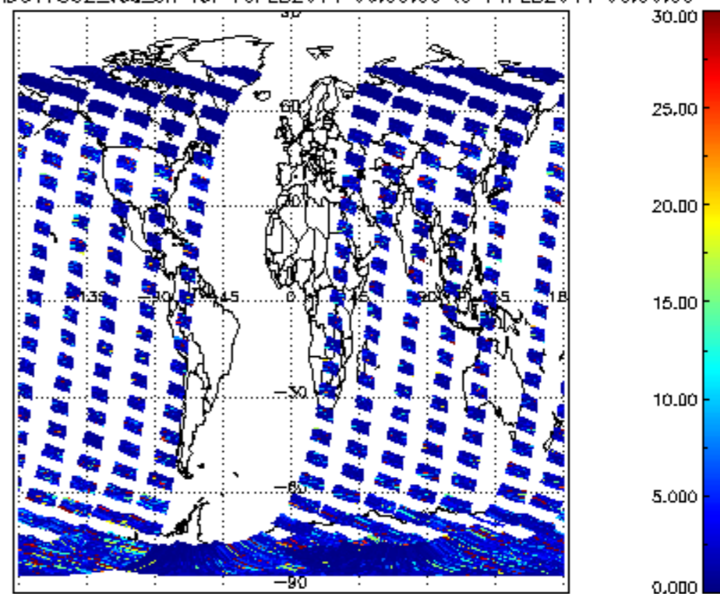
SCIOL2P_NADUV7S02_vcd_err for 10FEB2011 00:00:00 to 11FEB2011 00:00:00
