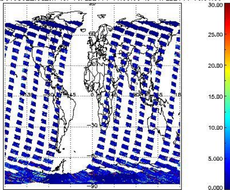
SCIOL2P_NADUV5SO2_vcd_err for 10FEB2011 00:00:00 to 11FEB2011 00:00:00
