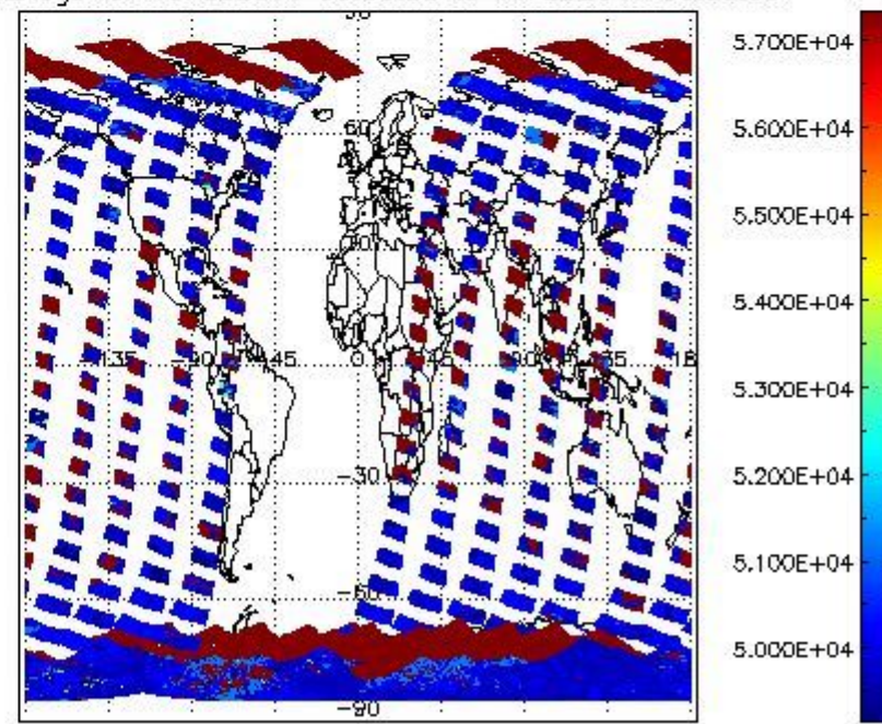
cloud_flags for 10FEB2011 00:00:00 to 11FEB2011 00:00:00
