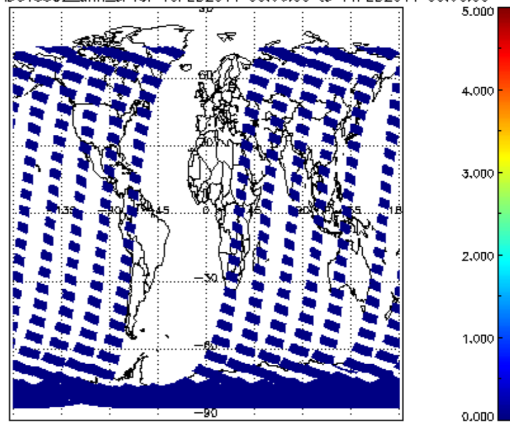
SCIOL2P_NADUV5S02_amf_cl for 10FEB2011 00:00:00 to 11FEB2011 00:00:00
