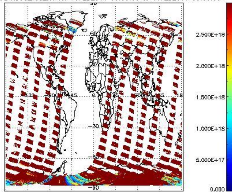
SCIDL2P_NADIR3CO_vcd_err for 10FEB2011 00:00:00 to 11FEB2011 00:00:00
