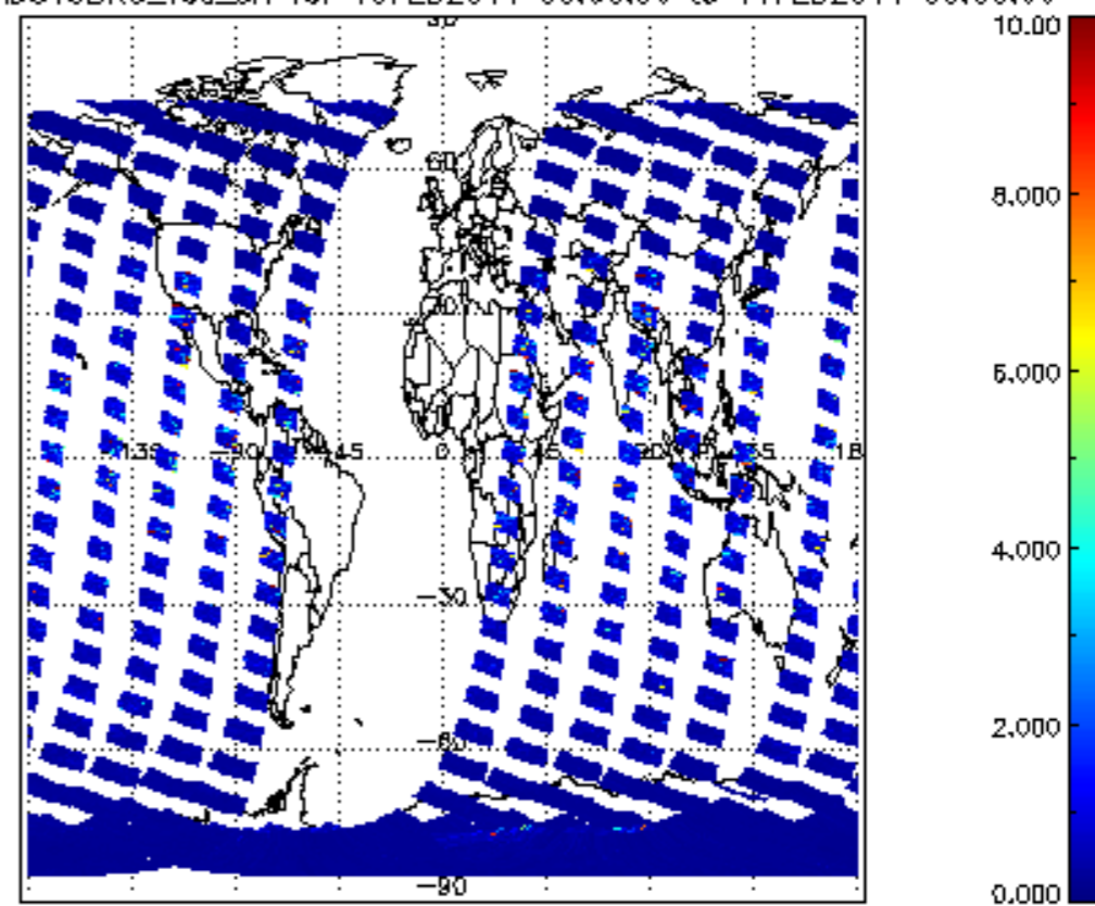
SCIOL2P_NADUV3BRO_vcd_err for 10FEB2011 00:00:00 to 11FEB2011 00:00:00
