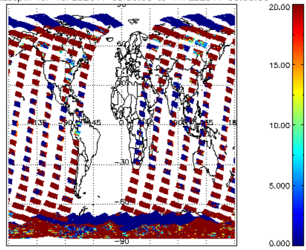
cl_lopt_depth for 10FEB2011 00:00:00 to 11FEB2011 00:00:00
