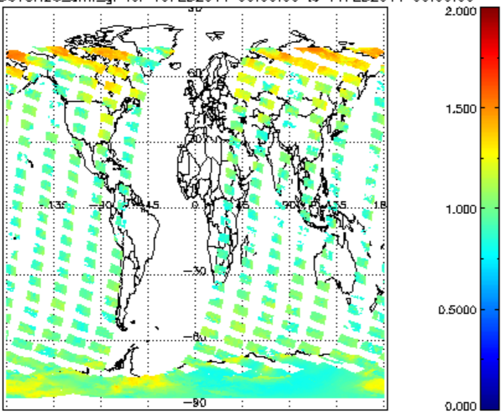
SCIOL2P_NADUV8H2O_amf_gr for 10FEB2011 00:00:00 to 11FEB2011 00:00:00
