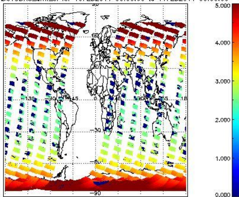
SCIOL2P_NADUV3BRO_amf_cl for 10FEB2011 00:00:00 to 11FEB2011 00:00:00
