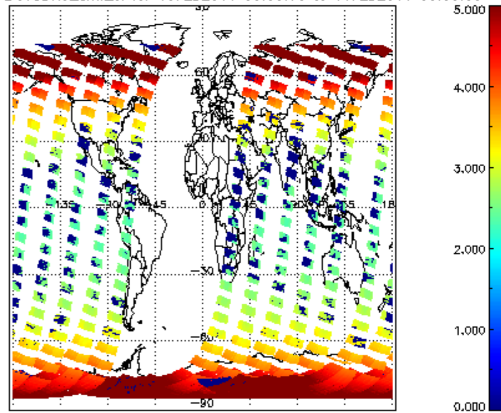
SCIOL2P_NADUV3BRO_amf_cl for 10FEB2011 00:00:00 to 11FEB2011 00:00:00
