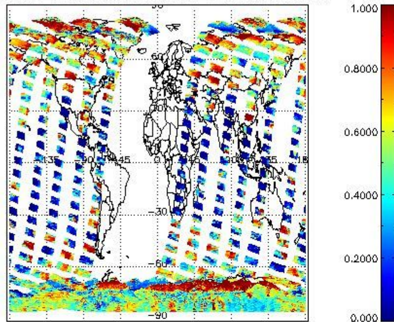
cL_frac for 10FEB2011 00:00:00 to 11FEB2011 00:00:00
