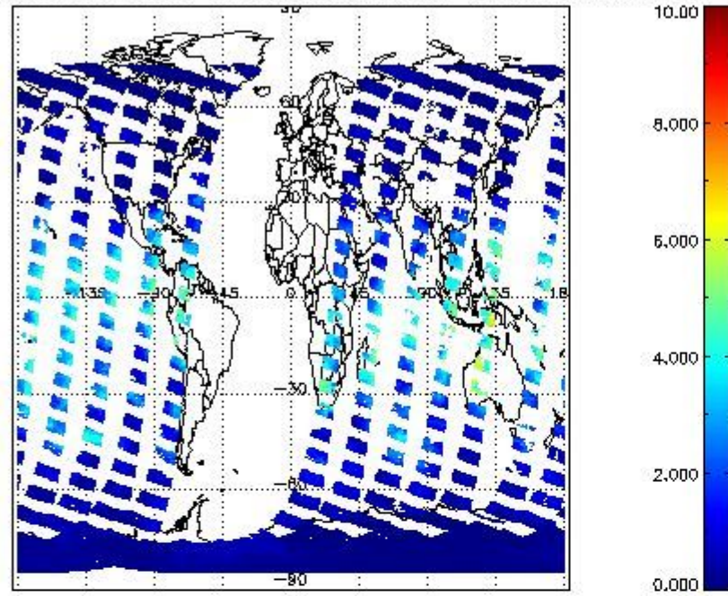
SCIOL2P_NADUV8H2O_vcd for 10FEB2011 00:00:00 to 11FEB2011 00:00:00
