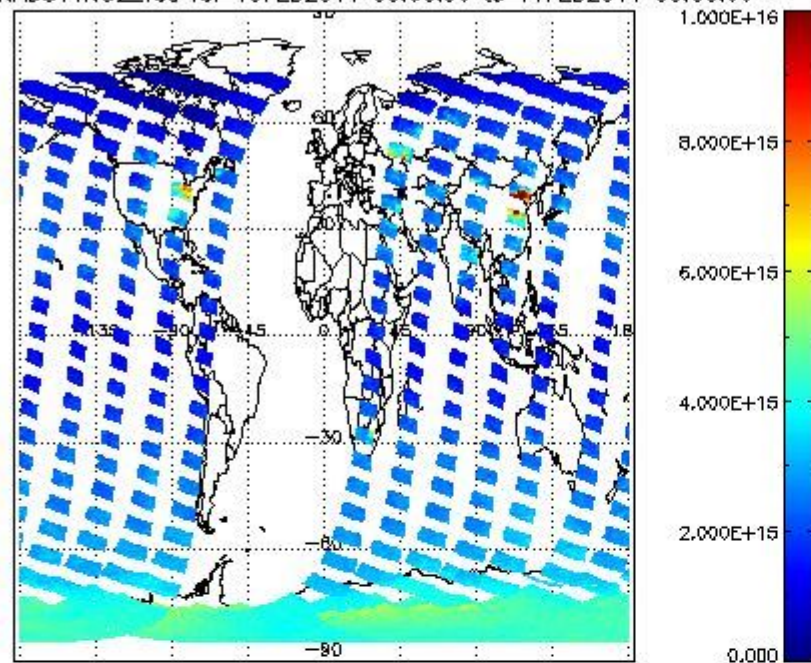
SCIOL2P_NADUV1N02_vcd for 10FEB2011 00:00:00 to 11FEB2011 00:00:00
