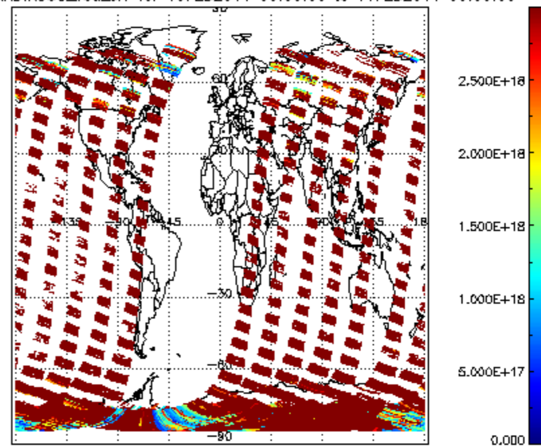
SCIOL2P_NADIR3CO_vcd_err for 10FEB2011 00:00:00 to 11FEB2011 00:00:00
