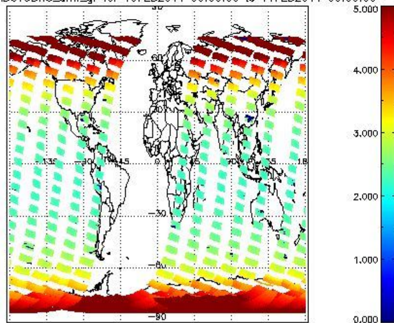
SCIOL2P_NADUV3BRO_amf_gr for 10FEB2011 00:00:00 to 11FEB2011 00:00:00
